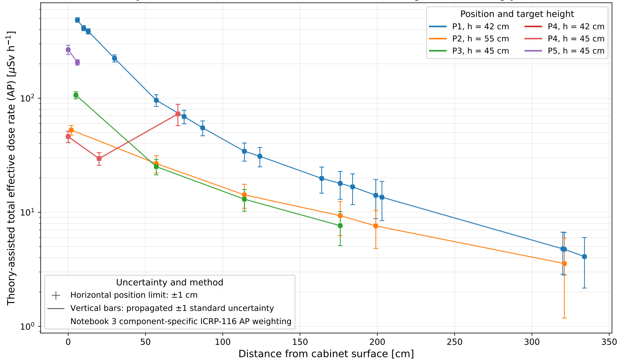
Theory-assisted measured total dose rate — lower heights — semi-log y scale
