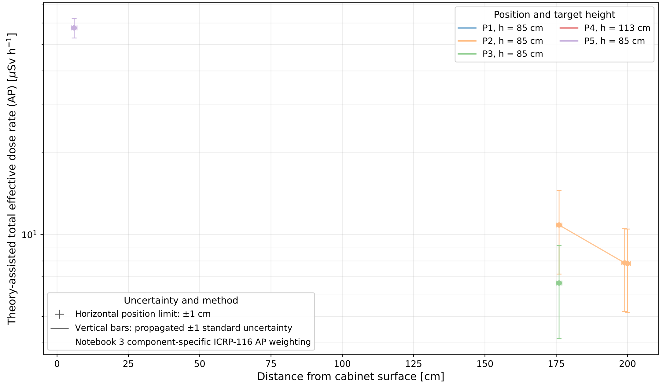
Theory-assisted measured total dose rate — upper heights — semi-log y scale
