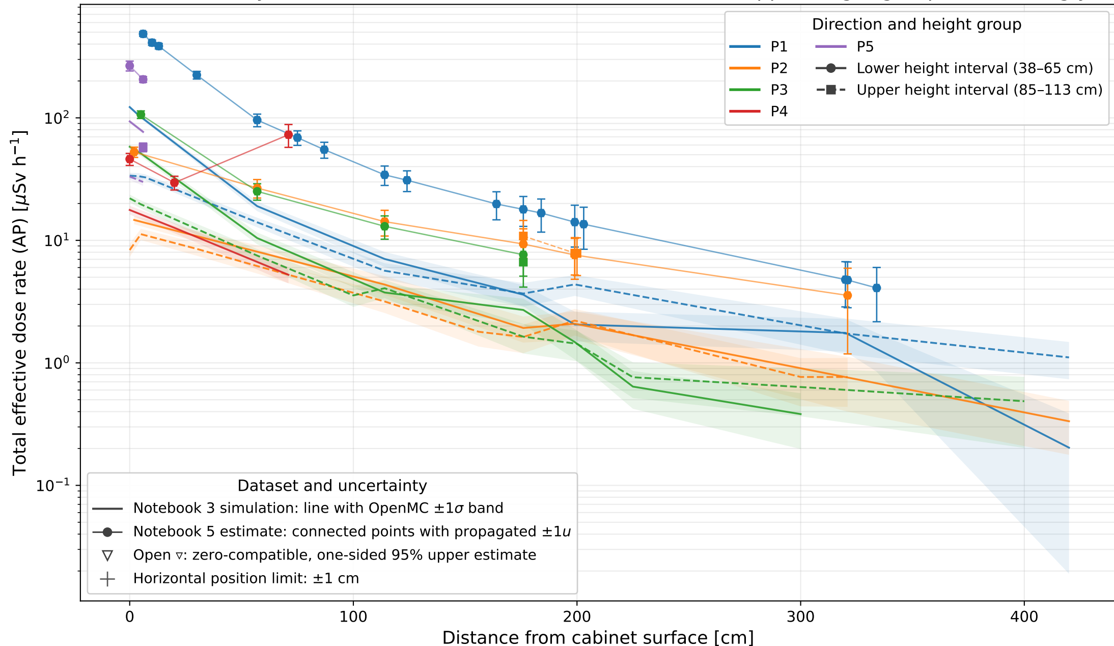
Simulated and theory-assisted measured total AP field — lower and upper height groups — semi-log y scale
