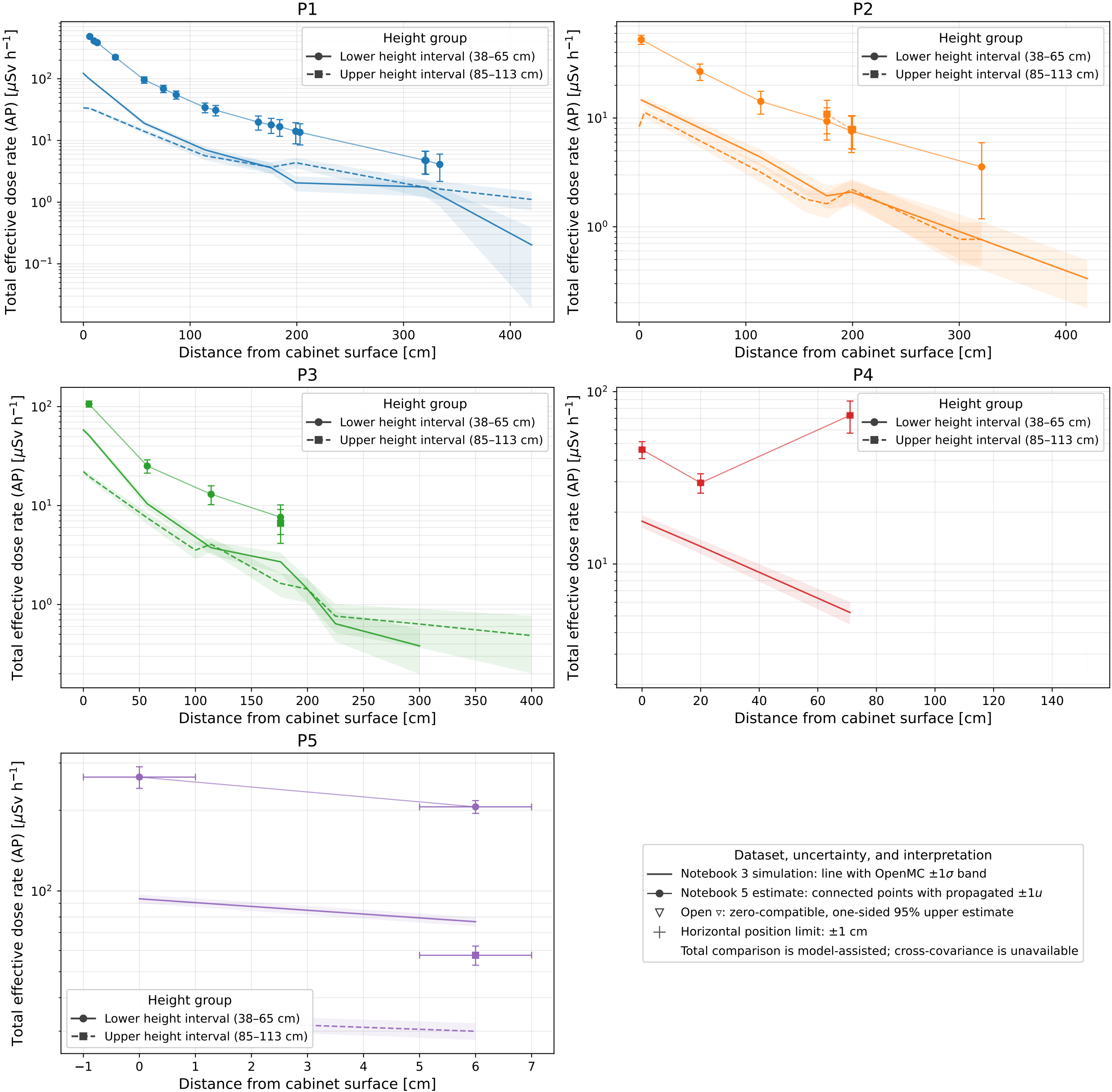
Simulated and theory-assisted measured total AP field at P1-P5 — lower and upper height groups — semi-log y scale
