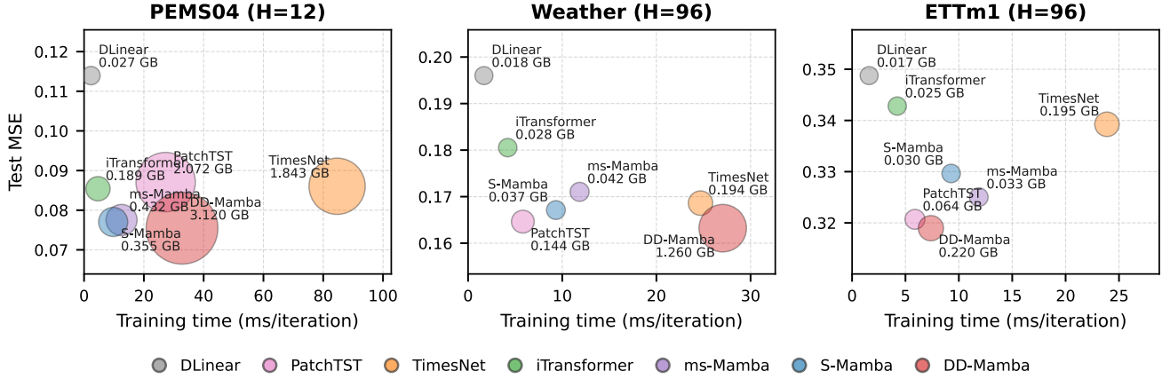
Figure 2: Matched training-efficiency comparison on PEMS04 ( H = 12 ), Weather ( H = 96 ), and ETTm1 ( H = 96 ). Horizontal position is mean optimizer-loop time, vertical position is mean test MSE, and bubble area is linear in mean peak allocated GPU memory; direct annotations report peak memory in GB.
