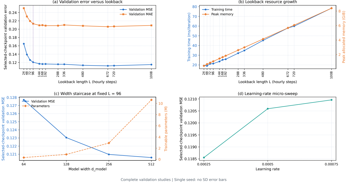
Figure 4: Validation-only capacity analysis on ECL at horizon 96. Panels (a)–(b) relate lookback length to selected-checkpoint error and resource use, while panels (c)–(d) show the model-width and learning-rate sweeps. All points are single-seed results; no variability bars are available.
