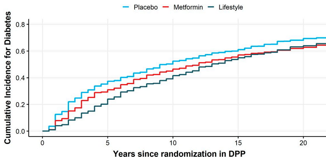
Figure 2—Cumulative incidence of diabetes during DPP and DPPOS (31). The DPP (1996–2002) was conducted for an average of 2.8 years (range 1.8–4.6), after which DPP participants were invited to join the DPPOS (2003–present).
