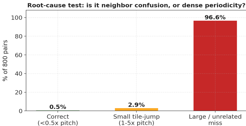
Figure 1 — Root-cause breakdown across all 800 pairs. Genuine “one tile over” mistakes account for under 3% of failures.
