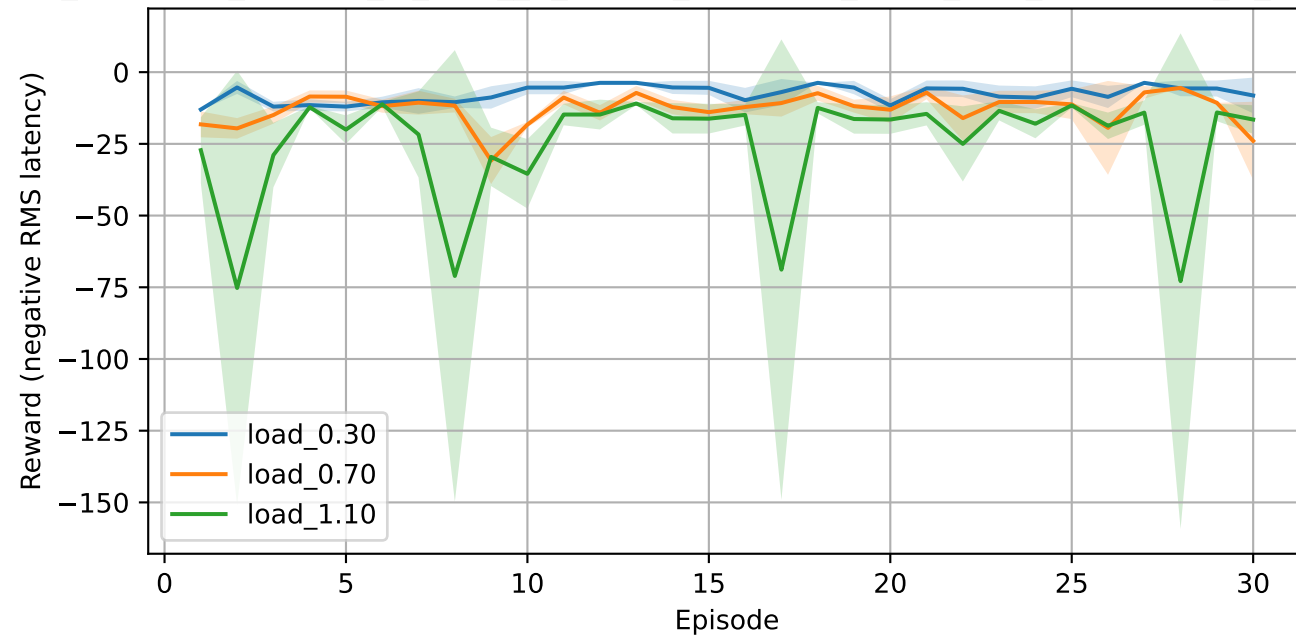
Convergence: Reward vs Episode
