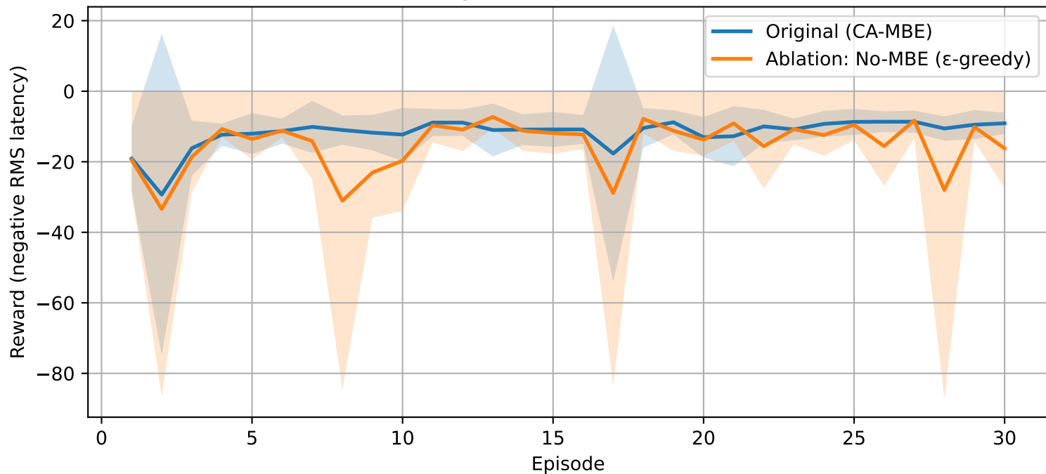
Convergence: CA-MBE vs No-MBE
