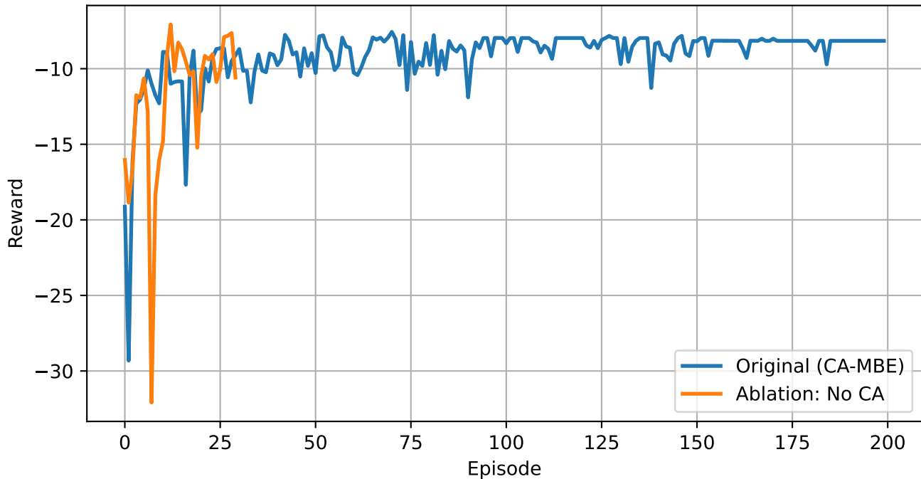
Convergence Comparison: CA-MBE vs No-CA
