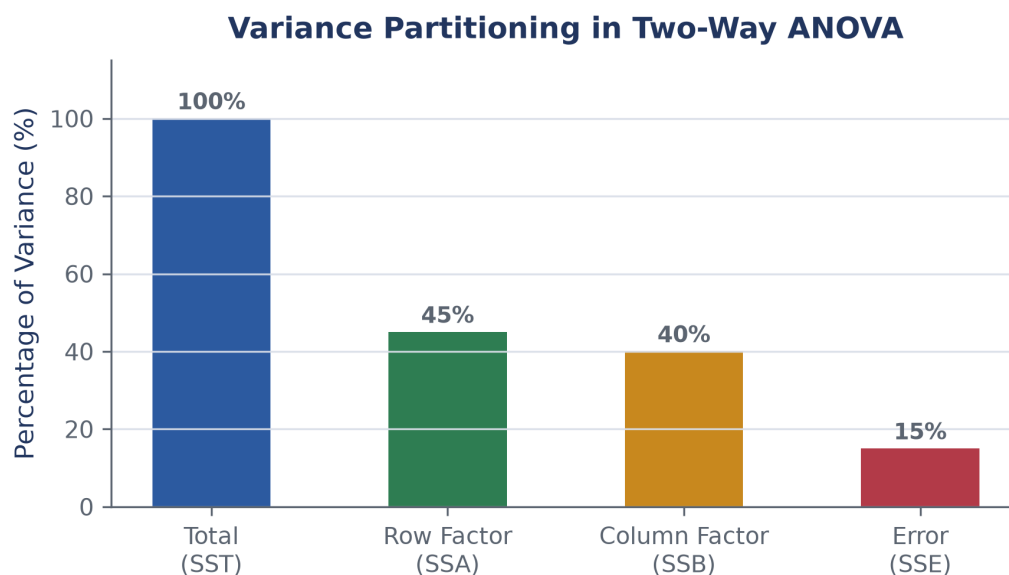
Figure 1: ANOVA divides total dataset variation into row factor, column factor, and residual error components.
