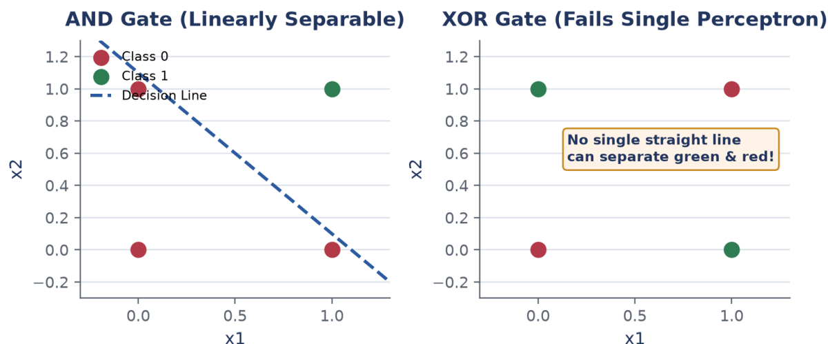
Figure 1: Linear boundary for AND gate vs non-linear boundary requirement for XOR gate.
