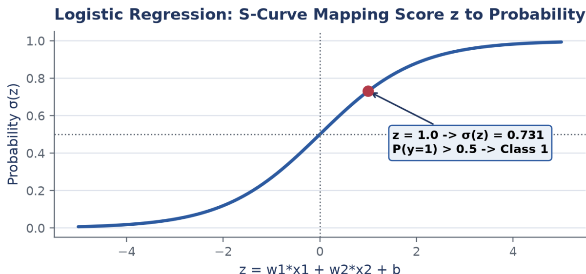
Figure 2: Sigmoid activation function mapping unbounded scores z into probability range (0, 1) .
