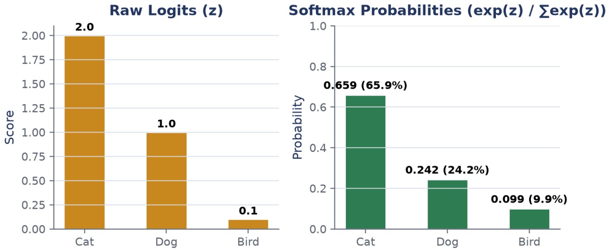
Figure 3: Softmax operation converting raw logits \mathbf{z} into a sum-to-one probability distribution.
