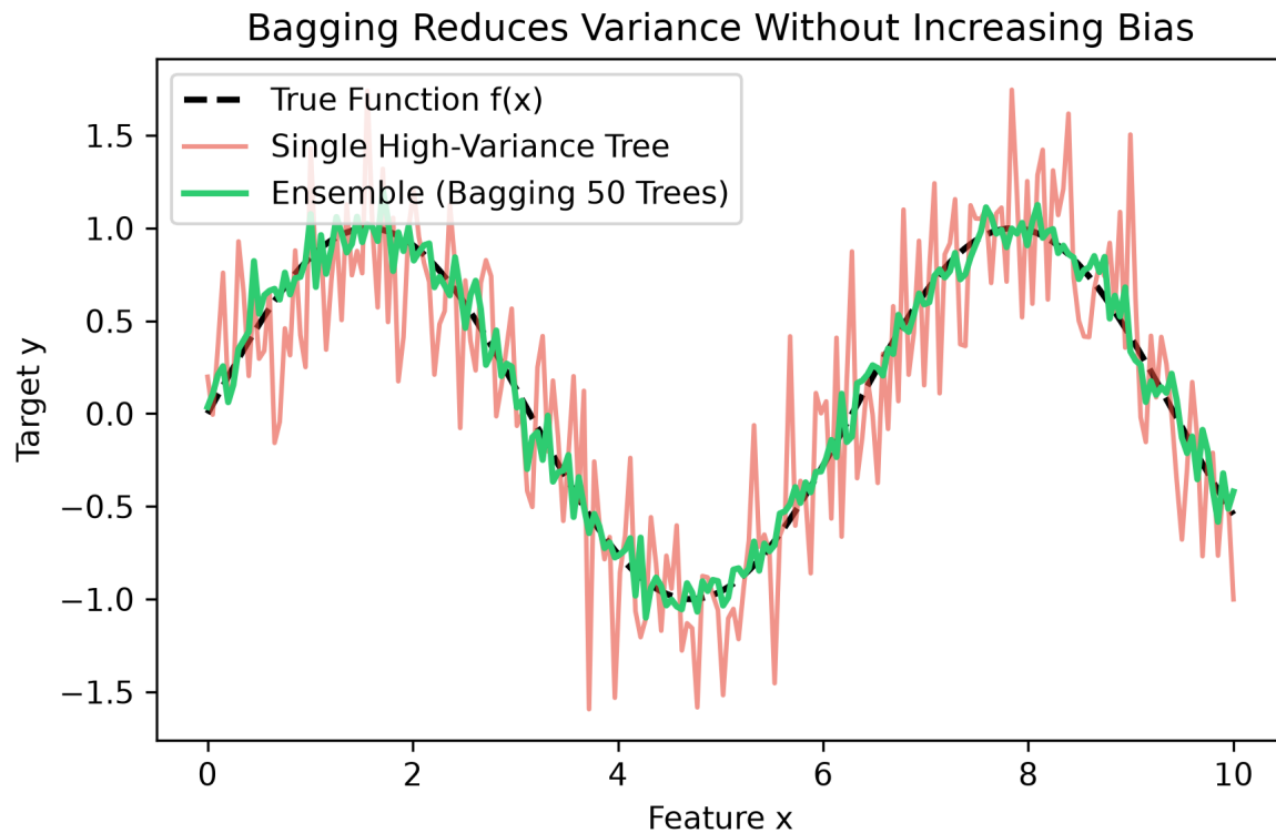
Figure 1: Bagging reduces variance without increasing bias by averaging predictions from multiple bootstrap-trained decision trees.
