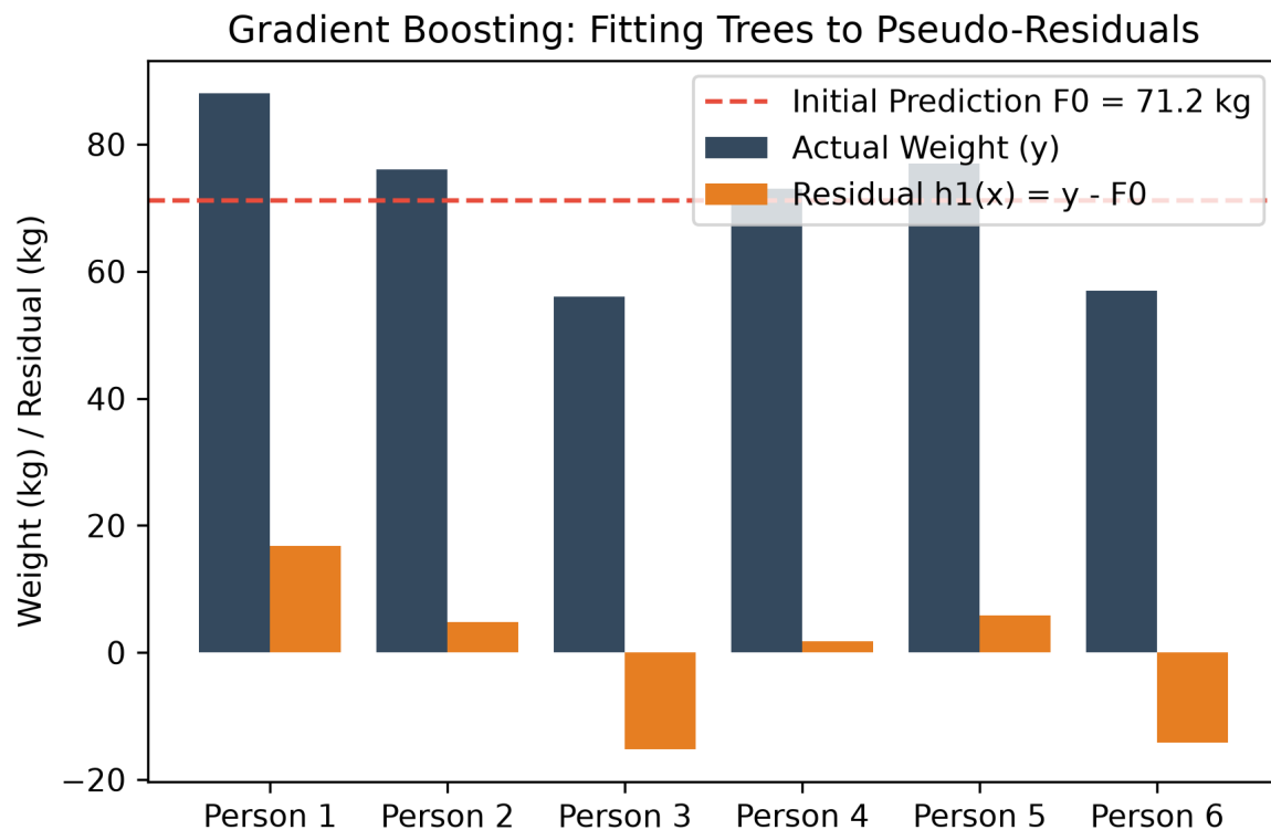
Figure 3: Gradient Boosting fits successive regression trees to the target residuals y - F_{m-1}(x) .
