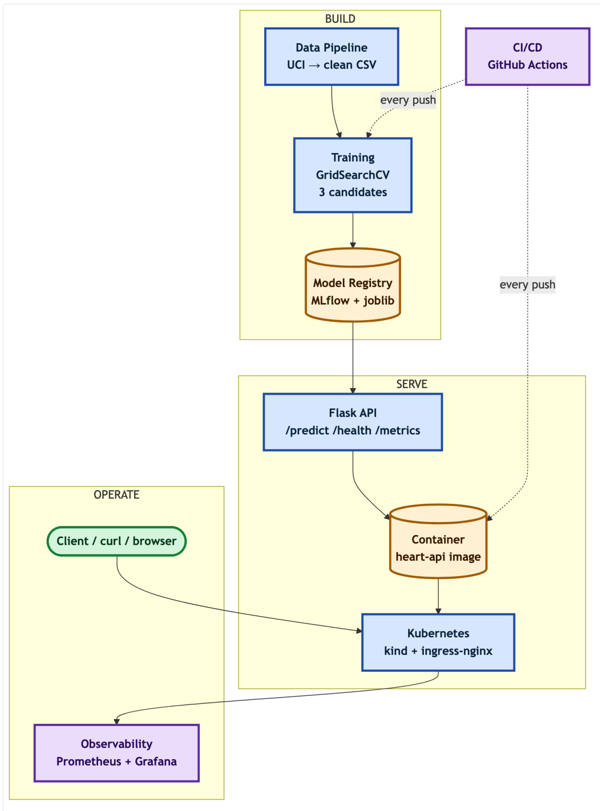
End-to-end MLOps pipeline architecture
