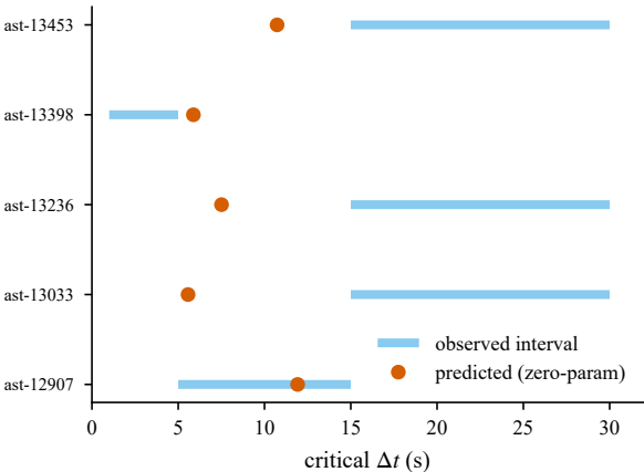
predicted vs observed critical \Delta t (5 pilot traj.)
