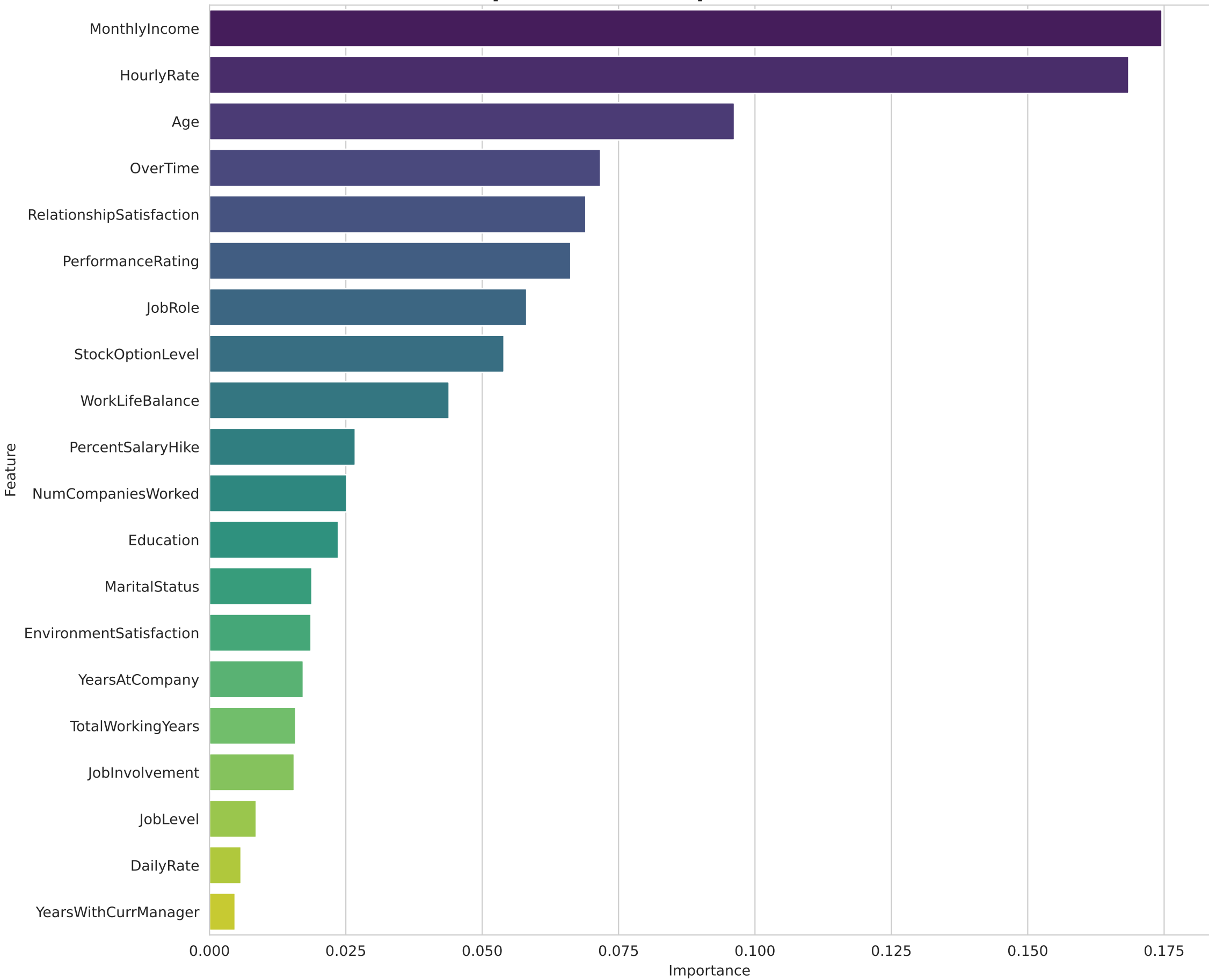
Top 20 Feature Importances in TabNet
