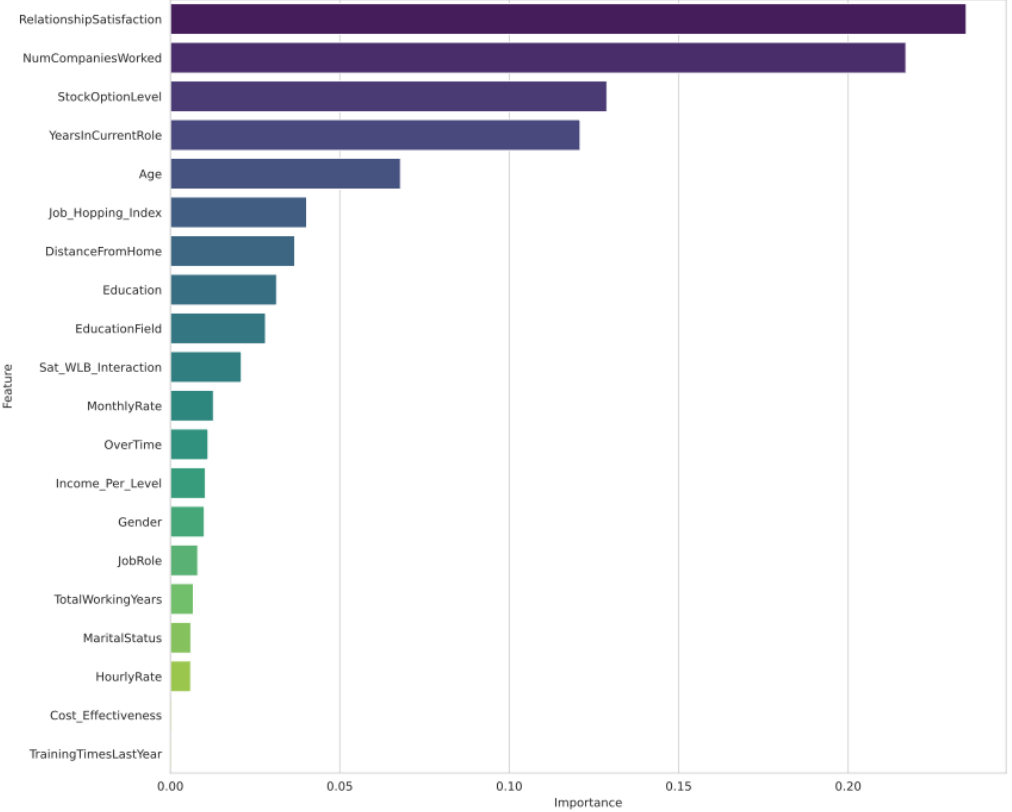
Top 20 Feature Importances in TabNet
