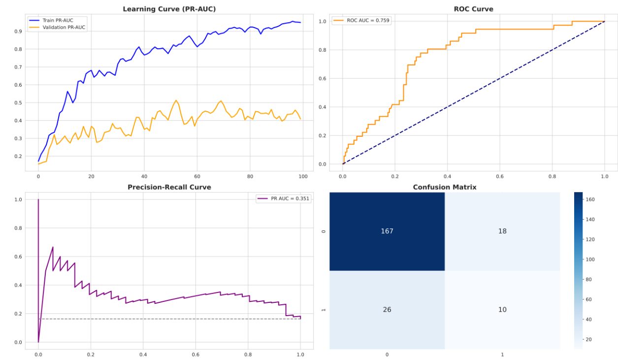
TabNet Performance Dashboard
