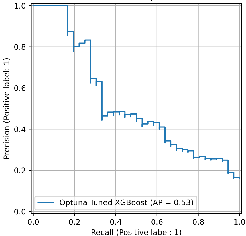
Precision-Recall Curve for Optuna Tuned XGBoost
