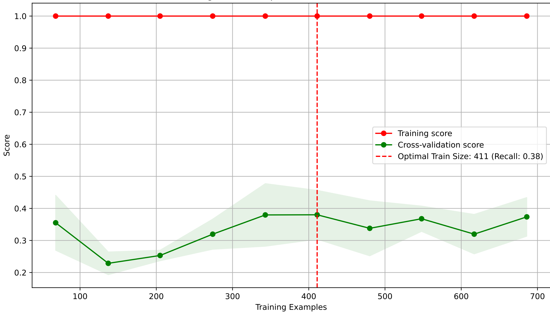
Learning Curve for Optuna Tuned XGBoost (Recall)
