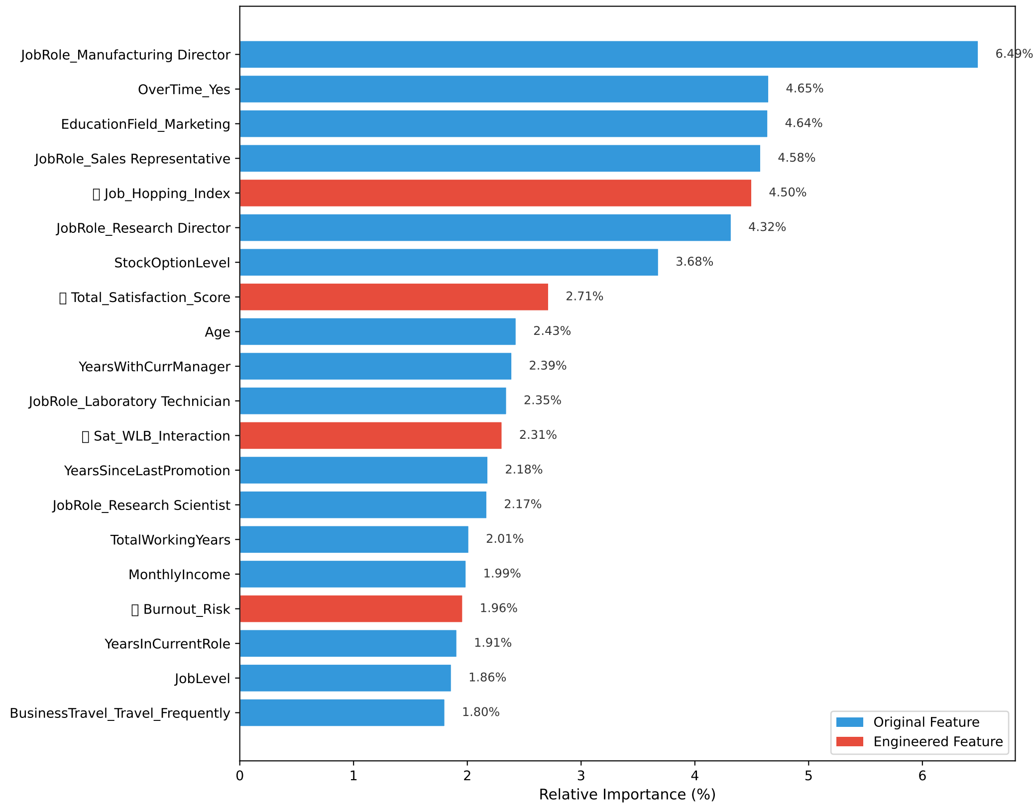
Top 20 Feature Importance (gain)
