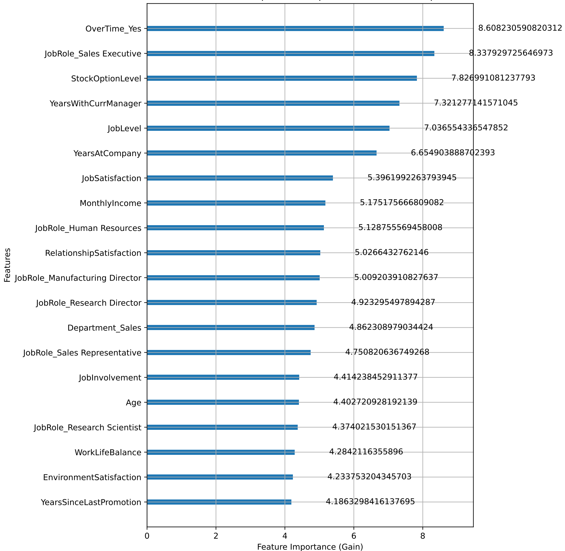
XGBoost Feature Importance (Optuna Tuned Model - Top 20)
