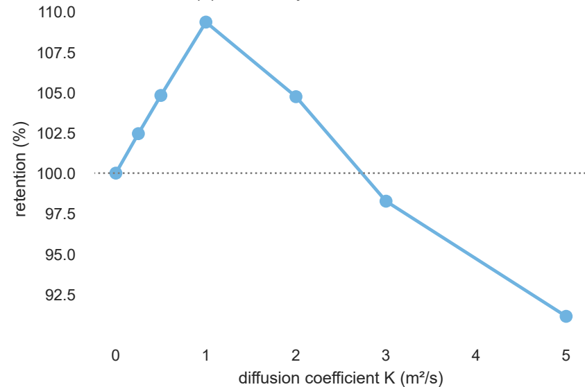
(a) Sensitivity to diffusion coefficient
