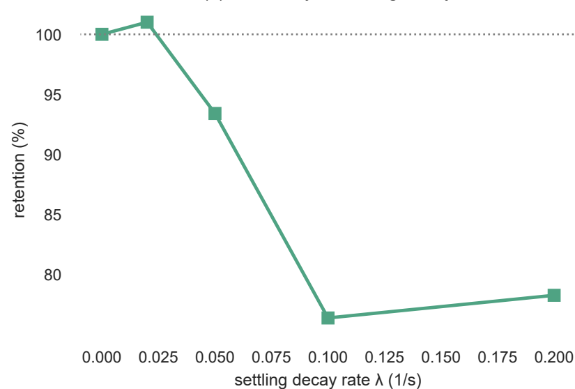
(b) Sensitivity to settling decay
