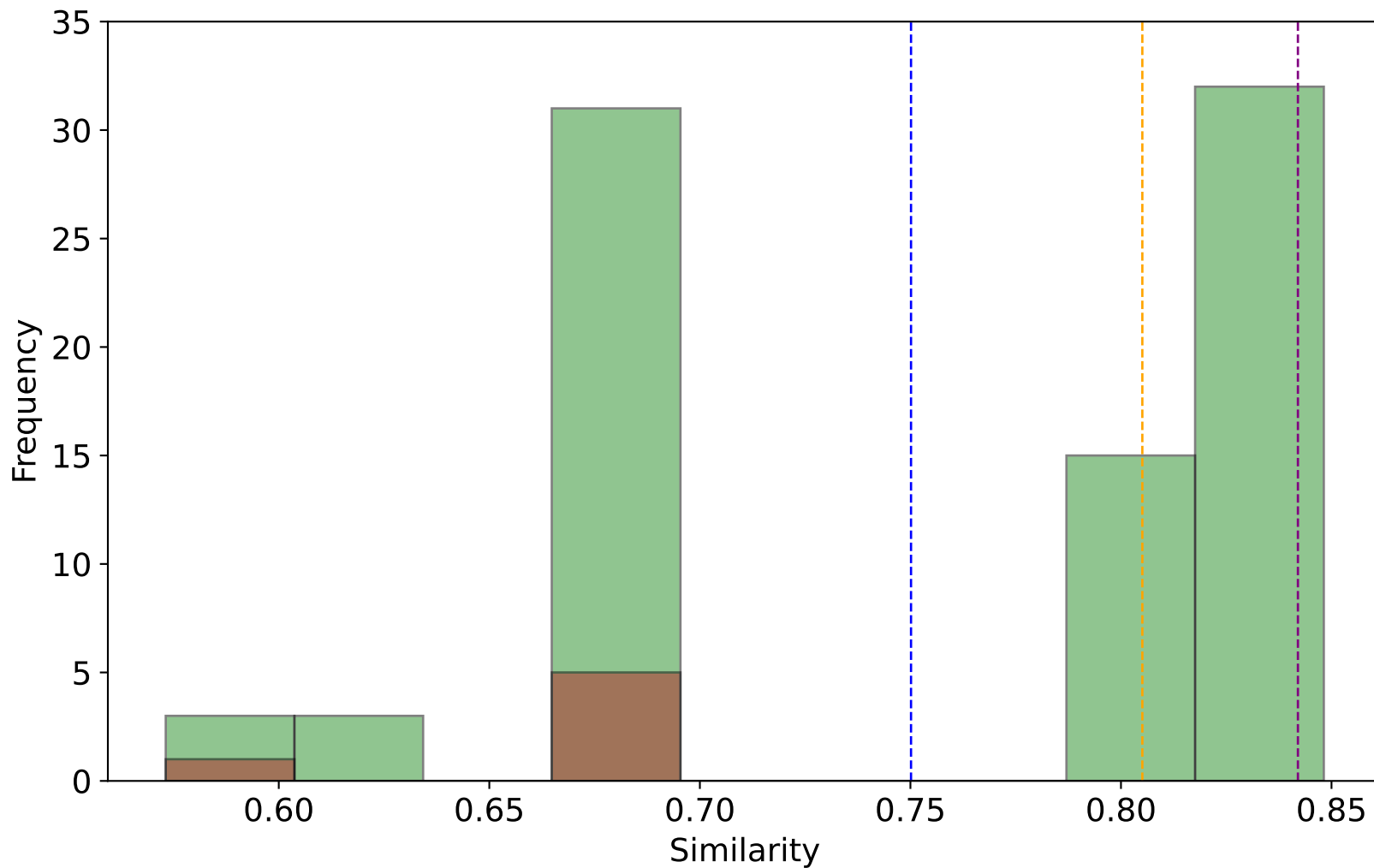
Top Sentences Semantic Pass/Fail Distribution model: gpt-4o-2024-08-06 nx: 3, ny: 1, nz: 18, median: 0.8050745129585266
