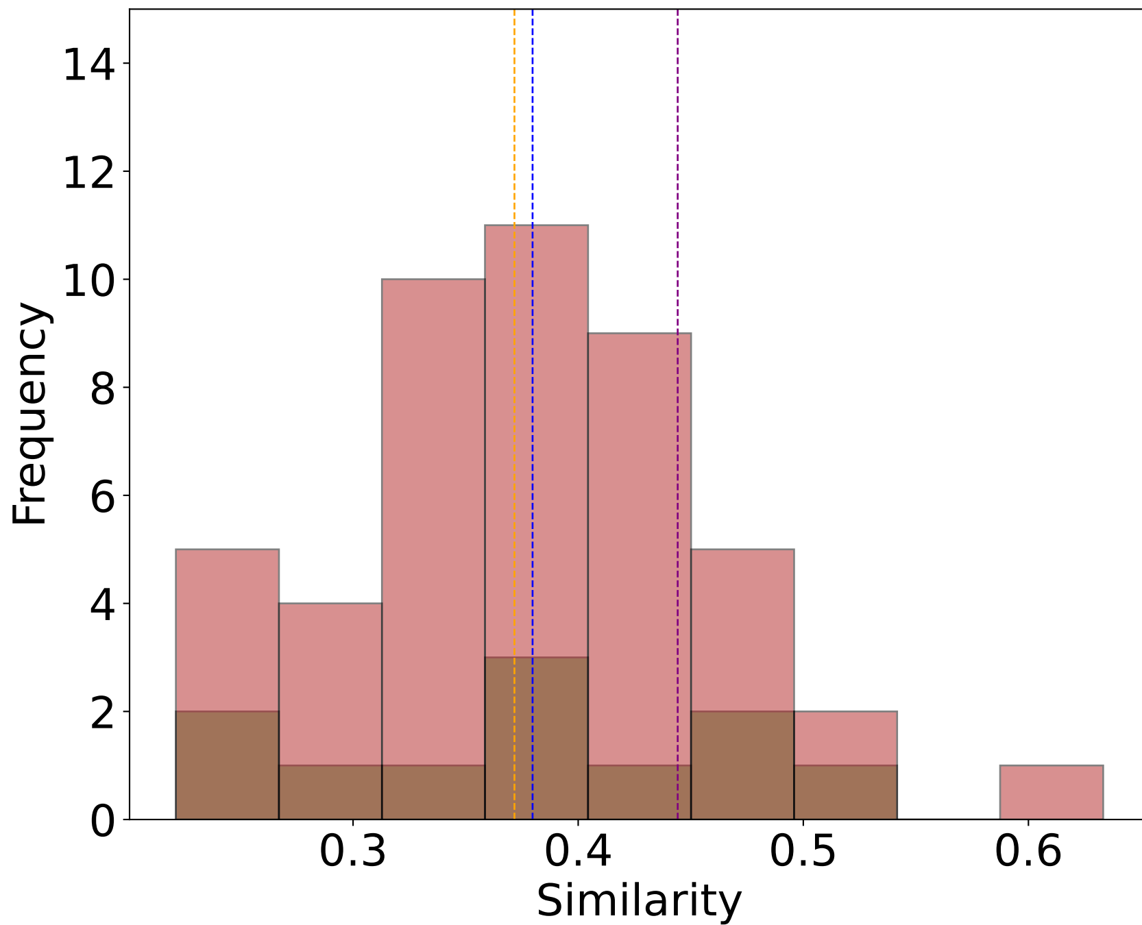
Bottom Sentences Semantic Pass/Fail Distribution model: Qwen3-1.7B nx: 3, ny: 1, nz: 18, median: 0.3716927766799927
