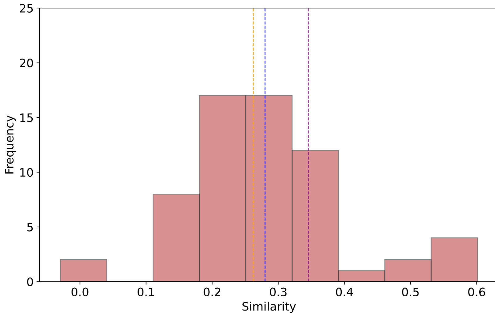
Bottom Sentences Semantic Pass/Fail Distribution model: DeepSeek-R1-Distill-Qwen-1.5B nx: 2, ny: 2, nz: 18
