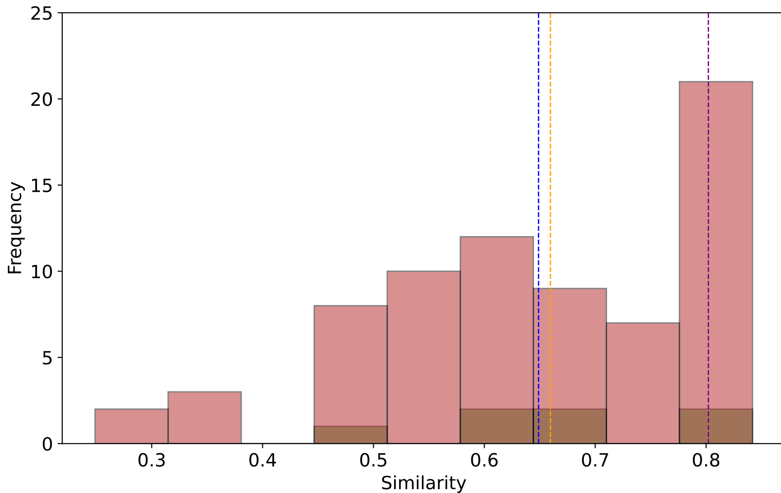
Top Sentences Semantic Pass/Fail Distribution model: DeepSeek-R1-Distill-Qwen-1.5B nx: 2, ny: 2, nz: 18
