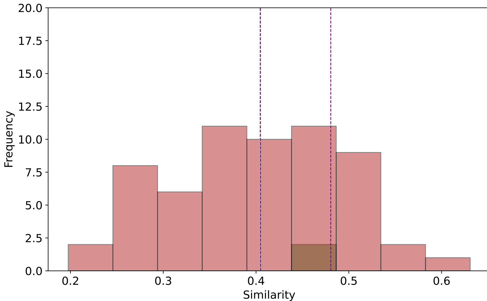
Bottom Sentences Semantic Pass/Fail Distribution model: Qwen3-1.7B nx: 2, ny: 2, nz: 18
