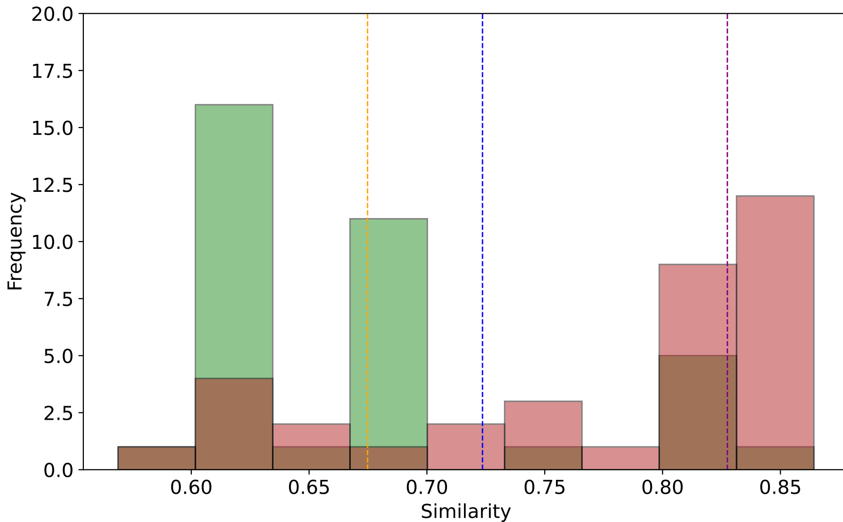
Top Sentences Semantic Pass/Fail Distribution model: Qwen3-1.7B nx: 2, ny: 2, nz: 18
