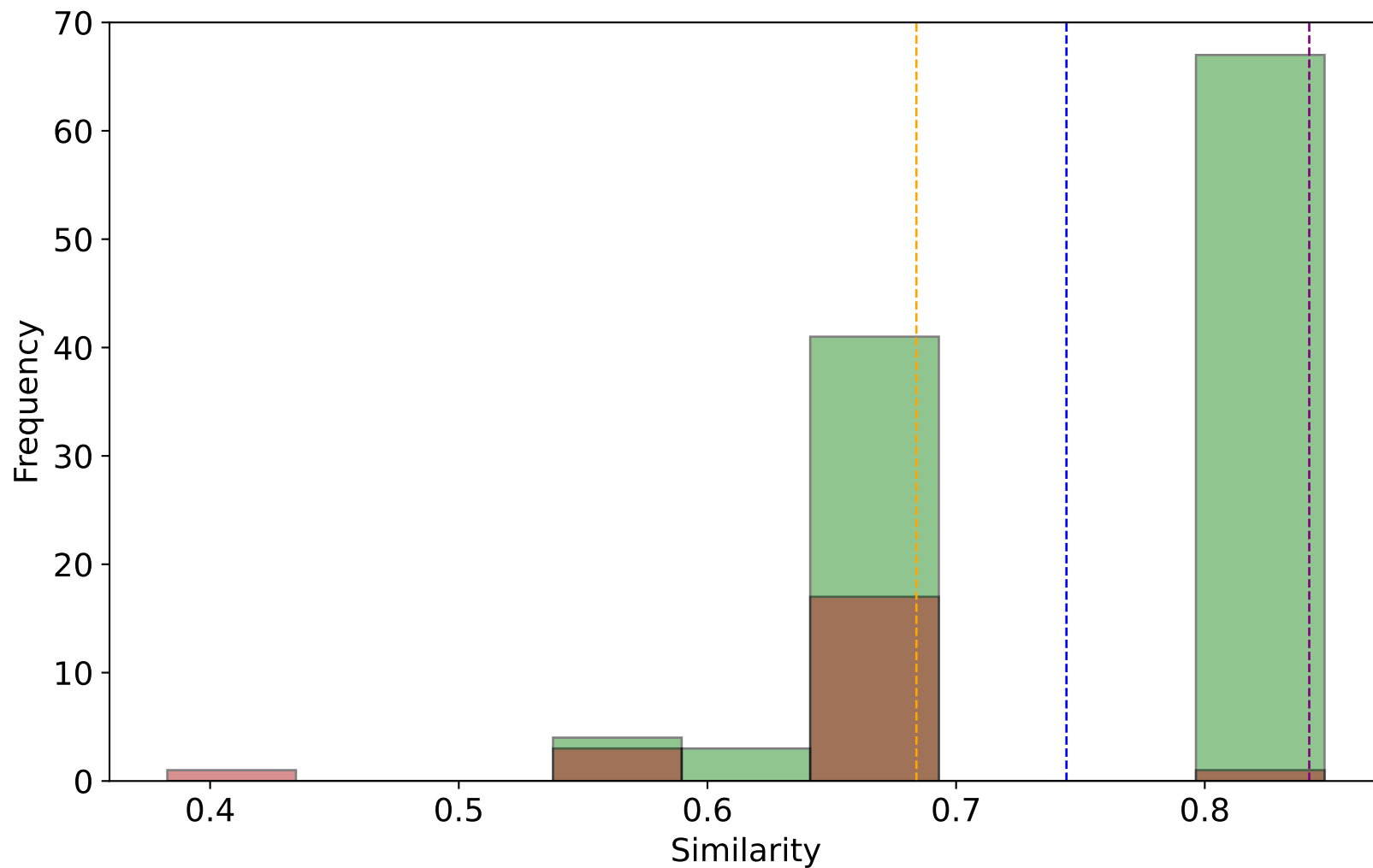
Top Sentences Semantic Pass/Fail Distribution model: gpt-4o-2024-08-06 nx: 2, ny: 2, nz: 18
