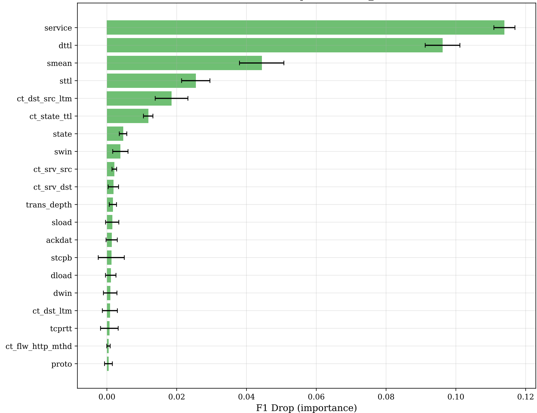
Permutation Feature Importance — ft_transformer
