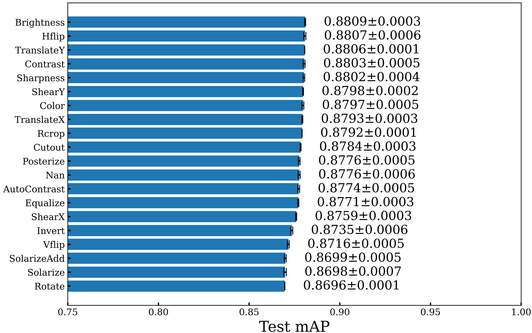
Augmentation
