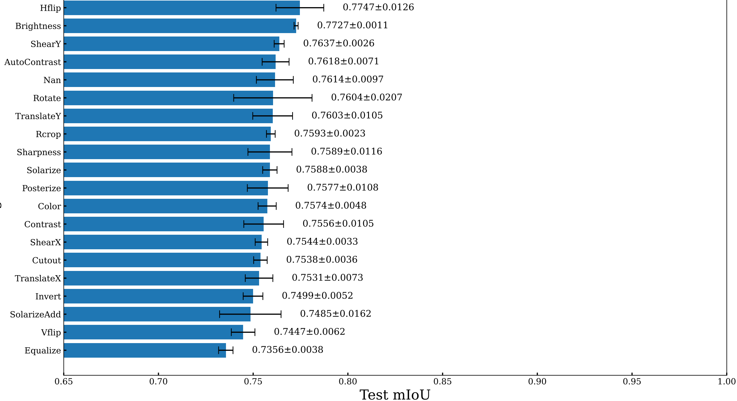
Augmentation
