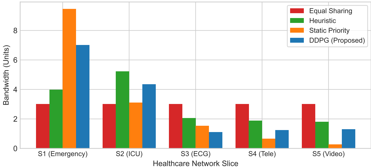
Average Allocated Bandwidth per Network Slice
