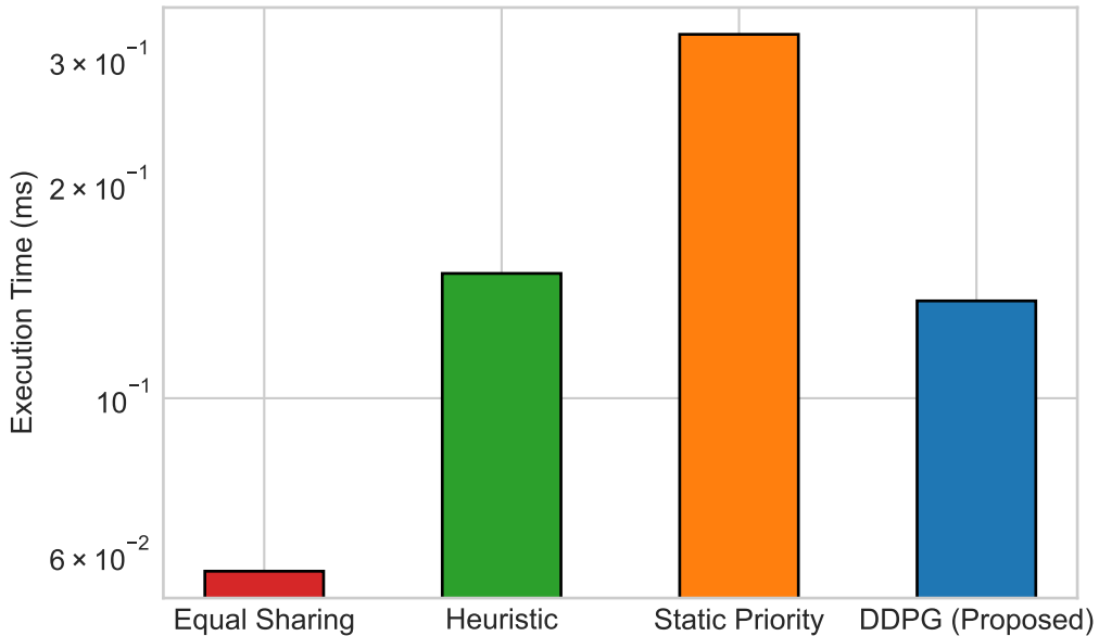
Step Decision Execution Time (2000 Patients)
