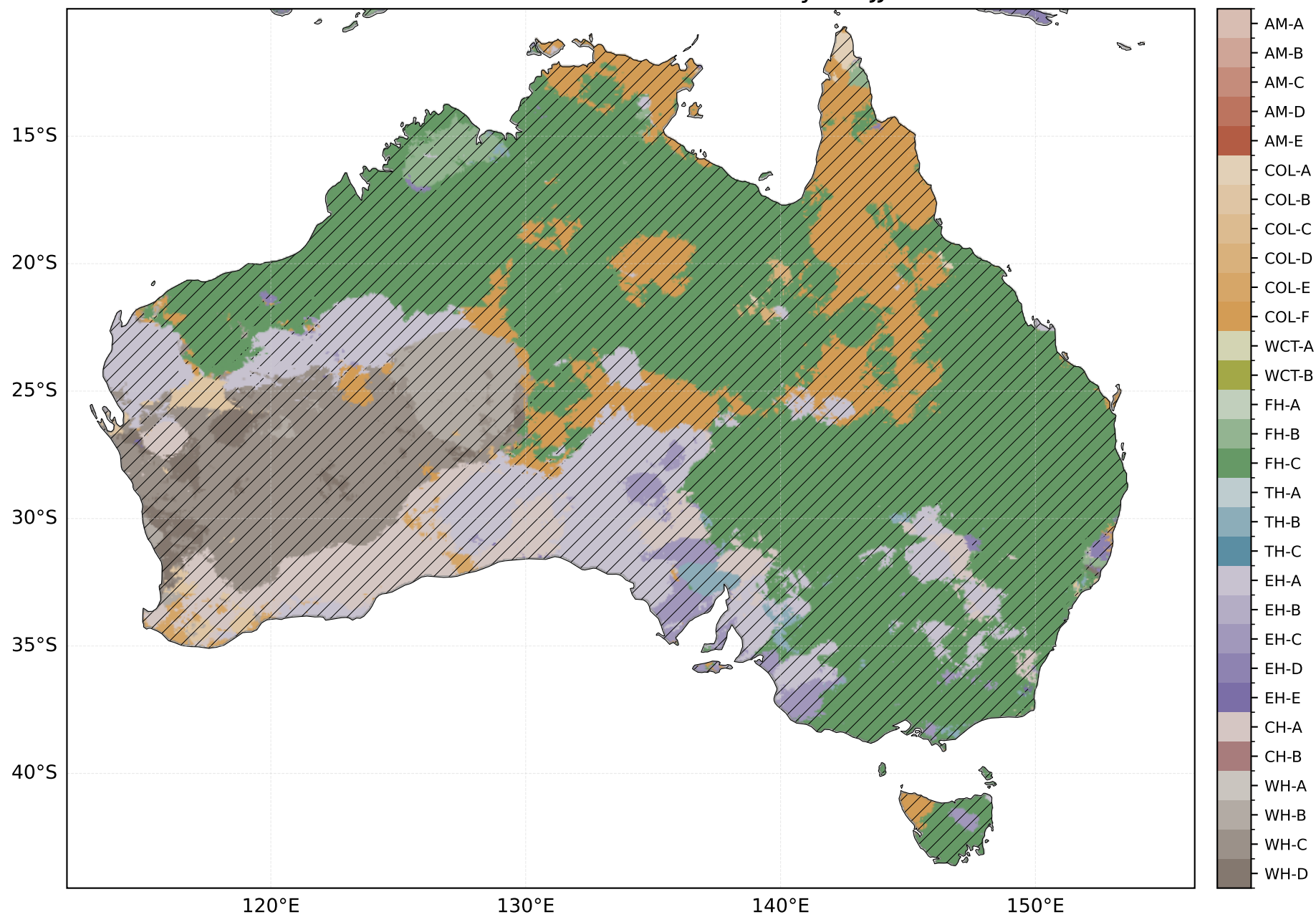
Dominant SWT for 5% coldest days in JJA
