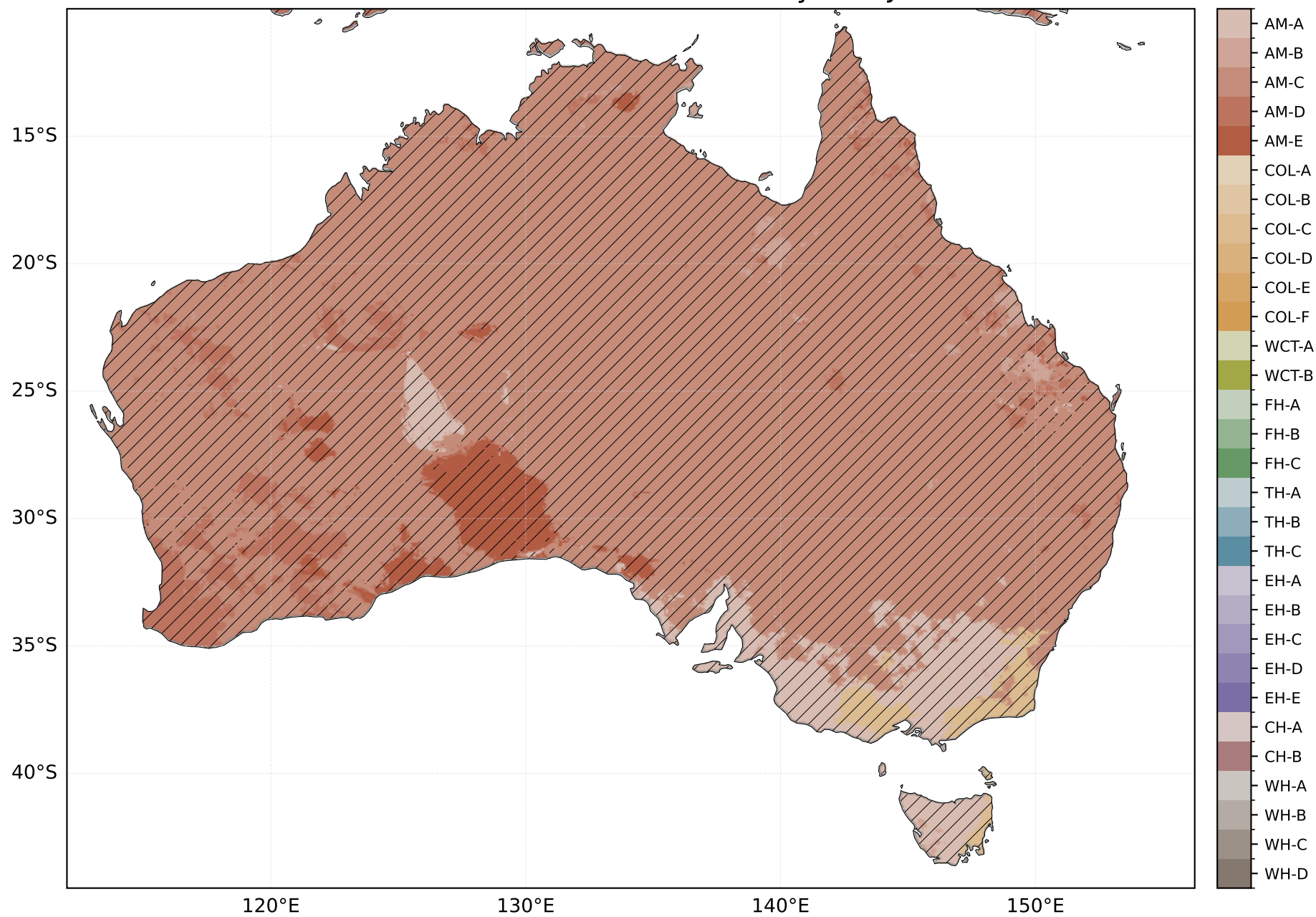
Dominant SWT for 5% wettest days in DJF
