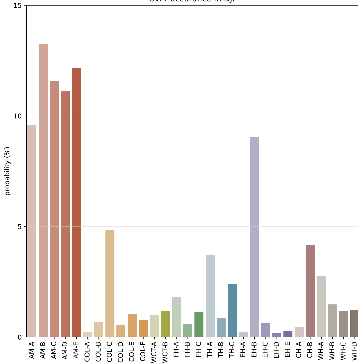
SWT occurance in DJF
