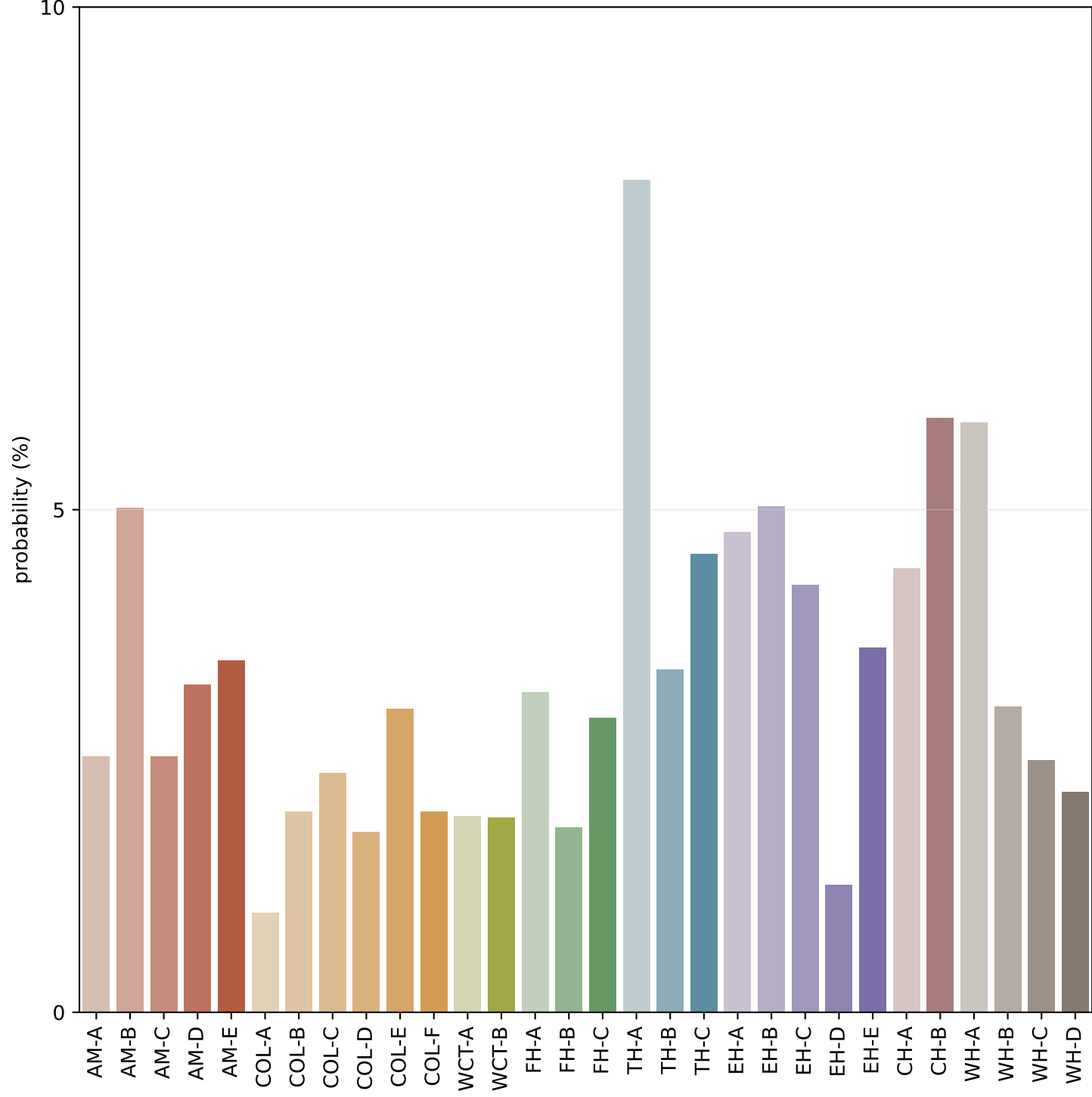
SWT occurance in MAM
