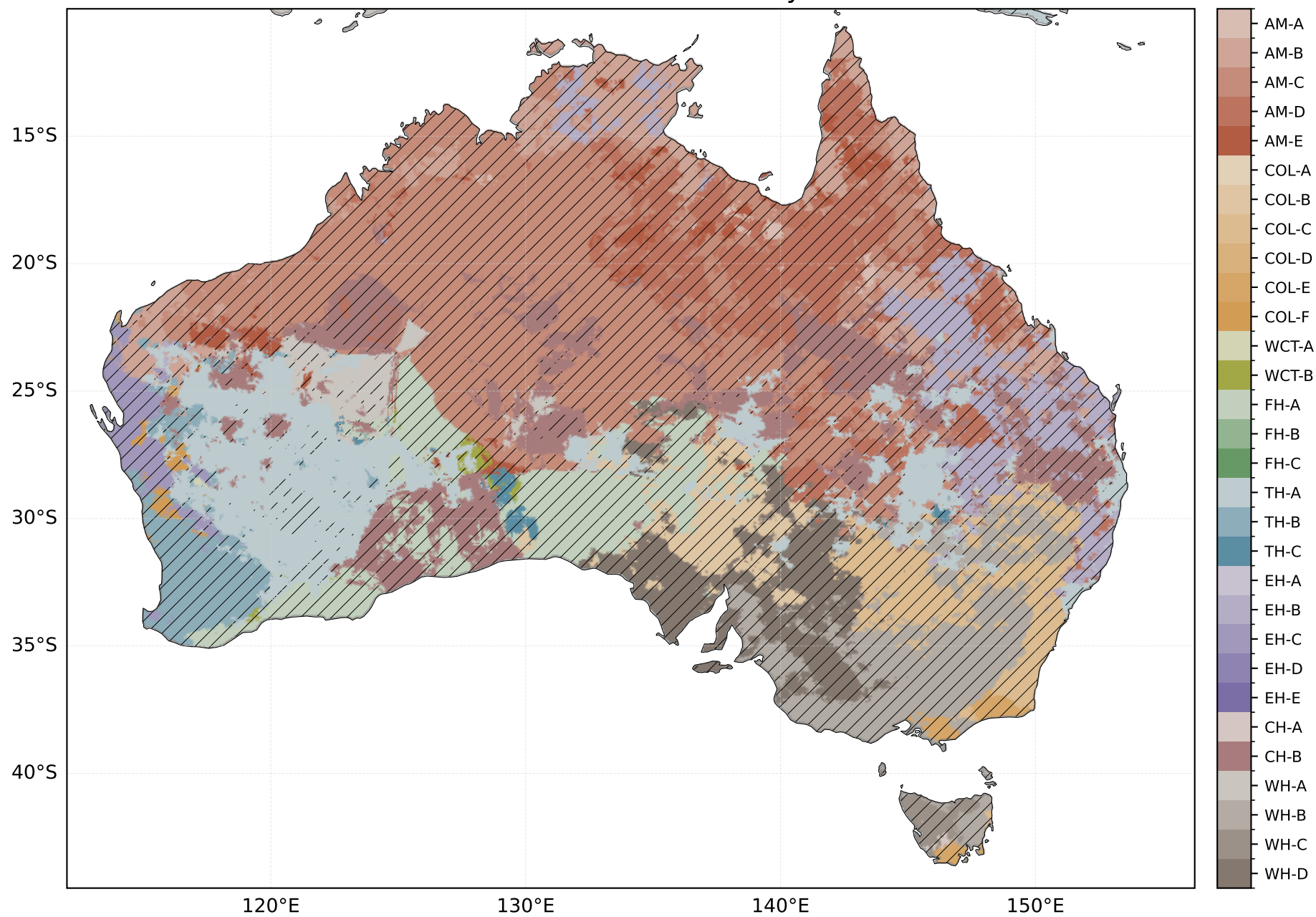
Dominant SWT for 5% wettest days in MAM
