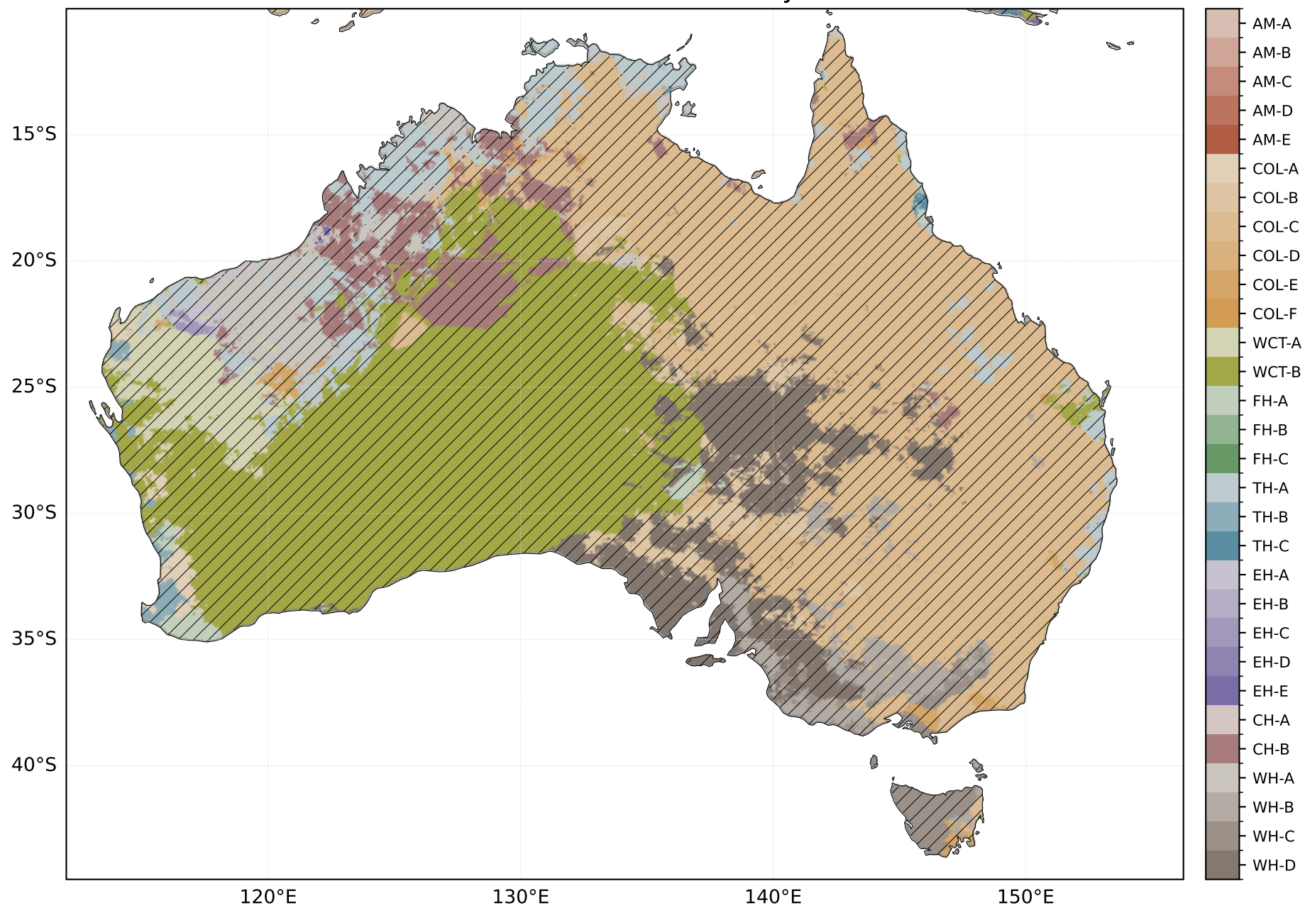
Dominant SWT for 5% wettest days in SON
