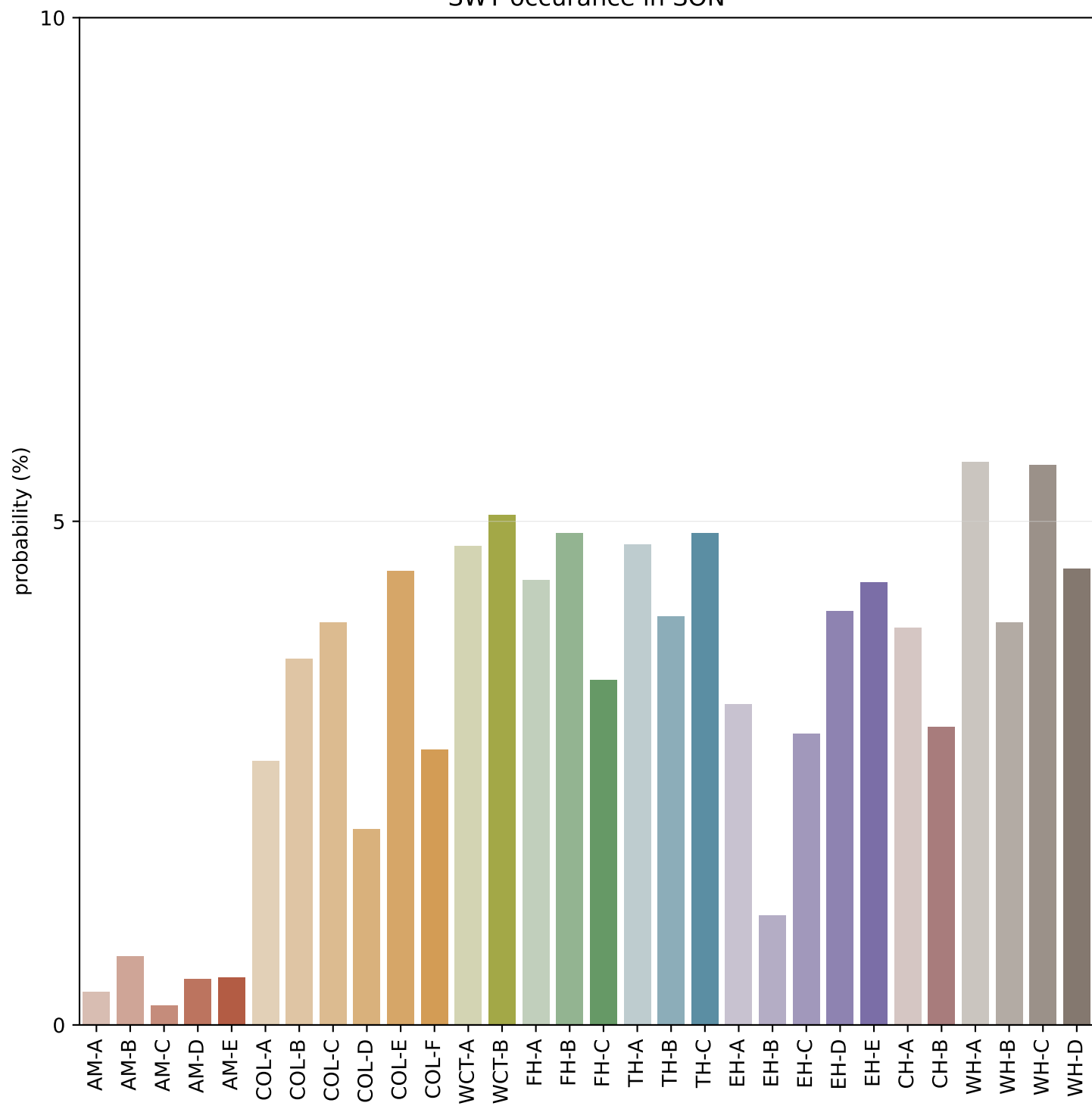
SWT occurance in SON
