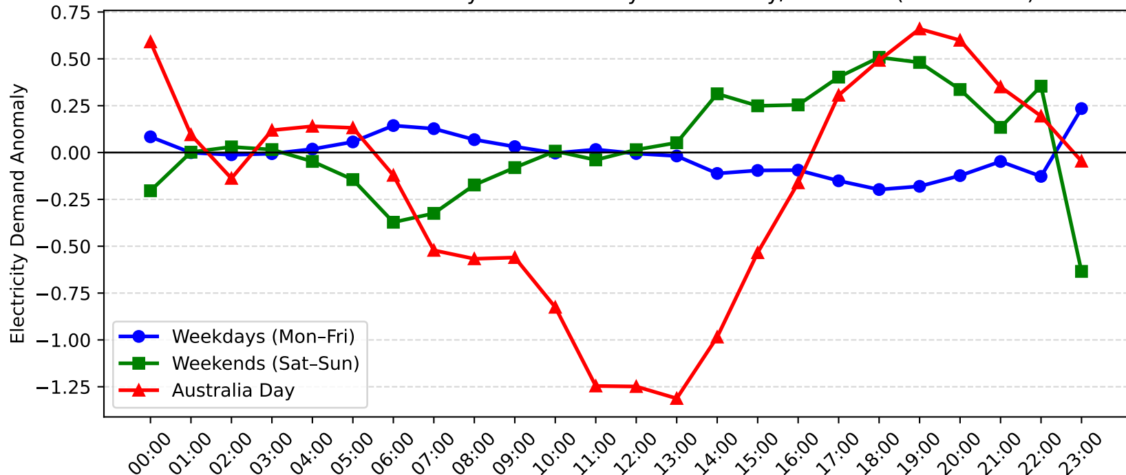
Telarah Demand Anomaly: Australia Day vs Weekday/Weekend (2006-2007)
