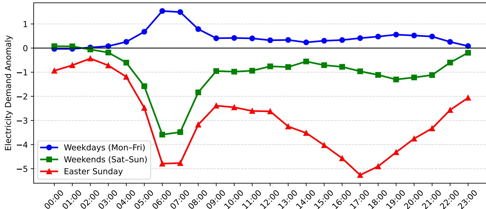
Revesby Demand Anomaly: Easter Sunday vs Weekday/Weekend (2013-2014)
