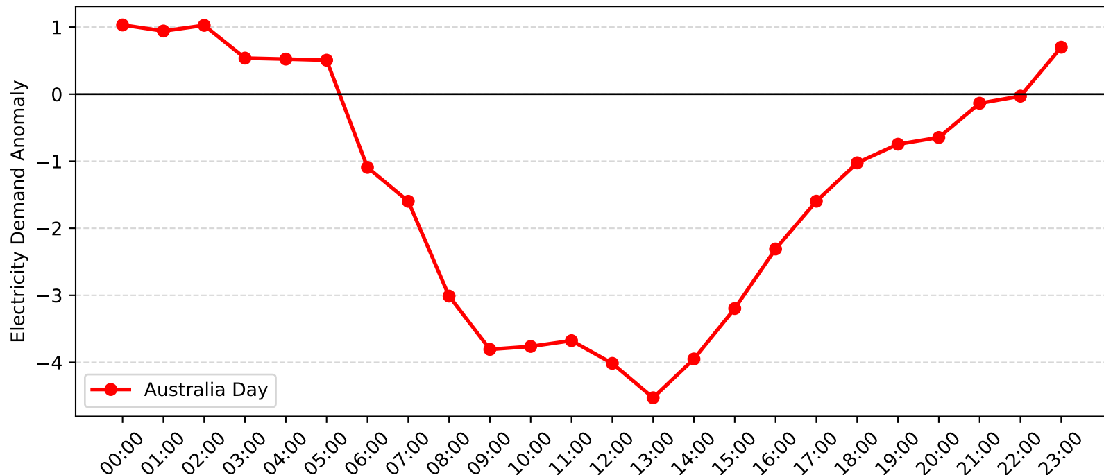
Green Square Demand Anomaly: Australia Day (2010-2011)
