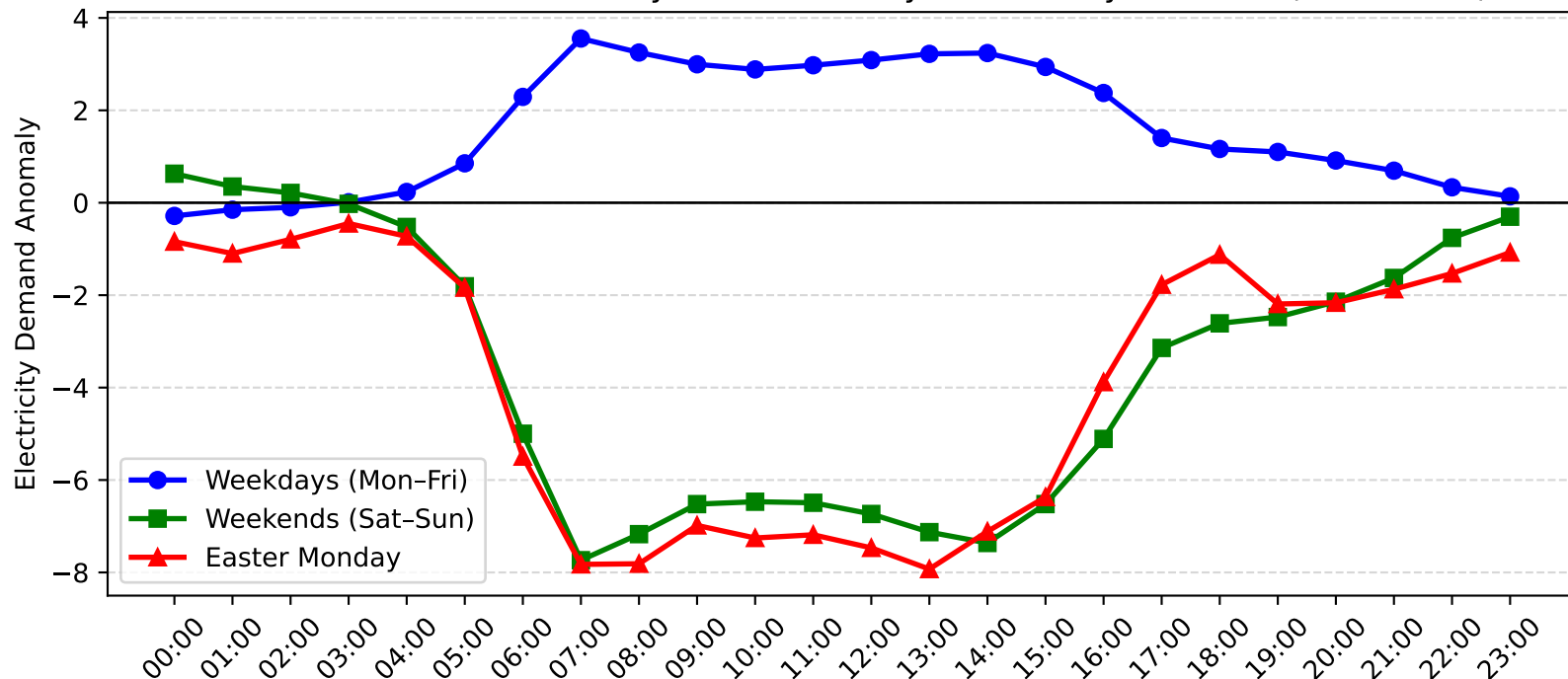
Marrickville Demand Anomaly: Easter Monday vs Weekday/Weekend (2009-2010)
