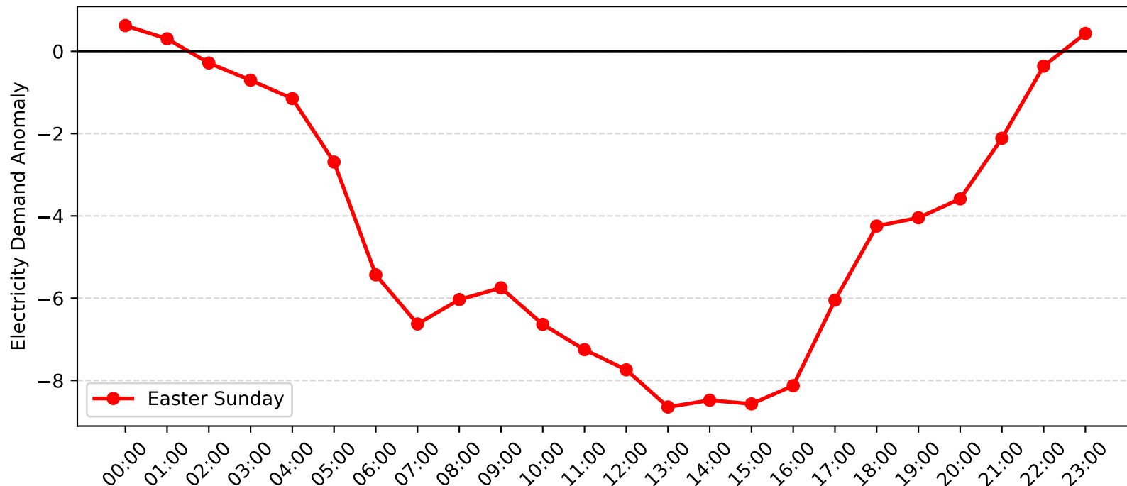
Sefton Demand Anomaly: Easter Sunday (2005-2006)
