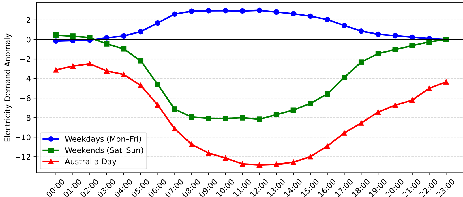
Homebush Bay Demand Anomaly: Australia Day vs Weekday/Weekend (2017-2018)
