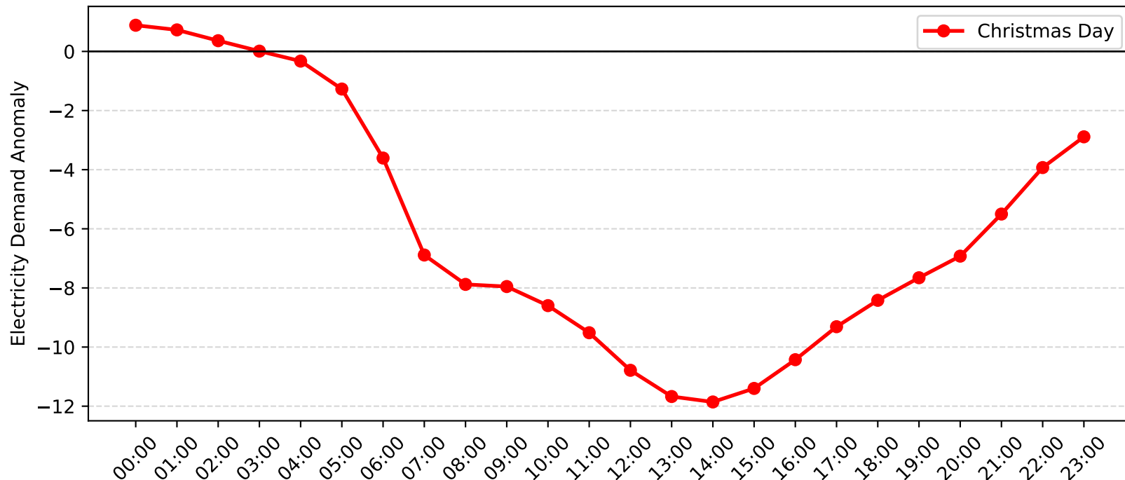
Marrickville Demand Anomaly: Christmas Day (2011-2012)
