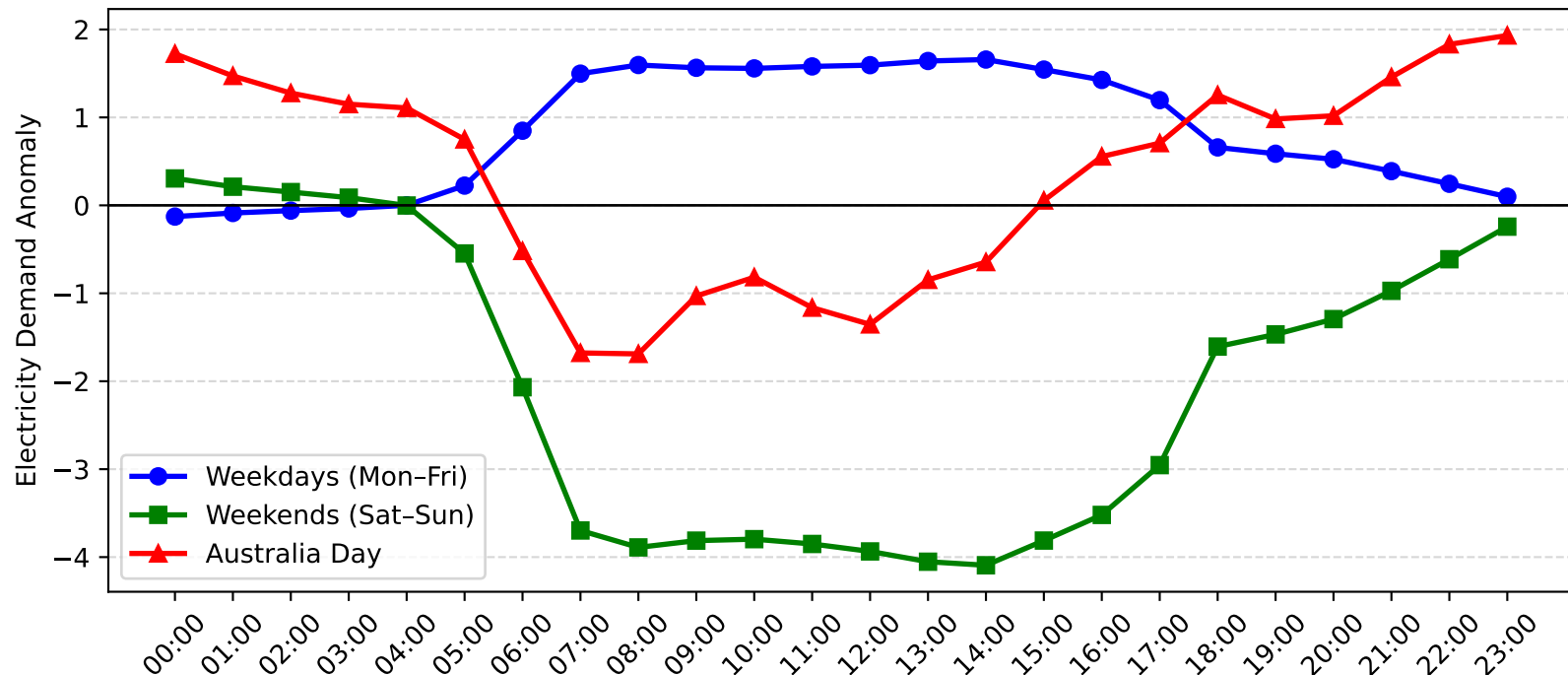
Concord Demand Anomaly: Australia Day vs Weekday/Weekend (2012-2013)
