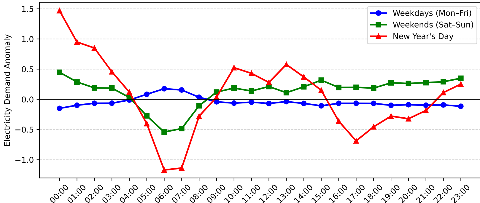
Noraville Demand Anomaly: New Year's Day vs Weekday/Weekend (2014-2015)
