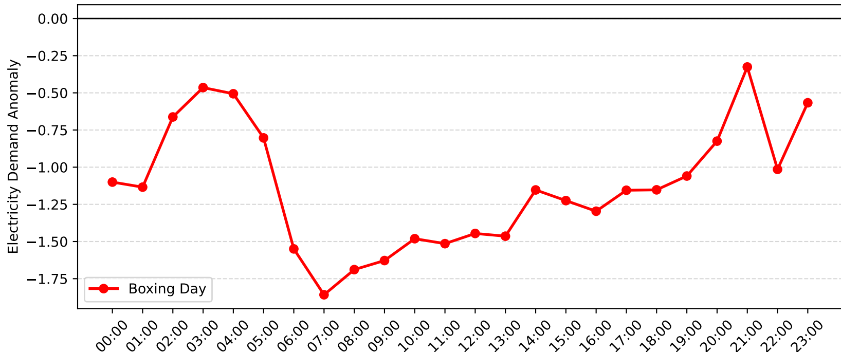
Gateshead Demand Anomaly: Boxing Day (2015-2016)
