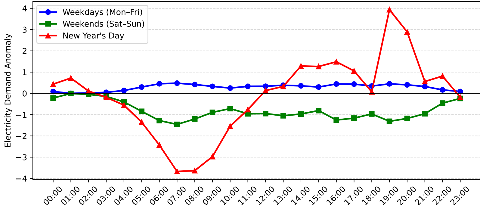
Charmhaven Demand Anomaly: New Year's Day vs Weekday/Weekend (2008-2009)
