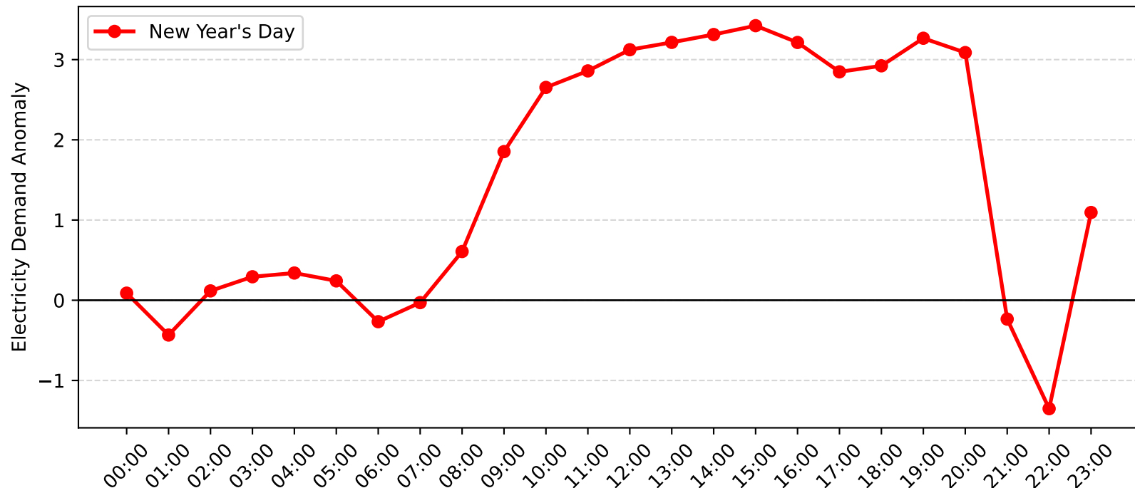
Swansea Demand Anomaly: New Year's Day (2006-2007)
