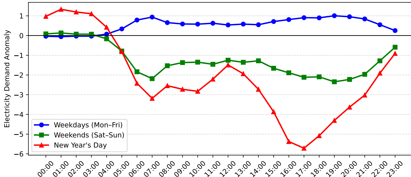
Revesby Demand Anomaly: New Year's Day vs Weekday/Weekend (2017-2018)
