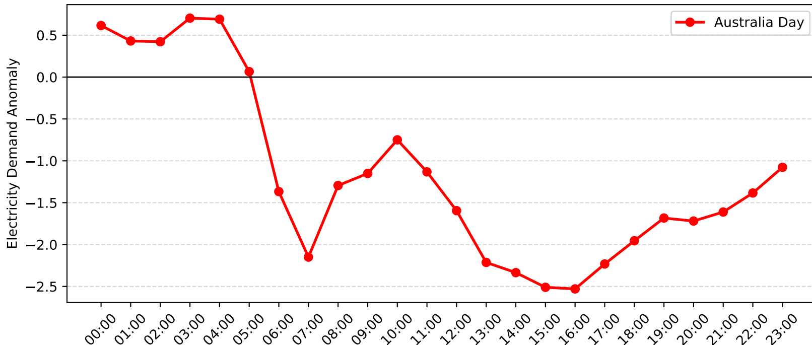
Dee Why West Demand Anomaly: Australia Day (2015-2016)
