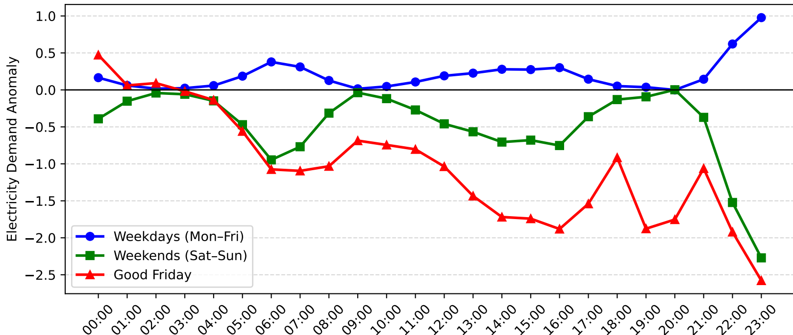
Muswellbrook Demand Anomaly: Good Friday vs Weekday/Weekend (2008-2009)
