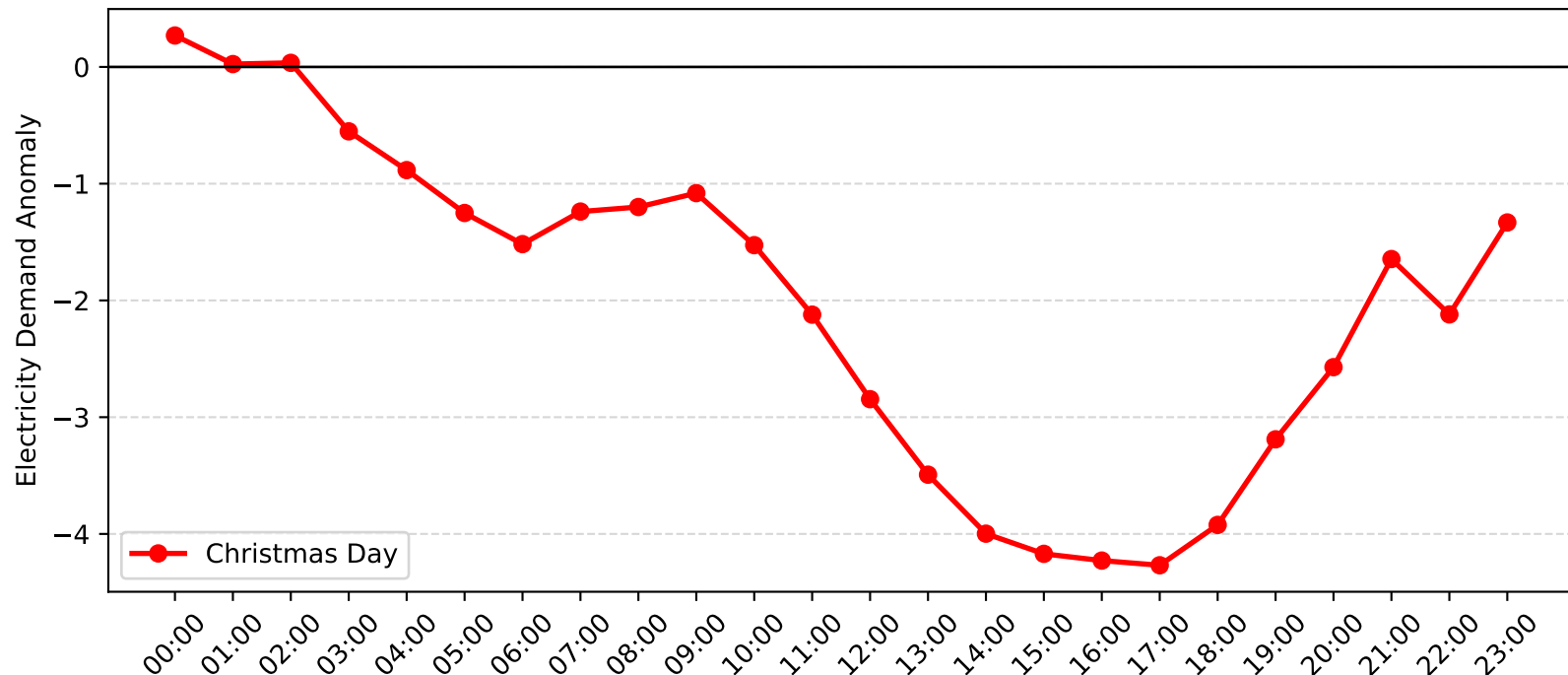
Cardiff Demand Anomaly: Christmas Day (2013-2014)
