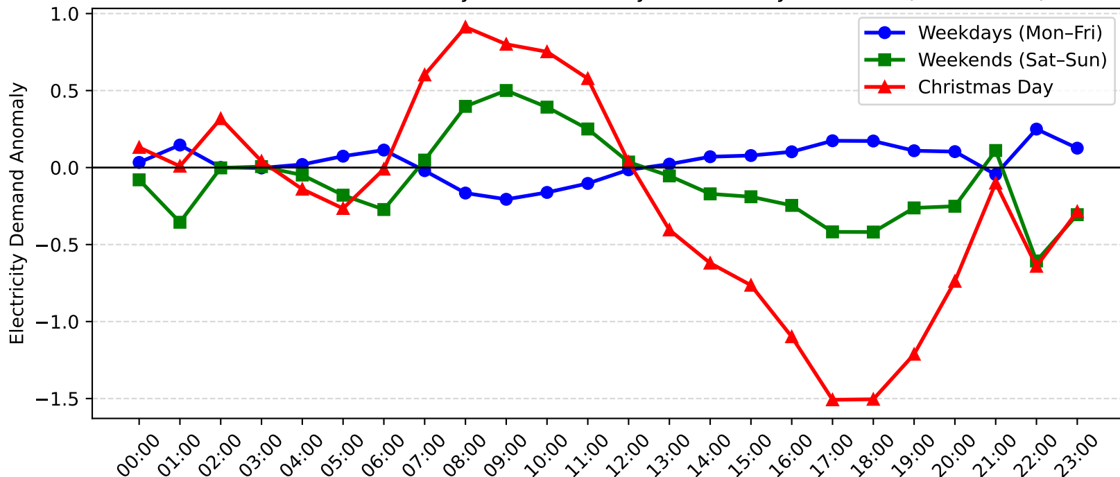
Swansea Demand Anomaly: Christmas Day vs Weekday/Weekend (2015-2016)
