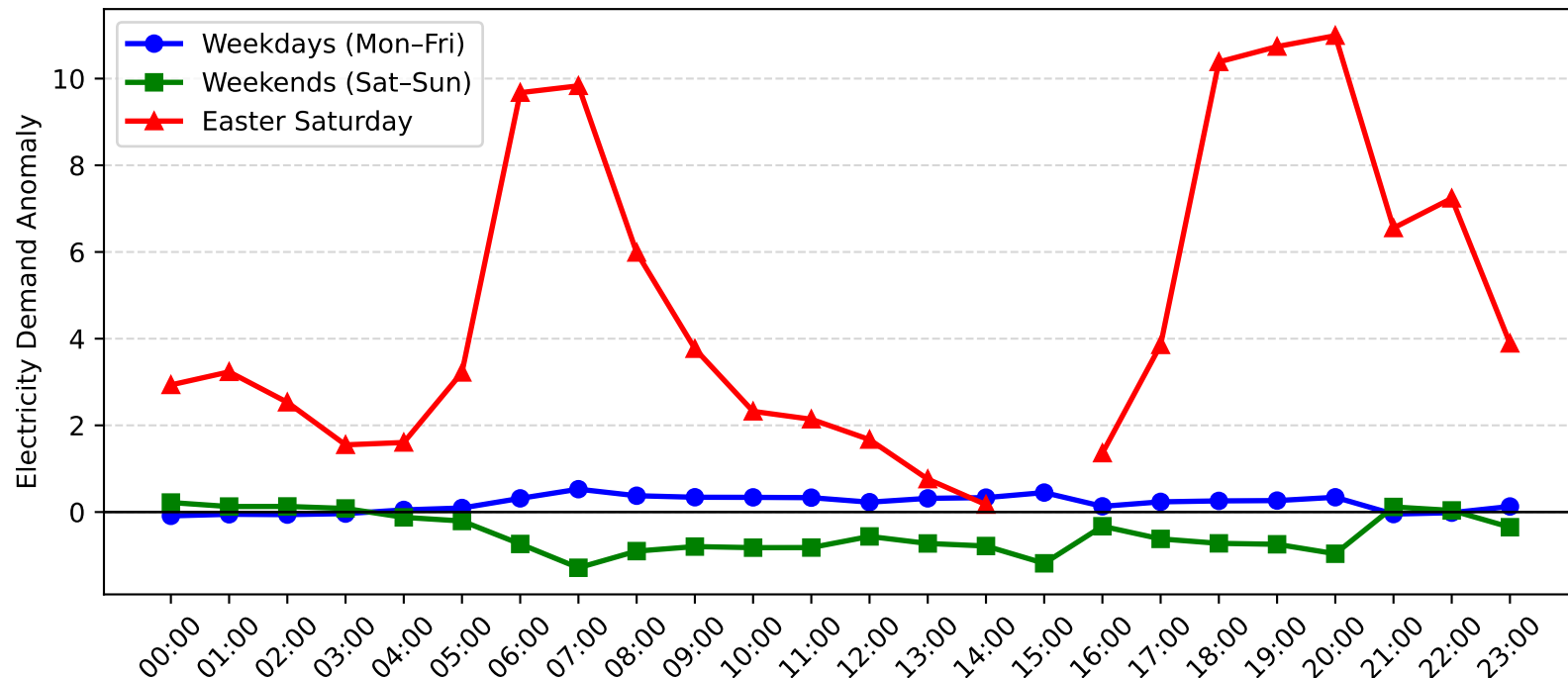
Mortdale Demand Anomaly: Easter Saturday vs Weekday/Weekend (2004-2005)
