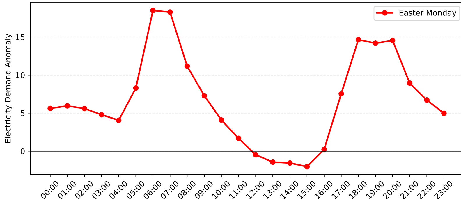
Pennant Hills Demand Anomaly: Easter Monday (2004-2005)
