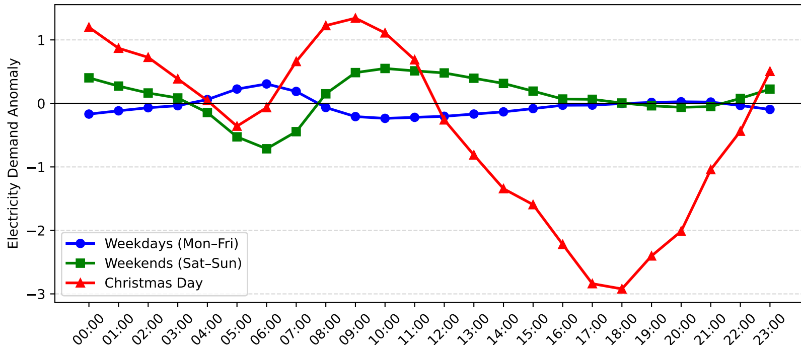
Umina Demand Anomaly: Christmas Day vs Weekday/Weekend (2011-2012)
