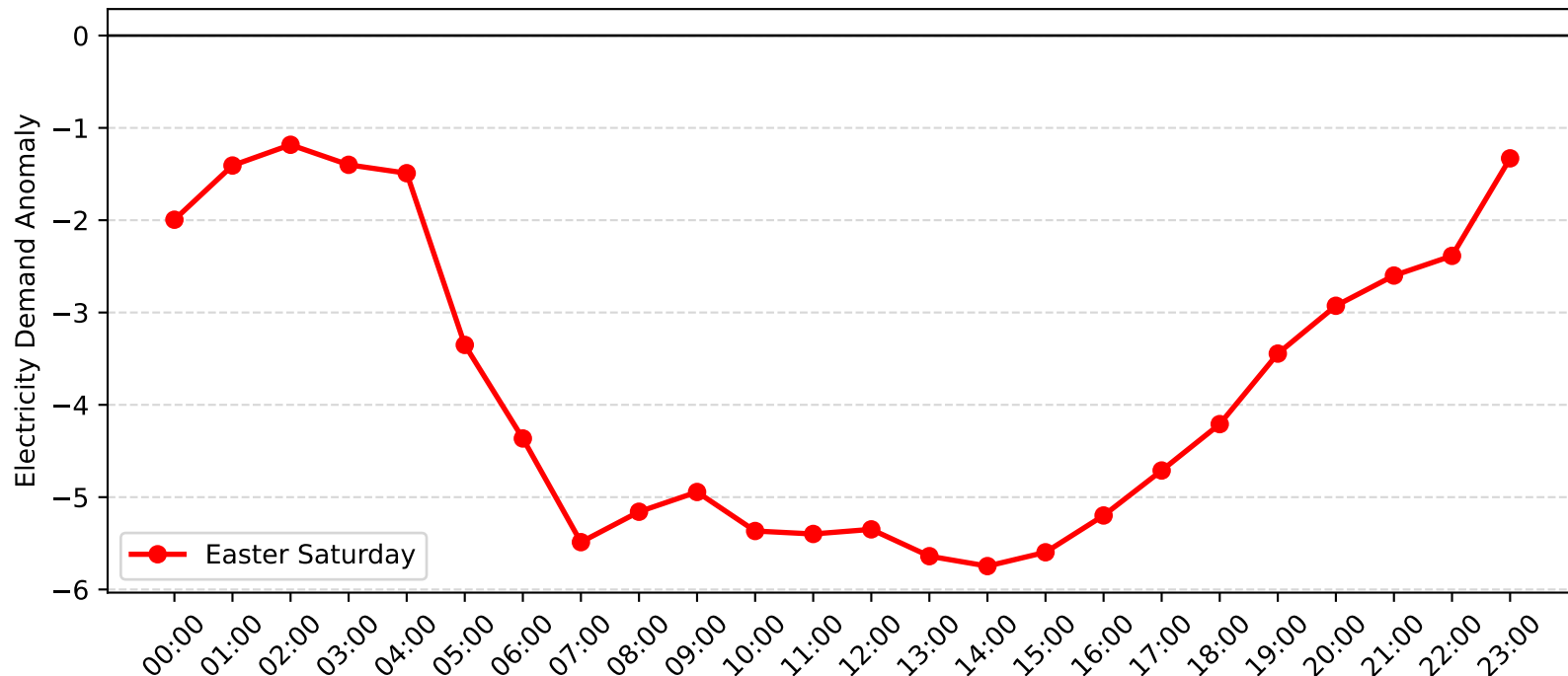
Potts Hill Demand Anomaly: Easter Saturday (2015-2016)
