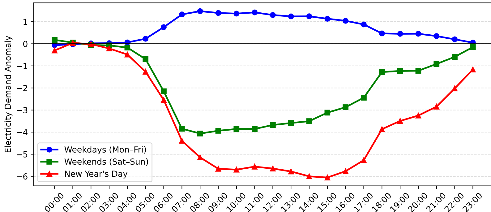
Concord Demand Anomaly: New Year's Day vs Weekday/Weekend (2015-2016)
