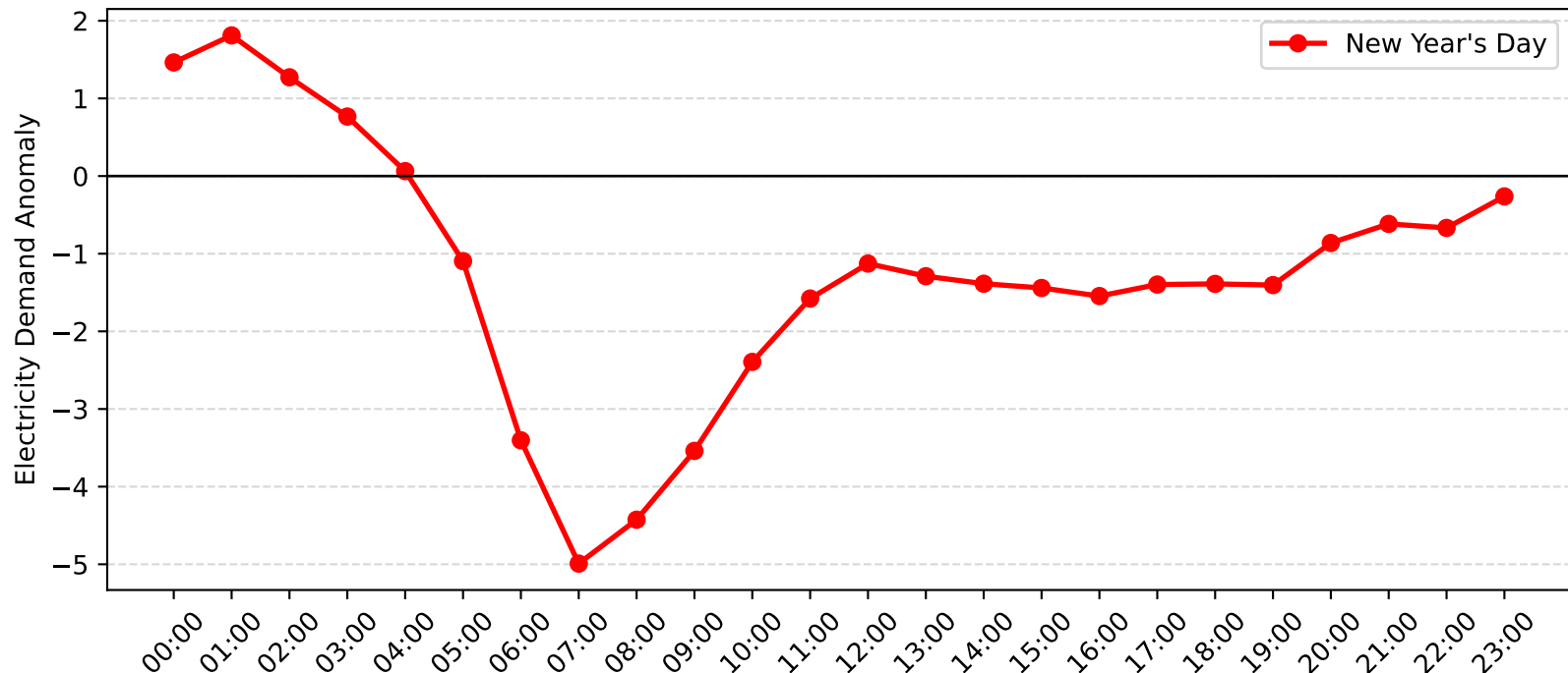
Mortdale Demand Anomaly: New Year's Day (2012-2013)
