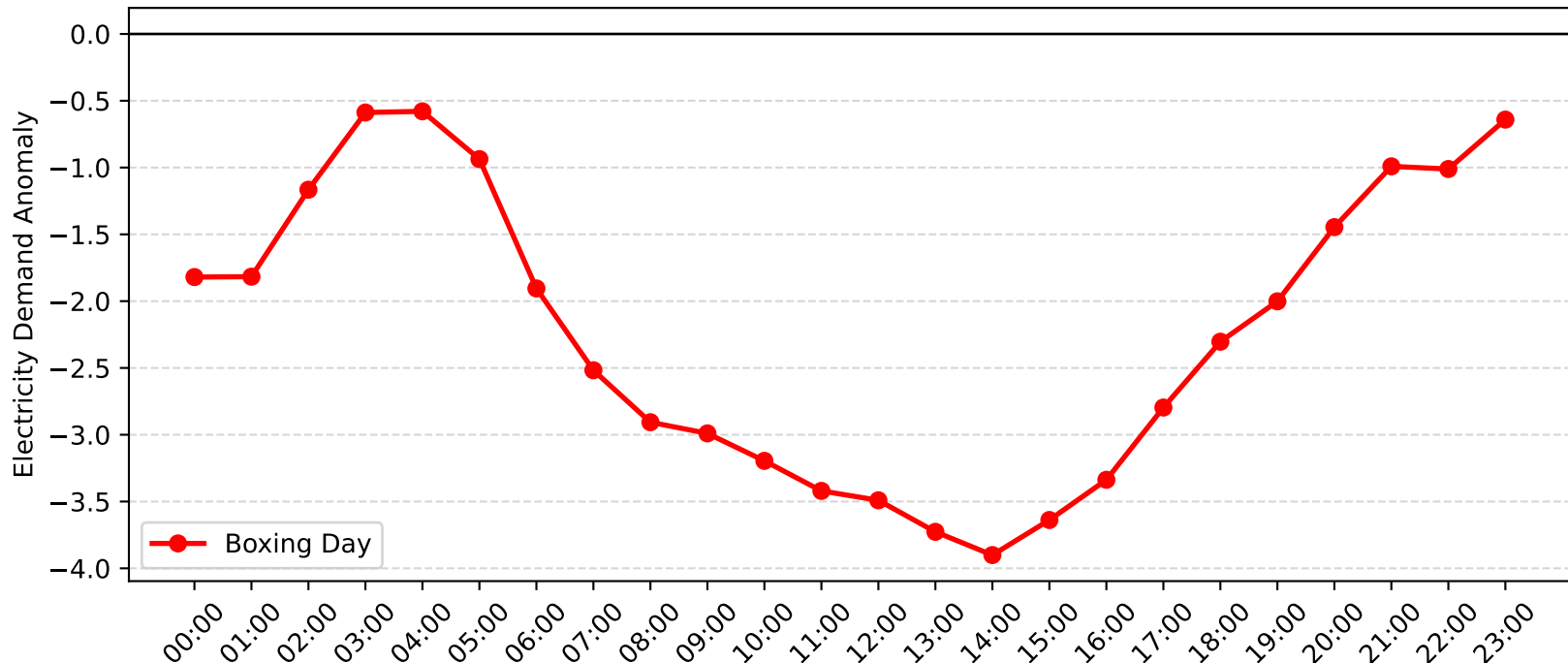
Gateshead Demand Anomaly: Boxing Day (2005-2006)
