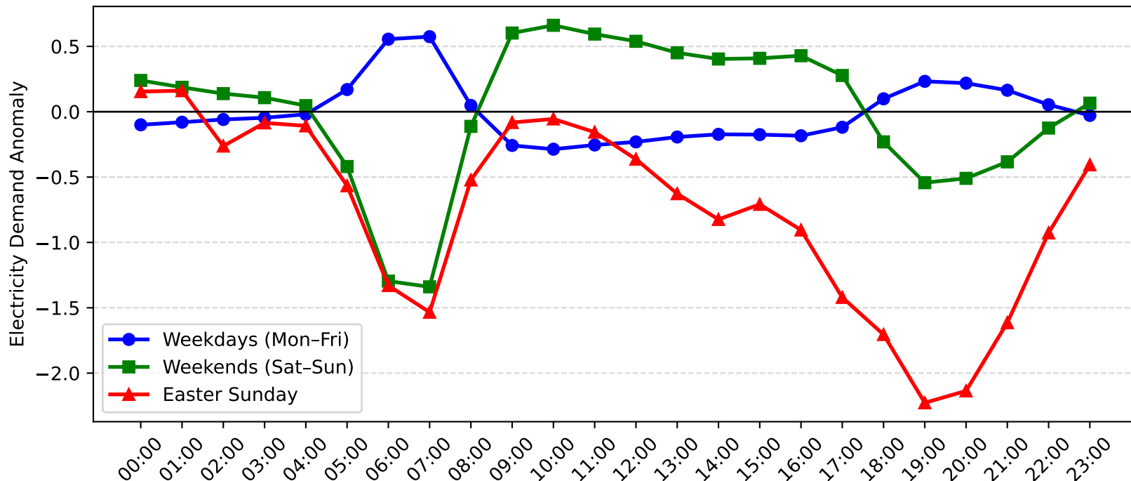
Harbord Demand Anomaly: Easter Sunday vs Weekday/Weekend (2014-2015)
