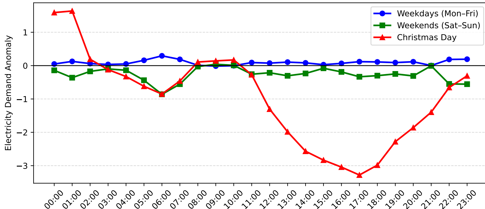
Morisset Demand Anomaly: Christmas Day vs Weekday/Weekend (2013-2014)
