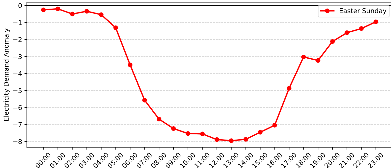
Newcastle Cbd Demand Anomaly: Easter Sunday (2011-2012)
