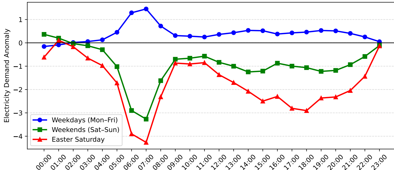
Mortdale Demand Anomaly: Easter Saturday vs Weekday/Weekend (2015-2016)
