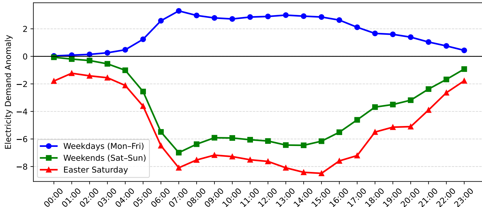
Sefton Demand Anomaly: Easter Saturday vs Weekday/Weekend (2009-2010)
