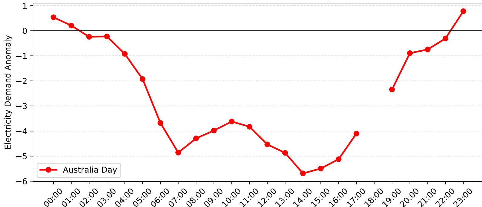
Punchbowl Demand Anomaly: Australia Day (2005-2006)
