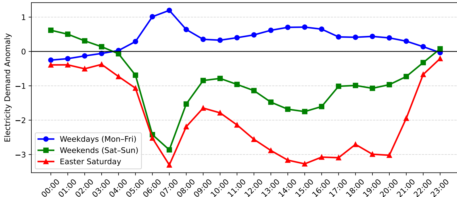
Five Dock Demand Anomaly: Easter Saturday vs Weekday/Weekend (2007-2008)
