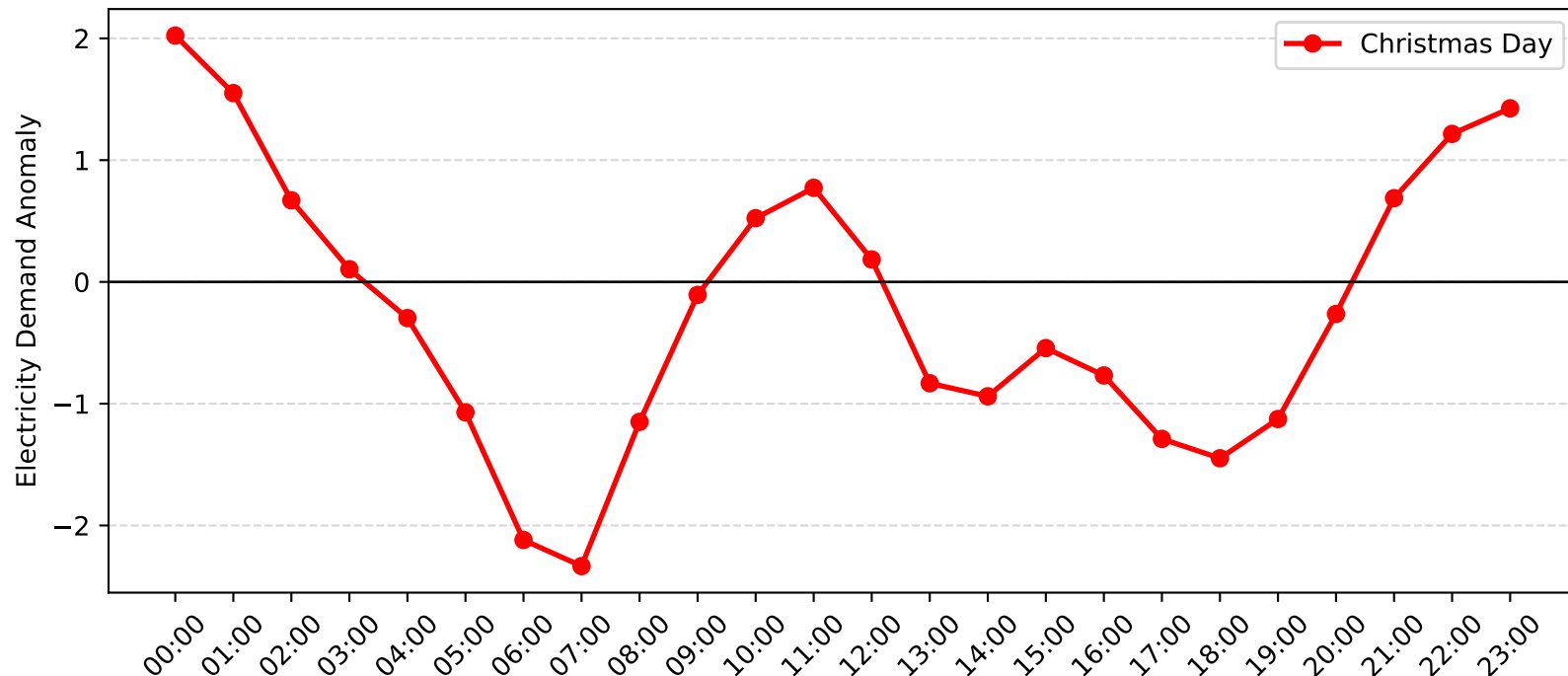
Mortdale Demand Anomaly: Christmas Day (2010-2011)
