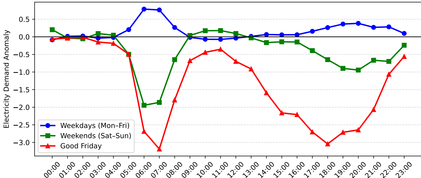
Balgowlah North Demand Anomaly: Good Friday vs Weekday/Weekend (2015-2016)
