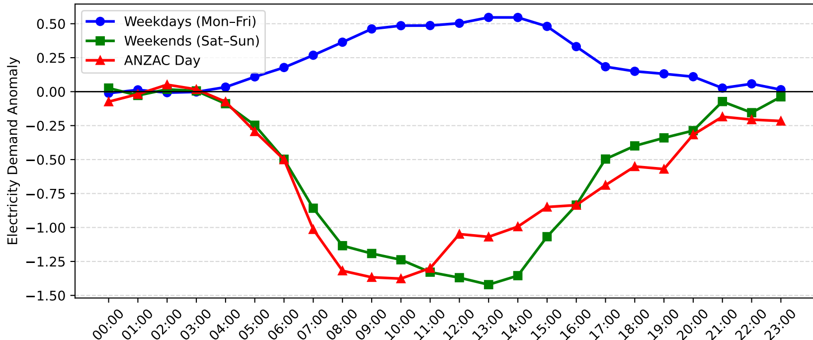
Broadmeadow Demand Anomaly: ANZAC Day vs Weekday/Weekend (2014-2015)
