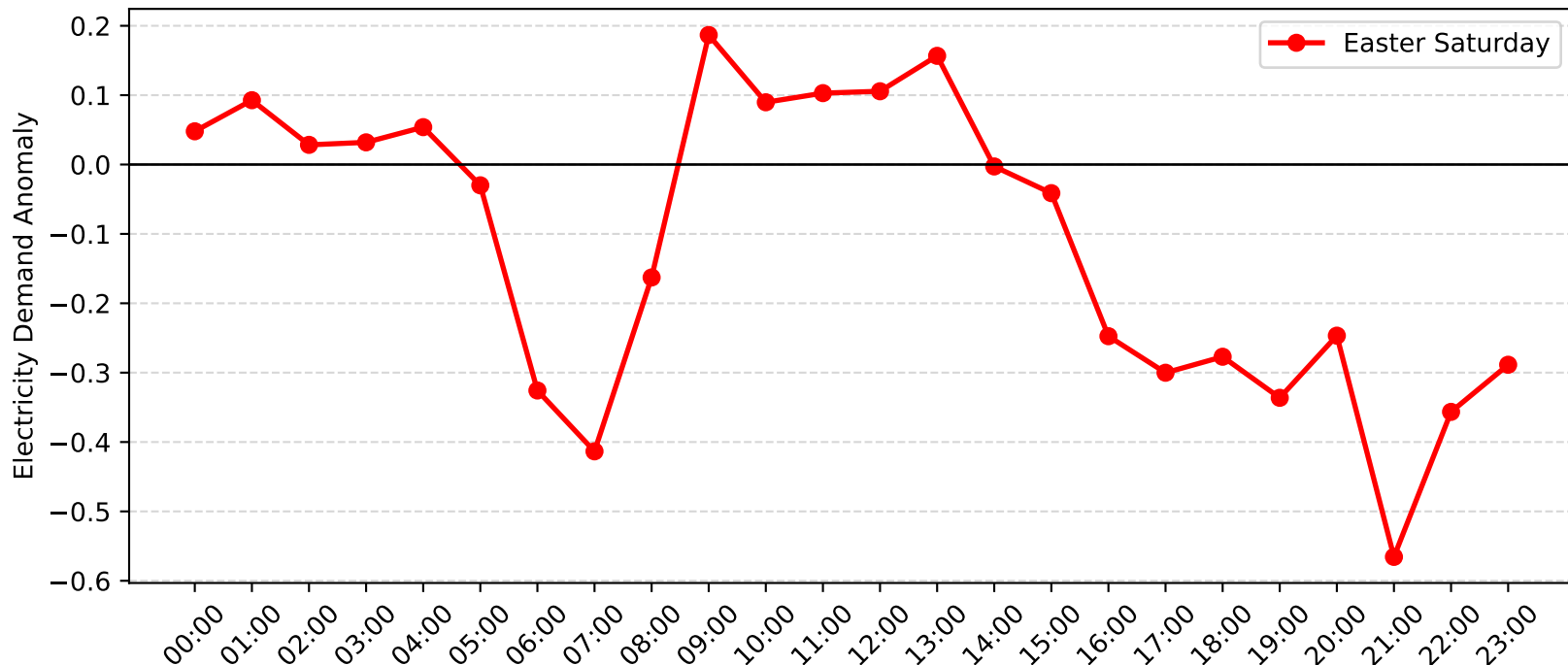
Jesmond Demand Anomaly: Easter Saturday (2010-2011)
