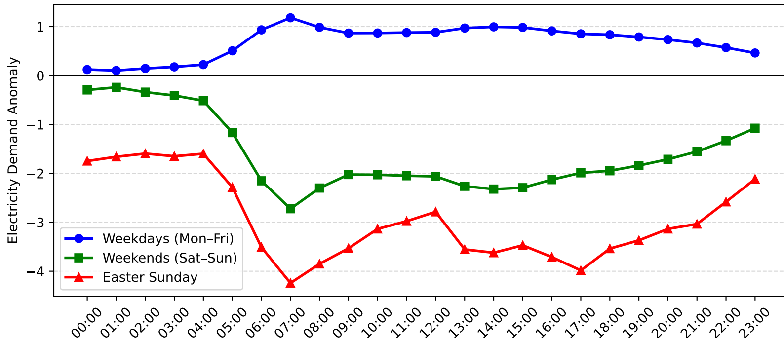
Bass Hill Demand Anomaly: Easter Sunday vs Weekday/Weekend (2011-2012)
