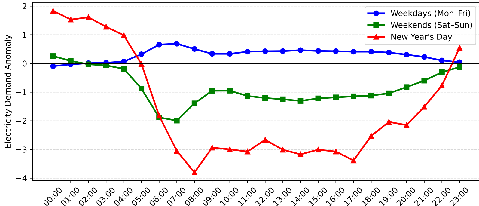
Dee Why West Demand Anomaly: New Year's Day vs Weekday/Weekend (2015-2016)
