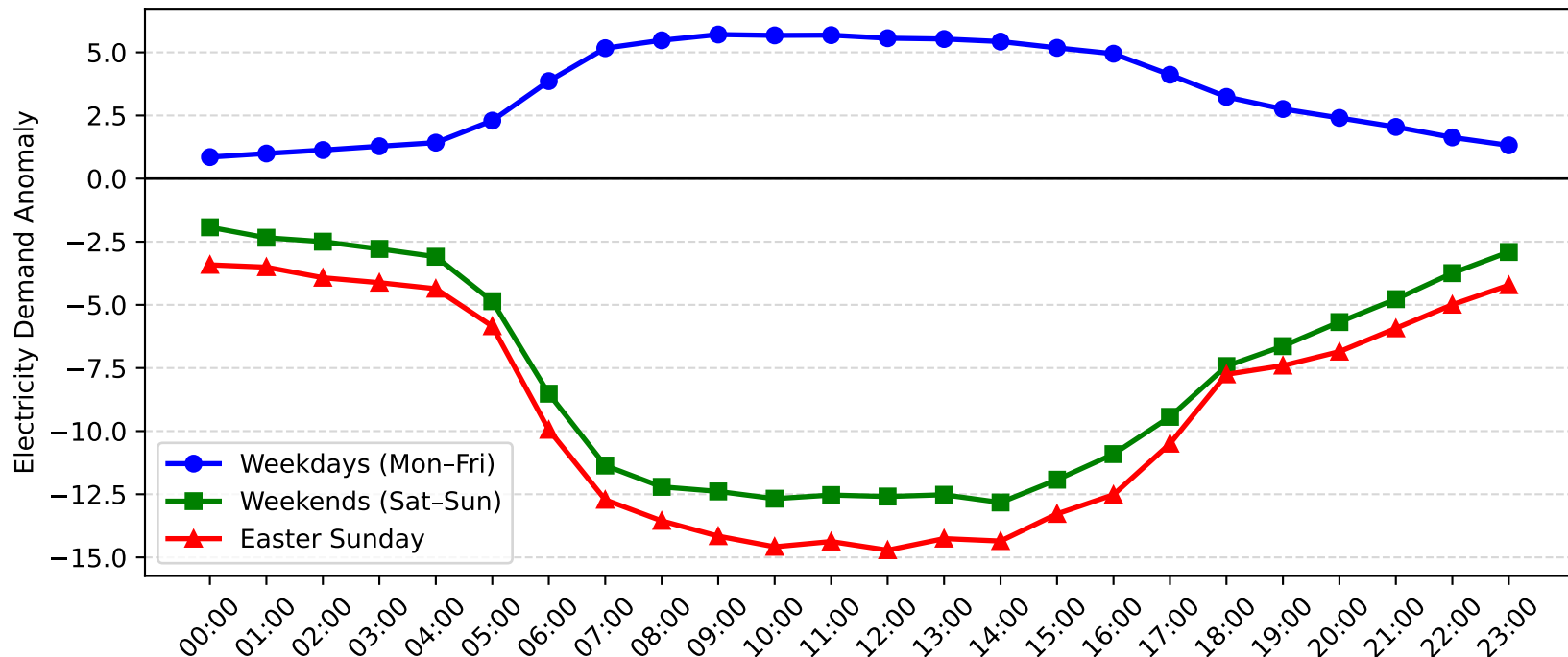
Flemington Demand Anomaly: Easter Sunday vs Weekday/Weekend (2010-2011)
