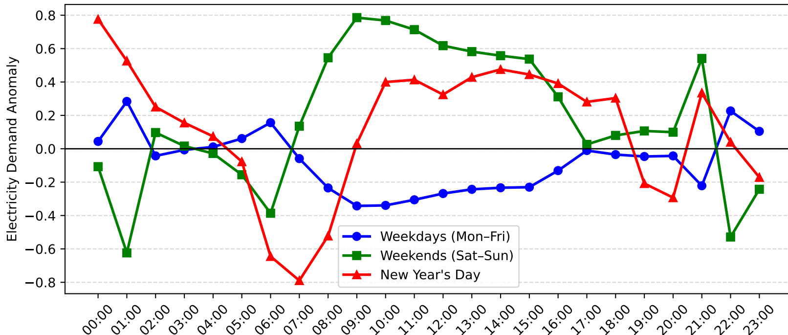
Swansea Demand Anomaly: New Year's Day vs Weekday/Weekend (2007-2008)
