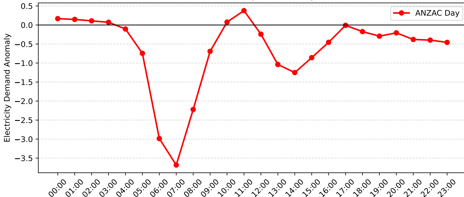
Five Dock Demand Anomaly: ANZAC Day (2006-2007)
