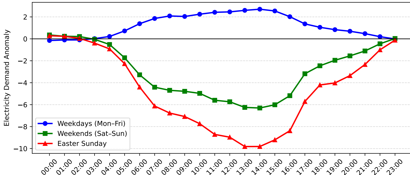
West Gosford Demand Anomaly: Easter Sunday vs Weekday/Weekend (2006-2007)
