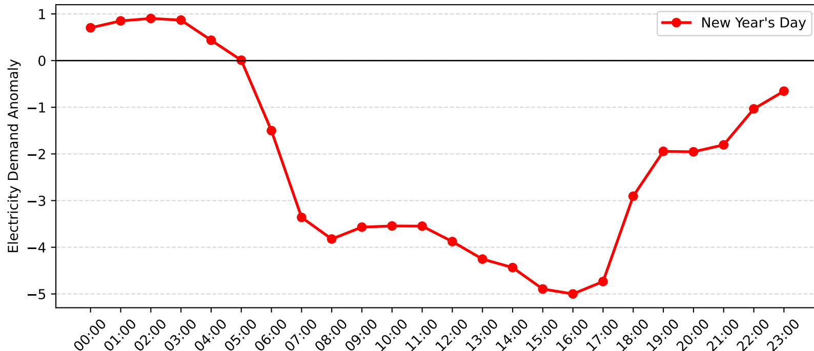
Pymble Demand Anomaly: New Year's Day (2017-2018)
