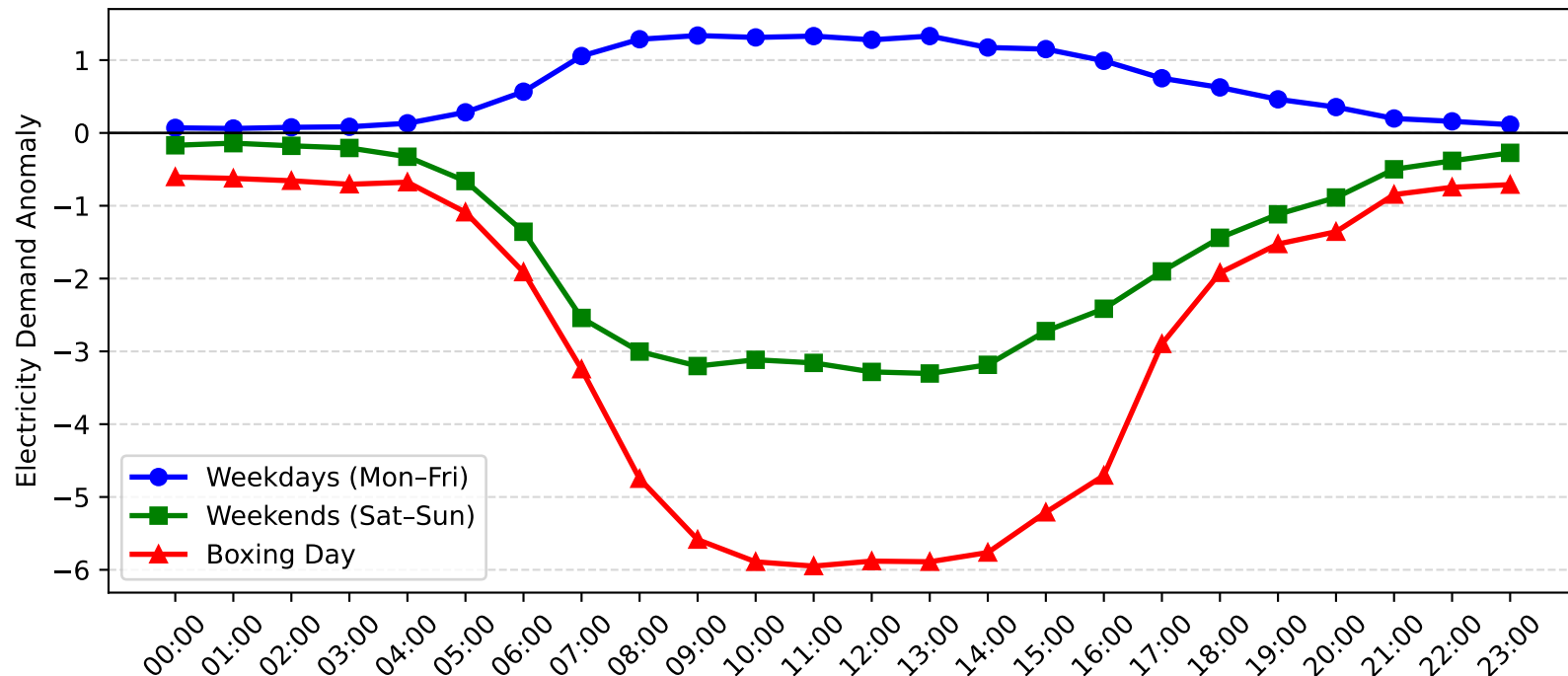
Auburn Demand Anomaly: Boxing Day vs Weekday/Weekend (2005-2006)
