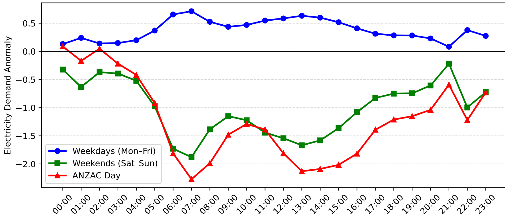
Cardiff Demand Anomaly: ANZAC Day vs Weekday/Weekend (2013-2014)
