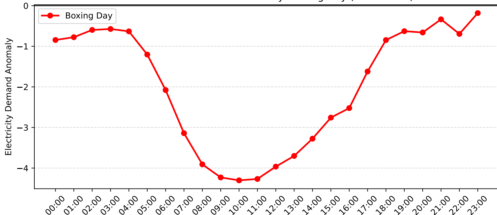
Broadmeadow Demand Anomaly: Boxing Day (2015-2016)
