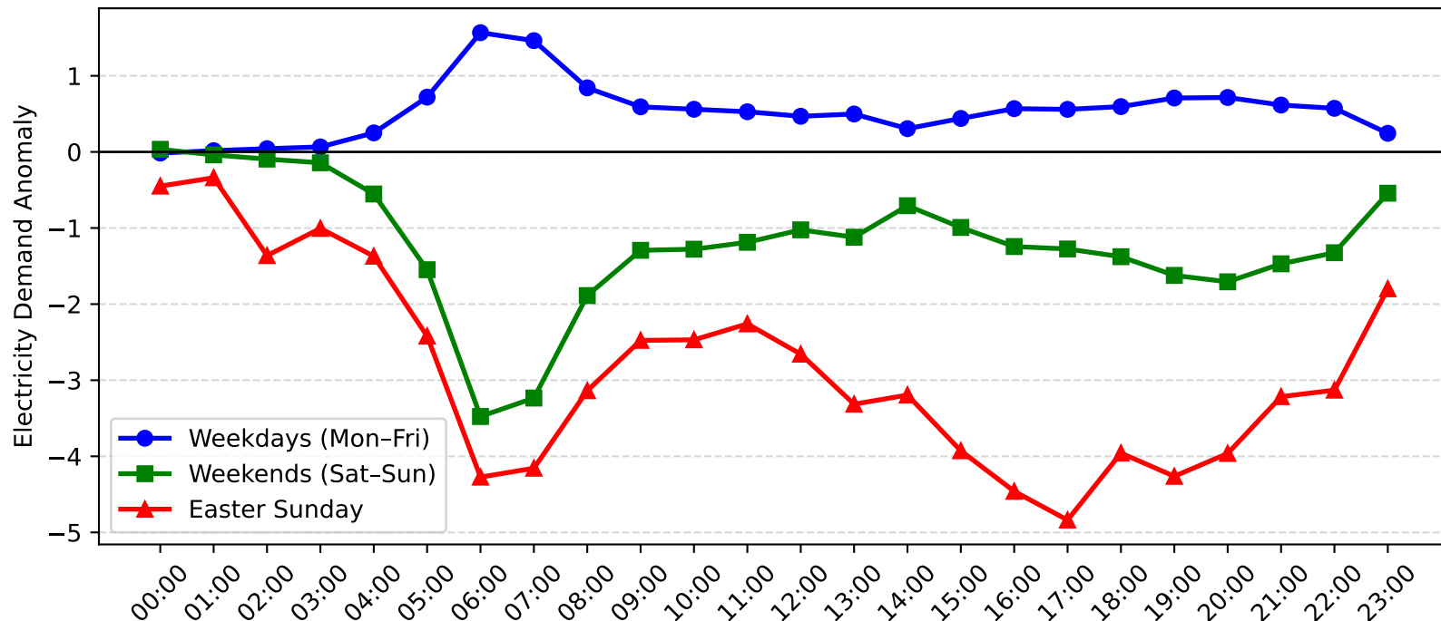
Revesby Demand Anomaly: Easter Sunday vs Weekday/Weekend (2009-2010)
