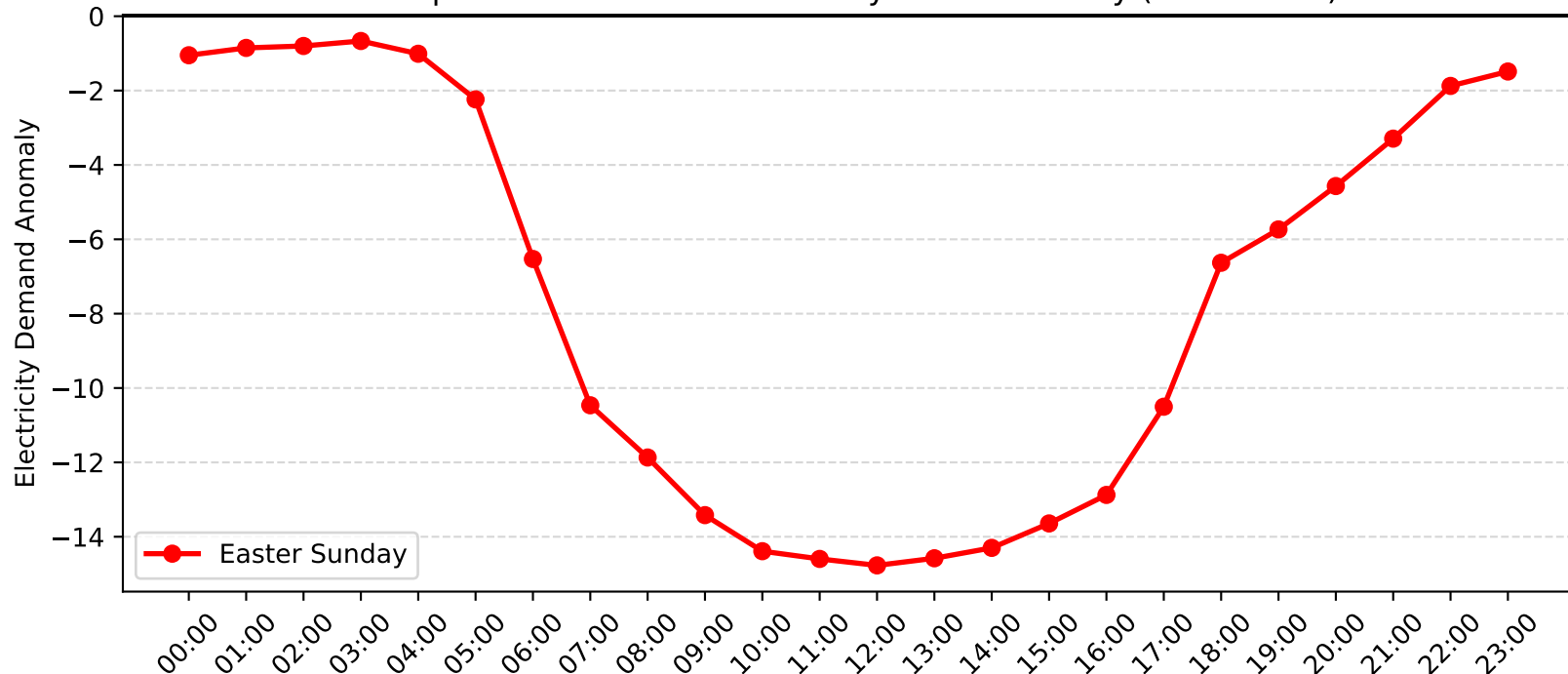
Macquarie Park Demand Anomaly: Easter Sunday (2012-2013)
