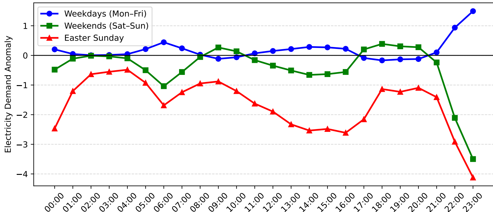
Muswellbrook Demand Anomaly: Easter Sunday vs Weekday/Weekend (2006-2007)
