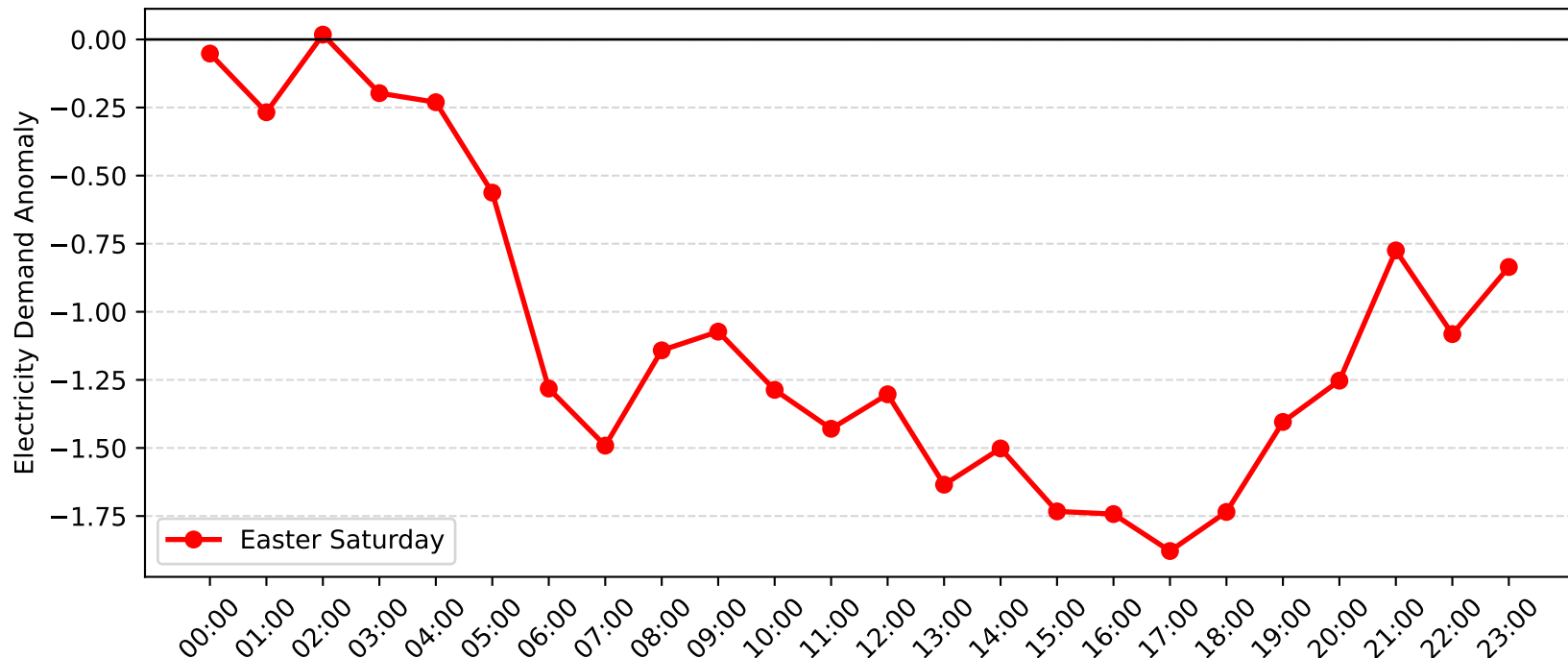
Maryland Demand Anomaly: Easter Saturday (2013-2014)
