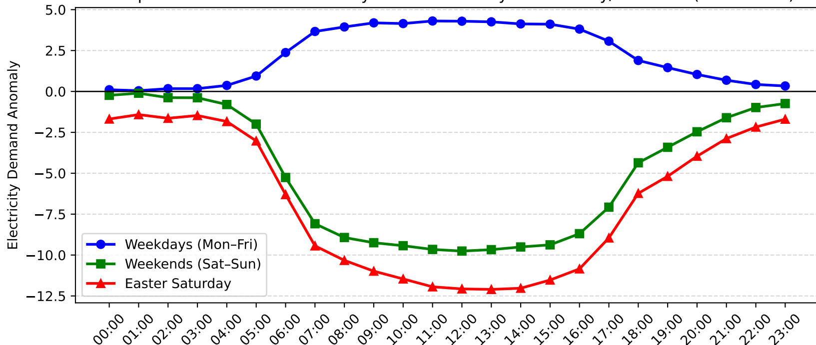
Macquarie Park Demand Anomaly: Easter Saturday vs Weekday/Weekend (2010-2011)
