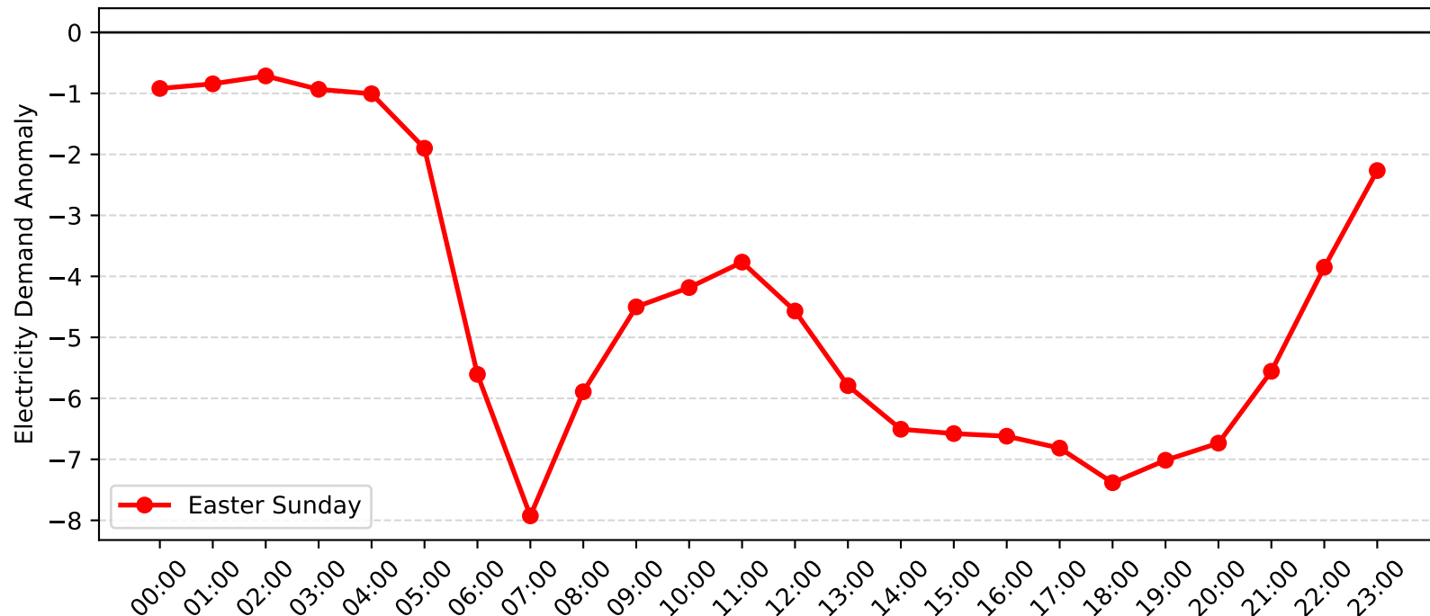
Mosman Demand Anomaly: Easter Sunday (2016-2017)
