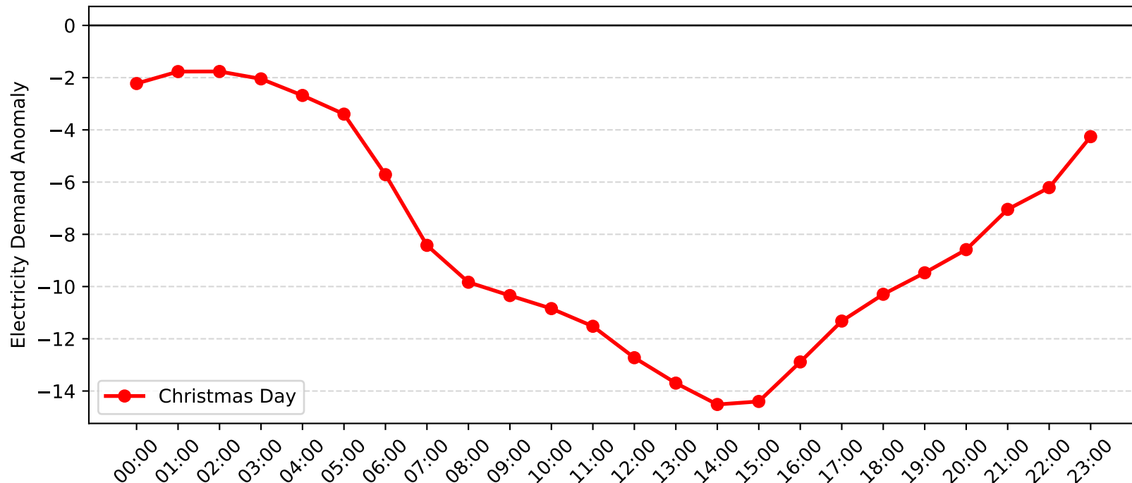
Marrickville Demand Anomaly: Christmas Day (2013-2014)
