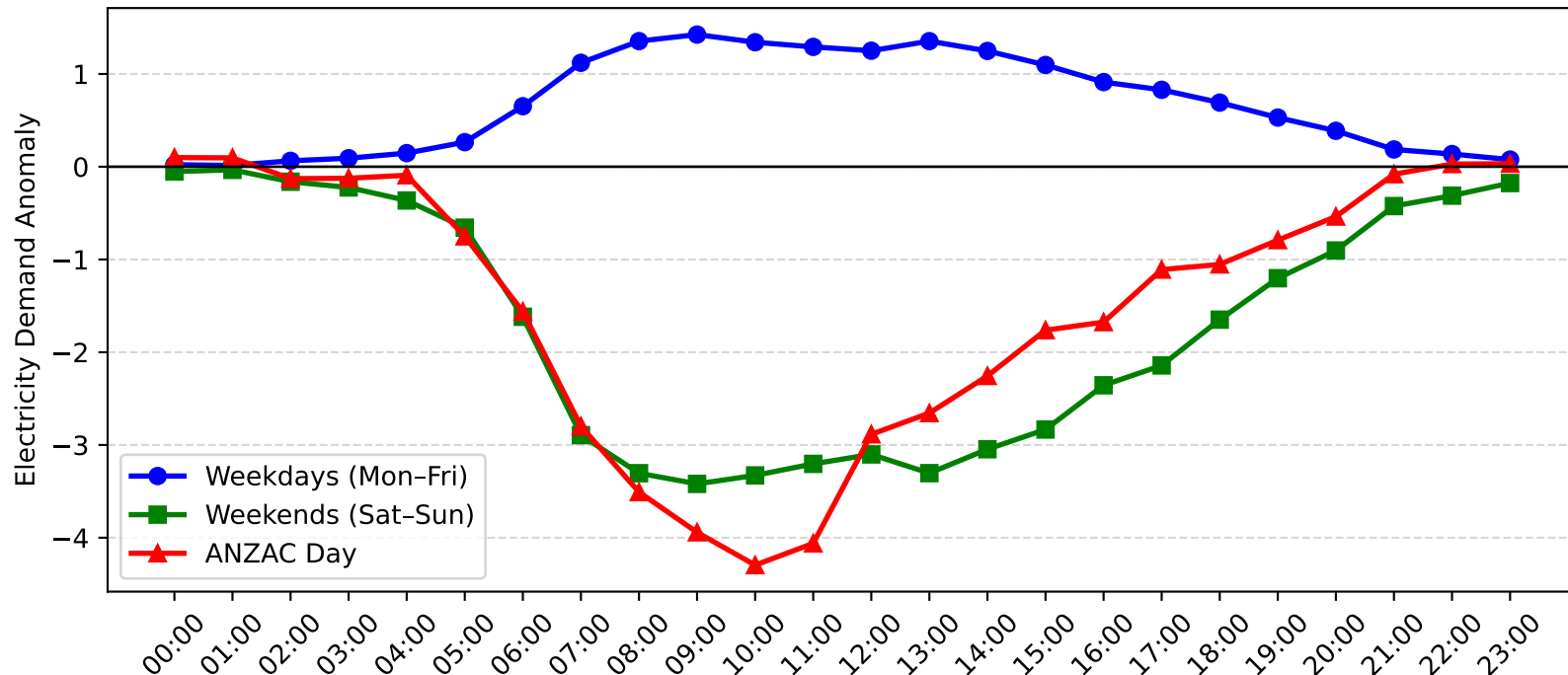
Auburn Demand Anomaly: ANZAC Day vs Weekday/Weekend (2008-2009)
