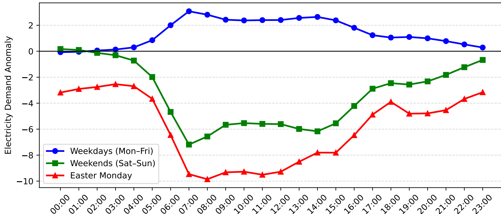
Marrickville Demand Anomaly: Easter Monday vs Weekday/Weekend (2014-2015)
