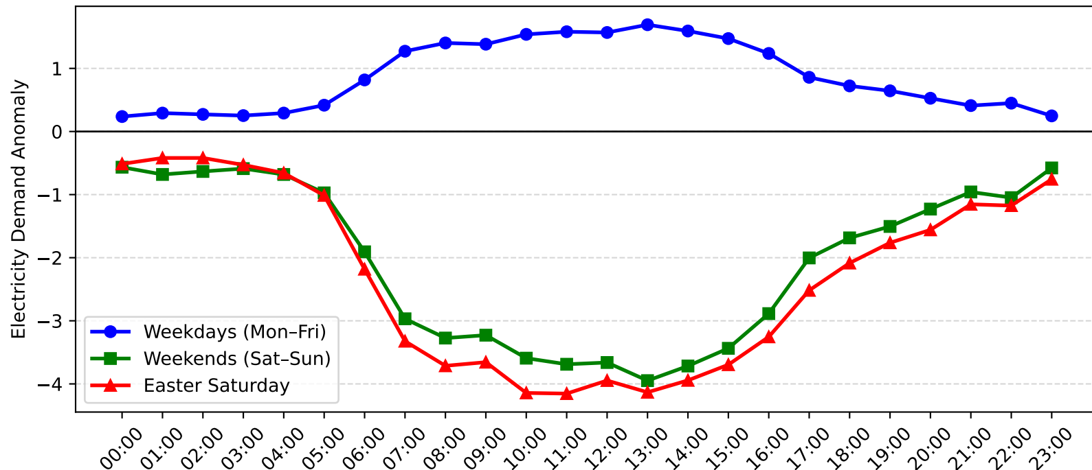
Mayfield West Demand Anomaly: Easter Saturday vs Weekday/Weekend (2012-2013)
