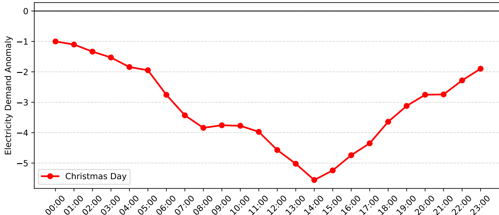
Bass Hill Demand Anomaly: Christmas Day (2005-2006)
