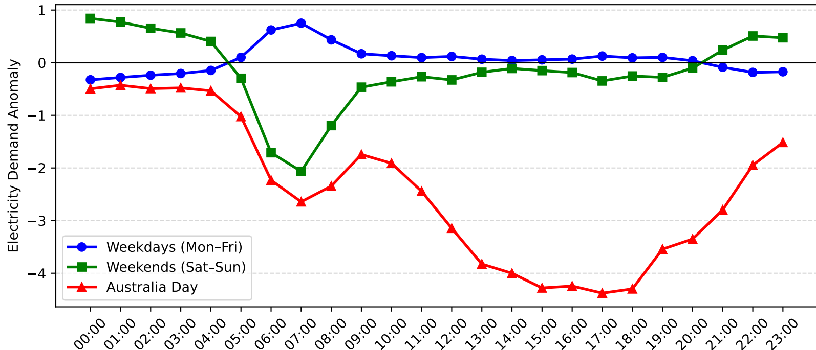
Dee Why West Demand Anomaly: Australia Day vs Weekday/Weekend (2017-2018)
