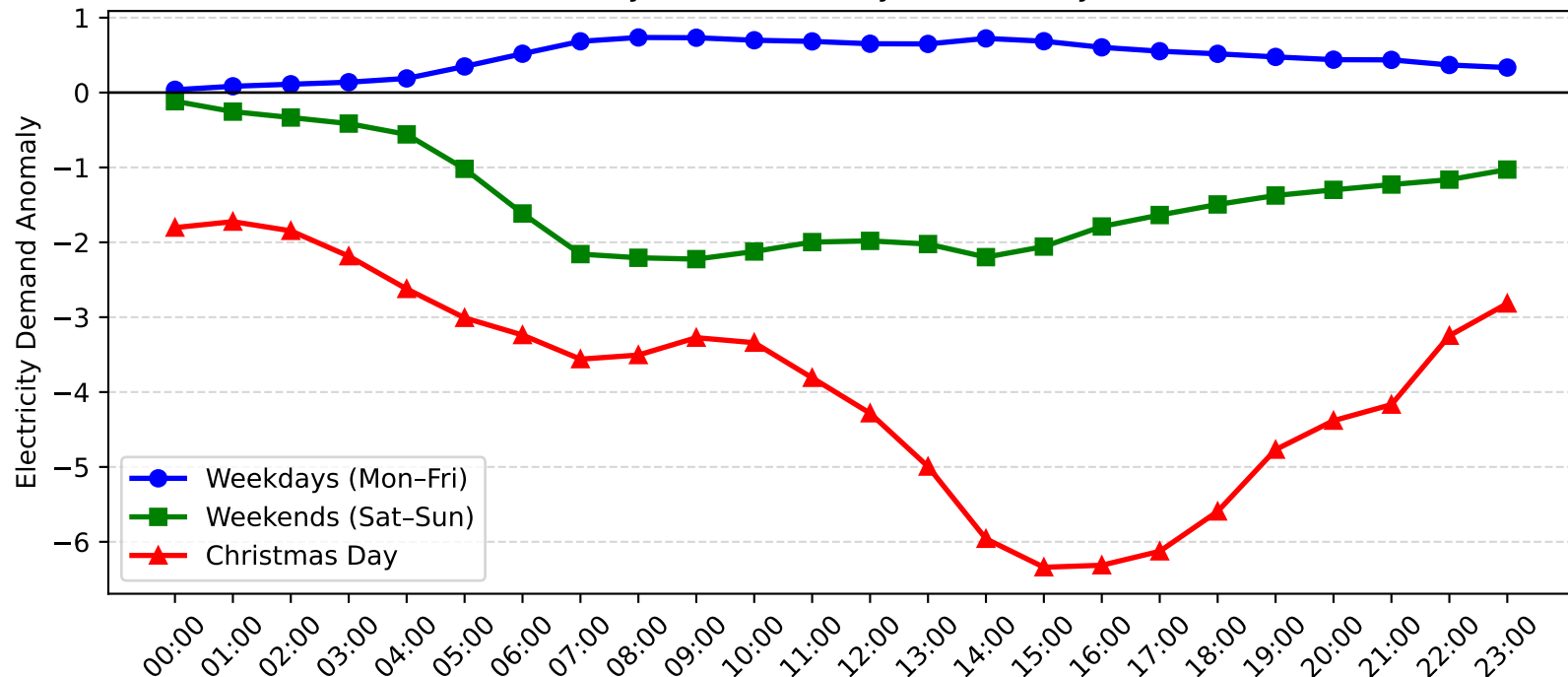
Bass Hill Demand Anomaly: Christmas Day vs Weekday/Weekend (2013-2014)
