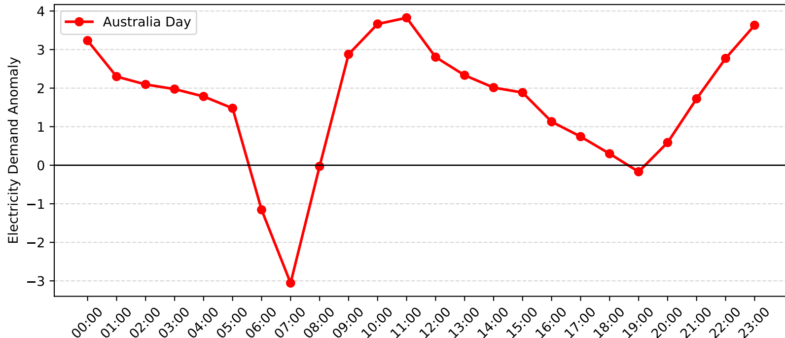
Mosman Demand Anomaly: Australia Day (2012-2013)
