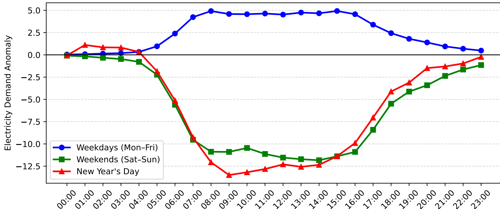
Zetland Demand Anomaly: New Year's Day vs Weekday/Weekend (2006-2007)
