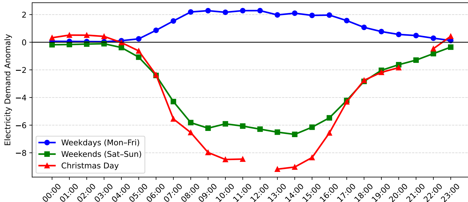
Green Square Demand Anomaly: Christmas Day vs Weekday/Weekend (2014-2015)
