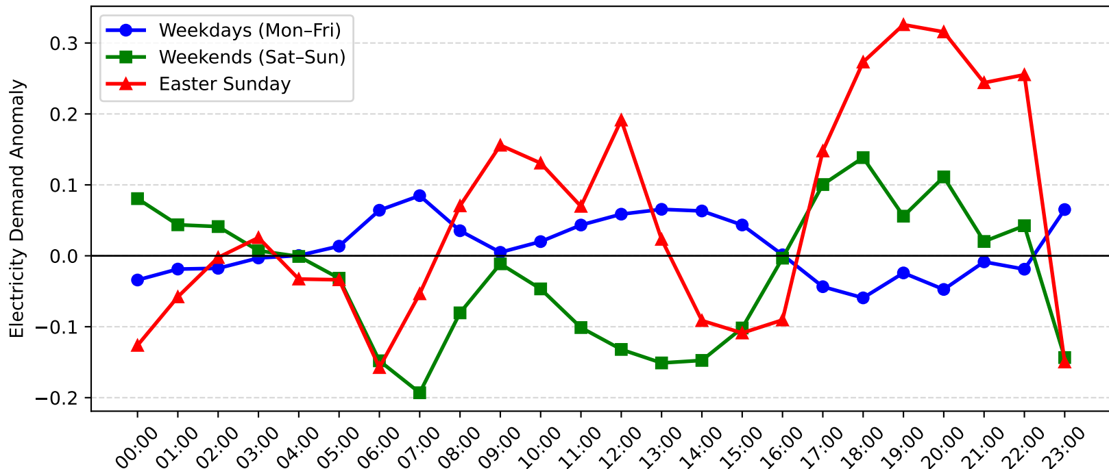
Rothbury Demand Anomaly: Easter Sunday vs Weekday/Weekend (2008-2009)
