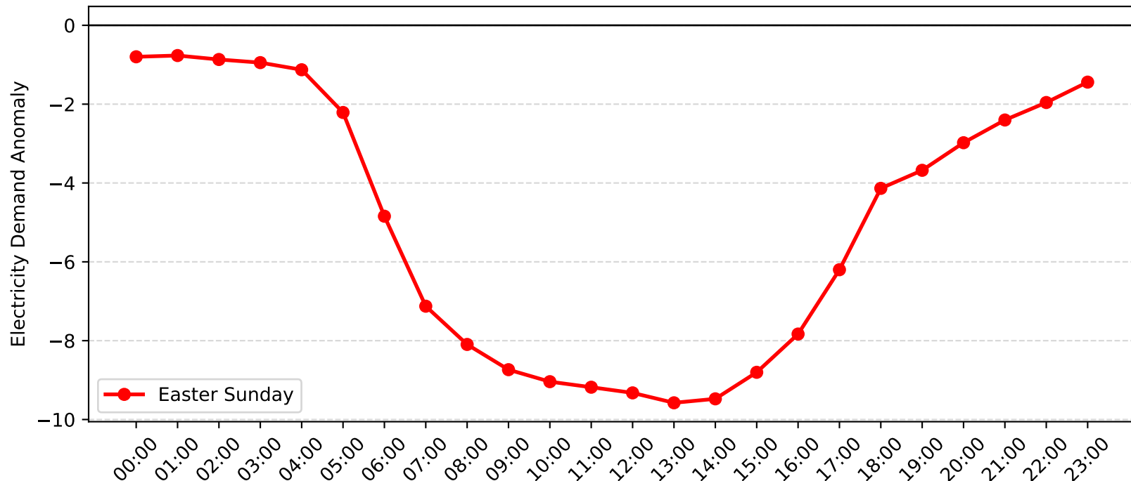
Mascot Demand Anomaly: Easter Sunday (2014-2015)
