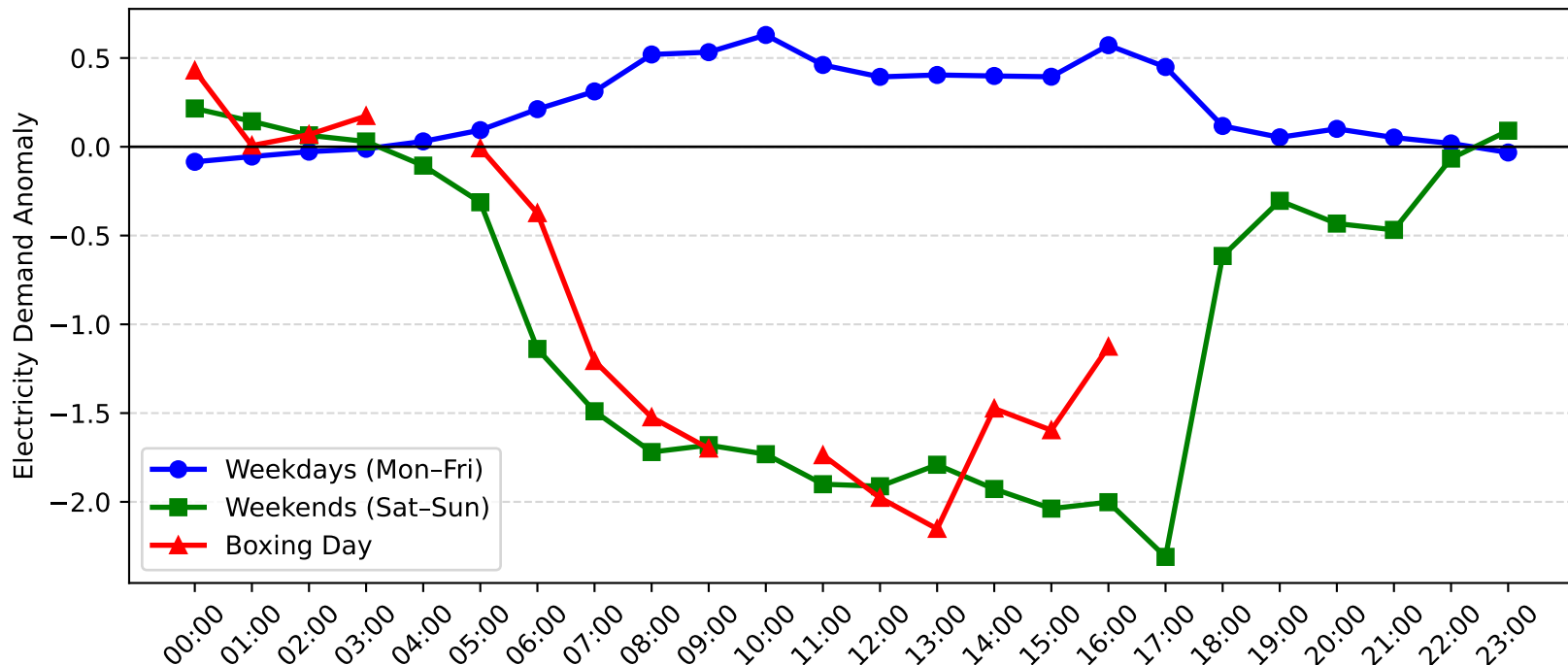
Potts Hill Demand Anomaly: Boxing Day vs Weekday/Weekend (2012-2013)
