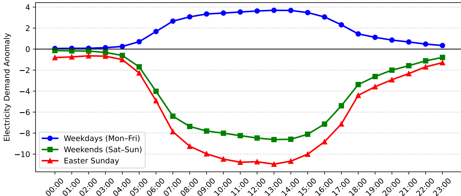
Mascot Demand Anomaly: Easter Sunday vs Weekday/Weekend (2012-2013)
