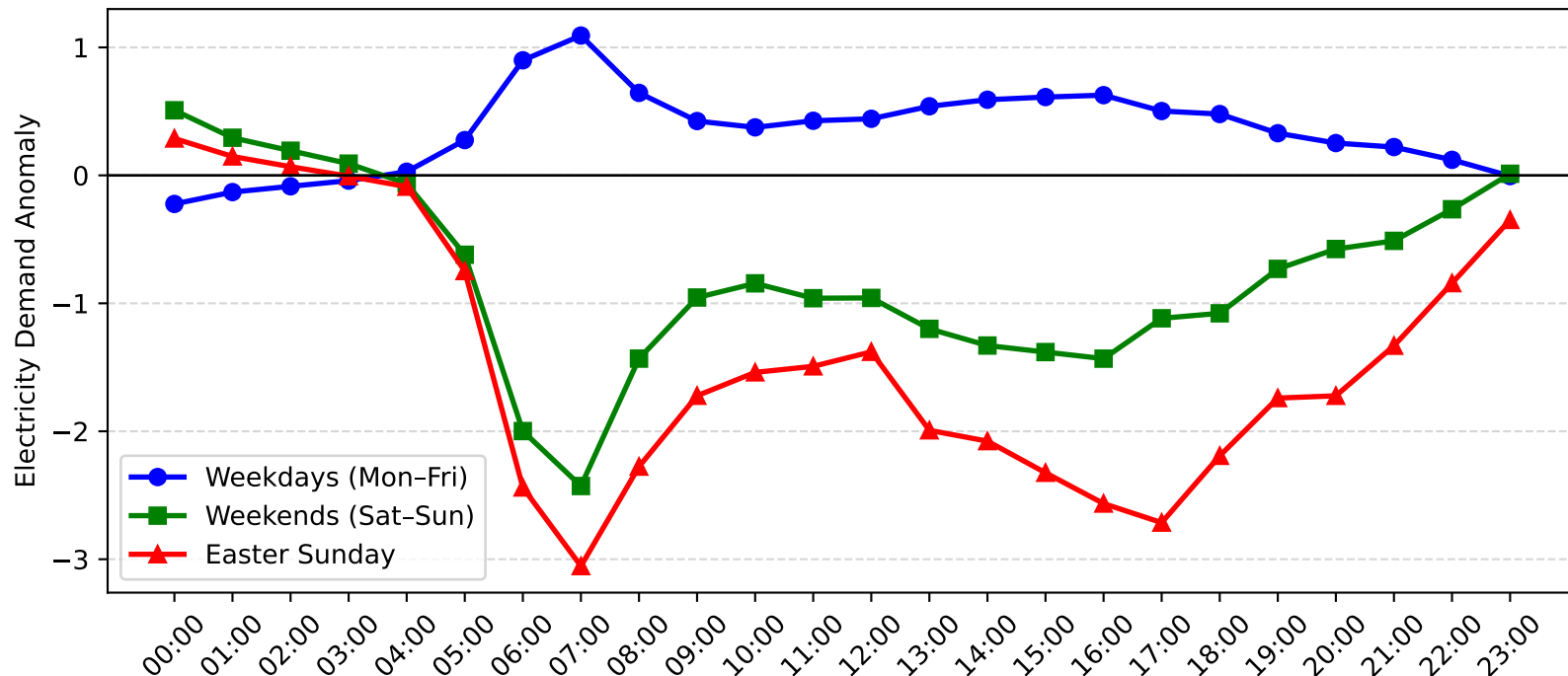
Blakehurst Demand Anomaly: Easter Sunday vs Weekday/Weekend (2008-2009)
