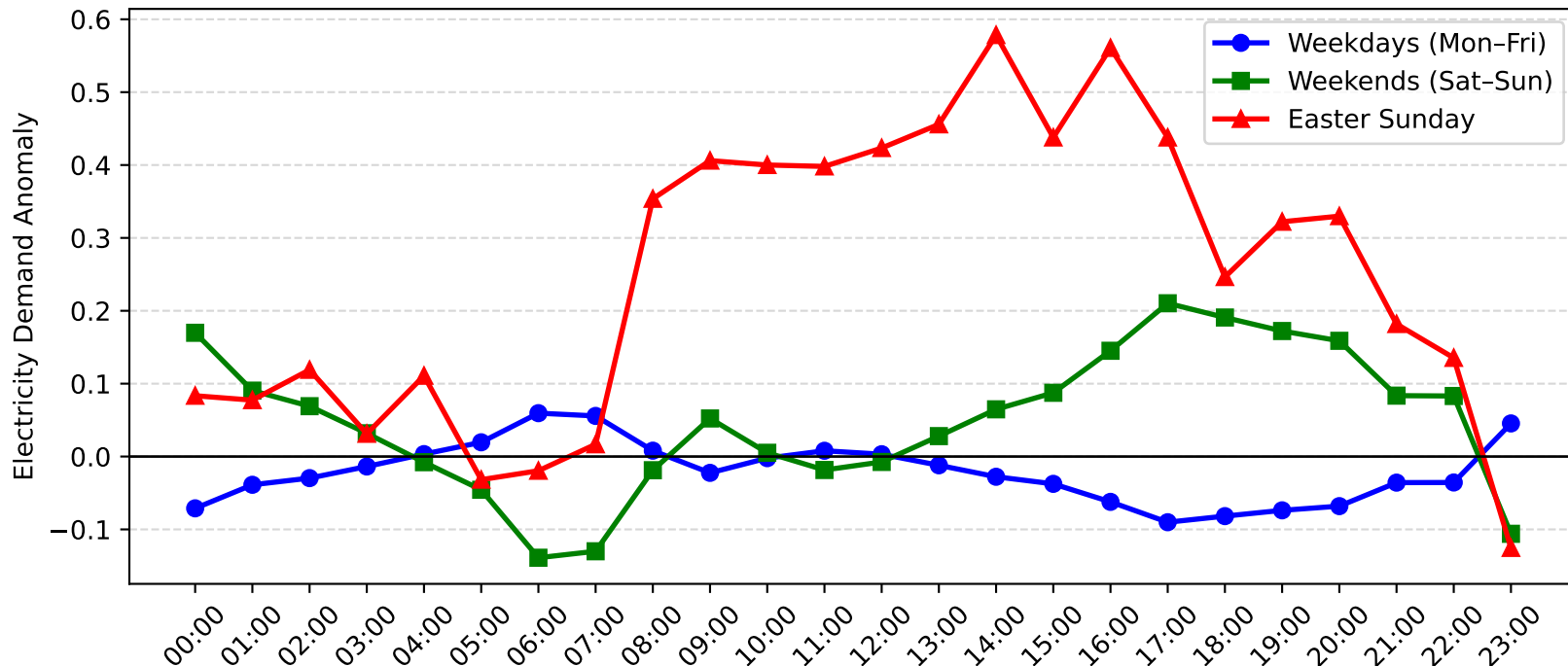
Rothbury Demand Anomaly: Easter Sunday vs Weekday/Weekend (2012-2013)
