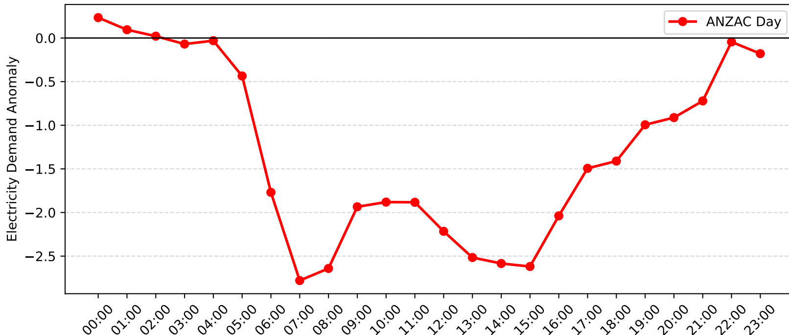
Beacon Hill Demand Anomaly: ANZAC Day (2007-2008)
