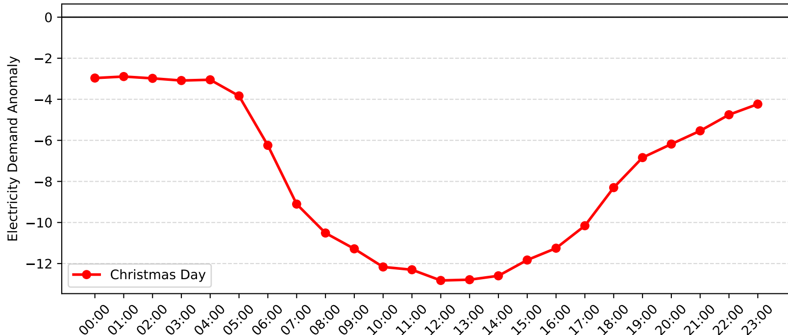
Macquarie Park Demand Anomaly: Christmas Day (2005-2006)
