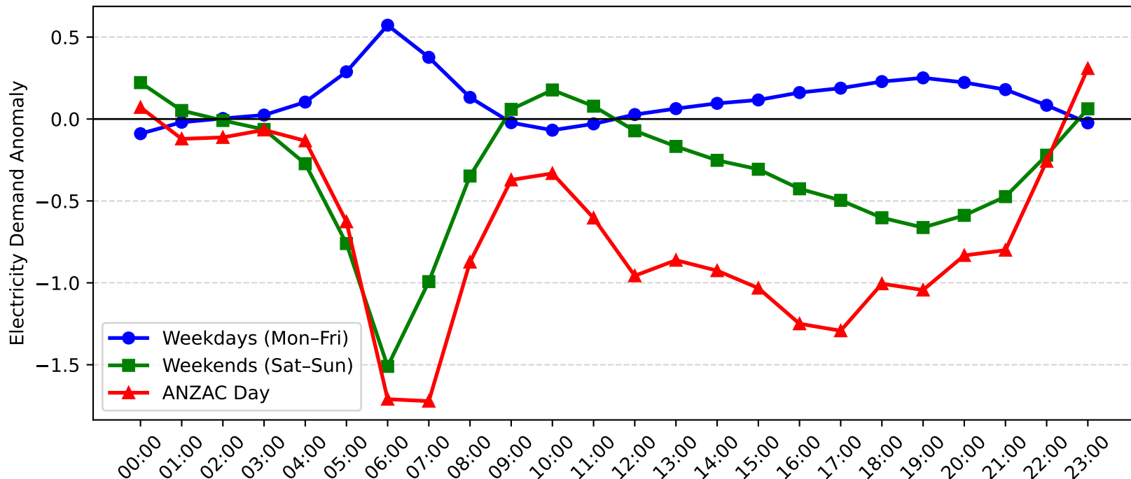
Woy Woy Demand Anomaly: ANZAC Day vs Weekday/Weekend (2013-2014)
