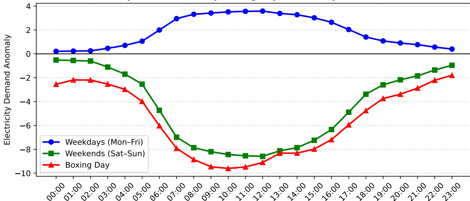
Homebush Bay Demand Anomaly: Boxing Day vs Weekday/Weekend (2015-2016)
