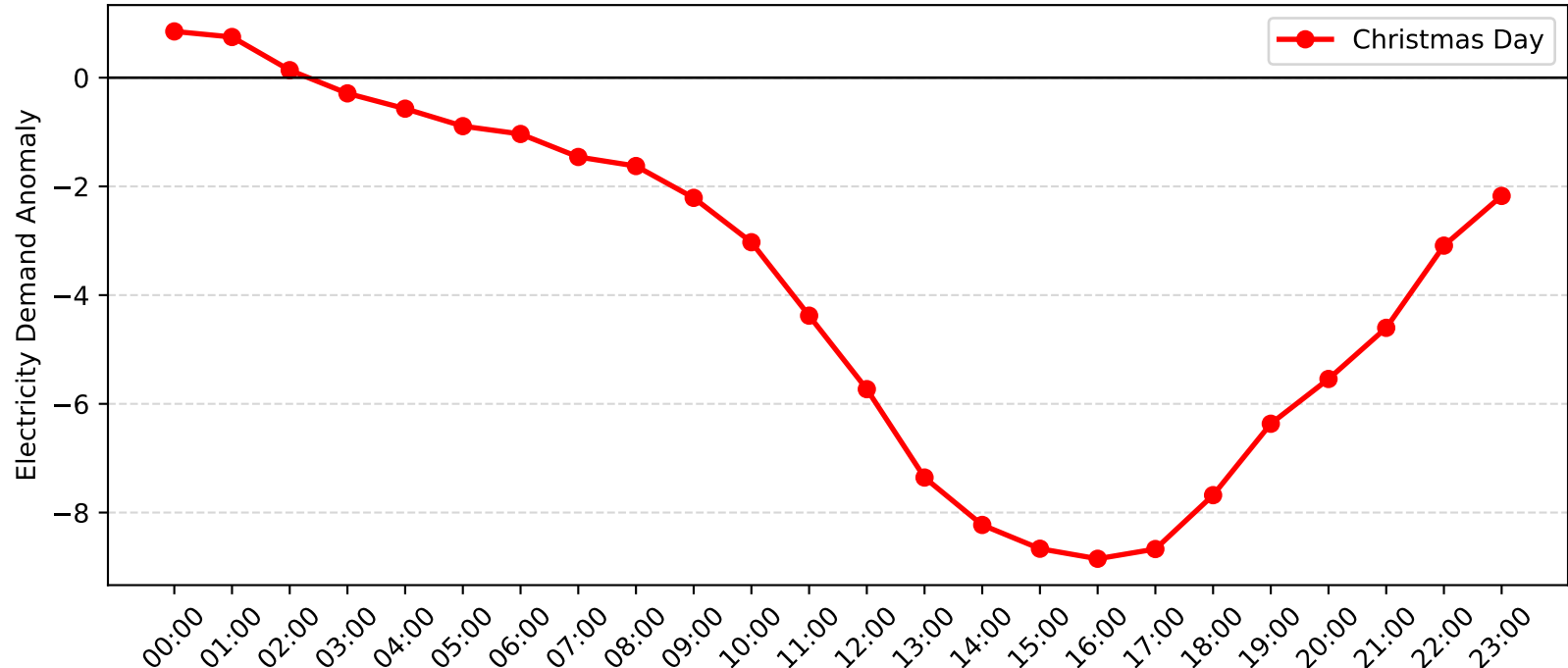
Jesmond Demand Anomaly: Christmas Day (2012-2013)
