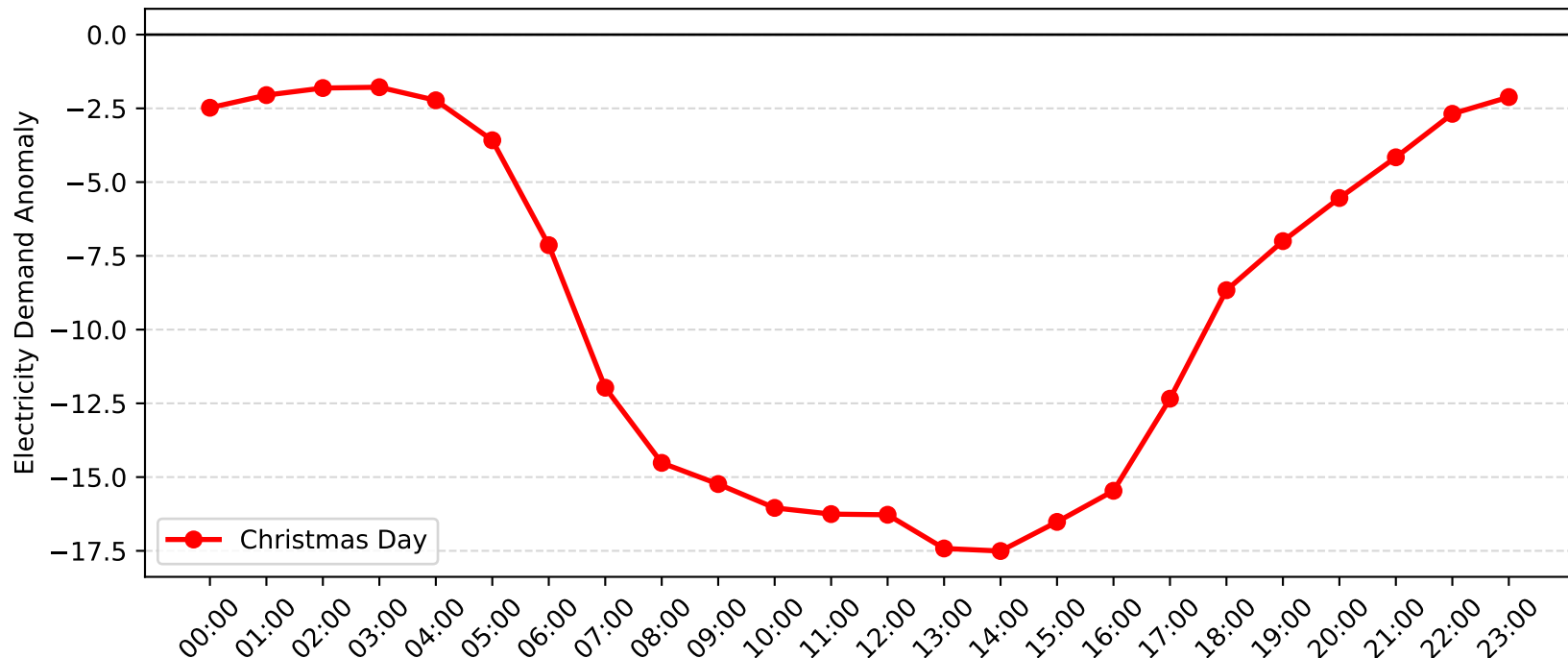
Gore Hill Demand Anomaly: Christmas Day (2010-2011)
