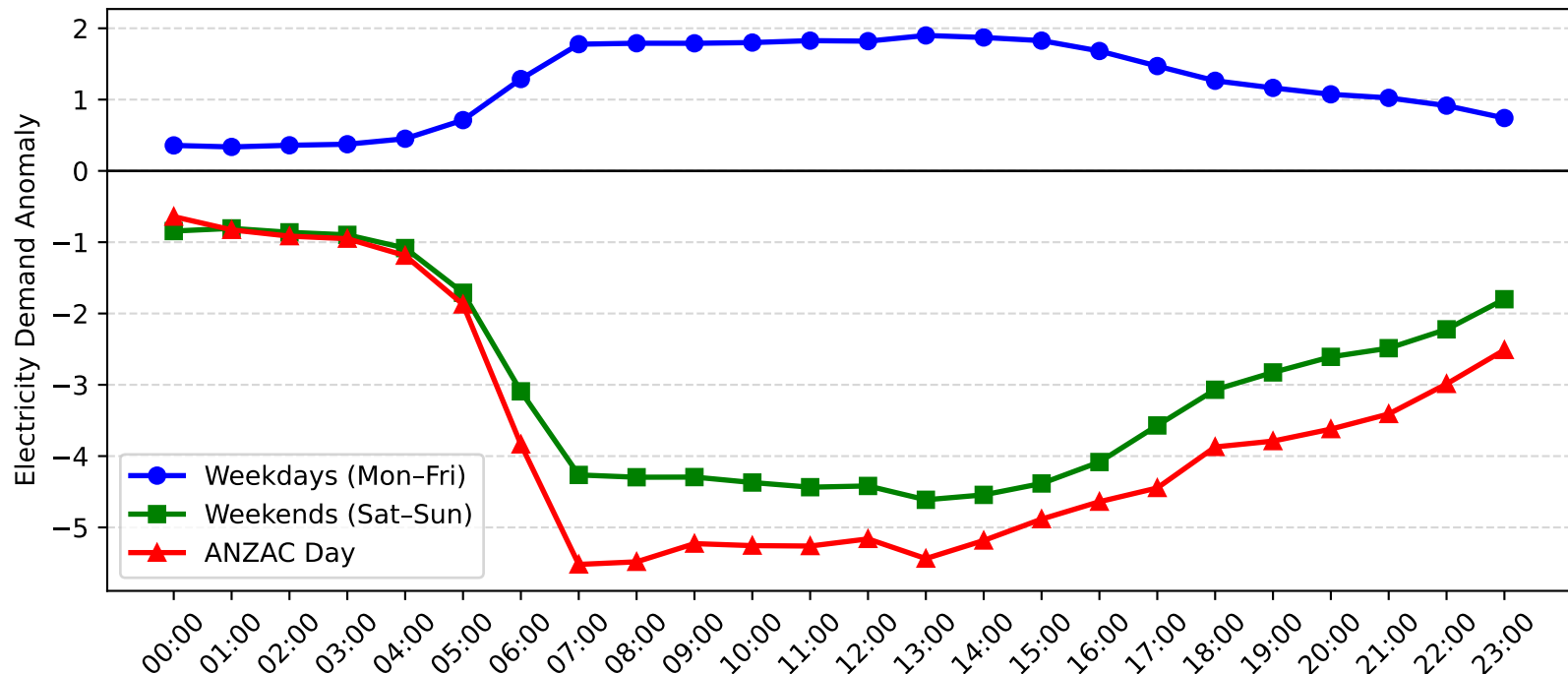
Leightonfield Demand Anomaly: ANZAC Day vs Weekday/Weekend (2014-2015)
