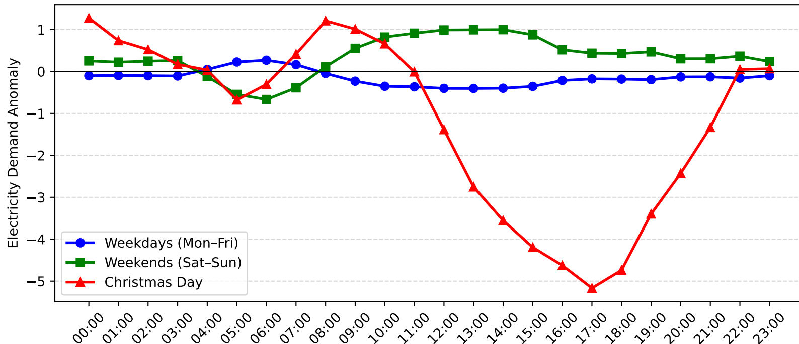
Umina Demand Anomaly: Christmas Day vs Weekday/Weekend (2006-2007)
