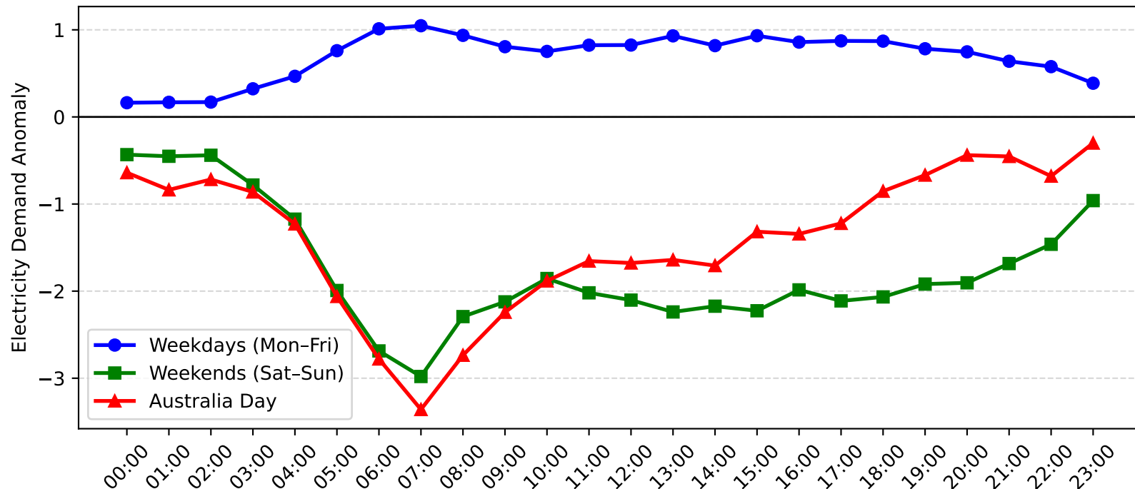
Lisarow Demand Anomaly: Australia Day vs Weekday/Weekend (2009-2010)
