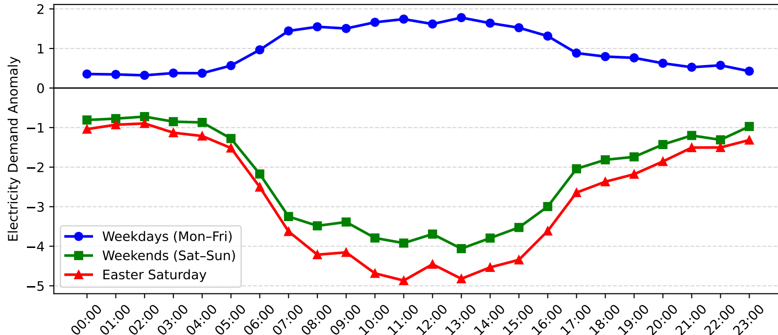
Mayfield West Demand Anomaly: Easter Saturday vs Weekday/Weekend (2016-2017)
