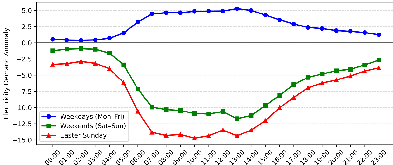
Milperra Demand Anomaly: Easter Sunday vs Weekday/Weekend (2008-2009)
