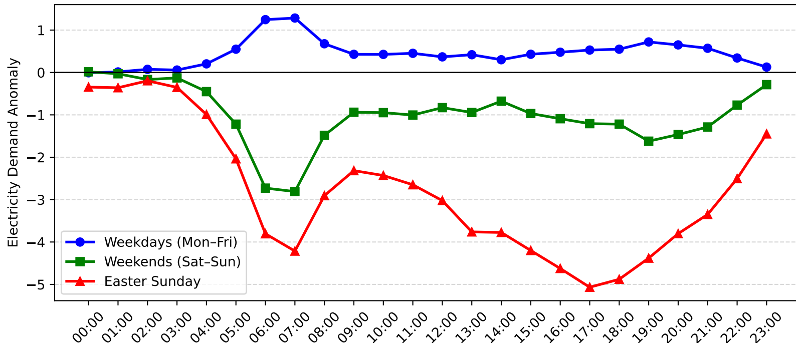
Revesby Demand Anomaly: Easter Sunday vs Weekday/Weekend (2016-2017)
