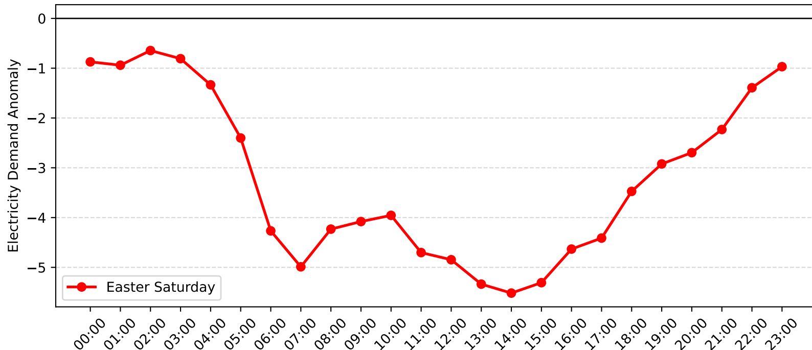
Kirrawee Demand Anomaly: Easter Saturday (2007-2008)
