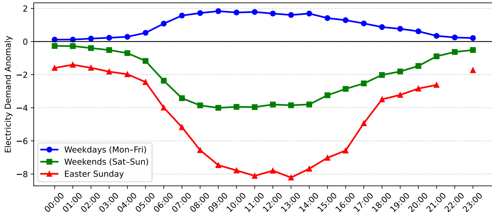
Auburn Demand Anomaly: Easter Sunday vs Weekday/Weekend (2010-2011)
