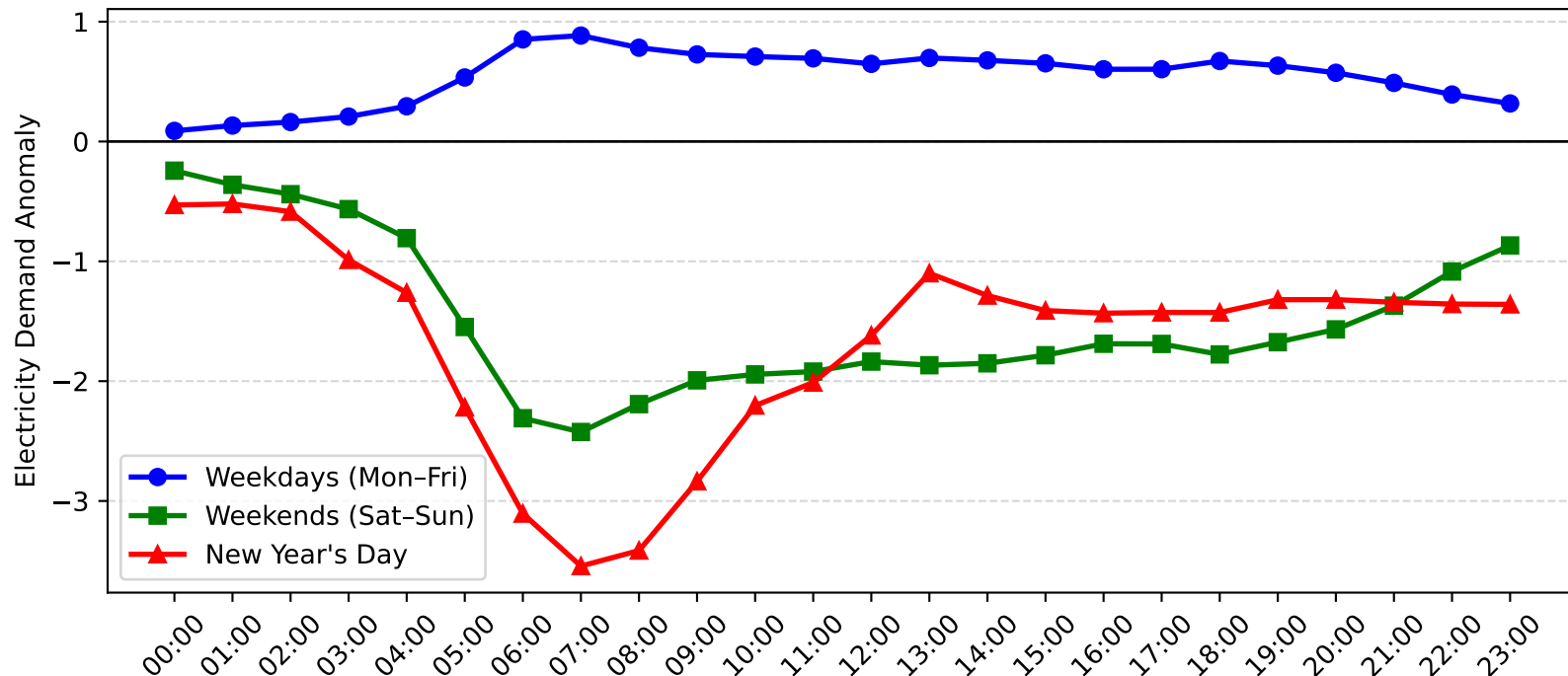
Lisarow Demand Anomaly: New Year's Day vs Weekday/Weekend (2013-2014)
