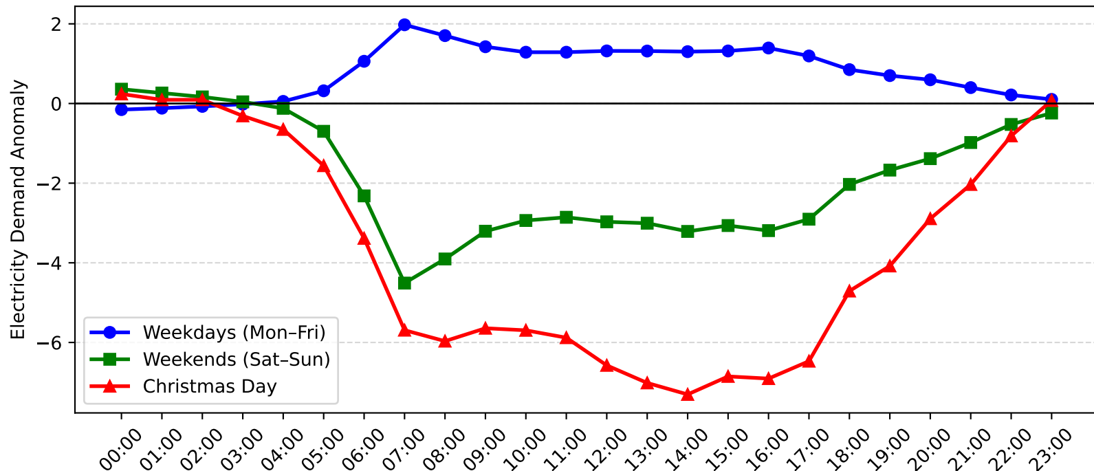
Chatswood Demand Anomaly: Christmas Day vs Weekday/Weekend (2010-2011)
