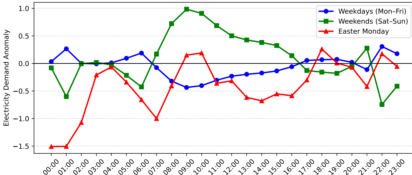
Swansea Demand Anomaly: Easter Monday vs Weekday/Weekend (2007-2008)
