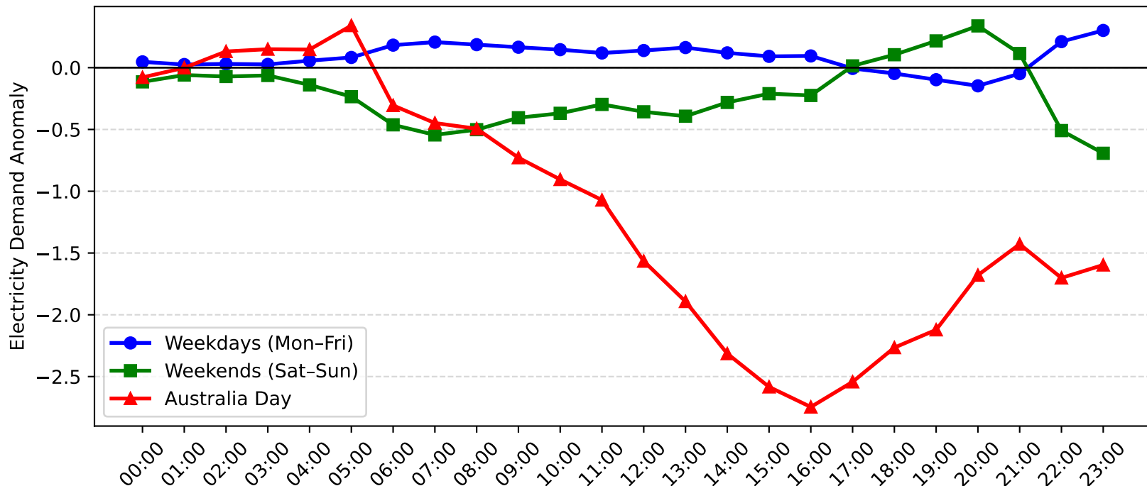
Muswellbrook Demand Anomaly: Australia Day vs Weekday/Weekend (2014-2015)
