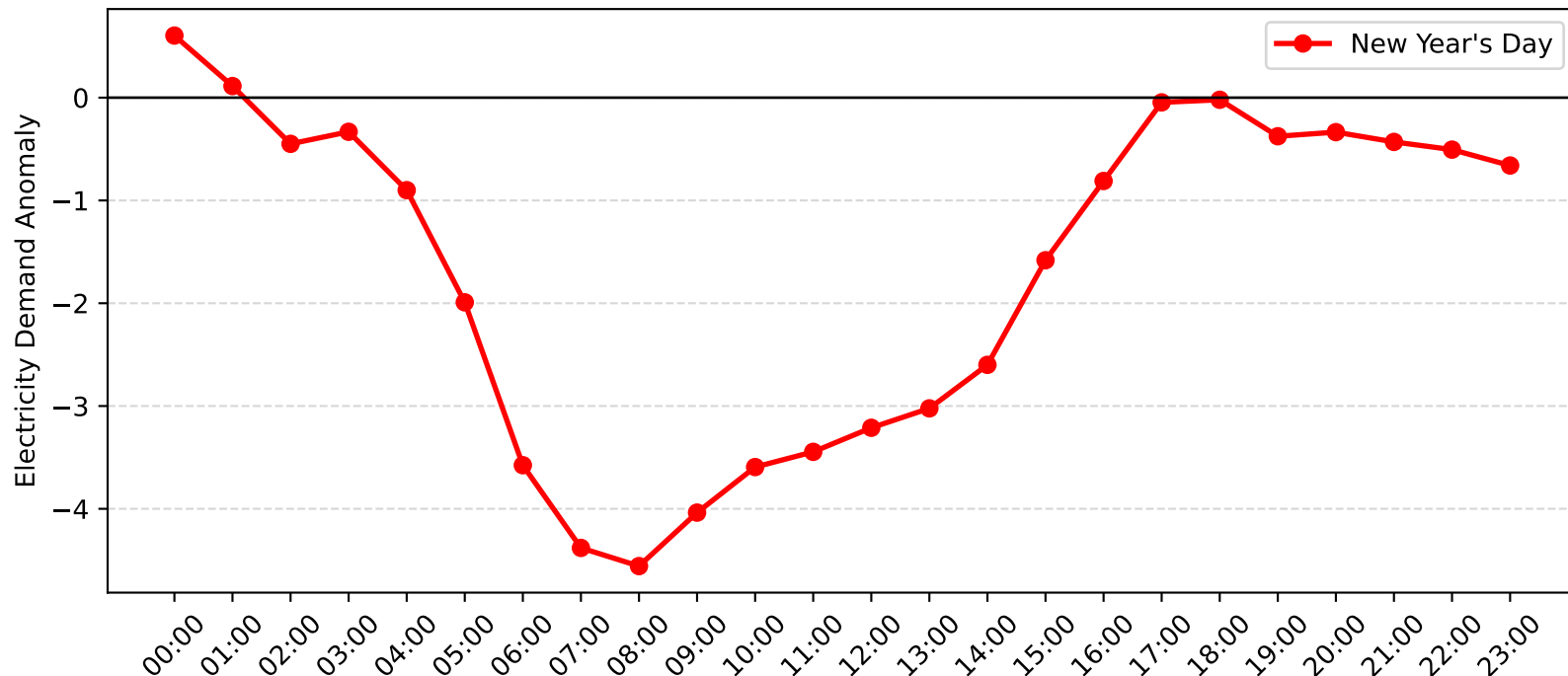
Wyong Demand Anomaly: New Year's Day (2012-2013)
