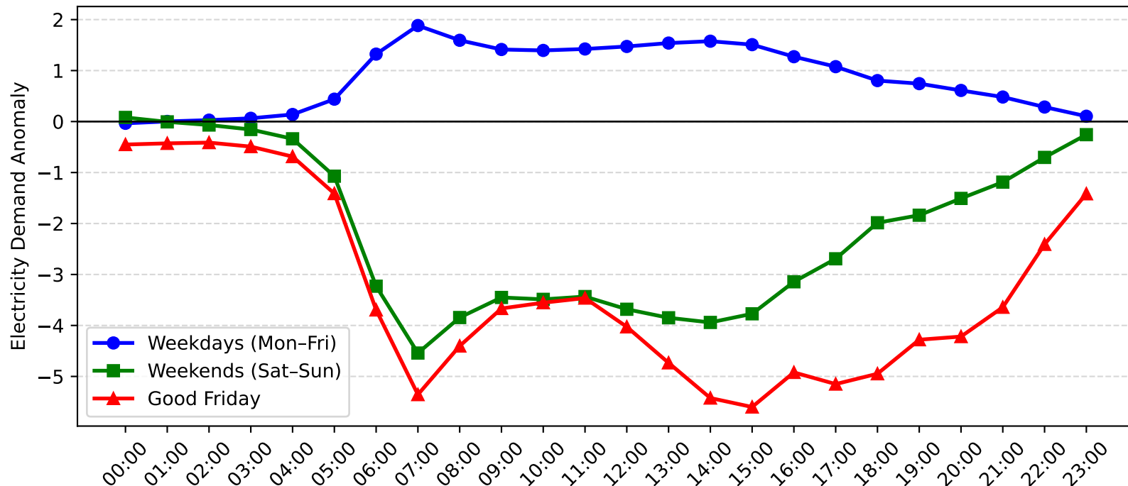
Hunters Hill Demand Anomaly: Good Friday vs Weekday/Weekend (2015-2016)
