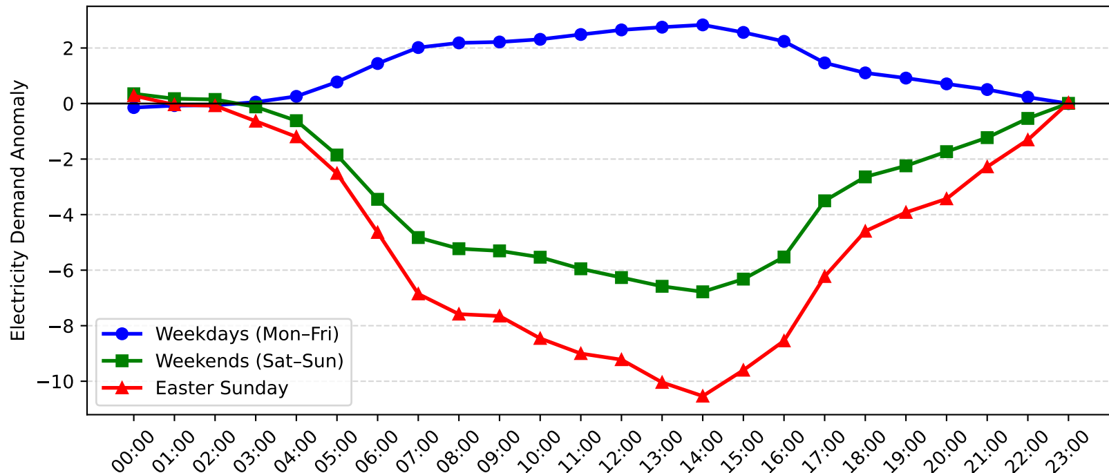
West Gosford Demand Anomaly: Easter Sunday vs Weekday/Weekend (2007-2008)
