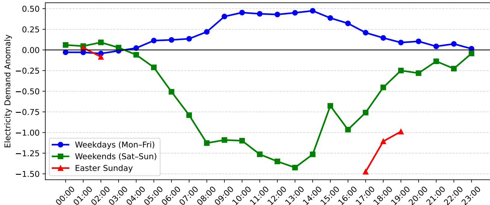
Broadmeadow Demand Anomaly: Easter Sunday vs Weekday/Weekend (2013-2014)
