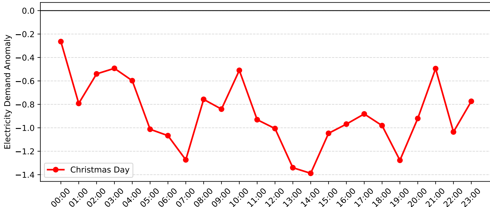
Cardiff Demand Anomaly: Christmas Day (2010-2011)
