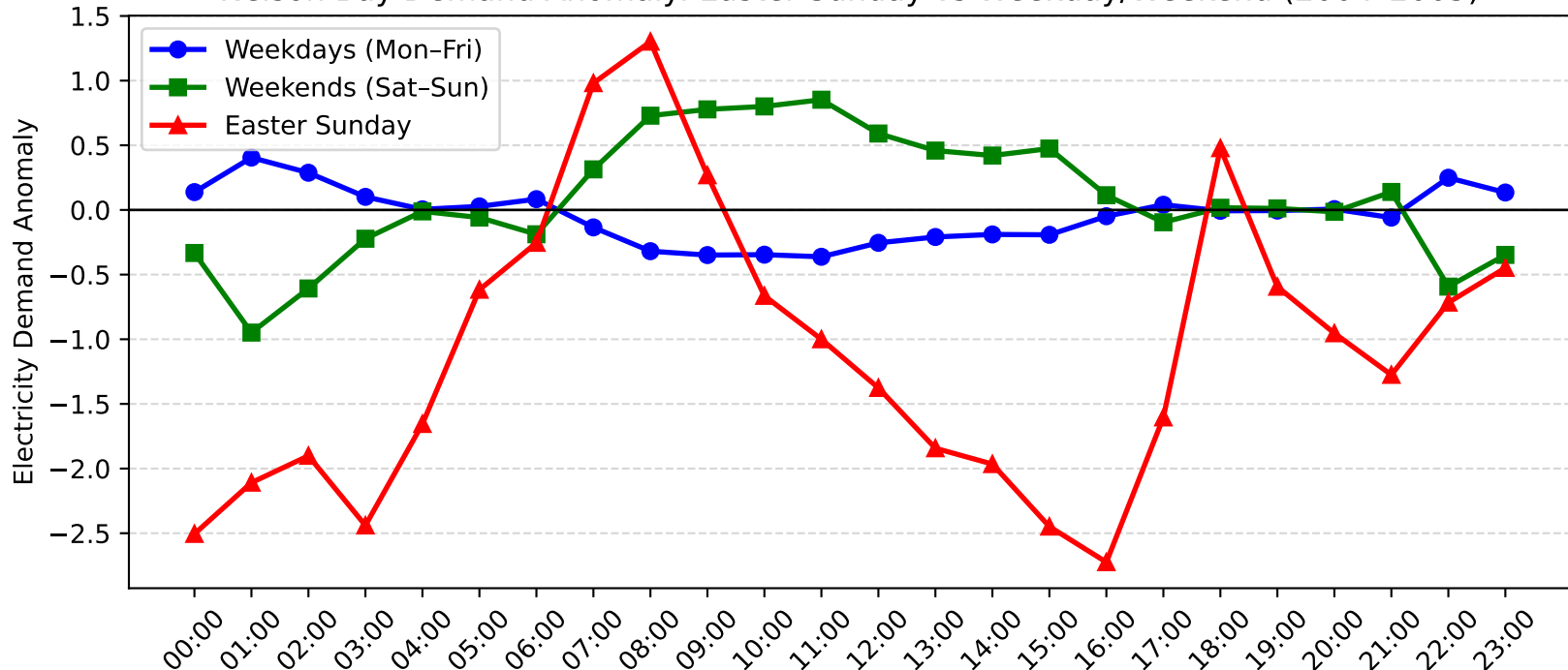
Nelson Bay Demand Anomaly: Easter Sunday vs Weekday/Weekend (2004-2005)
