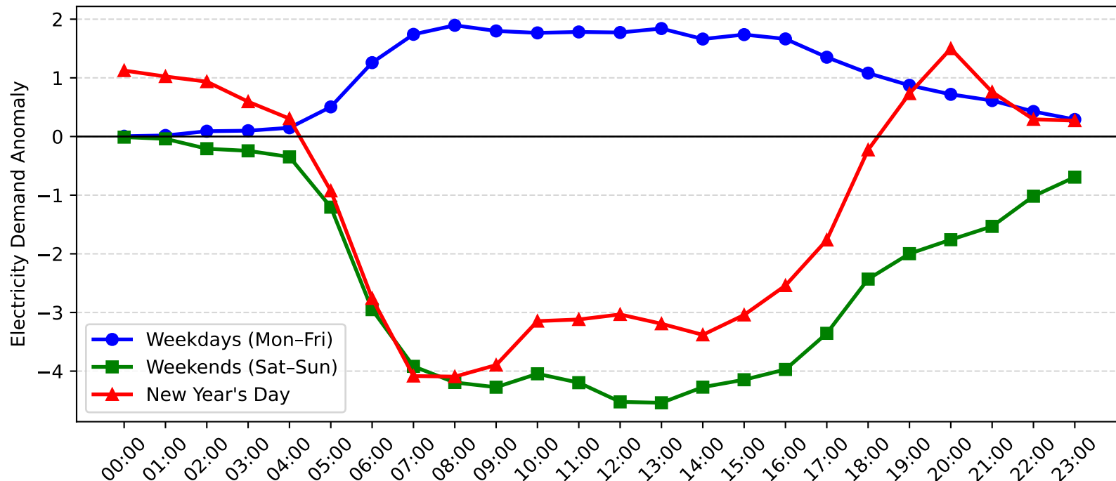
Concord Demand Anomaly: New Year's Day vs Weekday/Weekend (2006-2007)
