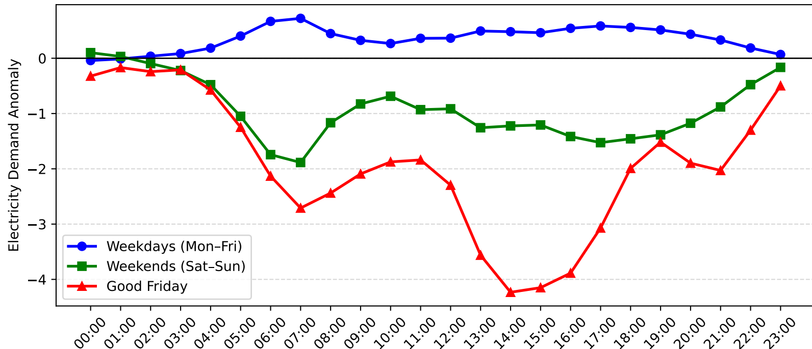
Charmhaven Demand Anomaly: Good Friday vs Weekday/Weekend (2007-2008)
