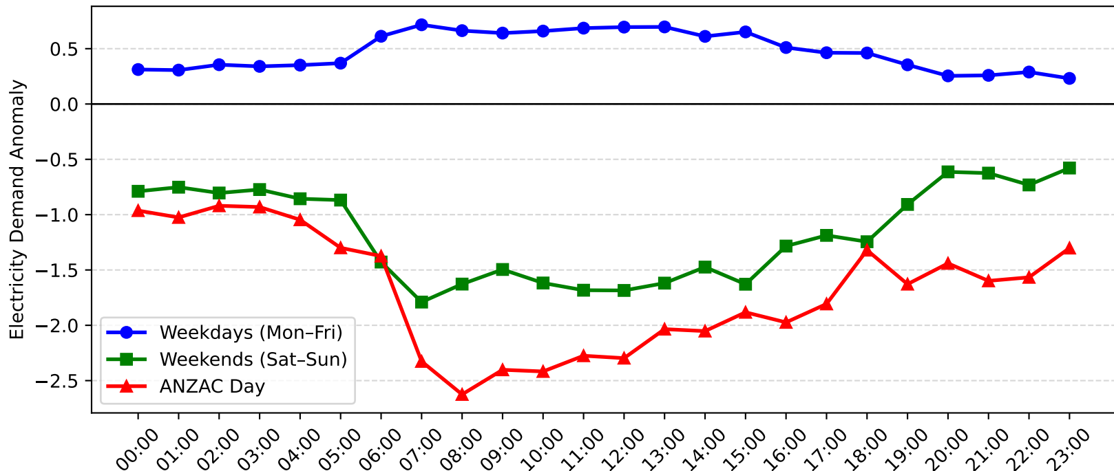
Leightonfield Demand Anomaly: ANZAC Day vs Weekday/Weekend (2004-2005)
