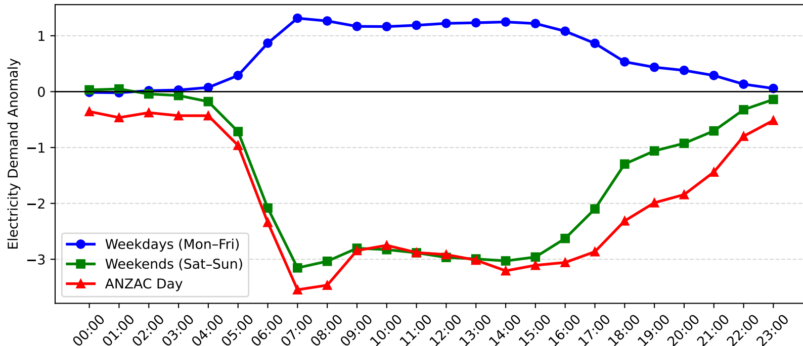
Beacon Hill Demand Anomaly: ANZAC Day vs Weekday/Weekend (2014-2015)
