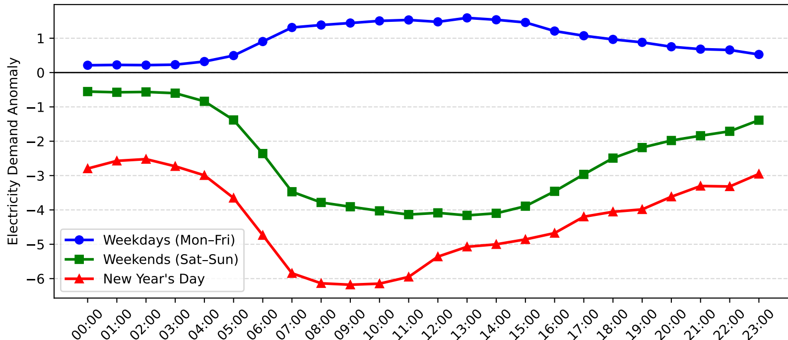
Leightonfield Demand Anomaly: New Year's Day vs Weekday/Weekend (2013-2014)
