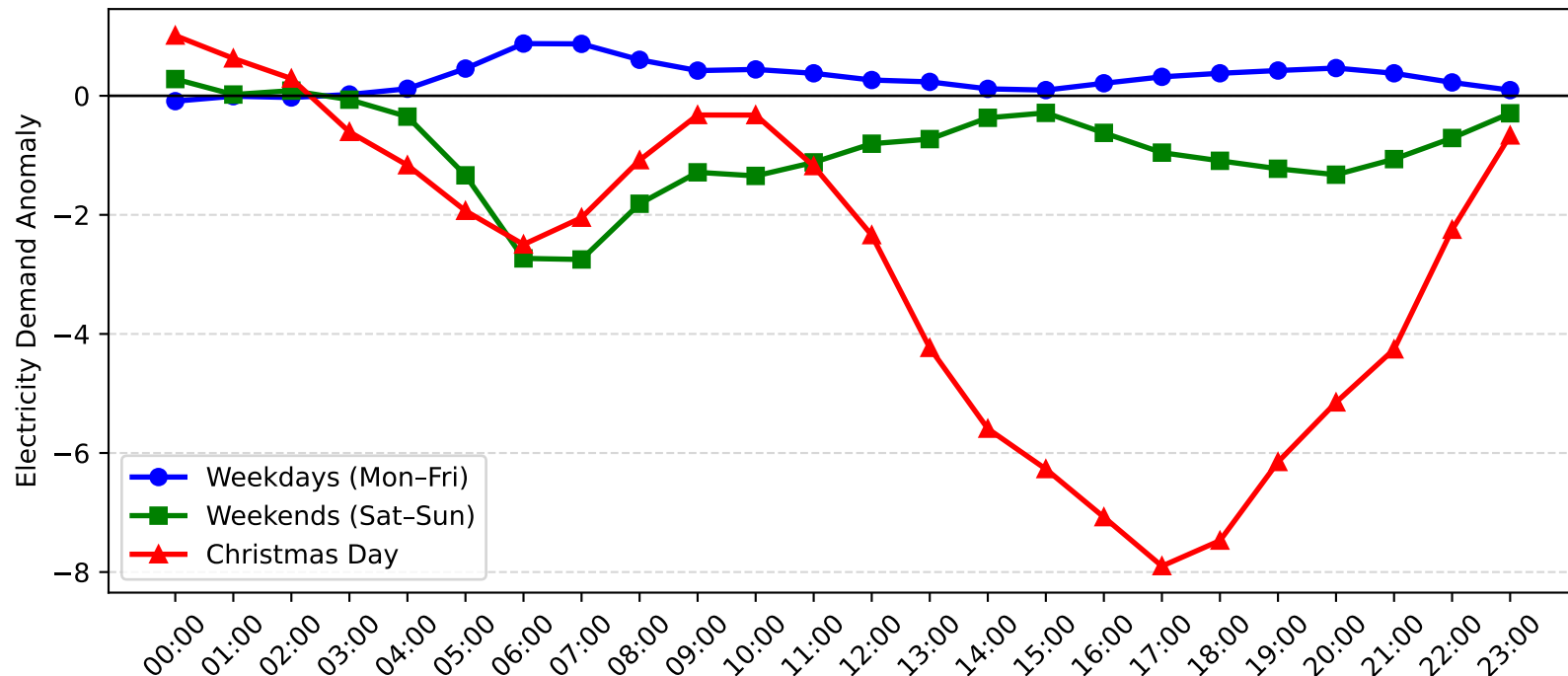
Revesby Demand Anomaly: Christmas Day vs Weekday/Weekend (2013-2014)
