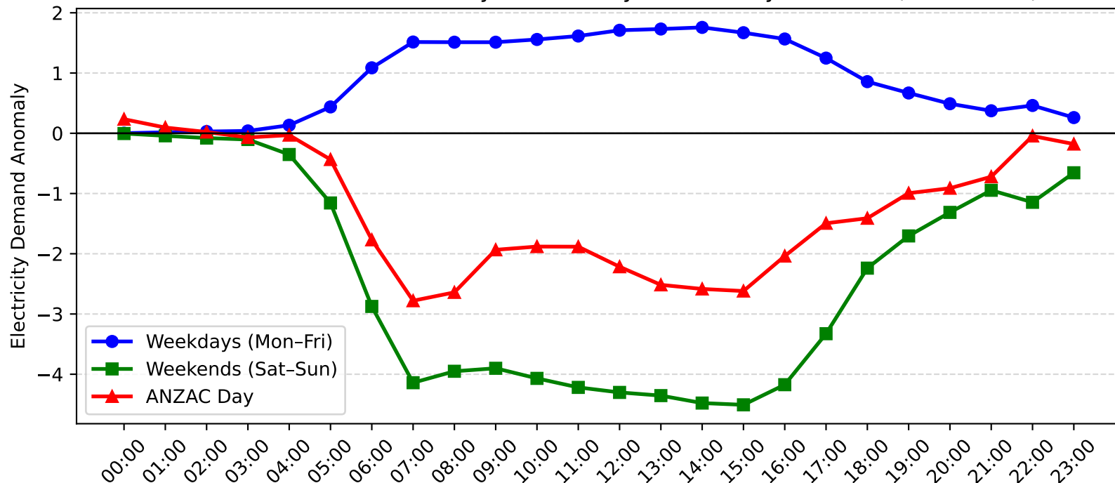
Beacon Hill Demand Anomaly: ANZAC Day vs Weekday/Weekend (2007-2008)
