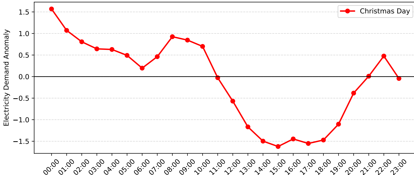
Telarah Demand Anomaly: Christmas Day (2014-2015)
