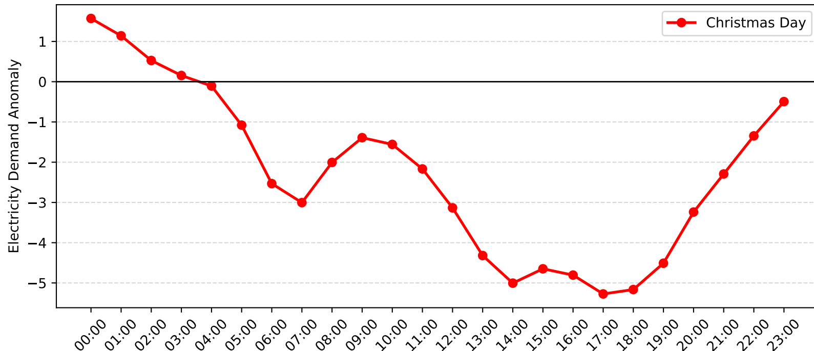
Mortdale Demand Anomaly: Christmas Day (2005-2006)
