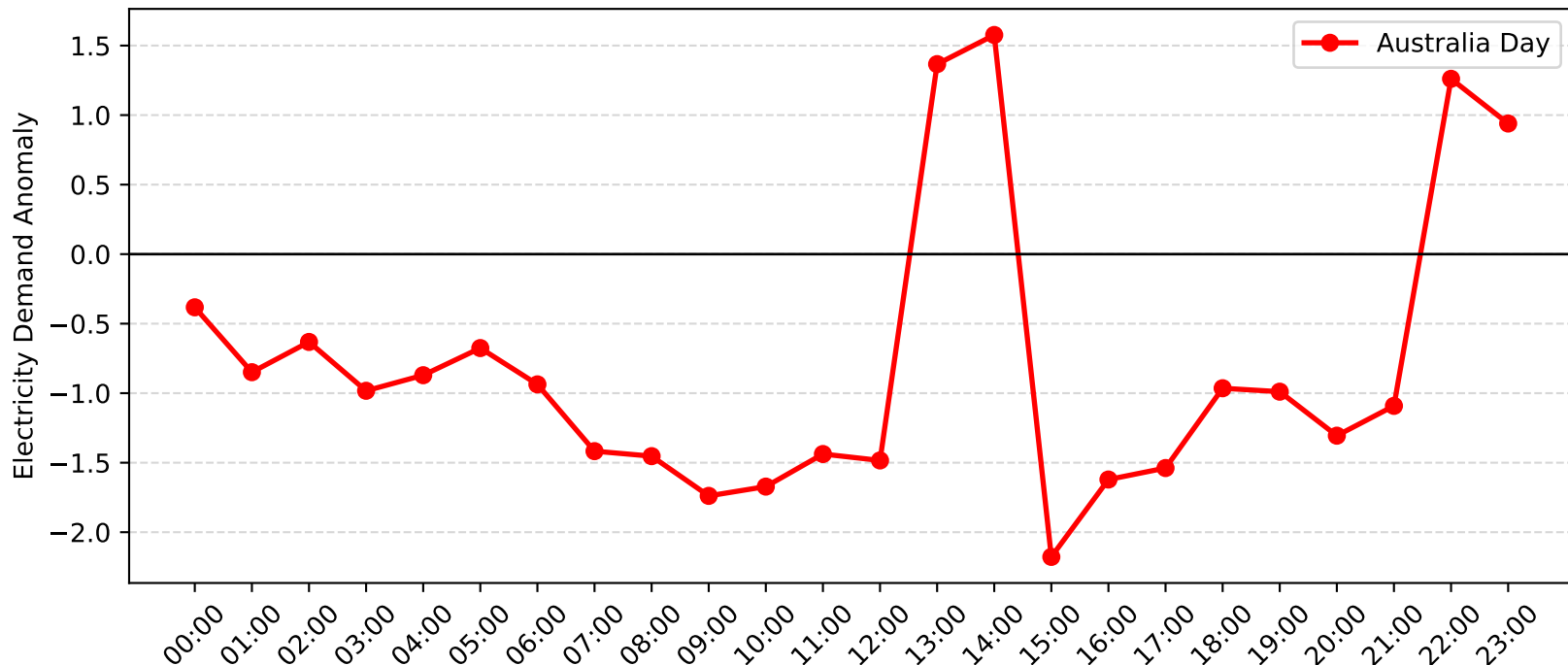
Green Square Demand Anomaly: Australia Day (2007-2008)
