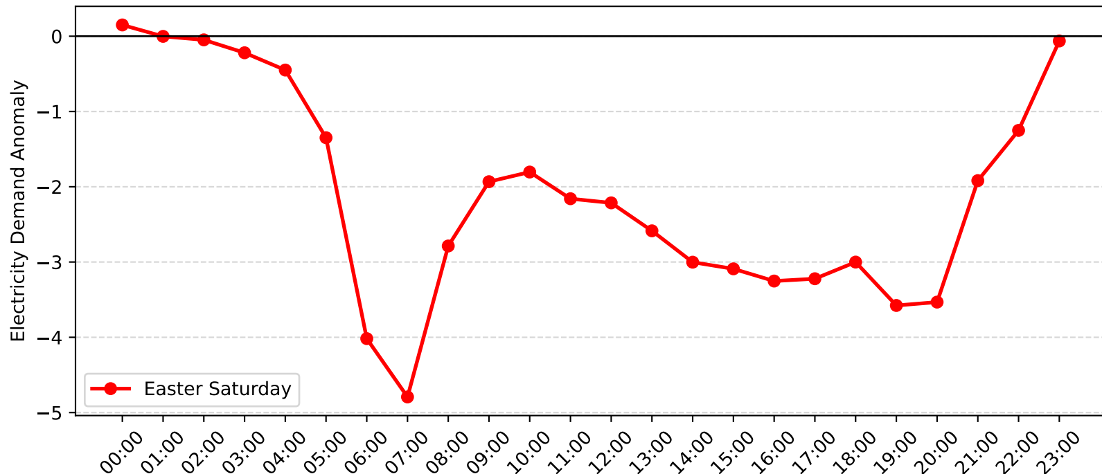
Mortdale Demand Anomaly: Easter Saturday (2008-2009)
