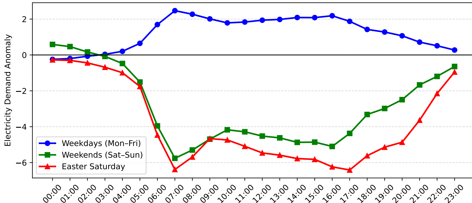
Burwood Demand Anomaly: Easter Saturday vs Weekday/Weekend (2012-2013)
