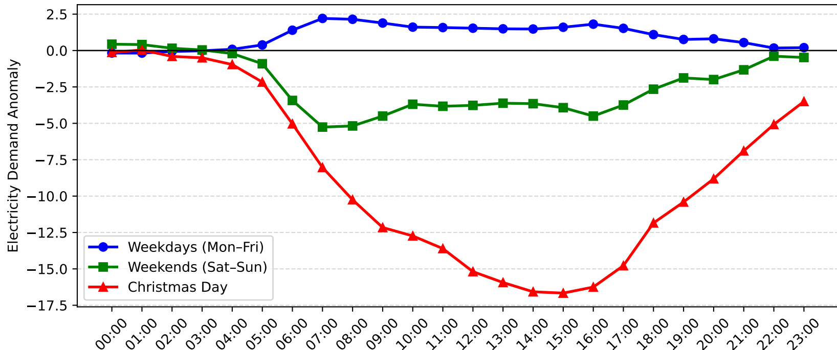
Burwood Demand Anomaly: Christmas Day vs Weekday/Weekend (2006-2007)
