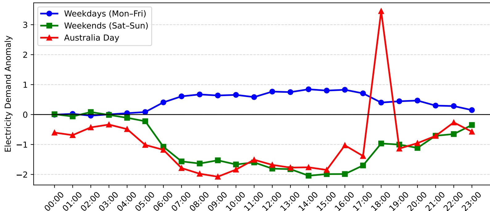
Punchbowl Demand Anomaly: Australia Day vs Weekday/Weekend (2004-2005)
