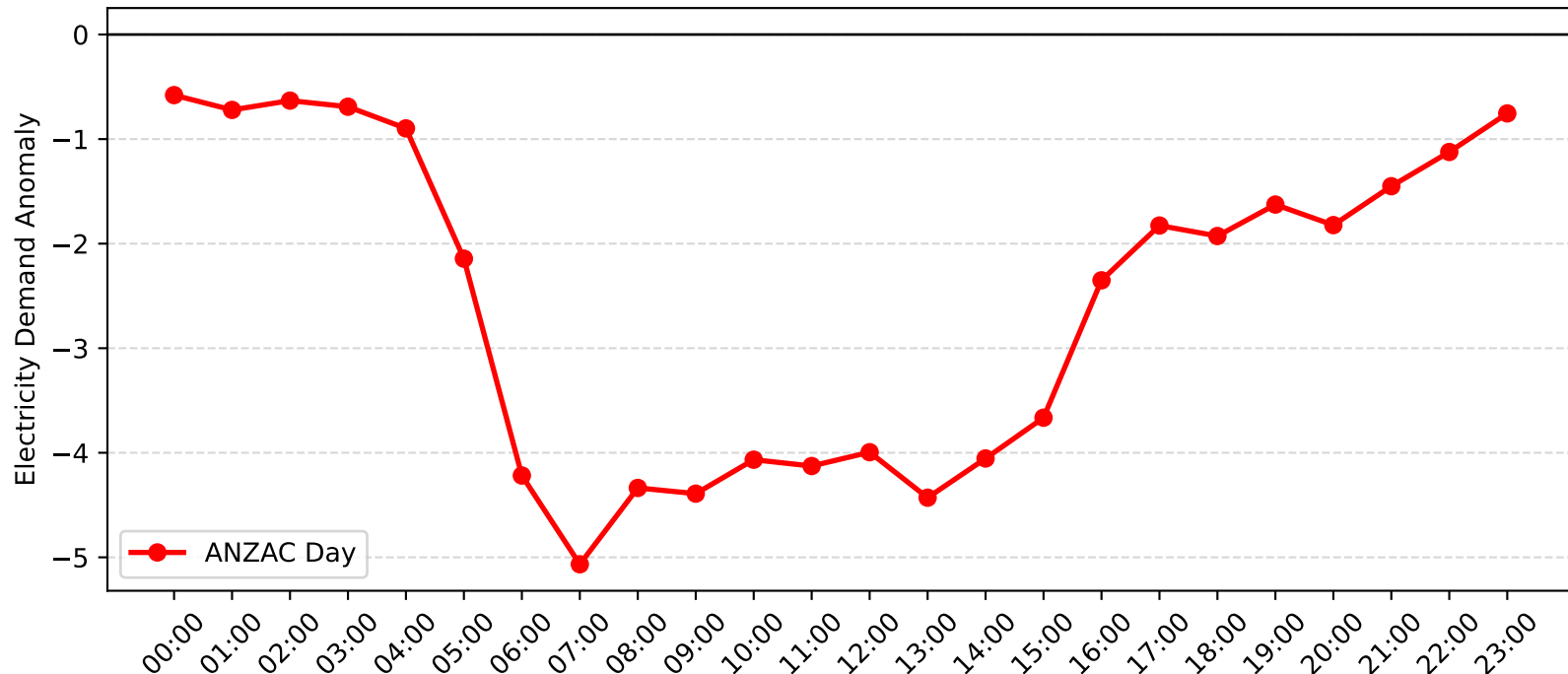
Wyong Demand Anomaly: ANZAC Day (2011-2012)
