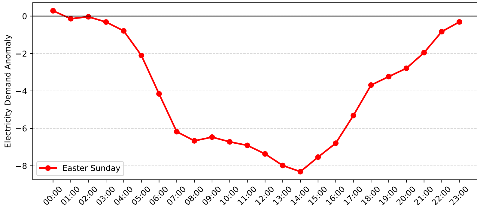
West Gosford Demand Anomaly: Easter Sunday (2008-2009)
