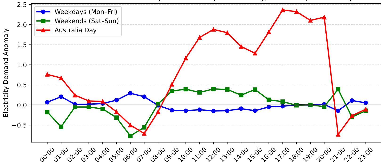
Morisset Demand Anomaly: Australia Day vs Weekday/Weekend (2011-2012)
