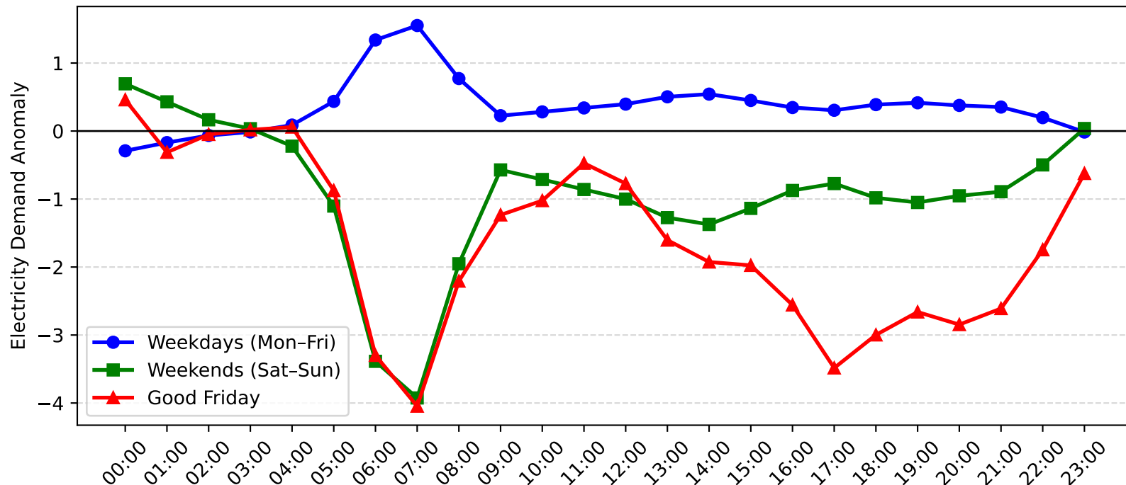
Mortdale Demand Anomaly: Good Friday vs Weekday/Weekend (2012-2013)
