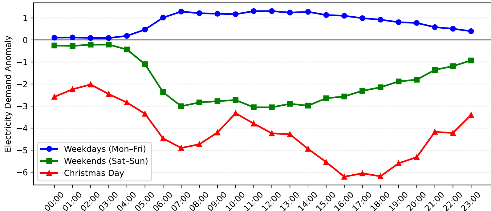
Matraverse Demand Anomaly: Christmas Day vs Weekday/Weekend (2016-2017)
