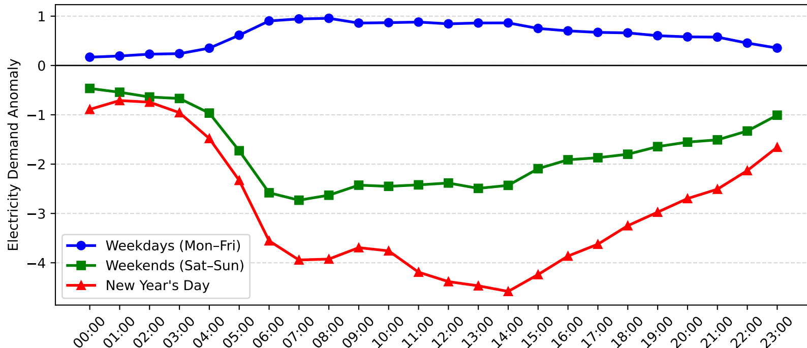
Lisarow Demand Anomaly: New Year's Day vs Weekday/Weekend (2015-2016)
