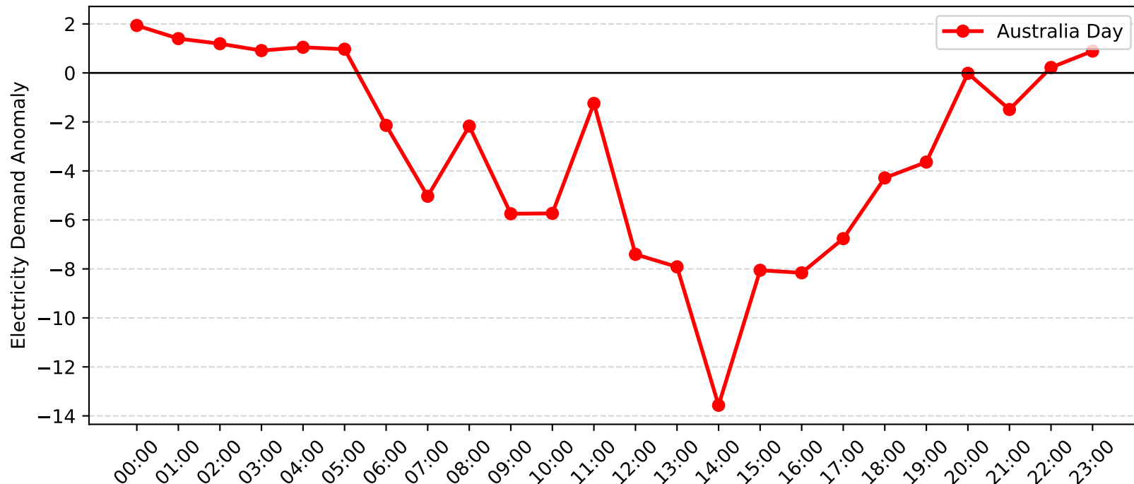
Castle Cove Demand Anomaly: Australia Day (2013-2014)
