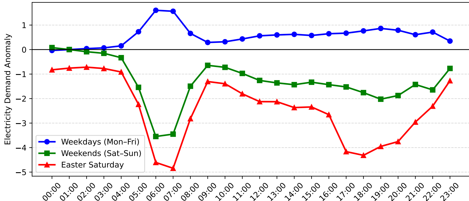
Dee Why West Demand Anomaly: Easter Saturday vs Weekday/Weekend (2010-2011)
