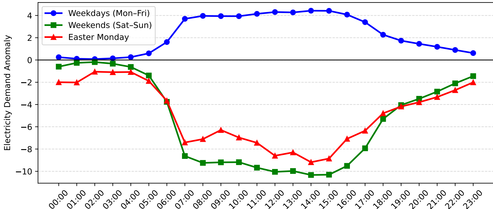
Gore Hill Demand Anomaly: Easter Monday vs Weekday/Weekend (2014-2015)
