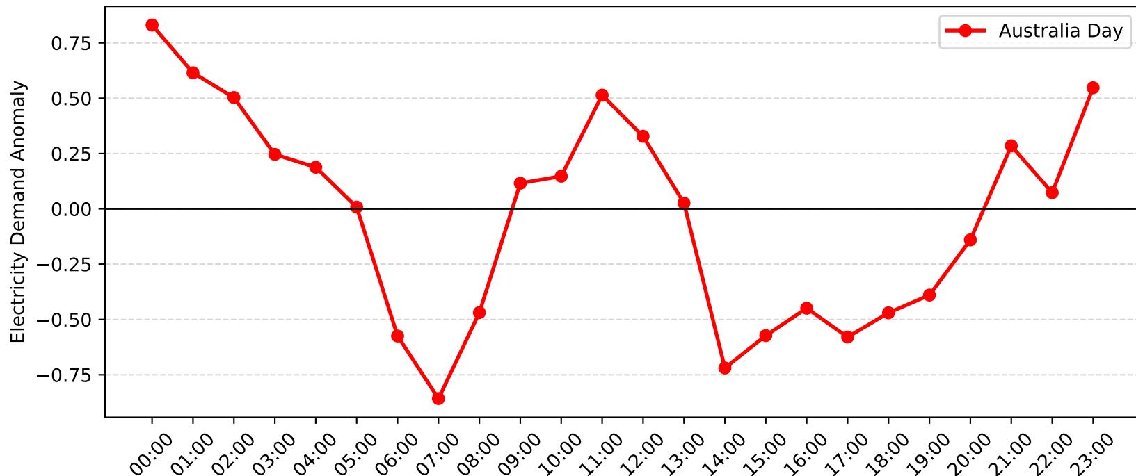
Adamstown Demand Anomaly: Australia Day (2012-2013)
