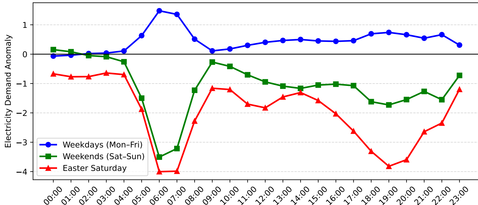
Dee Why West Demand Anomaly: Easter Saturday vs Weekday/Weekend (2011-2012)
