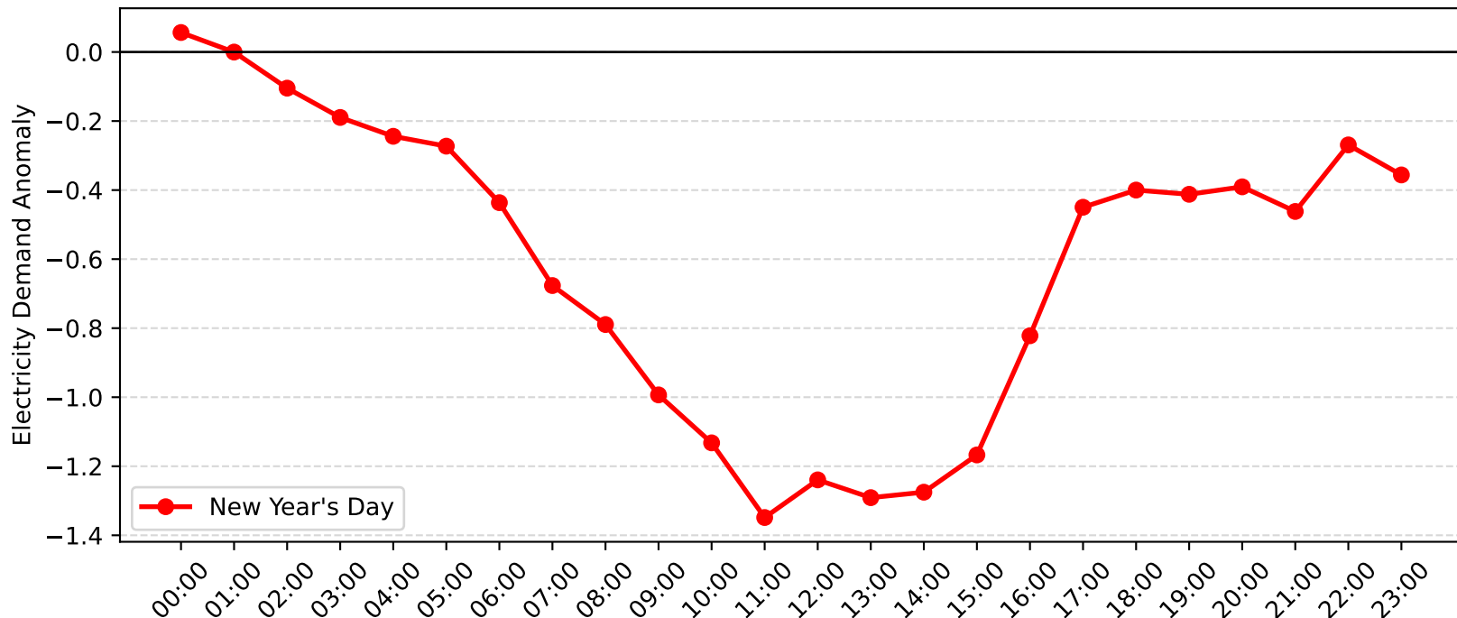
Rothbury Demand Anomaly: New Year's Day (2015-2016)
