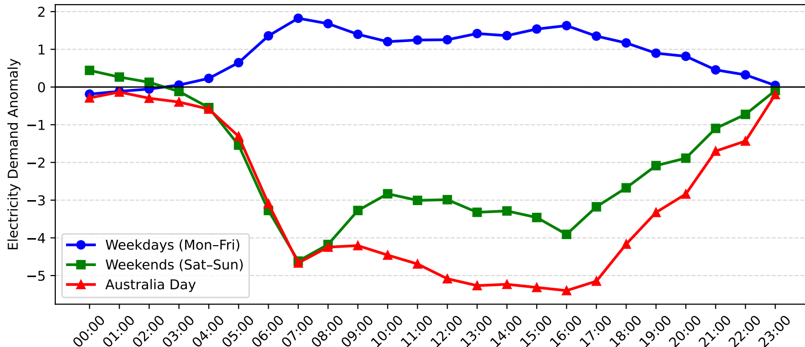
Punchbowl Demand Anomaly: Australia Day vs Weekday/Weekend (2008-2009)
