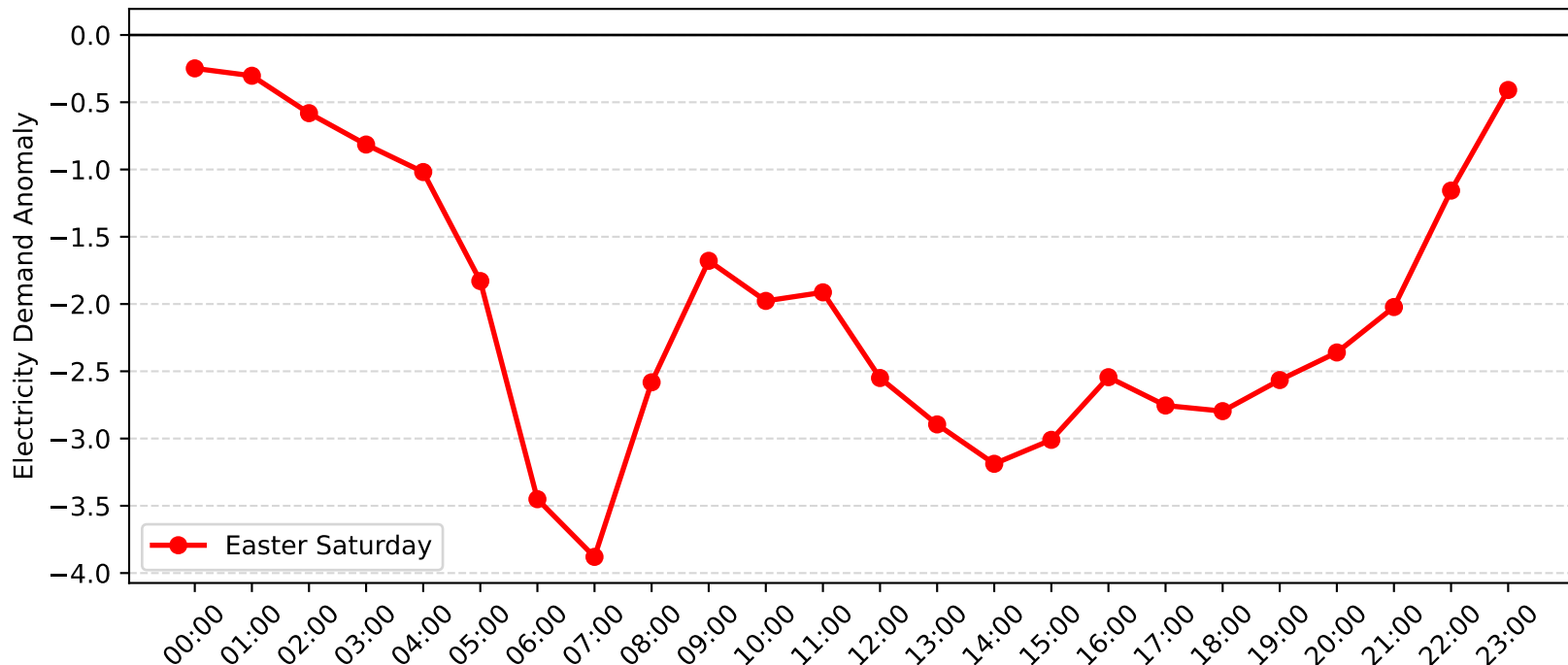
Mortdale Demand Anomaly: Easter Saturday (2016-2017)
