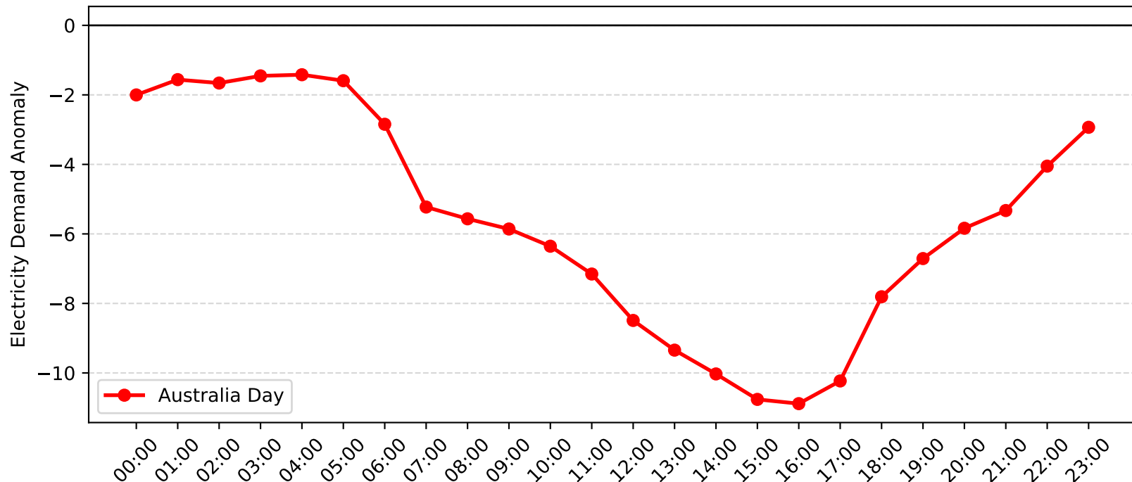
Epping Demand Anomaly: Australia Day (2017-2018)
