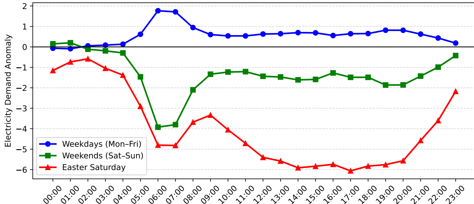
Pennant Hills Demand Anomaly: Easter Saturday vs Weekday/Weekend (2016-2017)
