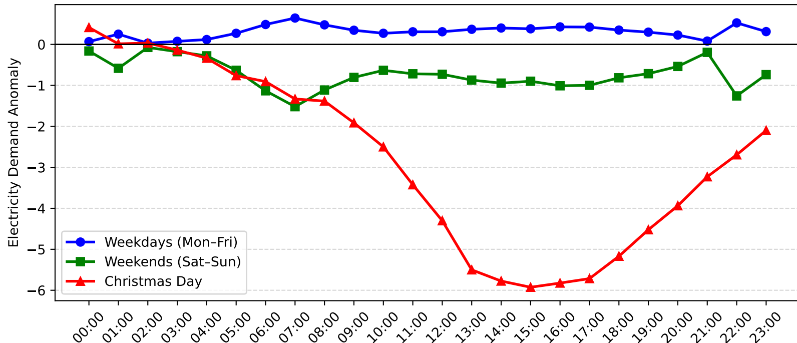
Jesmond Demand Anomaly: Christmas Day vs Weekday/Weekend (2011-2012)
