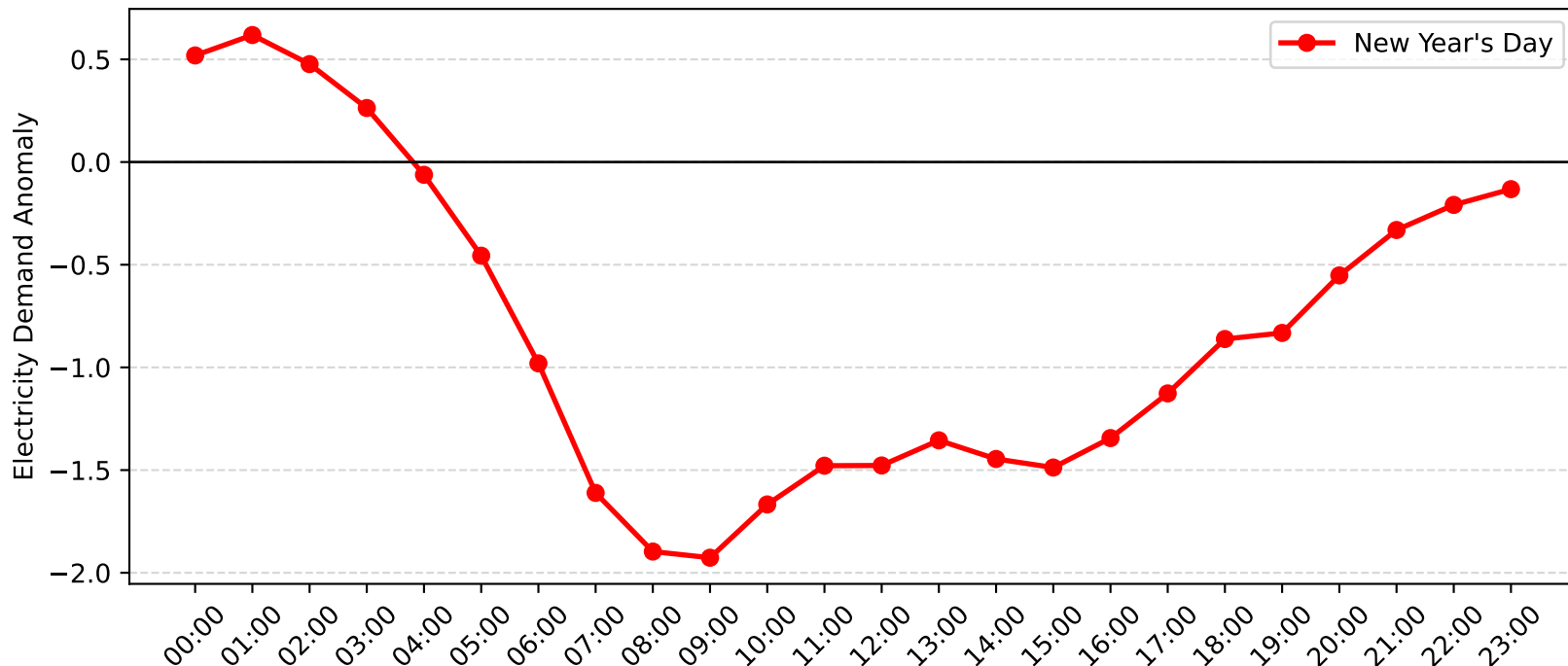
Rockdale Demand Anomaly: New Year's Day (2013-2014)
