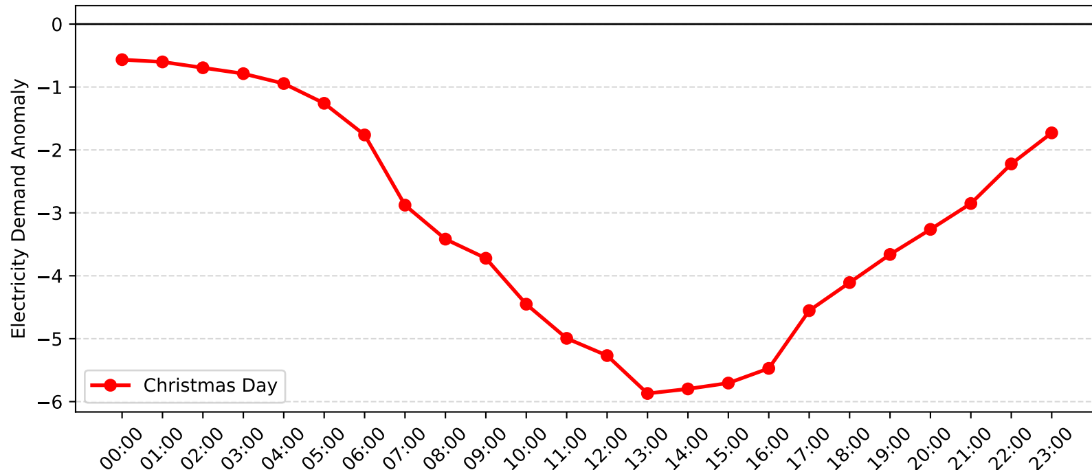
Mayfield West Demand Anomaly: Christmas Day (2012-2013)
