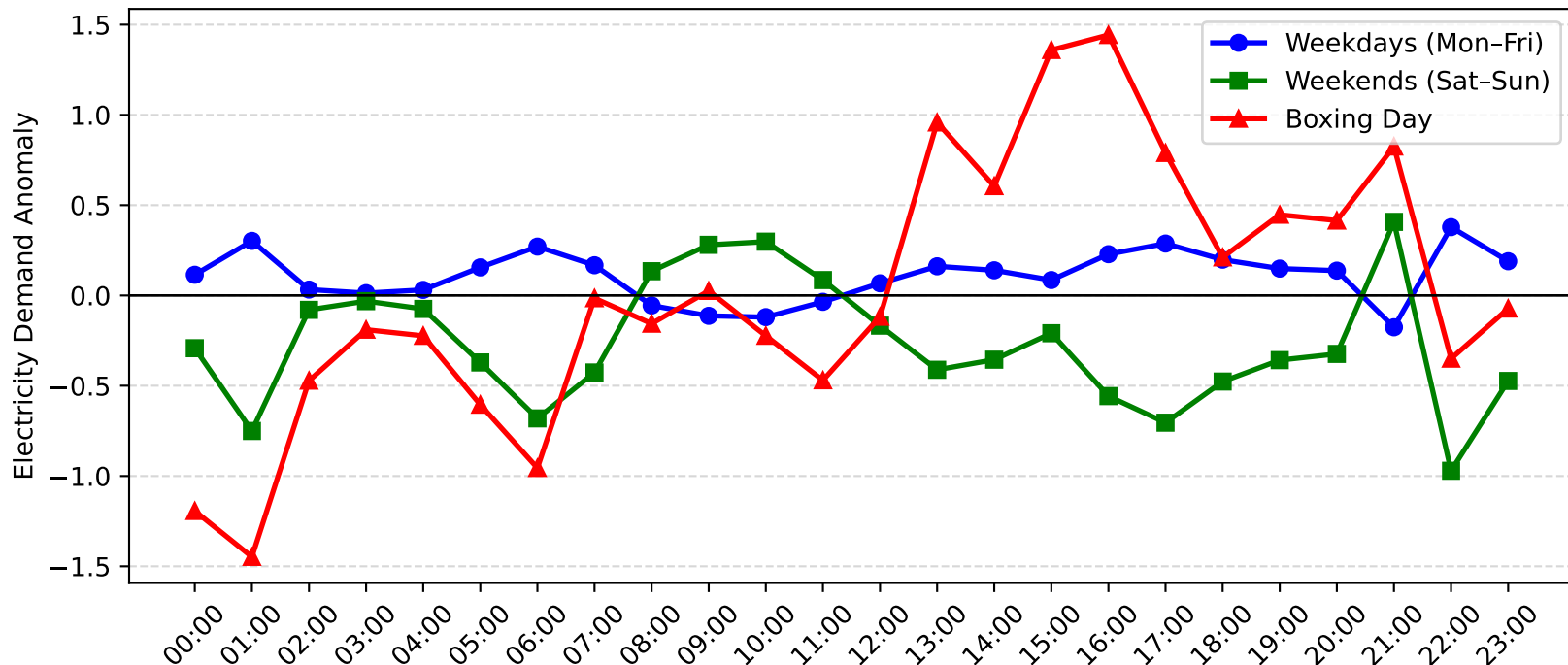
Nelson Bay Demand Anomaly: Boxing Day vs Weekday/Weekend (2014-2015)
