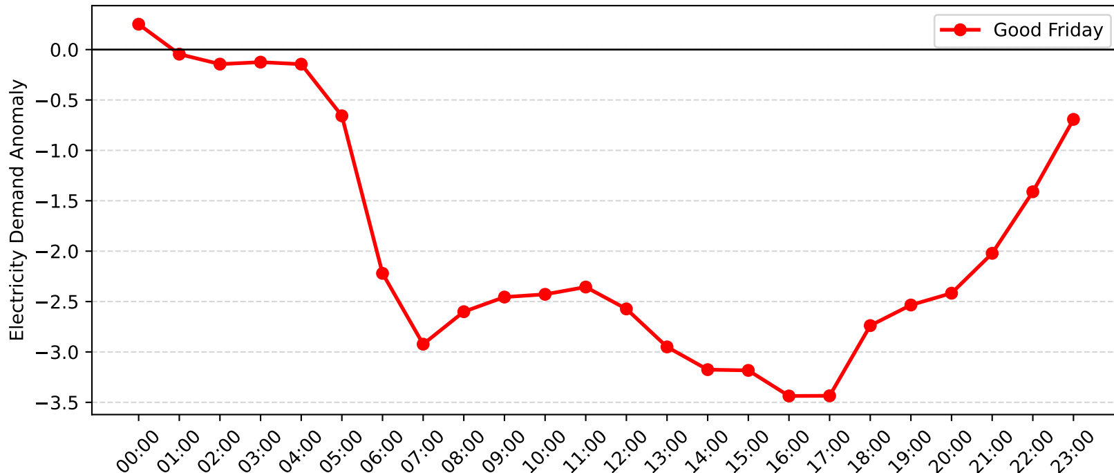
Pymble Demand Anomaly: Good Friday (2013-2014)
