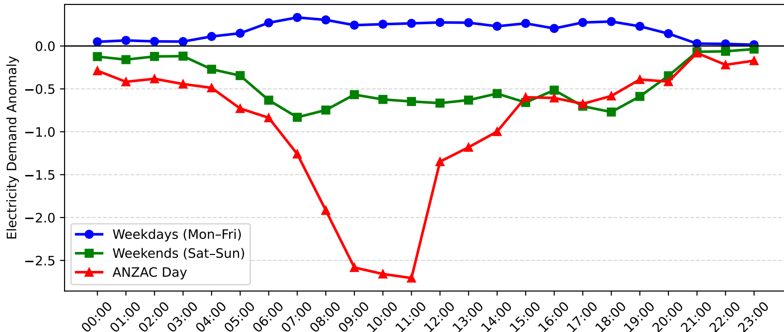
Auburn Demand Anomaly: ANZAC Day vs Weekday/Weekend (2004-2005)
