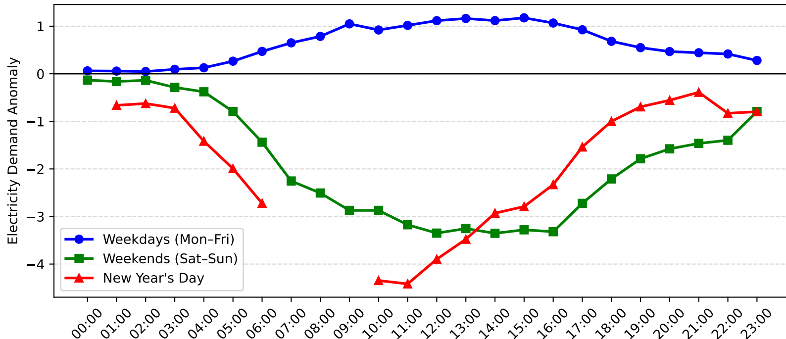
Lidcombe Demand Anomaly: New Year's Day vs Weekday/Weekend (2009-2010)
