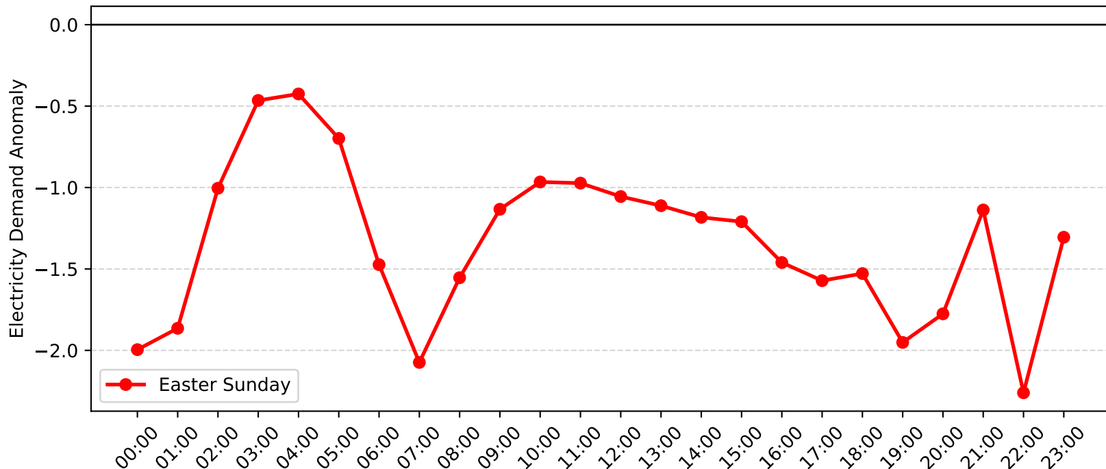
Adamstown Demand Anomaly: Easter Sunday (2011-2012)
