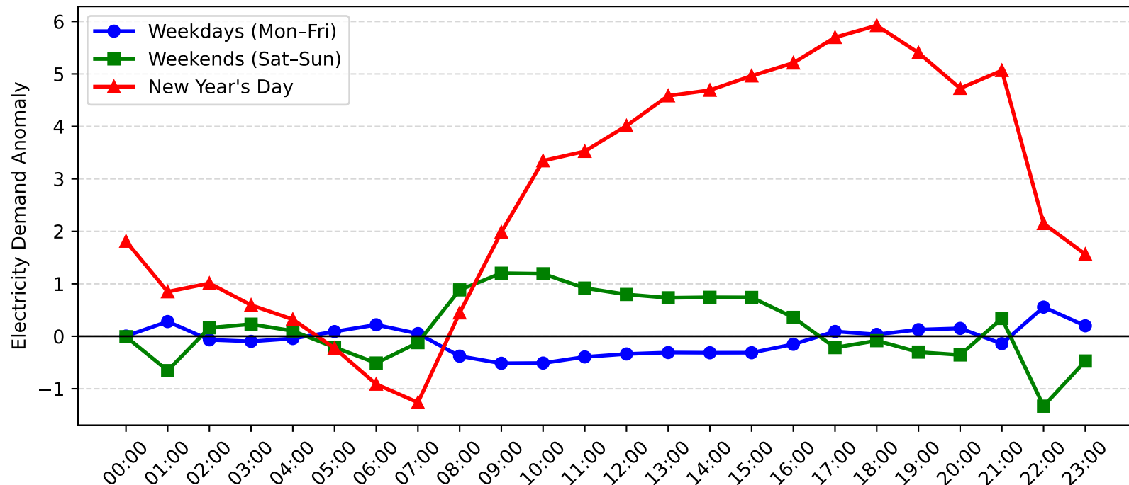
Nelson Bay Demand Anomaly: New Year's Day vs Weekday/Weekend (2012-2013)
