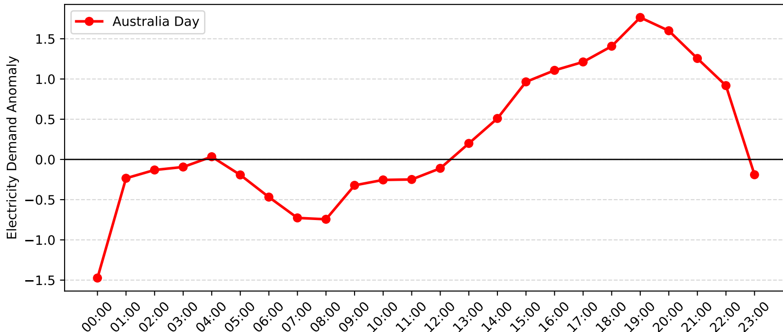
Telarah Demand Anomaly: Australia Day (2009-2010)
