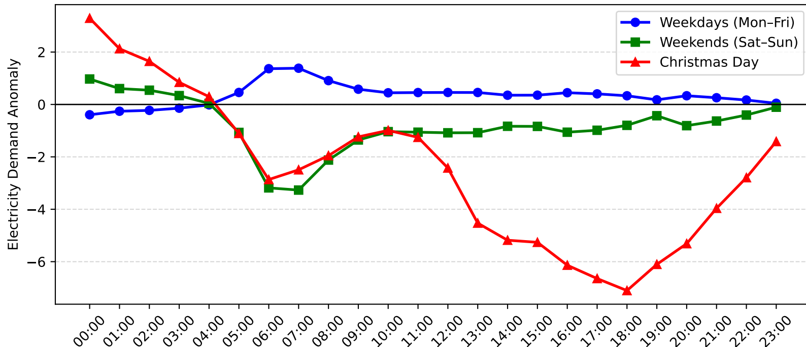
Pennant Hills Demand Anomaly: Christmas Day vs Weekday/Weekend (2011-2012)
