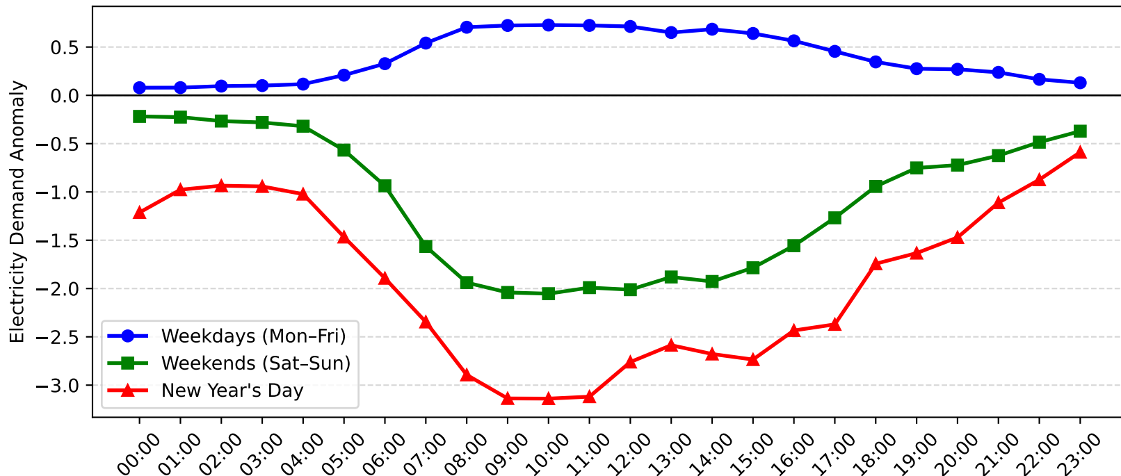
Lidcombe Demand Anomaly: New Year's Day vs Weekday/Weekend (2015-2016)
