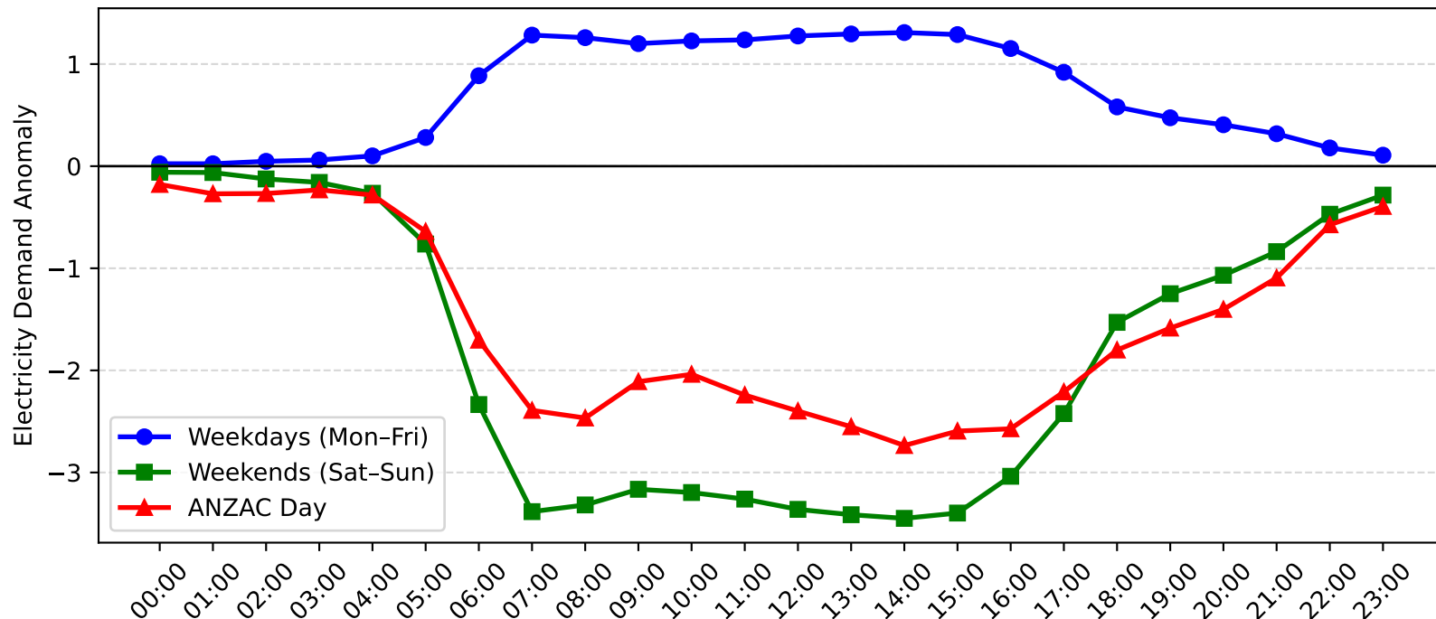
Beacon Hill Demand Anomaly: ANZAC Day vs Weekday/Weekend (2013-2014)
