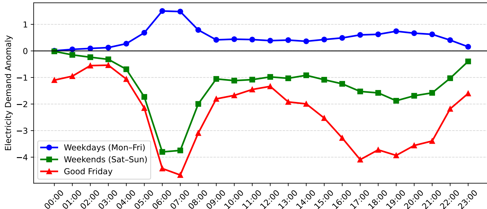
Revesby Demand Anomaly: Good Friday vs Weekday/Weekend (2014-2015)
