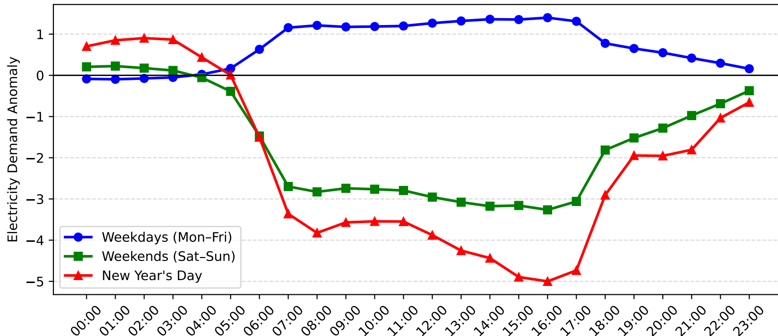
Pymble Demand Anomaly: New Year's Day vs Weekday/Weekend (2017-2018)
