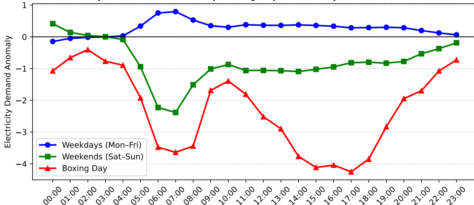
Dee Why West Demand Anomaly: Boxing Day vs Weekday/Weekend (2013-2014)
