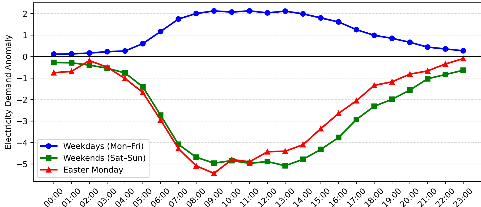
Auburn Demand Anomaly: Easter Monday vs Weekday/Weekend (2012-2013)
