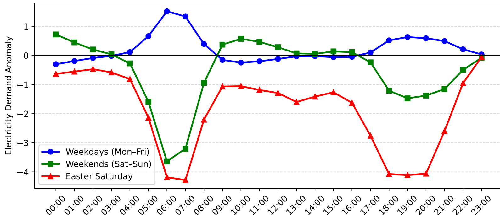
Cronulla Demand Anomaly: Easter Saturday vs Weekday/Weekend (2012-2013)
