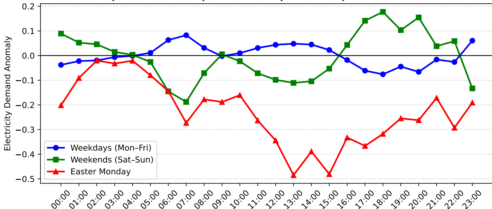
Rothbury Demand Anomaly: Easter Monday vs Weekday/Weekend (2008-2009)
