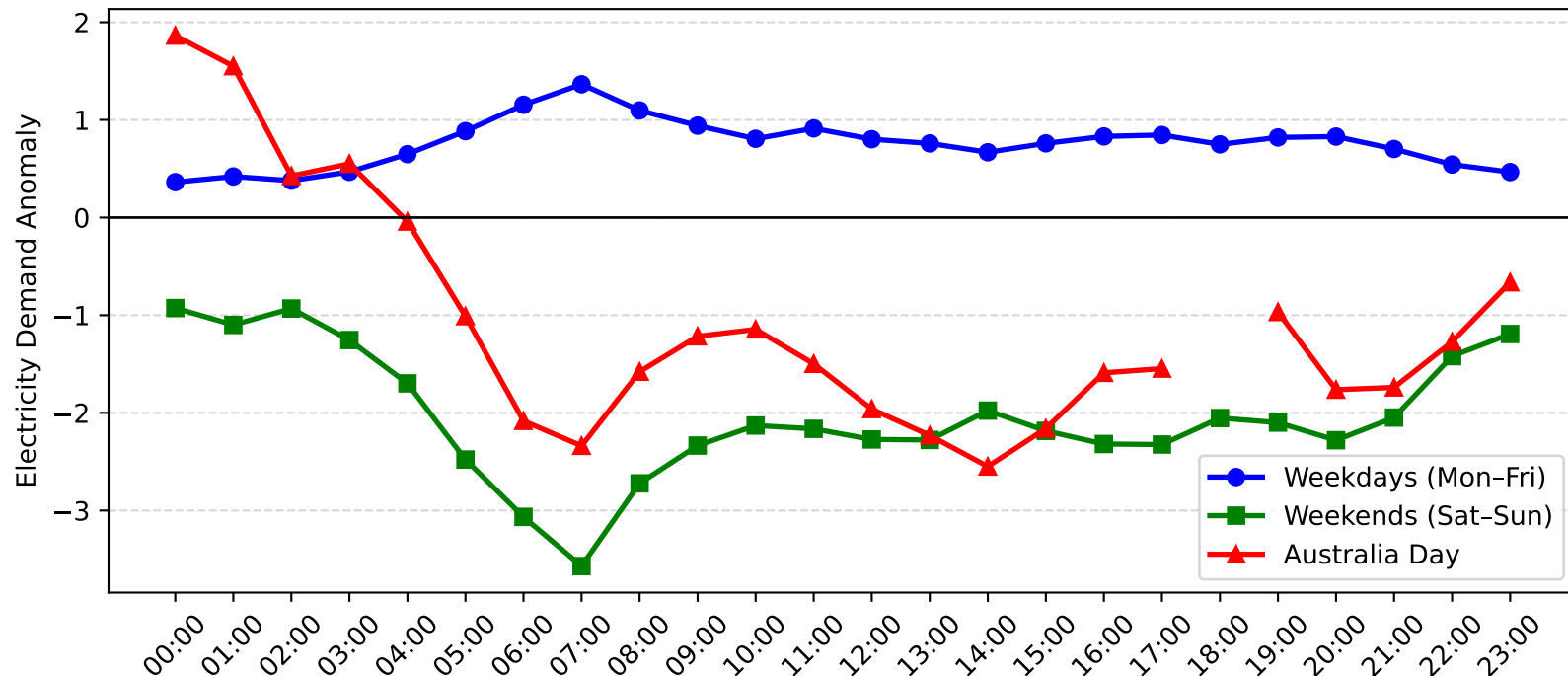
Lisarow Demand Anomaly: Australia Day vs Weekday/Weekend (2005-2006)
