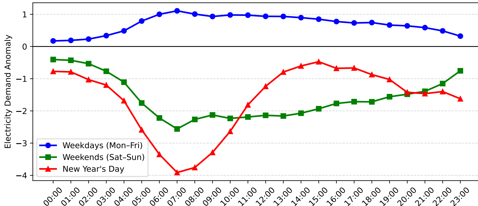
Lisarow Demand Anomaly: New Year's Day vs Weekday/Weekend (2011-2012)
