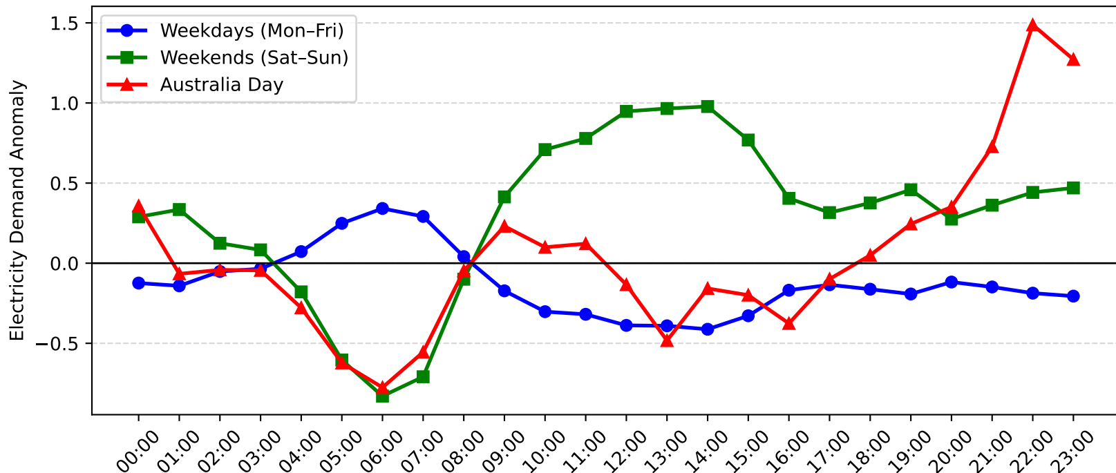
Umina Demand Anomaly: Australia Day vs Weekday/Weekend (2007-2008)
