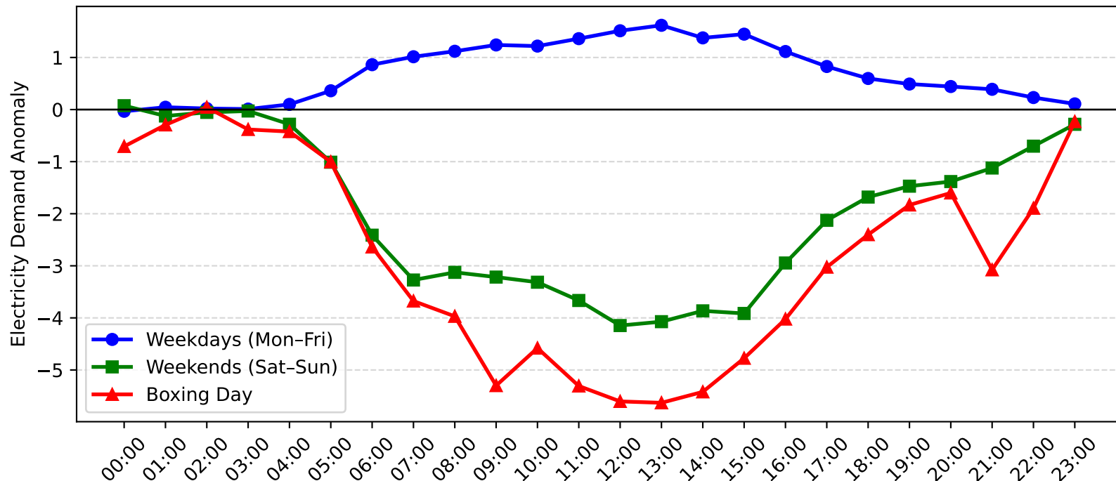
Wyong Demand Anomaly: Boxing Day vs Weekday/Weekend (2008-2009)
