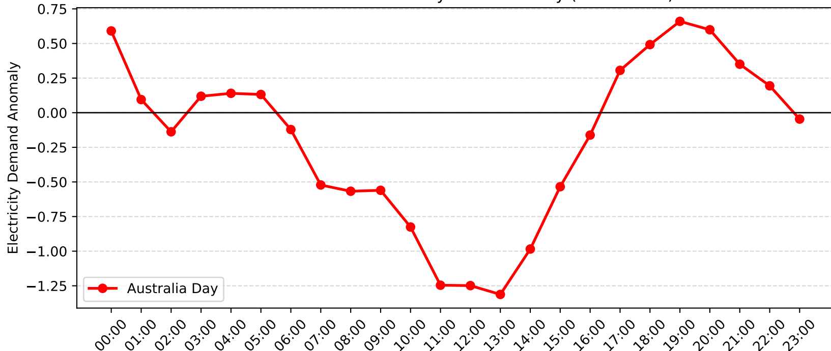
Telarah Demand Anomaly: Australia Day (2006-2007)
