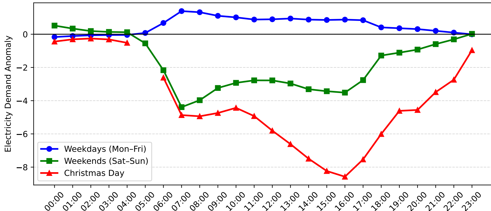
Chatswood Demand Anomaly: Christmas Day vs Weekday/Weekend (2013-2014)
