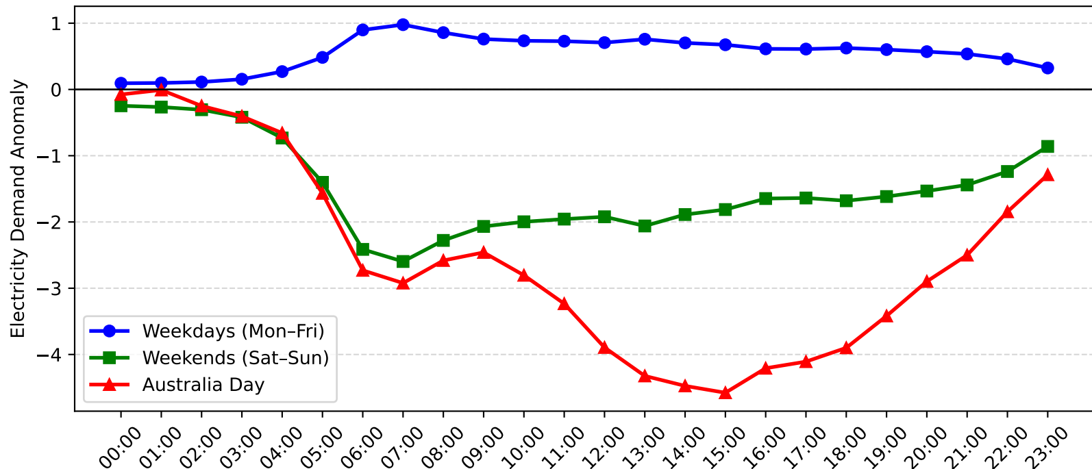
Lisarow Demand Anomaly: Australia Day vs Weekday/Weekend (2016-2017)
