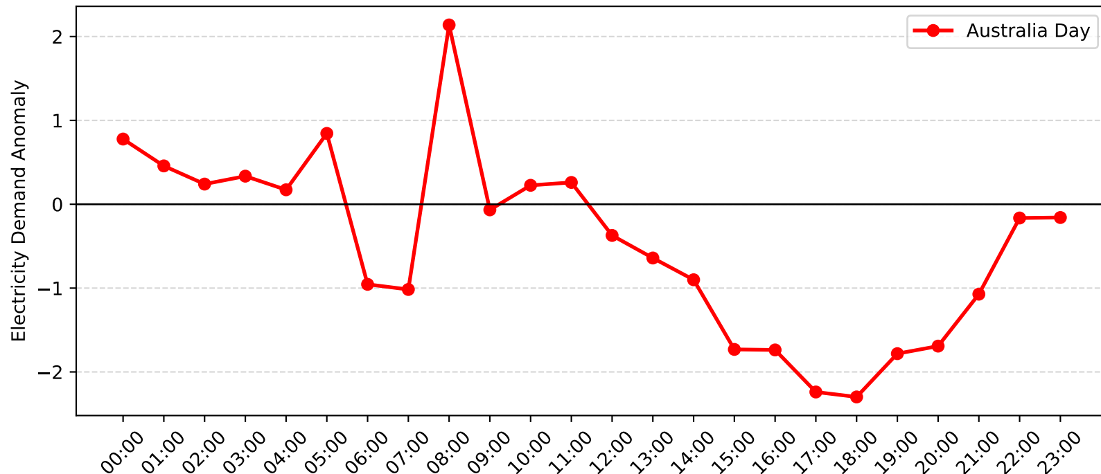
Charmhaven Demand Anomaly: Australia Day (2013-2014)
