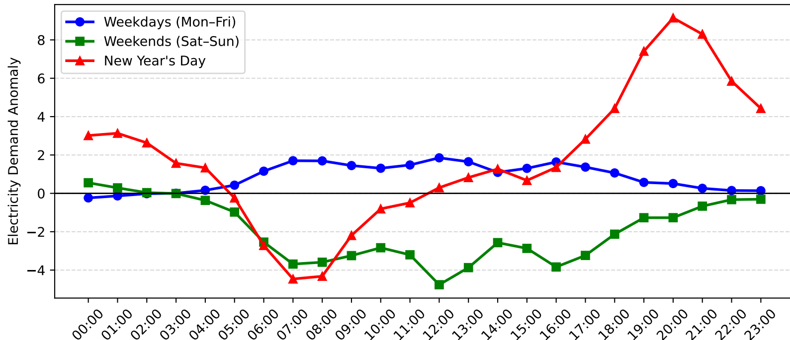
Meadowbank Demand Anomaly: New Year's Day vs Weekday/Weekend (2005-2006)
