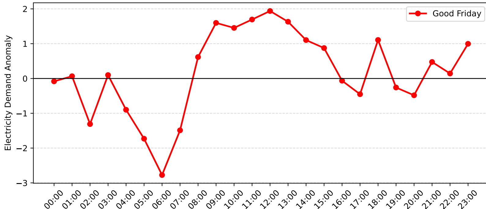
Avoca Demand Anomaly: Good Friday (2006-2007)
