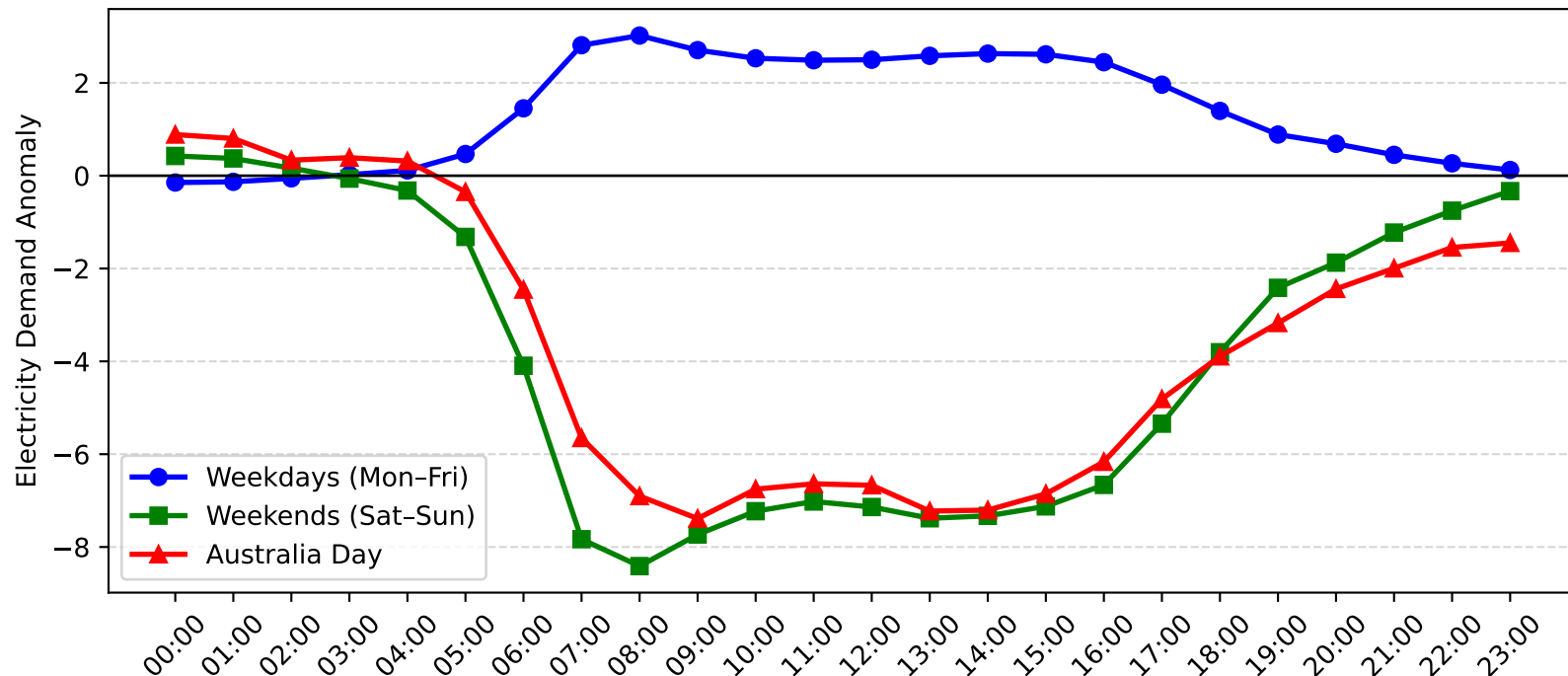
Zetland Demand Anomaly: Australia Day vs Weekday/Weekend (2015-2016)
