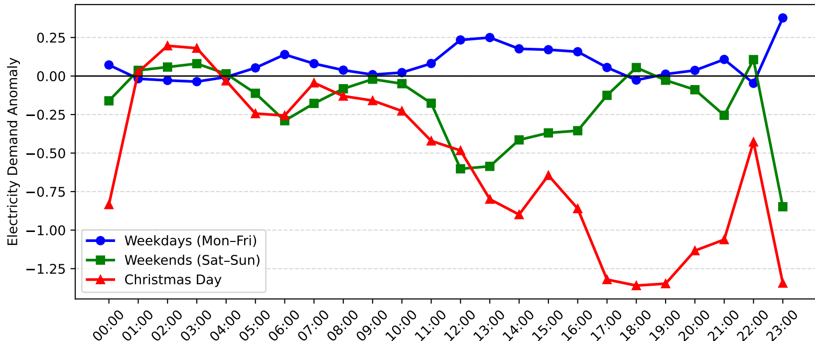
Telarah Demand Anomaly: Christmas Day vs Weekday/Weekend (2004-2005)
