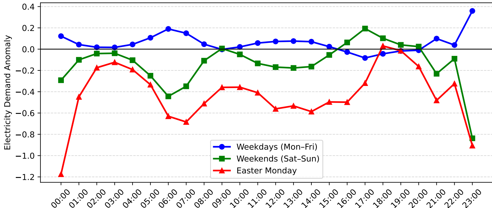
Telarah Demand Anomaly: Easter Monday vs Weekday/Weekend (2012-2013)
