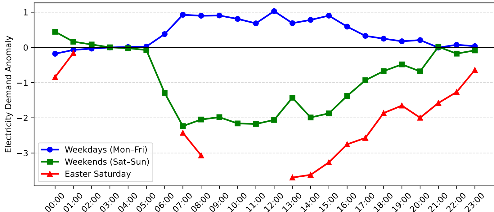
Potts Hill Demand Anomaly: Easter Saturday vs Weekday/Weekend (2013-2014)
