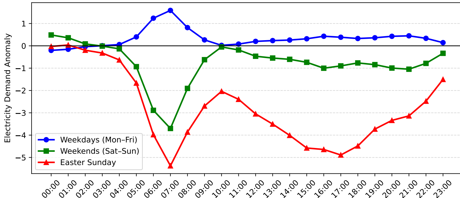
Dulwich Hill Demand Anomaly: Easter Sunday vs Weekday/Weekend (2013-2014)
