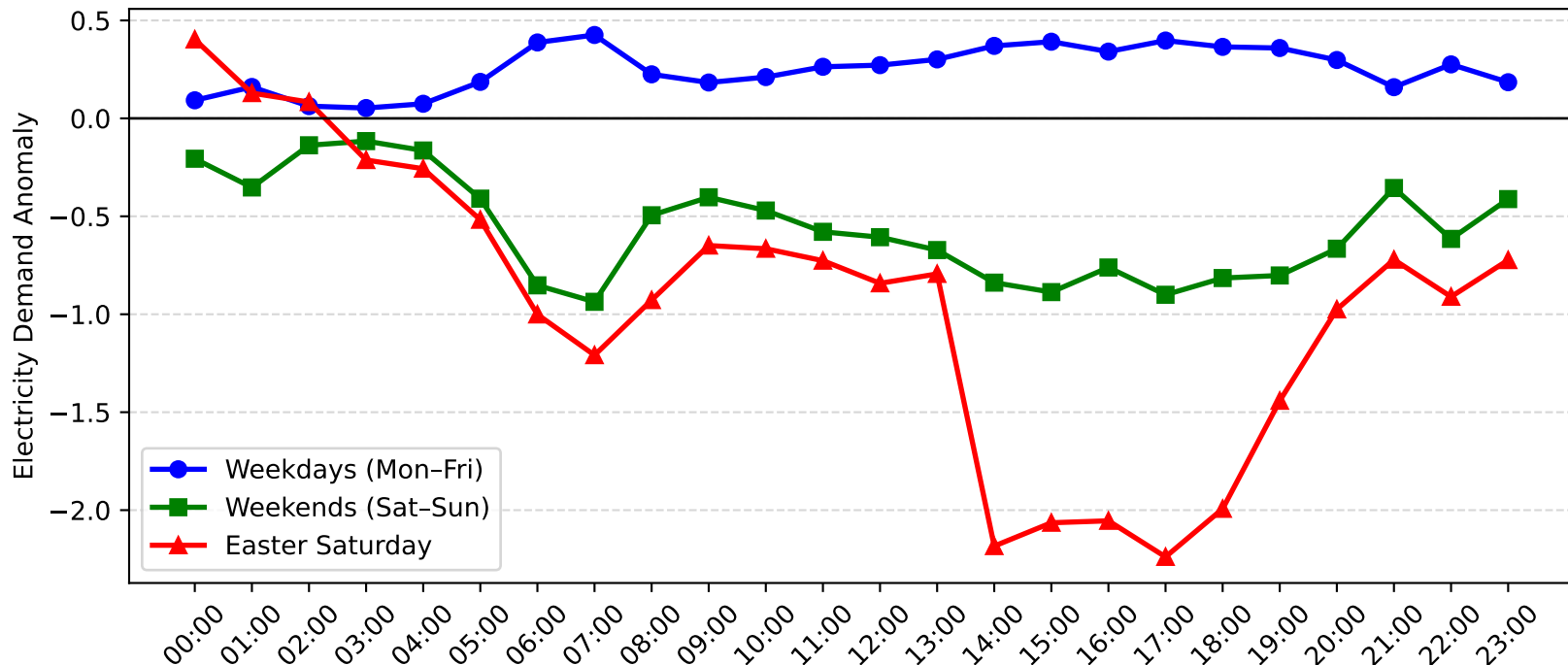
Maryland Demand Anomaly: Easter Saturday vs Weekday/Weekend (2016-2017)
