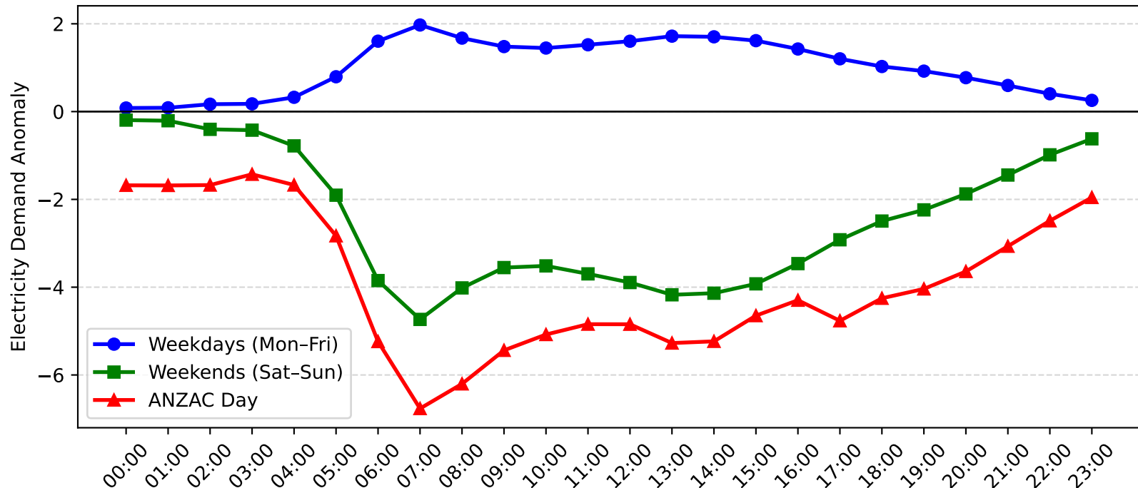
Sefton Demand Anomaly: ANZAC Day vs Weekday/Weekend (2014-2015)
