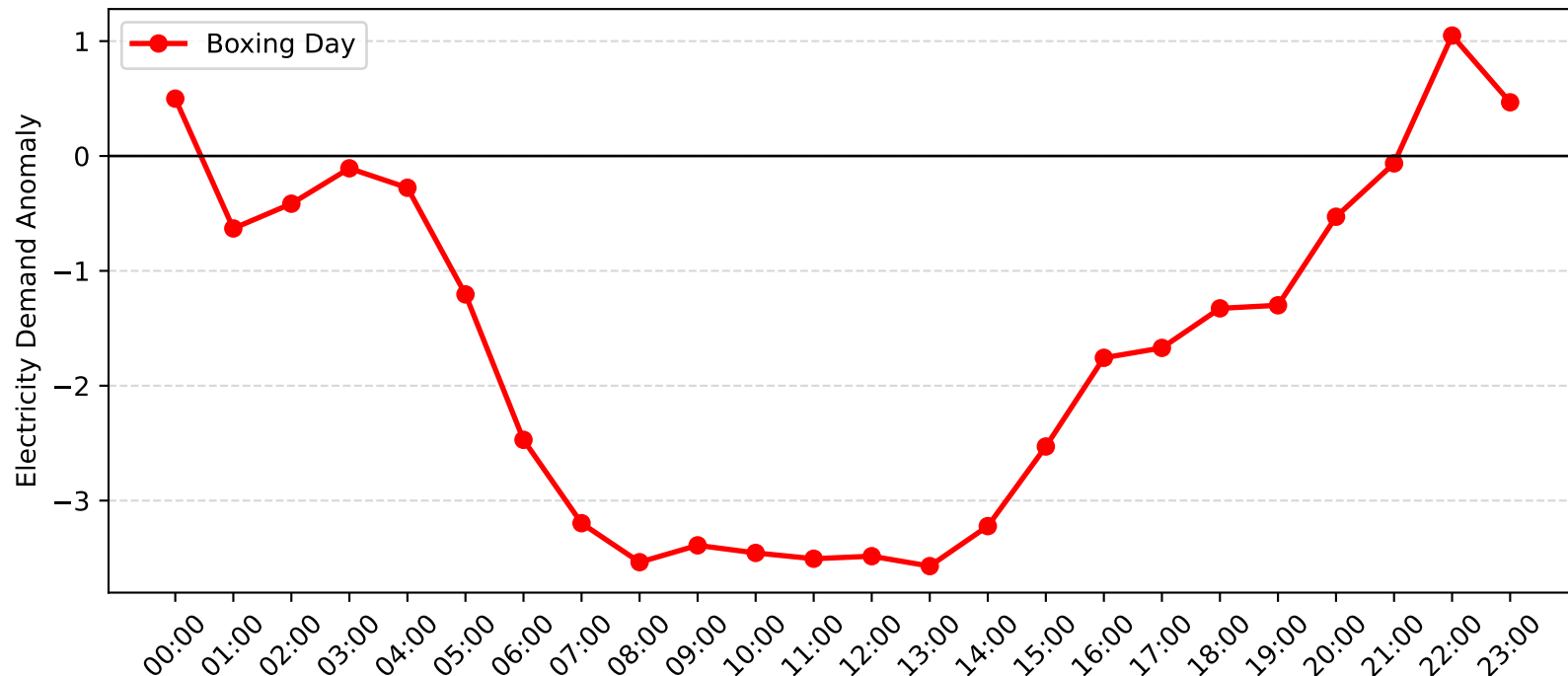
Wyong Demand Anomaly: Boxing Day (2004-2005)
