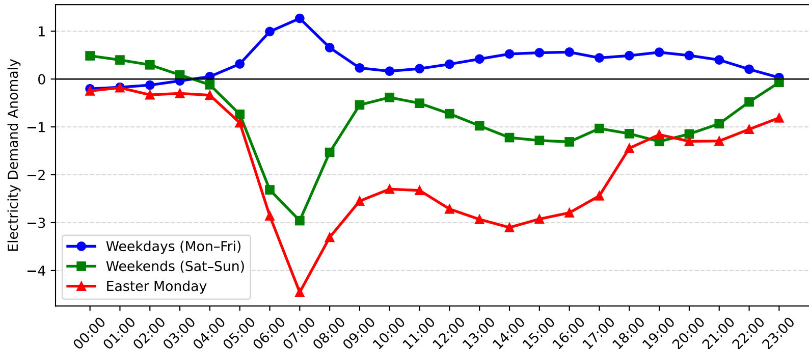
Five Dock Demand Anomaly: Easter Monday vs Weekday/Weekend (2012-2013)
