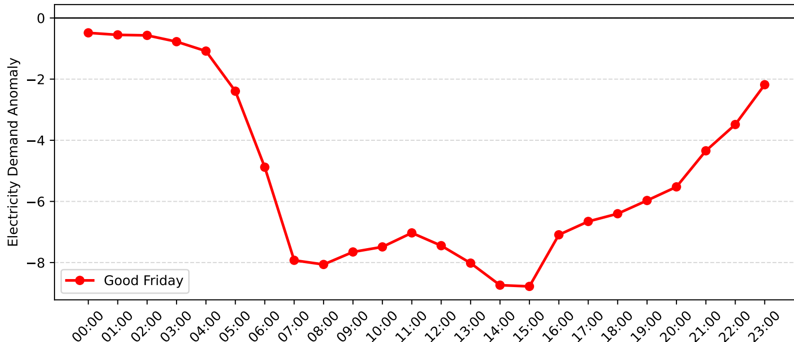
Marrickville Demand Anomaly: Good Friday (2015-2016)
