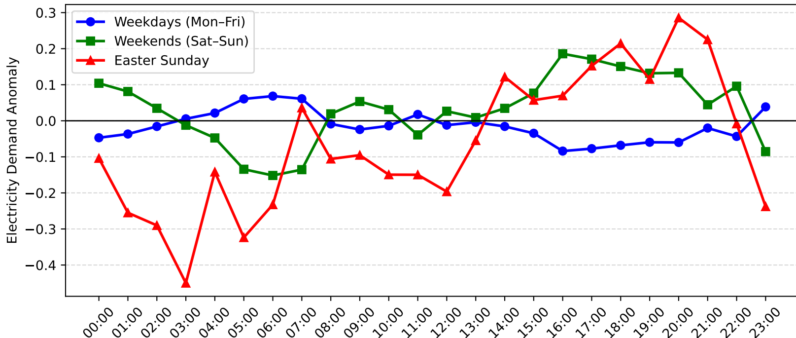
Rothbury Demand Anomaly: Easter Sunday vs Weekday/Weekend (2017-2018)
