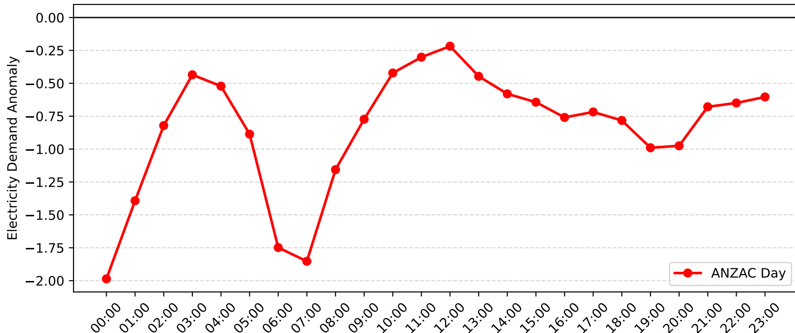
Morisset Demand Anomaly: ANZAC Day (2010-2011)
