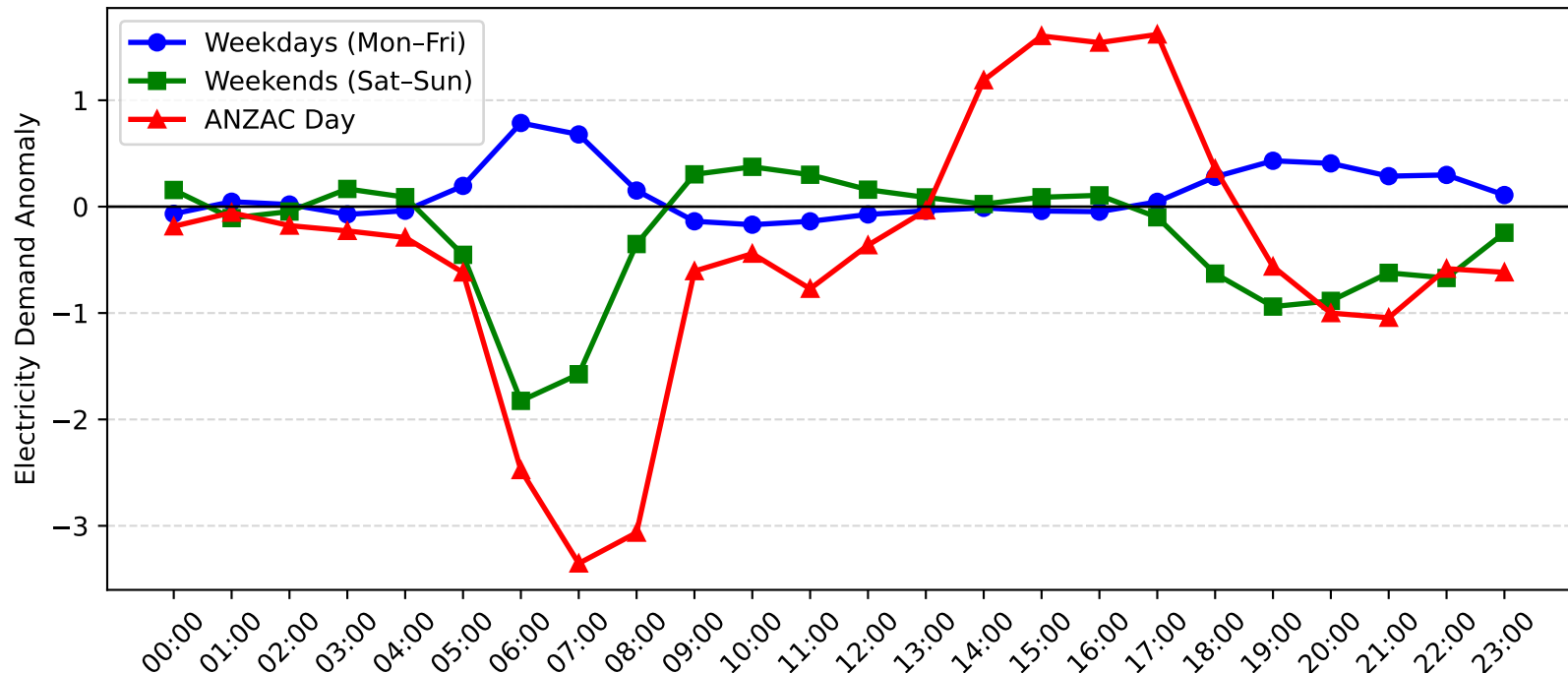
Balgowlah North Demand Anomaly: ANZAC Day vs Weekday/Weekend (2016-2017)
