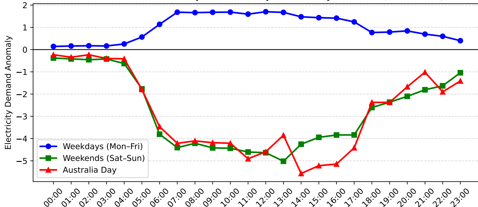
Potts Hill Demand Anomaly: Australia Day vs Weekday/Weekend (2015-2016)
