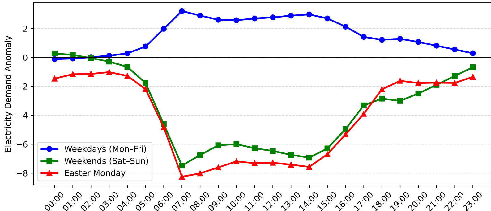
Marrickville Demand Anomaly: Easter Monday vs Weekday/Weekend (2012-2013)
