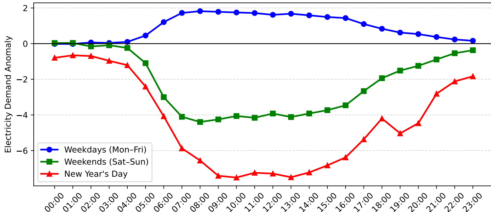
Concord Demand Anomaly: New Year's Day vs Weekday/Weekend (2007-2008)
