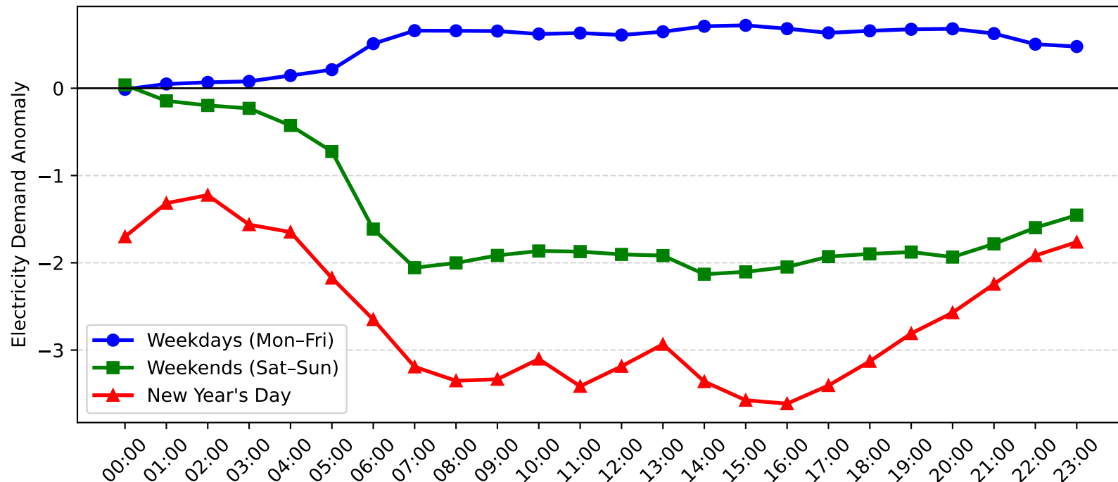
Enfield Demand Anomaly: New Year's Day vs Weekday/Weekend (2014-2015)
