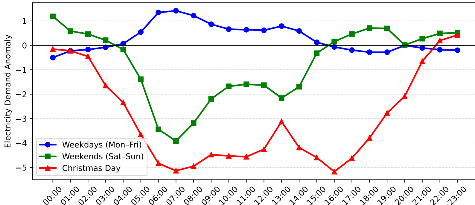
Pennant Hills Demand Anomaly: Christmas Day vs Weekday/Weekend (2009-2010)
