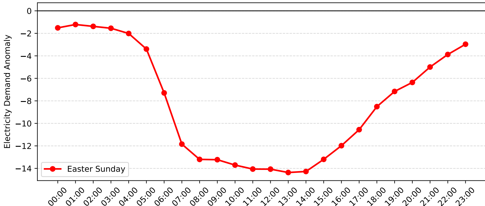
St. Peters Demand Anomaly: Easter Sunday (2013-2014)
