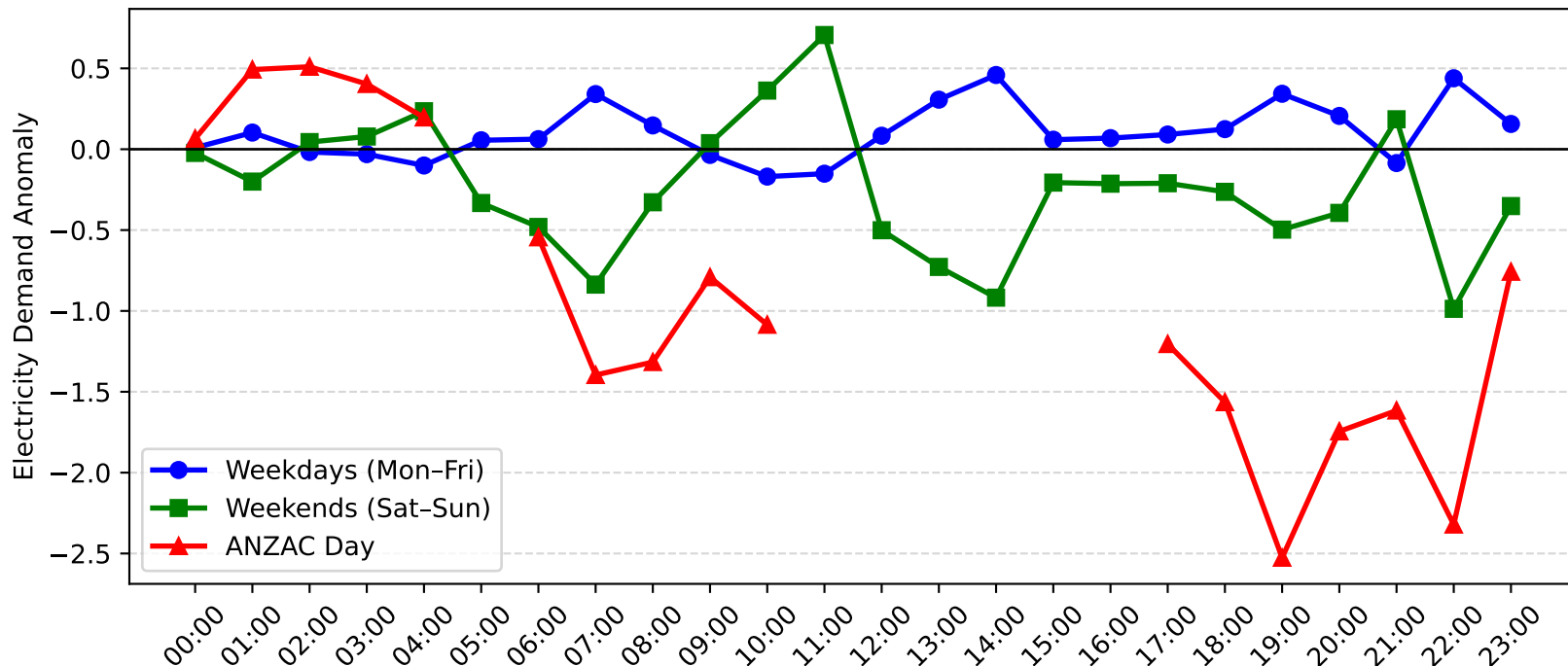
Adamstown Demand Anomaly: ANZAC Day vs Weekday/Weekend (2015-2016)
