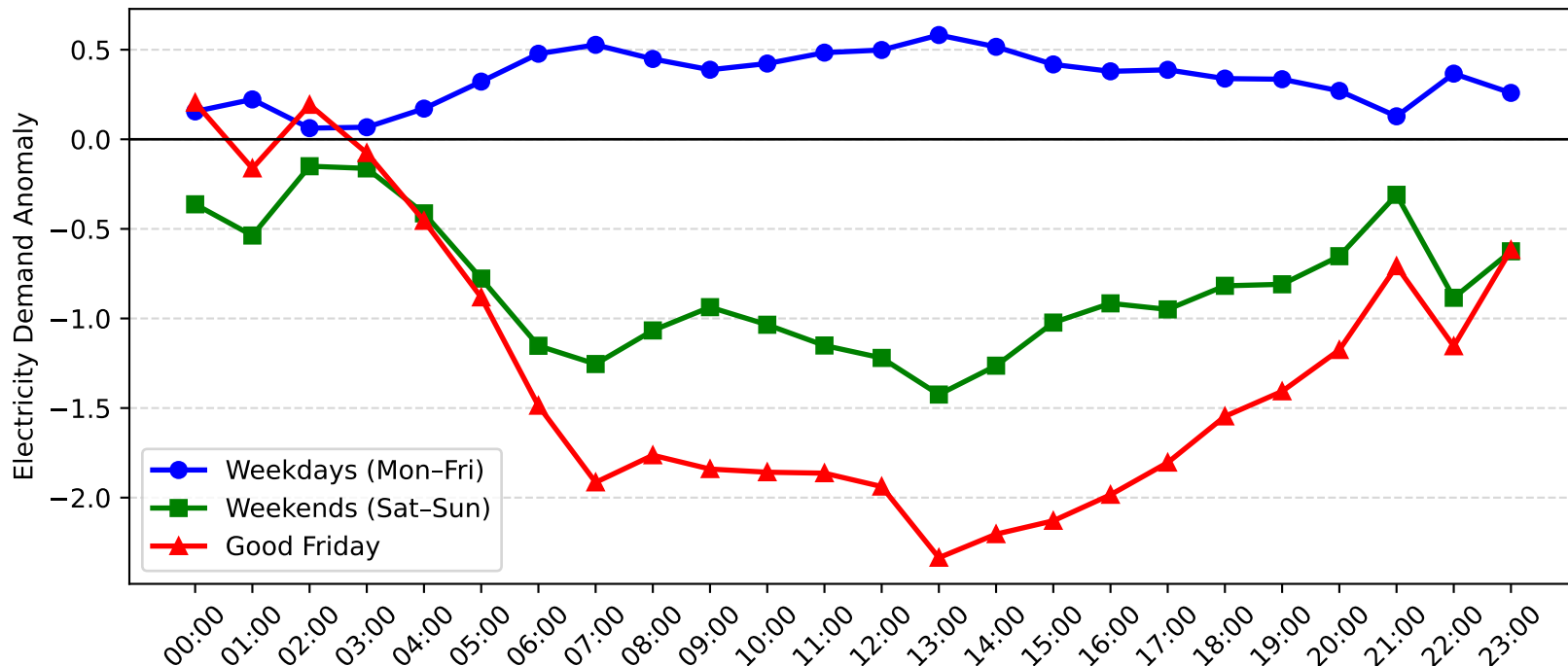
Gateshead Demand Anomaly: Good Friday vs Weekday/Weekend (2016-2017)
