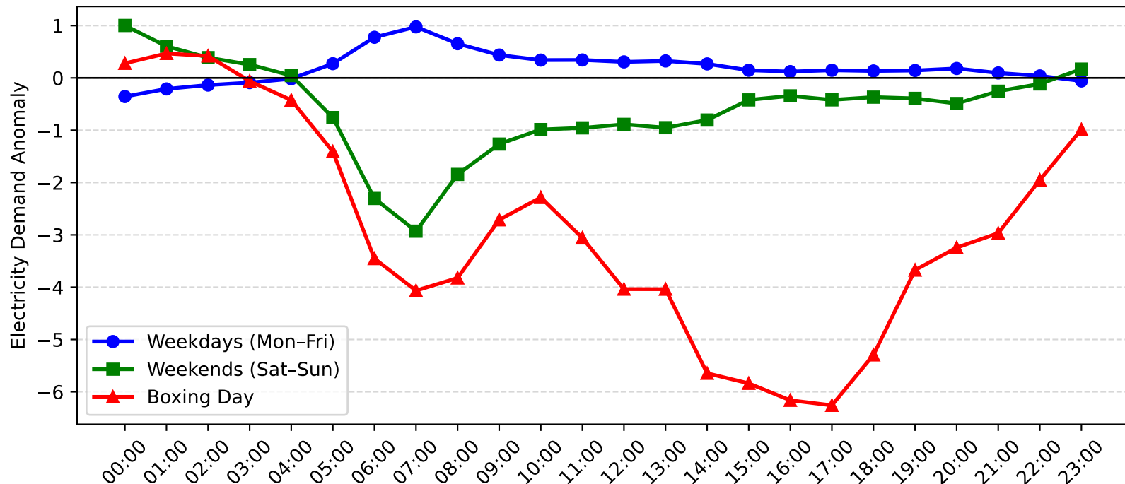
Mortdale Demand Anomaly: Boxing Day vs Weekday/Weekend (2013-2014)
