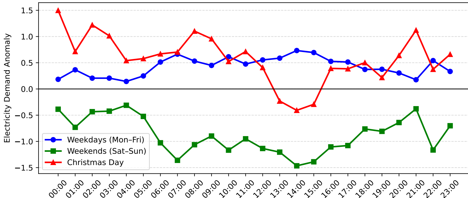
Jesmond Demand Anomaly: Christmas Day vs Weekday/Weekend (2010-2011)
