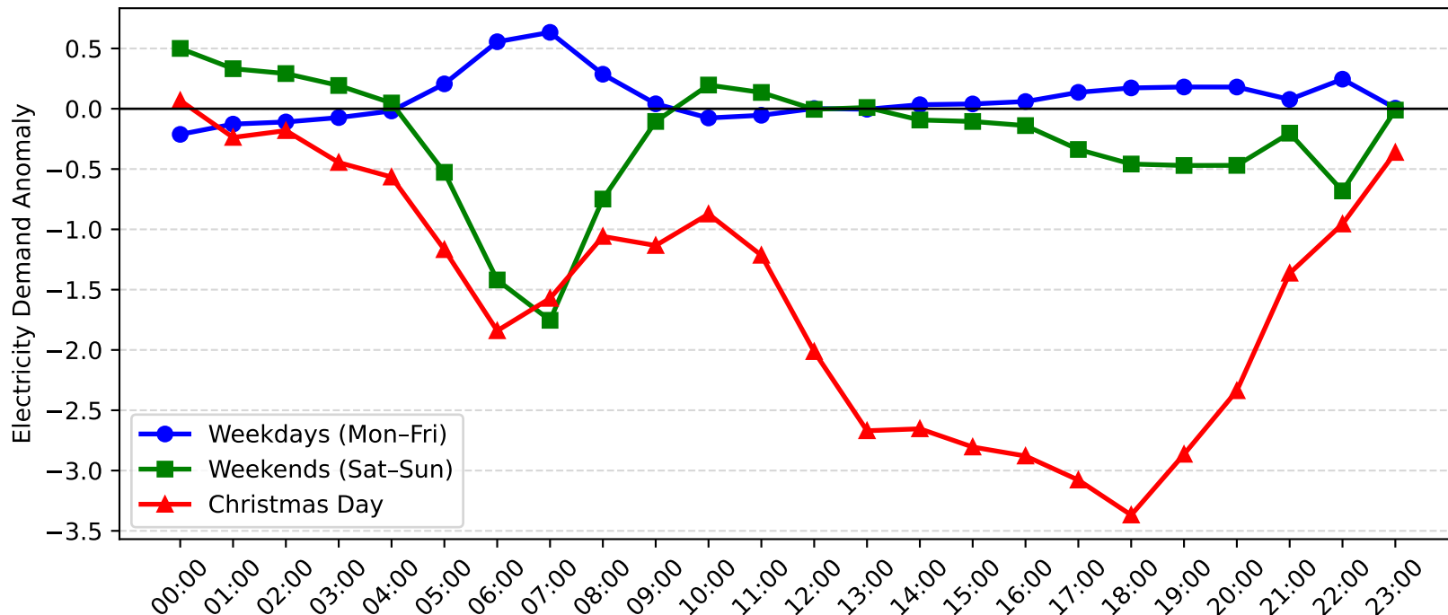
Harbord Demand Anomaly: Christmas Day vs Weekday/Weekend (2009-2010)
