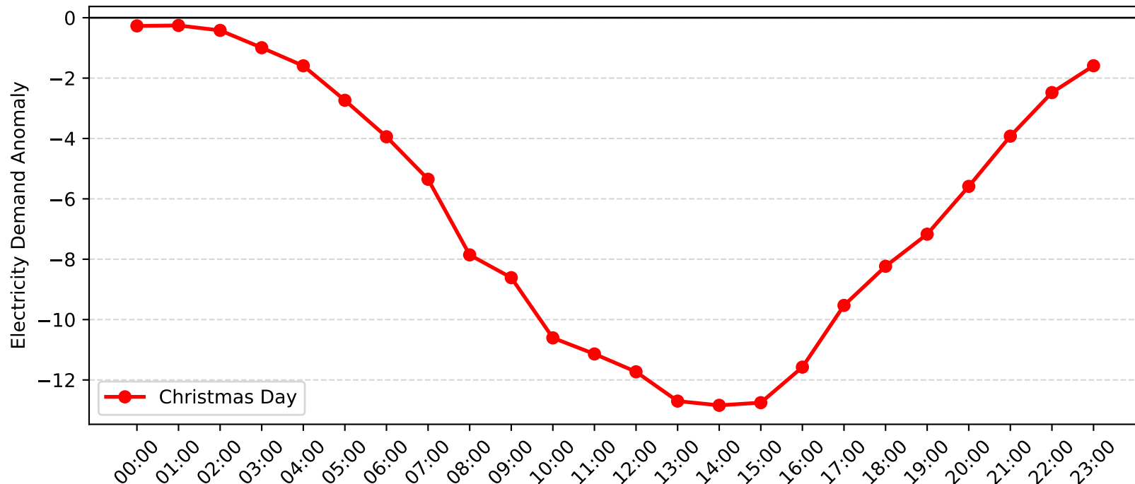
West Gosford Demand Anomaly: Christmas Day (2014-2015)
