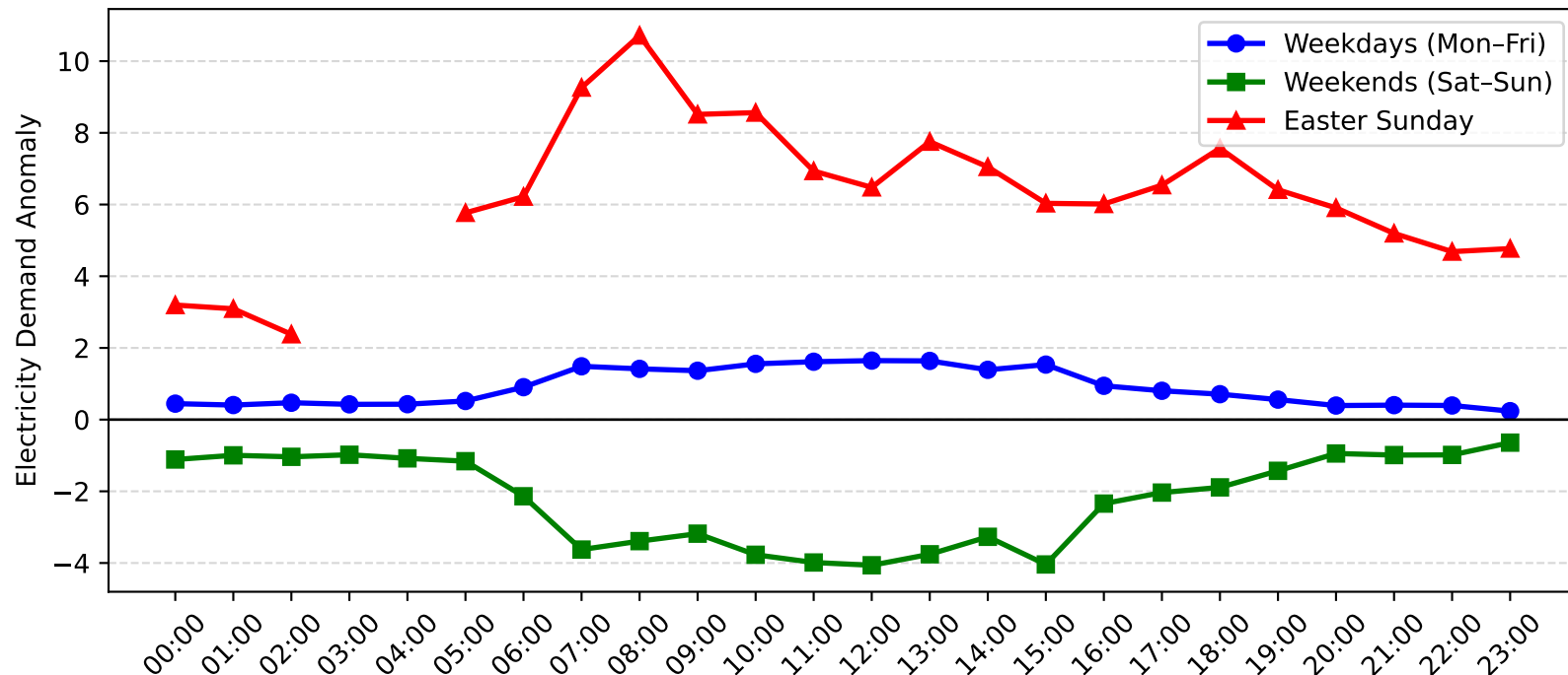
Milperra Demand Anomaly: Easter Sunday vs Weekday/Weekend (2004-2005)
