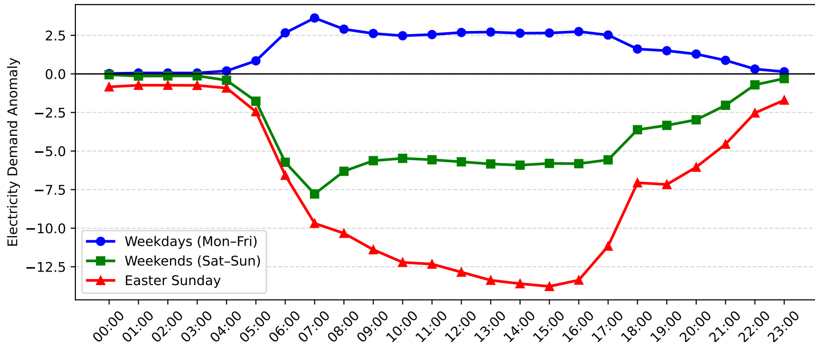
Epping Demand Anomaly: Easter Sunday vs Weekday/Weekend (2009-2010)
