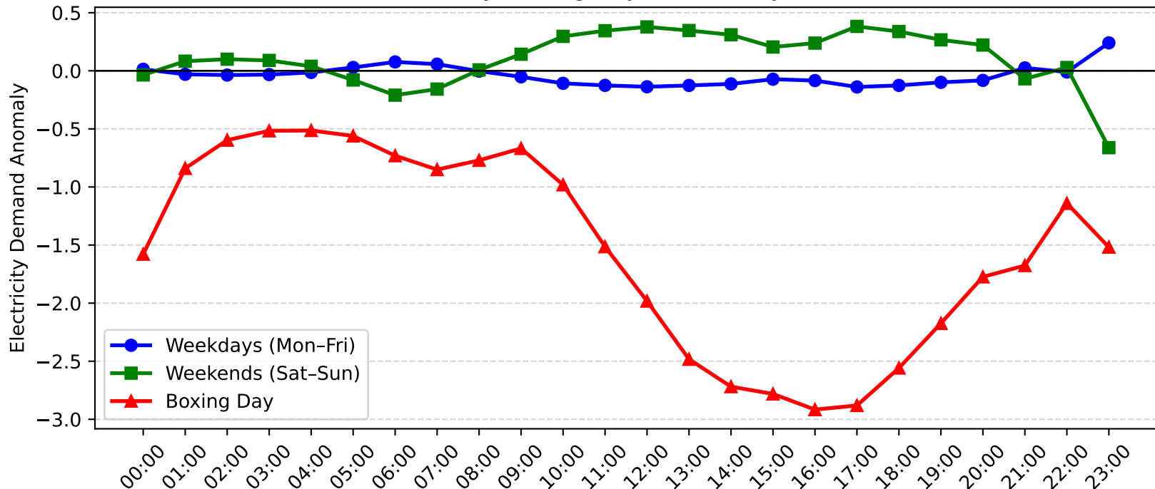
Telarah Demand Anomaly: Boxing Day vs Weekday/Weekend (2012-2013)
