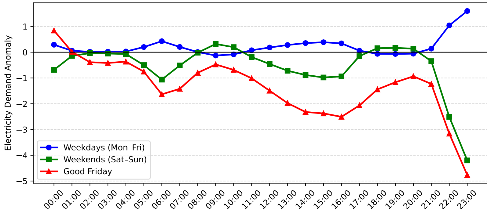
Muswellbrook Demand Anomaly: Good Friday vs Weekday/Weekend (2005-2006)
