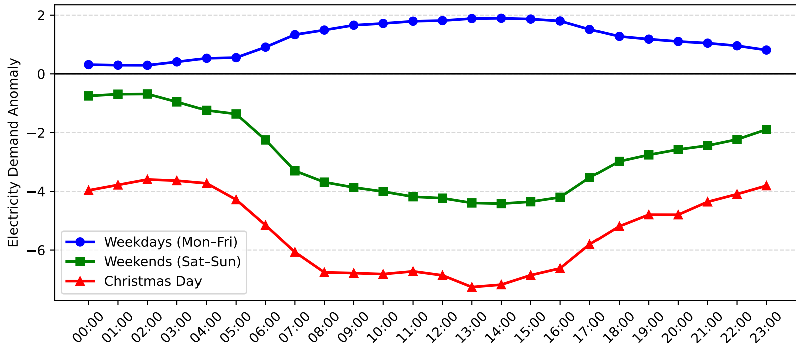
Leightonfield Demand Anomaly: Christmas Day vs Weekday/Weekend (2016-2017)
