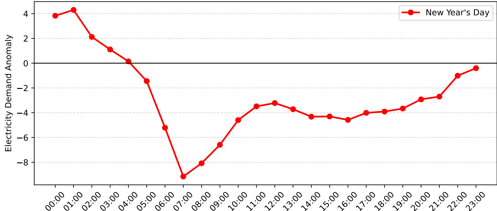
Mosman Demand Anomaly: New Year's Day (2011-2012)
