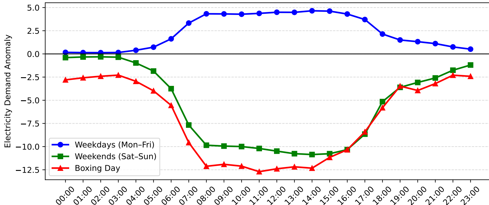
Gore Hill Demand Anomaly: Boxing Day vs Weekday/Weekend (2015-2016)
