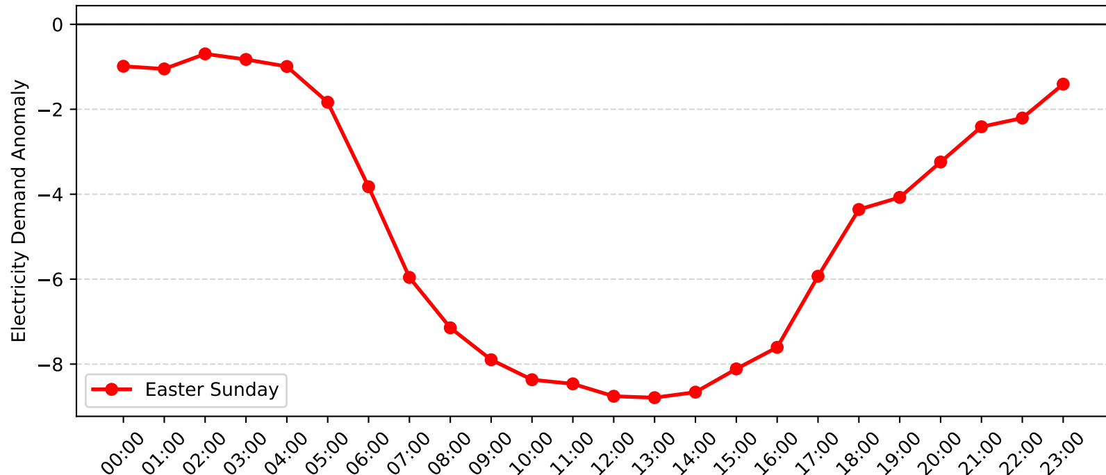
Newcastle Cbd Demand Anomaly: Easter Sunday (2017-2018)
