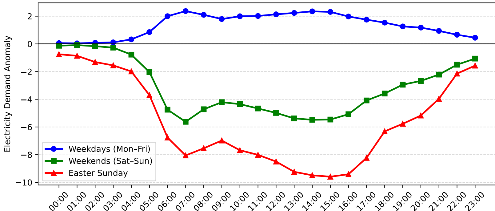
Sefton Demand Anomaly: Easter Sunday vs Weekday/Weekend (2006-2007)
