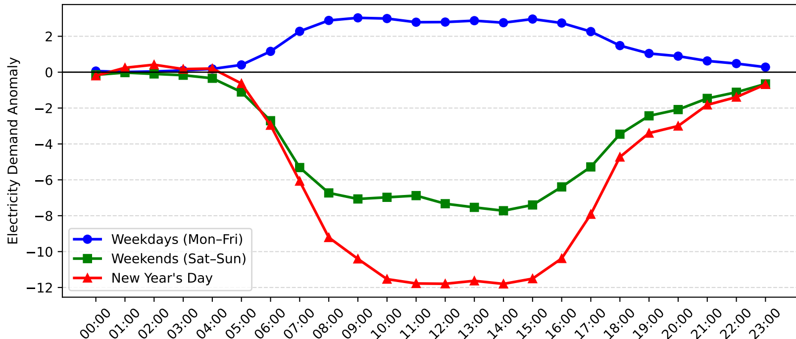
Green Square Demand Anomaly: New Year's Day vs Weekday/Weekend (2017-2018)
