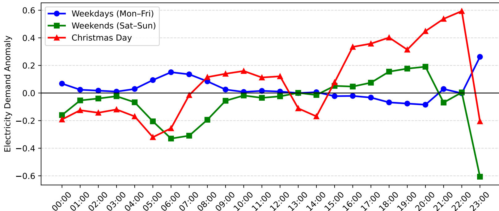
Telarah Demand Anomaly: Christmas Day vs Weekday/Weekend (2010-2011)
