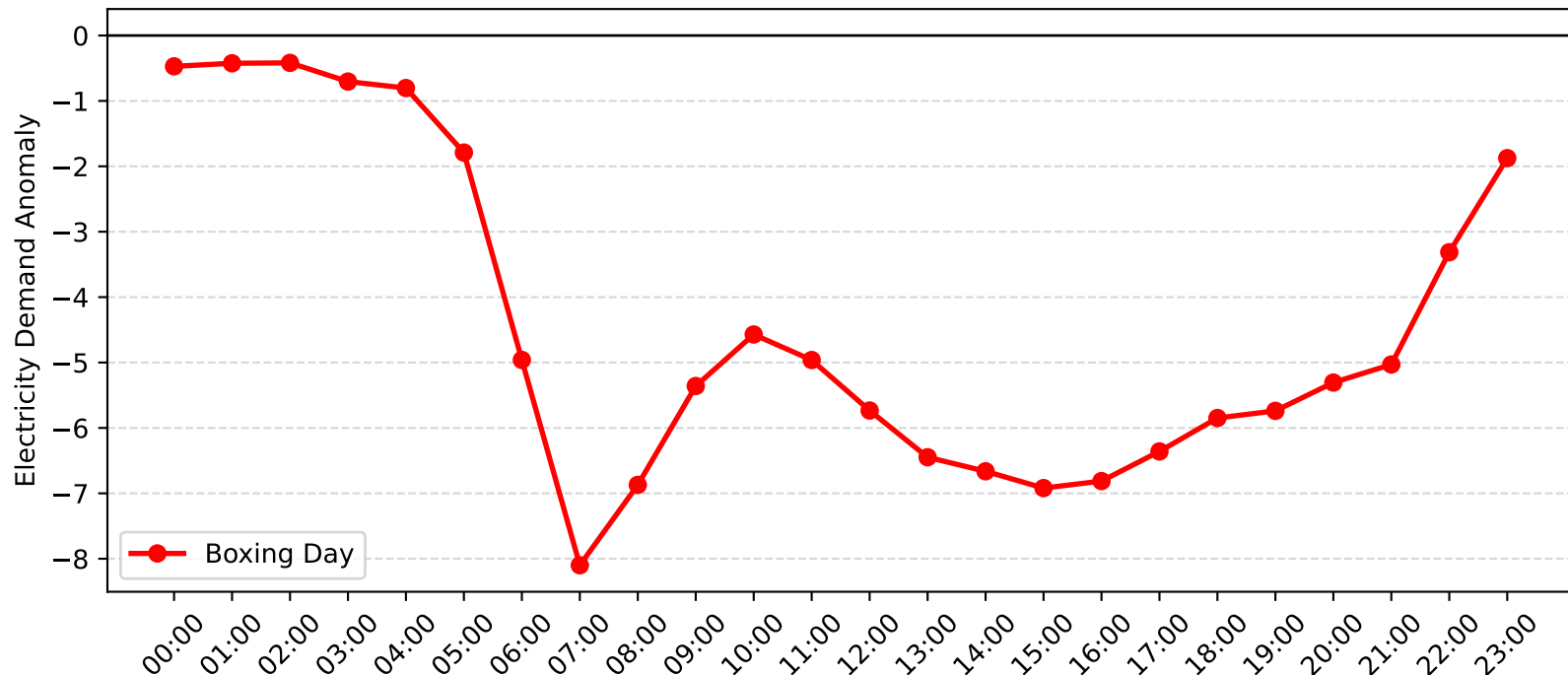
Mosman Demand Anomaly: Boxing Day (2011-2012)
