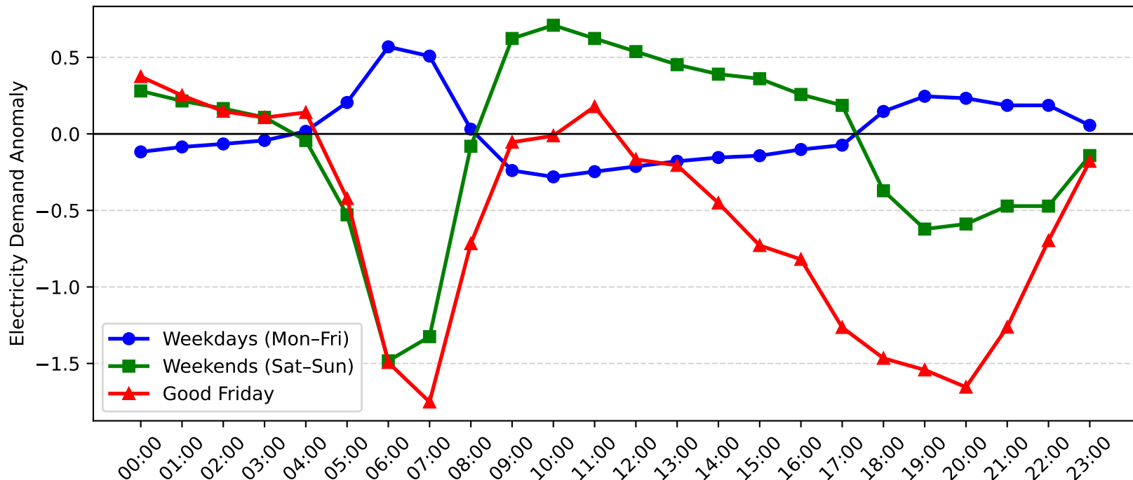
Harbord Demand Anomaly: Good Friday vs Weekday/Weekend (2012-2013)
