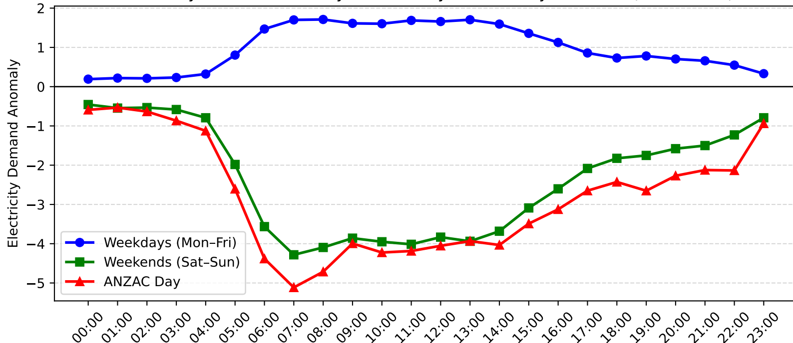
Somersby Demand Anomaly: ANZAC Day vs Weekday/Weekend (2008-2009)
