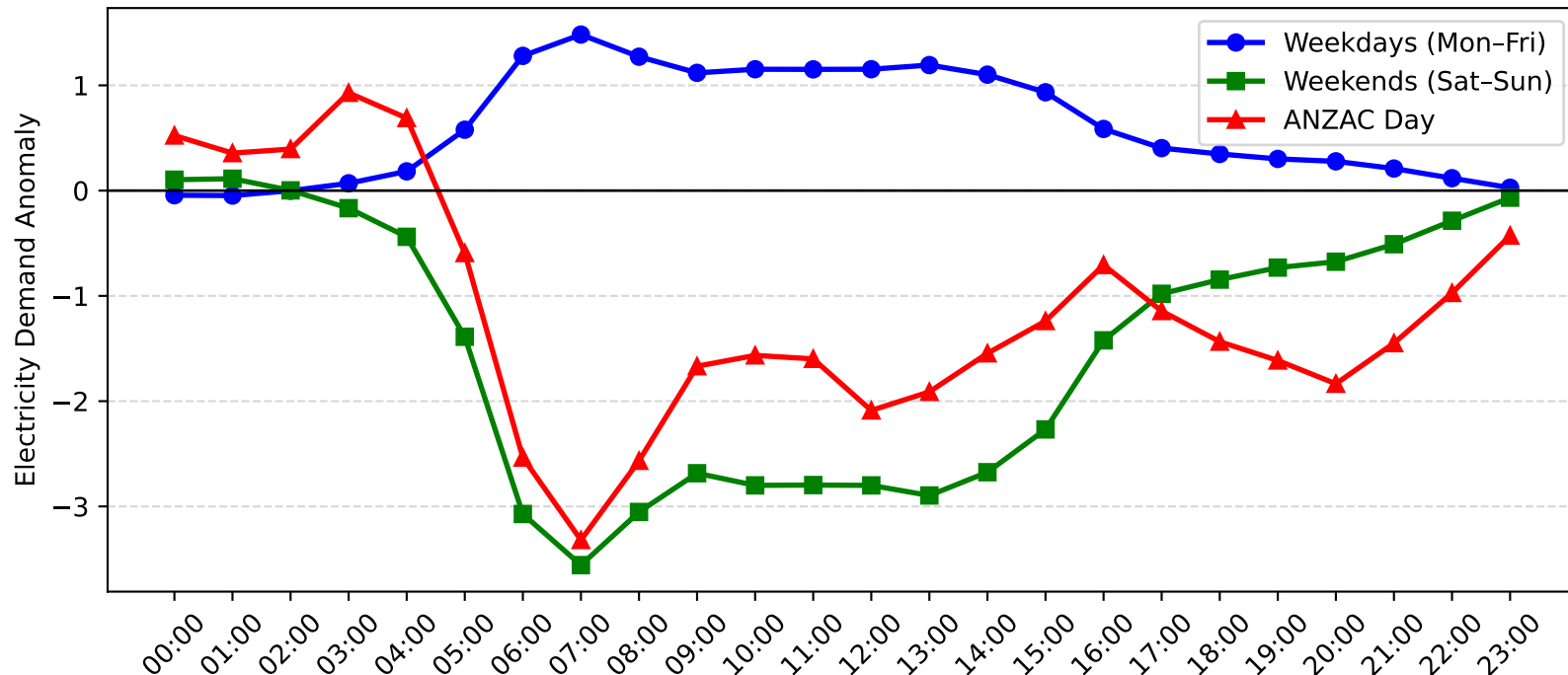
Wyong Demand Anomaly: ANZAC Day vs Weekday/Weekend (2014-2015)
