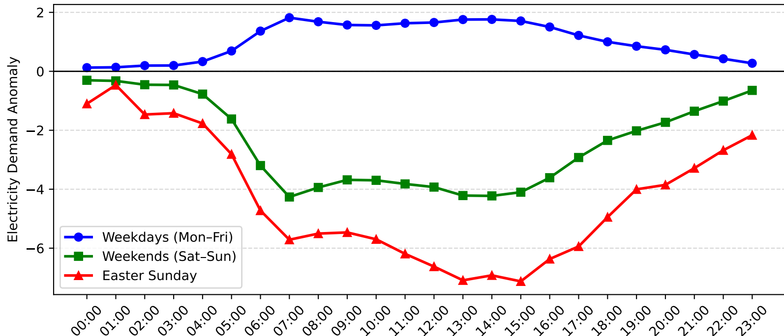
Sefton Demand Anomaly: Easter Sunday vs Weekday/Weekend (2015-2016)
