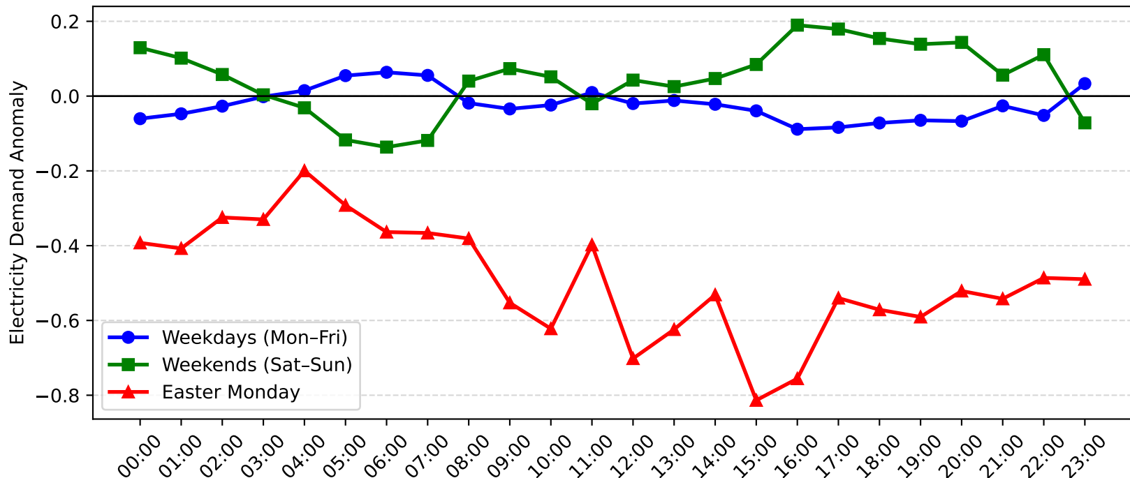
Rothbury Demand Anomaly: Easter Monday vs Weekday/Weekend (2017-2018)
