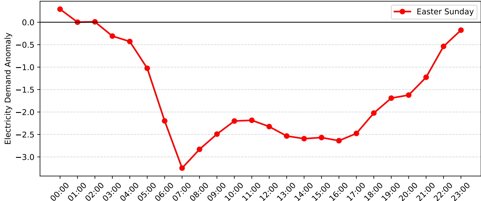
Rockdale Demand Anomaly: Easter Sunday (2008-2009)
