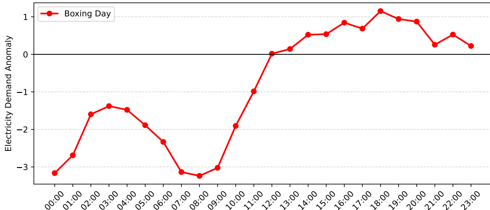
Jesmond Demand Anomaly: Boxing Day (2016-2017)
