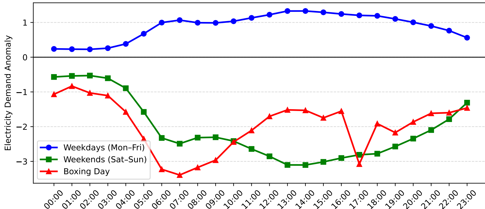
Lisarow Demand Anomaly: Boxing Day vs Weekday/Weekend (2016-2017)
