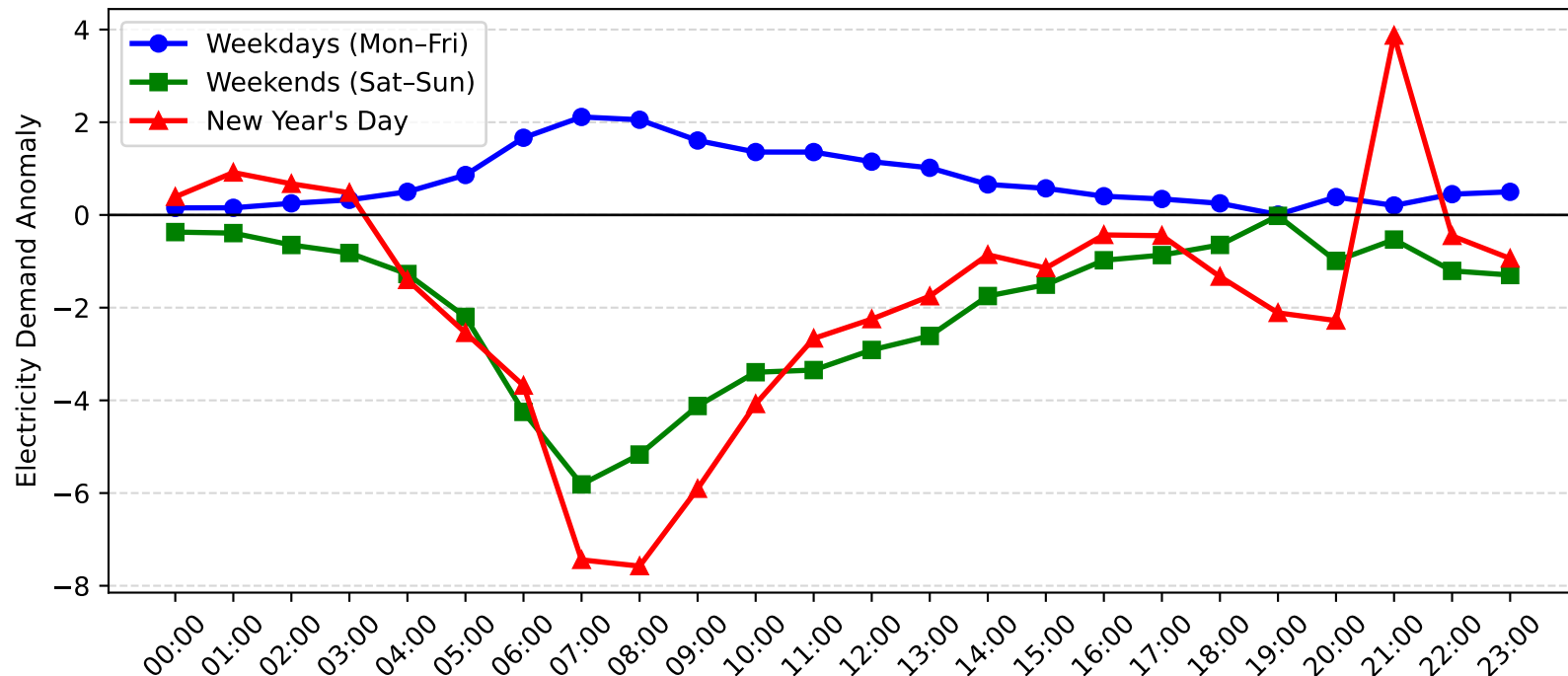
Meadowbank Demand Anomaly: New Year's Day vs Weekday/Weekend (2010-2011)
