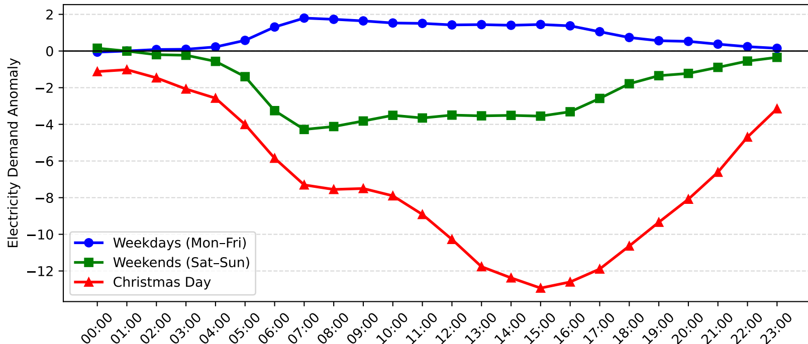
Sefton Demand Anomaly: Christmas Day vs Weekday/Weekend (2006-2007)
