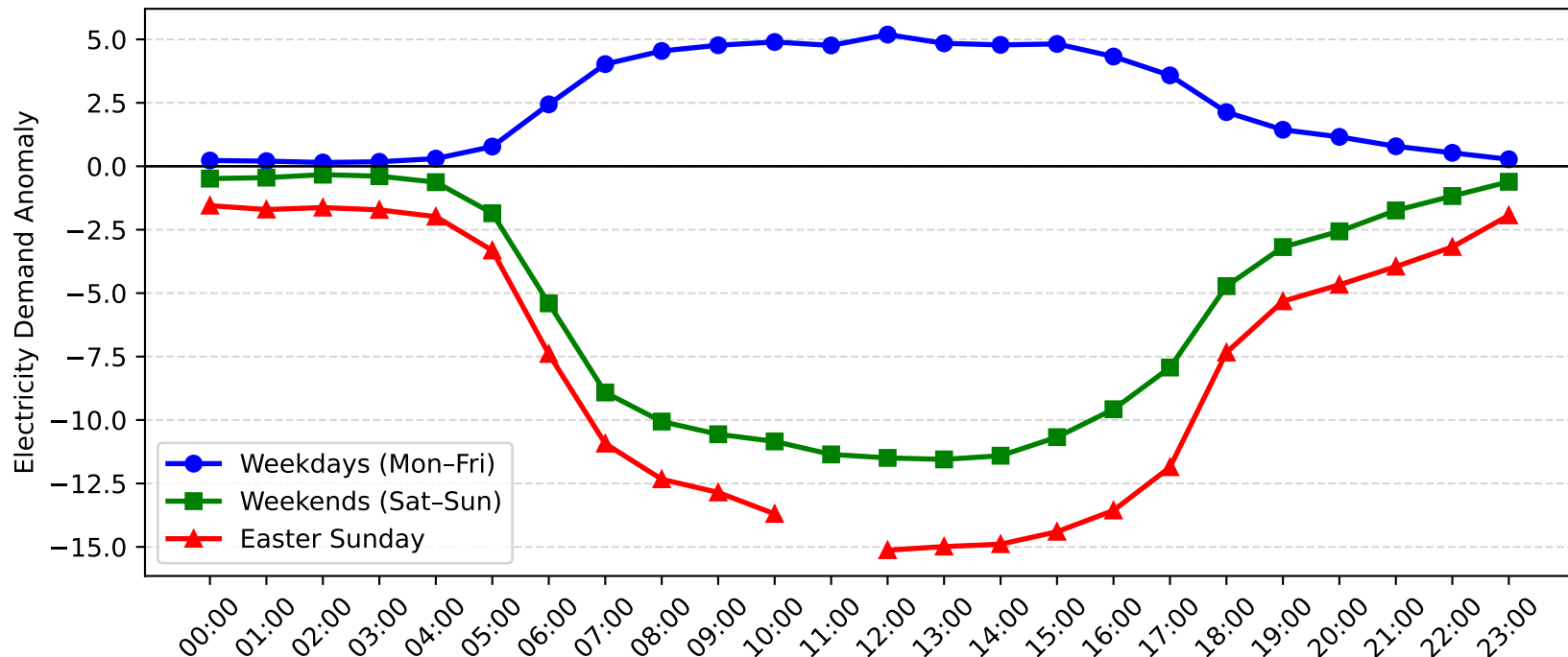
Macquarie Park Demand Anomaly: Easter Sunday vs Weekday/Weekend (2017-2018)
