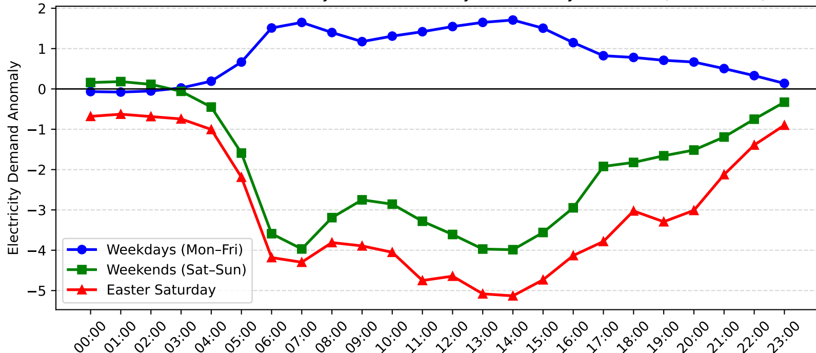
Kirrawee Demand Anomaly: Easter Saturday vs Weekday/Weekend (2006-2007)
