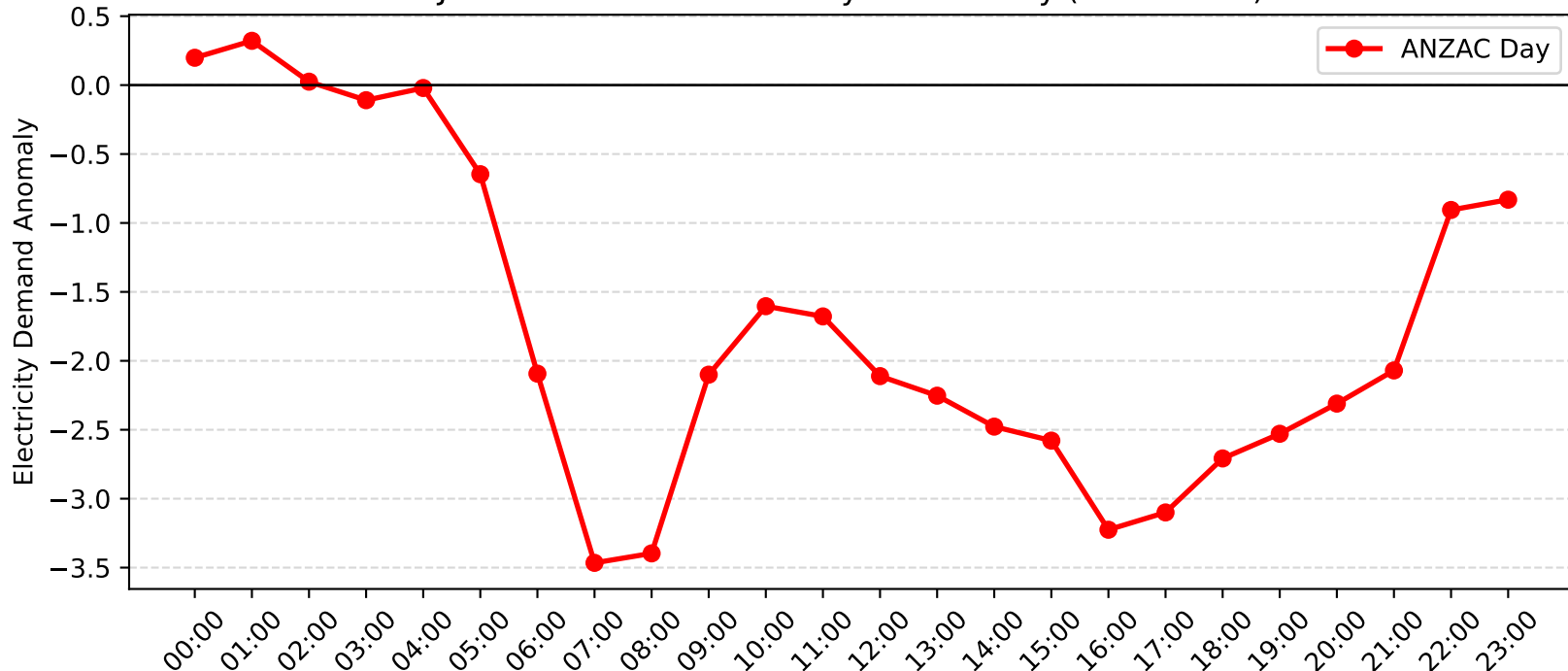
Jesmond Demand Anomaly: ANZAC Day (2013-2014)
