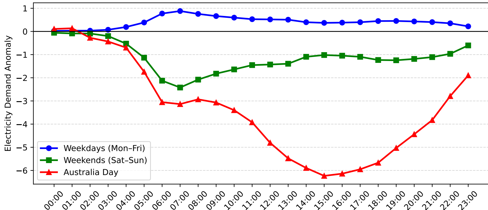
Lisarow Demand Anomaly: Australia Day vs Weekday/Weekend (2017-2018)
