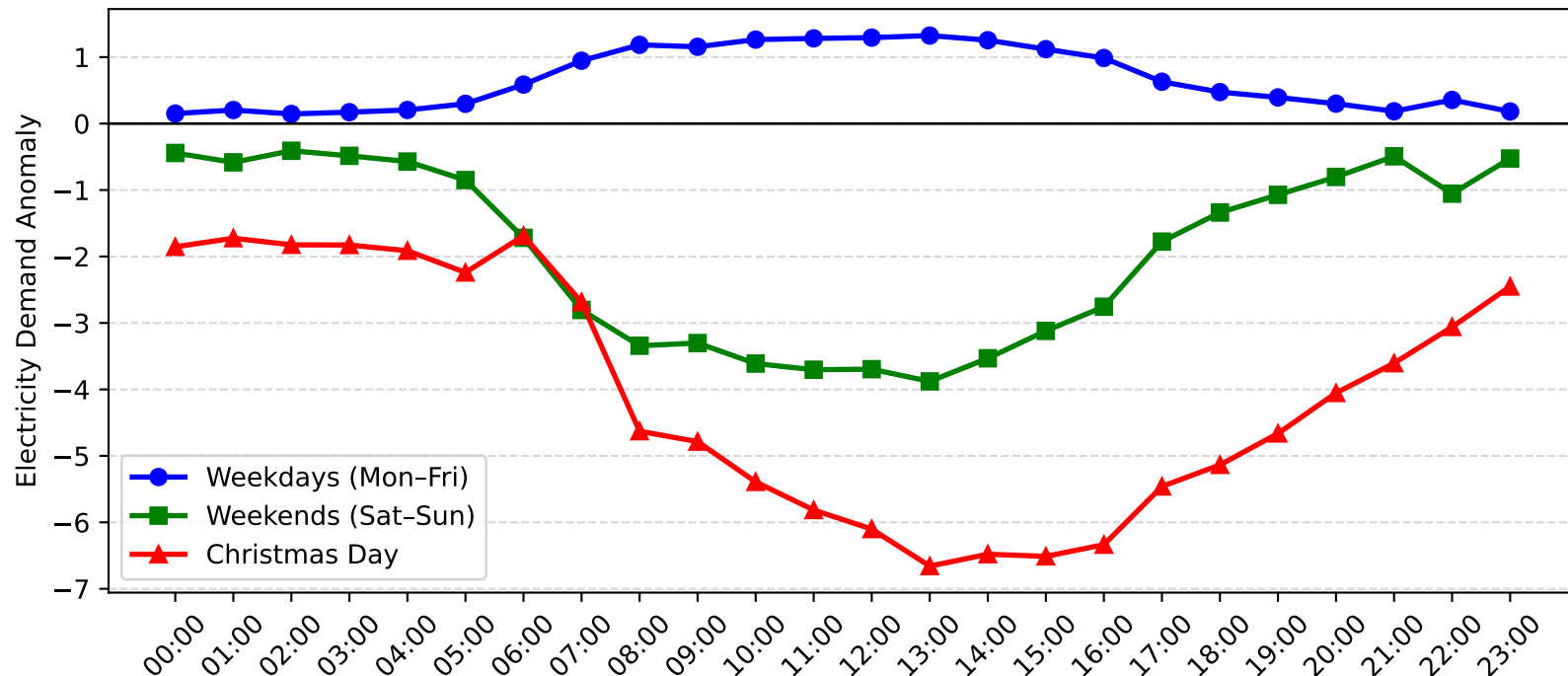
Mayfield West Demand Anomaly: Christmas Day vs Weekday/Weekend (2013-2014)
