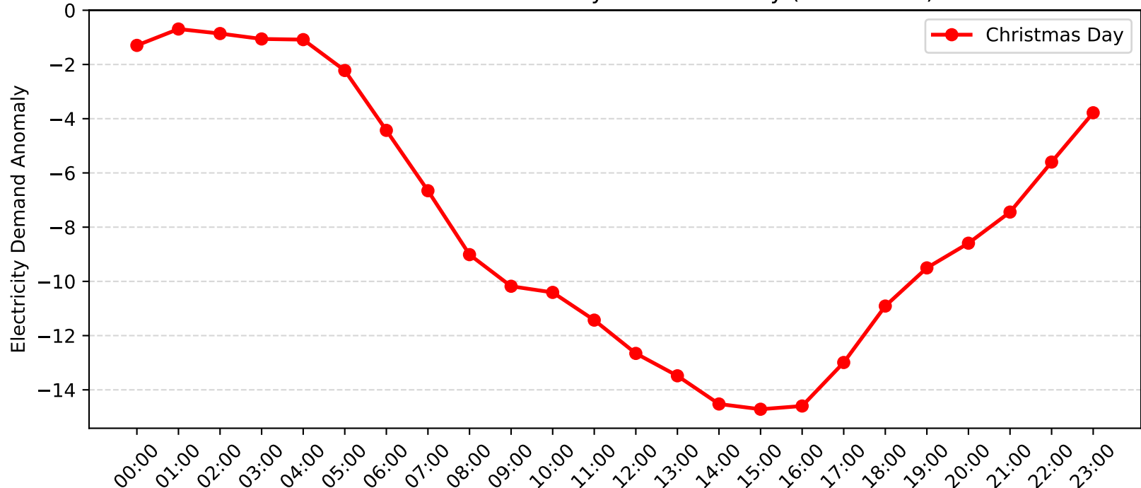
Burwood Demand Anomaly: Christmas Day (2013-2014)
