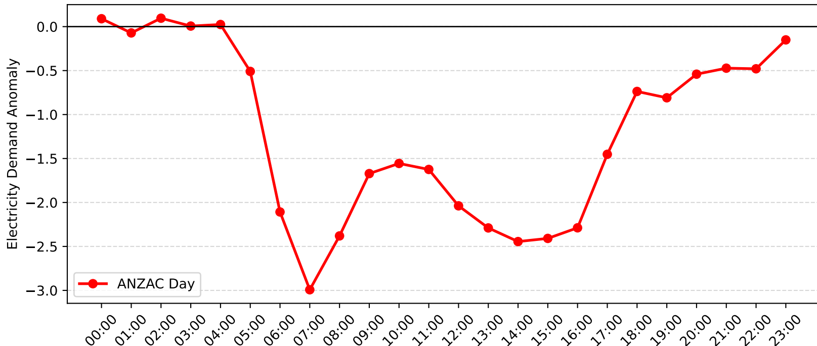
Pymble Demand Anomaly: ANZAC Day (2012-2013)
