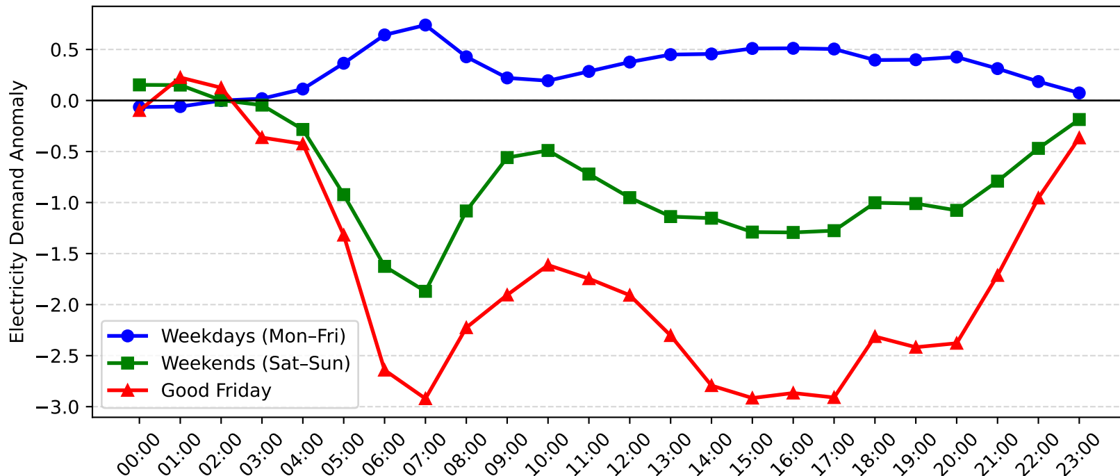
Charmhaven Demand Anomaly: Good Friday vs Weekday/Weekend (2014-2015)
