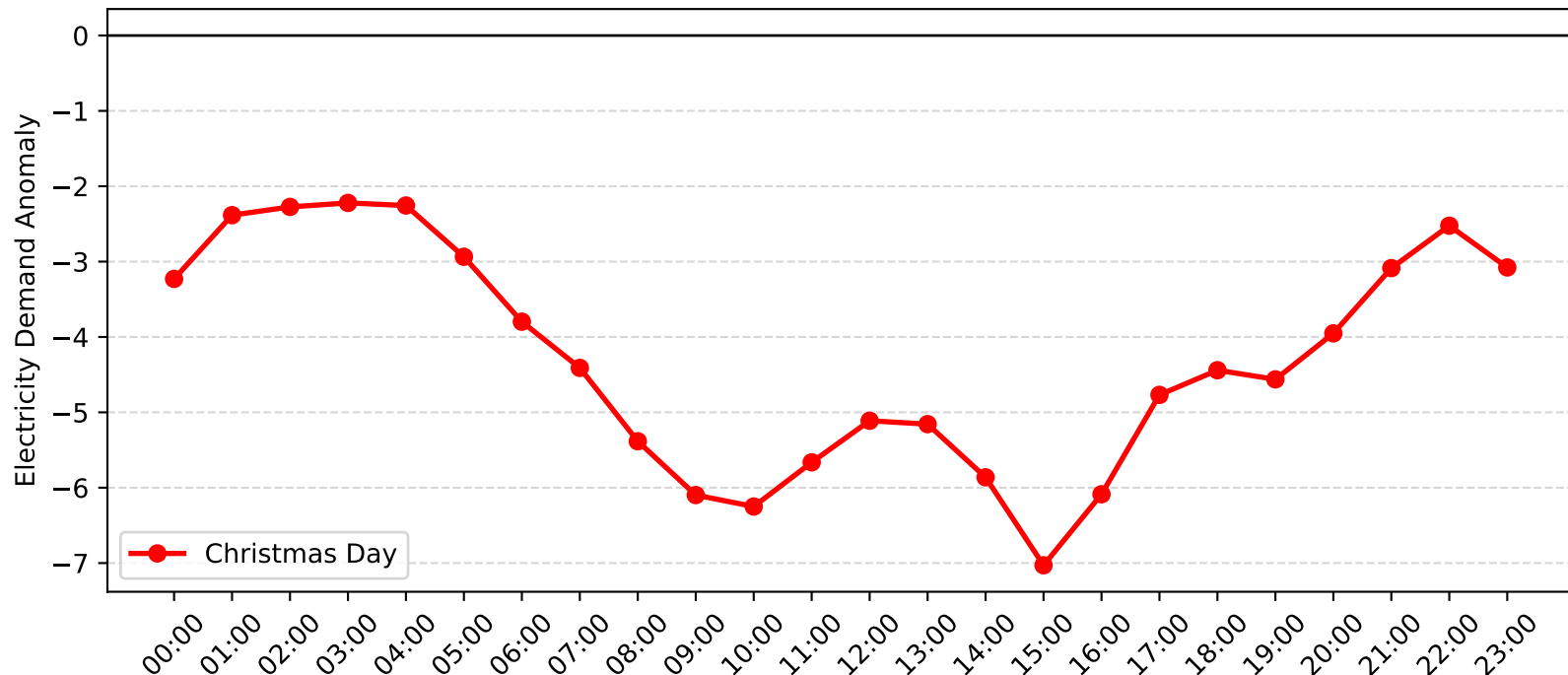
Rutherford Demand Anomaly: Christmas Day (2016-2017)
