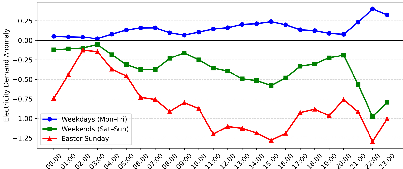
Muswellbrook Demand Anomaly: Easter Sunday vs Weekday/Weekend (2017-2018)
