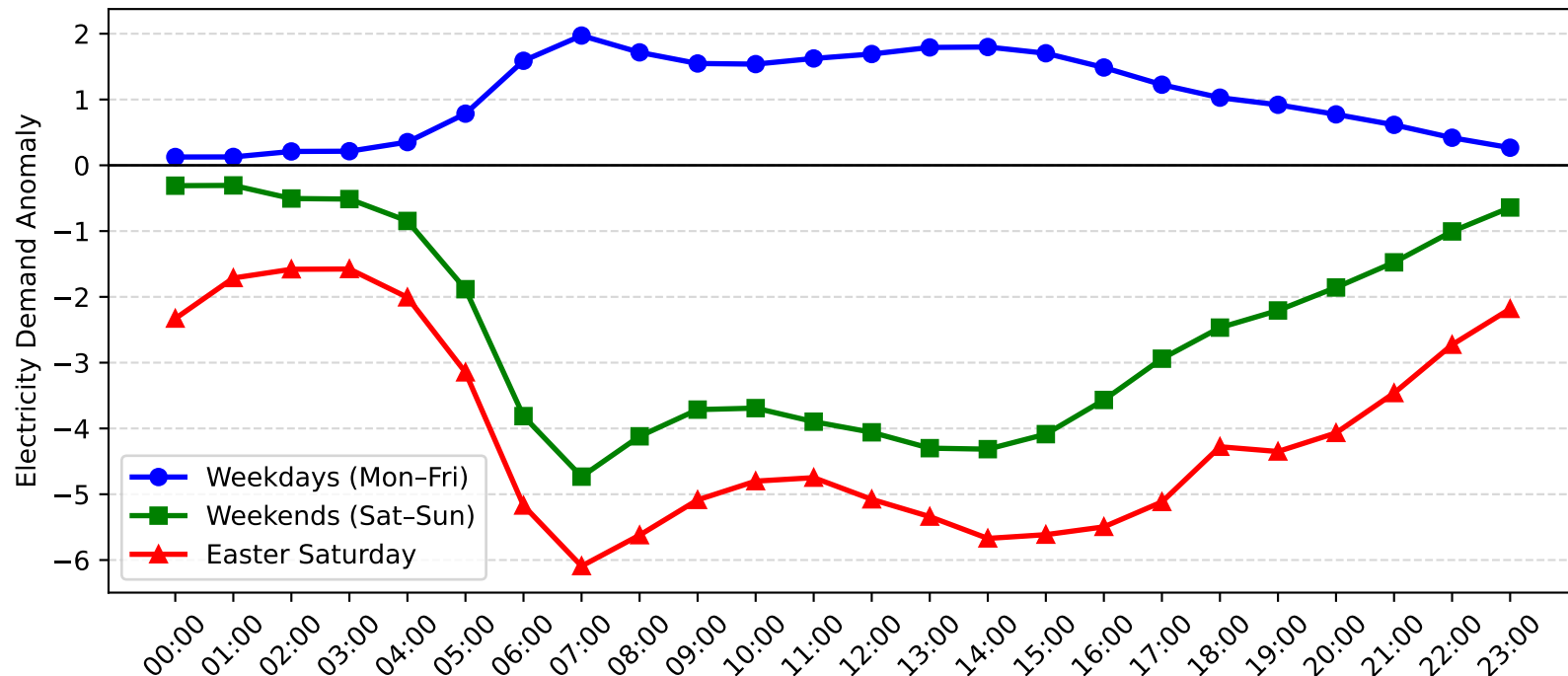
Sefton Demand Anomaly: Easter Saturday vs Weekday/Weekend (2014-2015)
