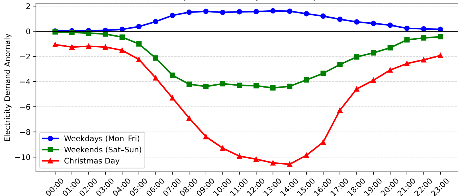
Auburn Demand Anomaly: Christmas Day vs Weekday/Weekend (2012-2013)
