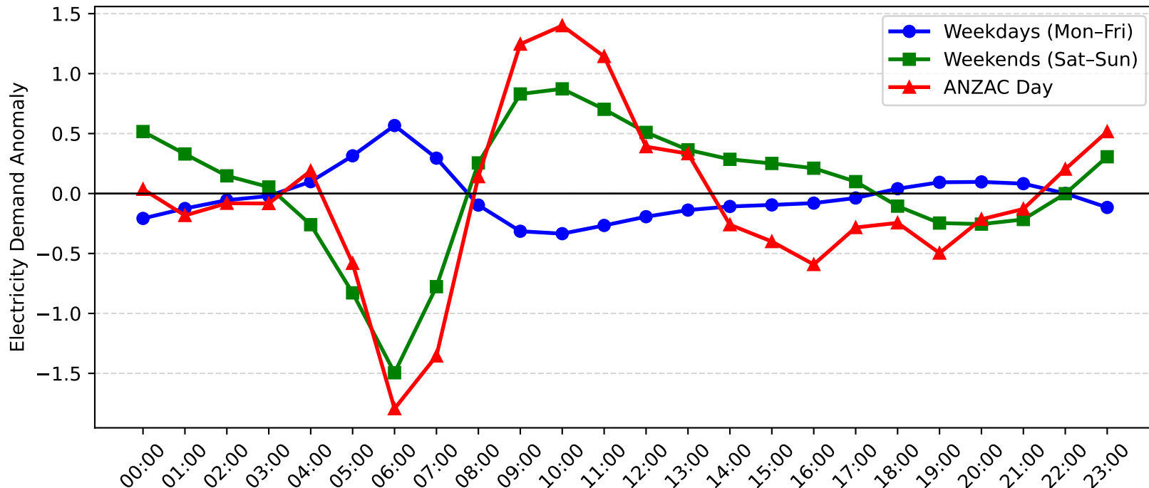
Umina Demand Anomaly: ANZAC Day vs Weekday/Weekend (2013-2014)
