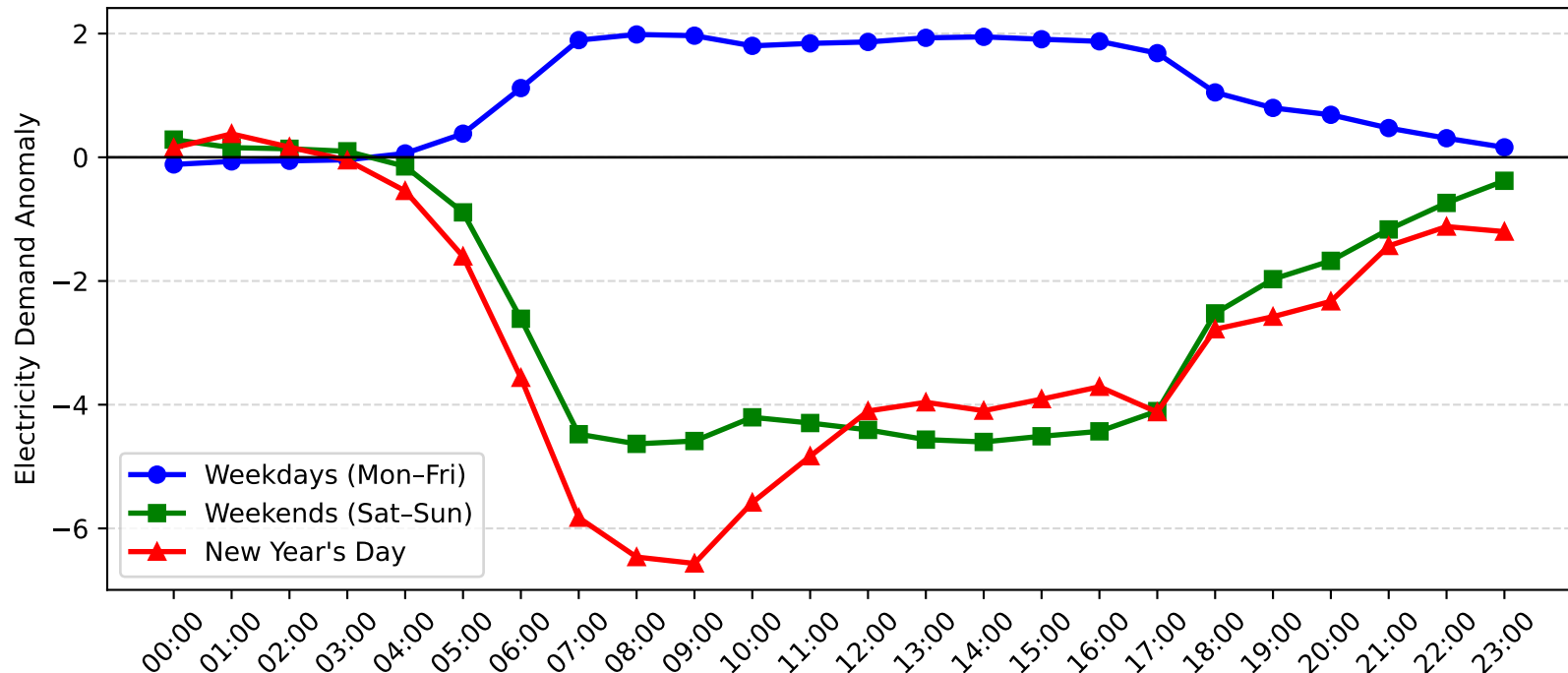
Top Ryde Demand Anomaly: New Year's Day vs Weekday/Weekend (2012-2013)
