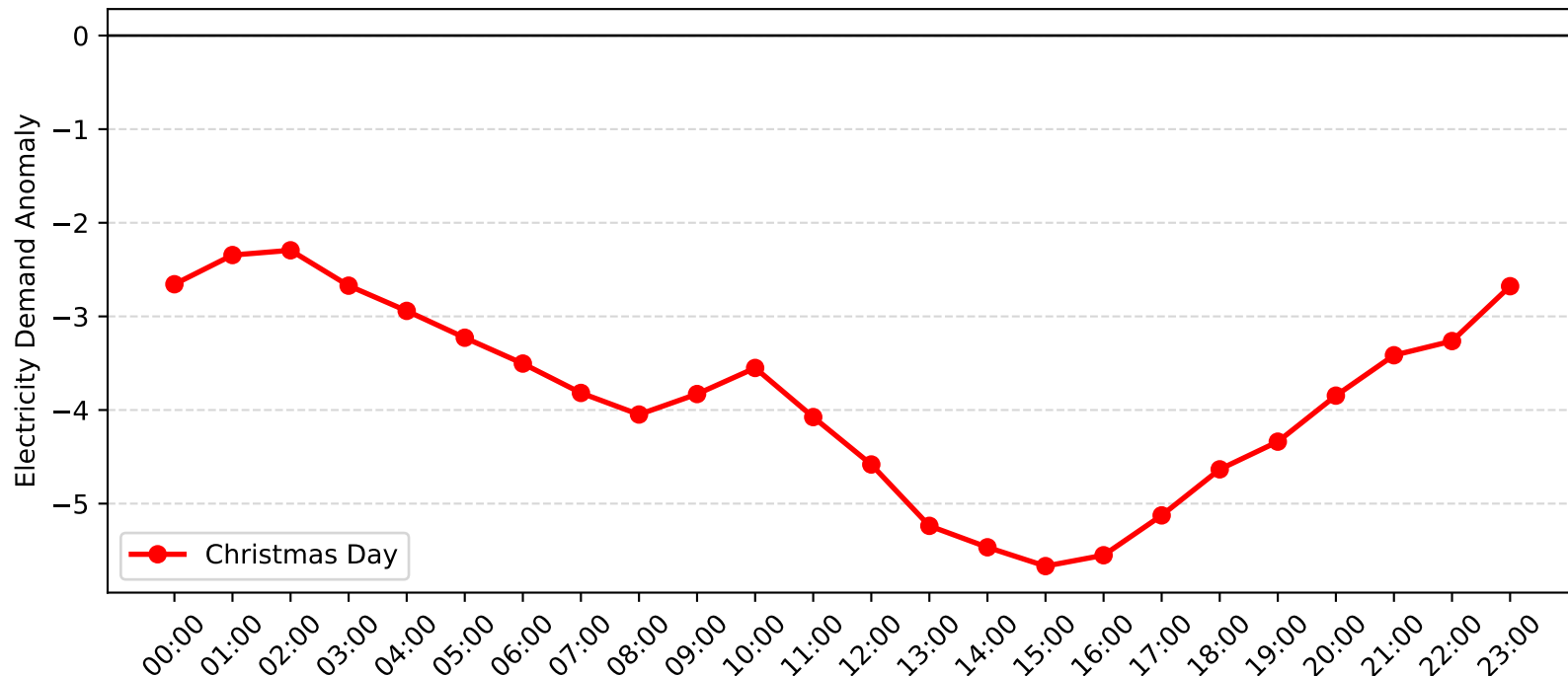
Bass Hill Demand Anomaly: Christmas Day (2015-2016)
