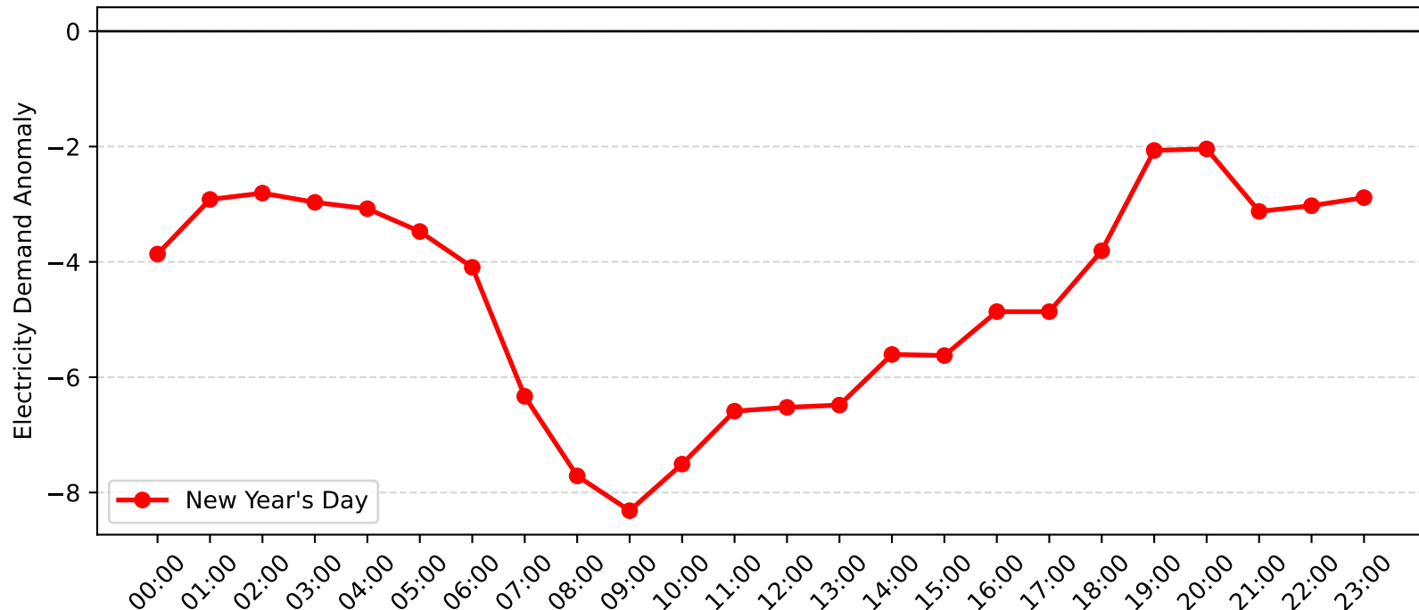
Green Square Demand Anomaly: New Year's Day (2008-2009)
