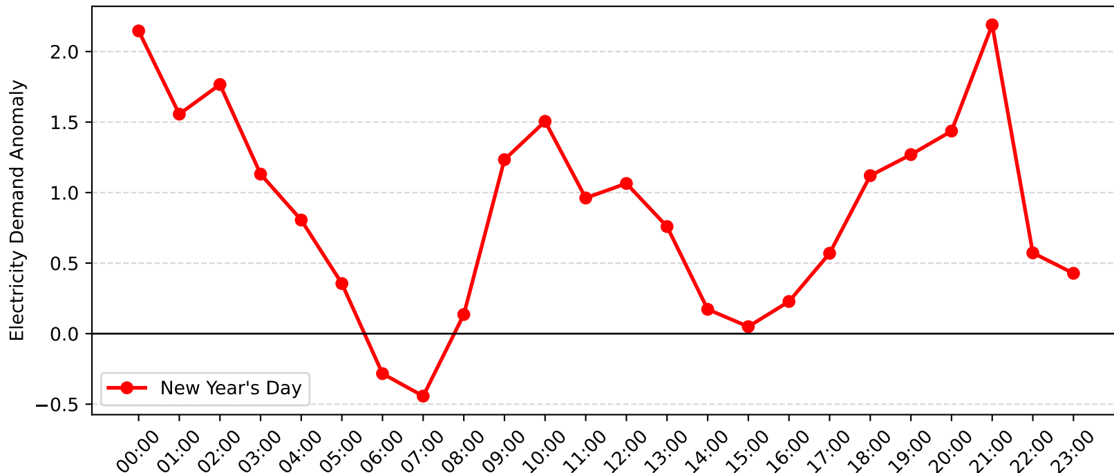
Nelson Bay Demand Anomaly: New Year's Day (2016-2017)
