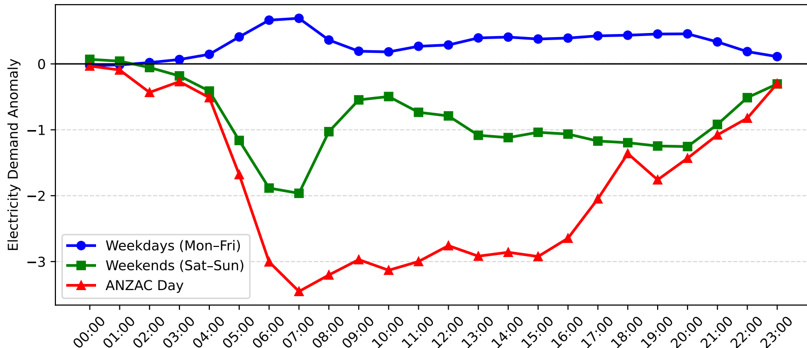
Charmhaven Demand Anomaly: ANZAC Day vs Weekday/Weekend (2012-2013)
