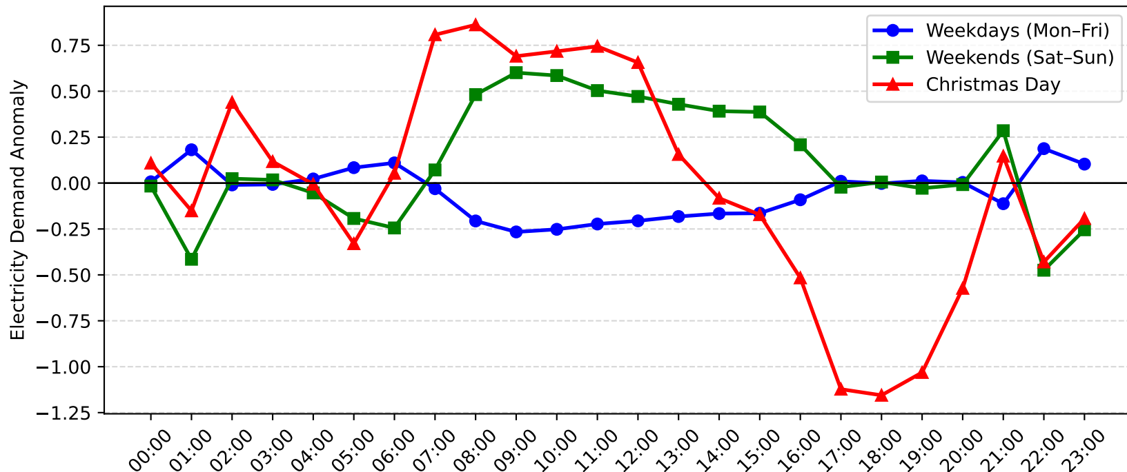
Swansea Demand Anomaly: Christmas Day vs Weekday/Weekend (2010-2011)
