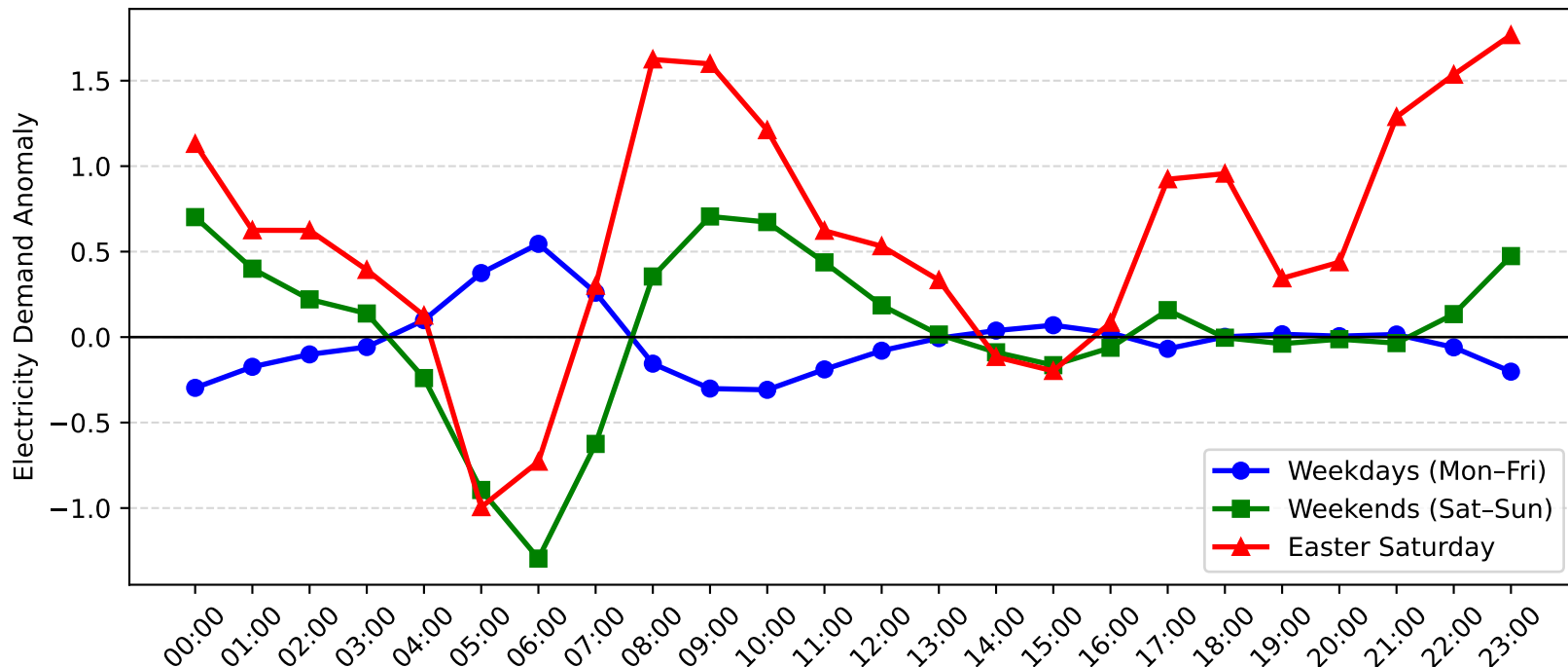
Umina Demand Anomaly: Easter Saturday vs Weekday/Weekend (2006-2007)
