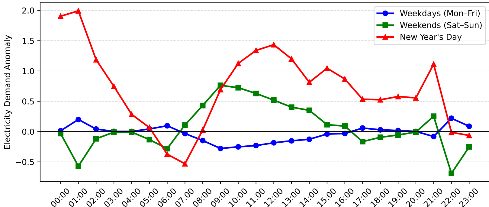
Swansea Demand Anomaly: New Year's Day vs Weekday/Weekend (2009-2010)
