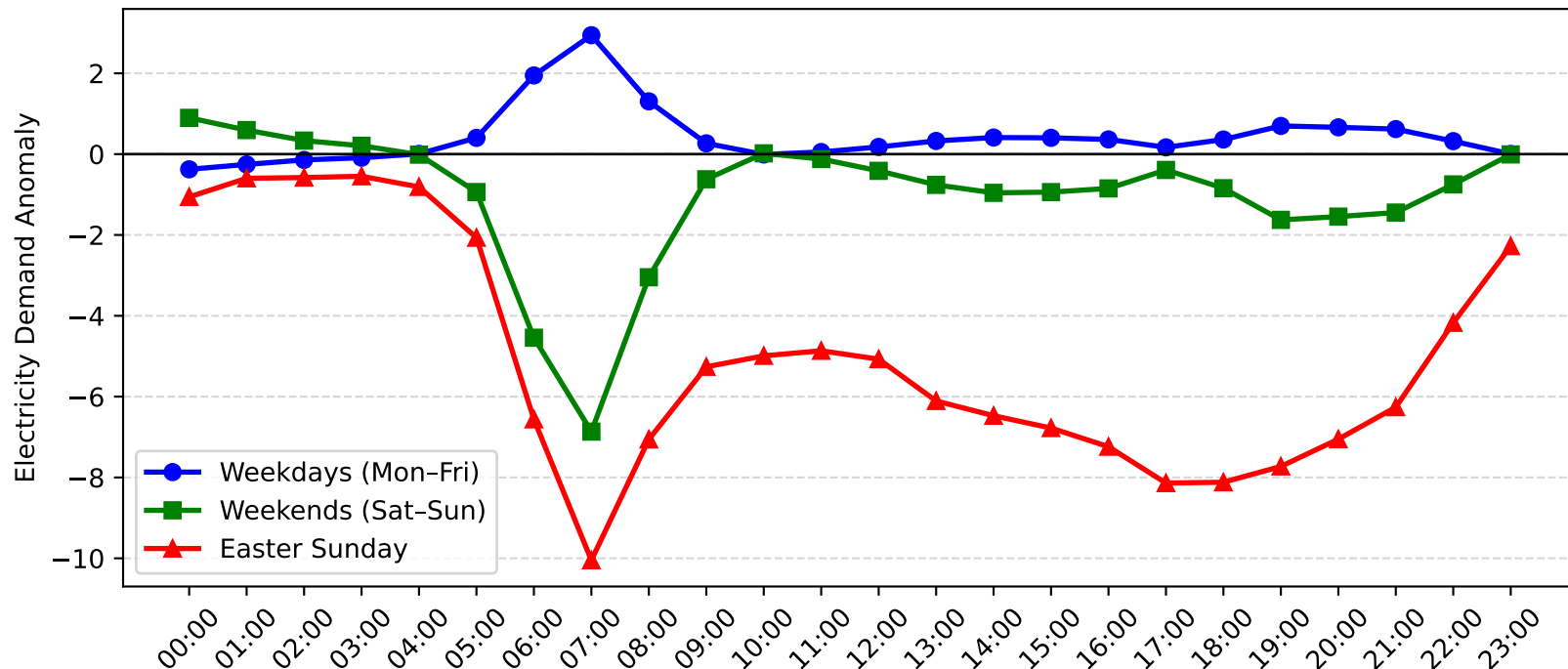
Mosman Demand Anomaly: Easter Sunday vs Weekday/Weekend (2012-2013)
