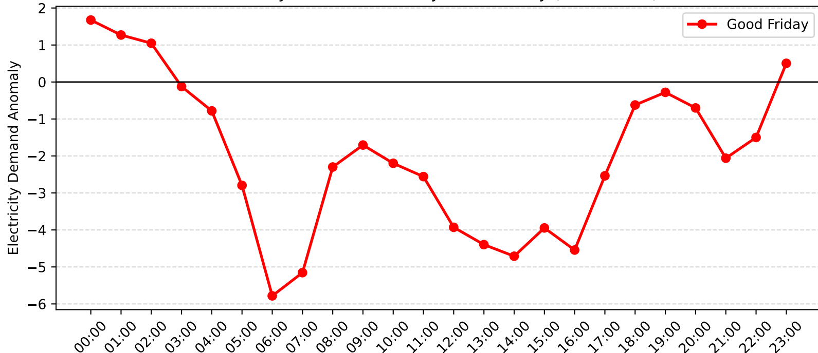
Revesby Demand Anomaly: Good Friday (2004-2005)
