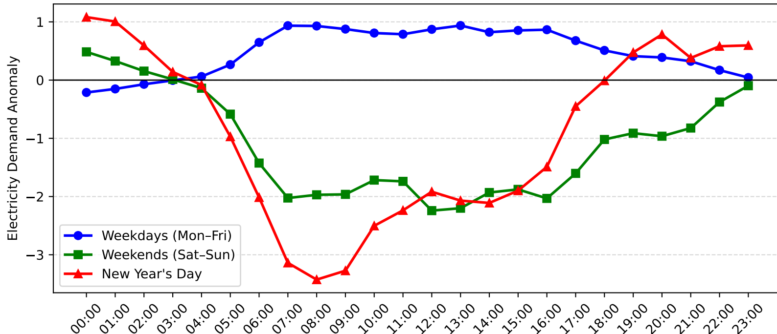
Rockdale Demand Anomaly: New Year's Day vs Weekday/Weekend (2005-2006)
