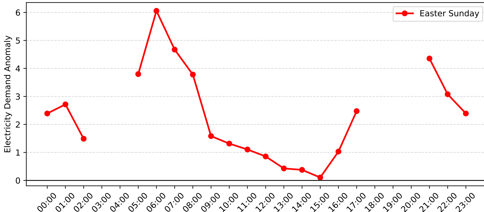
Berowra Demand Anomaly: Easter Sunday (2004-2005)
