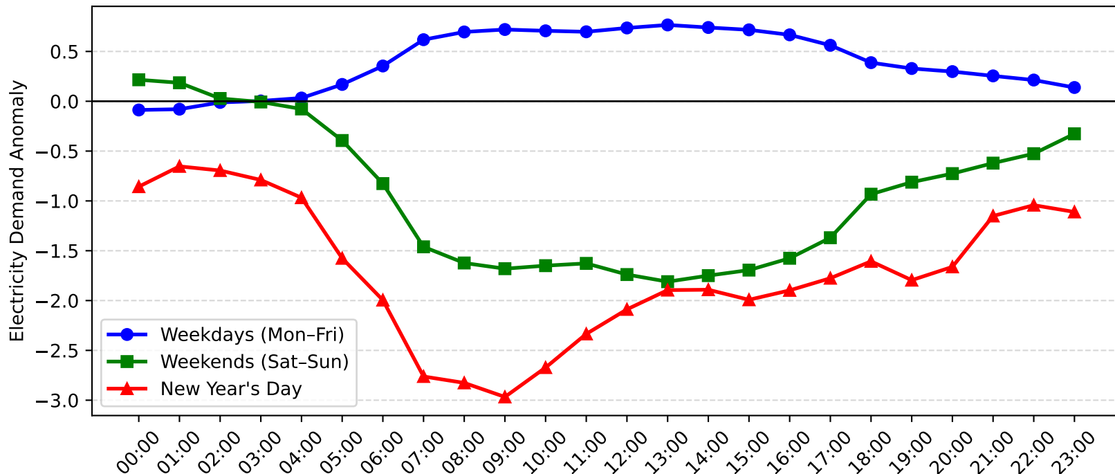
Lidcombe Demand Anomaly: New Year's Day vs Weekday/Weekend (2012-2013)
