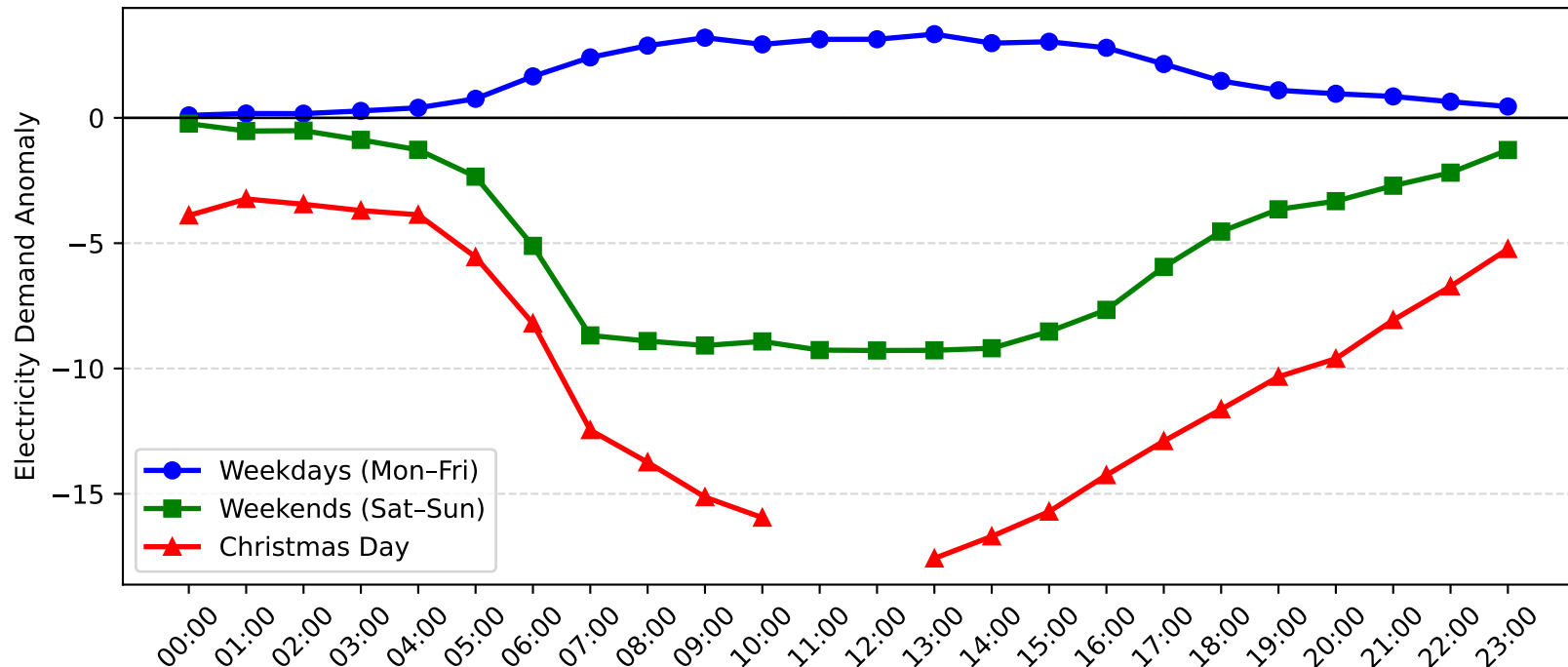
St. Peters Demand Anomaly: Christmas Day vs Weekday/Weekend (2008-2009)
