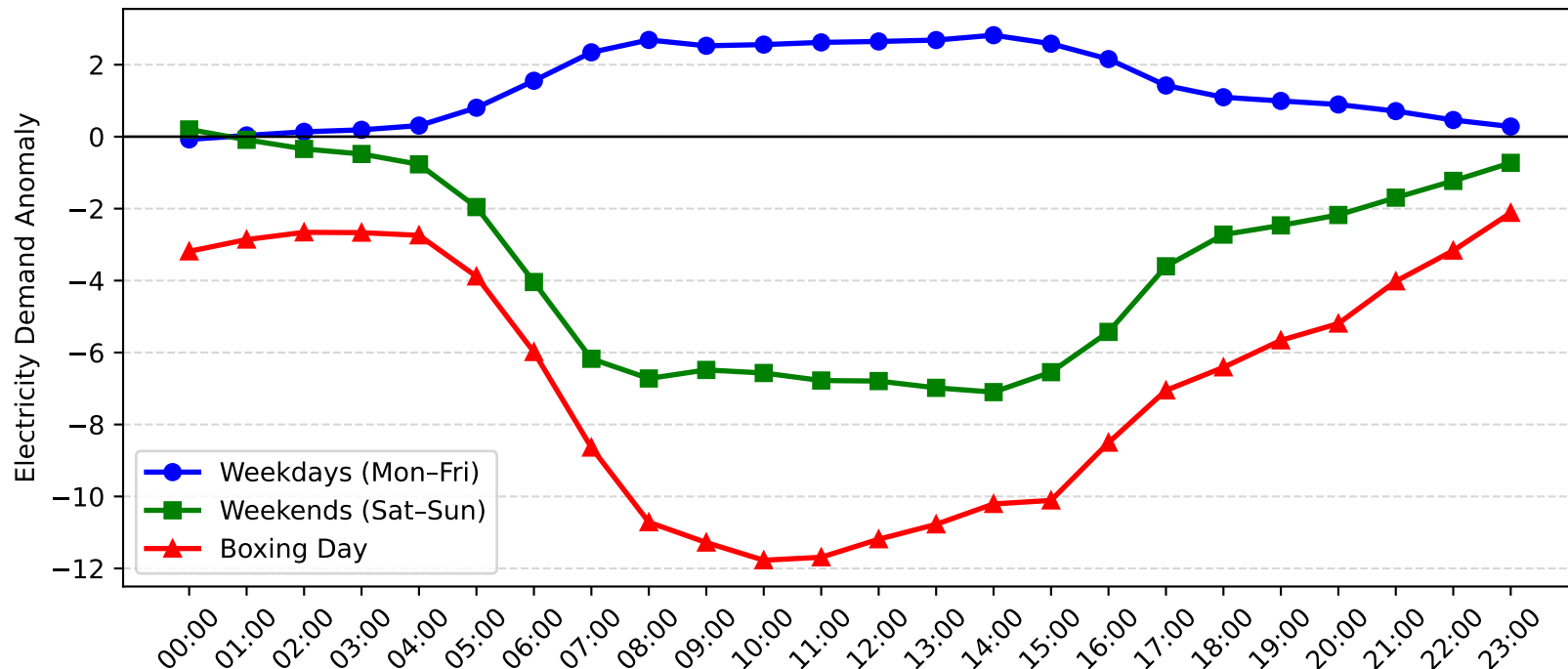
Marrickville Demand Anomaly: Boxing Day vs Weekday/Weekend (2014-2015)
