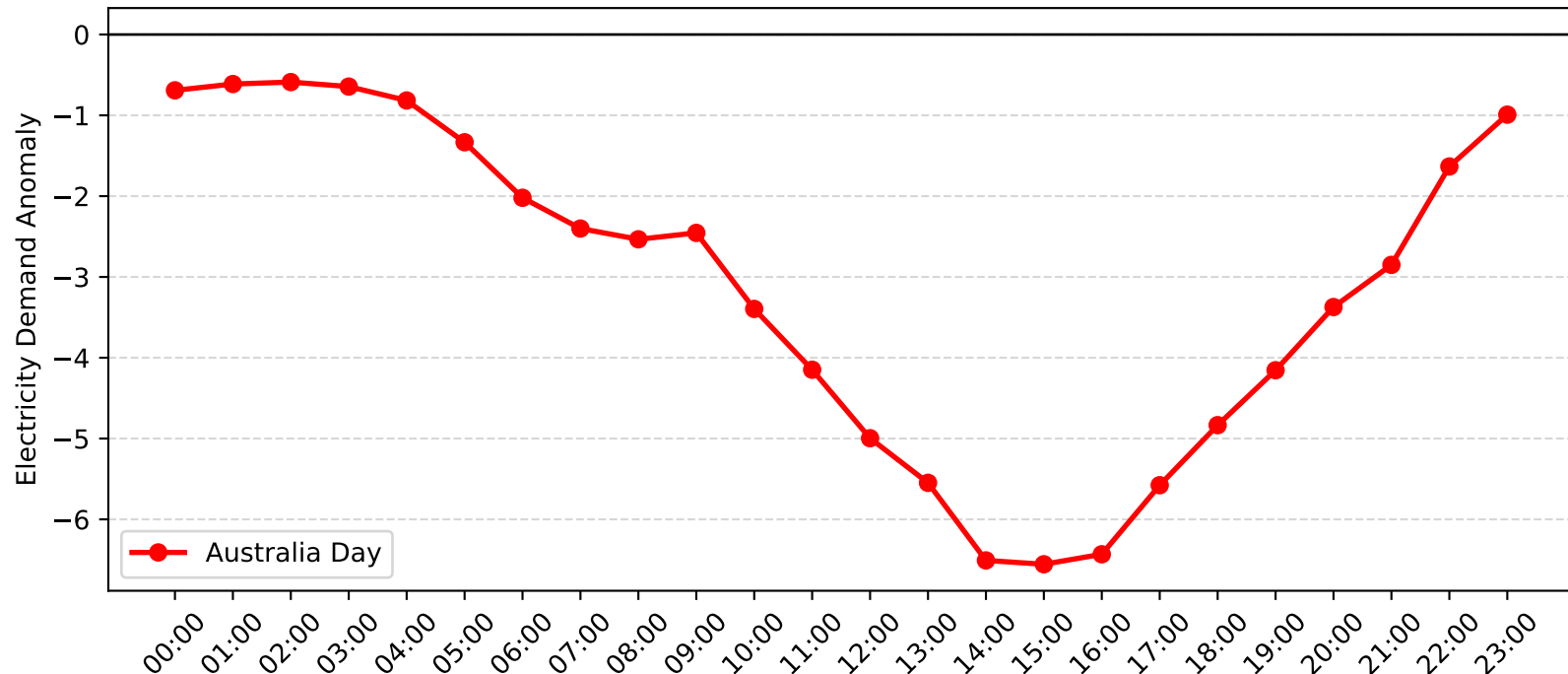
Charmhaven Demand Anomaly: Australia Day (2016-2017)
