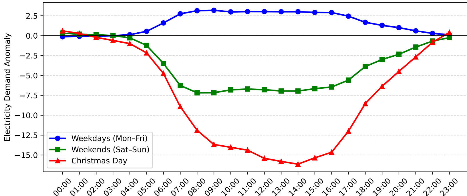
Castle Cove Demand Anomaly: Christmas Day vs Weekday/Weekend (2010-2011)
