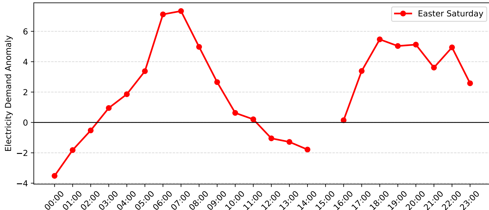
Erina Demand Anomaly: Easter Saturday (2004-2005)
