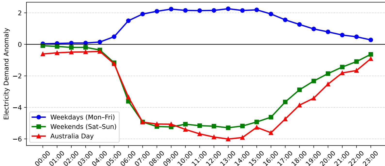
Concord Demand Anomaly: Australia Day vs Weekday/Weekend (2008-2009)
