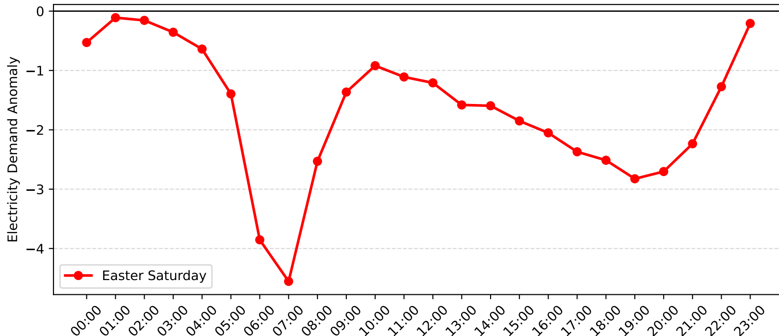
Mortdale Demand Anomaly: Easter Saturday (2014-2015)
