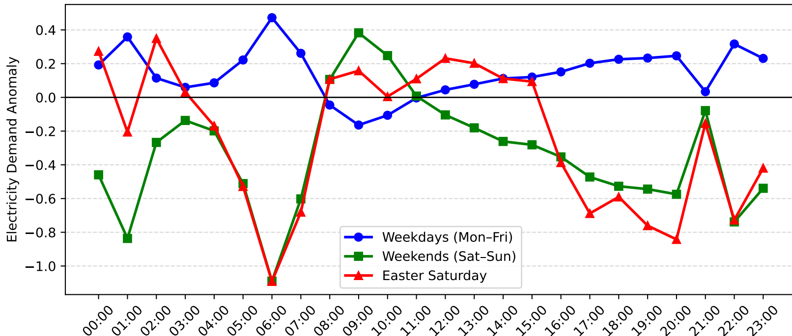
Morisset Demand Anomaly: Easter Saturday vs Weekday/Weekend (2011-2012)
