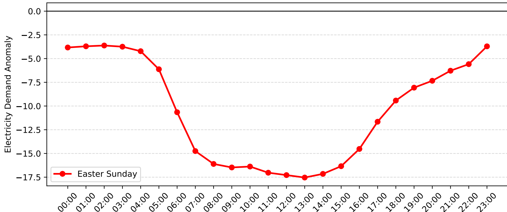
St. Peters Demand Anomaly: Easter Sunday (2007-2008)
