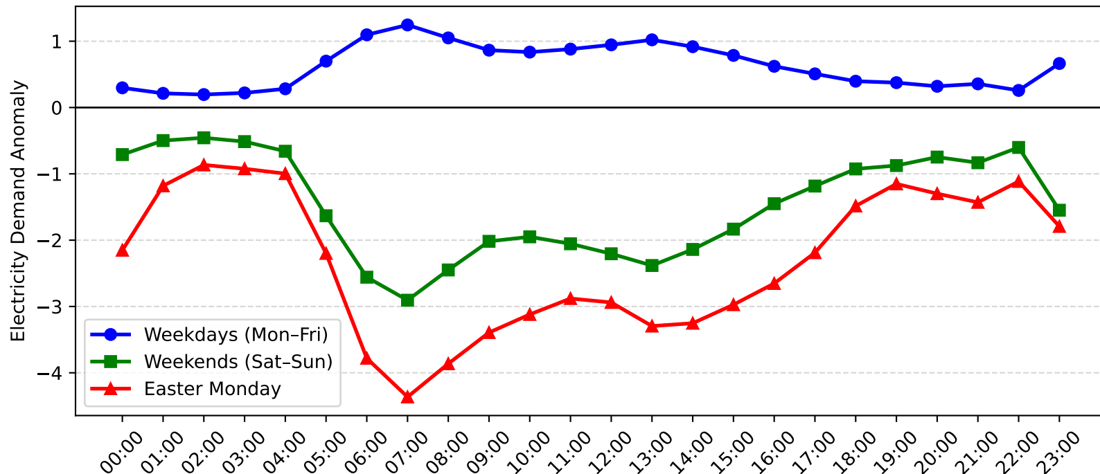
Rutherford Demand Anomaly: Easter Monday vs Weekday/Weekend (2012-2013)
