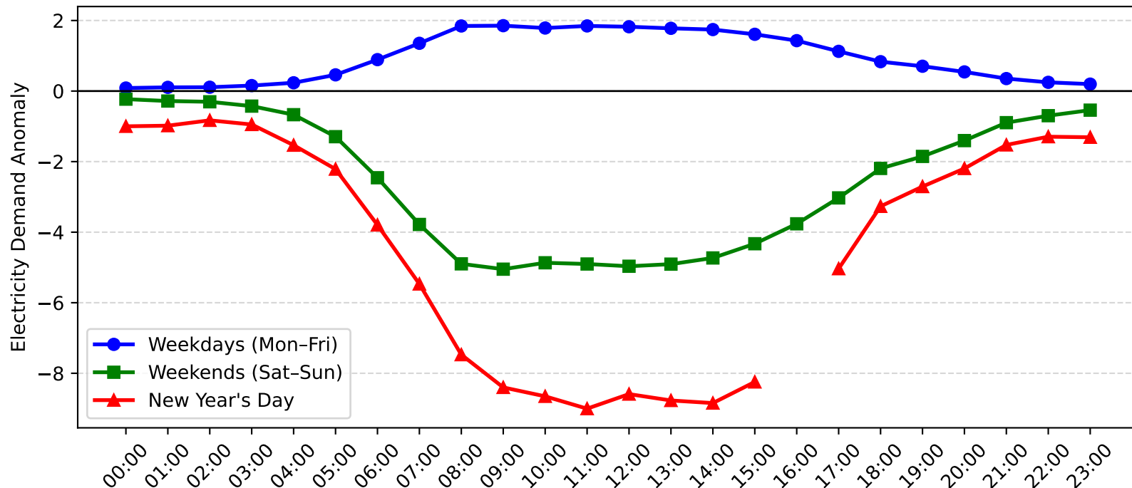
Auburn Demand Anomaly: New Year's Day vs Weekday/Weekend (2015-2016)
