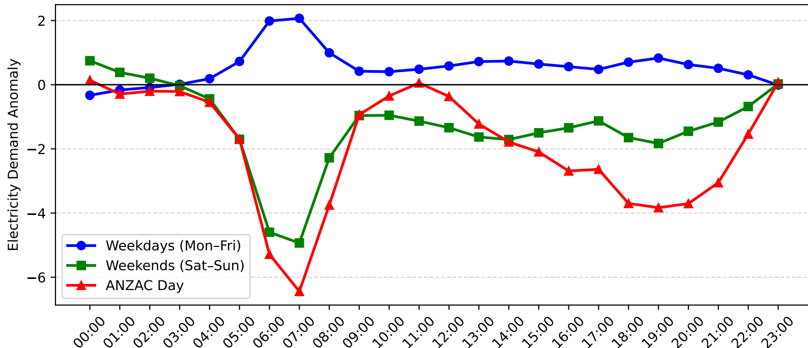
Mortdale Demand Anomaly: ANZAC Day vs Weekday/Weekend (2008-2009)
