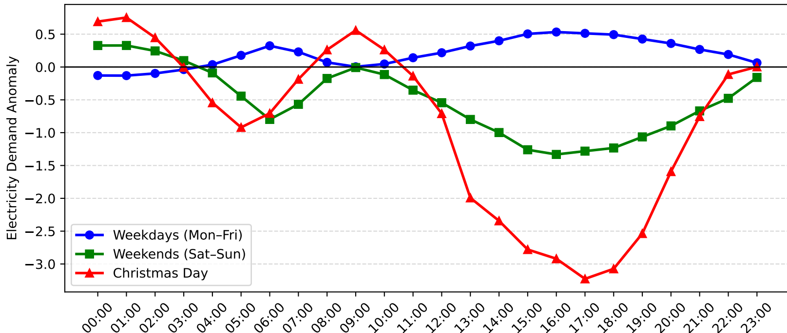
Umina Demand Anomaly: Christmas Day vs Weekday/Weekend (2015-2016)
