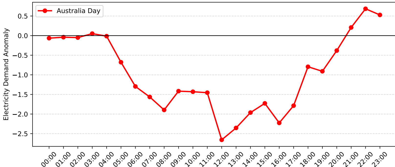
Erina Demand Anomaly: Australia Day (2007-2008)
