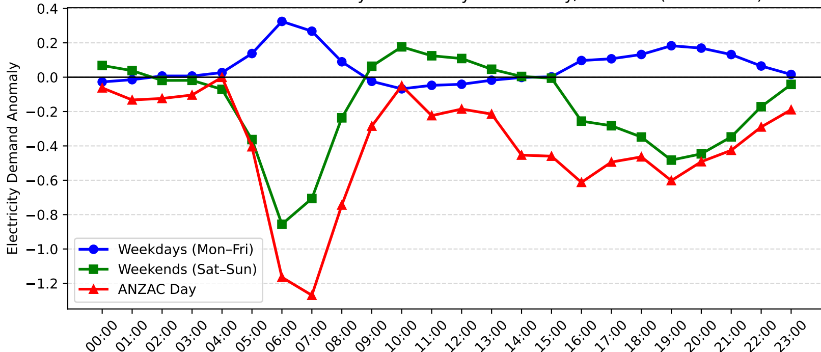
Narrabeen Demand Anomaly: ANZAC Day vs Weekday/Weekend (2013-2014)
