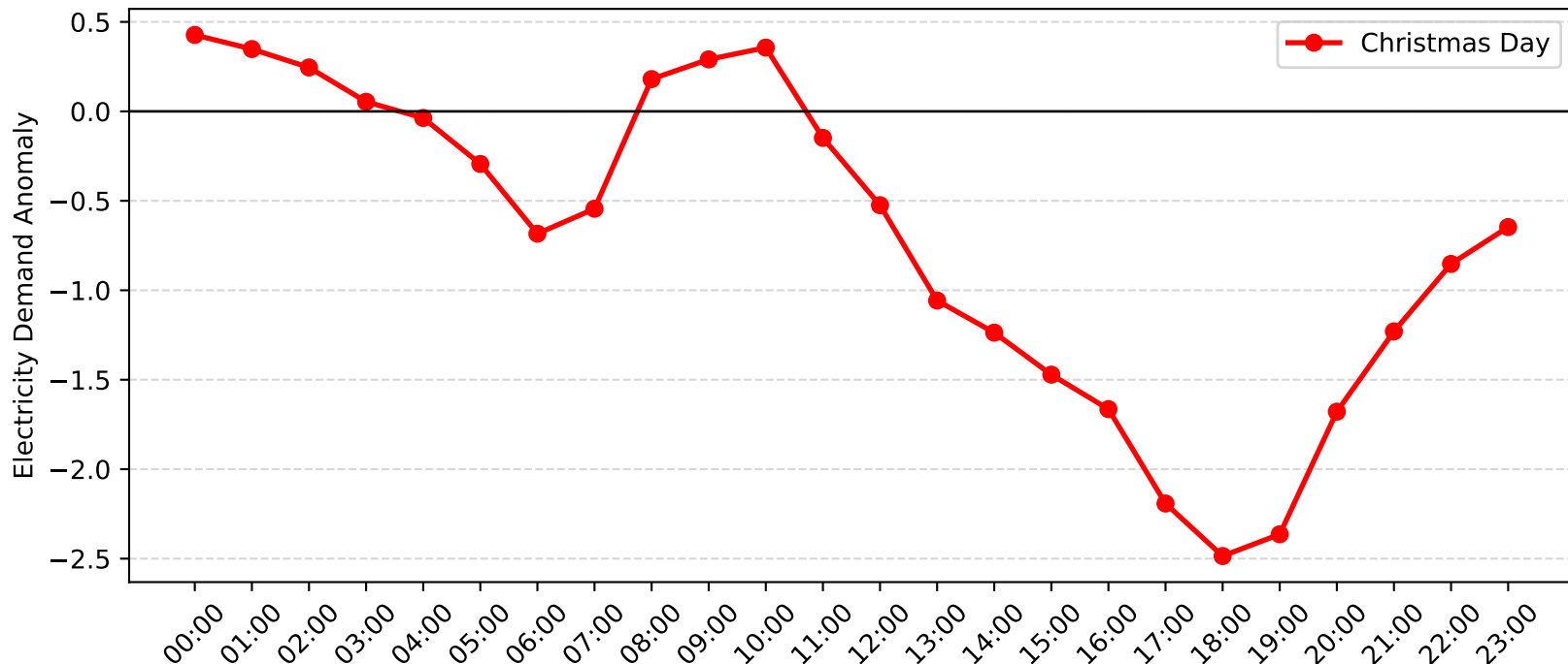
Harbord Demand Anomaly: Christmas Day (2005-2006)
