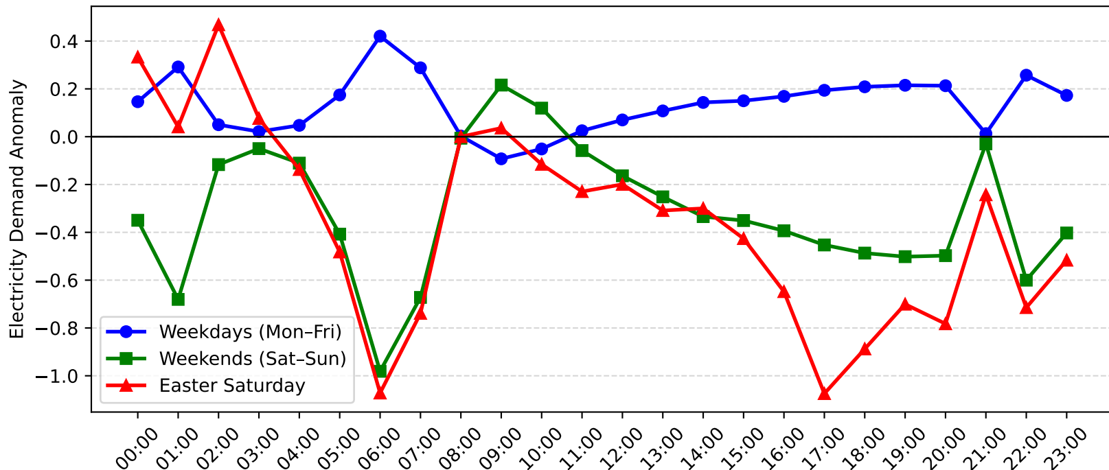
Morisset Demand Anomaly: Easter Saturday vs Weekday/Weekend (2012-2013)
