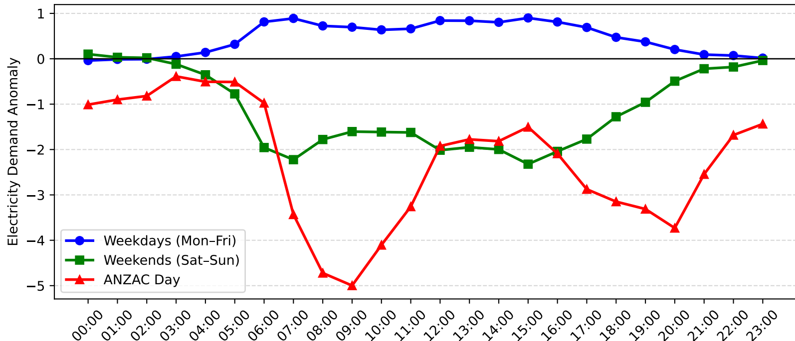
Epping Demand Anomaly: ANZAC Day vs Weekday/Weekend (2004-2005)
