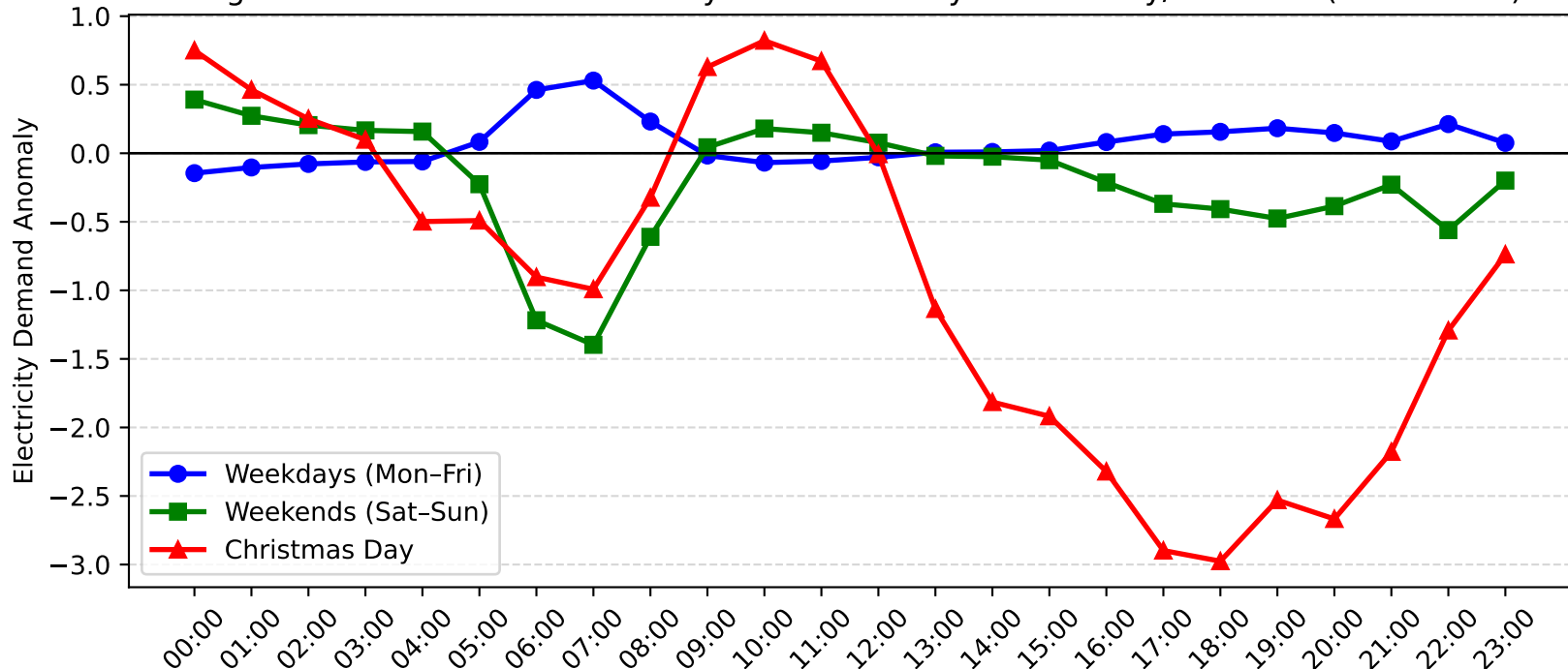
Balgowlah North Demand Anomaly: Christmas Day vs Weekday/Weekend (2012-2013)
