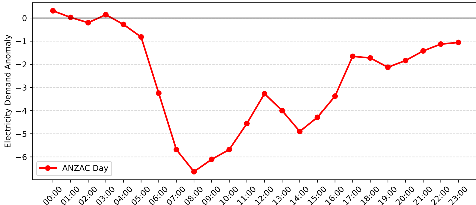
Zetland Demand Anomaly: ANZAC Day (2017-2018)
