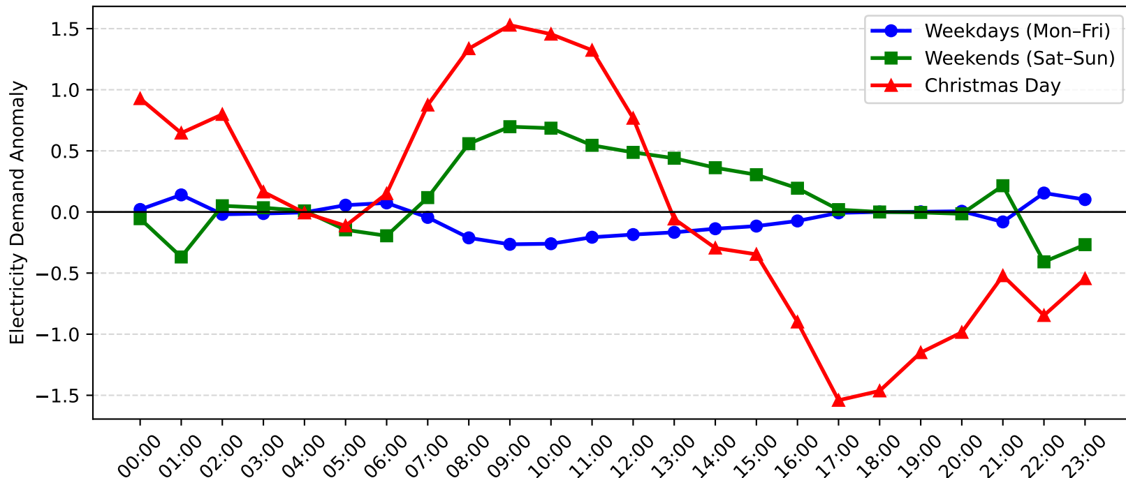
Swansea Demand Anomaly: Christmas Day vs Weekday/Weekend (2012-2013)
