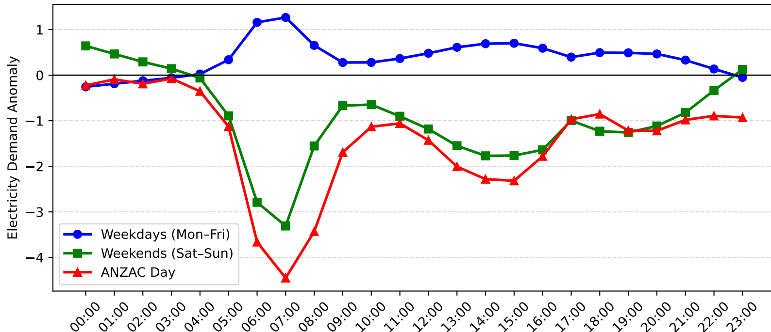
Five Dock Demand Anomaly: ANZAC Day vs Weekday/Weekend (2005-2006)
