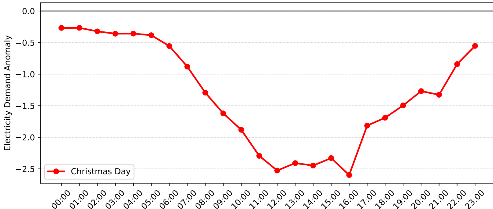
Rothbury Demand Anomaly: Christmas Day (2007-2008)
