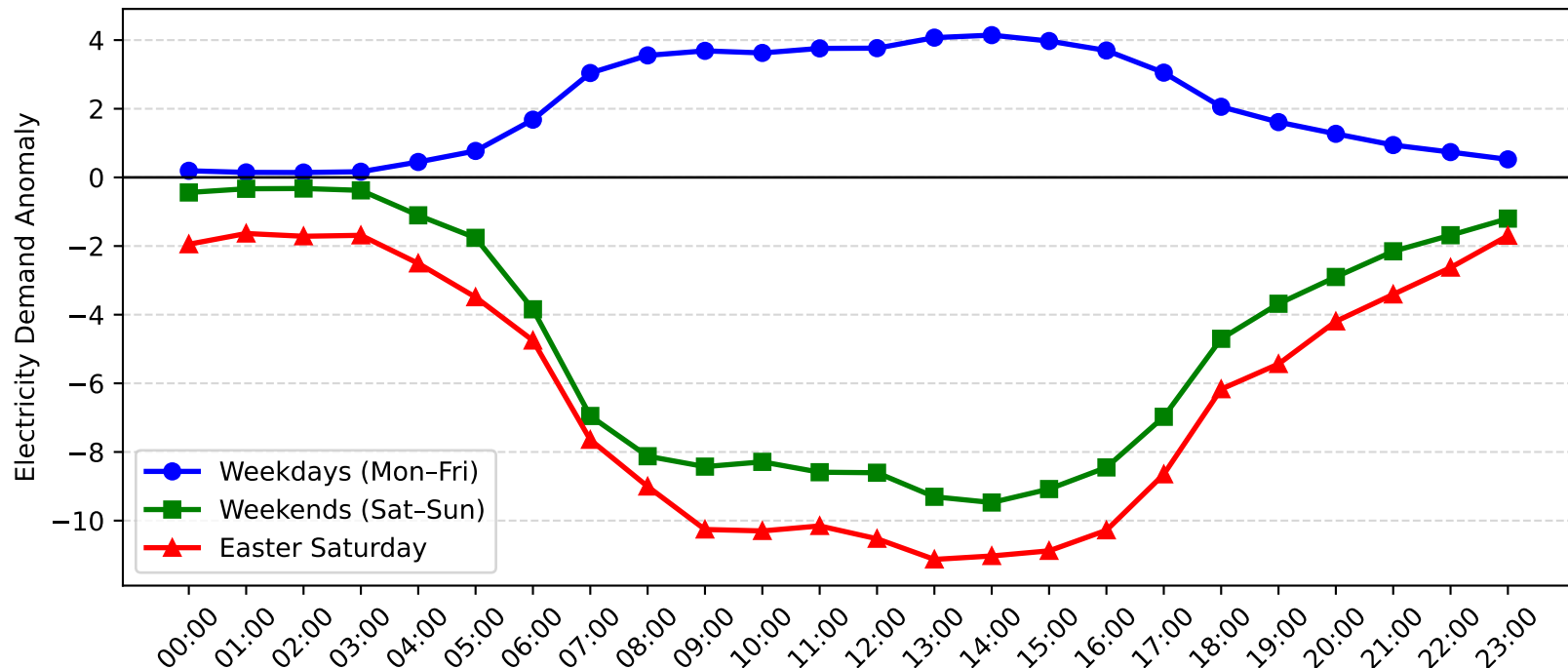
Gore Hill Demand Anomaly: Easter Saturday vs Weekday/Weekend (2017-2018)
