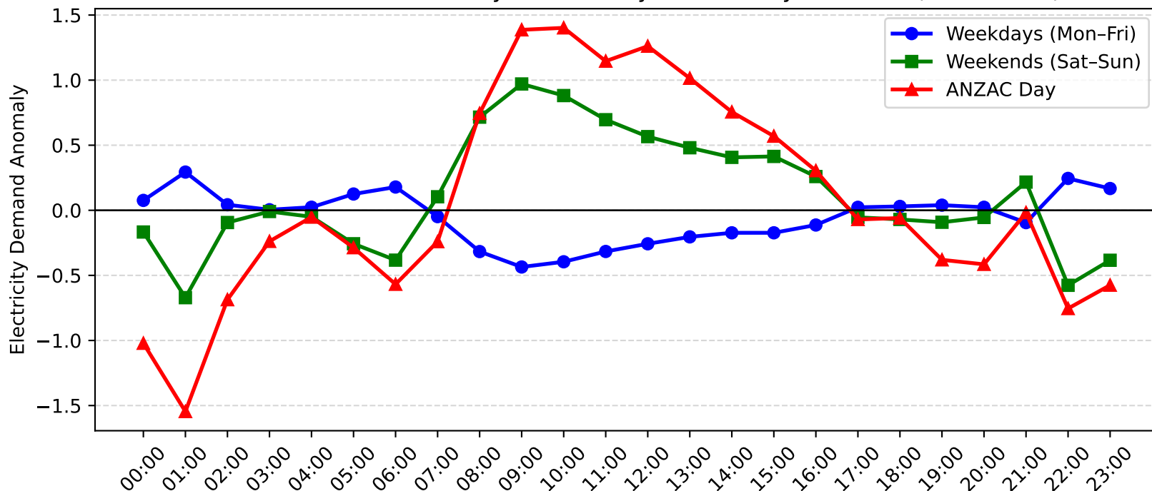
Swansea Demand Anomaly: ANZAC Day vs Weekday/Weekend (2010-2011)
