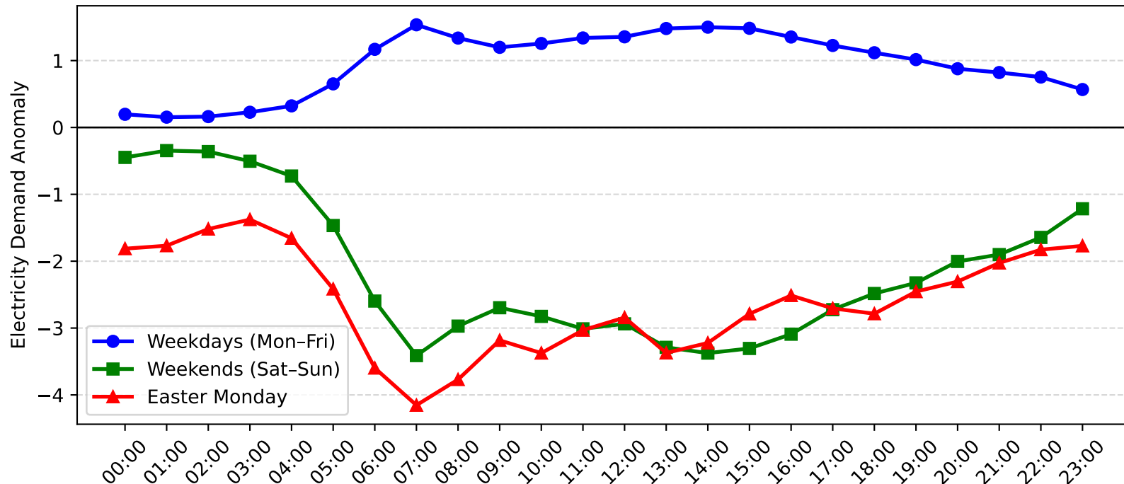
Bass Hill Demand Anomaly: Easter Monday vs Weekday/Weekend (2008-2009)
