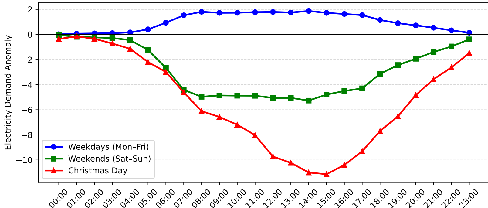
Top Ryde Demand Anomaly: Christmas Day vs Weekday/Weekend (2014-2015)
