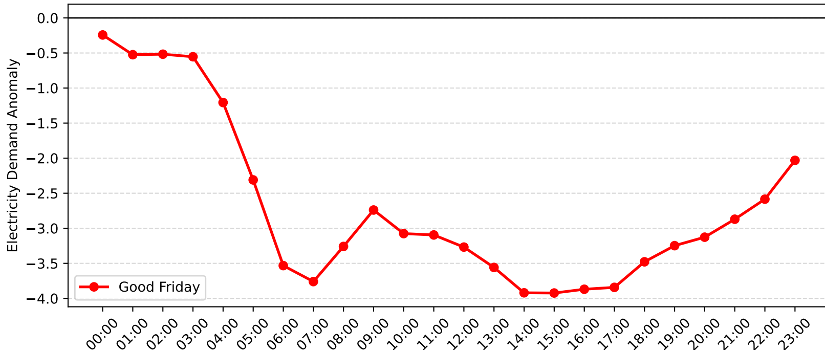
Lisarow Demand Anomaly: Good Friday (2016-2017)
