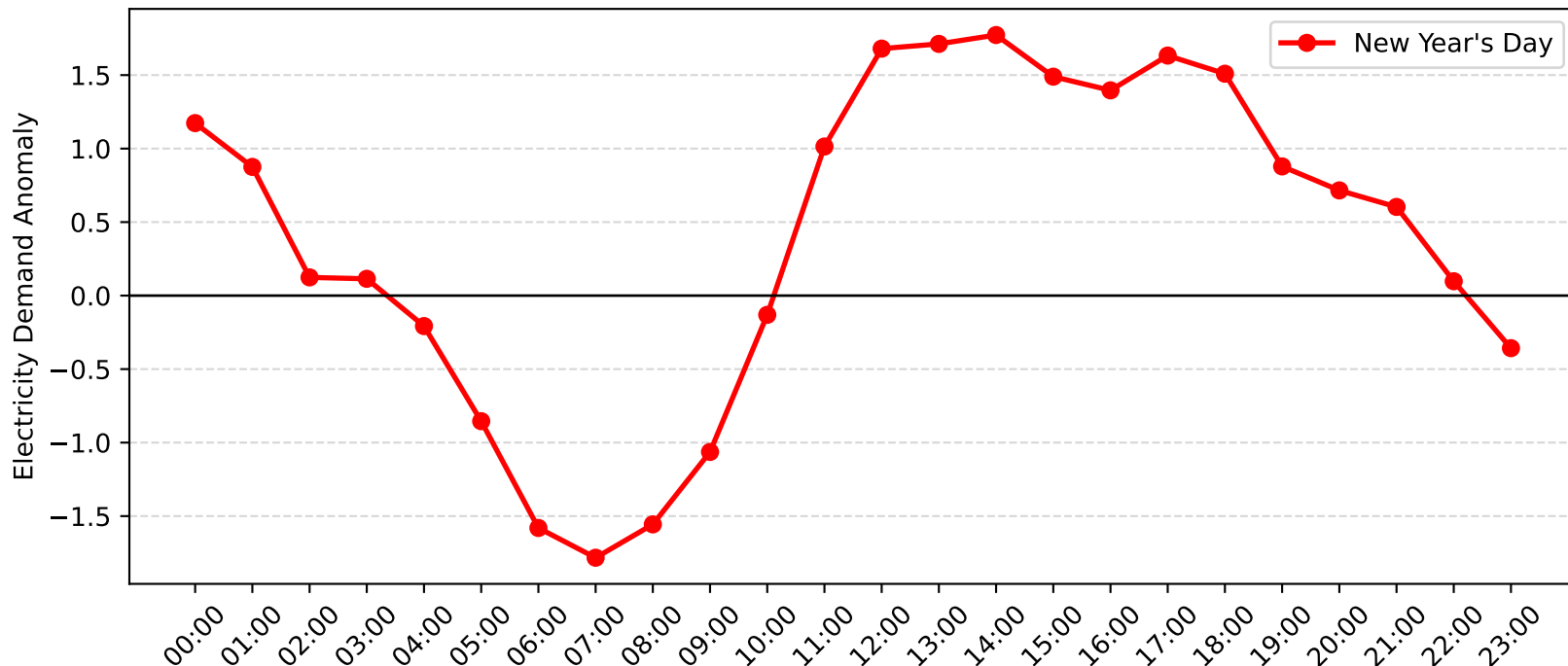
Woy Woy Demand Anomaly: New Year's Day (2011-2012)
