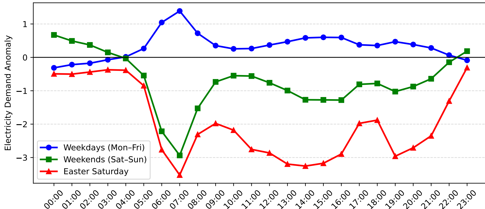
Five Dock Demand Anomaly: Easter Saturday vs Weekday/Weekend (2009-2010)
