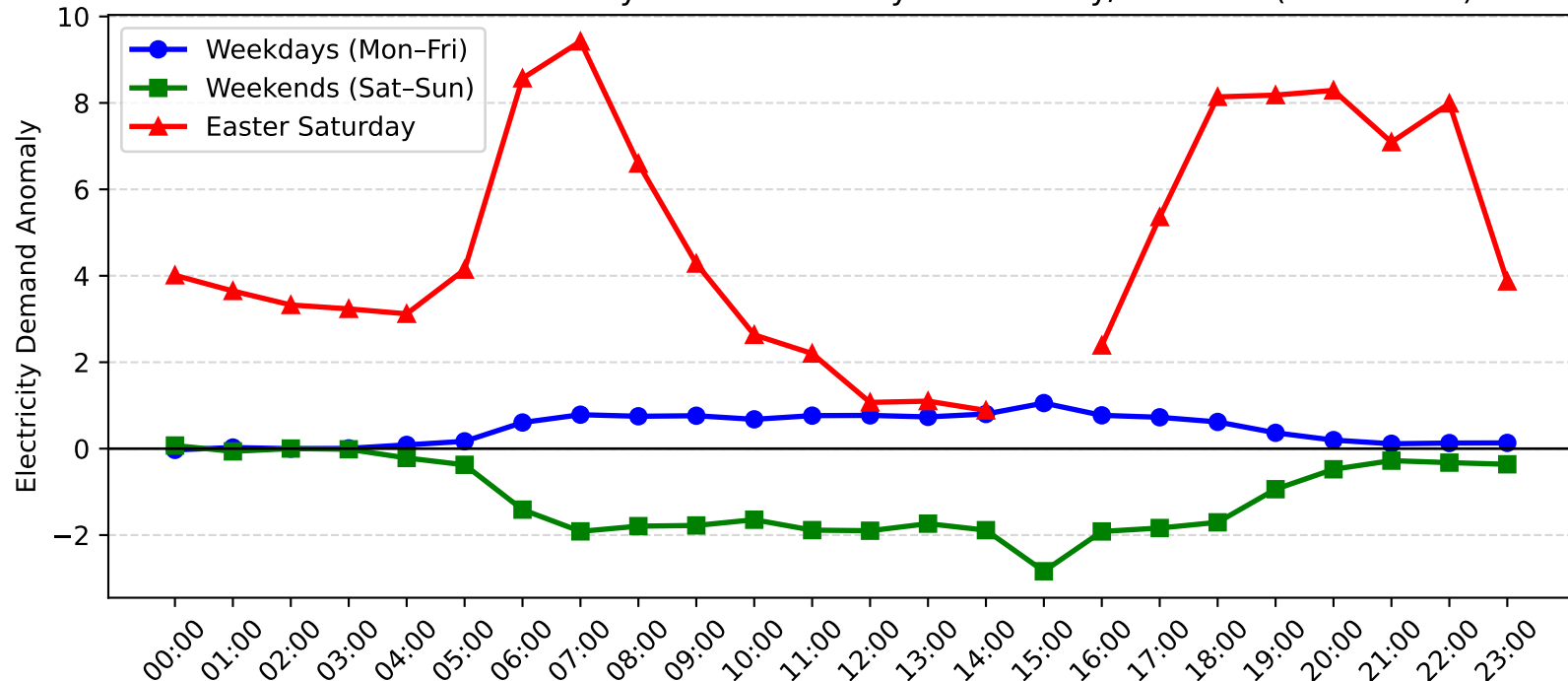
Burwood Demand Anomaly: Easter Saturday vs Weekday/Weekend (2004-2005)
