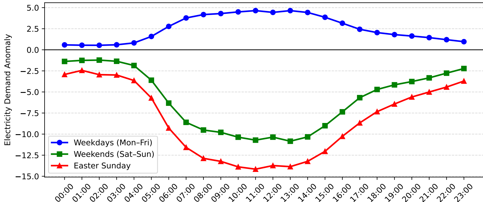
Milperra Demand Anomaly: Easter Sunday vs Weekday/Weekend (2015-2016)
