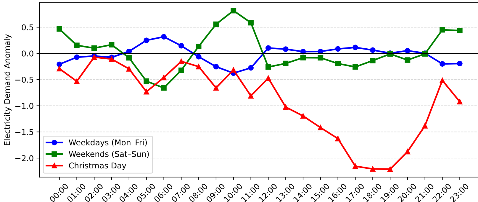
Umina Demand Anomaly: Christmas Day vs Weekday/Weekend (2004-2005)
