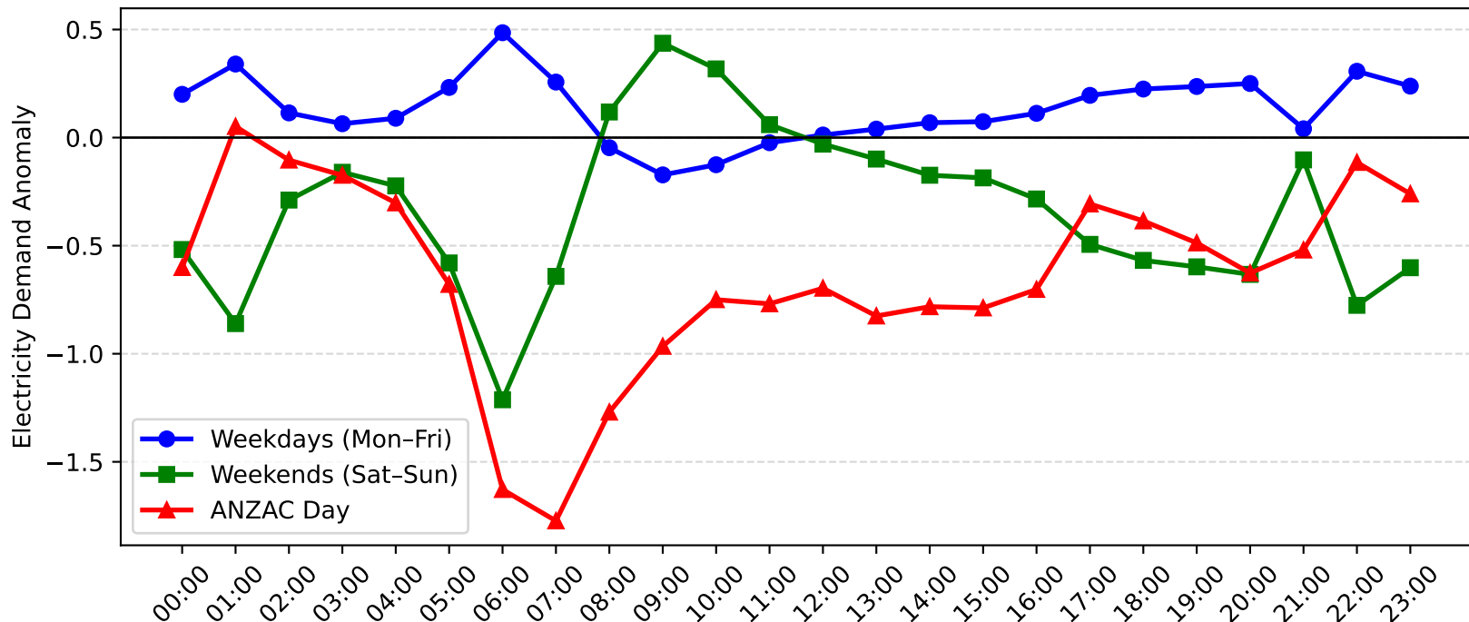
Morisset Demand Anomaly: ANZAC Day vs Weekday/Weekend (2011-2012)
