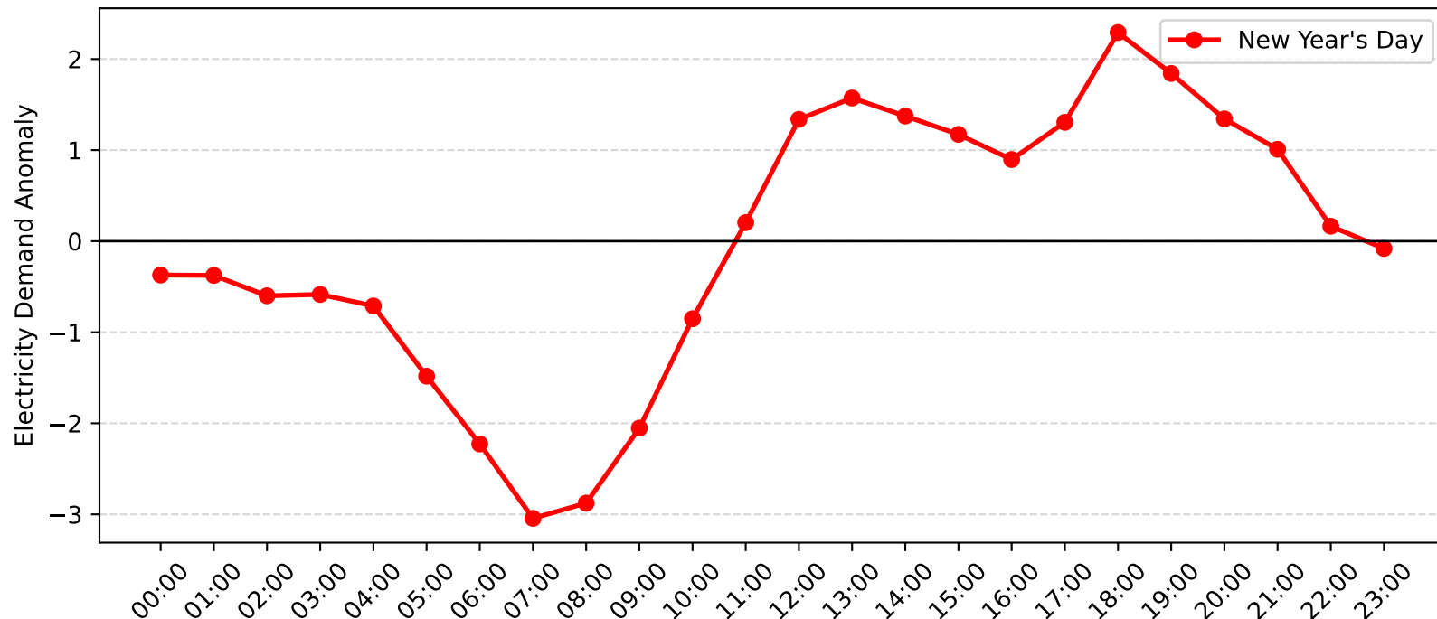
Jesmond Demand Anomaly: New Year's Day (2012-2013)
