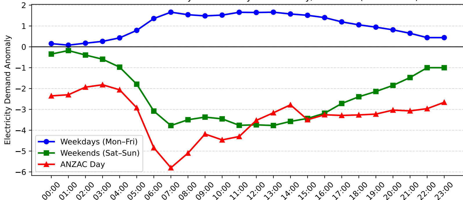
Sefton Demand Anomaly: ANZAC Day vs Weekday/Weekend (2017-2018)
