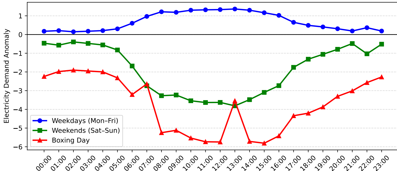
Mayfield West Demand Anomaly: Boxing Day vs Weekday/Weekend (2013-2014)
