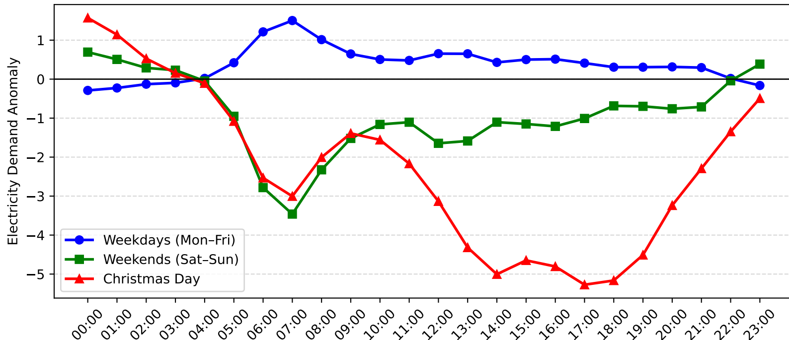
Mortdale Demand Anomaly: Christmas Day vs Weekday/Weekend (2005-2006)
