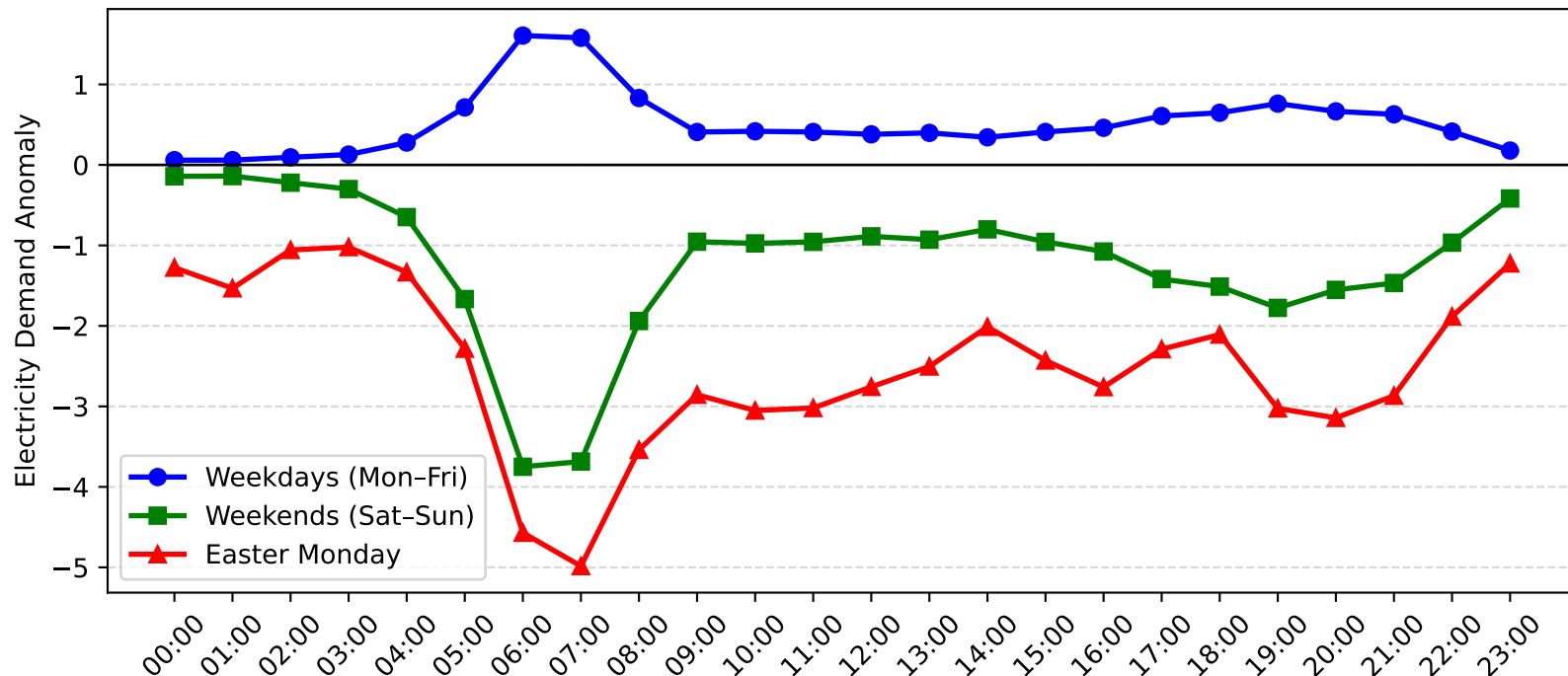
Revesby Demand Anomaly: Easter Monday vs Weekday/Weekend (2014-2015)
