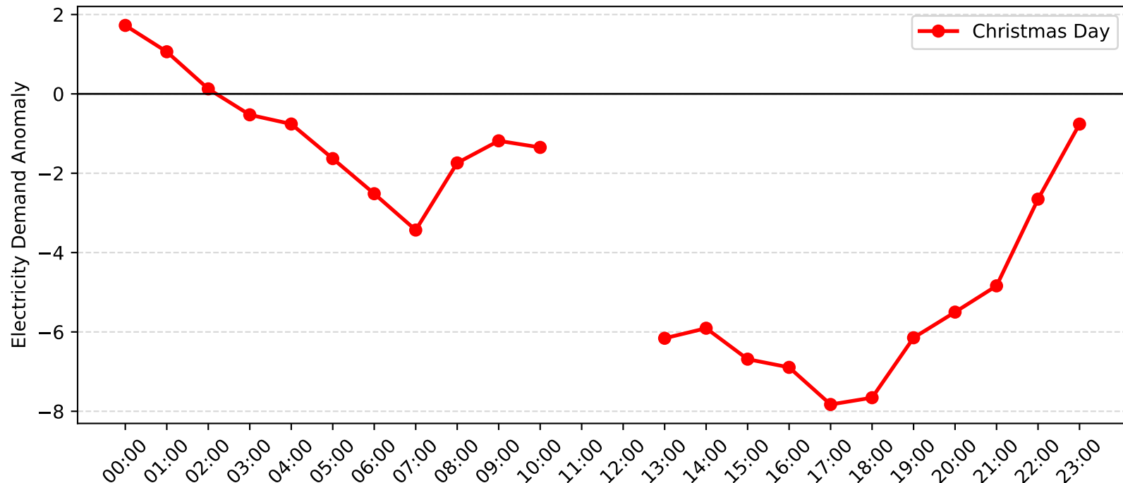
Mortdale Demand Anomaly: Christmas Day (2008-2009)
