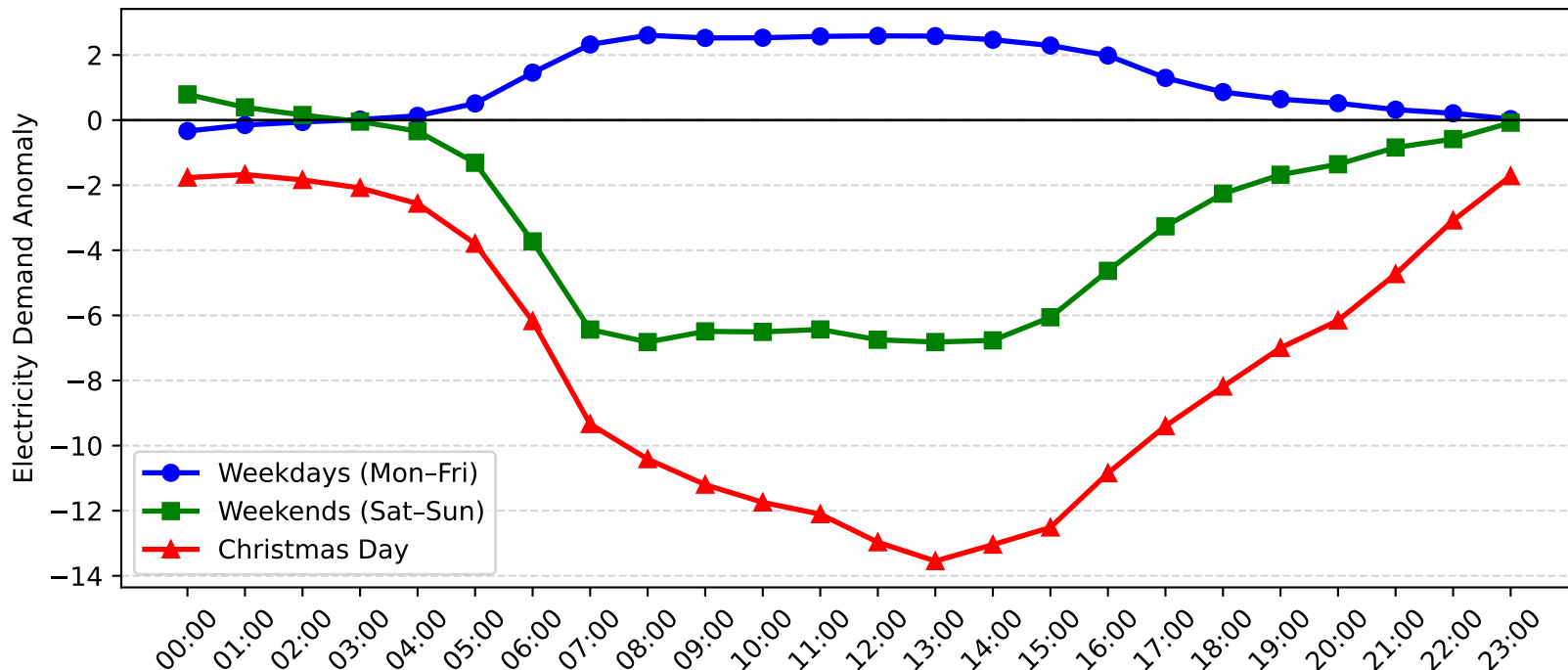
Marrickville Demand Anomaly: Christmas Day vs Weekday/Weekend (2009-2010)
