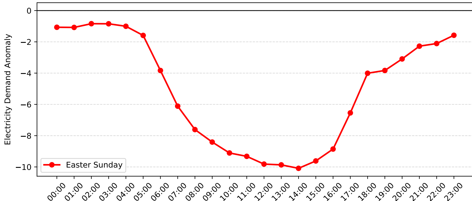
Newcastle Cbd Demand Anomaly: Easter Sunday (2009-2010)
