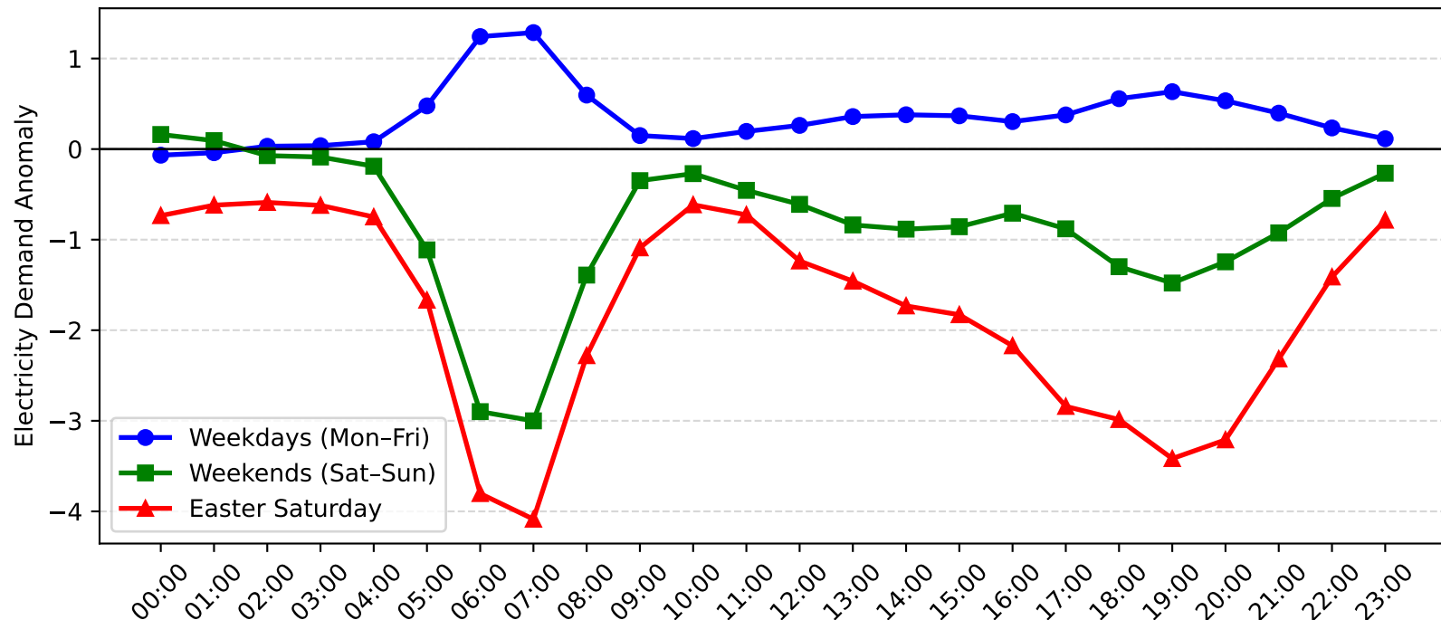
Dee Why West Demand Anomaly: Easter Saturday vs Weekday/Weekend (2014-2015)
