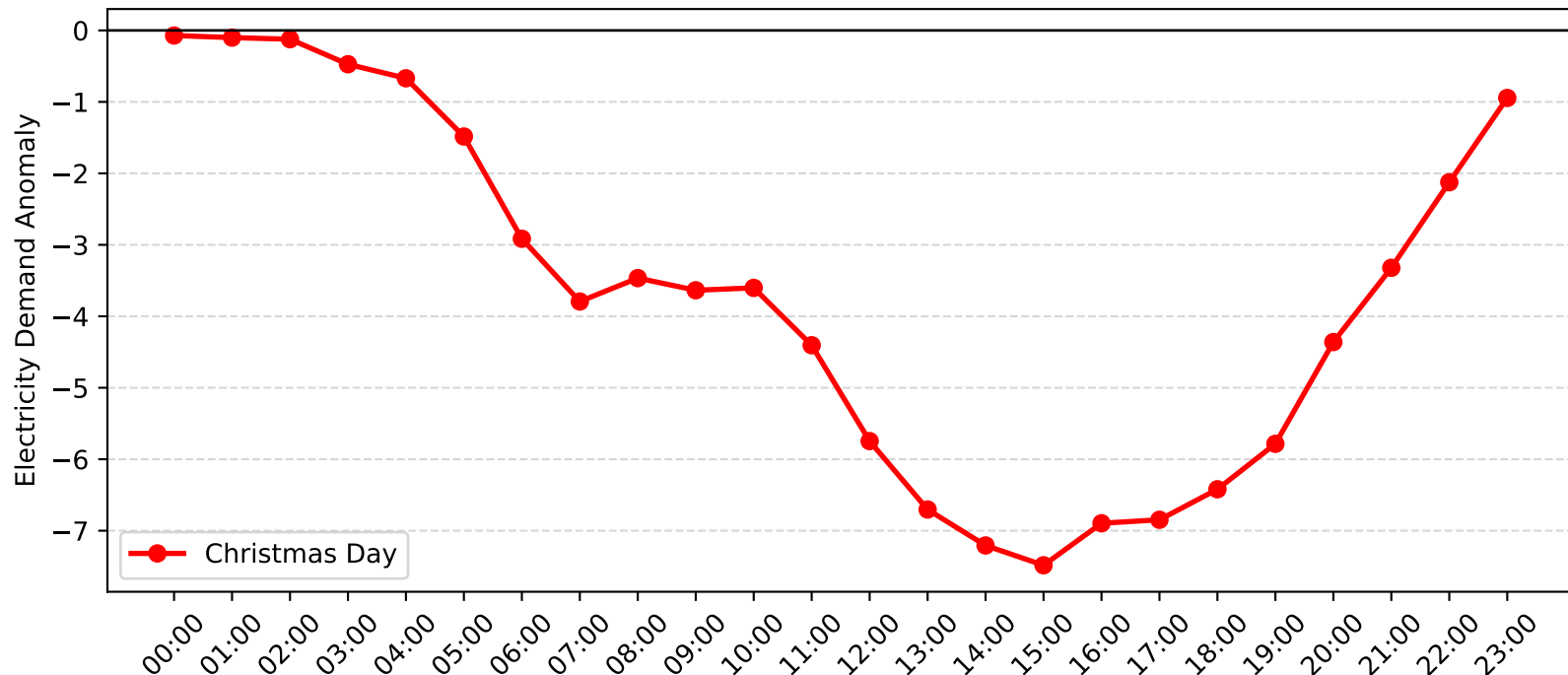
Hunters Hill Demand Anomaly: Christmas Day (2014-2015)
