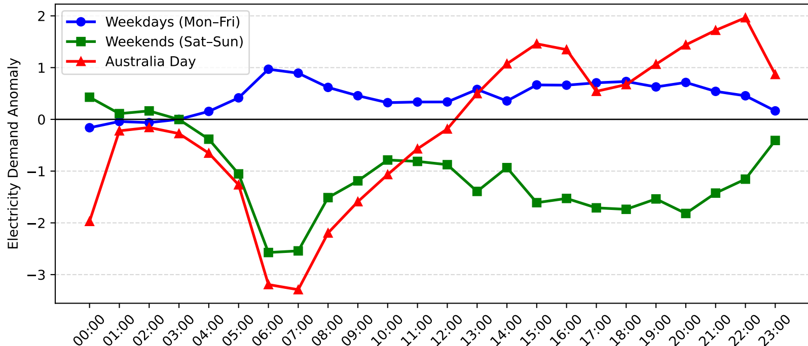
Revesby Demand Anomaly: Australia Day vs Weekday/Weekend (2009-2010)
