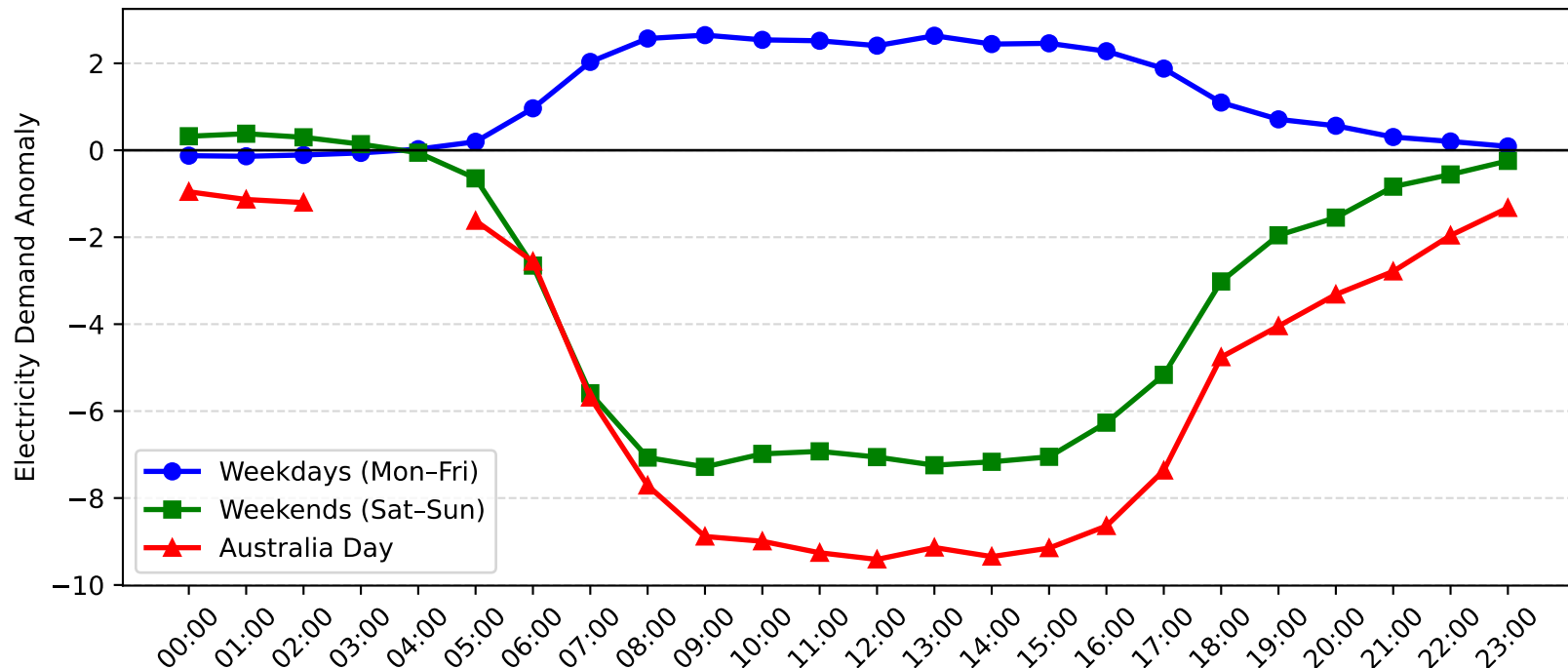
Green Square Demand Anomaly: Australia Day vs Weekday/Weekend (2017-2018)
