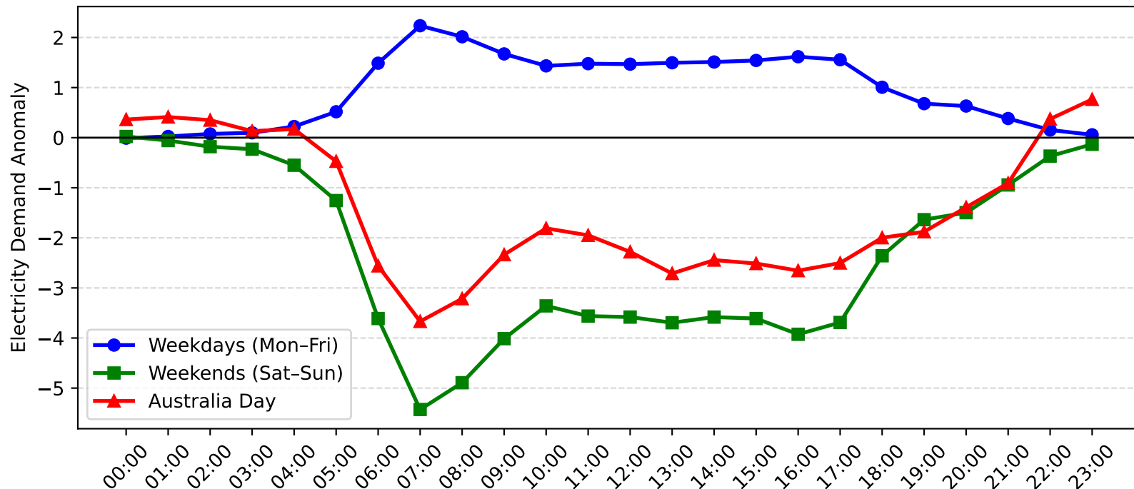
Chatswood Demand Anomaly: Australia Day vs Weekday/Weekend (2007-2008)
