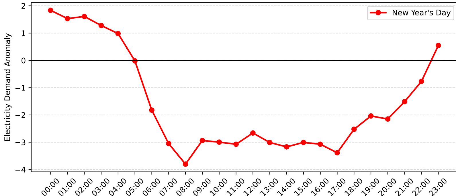
Dee Why West Demand Anomaly: New Year's Day (2015-2016)
