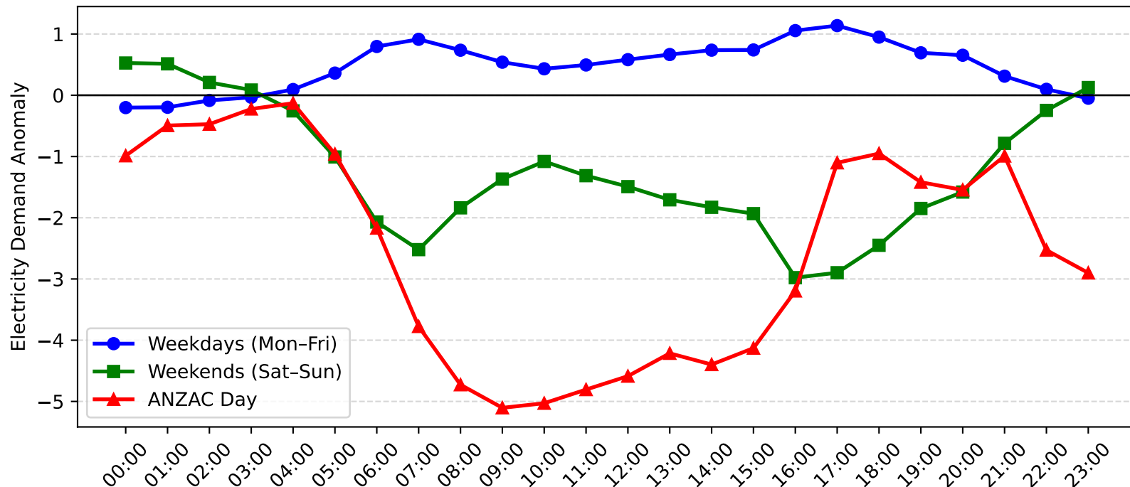
Erina Demand Anomaly: ANZAC Day vs Weekday/Weekend (2006-2007)
