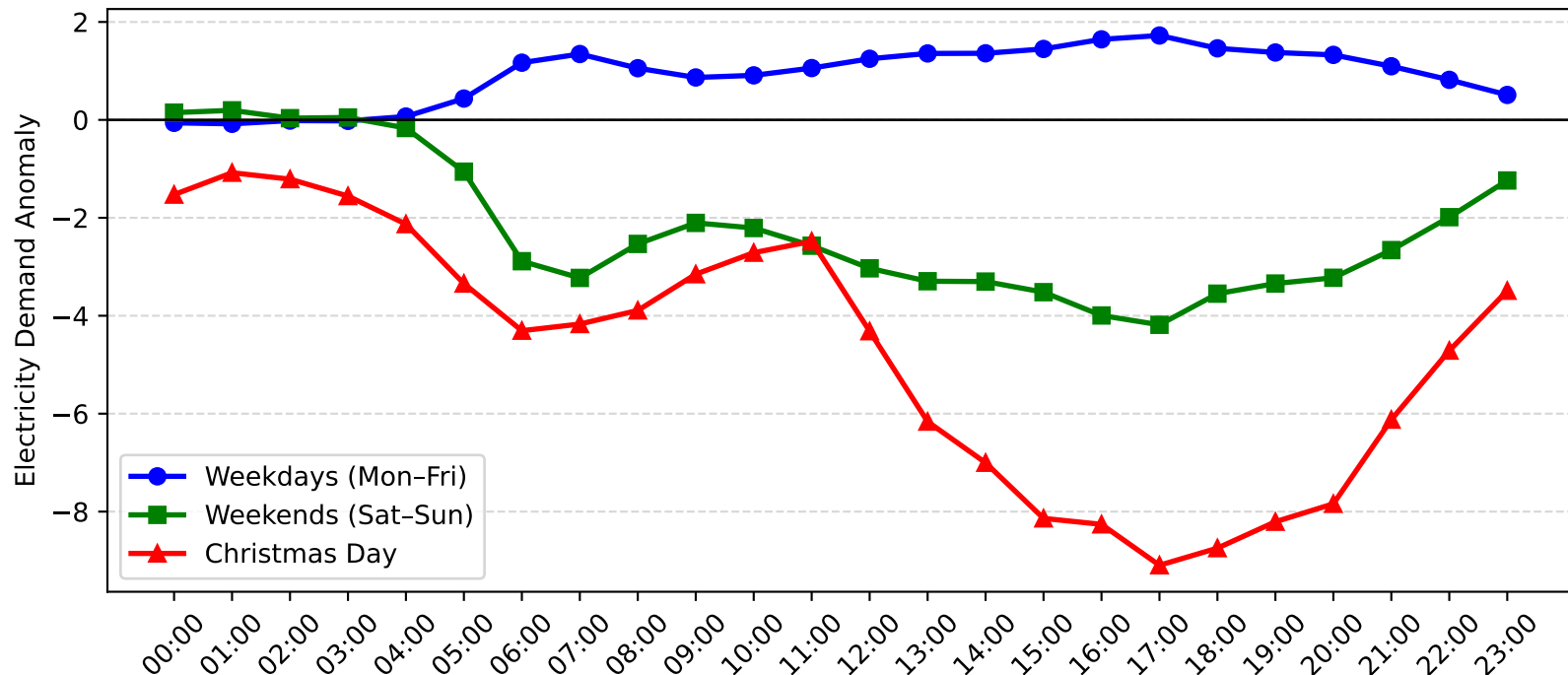
Pennant Hills Demand Anomaly: Christmas Day vs Weekday/Weekend (2015-2016)
