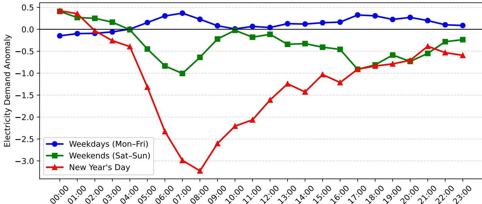
Charmhaven Demand Anomaly: New Year's Day vs Weekday/Weekend (2013-2014)
