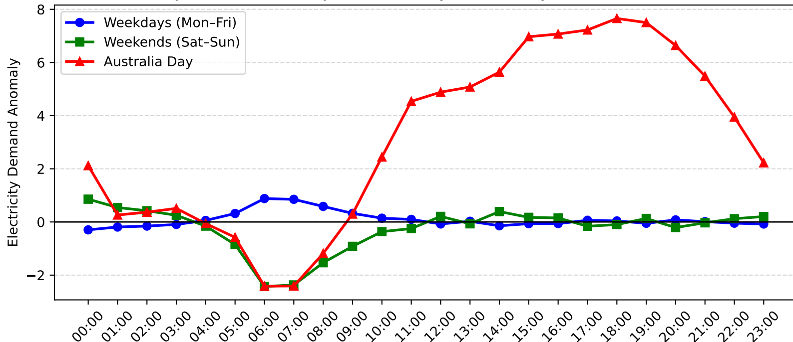
Revesby Demand Anomaly: Australia Day vs Weekday/Weekend (2010-2011)
