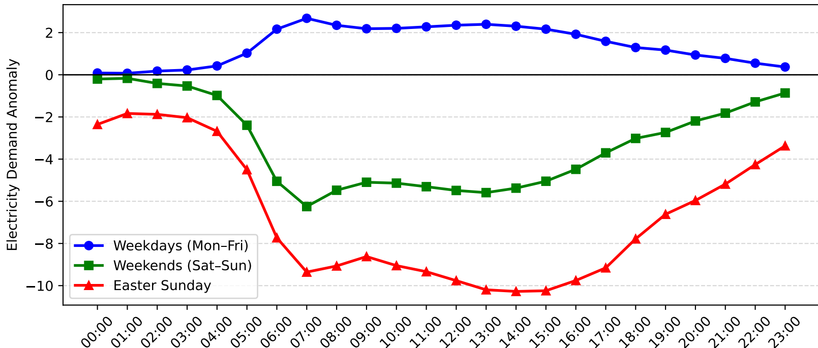
Sefton Demand Anomaly: Easter Sunday vs Weekday/Weekend (2013-2014)
