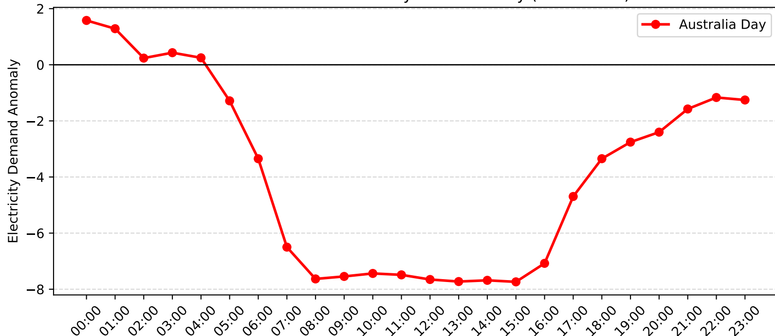
Gore Hill Demand Anomaly: Australia Day (2011-2012)
