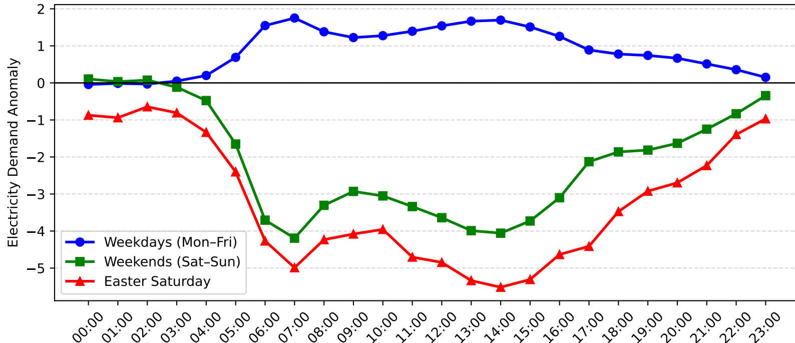
Kirrawee Demand Anomaly: Easter Saturday vs Weekday/Weekend (2007-2008)
