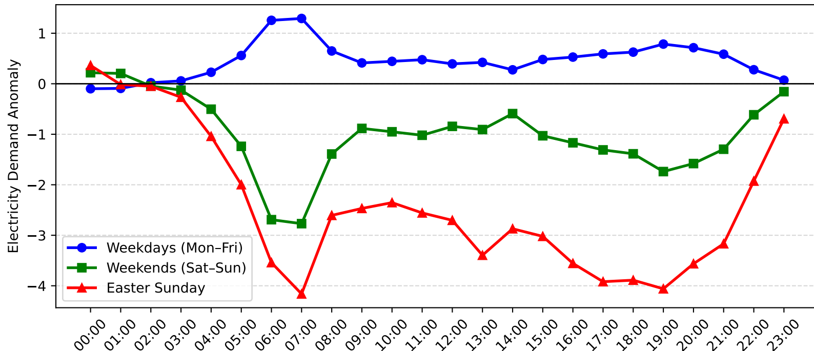
Revesby Demand Anomaly: Easter Sunday vs Weekday/Weekend (2017-2018)
