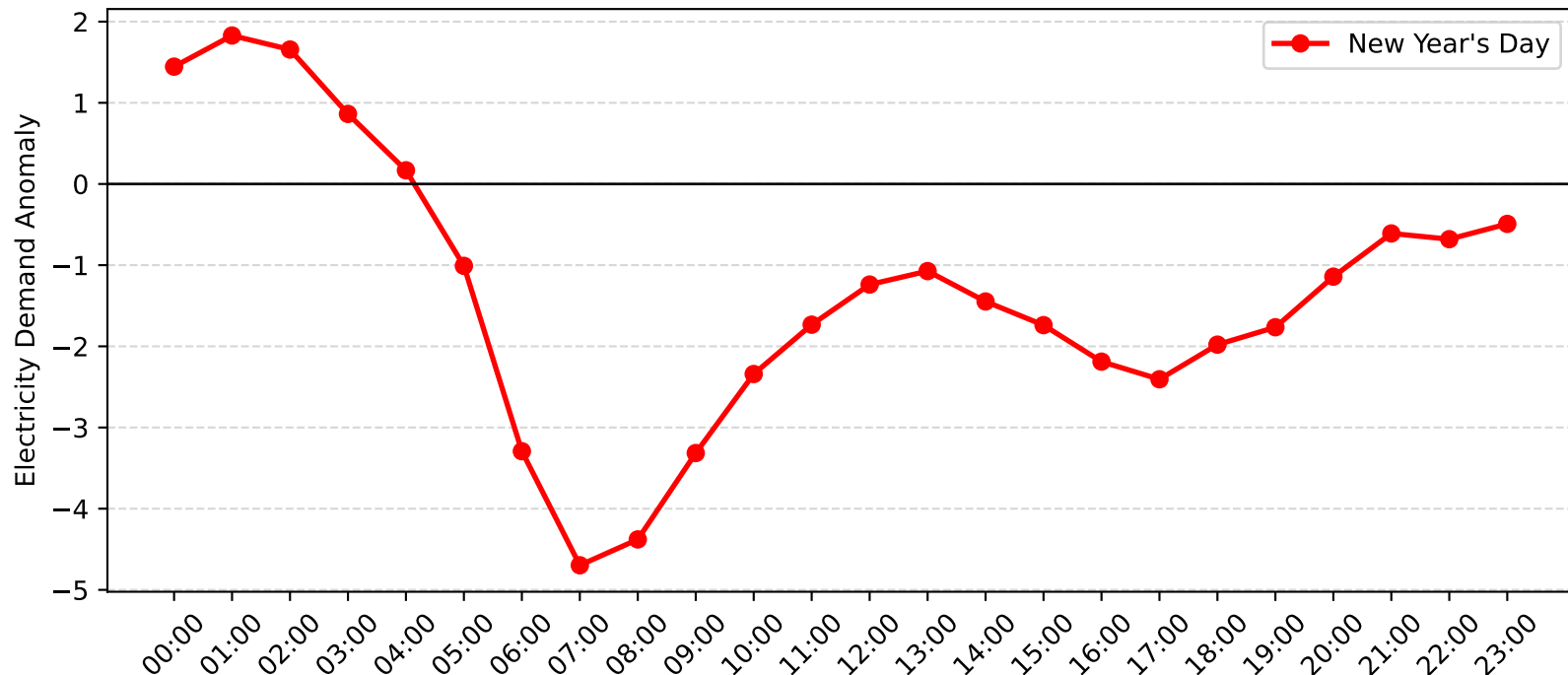
Mortdale Demand Anomaly: New Year's Day (2013-2014)
