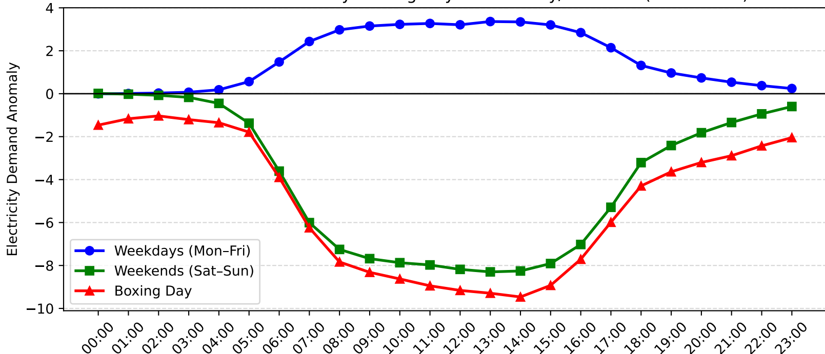
Mascot Demand Anomaly: Boxing Day vs Weekday/Weekend (2011-2012)
