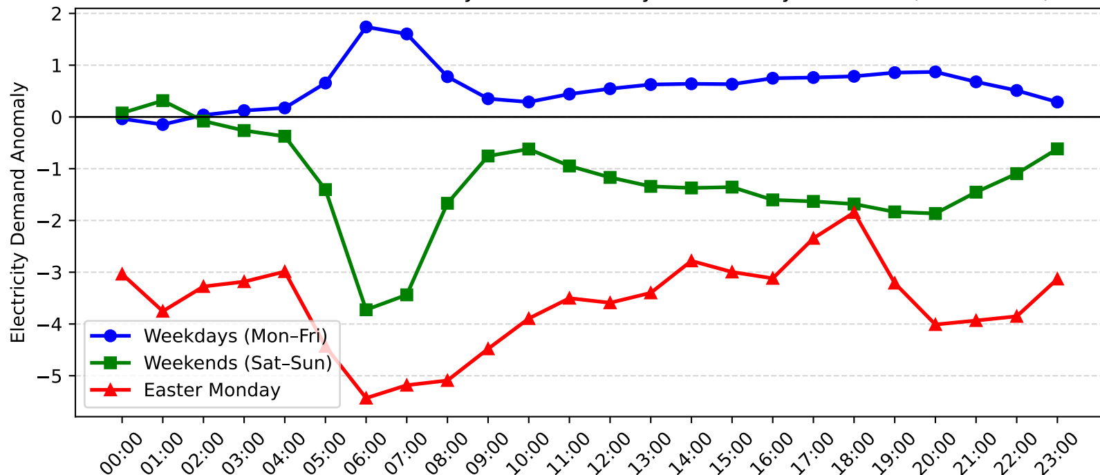
Pennant Hills Demand Anomaly: Easter Monday vs Weekday/Weekend (2017-2018)
