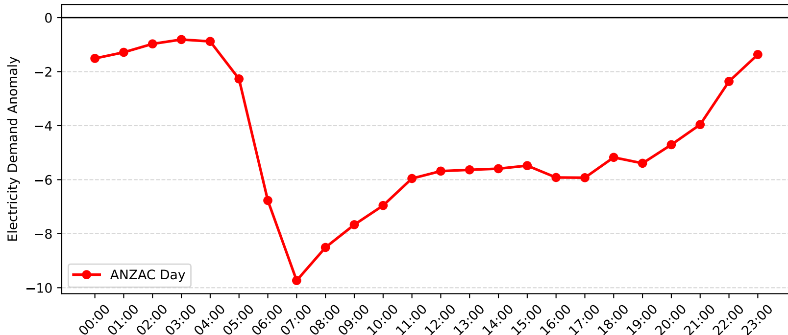
Epping Demand Anomaly: ANZAC Day (2010-2011)
