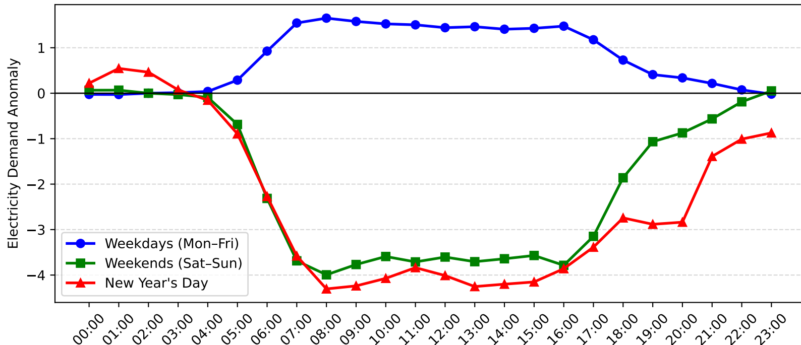
Pymble Demand Anomaly: New Year's Day vs Weekday/Weekend (2007-2008)
