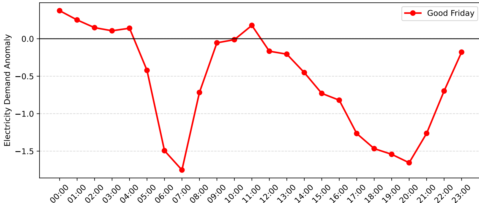
Harbord Demand Anomaly: Good Friday (2012-2013)
