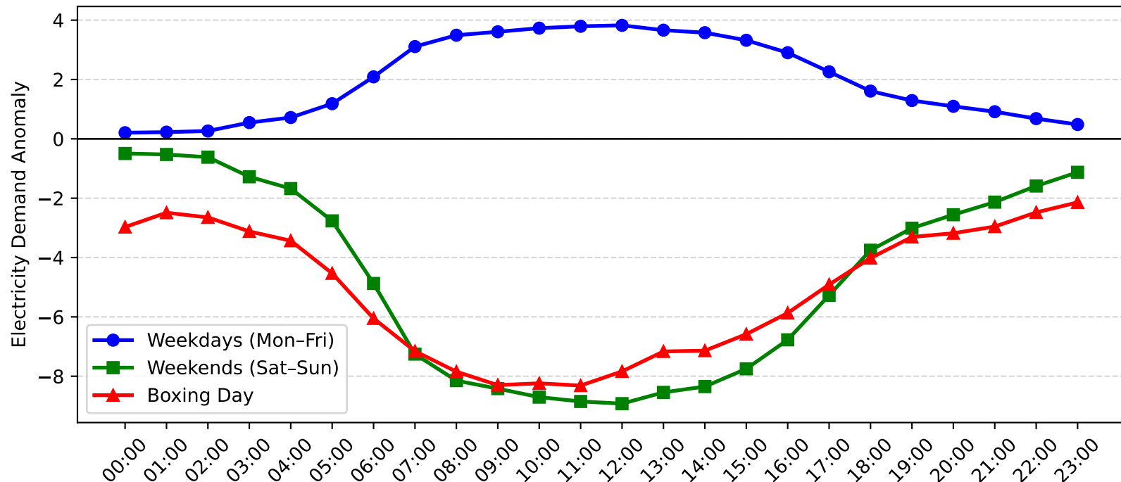
Homebush Bay Demand Anomaly: Boxing Day vs Weekday/Weekend (2016-2017)
