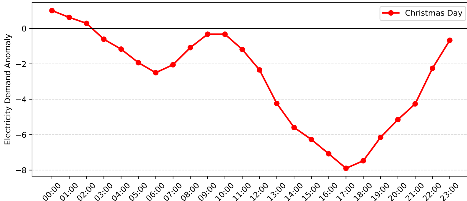
Revesby Demand Anomaly: Christmas Day (2013-2014)
