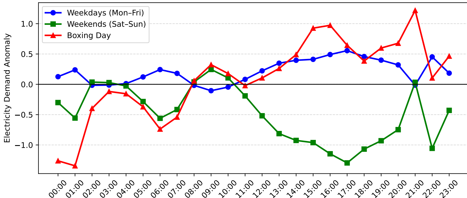
Nelson Bay Demand Anomaly: Boxing Day vs Weekday/Weekend (2015-2016)
