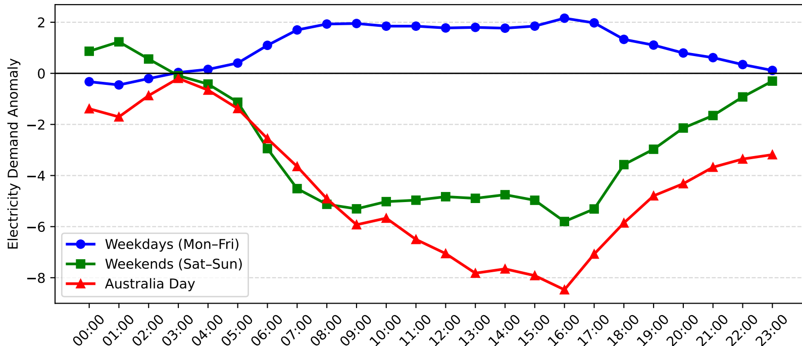
Greenacre Park Demand Anomaly: Australia Day vs Weekday/Weekend (2016-2017)
