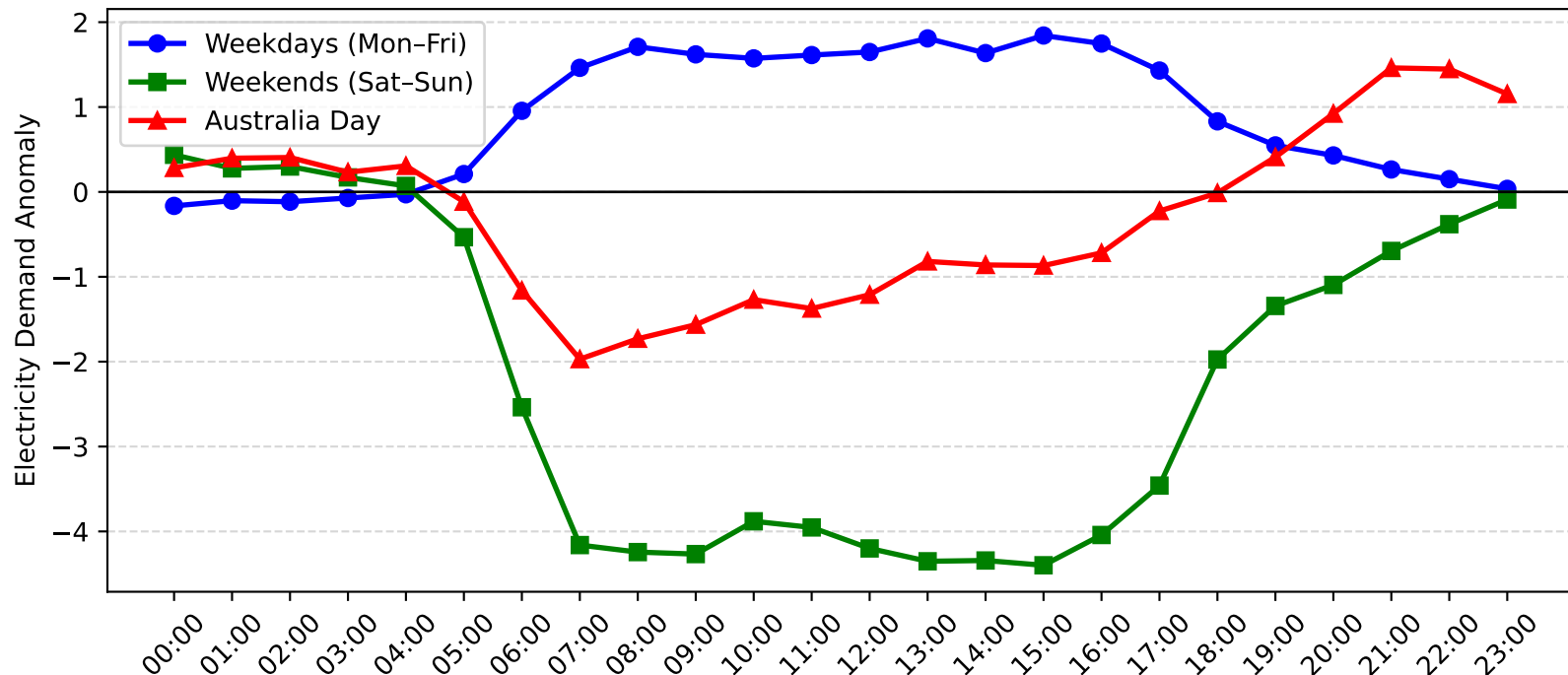
Pymble Demand Anomaly: Australia Day vs Weekday/Weekend (2009-2010)
