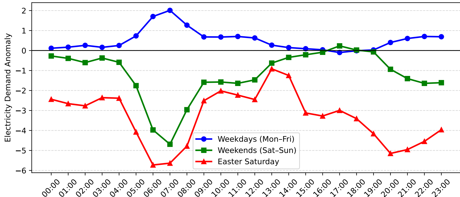
Meadowbank Demand Anomaly: Easter Saturday vs Weekday/Weekend (2014-2015)
