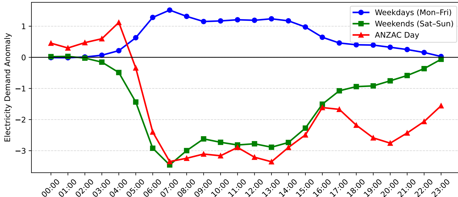
Wyong Demand Anomaly: ANZAC Day vs Weekday/Weekend (2015-2016)
