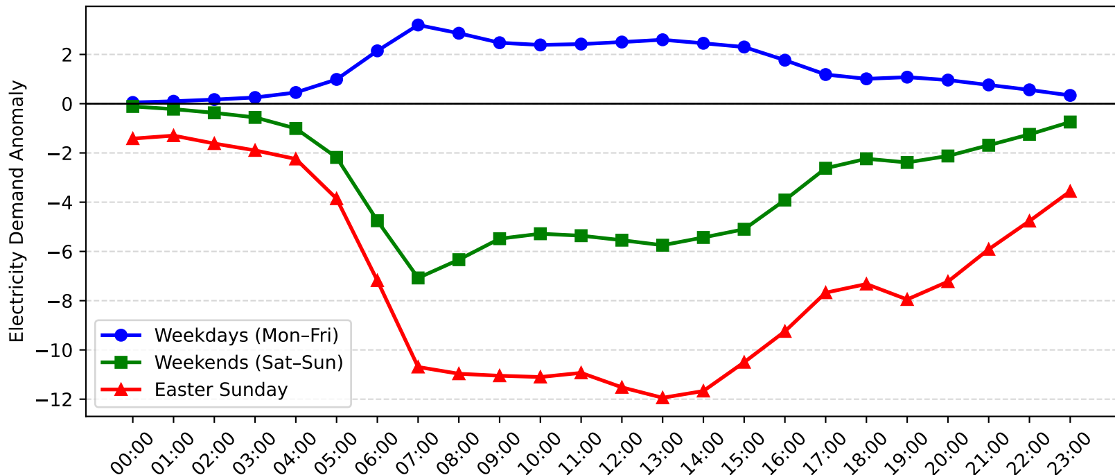
Marrickville Demand Anomaly: Easter Sunday vs Weekday/Weekend (2017-2018)
