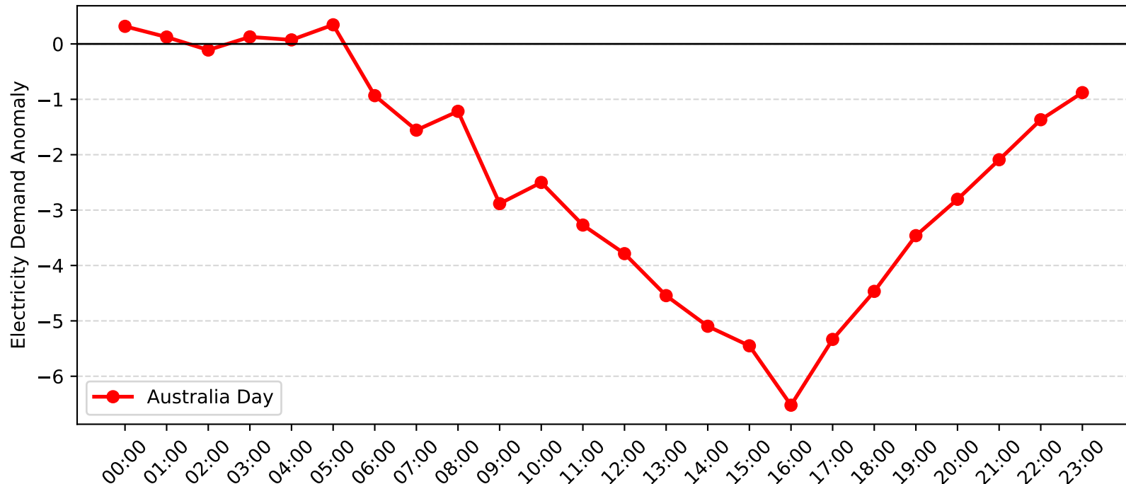
Erina Demand Anomaly: Australia Day (2014-2015)
