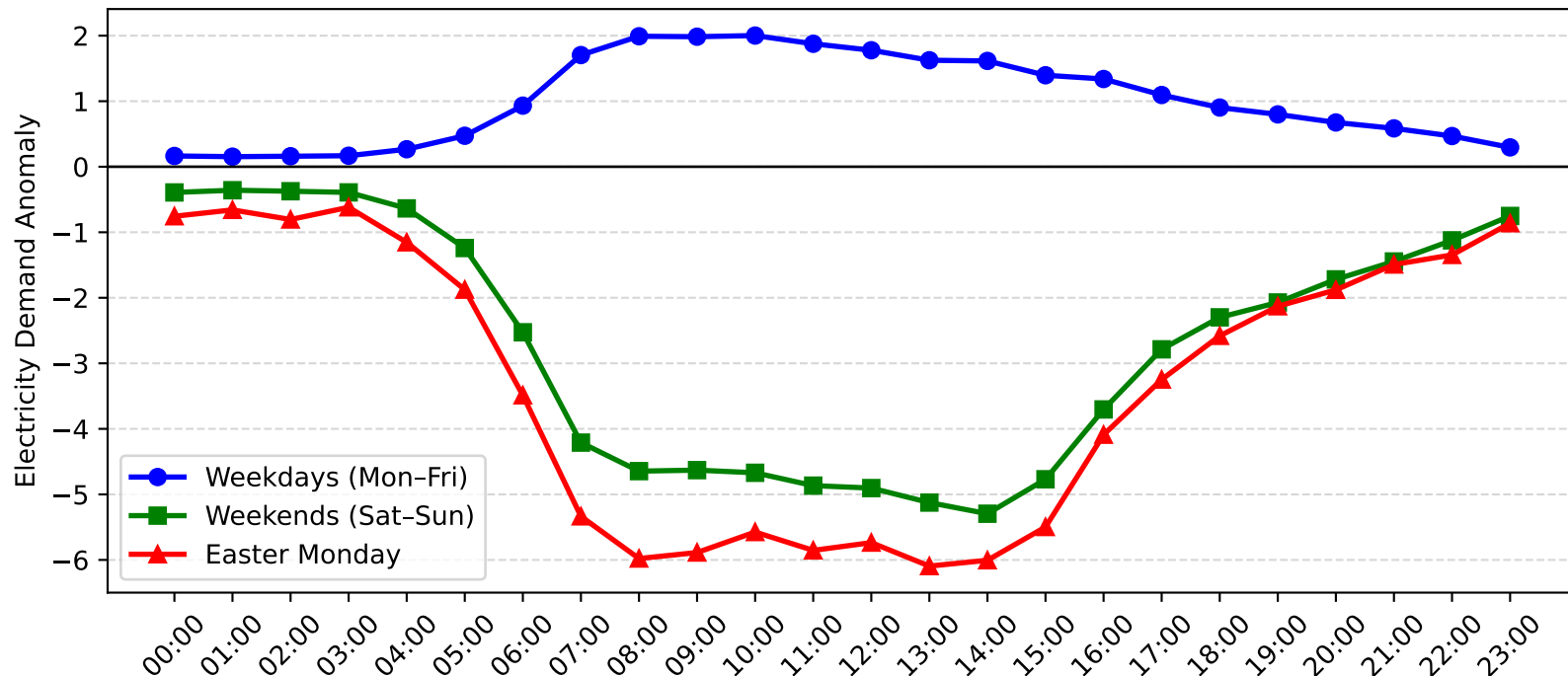
Bankstown Demand Anomaly: Easter Monday vs Weekday/Weekend (2012-2013)
