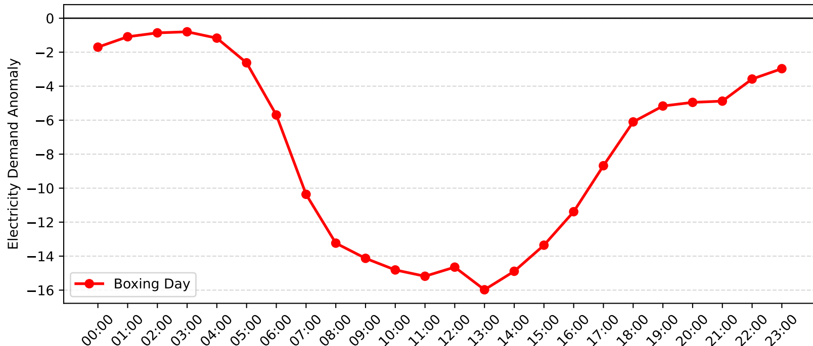
Gore Hill Demand Anomaly: Boxing Day (2010-2011)
