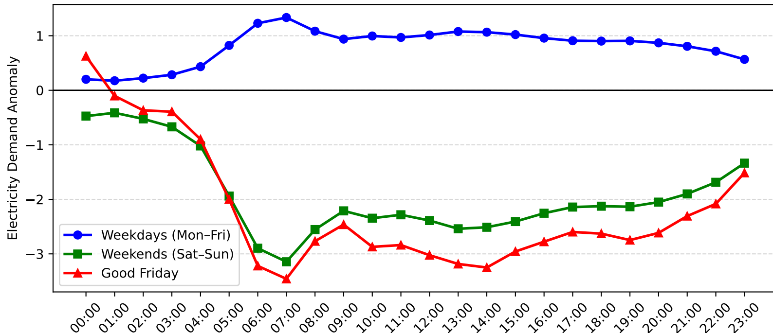
Lisarow Demand Anomaly: Good Friday vs Weekday/Weekend (2017-2018)
