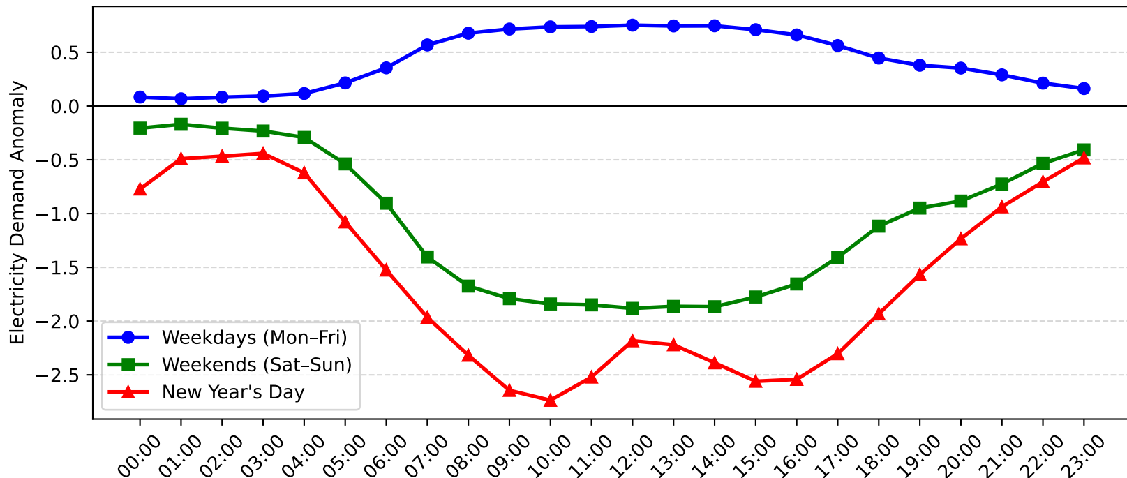
Lidcombe Demand Anomaly: New Year's Day vs Weekday/Weekend (2016-2017)
