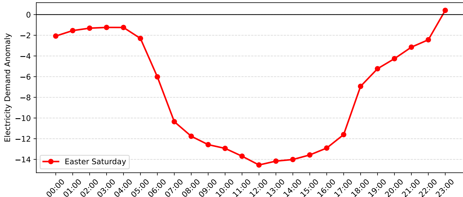
Macquarie Park Demand Anomaly: Easter Saturday (2015-2016)
