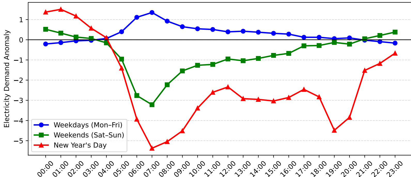
Mortdale Demand Anomaly: New Year's Day vs Weekday/Weekend (2007-2008)
