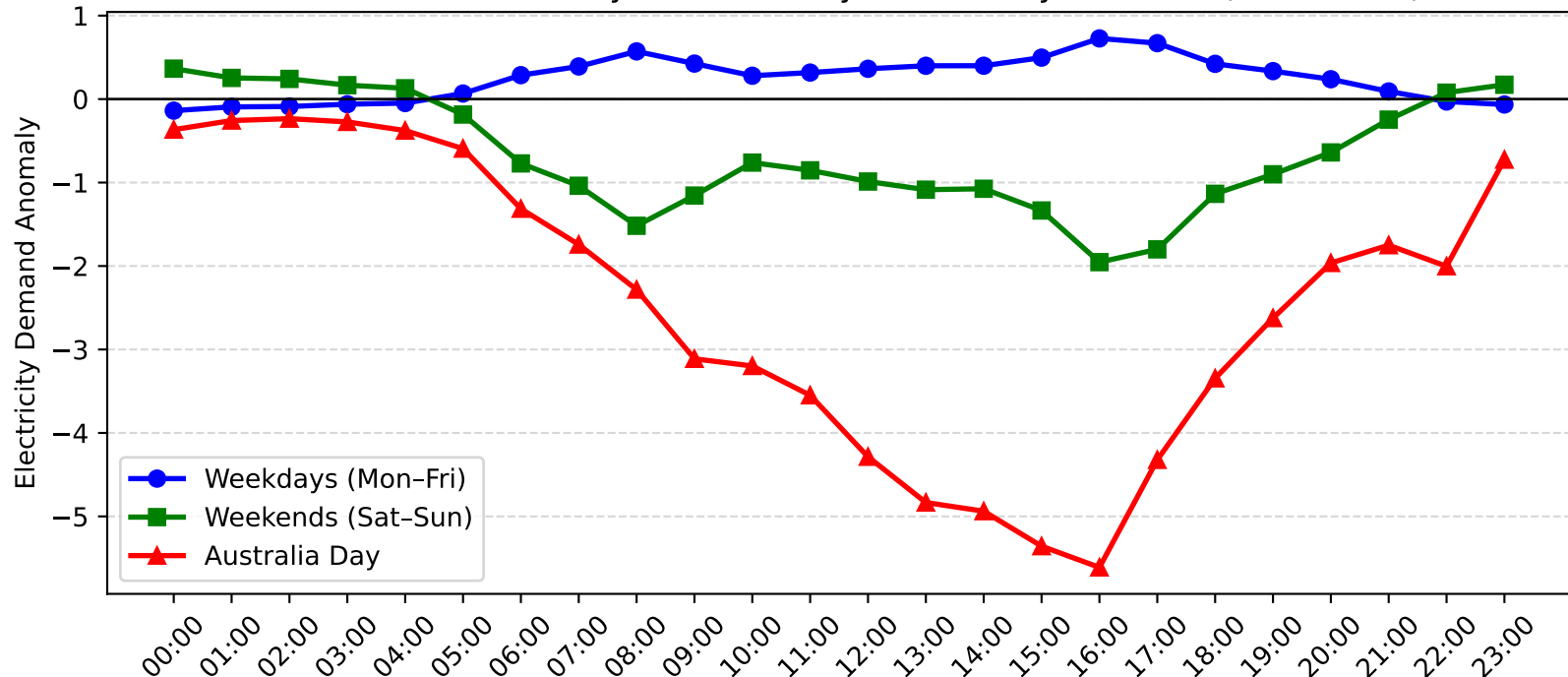
Erina Demand Anomaly: Australia Day vs Weekday/Weekend (2016-2017)
