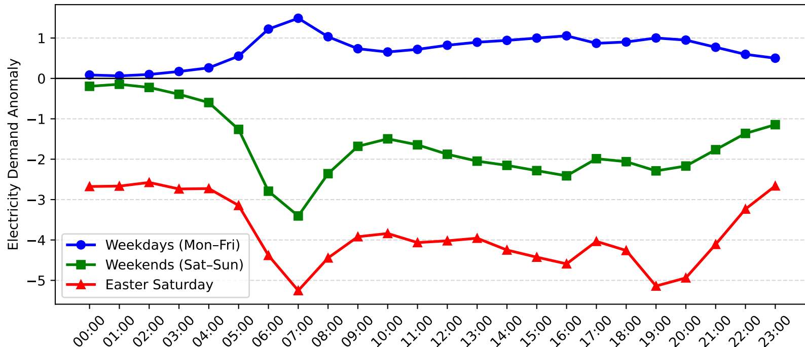
Five Dock Demand Anomaly: Easter Saturday vs Weekday/Weekend (2017-2018)
