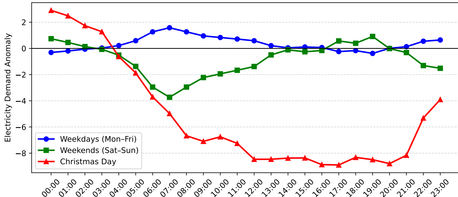
Meadowbank Demand Anomaly: Christmas Day vs Weekday/Weekend (2011-2012)
