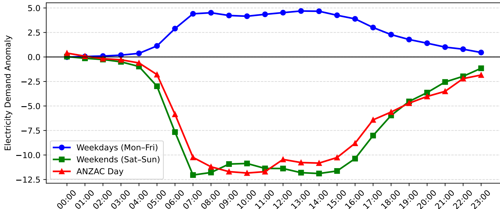
Zetland Demand Anomaly: ANZAC Day vs Weekday/Weekend (2007-2008)
