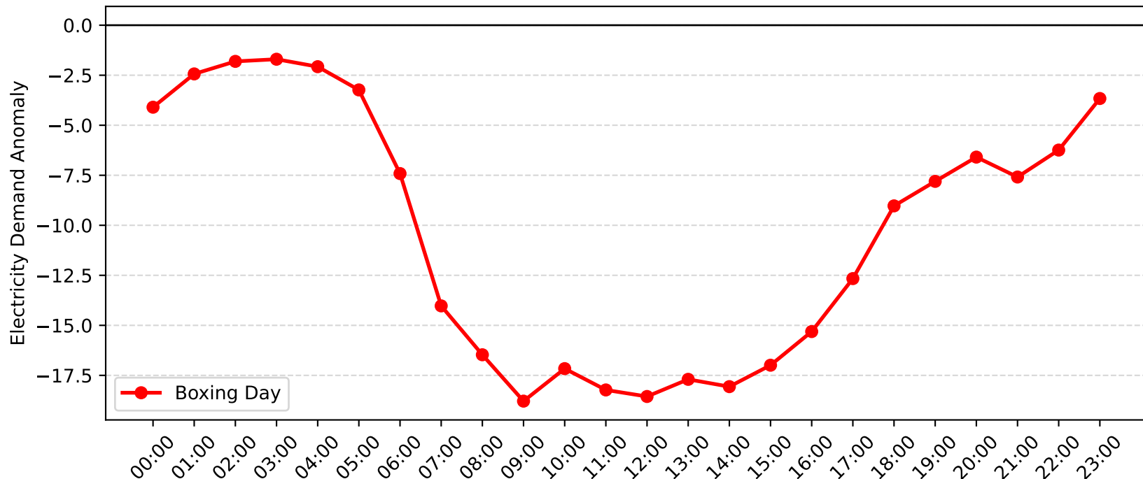
Gore Hill Demand Anomaly: Boxing Day (2008-2009)
