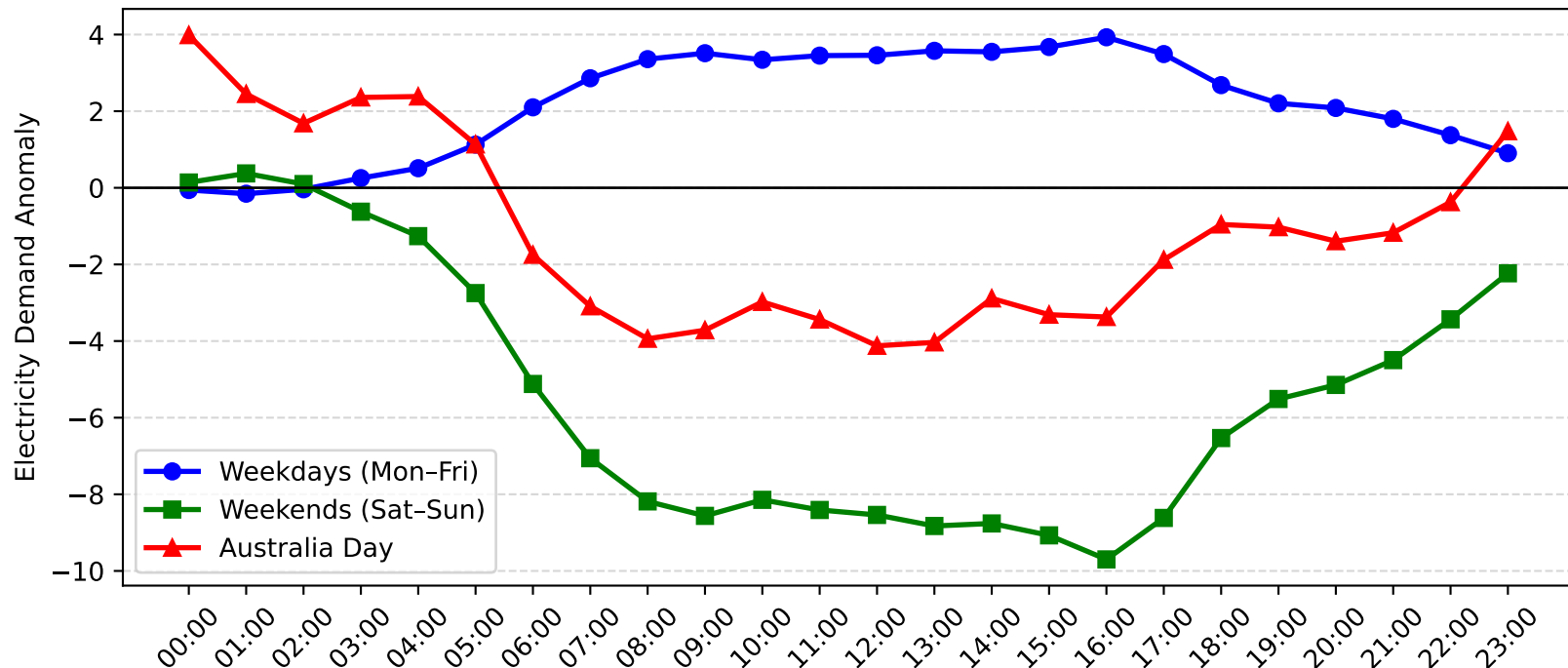
Greenacre Park Demand Anomaly: Australia Day vs Weekday/Weekend (2012-2013)
