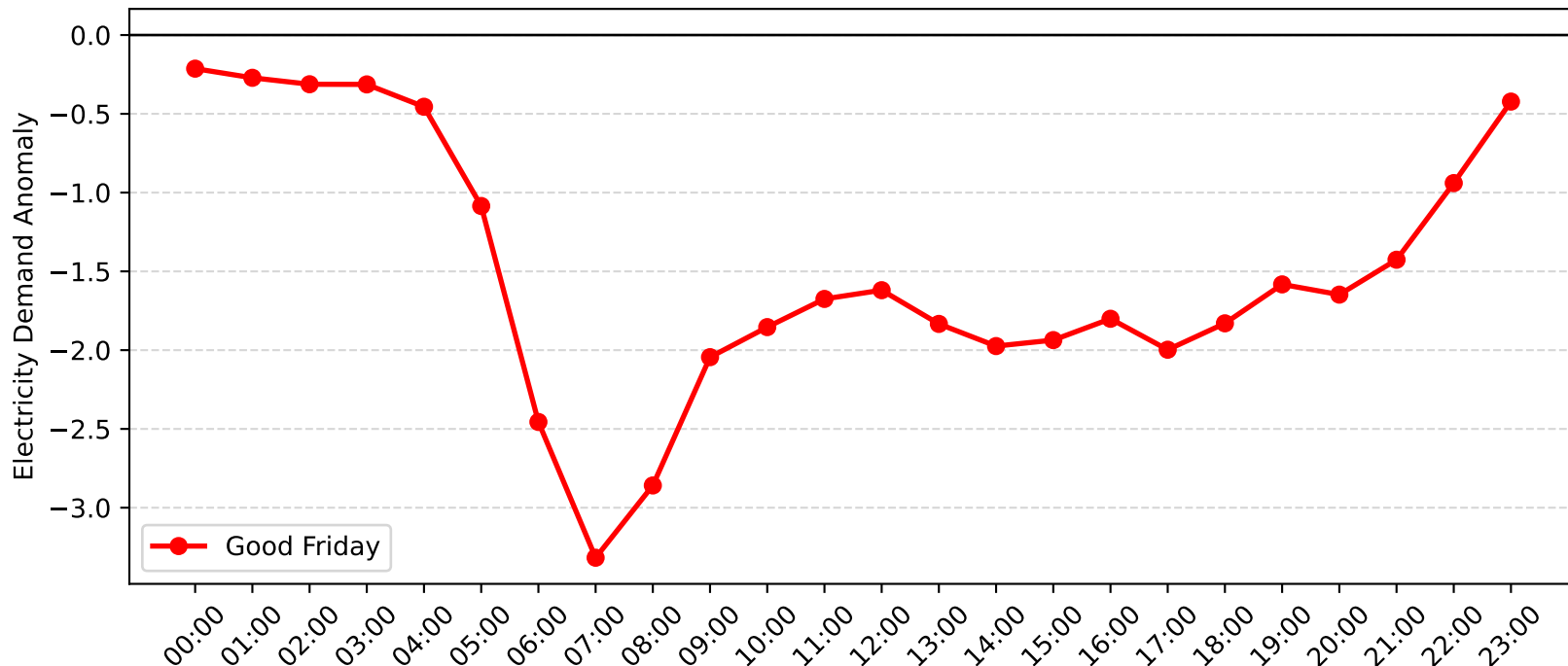
Arncliffe Demand Anomaly: Good Friday (2010-2011)
