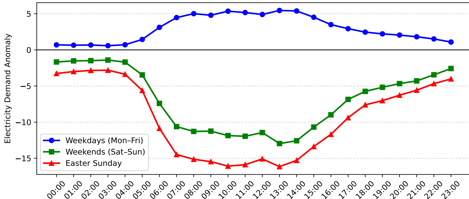
Milperra Demand Anomaly: Easter Sunday vs Weekday/Weekend (2006-2007)
