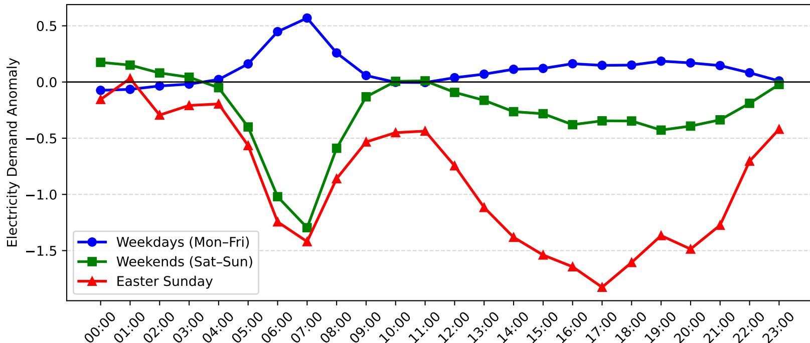
Blakehurst Demand Anomaly: Easter Sunday vs Weekday/Weekend (2015-2016)
