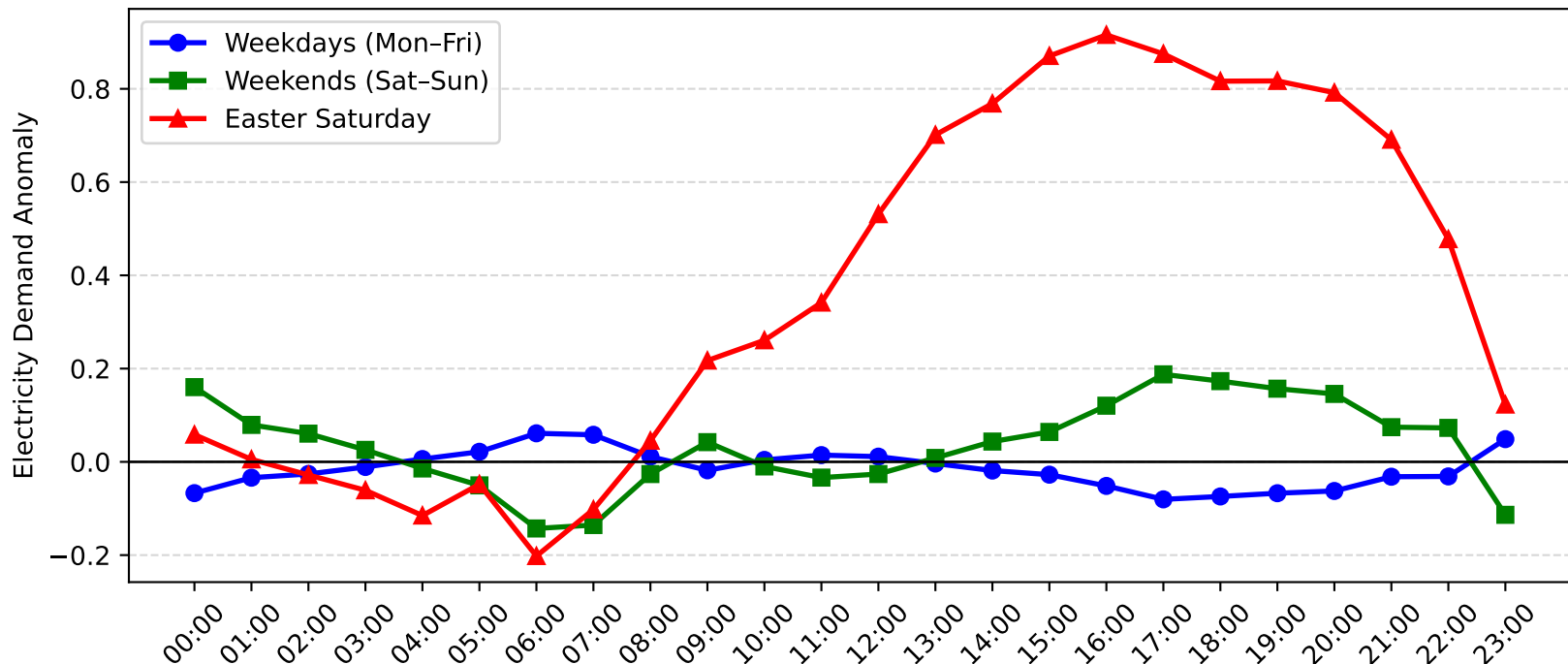
Rothbury Demand Anomaly: Easter Saturday vs Weekday/Weekend (2012-2013)
