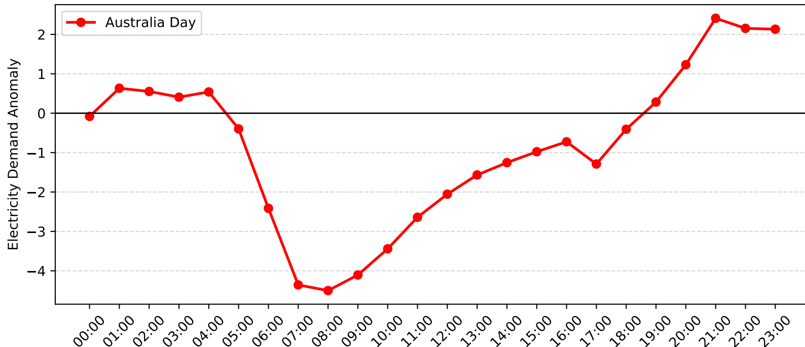
Punchbowl Demand Anomaly: Australia Day (2009-2010)
