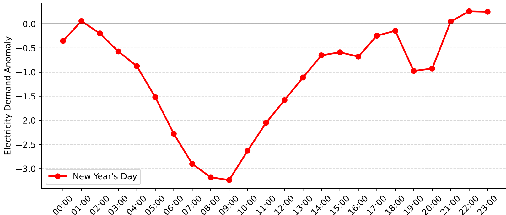
Lidcombe Demand Anomaly: New Year's Day (2010-2011)
