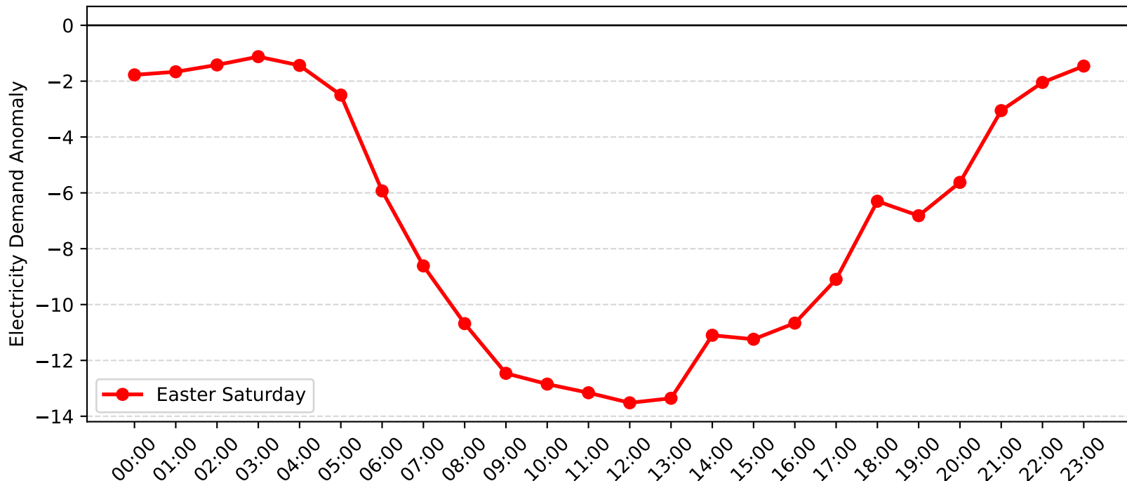
Macquarie Park Demand Anomaly: Easter Saturday (2008-2009)
