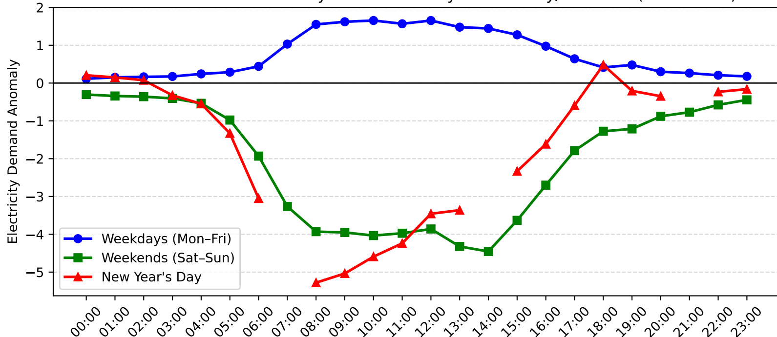
Bankstown Demand Anomaly: New Year's Day vs Weekday/Weekend (2010-2011)
