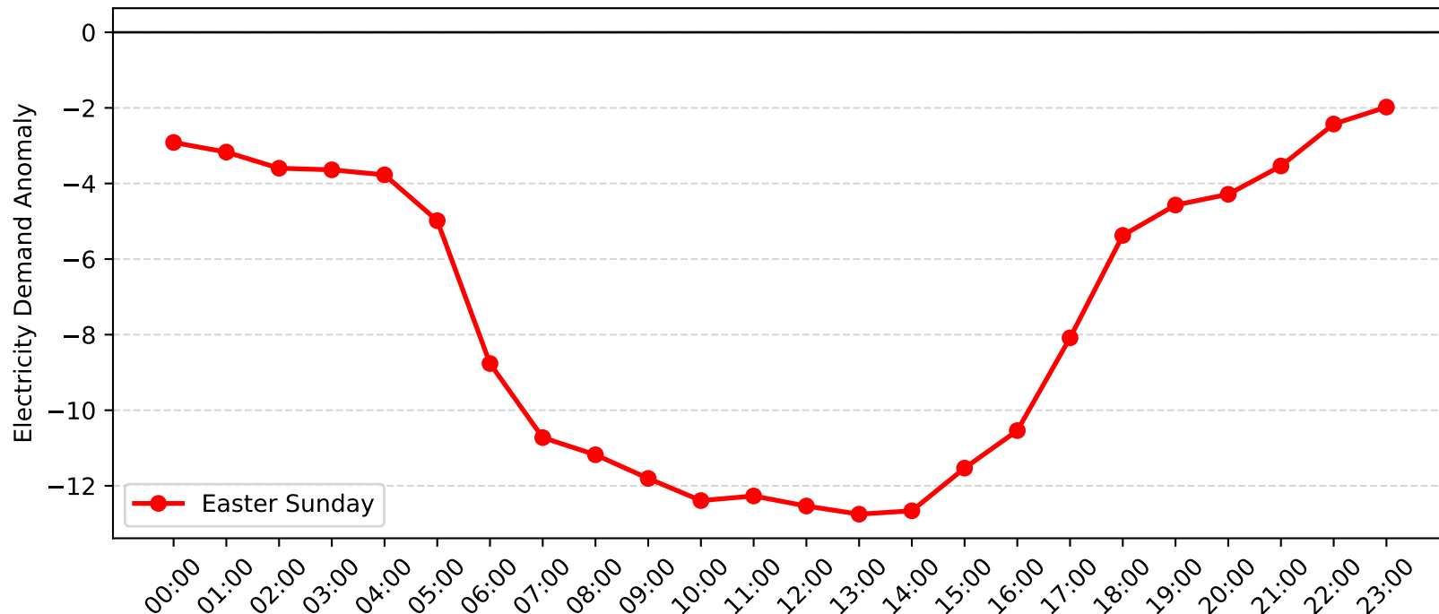
Flemington Demand Anomaly: Easter Sunday (2009-2010)
