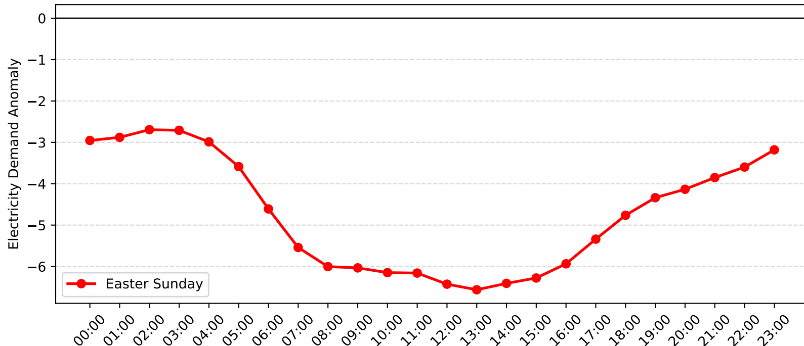
Leightonfield Demand Anomaly: Easter Sunday (2016-2017)
