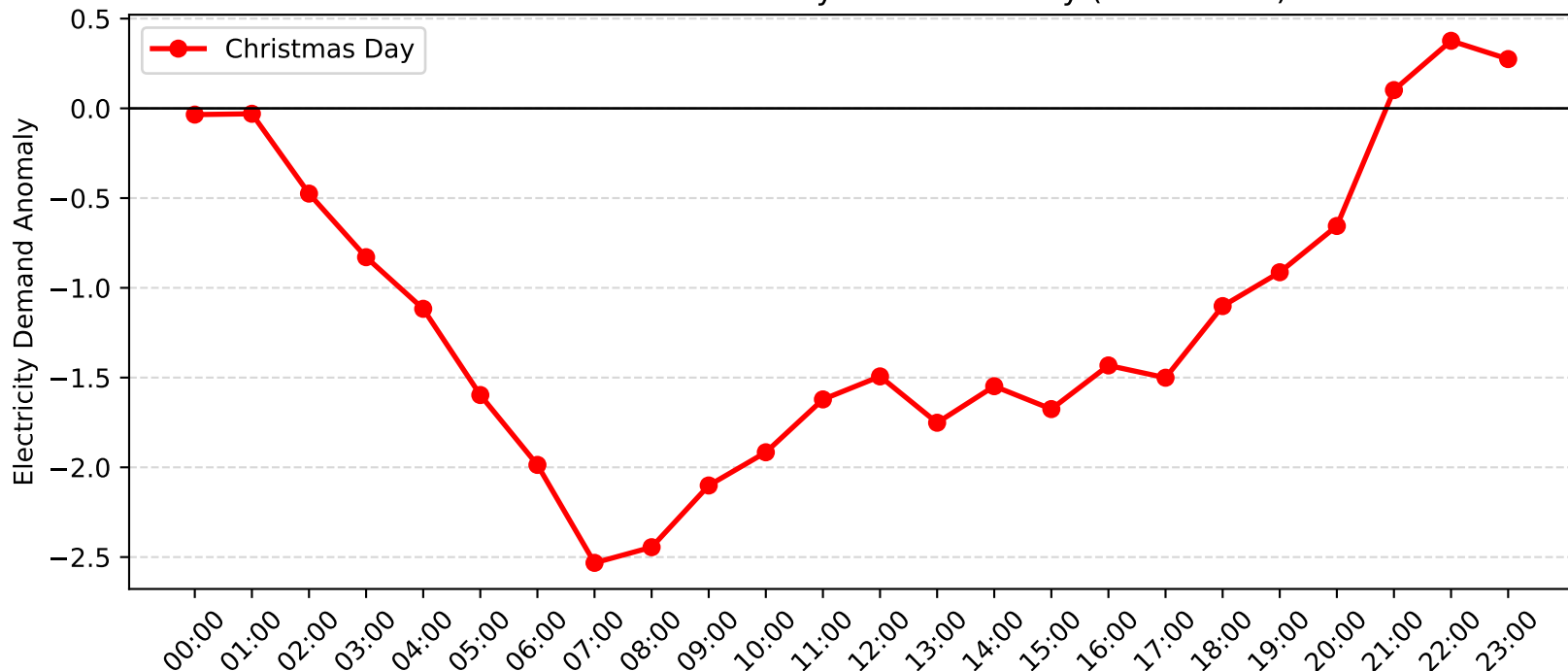
Bass Hill Demand Anomaly: Christmas Day (2010-2011)
