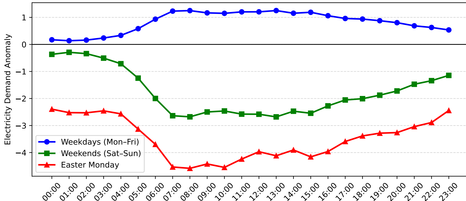
Bass Hill Demand Anomaly: Easter Monday vs Weekday/Weekend (2017-2018)
