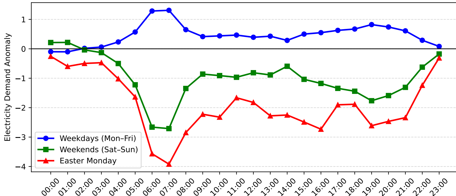
Revesby Demand Anomaly: Easter Monday vs Weekday/Weekend (2017-2018)
