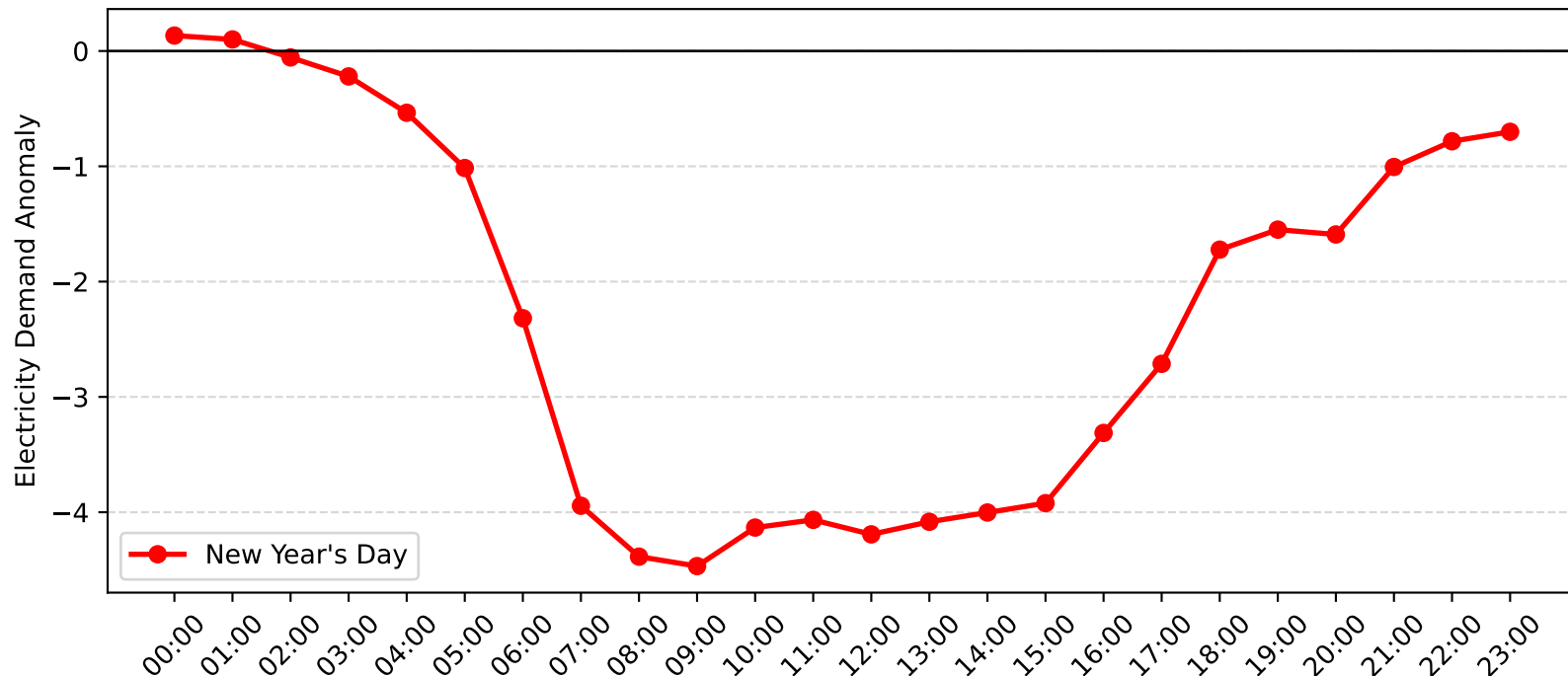
Beacon Hill Demand Anomaly: New Year's Day (2010-2011)
