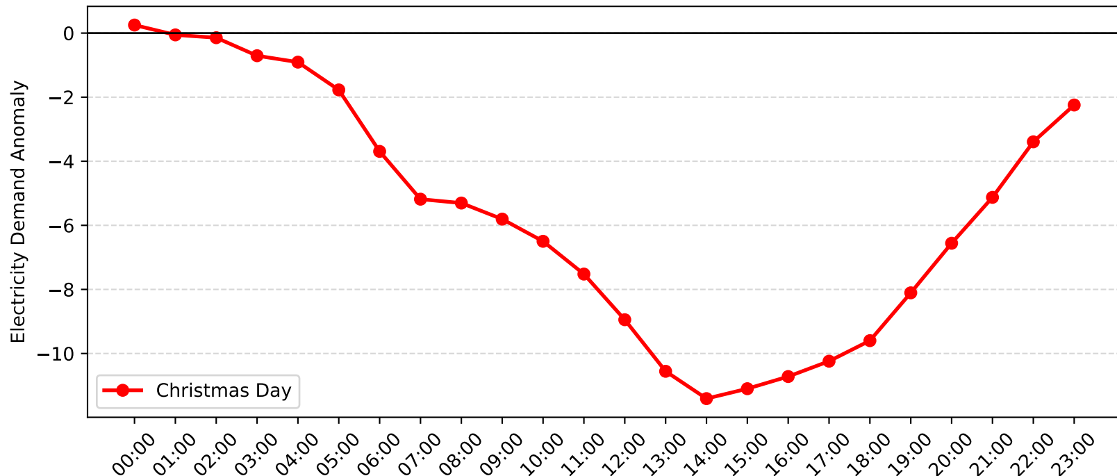
Hunters Hill Demand Anomaly: Christmas Day (2006-2007)
