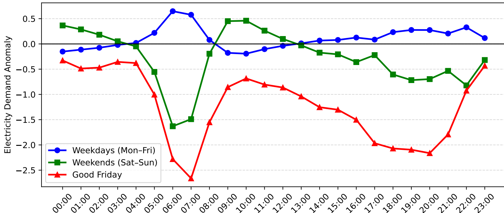
Harbord Demand Anomaly: Good Friday vs Weekday/Weekend (2005-2006)
