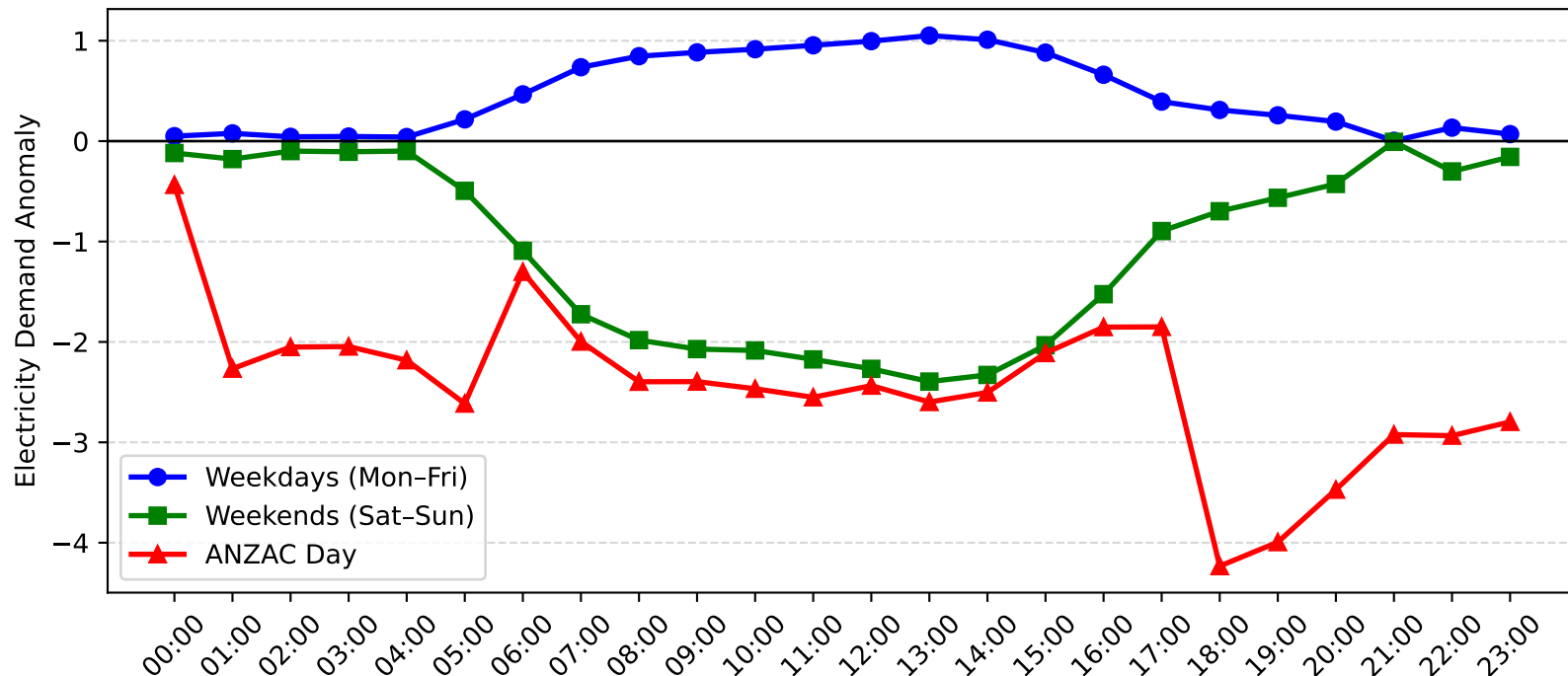
Broadmeadow Demand Anomaly: ANZAC Day vs Weekday/Weekend (2015-2016)
