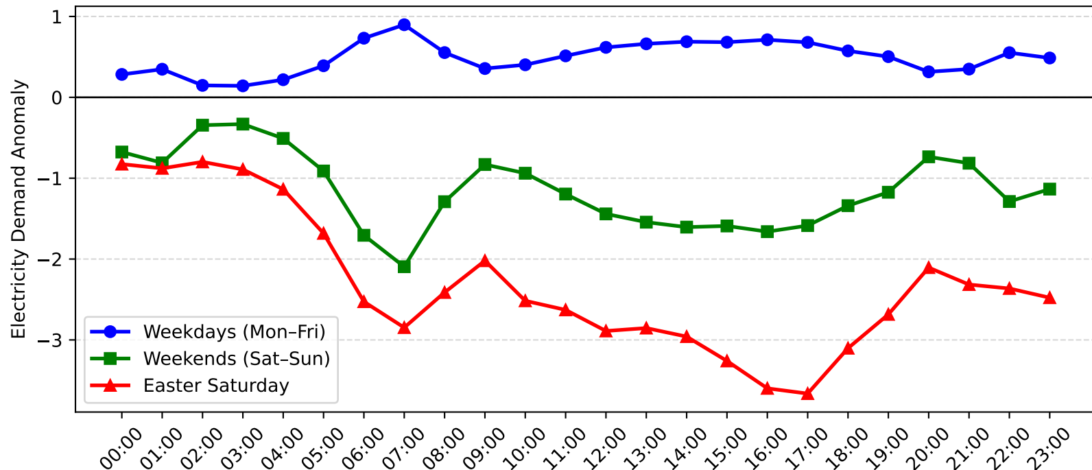
Jesmond Demand Anomaly: Easter Saturday vs Weekday/Weekend (2012-2013)
