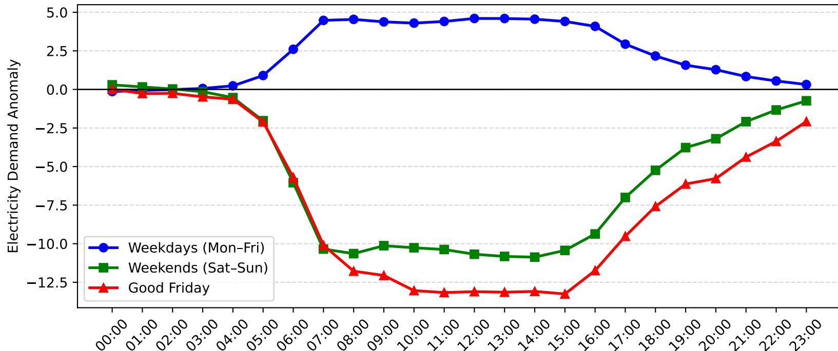
Zetland Demand Anomaly: Good Friday vs Weekday/Weekend (2009-2010)
