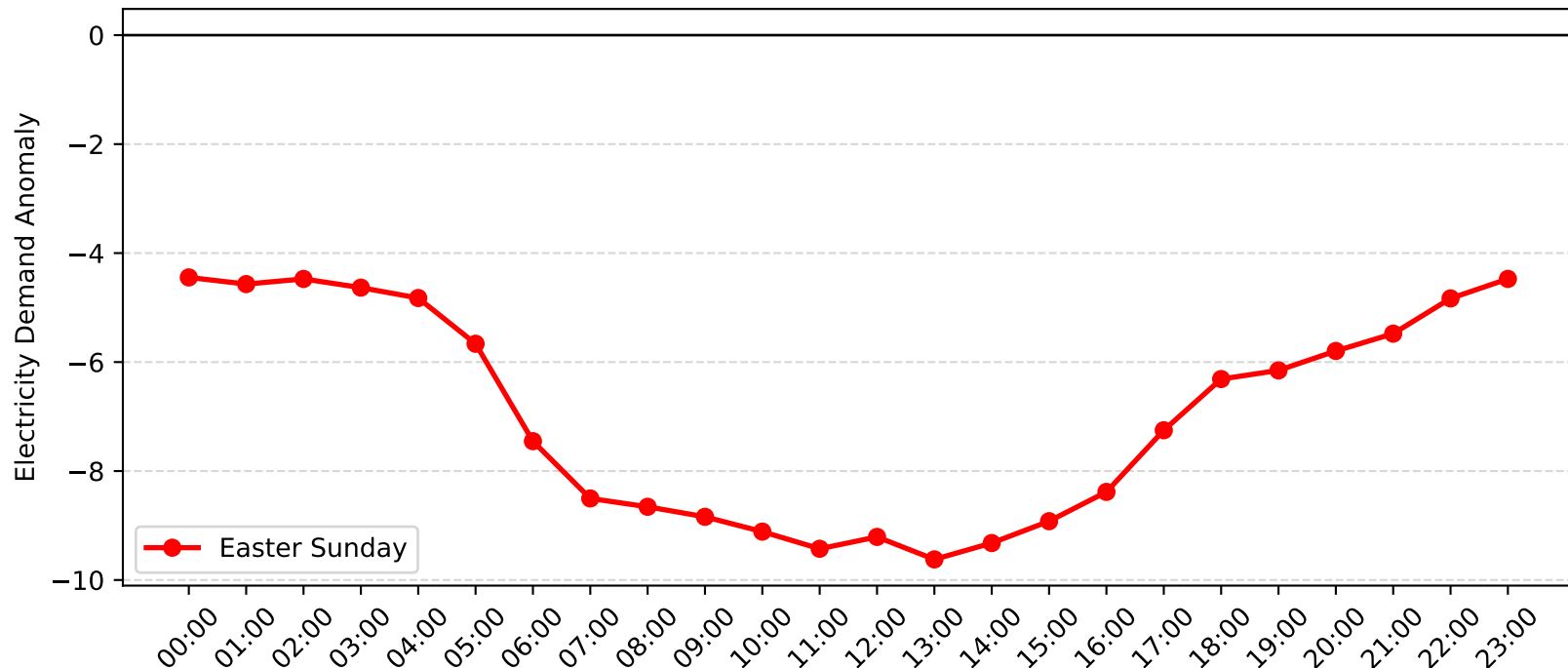
Leightonfield Demand Anomaly: Easter Sunday (2005-2006)
