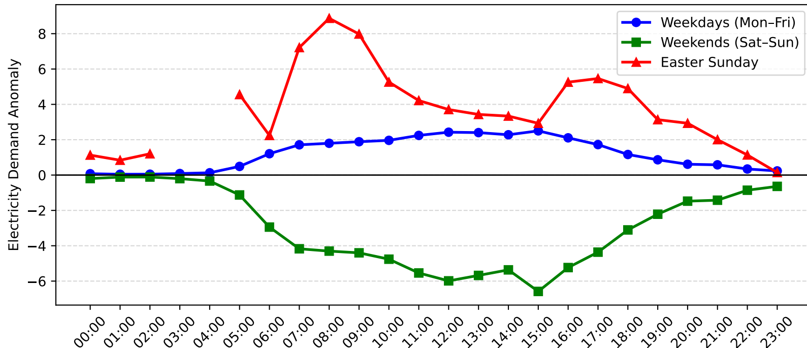
Gore Hill Demand Anomaly: Easter Sunday vs Weekday/Weekend (2004-2005)
