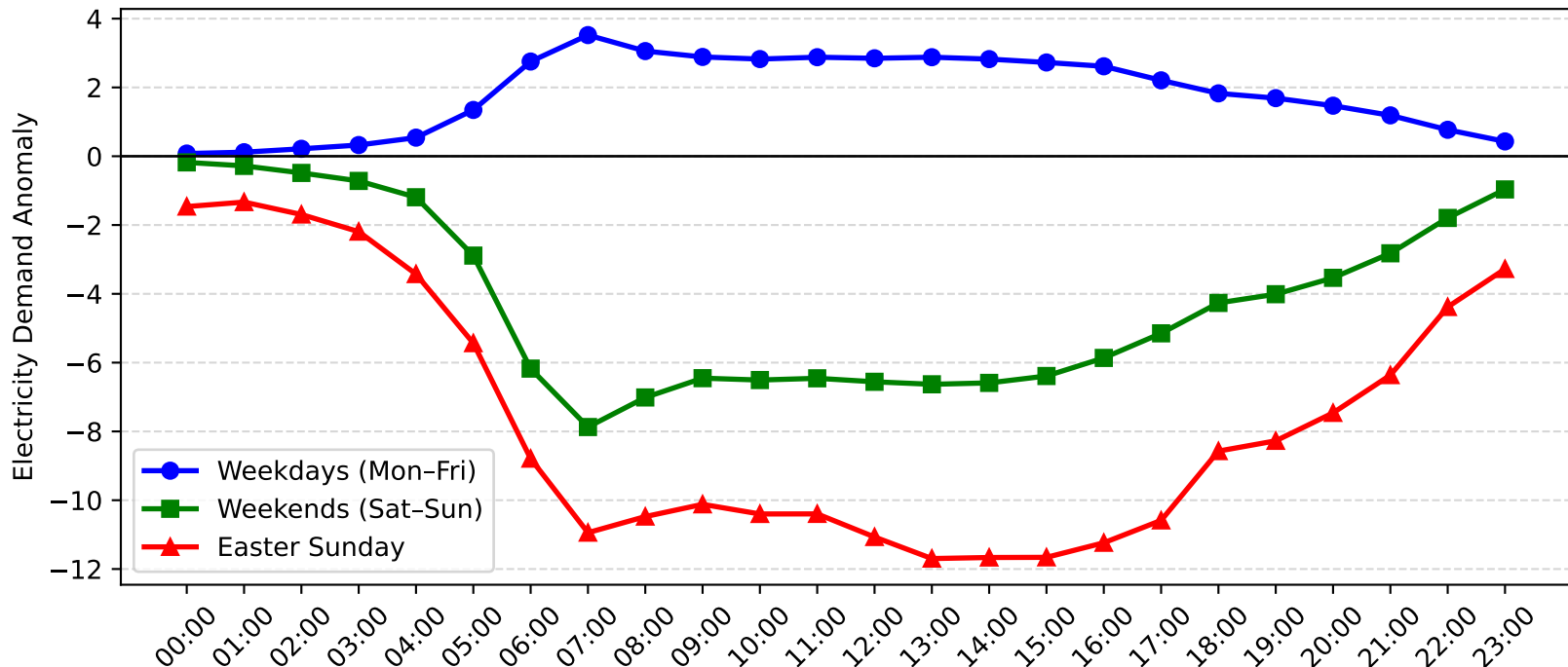
Sefton Demand Anomaly: Easter Sunday vs Weekday/Weekend (2010-2011)
