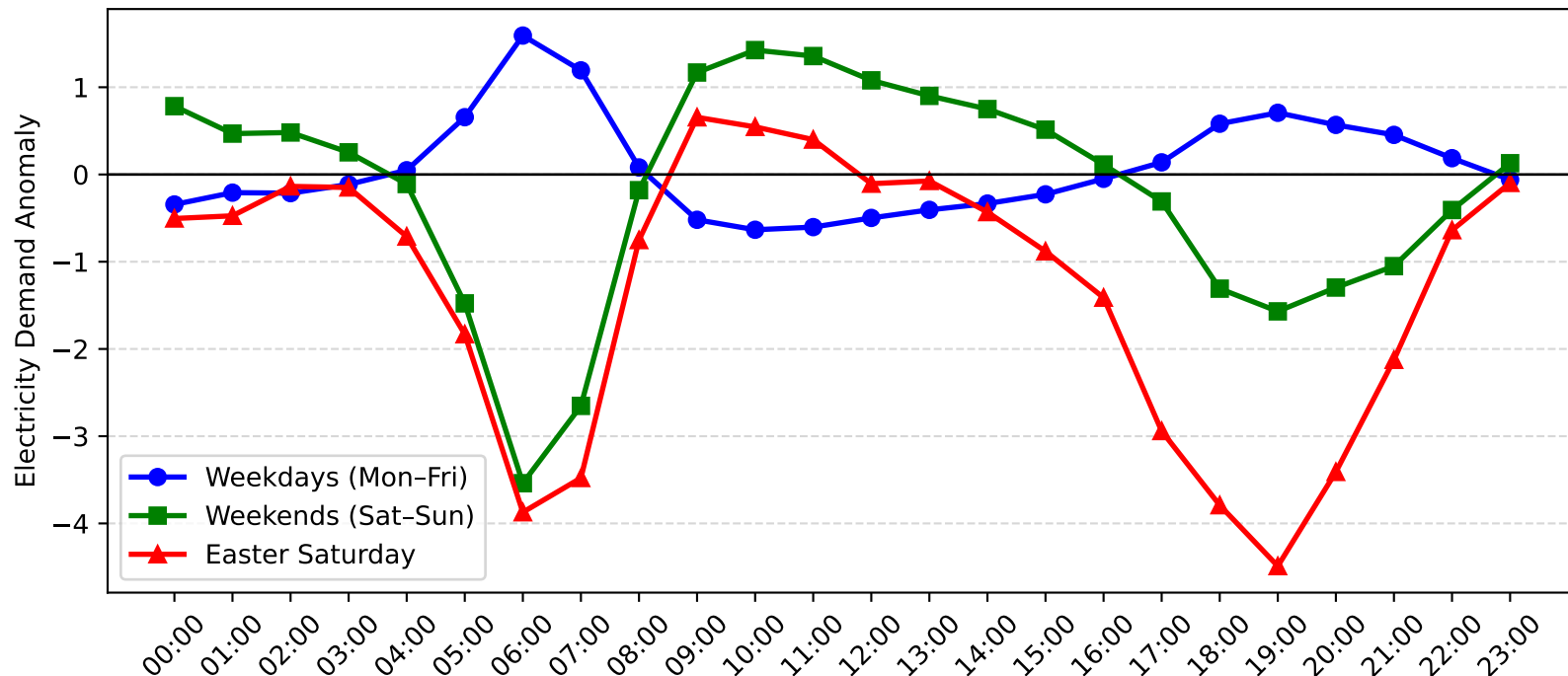
Cronulla Demand Anomaly: Easter Saturday vs Weekday/Weekend (2008-2009)
