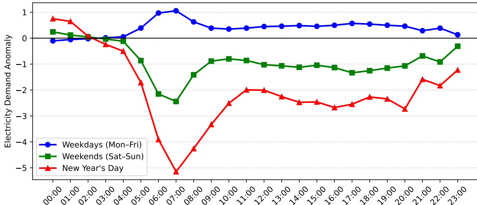
Dee Why West Demand Anomaly: New Year's Day vs Weekday/Weekend (2011-2012)
