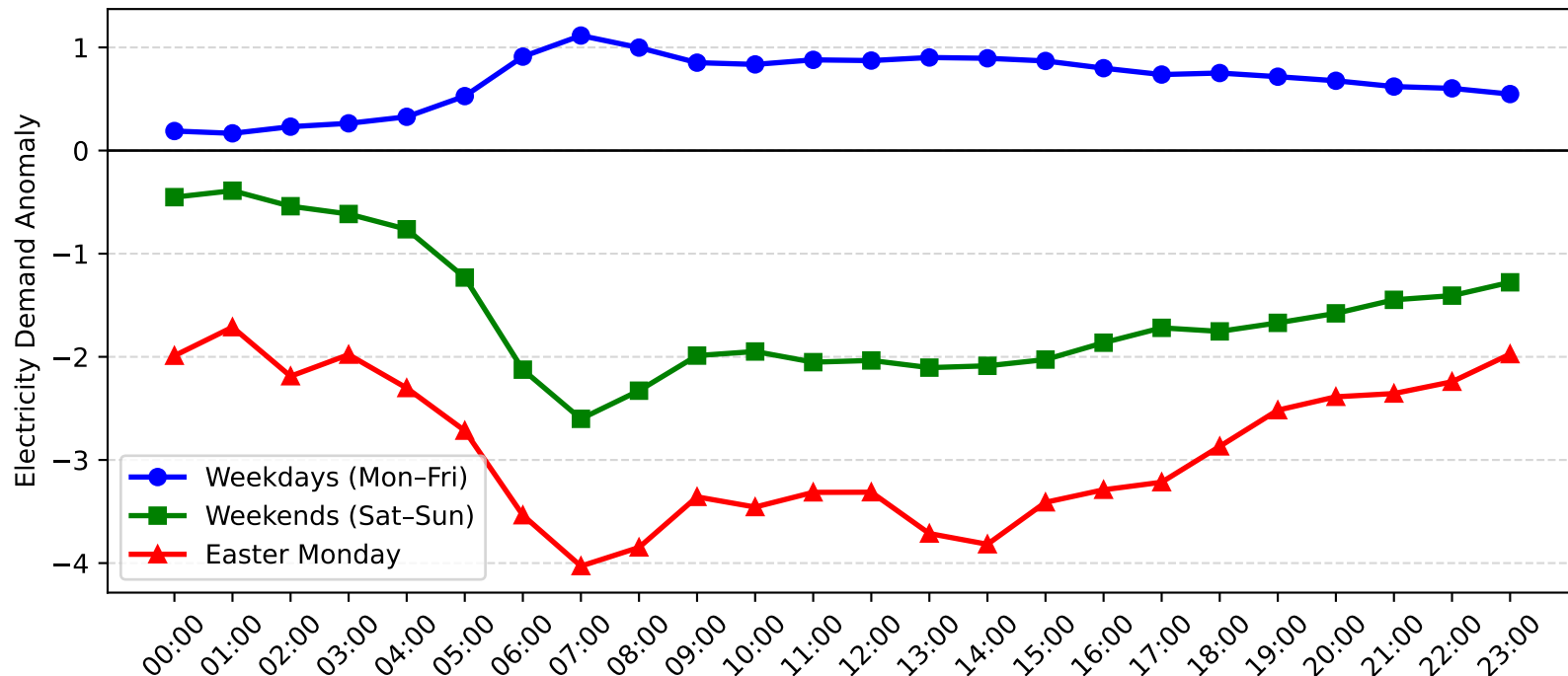
Bass Hill Demand Anomaly: Easter Monday vs Weekday/Weekend (2013-2014)
