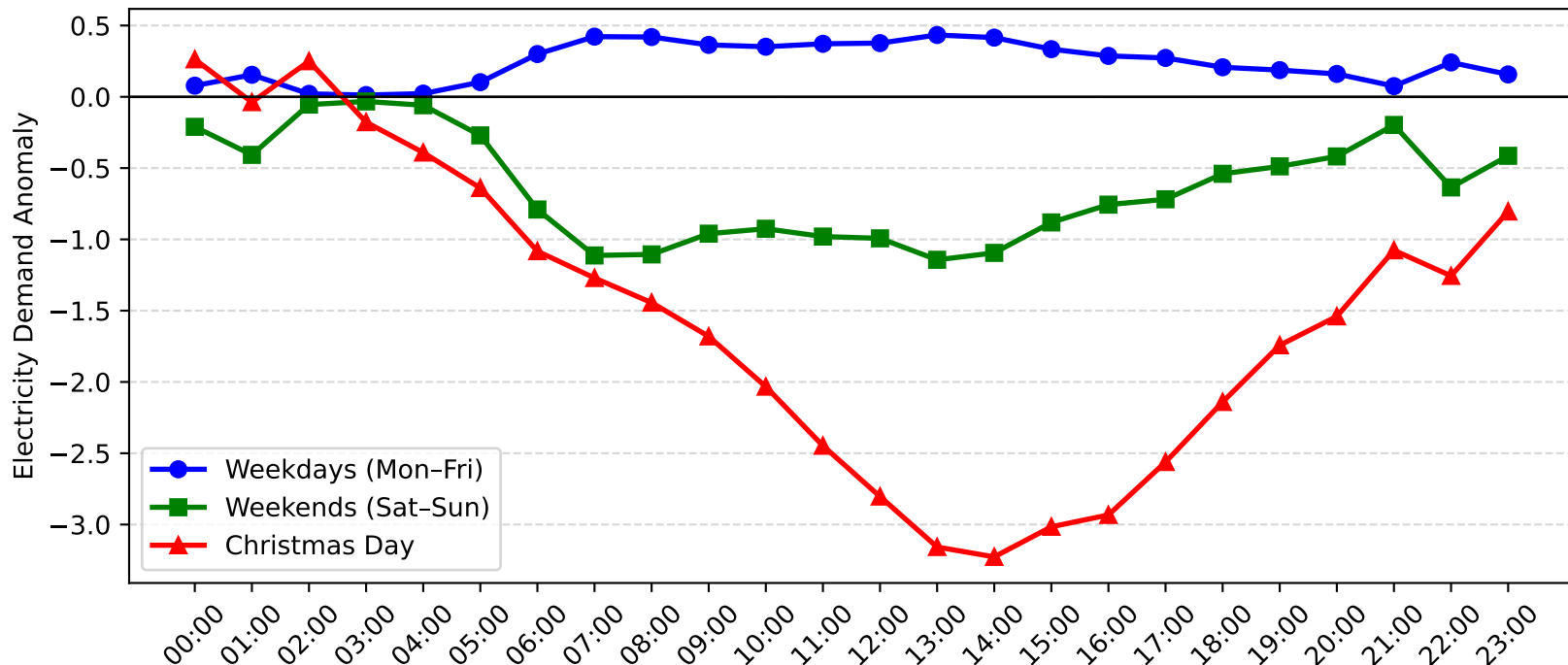
Gateshead Demand Anomaly: Christmas Day vs Weekday/Weekend (2012-2013)
