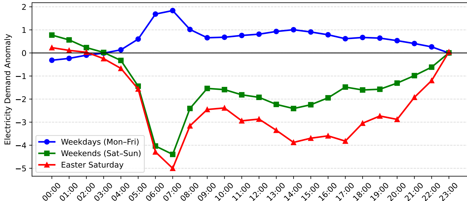
Mortdale Demand Anomaly: Easter Saturday vs Weekday/Weekend (2007-2008)
