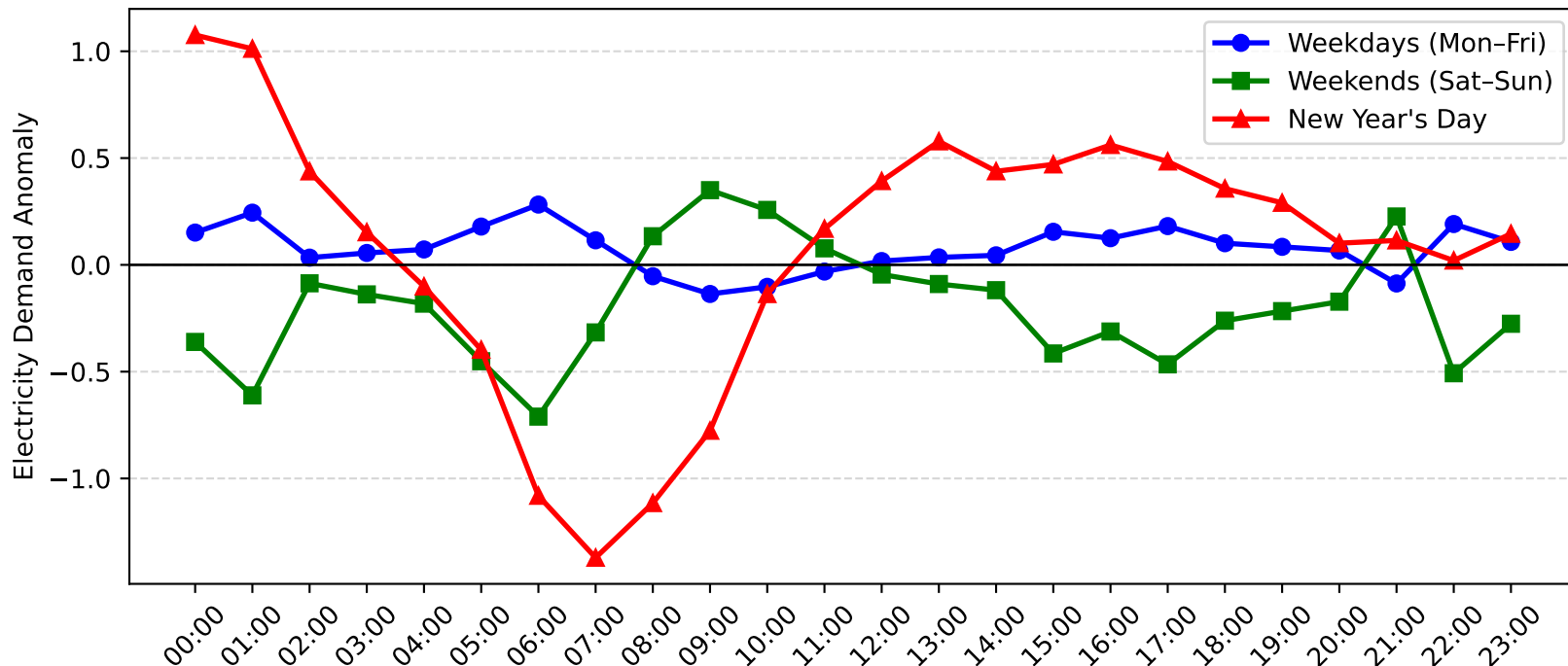
Morisset Demand Anomaly: New Year's Day vs Weekday/Weekend (2010-2011)
