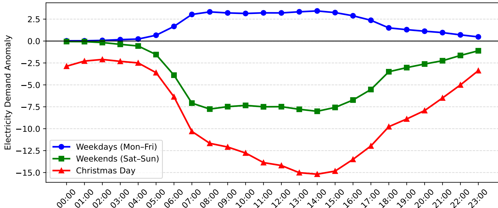
St. Peters Demand Anomaly: Christmas Day vs Weekday/Weekend (2016-2017)
