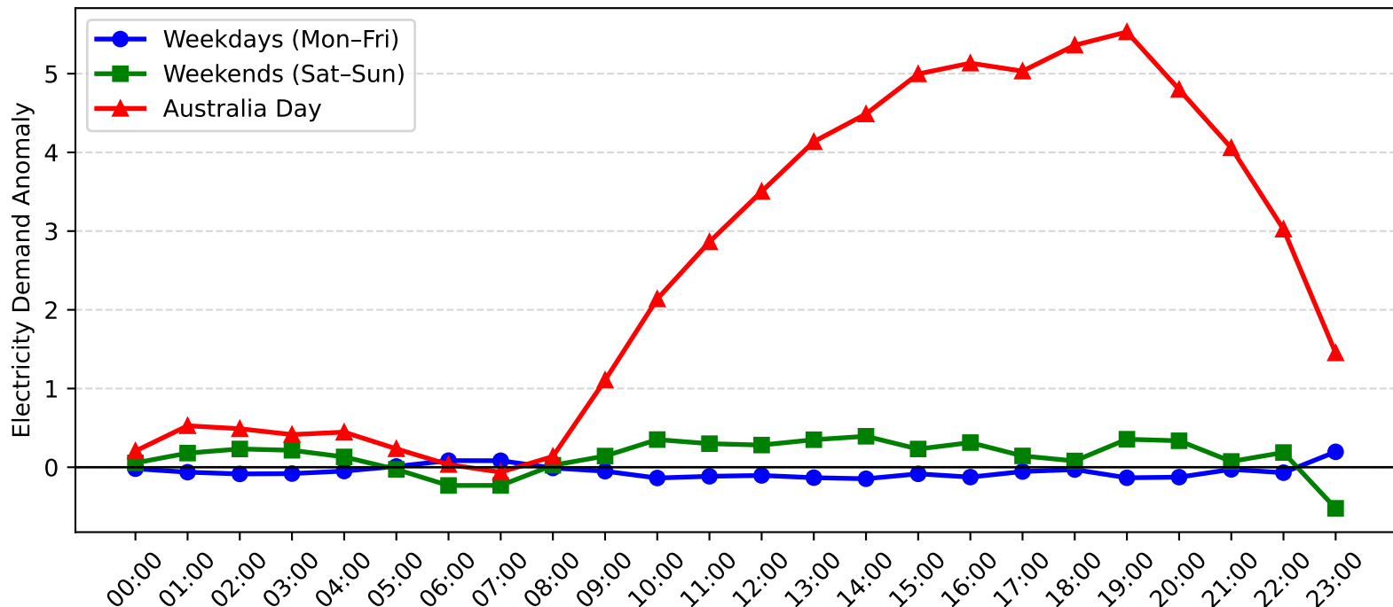
Telarah Demand Anomaly: Australia Day vs Weekday/Weekend (2010-2011)
