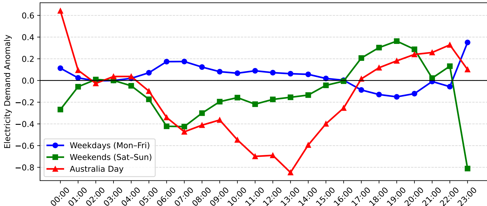
Telarah Demand Anomaly: Australia Day vs Weekday/Weekend (2007-2008)
