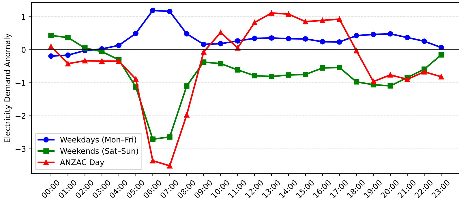
Mortdale Demand Anomaly: ANZAC Day vs Weekday/Weekend (2017-2018)
