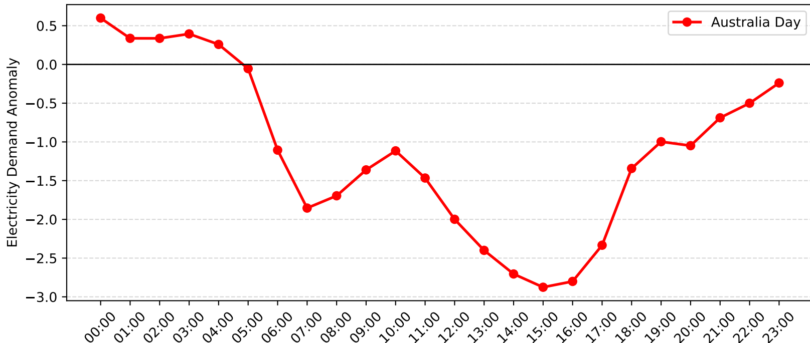
Pymble Demand Anomaly: Australia Day (2015-2016)
