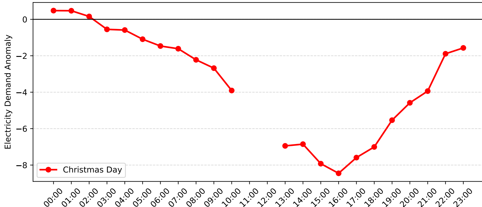
Charmhaven Demand Anomaly: Christmas Day (2008-2009)
