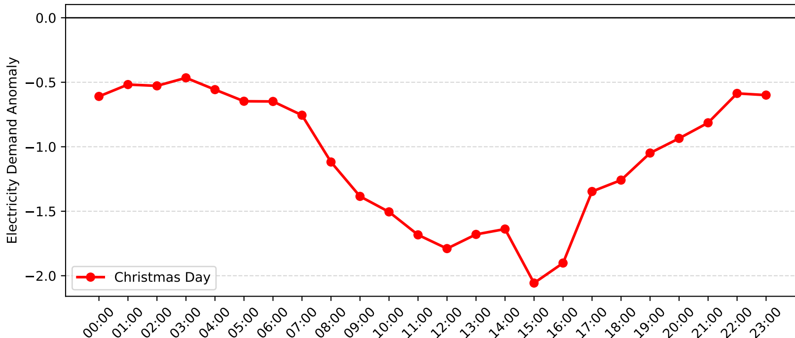
Rothbury Demand Anomaly: Christmas Day (2015-2016)
