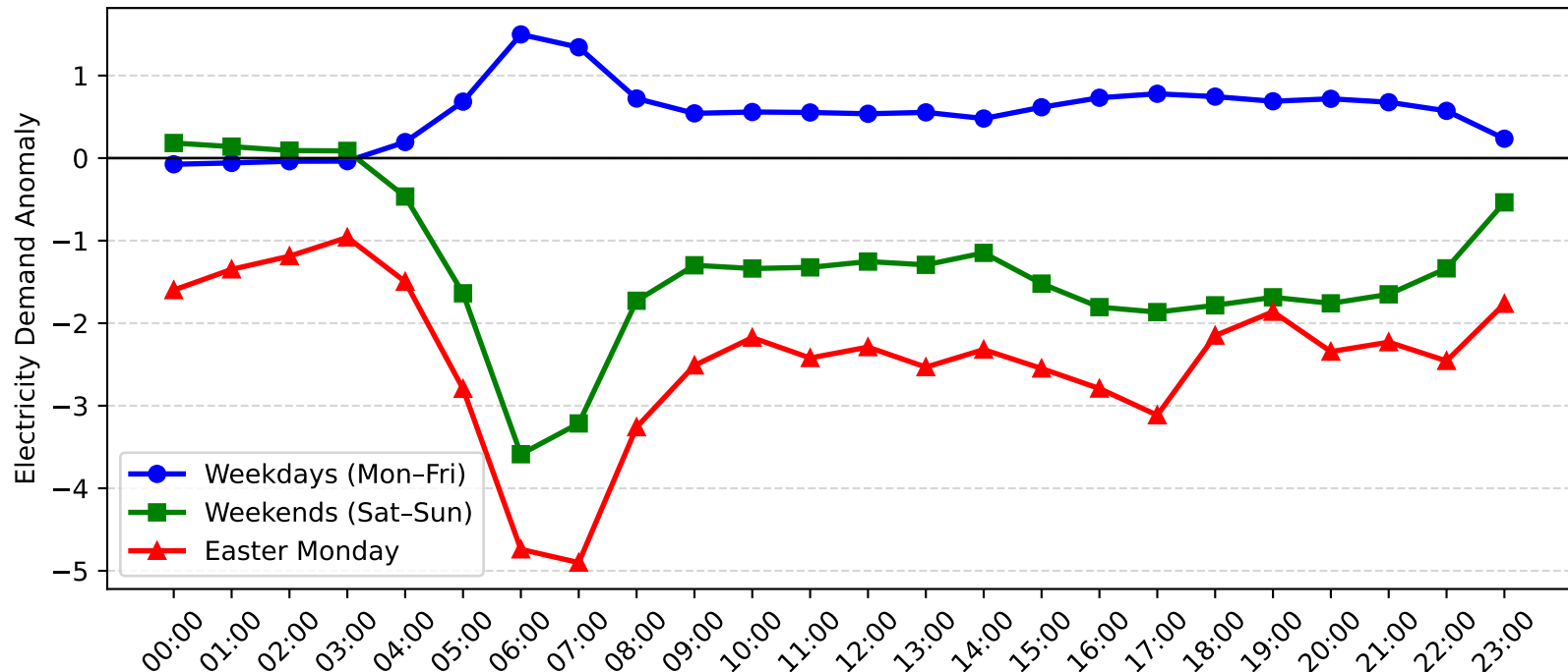
Revesby Demand Anomaly: Easter Monday vs Weekday/Weekend (2007-2008)
