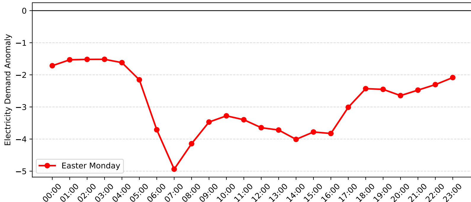
Five Dock Demand Anomaly: Easter Monday (2016-2017)
