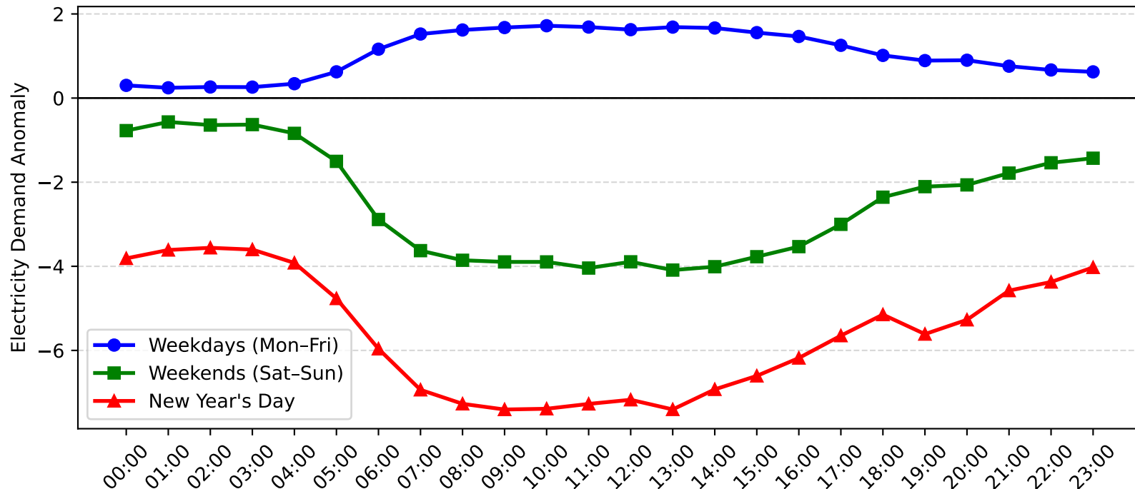
Leightonfield Demand Anomaly: New Year's Day vs Weekday/Weekend (2007-2008)
