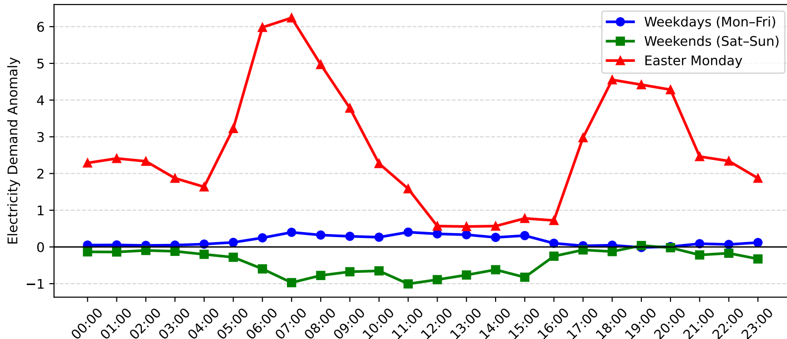
Wyong Demand Anomaly: Easter Monday vs Weekday/Weekend (2004-2005)
