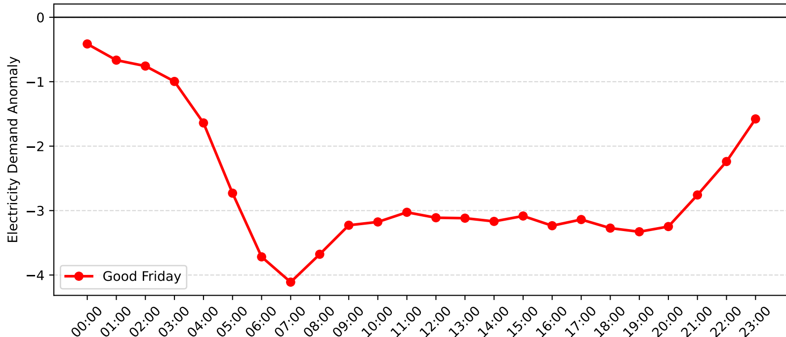
Lisarow Demand Anomaly: Good Friday (2011-2012)
