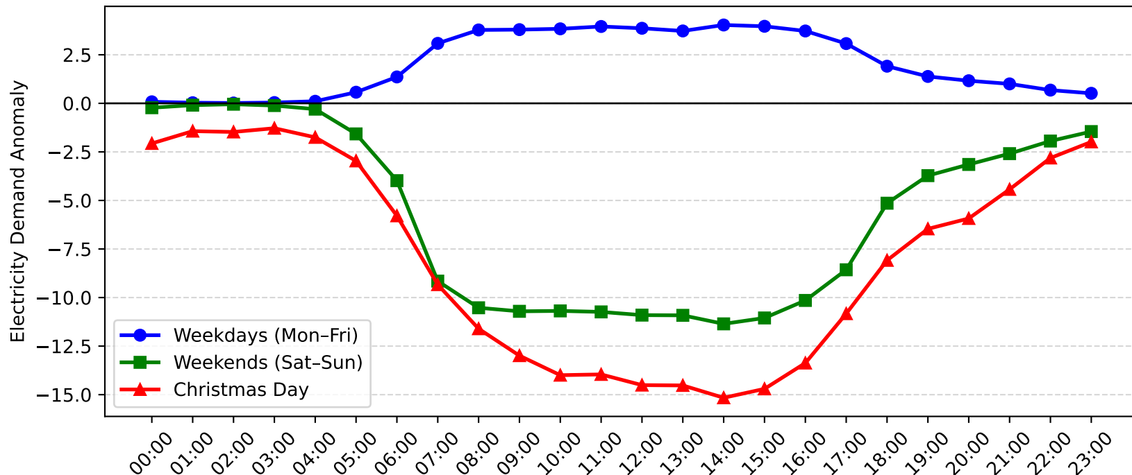
Gore Hill Demand Anomaly: Christmas Day vs Weekday/Weekend (2013-2014)
