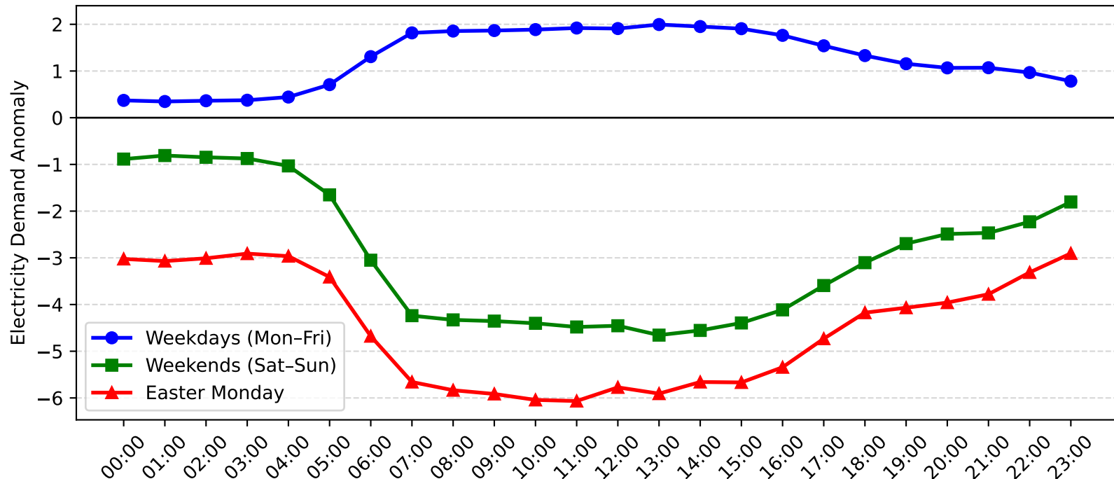
Leightonfield Demand Anomaly: Easter Monday vs Weekday/Weekend (2014-2015)
