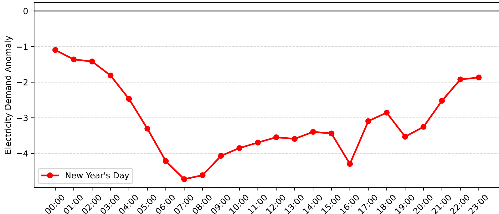
Lisarow Demand Anomaly: New Year's Day (2007-2008)
