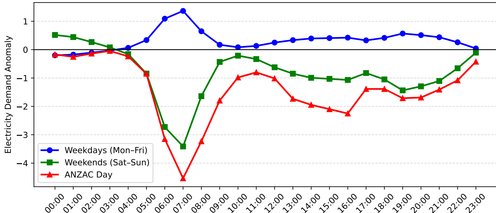
Five Dock Demand Anomaly: ANZAC Day vs Weekday/Weekend (2011-2012)
