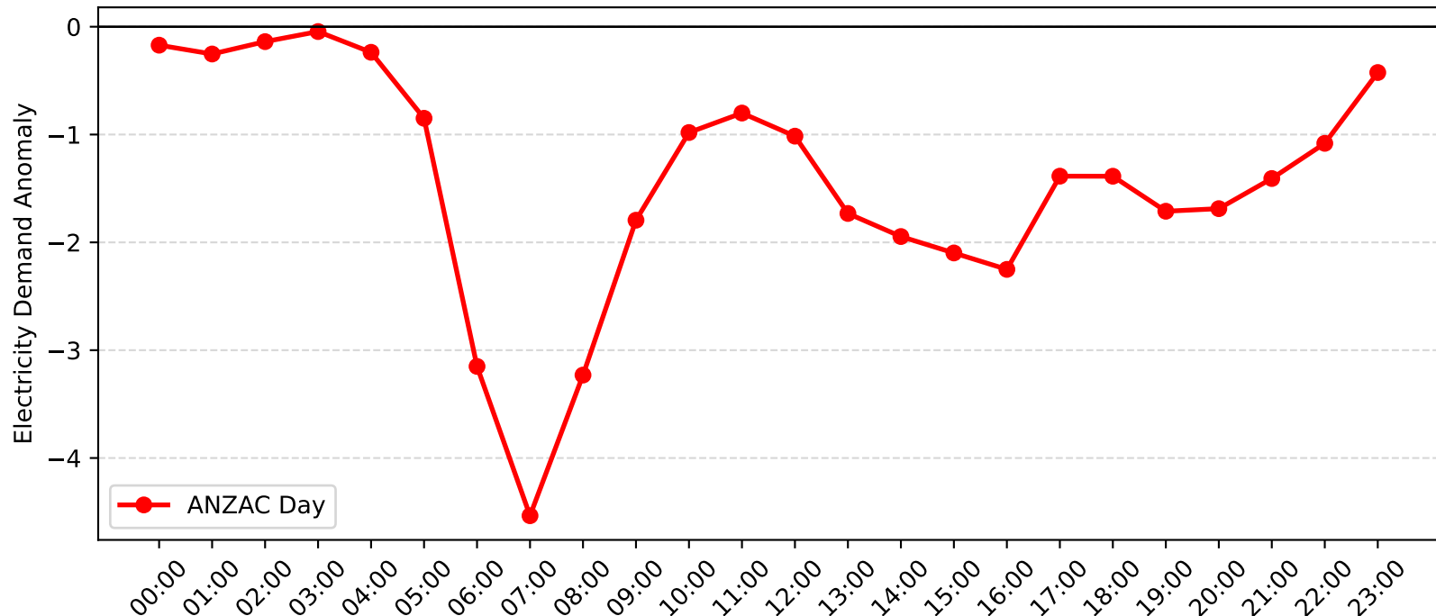
Five Dock Demand Anomaly: ANZAC Day (2011-2012)
