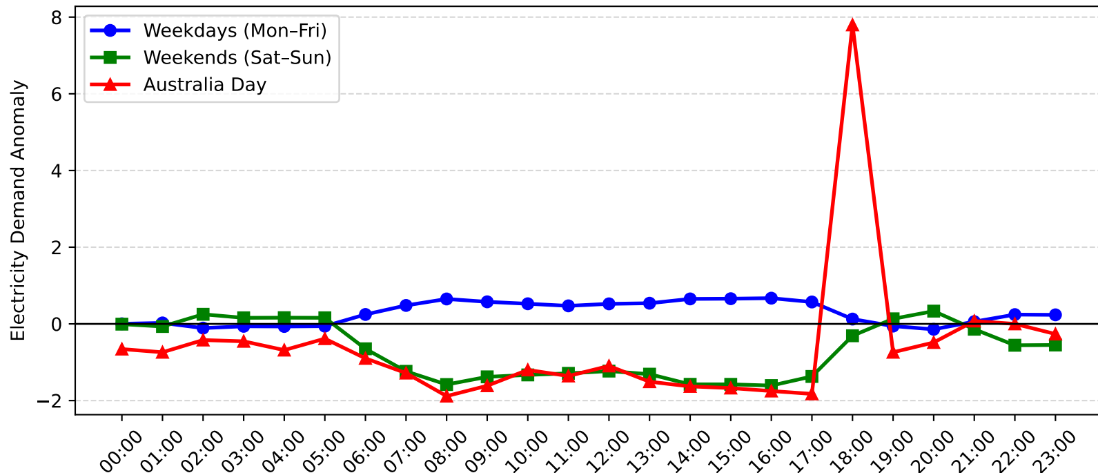
Mosman Demand Anomaly: Australia Day vs Weekday/Weekend (2004-2005)
