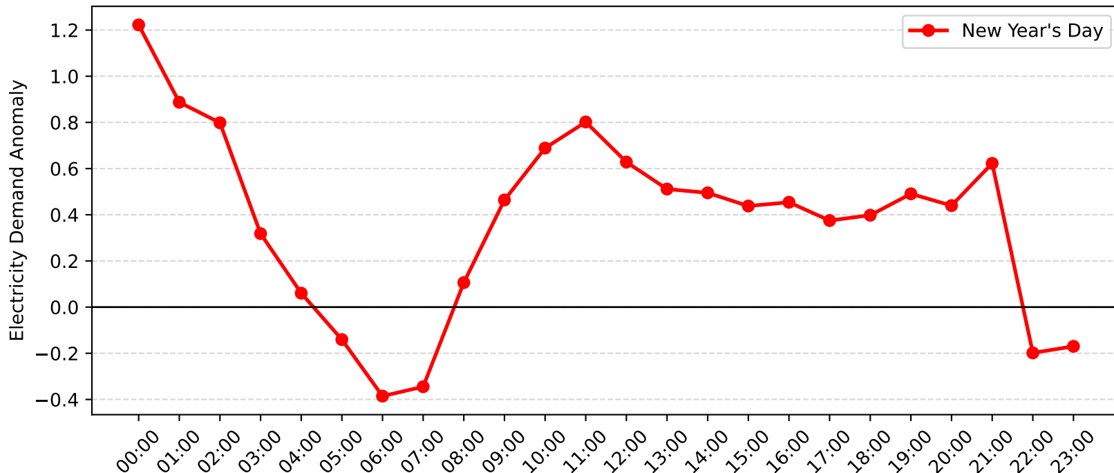
Swansea Demand Anomaly: New Year's Day (2013-2014)
