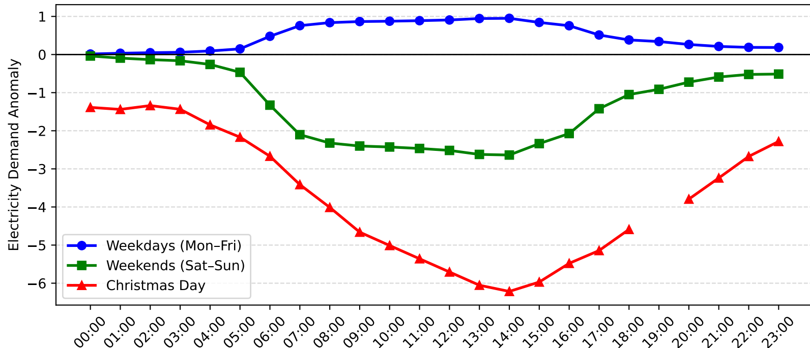
Caringbah Demand Anomaly: Christmas Day vs Weekday/Weekend (2012-2013)
