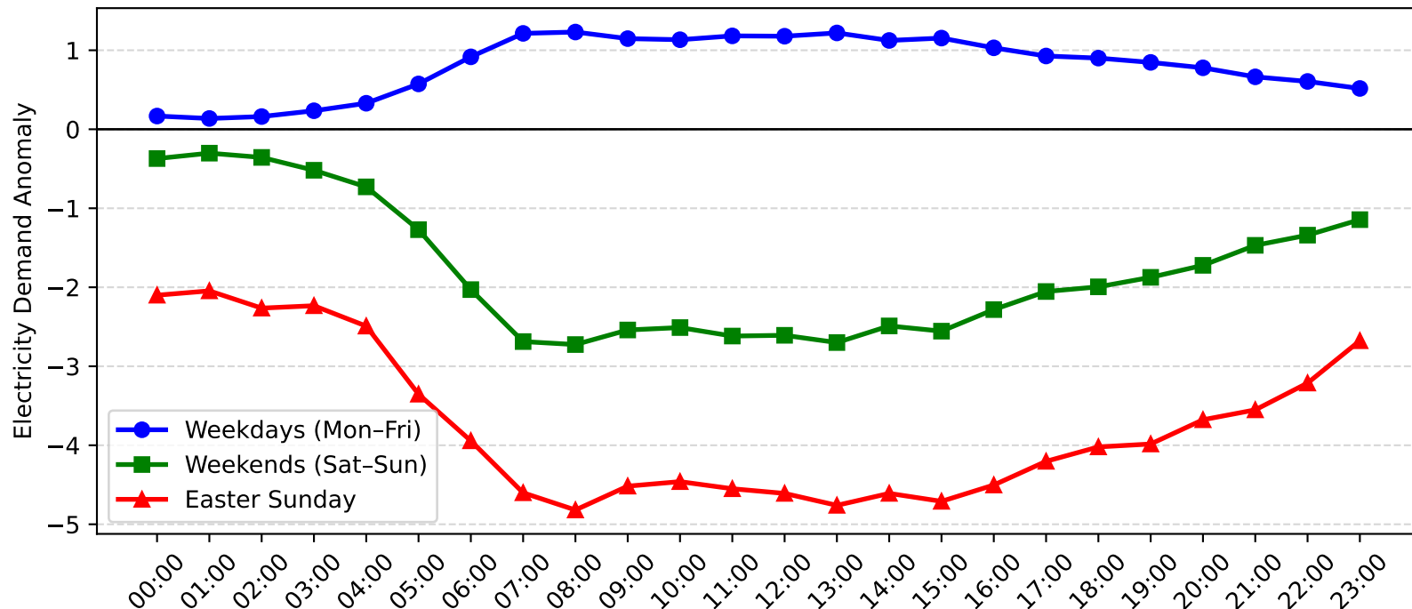
Bass Hill Demand Anomaly: Easter Sunday vs Weekday/Weekend (2017-2018)
