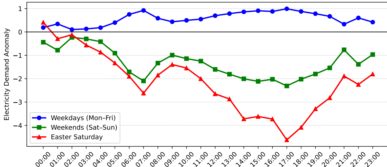
Jesmond Demand Anomaly: Easter Saturday vs Weekday/Weekend (2015-2016)
