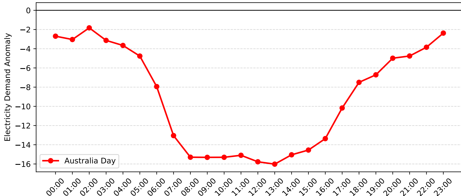
Gore Hill Demand Anomaly: Australia Day (2006-2007)
