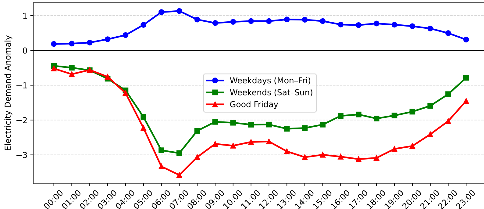
Lisarow Demand Anomaly: Good Friday vs Weekday/Weekend (2012-2013)
