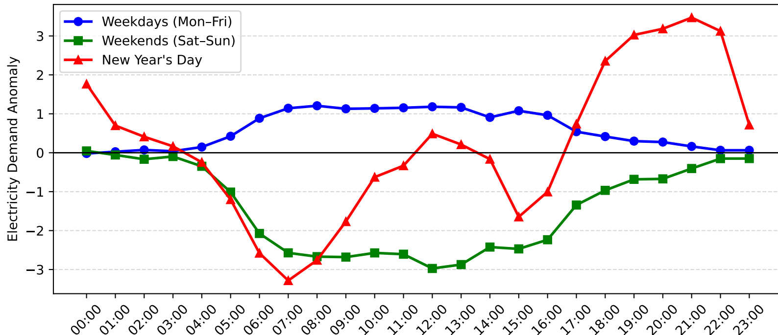
Wyong Demand Anomaly: New Year's Day vs Weekday/Weekend (2006-2007)
