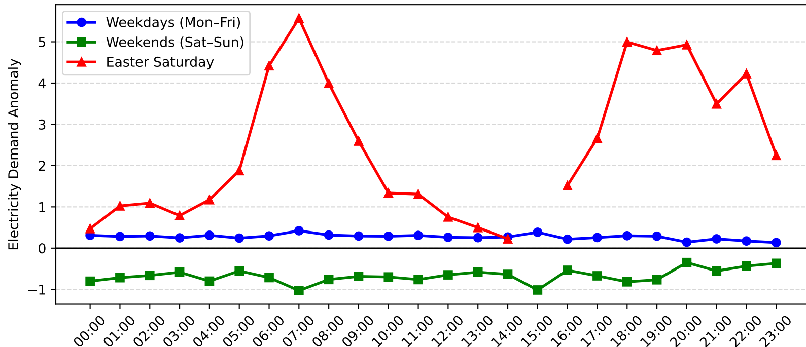
Lisarow Demand Anomaly: Easter Saturday vs Weekday/Weekend (2004-2005)
