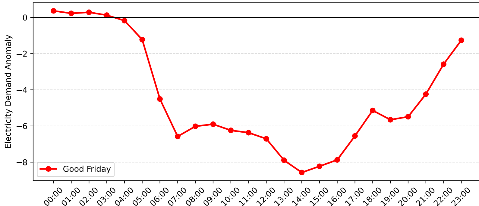
Hunters Hill Demand Anomaly: Good Friday (2007-2008)
