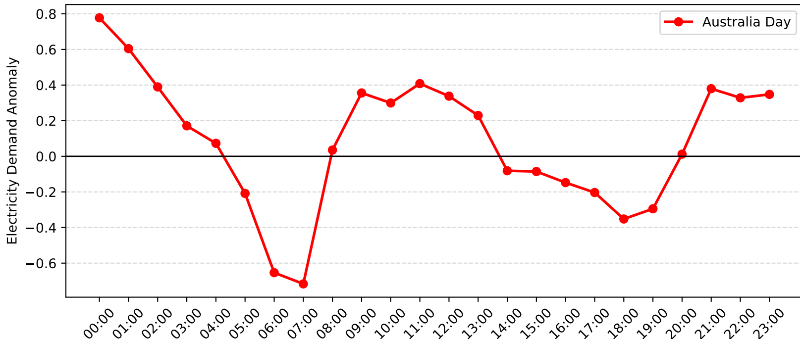
Morisset Demand Anomaly: Australia Day (2012-2013)
