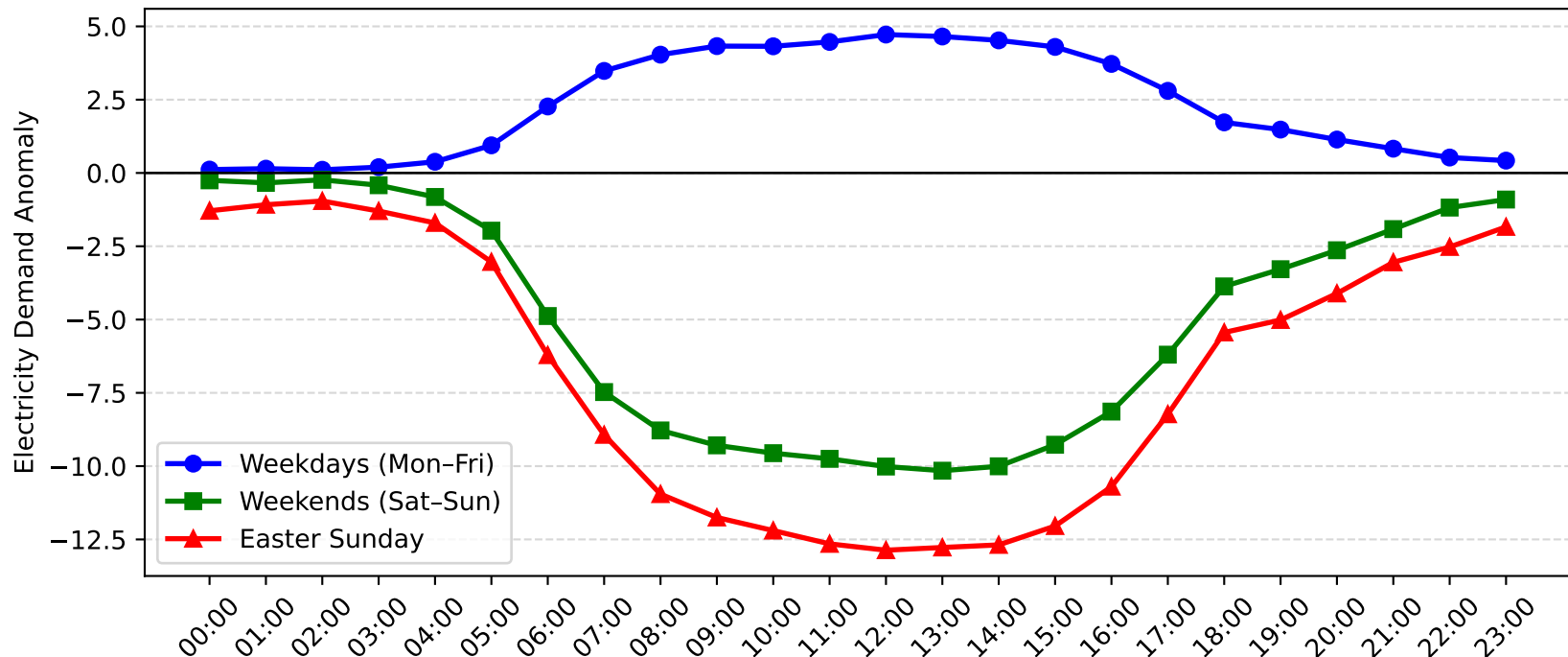
Mascot Demand Anomaly: Easter Sunday vs Weekday/Weekend (2009-2010)
