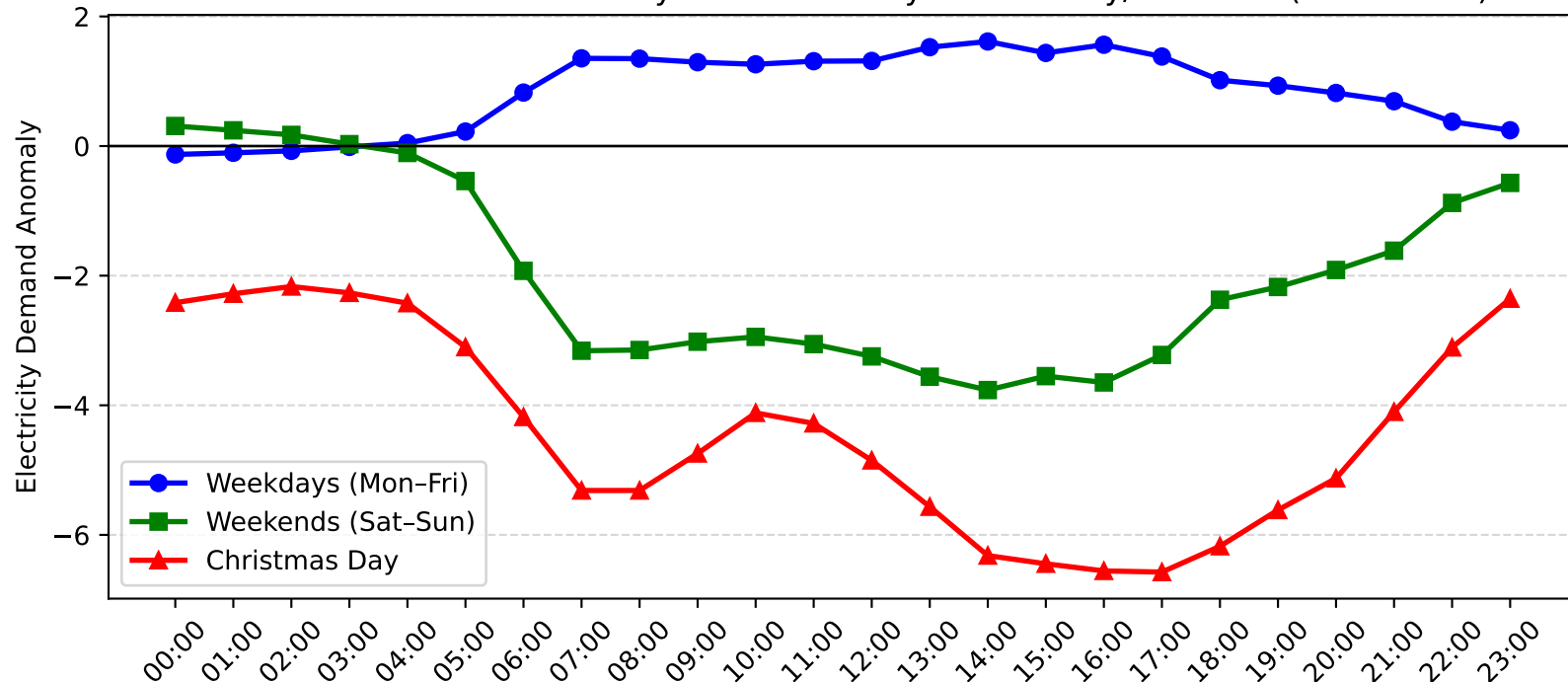
Hunters Hill Demand Anomaly: Christmas Day vs Weekday/Weekend (2016-2017)
