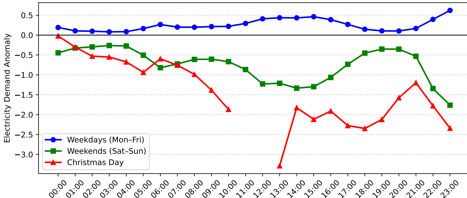
Muswellbrook Demand Anomaly: Christmas Day vs Weekday/Weekend (2008-2009)
