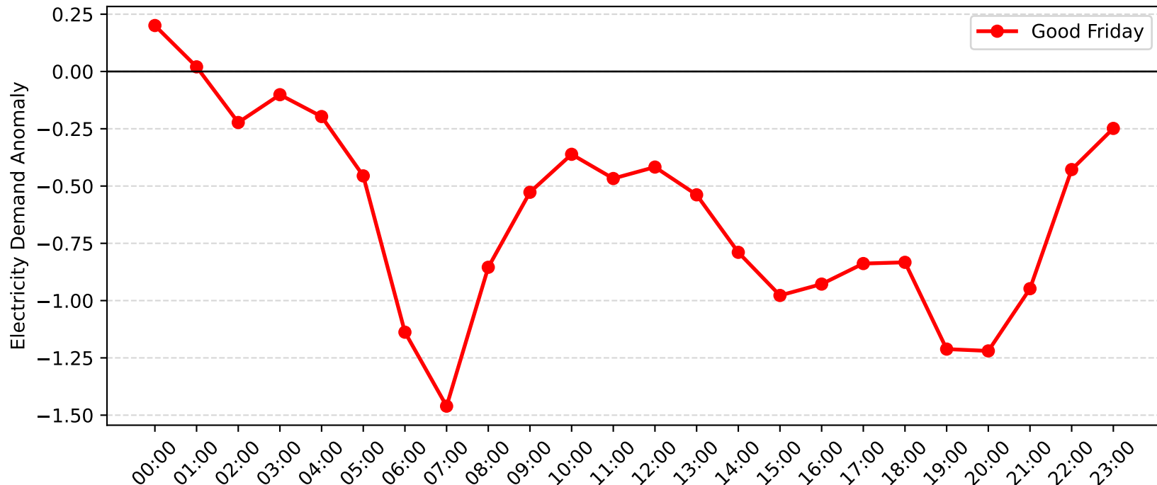
Blakehurst Demand Anomaly: Good Friday (2017-2018)
