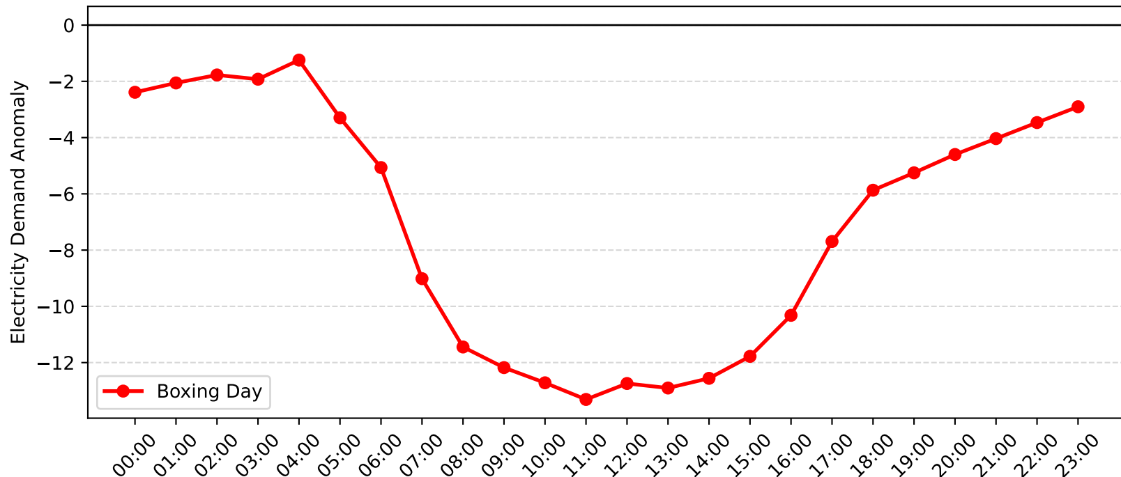
Gore Hill Demand Anomaly: Boxing Day (2011-2012)
