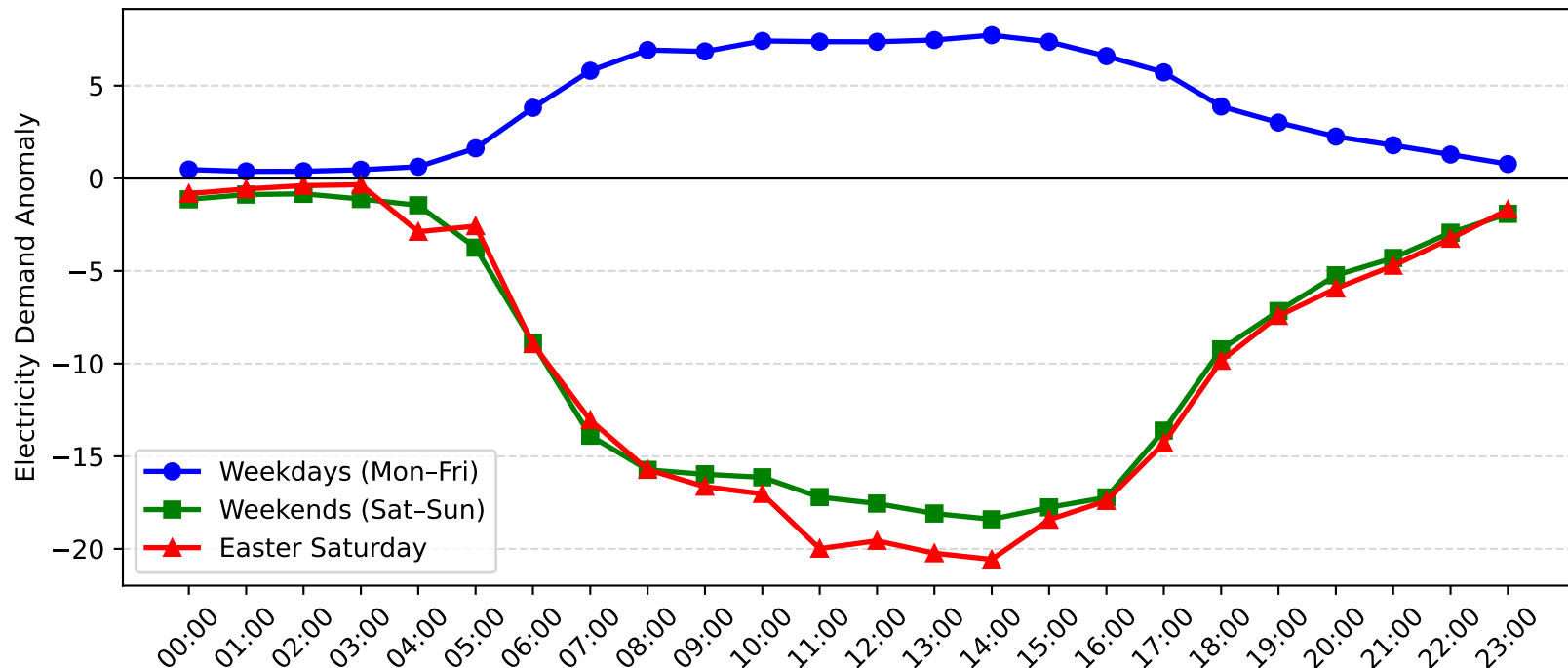
Gore Hill Demand Anomaly: Easter Saturday vs Weekday/Weekend (2005-2006)
