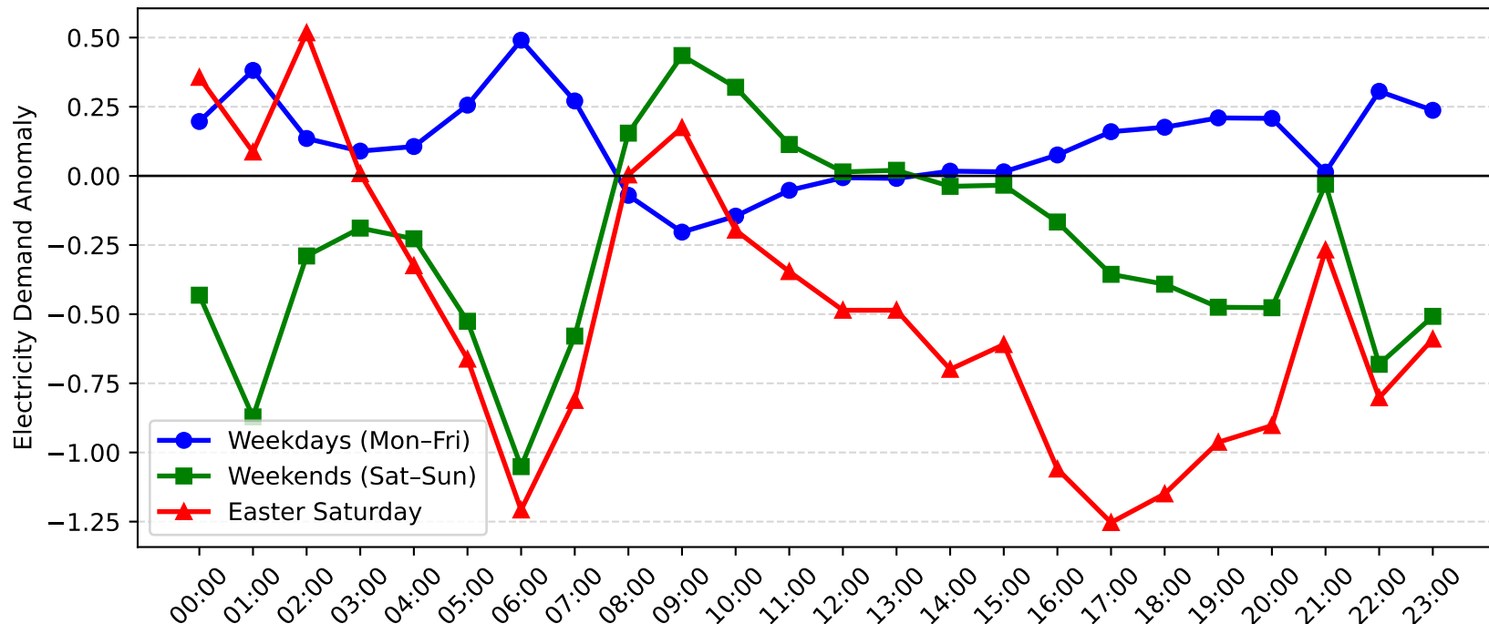
Morisset Demand Anomaly: Easter Saturday vs Weekday/Weekend (2010-2011)
