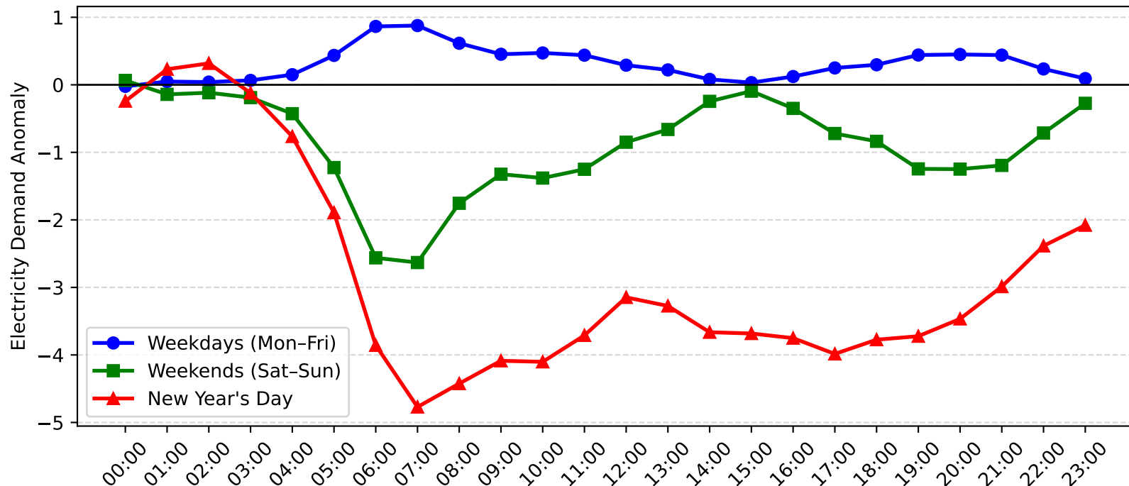
Revesby Demand Anomaly: New Year's Day vs Weekday/Weekend (2015-2016)
