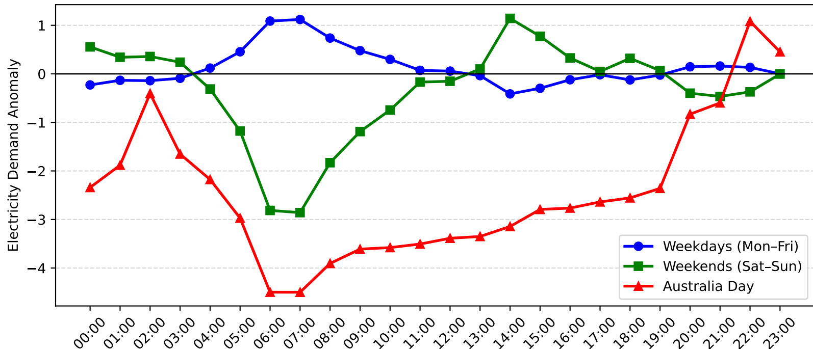
Revesby Demand Anomaly: Australia Day vs Weekday/Weekend (2006-2007)
