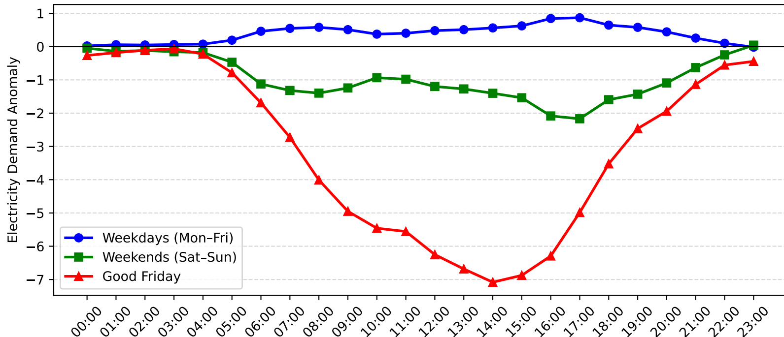
Erina Demand Anomaly: Good Friday vs Weekday/Weekend (2015-2016)
