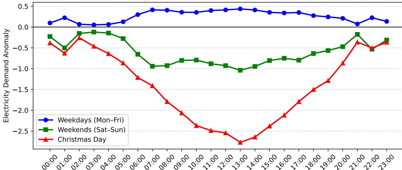
Gateshead Demand Anomaly: Christmas Day vs Weekday/Weekend (2010-2011)
