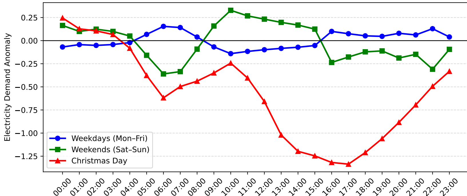
Narrabeen Demand Anomaly: Christmas Day vs Weekday/Weekend (2011-2012)
