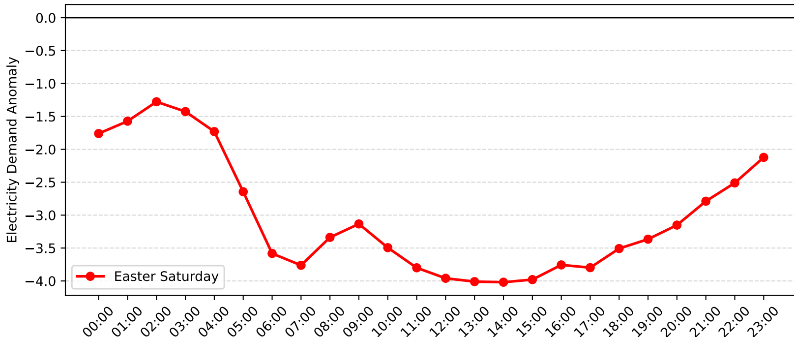
Lisarow Demand Anomaly: Easter Saturday (2016-2017)
