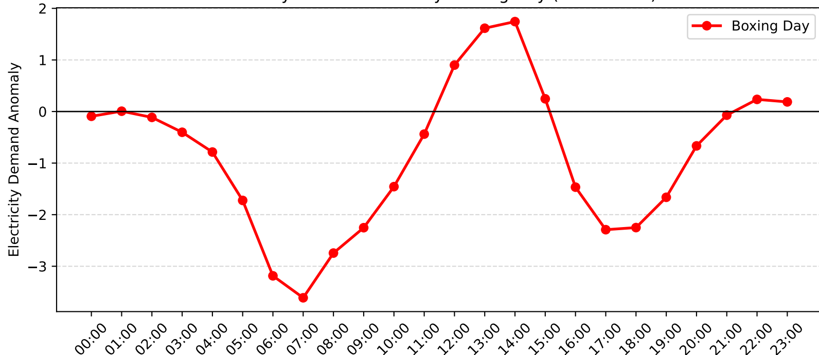
Revesby Demand Anomaly: Boxing Day (2015-2016)
