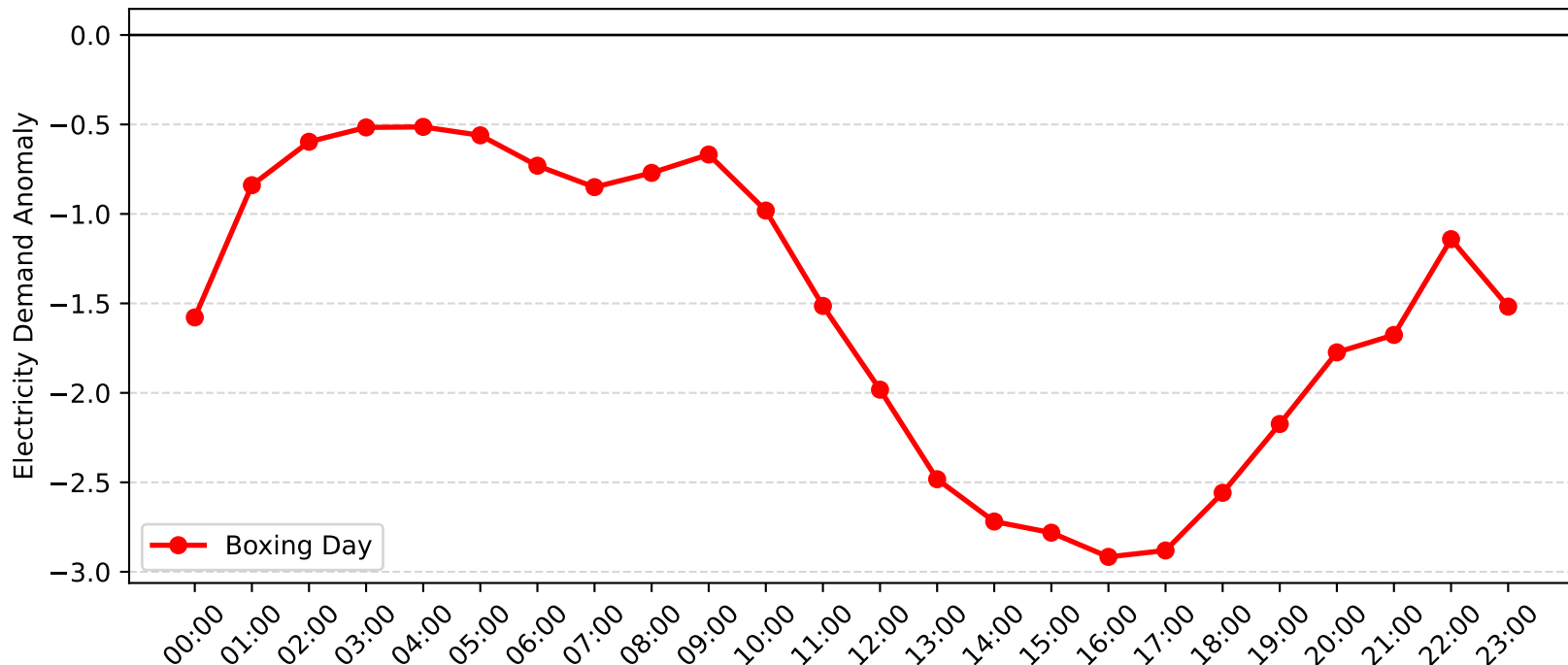
Telarah Demand Anomaly: Boxing Day (2012-2013)
