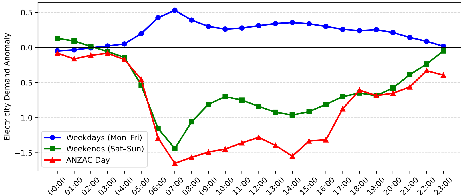
Rockdale Demand Anomaly: ANZAC Day vs Weekday/Weekend (2012-2013)
