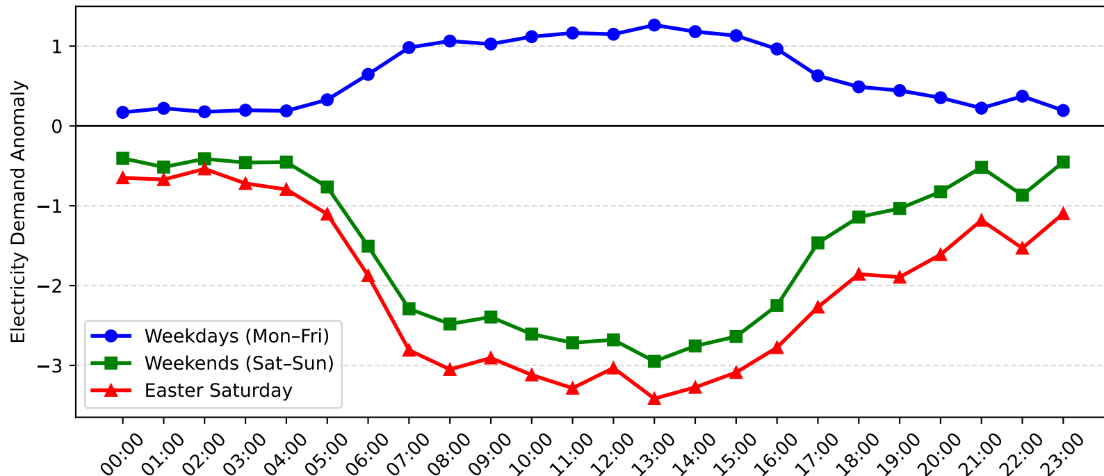
Mayfield West Demand Anomaly: Easter Saturday vs Weekday/Weekend (2014-2015)
