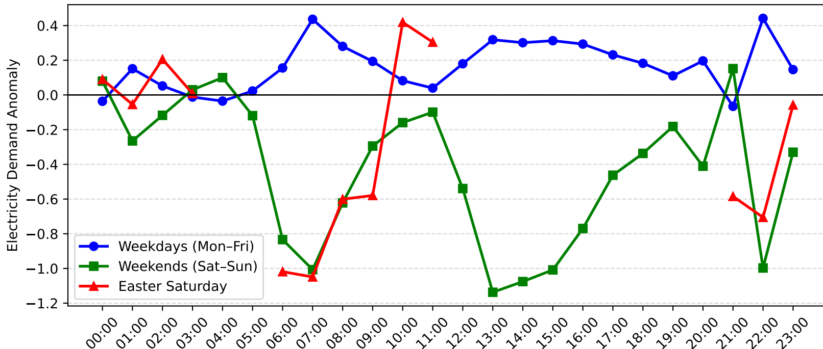
Adamstown Demand Anomaly: Easter Saturday vs Weekday/Weekend (2014-2015)
