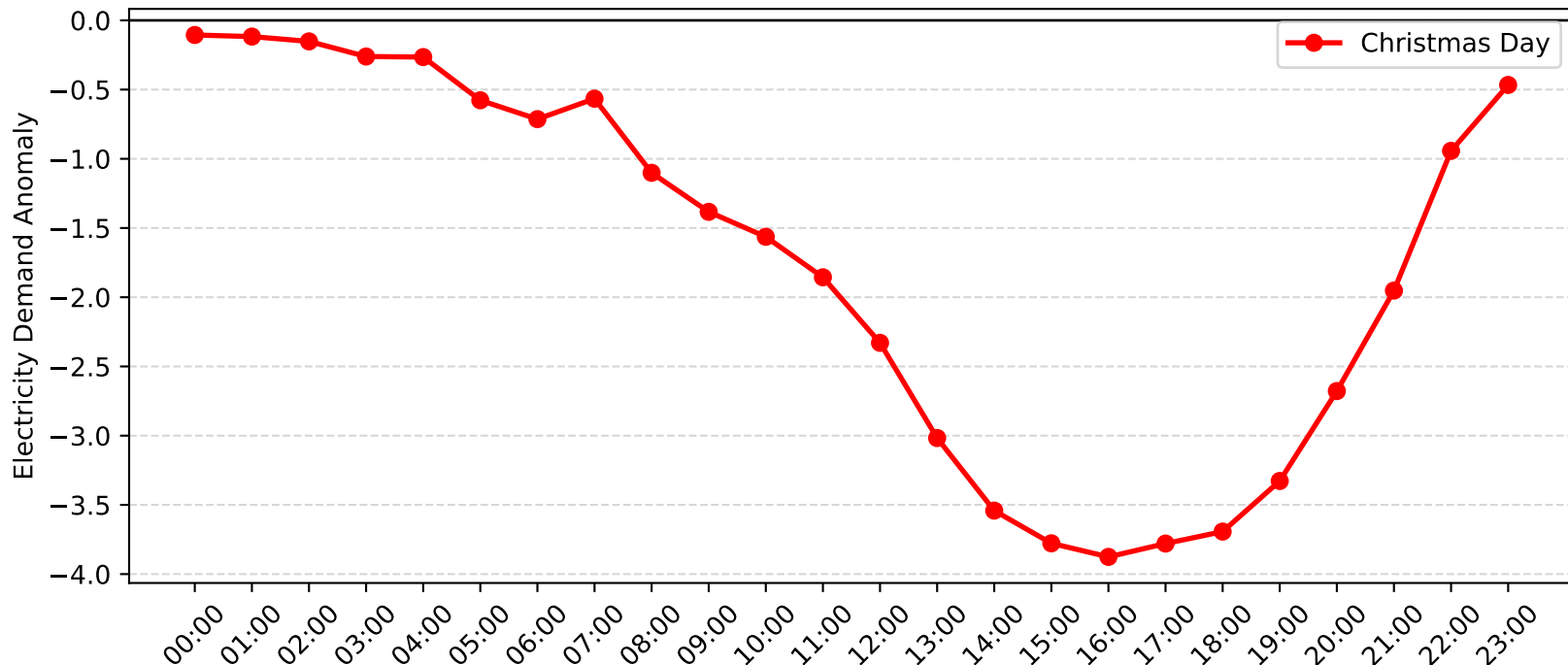
Muswellbrook Demand Anomaly: Christmas Day (2013-2014)
