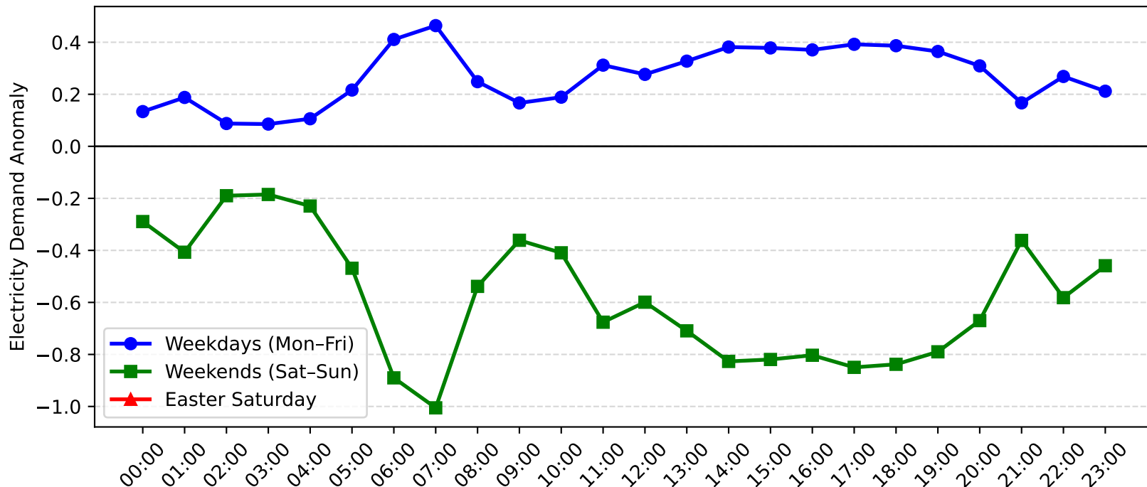
Maryland Demand Anomaly: Easter Saturday vs Weekday/Weekend (2017-2018)
