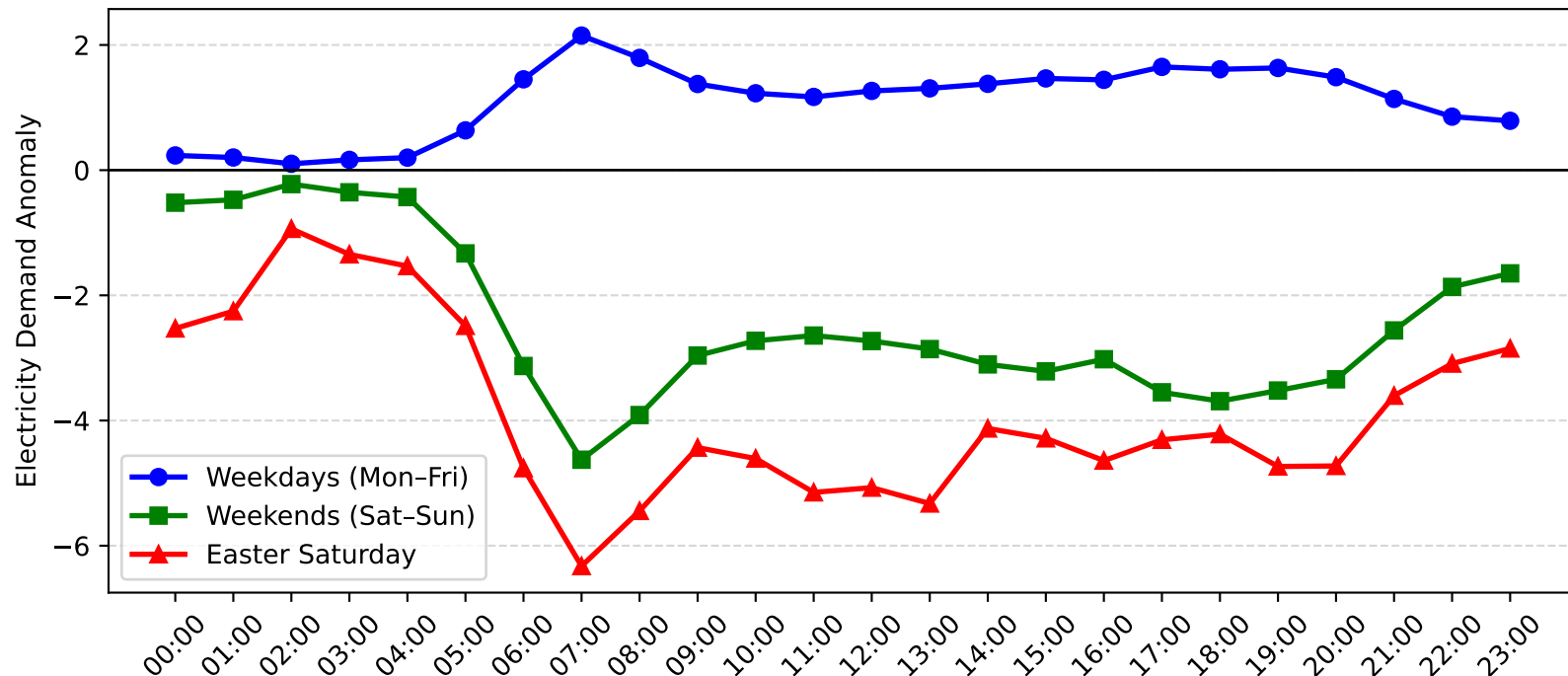
Maroubra Demand Anomaly: Easter Saturday vs Weekday/Weekend (2009-2010)
