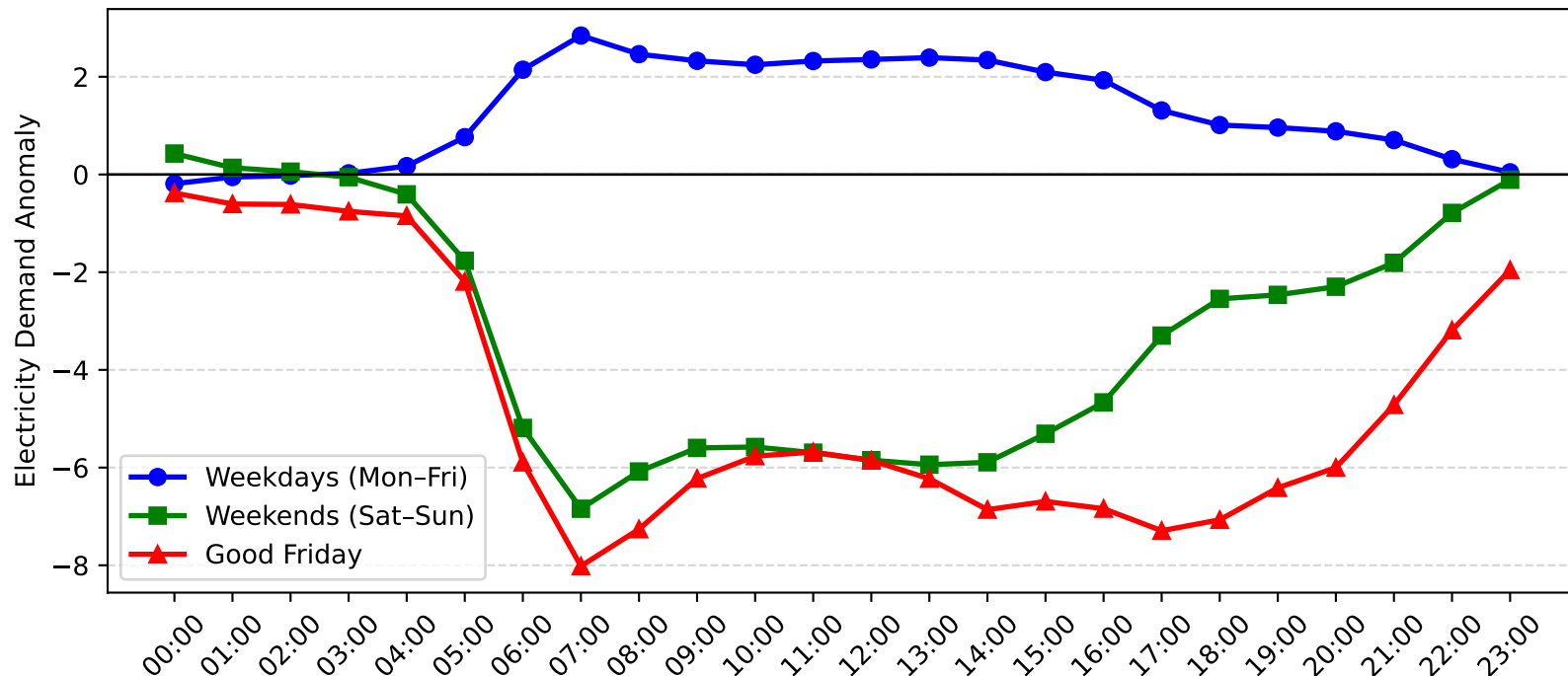
Hunters Hill Demand Anomaly: Good Friday vs Weekday/Weekend (2010-2011)
