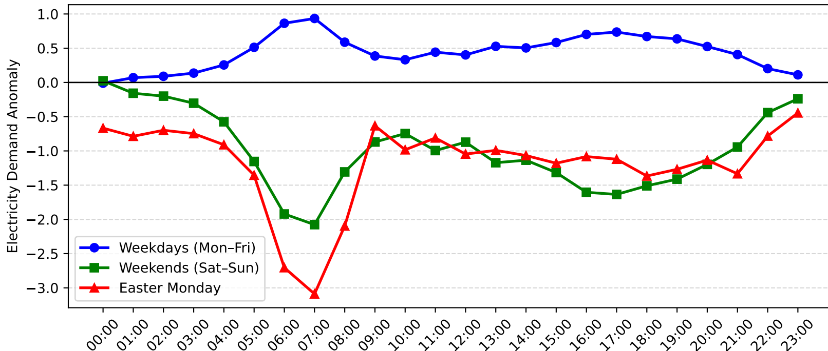
Charmhaven Demand Anomaly: Easter Monday vs Weekday/Weekend (2008-2009)
