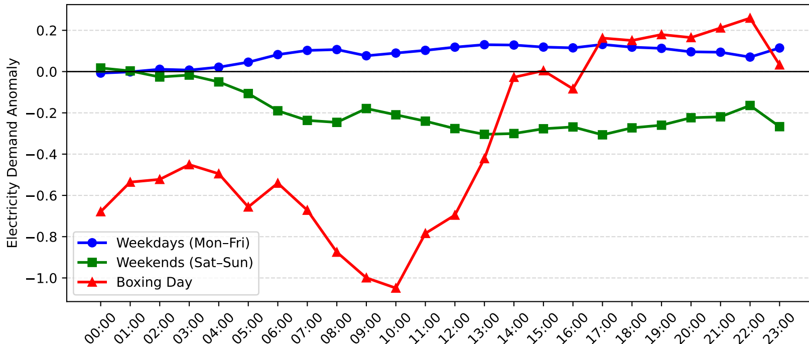
Rothbury Demand Anomaly: Boxing Day vs Weekday/Weekend (2015-2016)
