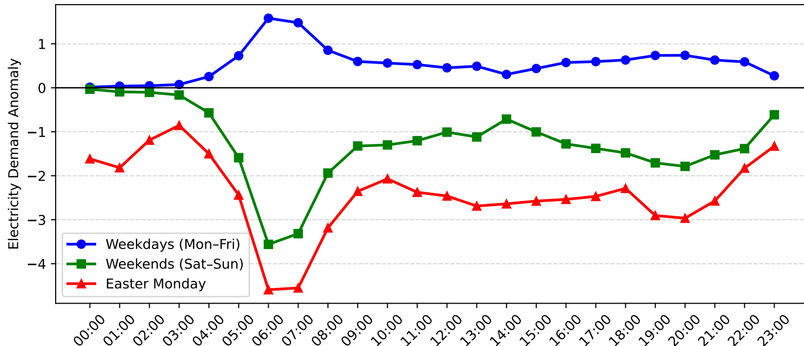
Revesby Demand Anomaly: Easter Monday vs Weekday/Weekend (2009-2010)
