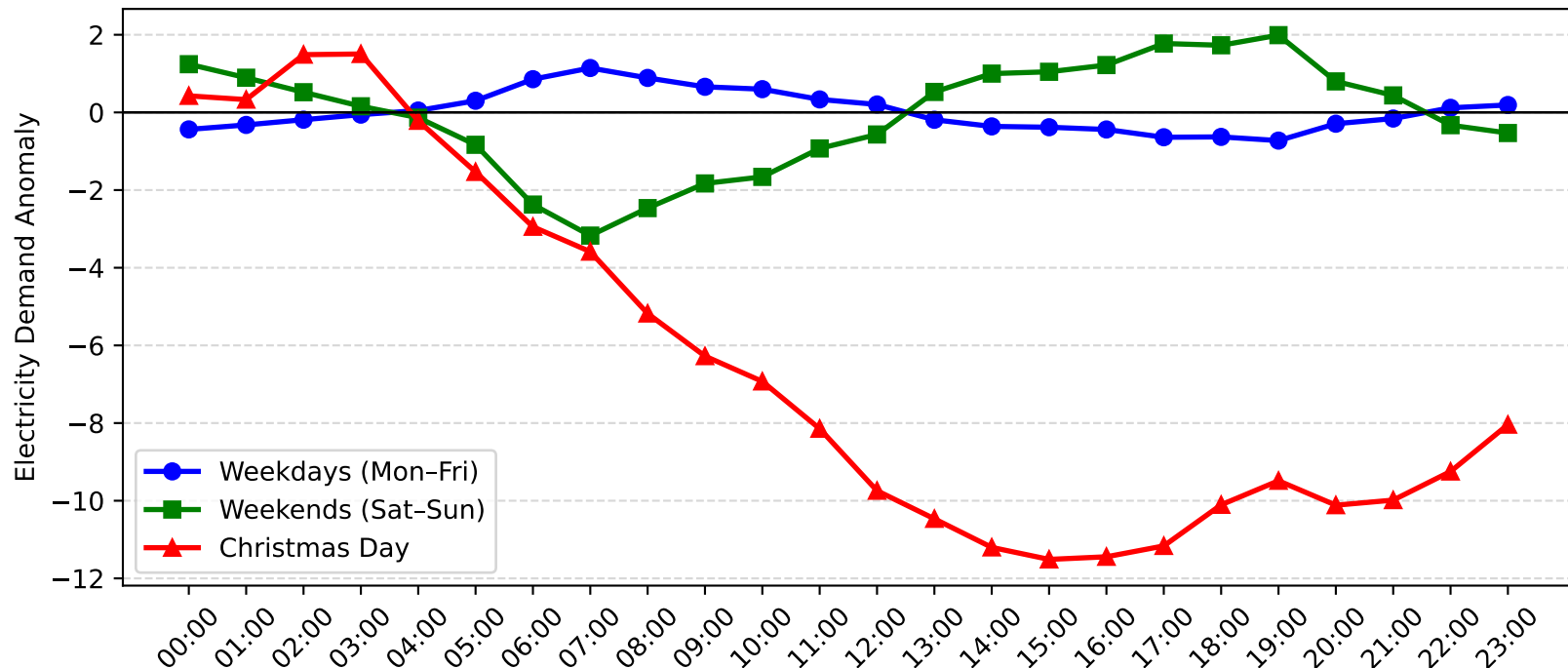
Meadowbank Demand Anomaly: Christmas Day vs Weekday/Weekend (2012-2013)
