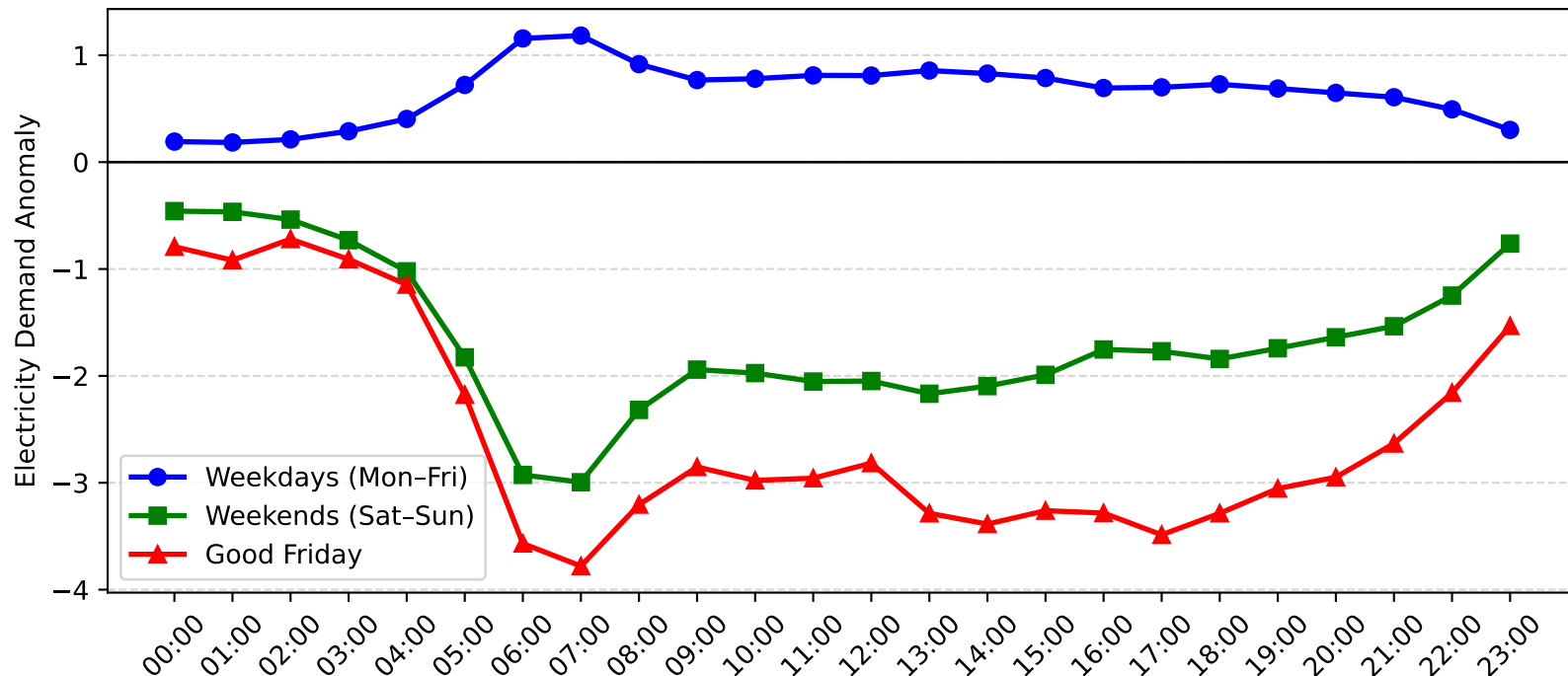
Lisarow Demand Anomaly: Good Friday vs Weekday/Weekend (2013-2014)
