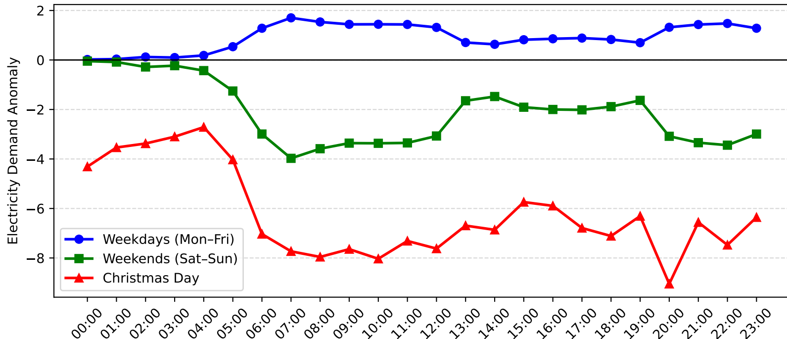
Meadowbank Demand Anomaly: Christmas Day vs Weekday/Weekend (2016-2017)
