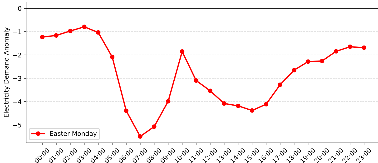
Kogarah Demand Anomaly: Easter Monday (2016-2017)
