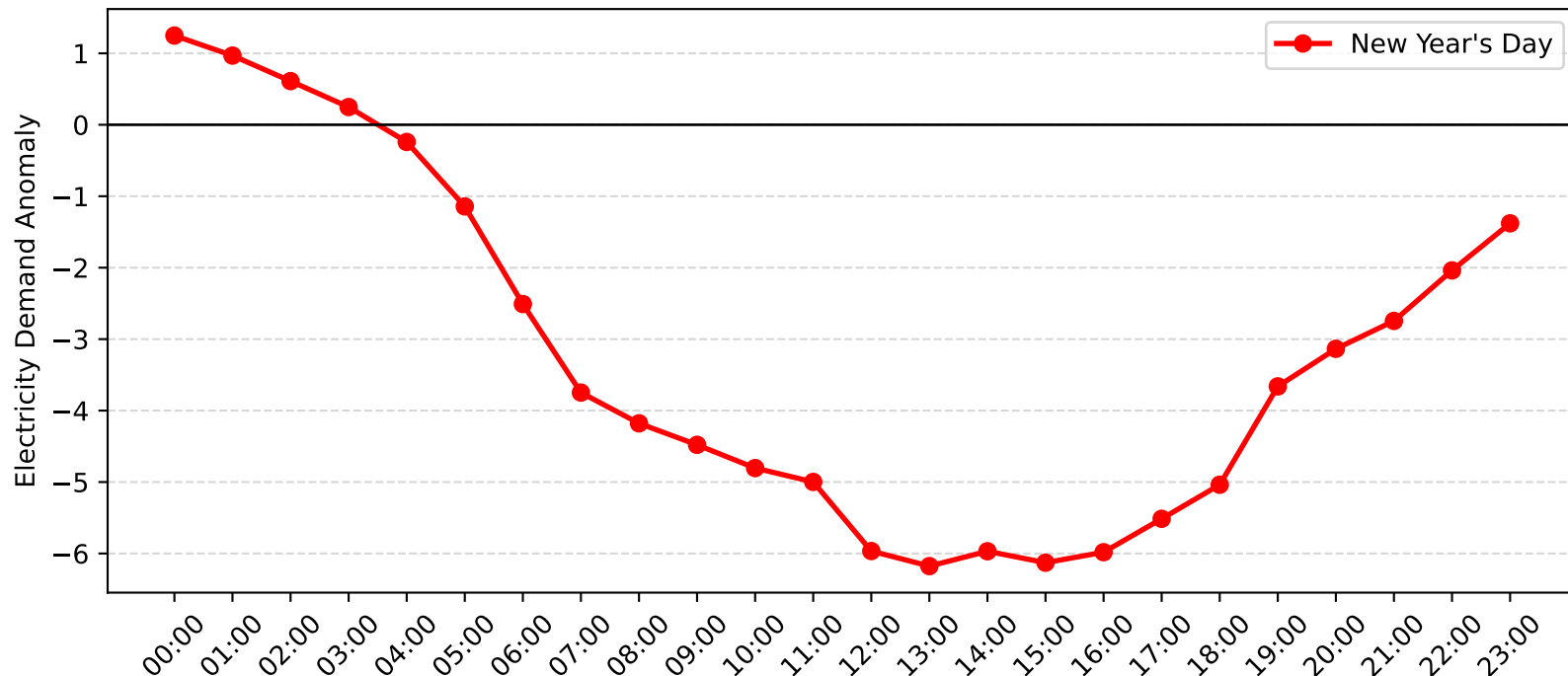
Wyong Demand Anomaly: New Year's Day (2017-2018)
