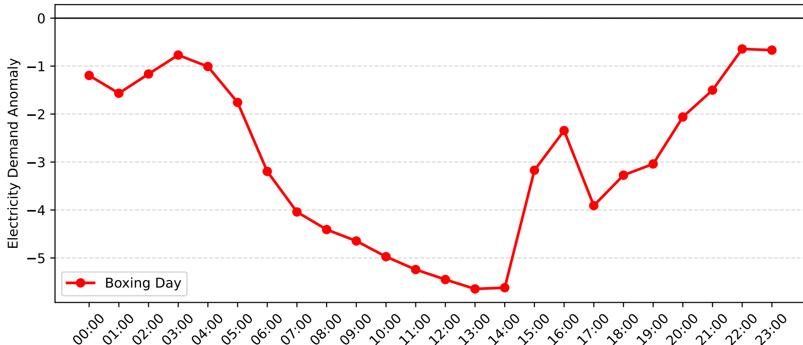
Wyong Demand Anomaly: Boxing Day (2005-2006)
