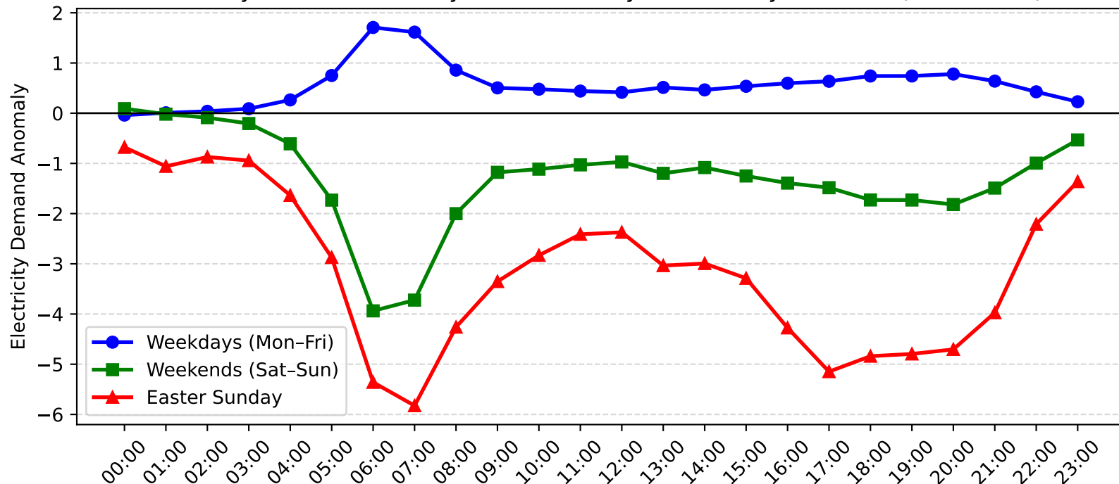
Revesby Demand Anomaly: Easter Sunday vs Weekday/Weekend (2011-2012)
