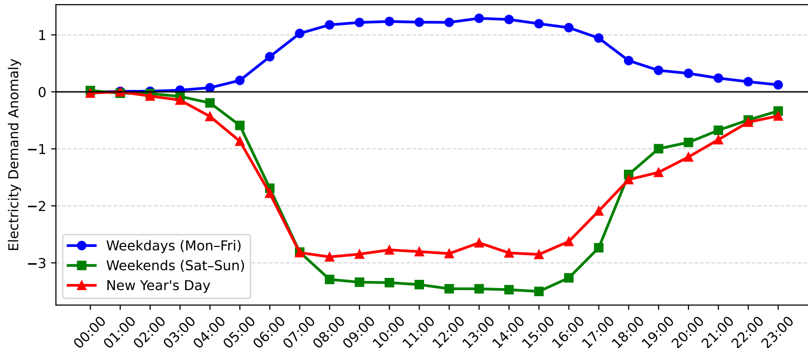
Beacon Hill Demand Anomaly: New Year's Day vs Weekday/Weekend (2013-2014)
