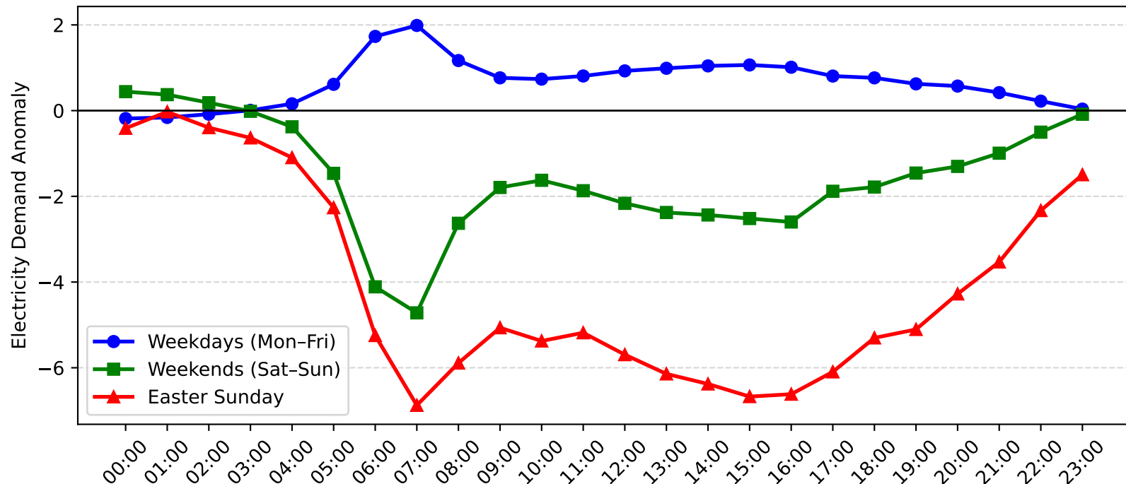
Dulwich Hill Demand Anomaly: Easter Sunday vs Weekday/Weekend (2006-2007)
