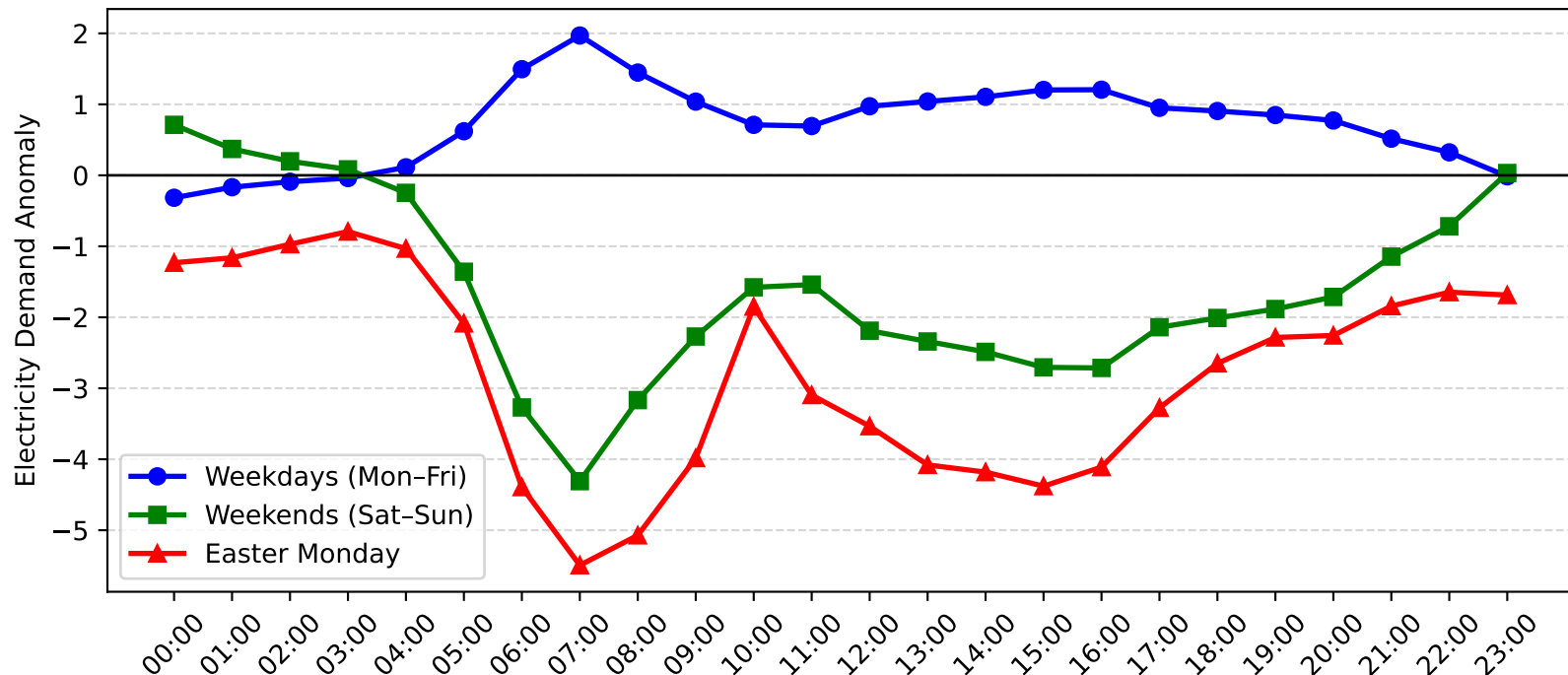
Kogarah Demand Anomaly: Easter Monday vs Weekday/Weekend (2016-2017)
