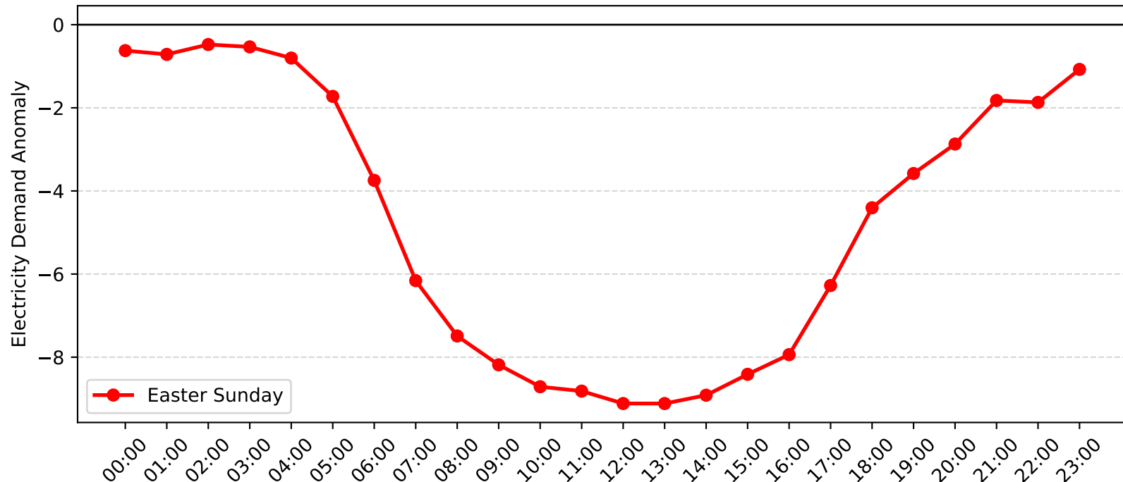
Newcastle Cbd Demand Anomaly: Easter Sunday (2016-2017)
