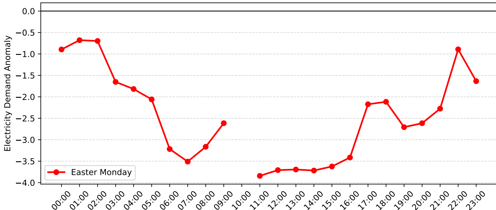
Bass Hill Demand Anomaly: Easter Monday (2005-2006)
