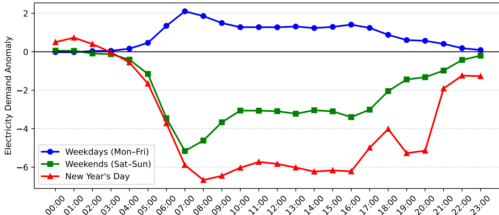
Chatswood Demand Anomaly: New Year's Day vs Weekday/Weekend (2007-2008)
