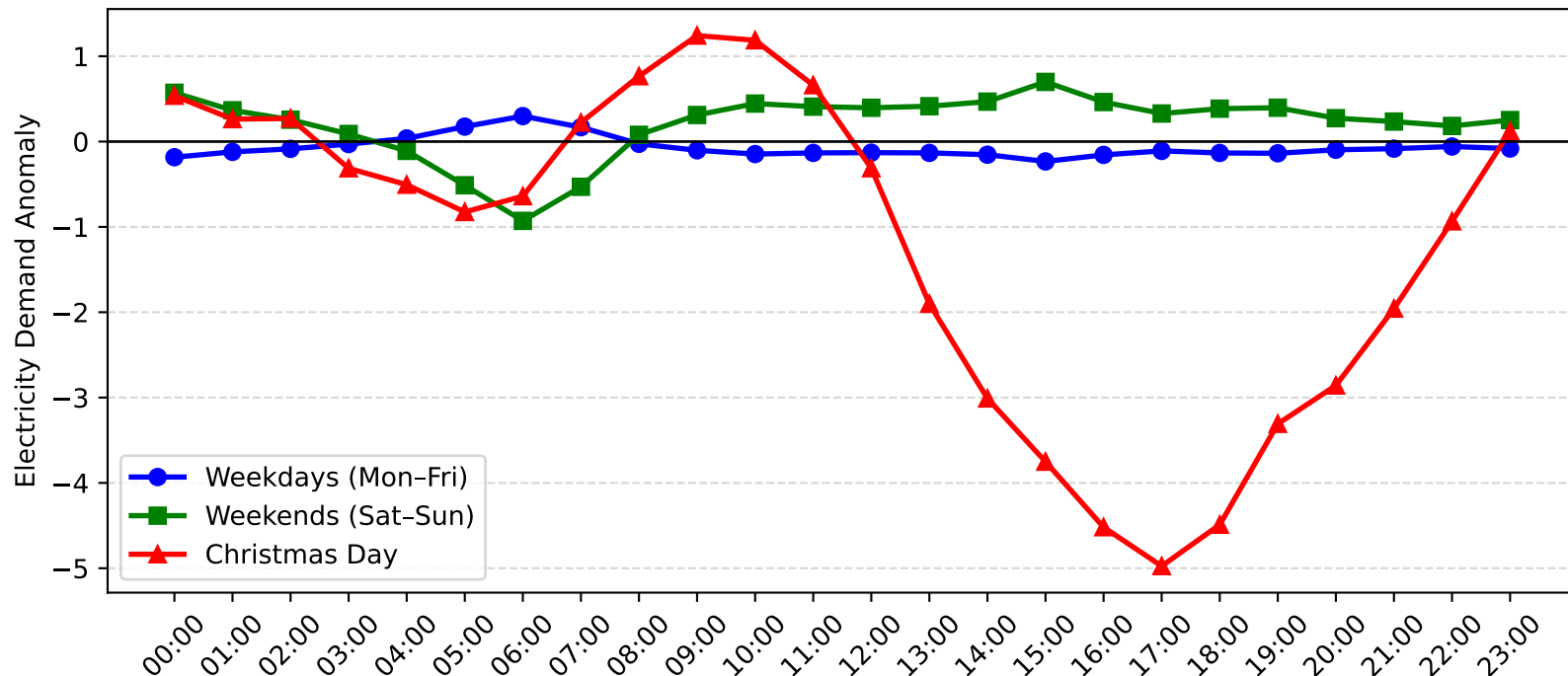
Umina Demand Anomaly: Christmas Day vs Weekday/Weekend (2013-2014)
