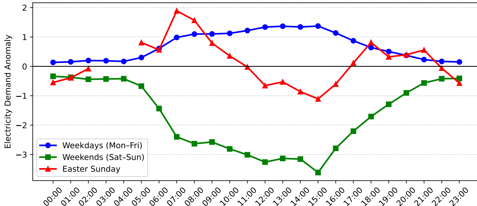
Mascot Demand Anomaly: Easter Sunday vs Weekday/Weekend (2004-2005)
