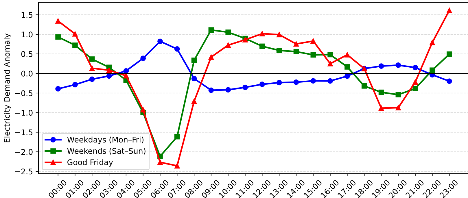
Avoca Demand Anomaly: Good Friday vs Weekday/Weekend (2011-2012)
