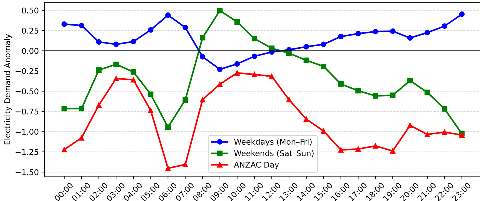
Morriset Demand Anomaly: ANZAC Day vs Weekday/Weekend (2009-2010)
