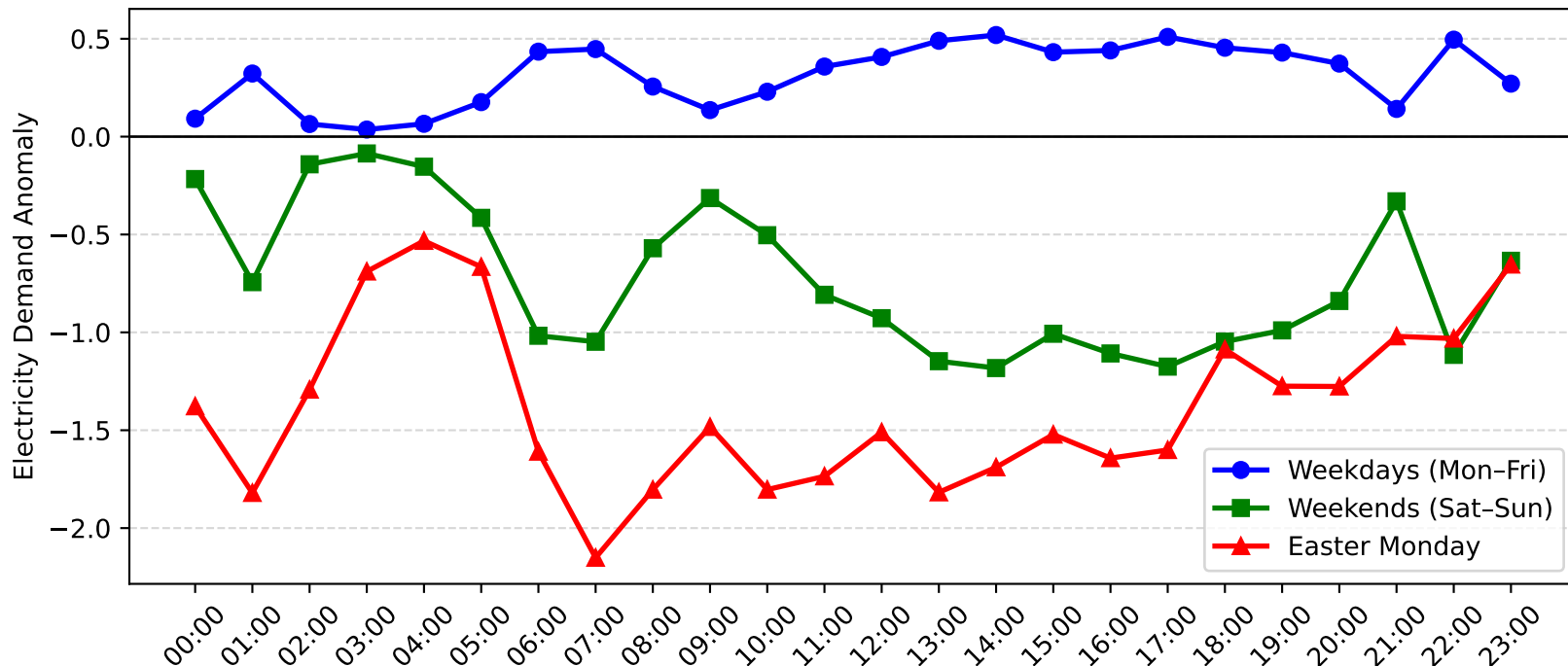
Gateshead Demand Anomaly: Easter Monday vs Weekday/Weekend (2006-2007)
