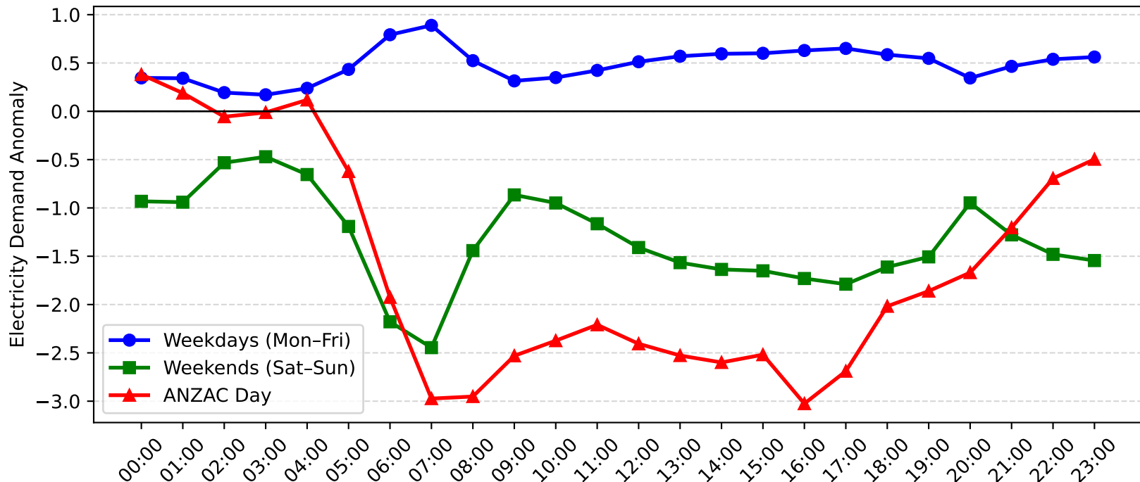
Jesmond Demand Anomaly: ANZAC Day vs Weekday/Weekend (2012-2013)
