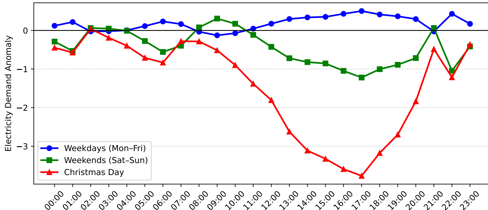
Nelson Bay Demand Anomaly: Christmas Day vs Weekday/Weekend (2015-2016)
