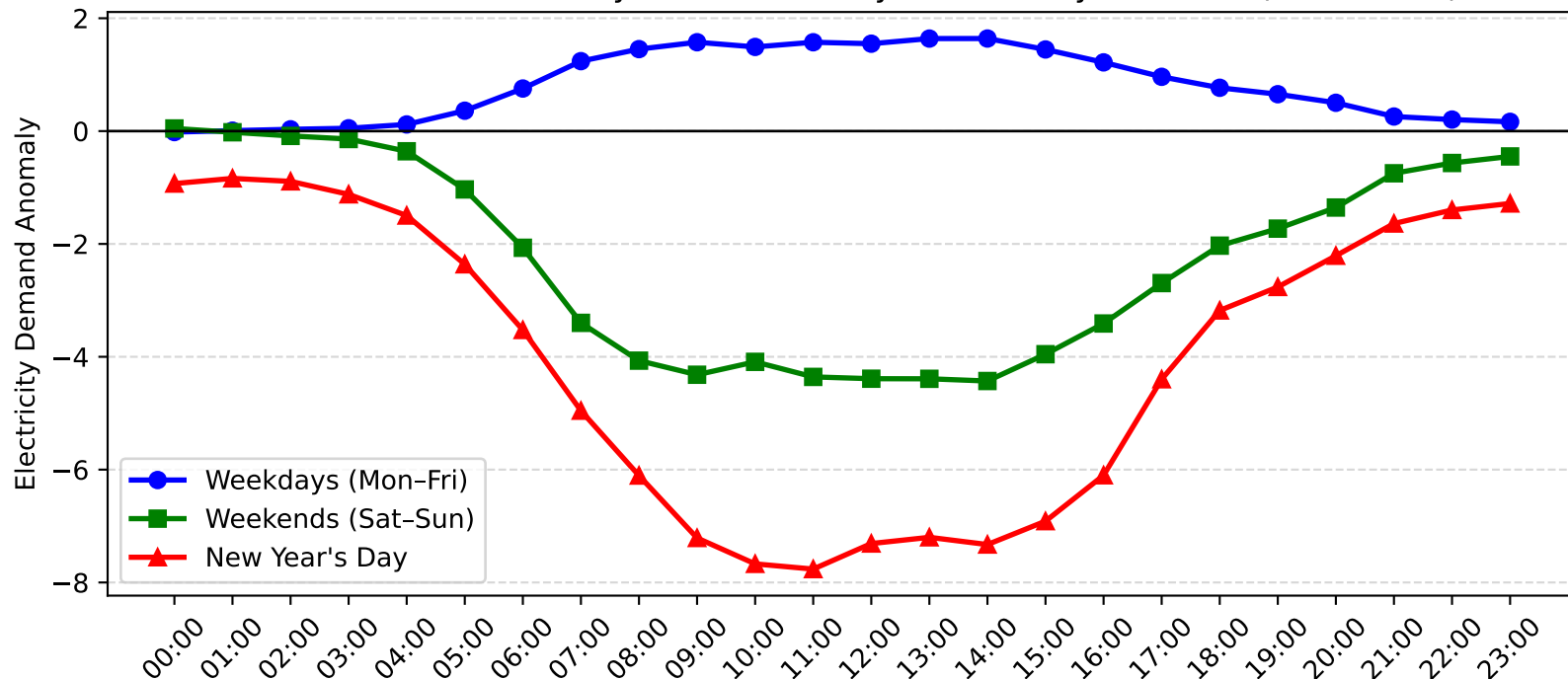
Auburn Demand Anomaly: New Year's Day vs Weekday/Weekend (2013-2014)
