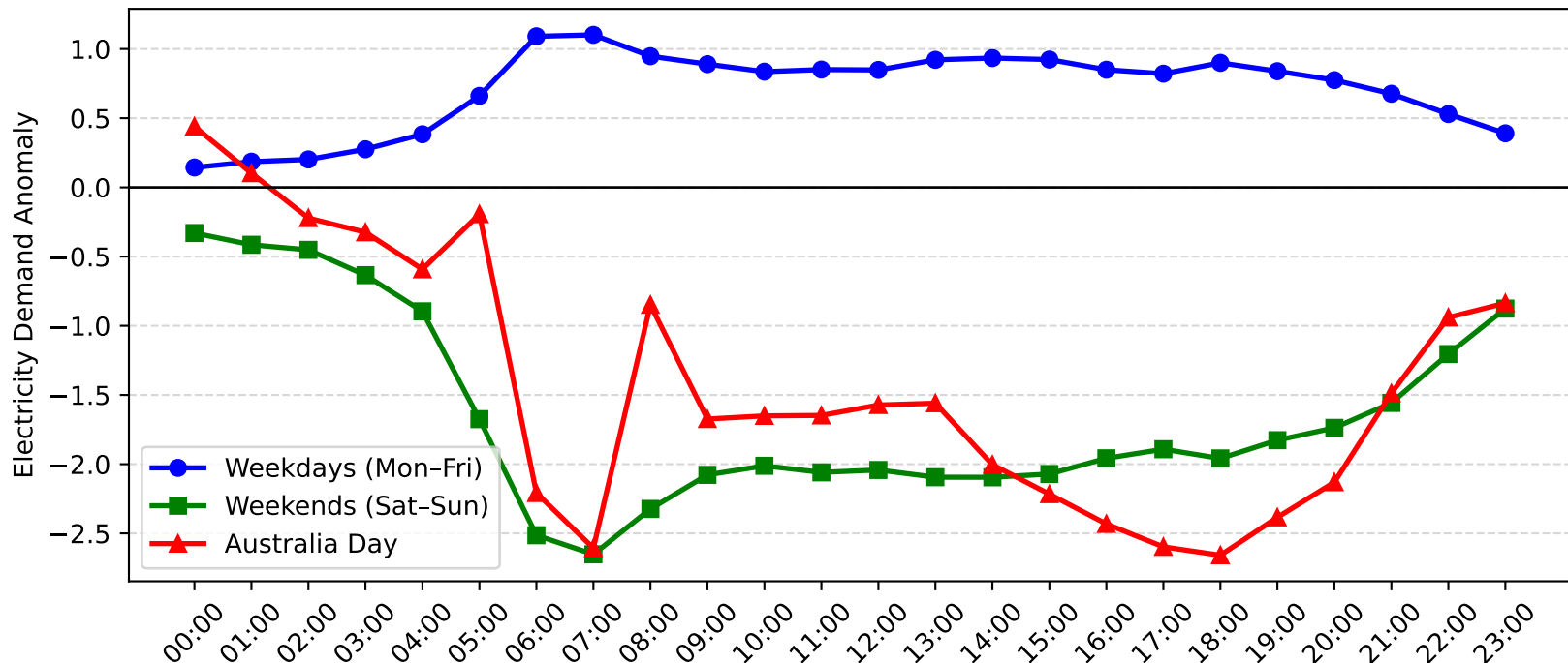
Lisarow Demand Anomaly: Australia Day vs Weekday/Weekend (2013-2014)
