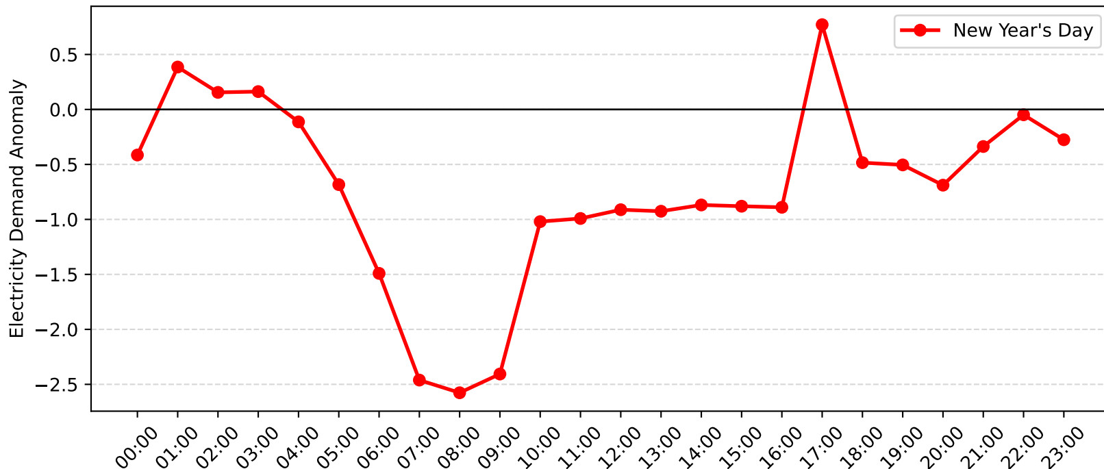
Narrabeen Demand Anomaly: New Year's Day (2009-2010)
