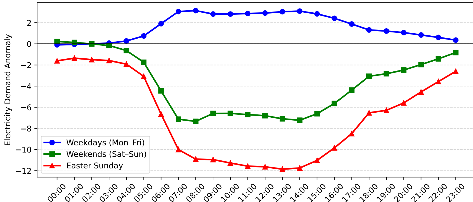
St. Peters Demand Anomaly: Easter Sunday vs Weekday/Weekend (2014-2015)
