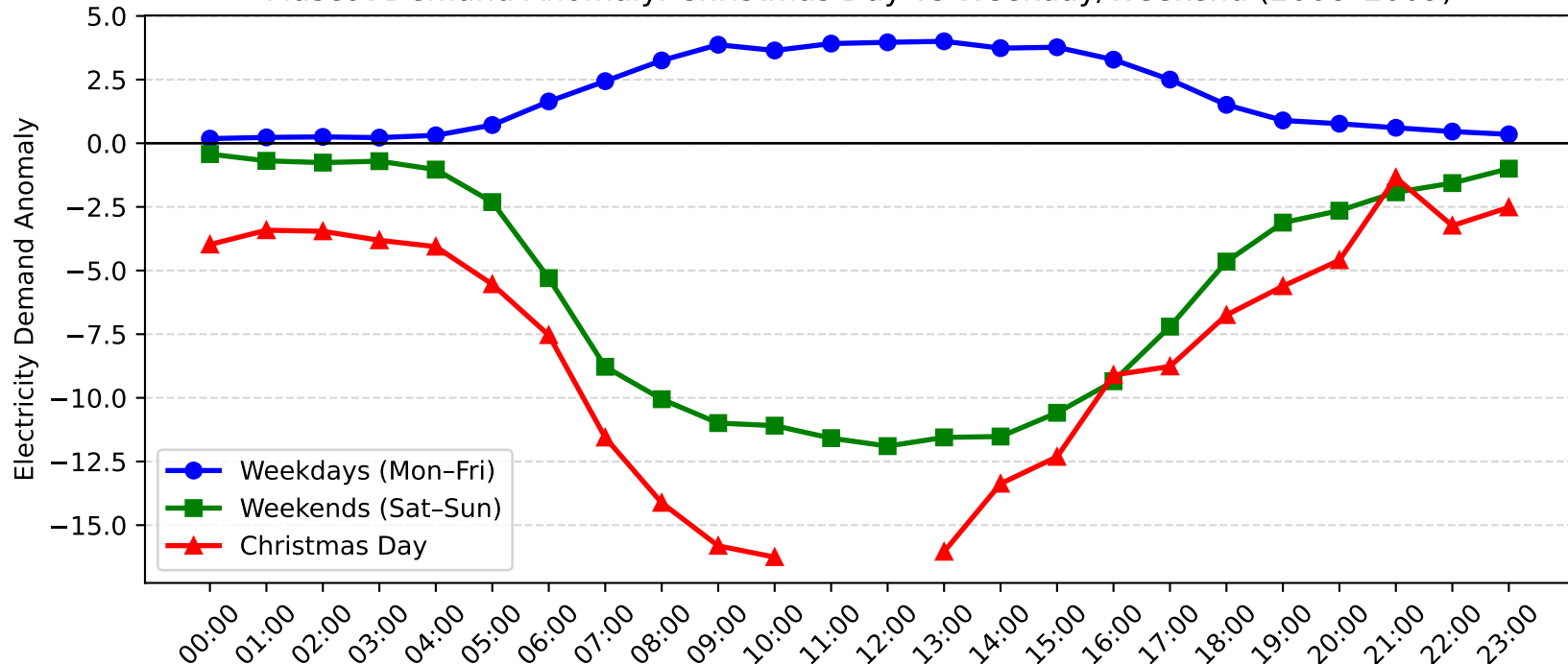
Mascot Demand Anomaly: Christmas Day vs Weekday/Weekend (2008-2009)
