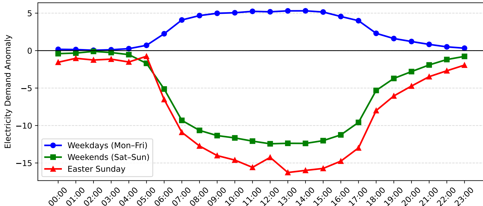
Macquarie Park Demand Anomaly: Easter Sunday vs Weekday/Weekend (2015-2016)
