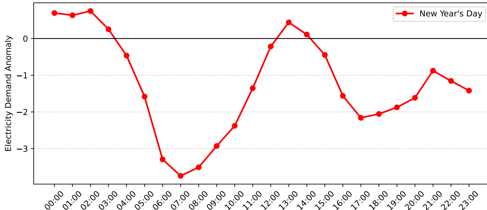
Revesby Demand Anomaly: New Year's Day (2013-2014)
