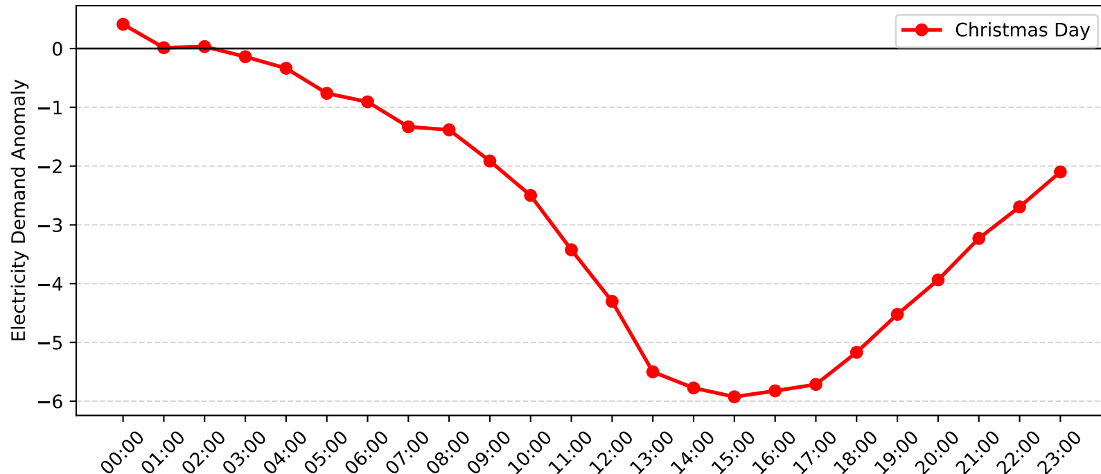
Jesmond Demand Anomaly: Christmas Day (2011-2012)
