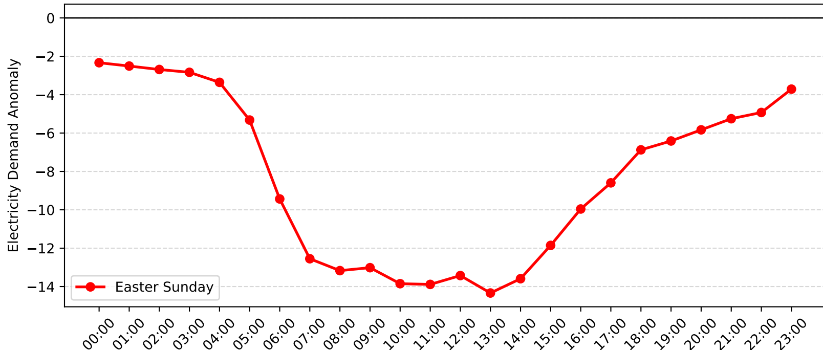
Milperra Demand Anomaly: Easter Sunday (2009-2010)
