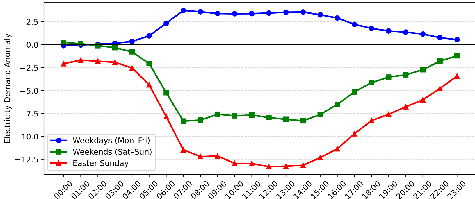
St. Peters Demand Anomaly: Easter Sunday vs Weekday/Weekend (2010-2011)
