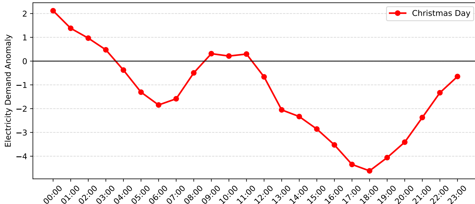
Revesby Demand Anomaly: Christmas Day (2011-2012)
