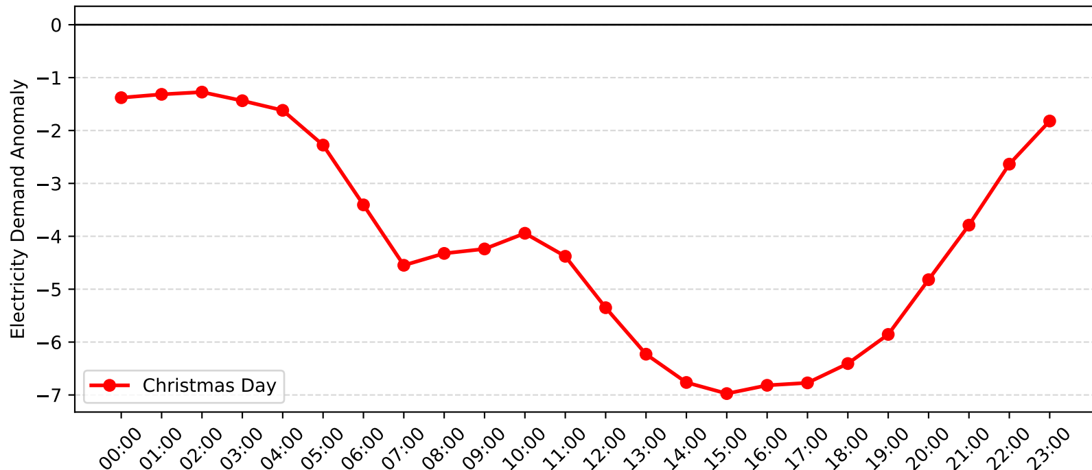
Hunters Hill Demand Anomaly: Christmas Day (2015-2016)
