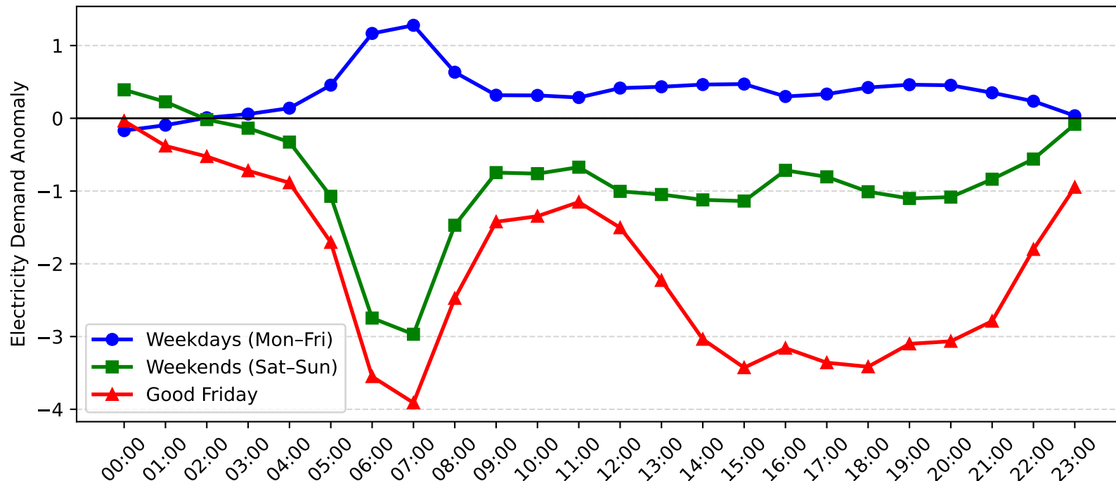
Mortdale Demand Anomaly: Good Friday vs Weekday/Weekend (2016-2017)
