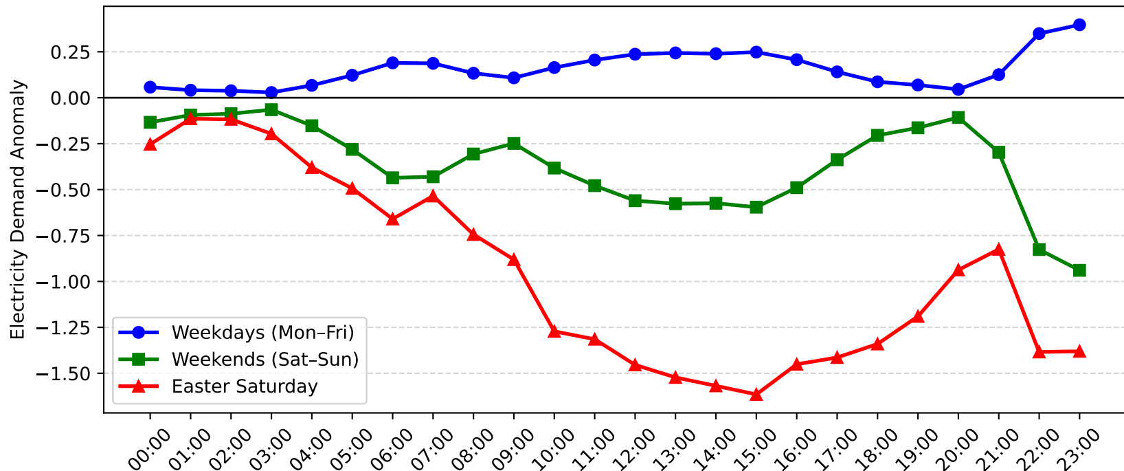
Muswellbrook Demand Anomaly: Easter Saturday vs Weekday/Weekend (2016-2017)
