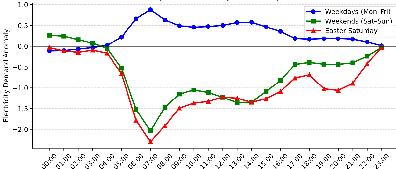
Arncliffe Demand Anomaly: Easter Saturday vs Weekday/Weekend (2011-2012)
