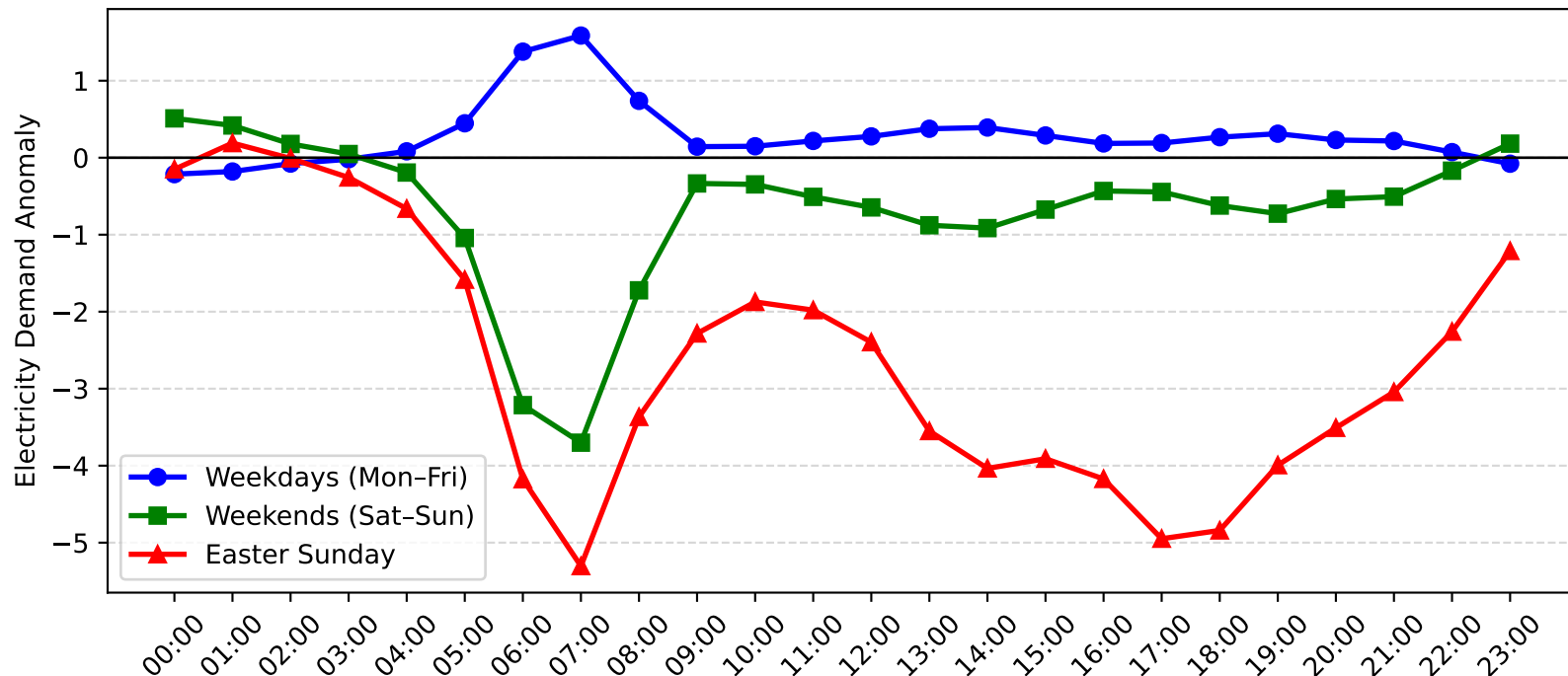
Mortdale Demand Anomaly: Easter Sunday vs Weekday/Weekend (2013-2014)
