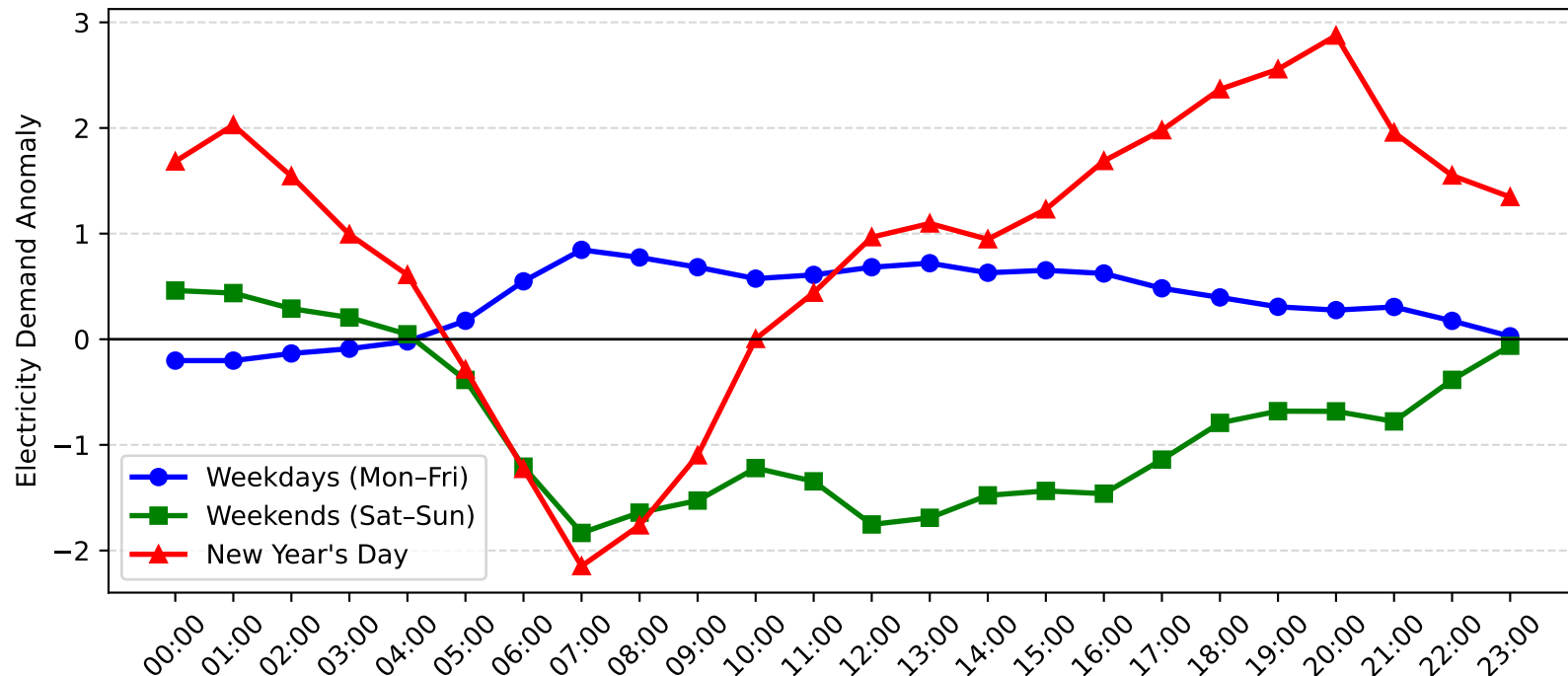
Arnccliffe Demand Anomaly: New Year's Day vs Weekday/Weekend (2005-2006)
