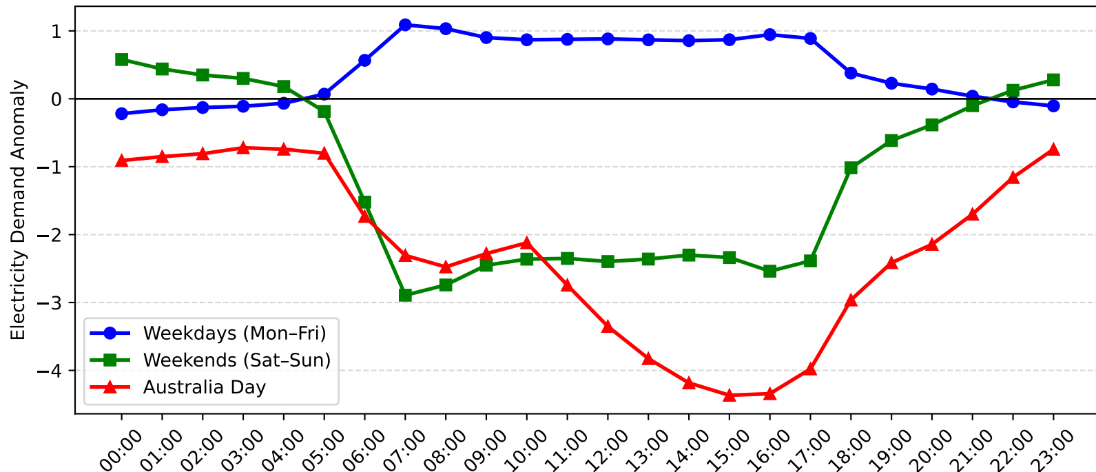
Pymble Demand Anomaly: Australia Day vs Weekday/Weekend (2016-2017)
