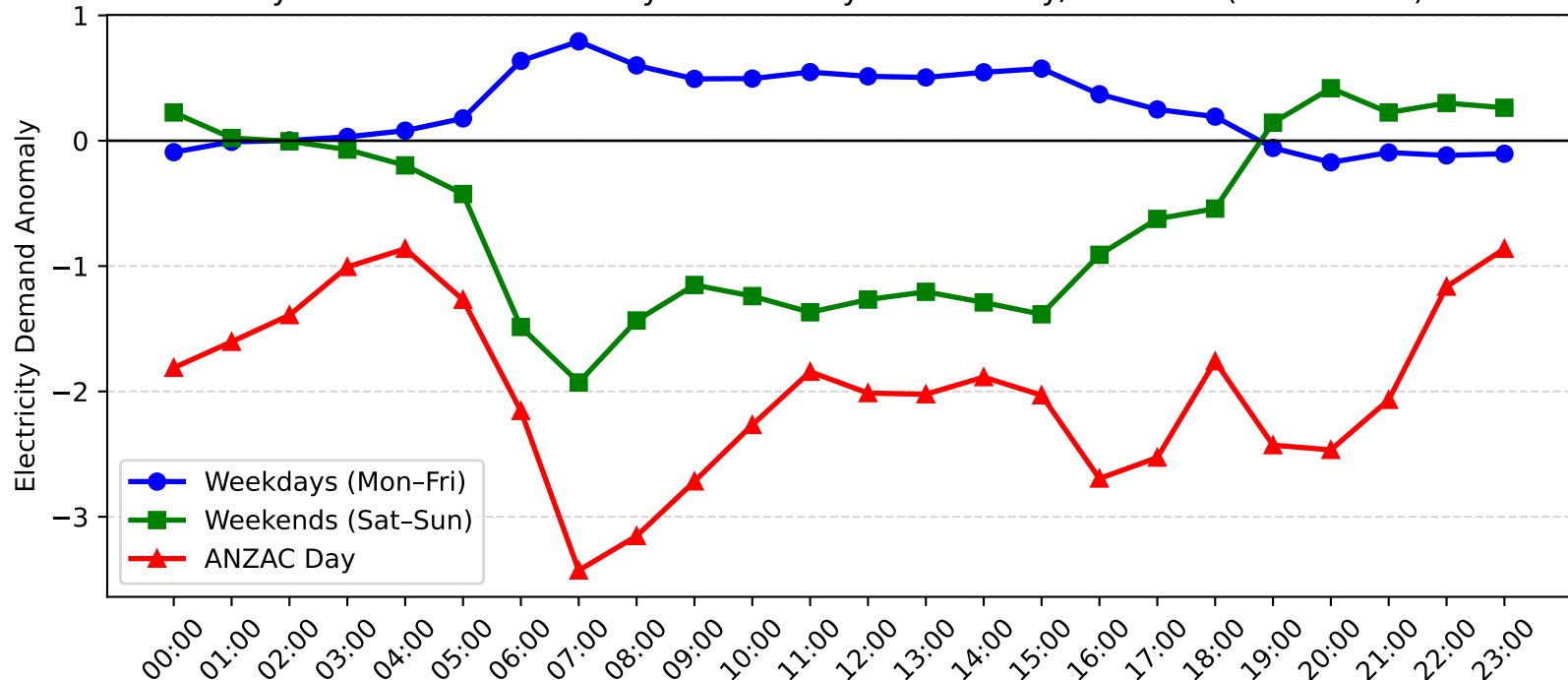
Pymble Demand Anomaly: ANZAC Day vs Weekday/Weekend (2004-2005)
