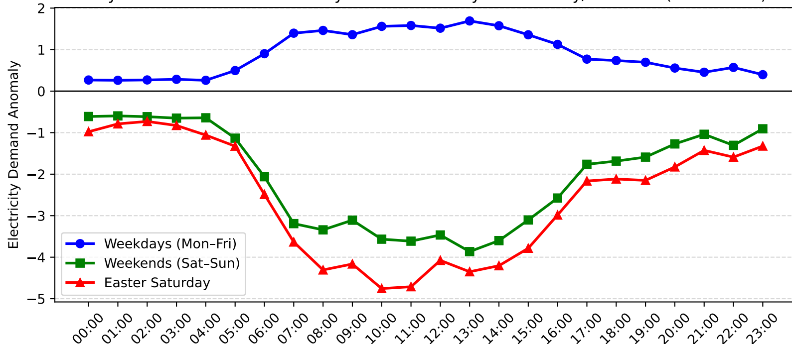
Mayfield West Demand Anomaly: Easter Saturday vs Weekday/Weekend (2017-2018)
