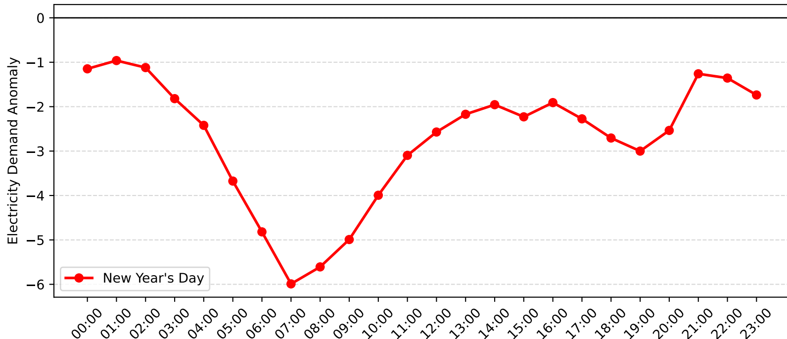
Enfield Demand Anomaly: New Year's Day (2010-2011)
