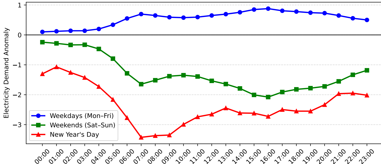
Enfield Demand Anomaly: New Year's Day vs Weekday/Weekend (2012-2013)
