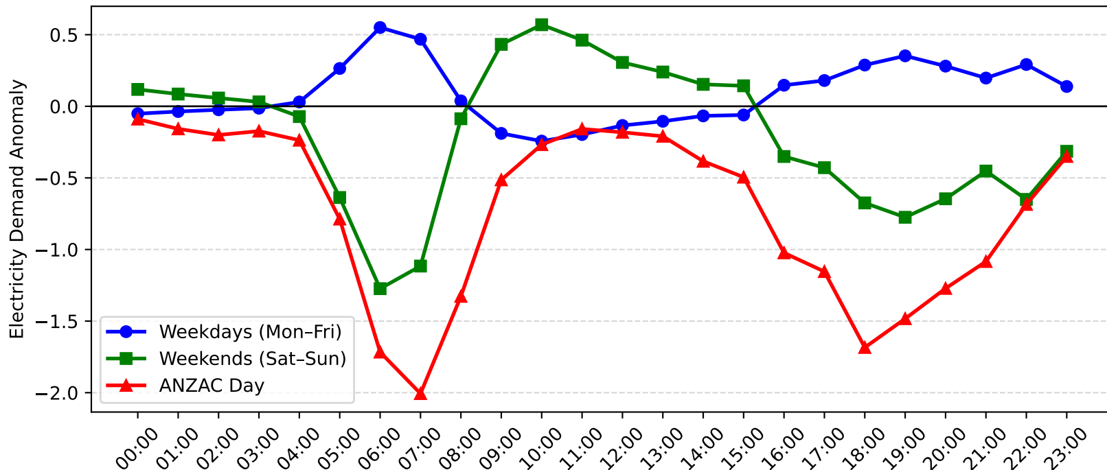
Narrabeen Demand Anomaly: ANZAC Day vs Weekday/Weekend (2008-2009)
