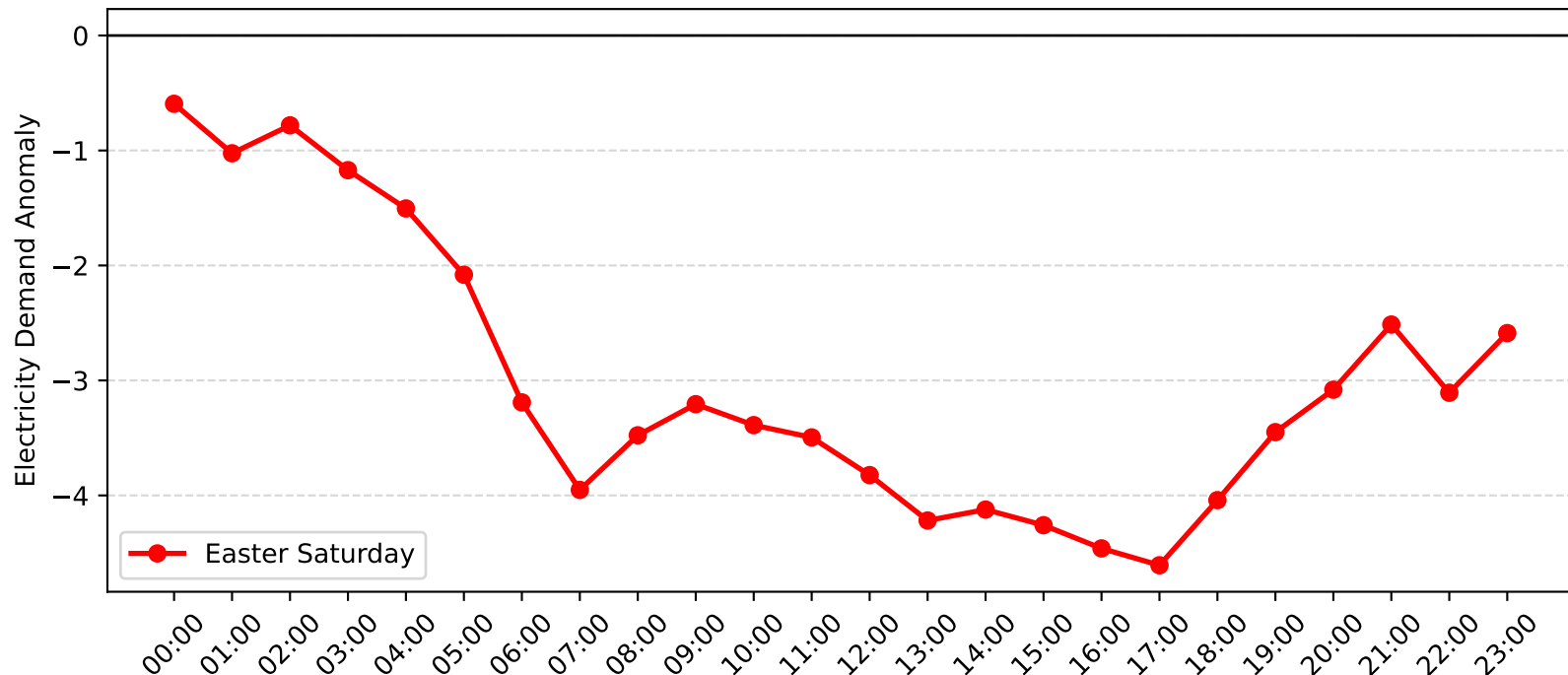
Jesmond Demand Anomaly: Easter Saturday (2013-2014)
