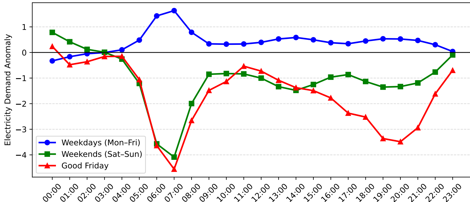
Mortdale Demand Anomaly: Good Friday vs Weekday/Weekend (2011-2012)
