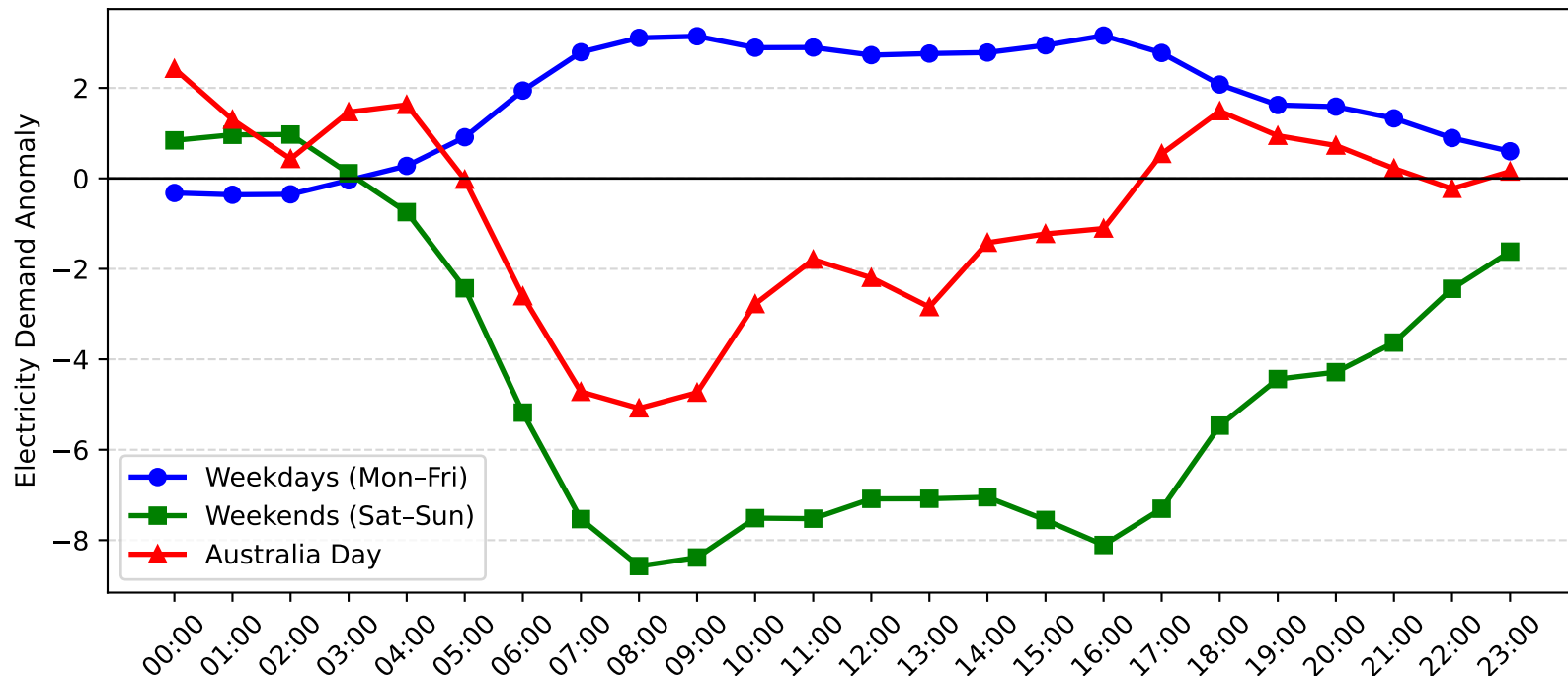
Greenacre Park Demand Anomaly: Australia Day vs Weekday/Weekend (2011-2012)
