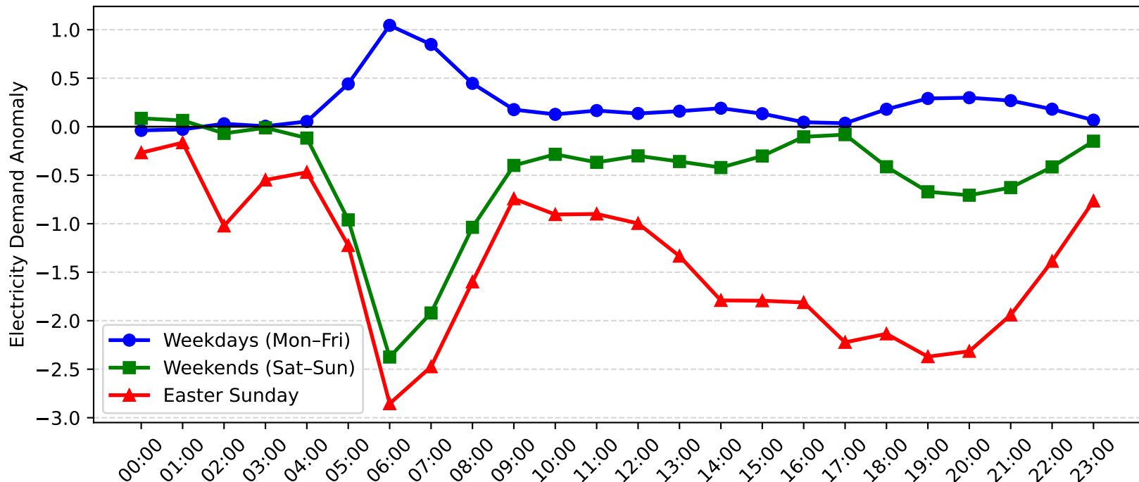
Berowra Demand Anomaly: Easter Sunday vs Weekday/Weekend (2010-2011)
