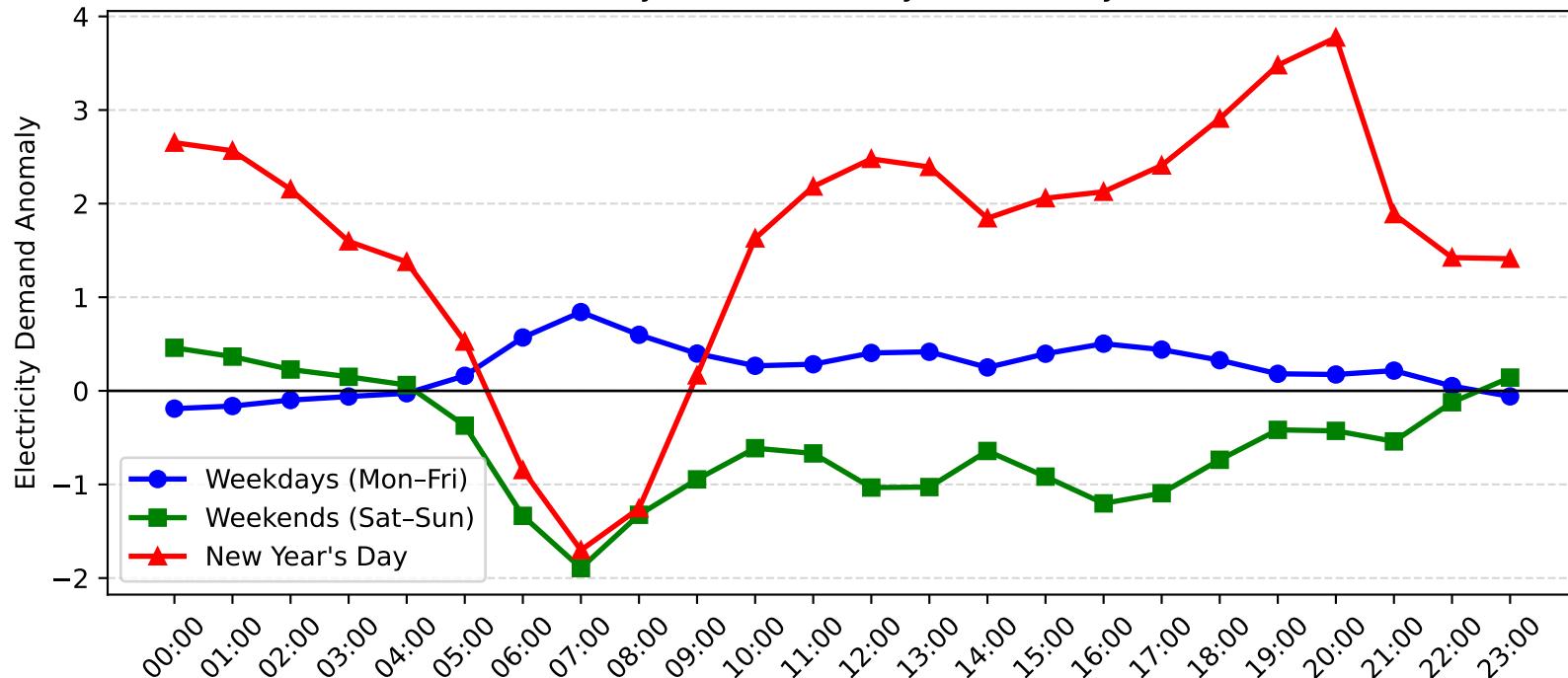
Blakehurst Demand Anomaly: New Year's Day vs Weekday/Weekend (2006-2007)
