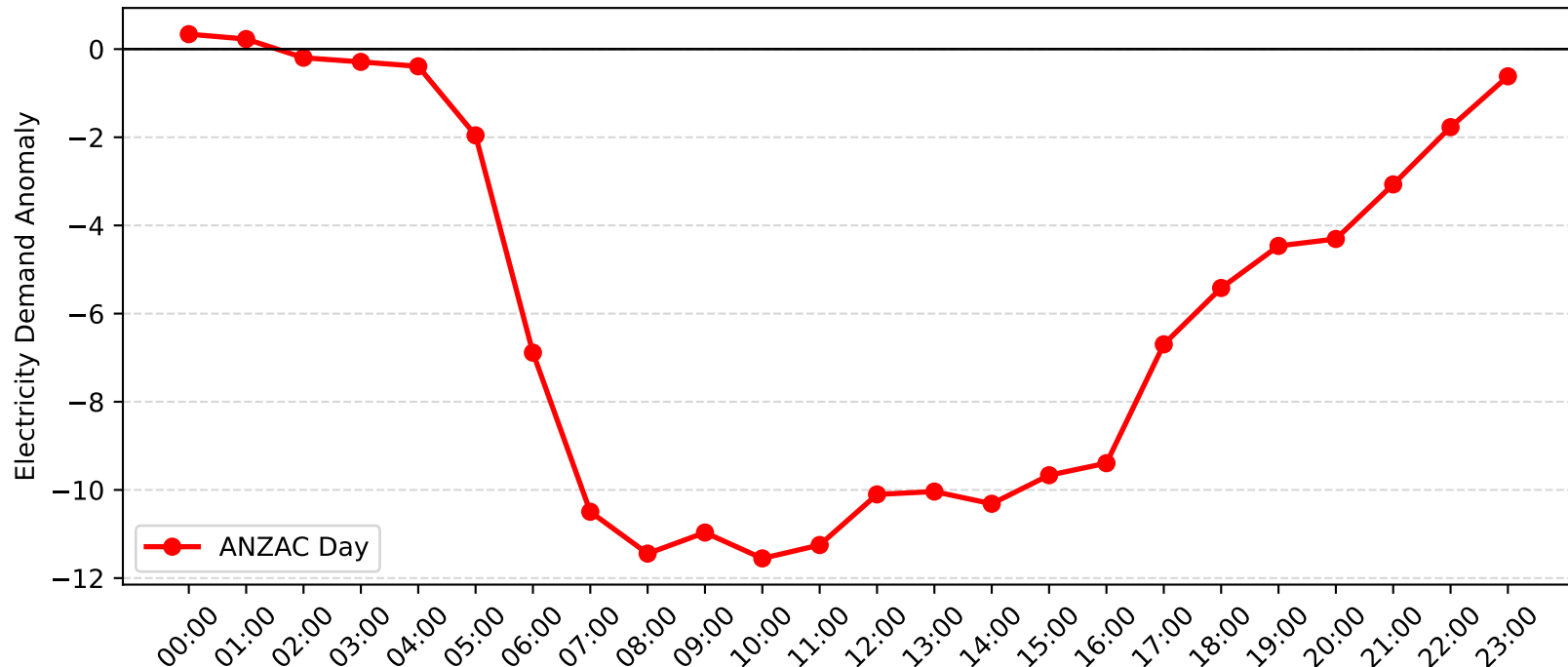
Zetland Demand Anomaly: ANZAC Day (2008-2009)
