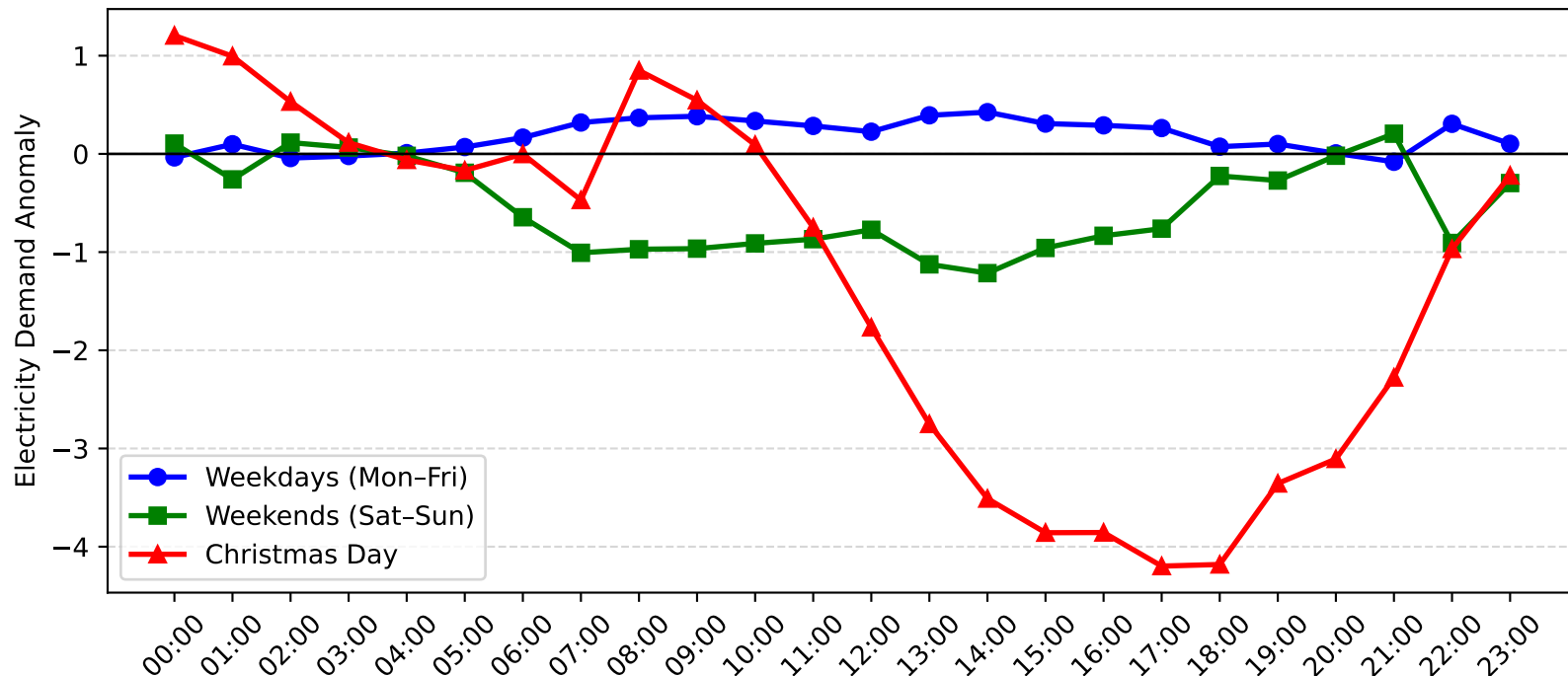
Adamstown Demand Anomaly: Christmas Day vs Weekday/Weekend (2013-2014)
