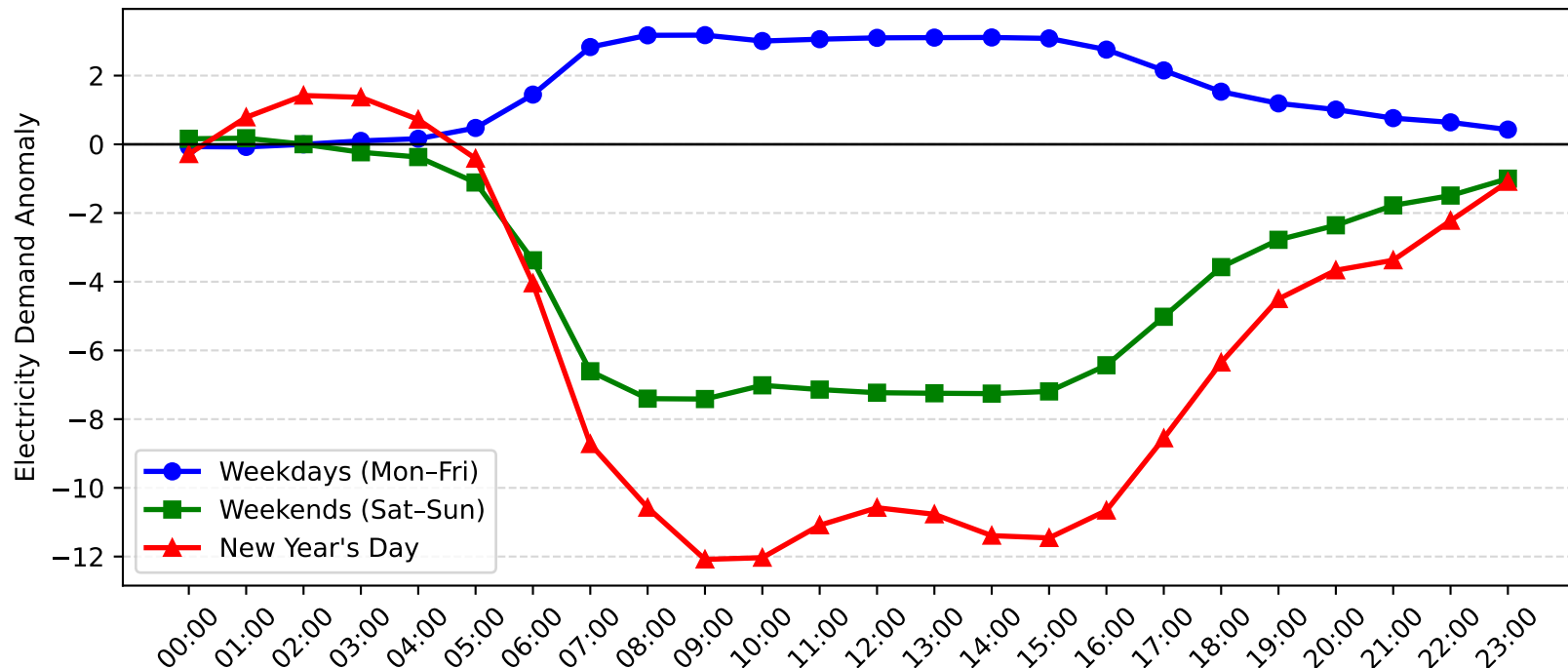
Zetland Demand Anomaly: New Year's Day vs Weekday/Weekend (2017-2018)
