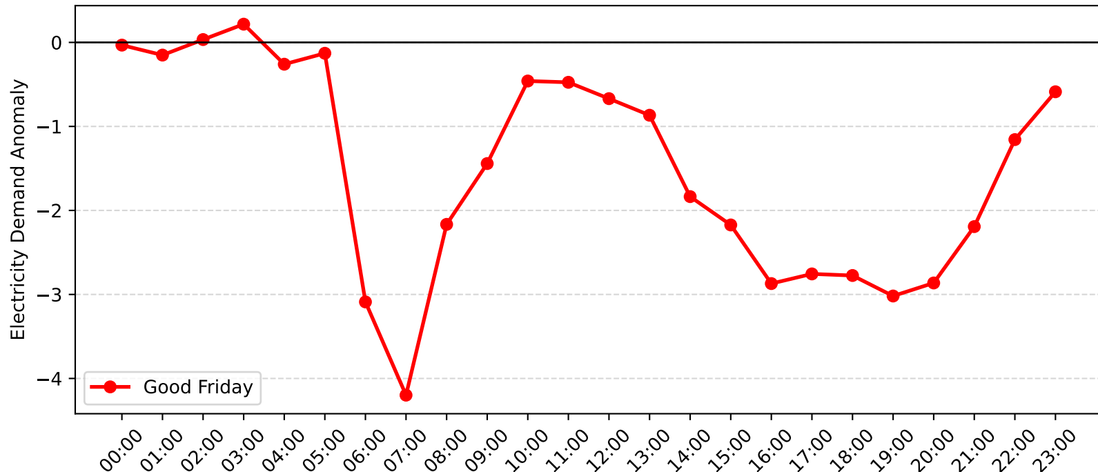
Balgowlah North Demand Anomaly: Good Friday (2014-2015)
