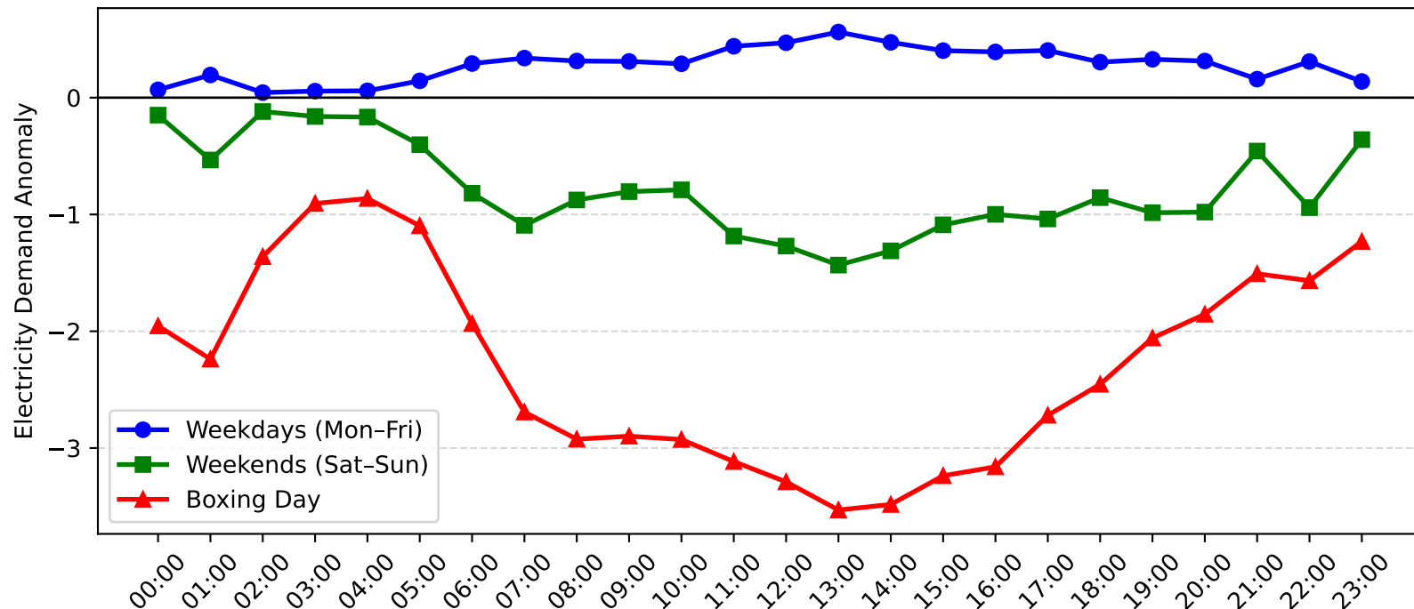
Gateshead Demand Anomaly: Boxing Day vs Weekday/Weekend (2008-2009)
