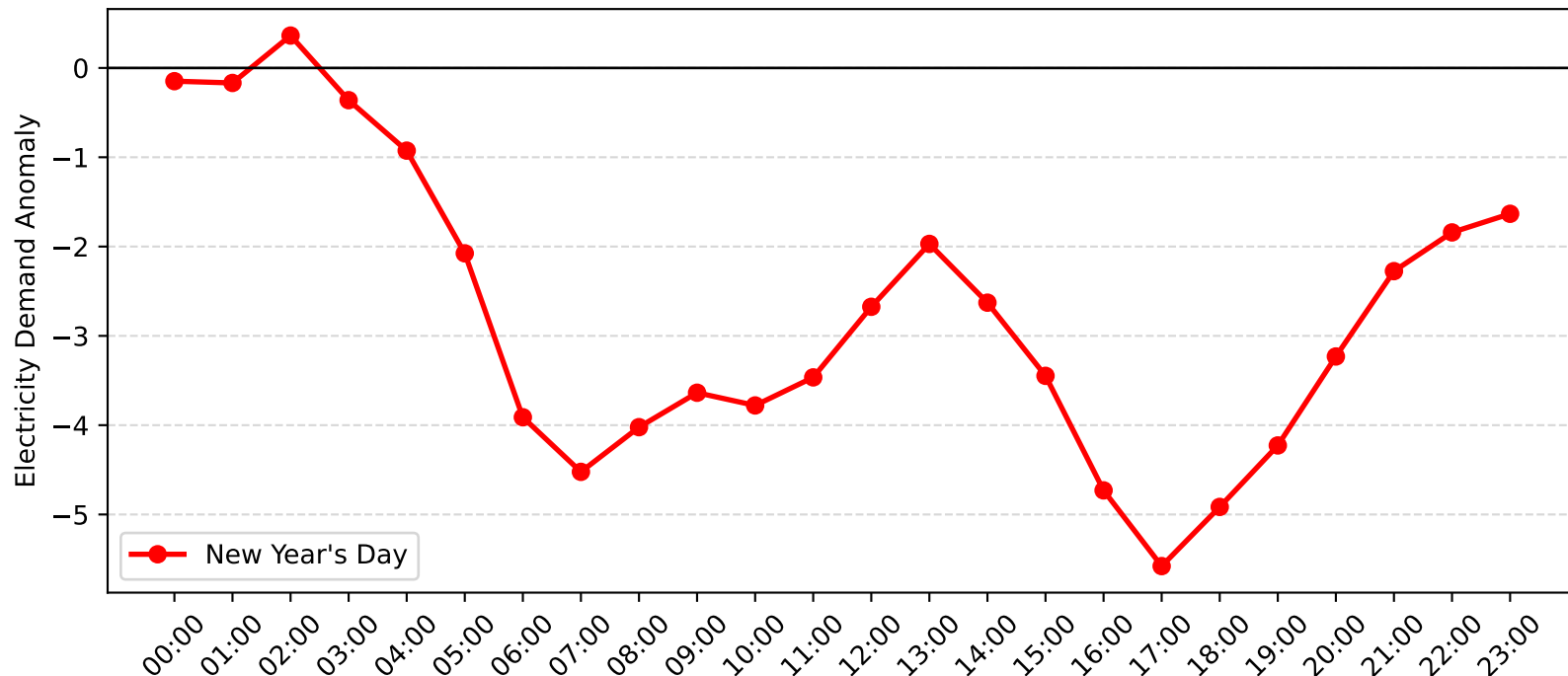
Revesby Demand Anomaly: New Year's Day (2014-2015)
