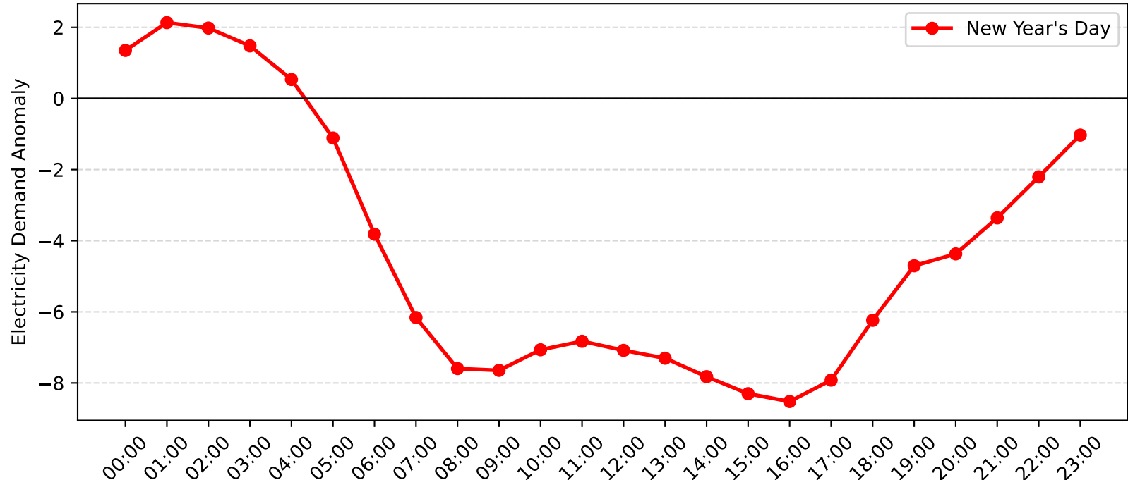
Kogarah Demand Anomaly: New Year's Day (2016-2017)
