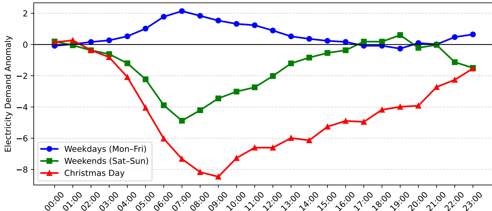
Meadowbank Demand Anomaly: Christmas Day vs Weekday/Weekend (2010-2011)
