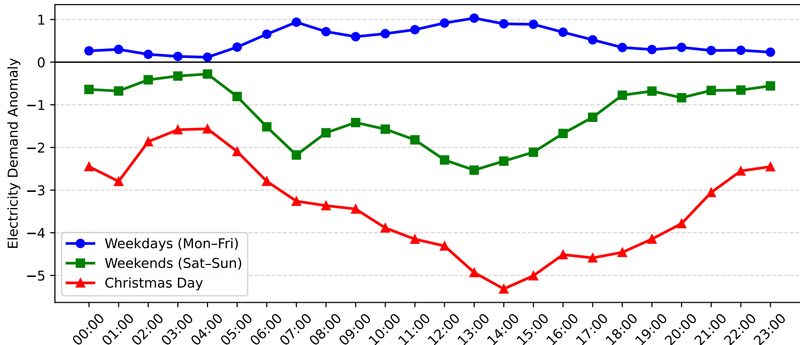
Rutherford Demand Anomaly: Christmas Day vs Weekday/Weekend (2005-2006)
