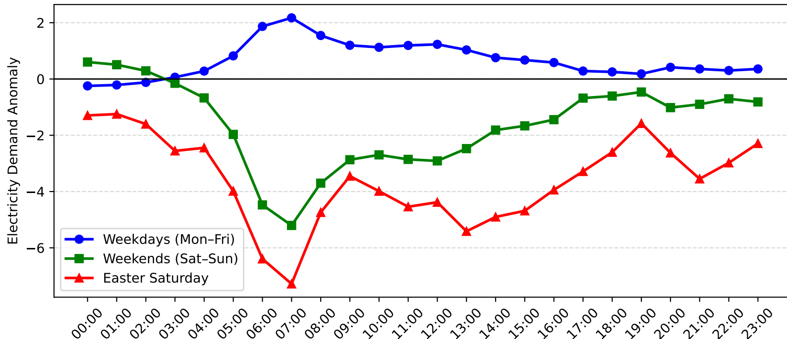
Meadowbank Demand Anomaly: Easter Saturday vs Weekday/Weekend (2007-2008)
