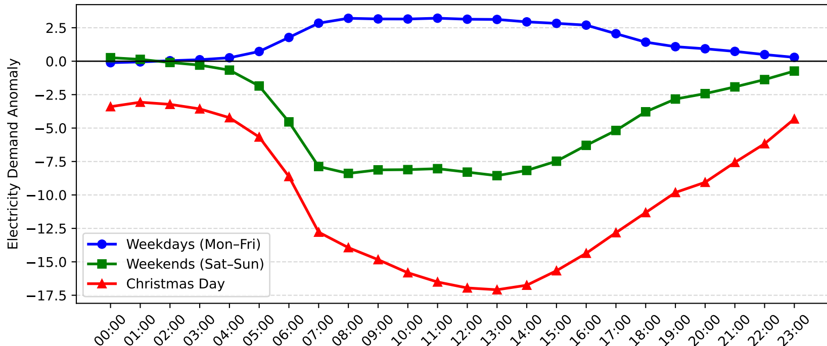
St. Peters Demand Anomaly: Christmas Day vs Weekday/Weekend (2009-2010)
