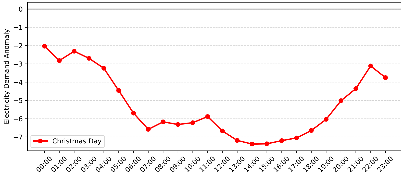
Matraverse Demand Anomaly: Christmas Day (2004-2005)
