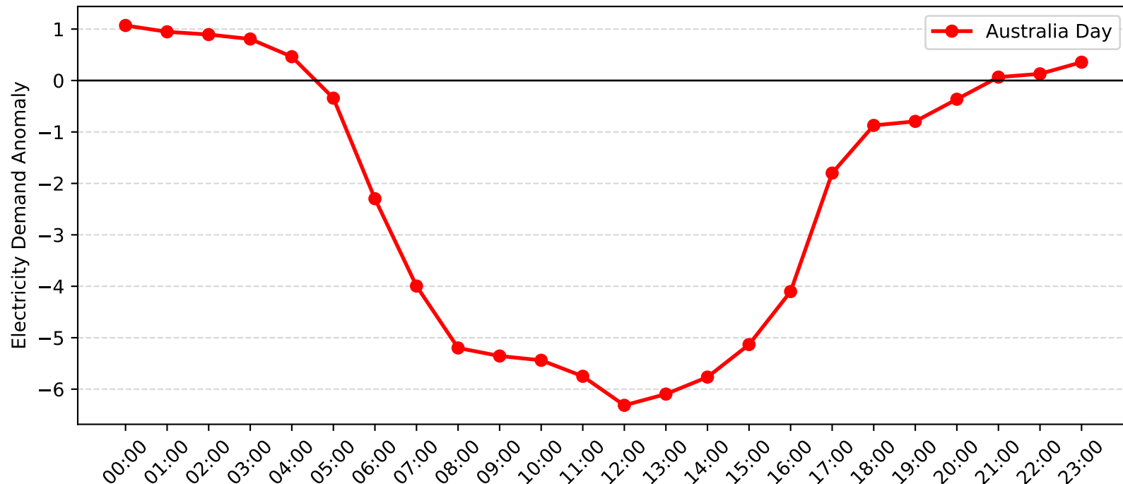
Mascot Demand Anomaly: Australia Day (2011-2012)
