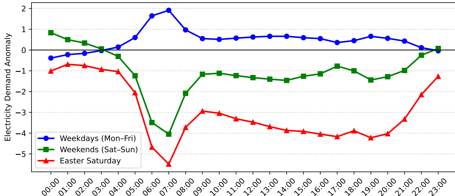
Mortdale Demand Anomaly: Easter Saturday vs Weekday/Weekend (2009-2010)
