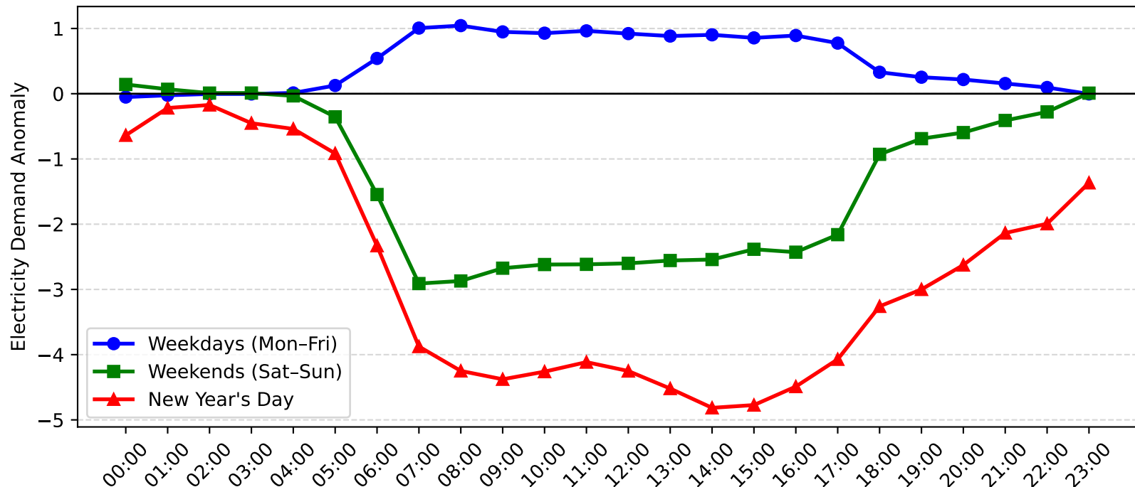
Pymble Demand Anomaly: New Year's Day vs Weekday/Weekend (2015-2016)
