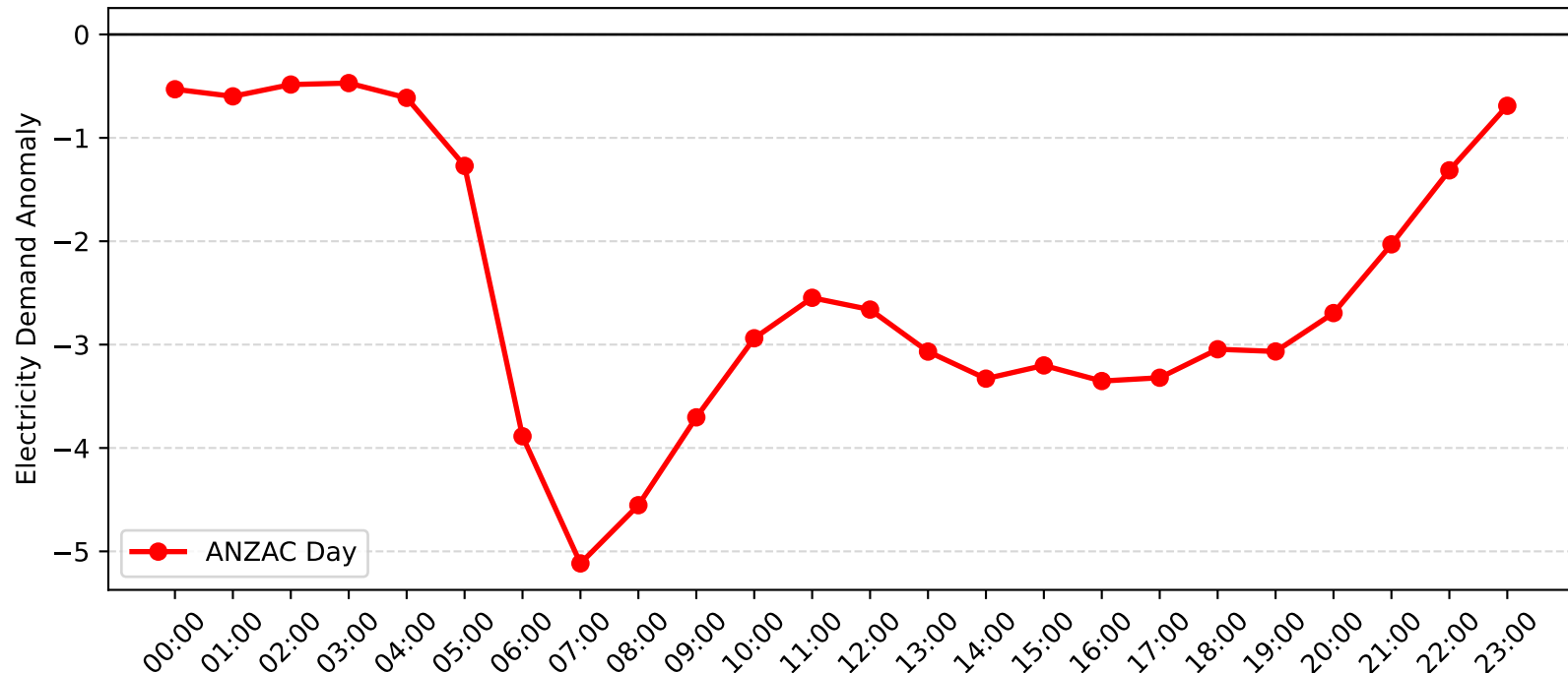
Pymble Demand Anomaly: ANZAC Day (2010-2011)
