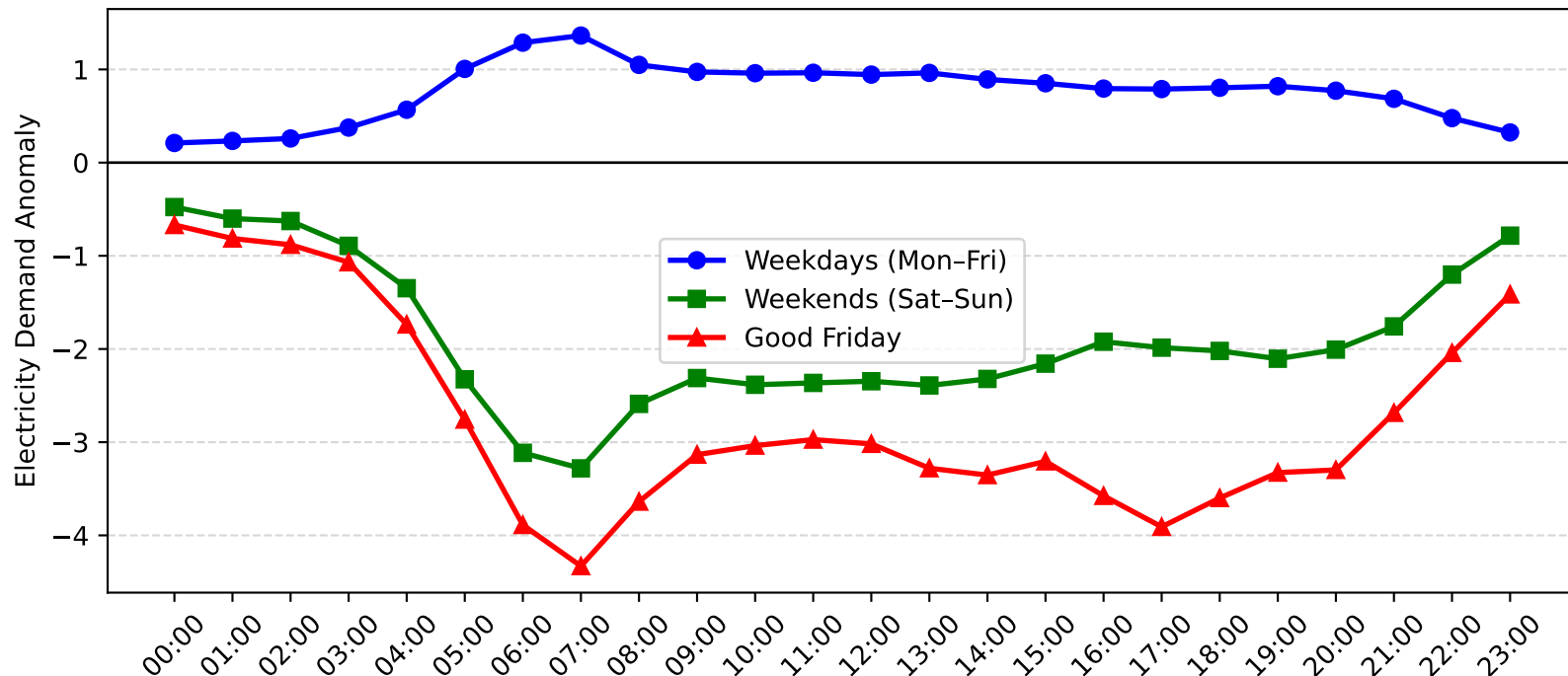
Lisarow Demand Anomaly: Good Friday vs Weekday/Weekend (2010-2011)
