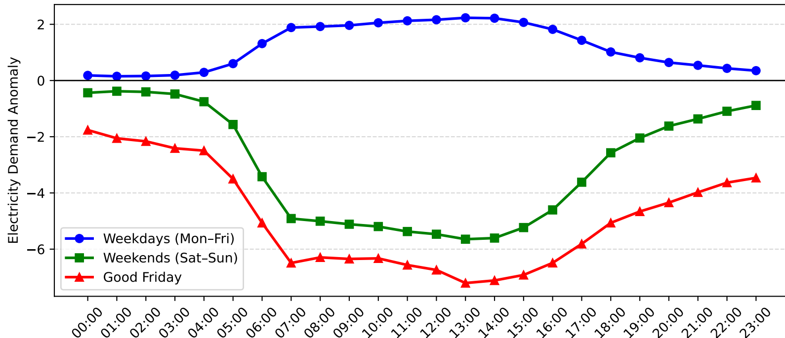
Botany Demand Anomaly: Good Friday vs Weekday/Weekend (2012-2013)
