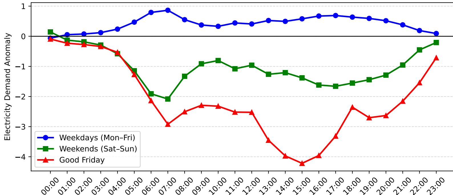
Charmhaven Demand Anomaly: Good Friday vs Weekday/Weekend (2008-2009)
