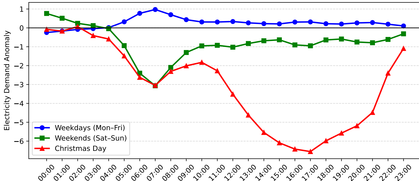
Dulwich Hill Demand Anomaly: Christmas Day vs Weekday/Weekend (2013-2014)
