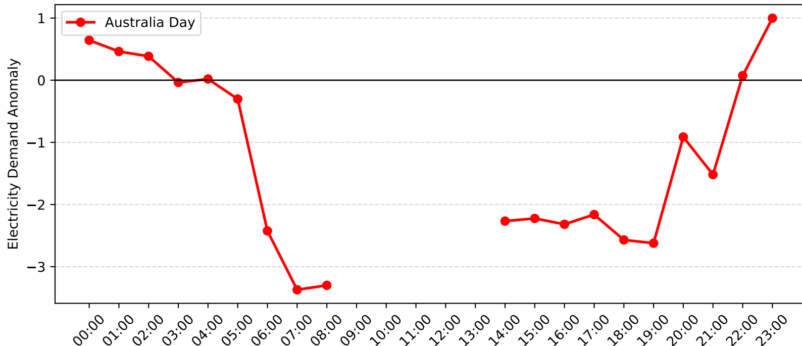
Dee Why West Demand Anomaly: Australia Day (2006-2007)
