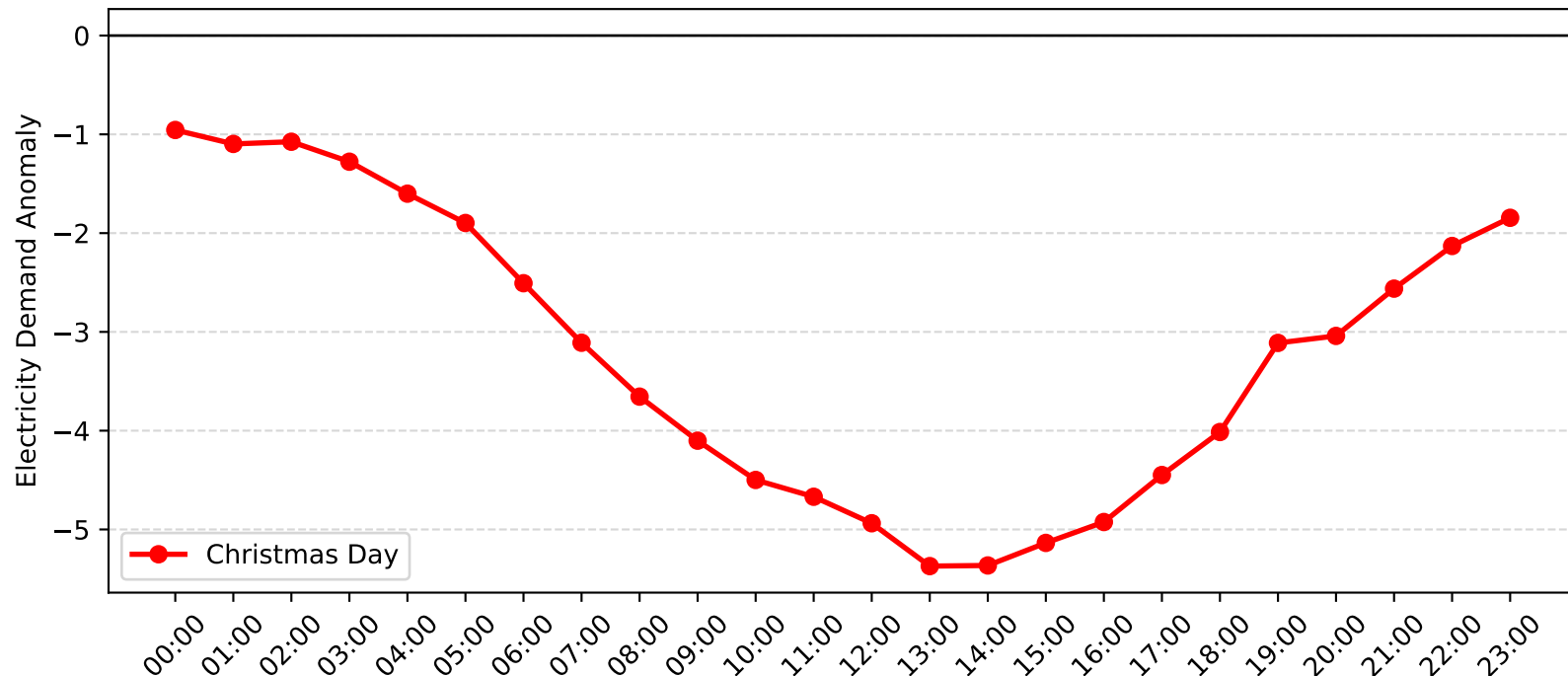
Caringbah Demand Anomaly: Christmas Day (2011-2012)
