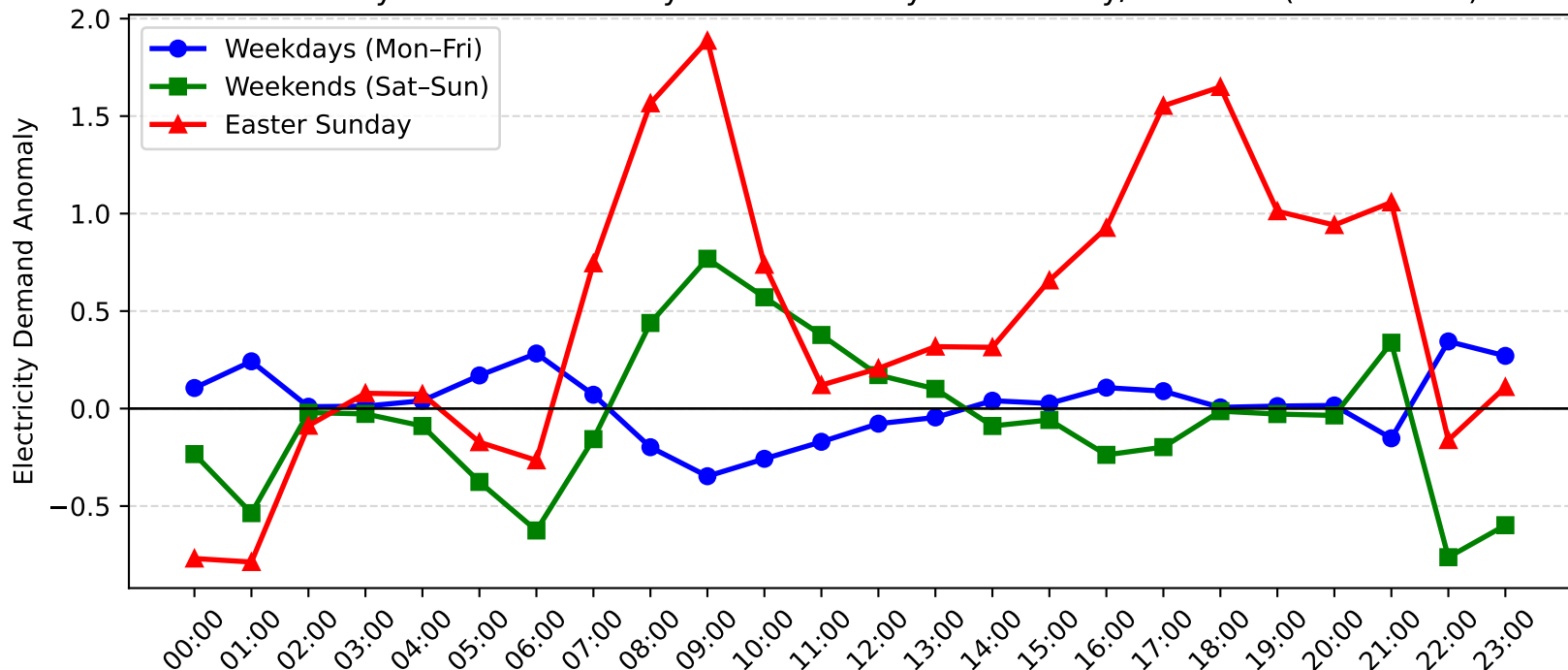
Nelson Bay Demand Anomaly: Easter Sunday vs Weekday/Weekend (2017-2018)
