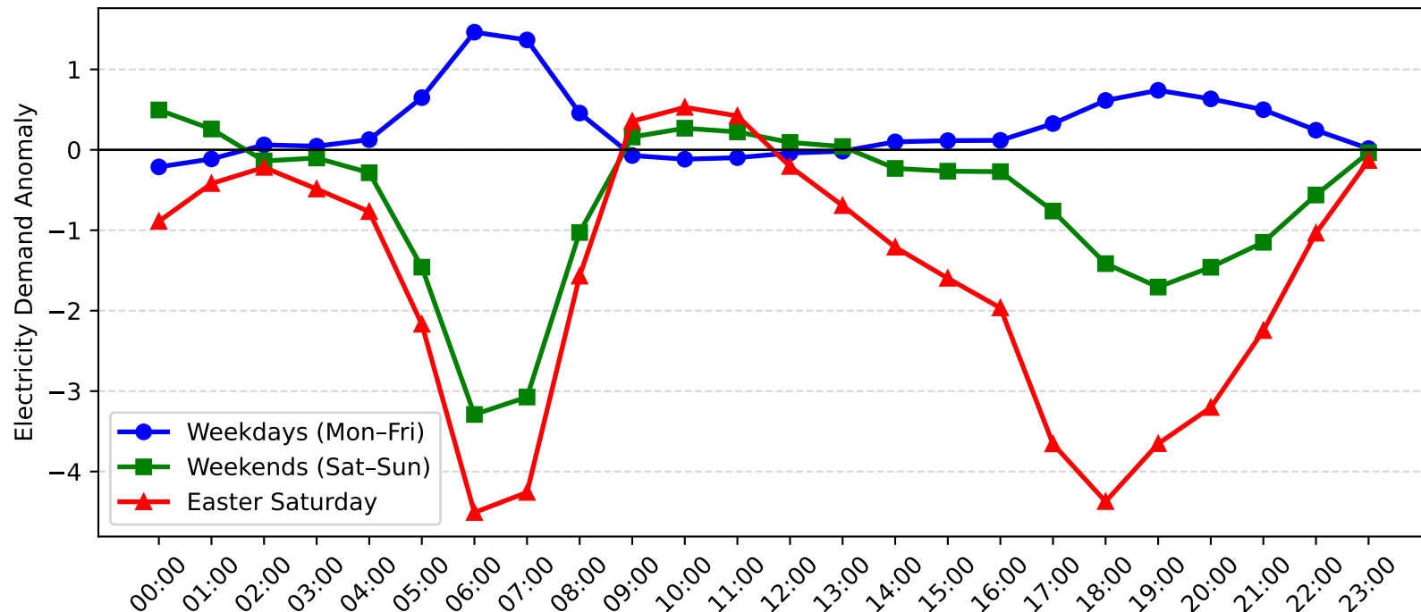
Cronulla Demand Anomaly: Easter Saturday vs Weekday/Weekend (2015-2016)
