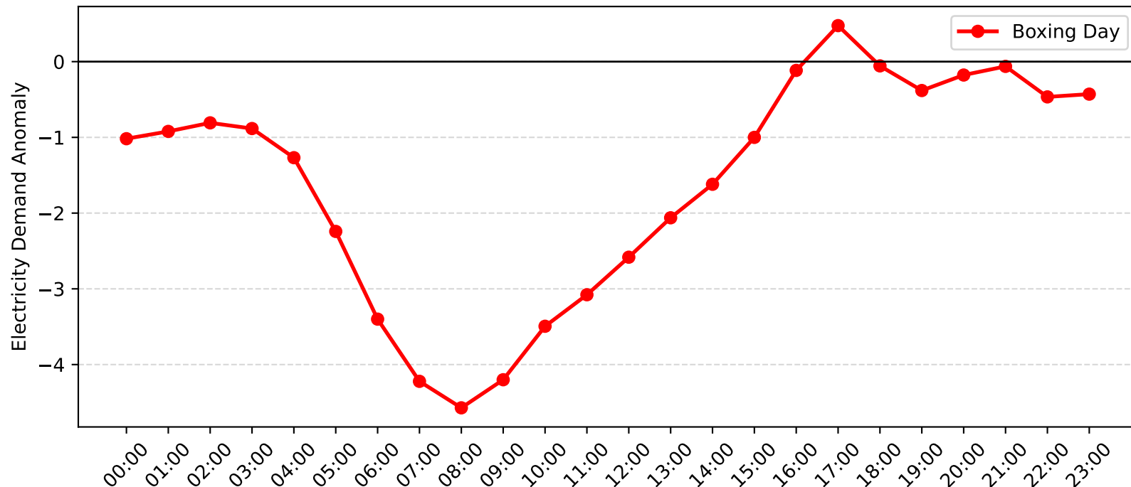
Wyong Demand Anomaly: Boxing Day (2016-2017)
