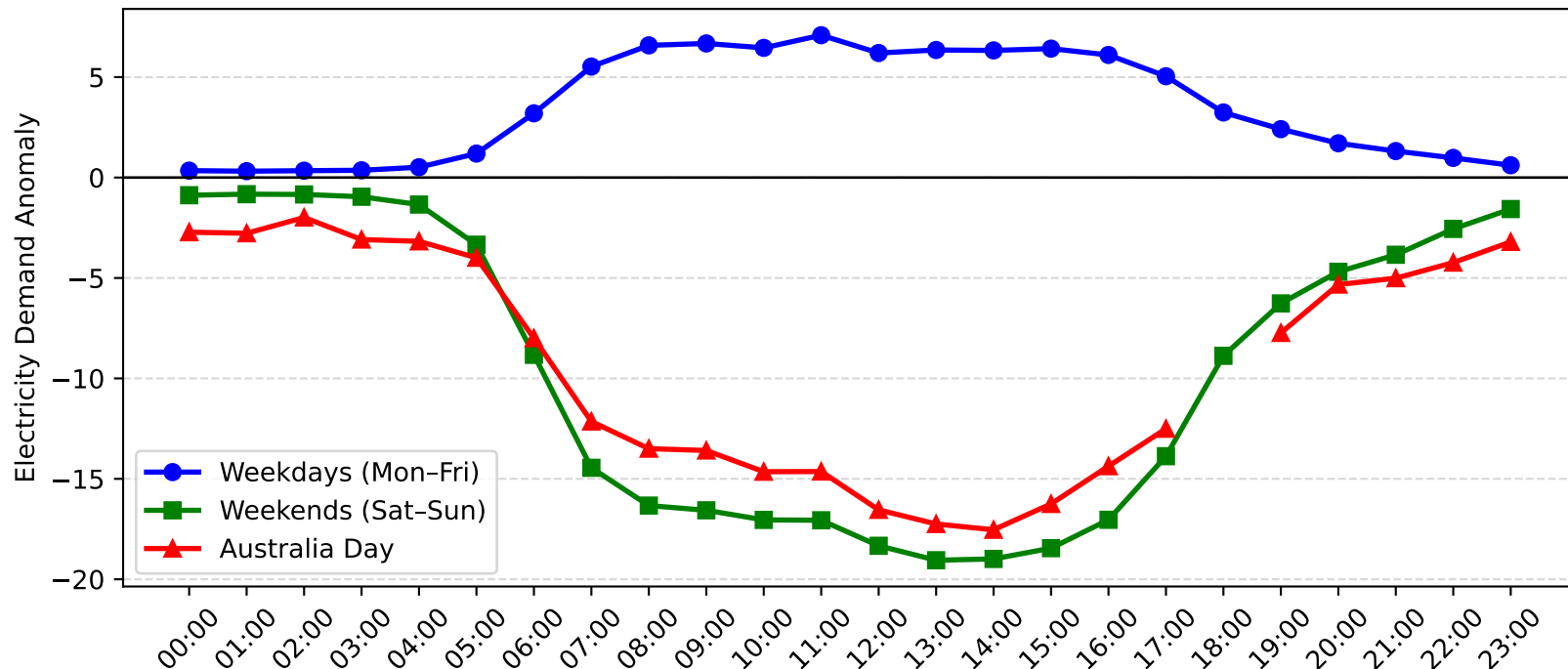
Gore Hill Demand Anomaly: Australia Day vs Weekday/Weekend (2005-2006)
