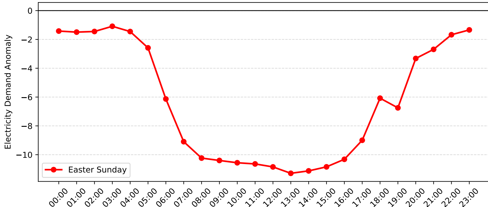
Macquarie Park Demand Anomaly: Easter Sunday (2008-2009)
