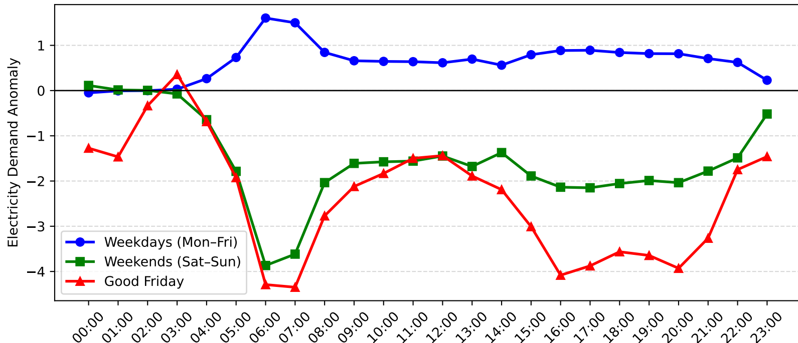
Revesby Demand Anomaly: Good Friday vs Weekday/Weekend (2008-2009)
