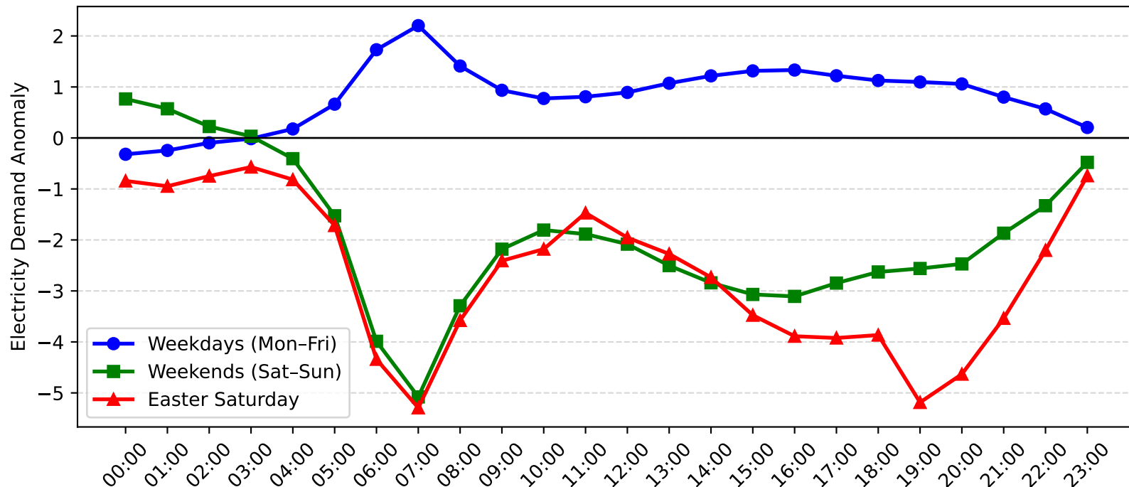
Kogarah Demand Anomaly: Easter Saturday vs Weekday/Weekend (2011-2012)
