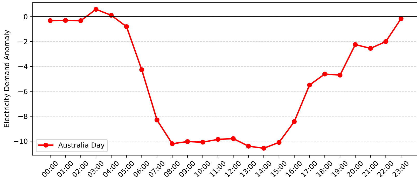
Zetland Demand Anomaly: Australia Day (2006-2007)
