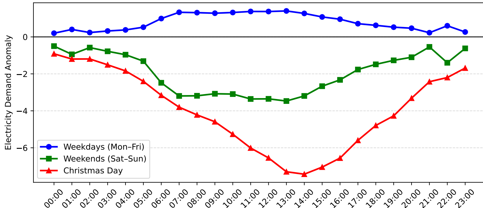
Cardiff Demand Anomaly: Christmas Day vs Weekday/Weekend (2006-2007)
