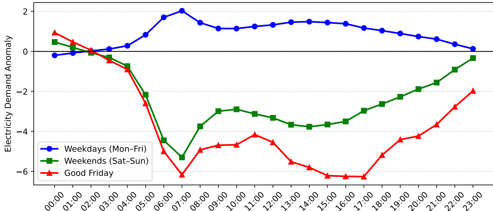
Campsie Demand Anomaly: Good Friday vs Weekday/Weekend (2012-2013)
