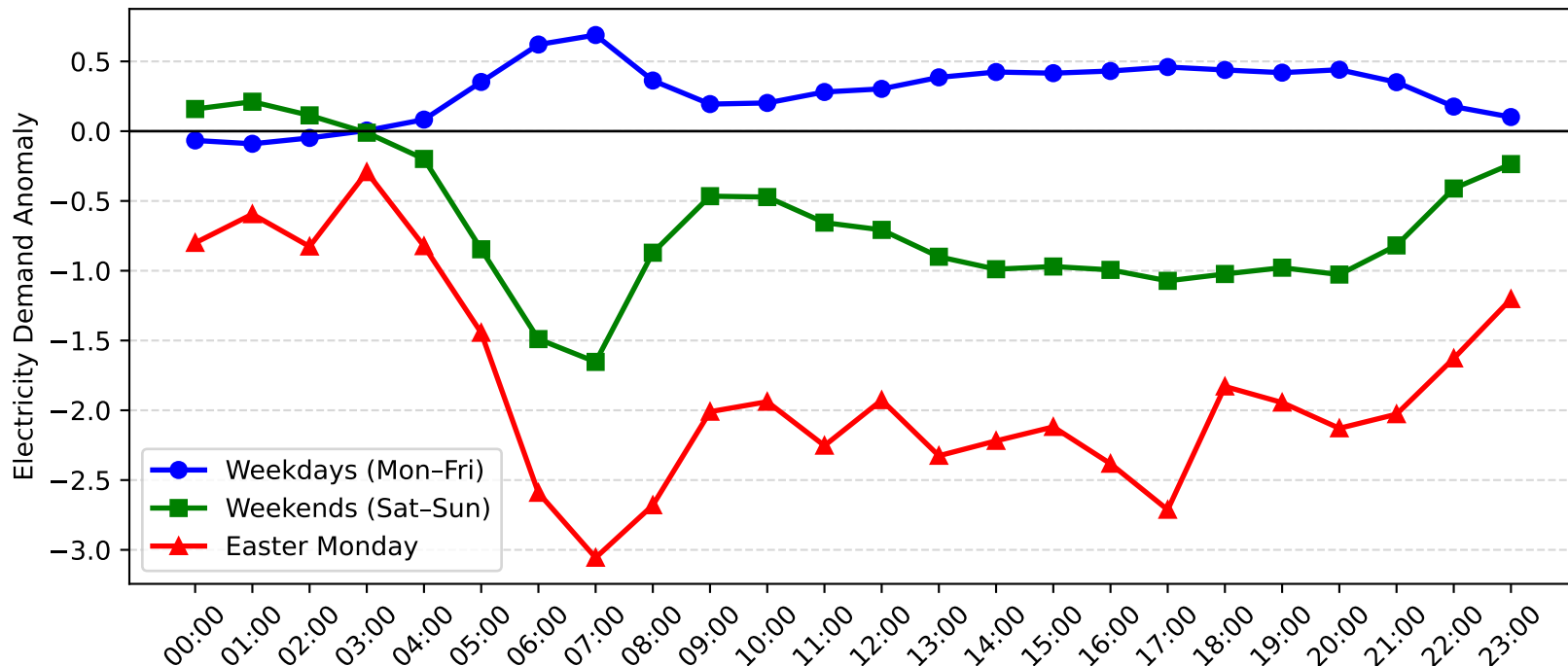
Charmhaven Demand Anomaly: Easter Monday vs Weekday/Weekend (2012-2013)
