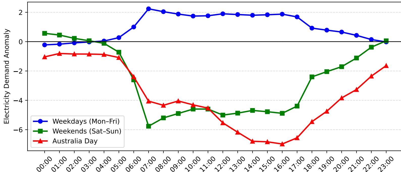
Epping Demand Anomaly: Australia Day vs Weekday/Weekend (2016-2017)
