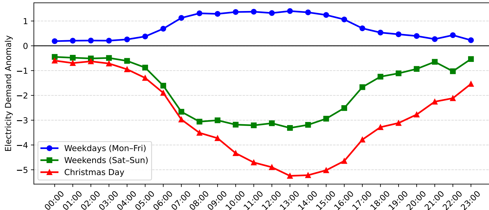
Mayfield West Demand Anomaly: Christmas Day vs Weekday/Weekend (2011-2012)
