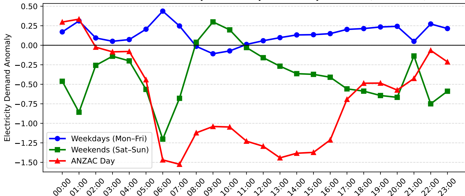
Morisset Demand Anomaly: ANZAC Day vs Weekday/Weekend (2012-2013)
