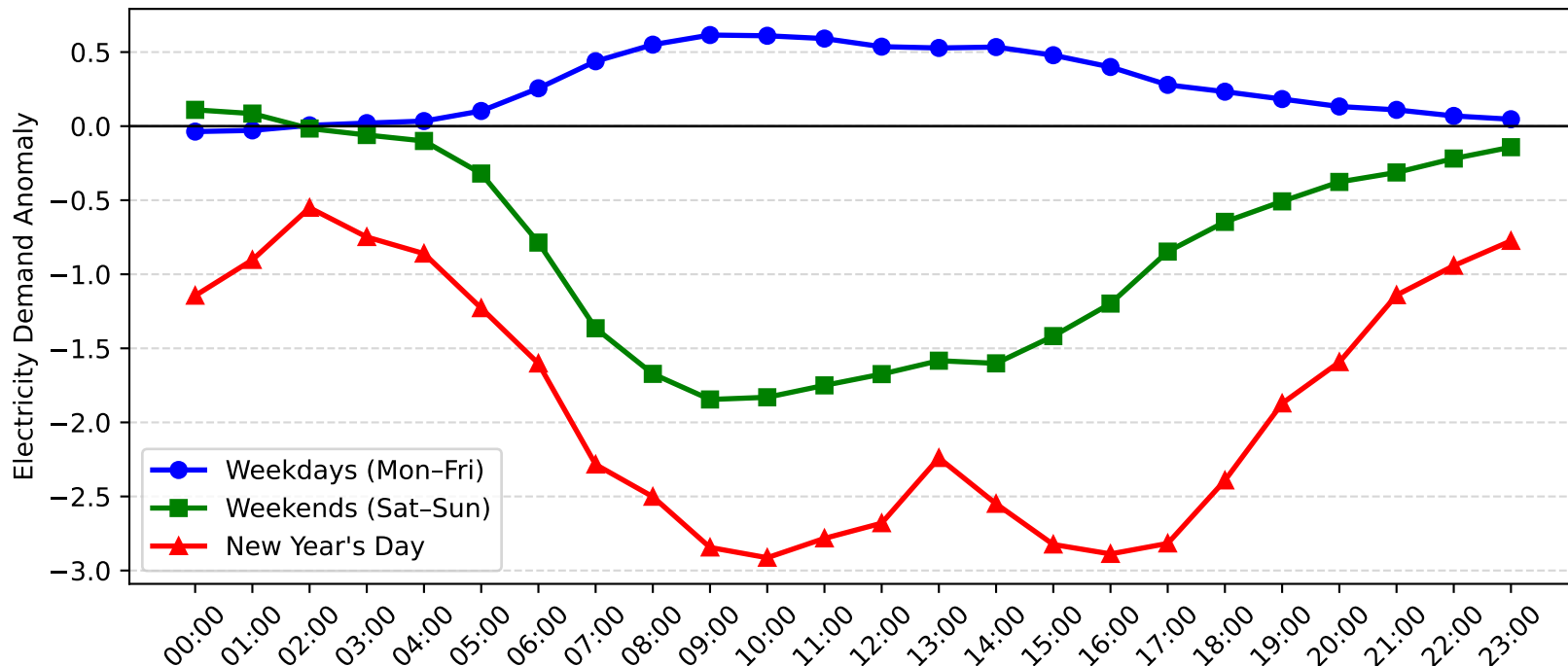
Lidcombe Demand Anomaly: New Year's Day vs Weekday/Weekend (2014-2015)
