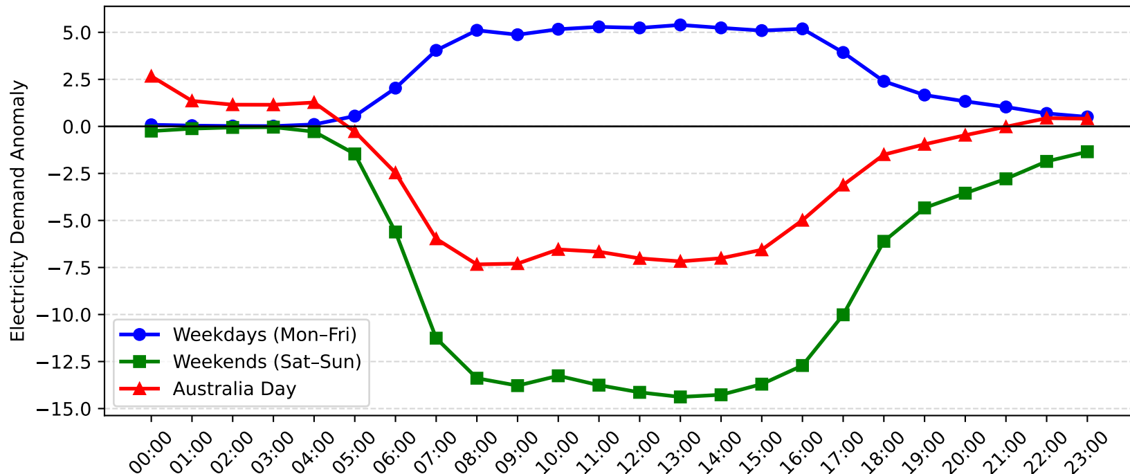
Gore Hill Demand Anomaly: Australia Day vs Weekday/Weekend (2010-2011)
