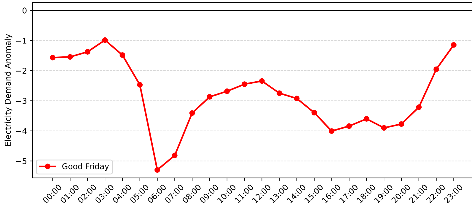
Revesby Demand Anomaly: Good Friday (2006-2007)
