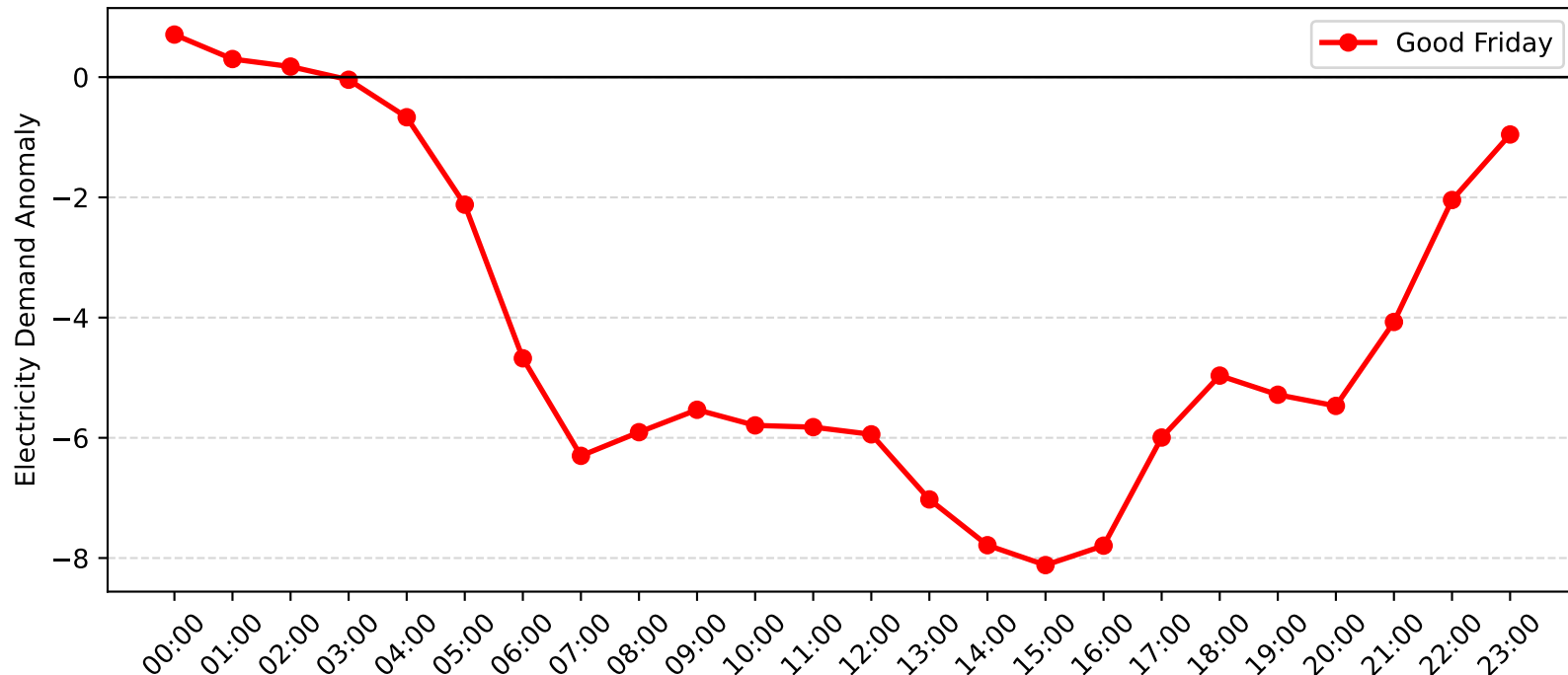
Campsie Demand Anomaly: Good Friday (2007-2008)
