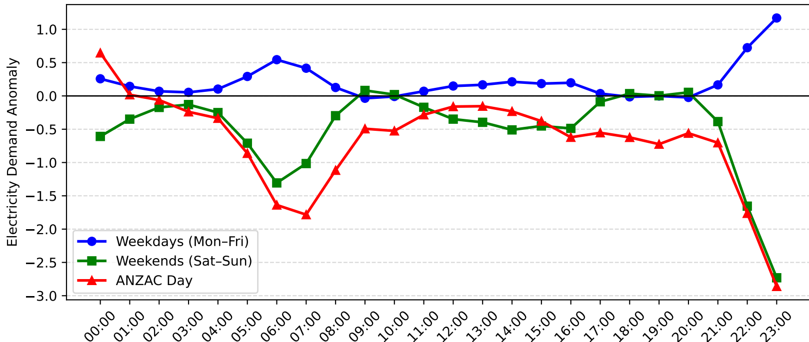
Muswellbrook Demand Anomaly: ANZAC Day vs Weekday/Weekend (2008-2009)
