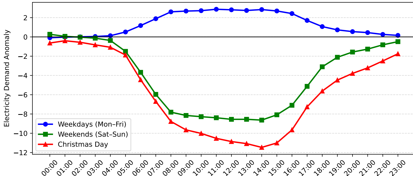
Mascot Demand Anomaly: Christmas Day vs Weekday/Weekend (2013-2014)
