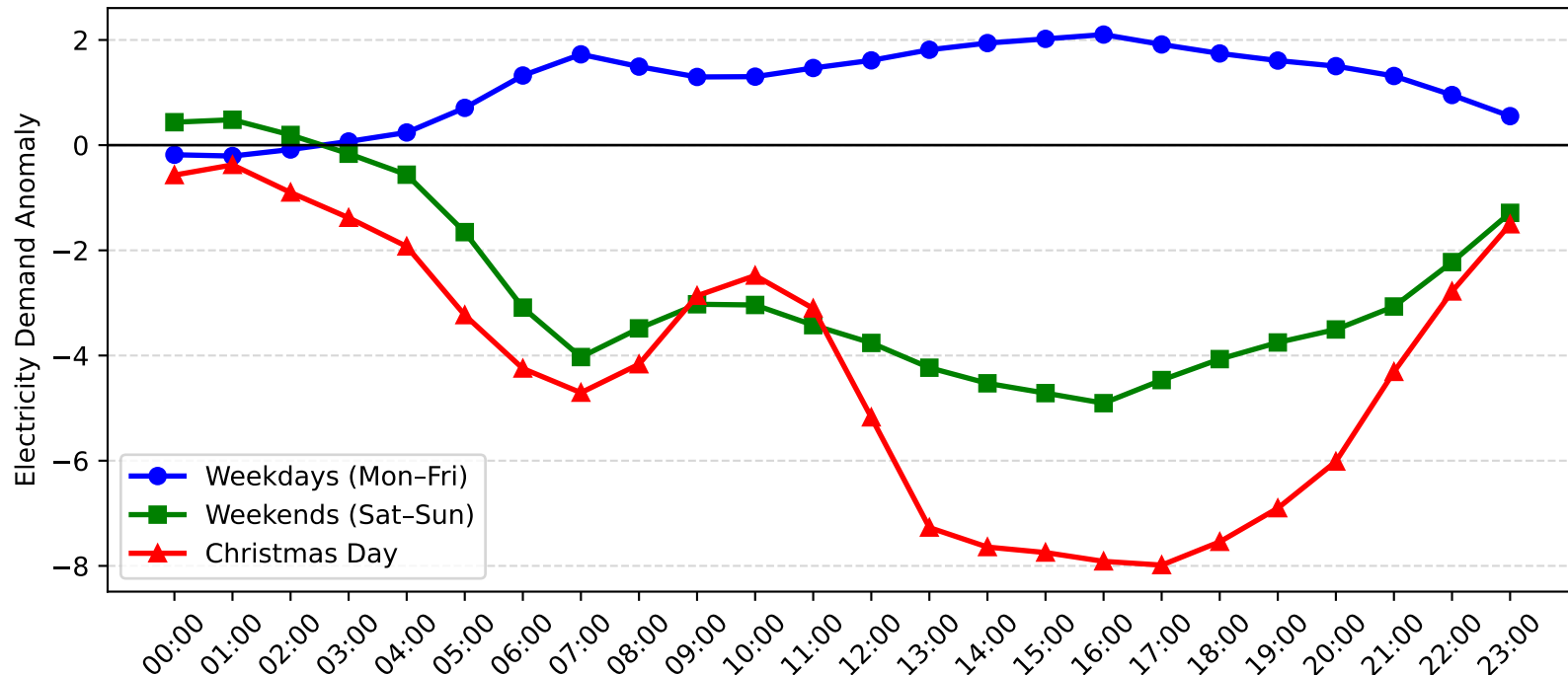
Campsie Demand Anomaly: Christmas Day vs Weekday/Weekend (2016-2017)
