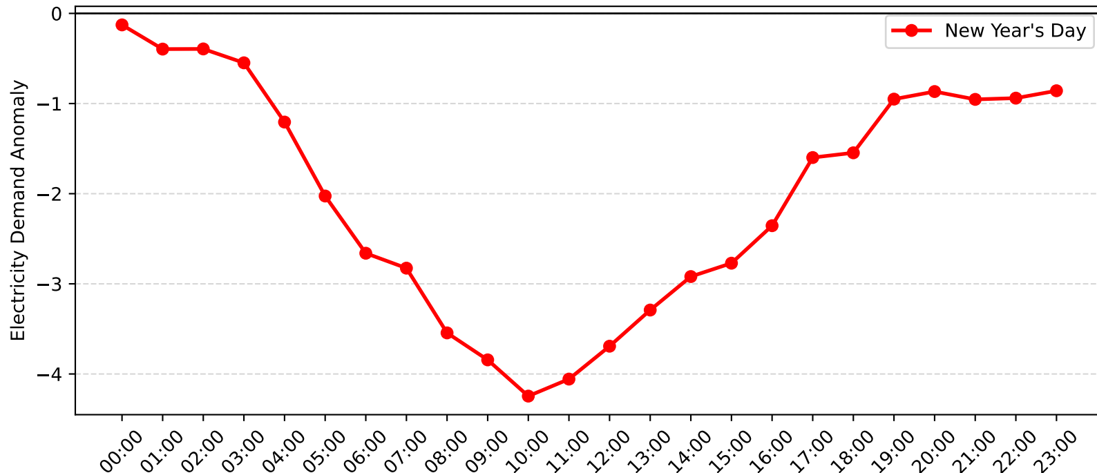
Lidcombe Demand Anomaly: New Year's Day (2008-2009)
