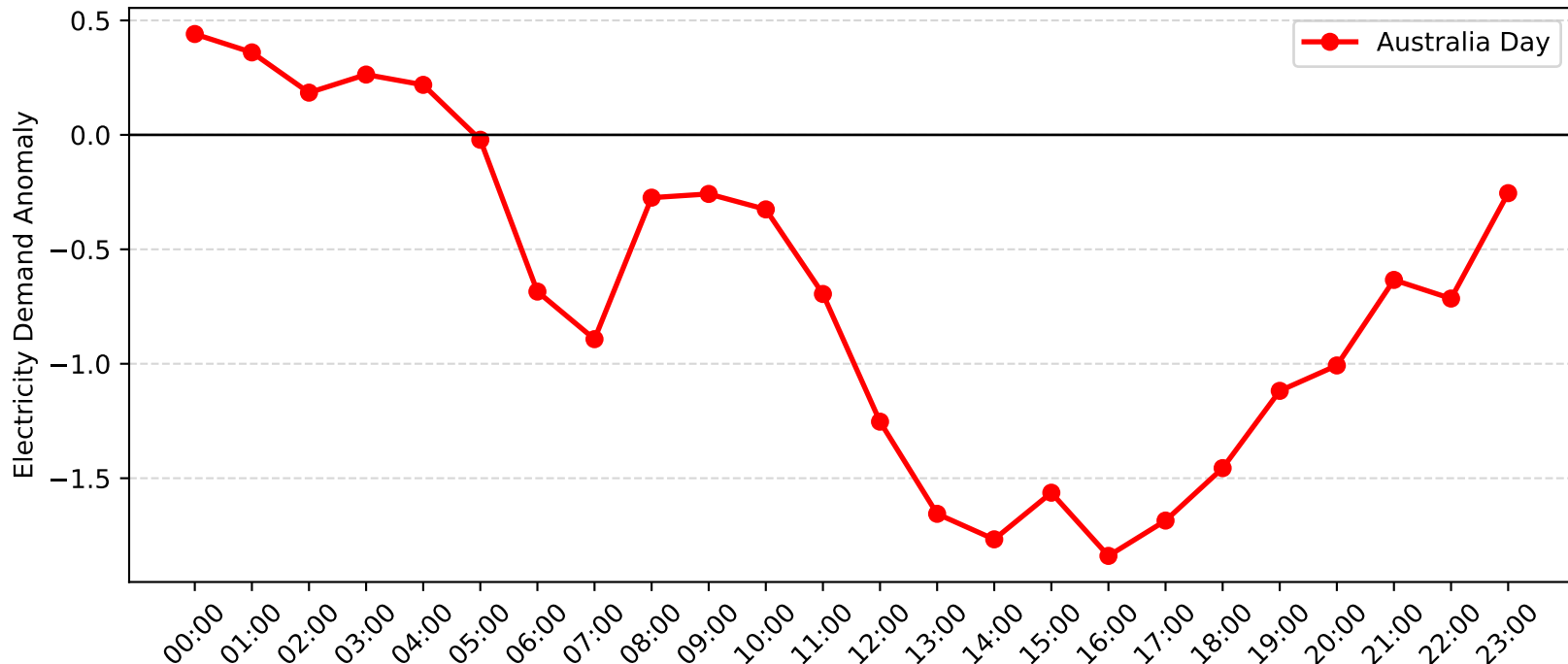
Morisset Demand Anomaly: Australia Day (2015-2016)
