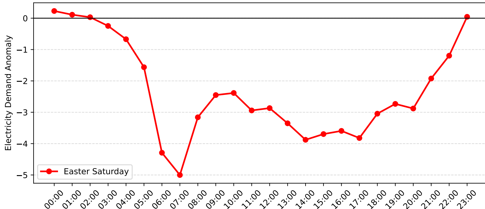
Mortdale Demand Anomaly: Easter Saturday (2007-2008)
