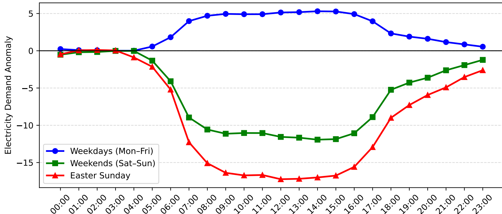
Gore Hill Demand Anomaly: Easter Sunday vs Weekday/Weekend (2012-2013)
