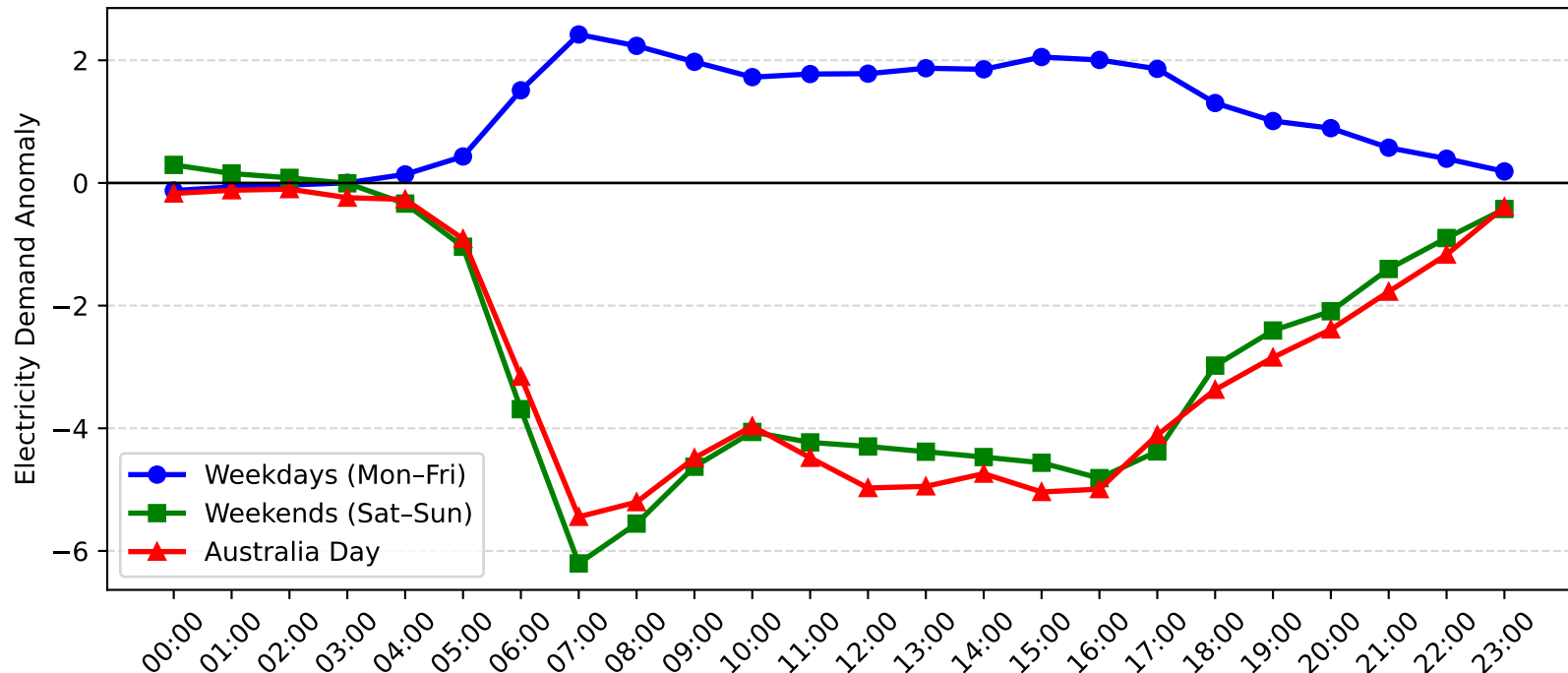
Chatswood Demand Anomaly: Australia Day vs Weekday/Weekend (2008-2009)
