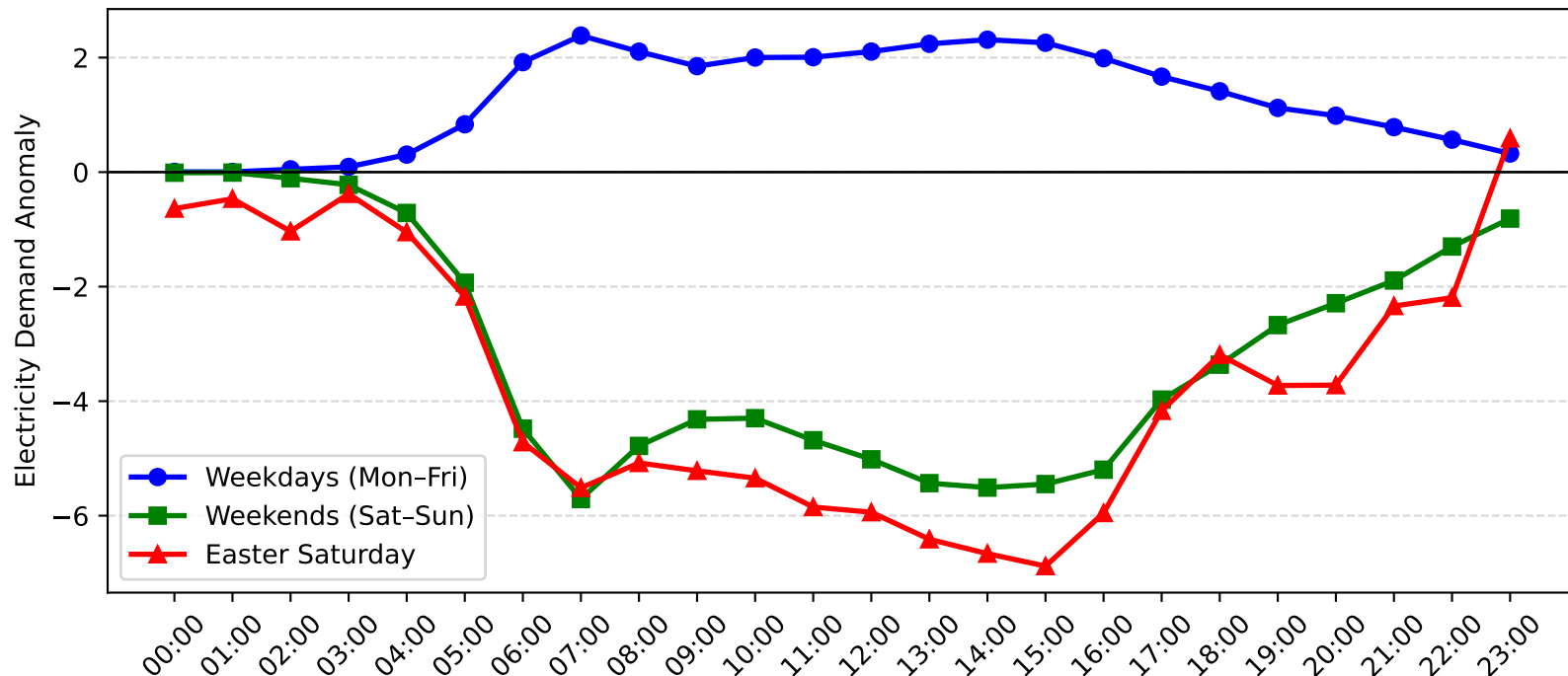
Sefton Demand Anomaly: Easter Saturday vs Weekday/Weekend (2005-2006)
