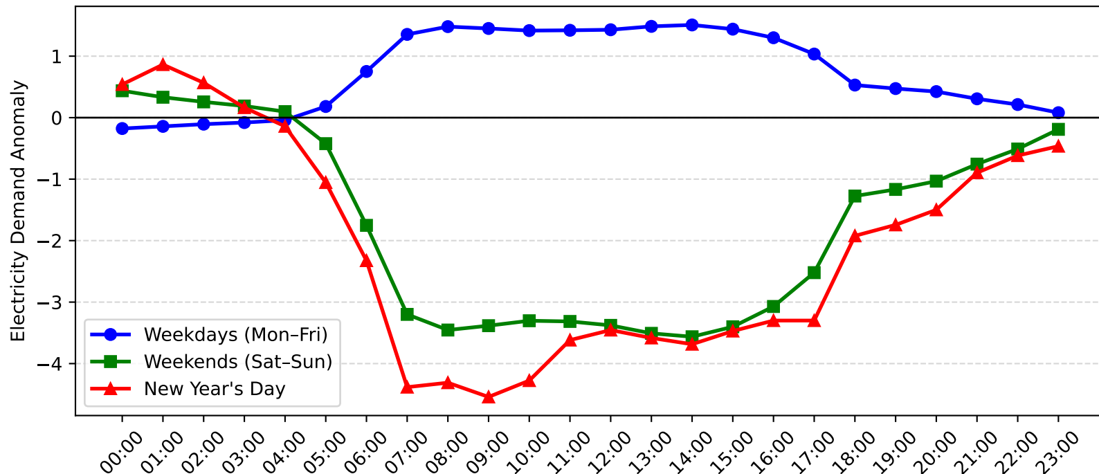
Concord Demand Anomaly: New Year's Day vs Weekday/Weekend (2012-2013)
