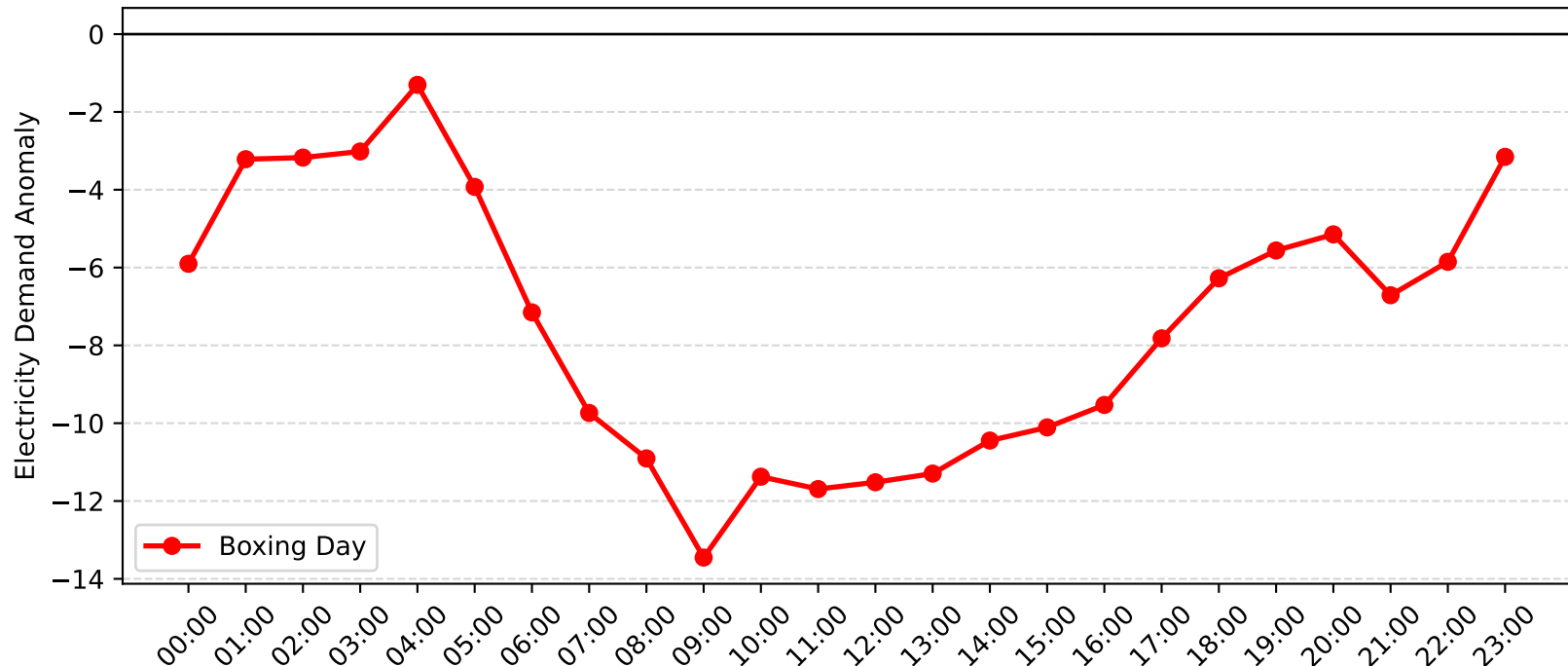
Macquarie Park Demand Anomaly: Boxing Day (2007-2008)
