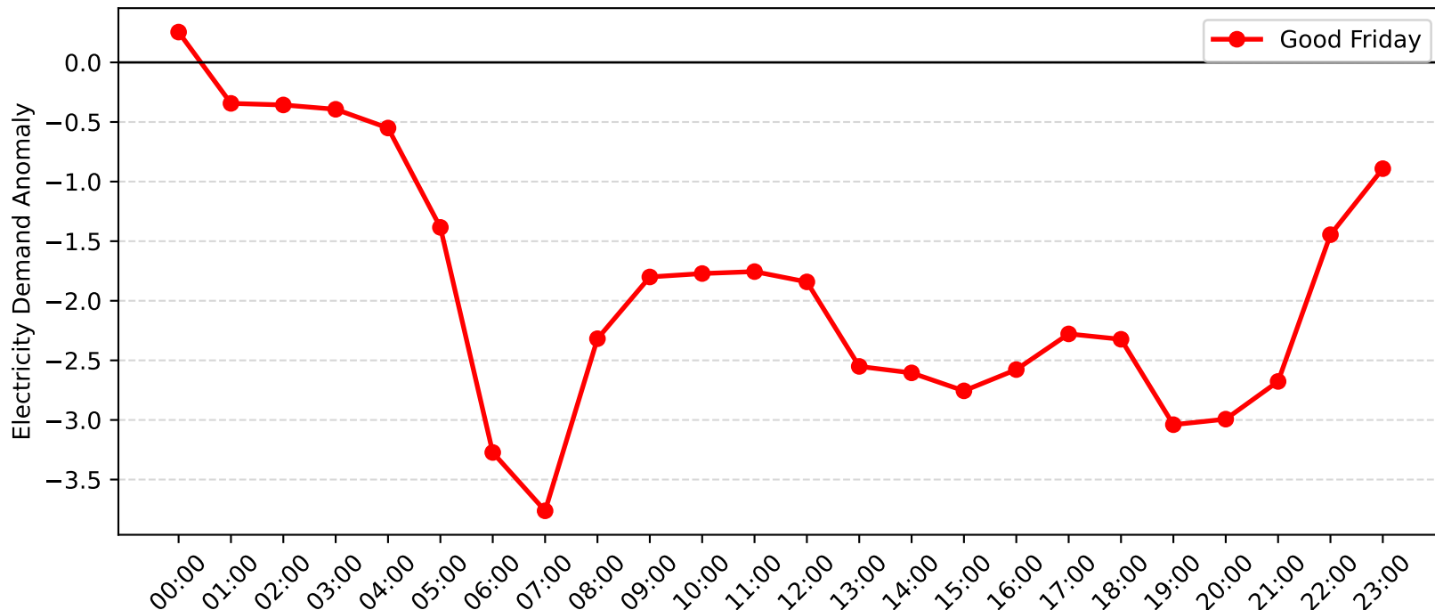
Mortdale Demand Anomaly: Good Friday (2017-2018)
