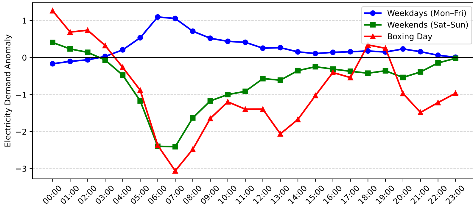
Revesby Demand Anomaly: Boxing Day vs Weekday/Weekend (2010-2011)
