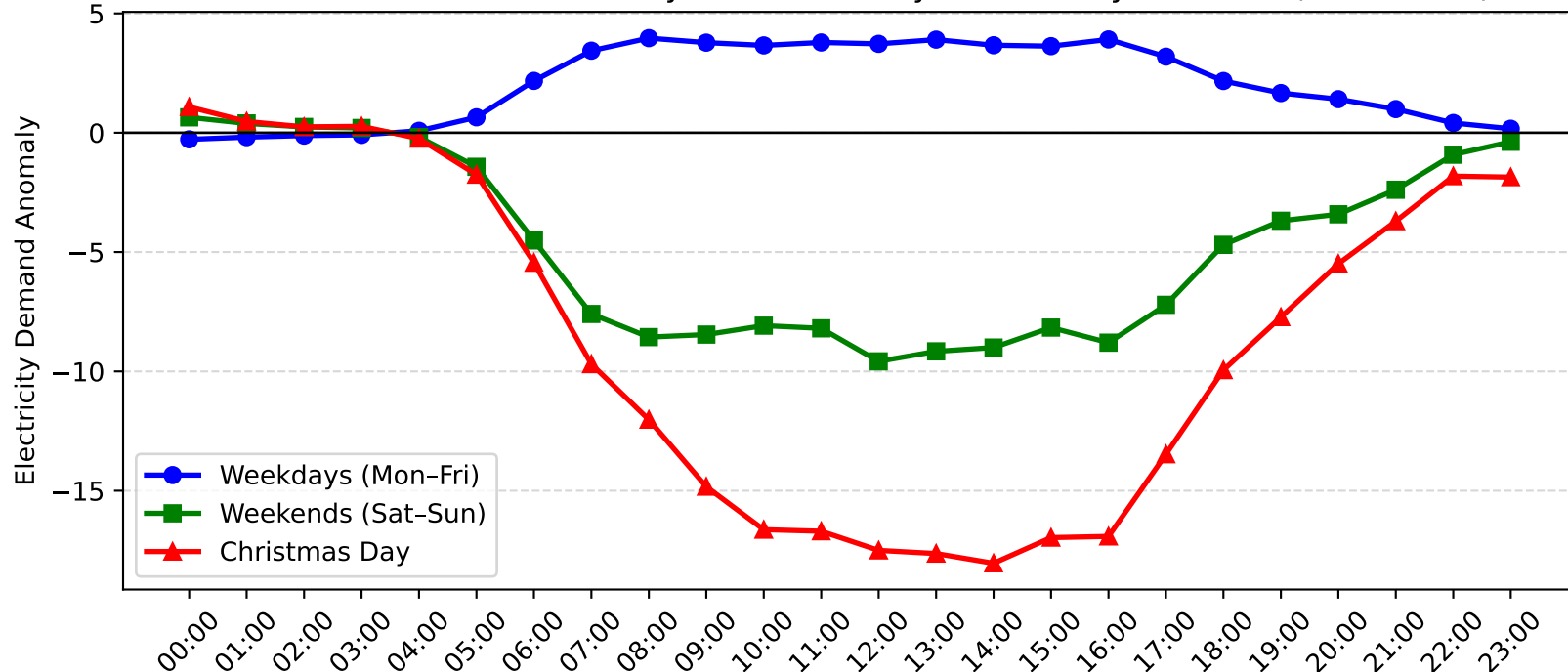
Castle Cove Demand Anomaly: Christmas Day vs Weekday/Weekend (2004-2005)
