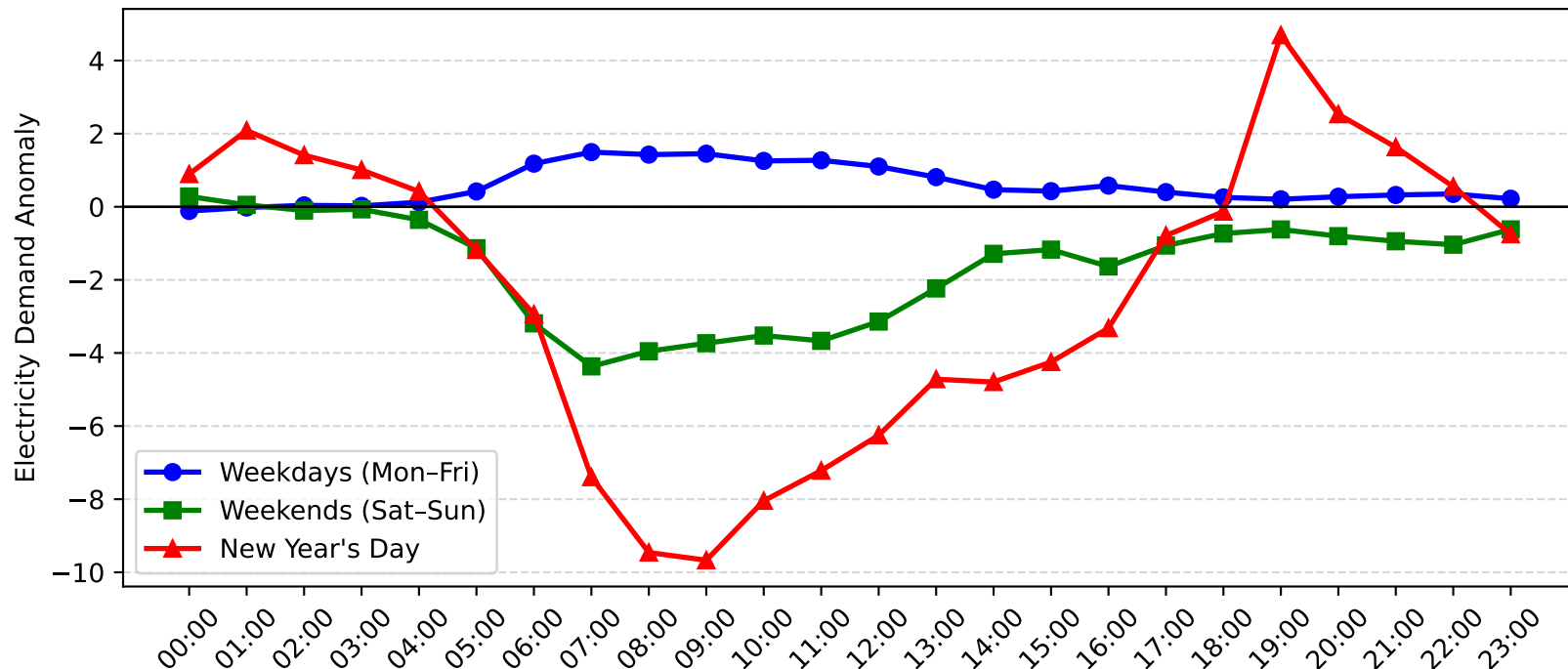
Meadowbank Demand Anomaly: New Year's Day vs Weekday/Weekend (2008-2009)
