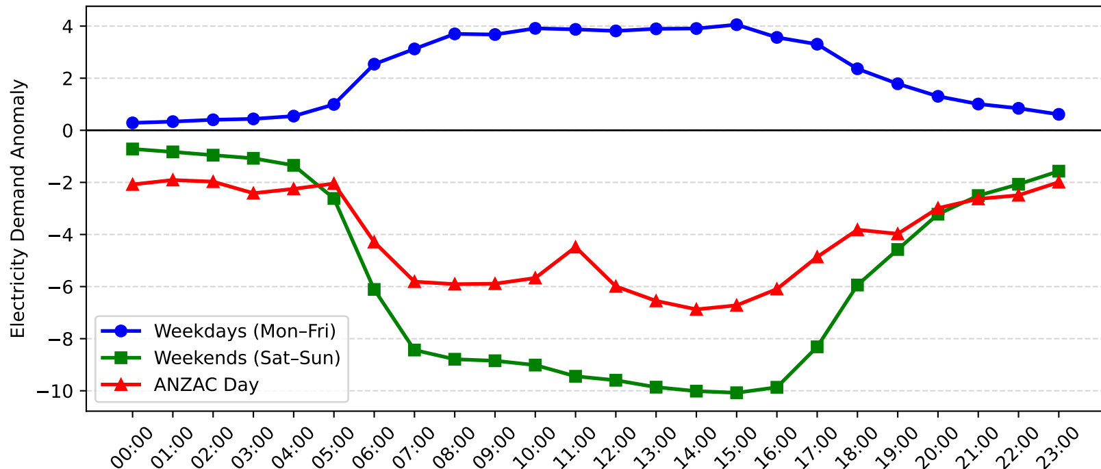
Macquarie Park Demand Anomaly: ANZAC Day vs Weekday/Weekend (2005-2006)
