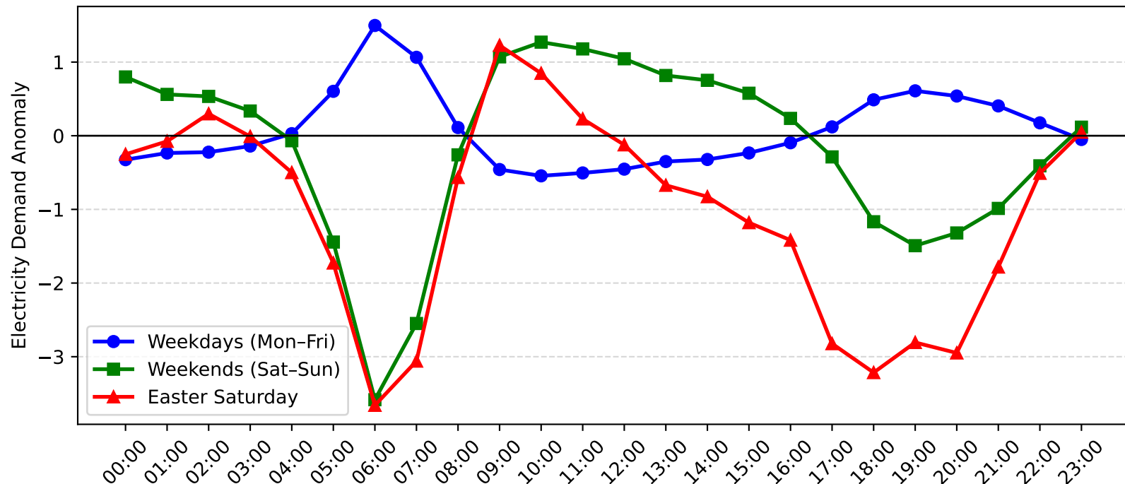
Cronulla Demand Anomaly: Easter Saturday vs Weekday/Weekend (2007-2008)
