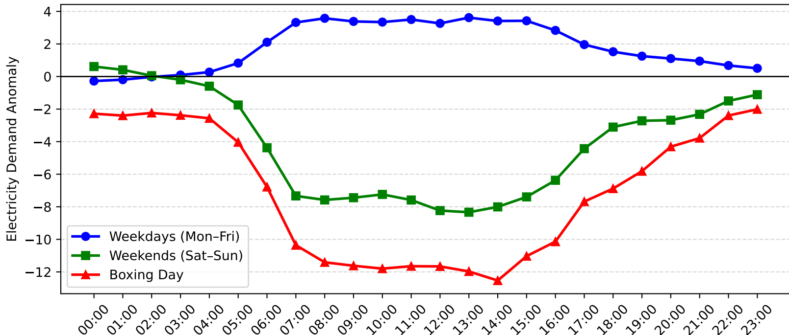
Marrickville Demand Anomaly: Boxing Day vs Weekday/Weekend (2004-2005)
