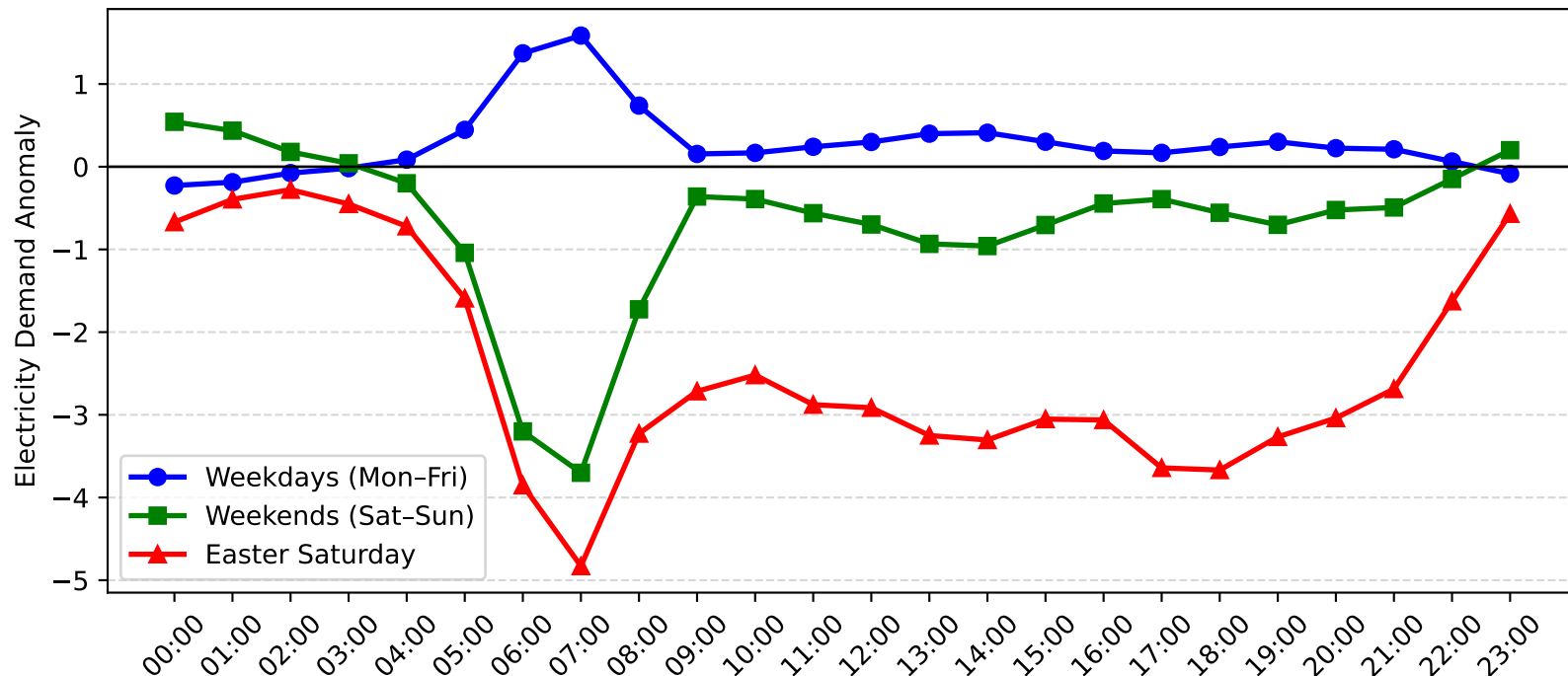
Mortdale Demand Anomaly: Easter Saturday vs Weekday/Weekend (2013-2014)
