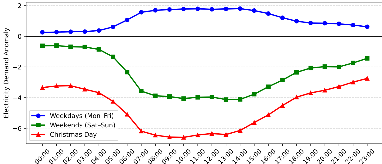
Leightonfield Demand Anomaly: Christmas Day vs Weekday/Weekend (2010-2011)
