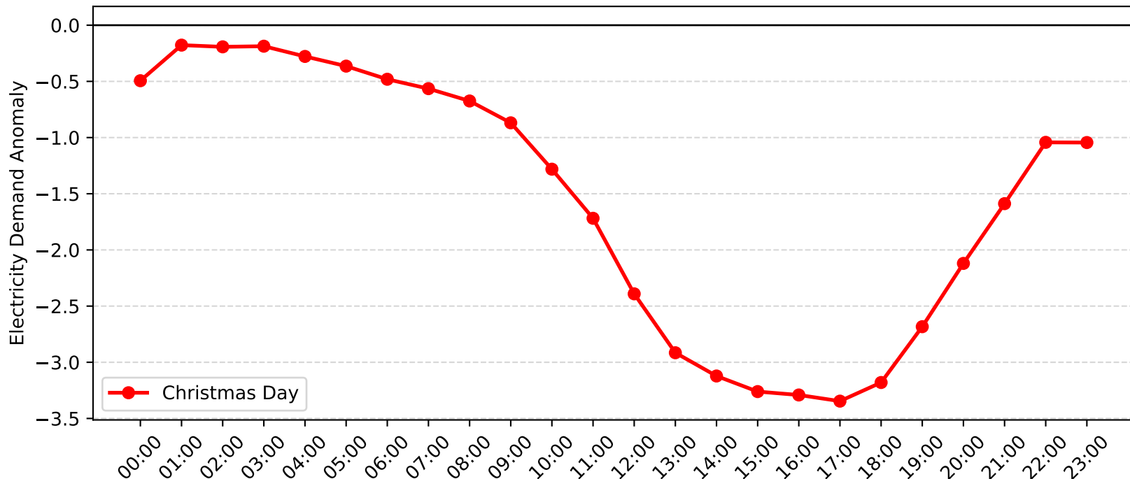
Telarah Demand Anomaly: Christmas Day (2006-2007)
