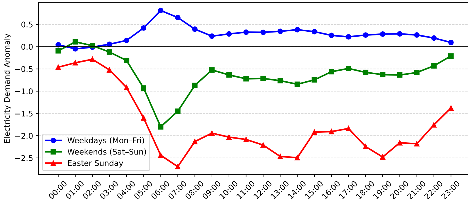
Berowra Demand Anomaly: Easter Sunday vs Weekday/Weekend (2017-2018)
