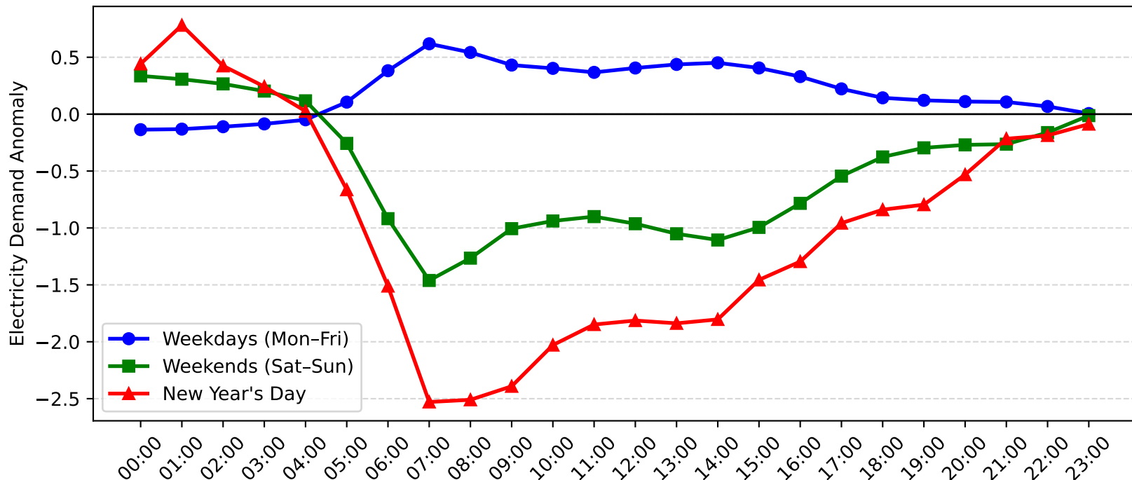
Arncliffe Demand Anomaly: New Year's Day vs Weekday/Weekend (2012-2013)
