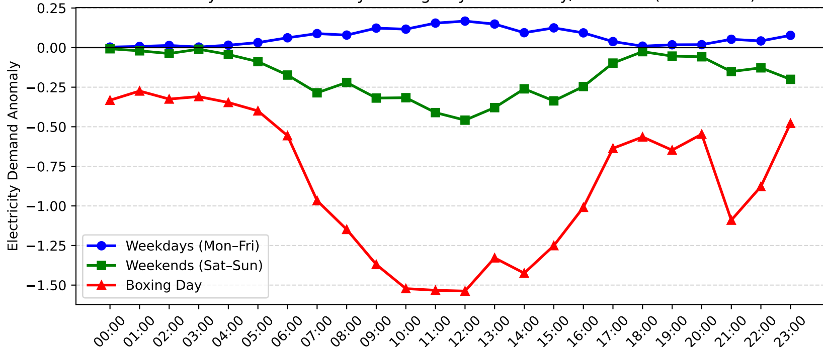
Rothbury Demand Anomaly: Boxing Day vs Weekday/Weekend (2008-2009)
