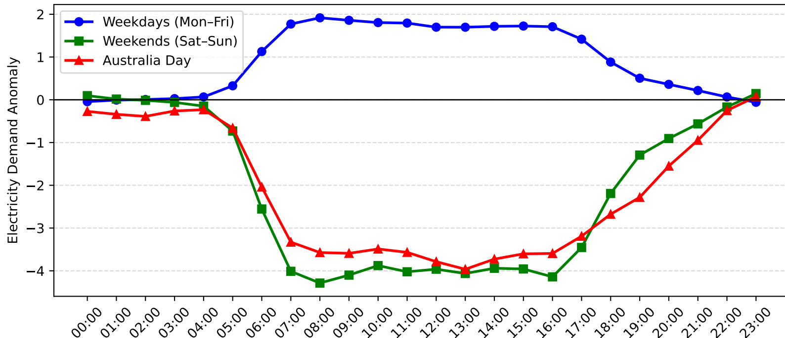
Pymble Demand Anomaly: Australia Day vs Weekday/Weekend (2007-2008)
