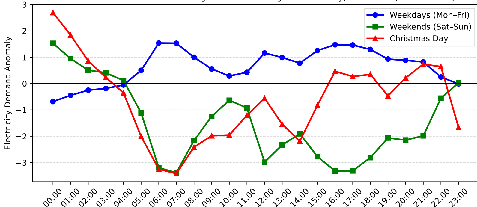
Pennant Hills Demand Anomaly: Christmas Day vs Weekday/Weekend (2004-2005)
