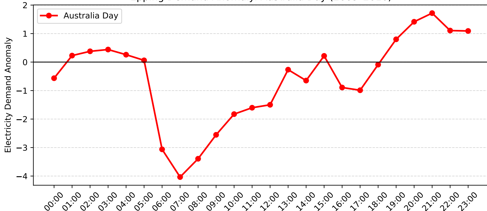
Epping Demand Anomaly: Australia Day (2009-2010)
