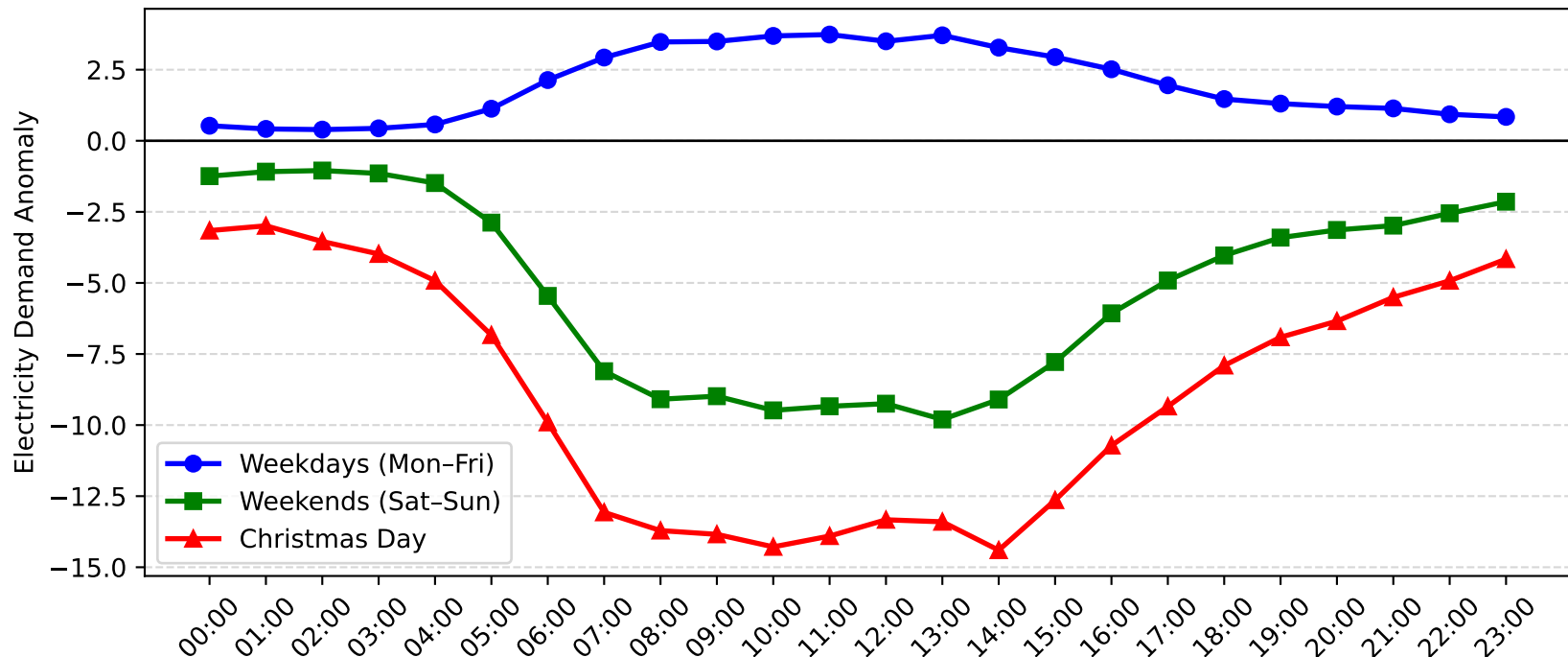
Milperra Demand Anomaly: Christmas Day vs Weekday/Weekend (2009-2010)
