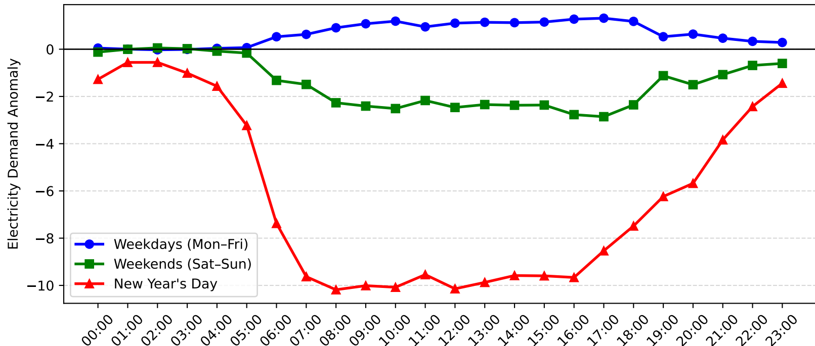
Burwood Demand Anomaly: New Year's Day vs Weekday/Weekend (2004-2005)
