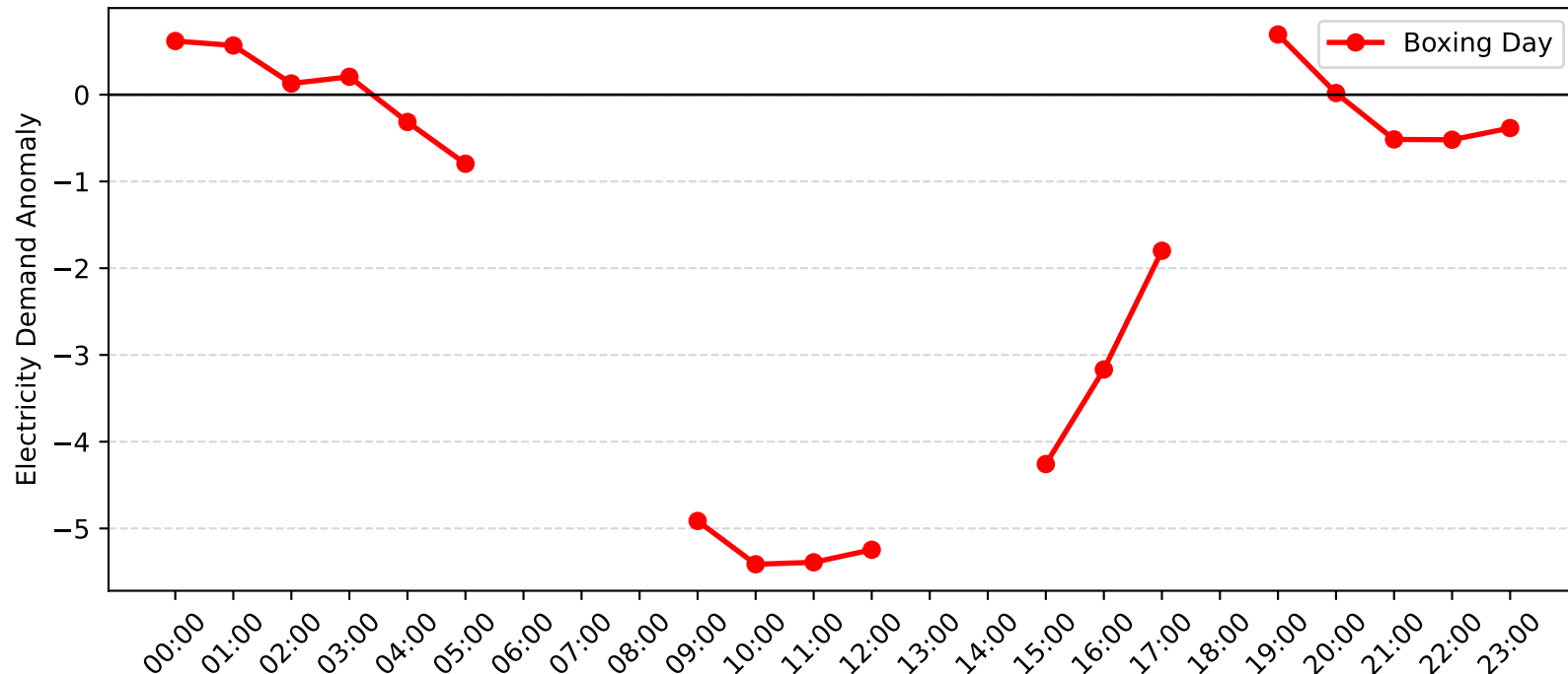
Bankstown Demand Anomaly: Boxing Day (2009-2010)
