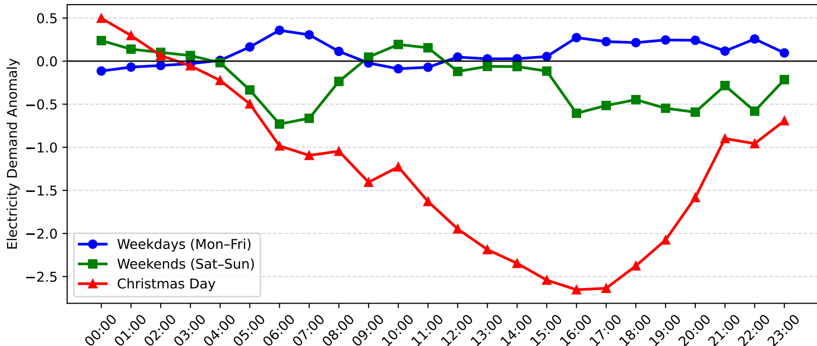
Narrabeen Demand Anomaly: Christmas Day vs Weekday/Weekend (2004-2005)
