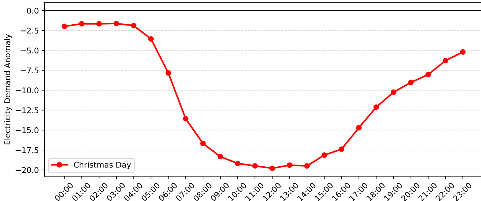
Gore Hill Demand Anomaly: Christmas Day (2005-2006)
