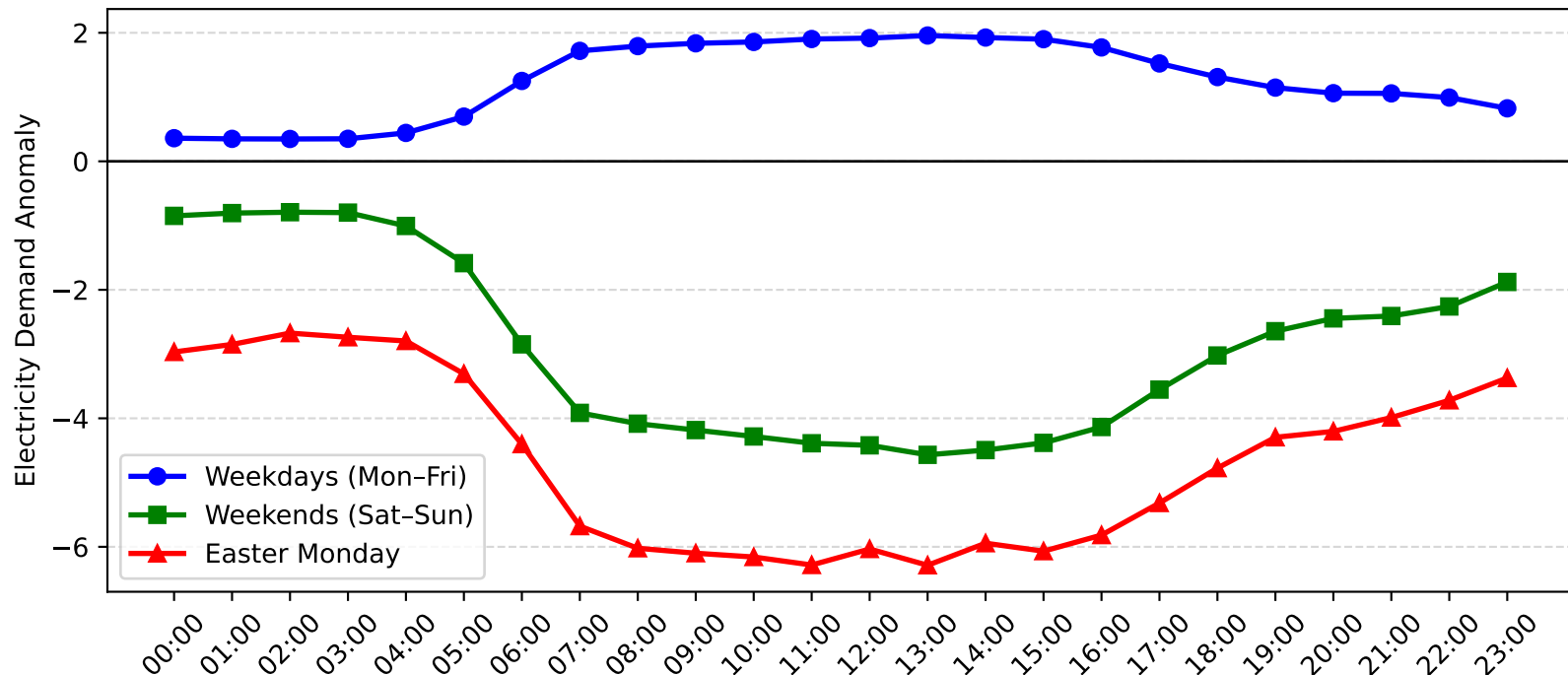
Leightonfield Demand Anomaly: Easter Monday vs Weekday/Weekend (2015-2016)
