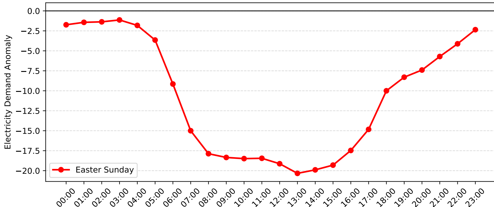
Gore Hill Demand Anomaly: Easter Sunday (2007-2008)
