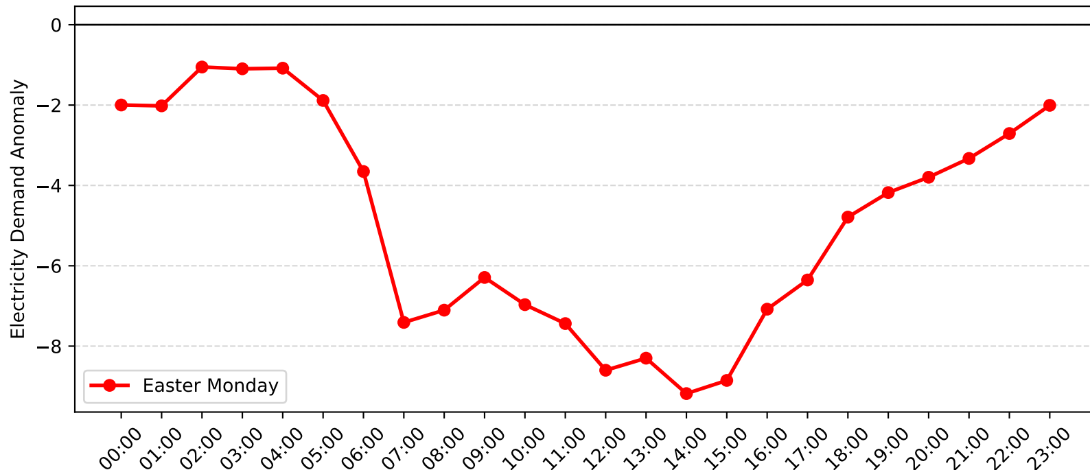
Gore Hill Demand Anomaly: Easter Monday (2014-2015)
