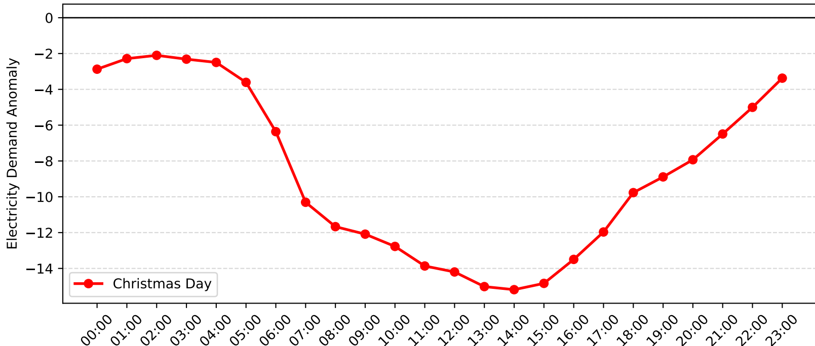
St. Peters Demand Anomaly: Christmas Day (2016-2017)
