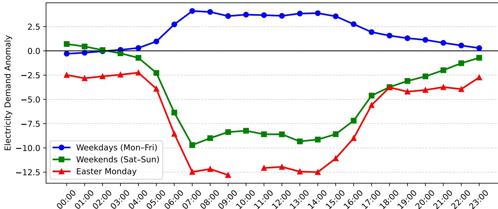
Marrickville Demand Anomaly: Easter Monday vs Weekday/Weekend (2005-2006)
