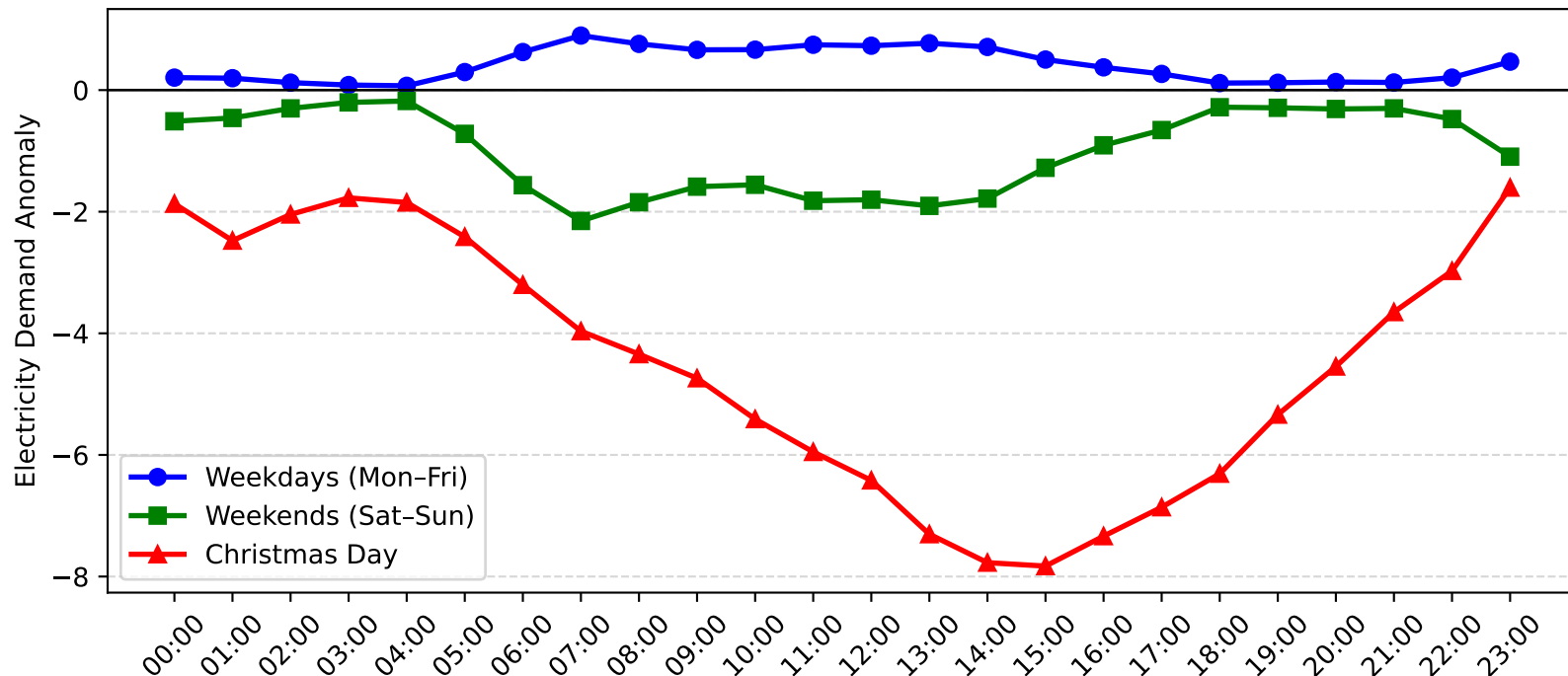
Rutherford Demand Anomaly: Christmas Day vs Weekday/Weekend (2006-2007)
