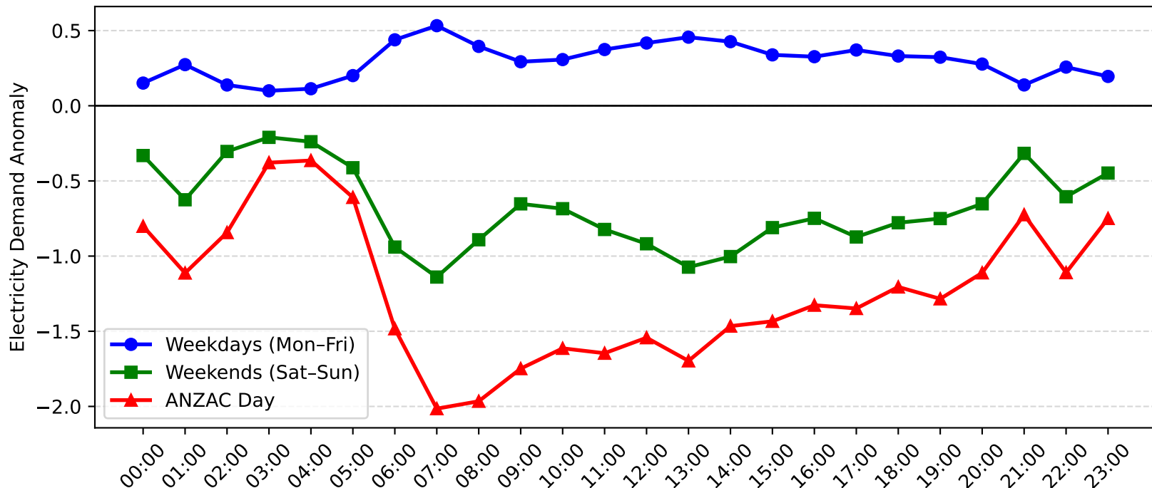
Gateshead Demand Anomaly: ANZAC Day vs Weekday/Weekend (2010-2011)
