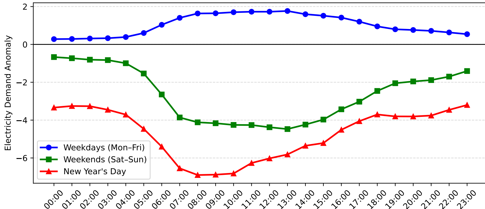
Leightonfield Demand Anomaly: New Year's Day vs Weekday/Weekend (2010-2011)
