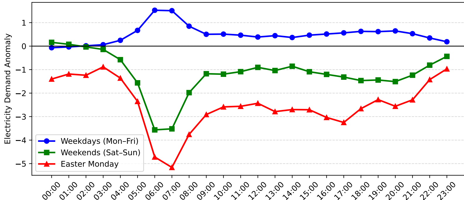
Revesby Demand Anomaly: Easter Monday vs Weekday/Weekend (2012-2013)
