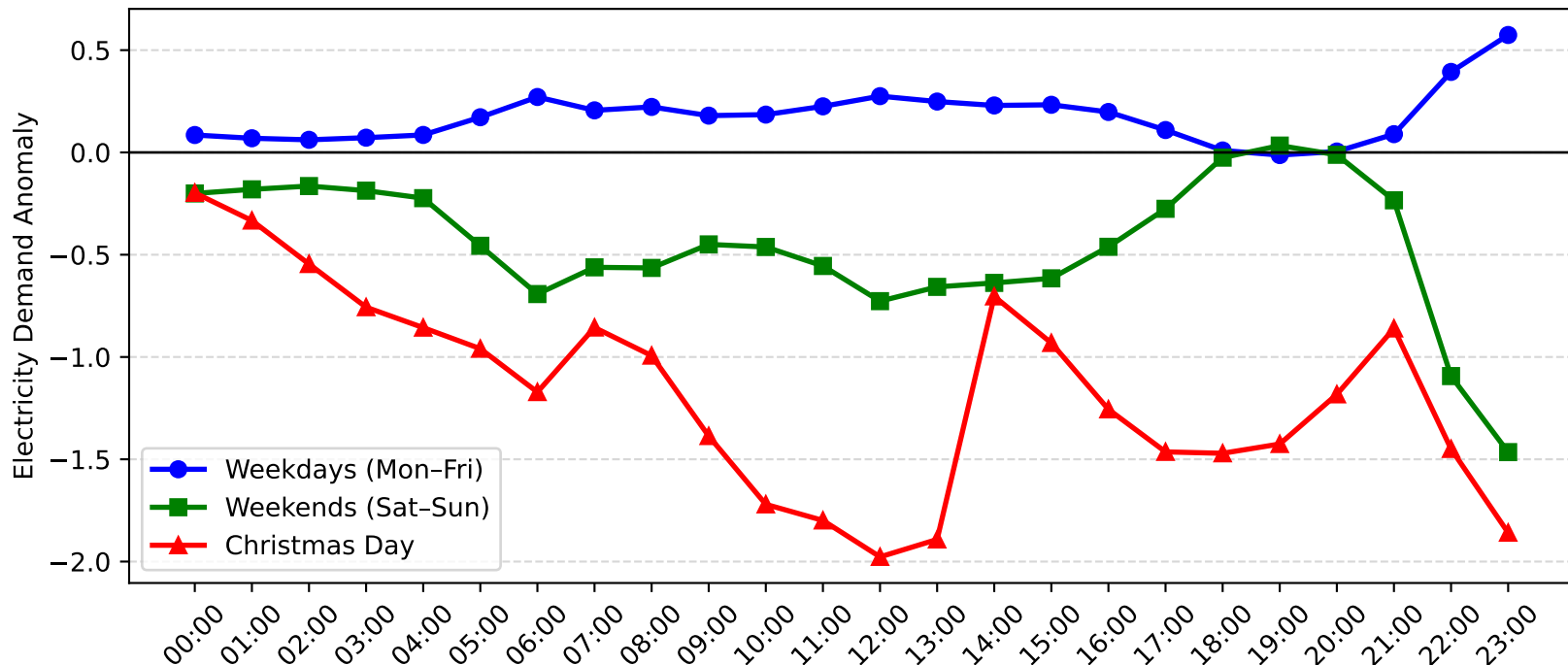
Muswellbrook Demand Anomaly: Christmas Day vs Weekday/Weekend (2009-2010)
