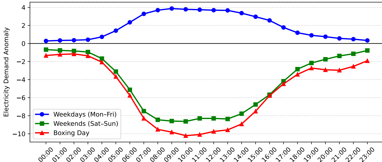
Homebush Bay Demand Anomaly: Boxing Day vs Weekday/Weekend (2010-2011)
