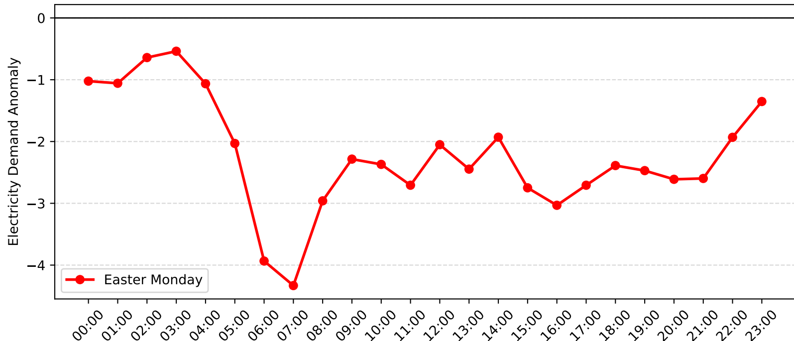
Revesby Demand Anomaly: Easter Monday (2015-2016)
