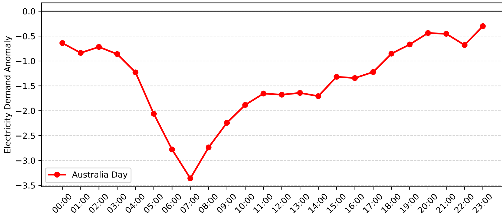
Lisarow Demand Anomaly: Australia Day (2009-2010)
