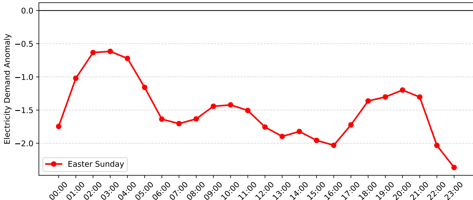
Muswellbrook Demand Anomaly: Easter Sunday (2010-2011)
