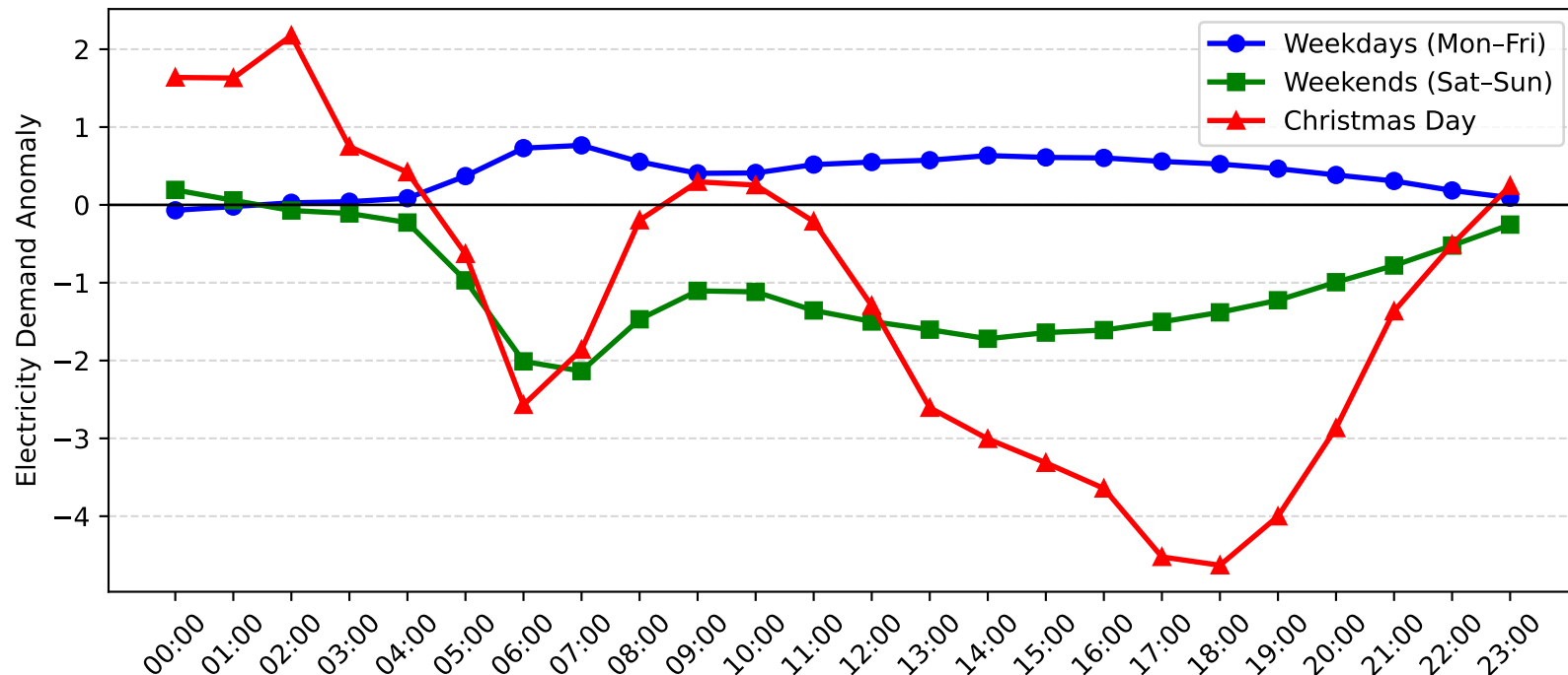
Dee Why West Demand Anomaly: Christmas Day vs Weekday/Weekend (2014-2015)
