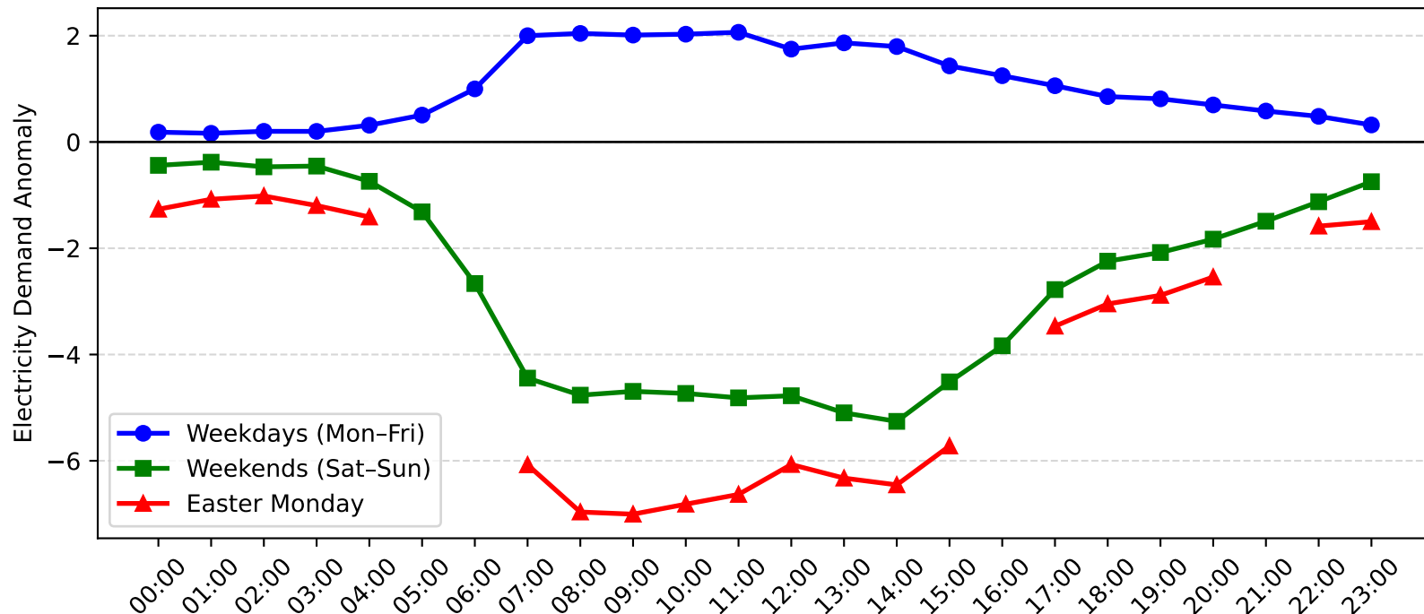
Bankstown Demand Anomaly: Easter Monday vs Weekday/Weekend (2010-2011)
