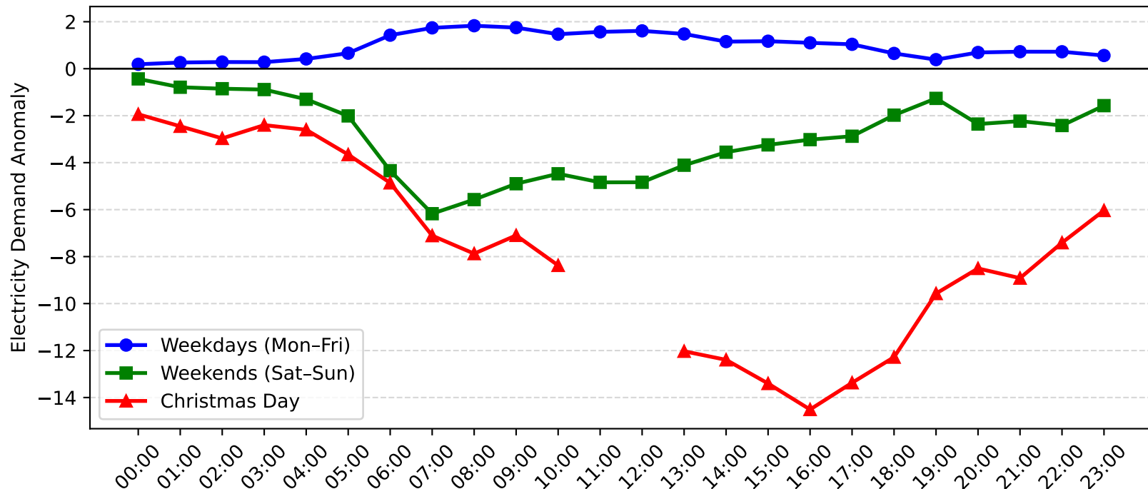
Meadowbank Demand Anomaly: Christmas Day vs Weekday/Weekend (2008-2009)
