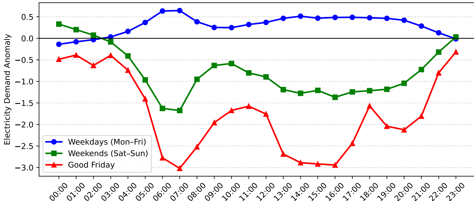
Charmhaven Demand Anomaly: Good Friday vs Weekday/Weekend (2006-2007)
