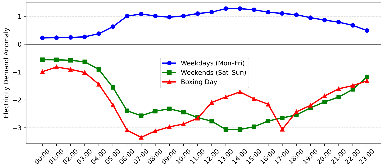
Lisarow Demand Anomaly: Boxing Day vs Weekday/Weekend (2015-2016)
