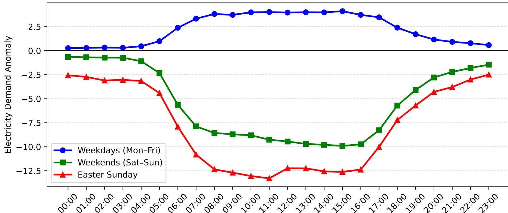
Macquarie Park Demand Anomaly: Easter Sunday vs Weekday/Weekend (2005-2006)
