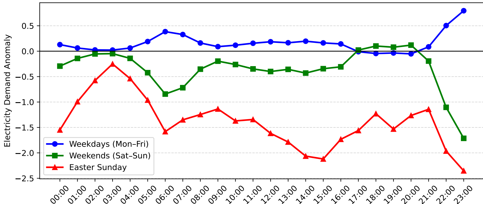
Muswellbrook Demand Anomaly: Easter Sunday vs Weekday/Weekend (2009-2010)
