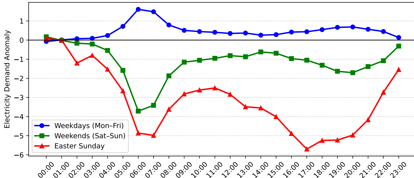
Revesby Demand Anomaly: Easter Sunday vs Weekday/Weekend (2010-2011)
