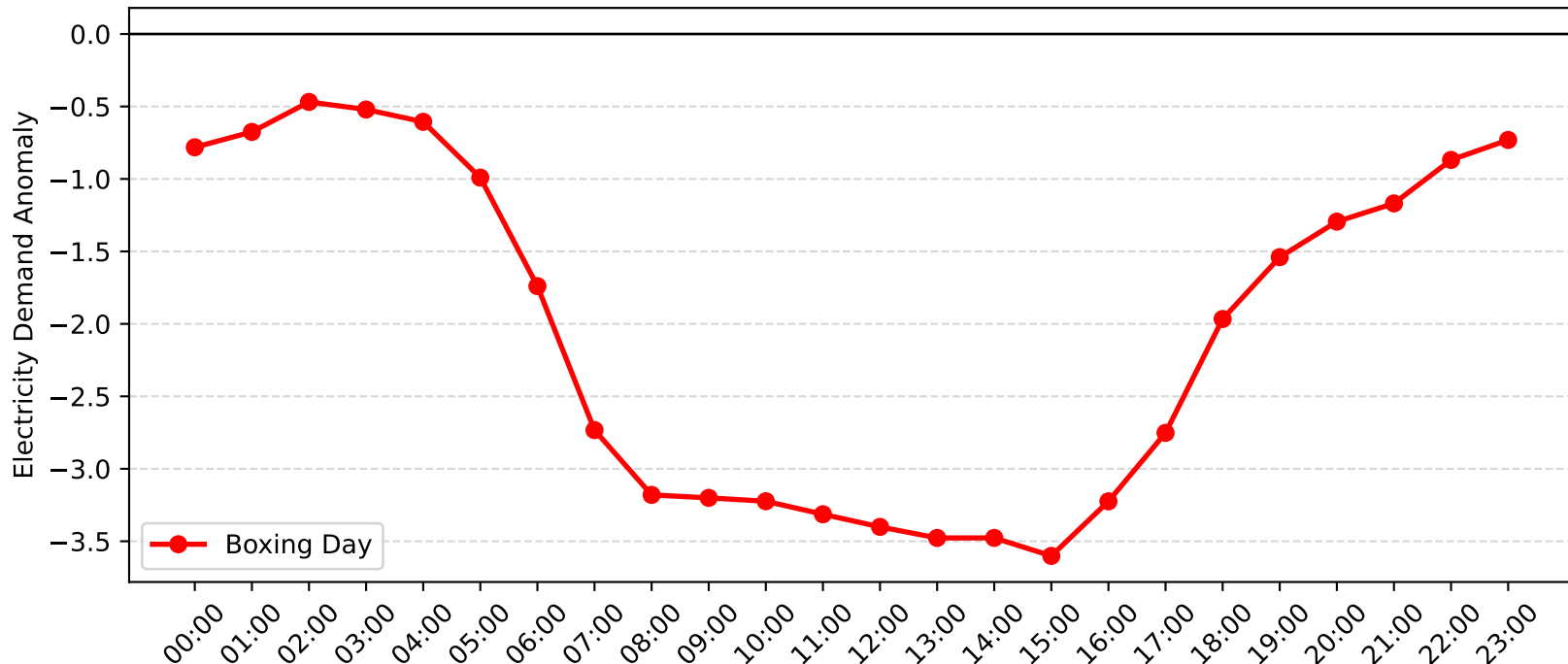
Beacon Hill Demand Anomaly: Boxing Day (2011-2012)
