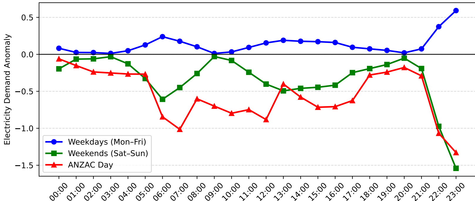
Muswellbrook Demand Anomaly: ANZAC Day vs Weekday/Weekend (2013-2014)
