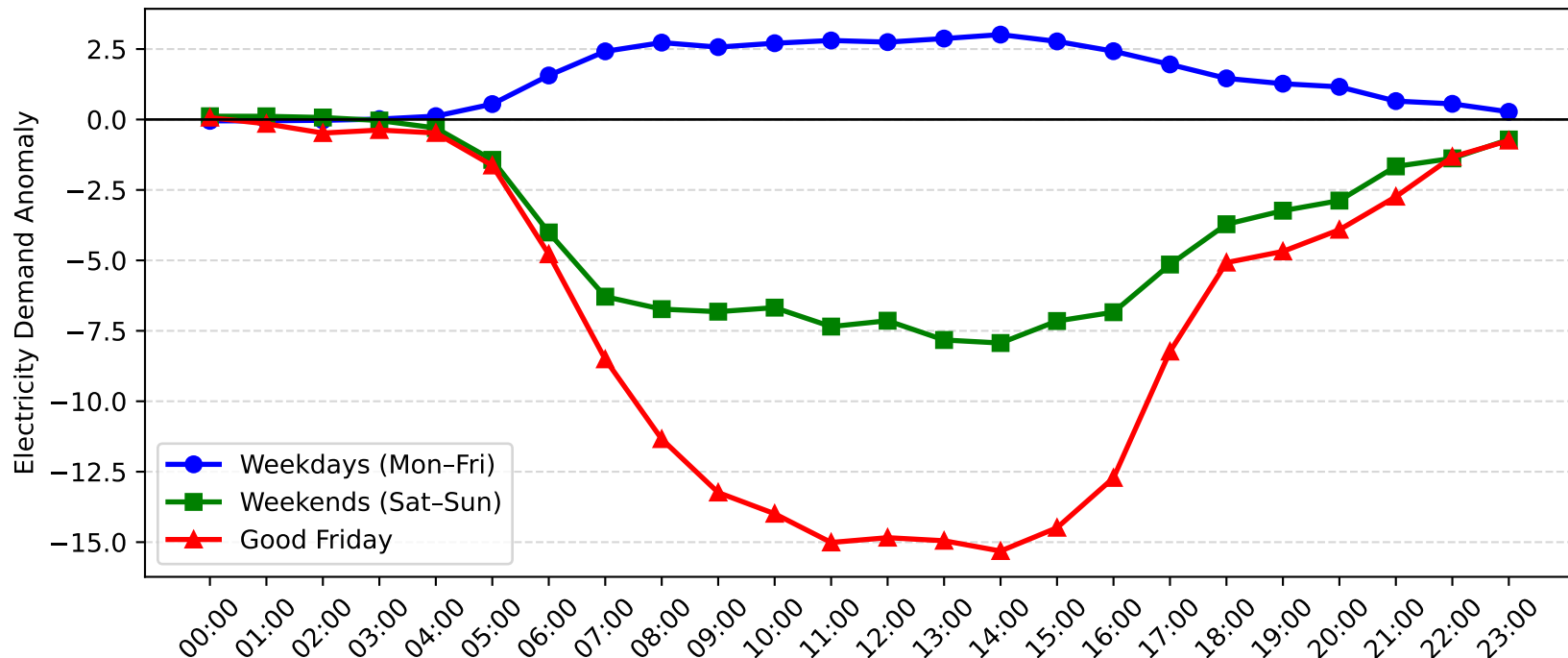
Brookvale Demand Anomaly: Good Friday vs Weekday/Weekend (2006-2007)
