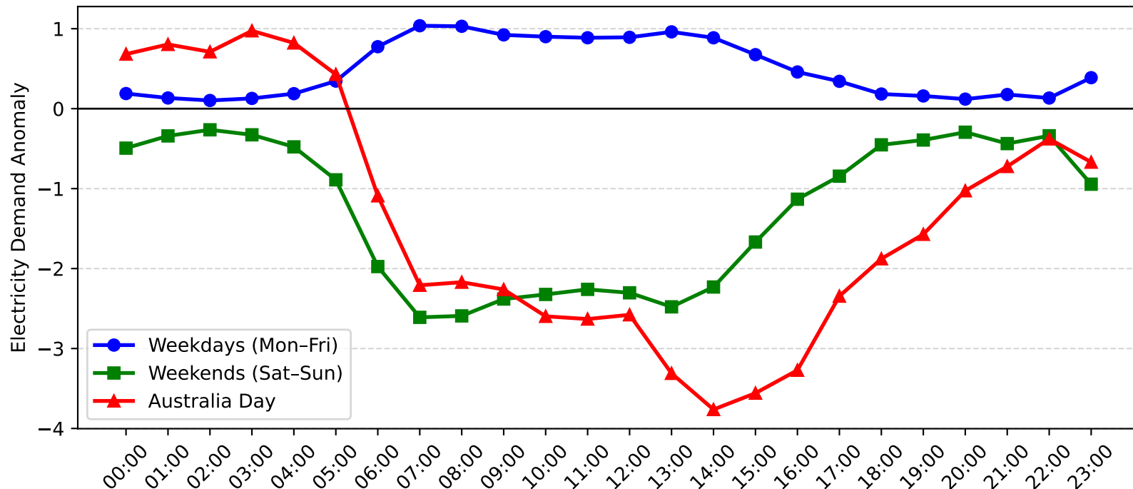
Rutherford Demand Anomaly: Australia Day vs Weekday/Weekend (2015-2016)
