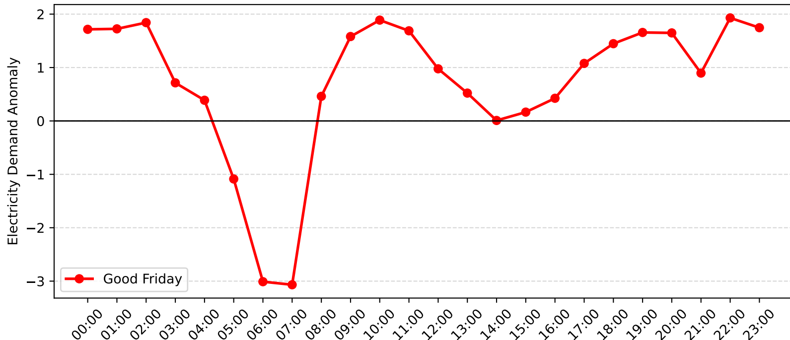
Avoca Demand Anomaly: Good Friday (2004-2005)
