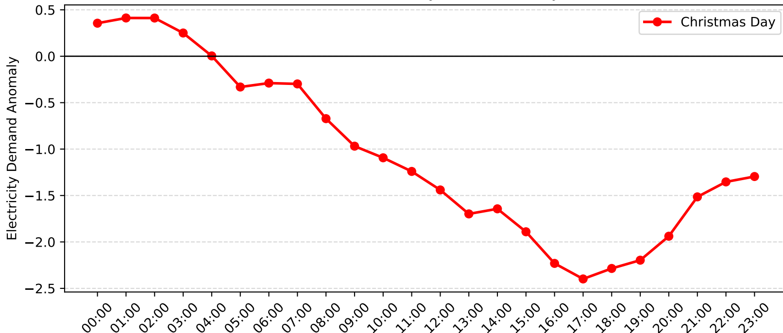
Muswellbrook Demand Anomaly: Christmas Day (2011-2012)
