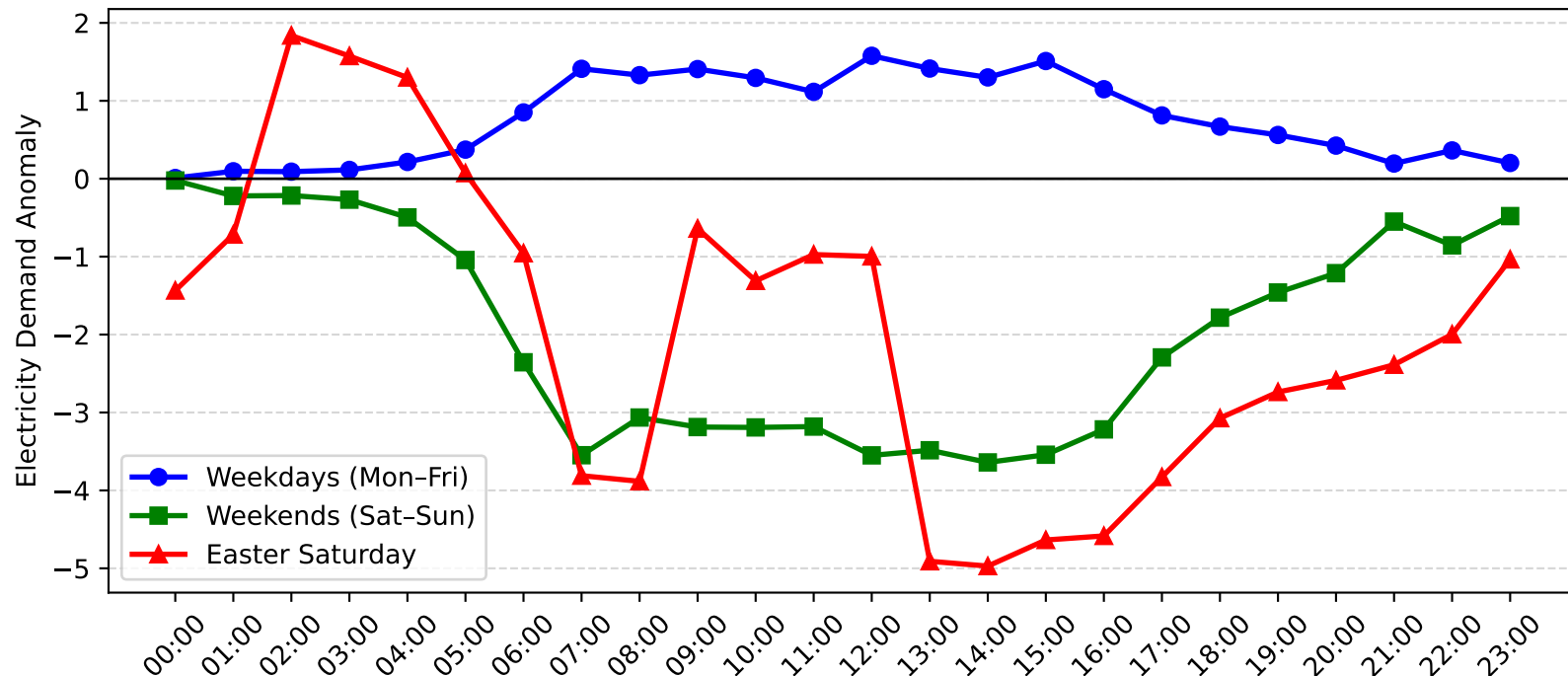
Potts Hill Demand Anomaly: Easter Saturday vs Weekday/Weekend (2014-2015)
