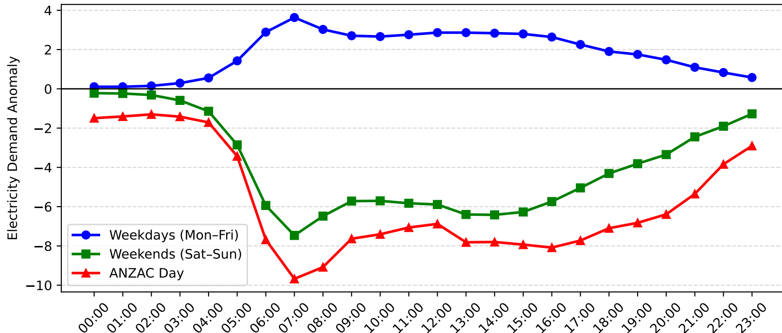
Sefton Demand Anomaly: ANZAC Day vs Weekday/Weekend (2009-2010)
