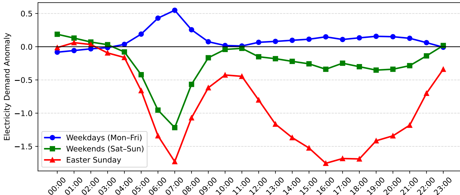
Blakehurst Demand Anomaly: Easter Sunday vs Weekday/Weekend (2016-2017)
