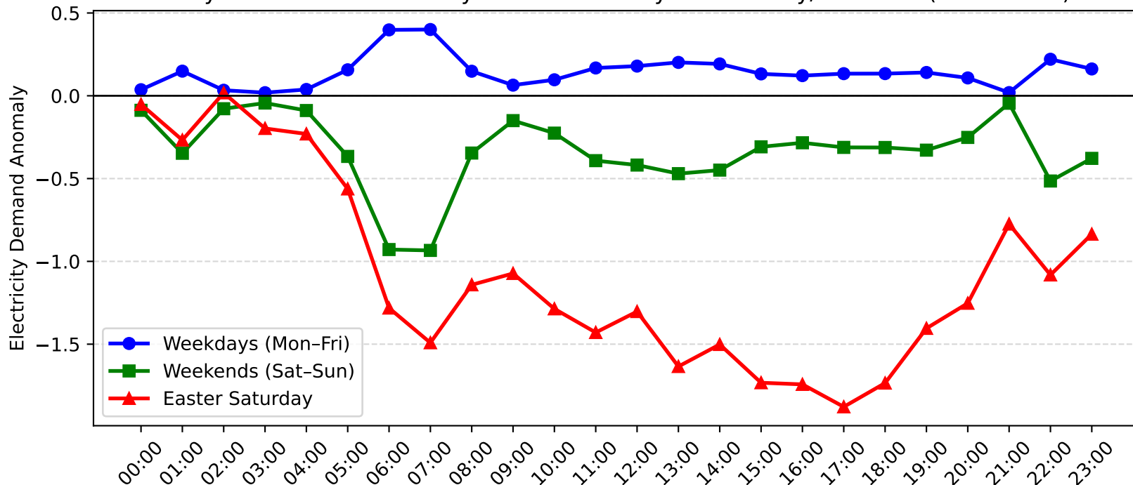
Maryland Demand Anomaly: Easter Saturday vs Weekday/Weekend (2013-2014)
