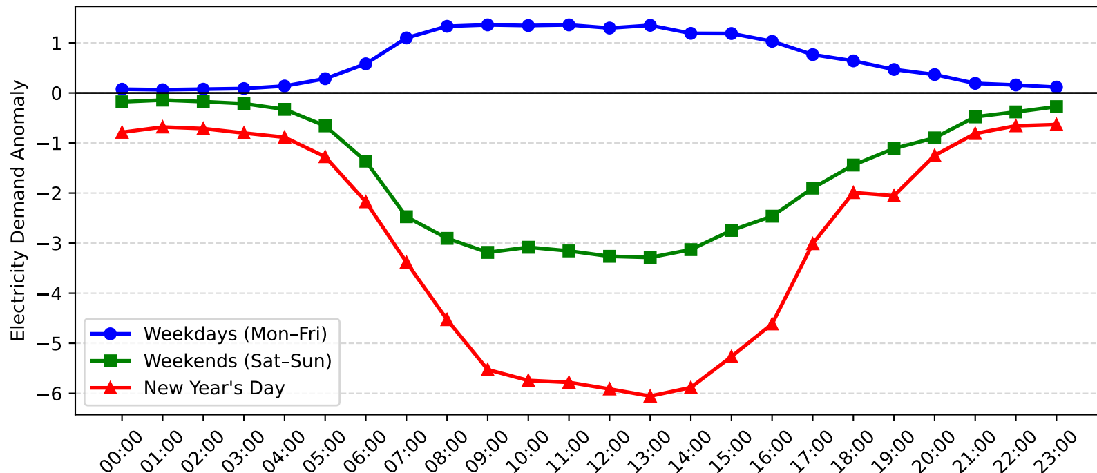
Auburn Demand Anomaly: New Year's Day vs Weekday/Weekend (2006-2007)
