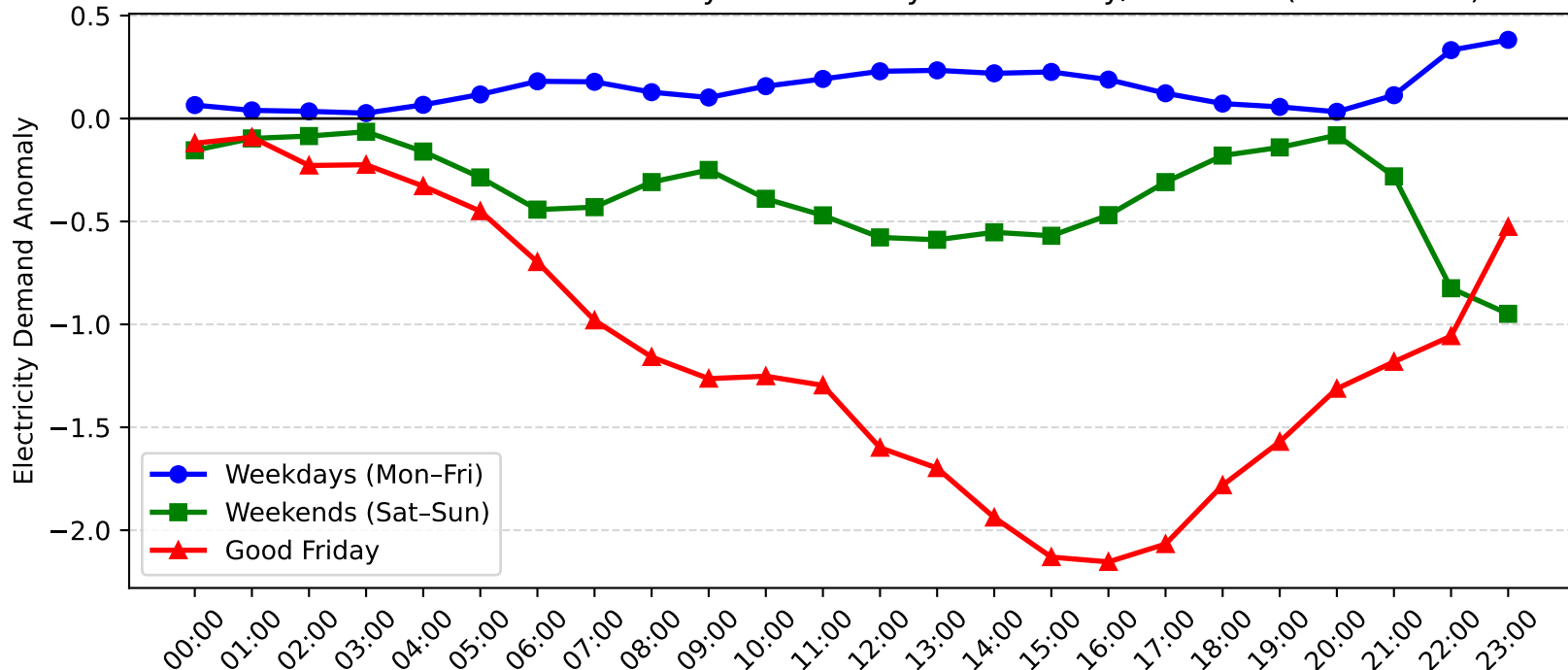
Muswellbrook Demand Anomaly: Good Friday vs Weekday/Weekend (2016-2017)
