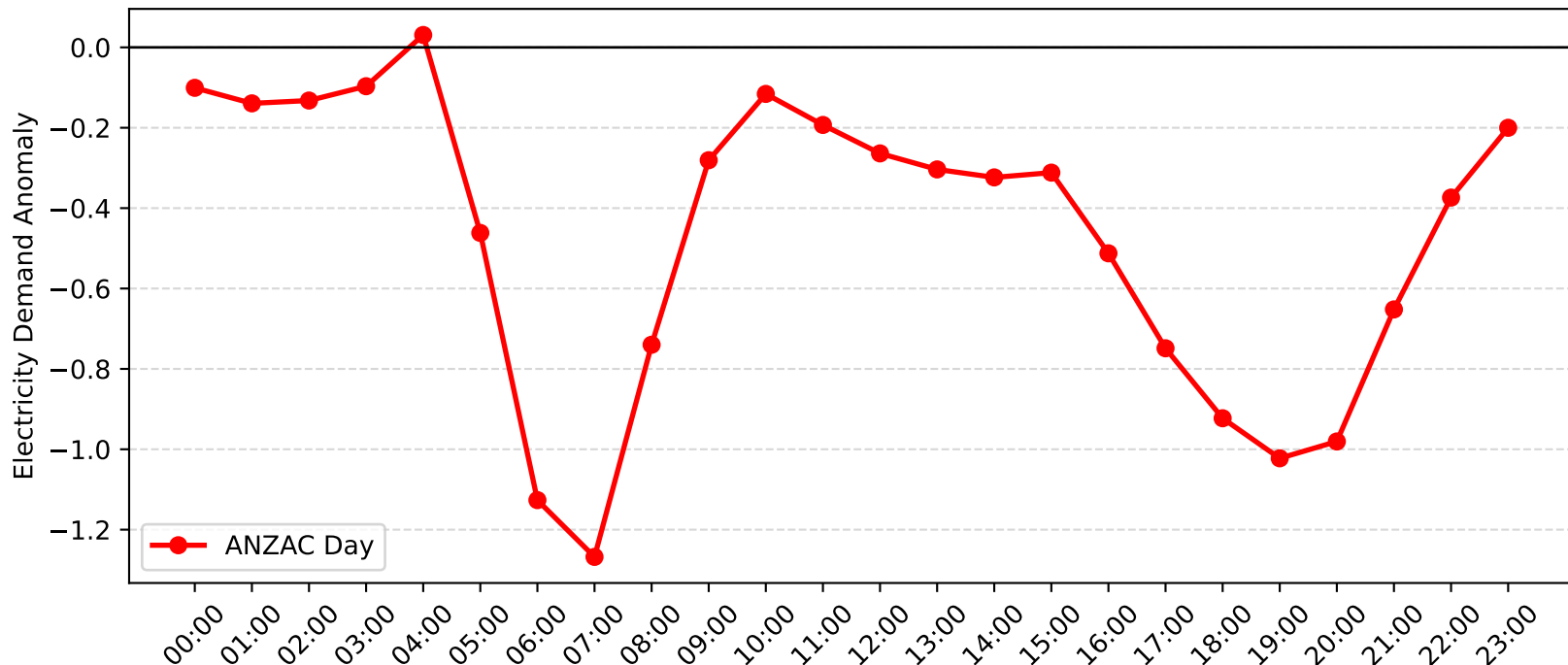
Narrabeen Demand Anomaly: ANZAC Day (2014-2015)
