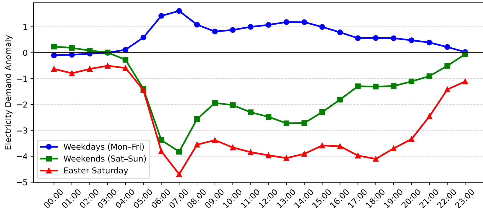
Kirrawee Demand Anomaly: Easter Saturday vs Weekday/Weekend (2012-2013)
