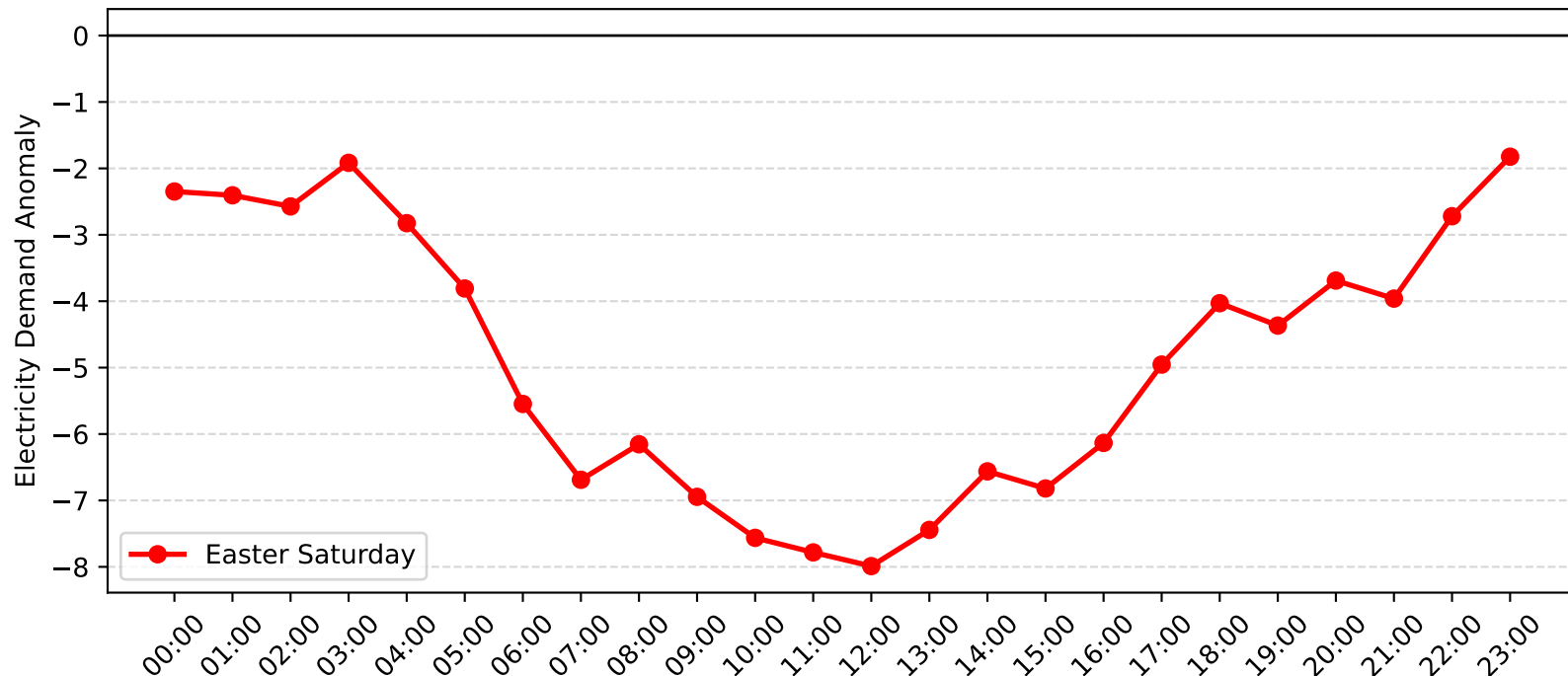
Potts Hill Demand Anomaly: Easter Saturday (2017-2018)
