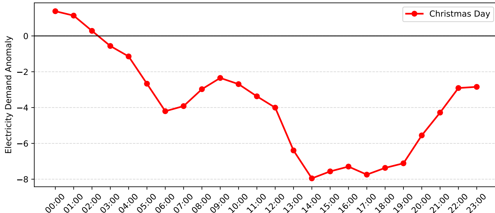
Pennant Hills Demand Anomaly: Christmas Day (2005-2006)
