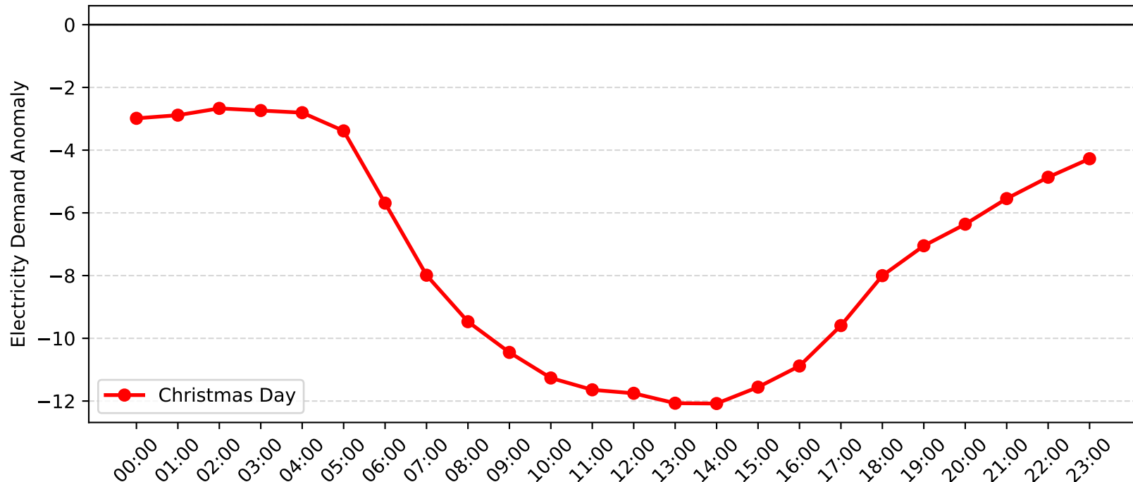
Macquarie Park Demand Anomaly: Christmas Day (2006-2007)
