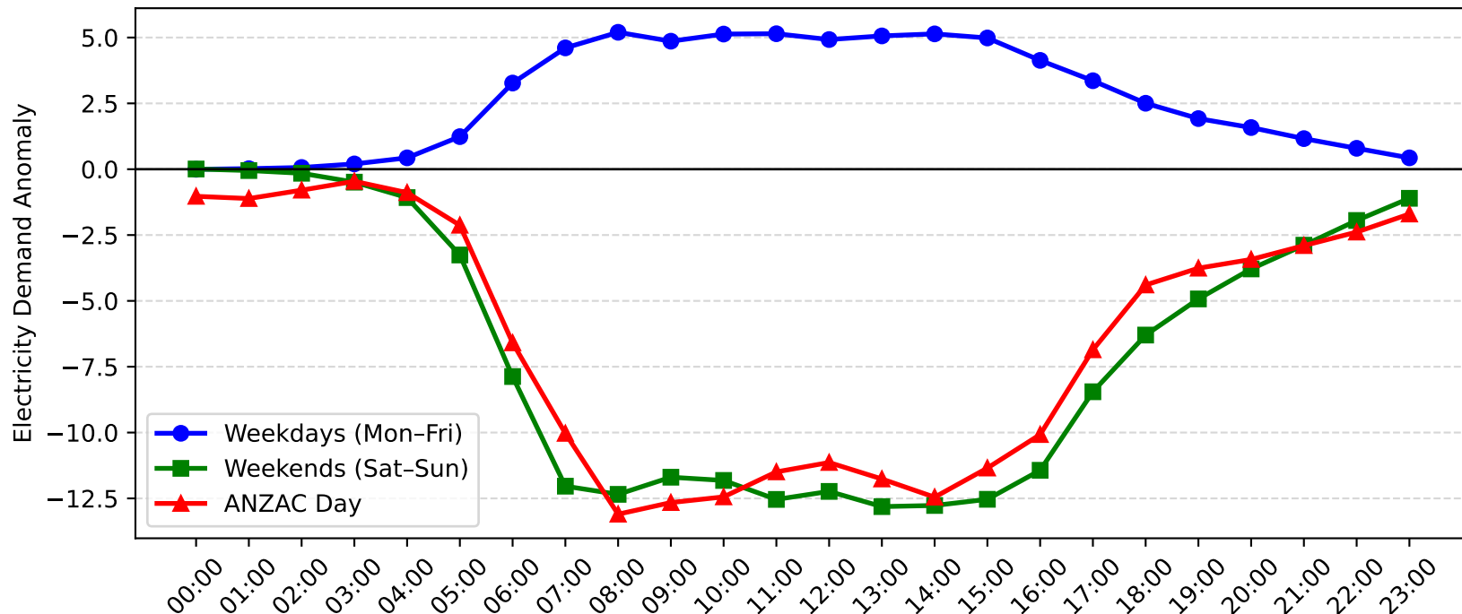
Zetland Demand Anomaly: ANZAC Day vs Weekday/Weekend (2005-2006)
