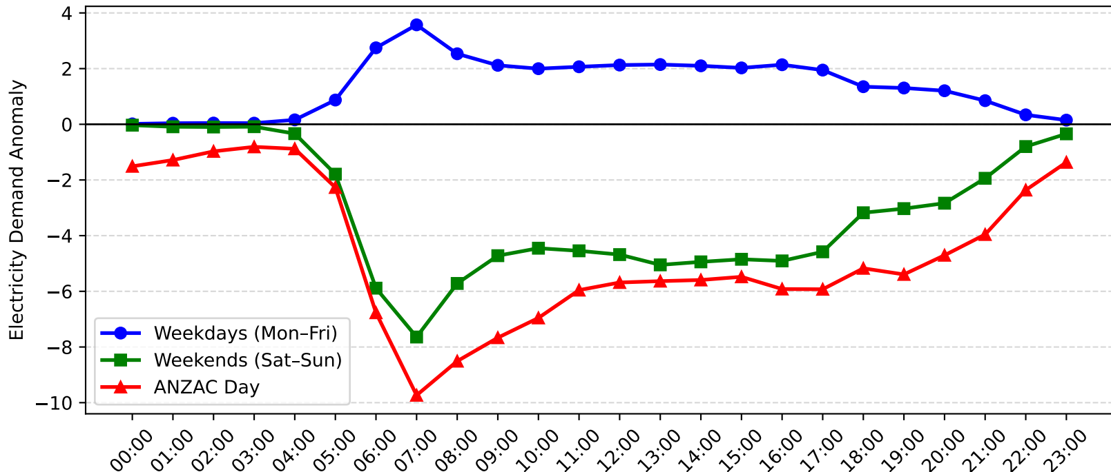
Epping Demand Anomaly: ANZAC Day vs Weekday/Weekend (2010-2011)
