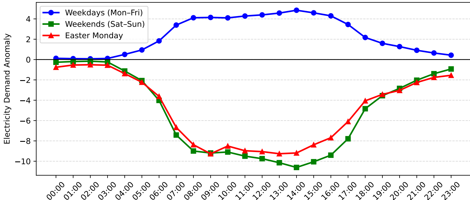
Gore Hill Demand Anomaly: Easter Monday vs Weekday/Weekend (2016-2017)
