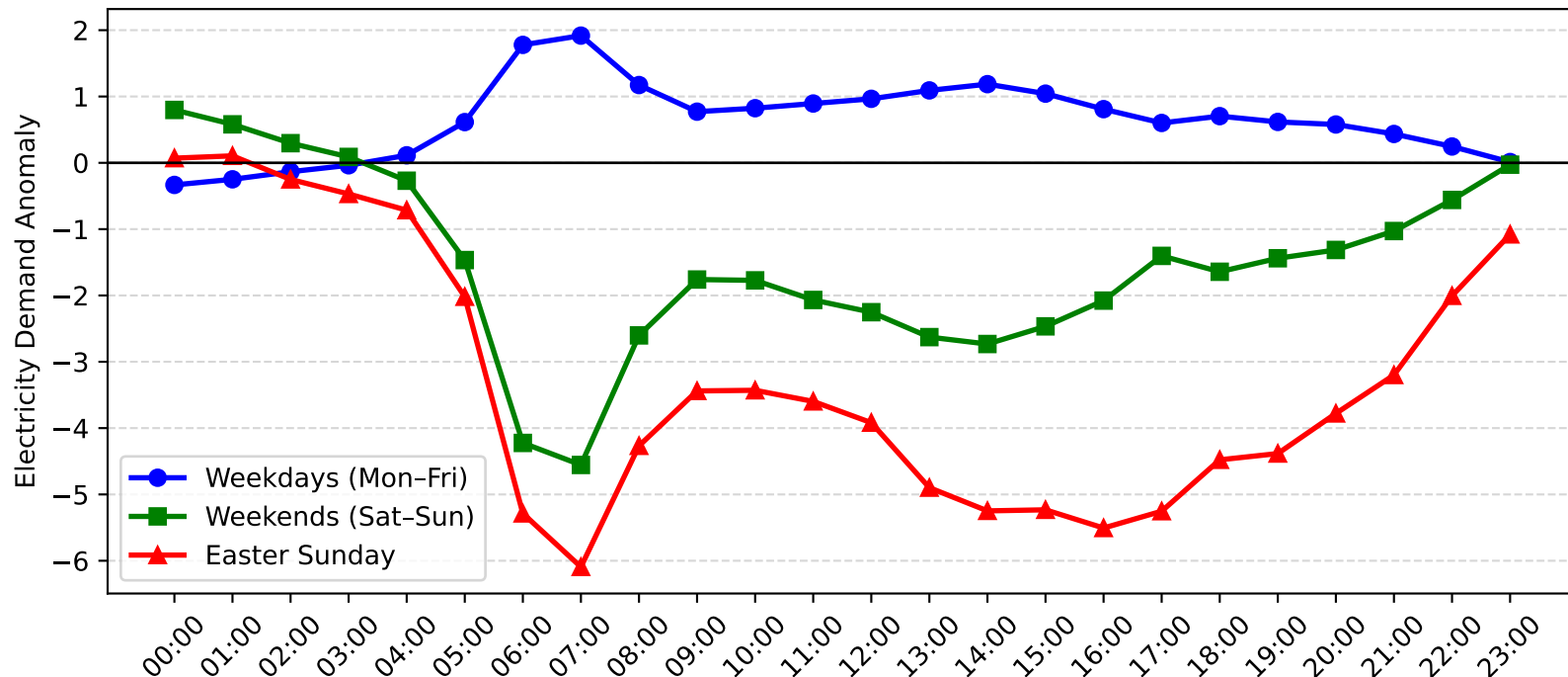
Mortdale Demand Anomaly: Easter Sunday vs Weekday/Weekend (2006-2007)
