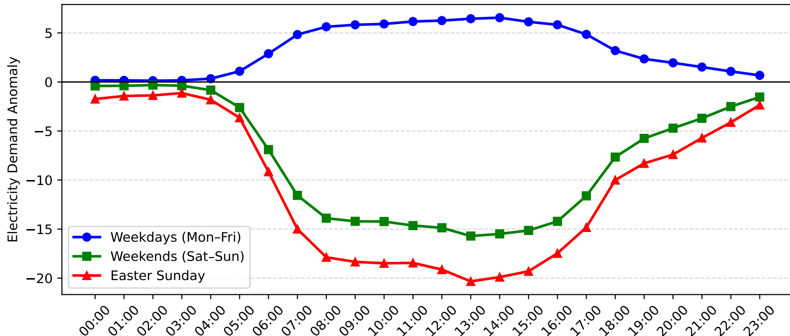
Gore Hill Demand Anomaly: Easter Sunday vs Weekday/Weekend (2007-2008)
