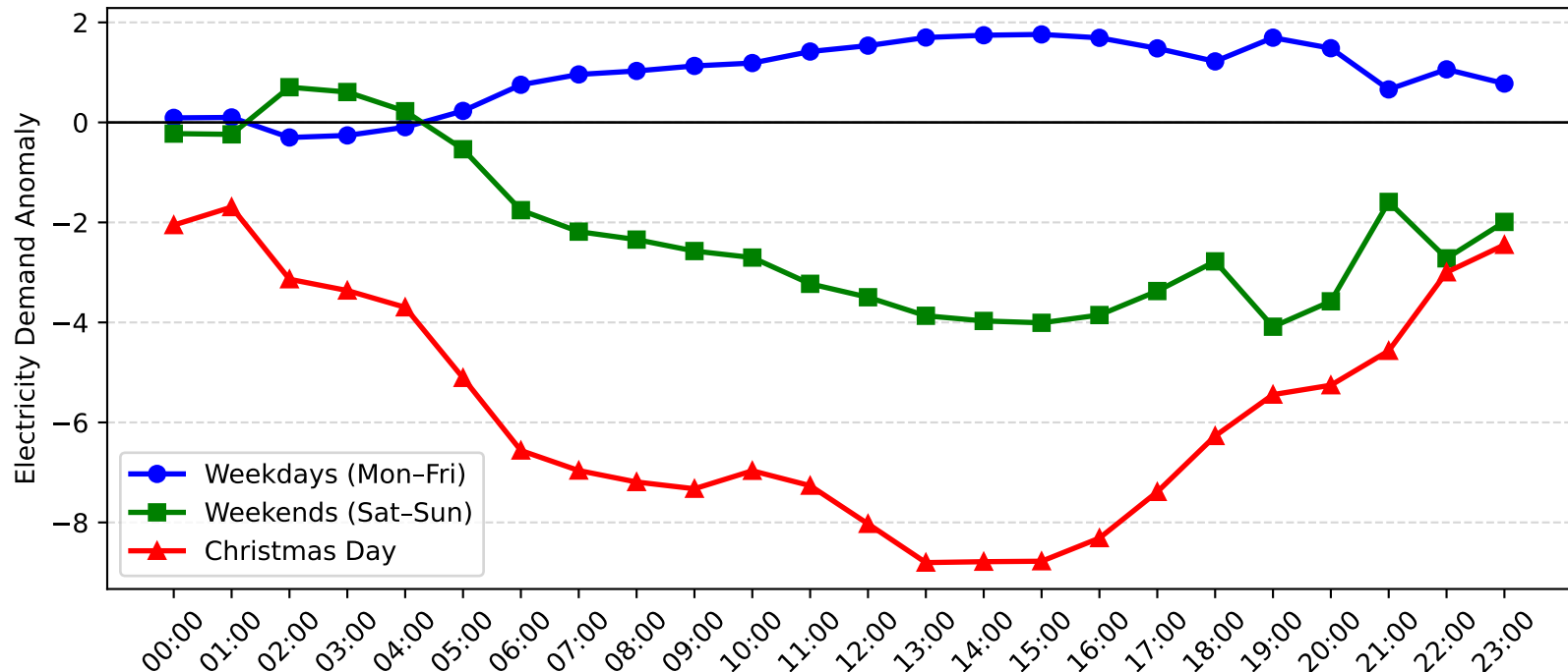
Sefton Demand Anomaly: Christmas Day vs Weekday/Weekend (2016-2017)
