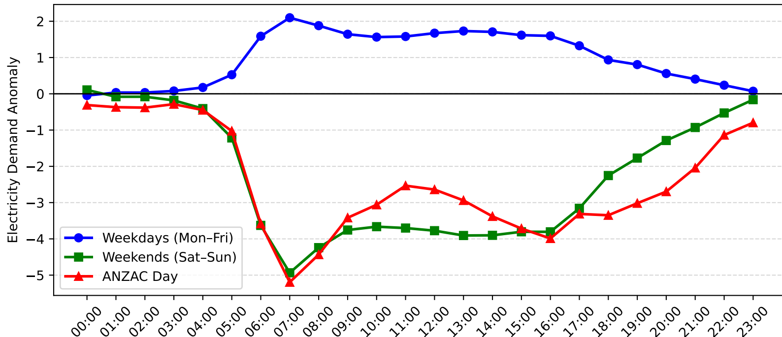
Pymble Demand Anomaly: ANZAC Day vs Weekday/Weekend (2008-2009)
