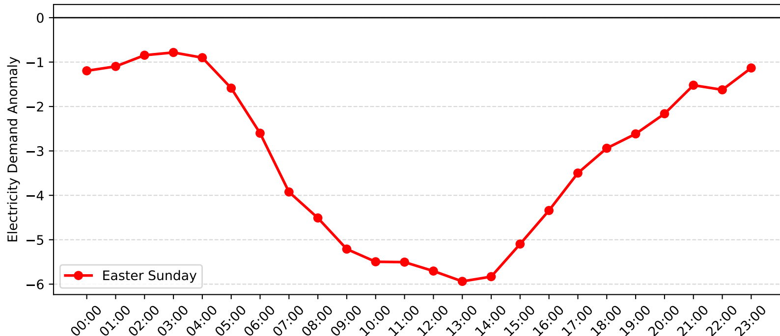
Broadmeadow Demand Anomaly: Easter Sunday (2016-2017)
