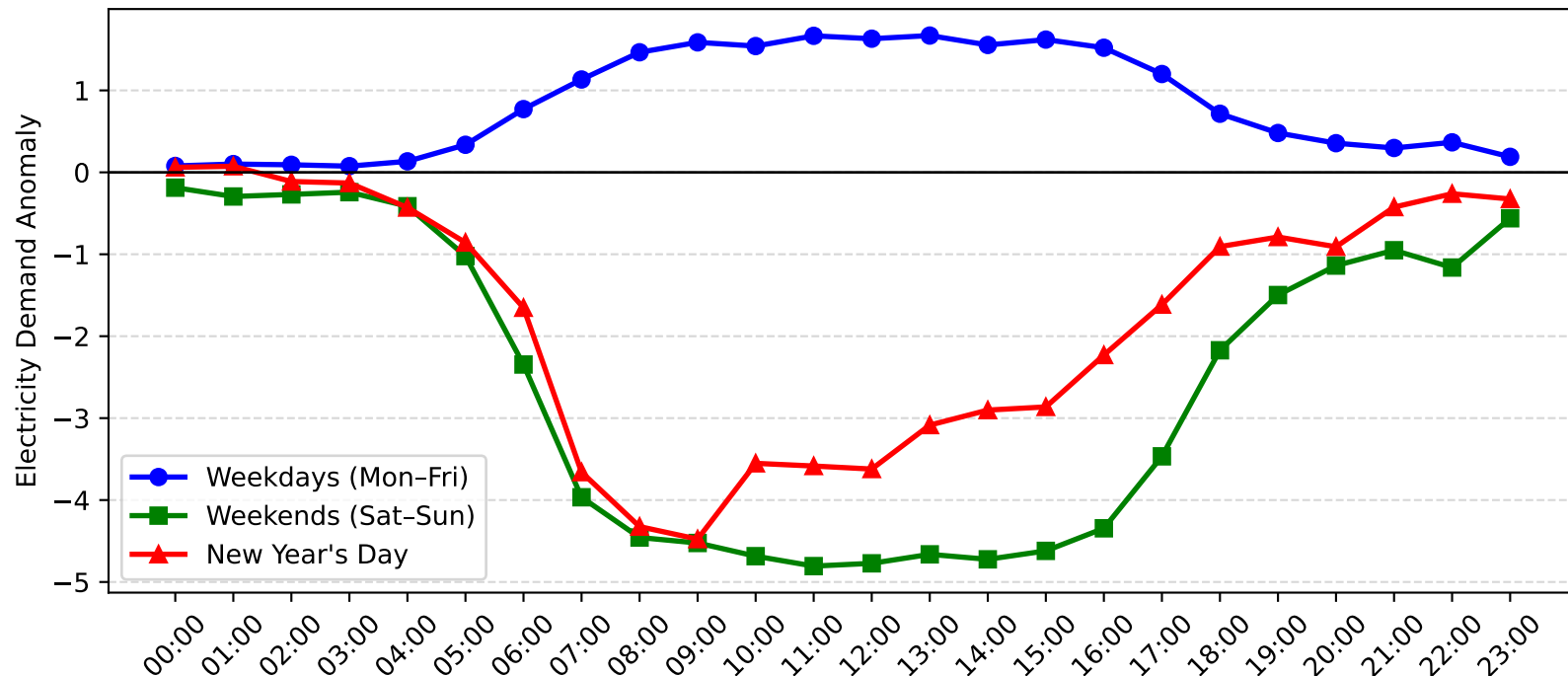
Beacon Hill Demand Anomaly: New Year's Day vs Weekday/Weekend (2009-2010)
