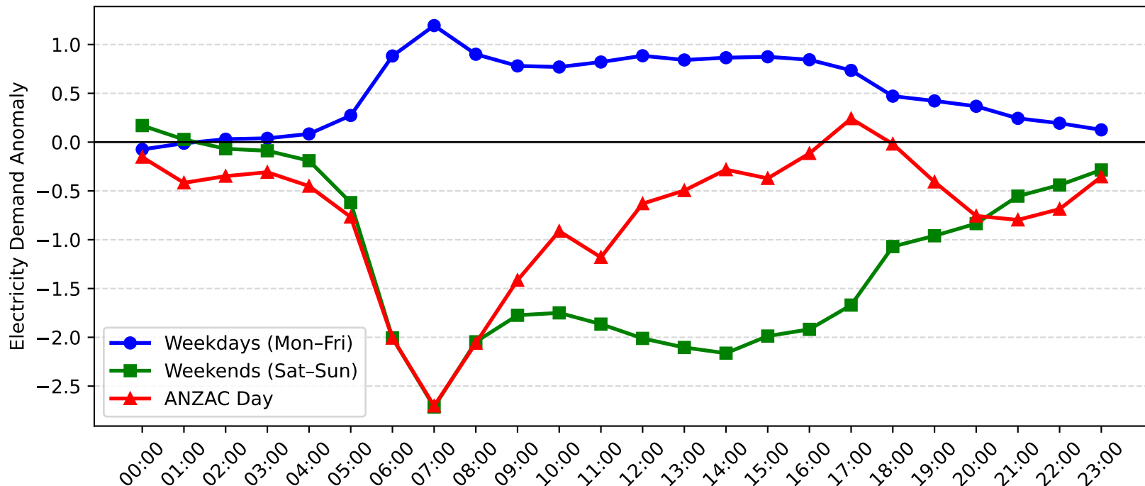
Pymble Demand Anomaly: ANZAC Day vs Weekday/Weekend (2017-2018)
