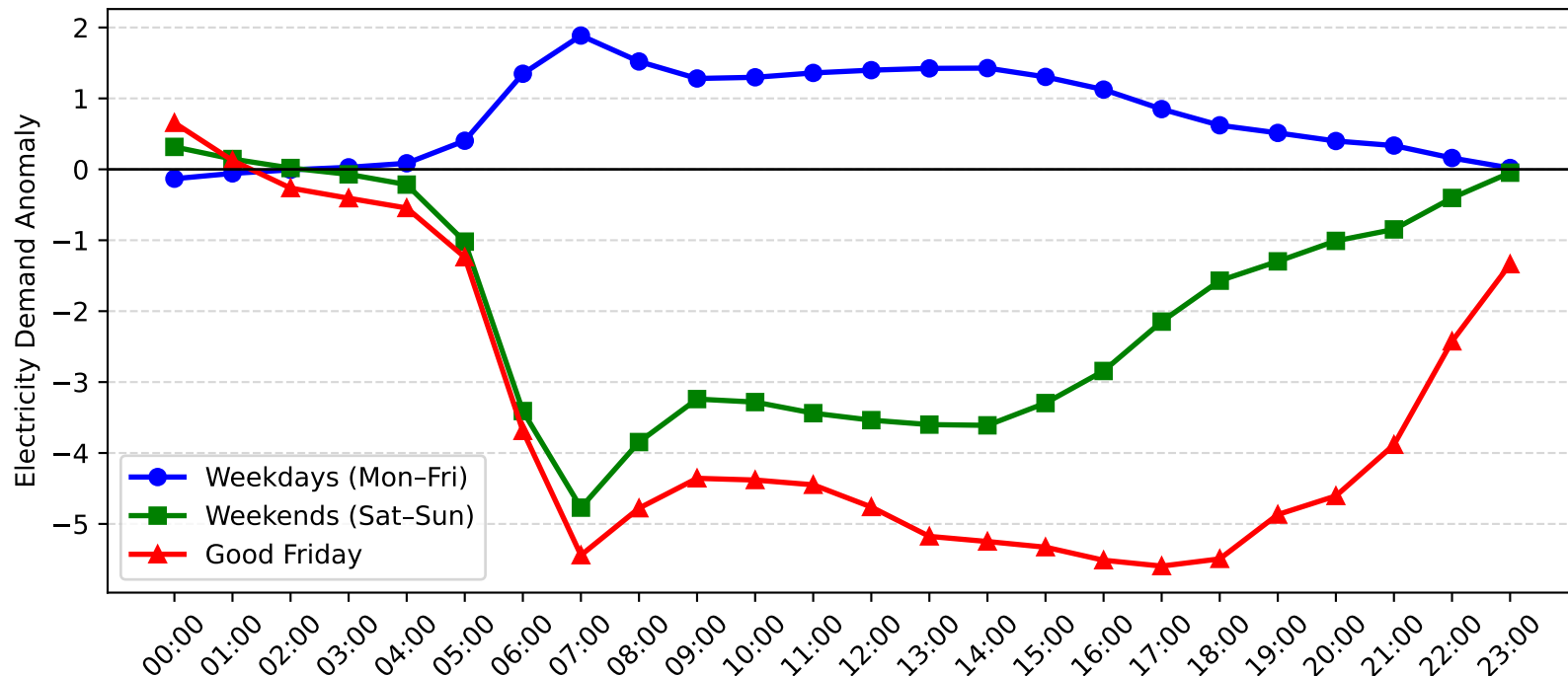
Hunters Hill Demand Anomaly: Good Friday vs Weekday/Weekend (2013-2014)
