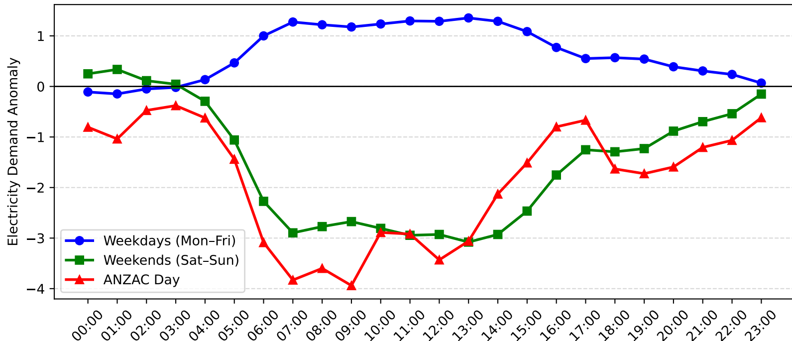
Wyong Demand Anomaly: ANZAC Day vs Weekday/Weekend (2017-2018)
