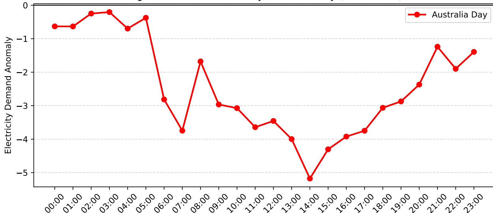
Argenton Demand Anomaly: Australia Day (2013-2014)
