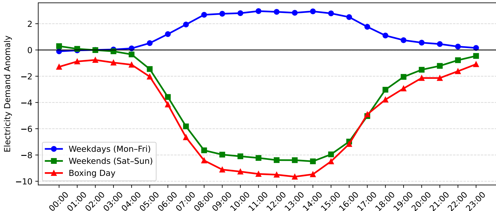
Mascot Demand Anomaly: Boxing Day vs Weekday/Weekend (2013-2014)
