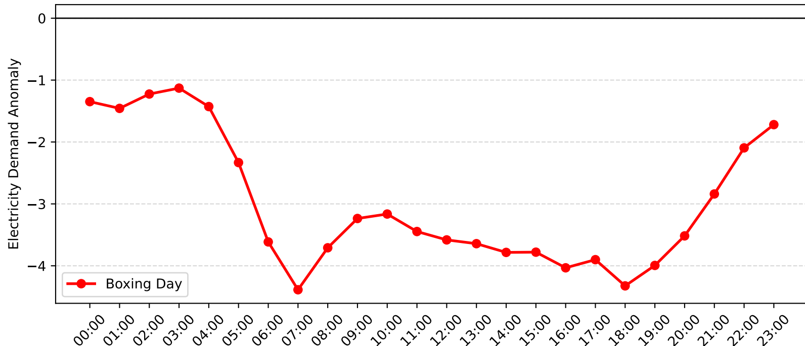
Dee Why West Demand Anomaly: Boxing Day (2016-2017)
