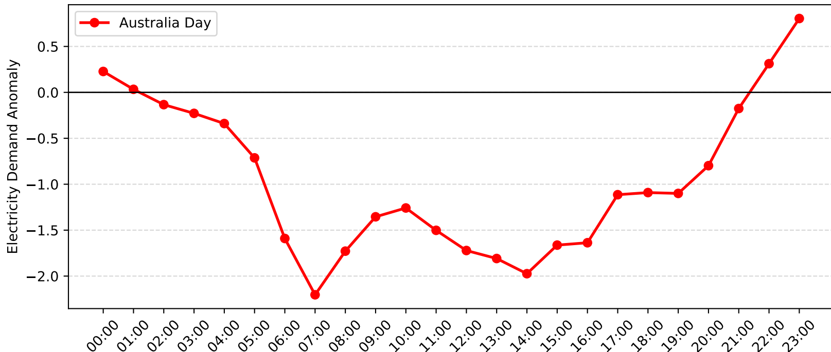
Rockdale Demand Anomaly: Australia Day (2007-2008)
