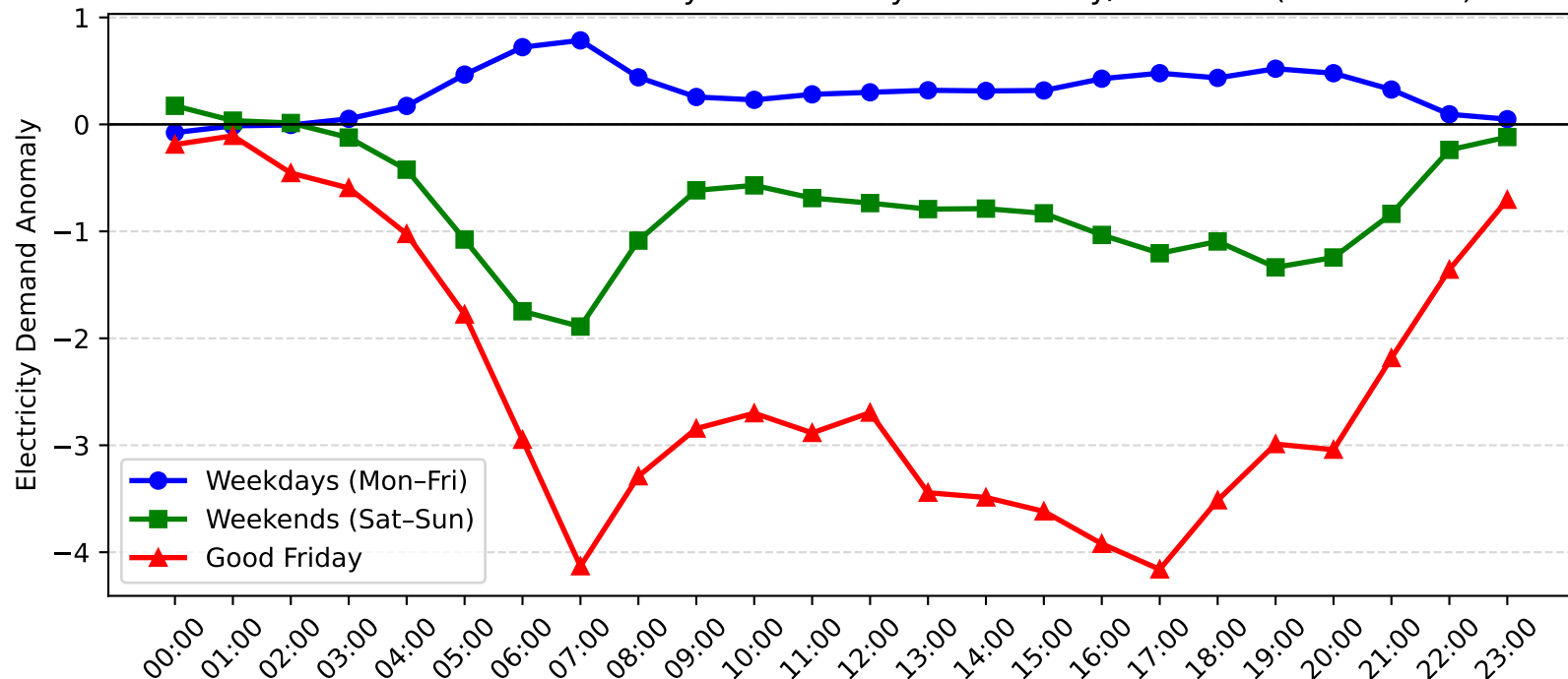
Charmhaven Demand Anomaly: Good Friday vs Weekday/Weekend (2010-2011)
