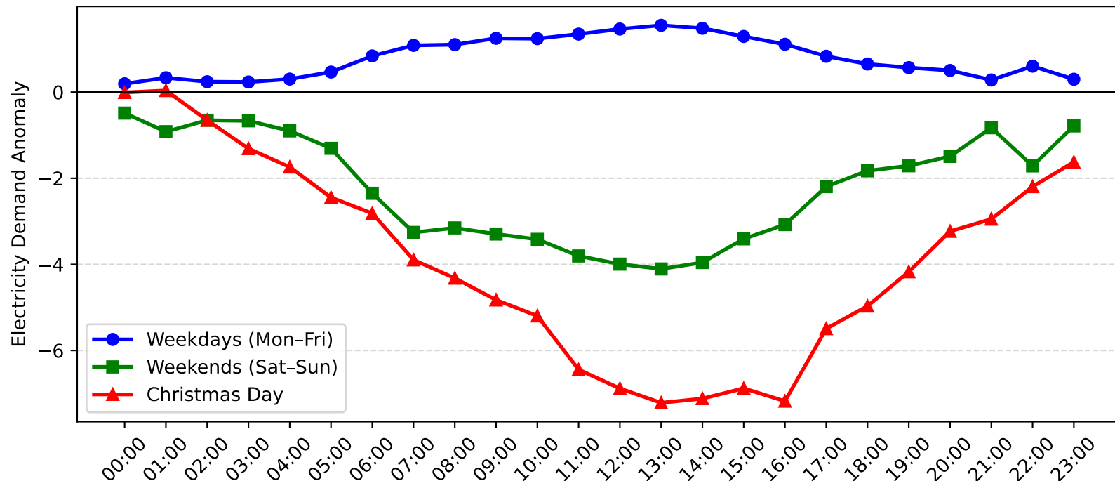
Cardiff Demand Anomaly: Christmas Day vs Weekday/Weekend (2007-2008)
