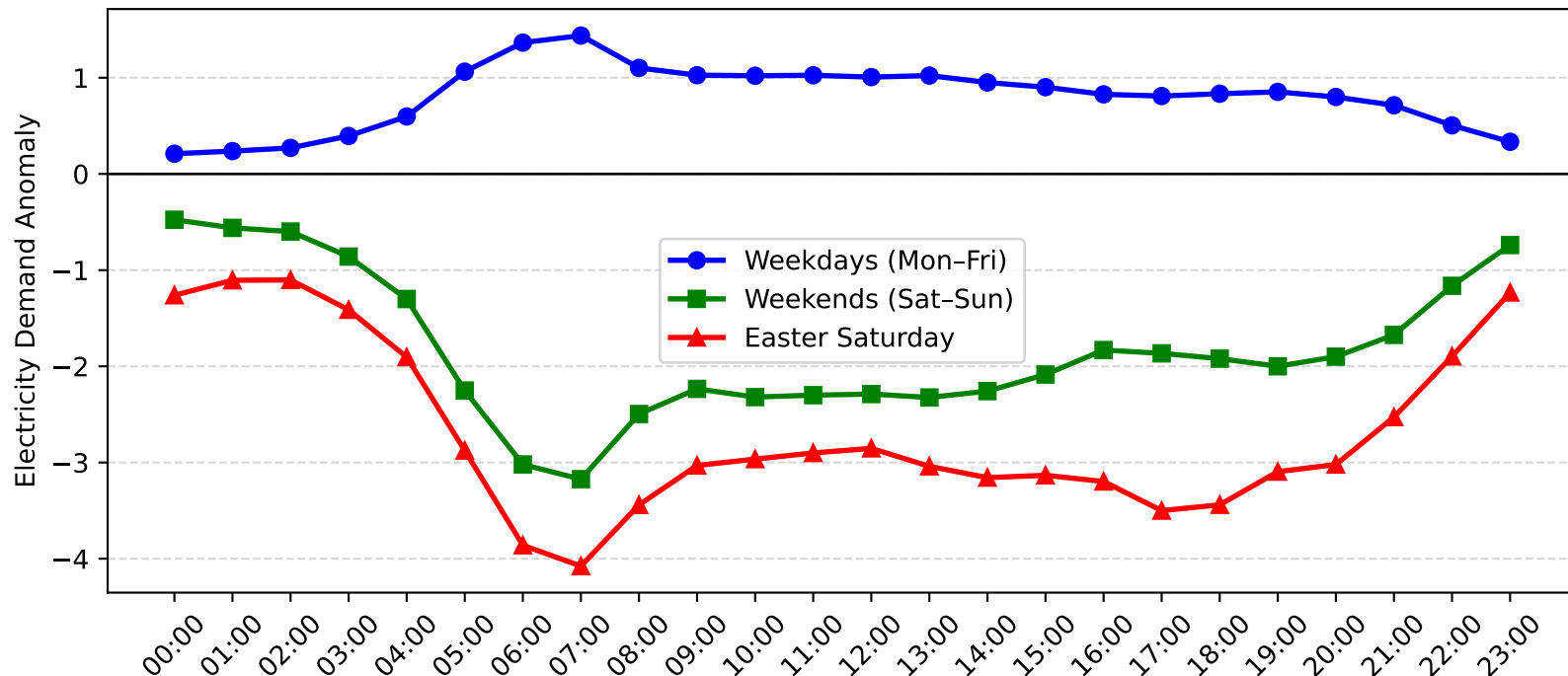
Lisarow Demand Anomaly: Easter Saturday vs Weekday/Weekend (2010-2011)
