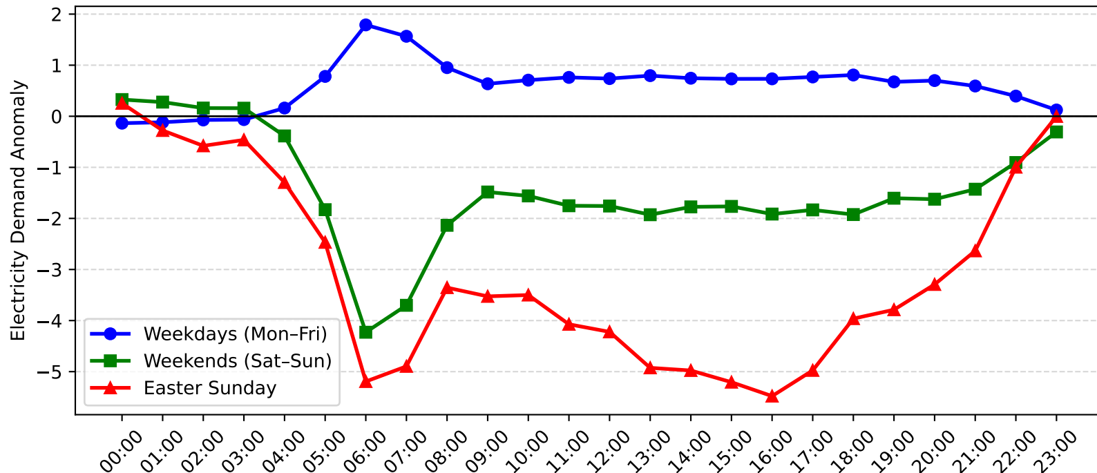
Revesby Demand Anomaly: Easter Sunday vs Weekday/Weekend (2005-2006)
