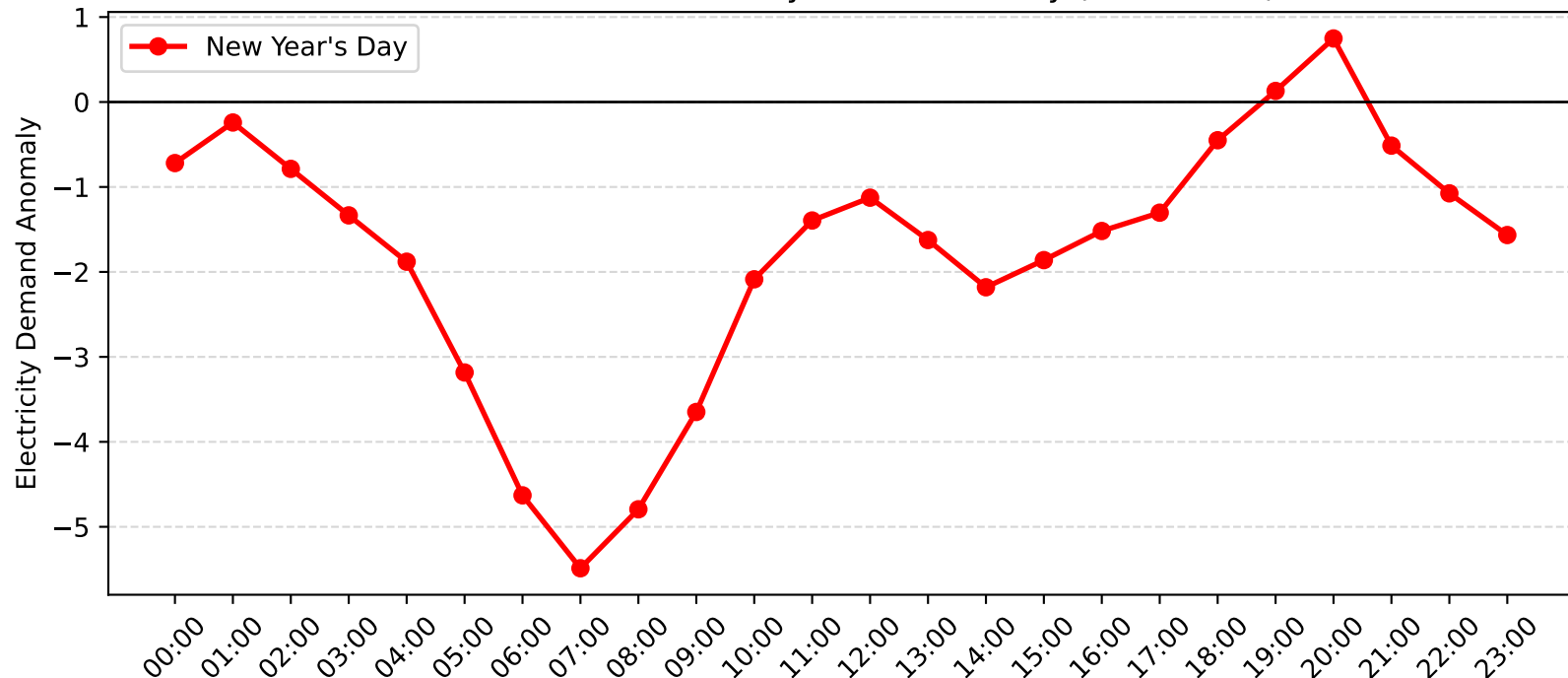
Enfield Demand Anomaly: New Year's Day (2006-2007)
