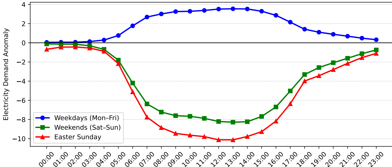
Mascot Demand Anomaly: Easter Sunday vs Weekday/Weekend (2011-2012)
