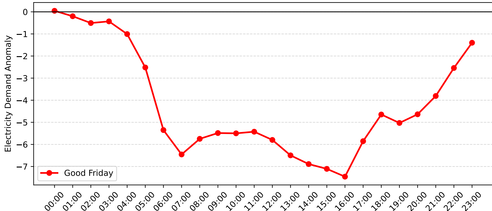
Campsie Demand Anomaly: Good Friday (2006-2007)
