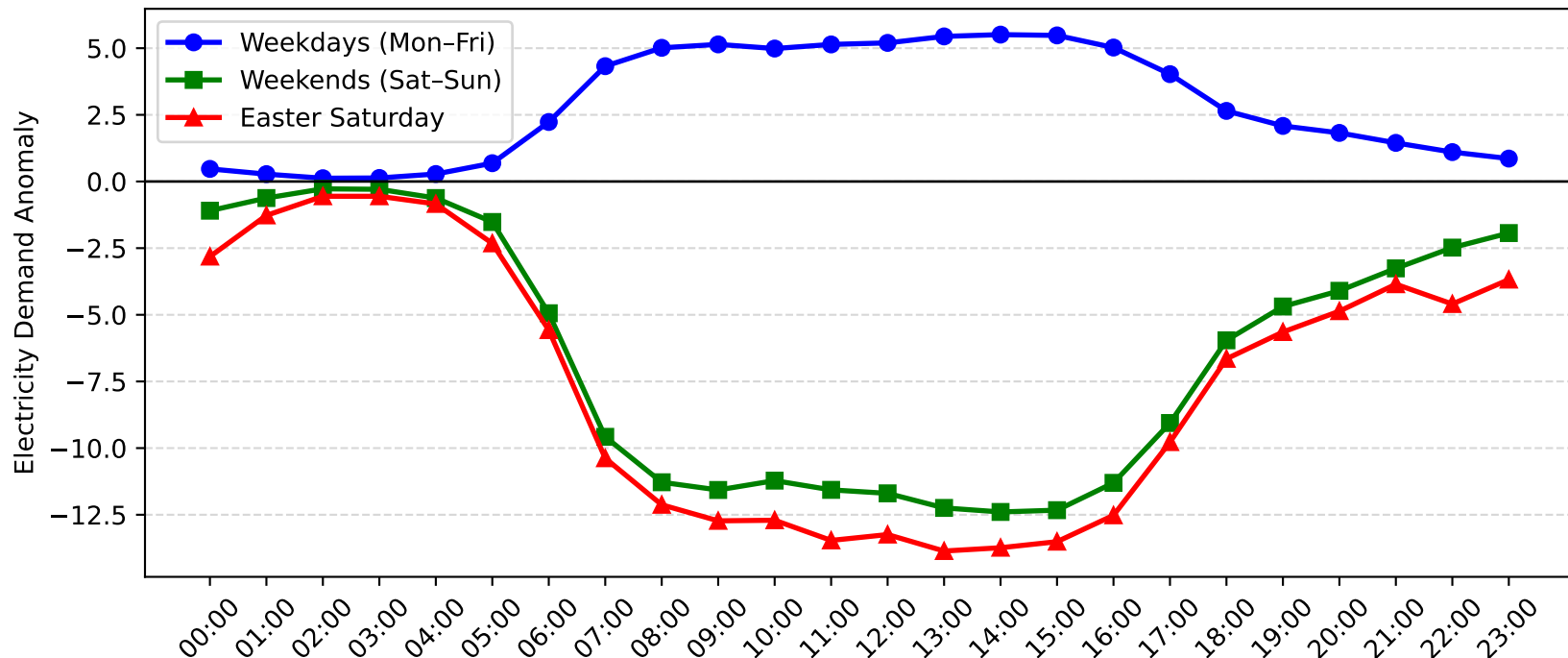
Gore Hill Demand Anomaly: Easter Saturday vs Weekday/Weekend (2011-2012)
