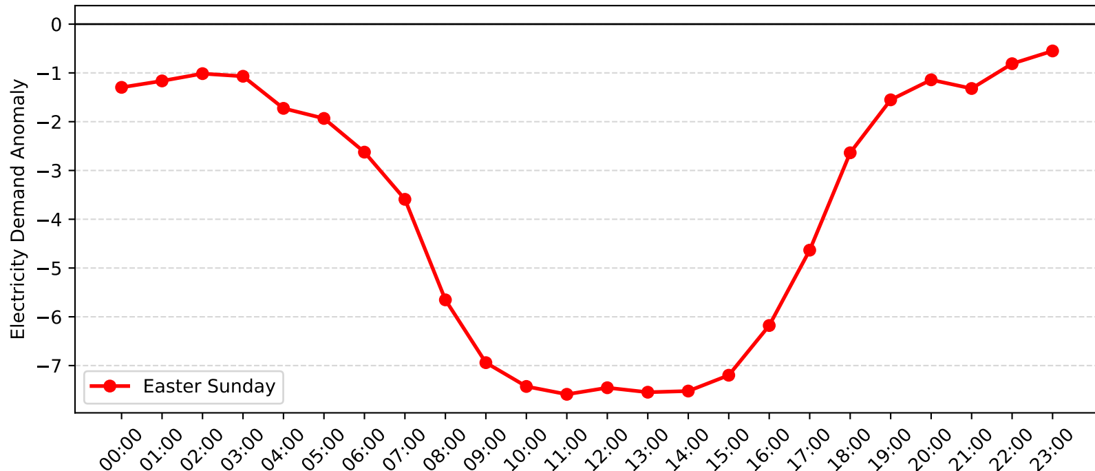
Green Square Demand Anomaly: Easter Sunday (2012-2013)
