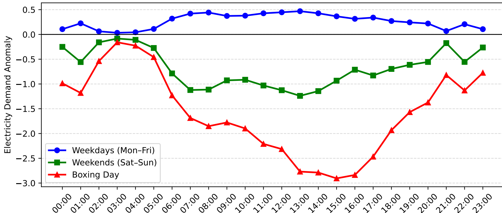
Gateshead Demand Anomaly: Boxing Day vs Weekday/Weekend (2009-2010)
