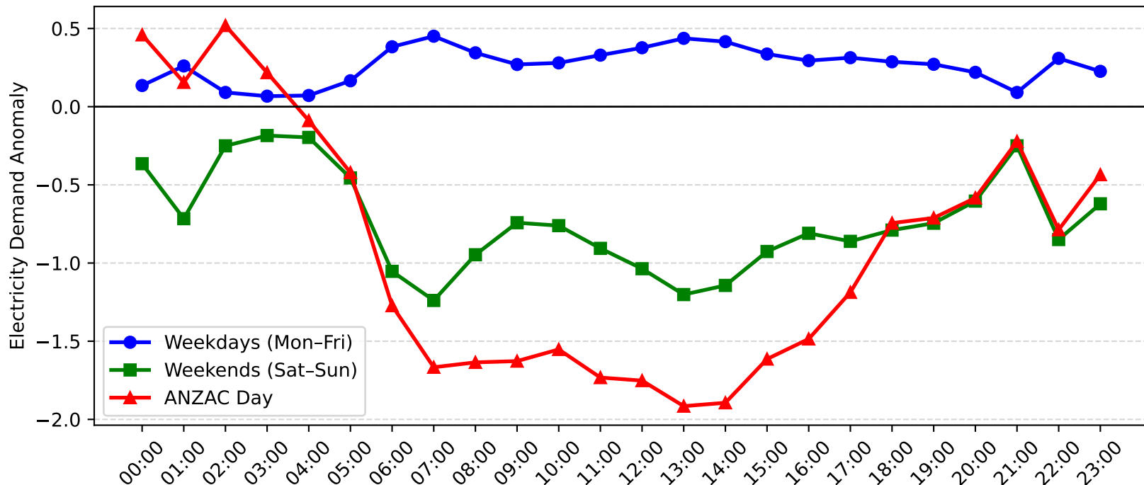
Gateshead Demand Anomaly: ANZAC Day vs Weekday/Weekend (2012-2013)
