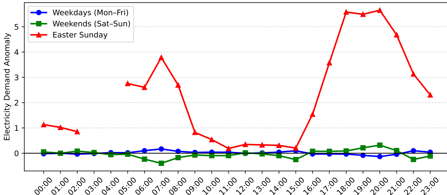
Harbord Demand Anomaly: Easter Sunday vs Weekday/Weekend (2004-2005)
