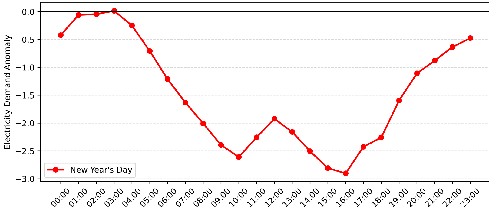
Lidcombe Demand Anomaly: New Year's Day (2017-2018)
