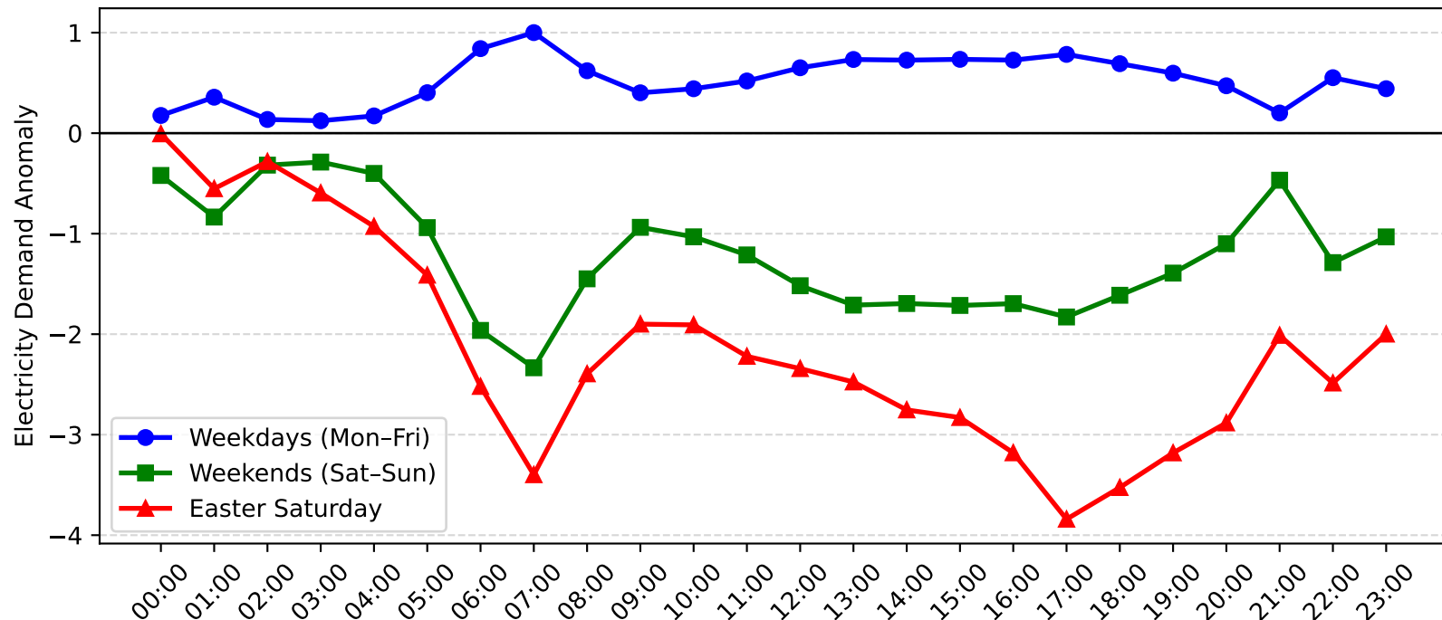
Jesmond Demand Anomaly: Easter Saturday vs Weekday/Weekend (2014-2015)
