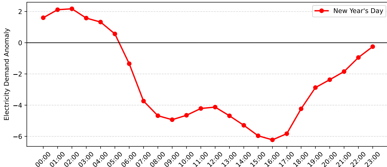
Concord Demand Anomaly: New Year's Day (2017-2018)
