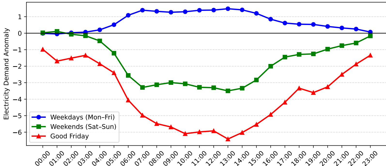
Wyong Demand Anomaly: Good Friday vs Weekday/Weekend (2017-2018)
