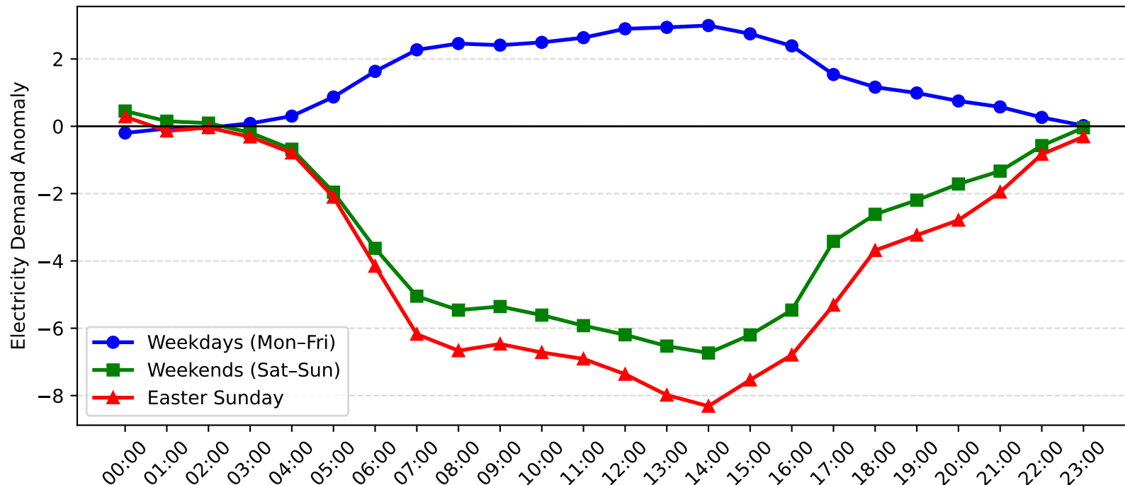
West Gosford Demand Anomaly: Easter Sunday vs Weekday/Weekend (2008-2009)
