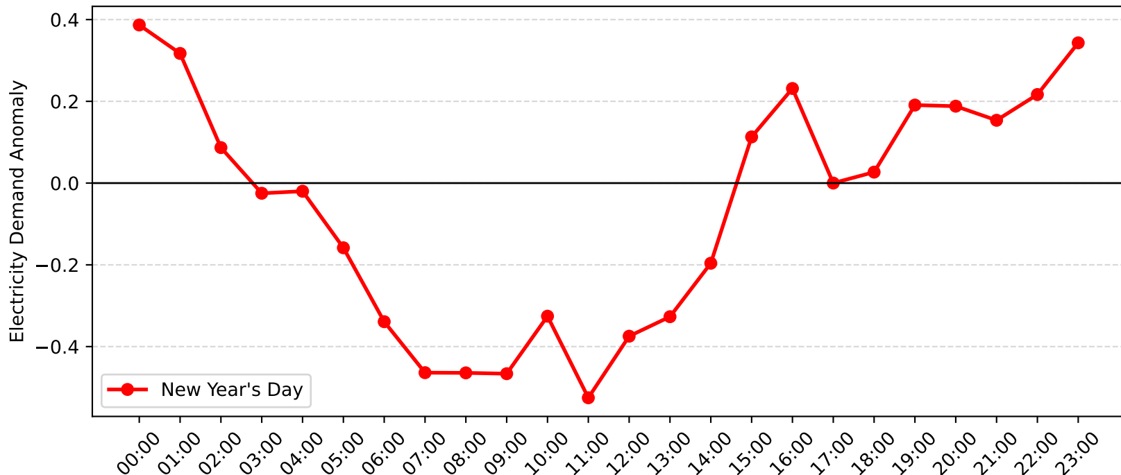
Rothbury Demand Anomaly: New Year's Day (2014-2015)
