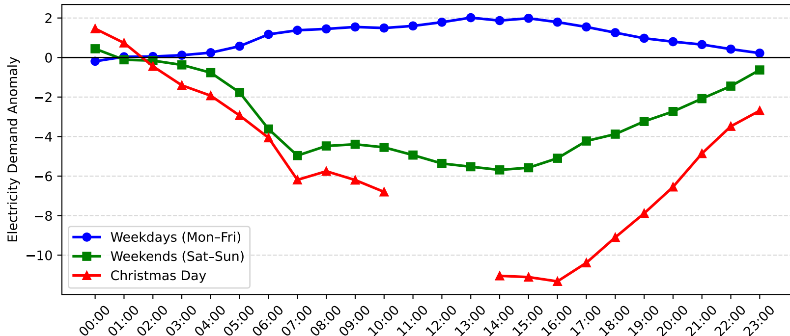
Campsie Demand Anomaly: Christmas Day vs Weekday/Weekend (2008-2009)
