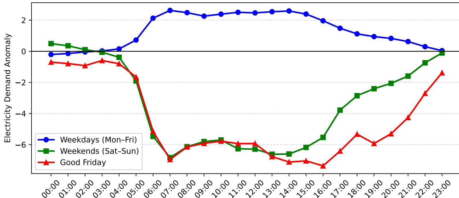
Hunters Hill Demand Anomaly: Good Friday vs Weekday/Weekend (2006-2007)
