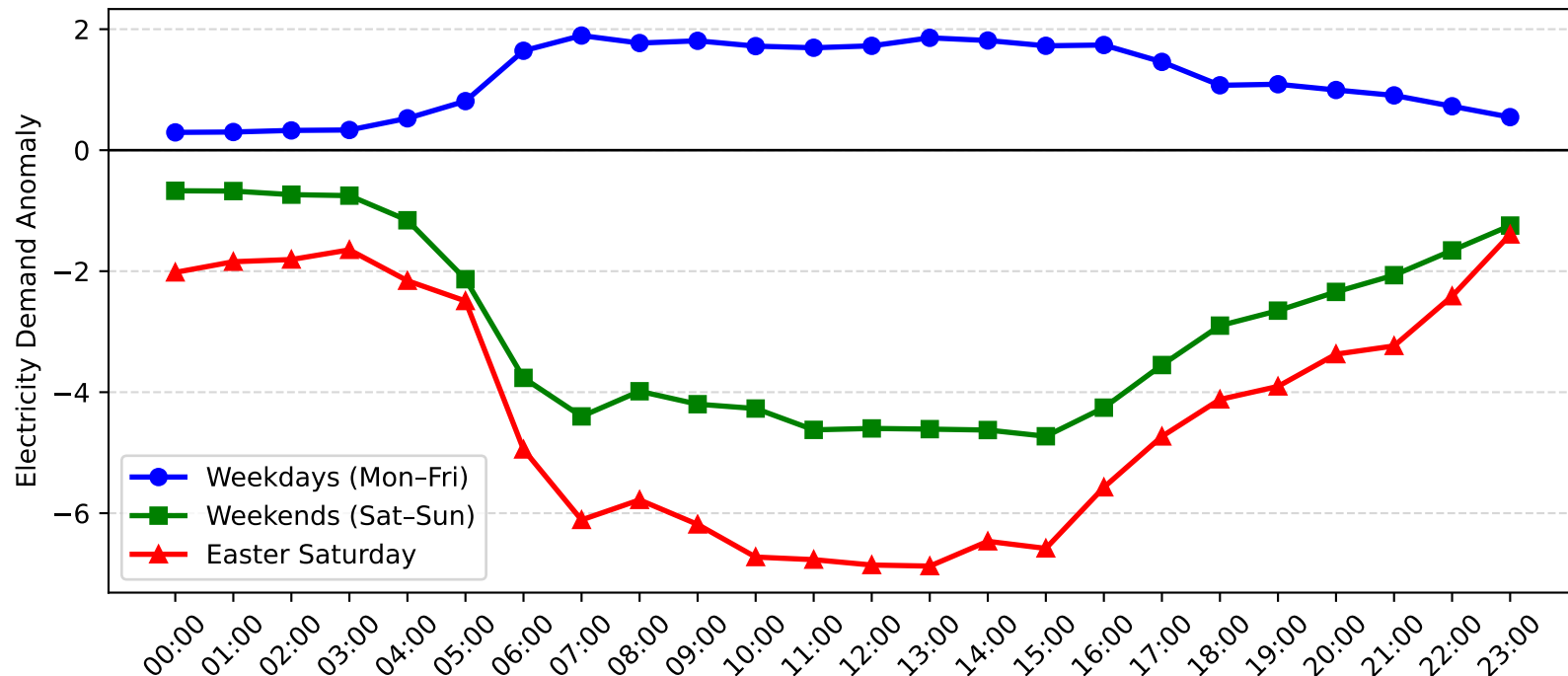
Potts Hill Demand Anomaly: Easter Saturday vs Weekday/Weekend (2016-2017)
