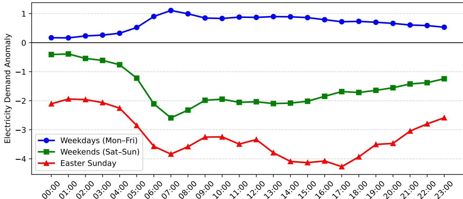
Bass Hill Demand Anomaly: Easter Sunday vs Weekday/Weekend (2013-2014)
