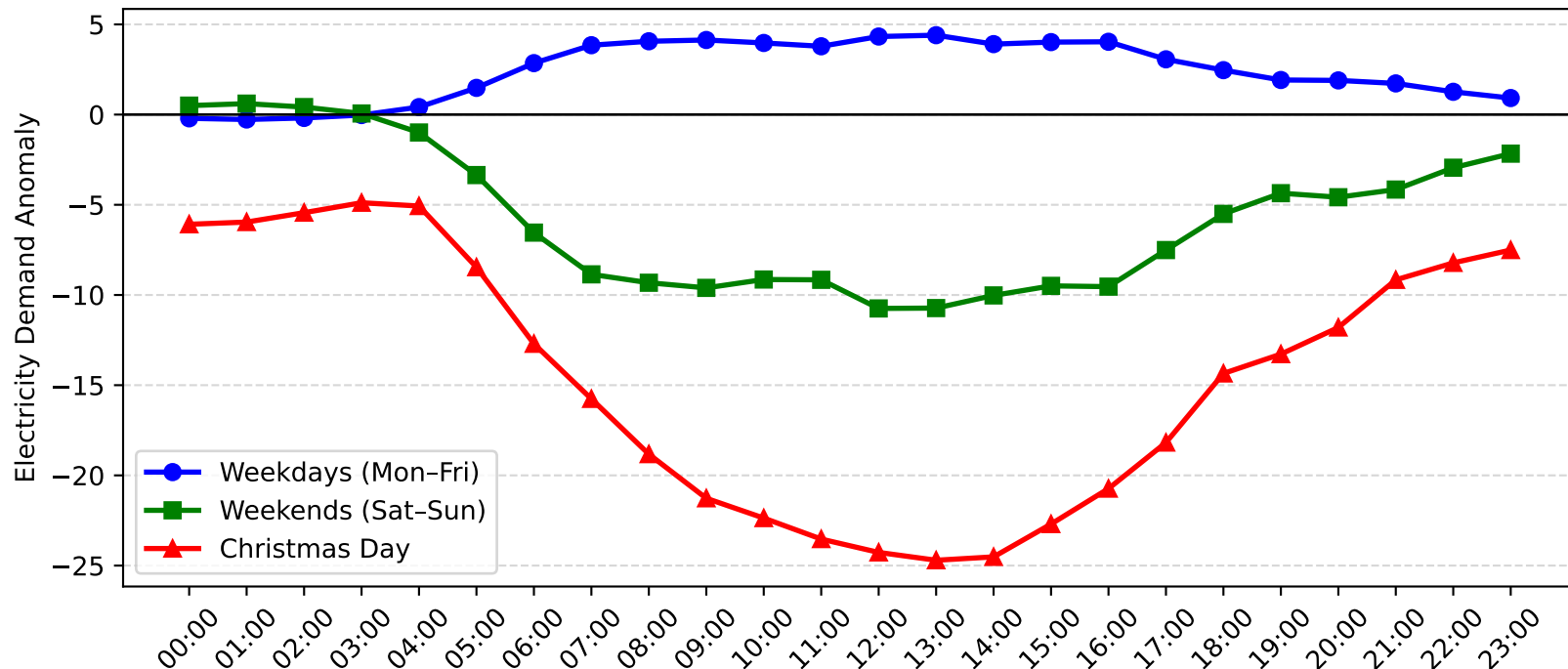
Greenacre Park Demand Anomaly: Christmas Day vs Weekday/Weekend (2005-2006)
