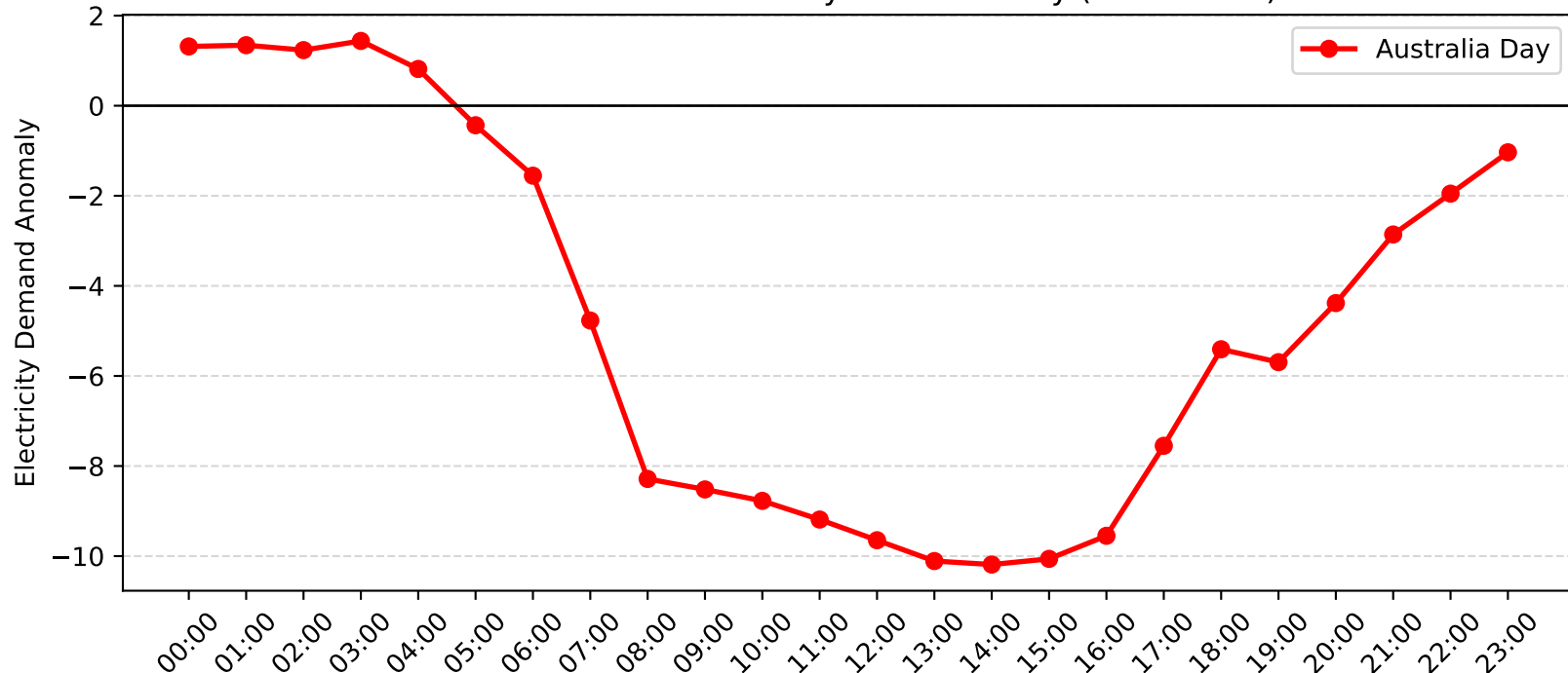
Gore Hill Demand Anomaly: Australia Day (2017-2018)
