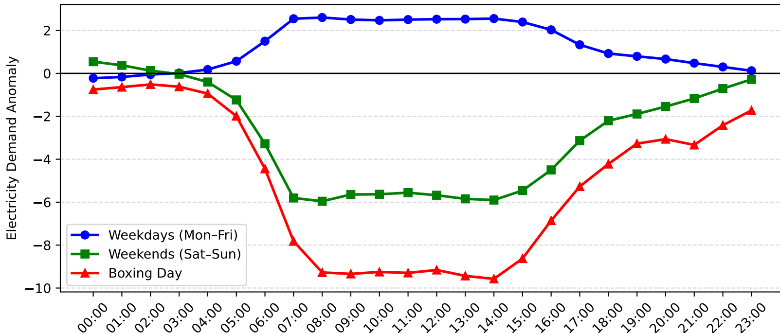
Marrickville Demand Anomaly: Boxing Day vs Weekday/Weekend (2010-2011)
