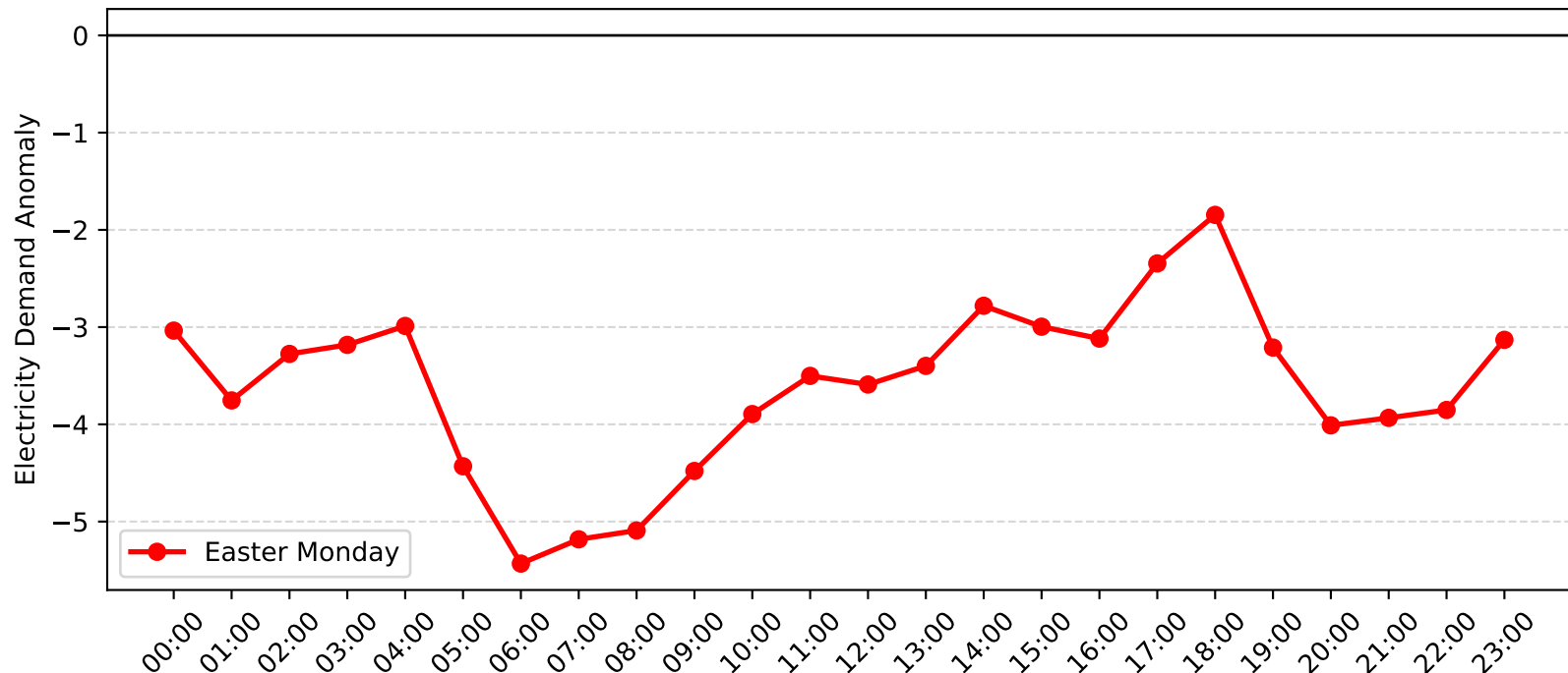
Pennant Hills Demand Anomaly: Easter Monday (2017-2018)
