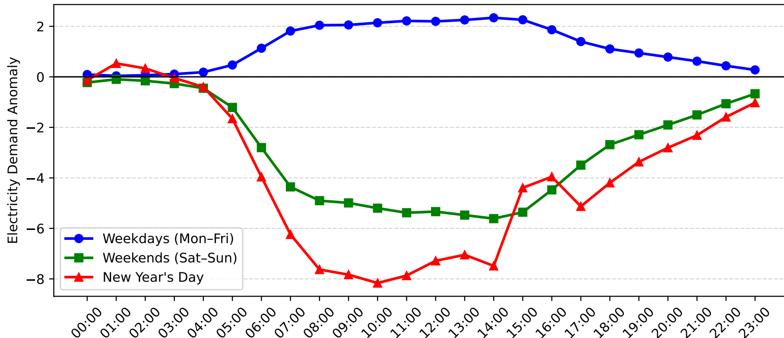
Bankstown Demand Anomaly: New Year's Day vs Weekday/Weekend (2016-2017)
