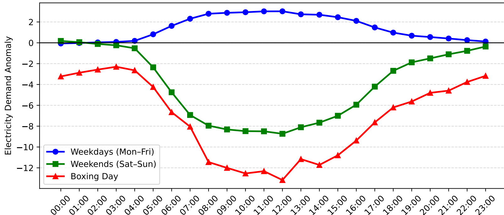
Homebush Bay Demand Anomaly: Boxing Day vs Weekday/Weekend (2013-2014)
