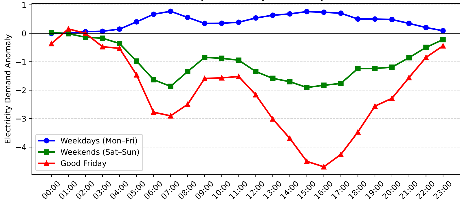
Charmhaven Demand Anomaly: Good Friday vs Weekday/Weekend (2015-2016)
