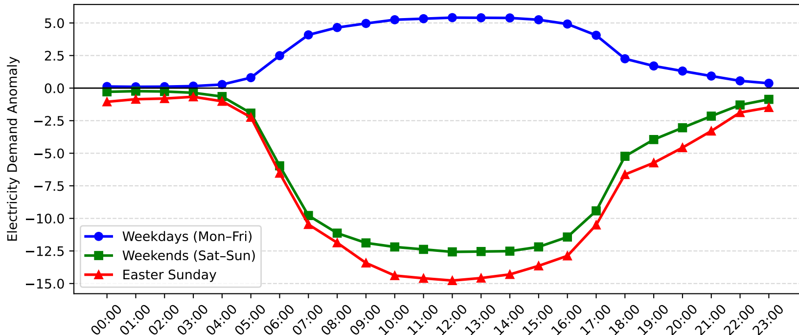
Macquarie Park Demand Anomaly: Easter Sunday vs Weekday/Weekend (2012-2013)
