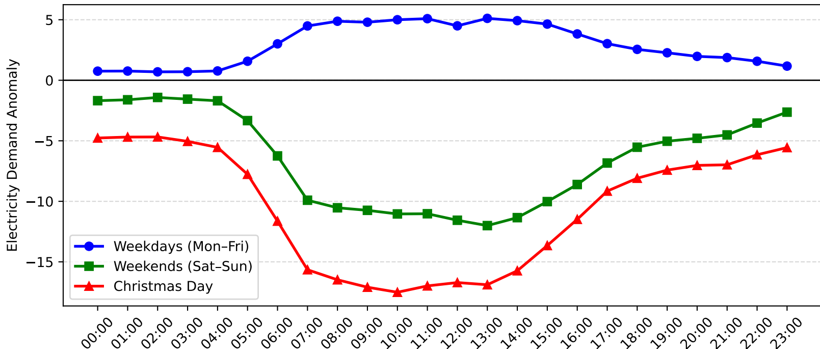
Milperra Demand Anomaly: Christmas Day vs Weekday/Weekend (2004-2005)
