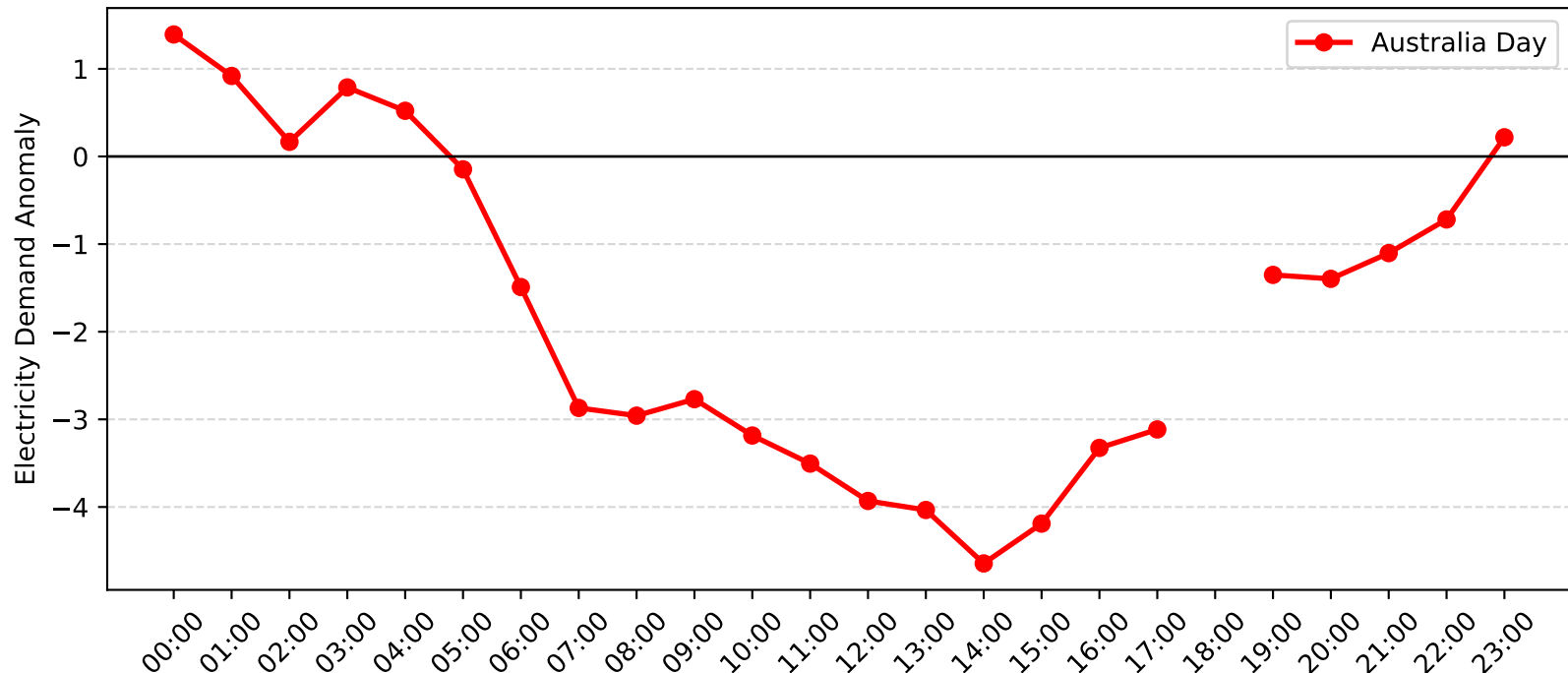
Concord Demand Anomaly: Australia Day (2005-2006)
