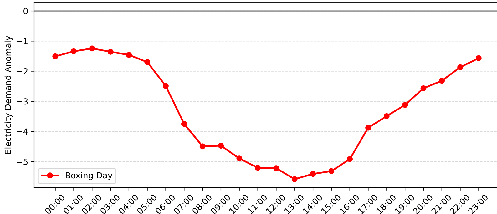
Mayfield West Demand Anomaly: Boxing Day (2012-2013)
