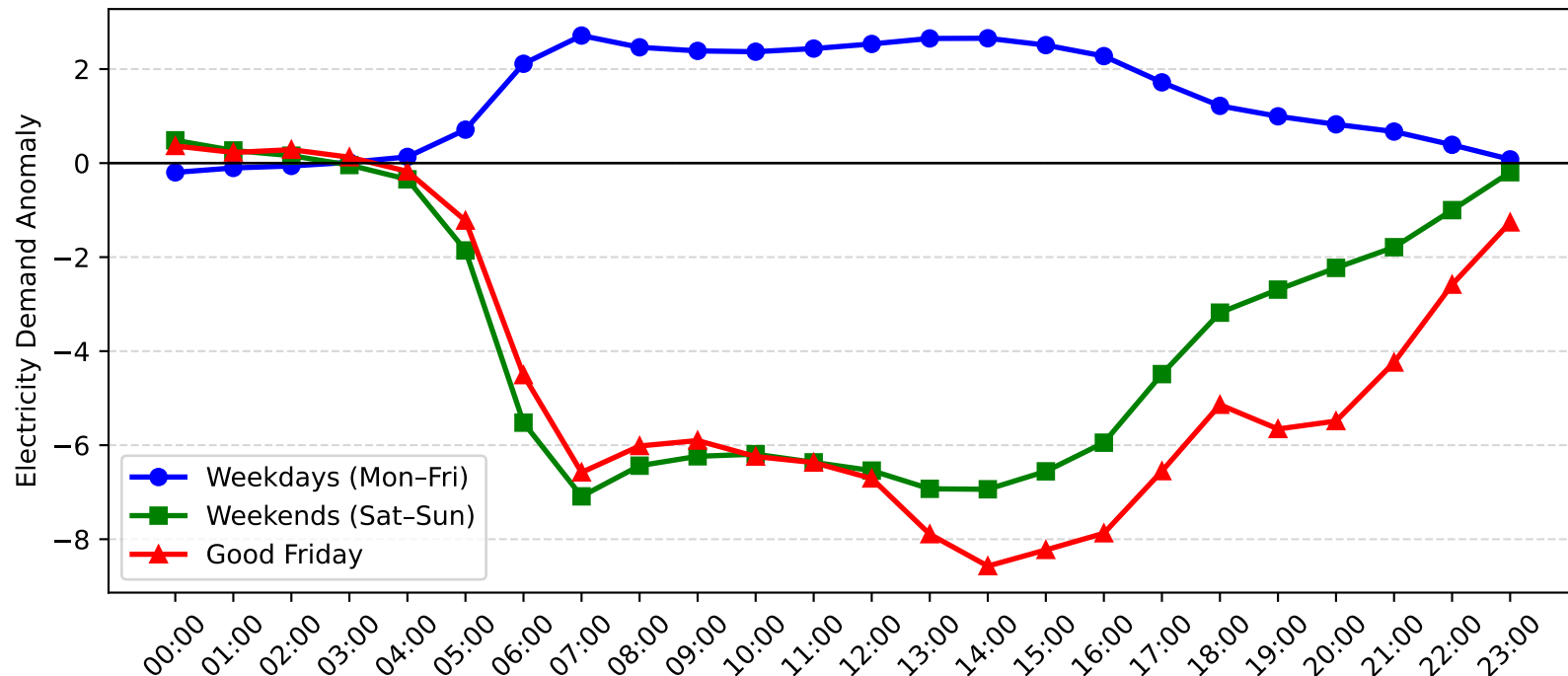
Hunters Hill Demand Anomaly: Good Friday vs Weekday/Weekend (2007-2008)
