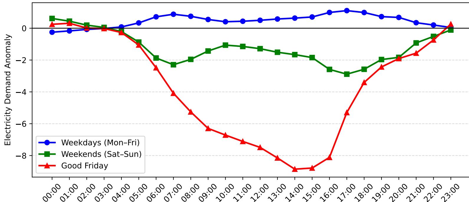
Erina Demand Anomaly: Good Friday vs Weekday/Weekend (2007-2008)
