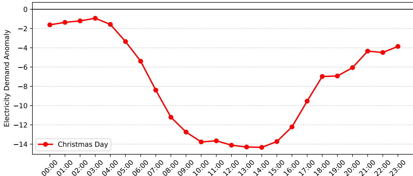
Gore Hill Demand Anomaly: Christmas Day (2014-2015)
