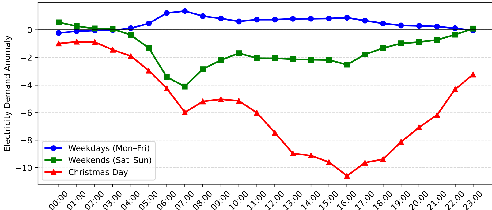
Dulwich Hill Demand Anomaly: Christmas Day vs Weekday/Weekend (2007-2008)
