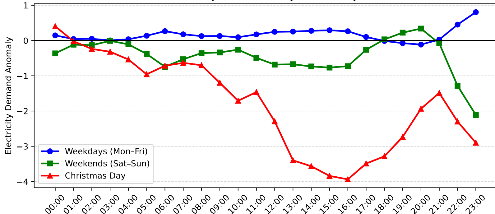
Muswellbrook Demand Anomaly: Christmas Day vs Weekday/Weekend (2007-2008)
