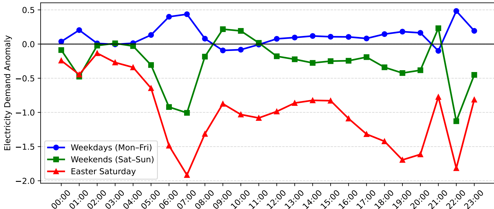
Adamstown Demand Anomaly: Easter Saturday vs Weekday/Weekend (2011-2012)
