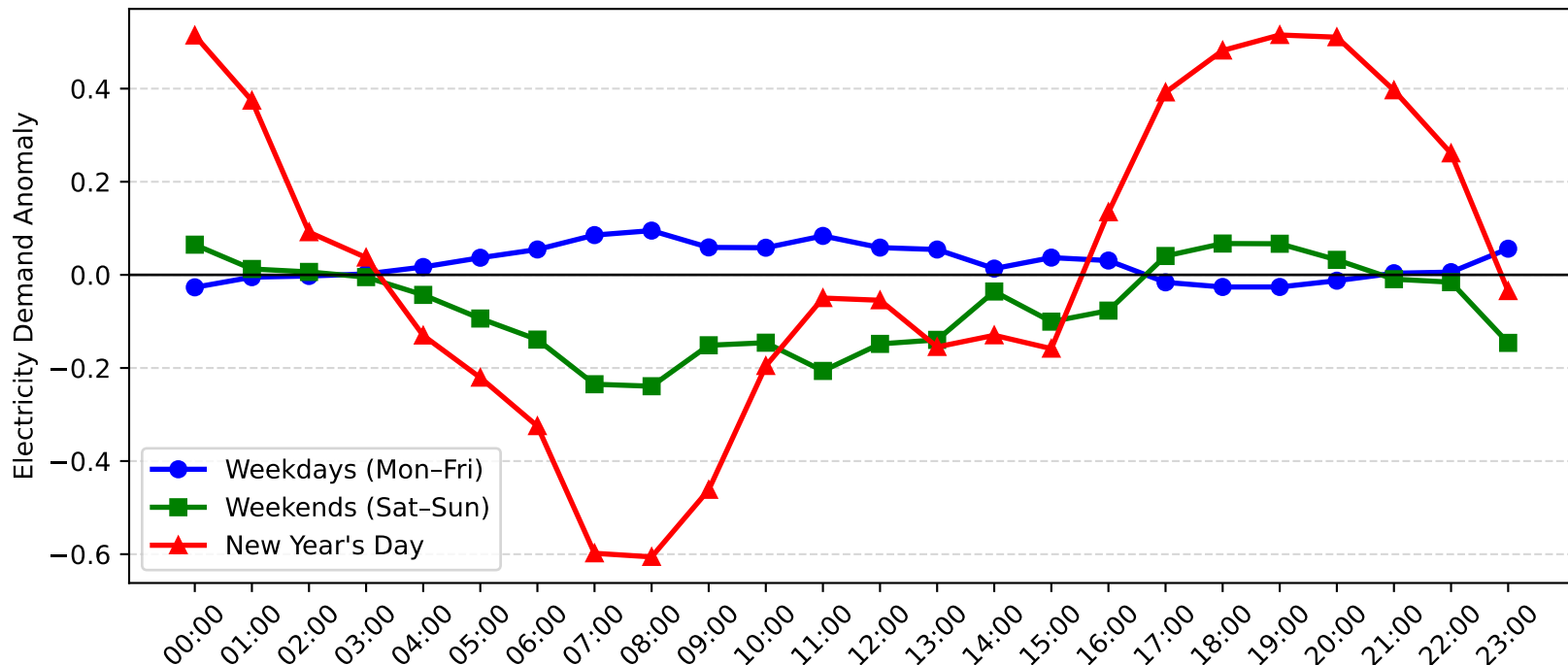
Rothbury Demand Anomaly: New Year's Day vs Weekday/Weekend (2010-2011)
