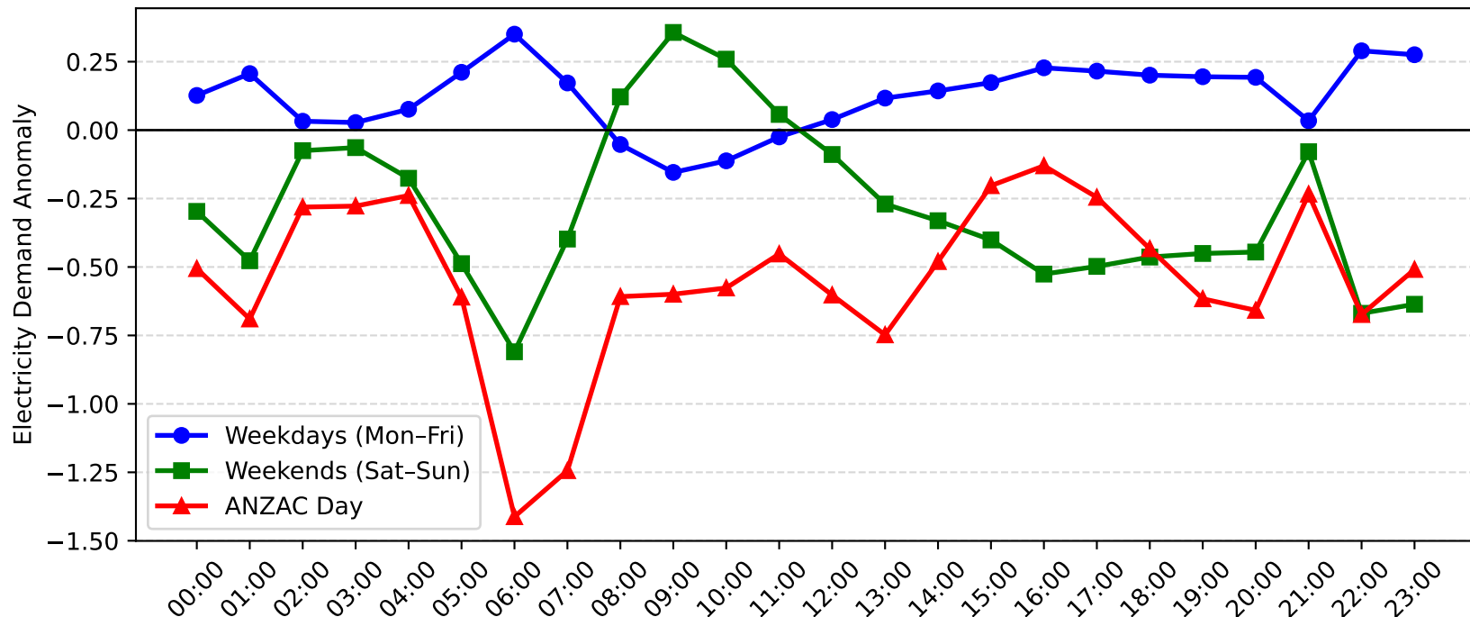
Morisset Demand Anomaly: ANZAC Day vs Weekday/Weekend (2016-2017)
