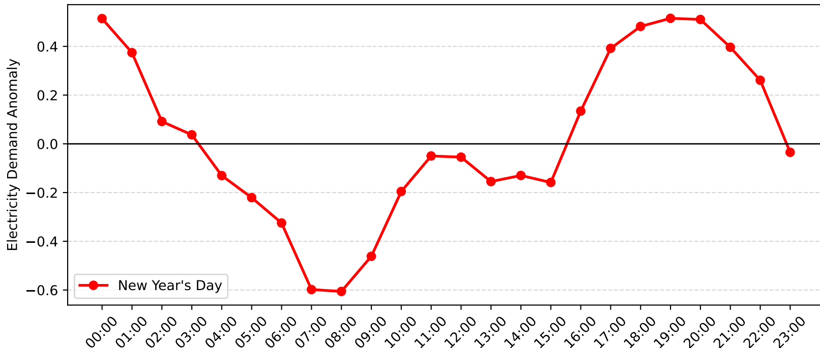
Rothbury Demand Anomaly: New Year's Day (2010-2011)
