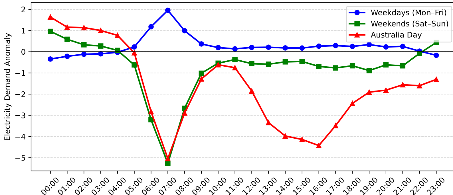
Mosman Demand Anomaly: Australia Day vs Weekday/Weekend (2015-2016)
