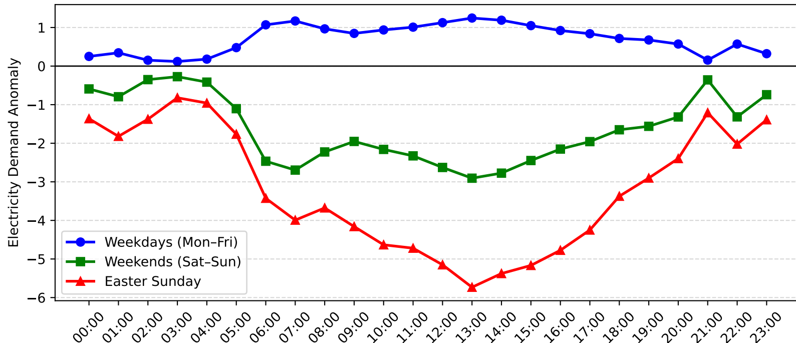
Argenton Demand Anomaly: Easter Sunday vs Weekday/Weekend (2015-2016)
