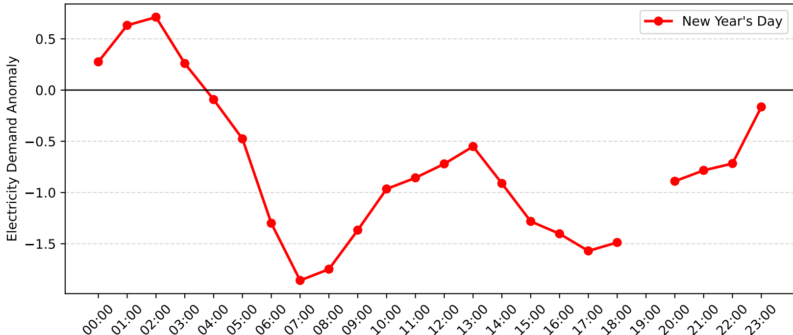
Blakehurst Demand Anomaly: New Year's Day (2014-2015)
