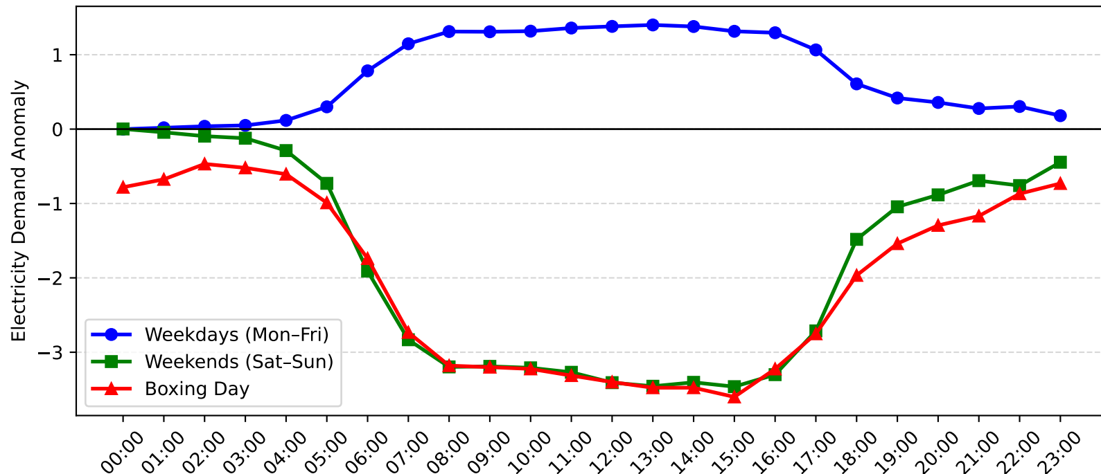
Beacon Hill Demand Anomaly: Boxing Day vs Weekday/Weekend (2011-2012)
