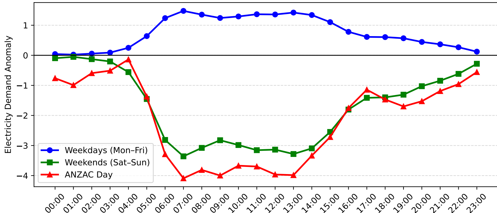
Wyong Demand Anomaly: ANZAC Day vs Weekday/Weekend (2016-2017)
