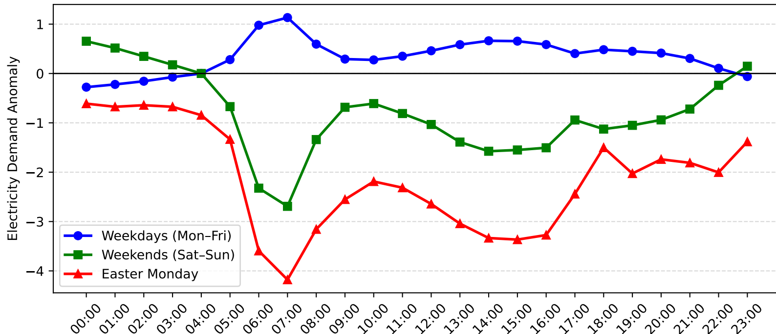
Five Dock Demand Anomaly: Easter Monday vs Weekday/Weekend (2006-2007)
