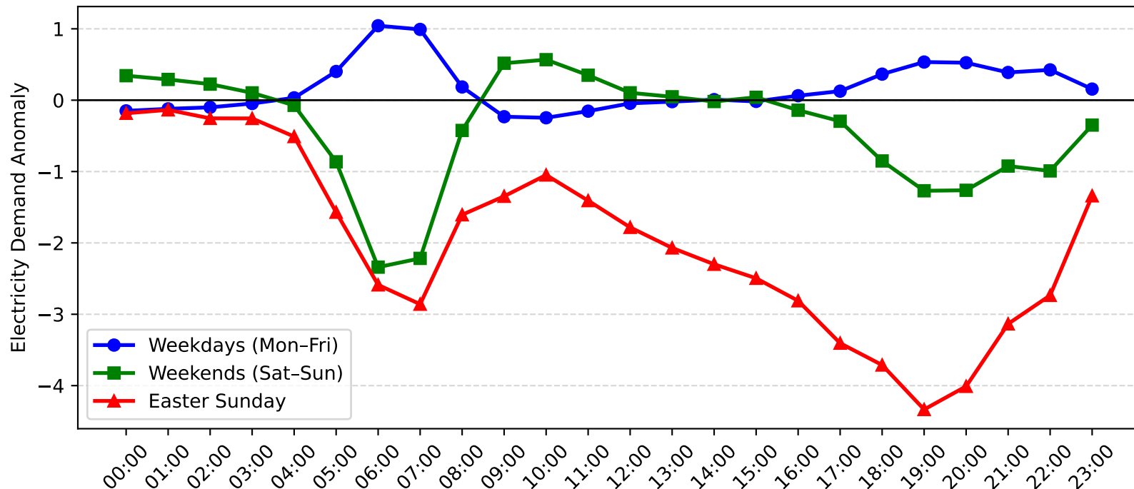
Harbord Demand Anomaly: Easter Sunday vs Weekday/Weekend (2010-2011)
