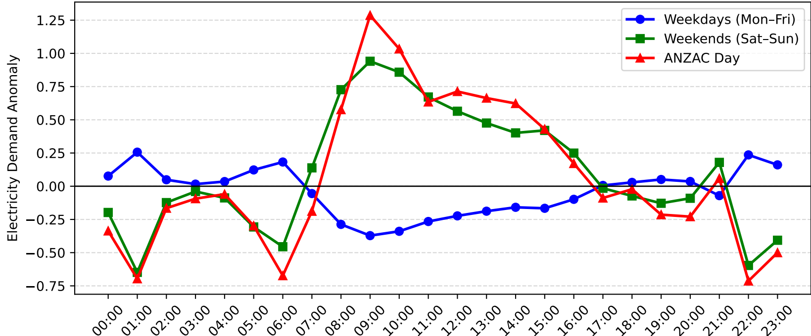
Swansea Demand Anomaly: ANZAC Day vs Weekday/Weekend (2011-2012)
