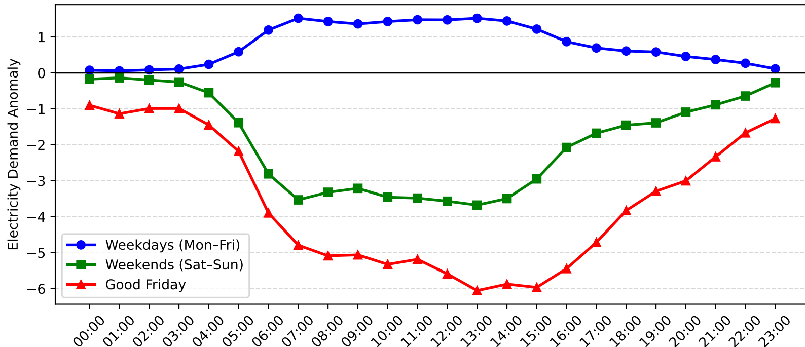
Wyong Demand Anomaly: Good Friday vs Weekday/Weekend (2016-2017)
