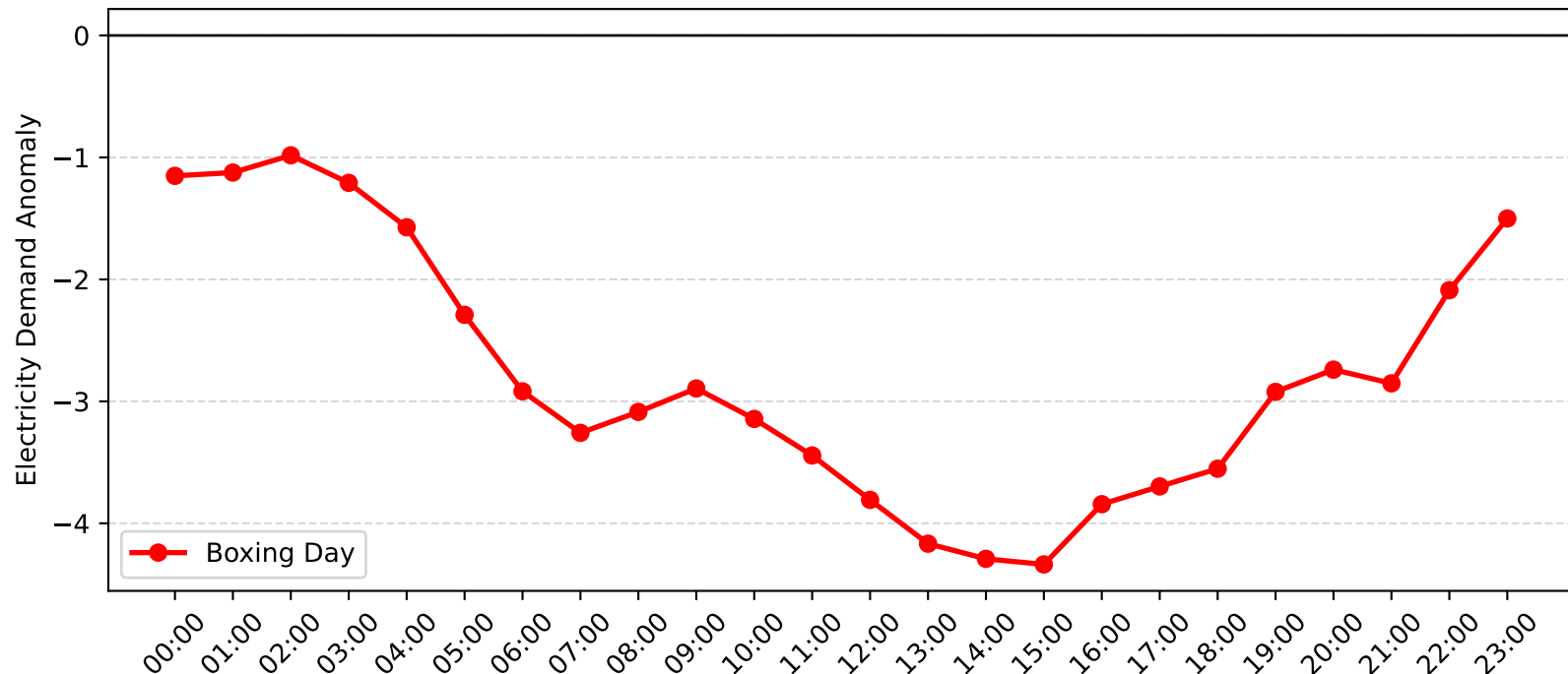
Lisarow Demand Anomaly: Boxing Day (2009-2010)
