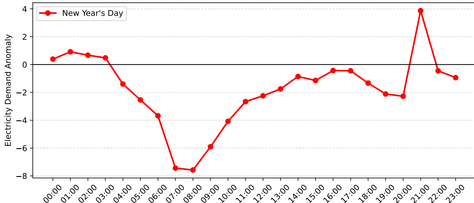
Meadowbank Demand Anomaly: New Year's Day (2010-2011)
