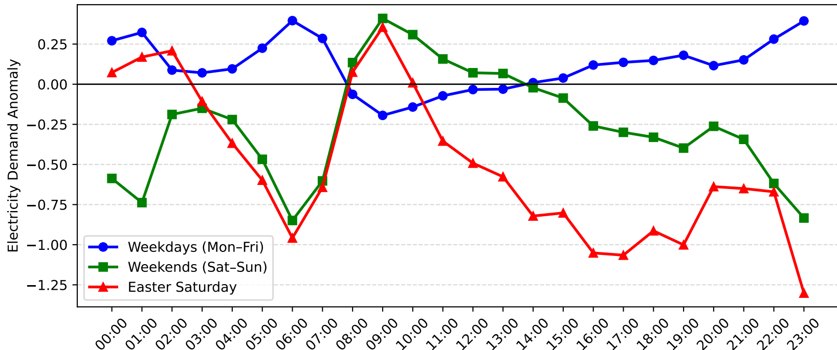
Morisset Demand Anomaly: Easter Saturday vs Weekday/Weekend (2009-2010)
