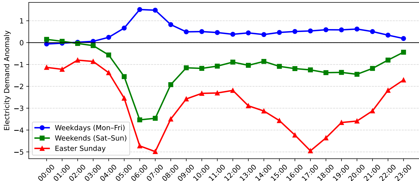
Revesby Demand Anomaly: Easter Sunday vs Weekday/Weekend (2012-2013)
