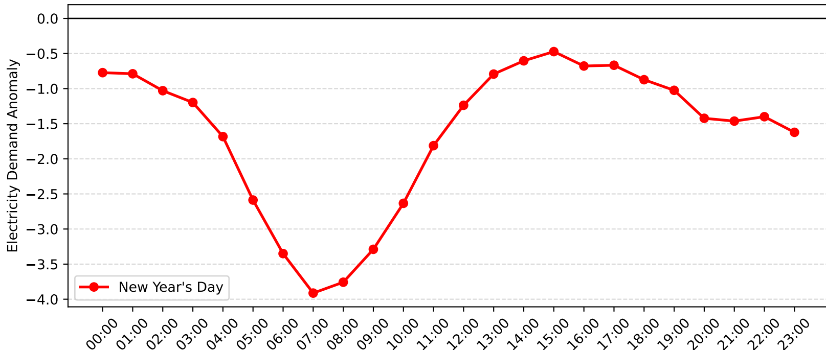
Lisarow Demand Anomaly: New Year's Day (2011-2012)
