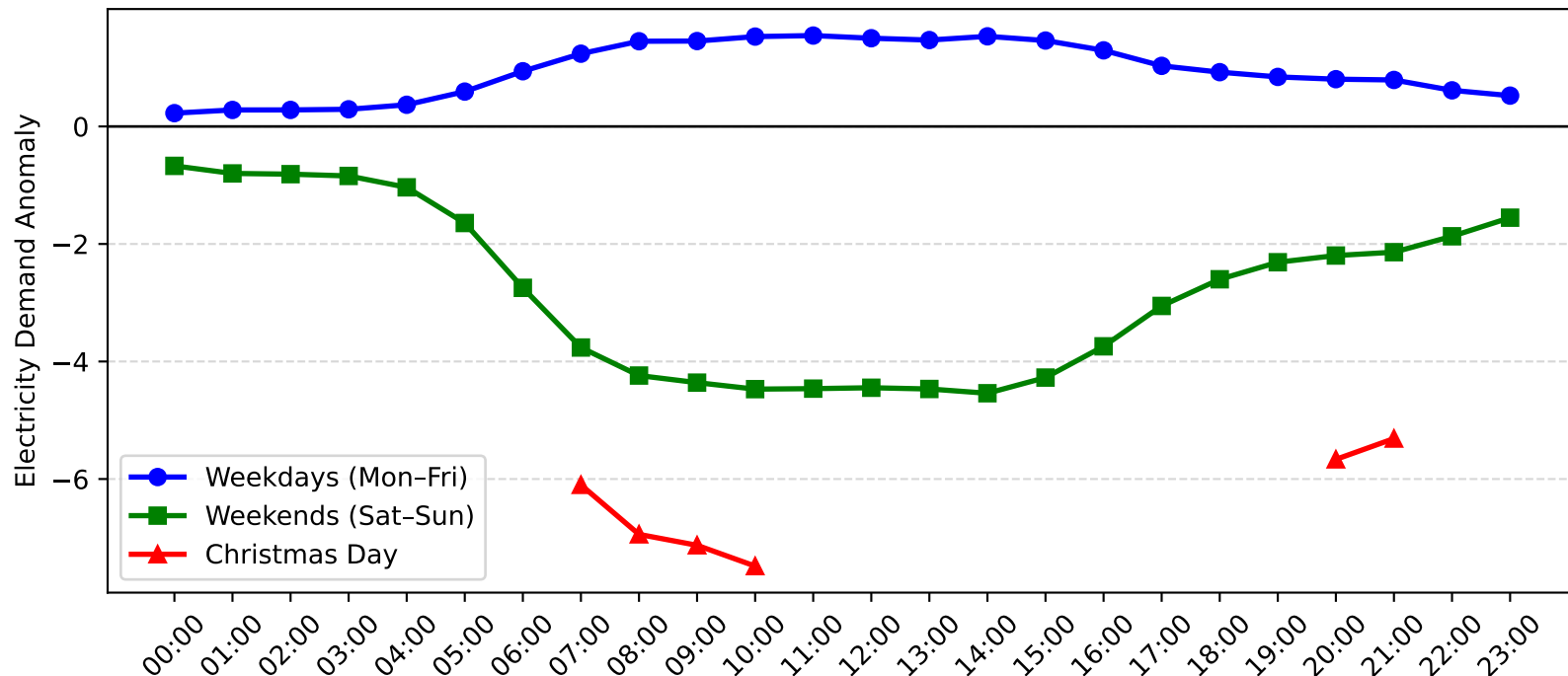
Leightonfield Demand Anomaly: Christmas Day vs Weekday/Weekend (2013-2014)
