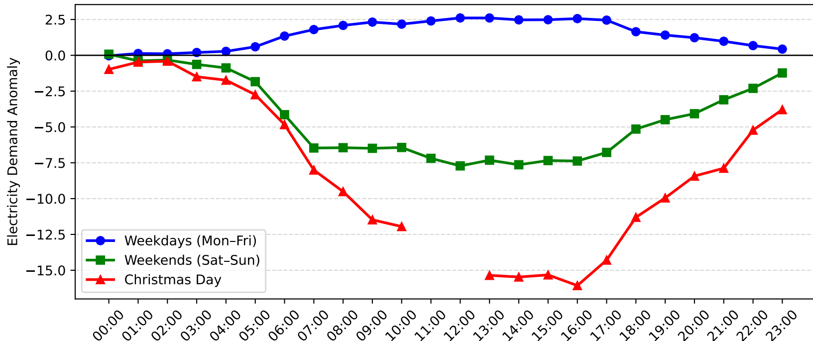
Burwood Demand Anomaly: Christmas Day vs Weekday/Weekend (2008-2009)
