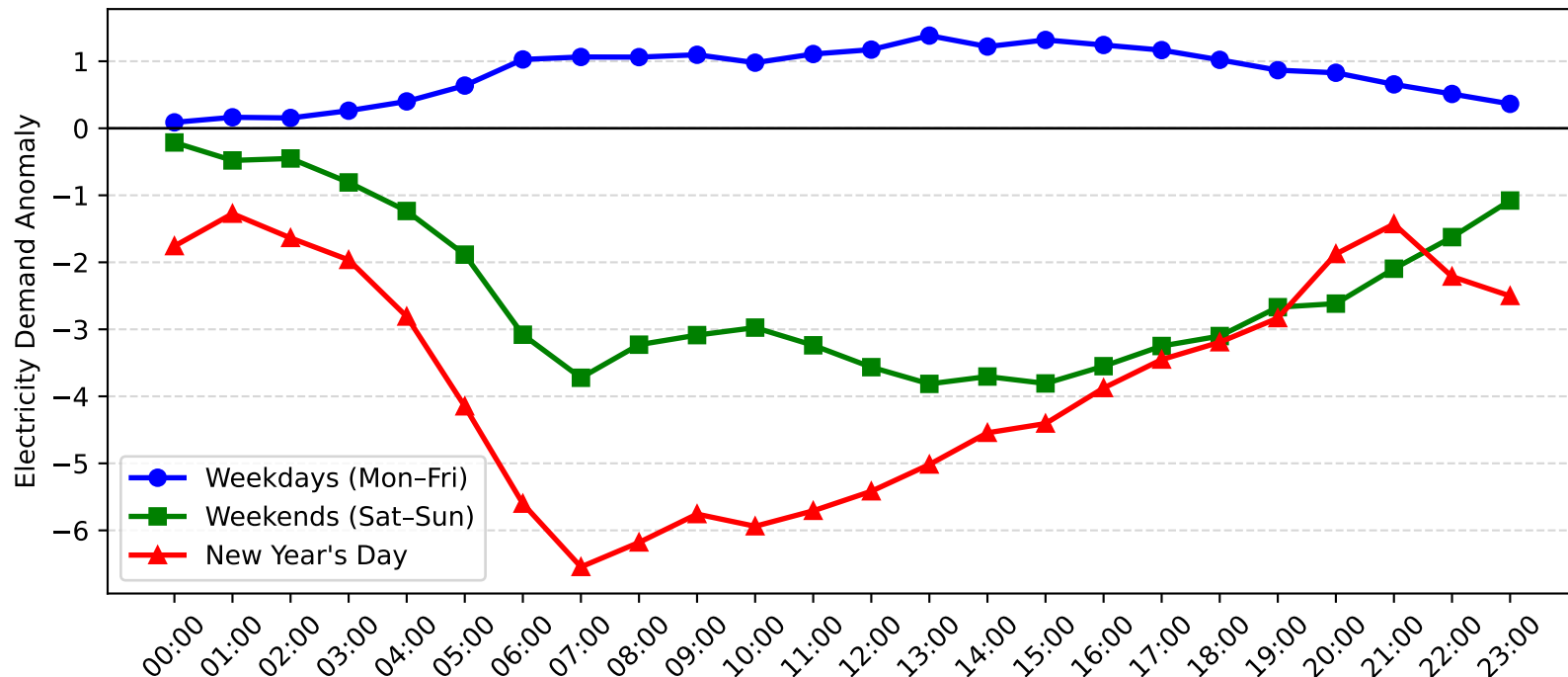
Enfield Demand Anomaly: New Year's Day vs Weekday/Weekend (2009-2010)
