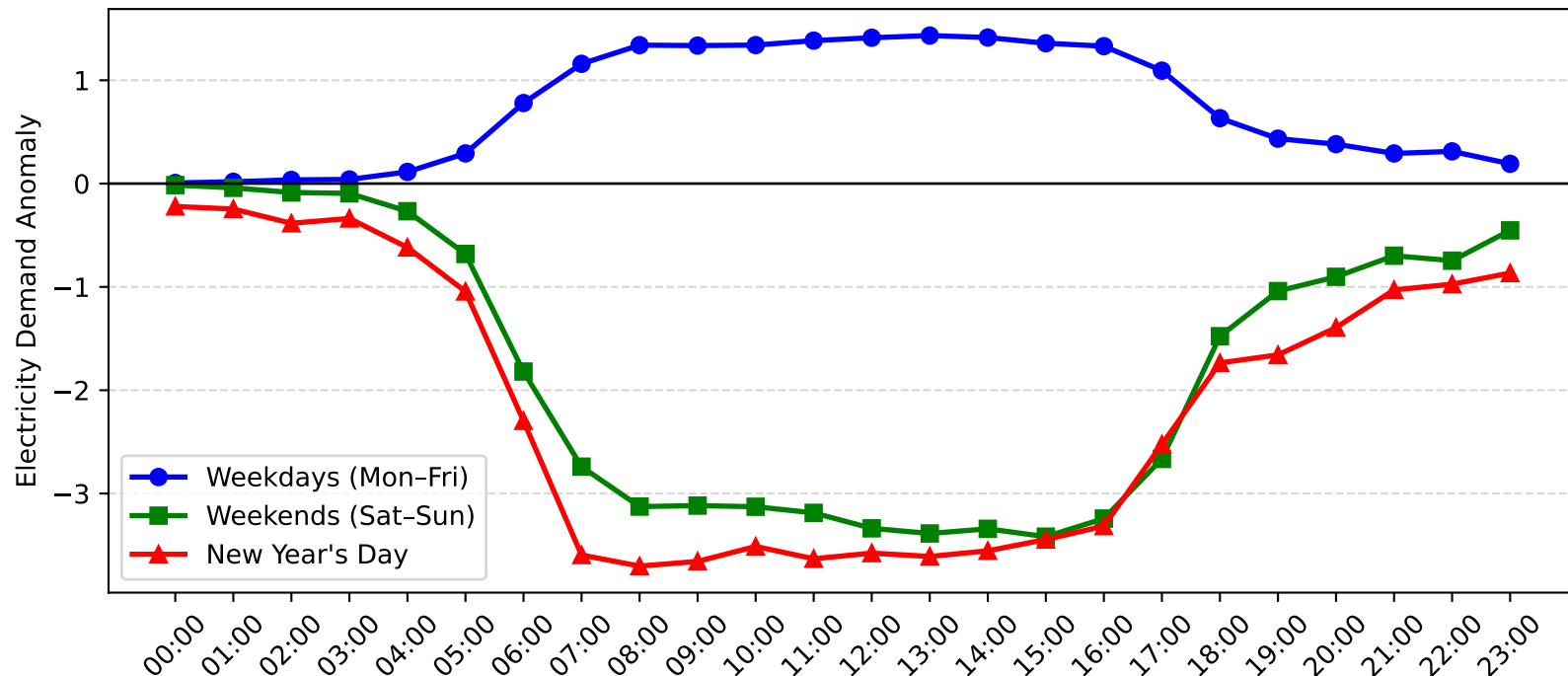
Beacon Hill Demand Anomaly: New Year's Day vs Weekday/Weekend (2012-2013)
