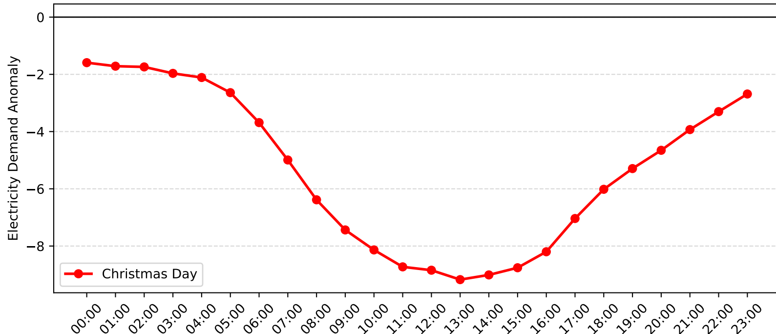
Caringbah Demand Anomaly: Christmas Day (2006-2007)
