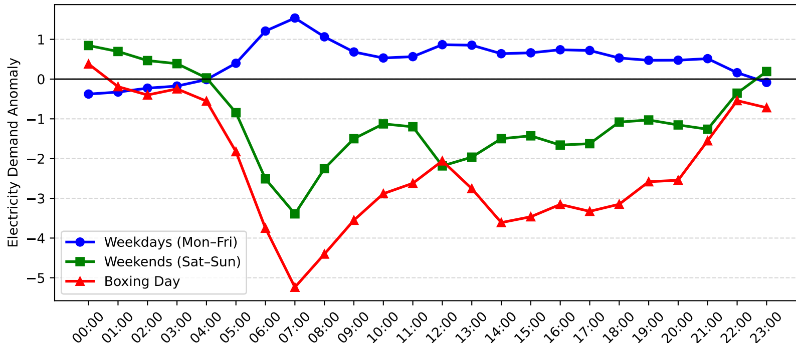
Mortdale Demand Anomaly: Boxing Day vs Weekday/Weekend (2004-2005)
