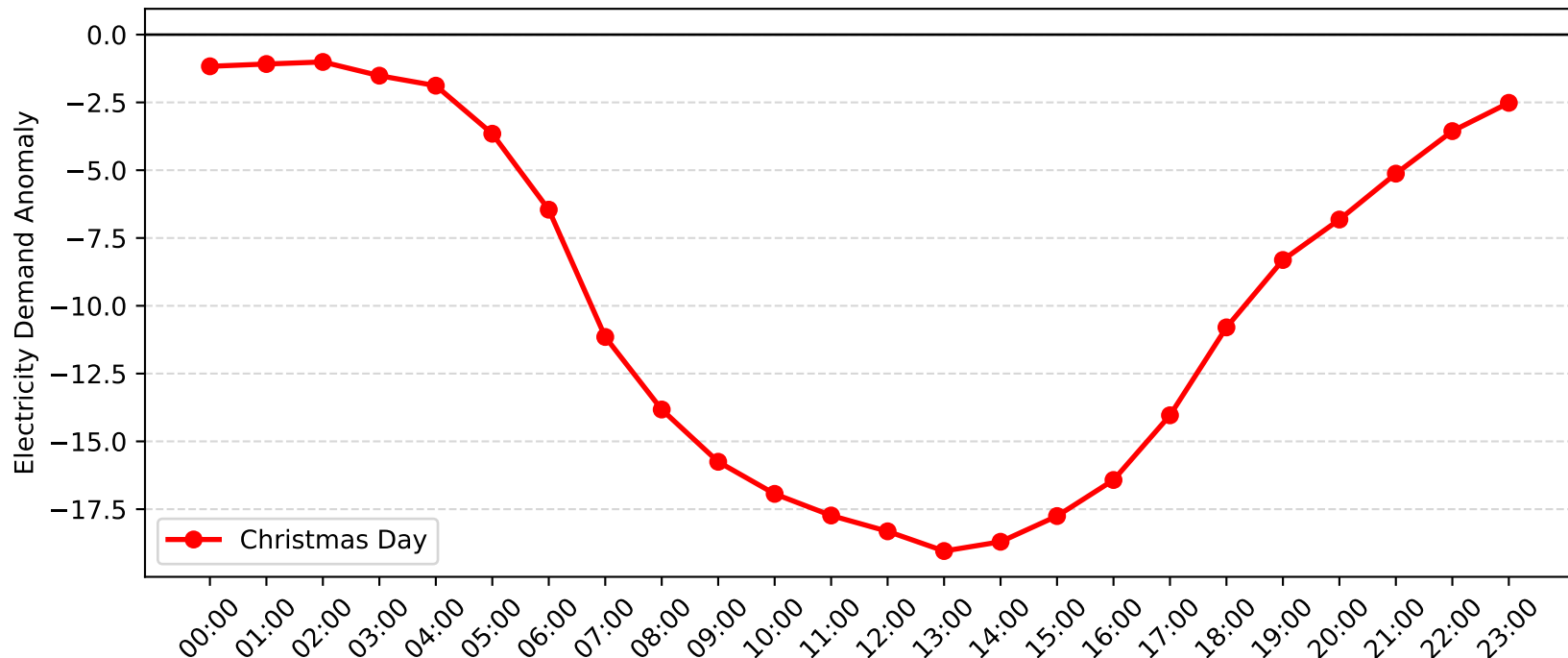
Zetland Demand Anomaly: Christmas Day (2010-2011)
