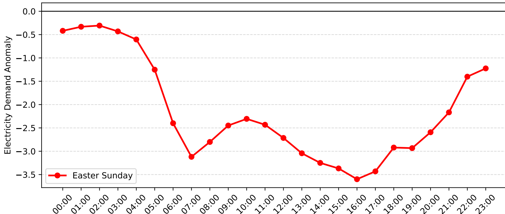
Blakehurst Demand Anomaly: Easter Sunday (2009-2010)
