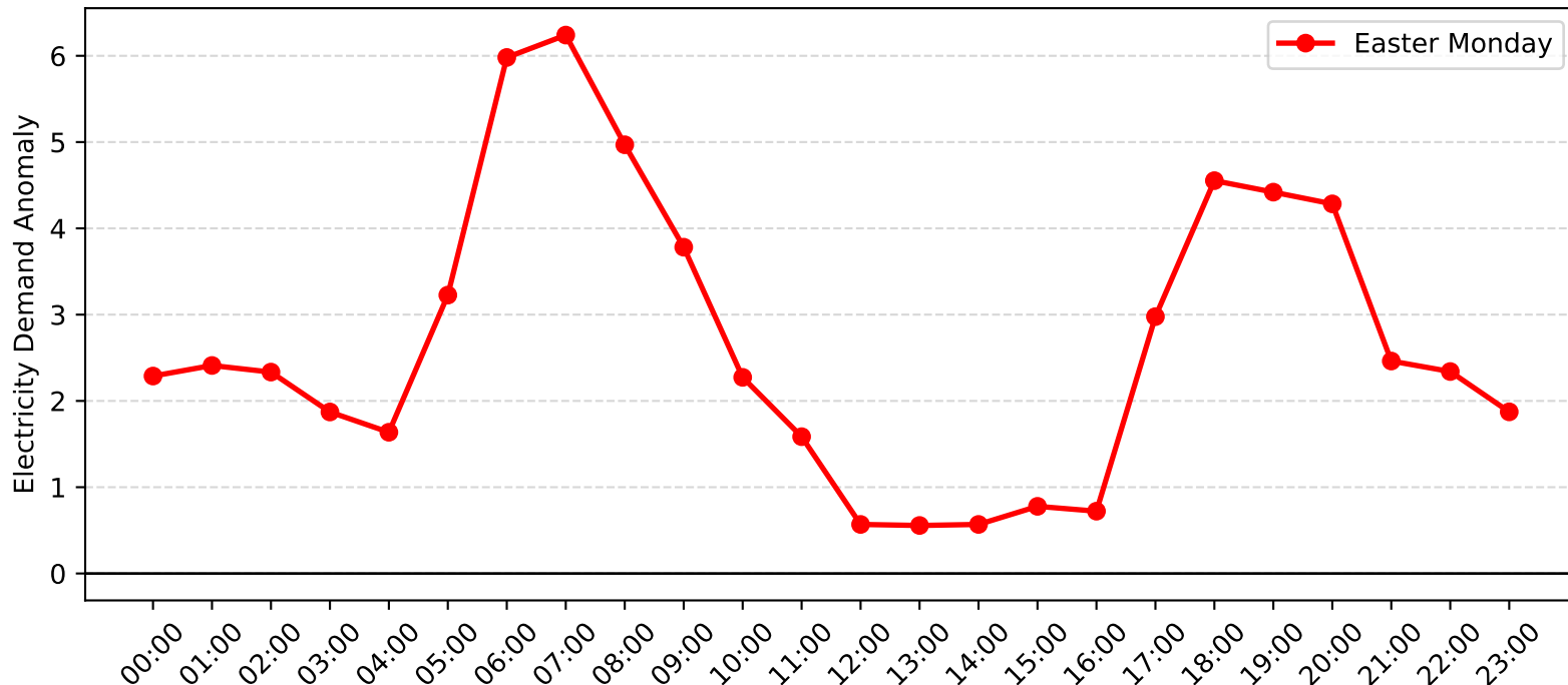
Wyong Demand Anomaly: Easter Monday (2004-2005)
