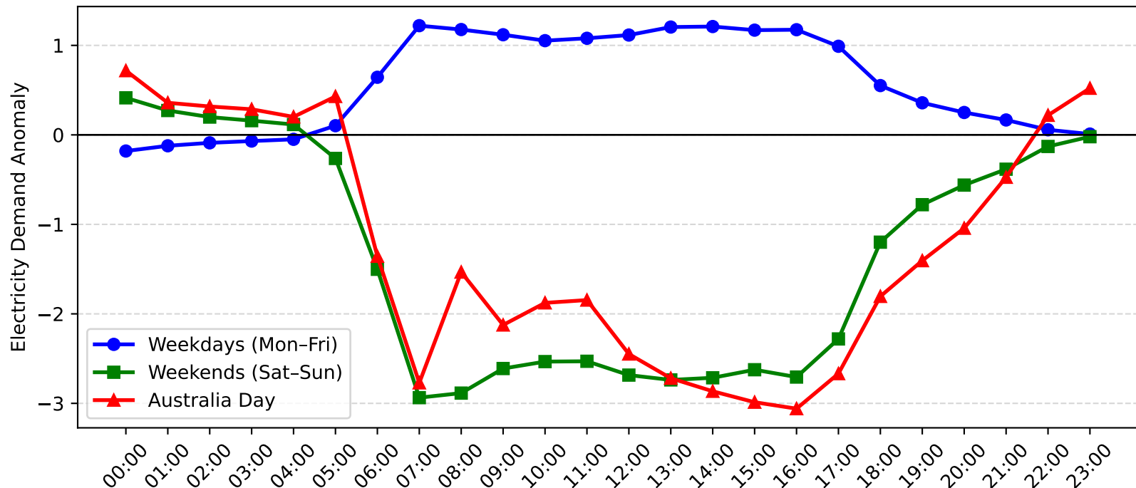
Pymble Demand Anomaly: Australia Day vs Weekday/Weekend (2013-2014)
