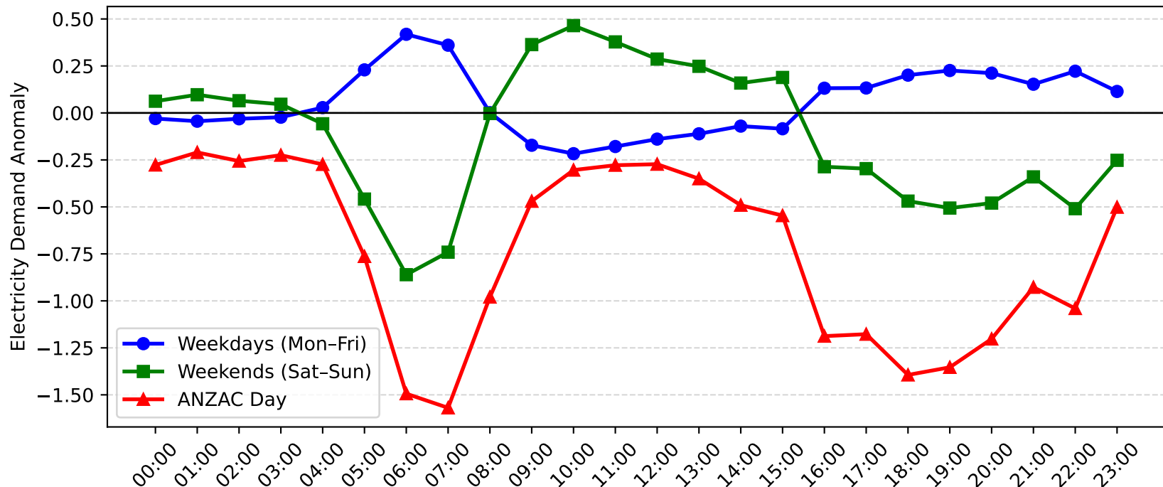
Narrabeen Demand Anomaly: ANZAC Day vs Weekday/Weekend (2009-2010)
