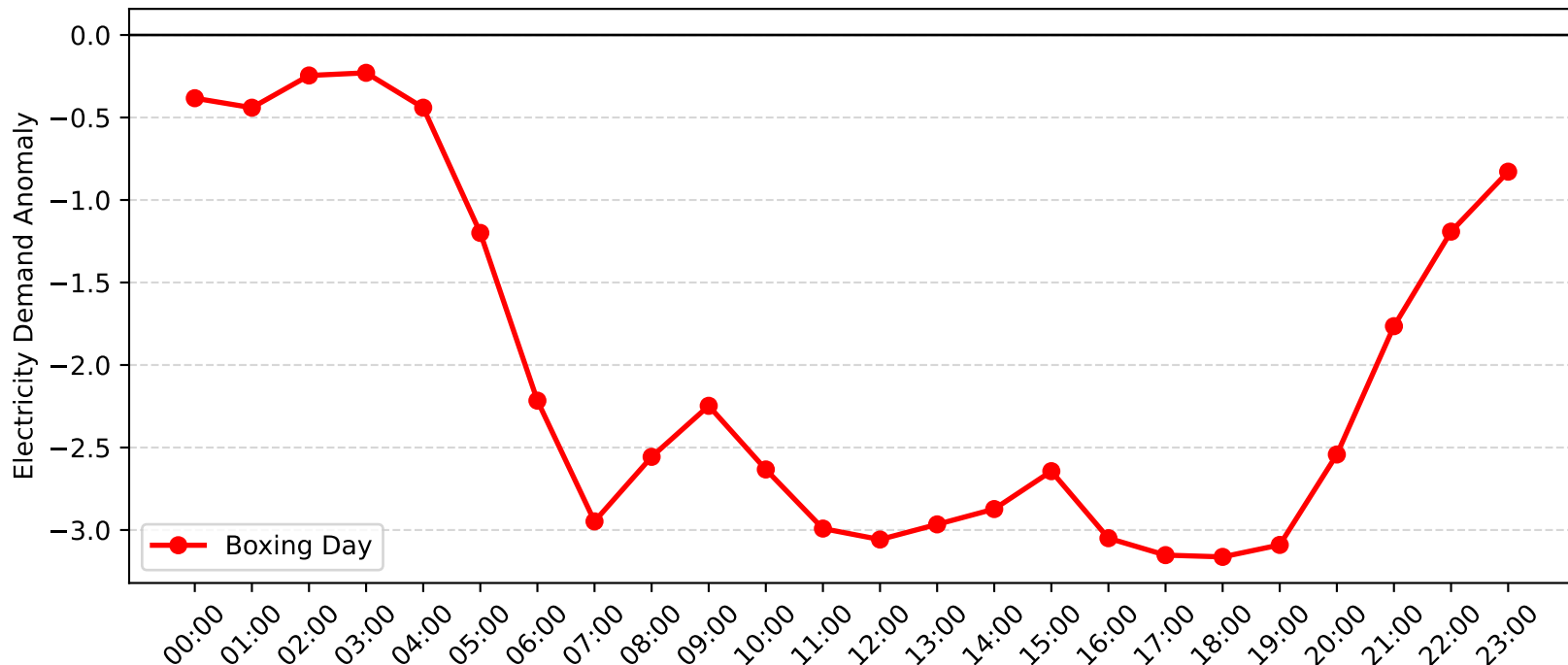
Dee Why West Demand Anomaly: Boxing Day (2015-2016)
