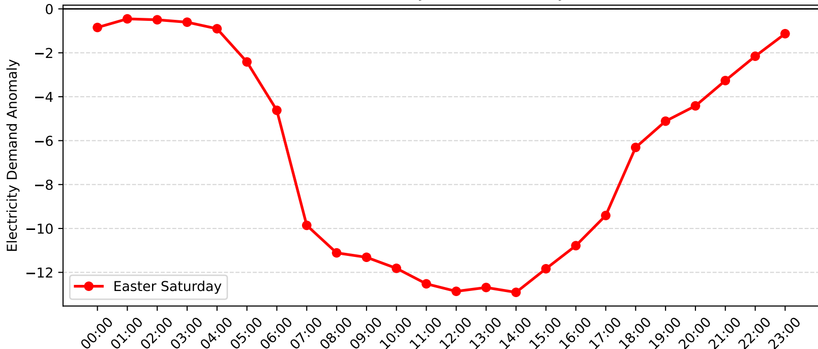
Gore Hill Demand Anomaly: Easter Saturday (2013-2014)
