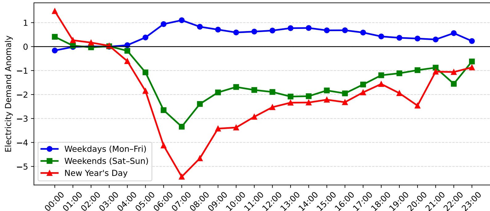
Dee Why West Demand Anomaly: New Year's Day vs Weekday/Weekend (2008-2009)
