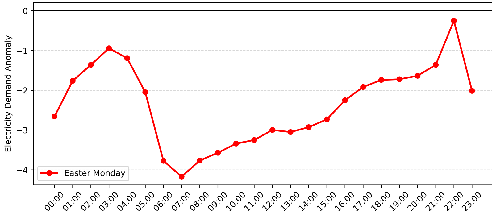
Rutherford Demand Anomaly: Easter Monday (2010-2011)
