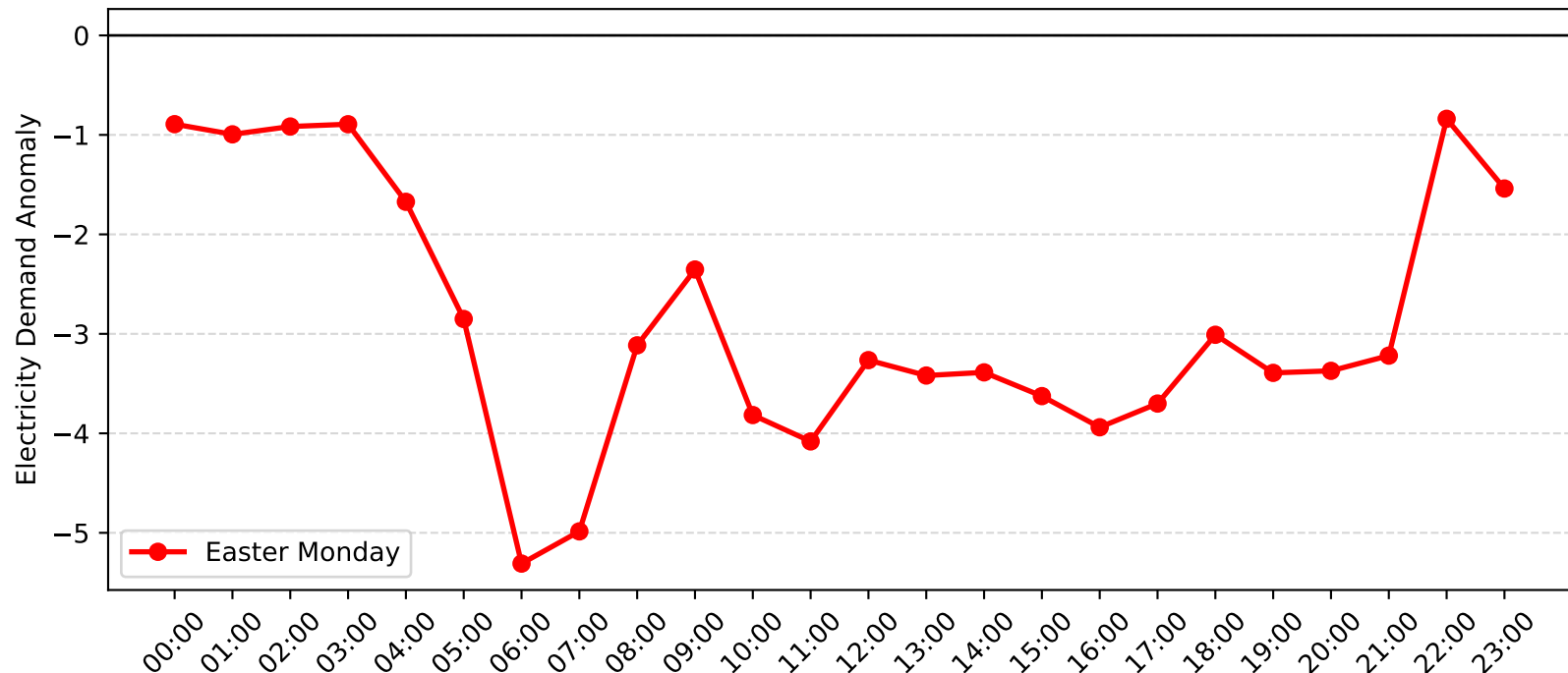
Revesby Demand Anomaly: Easter Monday (2006-2007)
