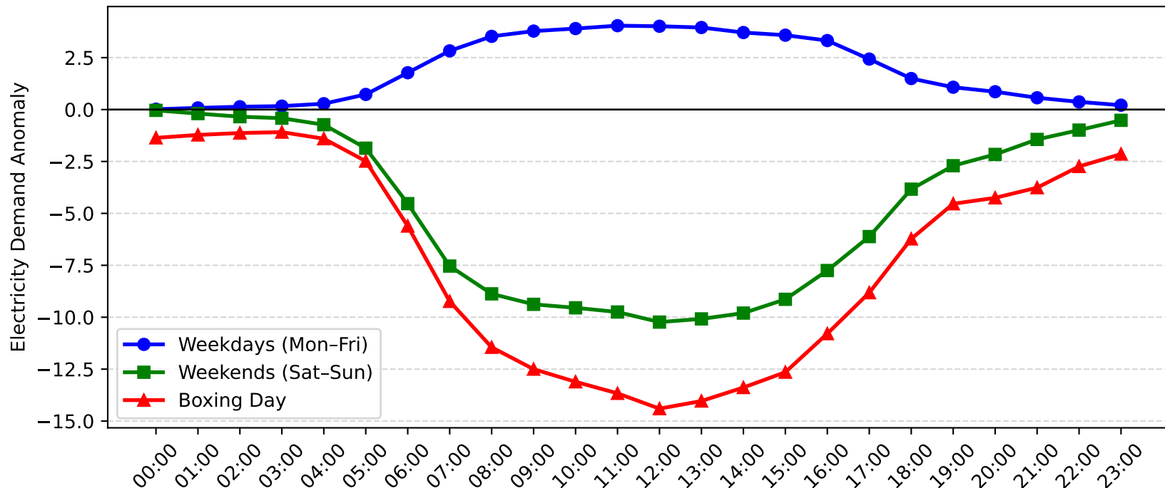
Mascot Demand Anomaly: Boxing Day vs Weekday/Weekend (2009-2010)
