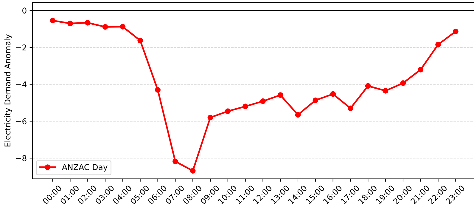
Epping Demand Anomaly: ANZAC Day (2015-2016)
