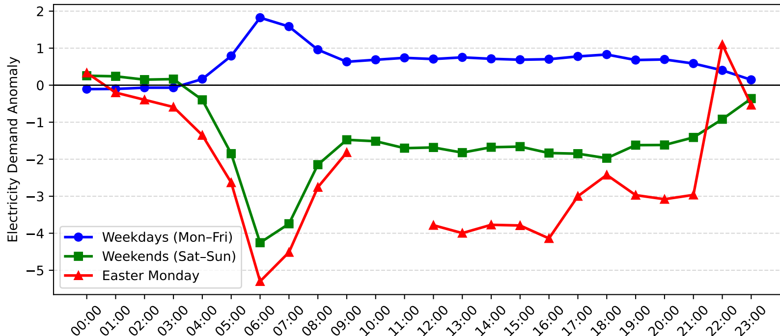
Revesby Demand Anomaly: Easter Monday vs Weekday/Weekend (2005-2006)
