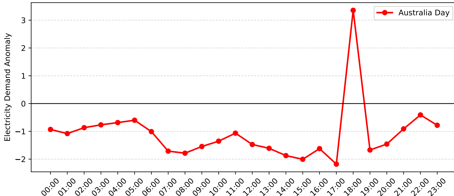
Pymble Demand Anomaly: Australia Day (2004-2005)
