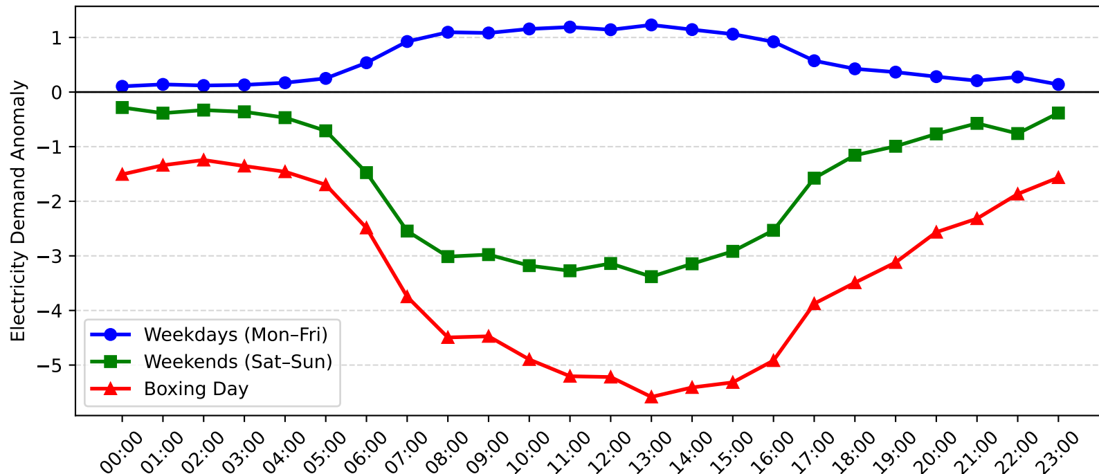
Mayfield West Demand Anomaly: Boxing Day vs Weekday/Weekend (2012-2013)
