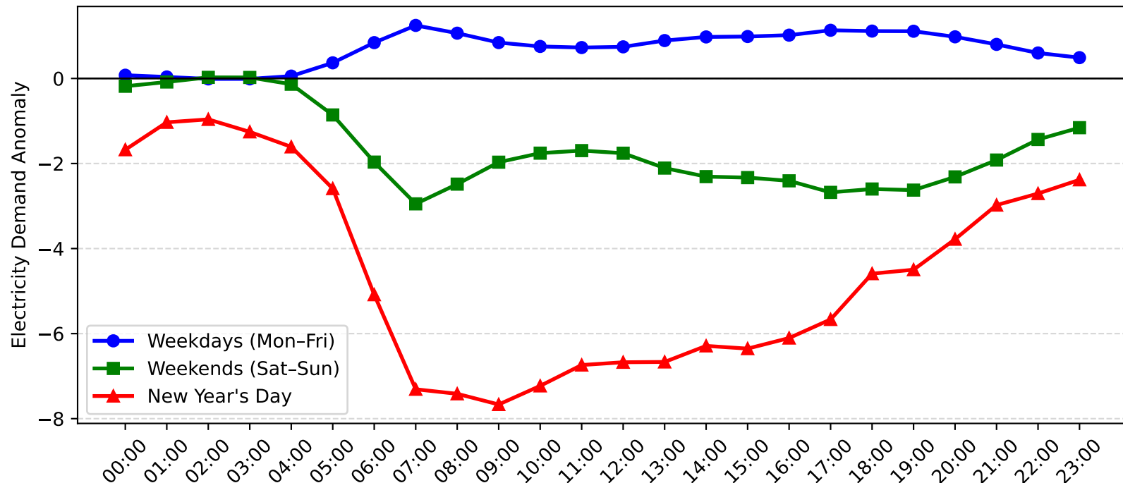
Maroubra Demand Anomaly: New Year's Day vs Weekday/Weekend (2012-2013)
