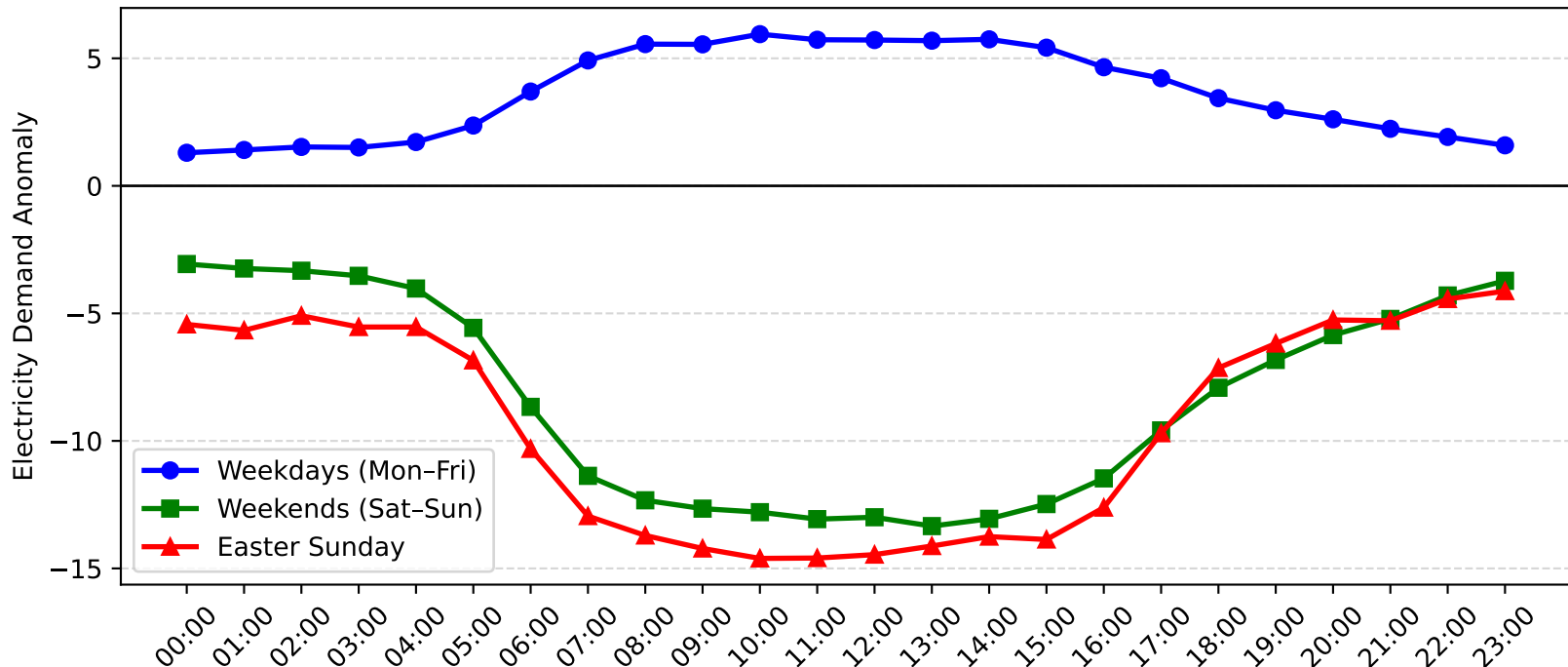
Flemington Demand Anomaly: Easter Sunday vs Weekday/Weekend (2006-2007)
