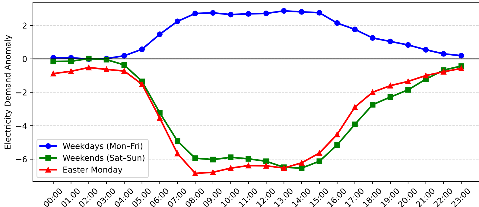
Brookvale Demand Anomaly: Easter Monday vs Weekday/Weekend (2016-2017)
