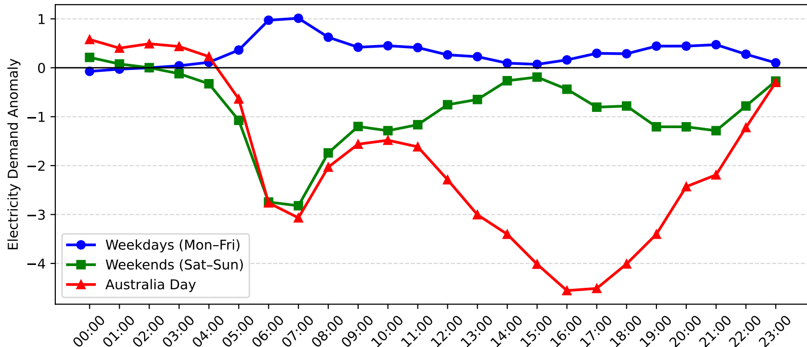
Revesby Demand Anomaly: Australia Day vs Weekday/Weekend (2015-2016)
