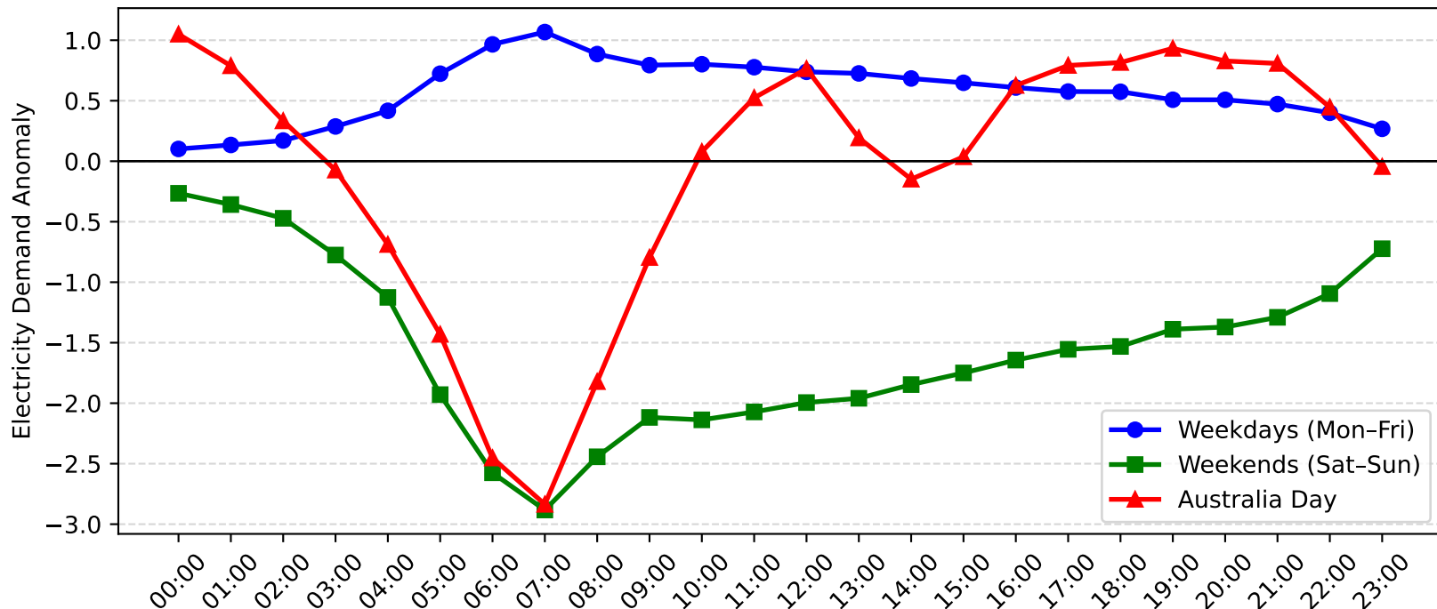
Lisarow Demand Anomaly: Australia Day vs Weekday/Weekend (2011-2012)
