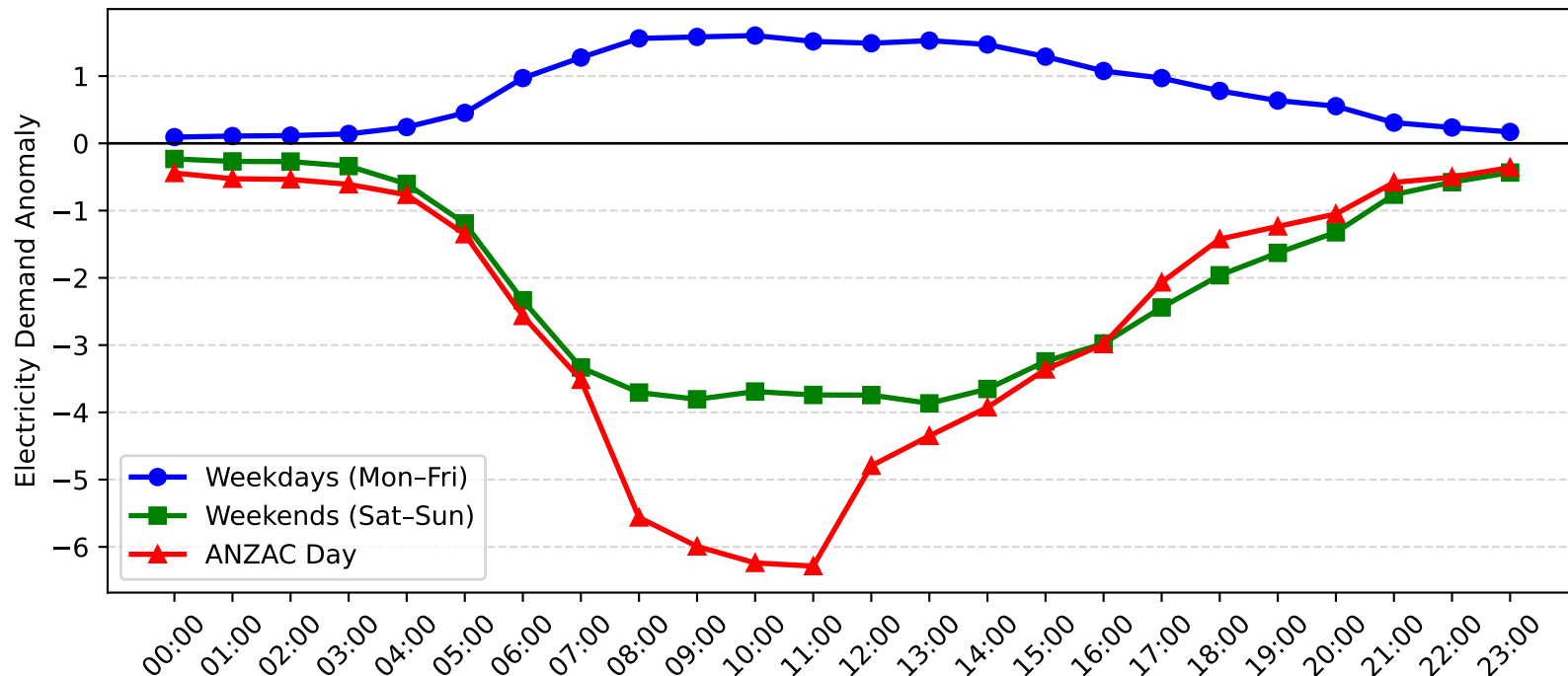
Auburn Demand Anomaly: ANZAC Day vs Weekday/Weekend (2005-2006)
