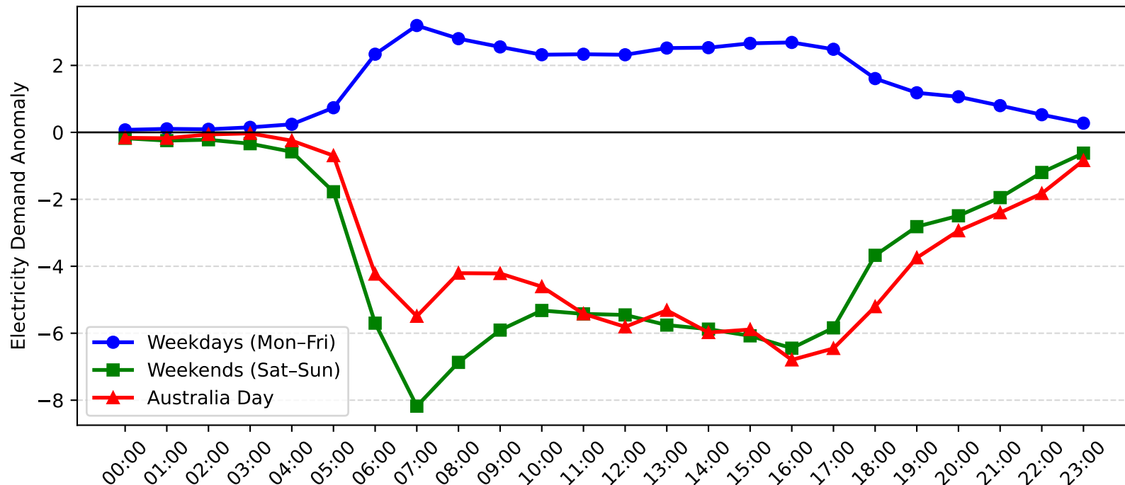
Epping Demand Anomaly: Australia Day vs Weekday/Weekend (2008-2009)
