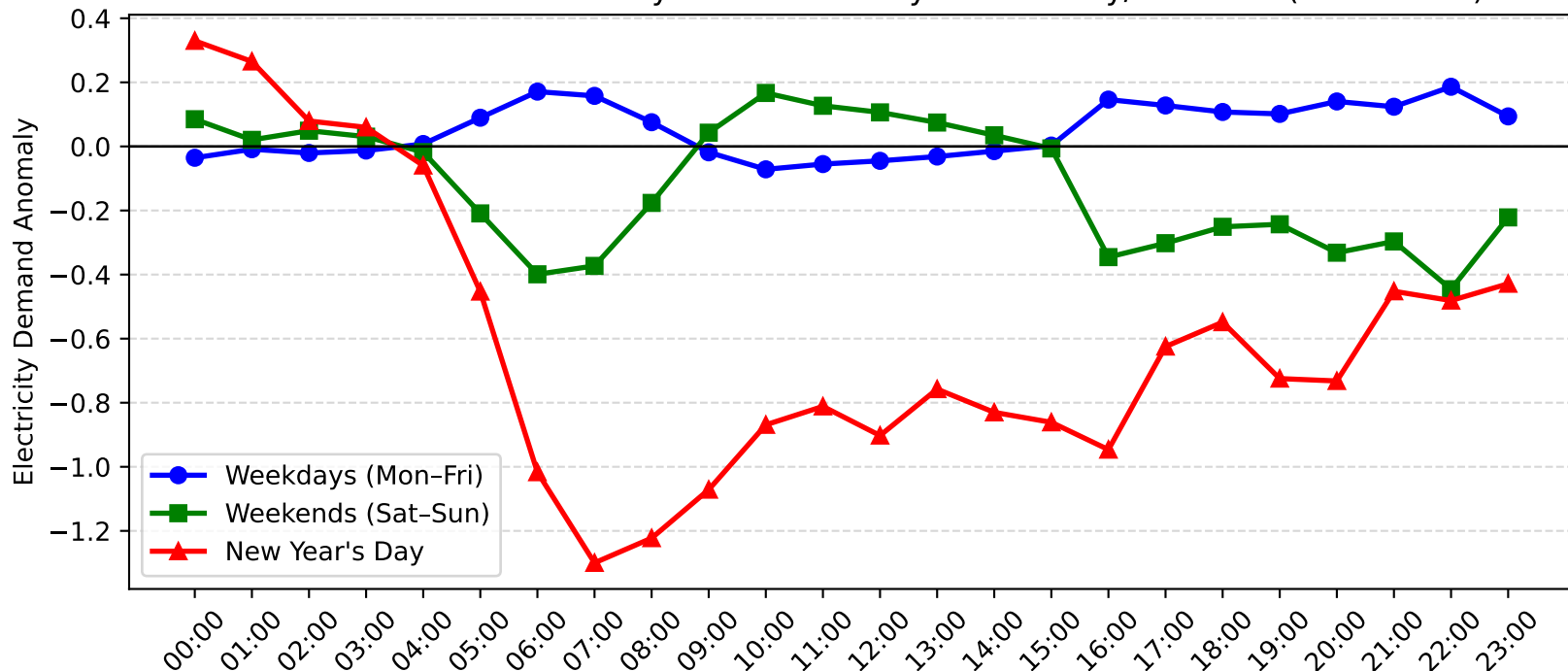
Narrabeen Demand Anomaly: New Year's Day vs Weekday/Weekend (2012-2013)
