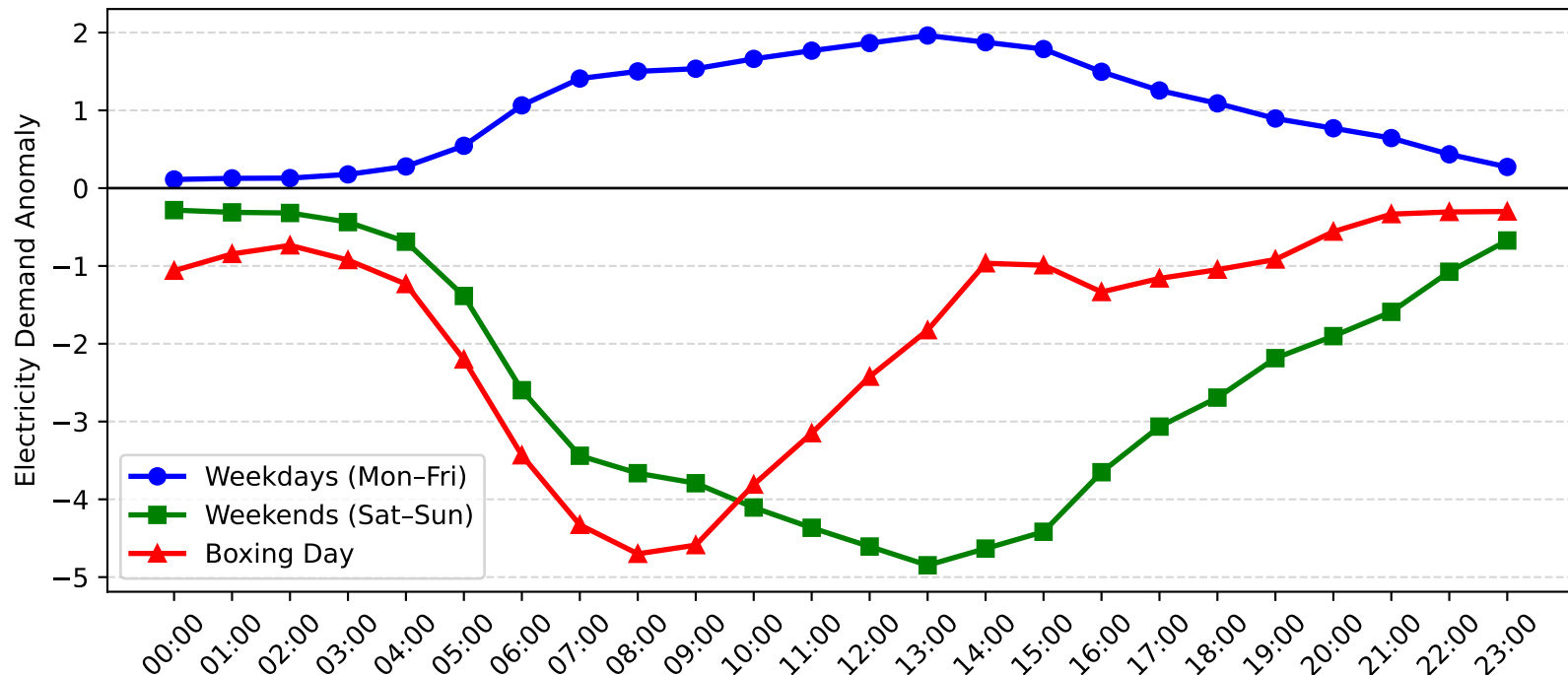
Wyong Demand Anomaly: Boxing Day vs Weekday/Weekend (2015-2016)
