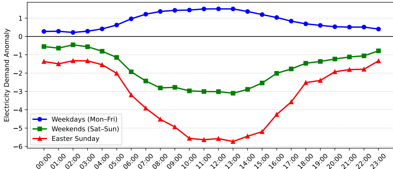
Argenton Demand Anomaly: Easter Sunday vs Weekday/Weekend (2009-2010)
