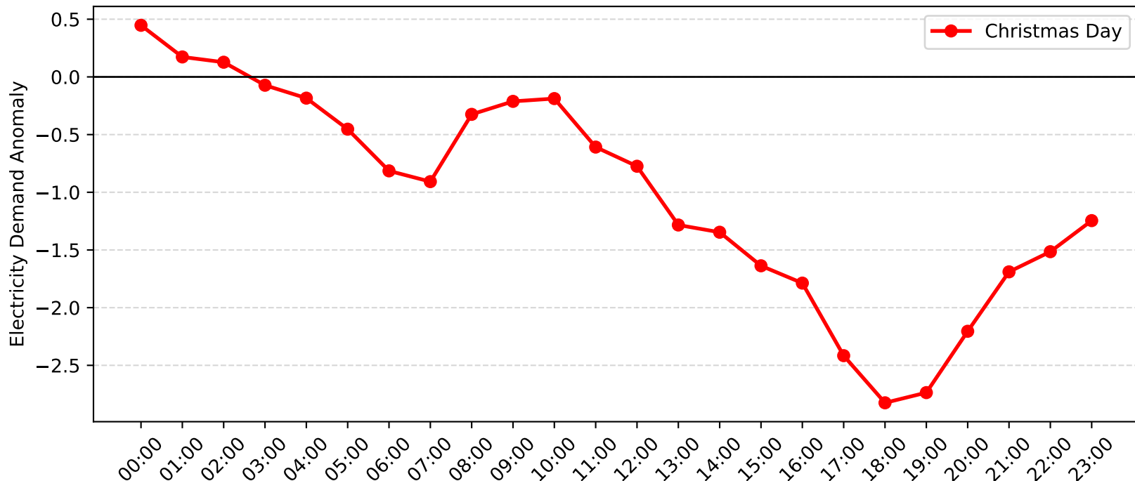
Harbord Demand Anomaly: Christmas Day (2004-2005)
