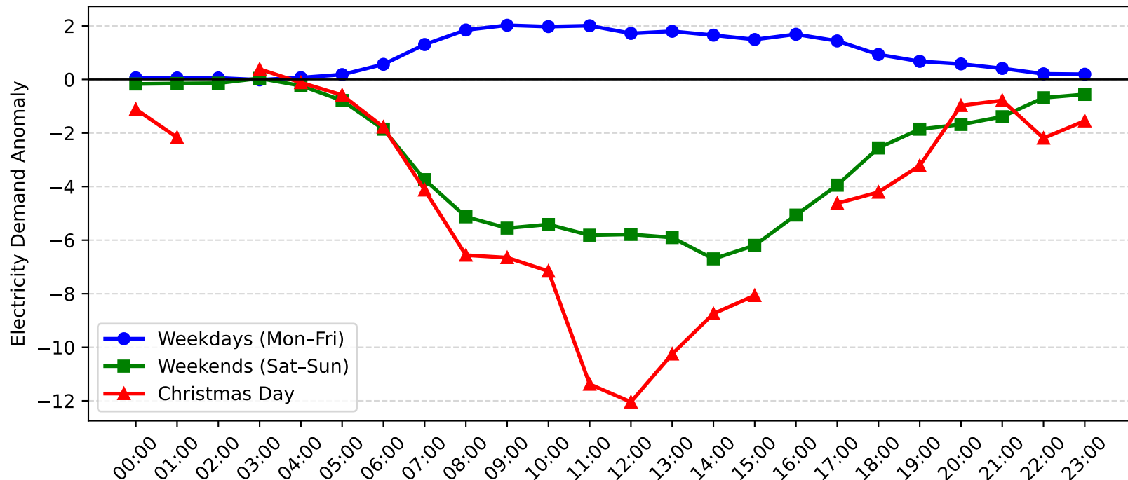
Green Square Demand Anomaly: Christmas Day vs Weekday/Weekend (2012-2013)
