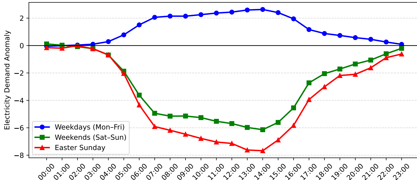
West Gosford Demand Anomaly: Easter Sunday vs Weekday/Weekend (2012-2013)
