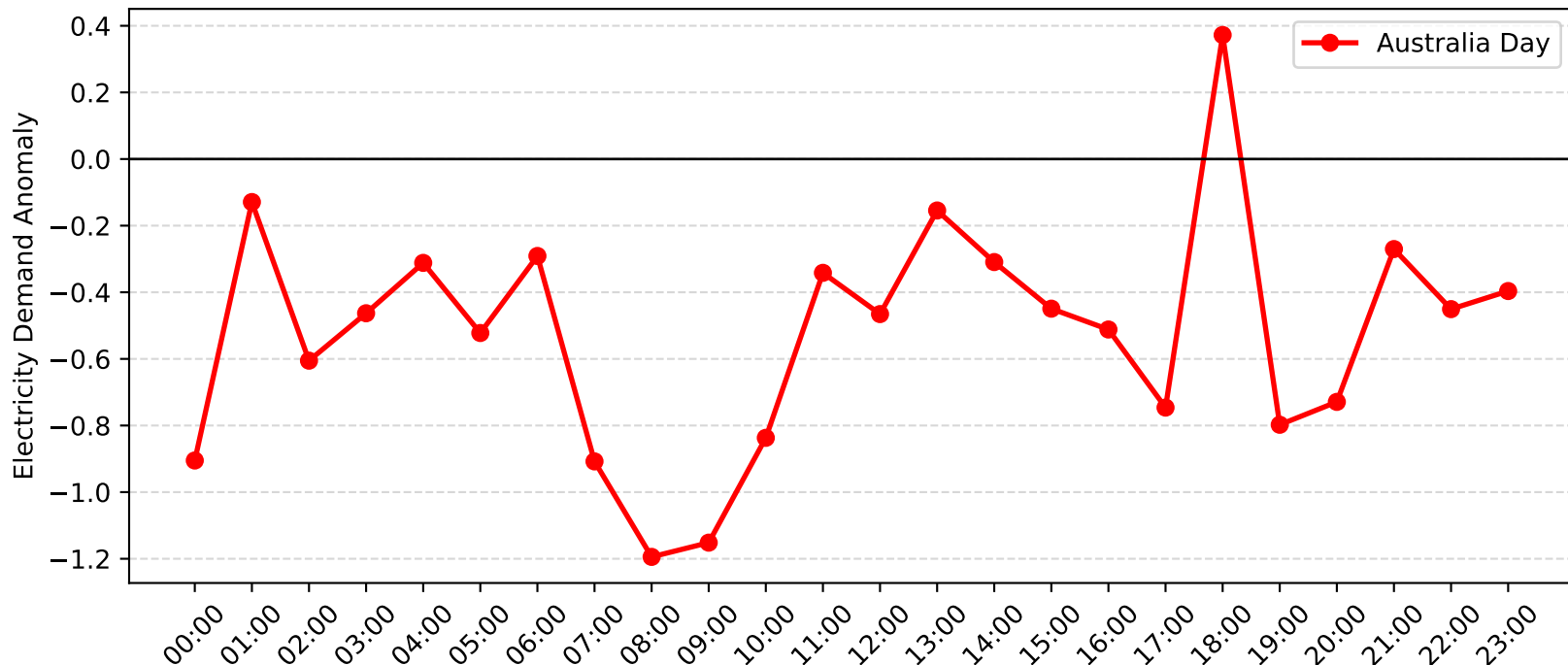
Avoca Demand Anomaly: Australia Day (2004-2005)
