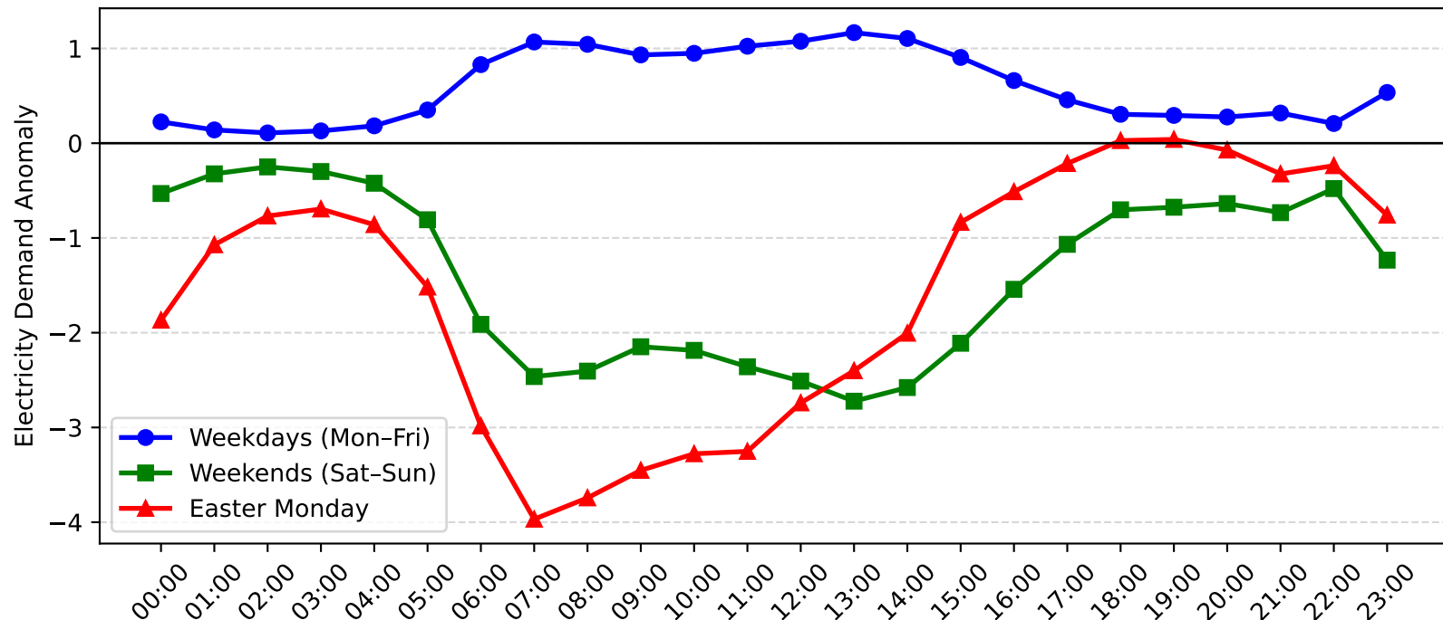
Rutherford Demand Anomaly: Easter Monday vs Weekday/Weekend (2015-2016)
