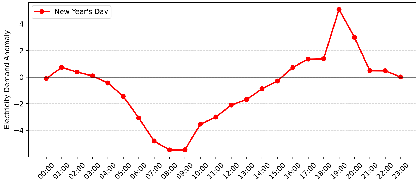
Wyong Demand Anomaly: New Year's Day (2008-2009)
