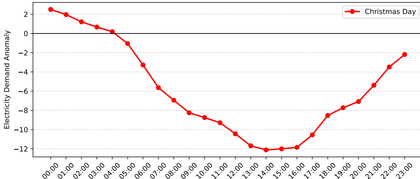
Burwood Demand Anomaly: Christmas Day (2011-2012)
