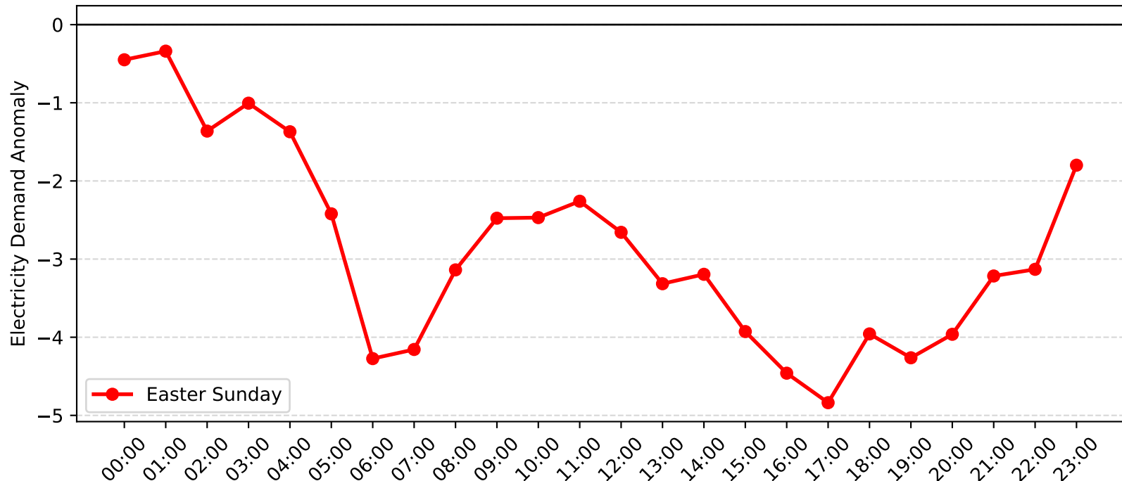
Revesby Demand Anomaly: Easter Sunday (2009-2010)
