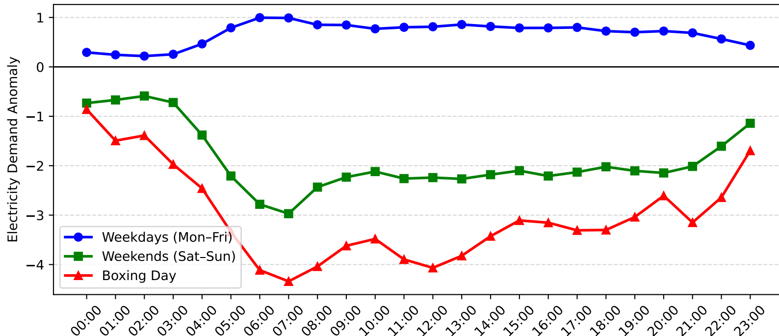
Lisarow Demand Anomaly: Boxing Day vs Weekday/Weekend (2007-2008)
