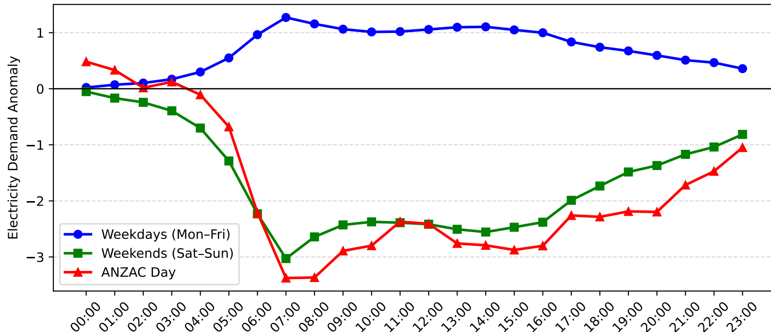
Lidcombe Demand Anomaly: ANZAC Day vs Weekday/Weekend (2008-2009)
