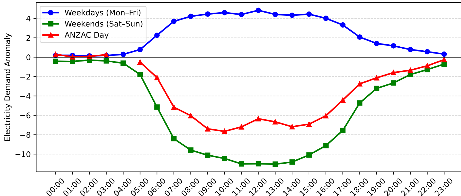
Macquarie Park Demand Anomaly: ANZAC Day vs Weekday/Weekend (2017-2018)
