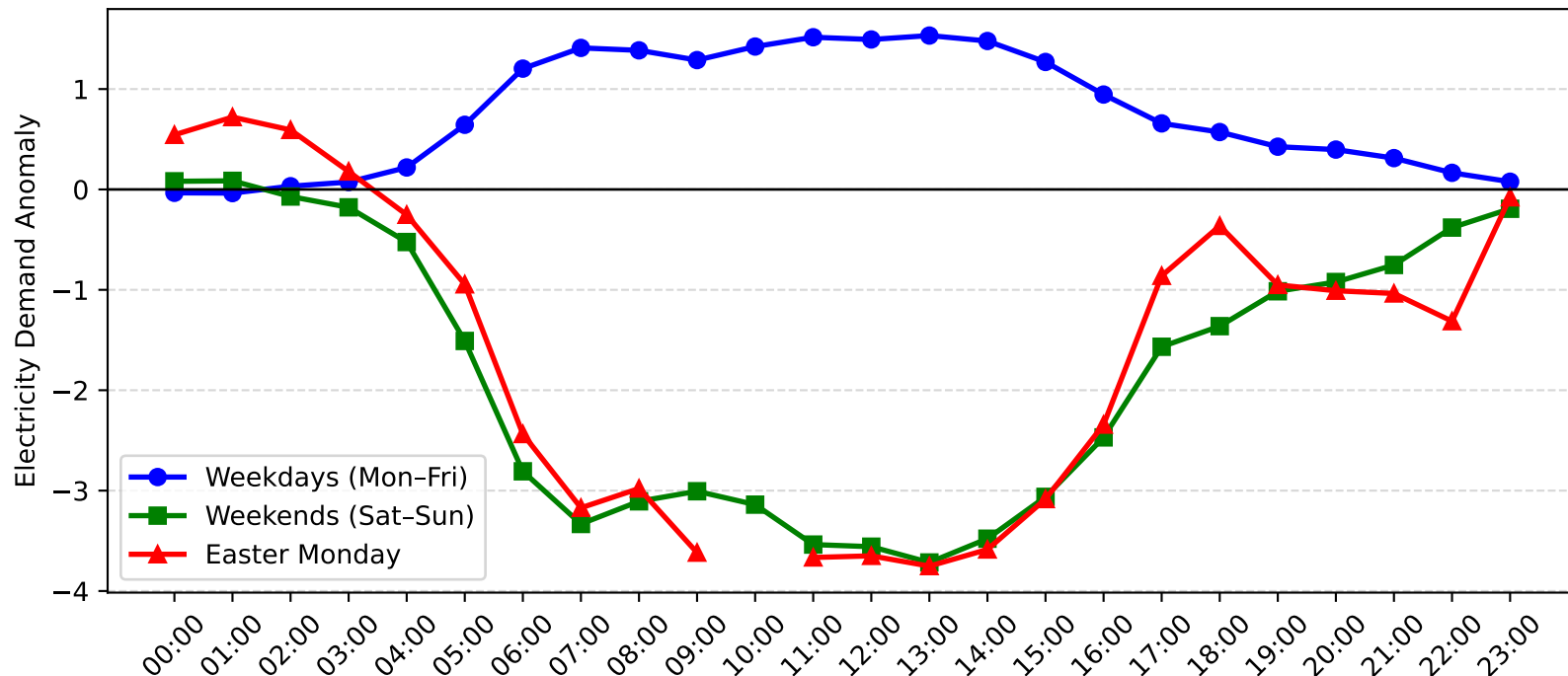
Wyong Demand Anomaly: Easter Monday vs Weekday/Weekend (2005-2006)
