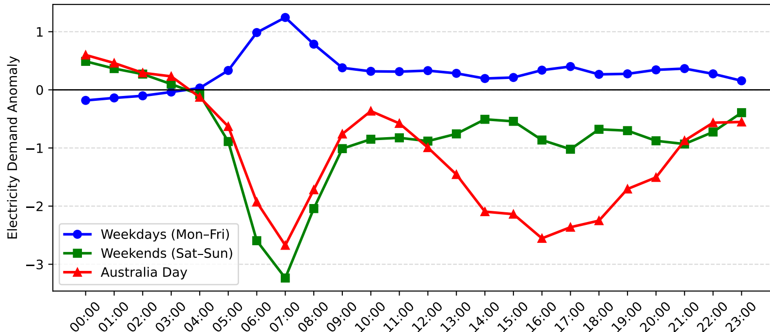
Dulwich Hill Demand Anomaly: Australia Day vs Weekday/Weekend (2015-2016)
