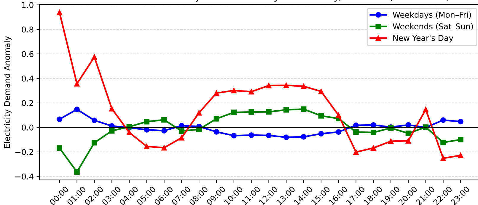
Swansea Demand Anomaly: New Year's Day vs Weekday/Weekend (2004-2005)
