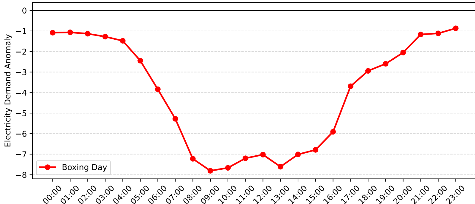
Auburn Demand Anomaly: Boxing Day (2014-2015)
