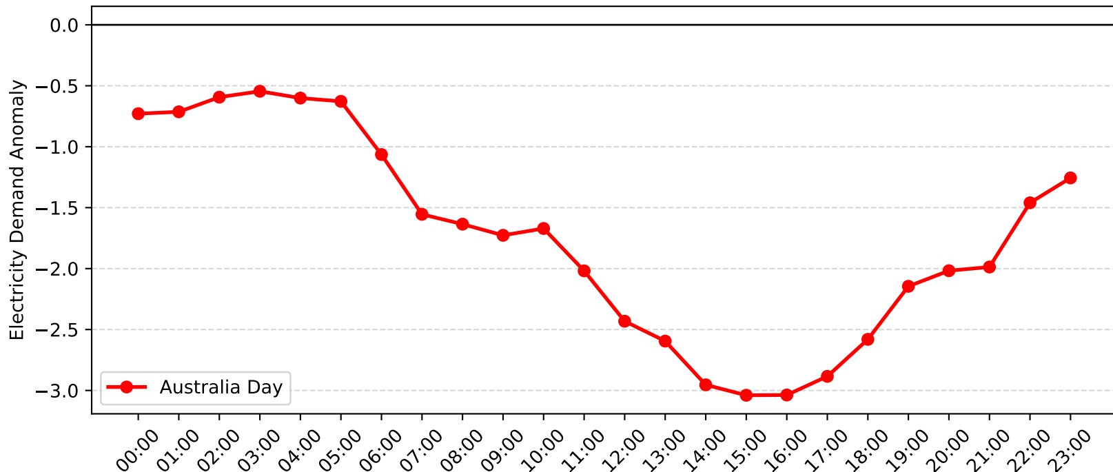
Rockdale Demand Anomaly: Australia Day (2017-2018)
