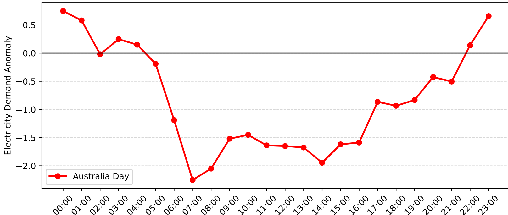
Rockdale Demand Anomaly: Australia Day (2006-2007)
