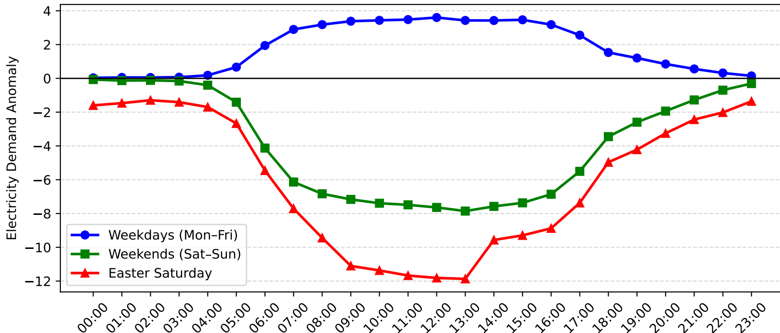
Macquarie Park Demand Anomaly: Easter Saturday vs Weekday/Weekend (2009-2010)
