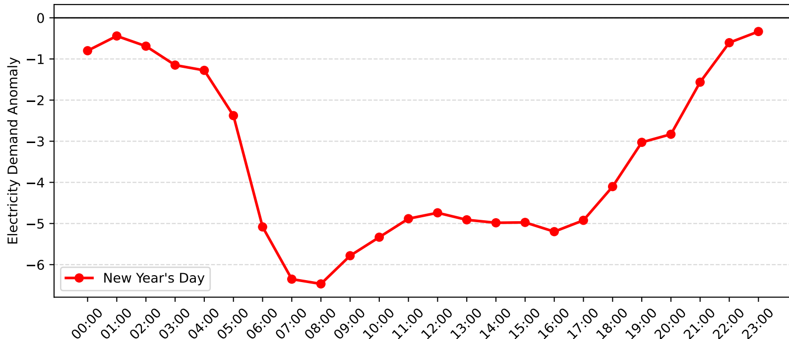
Pymble Demand Anomaly: New Year's Day (2004-2005)
