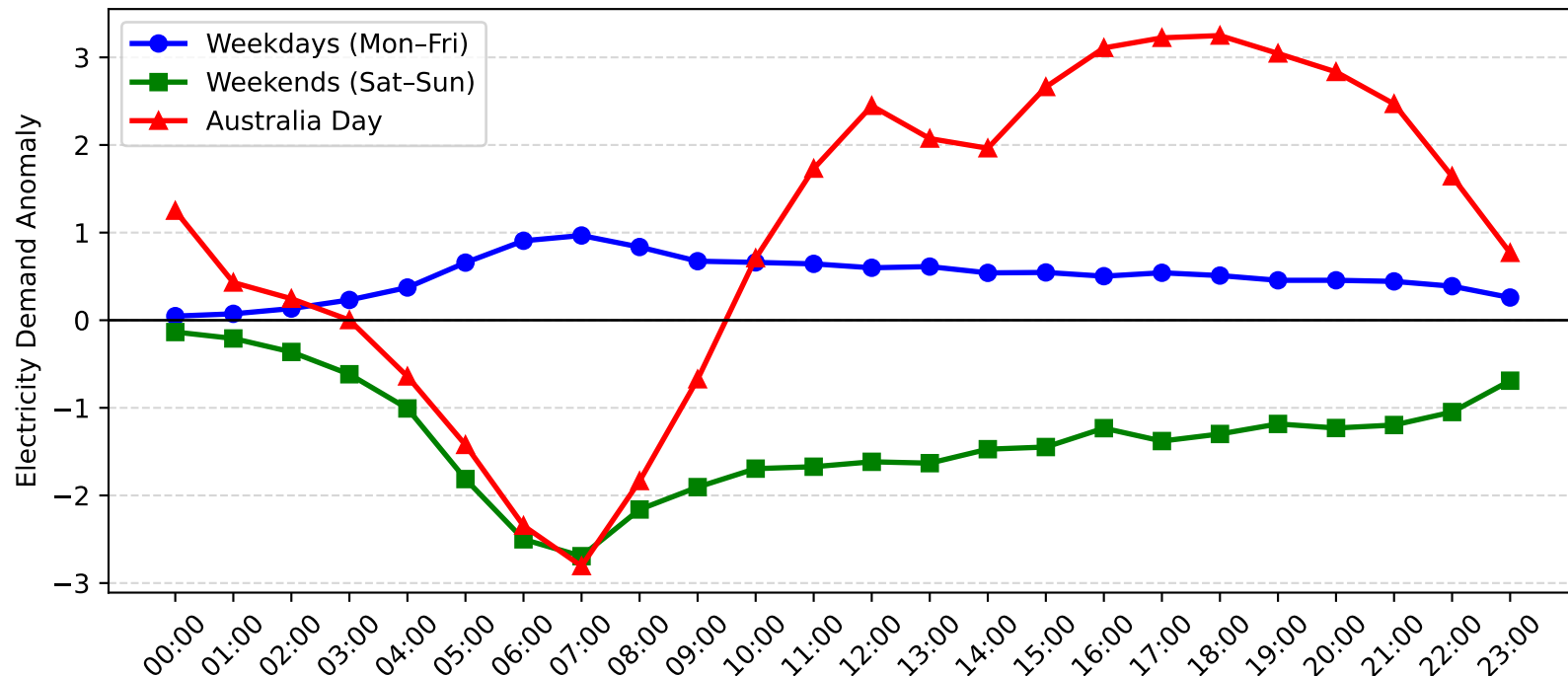
Lisarow Demand Anomaly: Australia Day vs Weekday/Weekend (2010-2011)
