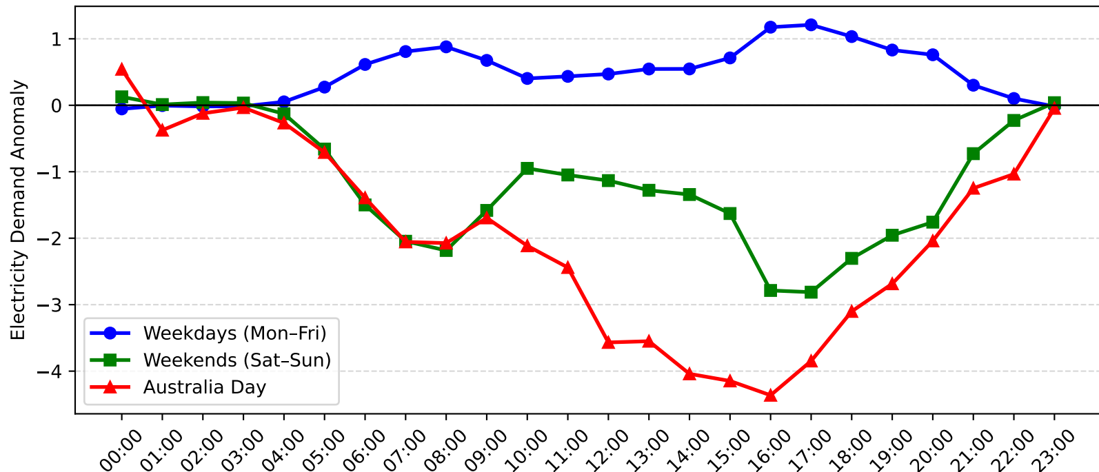
Erina Demand Anomaly: Australia Day vs Weekday/Weekend (2008-2009)
