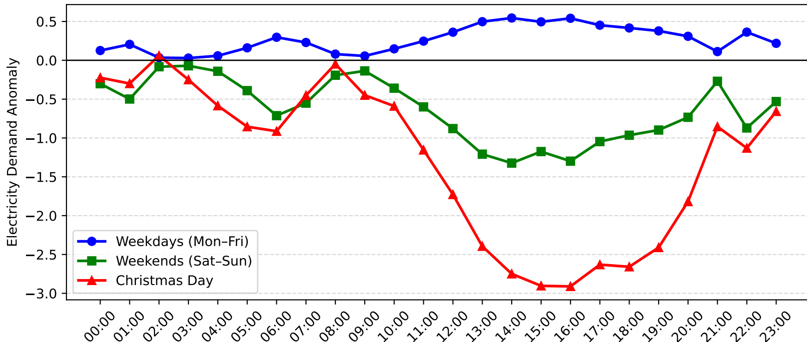
Morisset Demand Anomaly: Christmas Day vs Weekday/Weekend (2015-2016)
