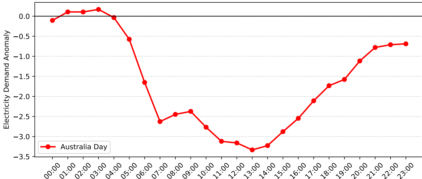
Rutherford Demand Anomaly: Australia Day (2008-2009)
