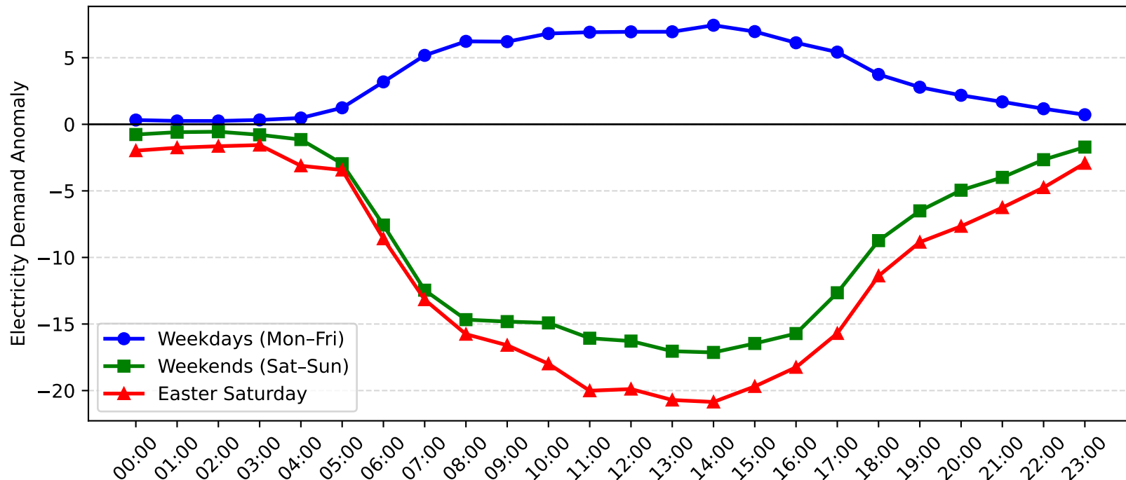
Gore Hill Demand Anomaly: Easter Saturday vs Weekday/Weekend (2006-2007)
