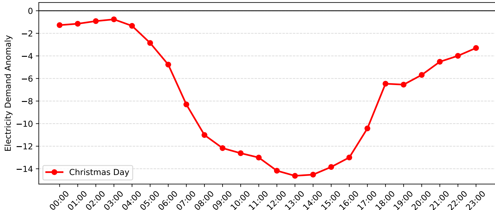
Gore Hill Demand Anomaly: Christmas Day (2015-2016)
