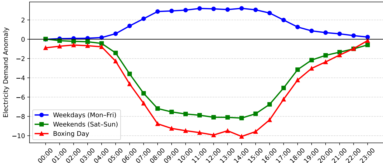
Mascot Demand Anomaly: Boxing Day vs Weekday/Weekend (2014-2015)
