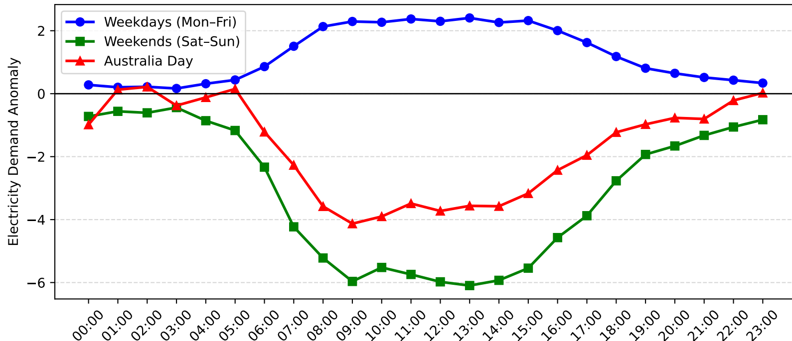
Green Square Demand Anomaly: Australia Day vs Weekday/Weekend (2009-2010)
