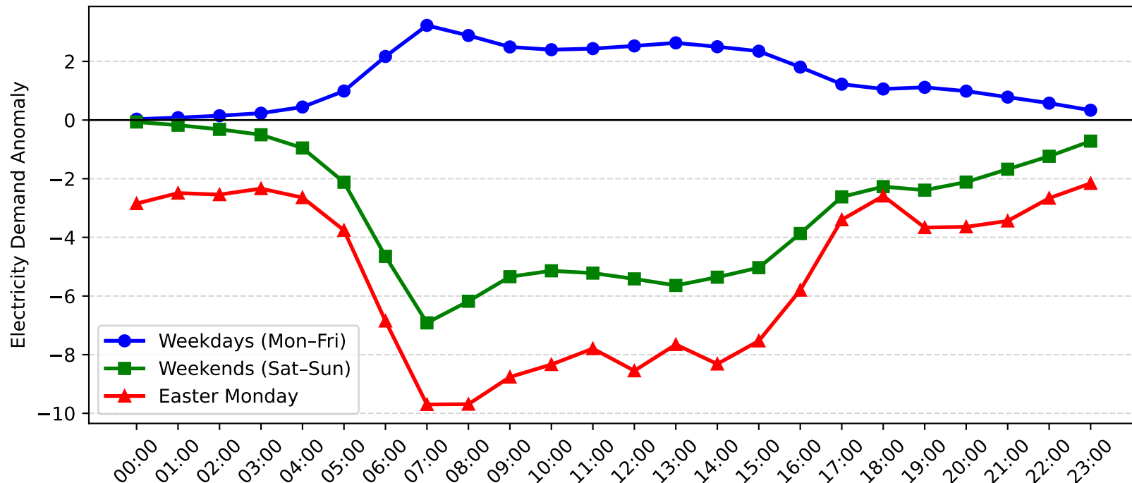
Marrickville Demand Anomaly: Easter Monday vs Weekday/Weekend (2017-2018)
