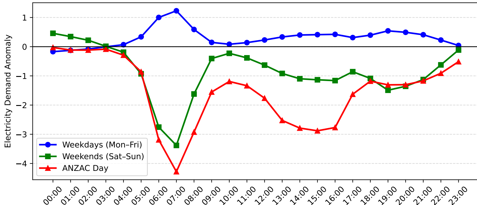
Five Dock Demand Anomaly: ANZAC Day vs Weekday/Weekend (2012-2013)
