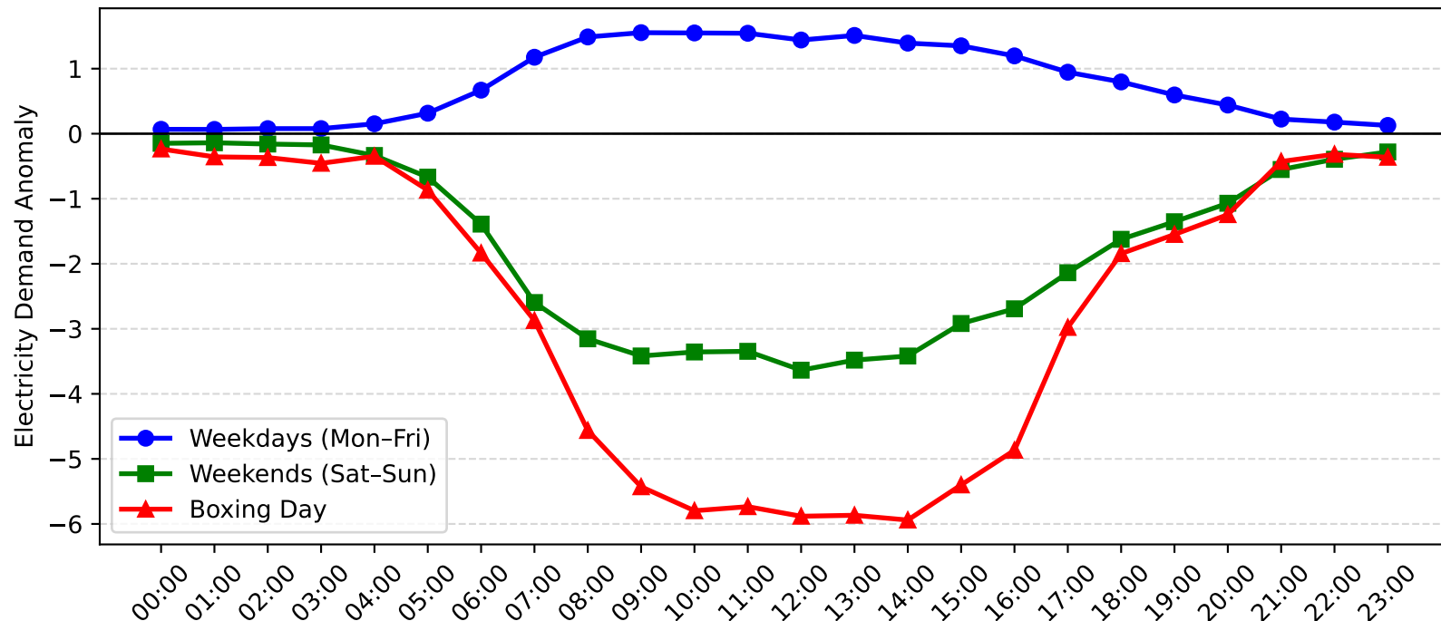
Auburn Demand Anomaly: Boxing Day vs Weekday/Weekend (2004-2005)
