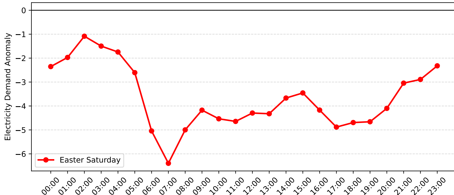
Maroubra Demand Anomaly: Easter Saturday (2010-2011)
