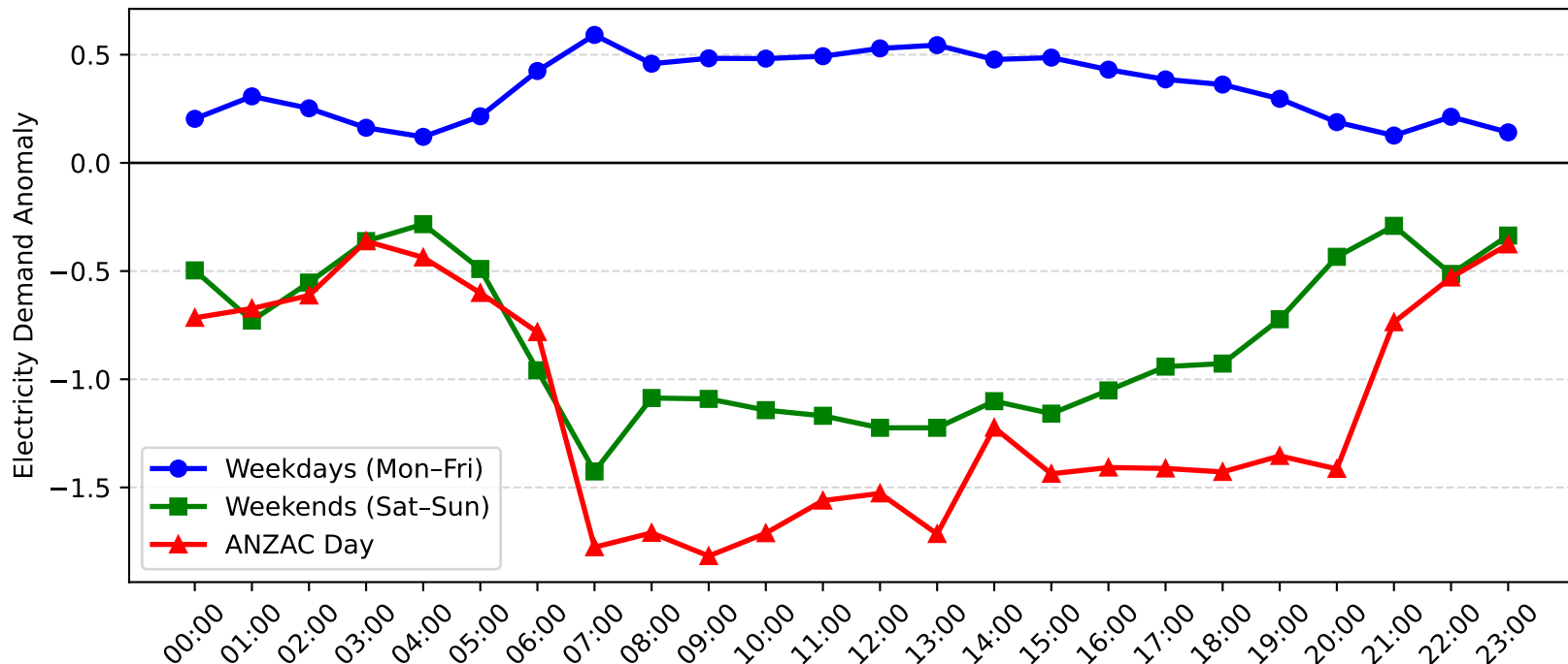
Cardiff Demand Anomaly: ANZAC Day vs Weekday/Weekend (2004-2005)
