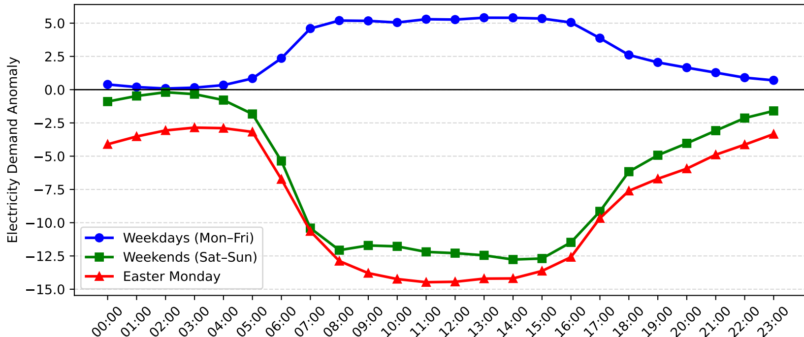
Gore Hill Demand Anomaly: Easter Monday vs Weekday/Weekend (2010-2011)
