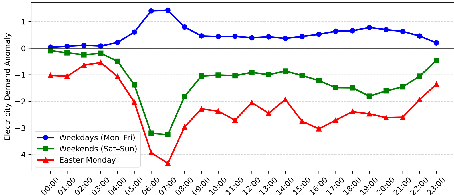
Revesby Demand Anomaly: Easter Monday vs Weekday/Weekend (2015-2016)
