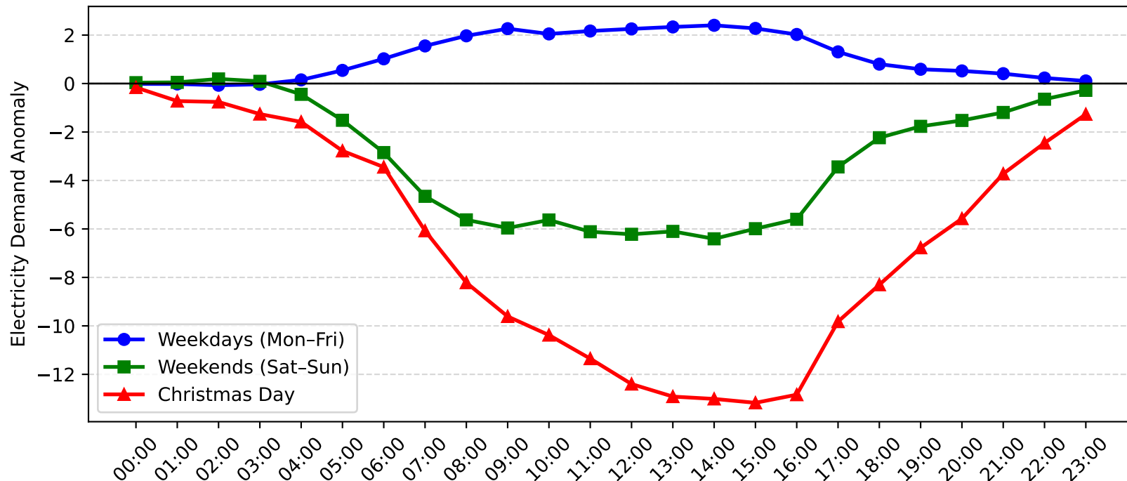
West Gosford Demand Anomaly: Christmas Day vs Weekday/Weekend (2007-2008)
