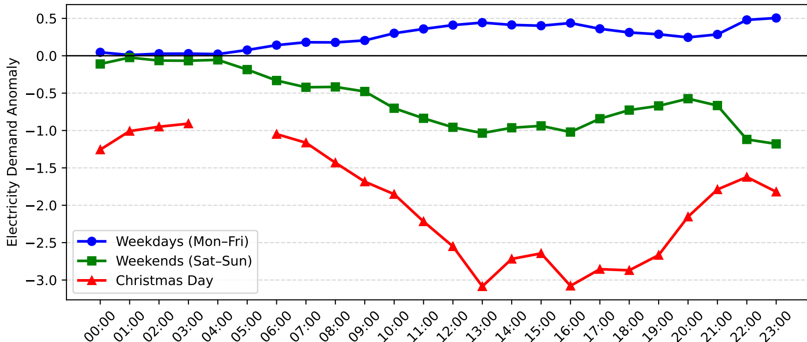
Muswellbrook Demand Anomaly: Christmas Day vs Weekday/Weekend (2016-2017)
