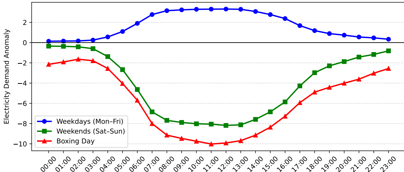
Homebush Bay Demand Anomaly: Boxing Day vs Weekday/Weekend (2011-2012)
