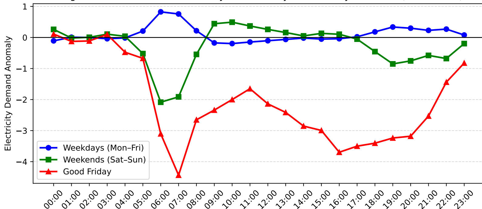
Balgowlah North Demand Anomaly: Good Friday vs Weekday/Weekend (2013-2014)
