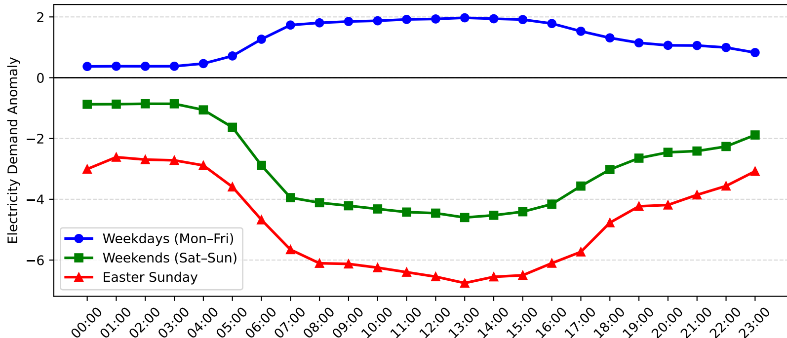
Leightonfield Demand Anomaly: Easter Sunday vs Weekday/Weekend (2015-2016)
