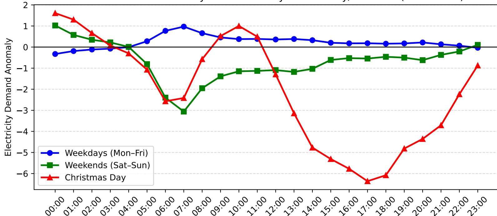
Mortdale Demand Anomaly: Christmas Day vs Weekday/Weekend (2013-2014)
