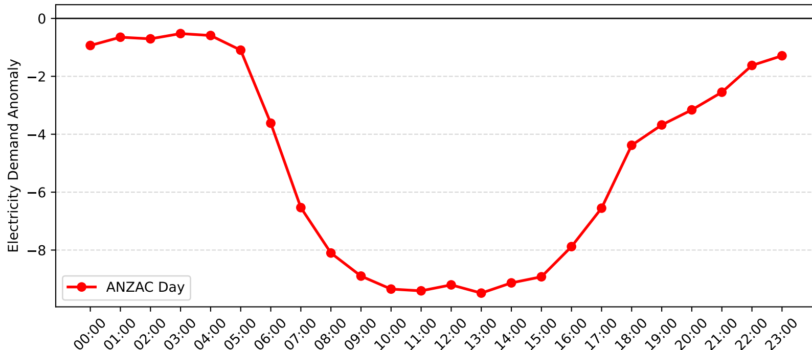
Macquarie Park Demand Anomaly: ANZAC Day (2011-2012)
