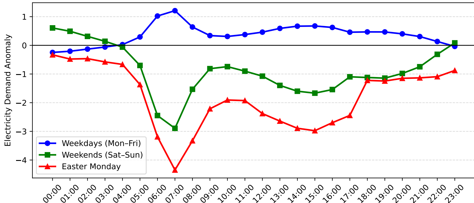
Five Dock Demand Anomaly: Easter Monday vs Weekday/Weekend (2007-2008)
