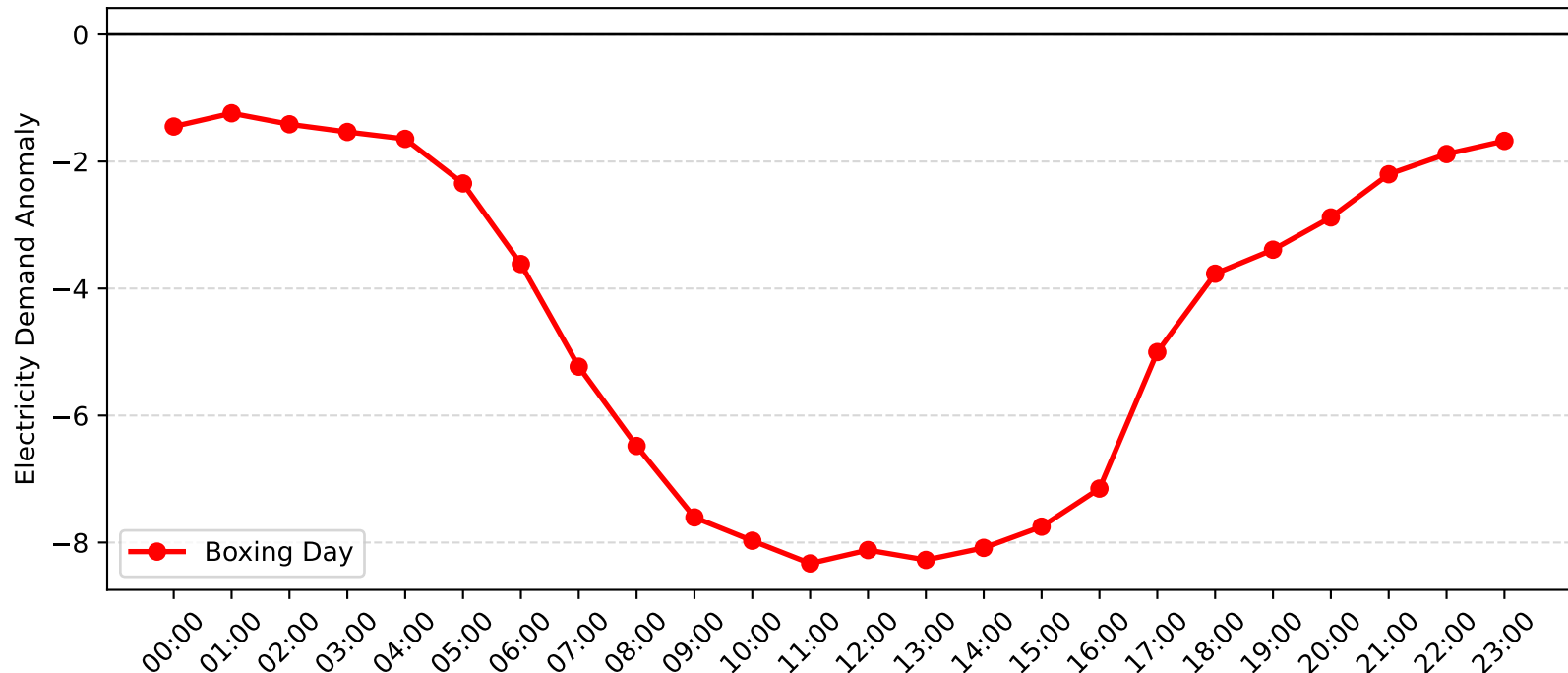
Auburn Demand Anomaly: Boxing Day (2011-2012)
