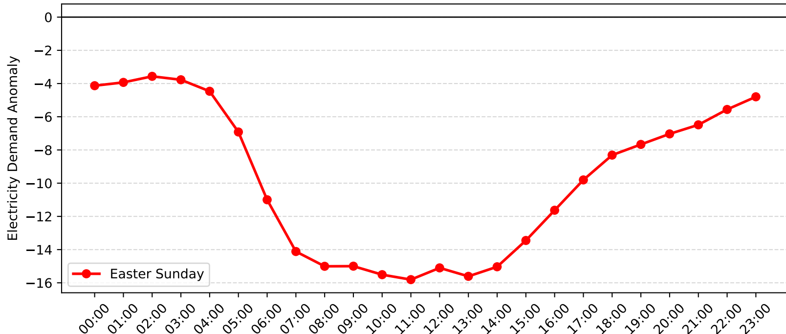
Milperra Demand Anomaly: Easter Sunday (2012-2013)
