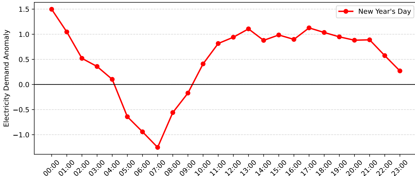
Noraville Demand Anomaly: New Year's Day (2011-2012)
