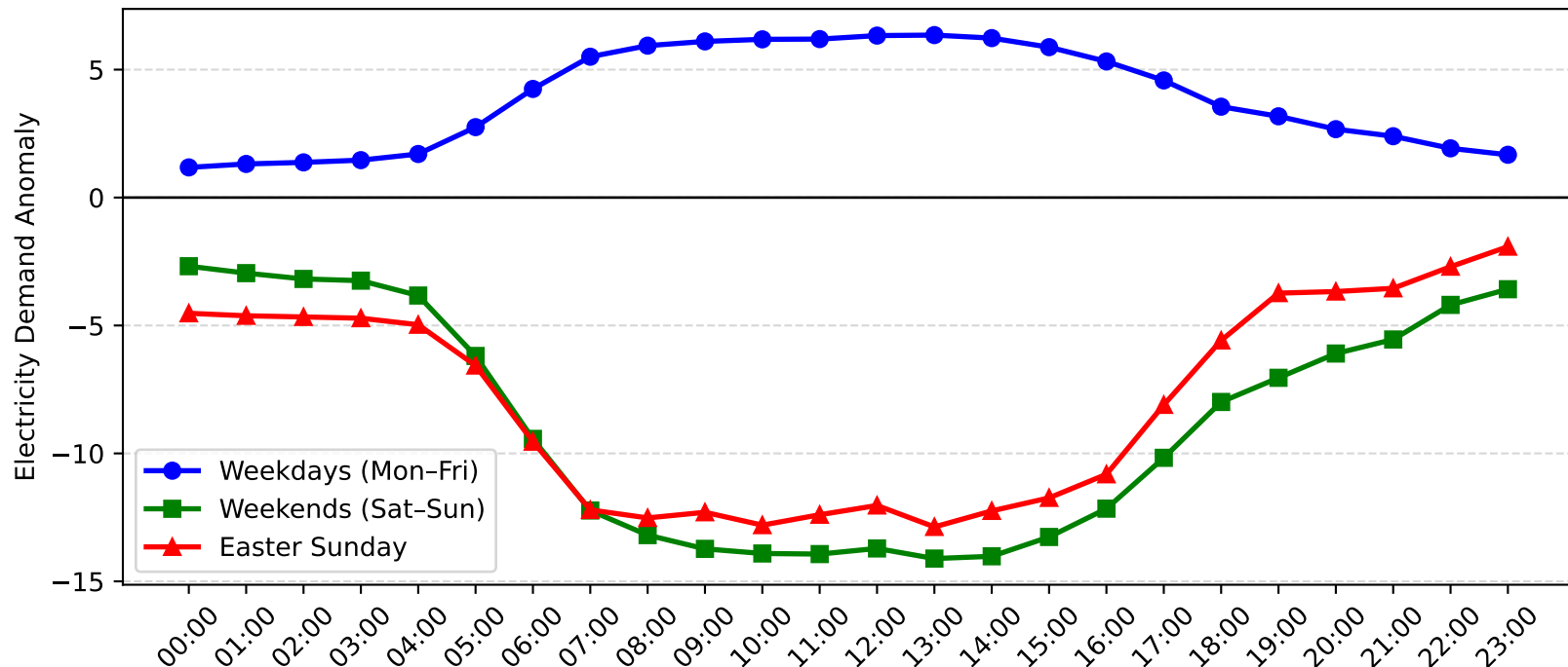
Flemington Demand Anomaly: Easter Sunday vs Weekday/Weekend (2008-2009)
