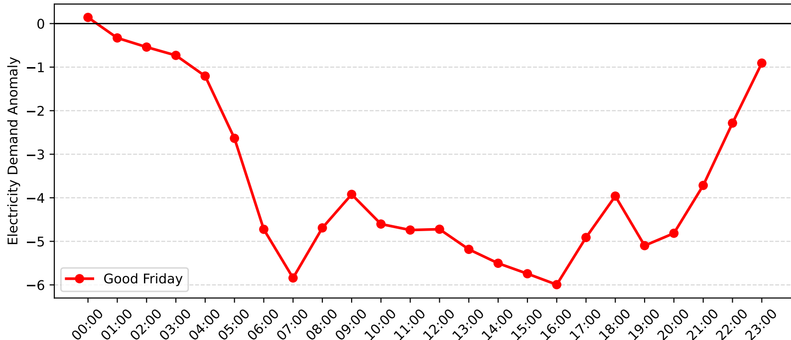
Campsie Demand Anomaly: Good Friday (2017-2018)
