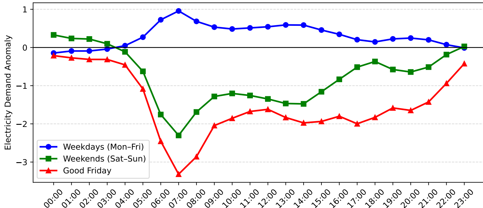
Arnccliffe Demand Anomaly: Good Friday vs Weekday/Weekend (2010-2011)
