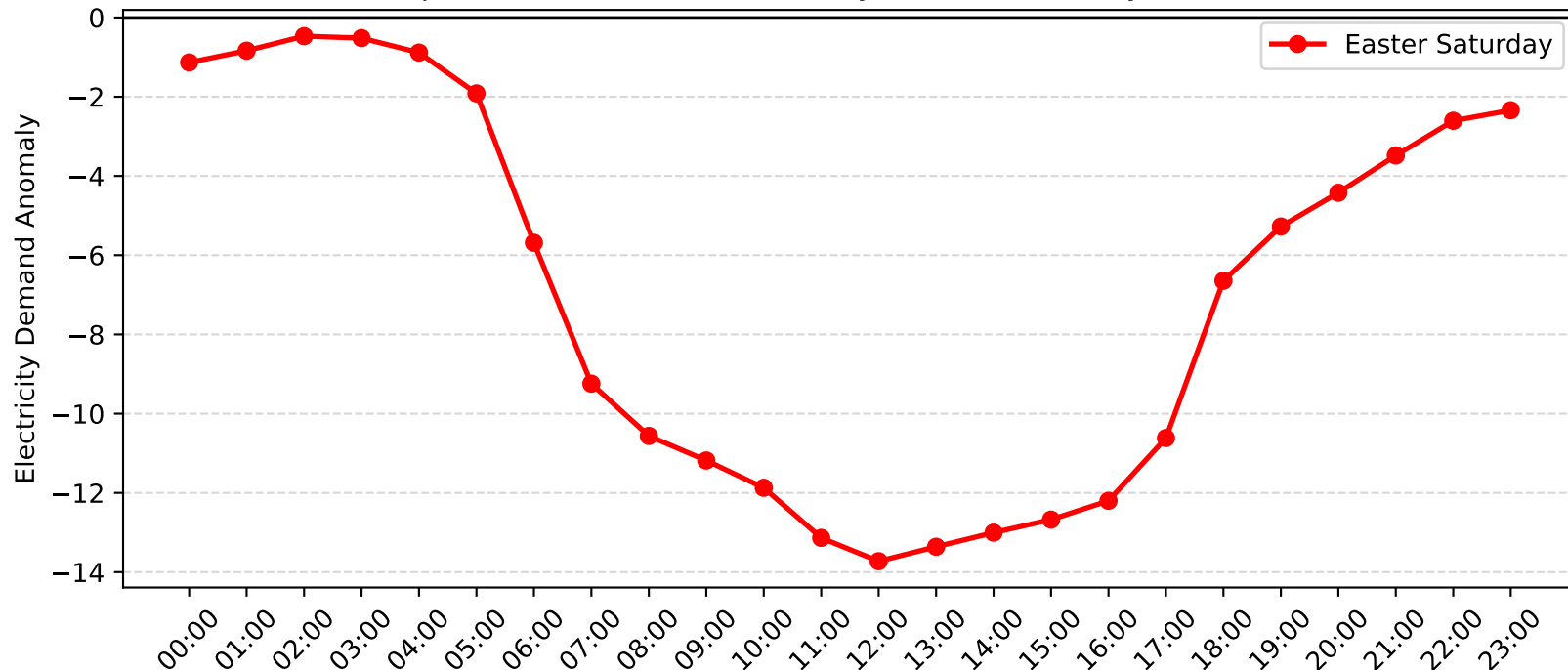
Macquarie Park Demand Anomaly: Easter Saturday (2014-2015)
