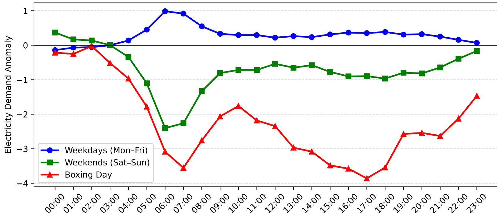
Revesby Demand Anomaly: Boxing Day vs Weekday/Weekend (2011-2012)
