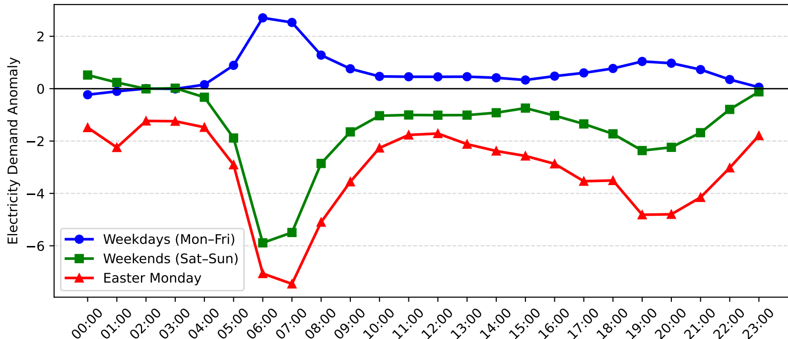
Pennant Hills Demand Anomaly: Easter Monday vs Weekday/Weekend (2010-2011)
