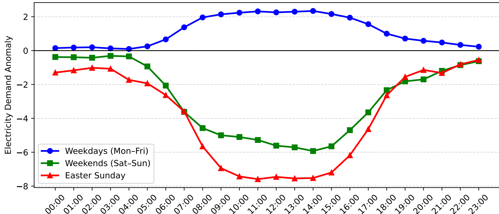
Green Square Demand Anomaly: Easter Sunday vs Weekday/Weekend (2012-2013)
