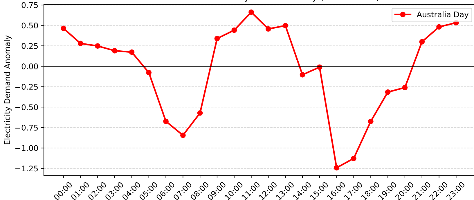
Erina Demand Anomaly: Australia Day (2012-2013)
