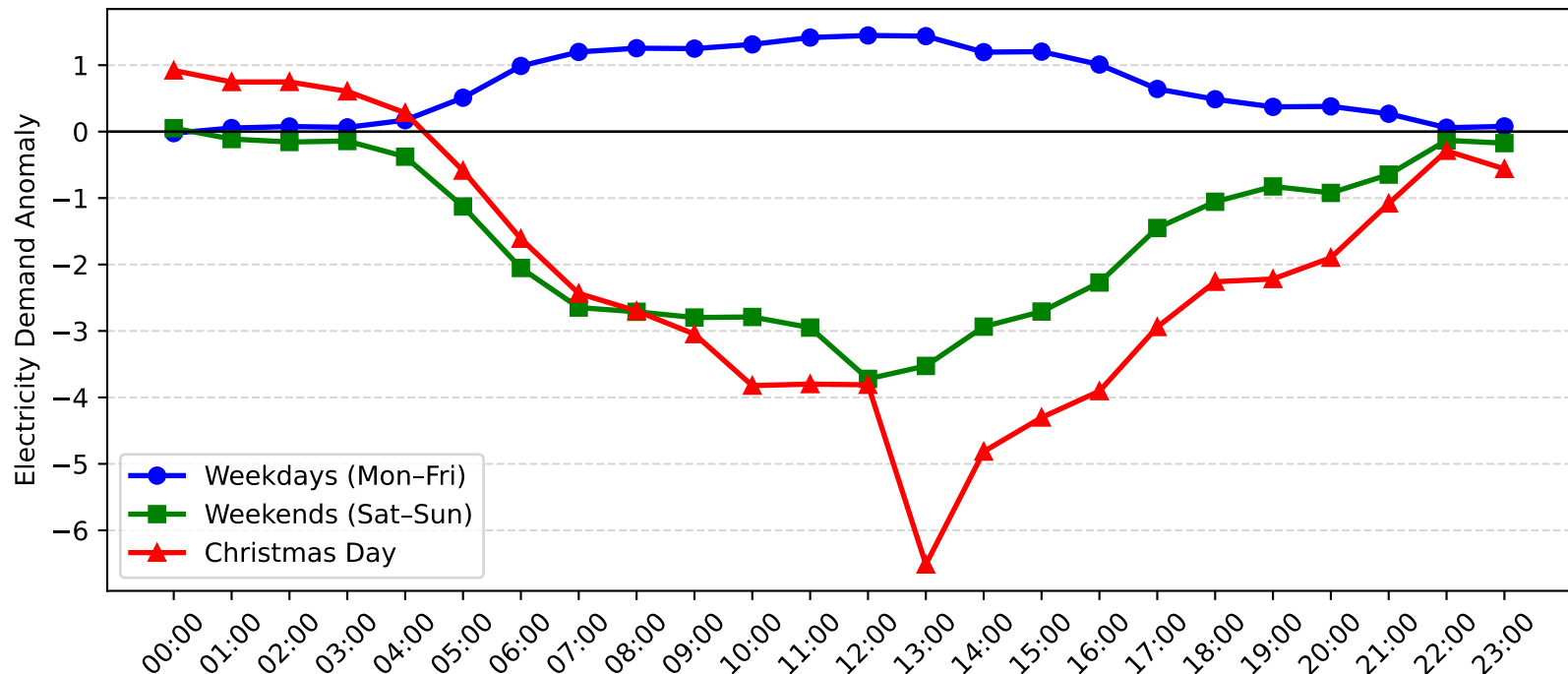
Wyong Demand Anomaly: Christmas Day vs Weekday/Weekend (2004-2005)
