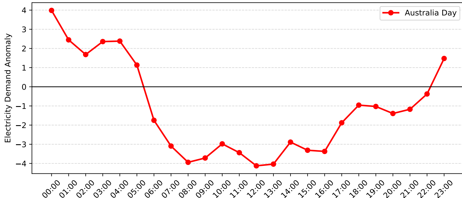
Greenacre Park Demand Anomaly: Australia Day (2012-2013)
