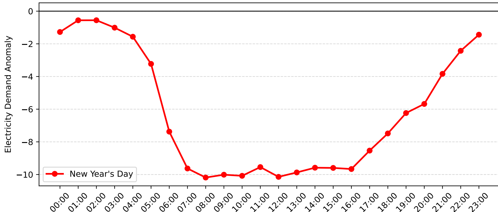
Burwood Demand Anomaly: New Year's Day (2004-2005)
