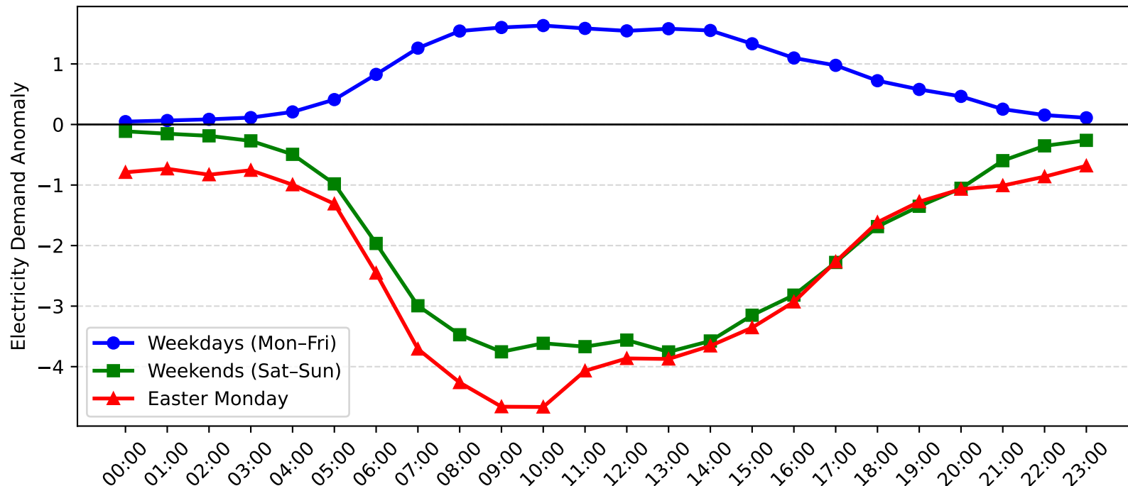
Auburn Demand Anomaly: Easter Monday vs Weekday/Weekend (2006-2007)
