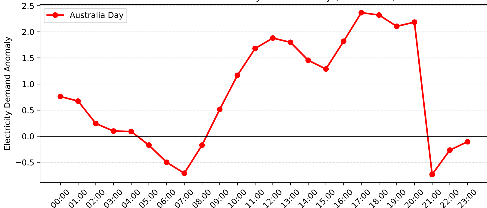
Morisset Demand Anomaly: Australia Day (2011-2012)
