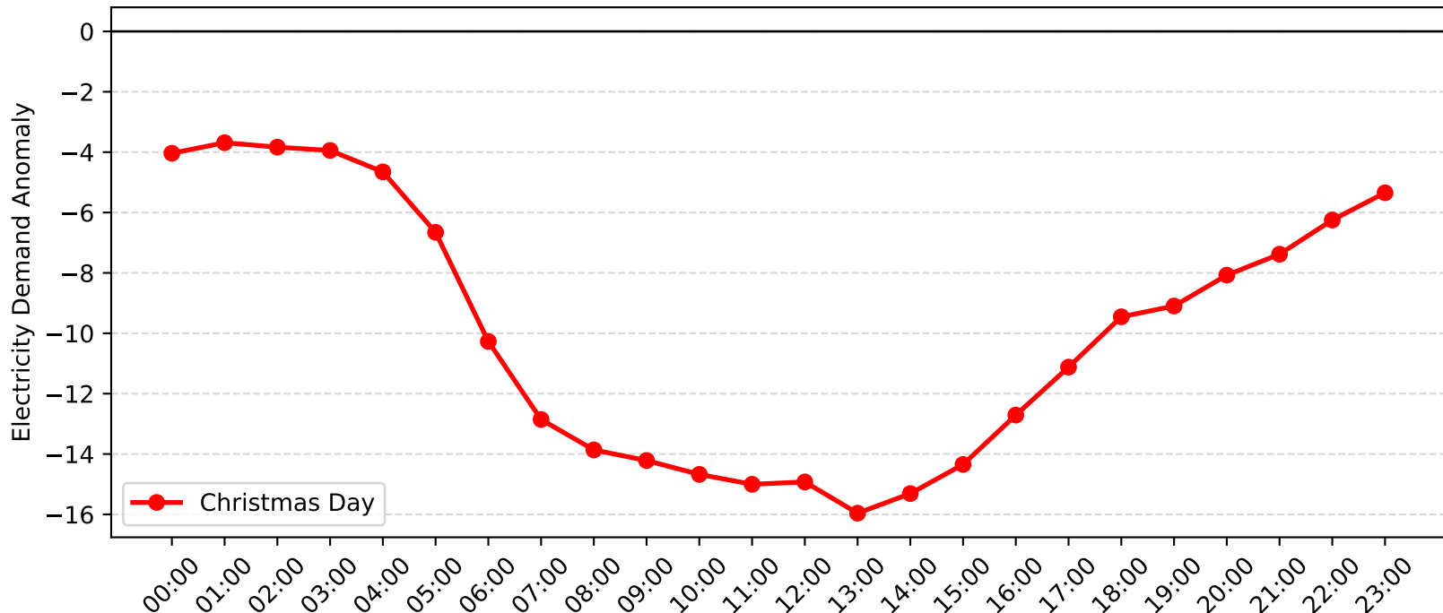
Milperra Demand Anomaly: Christmas Day (2006-2007)
