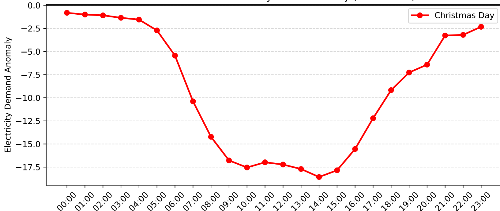
Brookvale Demand Anomaly: Christmas Day (2007-2008)
