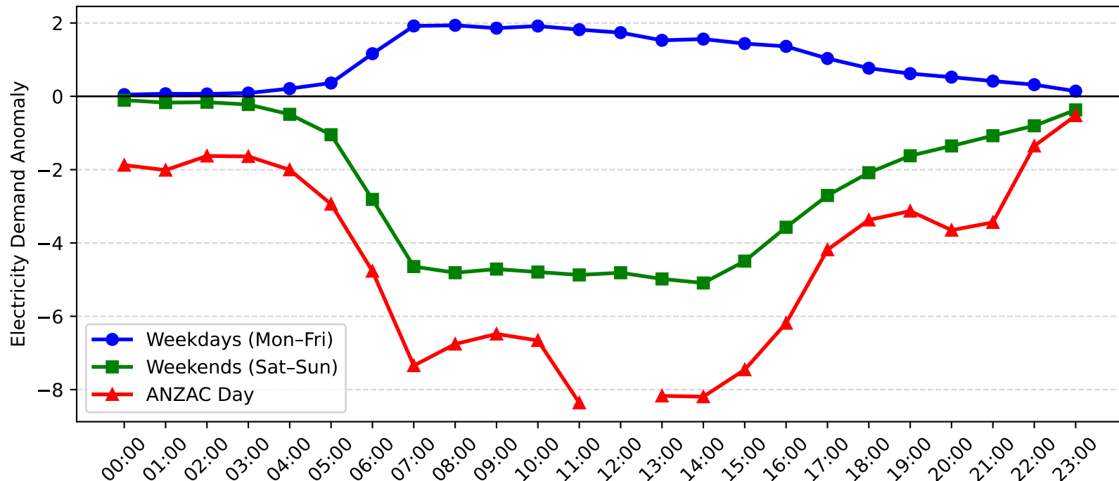
Bankstown Demand Anomaly: ANZAC Day vs Weekday/Weekend (2013-2014)
