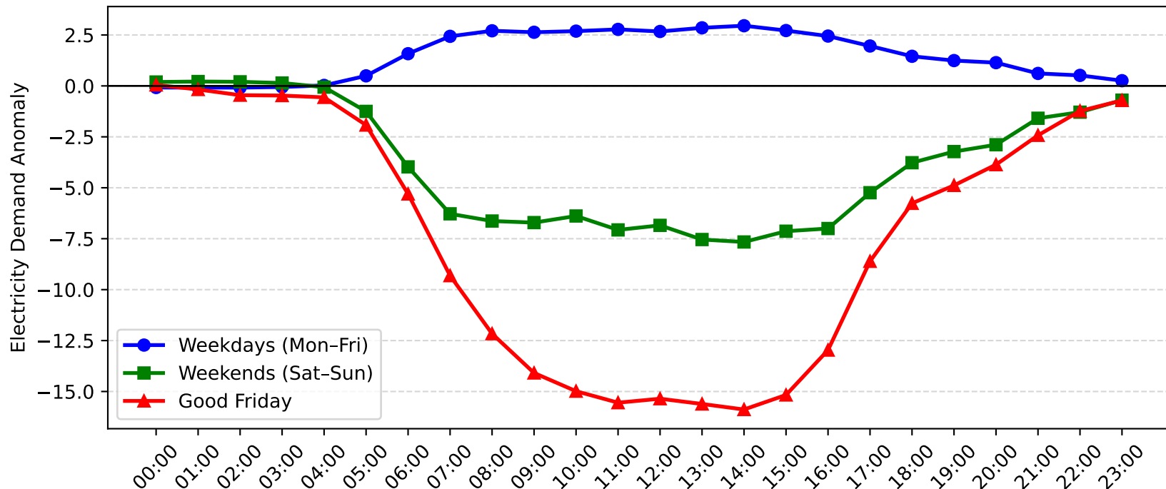
Brookvale Demand Anomaly: Good Friday vs Weekday/Weekend (2005-2006)
