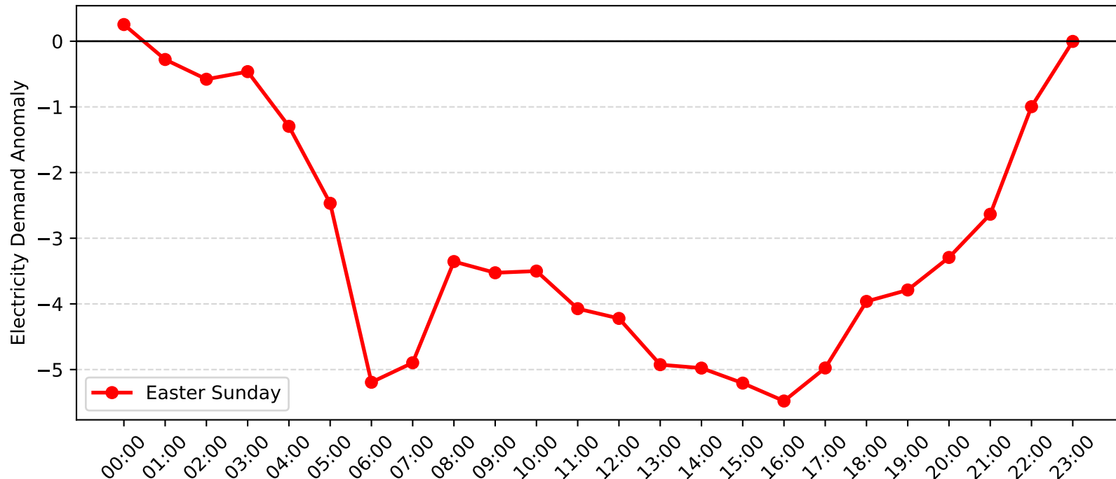
Revesby Demand Anomaly: Easter Sunday (2005-2006)
