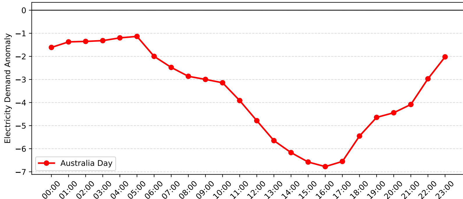
Pymble Demand Anomaly: Australia Day (2017-2018)
