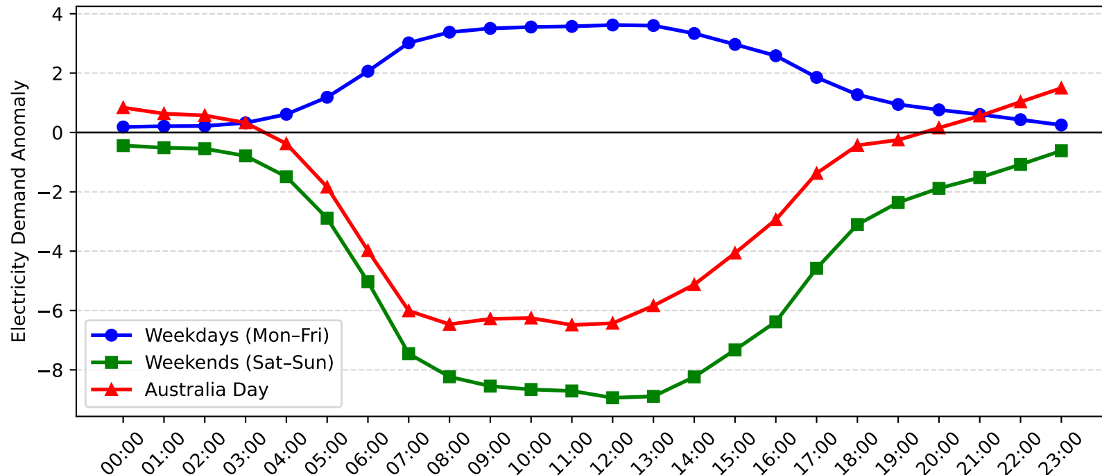
Homebush Bay Demand Anomaly: Australia Day vs Weekday/Weekend (2012-2013)
