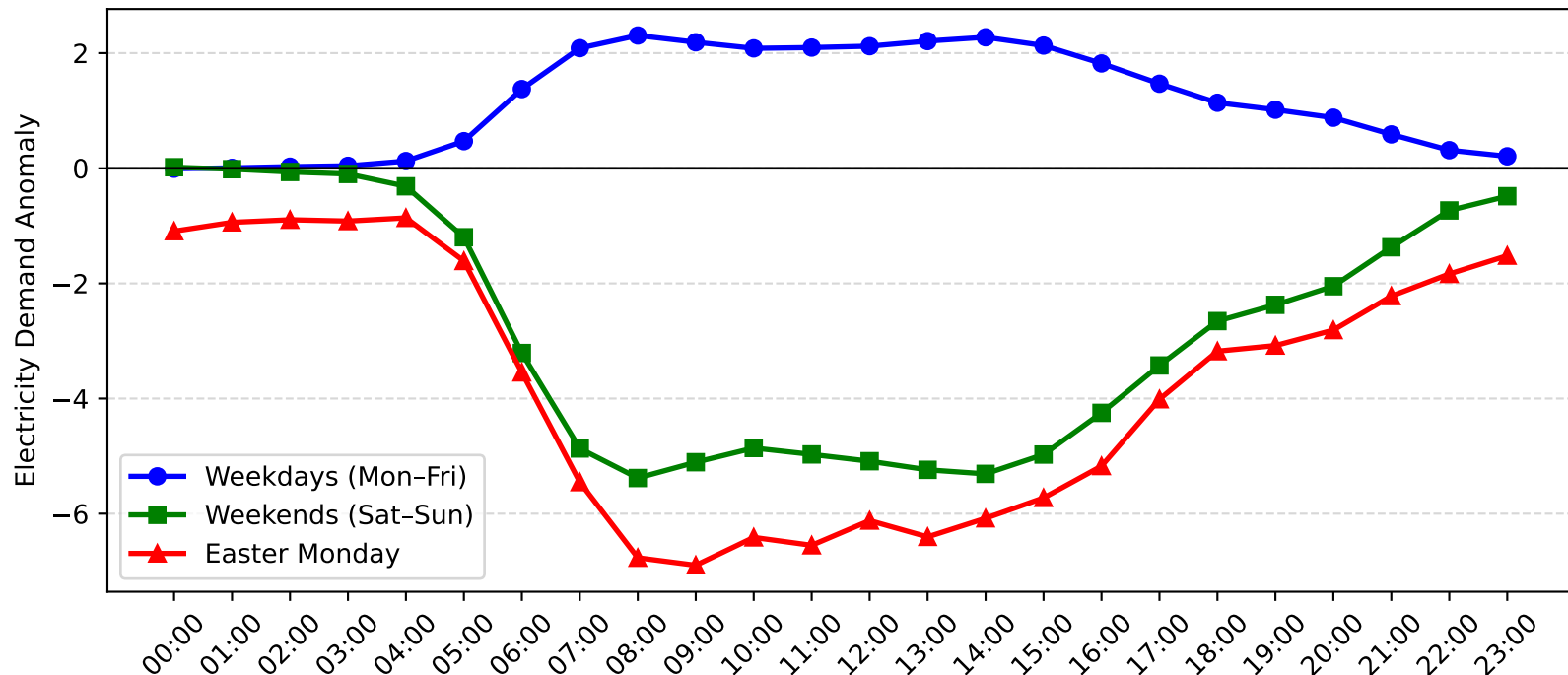
Brookvale Demand Anomaly: Easter Monday vs Weekday/Weekend (2014-2015)
