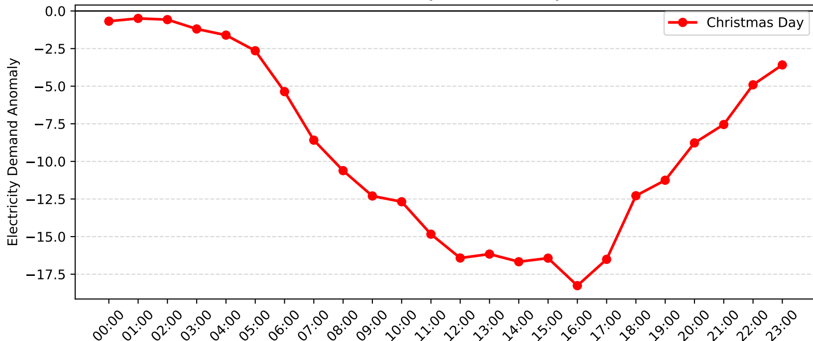
Burwood Demand Anomaly: Christmas Day (2007-2008)
