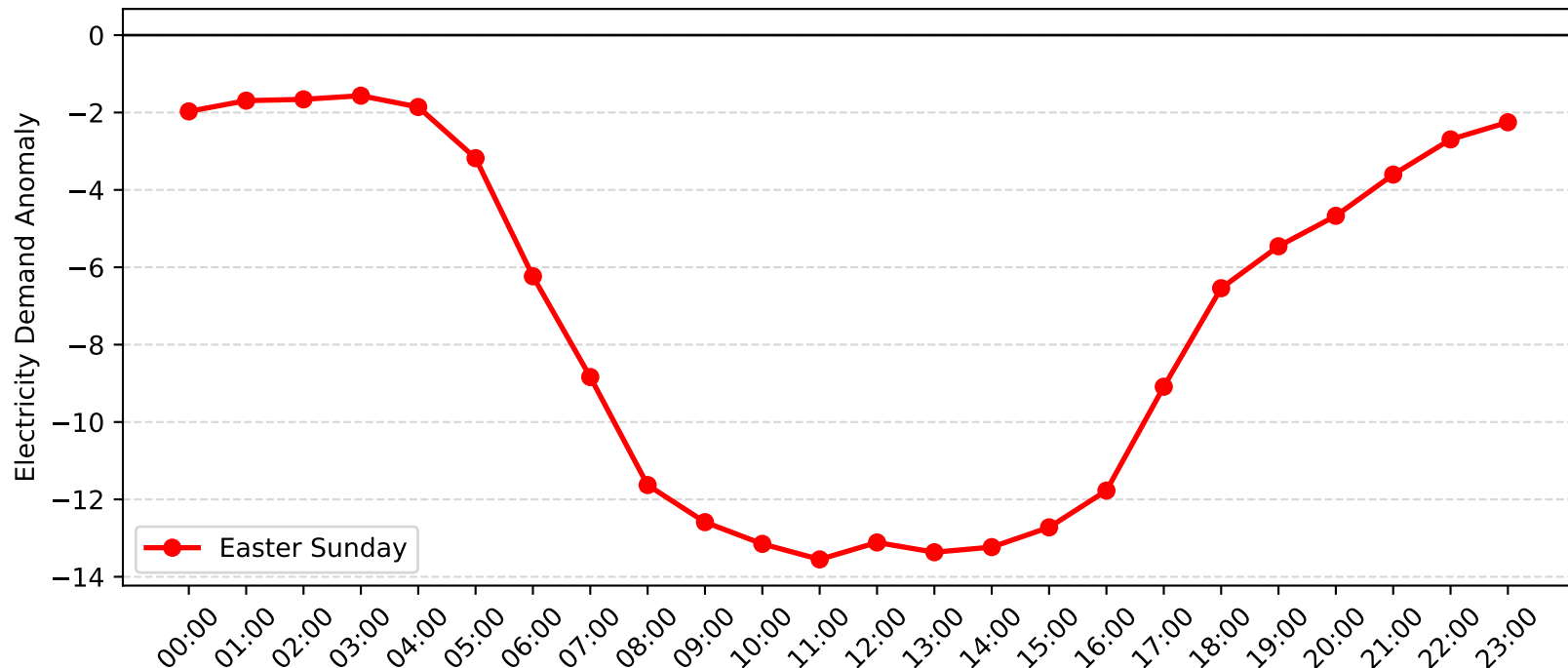
Mascot Demand Anomaly: Easter Sunday (2005-2006)
