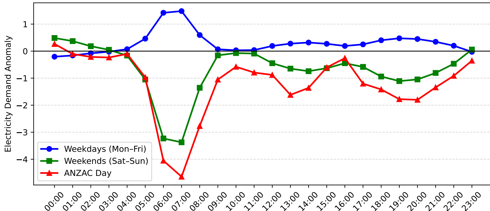
Mortdale Demand Anomaly: ANZAC Day vs Weekday/Weekend (2015-2016)
