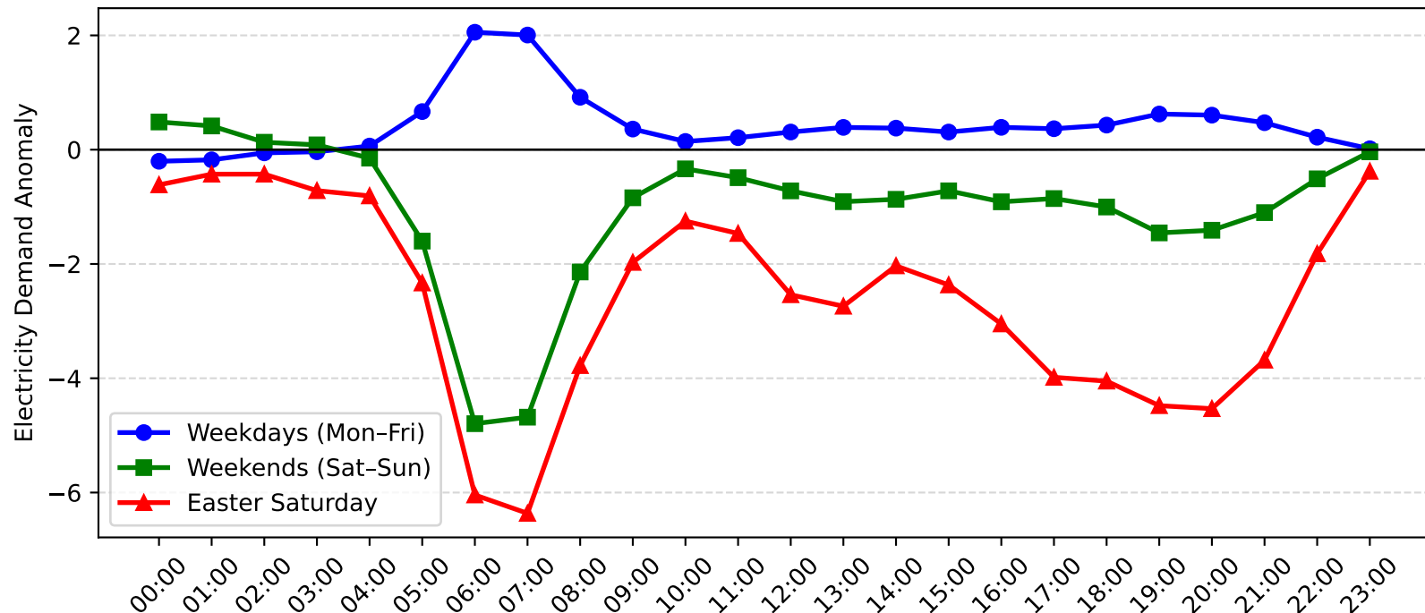
Pennant Hills Demand Anomaly: Easter Saturday vs Weekday/Weekend (2014-2015)
