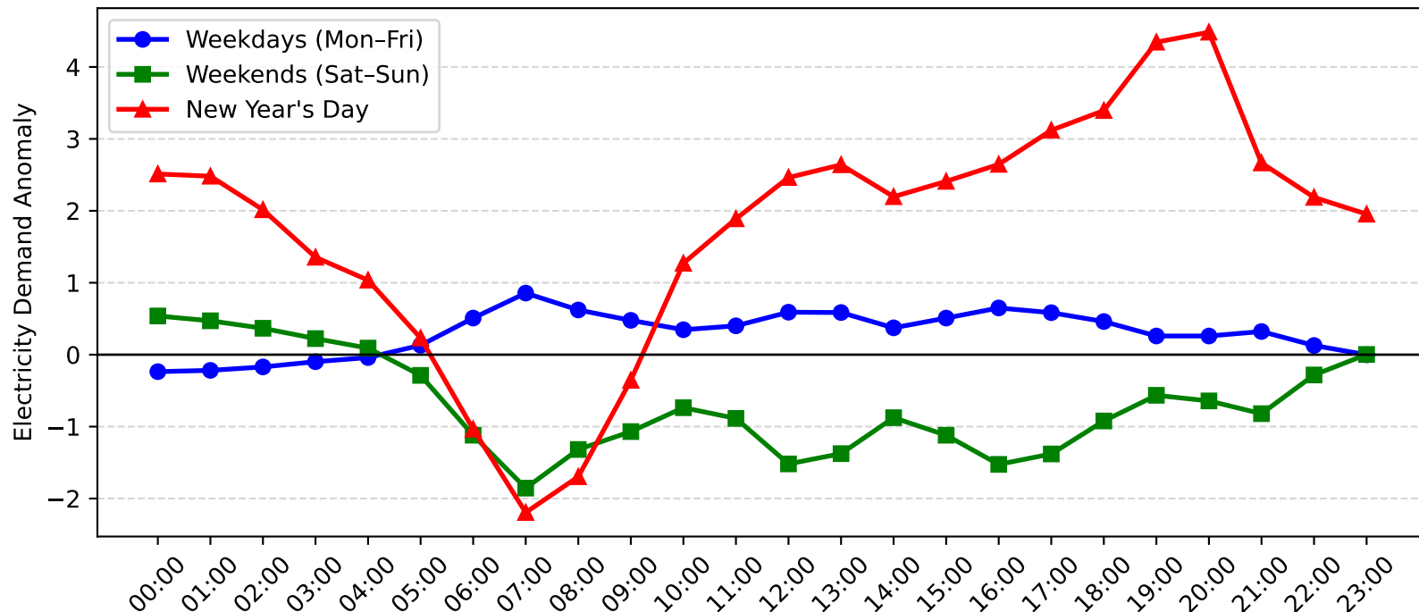
Blakehurst Demand Anomaly: New Year's Day vs Weekday/Weekend (2005-2006)
