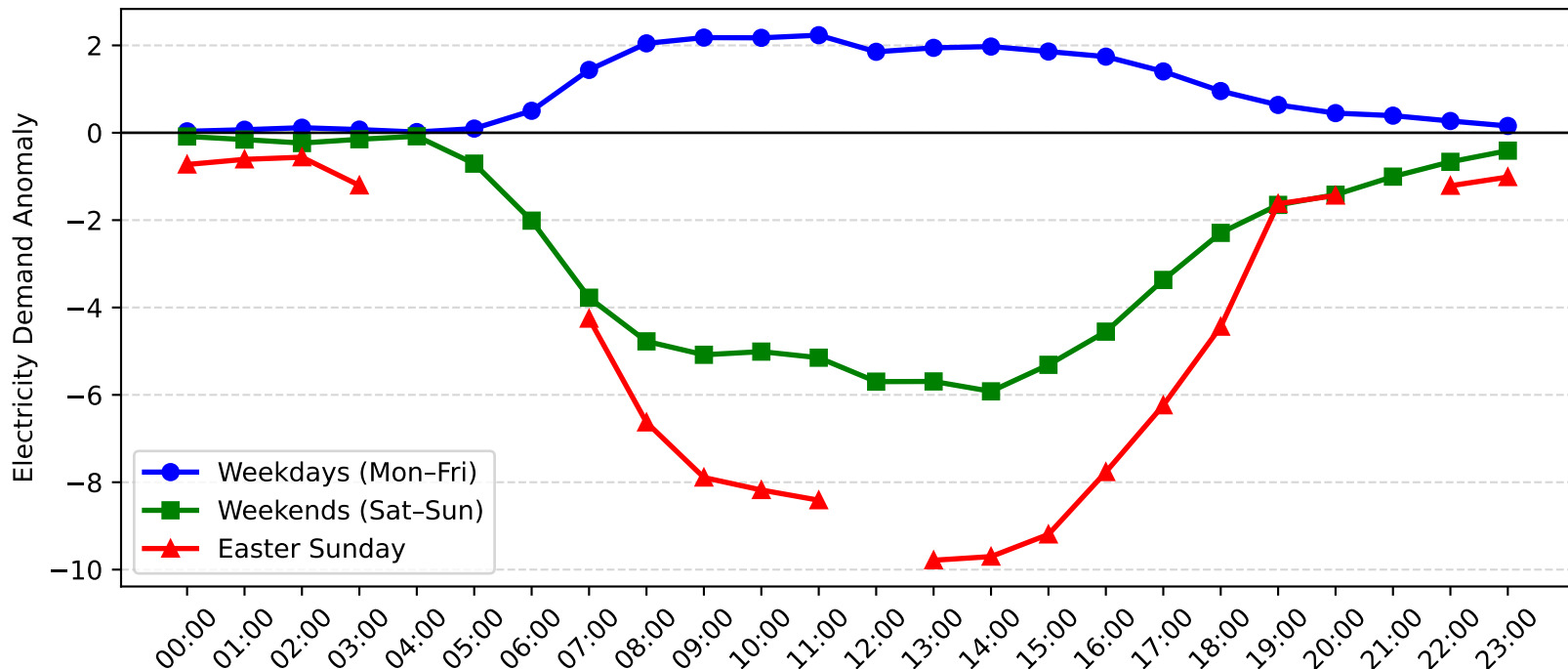
Green Square Demand Anomaly: Easter Sunday vs Weekday/Weekend (2013-2014)
