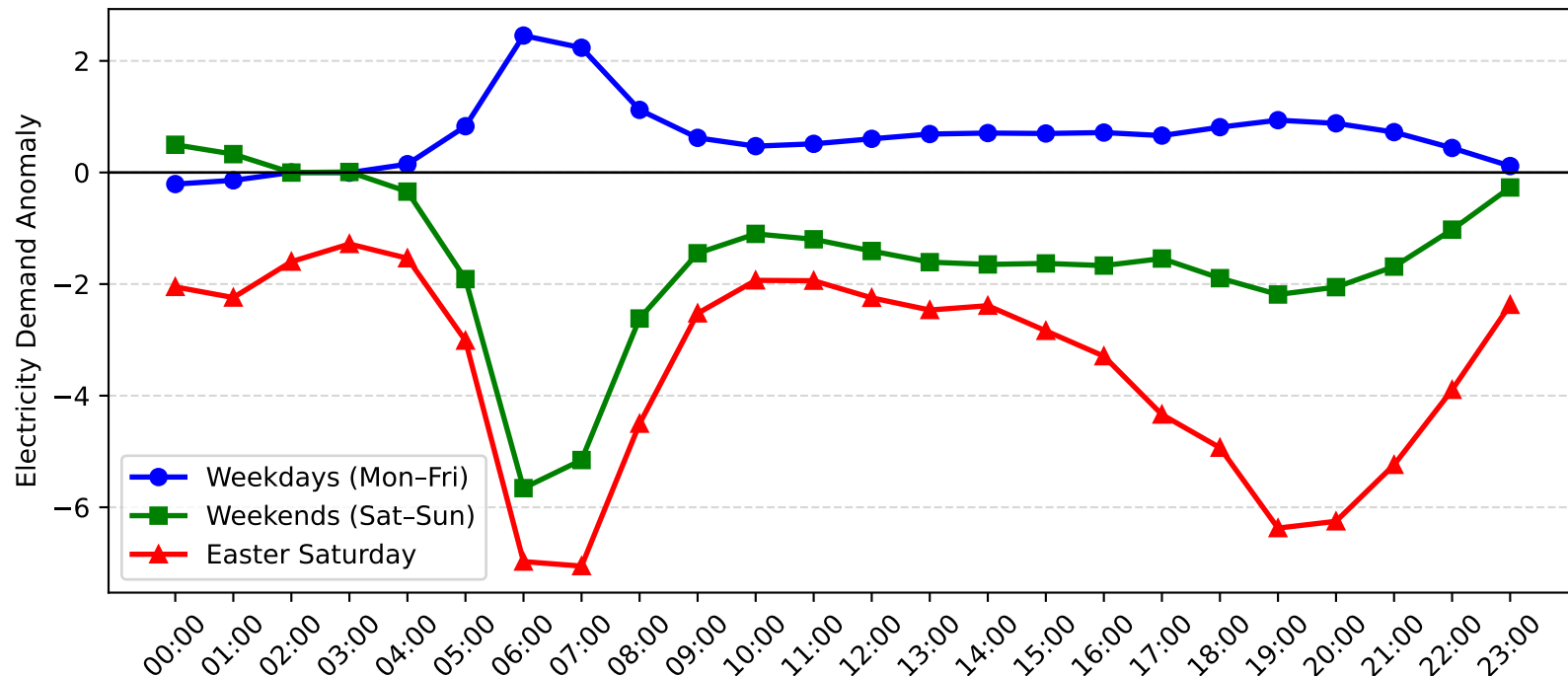
Pennant Hills Demand Anomaly: Easter Saturday vs Weekday/Weekend (2011-2012)
