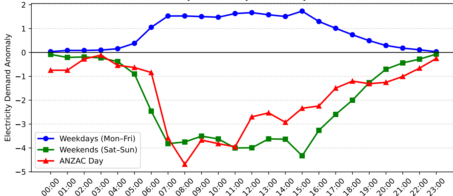
Zetland Demand Anomaly: ANZAC Day vs Weekday/Weekend (2004-2005)
