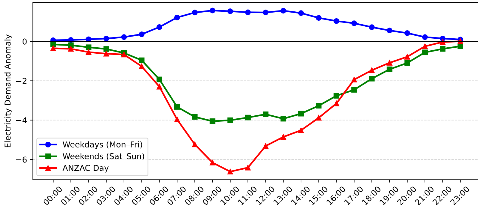
Auburn Demand Anomaly: ANZAC Day vs Weekday/Weekend (2007-2008)
