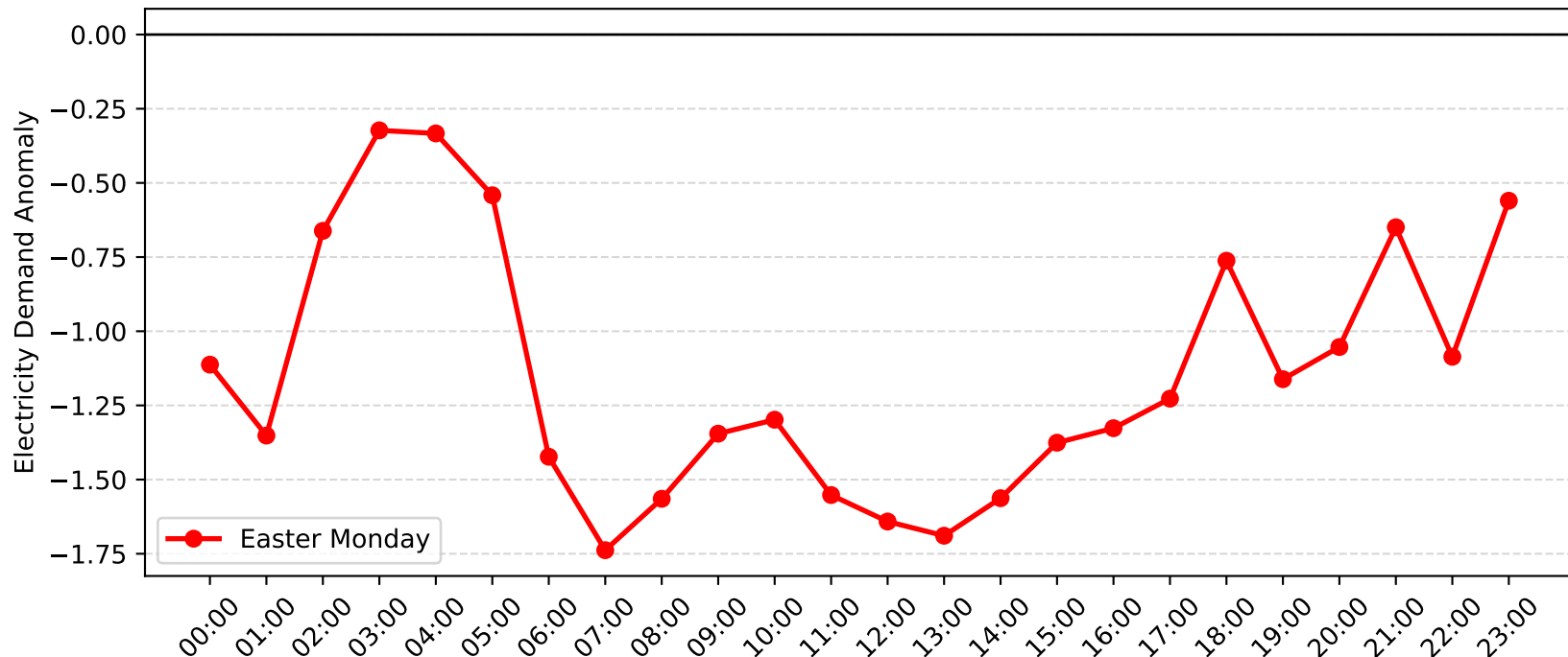
Gateshead Demand Anomaly: Easter Monday (2009-2010)
