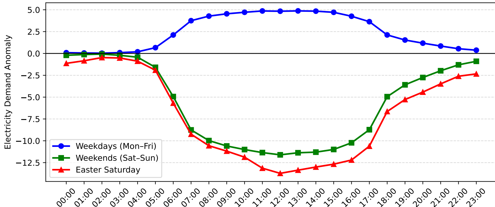
Macquarie Park Demand Anomaly: Easter Saturday vs Weekday/Weekend (2014-2015)
