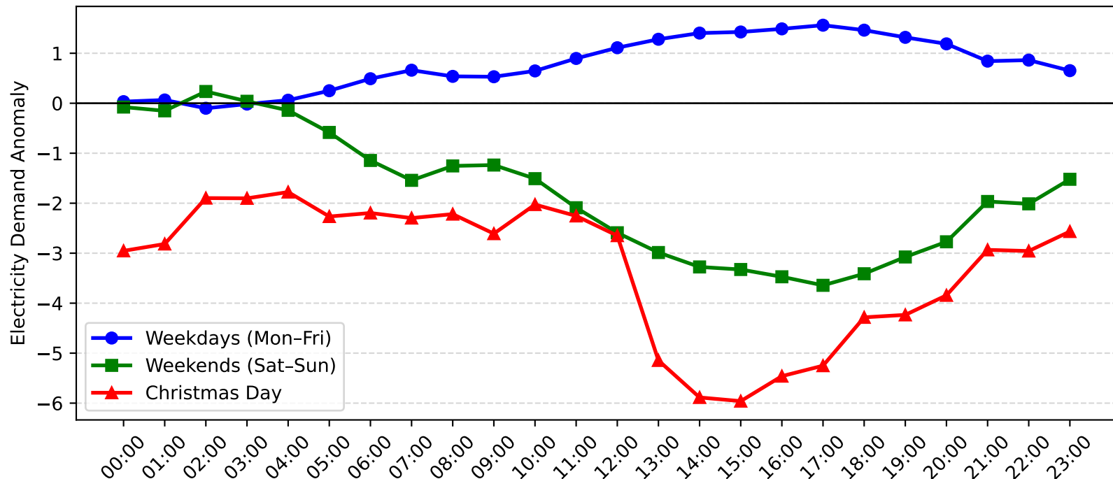
Jesmond Demand Anomaly: Christmas Day vs Weekday/Weekend (2016-2017)
