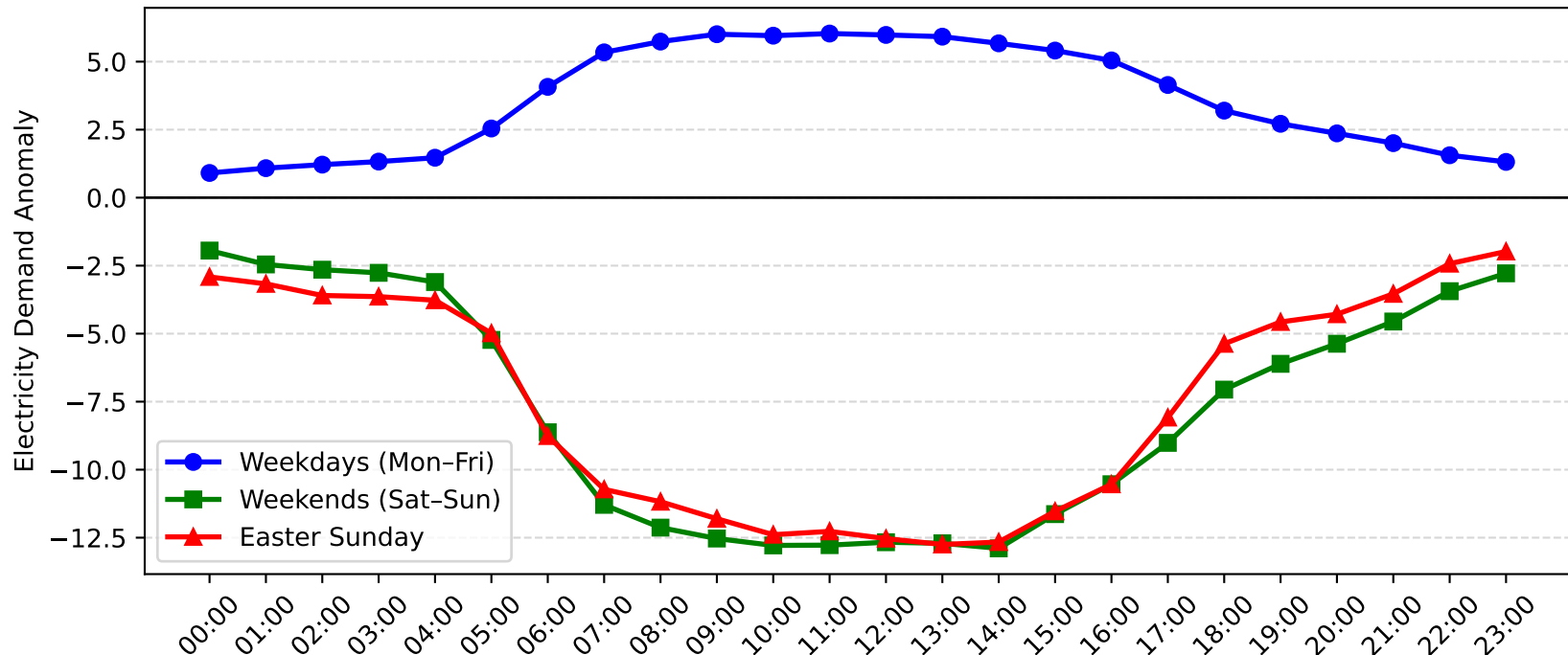
Flemington Demand Anomaly: Easter Sunday vs Weekday/Weekend (2009-2010)
