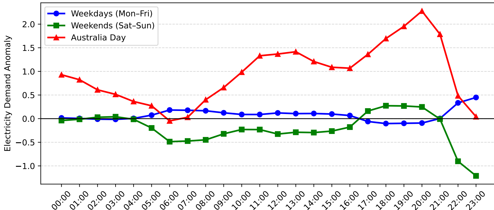
Muswellbrook Demand Anomaly: Australia Day vs Weekday/Weekend (2011-2012)
