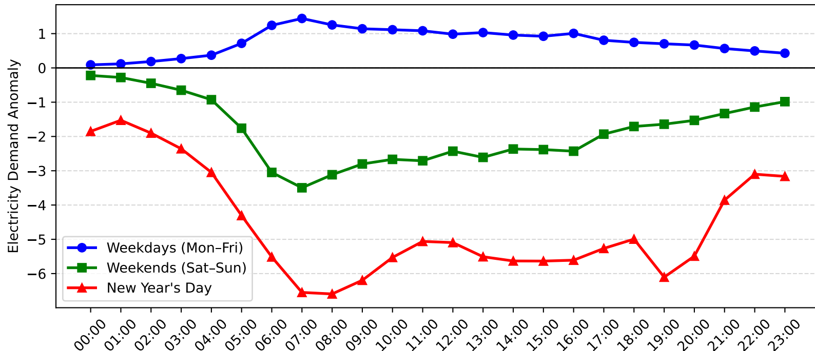
Enfield Demand Anomaly: New Year's Day vs Weekday/Weekend (2007-2008)
