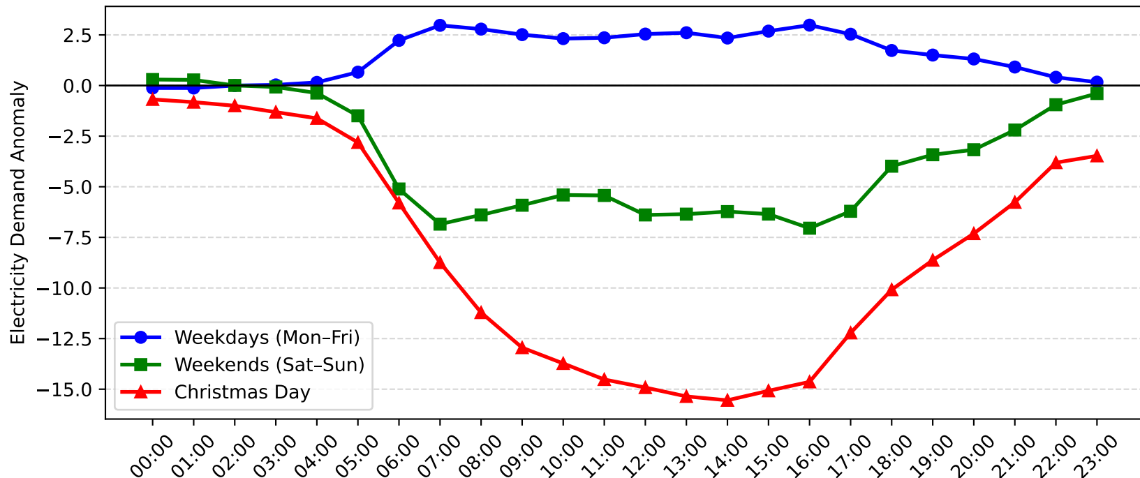
Epping Demand Anomaly: Christmas Day vs Weekday/Weekend (2005-2006)
