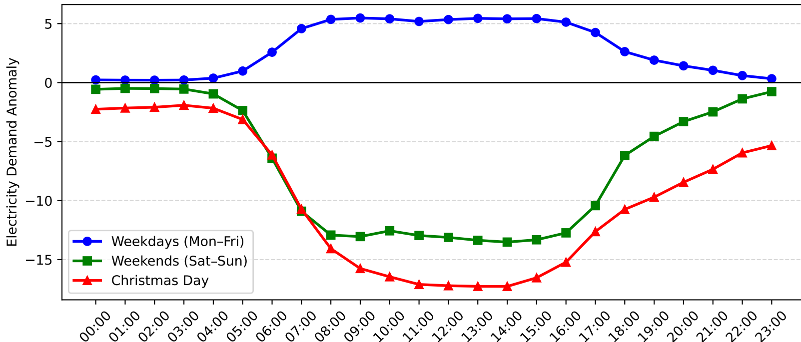
Gore Hill Demand Anomaly: Christmas Day vs Weekday/Weekend (2006-2007)
