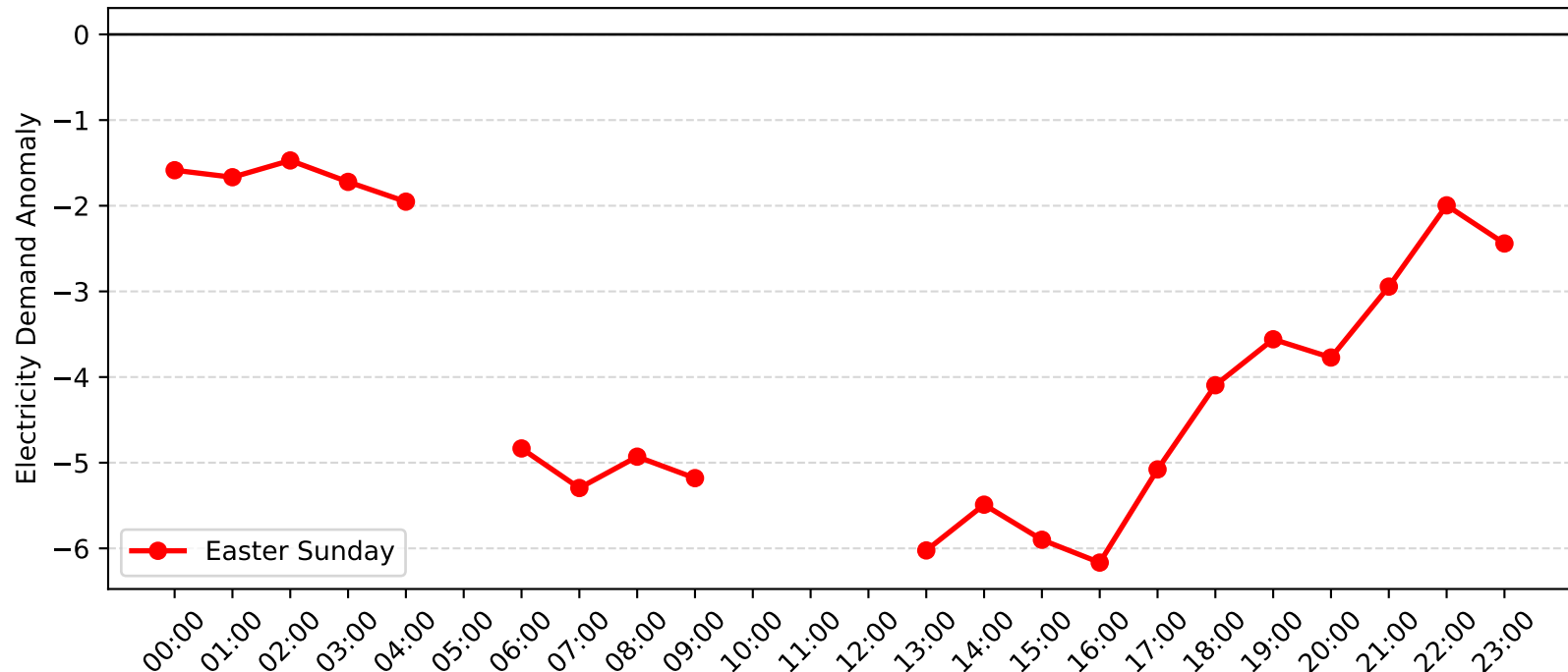
Potts Hill Demand Anomaly: Easter Sunday (2017-2018)
