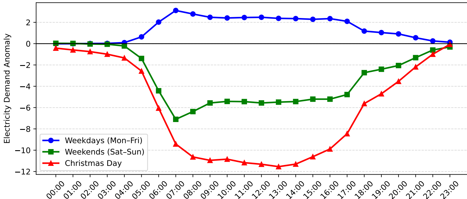
Epping Demand Anomaly: Christmas Day vs Weekday/Weekend (2010-2011)
