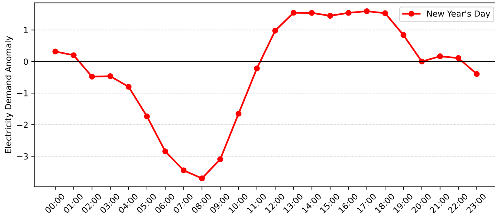
Charmhaven Demand Anomaly: New Year's Day (2011-2012)
