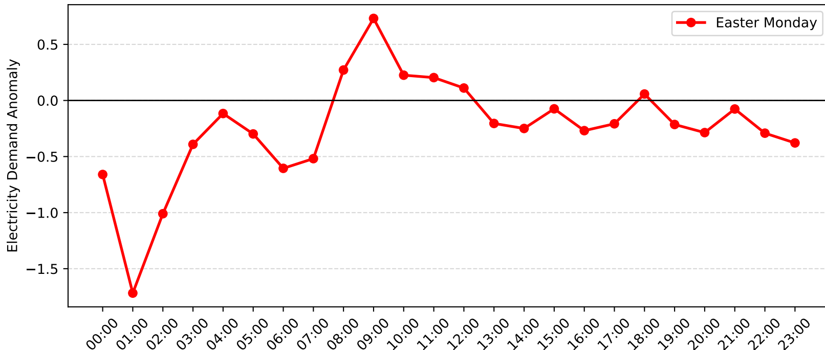
Swansea Demand Anomaly: Easter Monday (2006-2007)
