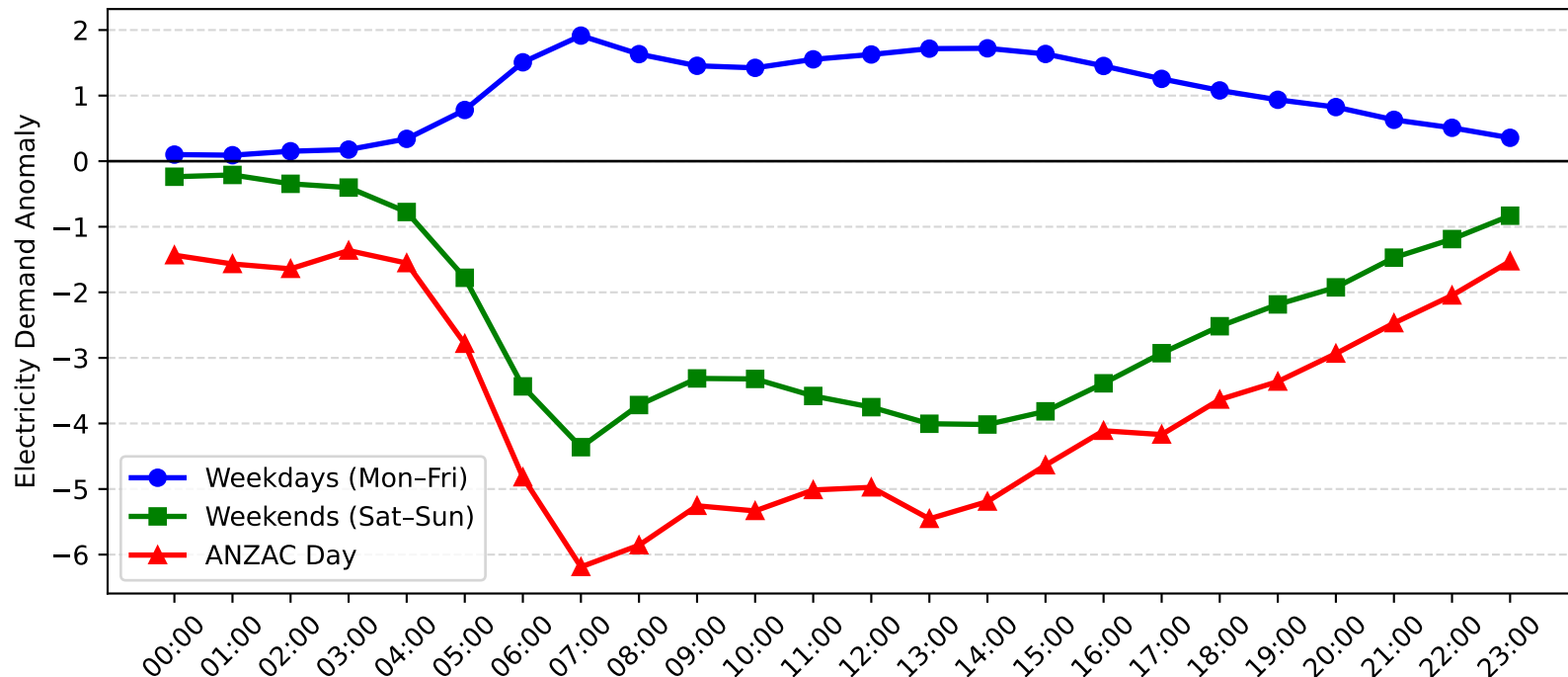
Sefton Demand Anomaly: ANZAC Day vs Weekday/Weekend (2015-2016)
