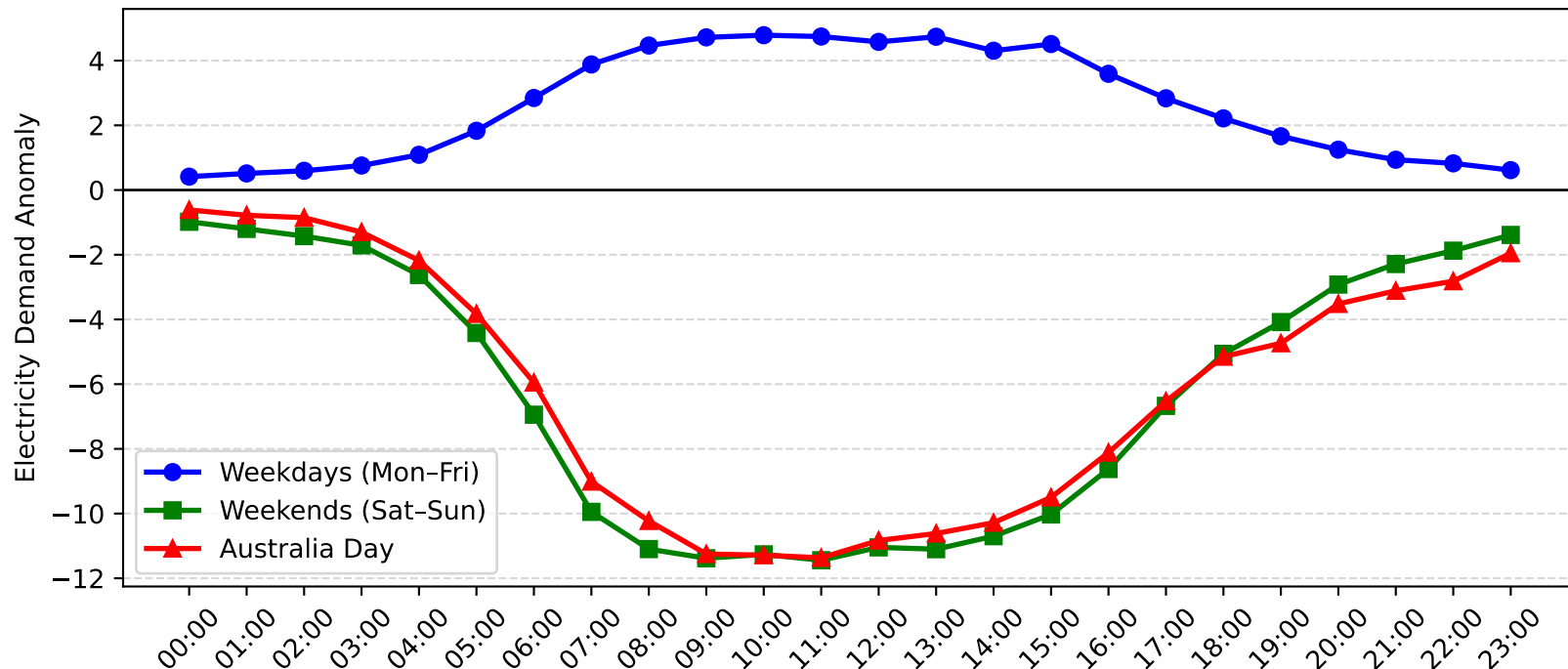
Homebush Bay Demand Anomaly: Australia Day vs Weekday/Weekend (2008-2009)
