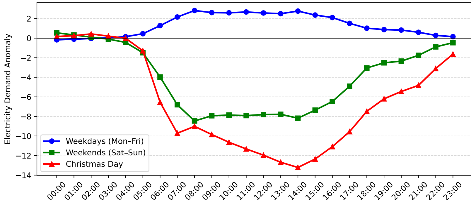
St. Peters Demand Anomaly: Christmas Day vs Weekday/Weekend (2013-2014)
