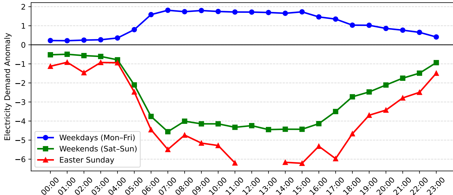
Potts Hill Demand Anomaly: Easter Sunday vs Weekday/Weekend (2015-2016)
