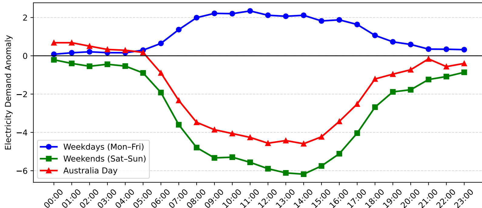
Green Square Demand Anomaly: Australia Day vs Weekday/Weekend (2012-2013)
