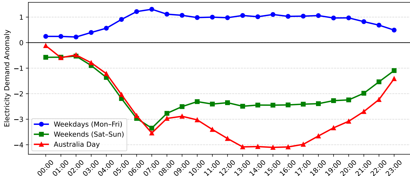
Lisarow Demand Anomaly: Australia Day vs Weekday/Weekend (2008-2009)
