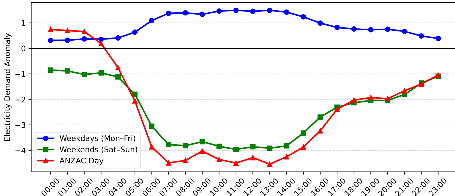
Somersby Demand Anomaly: ANZAC Day vs Weekday/Weekend (2012-2013)
