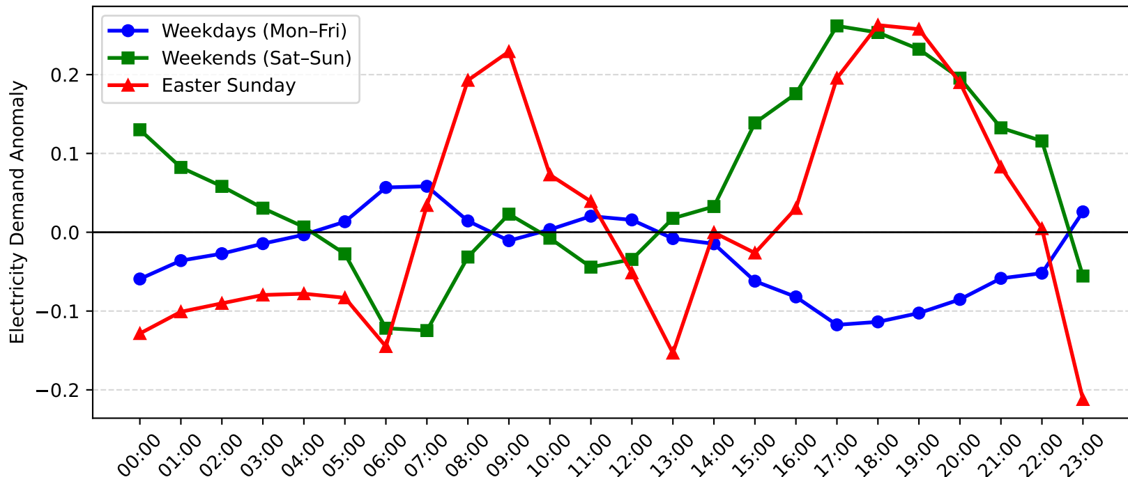
Rothbury Demand Anomaly: Easter Sunday vs Weekday/Weekend (2010-2011)
