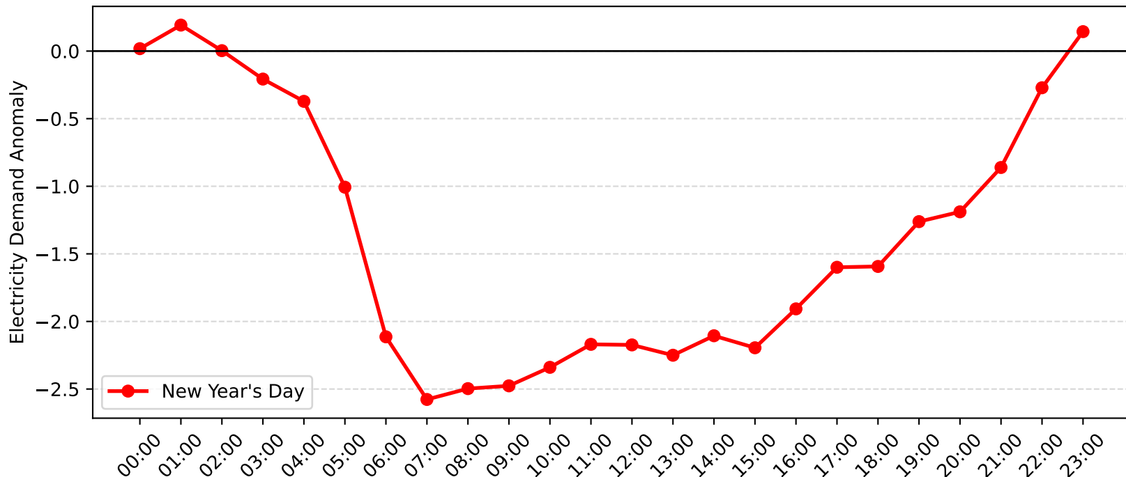
Rockdale Demand Anomaly: New Year's Day (2004-2005)
