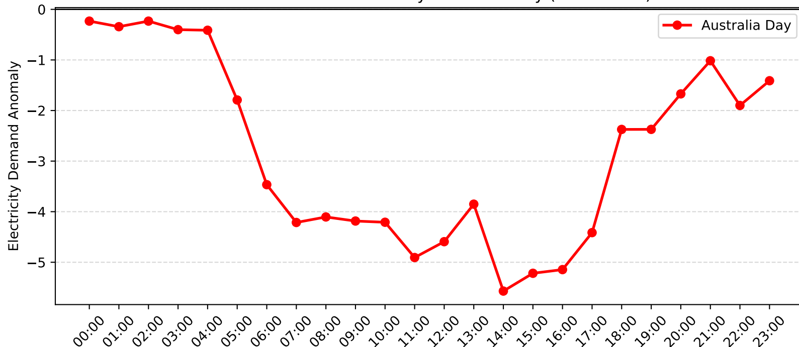
Potts Hill Demand Anomaly: Australia Day (2015-2016)
