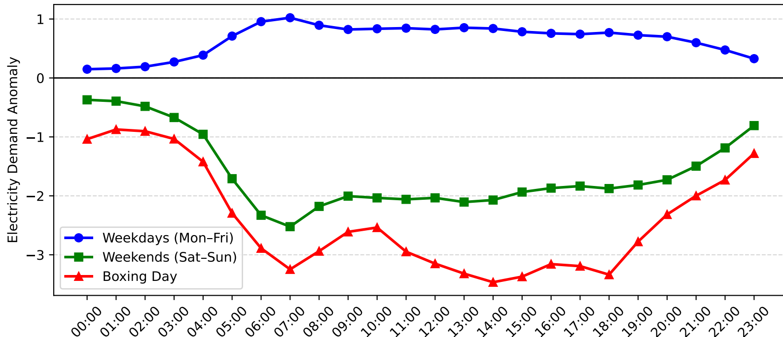
Lisarow Demand Anomaly: Boxing Day vs Weekday/Weekend (2011-2012)
