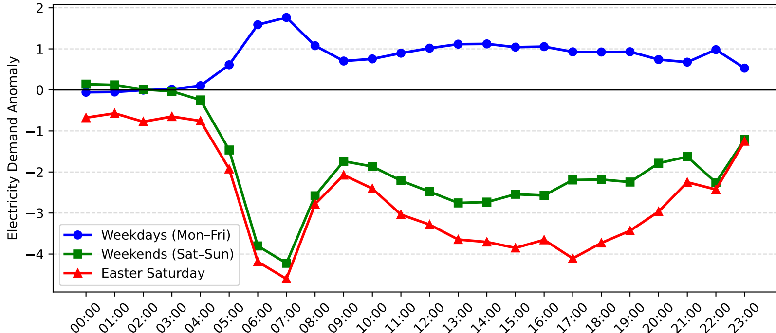
Dee Why West Demand Anomaly: Easter Saturday vs Weekday/Weekend (2007-2008)
