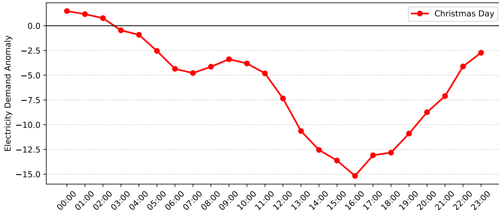
Pennant Hills Demand Anomaly: Christmas Day (2007-2008)
