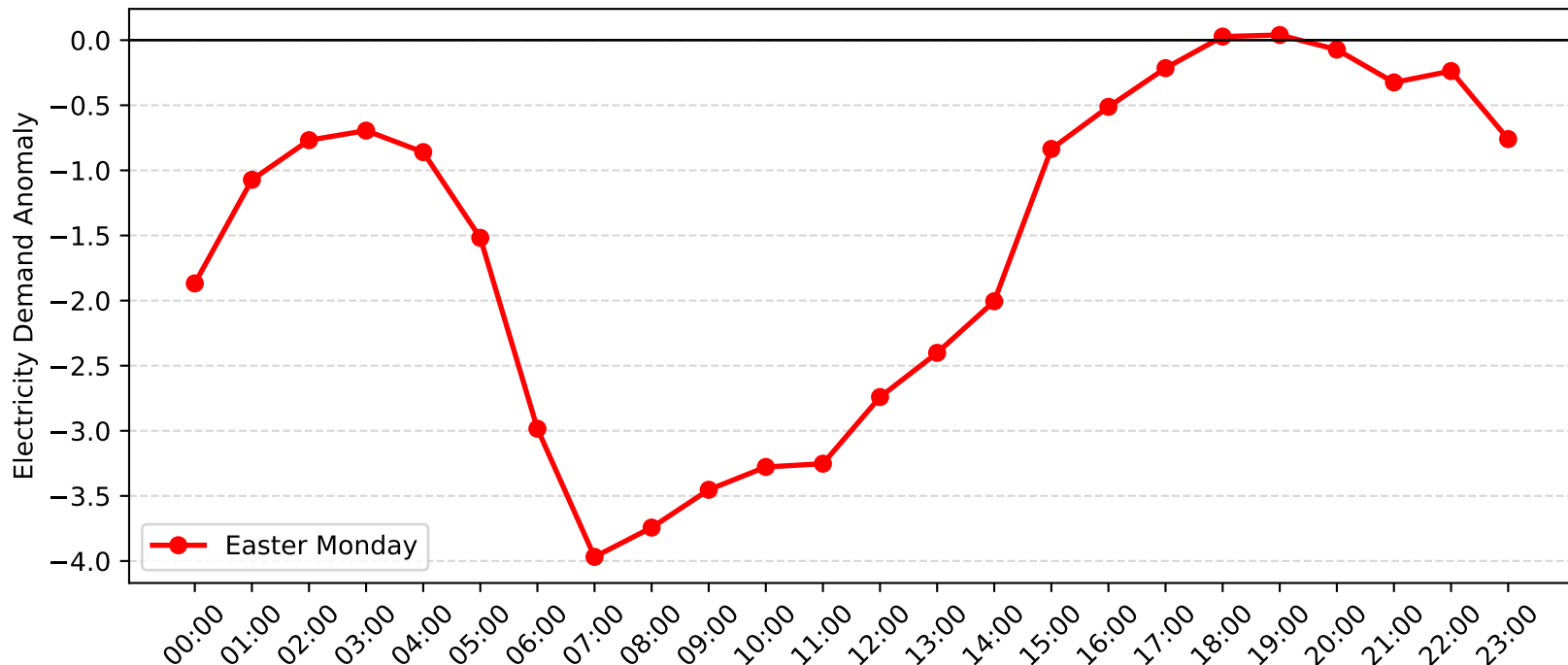
Rutherford Demand Anomaly: Easter Monday (2015-2016)
