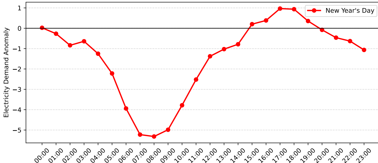
Wyong Demand Anomaly: New Year's Day (2011-2012)
