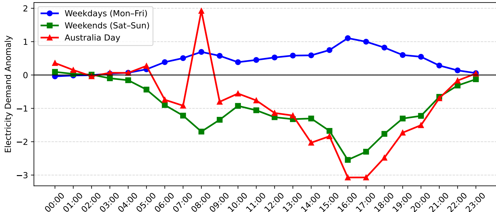
Erina Demand Anomaly: Australia Day vs Weekday/Weekend (2013-2014)
