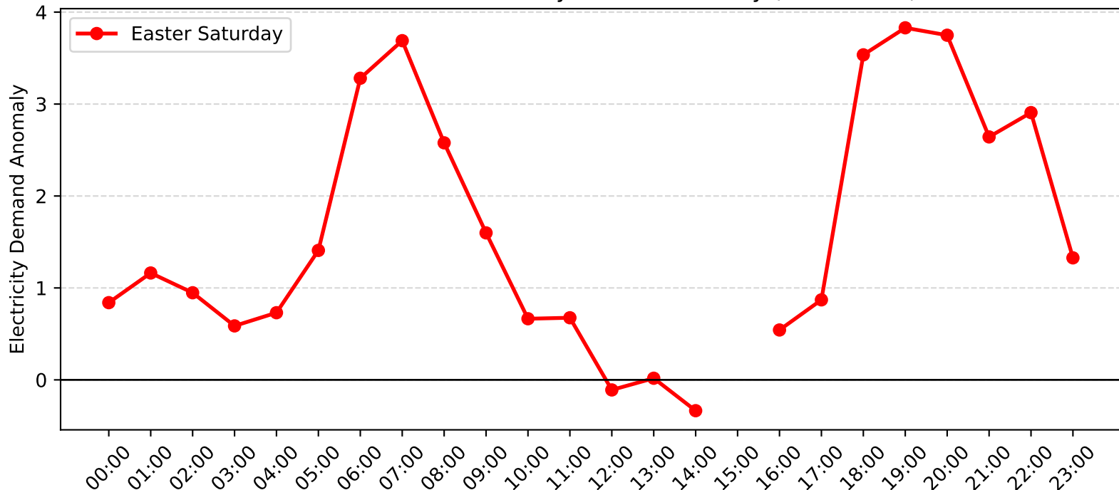
Arncliffe Demand Anomaly: Easter Saturday (2004-2005)
