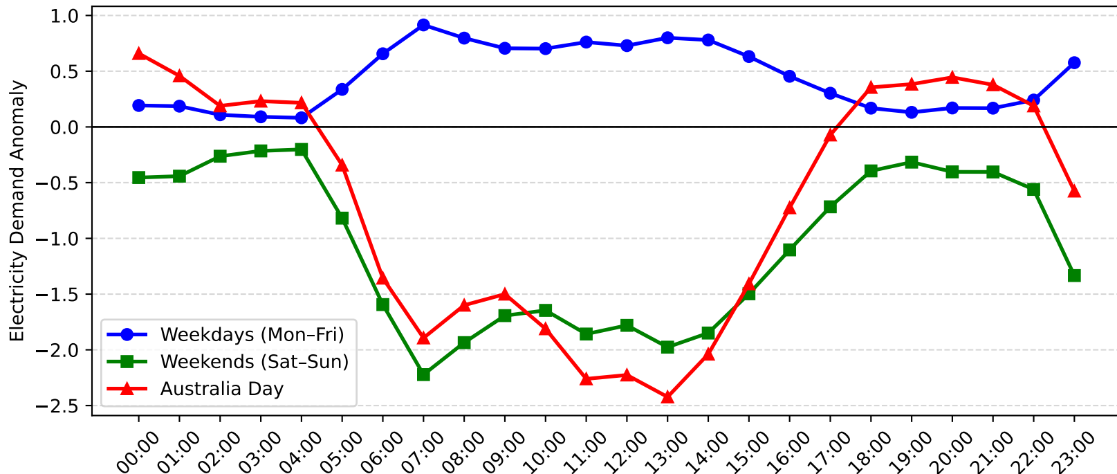
Rutherford Demand Anomaly: Australia Day vs Weekday/Weekend (2007-2008)
