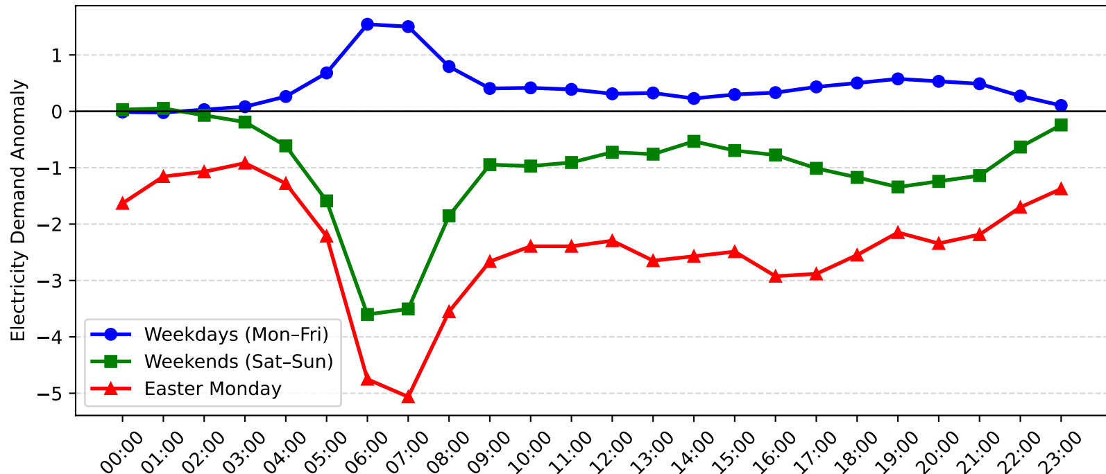
Revesby Demand Anomaly: Easter Monday vs Weekday/Weekend (2013-2014)
