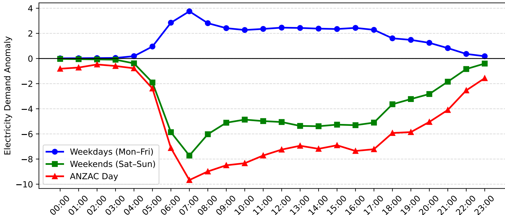
Epping Demand Anomaly: ANZAC Day vs Weekday/Weekend (2009-2010)
