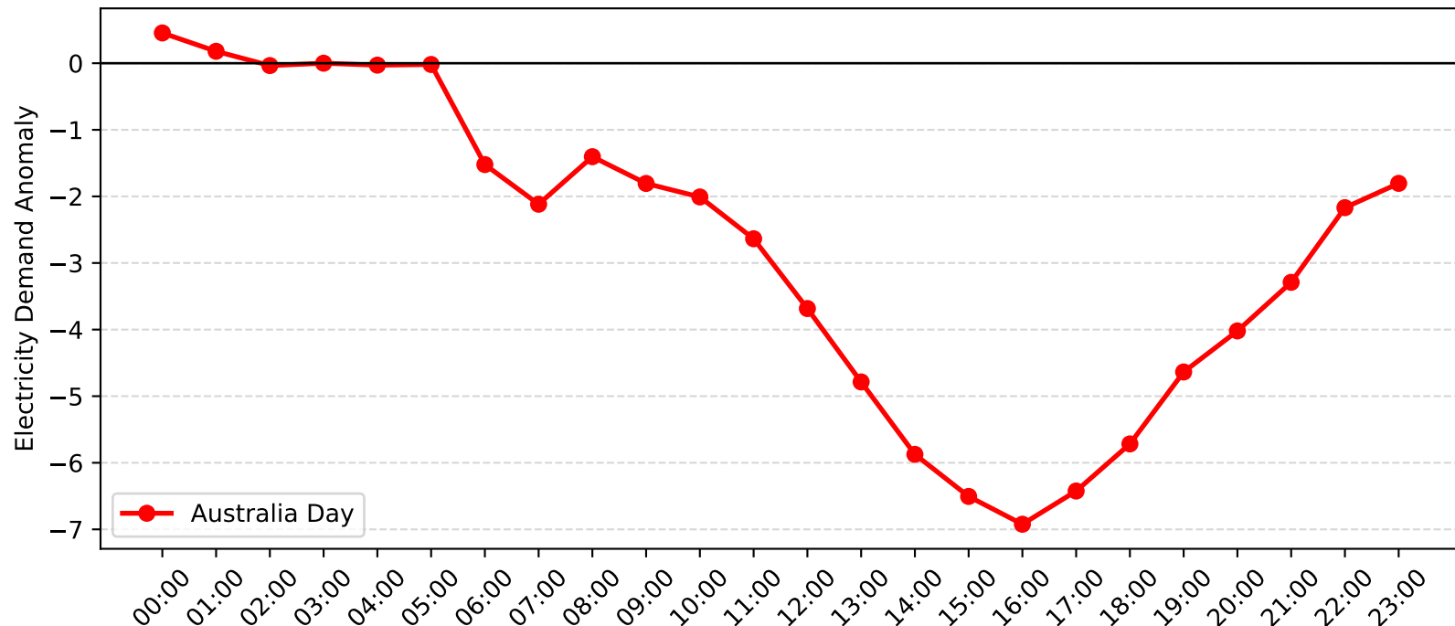
Charmhaven Demand Anomaly: Australia Day (2014-2015)
