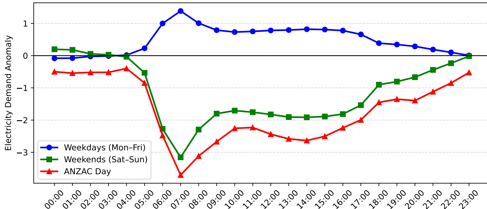
Pymble Demand Anomaly: ANZAC Day vs Weekday/Weekend (2015-2016)
