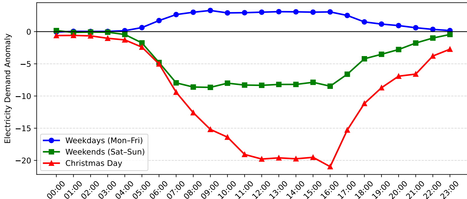
Castle Cove Demand Anomaly: Christmas Day vs Weekday/Weekend (2007-2008)
