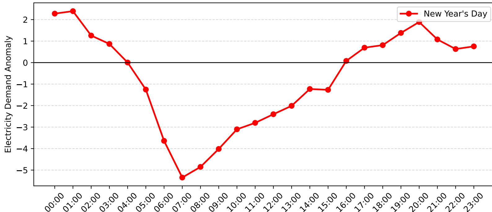
Mortdale Demand Anomaly: New Year's Day (2009-2010)
