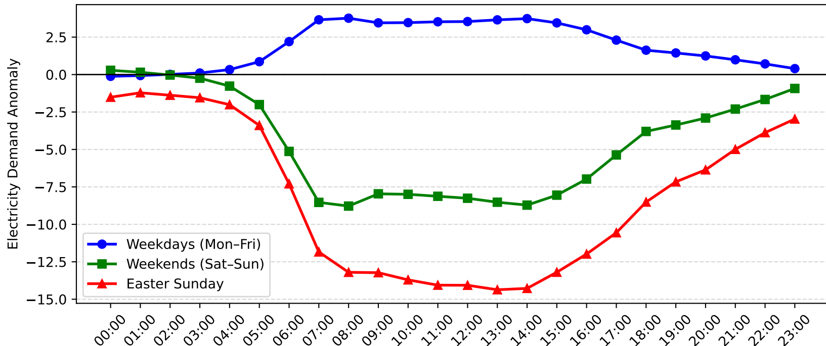
St. Peters Demand Anomaly: Easter Sunday vs Weekday/Weekend (2013-2014)
