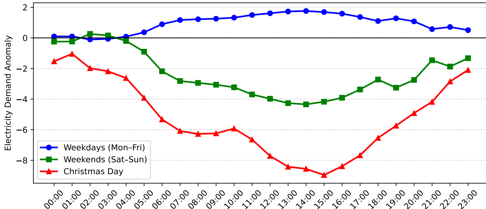
Sefton Demand Anomaly: Christmas Day vs Weekday/Weekend (2015-2016)
