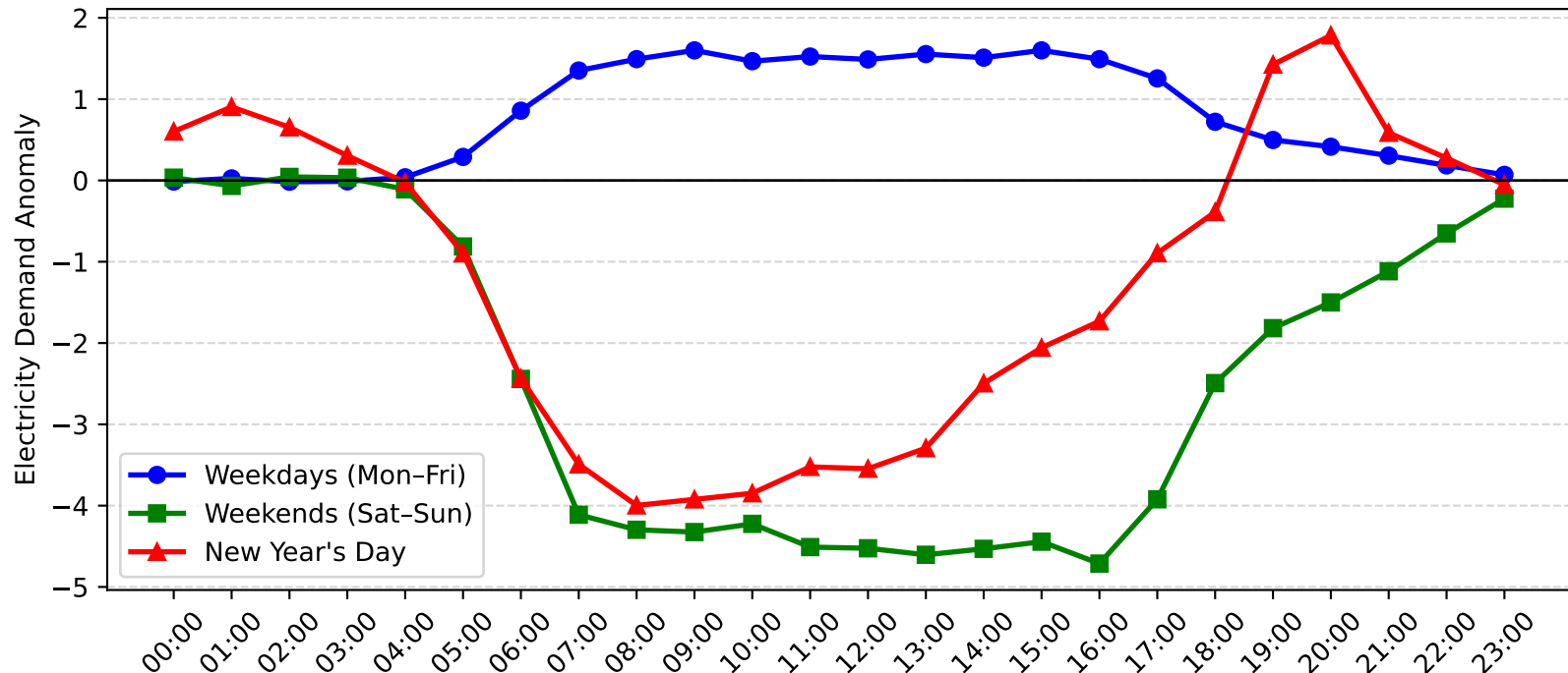
Pymble Demand Anomaly: New Year's Day vs Weekday/Weekend (2008-2009)
