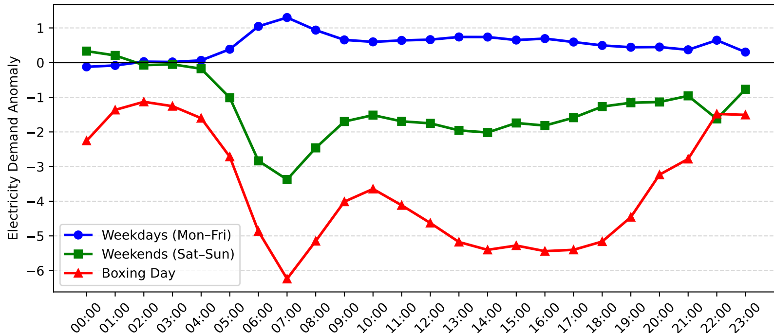
Dee Why West Demand Anomaly: Boxing Day vs Weekday/Weekend (2006-2007)
