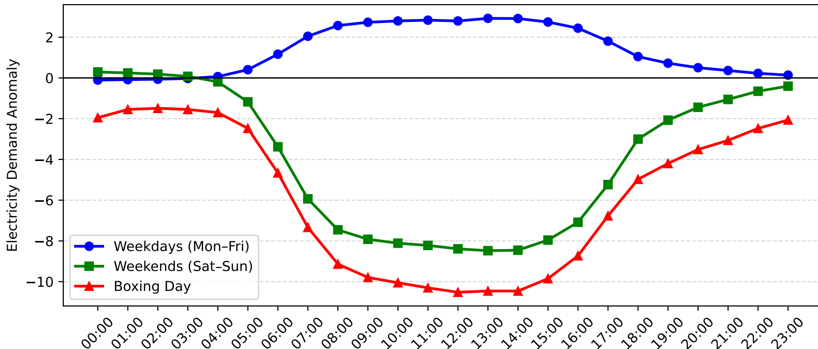
Mascot Demand Anomaly: Boxing Day vs Weekday/Weekend (2012-2013)
