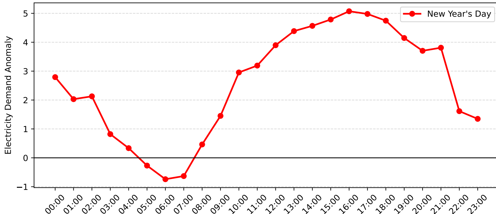
Nelson Bay Demand Anomaly: New Year's Day (2013-2014)
