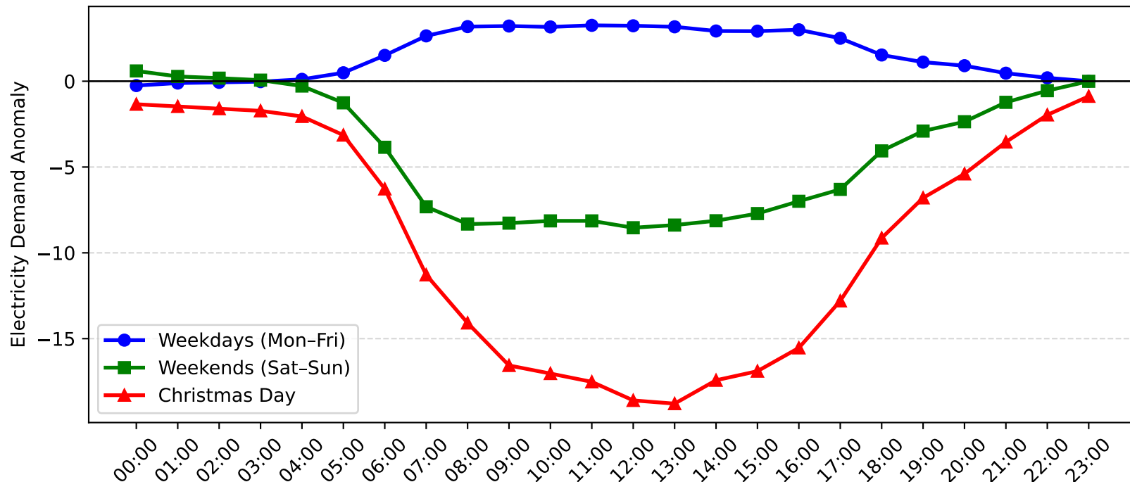
Castle Cove Demand Anomaly: Christmas Day vs Weekday/Weekend (2009-2010)
