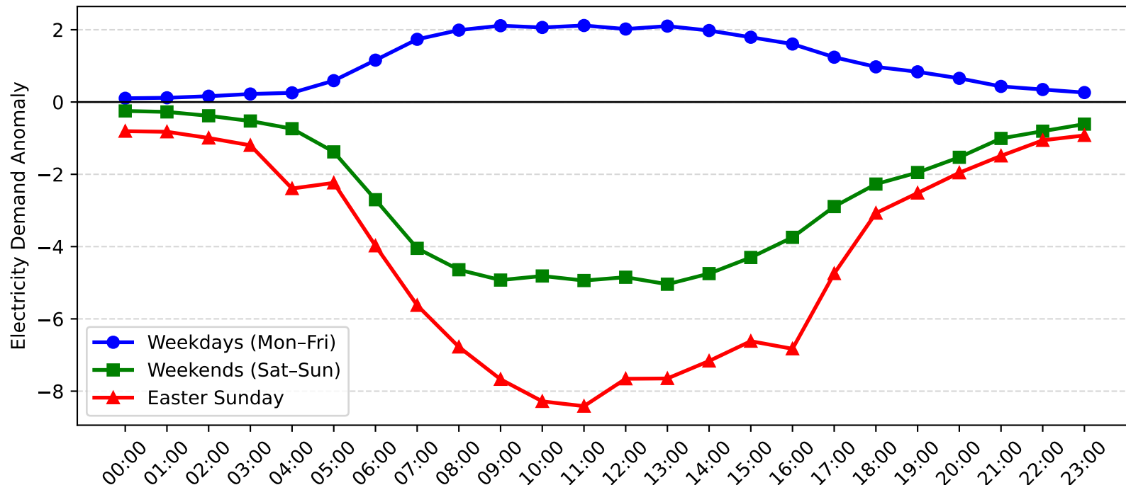
Auburn Demand Anomaly: Easter Sunday vs Weekday/Weekend (2012-2013)
