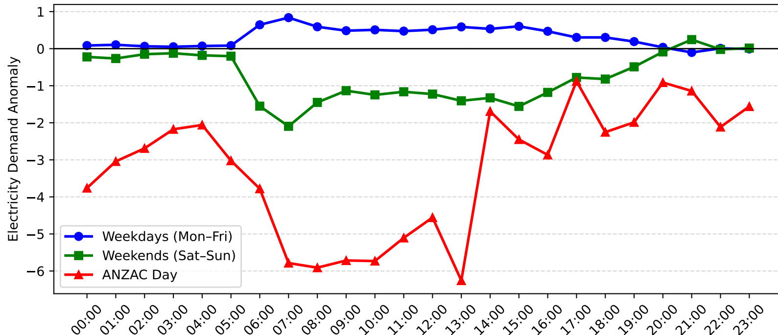
Chatswood Demand Anomaly: ANZAC Day vs Weekday/Weekend (2004-2005)
