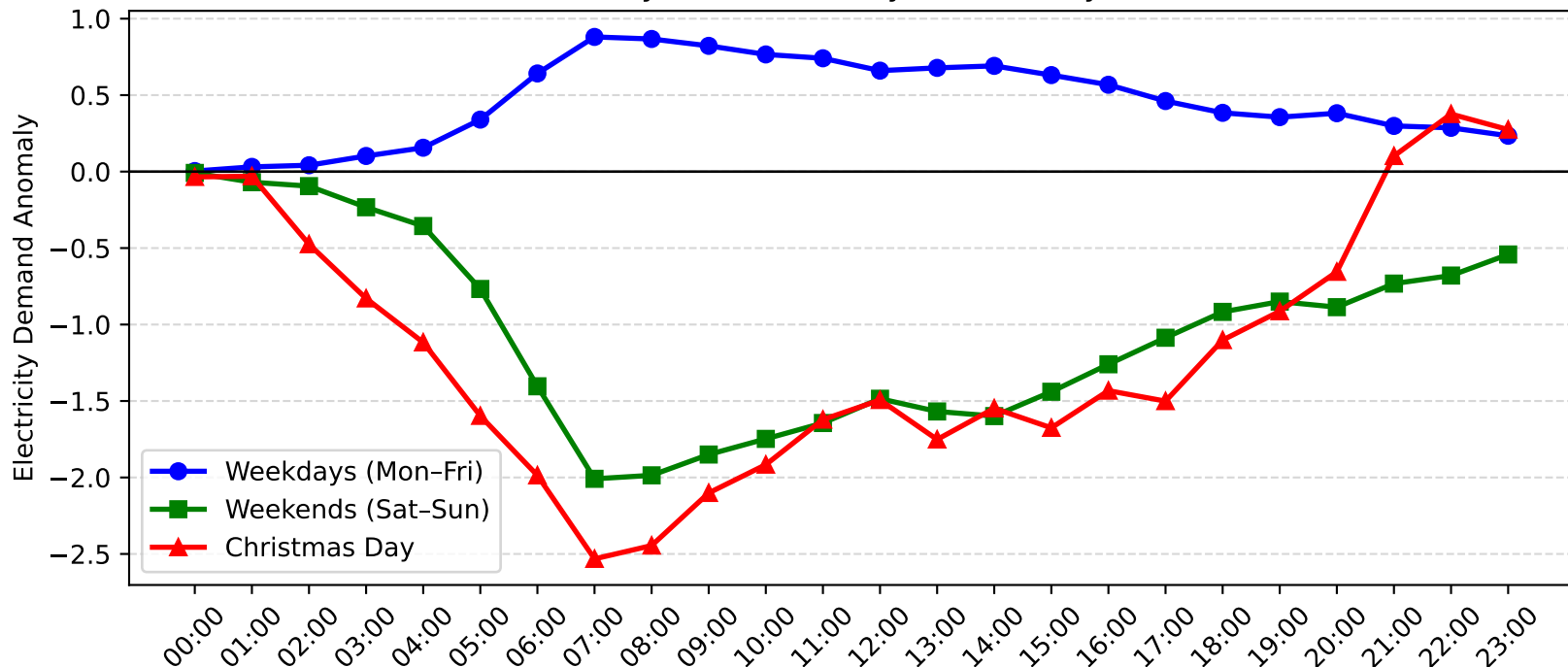
Bass Hill Demand Anomaly: Christmas Day vs Weekday/Weekend (2010-2011)
