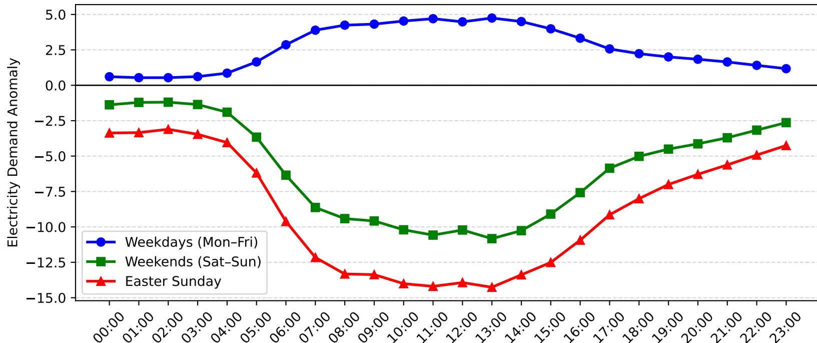
Milperra Demand Anomaly: Easter Sunday vs Weekday/Weekend (2016-2017)
