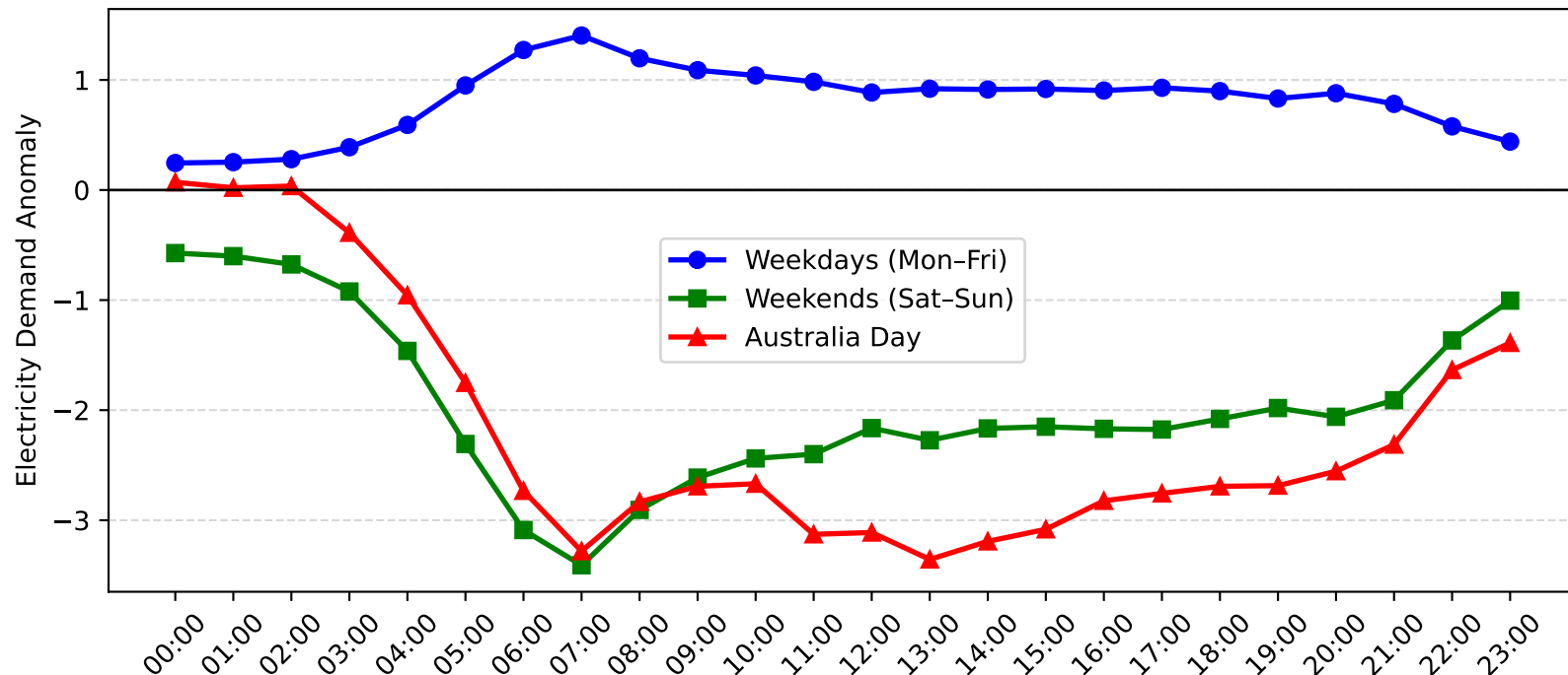
Lisarow Demand Anomaly: Australia Day vs Weekday/Weekend (2007-2008)
