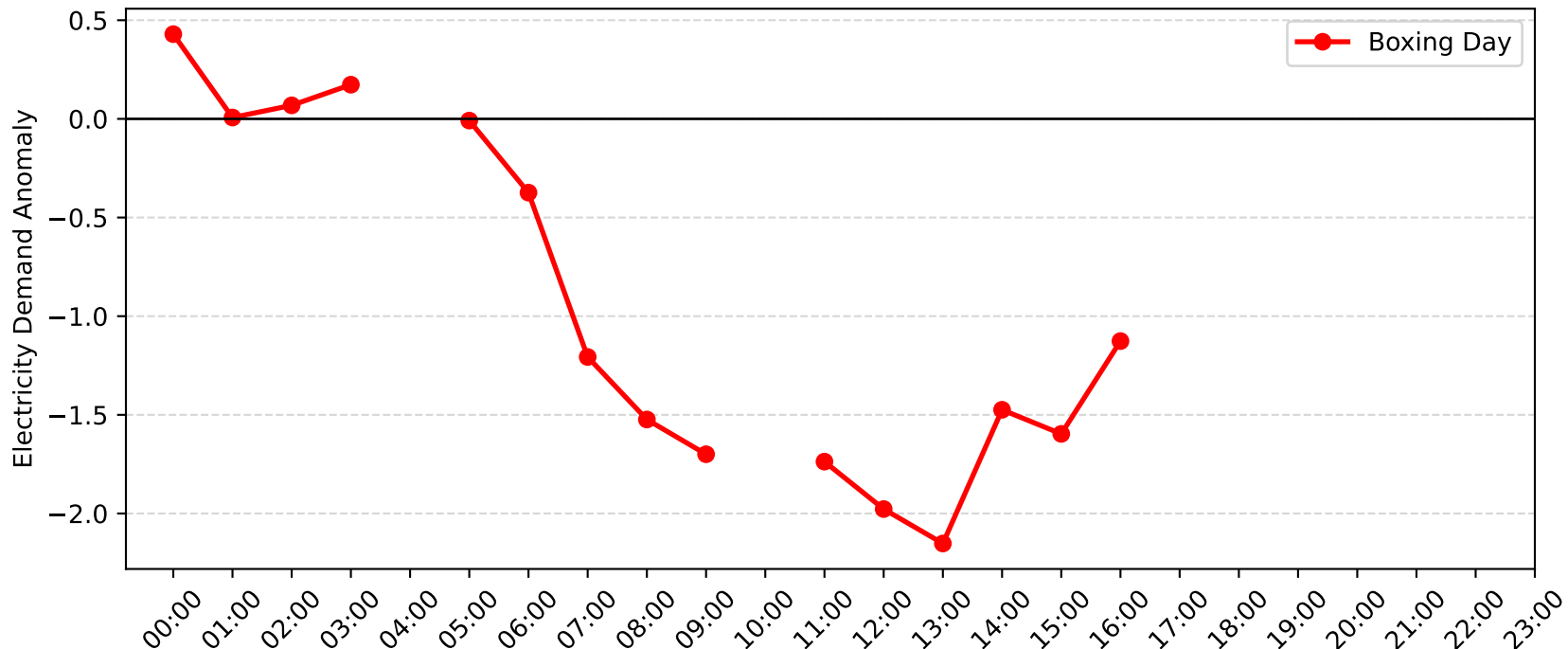
Potts Hill Demand Anomaly: Boxing Day (2012-2013)
