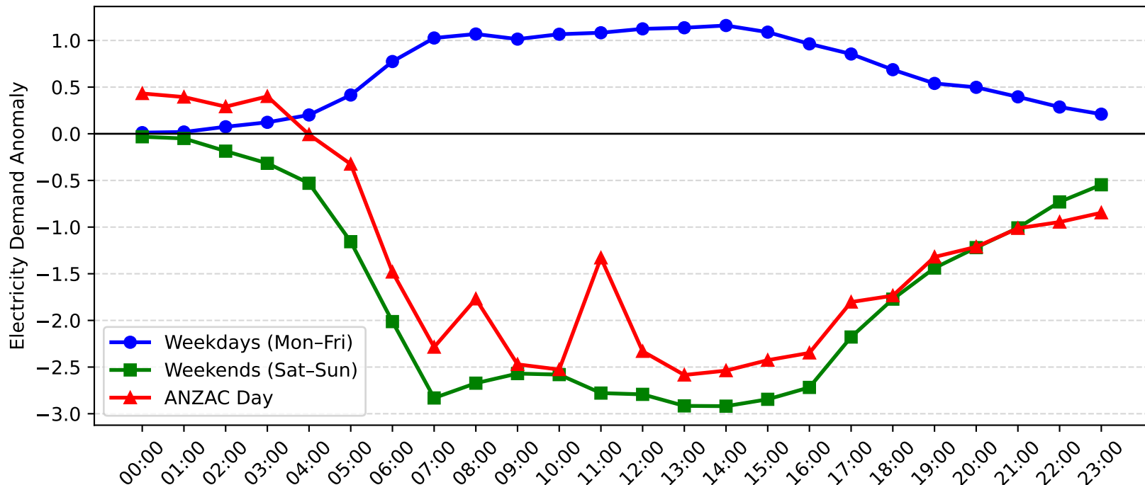
Lidcombe Demand Anomaly: ANZAC Day vs Weekday/Weekend (2006-2007)
