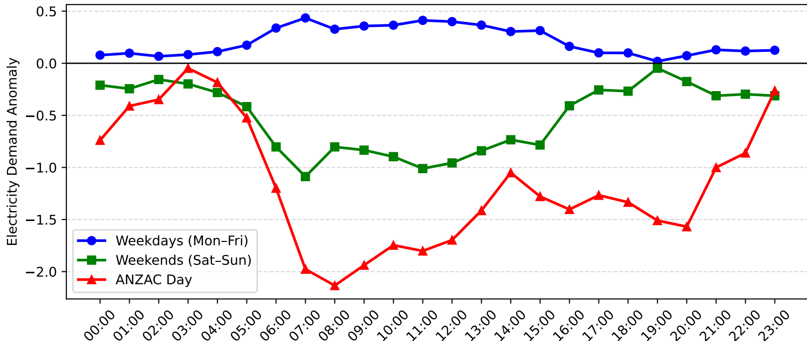
Wyong Demand Anomaly: ANZAC Day vs Weekday/Weekend (2004-2005)
