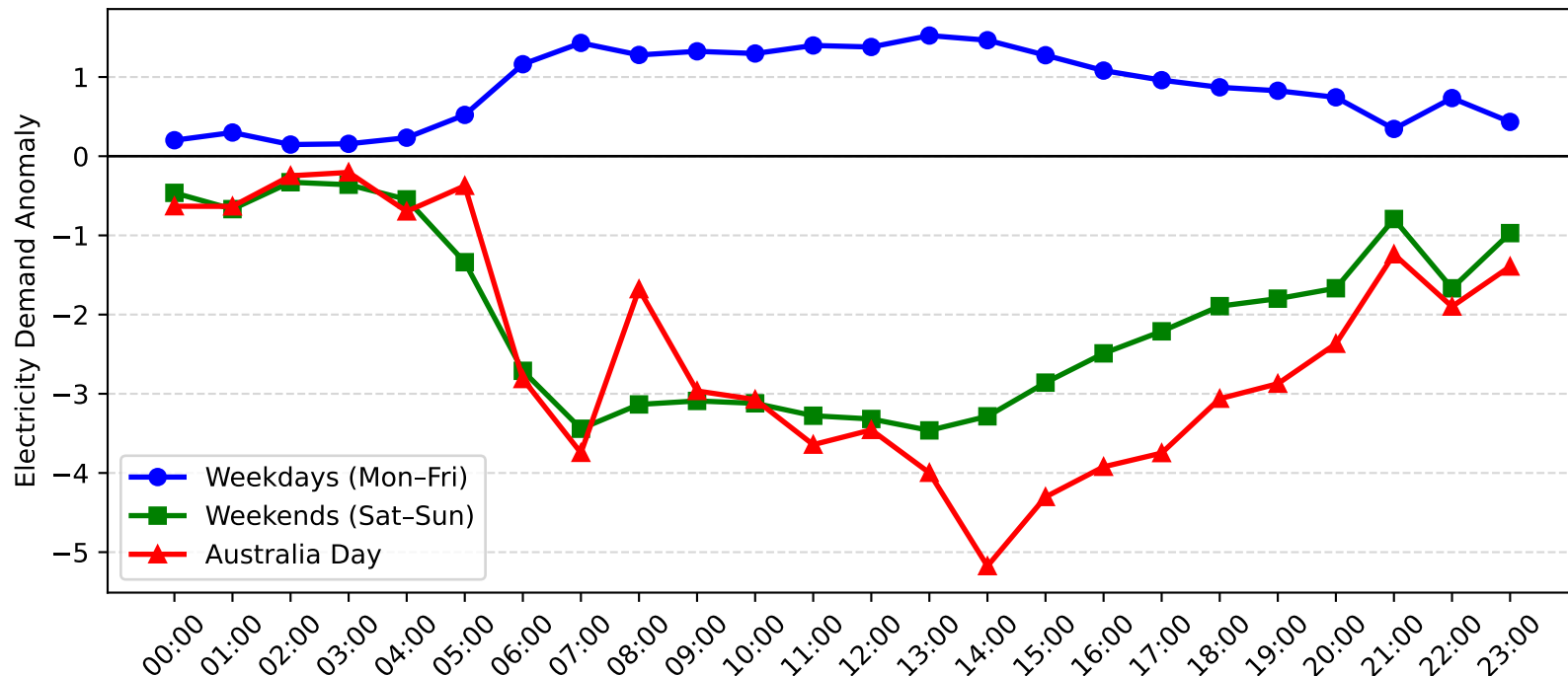
Argenton Demand Anomaly: Australia Day vs Weekday/Weekend (2013-2014)
