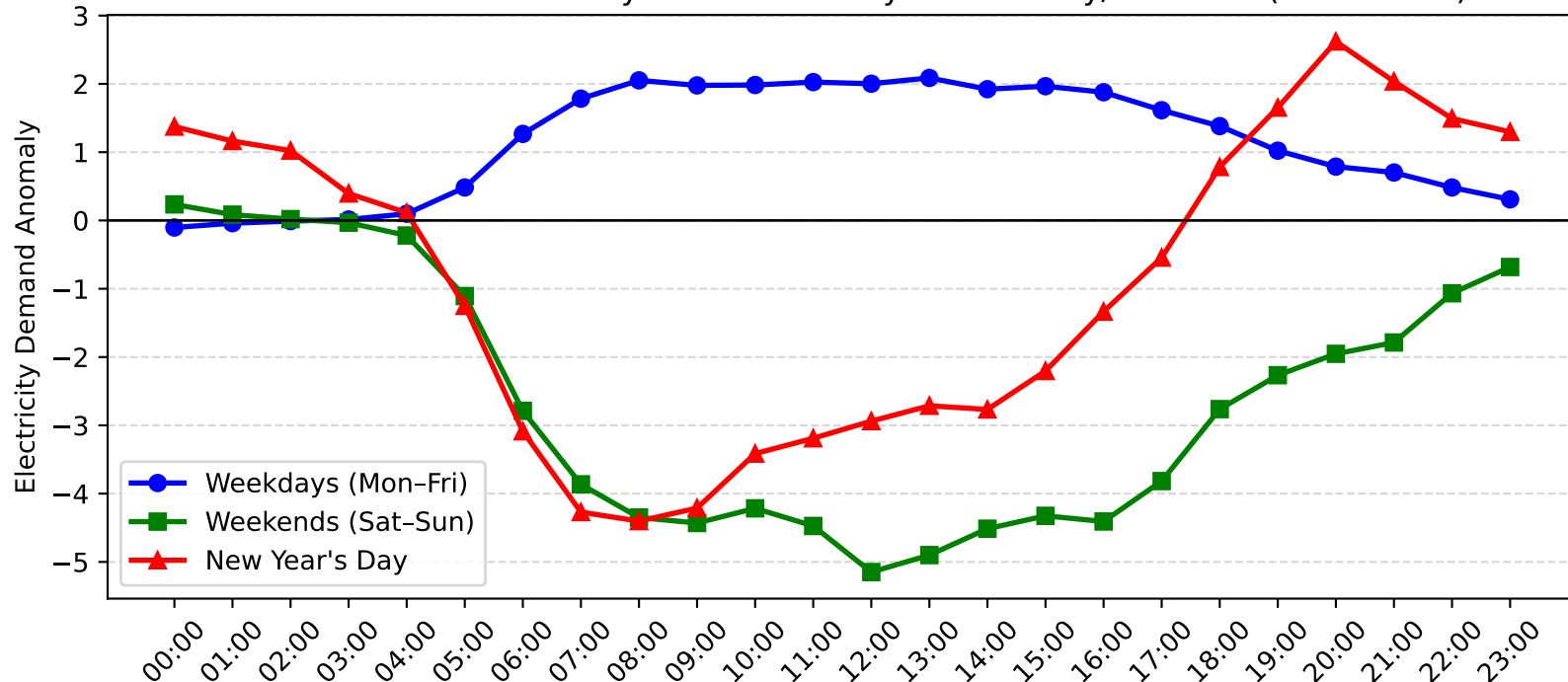
Concord Demand Anomaly: New Year's Day vs Weekday/Weekend (2005-2006)
