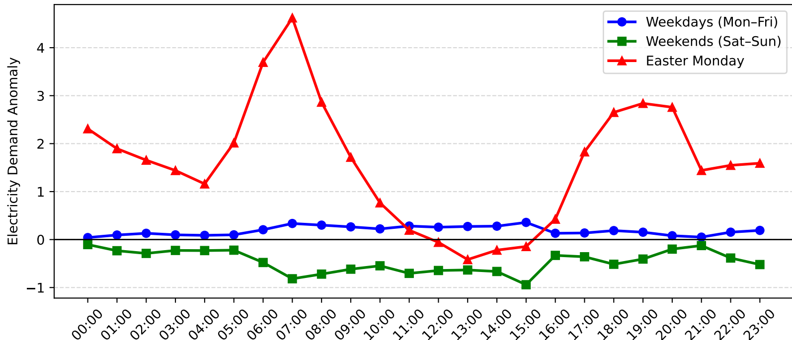
Bass Hill Demand Anomaly: Easter Monday vs Weekday/Weekend (2004-2005)
