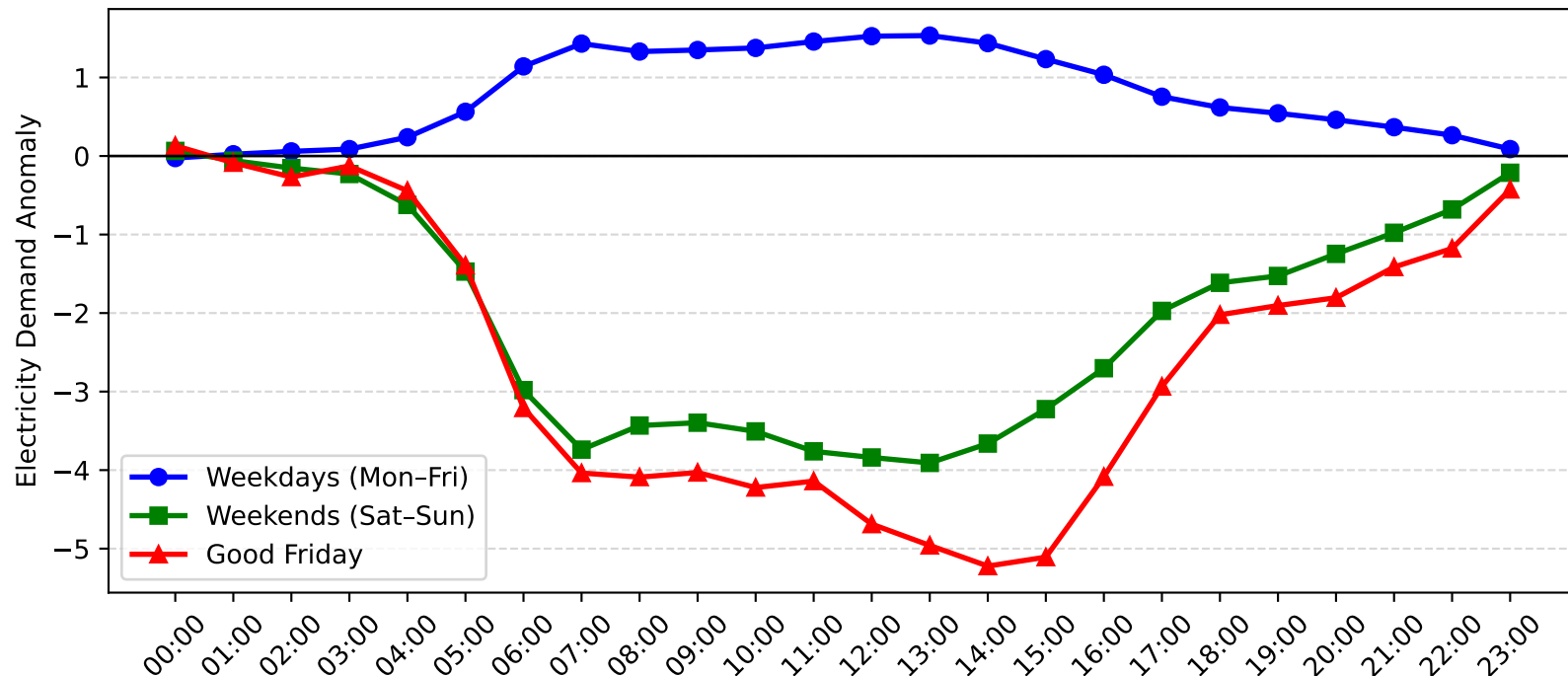
Wyong Demand Anomaly: Good Friday vs Weekday/Weekend (2007-2008)
