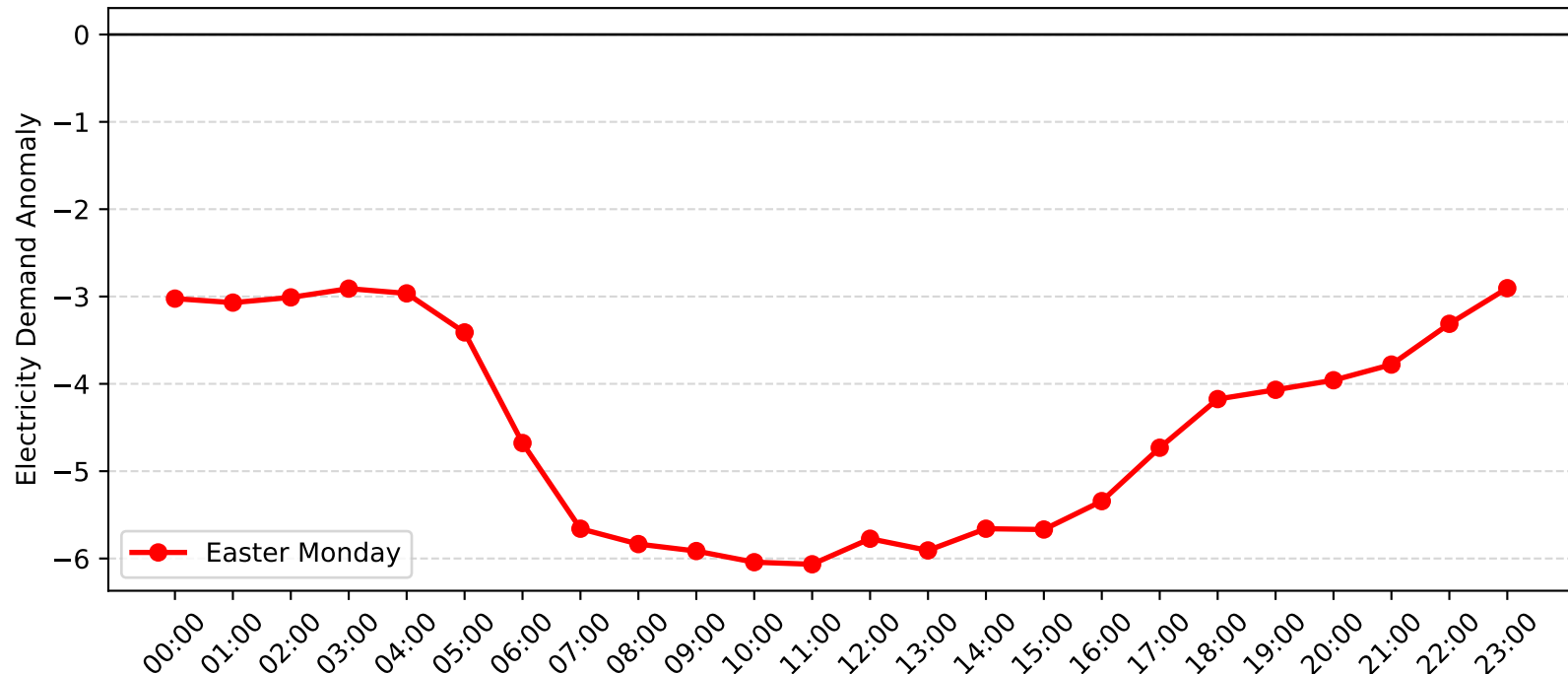
Leightonfield Demand Anomaly: Easter Monday (2014-2015)
