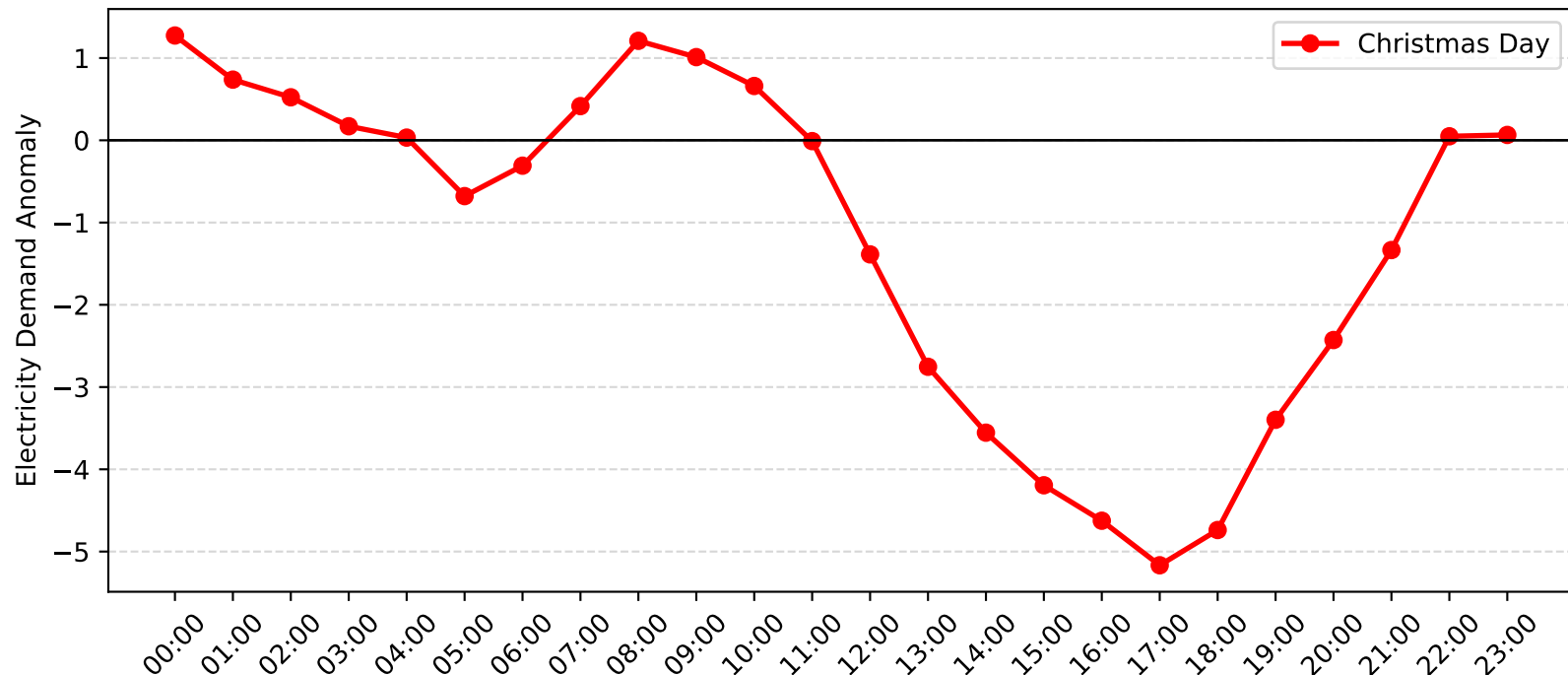
Umina Demand Anomaly: Christmas Day (2006-2007)
