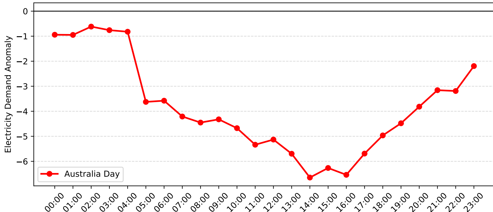
Potts Hill Demand Anomaly: Australia Day (2016-2017)
