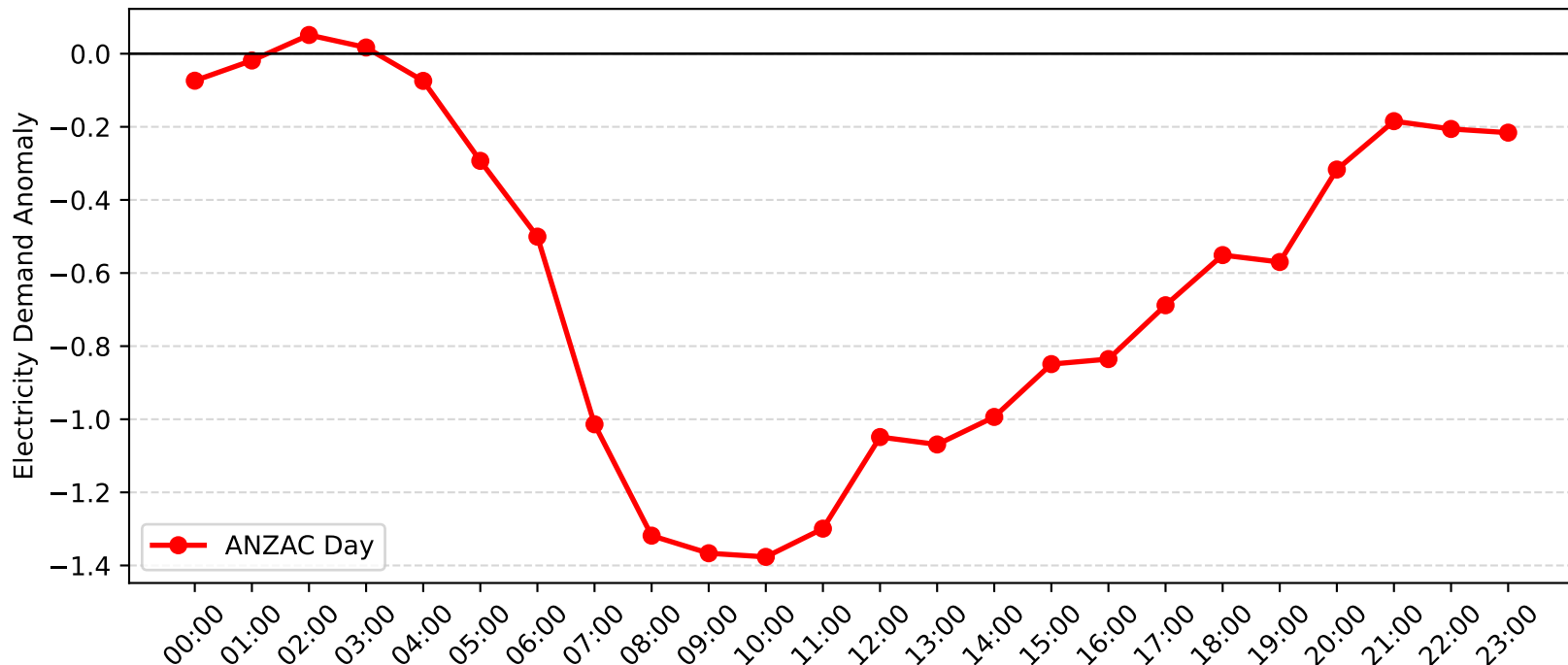
Broadmeadow Demand Anomaly: ANZAC Day (2014-2015)
