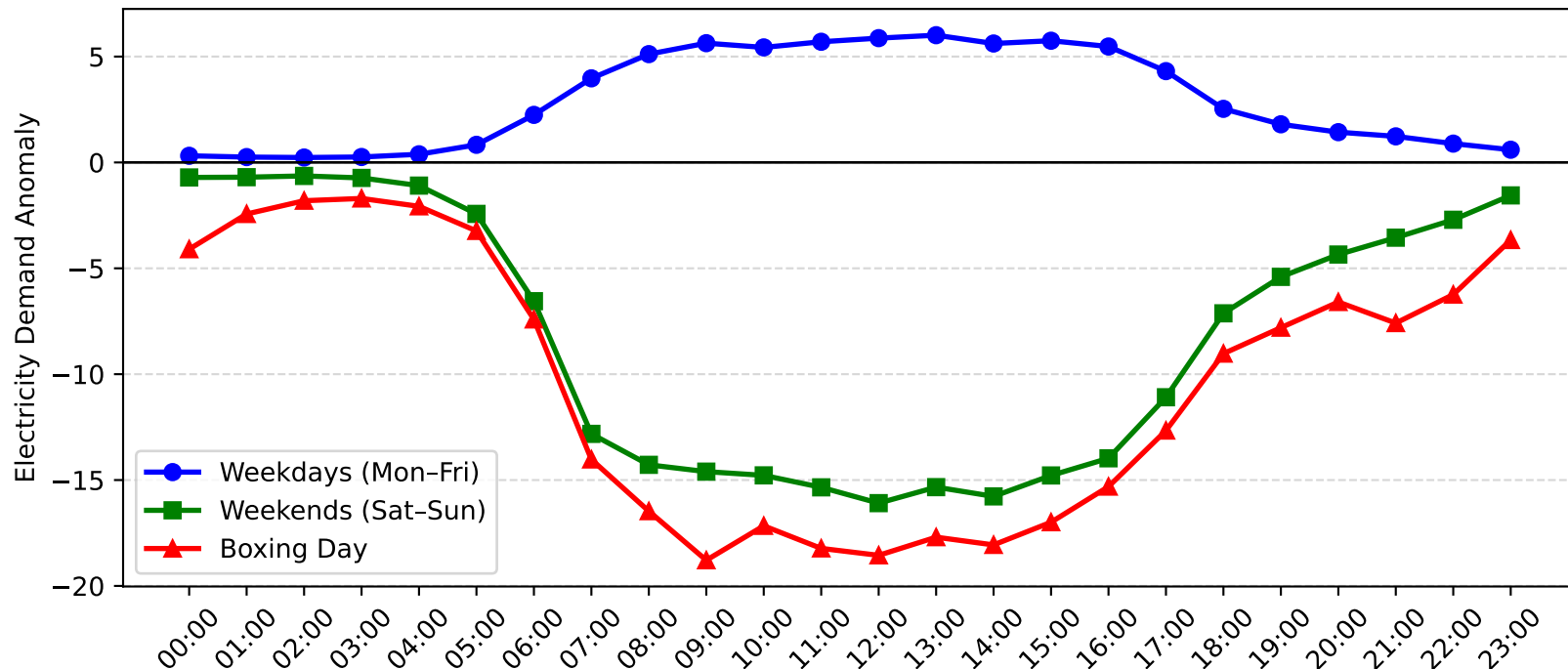
Gore Hill Demand Anomaly: Boxing Day vs Weekday/Weekend (2008-2009)
