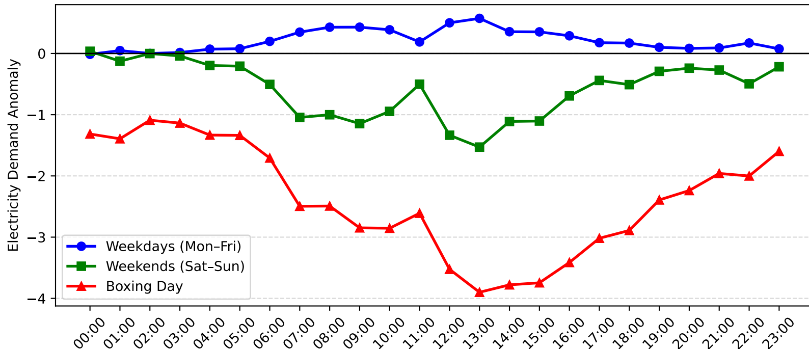
Mayfield West Demand Anomaly: Boxing Day vs Weekday/Weekend (2008-2009)
