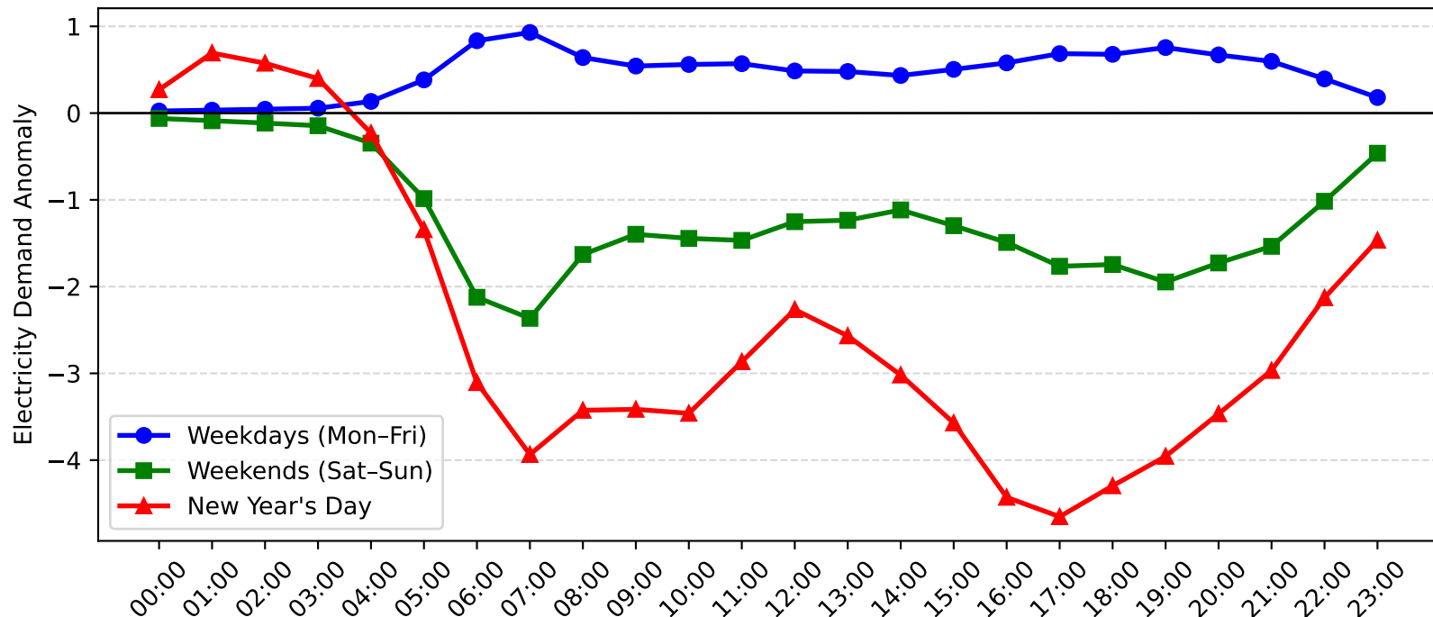
Revesby Demand Anomaly: New Year's Day vs Weekday/Weekend (2016-2017)
