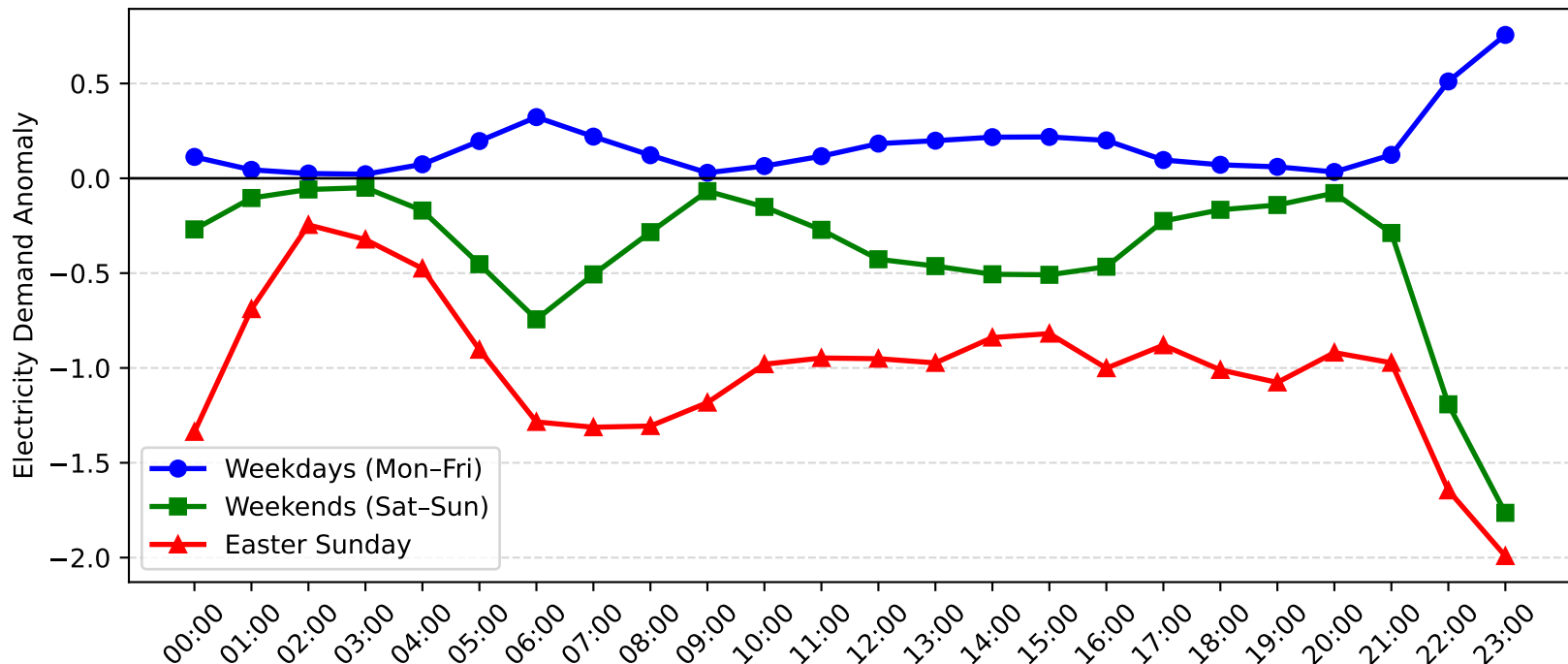
Muswellbrook Demand Anomaly: Easter Sunday vs Weekday/Weekend (2011-2012)
