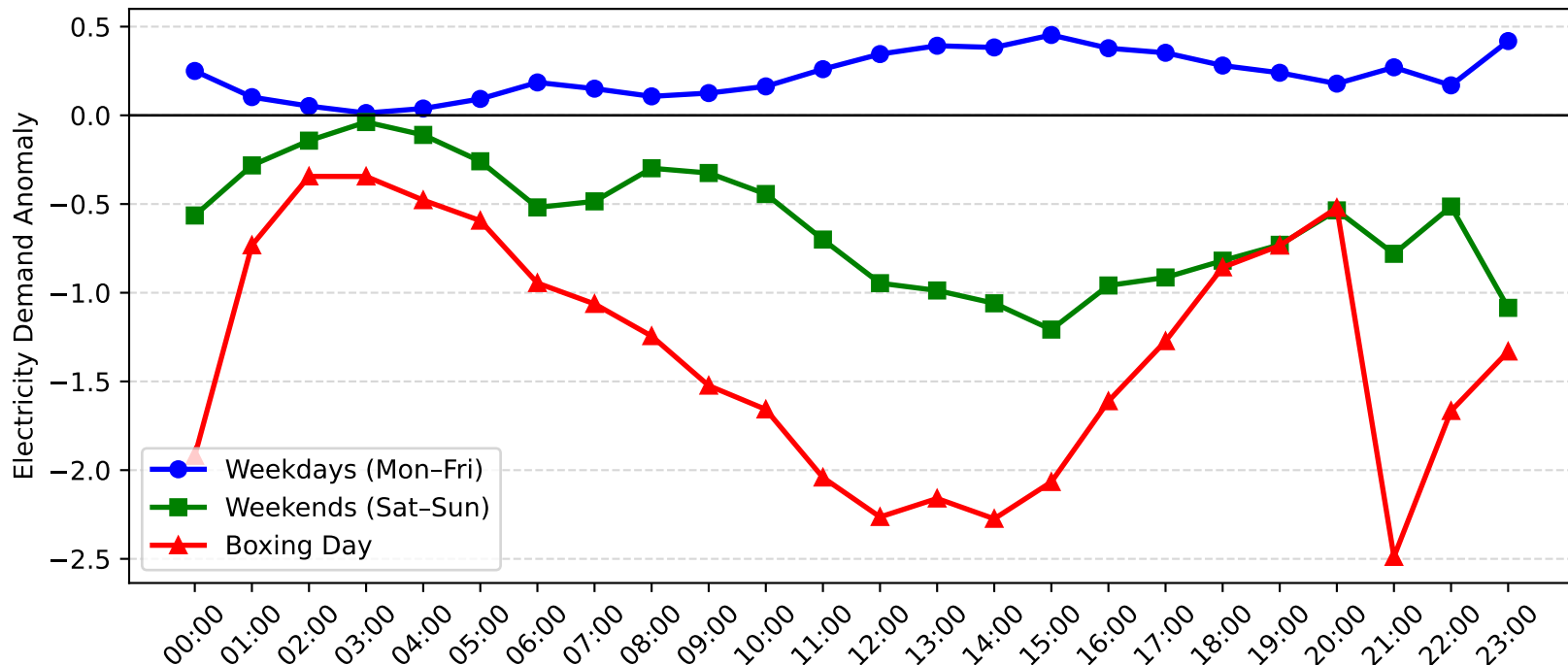
Telarah Demand Anomaly: Boxing Day vs Weekday/Weekend (2008-2009)
