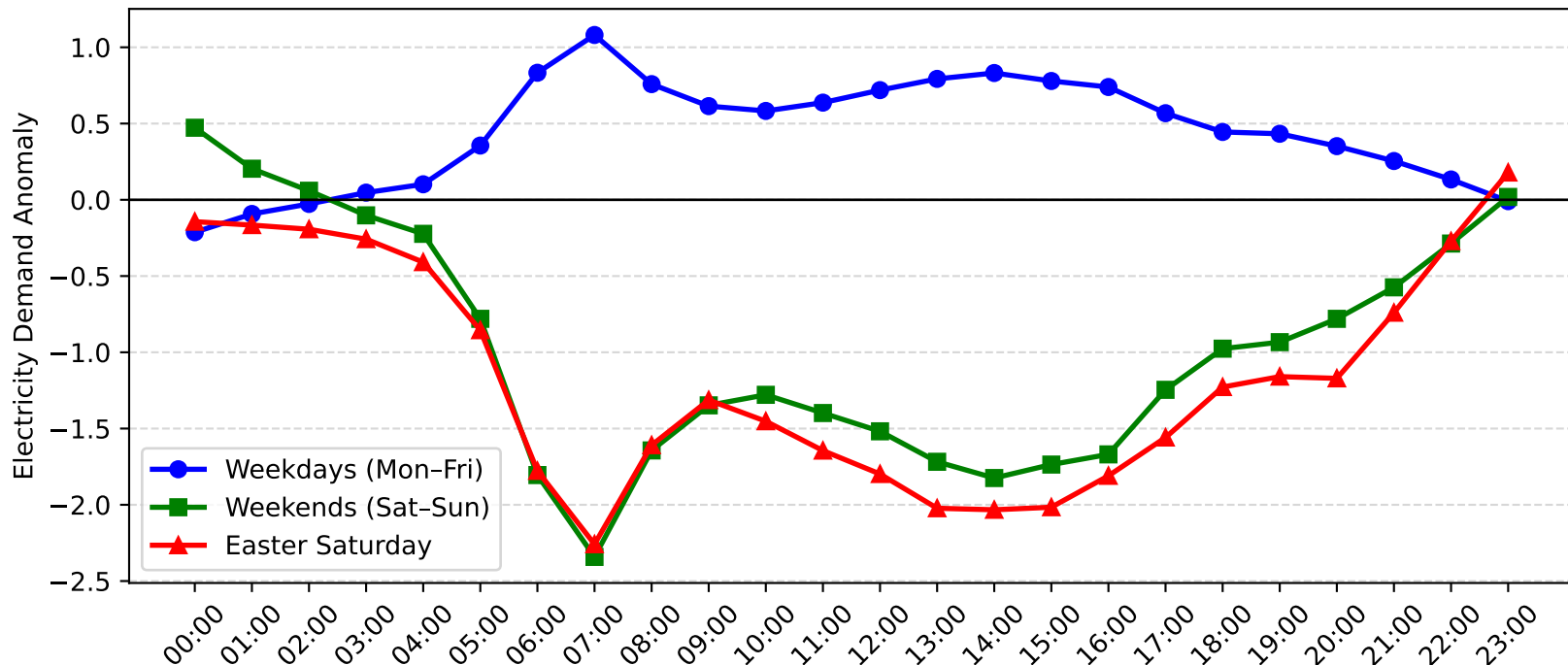
Rockdale Demand Anomaly: Easter Saturday vs Weekday/Weekend (2008-2009)
