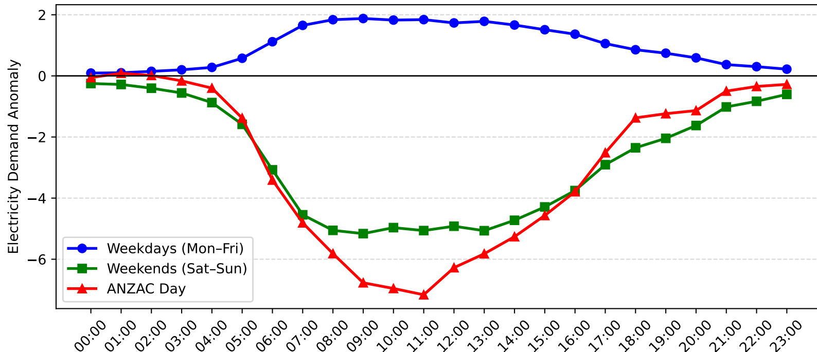
Auburn Demand Anomaly: ANZAC Day vs Weekday/Weekend (2012-2013)
