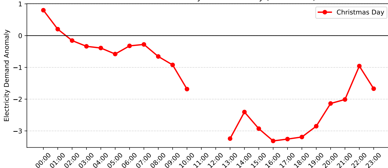
Telarah Demand Anomaly: Christmas Day (2008-2009)
