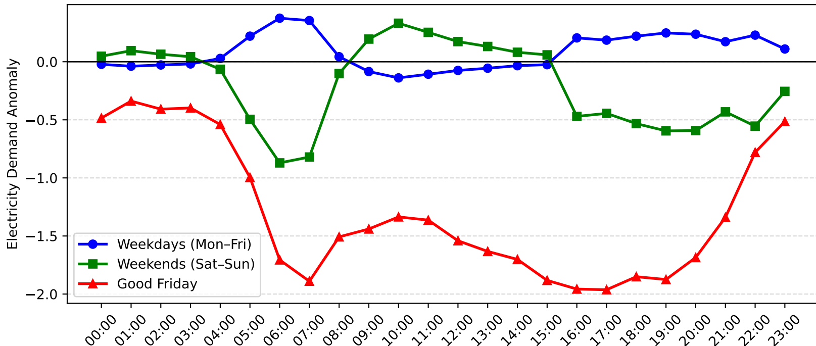
Narrabeen Demand Anomaly: Good Friday vs Weekday/Weekend (2009-2010)
