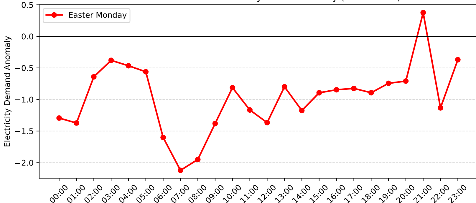
Charlestown Demand Anomaly: Easter Monday (2016-2017)
