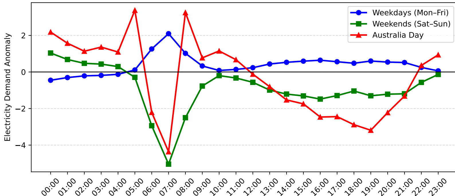
Mosman Demand Anomaly: Australia Day vs Weekday/Weekend (2013-2014)
