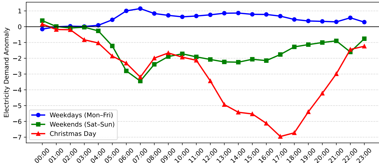
Dee Why West Demand Anomaly: Christmas Day vs Weekday/Weekend (2007-2008)
