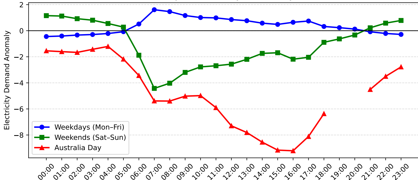
Chatswood Demand Anomaly: Australia Day vs Weekday/Weekend (2017-2018)
