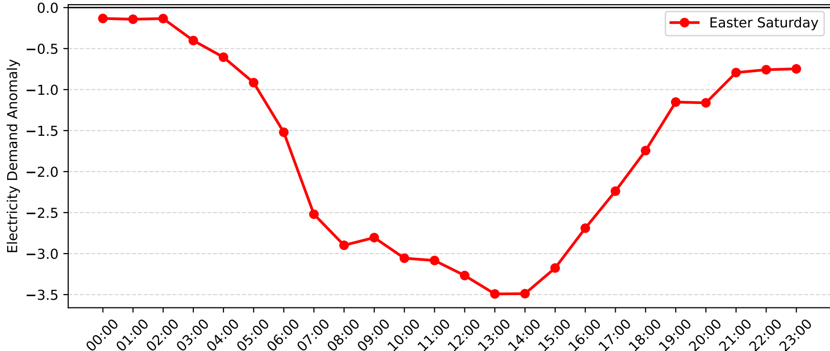
Mayfield West Demand Anomaly: Easter Saturday (2009-2010)
