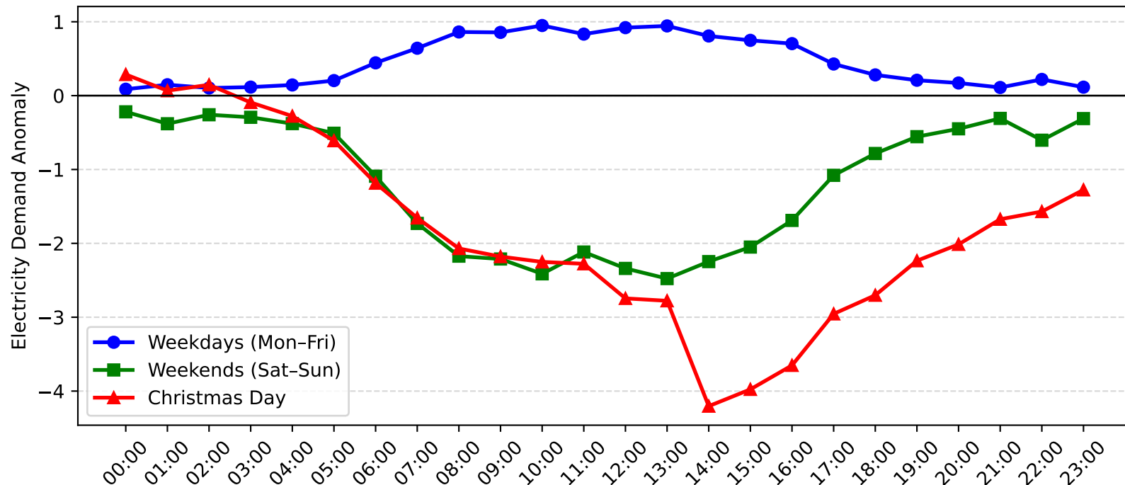
Mayfield West Demand Anomaly: Christmas Day vs Weekday/Weekend (2009-2010)
