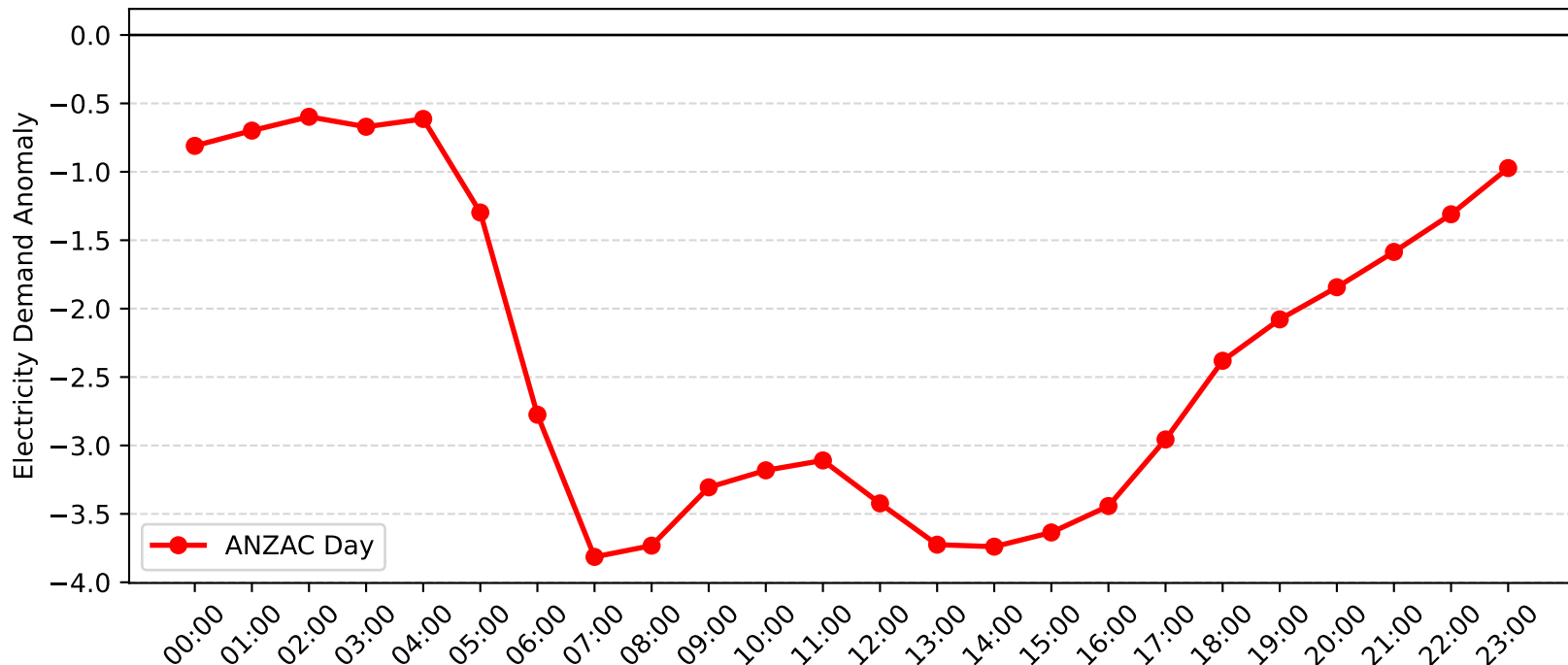
Beacon Hill Demand Anomaly: ANZAC Day (2010-2011)
