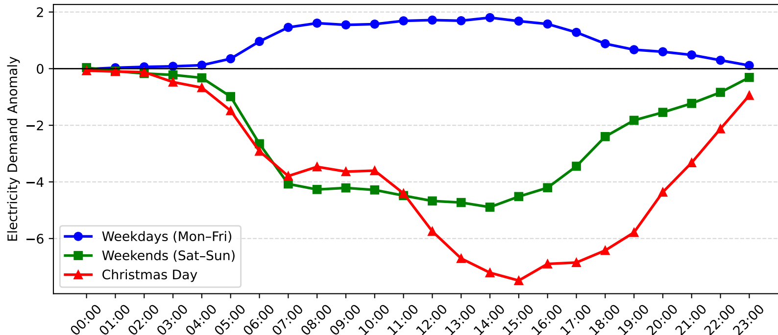
Hunters Hill Demand Anomaly: Christmas Day vs Weekday/Weekend (2014-2015)
