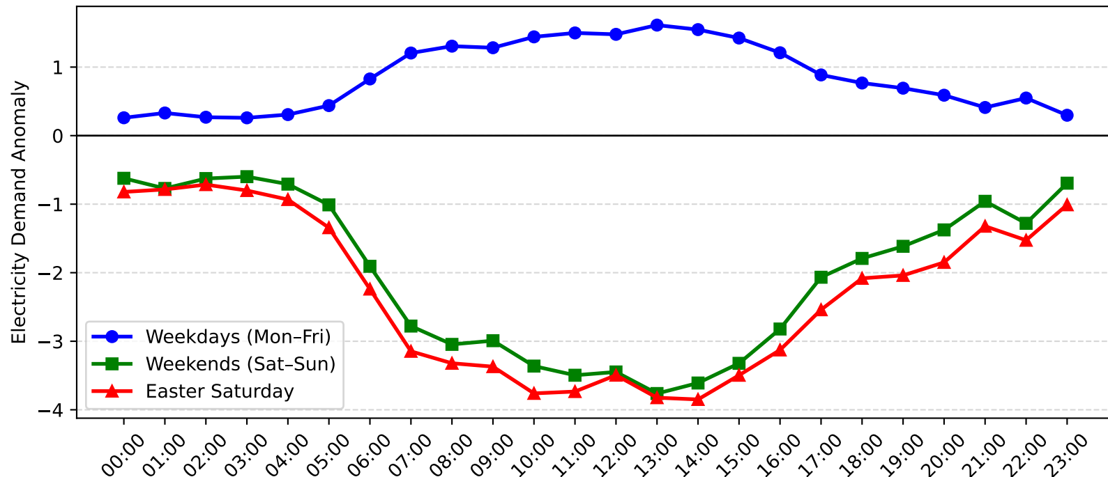
Mayfield West Demand Anomaly: Easter Saturday vs Weekday/Weekend (2011-2012)
