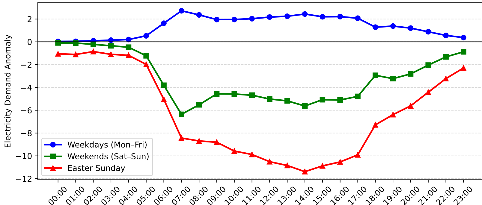
Epping Demand Anomaly: Easter Sunday vs Weekday/Weekend (2013-2014)
