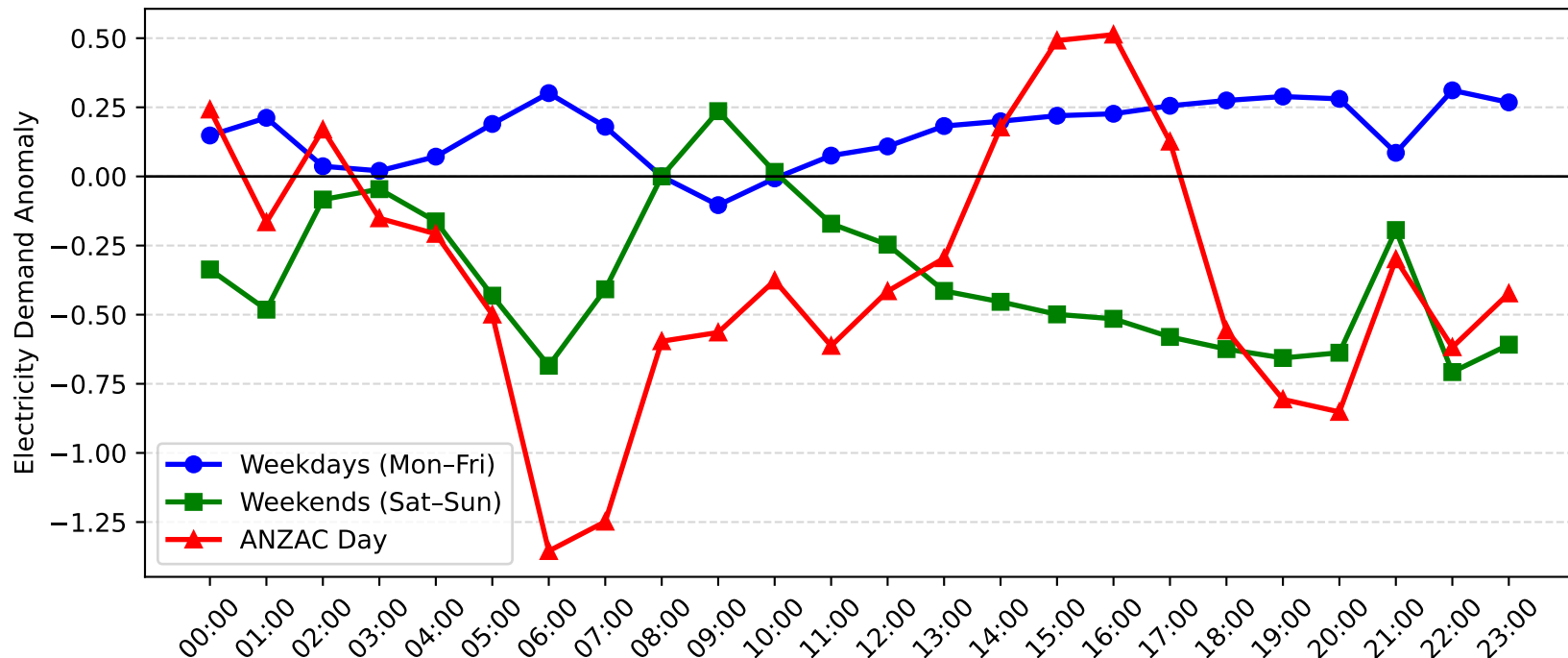
Morisset Demand Anomaly: ANZAC Day vs Weekday/Weekend (2017-2018)
