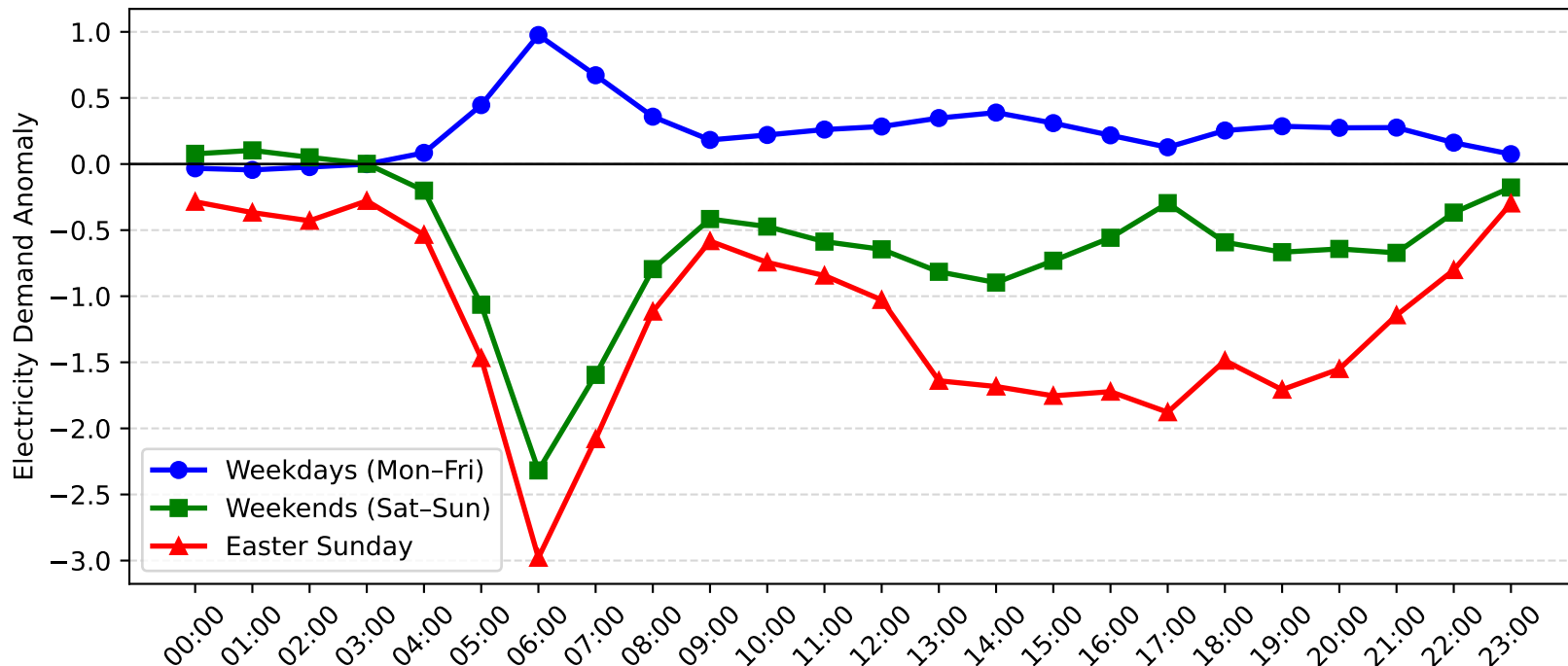
Berowra Demand Anomaly: Easter Sunday vs Weekday/Weekend (2006-2007)
