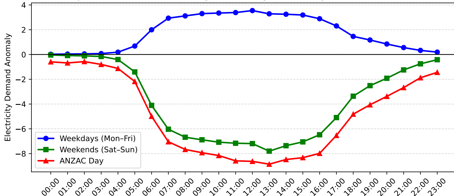
Macquarie Park Demand Anomaly: ANZAC Day vs Weekday/Weekend (2009-2010)
