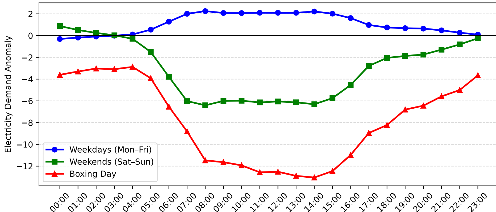
Marrickville Demand Anomaly: Boxing Day vs Weekday/Weekend (2013-2014)
