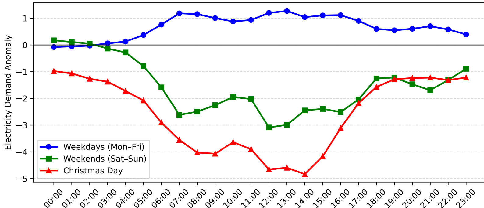
Bass Hill Demand Anomaly: Christmas Day vs Weekday/Weekend (2004-2005)
