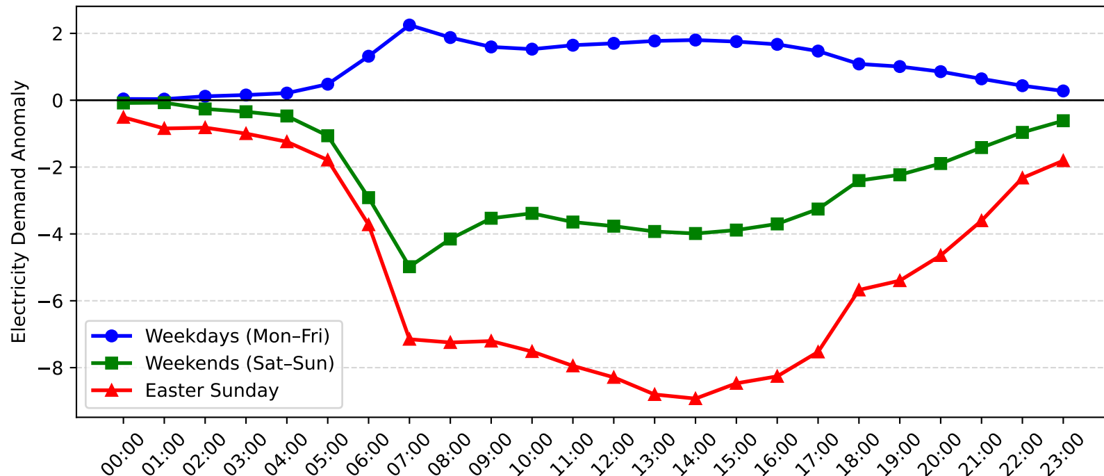
Epping Demand Anomaly: Easter Sunday vs Weekday/Weekend (2017-2018)
