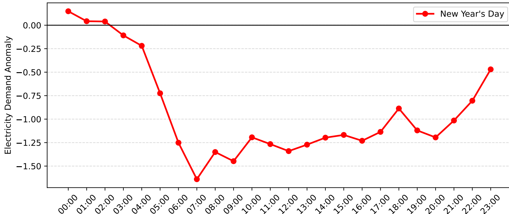
Narrabeen Demand Anomaly: New Year's Day (2014-2015)
