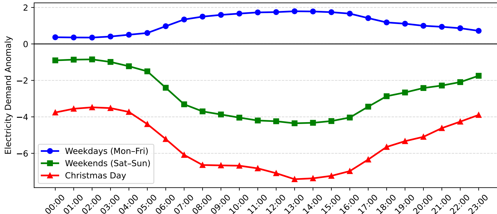
Leightonfield Demand Anomaly: Christmas Day vs Weekday/Weekend (2015-2016)
