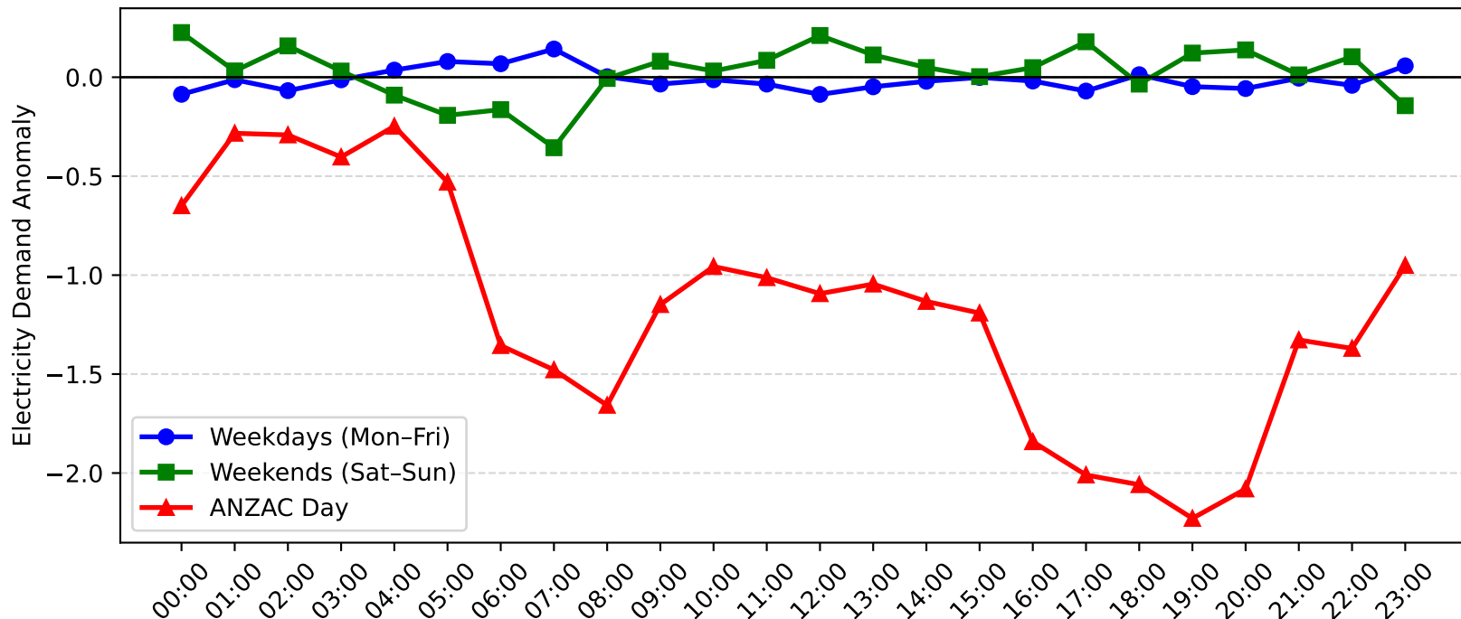
Woy Woy Demand Anomaly: ANZAC Day vs Weekday/Weekend (2004-2005)
