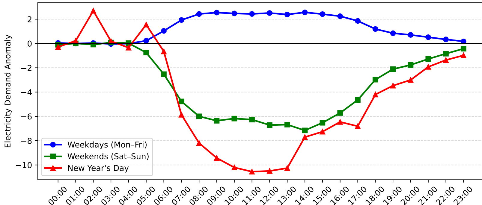
Green Square Demand Anomaly: New Year's Day vs Weekday/Weekend (2016-2017)
