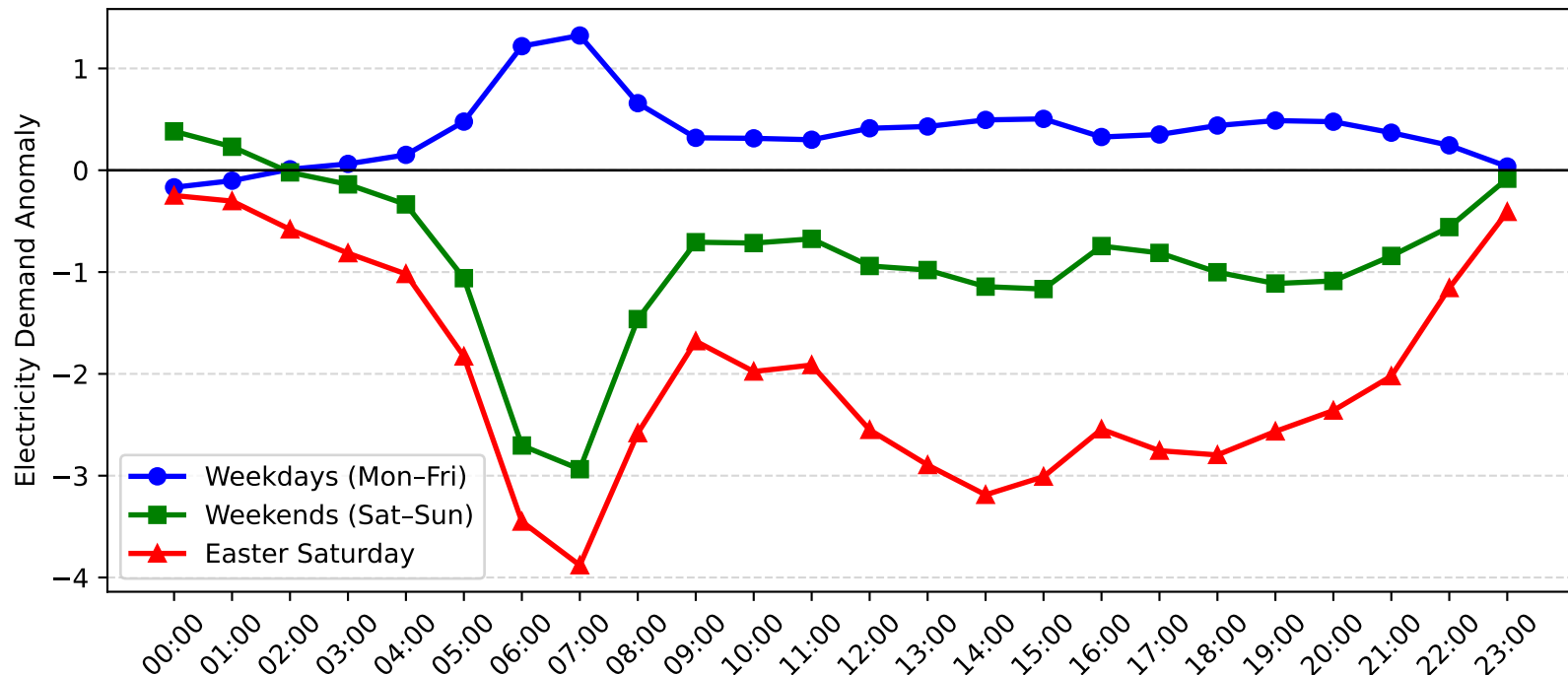
Mortdale Demand Anomaly: Easter Saturday vs Weekday/Weekend (2016-2017)
