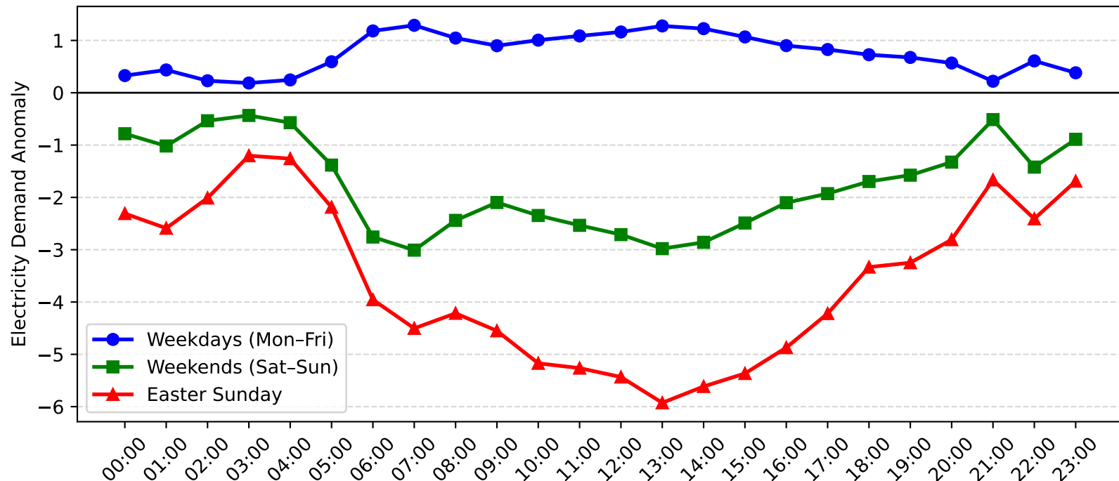
Argenton Demand Anomaly: Easter Sunday vs Weekday/Weekend (2014-2015)
