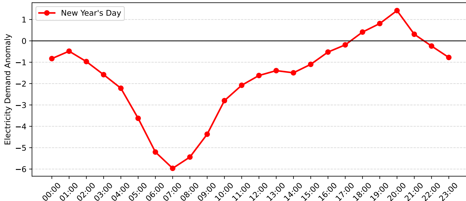
Enfield Demand Anomaly: New Year's Day (2005-2006)
