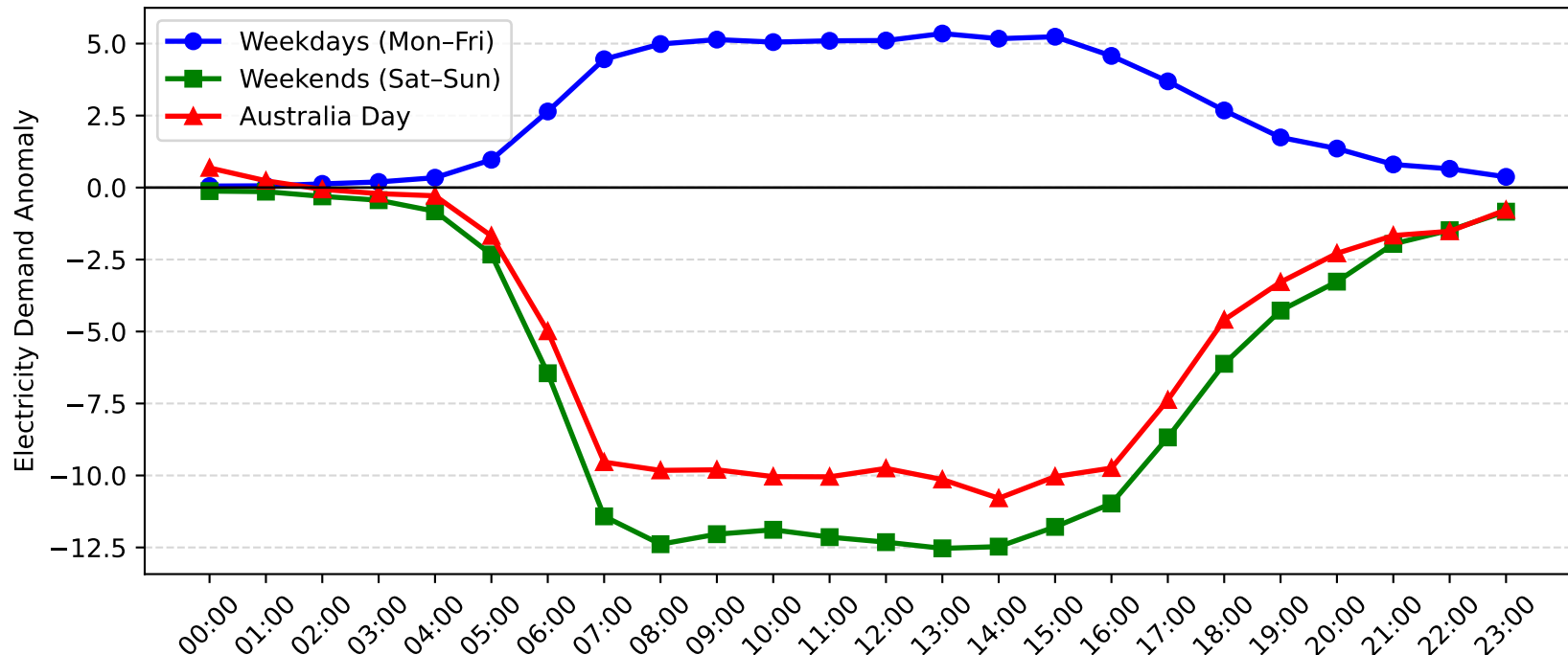
Zetland Demand Anomaly: Australia Day vs Weekday/Weekend (2008-2009)
