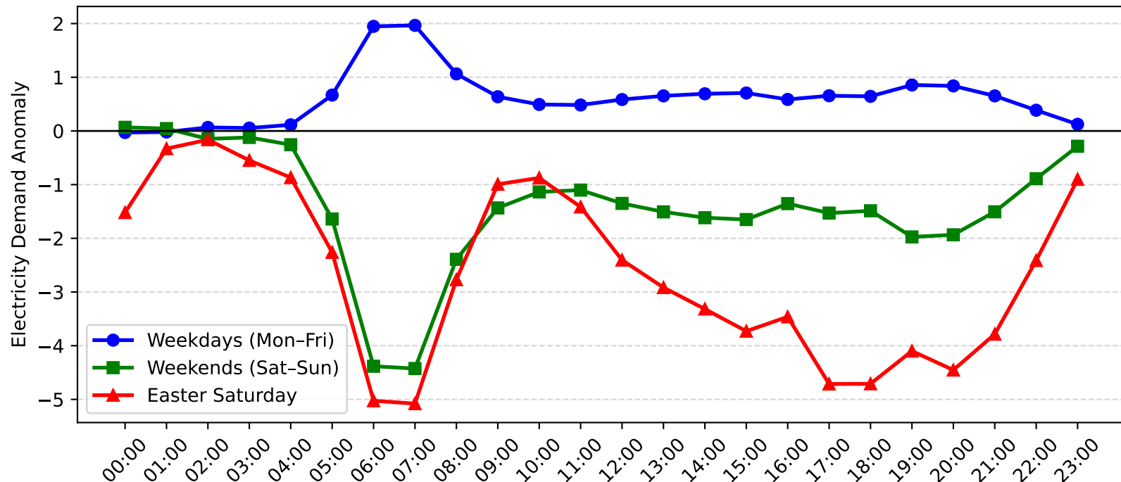
Pennant Hills Demand Anomaly: Easter Saturday vs Weekday/Weekend (2015-2016)
