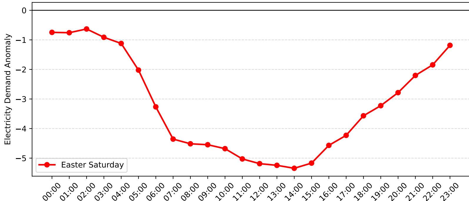
Sefton Demand Anomaly: Easter Saturday (2016-2017)
