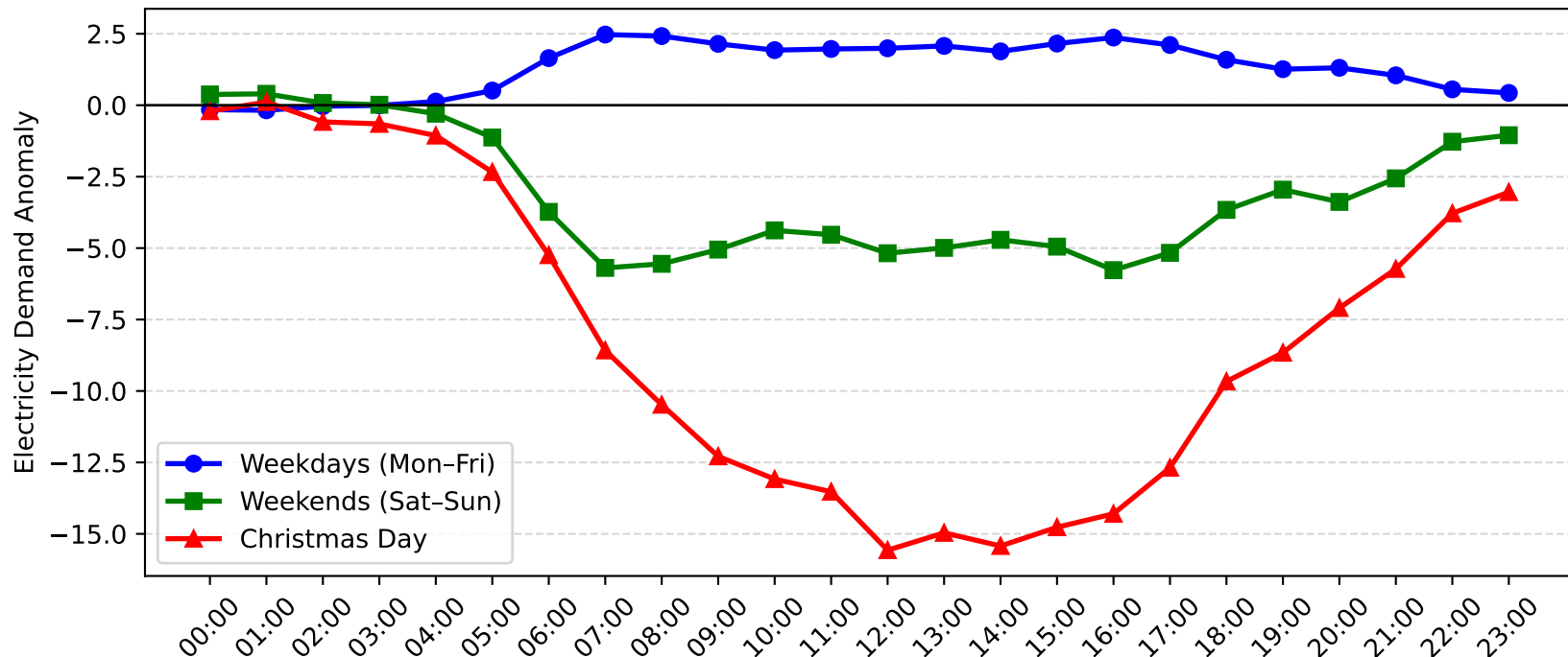
Burwood Demand Anomaly: Christmas Day vs Weekday/Weekend (2005-2006)
