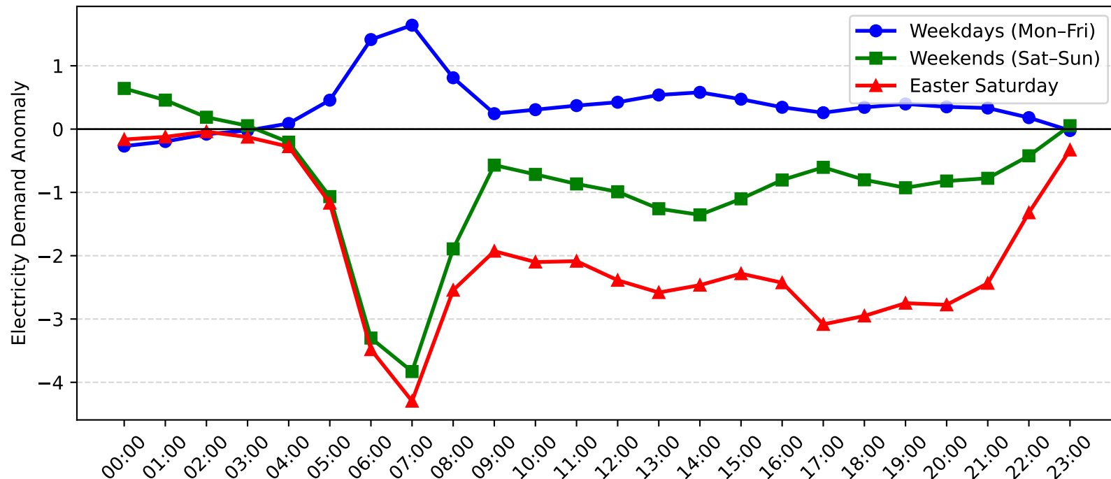
Mortdale Demand Anomaly: Easter Saturday vs Weekday/Weekend (2012-2013)
