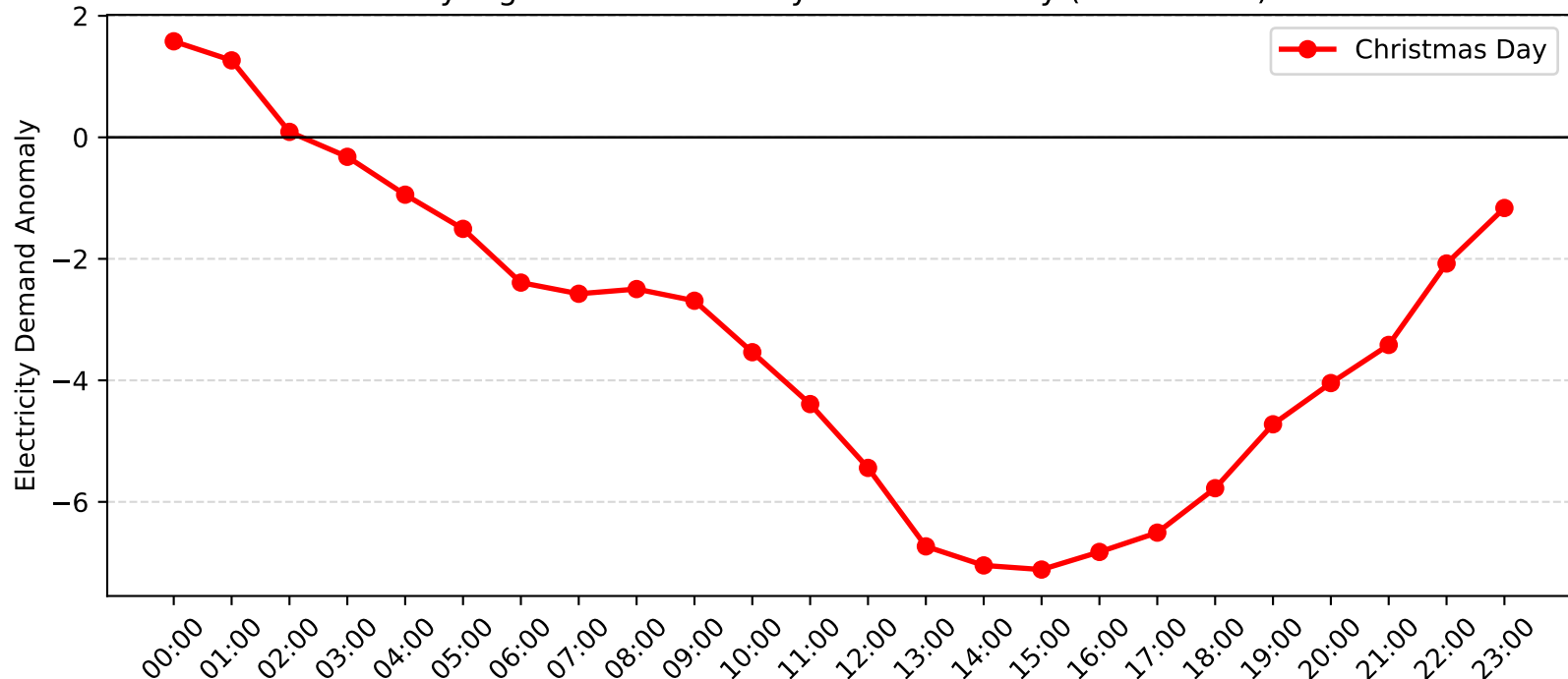
Wyong Demand Anomaly: Christmas Day (2012-2013)
