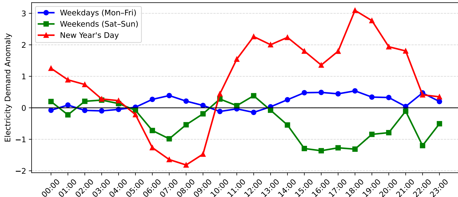
Charlestown Demand Anomaly: New Year's Day vs Weekday/Weekend (2012-2013)
