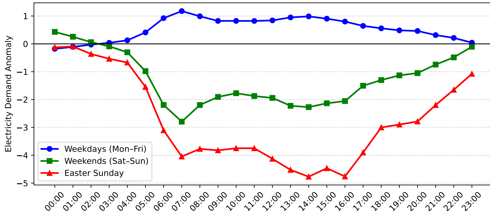
Rockdale Demand Anomaly: Easter Sunday vs Weekday/Weekend (2006-2007)
