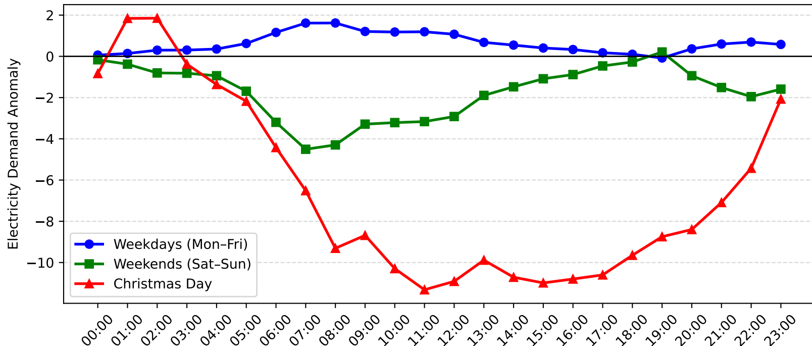
Meadowbank Demand Anomaly: Christmas Day vs Weekday/Weekend (2014-2015)
