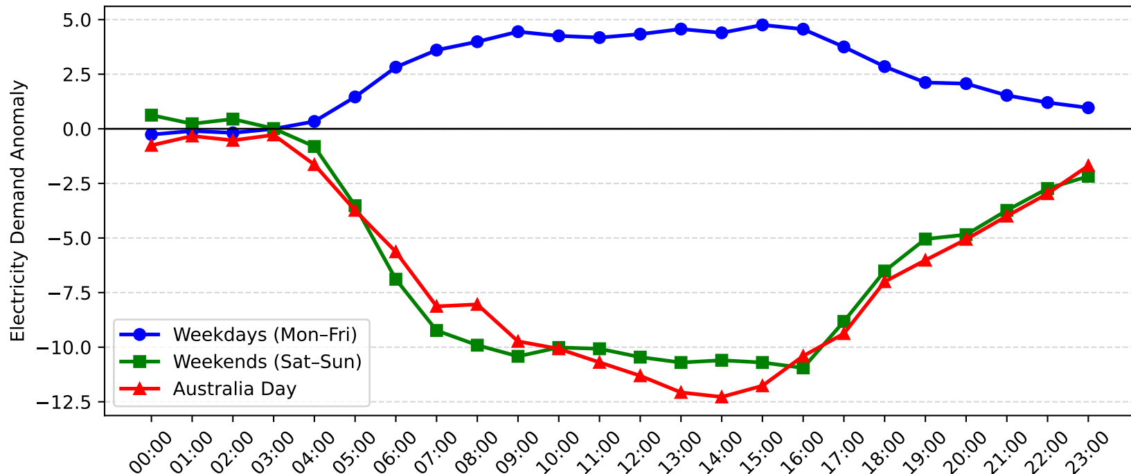
Greenacre Park Demand Anomaly: Australia Day vs Weekday/Weekend (2008-2009)
