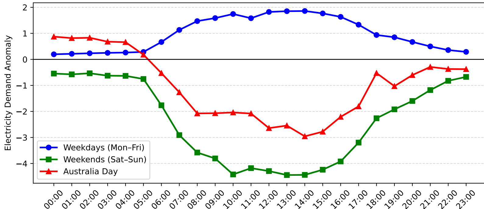
Mascot Demand Anomaly: Australia Day vs Weekday/Weekend (2004-2005)
