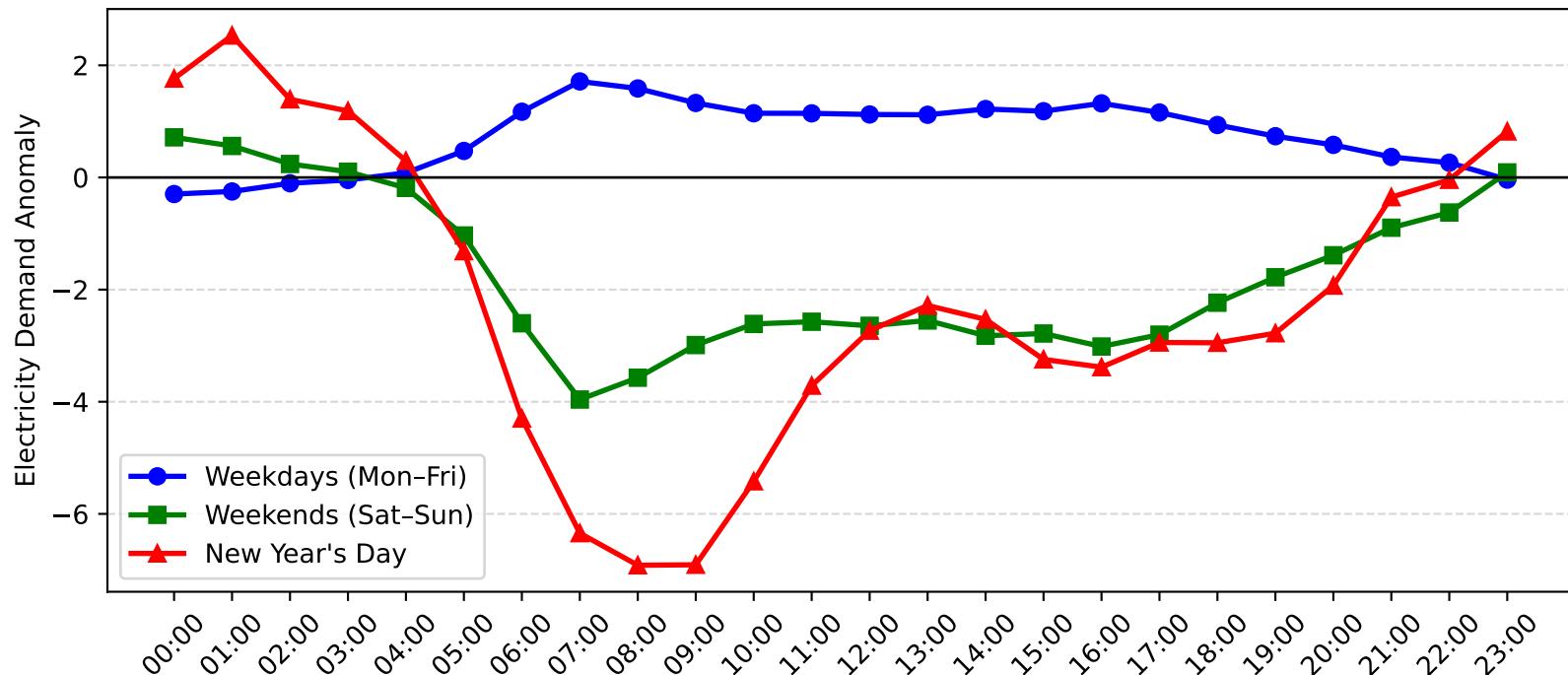
Kogarah Demand Anomaly: New Year's Day vs Weekday/Weekend (2011-2012)
