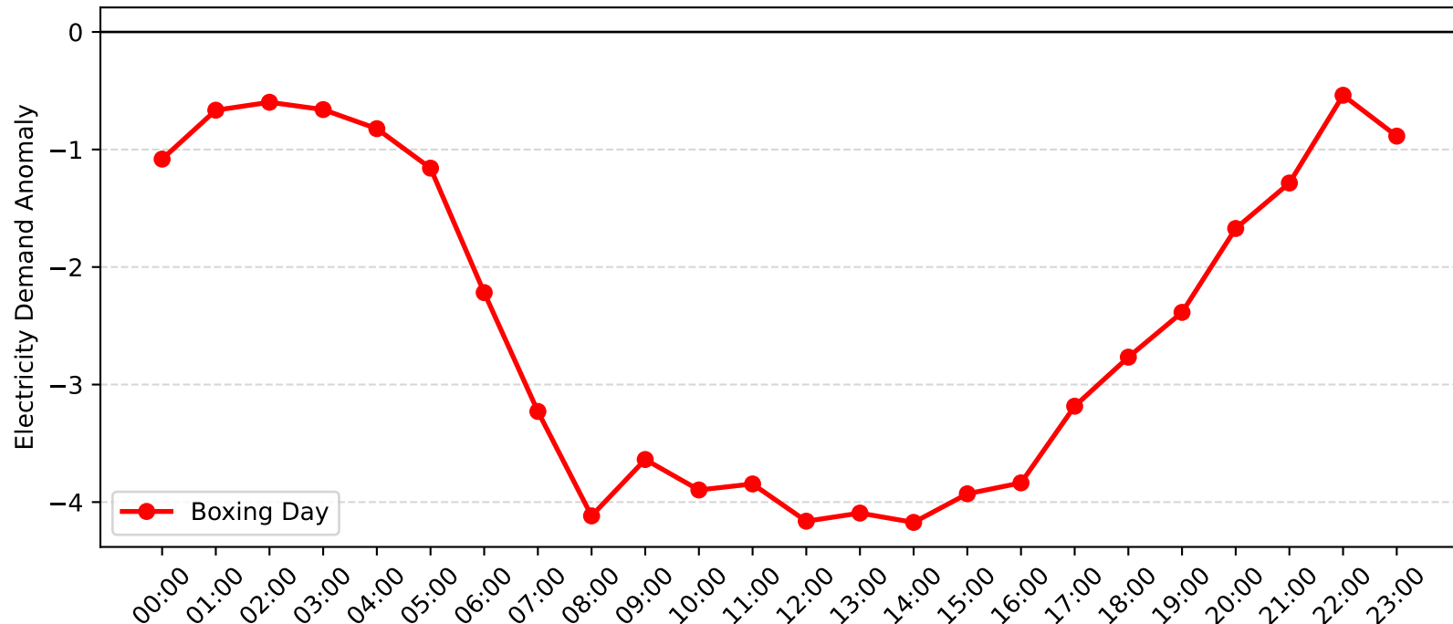
Beacon Hill Demand Anomaly: Boxing Day (2007-2008)
