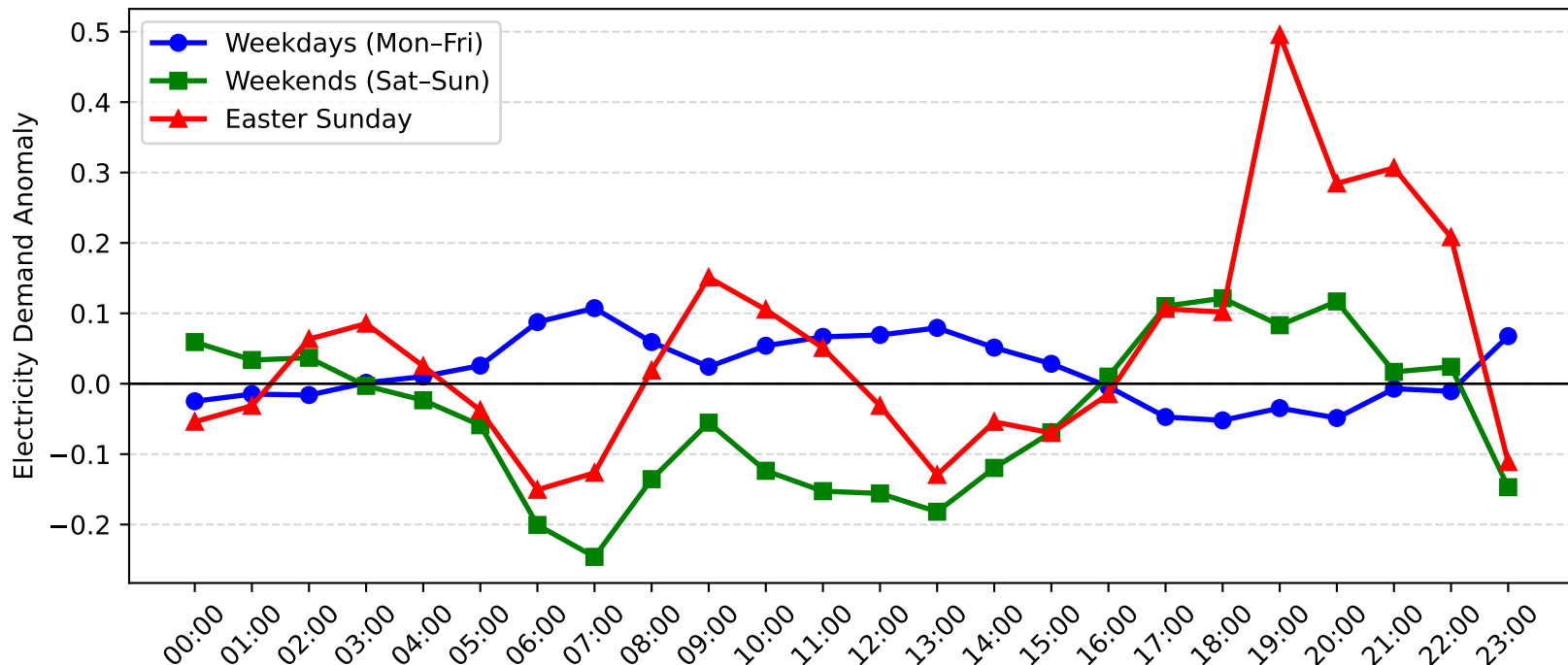
Rothbury Demand Anomaly: Easter Sunday vs Weekday/Weekend (2007-2008)
