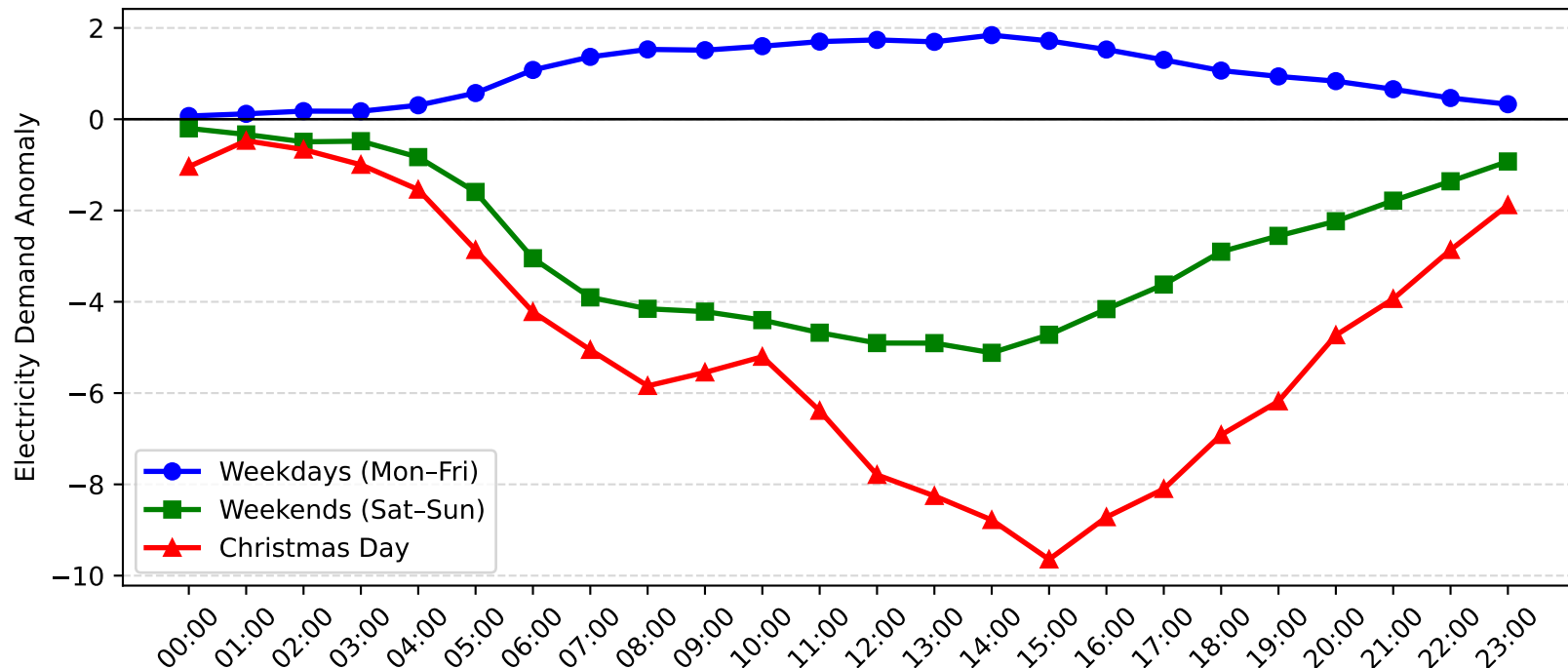
Sefton Demand Anomaly: Christmas Day vs Weekday/Weekend (2014-2015)
