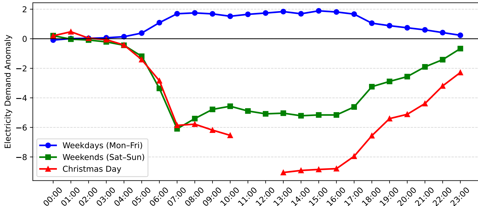
Chatswood Demand Anomaly: Christmas Day vs Weekday/Weekend (2008-2009)
