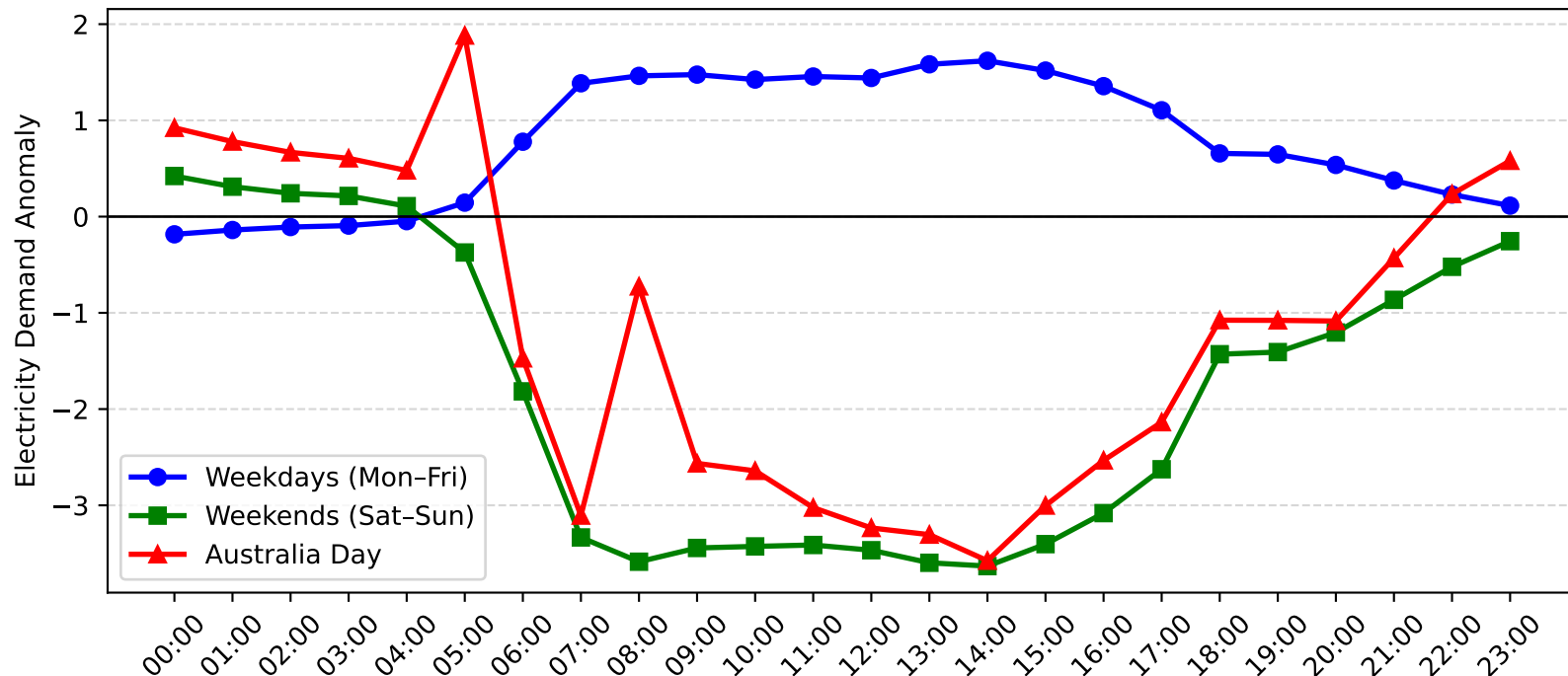
Concord Demand Anomaly: Australia Day vs Weekday/Weekend (2013-2014)
