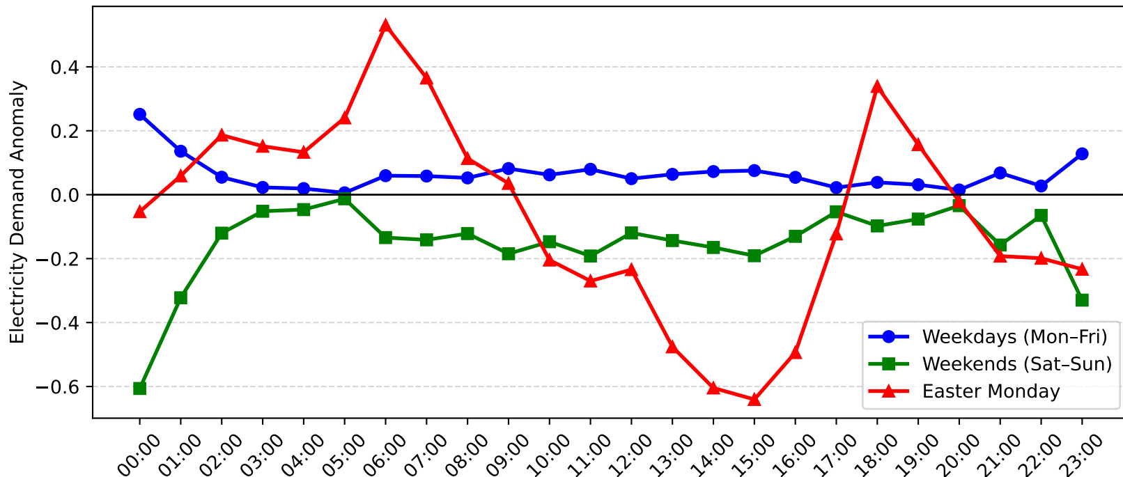
Telarah Demand Anomaly: Easter Monday vs Weekday/Weekend (2004-2005)
