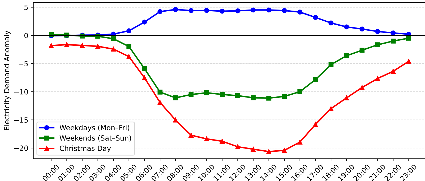
Zetland Demand Anomaly: Christmas Day vs Weekday/Weekend (2006-2007)
