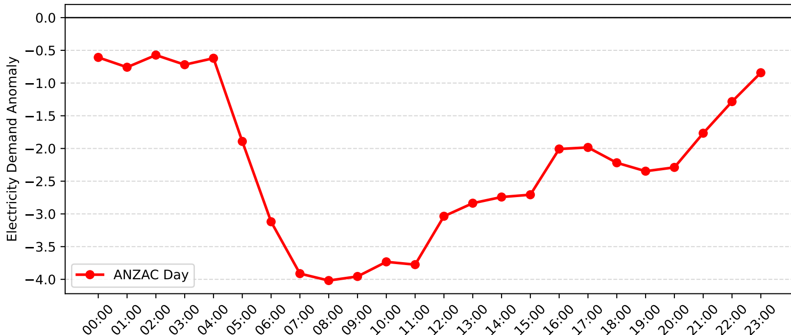
Charmhaven Demand Anomaly: ANZAC Day (2015-2016)
