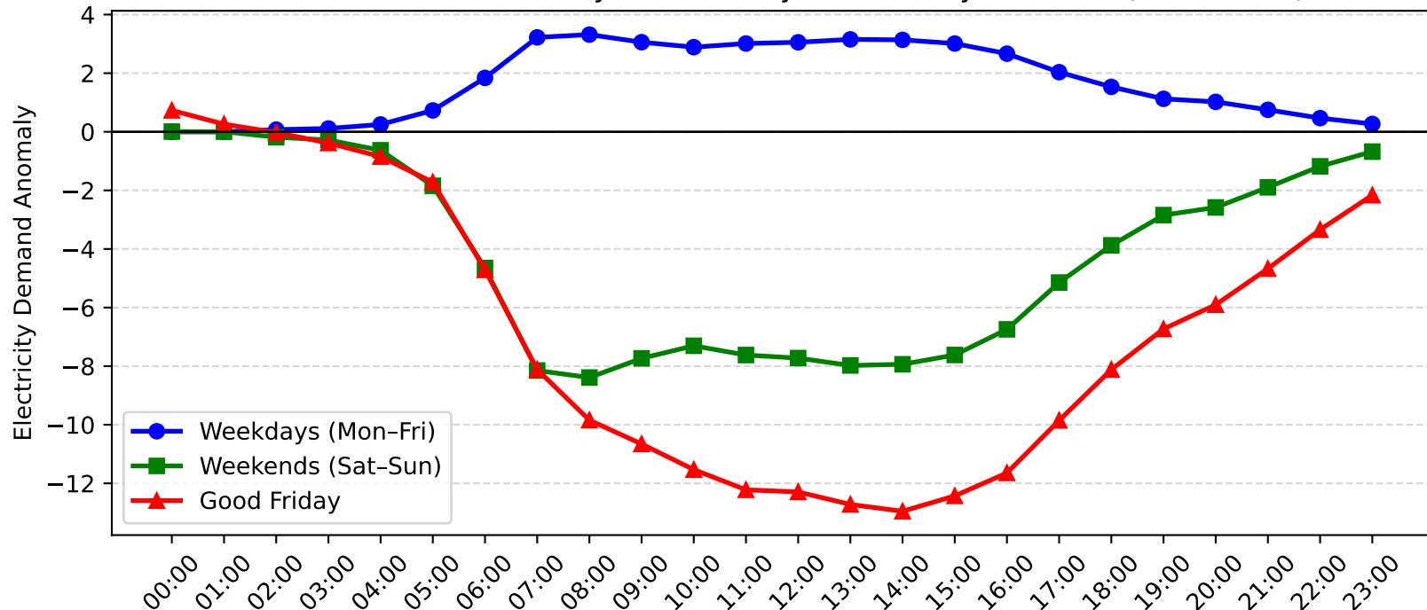
Zetland Demand Anomaly: Good Friday vs Weekday/Weekend (2013-2014)
