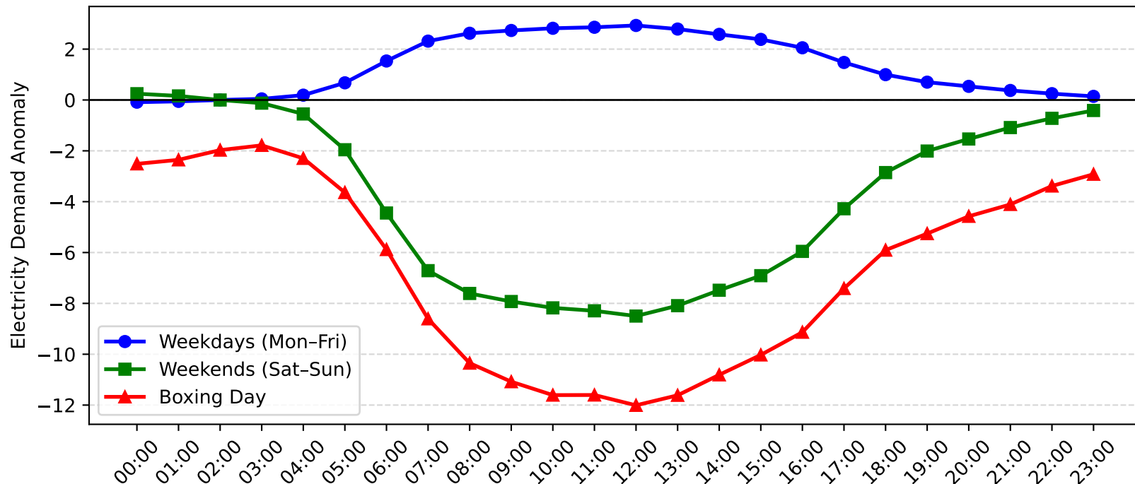
Homebush Bay Demand Anomaly: Boxing Day vs Weekday/Weekend (2012-2013)
