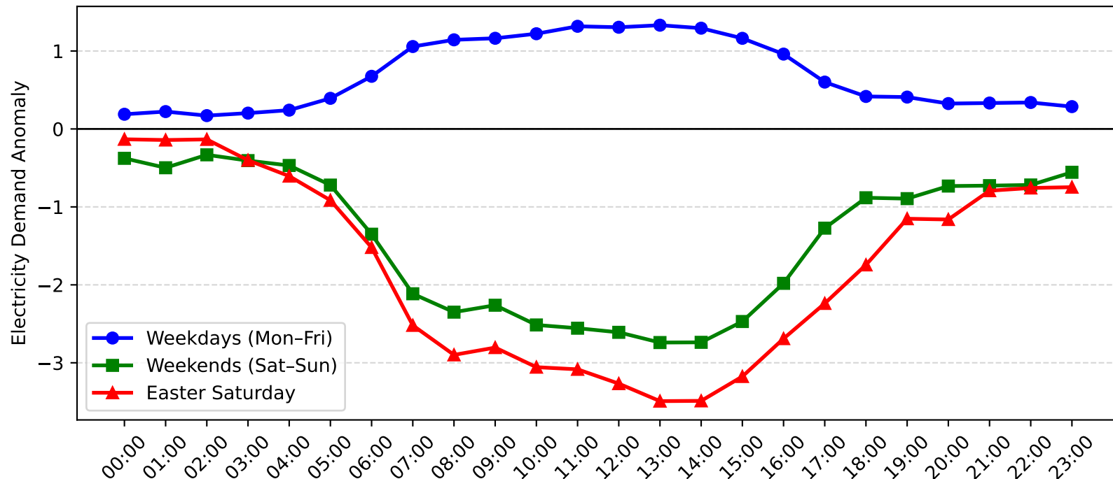
Mayfield West Demand Anomaly: Easter Saturday vs Weekday/Weekend (2009-2010)
