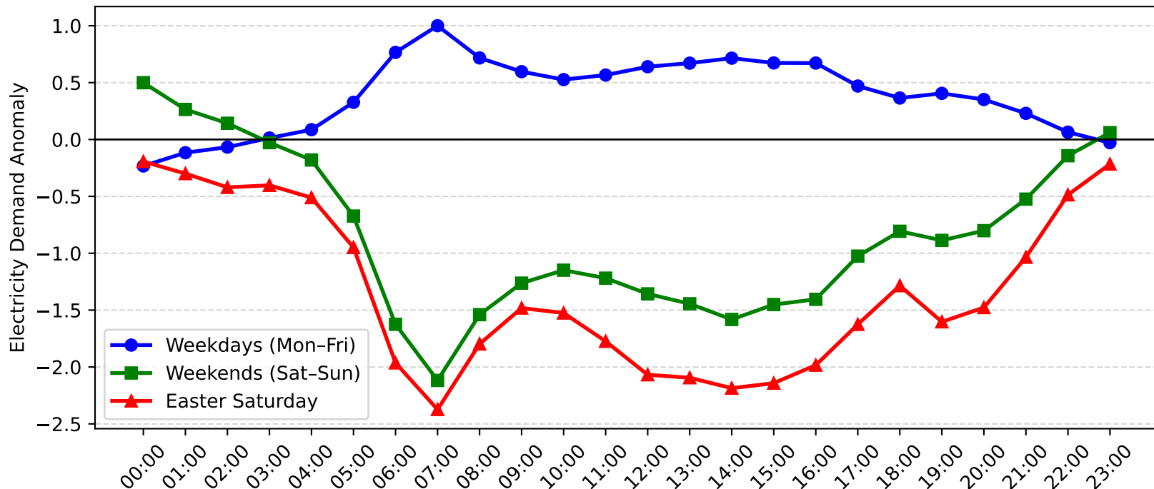
Rockdale Demand Anomaly: Easter Saturday vs Weekday/Weekend (2009-2010)
