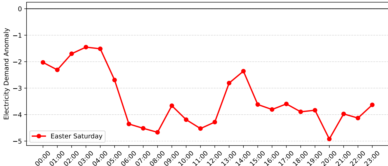
Meadowbank Demand Anomaly: Easter Saturday (2013-2014)
