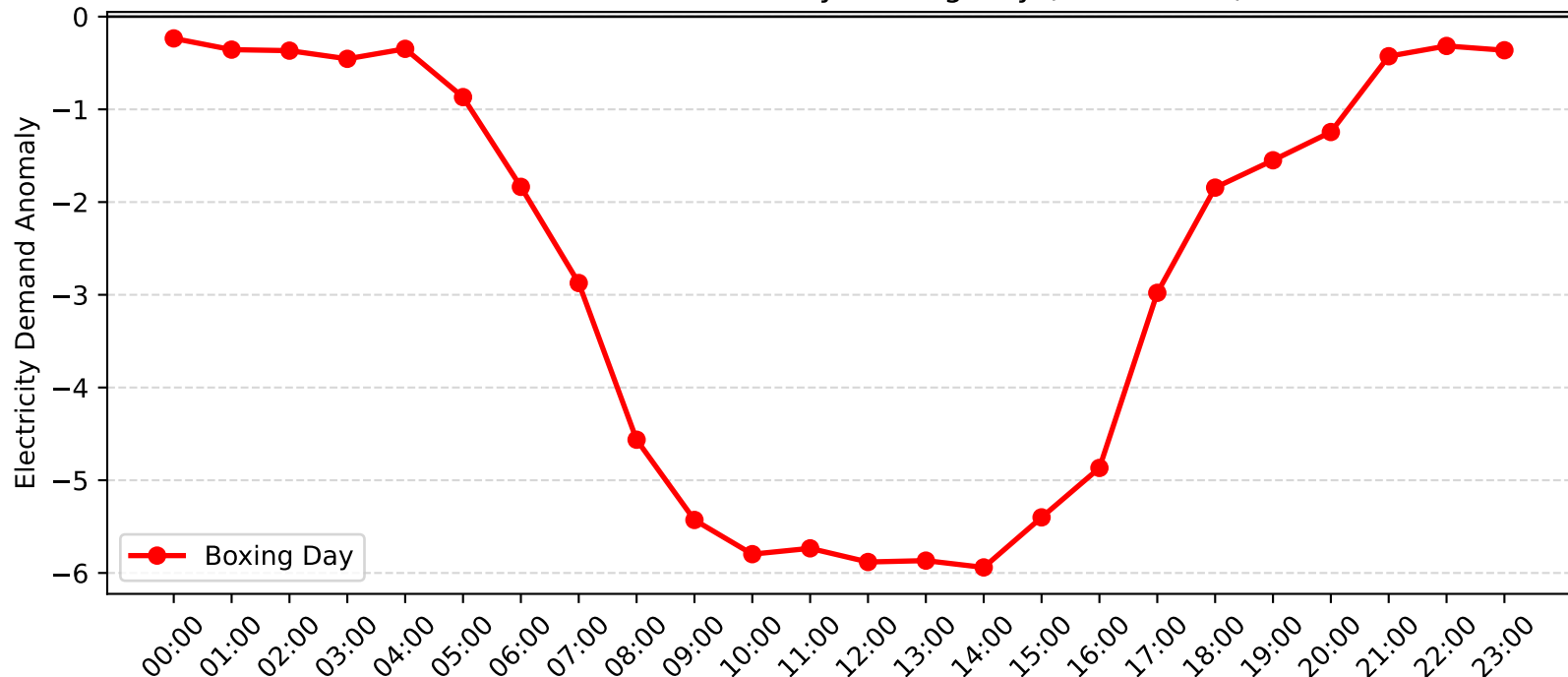
Auburn Demand Anomaly: Boxing Day (2004-2005)
