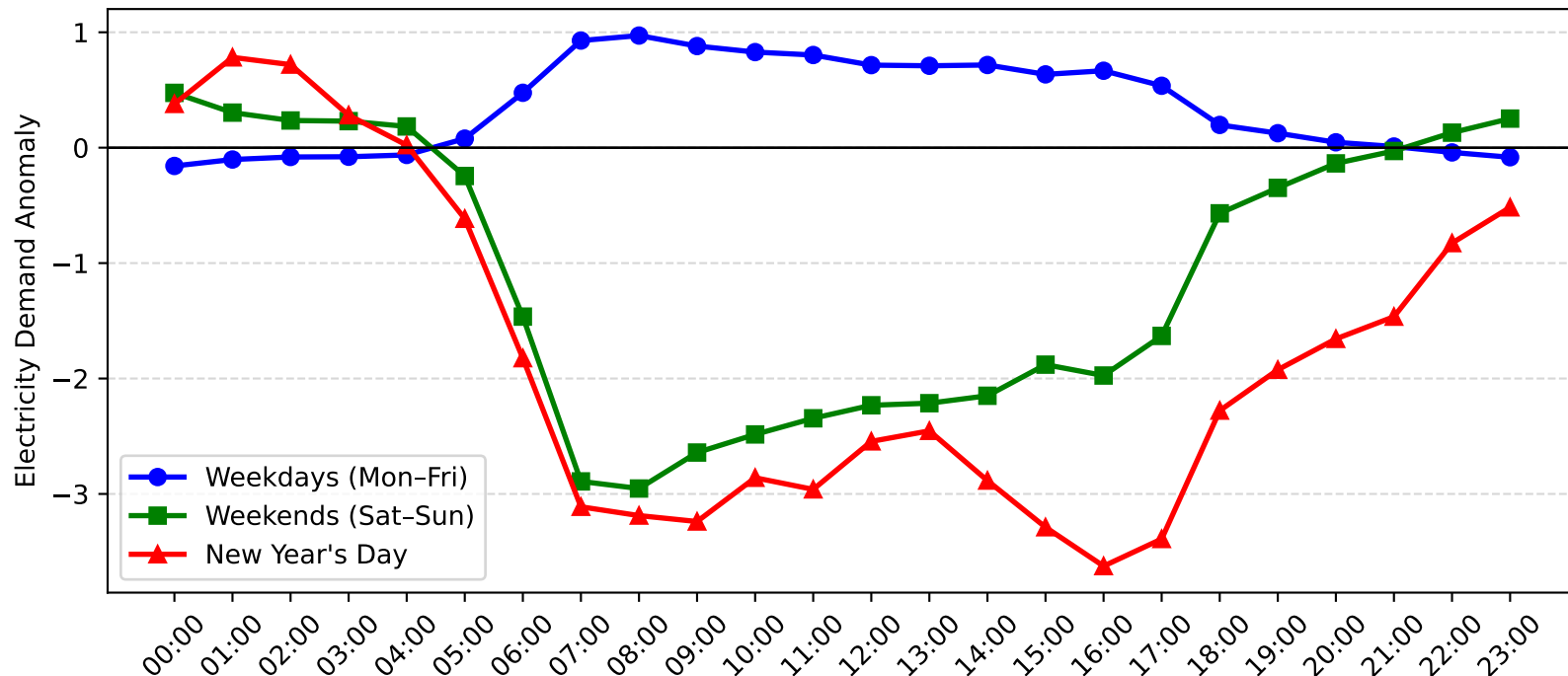
Pymble Demand Anomaly: New Year's Day vs Weekday/Weekend (2014-2015)
