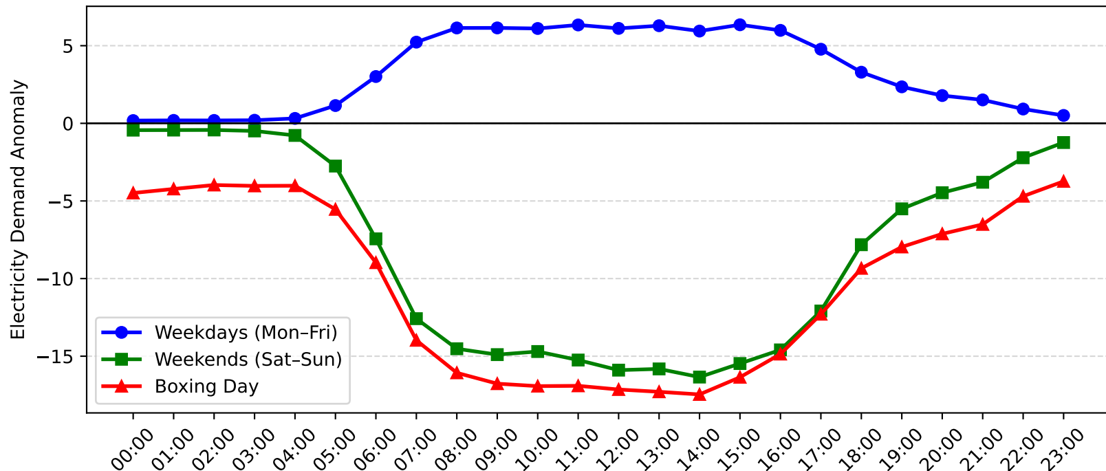
Gore Hill Demand Anomaly: Boxing Day vs Weekday/Weekend (2005-2006)
