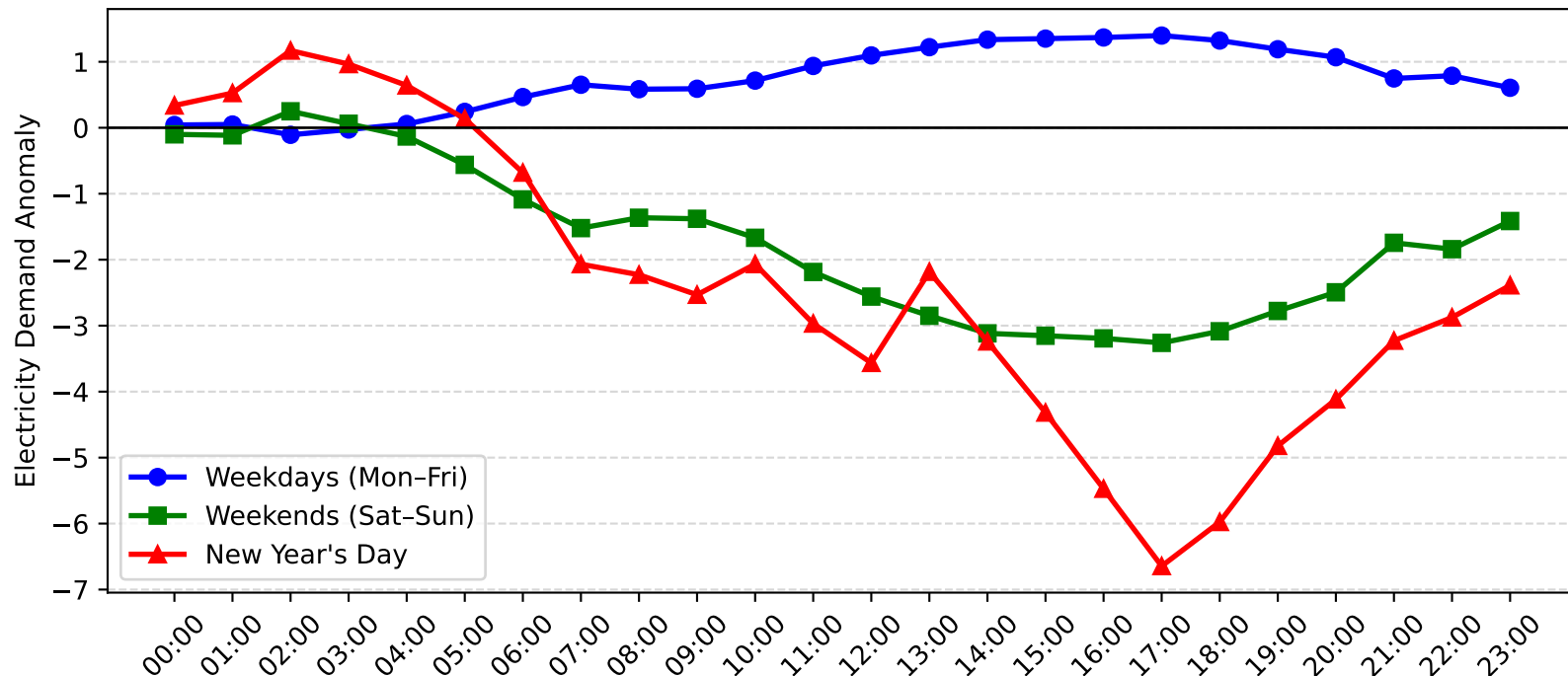
Jesmond Demand Anomaly: New Year's Day vs Weekday/Weekend (2017-2018)
