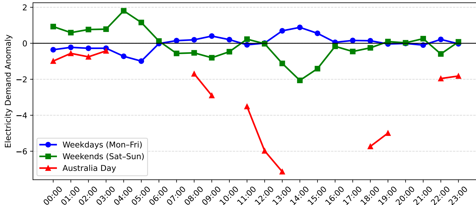
Adamstown Demand Anomaly: Australia Day vs Weekday/Weekend (2017-2018)
