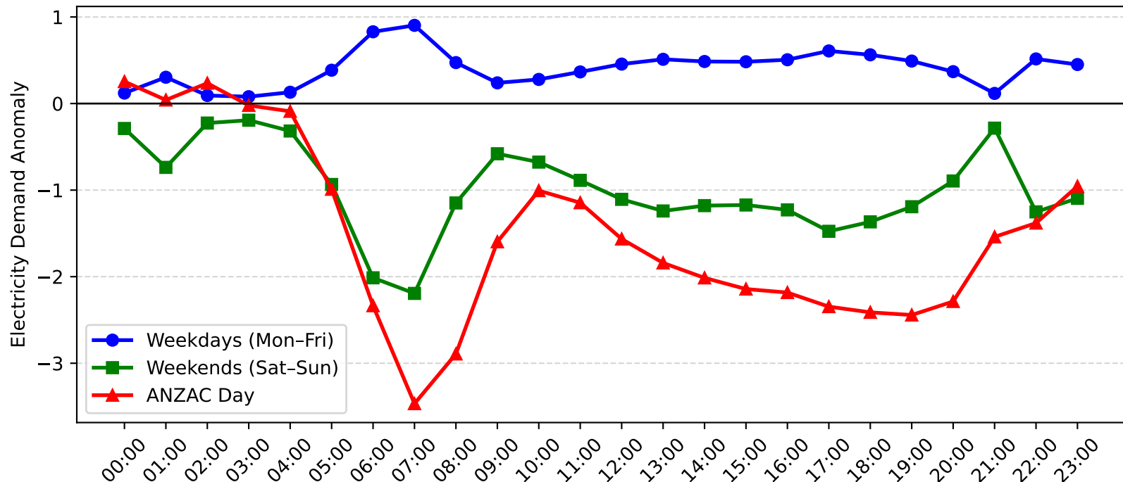
Jesmond Demand Anomaly: ANZAC Day vs Weekday/Weekend (2014-2015)
