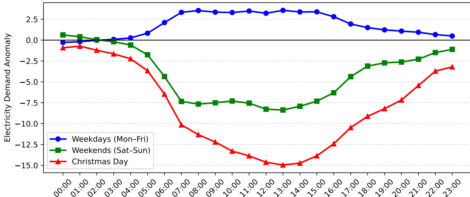
Marrickville Demand Anomaly: Christmas Day vs Weekday/Weekend (2004-2005)
