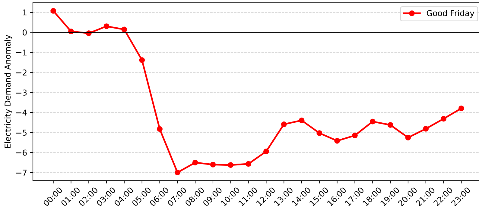
Meadowbank Demand Anomaly: Good Friday (2011-2012)
