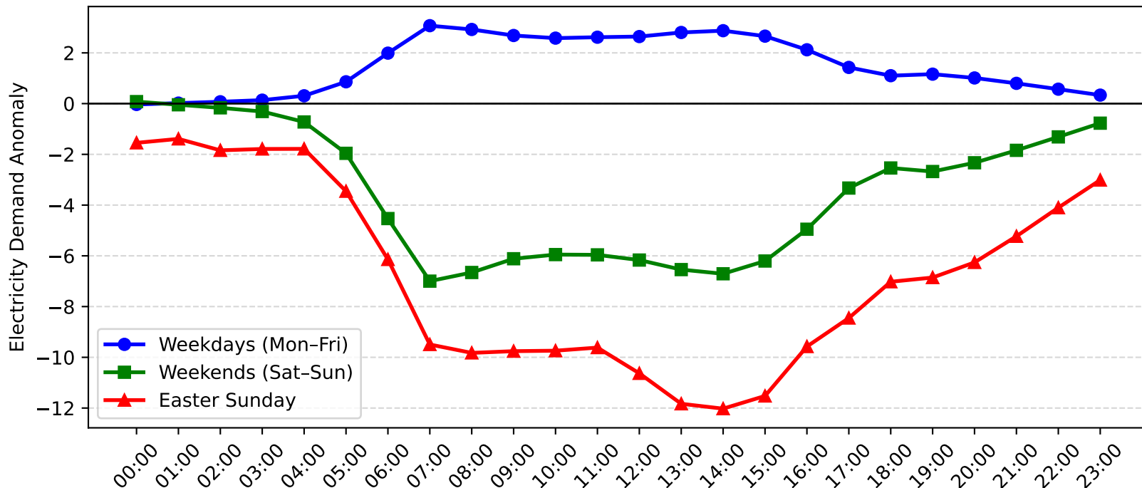
Marrickville Demand Anomaly: Easter Sunday vs Weekday/Weekend (2015-2016)
