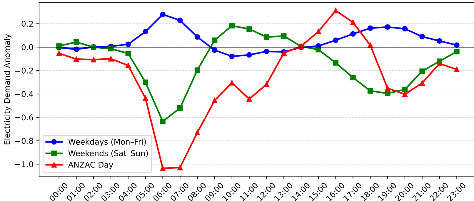
Narrabeen Demand Anomaly: ANZAC Day vs Weekday/Weekend (2016-2017)
