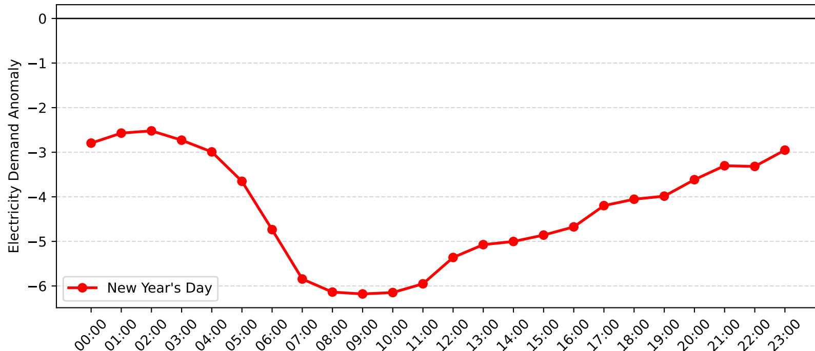
Leightonfield Demand Anomaly: New Year's Day (2013-2014)
