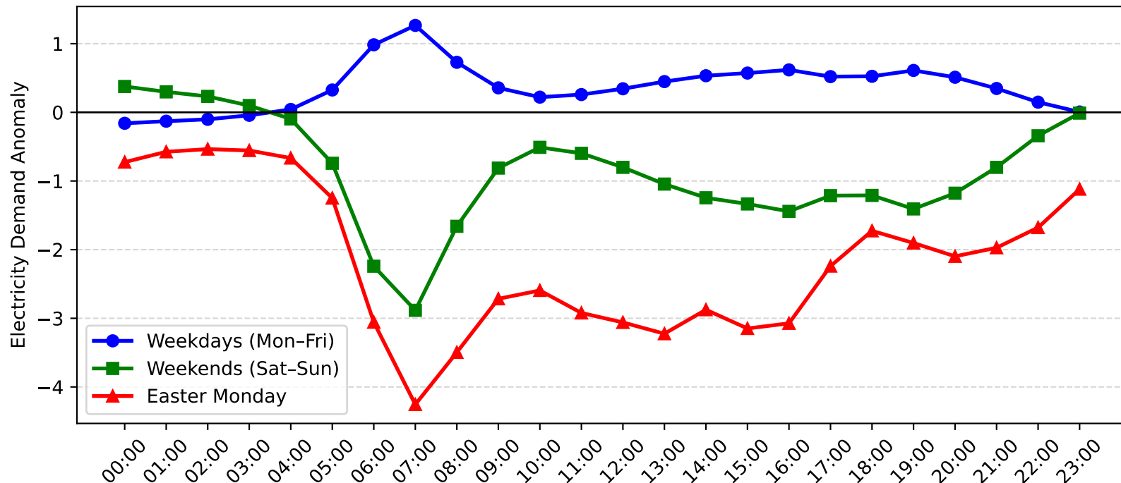
Five Dock Demand Anomaly: Easter Monday vs Weekday/Weekend (2015-2016)
