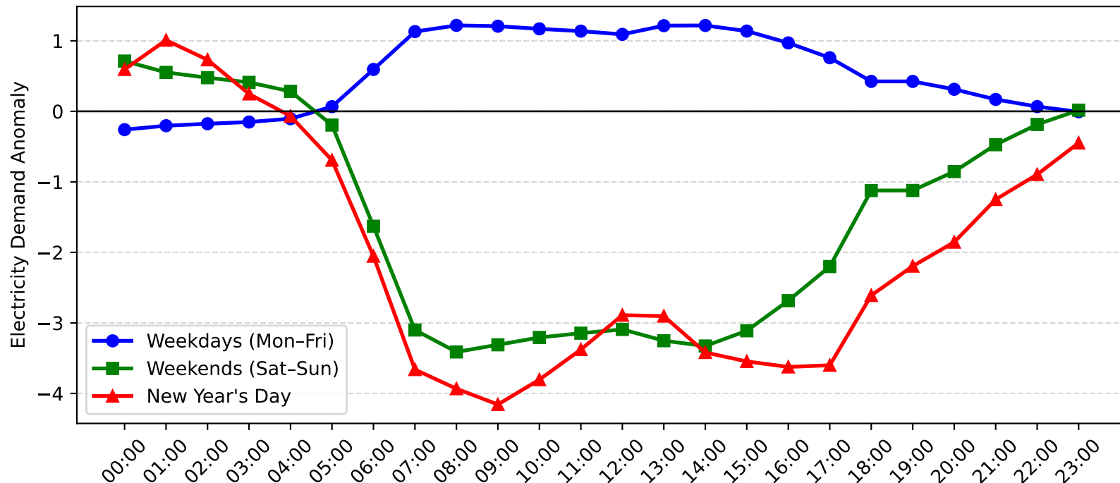
Concord Demand Anomaly: New Year's Day vs Weekday/Weekend (2013-2014)
