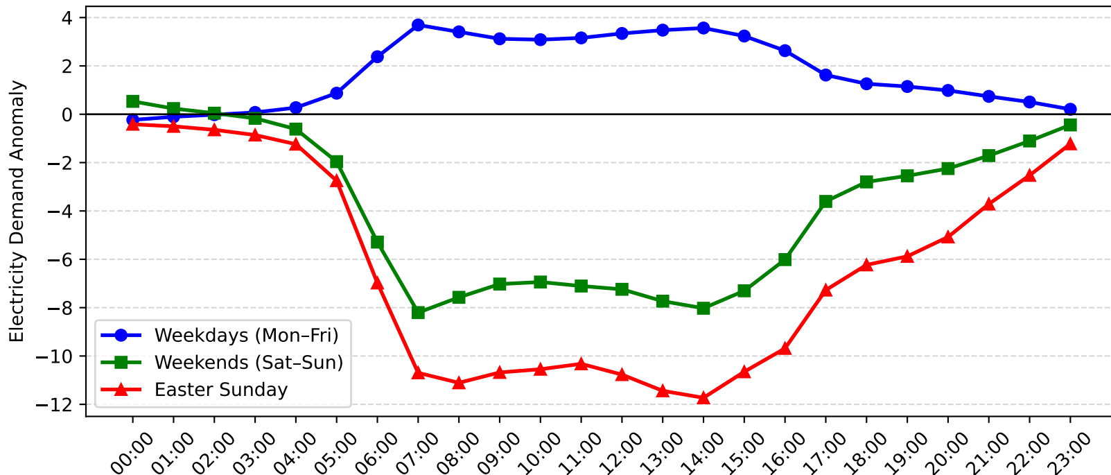
Marrickville Demand Anomaly: Easter Sunday vs Weekday/Weekend (2008-2009)
