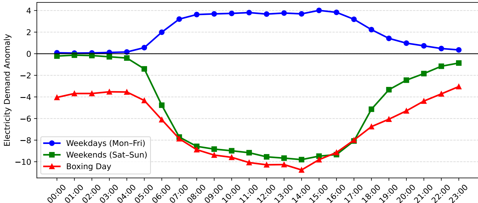
Macquarie Park Demand Anomaly: Boxing Day vs Weekday/Weekend (2005-2006)
