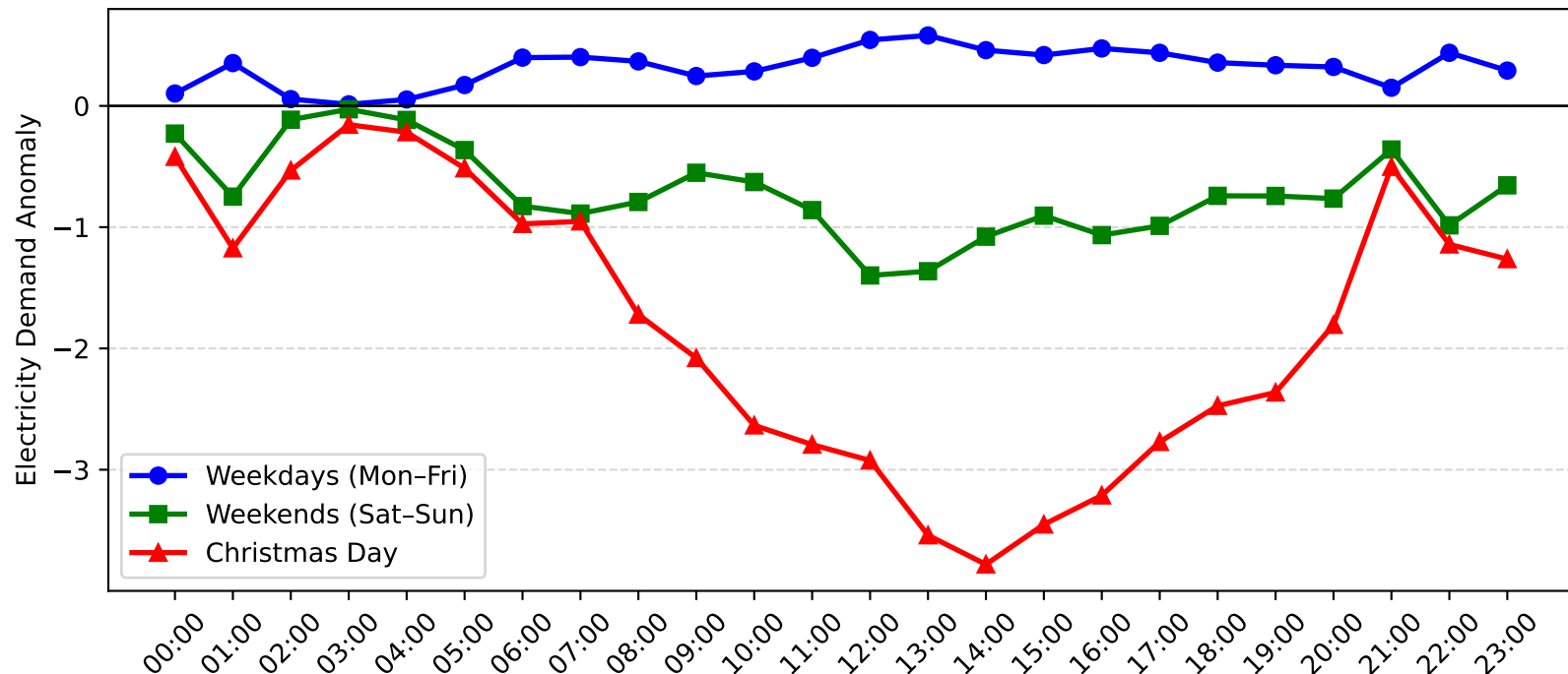
Gateshead Demand Anomaly: Christmas Day vs Weekday/Weekend (2004-2005)
