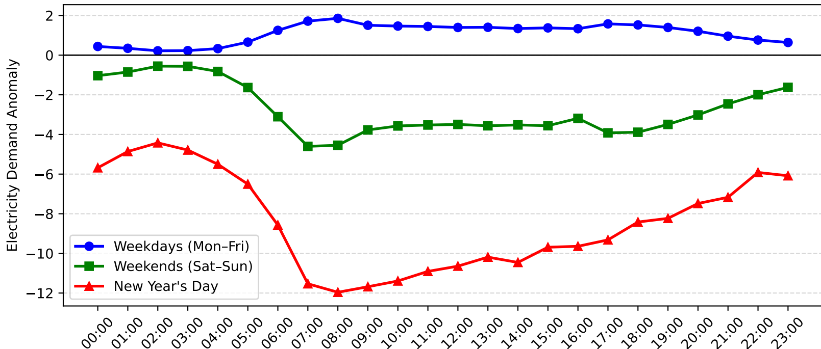
Maroubra Demand Anomaly: New Year's Day vs Weekday/Weekend (2010-2011)
