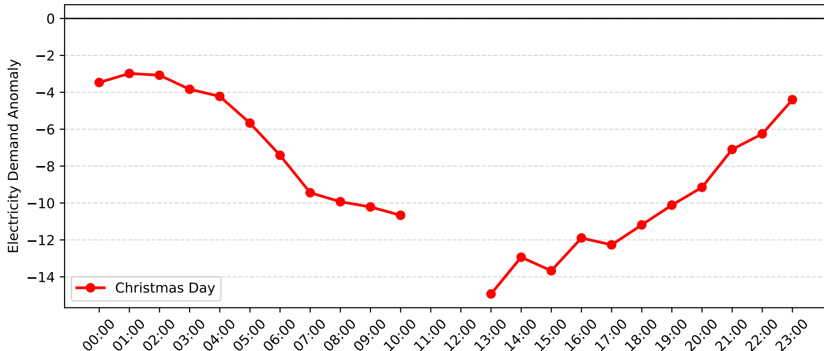
Sefton Demand Anomaly: Christmas Day (2008-2009)
