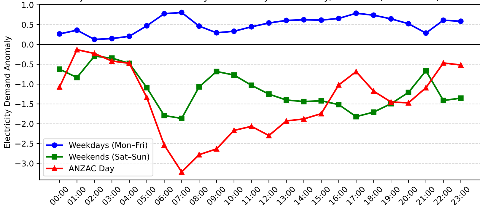
Jesmond Demand Anomaly: ANZAC Day vs Weekday/Weekend (2016-2017)
