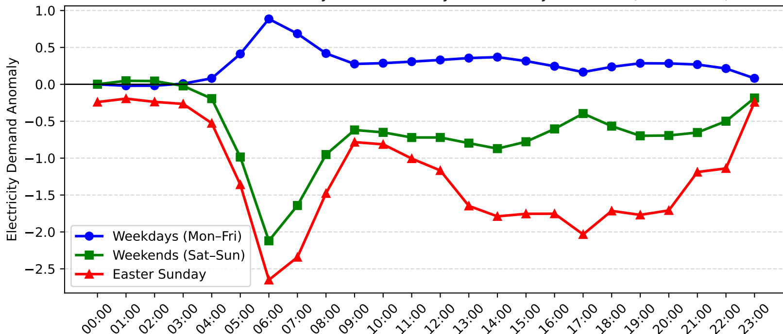
Berowra Demand Anomaly: Easter Sunday vs Weekday/Weekend (2007-2008)
