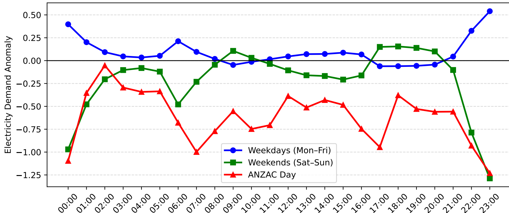
Muswellbrook Demand Anomaly: ANZAC Day vs Weekday/Weekend (2004-2005)
