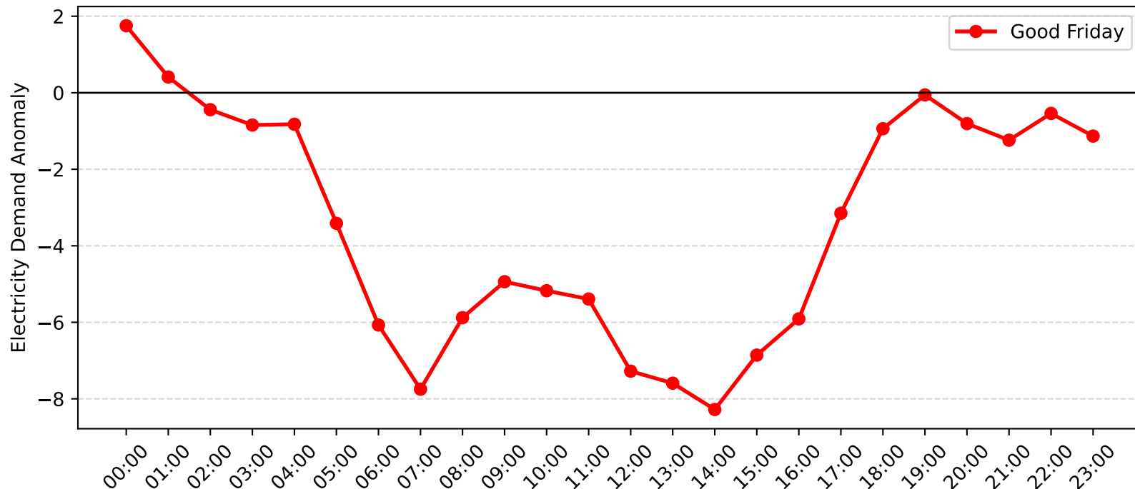
Meadowbank Demand Anomaly: Good Friday (2004-2005)
