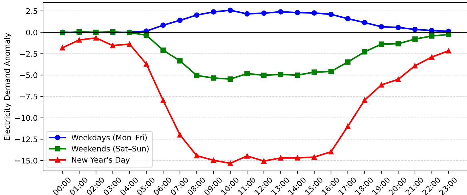
Zetland Demand Anomaly: New Year's Day vs Weekday/Weekend (2004-2005)
