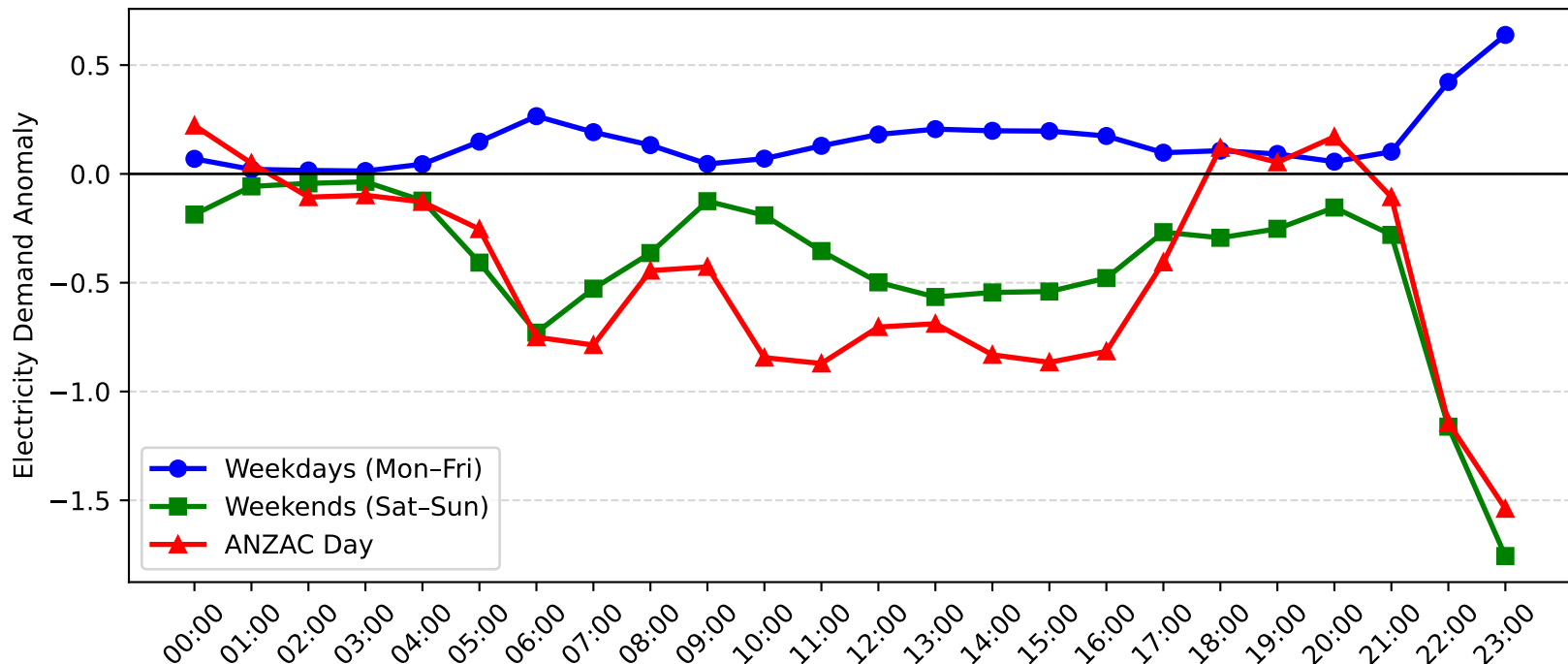
Muswellbrook Demand Anomaly: ANZAC Day vs Weekday/Weekend (2012-2013)
