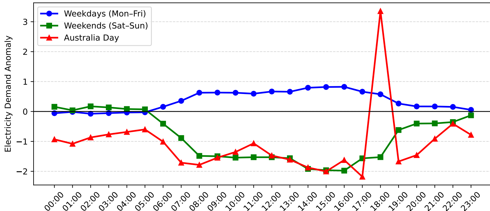
Pymble Demand Anomaly: Australia Day vs Weekday/Weekend (2004-2005)
