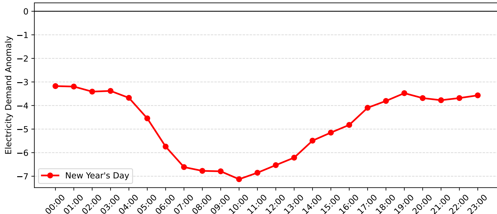
Leightonfield Demand Anomaly: New Year's Day (2008-2009)
