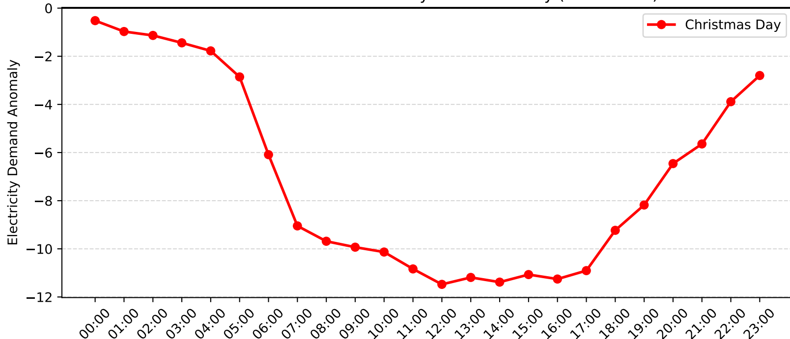
Chatswood Demand Anomaly: Christmas Day (2004-2005)
