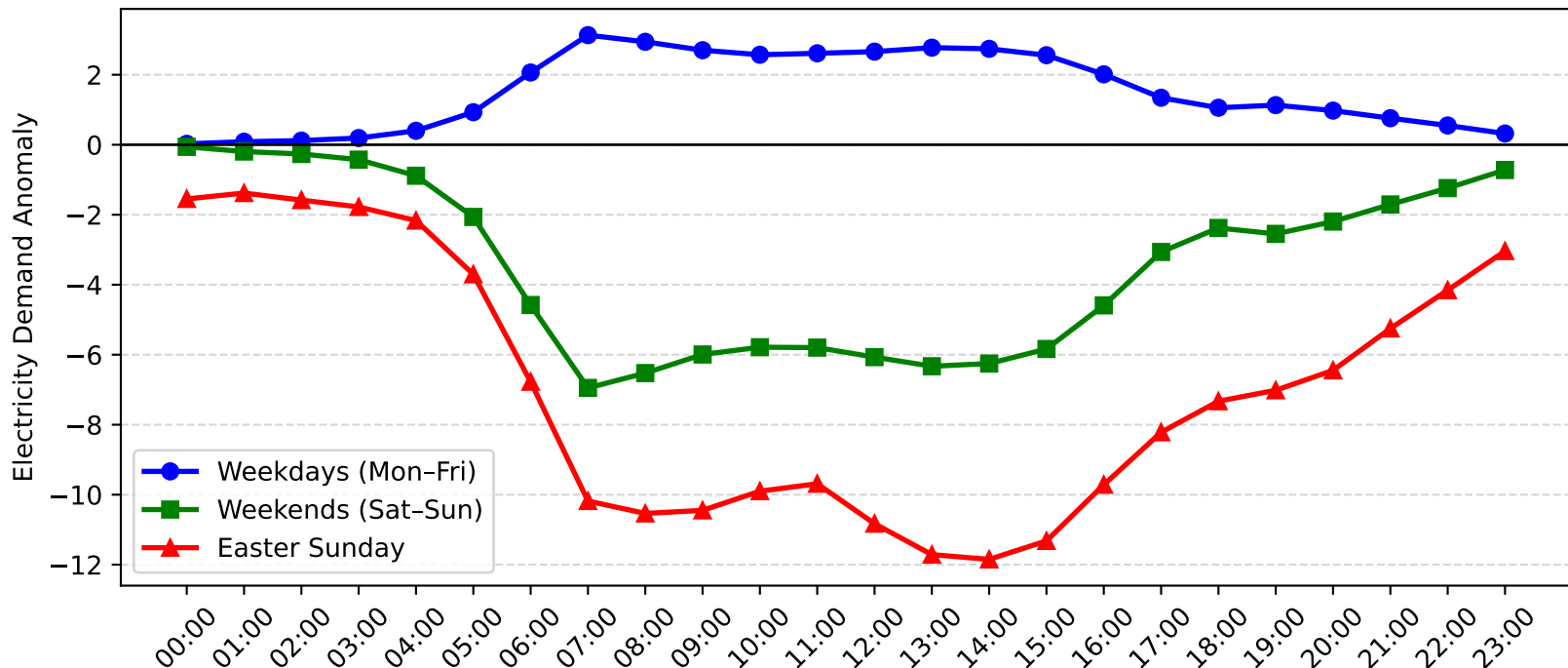
Marrickville Demand Anomaly: Easter Sunday vs Weekday/Weekend (2016-2017)
