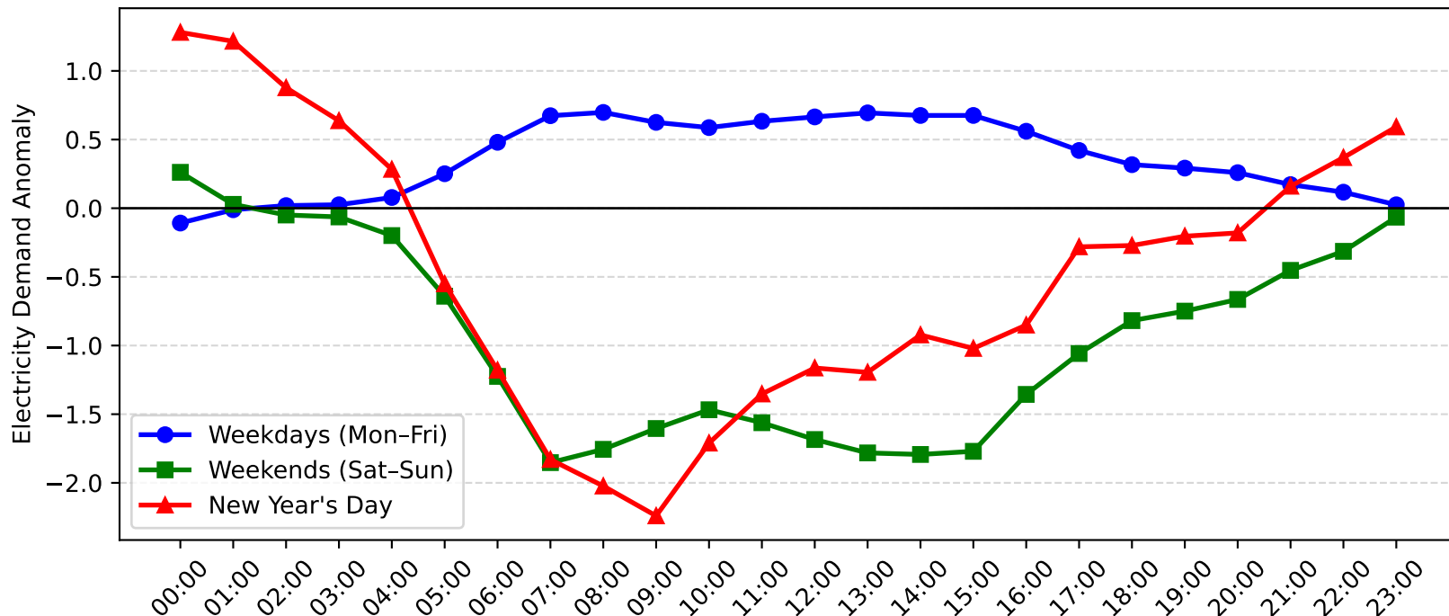
Rockdale Demand Anomaly: New Year's Day vs Weekday/Weekend (2010-2011)
