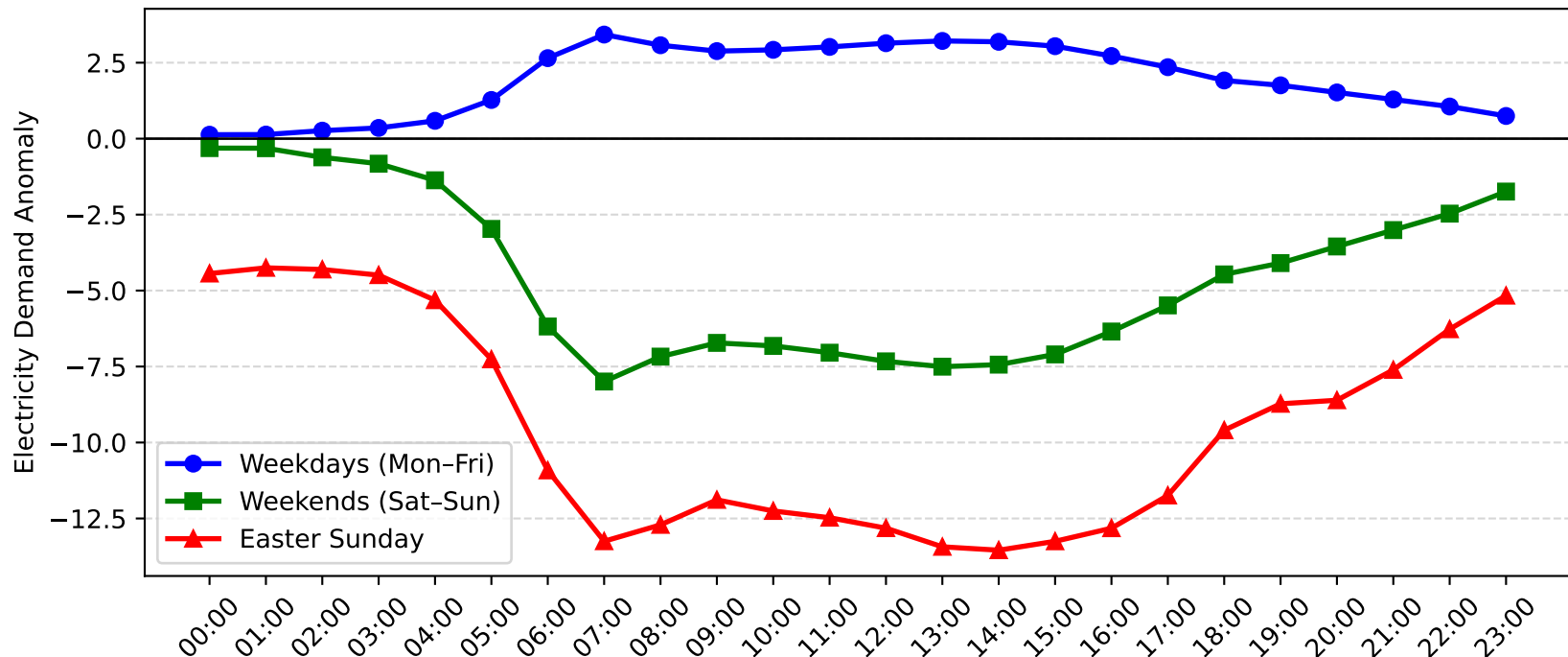
Sefton Demand Anomaly: Easter Sunday vs Weekday/Weekend (2012-2013)
