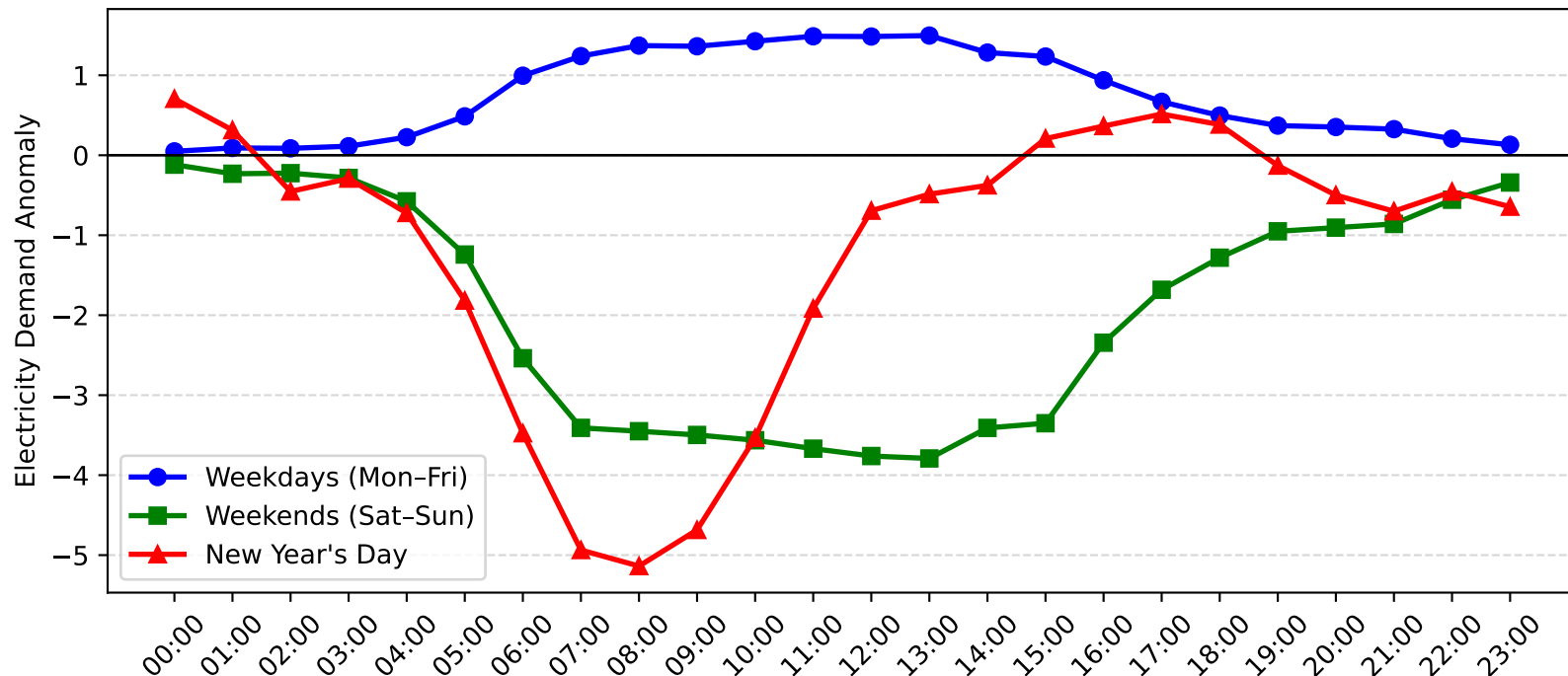
Wyong Demand Anomaly: New Year's Day vs Weekday/Weekend (2010-2011)
