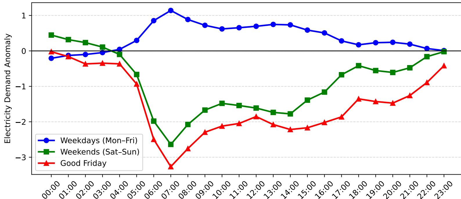
Arncliffe Demand Anomaly: Good Friday vs Weekday/Weekend (2009-2010)
