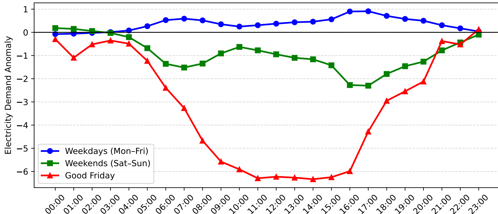
Erina Demand Anomaly: Good Friday vs Weekday/Weekend (2011-2012)
