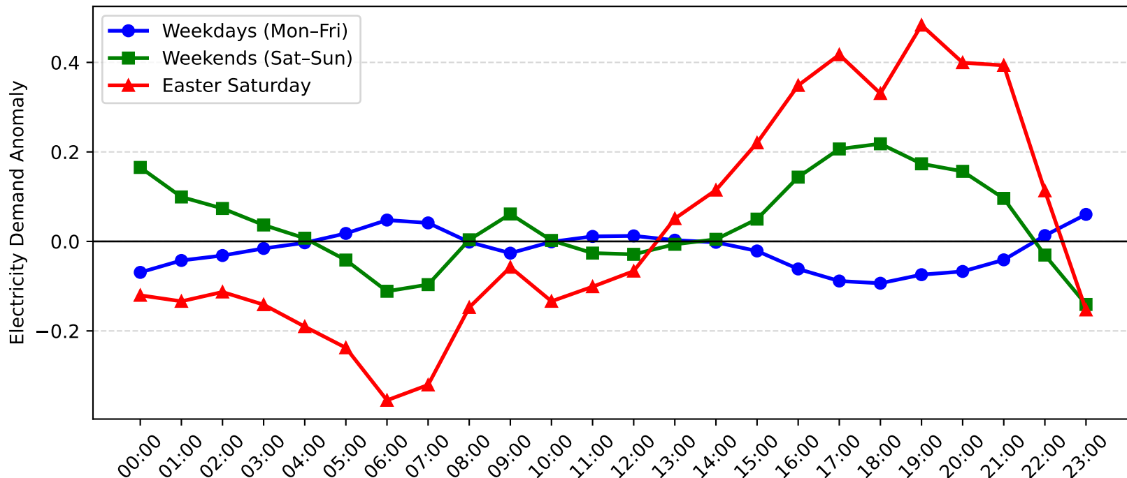
Rothbury Demand Anomaly: Easter Saturday vs Weekday/Weekend (2013-2014)
