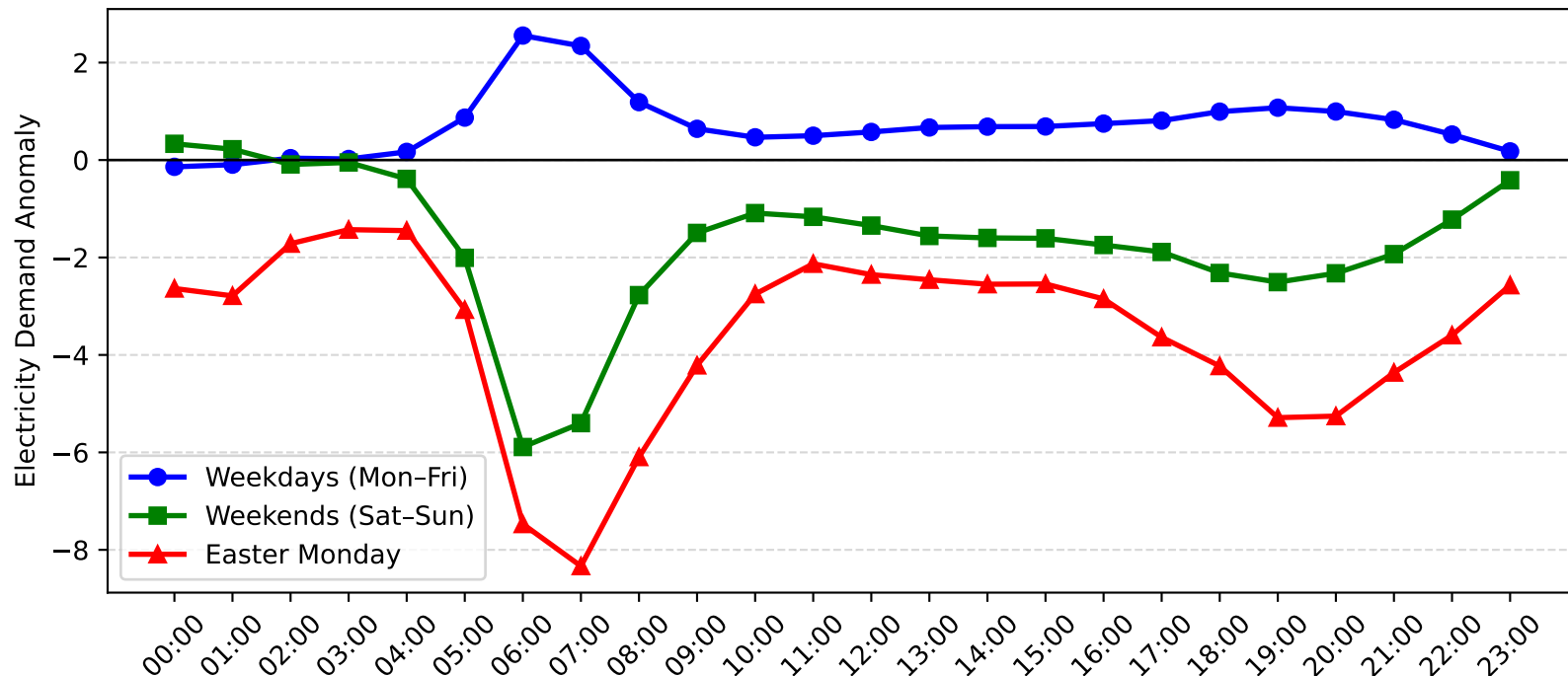
Pennant Hills Demand Anomaly: Easter Monday vs Weekday/Weekend (2011-2012)
