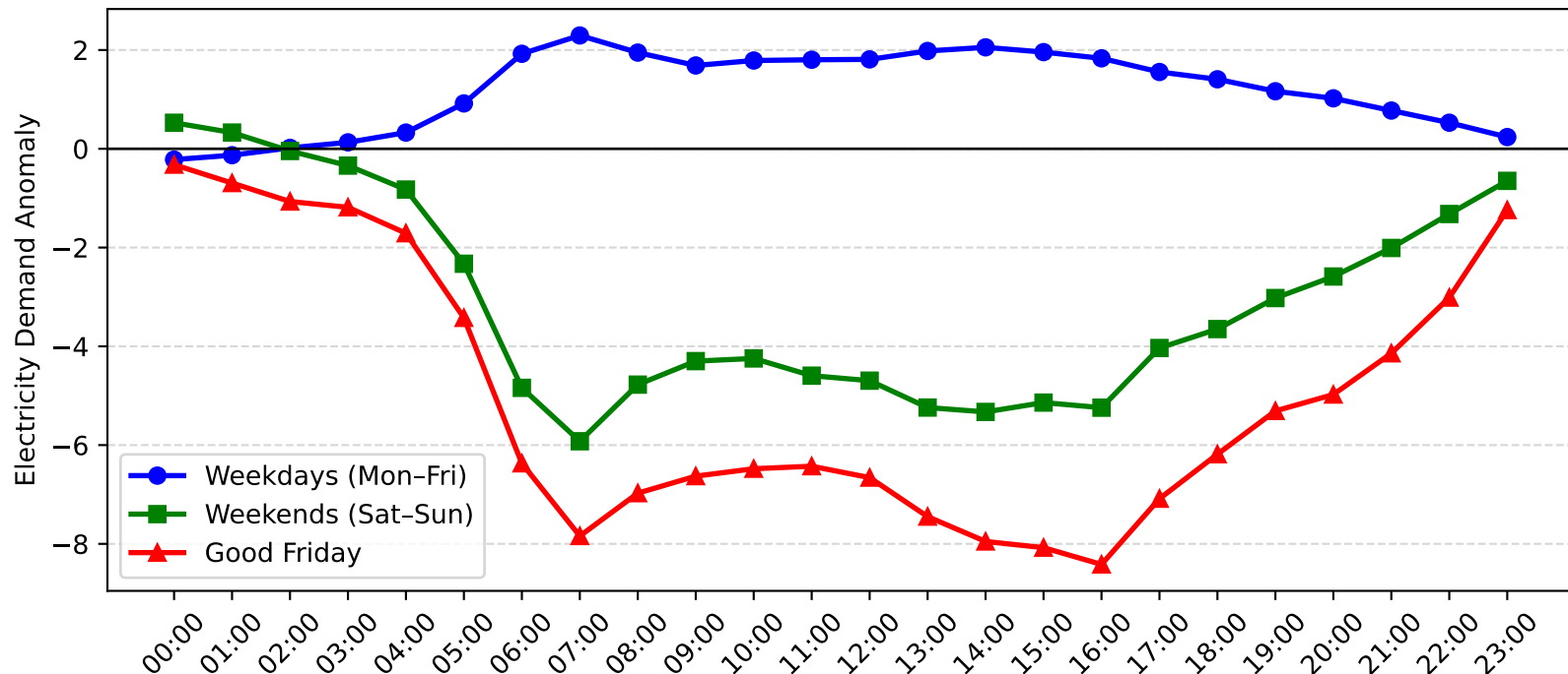
Campsie Demand Anomaly: Good Friday vs Weekday/Weekend (2005-2006)
