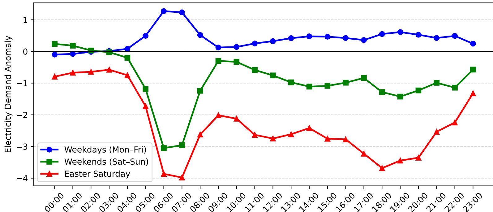
Dee Why West Demand Anomaly: Easter Saturday vs Weekday/Weekend (2012-2013)
