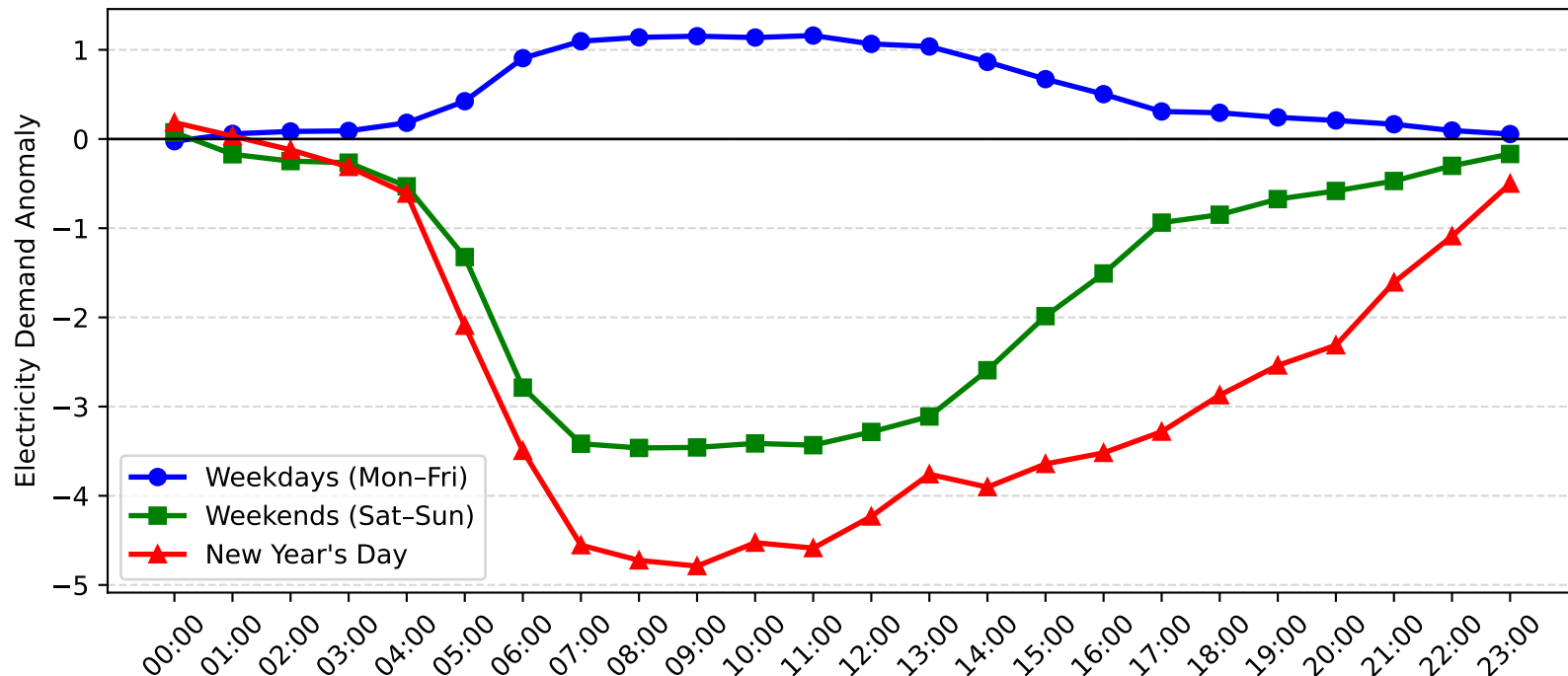
Wyong Demand Anomaly: New Year's Day vs Weekday/Weekend (2014-2015)
