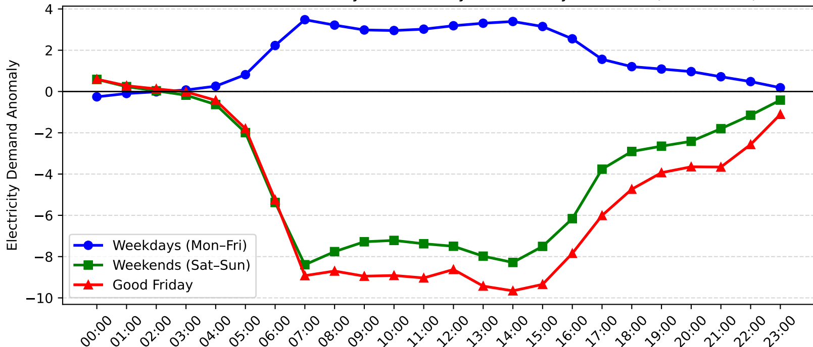
Marrickville Demand Anomaly: Good Friday vs Weekday/Weekend (2008-2009)
