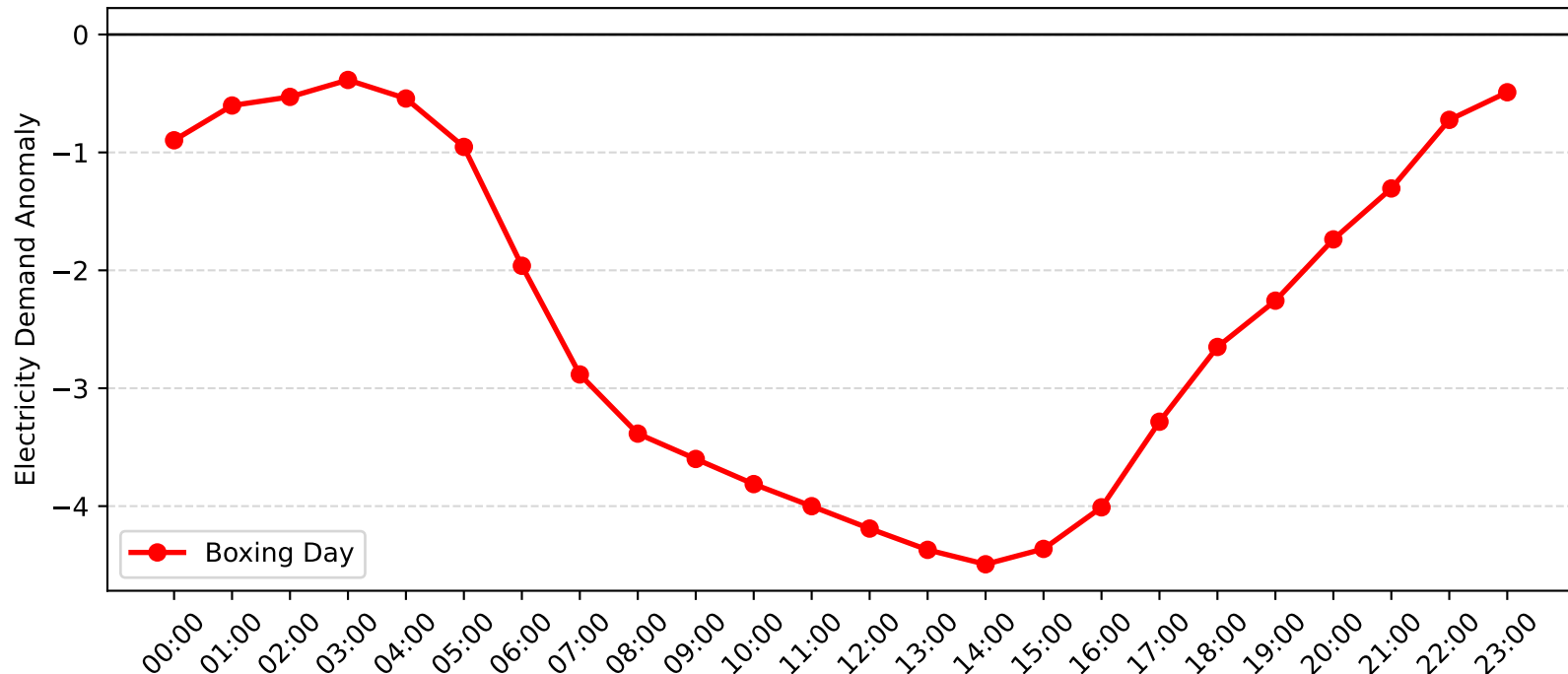
Gateshead Demand Anomaly: Boxing Day (2006-2007)
