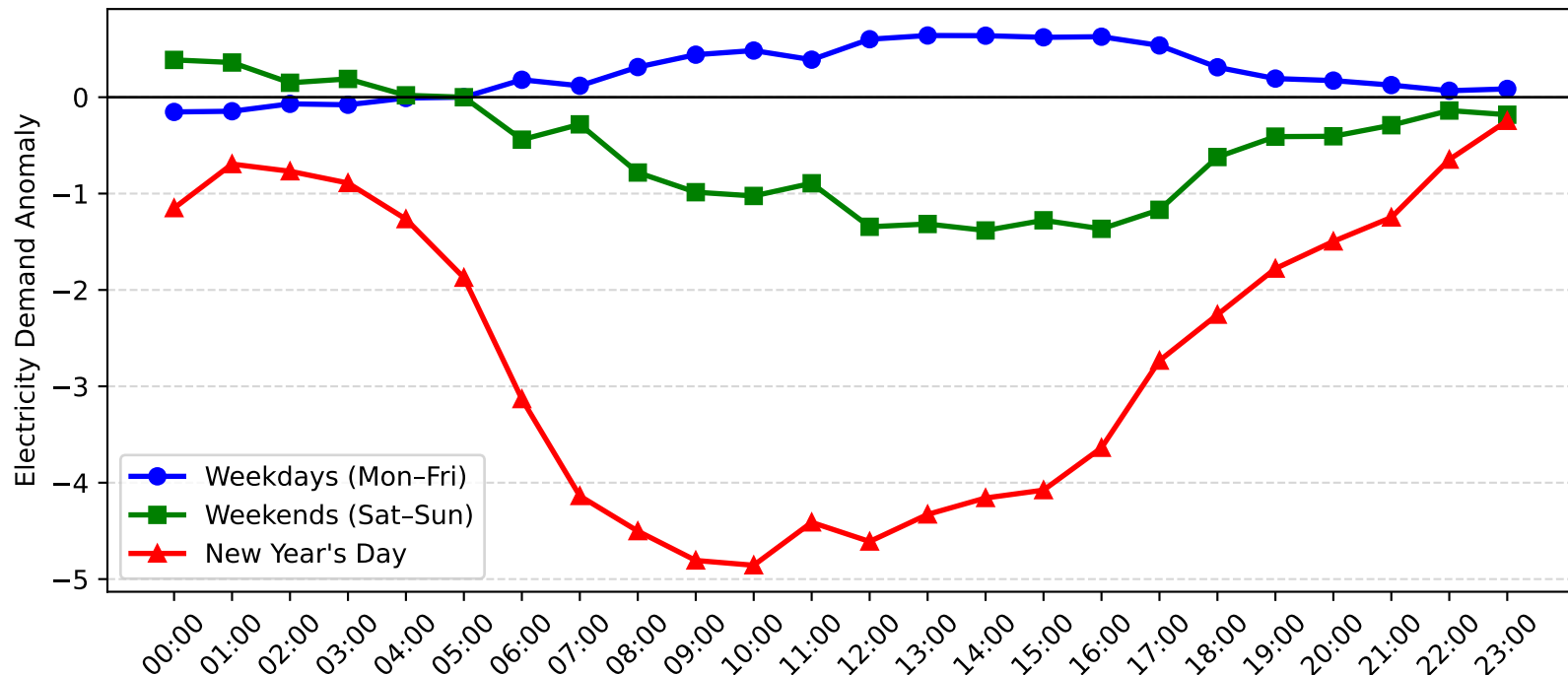
Lidcombe Demand Anomaly: New Year's Day vs Weekday/Weekend (2004-2005)
