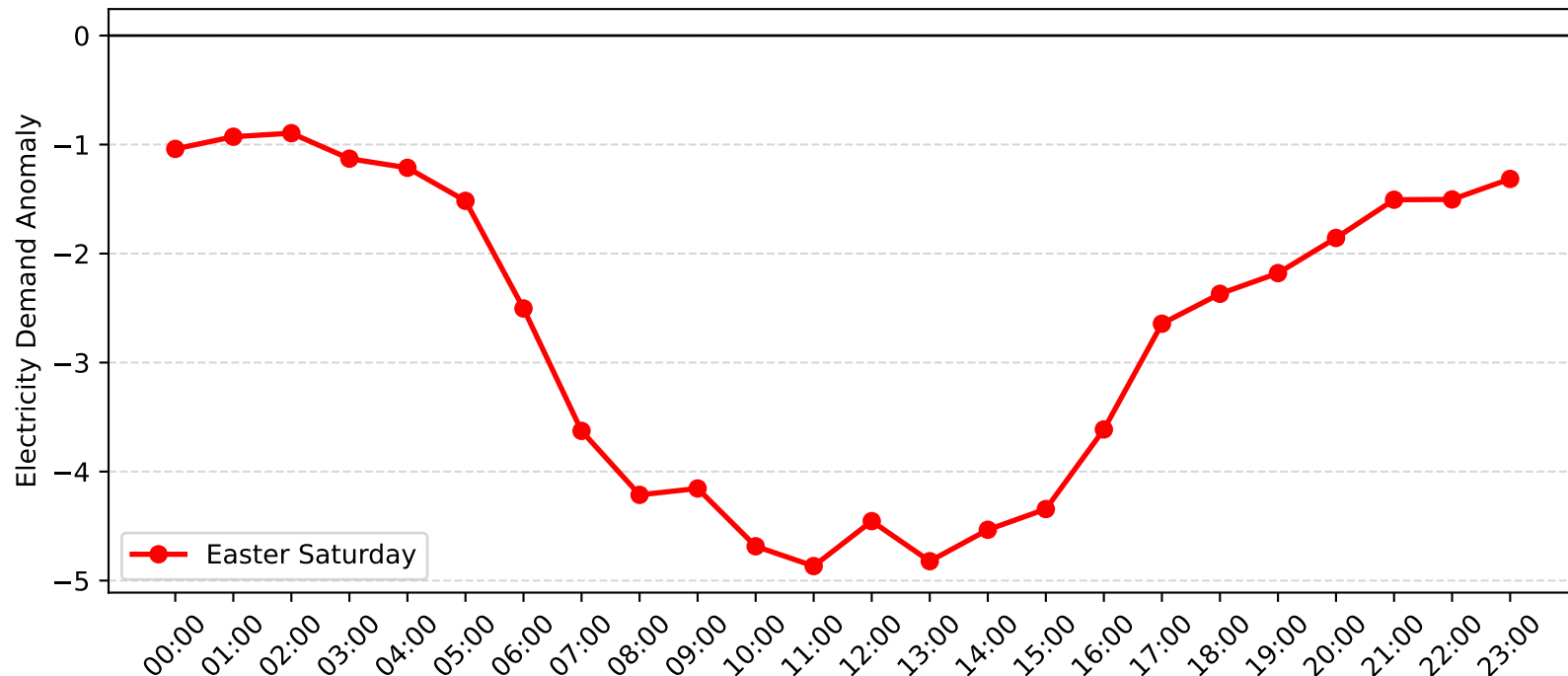
Mayfield West Demand Anomaly: Easter Saturday (2016-2017)
