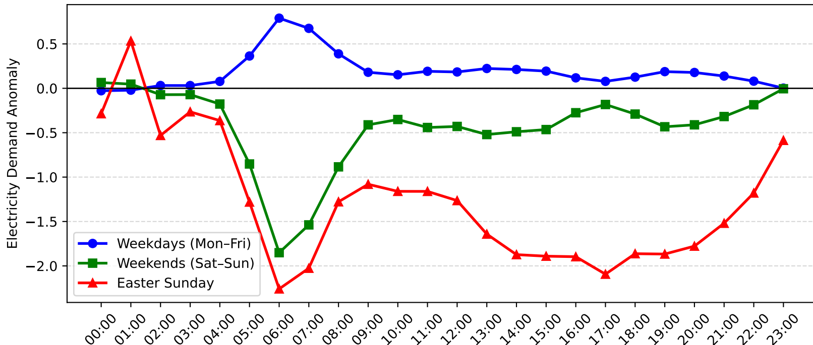
Berowra Demand Anomaly: Easter Sunday vs Weekday/Weekend (2015-2016)
