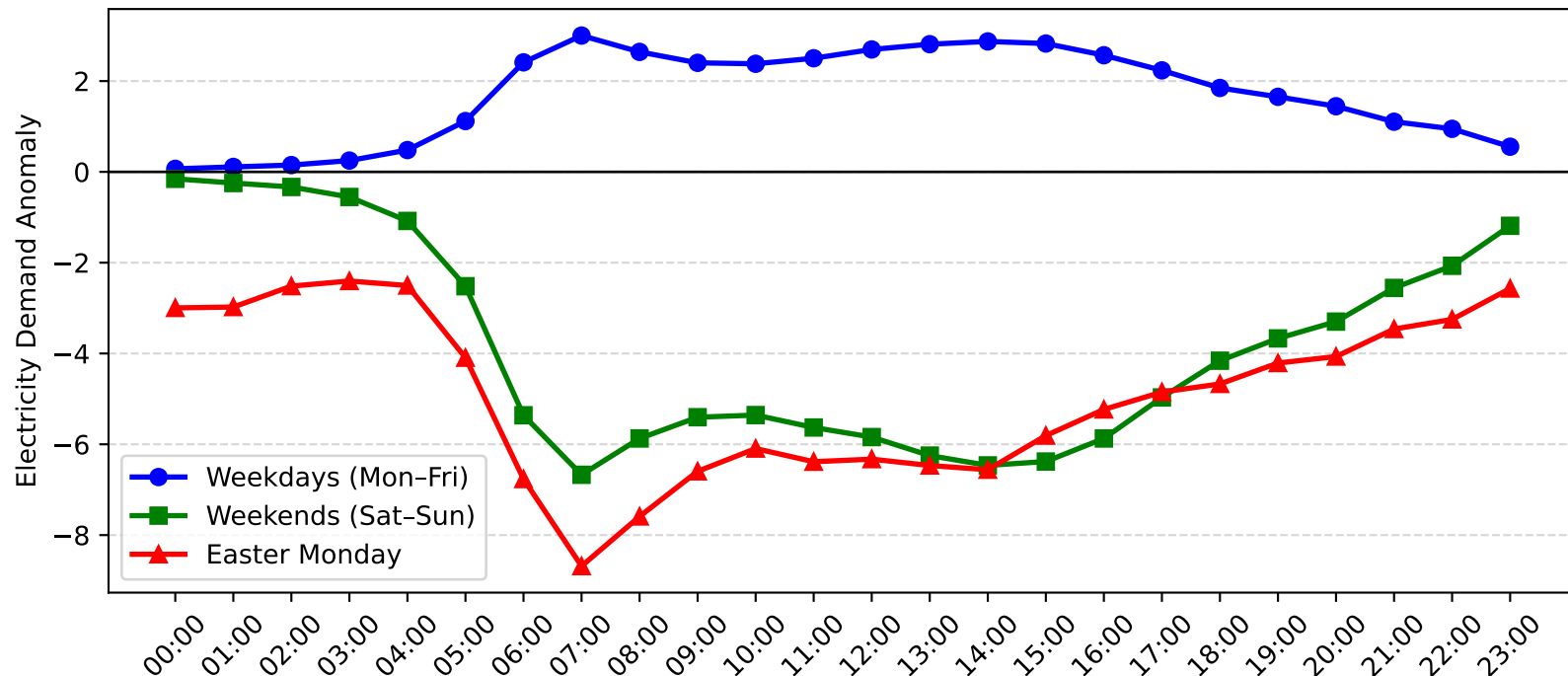
Sefton Demand Anomaly: Easter Monday vs Weekday/Weekend (2008-2009)
