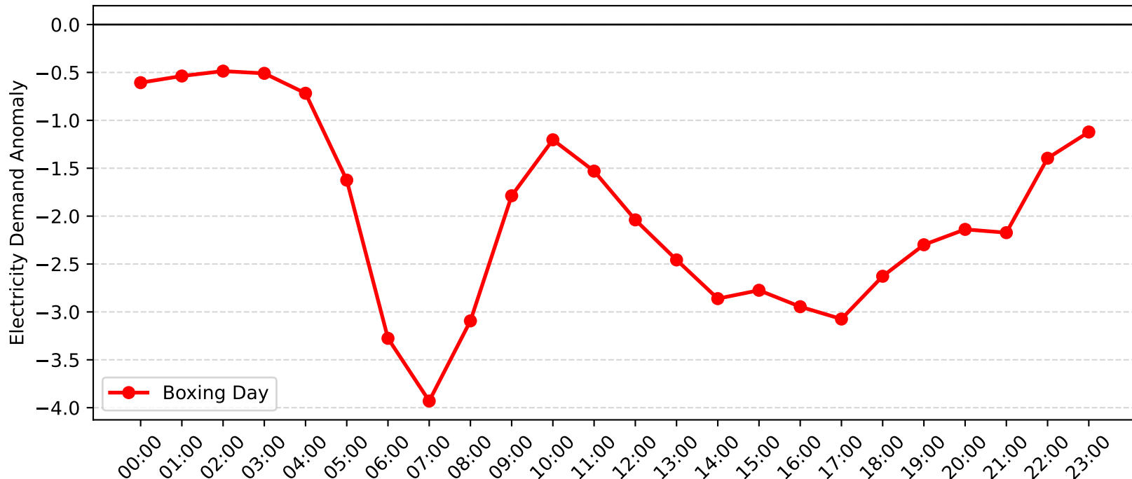
Dee Why West Demand Anomaly: Boxing Day (2011-2012)
