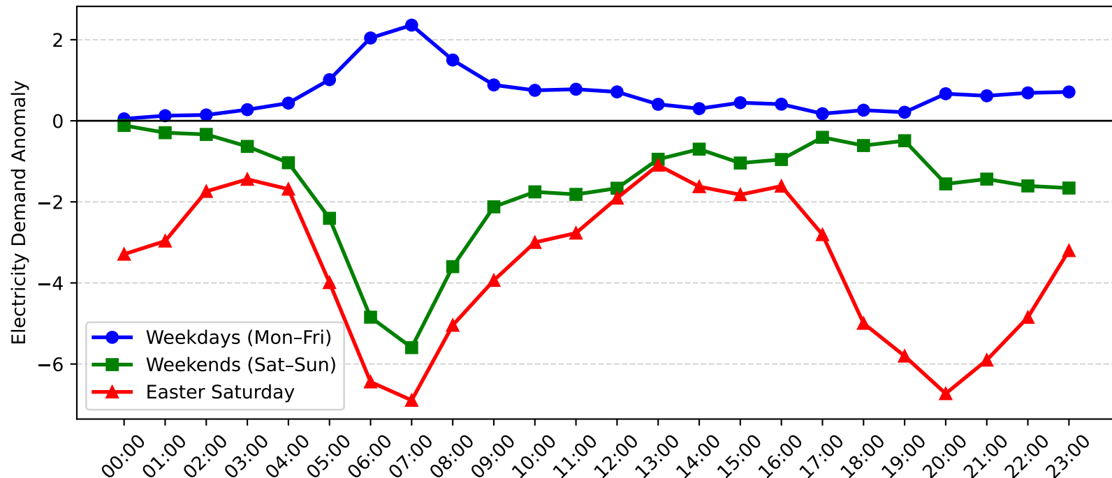
Meadowbank Demand Anomaly: Easter Saturday vs Weekday/Weekend (2011-2012)
