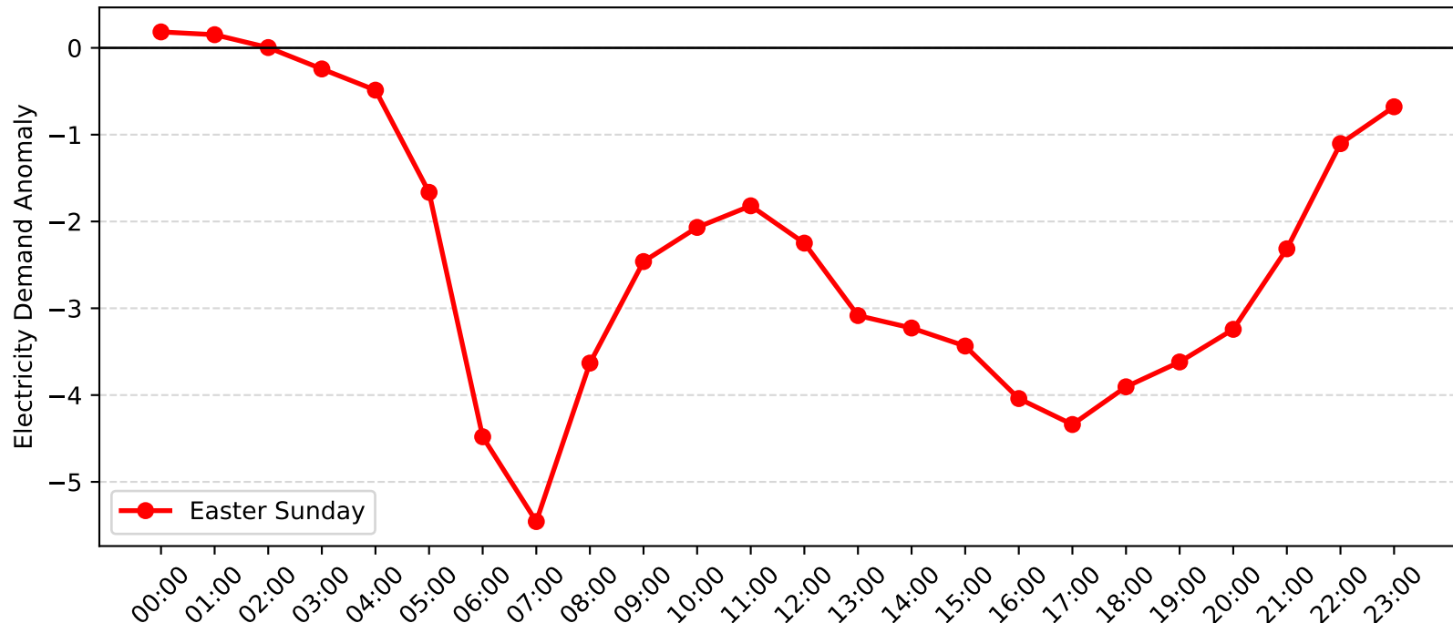
Mortdale Demand Anomaly: Easter Sunday (2008-2009)
