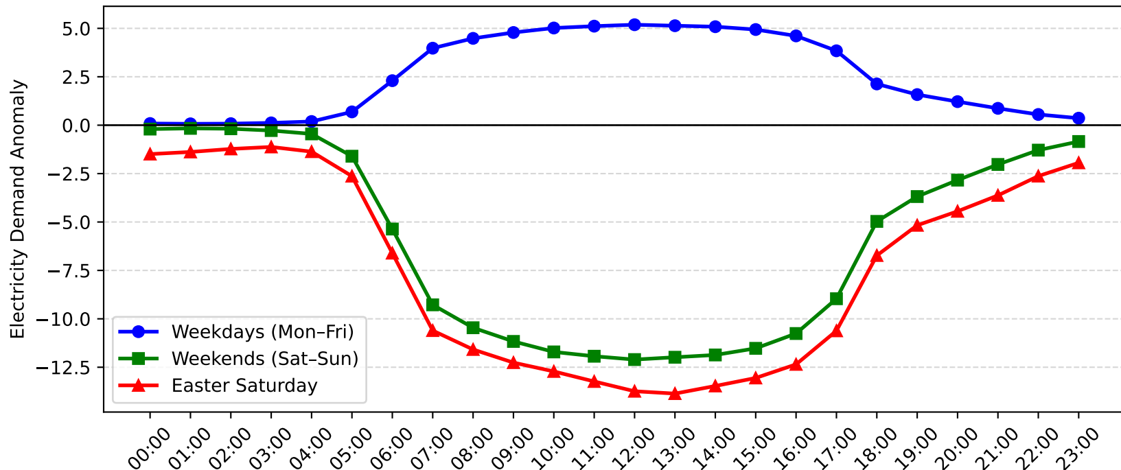
Macquarie Park Demand Anomaly: Easter Saturday vs Weekday/Weekend (2013-2014)
