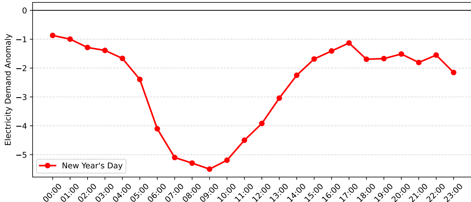
Rutherford Demand Anomaly: New Year's Day (2014-2015)
