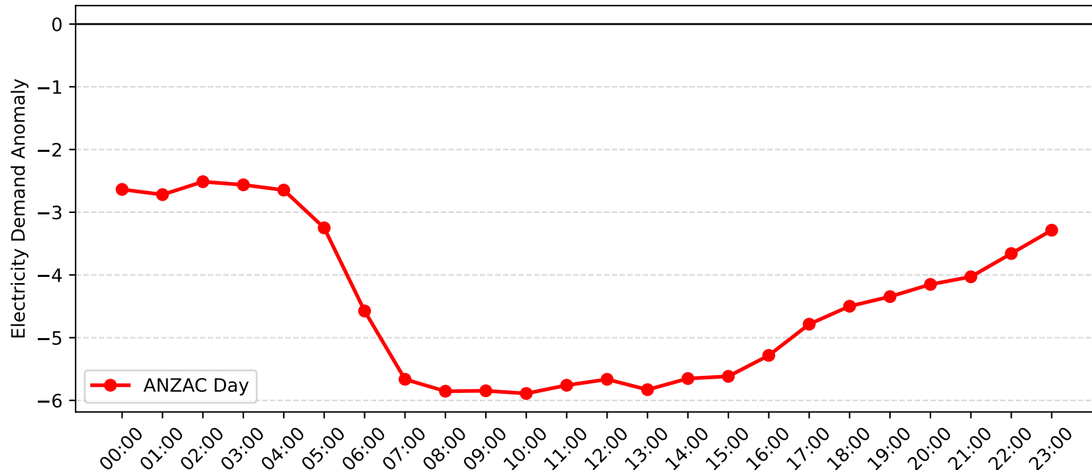
Leightonfield Demand Anomaly: ANZAC Day (2016-2017)
