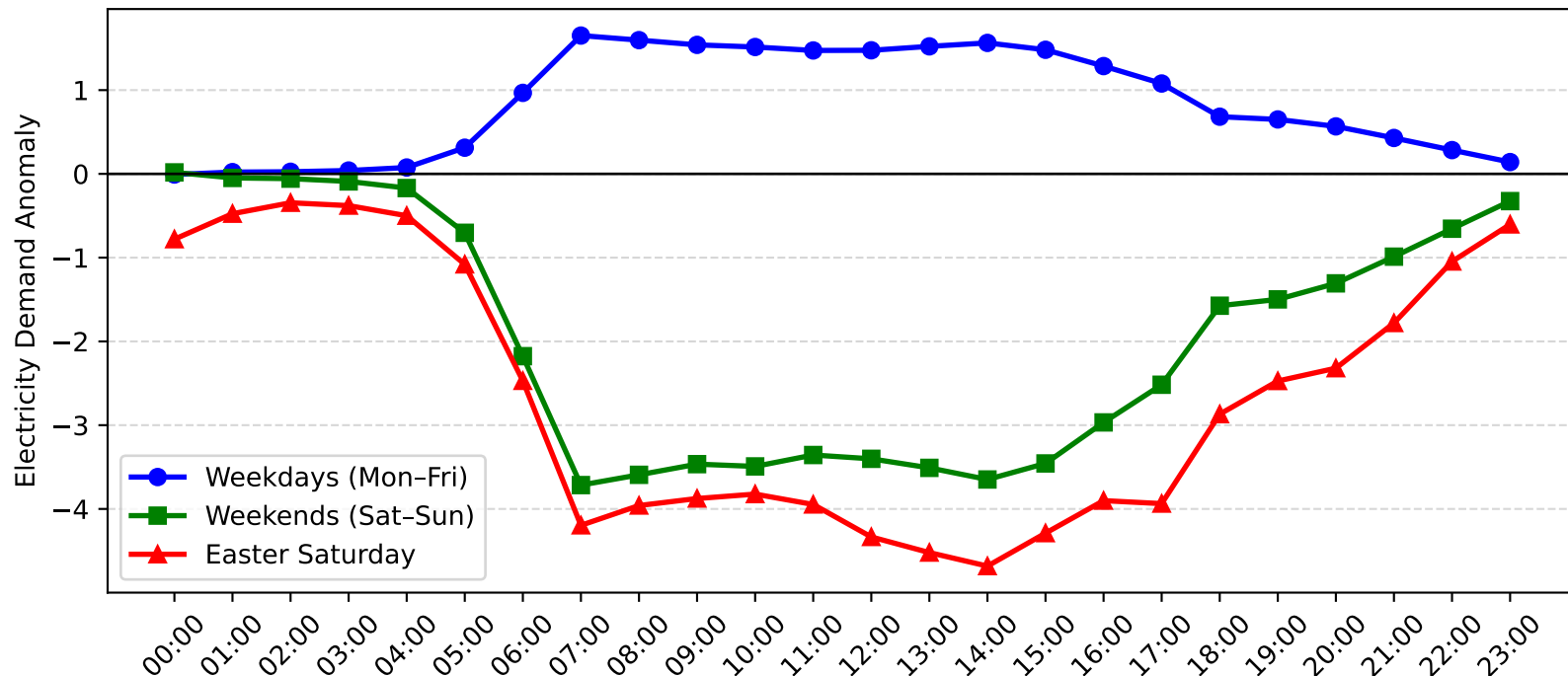
Concord Demand Anomaly: Easter Saturday vs Weekday/Weekend (2015-2016)
