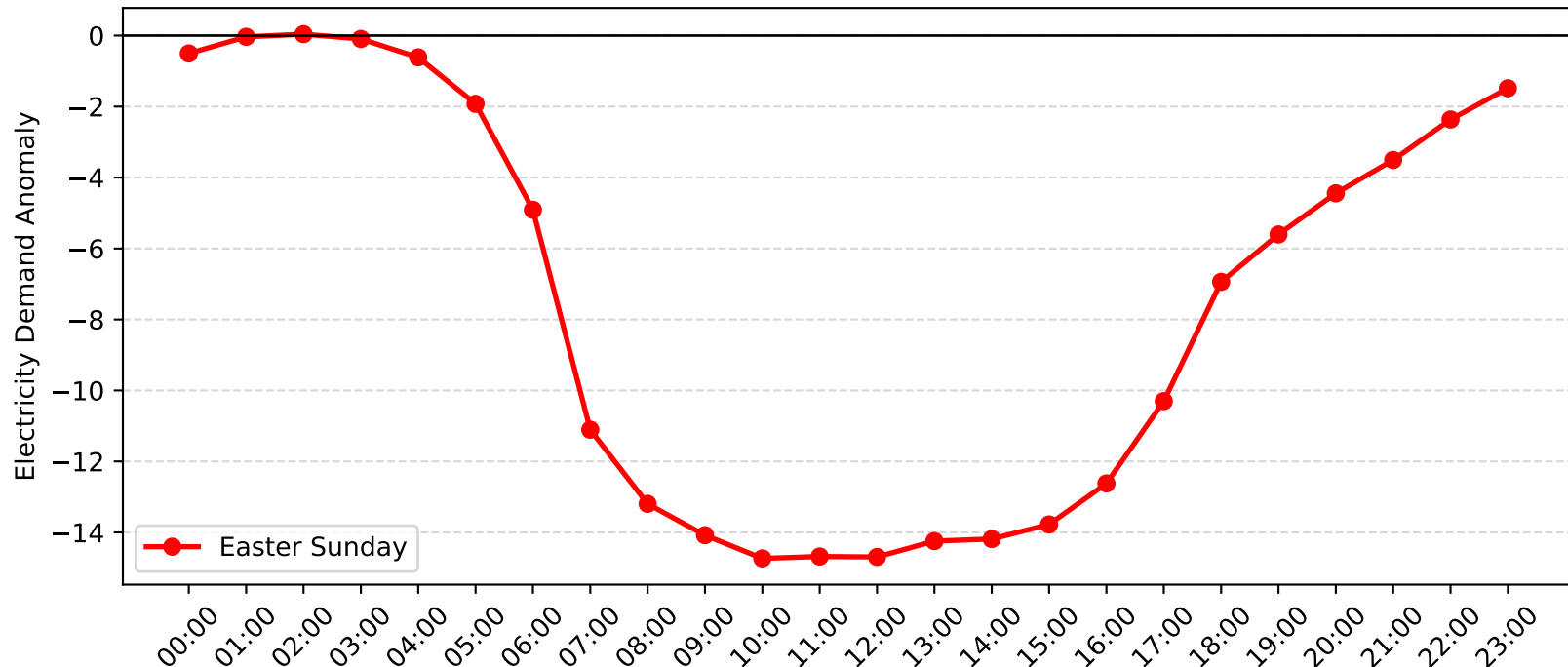
Gore Hill Demand Anomaly: Easter Sunday (2013-2014)
