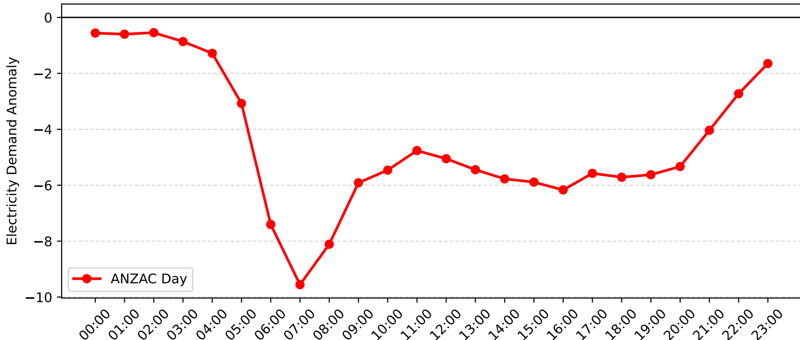
Sefton Demand Anomaly: ANZAC Day (2008-2009)
