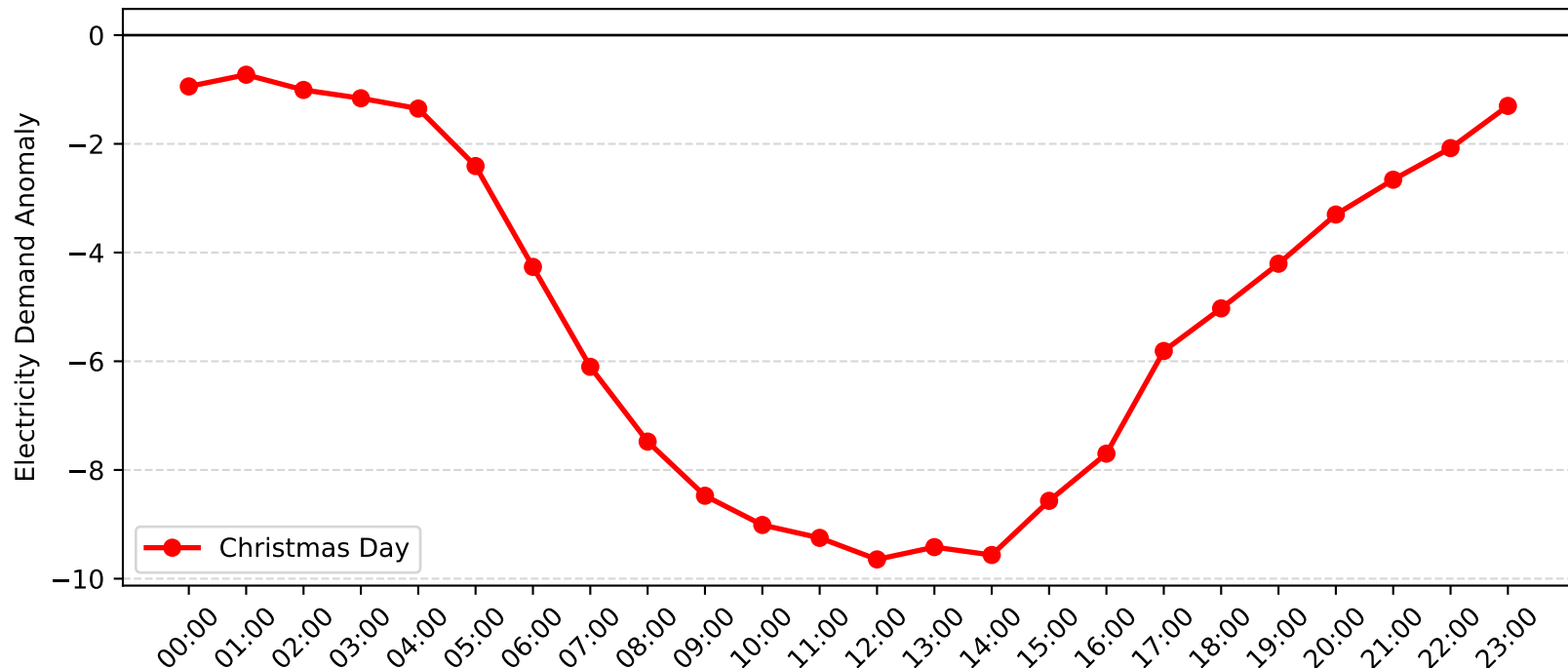
Mascot Demand Anomaly: Christmas Day (2014-2015)
