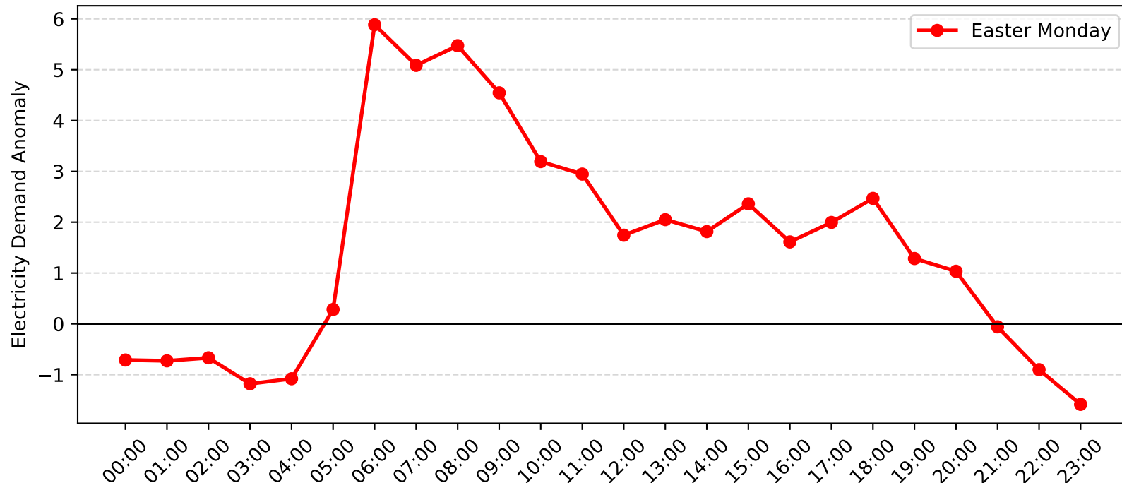
Gore Hill Demand Anomaly: Easter Monday (2004-2005)
