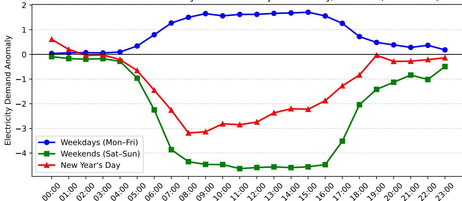
Beacon Hill Demand Anomaly: New Year's Day vs Weekday/Weekend (2008-2009)
