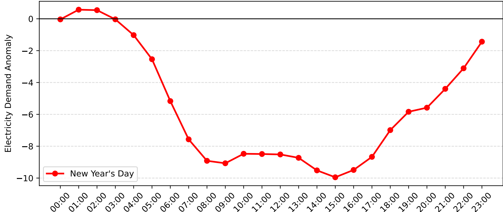
Kogarah Demand Anomaly: New Year's Day (2015-2016)
