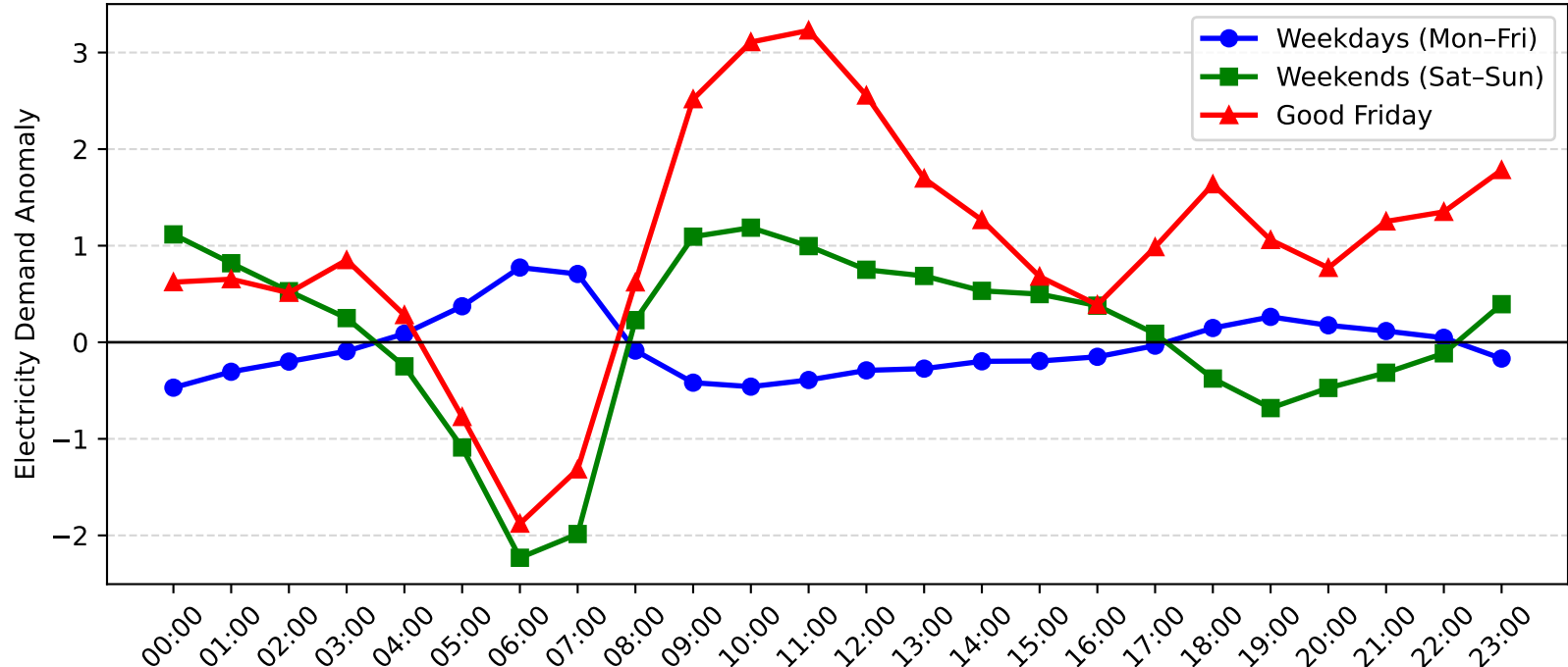
Avoca Demand Anomaly: Good Friday vs Weekday/Weekend (2007-2008)
