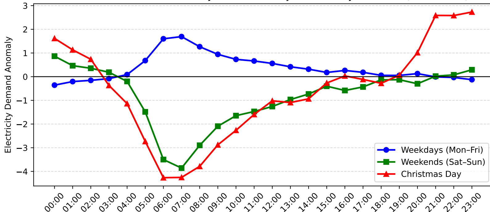
Pennant Hills Demand Anomaly: Christmas Day vs Weekday/Weekend (2010-2011)
