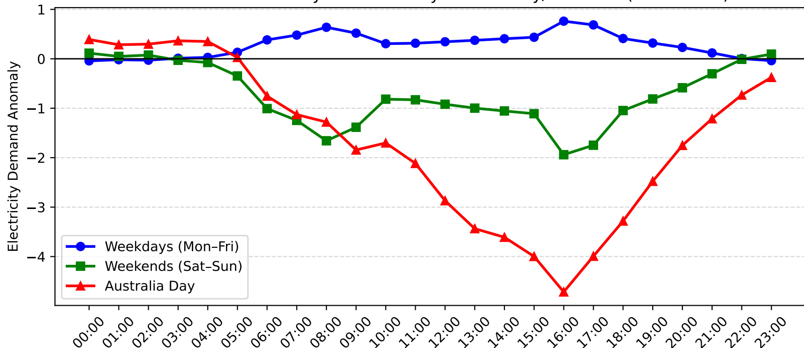
Erina Demand Anomaly: Australia Day vs Weekday/Weekend (2015-2016)
