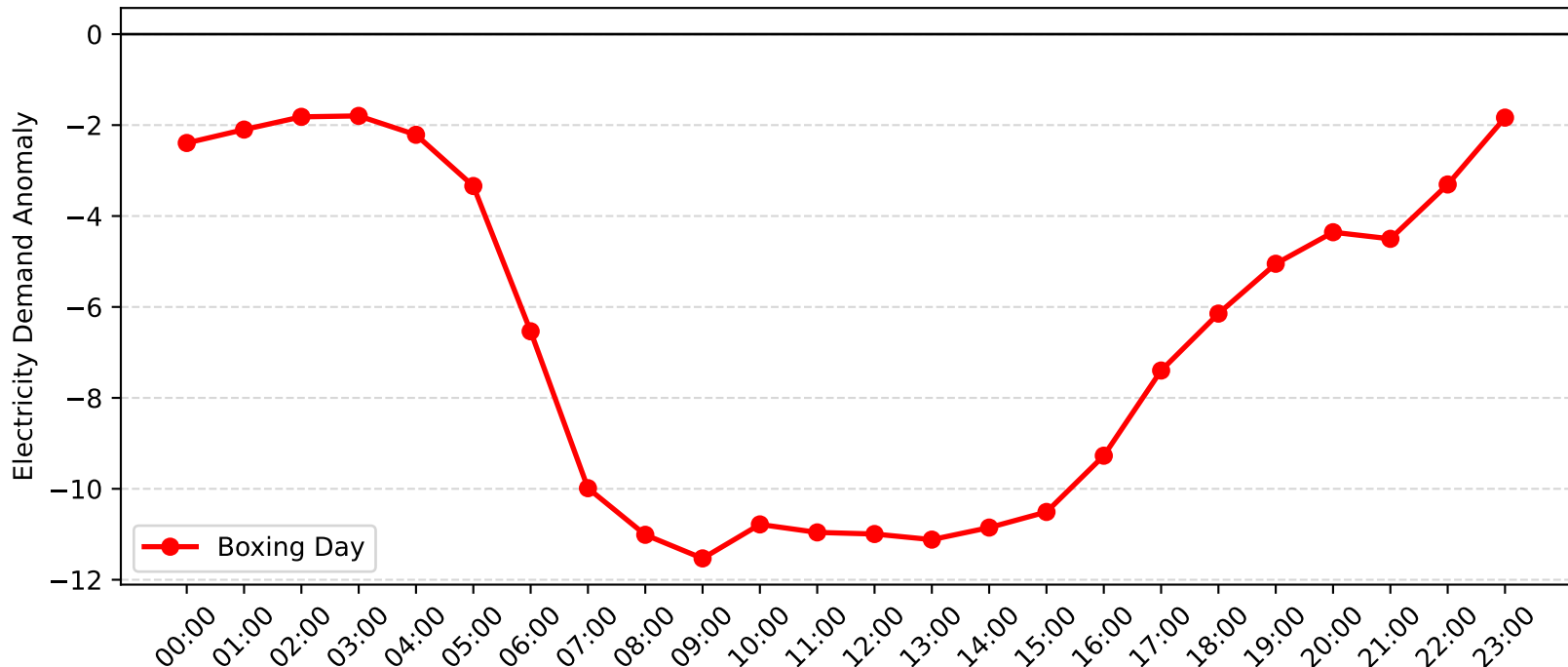
Marrickville Demand Anomaly: Boxing Day (2007-2008)
