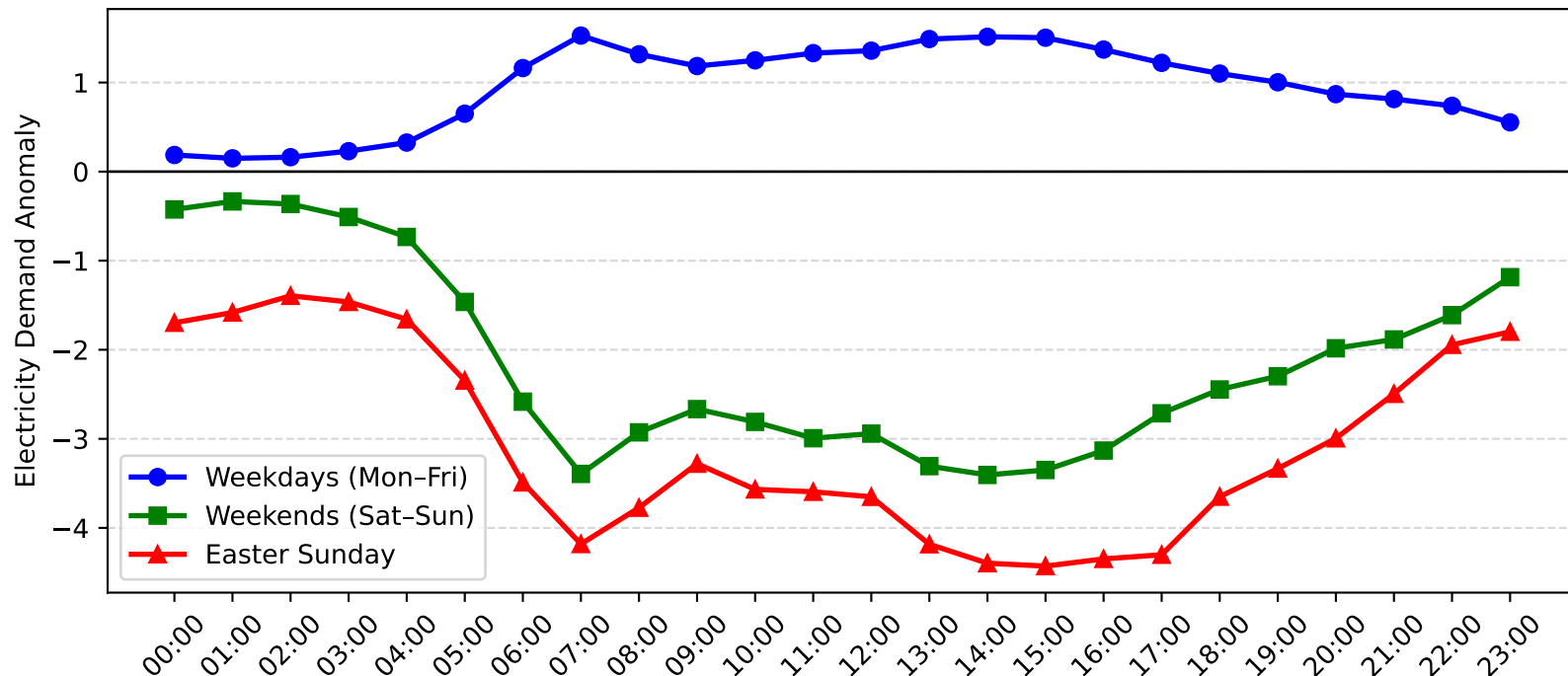
Bass Hill Demand Anomaly: Easter Sunday vs Weekday/Weekend (2008-2009)
