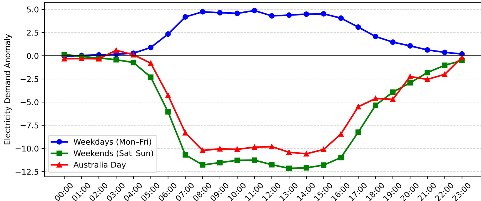
Zetland Demand Anomaly: Australia Day vs Weekday/Weekend (2006-2007)
