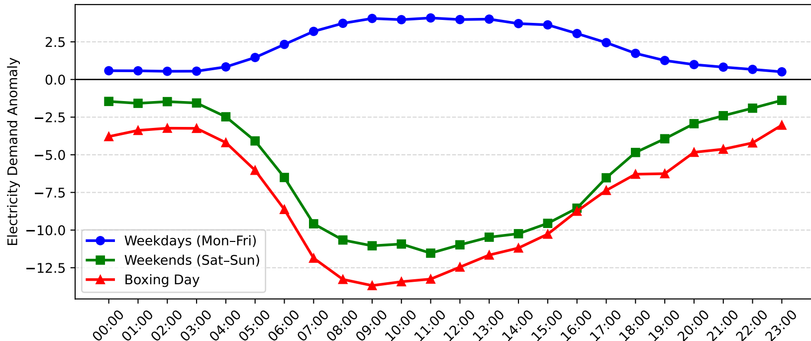
Homebush Bay Demand Anomaly: Boxing Day vs Weekday/Weekend (2007-2008)
