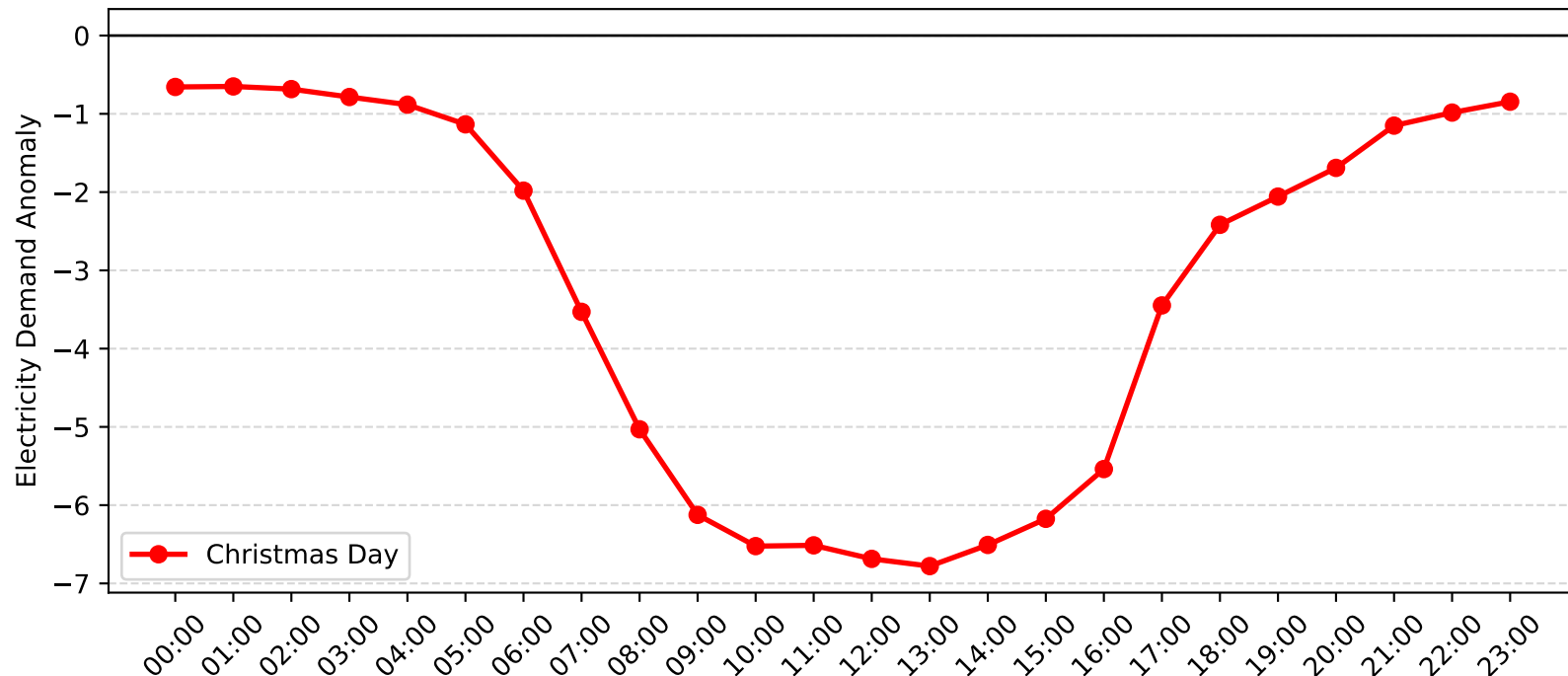
Auburn Demand Anomaly: Christmas Day (2006-2007)
