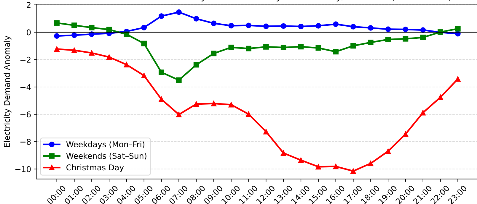
Dulwich Hill Demand Anomaly: Christmas Day vs Weekday/Weekend (2006-2007)
