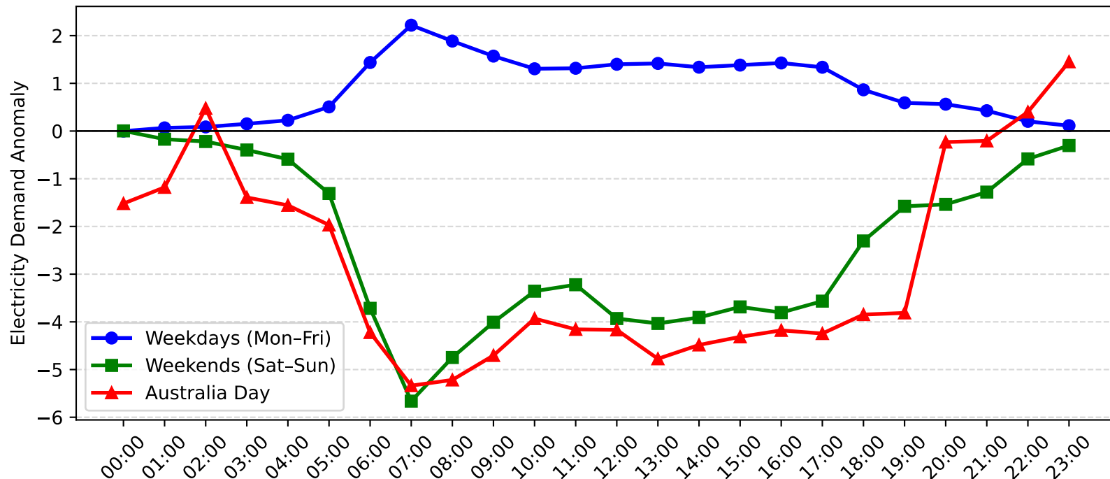
Chatswood Demand Anomaly: Australia Day vs Weekday/Weekend (2006-2007)
