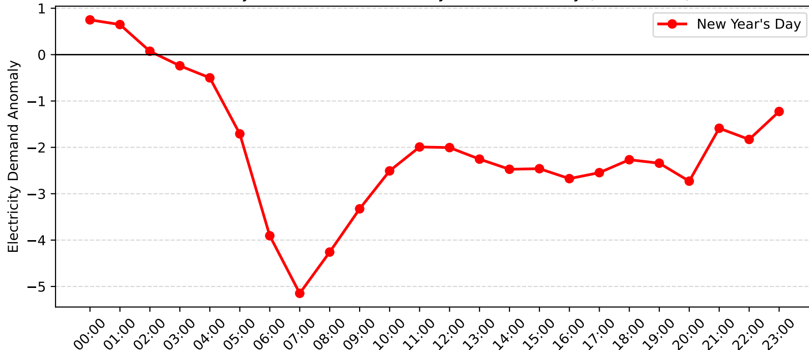
Dee Why West Demand Anomaly: New Year's Day (2011-2012)
