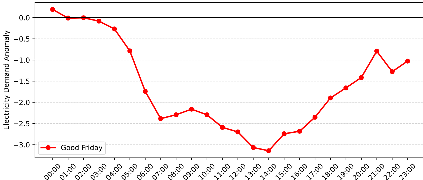
Gateshead Demand Anomaly: Good Friday (2005-2006)
