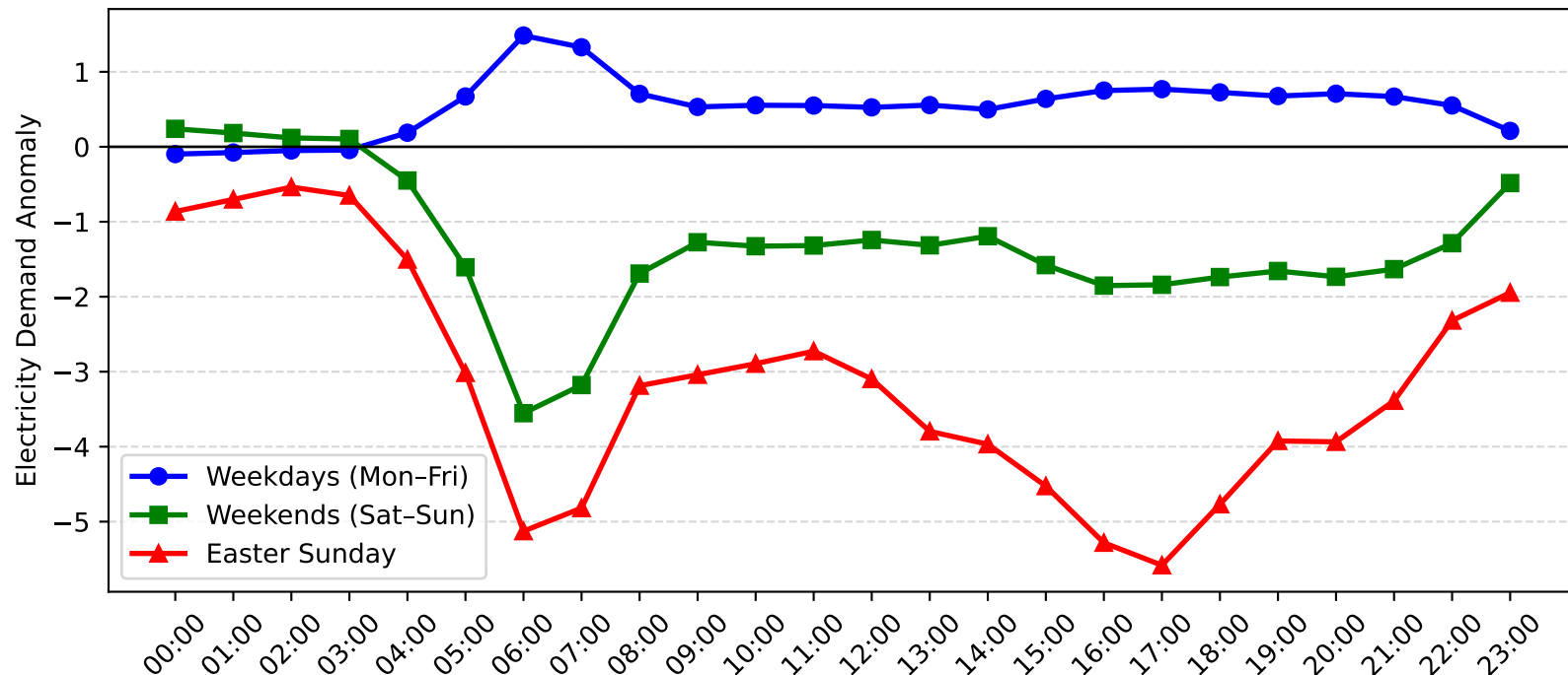
Revesby Demand Anomaly: Easter Sunday vs Weekday/Weekend (2007-2008)
