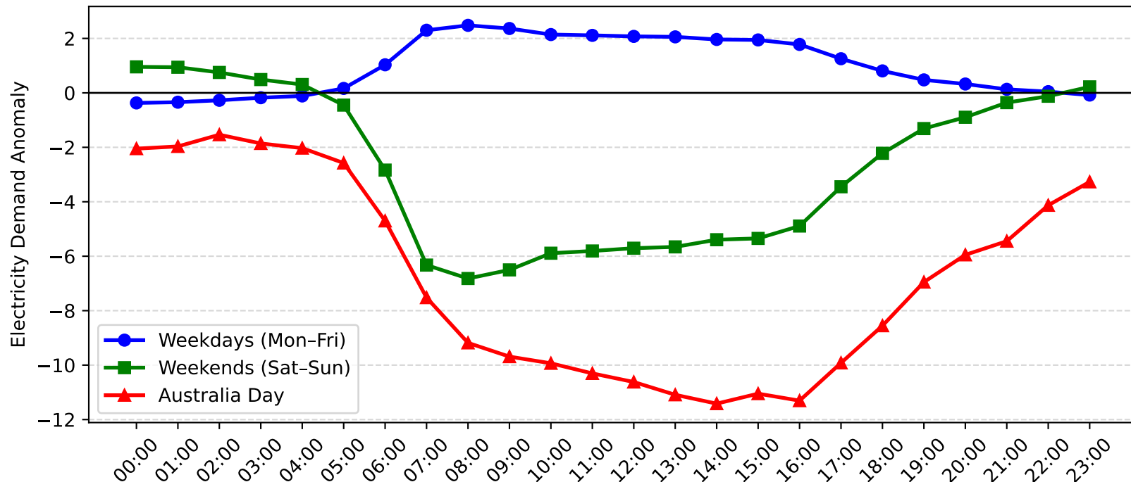
Zetland Demand Anomaly: Australia Day vs Weekday/Weekend (2017-2018)
