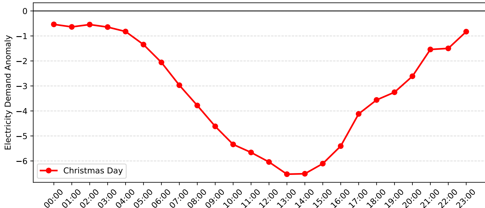
Broadmeadow Demand Anomaly: Christmas Day (2015-2016)
