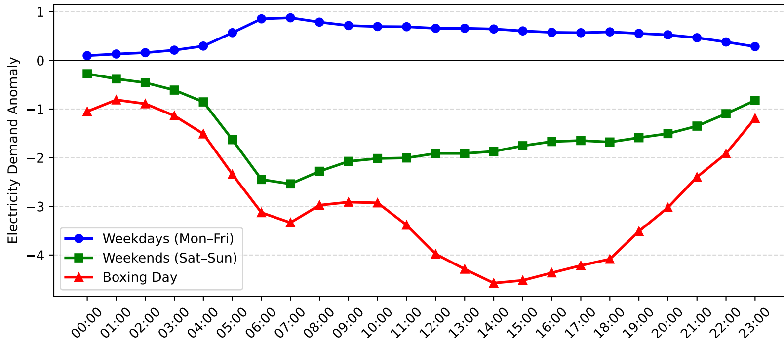
Lisarow Demand Anomaly: Boxing Day vs Weekday/Weekend (2012-2013)
