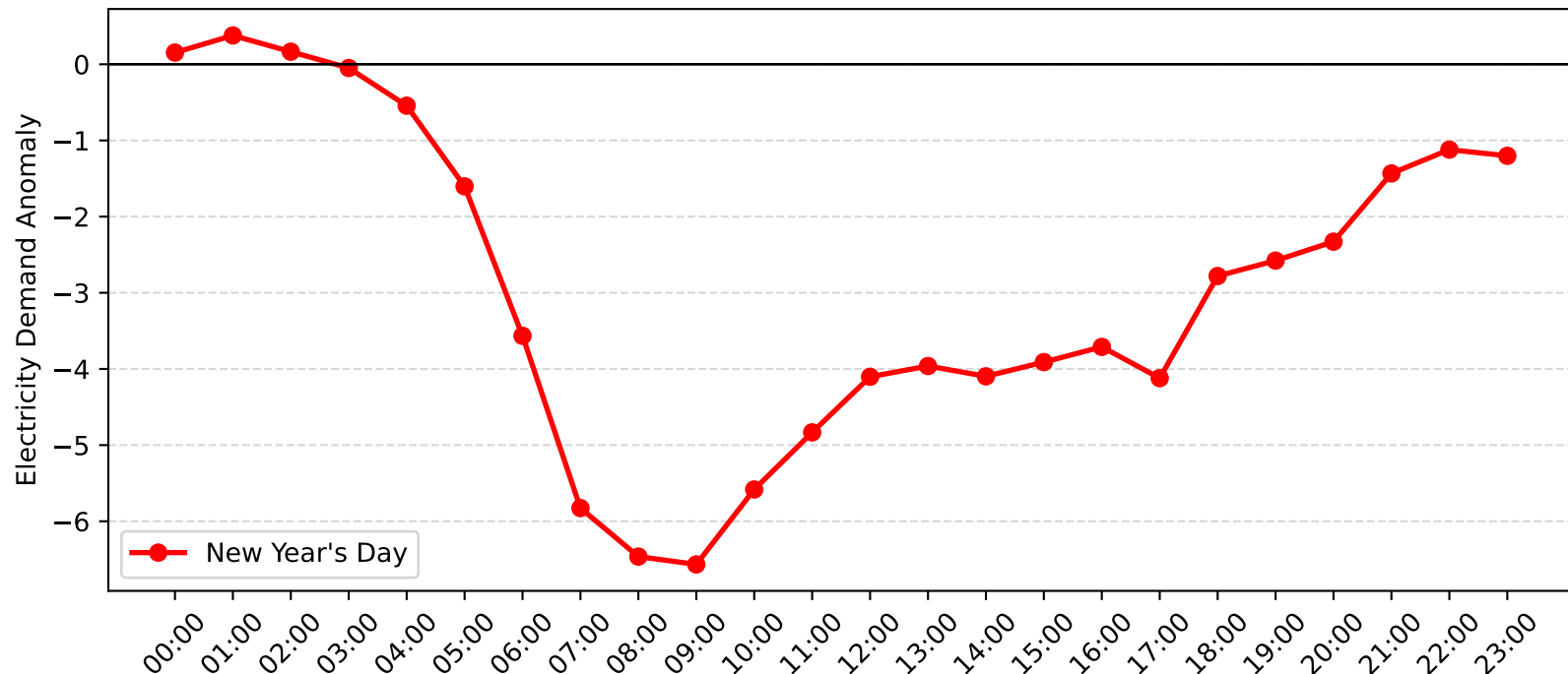
Top Ryde Demand Anomaly: New Year's Day (2012-2013)
