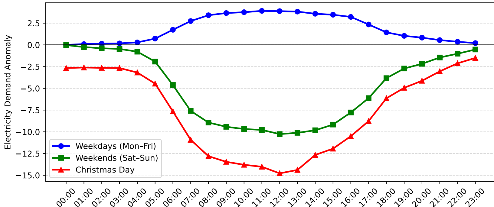
Mascot Demand Anomaly: Christmas Day vs Weekday/Weekend (2009-2010)
