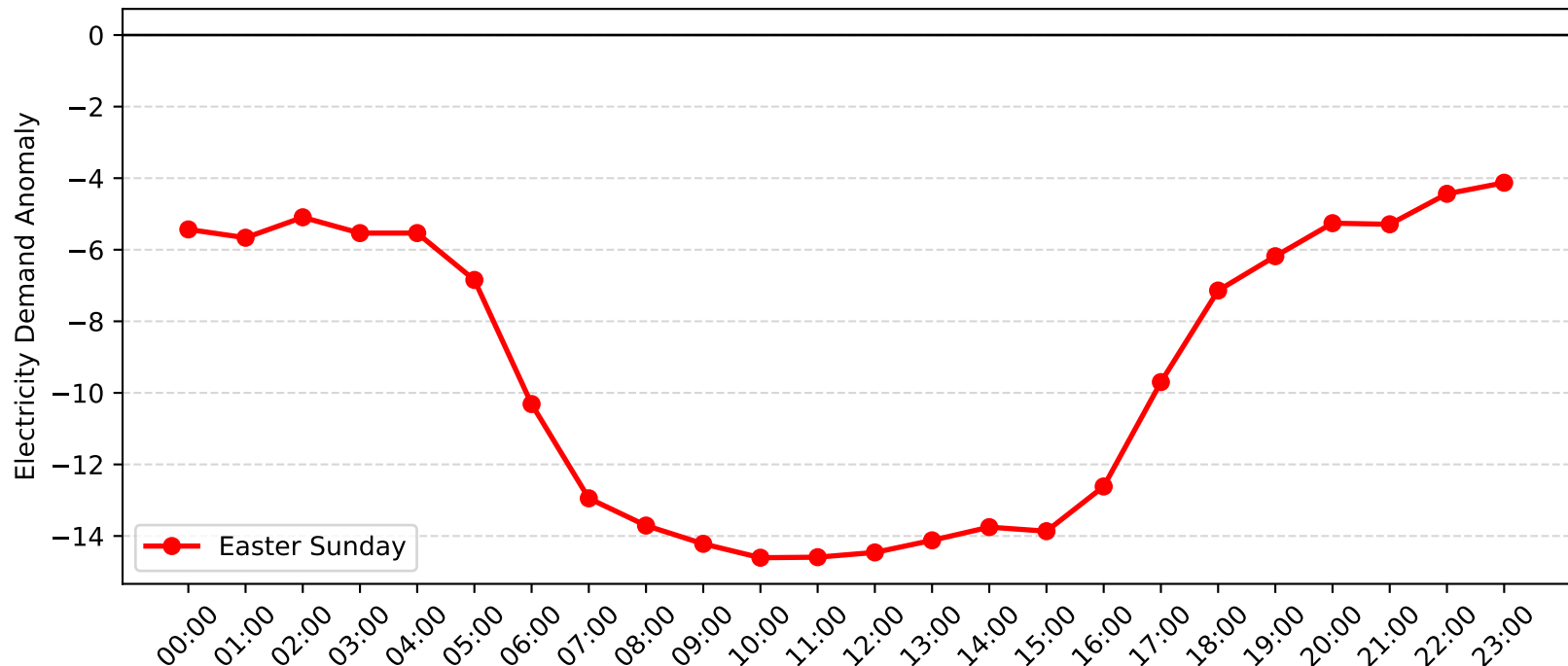
Flemington Demand Anomaly: Easter Sunday (2006-2007)
