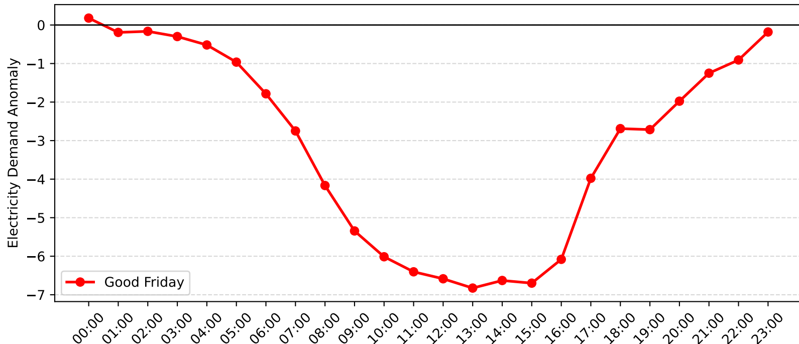
Erina Demand Anomaly: Good Friday (2017-2018)
