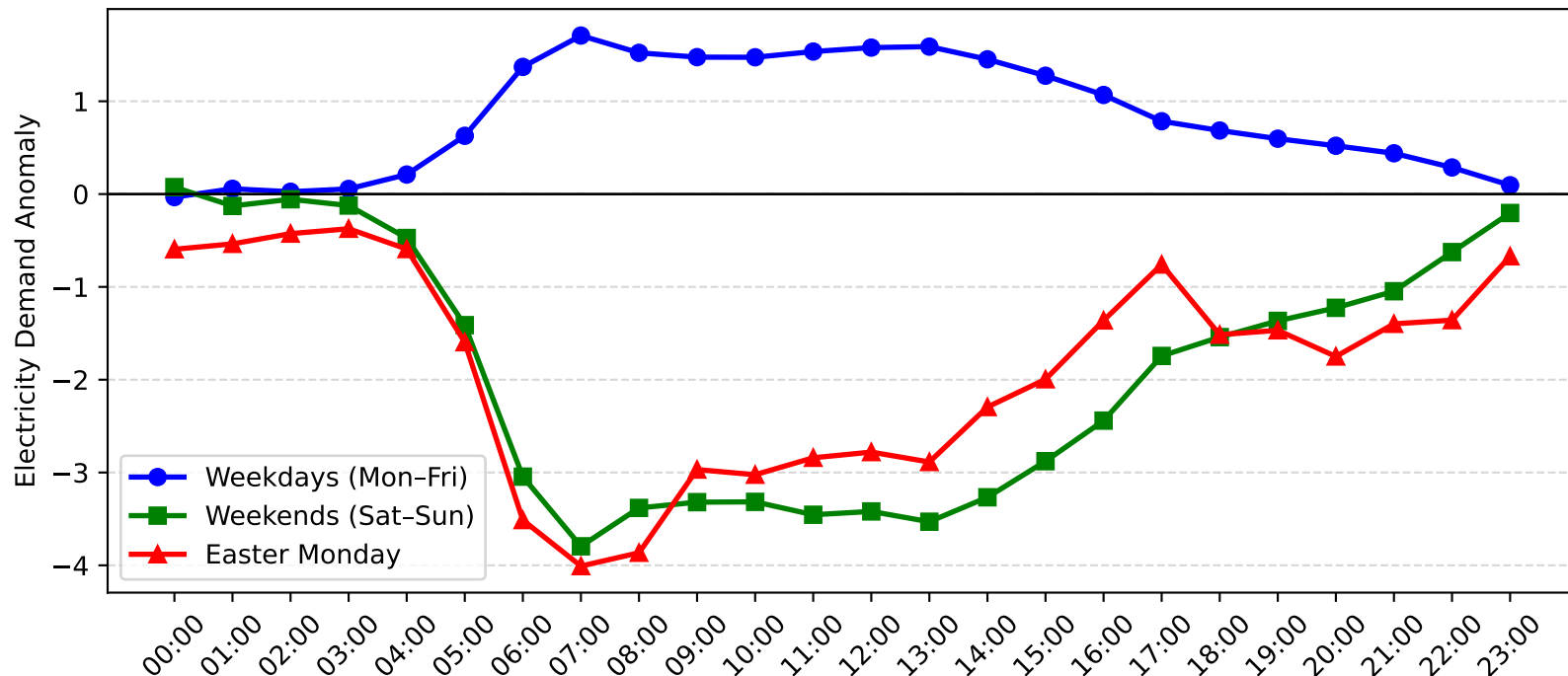
Wyong Demand Anomaly: Easter Monday vs Weekday/Weekend (2008-2009)
