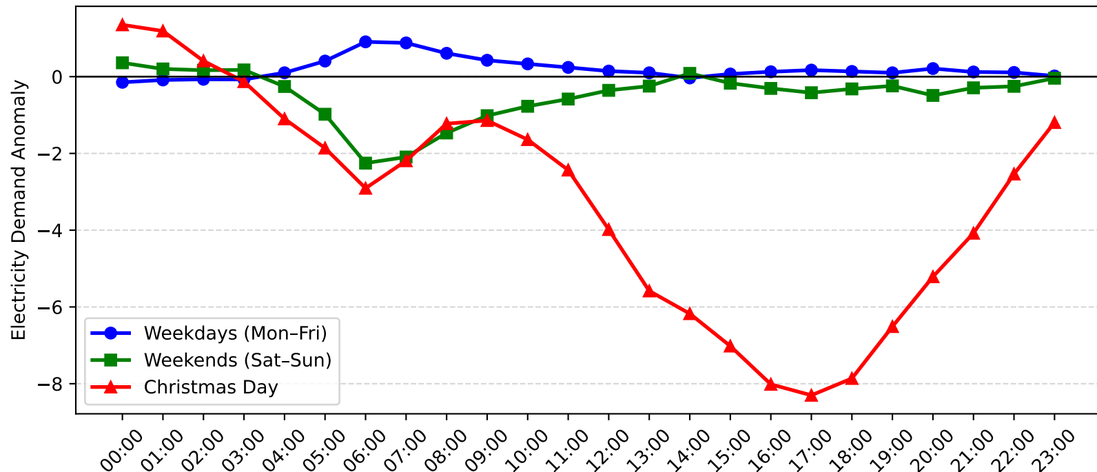
Revesby Demand Anomaly: Christmas Day vs Weekday/Weekend (2006-2007)
