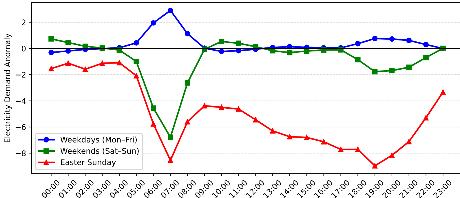
Mosman Demand Anomaly: Easter Sunday vs Weekday/Weekend (2014-2015)
