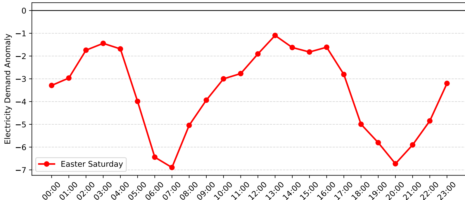
Meadowbank Demand Anomaly: Easter Saturday (2011-2012)
