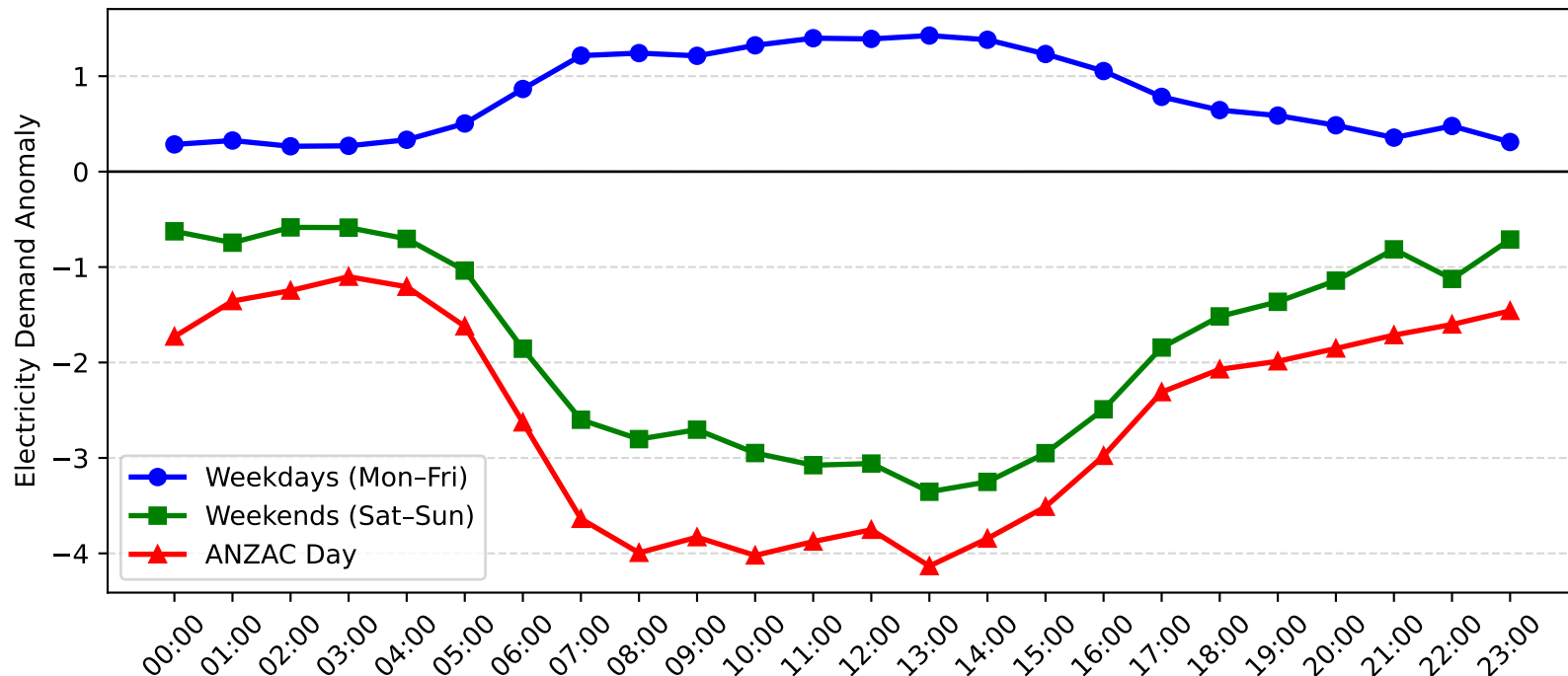
Mayfield West Demand Anomaly: ANZAC Day vs Weekday/Weekend (2010-2011)
