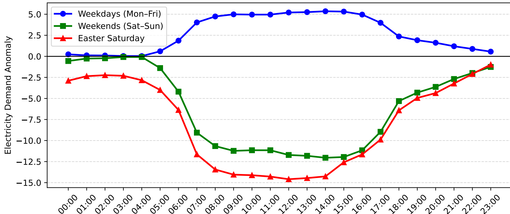
Gore Hill Demand Anomaly: Easter Saturday vs Weekday/Weekend (2012-2013)
