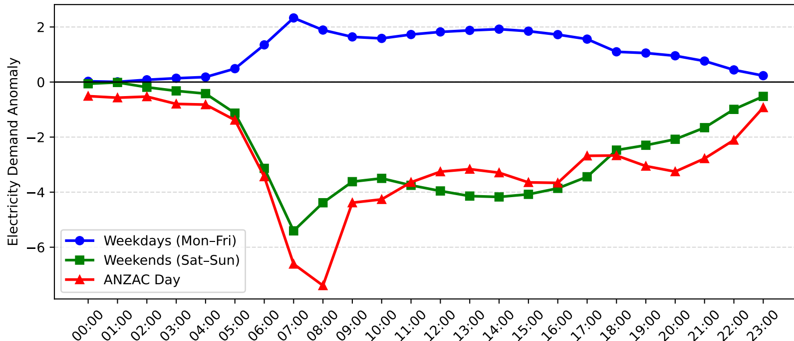
Epping Demand Anomaly: ANZAC Day vs Weekday/Weekend (2016-2017)
