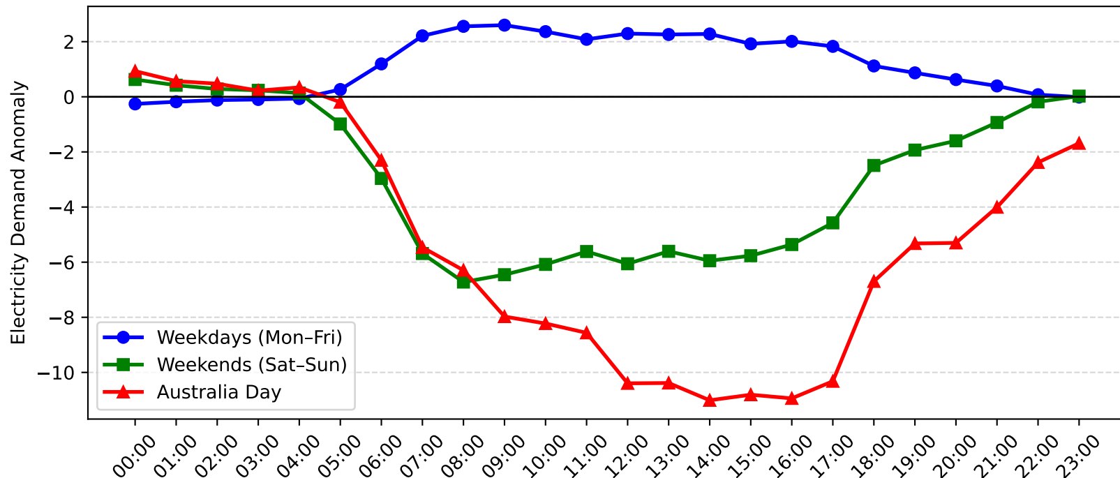
Castle Cove Demand Anomaly: Australia Day vs Weekday/Weekend (2014-2015)
