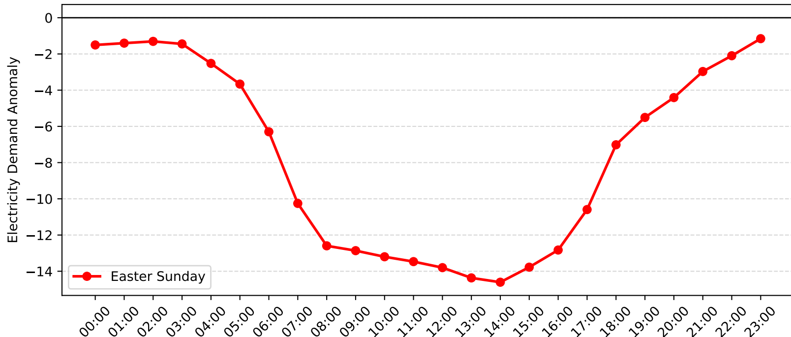
Gore Hill Demand Anomaly: Easter Sunday (2016-2017)
