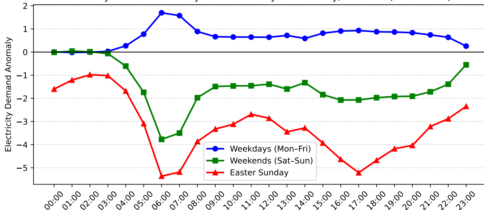
Revesby Demand Anomaly: Easter Sunday vs Weekday/Weekend (2008-2009)
