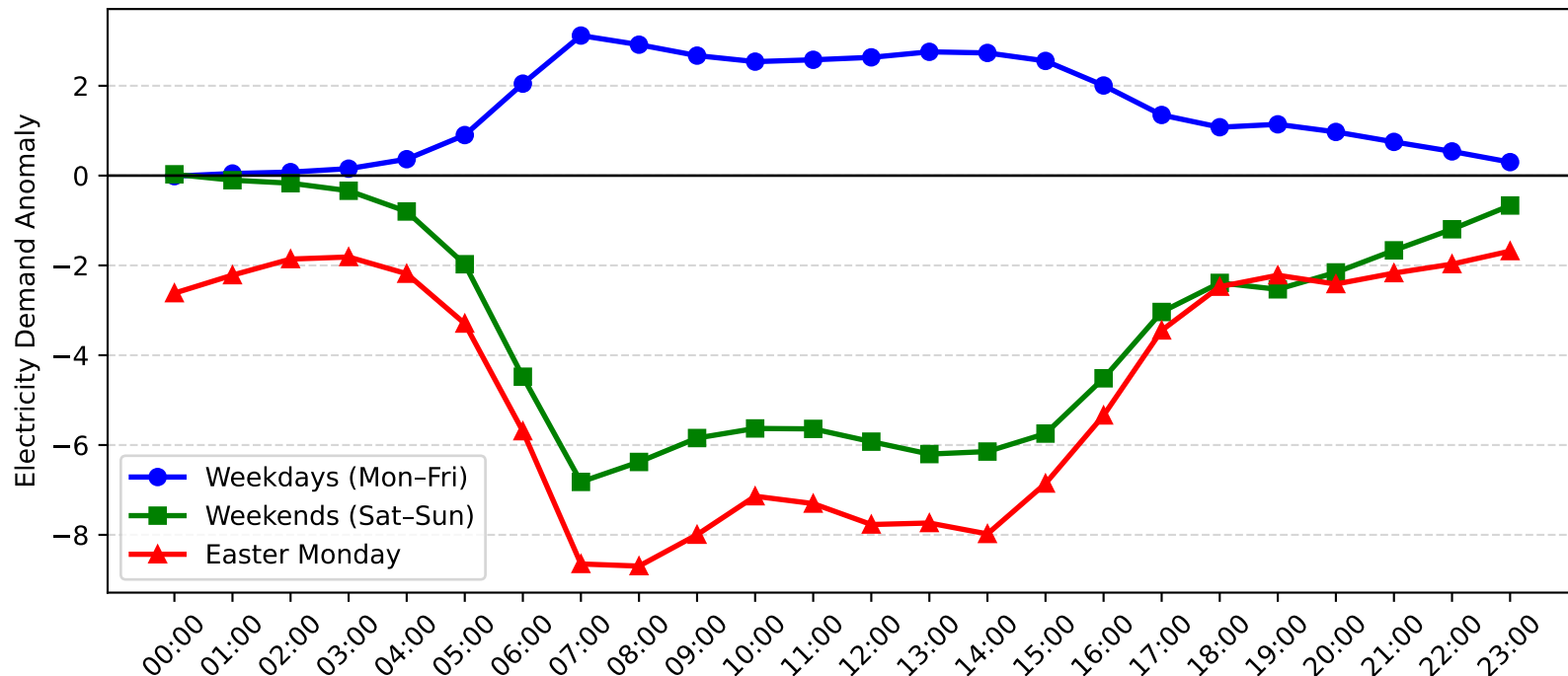
Marrickville Demand Anomaly: Easter Monday vs Weekday/Weekend (2016-2017)
