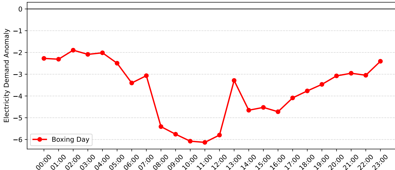
Mayfield West Demand Anomaly: Boxing Day (2014-2015)
