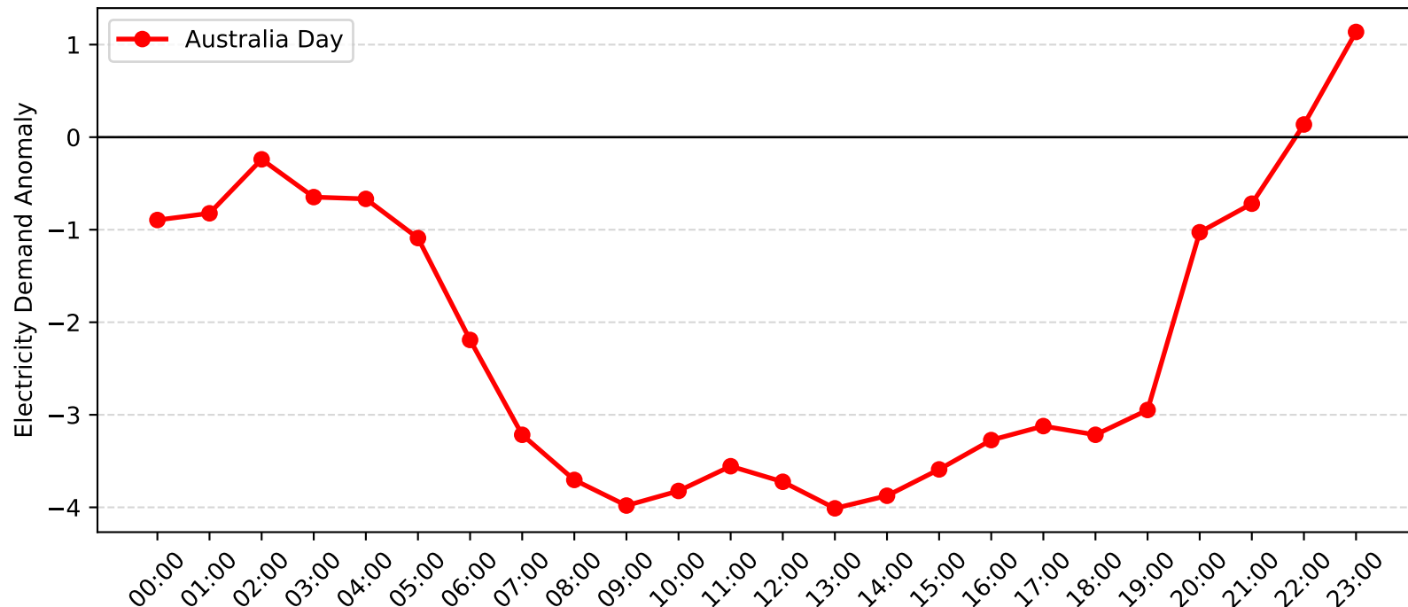
Pymble Demand Anomaly: Australia Day (2006-2007)
