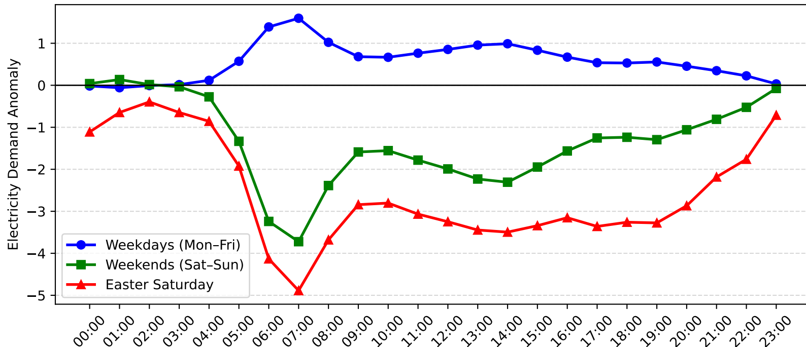
Kirrawee Demand Anomaly: Easter Saturday vs Weekday/Weekend (2014-2015)
