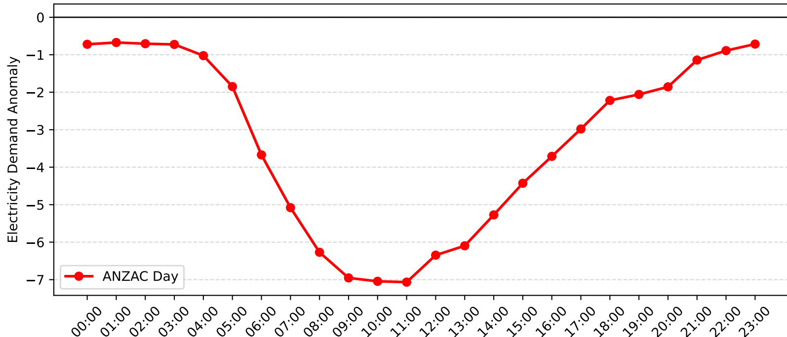
Auburn Demand Anomaly: ANZAC Day (2011-2012)
