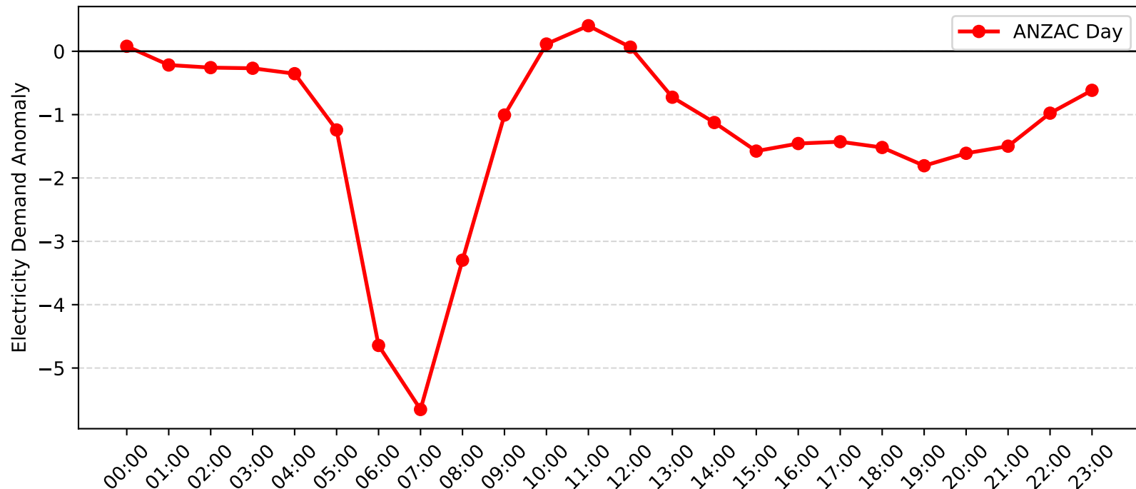
Mortdale Demand Anomaly: ANZAC Day (2011-2012)
