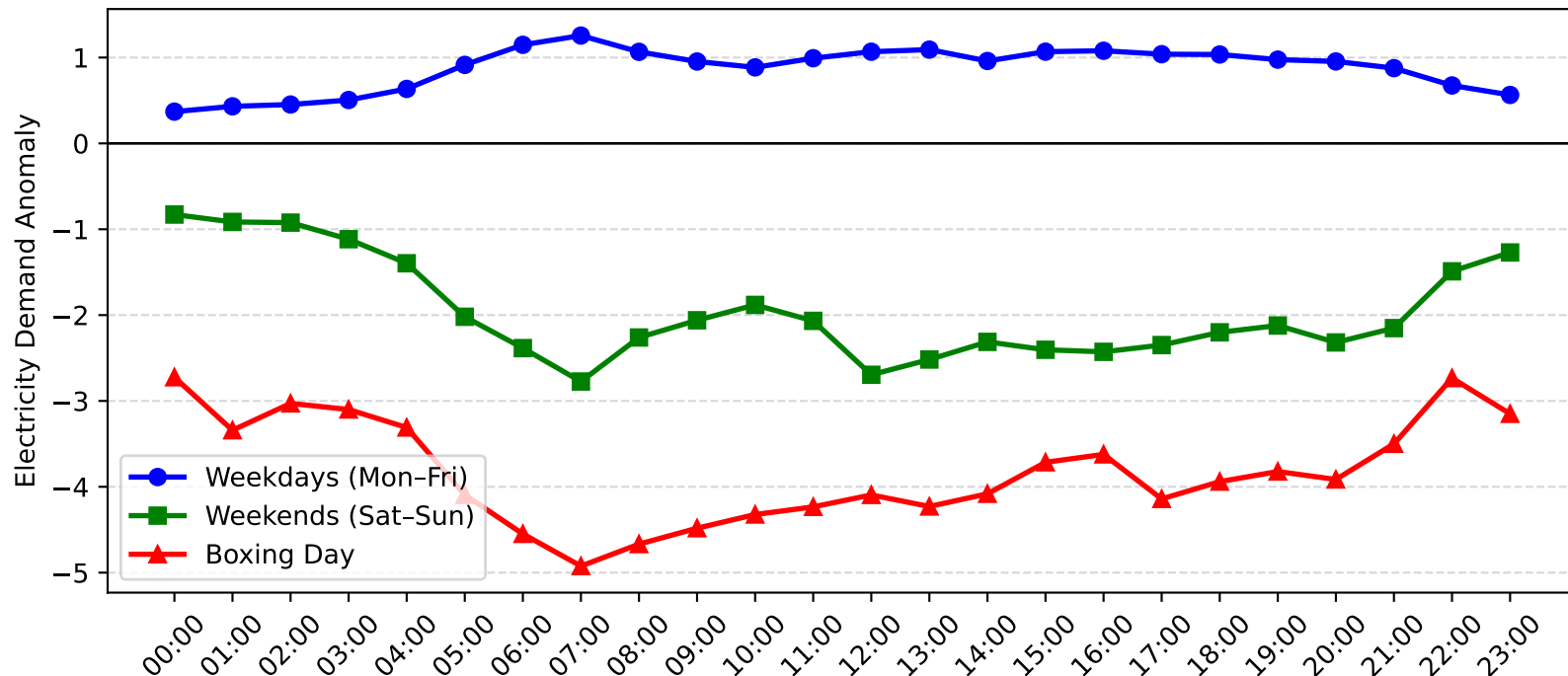
Lisarow Demand Anomaly: Boxing Day vs Weekday/Weekend (2004-2005)
