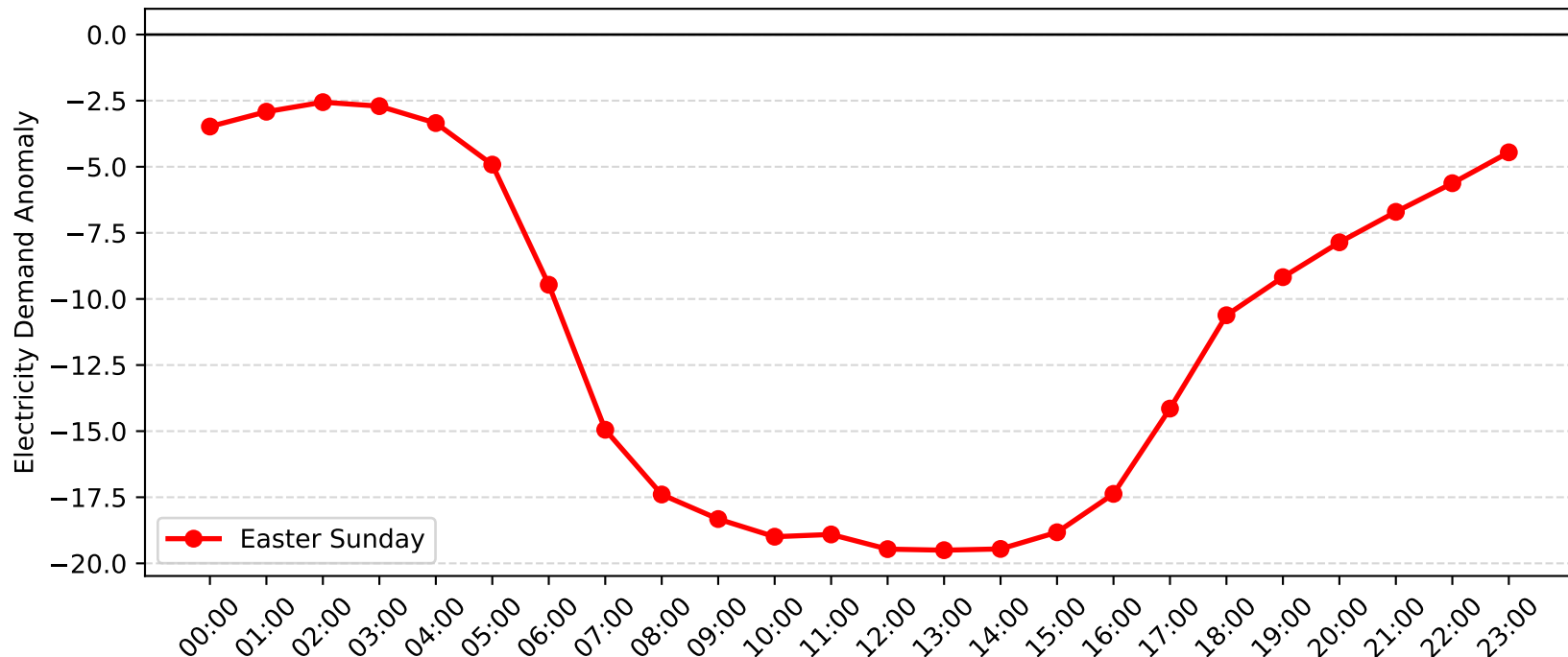
Gore Hill Demand Anomaly: Easter Sunday (2010-2011)
