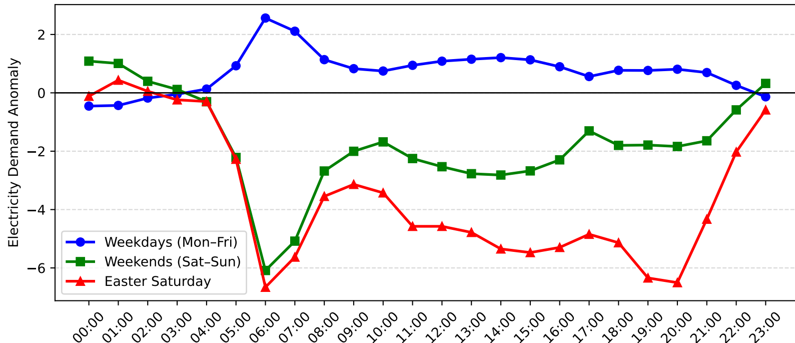
Pennant Hills Demand Anomaly: Easter Saturday vs Weekday/Weekend (2006-2007)
