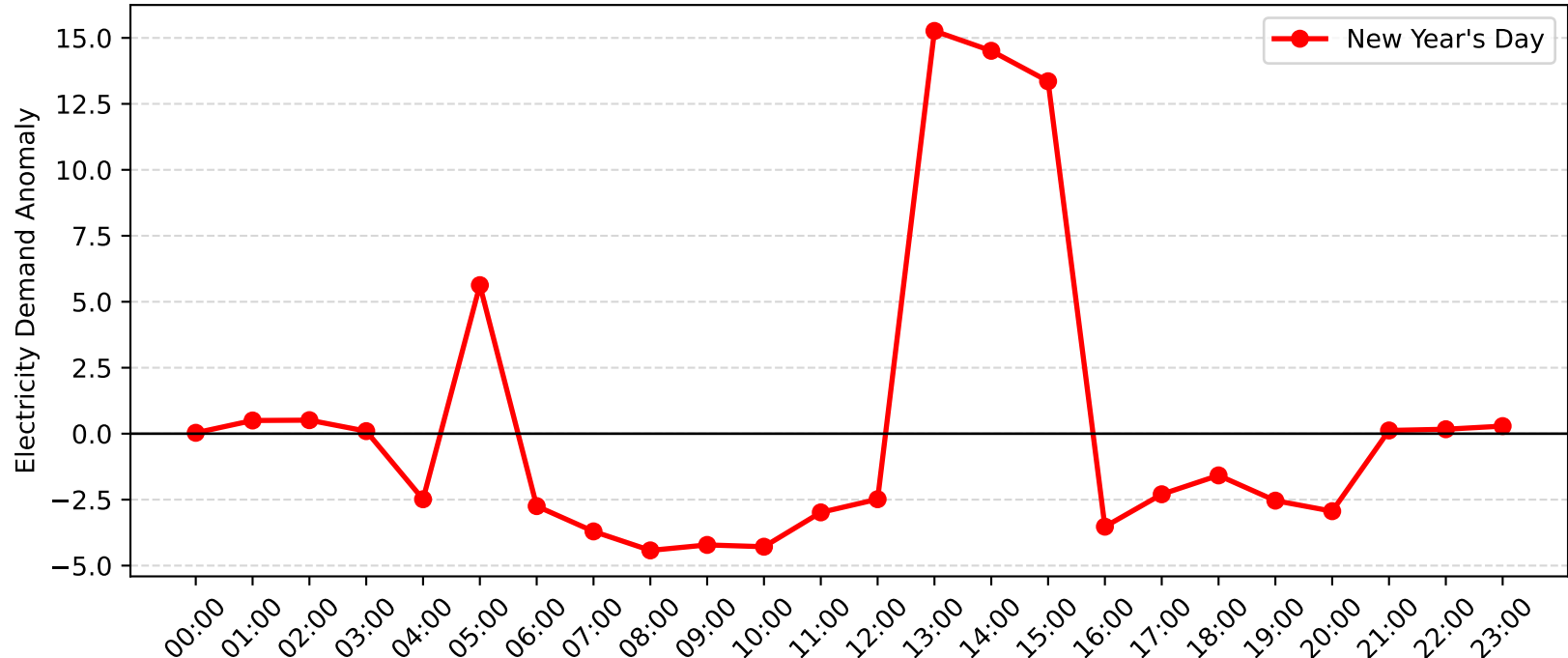
Kogarah Demand Anomaly: New Year's Day (2010-2011)
