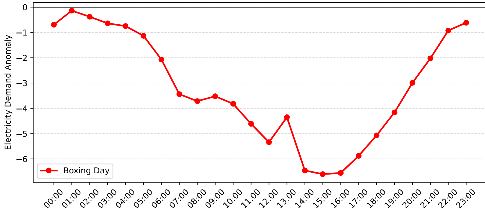
Jesmond Demand Anomaly: Boxing Day (2013-2014)
