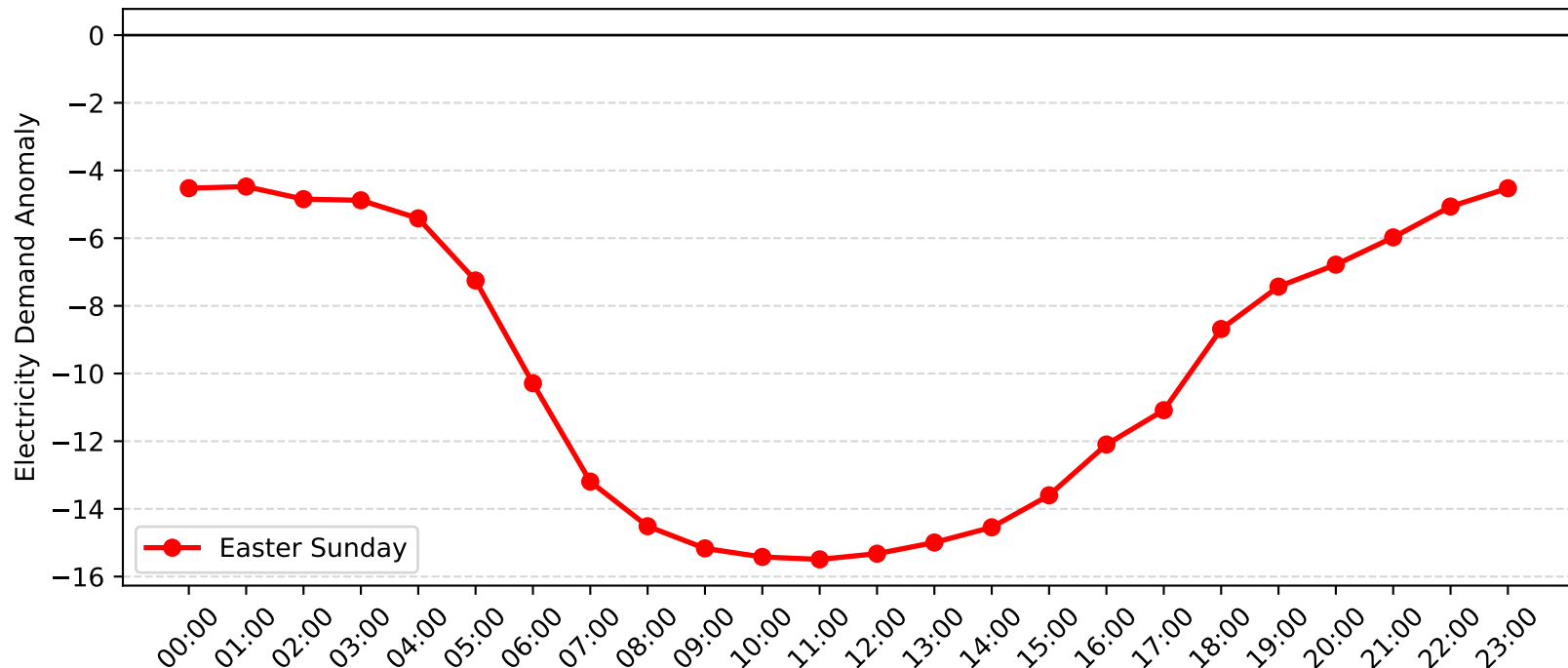
Flemington Demand Anomaly: Easter Sunday (2013-2014)
