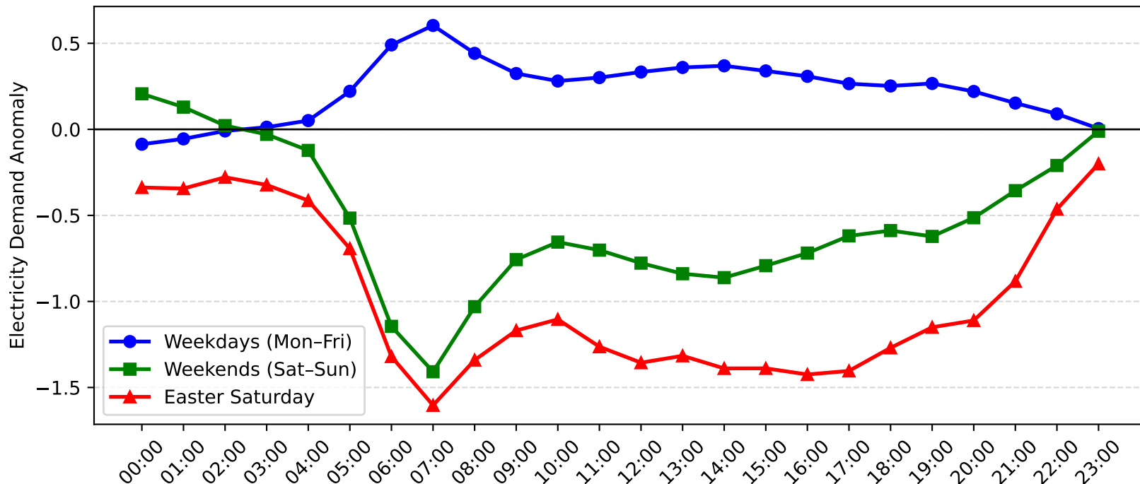
Rockdale Demand Anomaly: Easter Saturday vs Weekday/Weekend (2013-2014)
