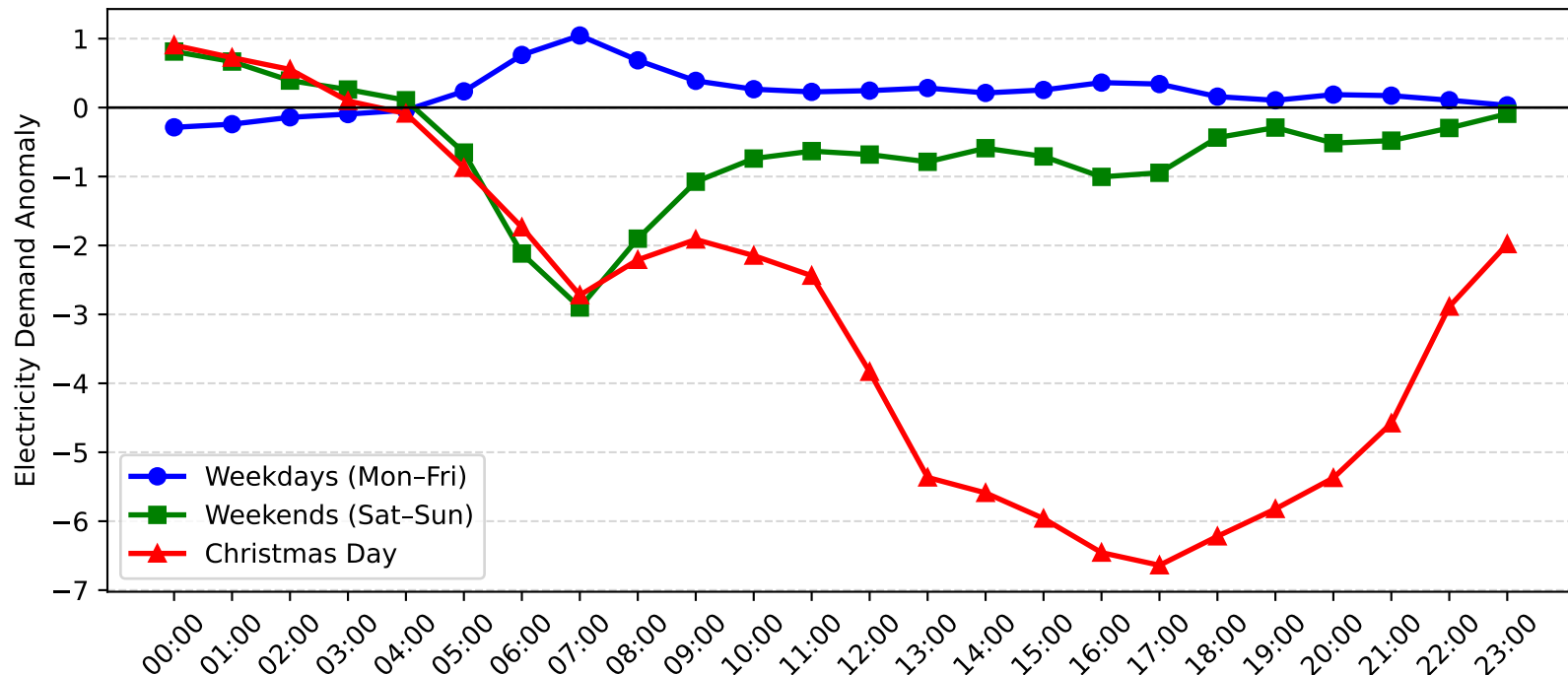
Dulwich Hill Demand Anomaly: Christmas Day vs Weekday/Weekend (2012-2013)
