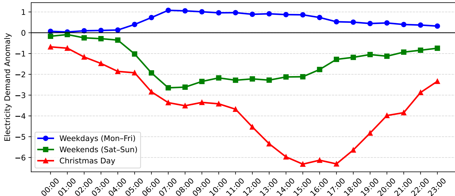
Bass Hill Demand Anomaly: Christmas Day vs Weekday/Weekend (2006-2007)
