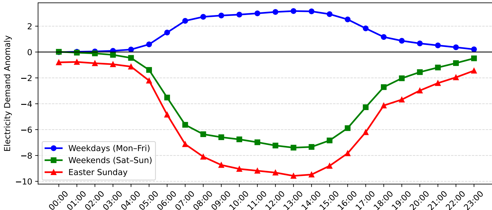
Mascot Demand Anomaly: Easter Sunday vs Weekday/Weekend (2014-2015)
