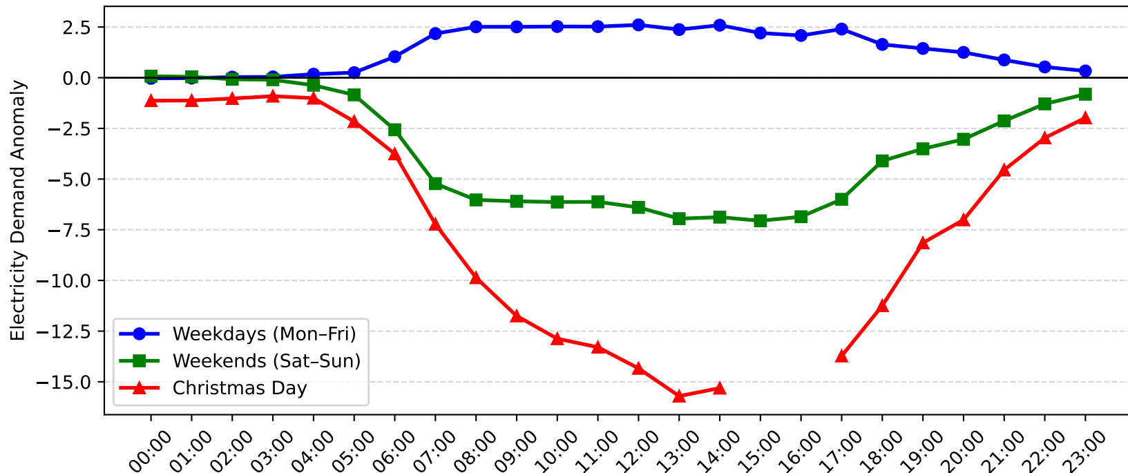
Castle Cove Demand Anomaly: Christmas Day vs Weekday/Weekend (2015-2016)
