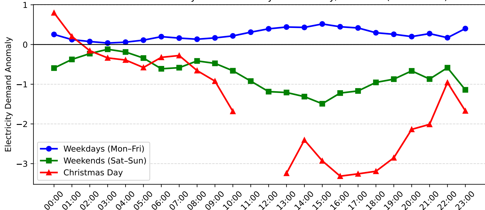
Telarah Demand Anomaly: Christmas Day vs Weekday/Weekend (2008-2009)
