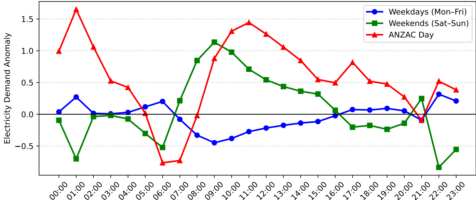
Swansea Demand Anomaly: ANZAC Day vs Weekday/Weekend (2007-2008)
