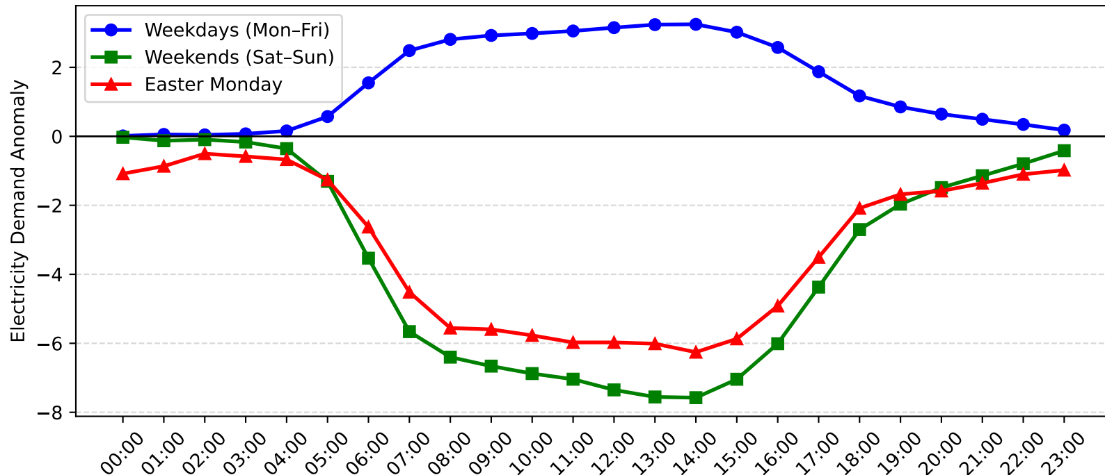
Mascot Demand Anomaly: Easter Monday vs Weekday/Weekend (2015-2016)
