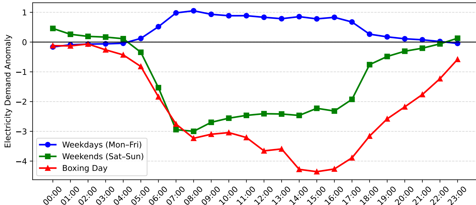
Pymble Demand Anomaly: Boxing Day vs Weekday/Weekend (2013-2014)
