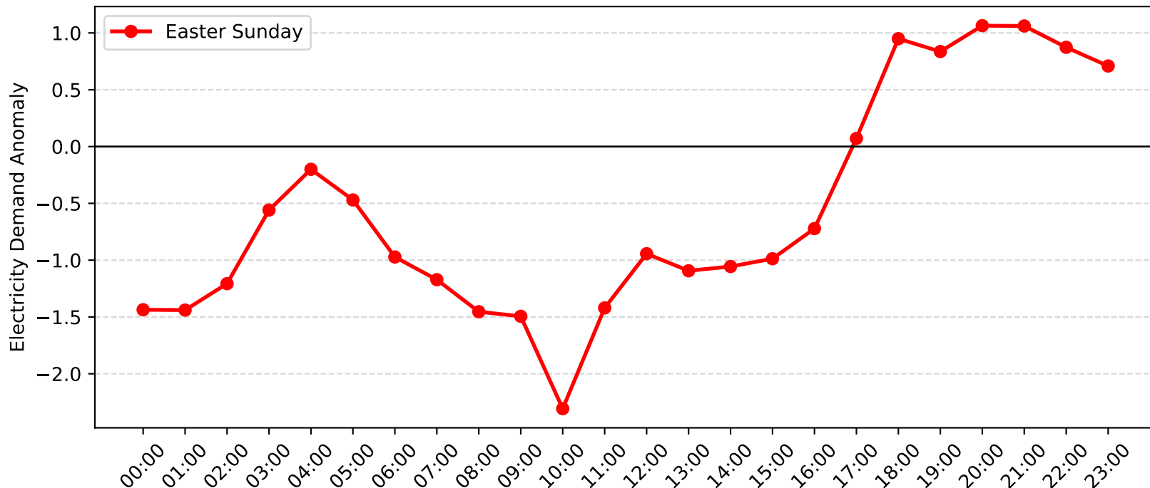
Gateshead Demand Anomaly: Easter Sunday (2004-2005)
