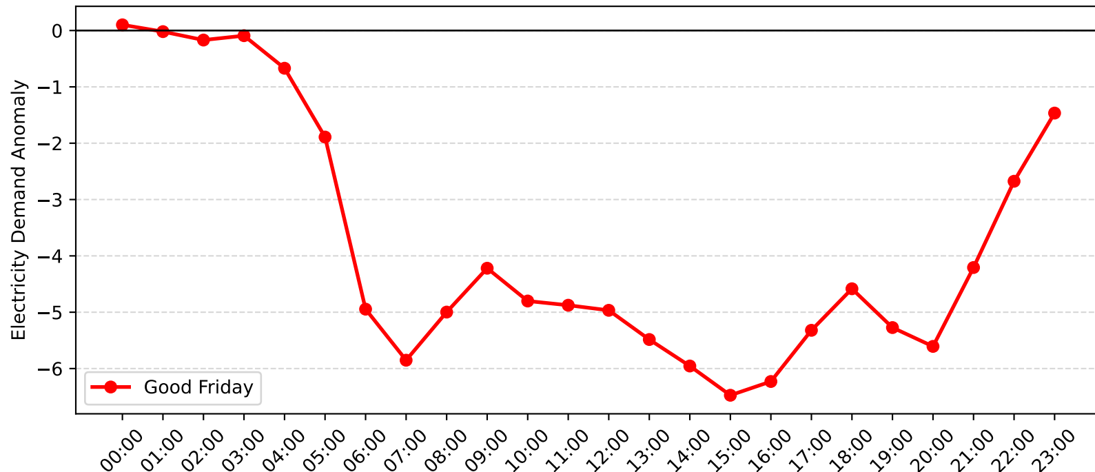
Dulwich Hill Demand Anomaly: Good Friday (2007-2008)
