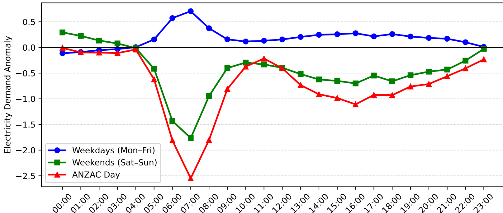
Blakehurst Demand Anomaly: ANZAC Day vs Weekday/Weekend (2011-2012)
