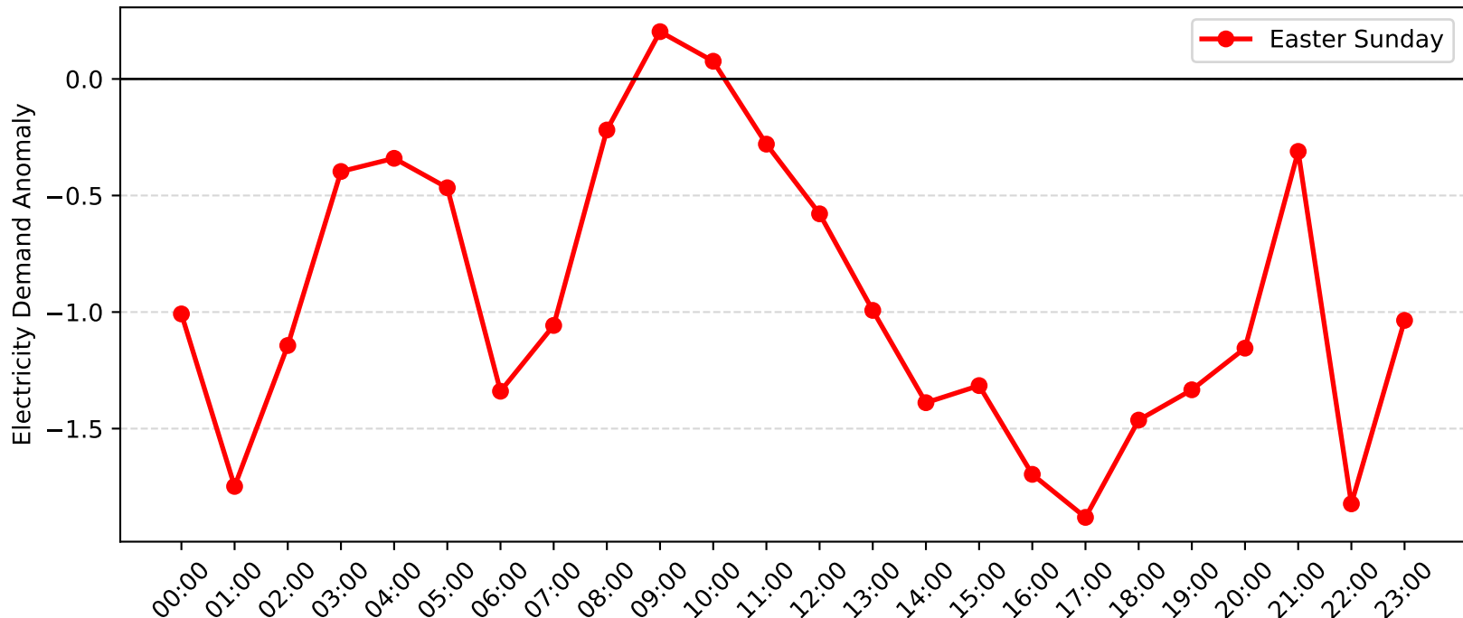
Jewells Demand Anomaly: Easter Sunday (2006-2007)
