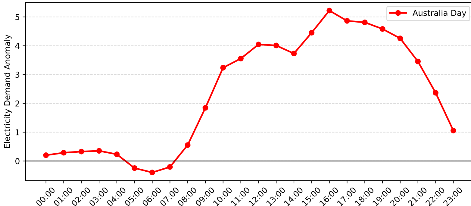
Woy Woy Demand Anomaly: Australia Day (2010-2011)
