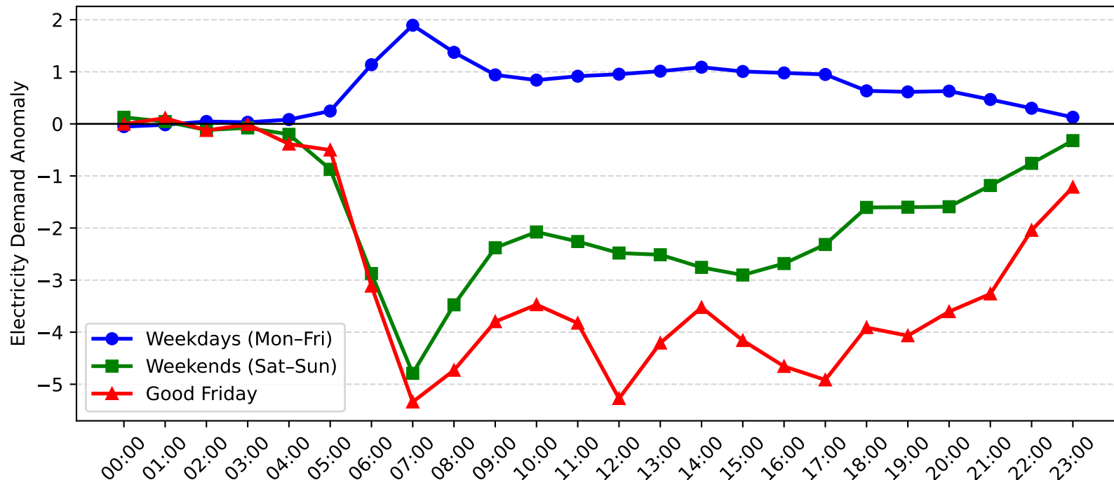
Chatswood Demand Anomaly: Good Friday vs Weekday/Weekend (2014-2015)
