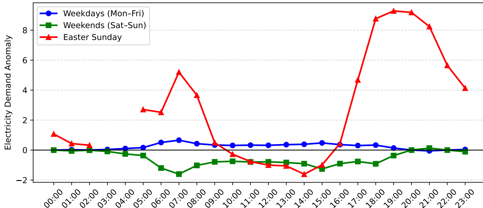
Dulwich Hill Demand Anomaly: Easter Sunday vs Weekday/Weekend (2004-2005)
