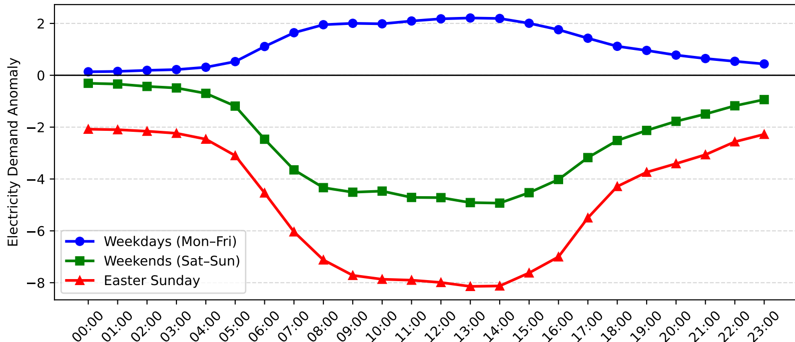
Caringbah Demand Anomaly: Easter Sunday vs Weekday/Weekend (2008-2009)
