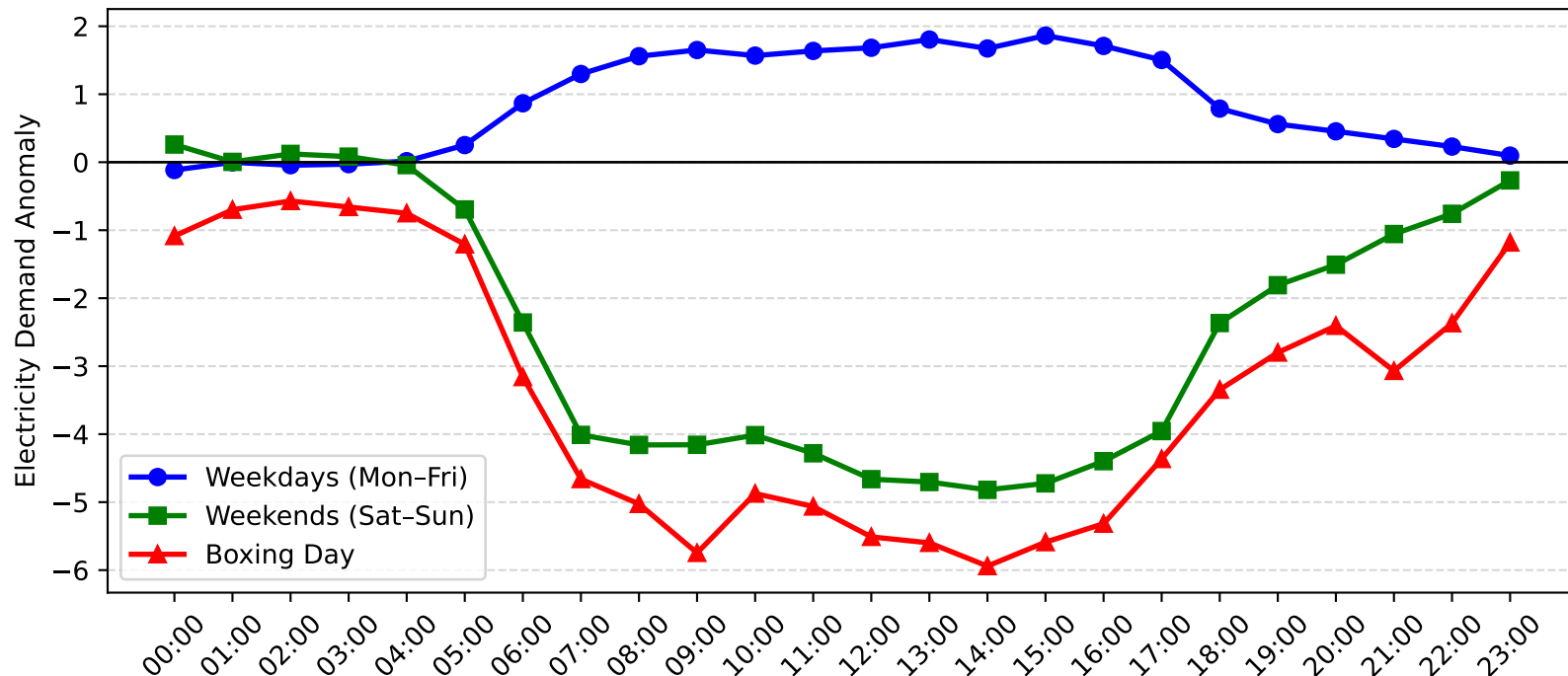
Pymble Demand Anomaly: Boxing Day vs Weekday/Weekend (2008-2009)
