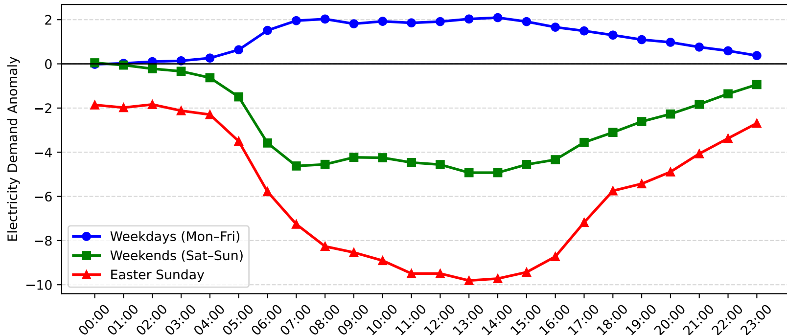
Caringbah Demand Anomaly: Easter Sunday vs Weekday/Weekend (2005-2006)
