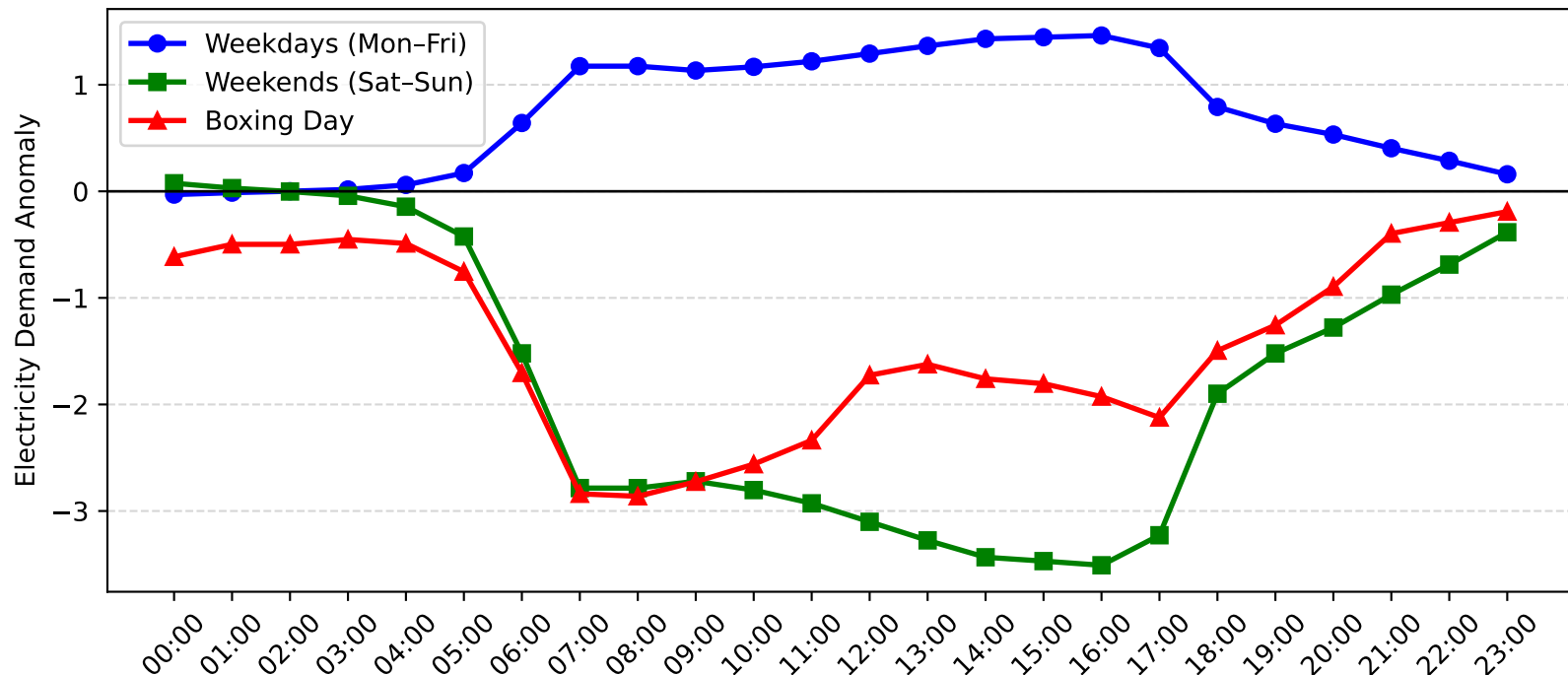
Pymble Demand Anomaly: Boxing Day vs Weekday/Weekend (2015-2016)
