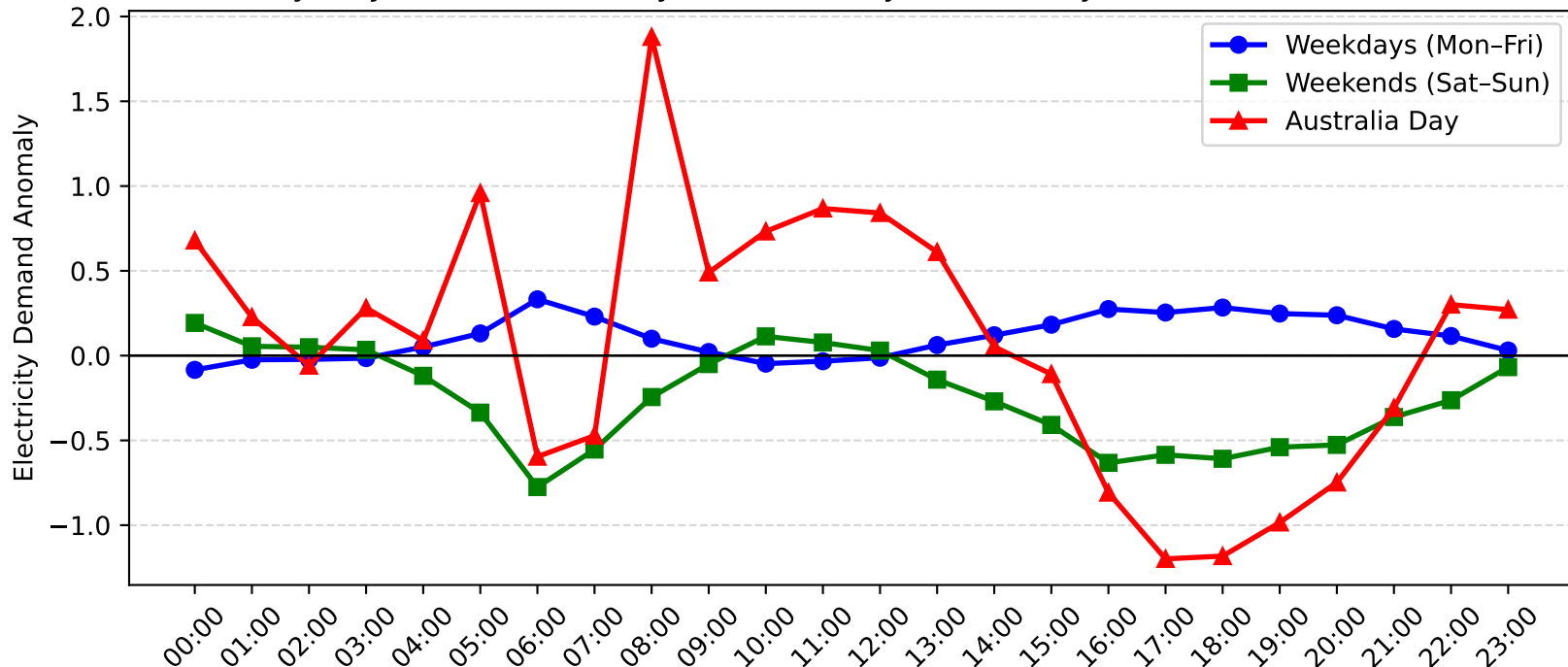
Woy Woy Demand Anomaly: Australia Day vs Weekday/Weekend (2013-2014)
