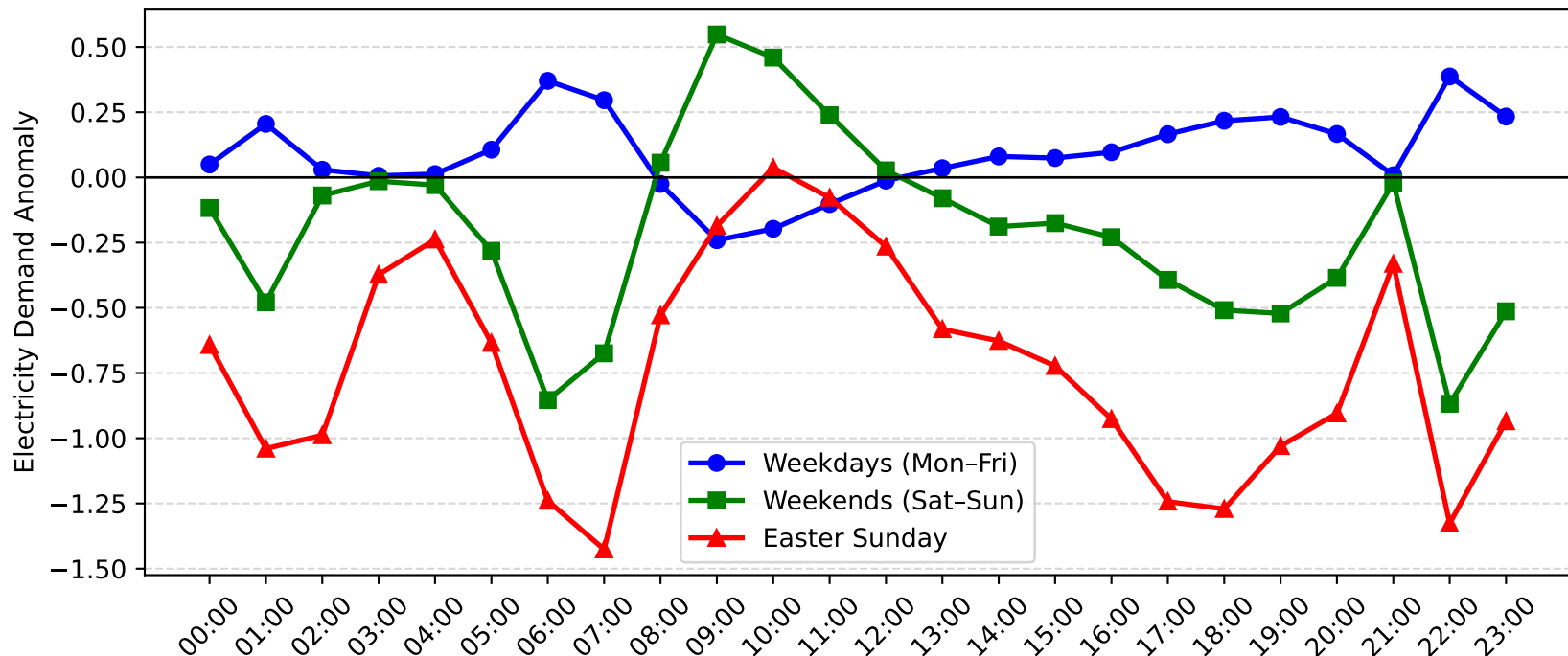
Jewells Demand Anomaly: Easter Sunday vs Weekday/Weekend (2008-2009)
