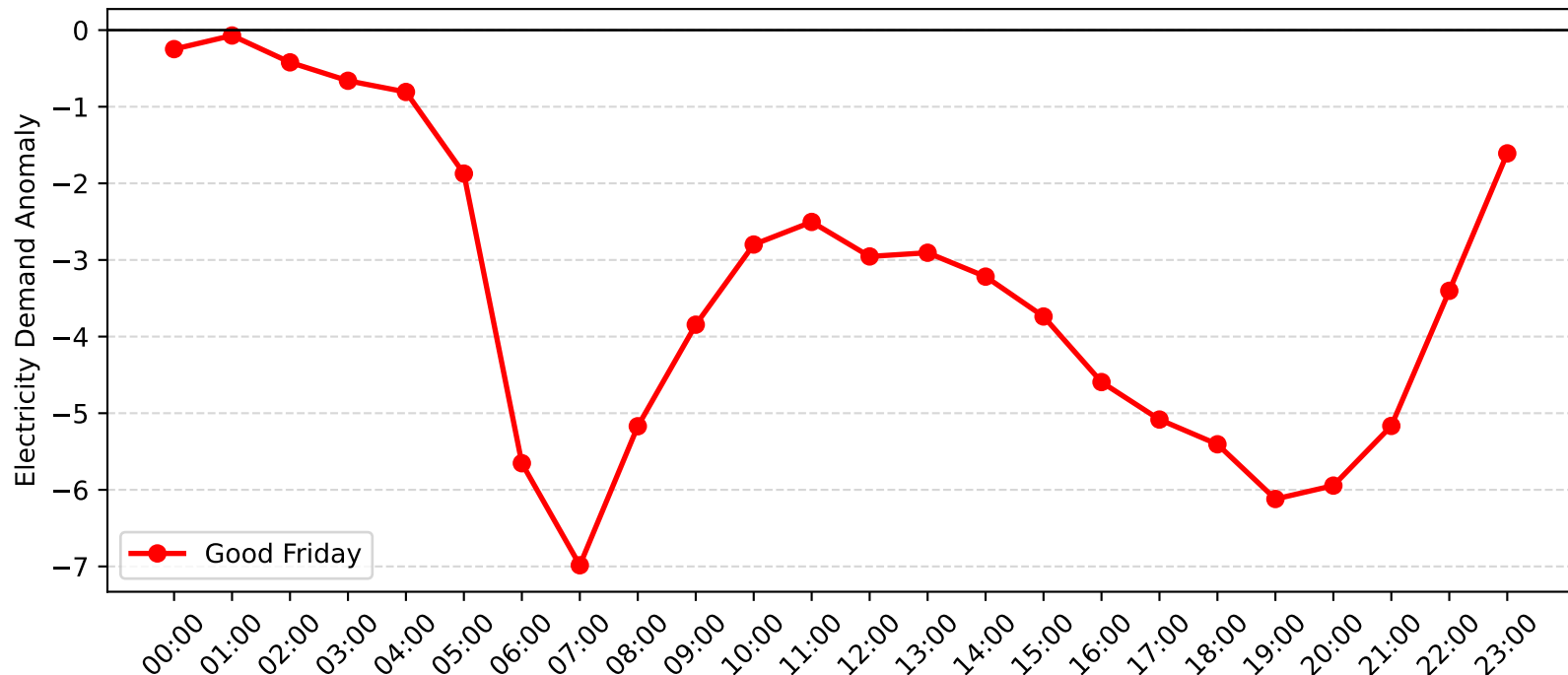
Pennant Hills Demand Anomaly: Good Friday (2014-2015)
