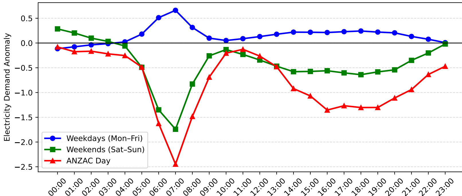
Blakehurst Demand Anomaly: ANZAC Day vs Weekday/Weekend (2013-2014)
