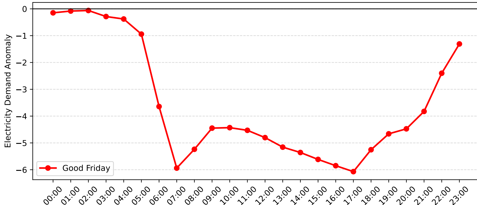
Chatswood Demand Anomaly: Good Friday (2010-2011)
