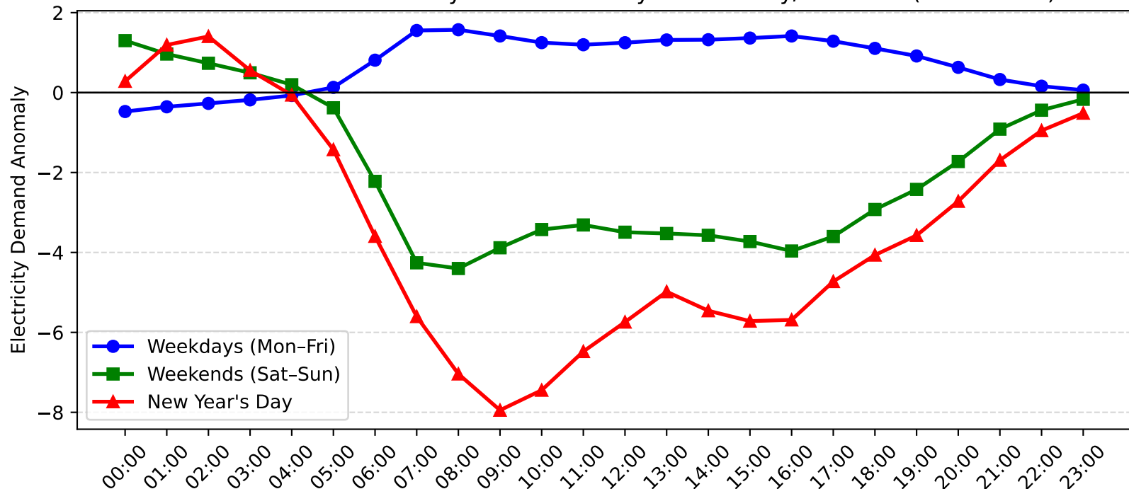
Burwood Demand Anomaly: New Year's Day vs Weekday/Weekend (2013-2014)
