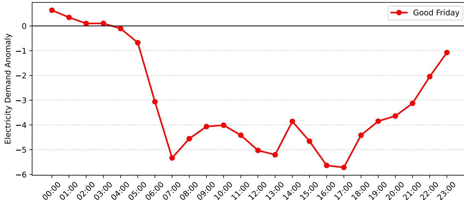
Chatswood Demand Anomaly: Good Friday (2013-2014)
