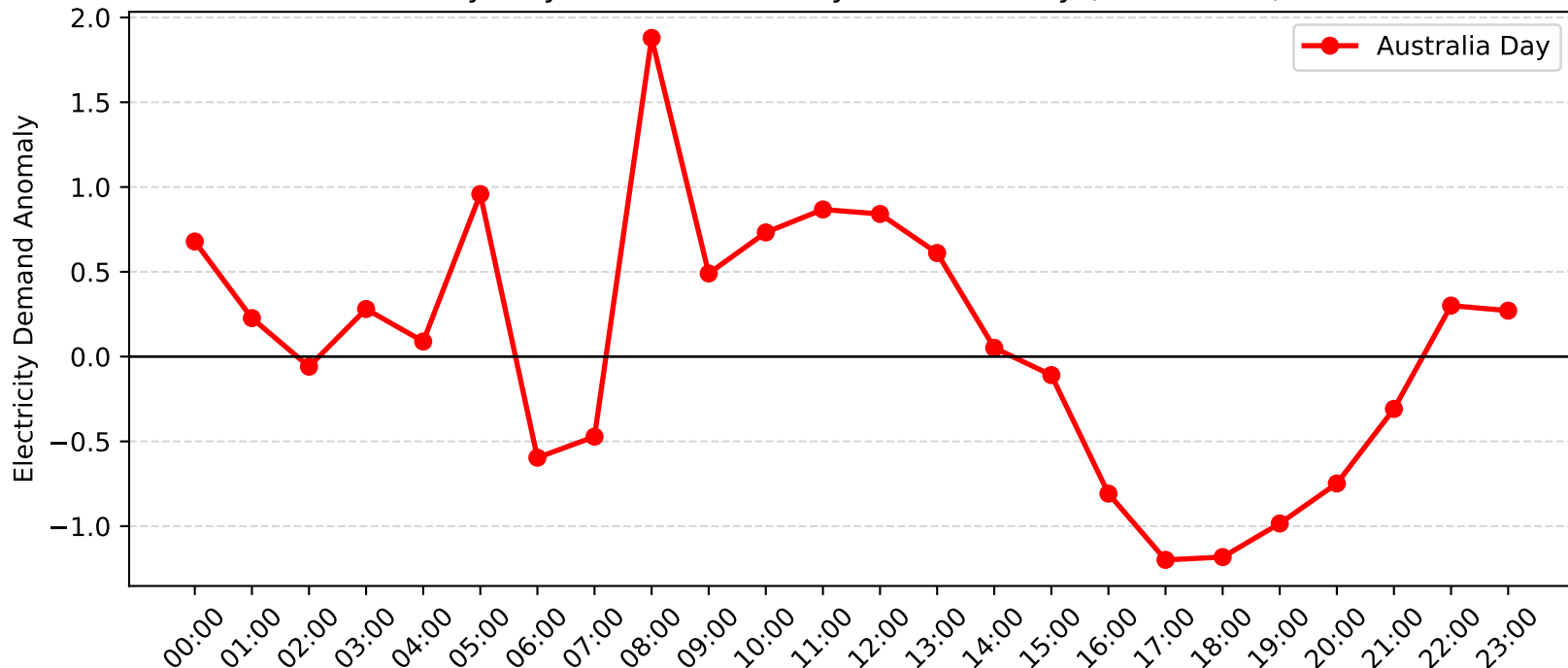
Woy Woy Demand Anomaly: Australia Day (2013-2014)
