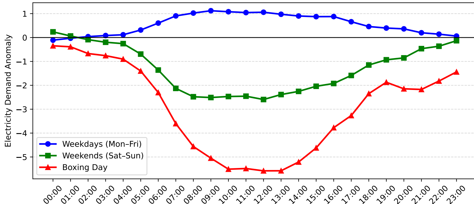
Lidcombe Demand Anomaly: Boxing Day vs Weekday/Weekend (2009-2010)
