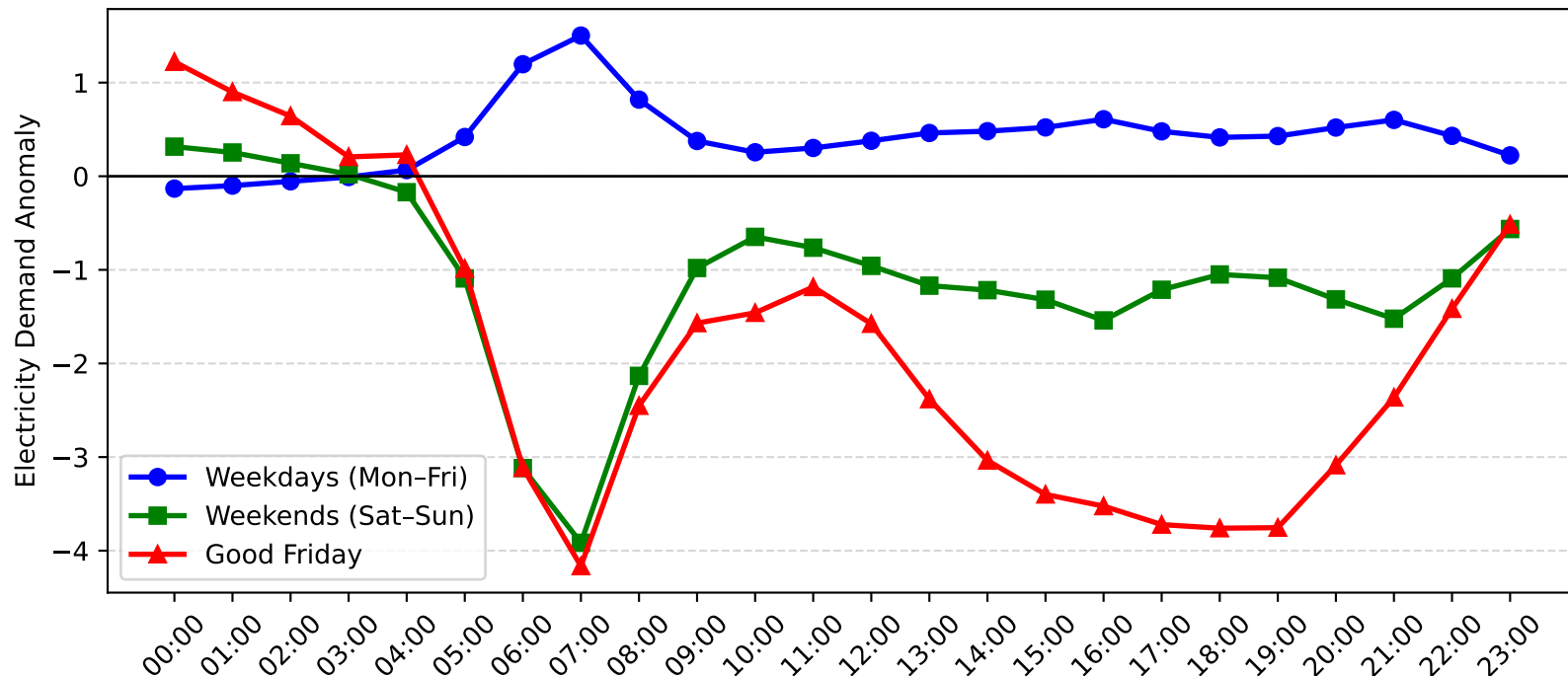
Dulwich Hill Demand Anomaly: Good Friday vs Weekday/Weekend (2012-2013)
