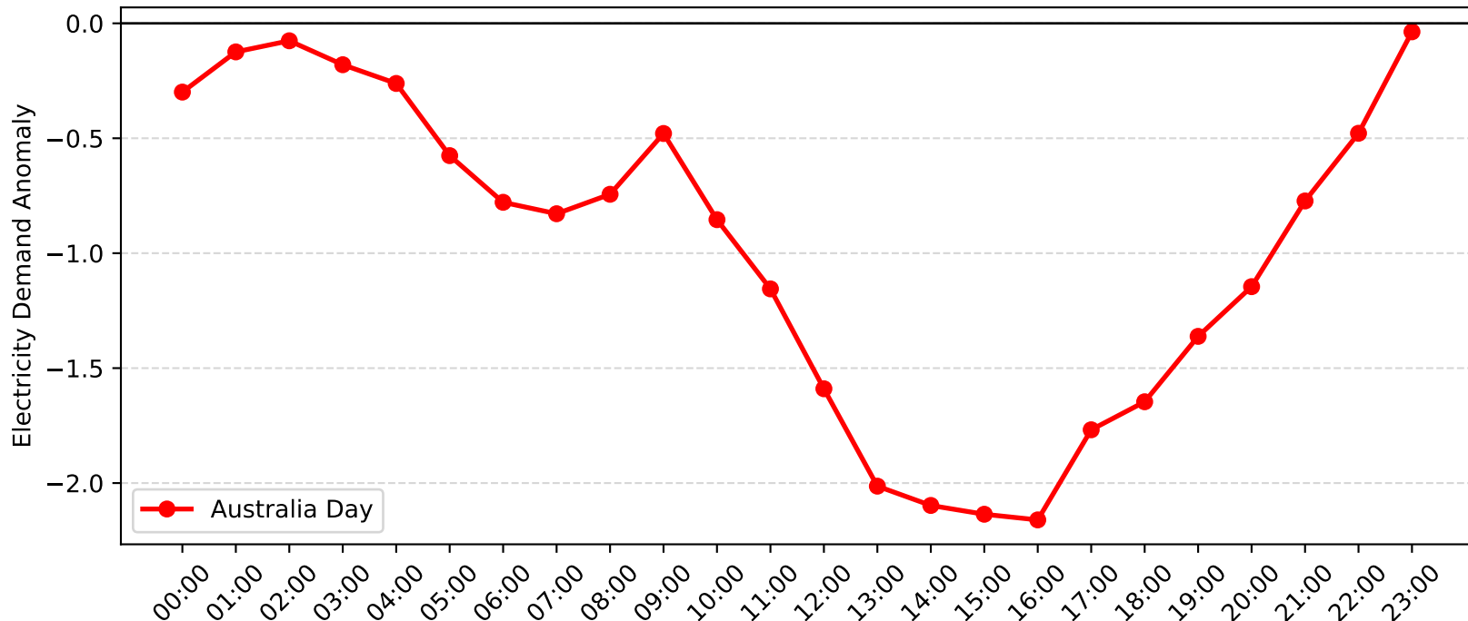
Woy Woy Demand Anomaly: Australia Day (2016-2017)
