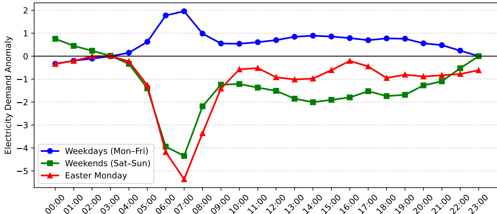
Mortdale Demand Anomaly: Easter Monday vs Weekday/Weekend (2008-2009)
