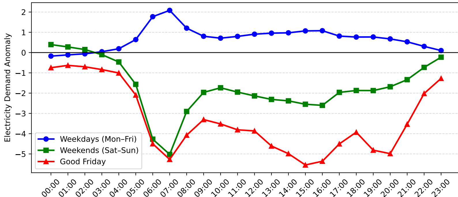
Dulwich Hill Demand Anomaly: Good Friday vs Weekday/Weekend (2008-2009)
