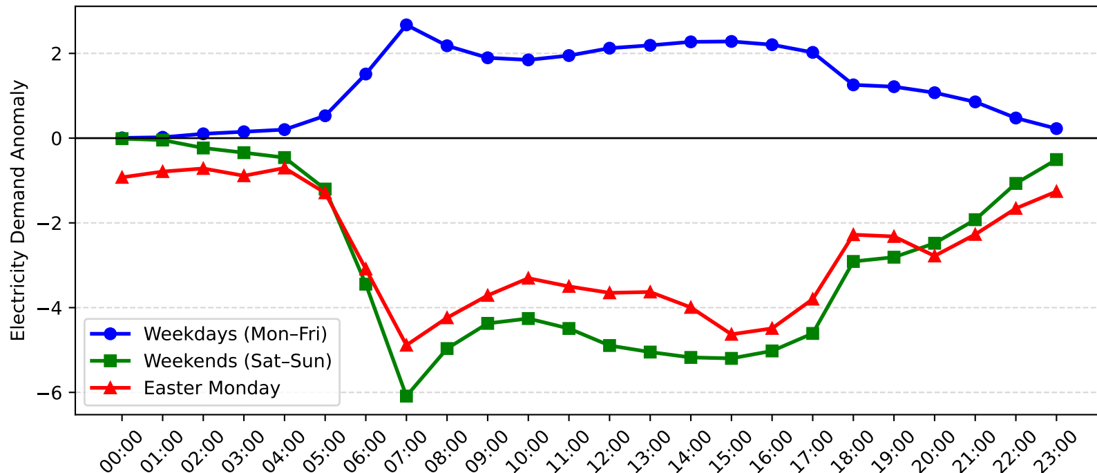
Epping Demand Anomaly: Easter Monday vs Weekday/Weekend (2015-2016)
