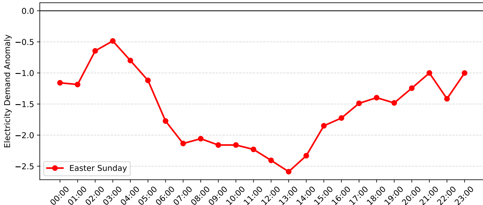
Gateshead Demand Anomaly: Easter Sunday (2017-2018)
