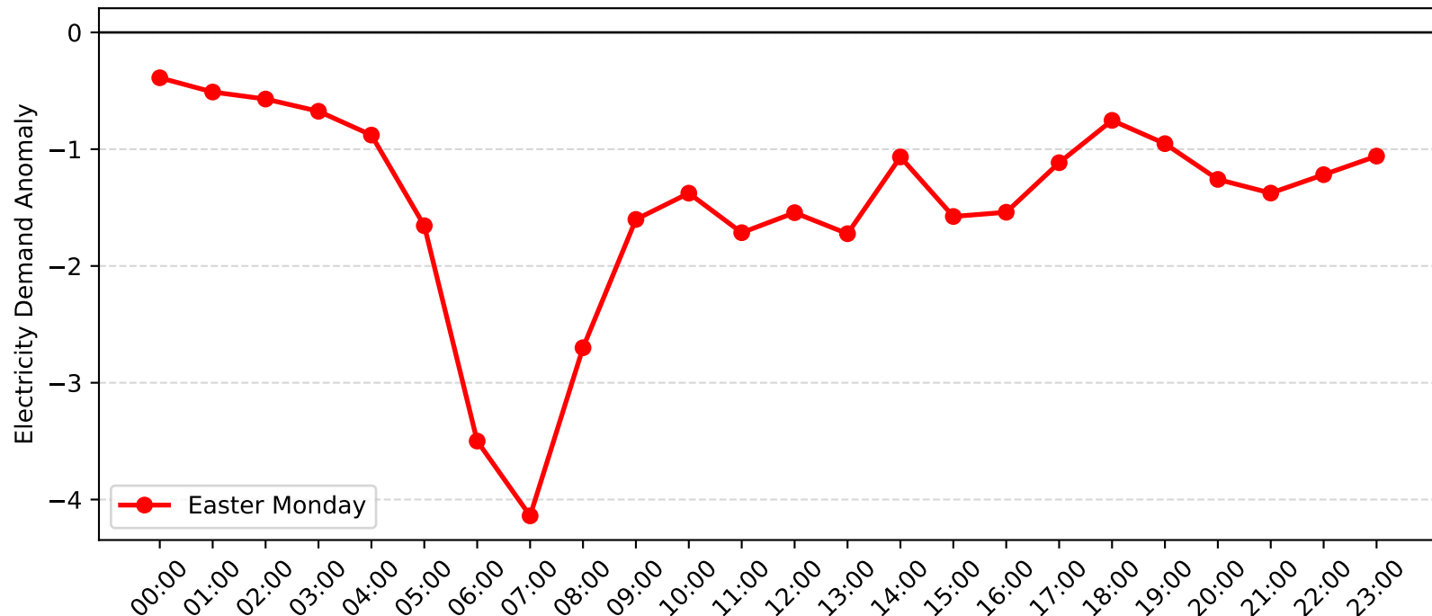
Mortdale Demand Anomaly: Easter Monday (2015-2016)
