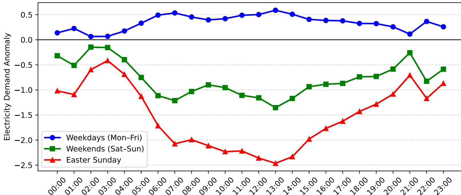
Gateshead Demand Anomaly: Easter Sunday vs Weekday/Weekend (2016-2017)
