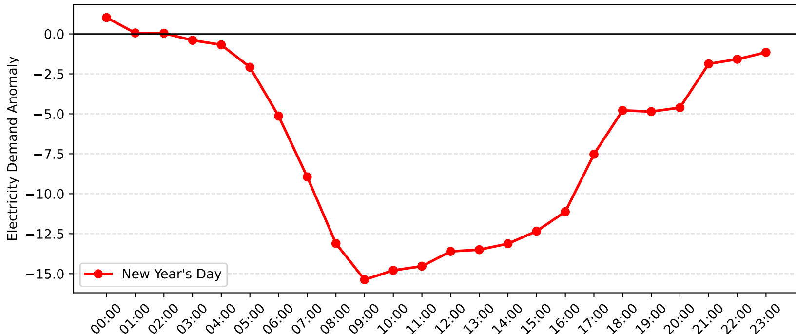
Brookvale Demand Anomaly: New Year's Day (2008-2009)
