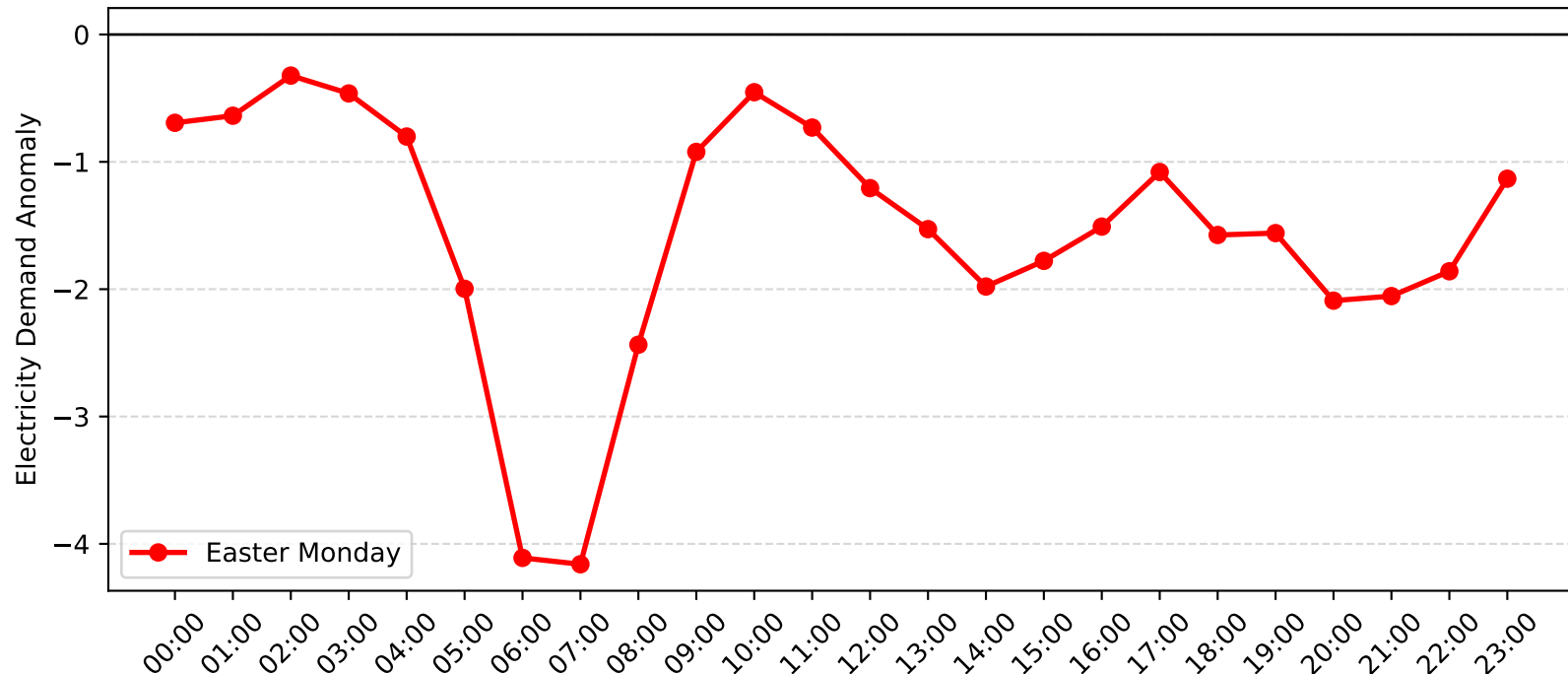
Cronulla Demand Anomaly: Easter Monday (2016-2017)
