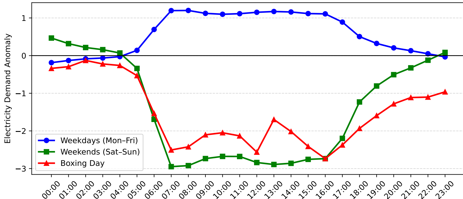
Pymble Demand Anomaly: Boxing Day vs Weekday/Weekend (2011-2012)
