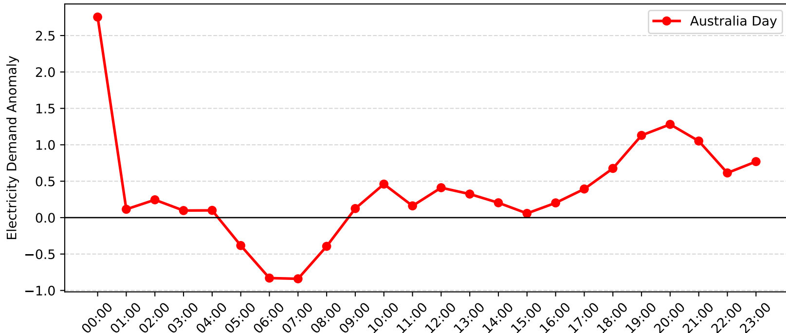
Woy Woy Demand Anomaly: Australia Day (2009-2010)
