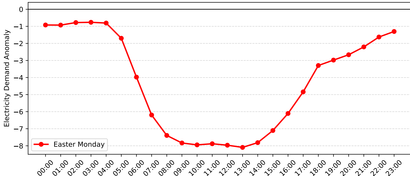
Mascot Demand Anomaly: Easter Monday (2011-2012)
