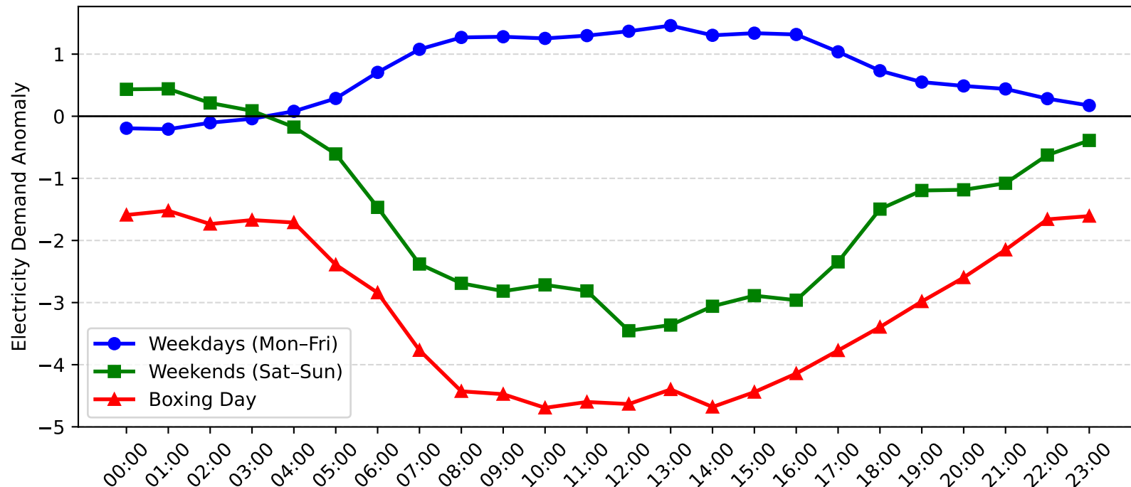
Lidcombe Demand Anomaly: Boxing Day vs Weekday/Weekend (2004-2005)
