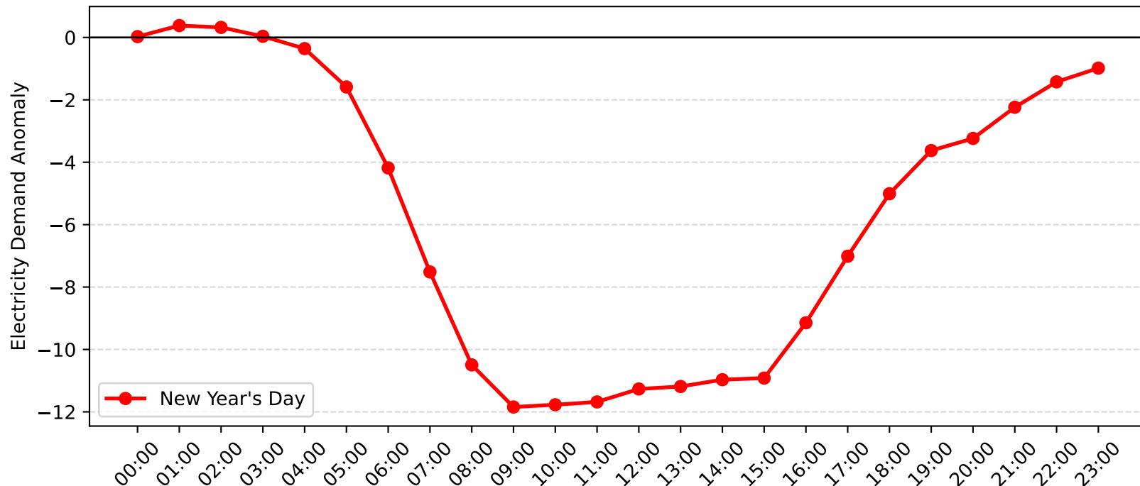
Brookvale Demand Anomaly: New Year's Day (2016-2017)
