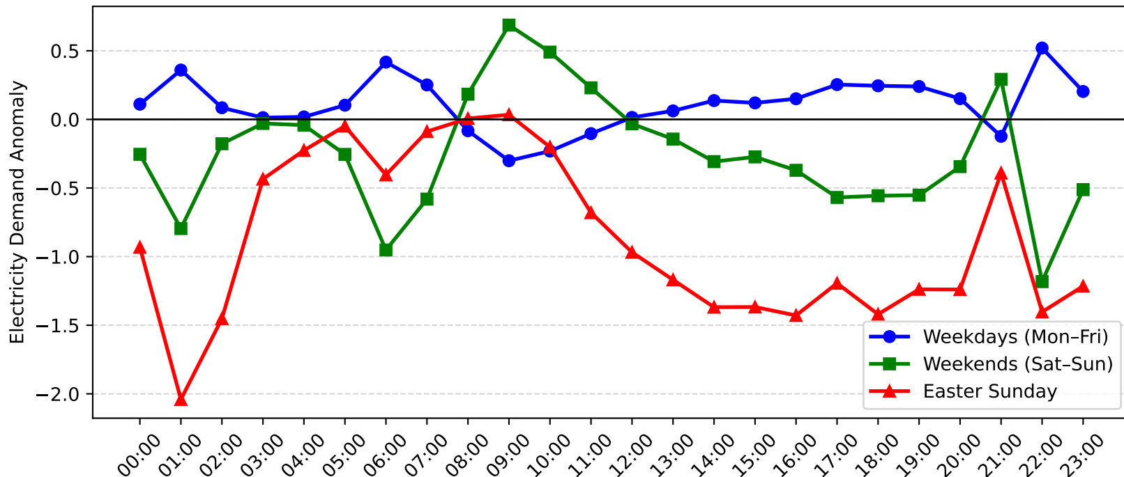
Jewells Demand Anomaly: Easter Sunday vs Weekday/Weekend (2005-2006)
