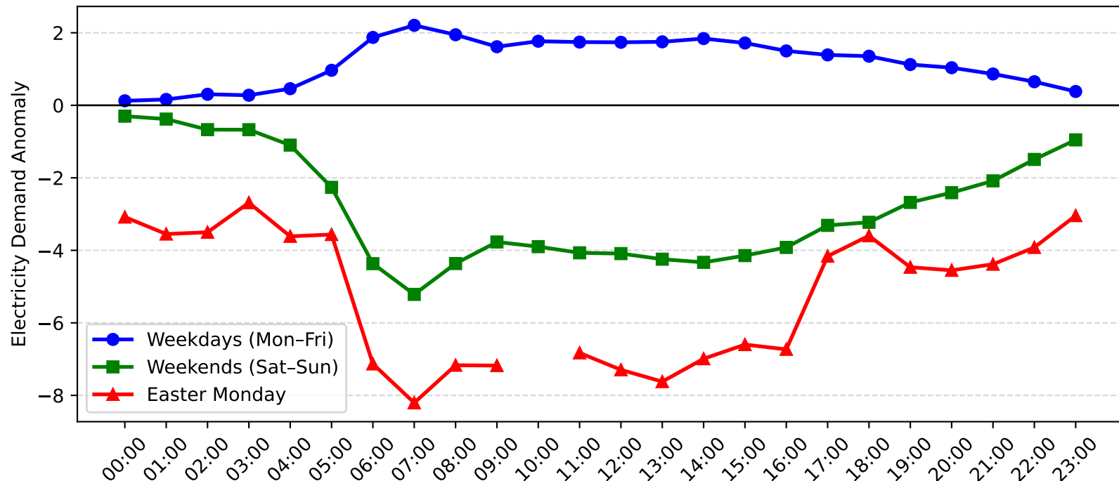
Matraverse Demand Anomaly: Easter Monday vs Weekday/Weekend (2005-2006)
