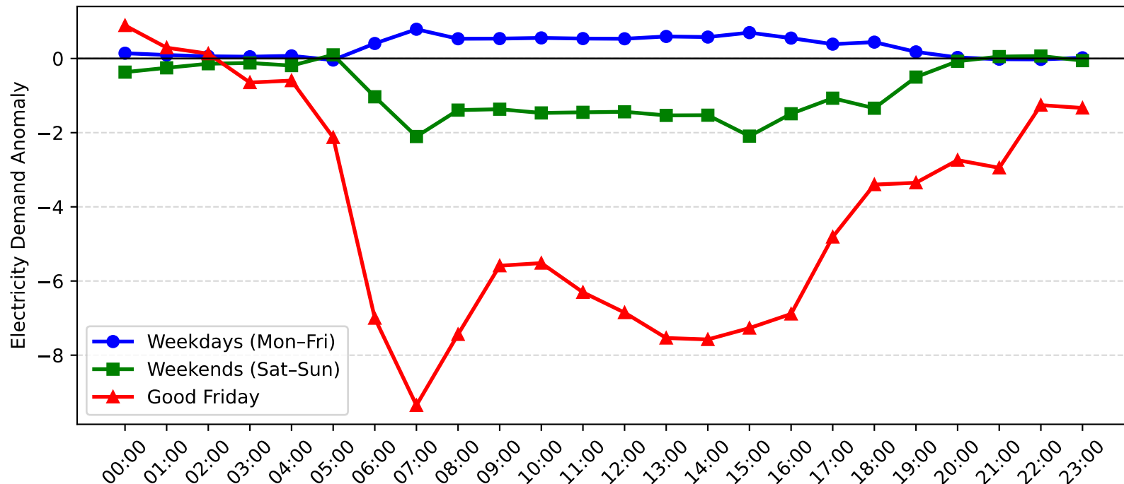
Chatswood Demand Anomaly: Good Friday vs Weekday/Weekend (2004-2005)
