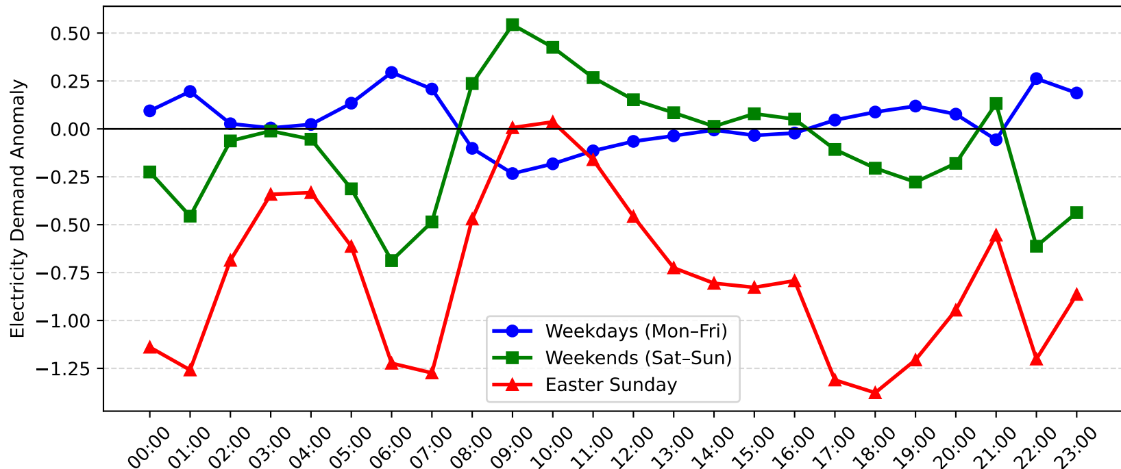
Jewells Demand Anomaly: Easter Sunday vs Weekday/Weekend (2013-2014)
