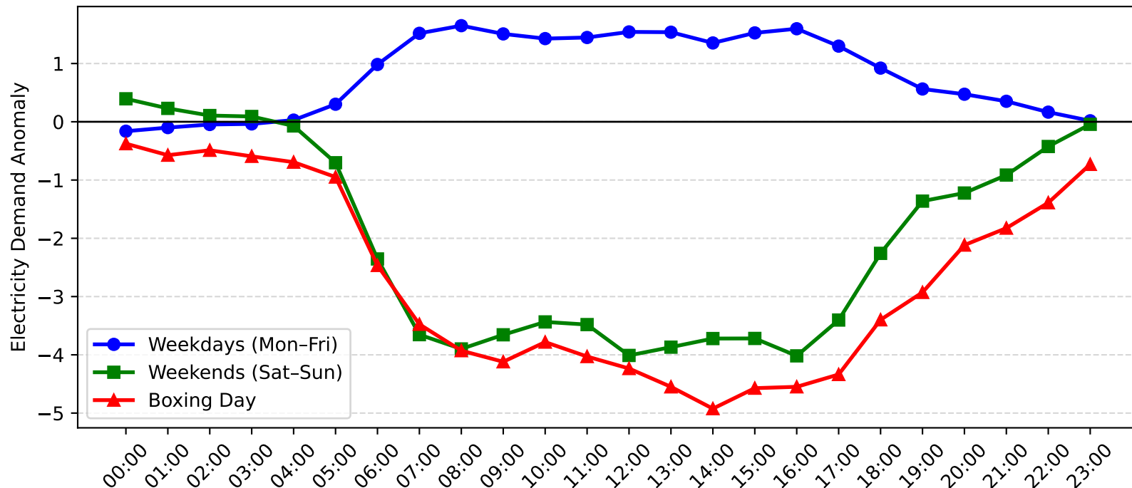
Pymble Demand Anomaly: Boxing Day vs Weekday/Weekend (2005-2006)
