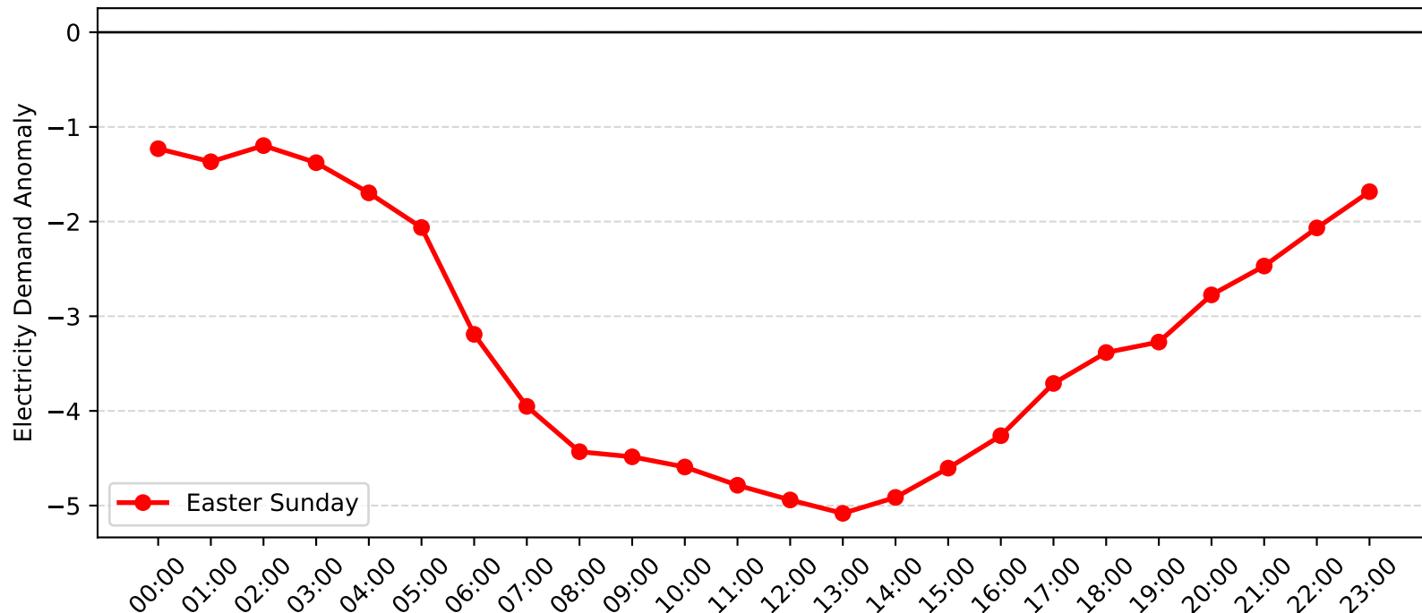
Caringbah Demand Anomaly: Easter Sunday (2017-2018)
