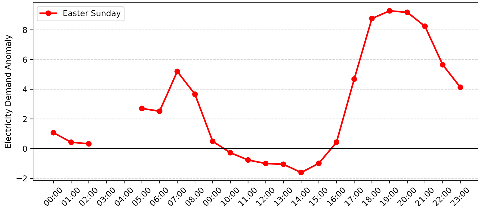
Dulwich Hill Demand Anomaly: Easter Sunday (2004-2005)
