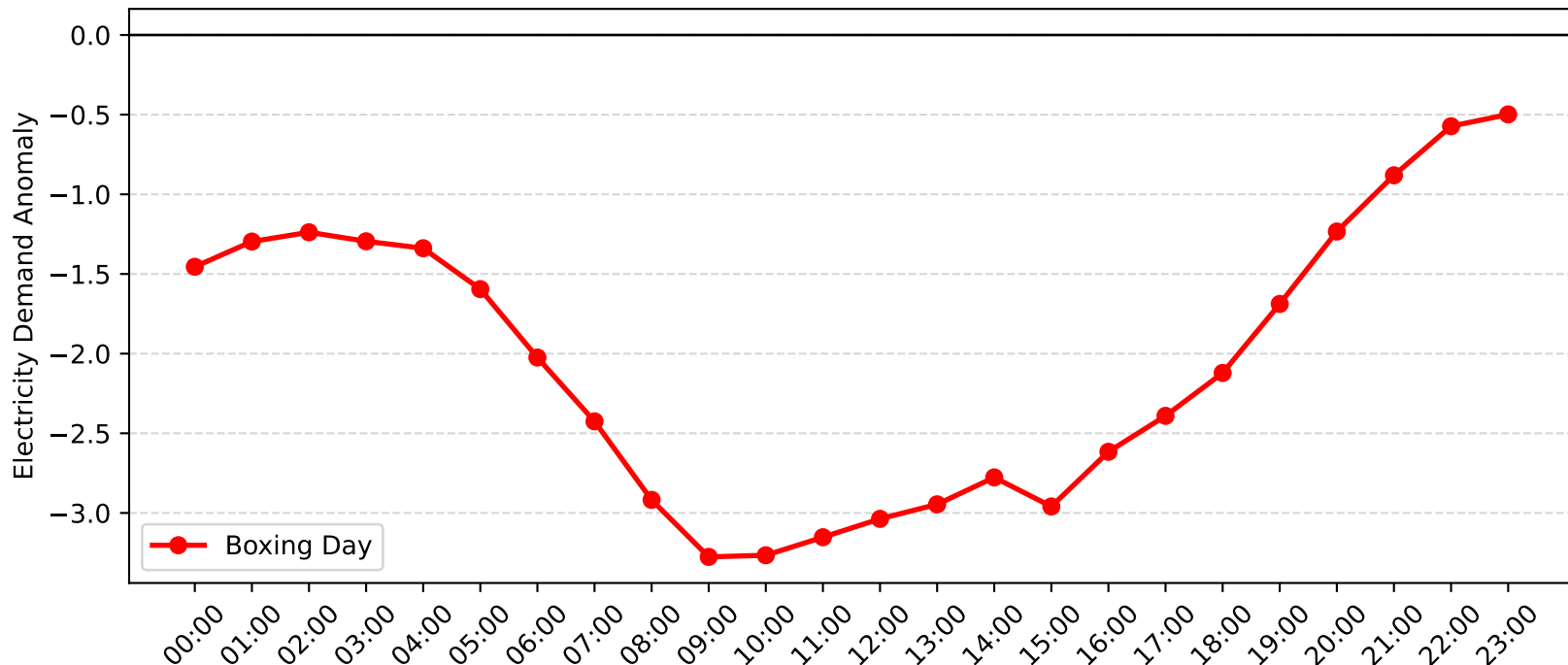
Lidcombe Demand Anomaly: Boxing Day (2014-2015)
