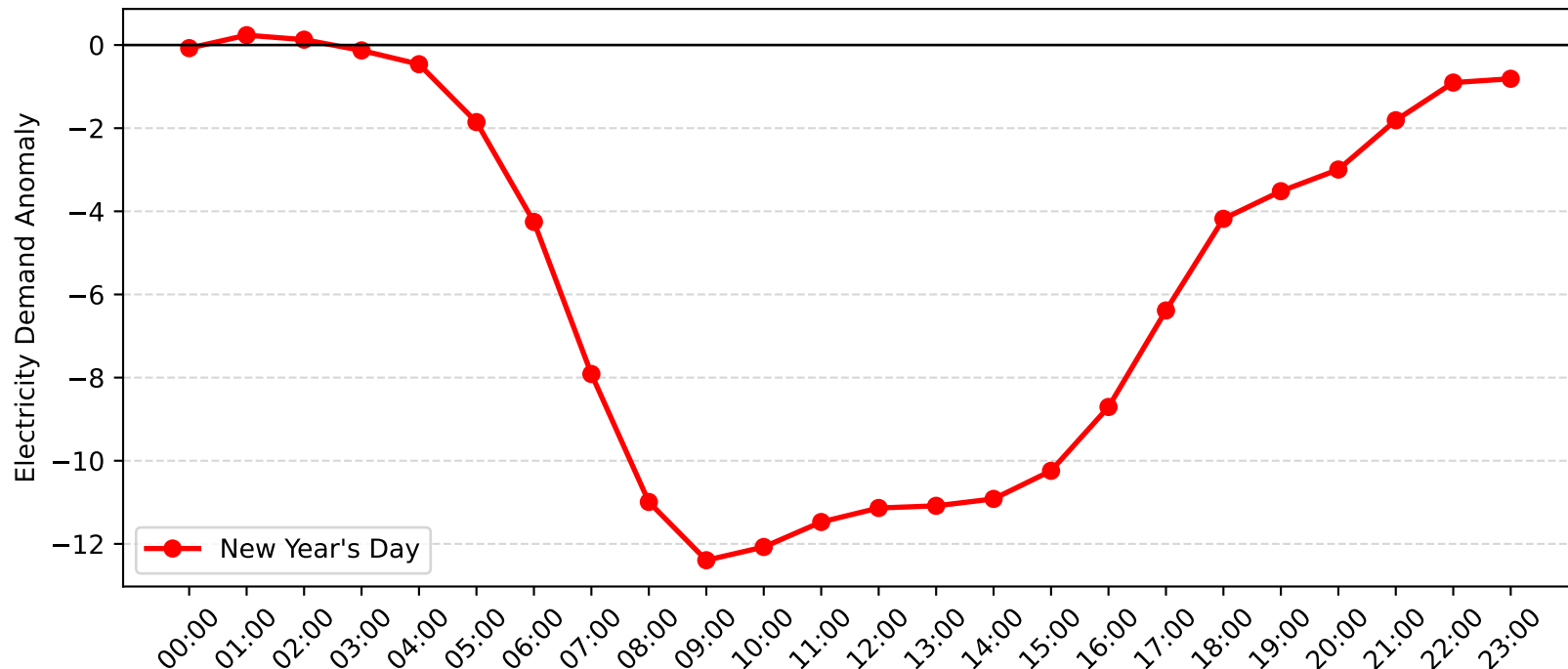
Brookvale Demand Anomaly: New Year's Day (2010-2011)
