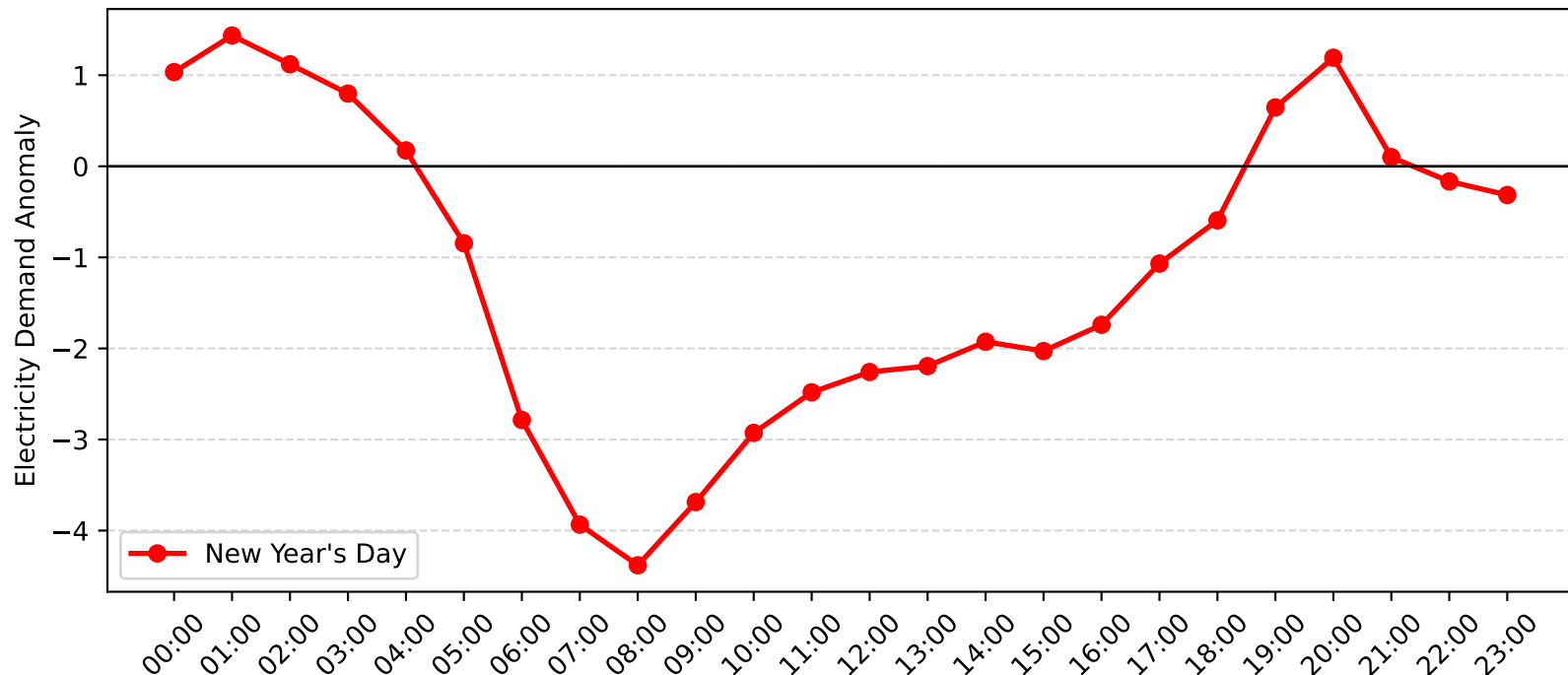
Five Dock Demand Anomaly: New Year's Day (2008-2009)
