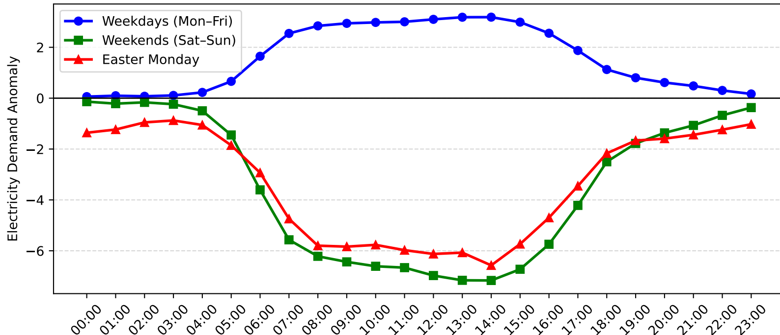
Mascot Demand Anomaly: Easter Monday vs Weekday/Weekend (2016-2017)
