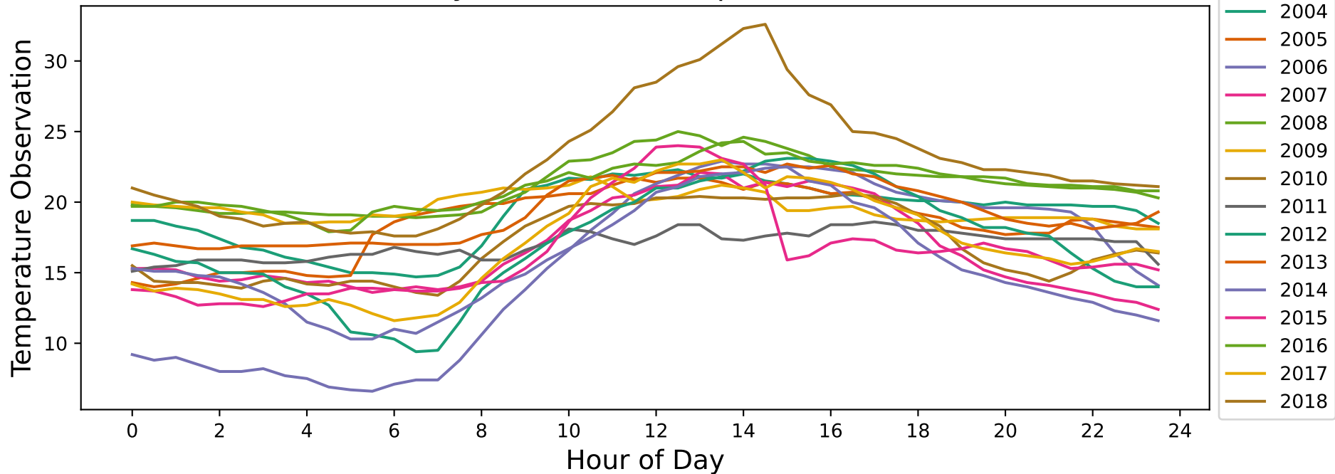
Easter Monday – Minimum Temperature (2004-2018)
