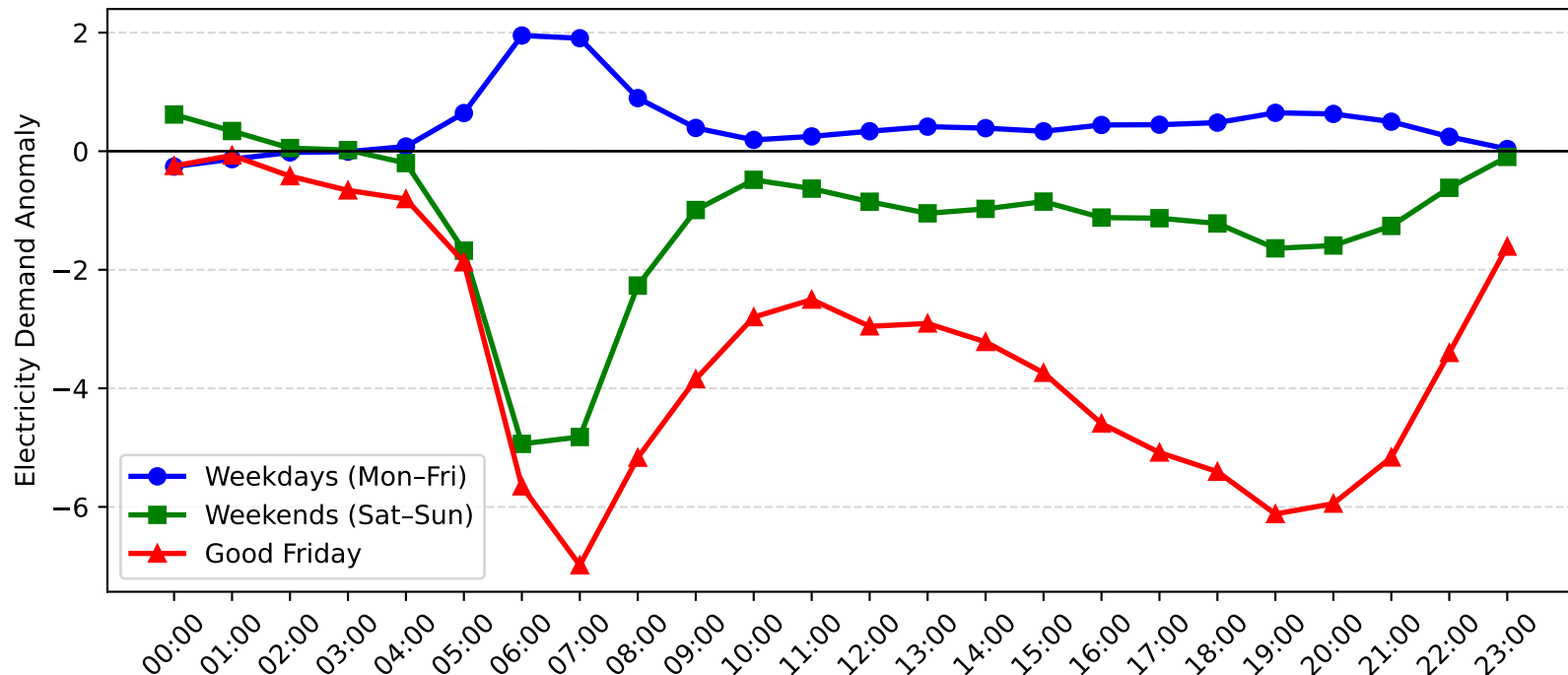
Pennant Hills Demand Anomaly: Good Friday vs Weekday/Weekend (2014-2015)
