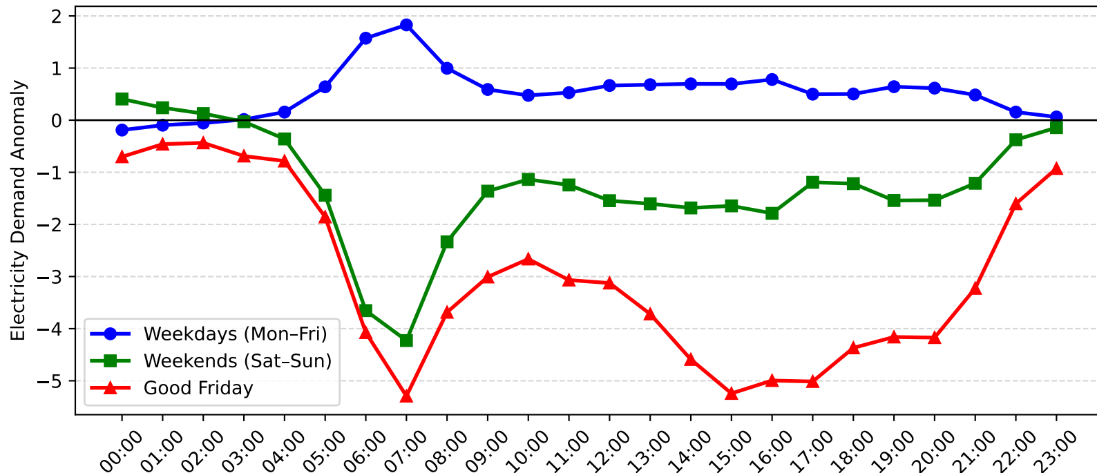
Dulwich Hill Demand Anomaly: Good Friday vs Weekday/Weekend (2009-2010)
