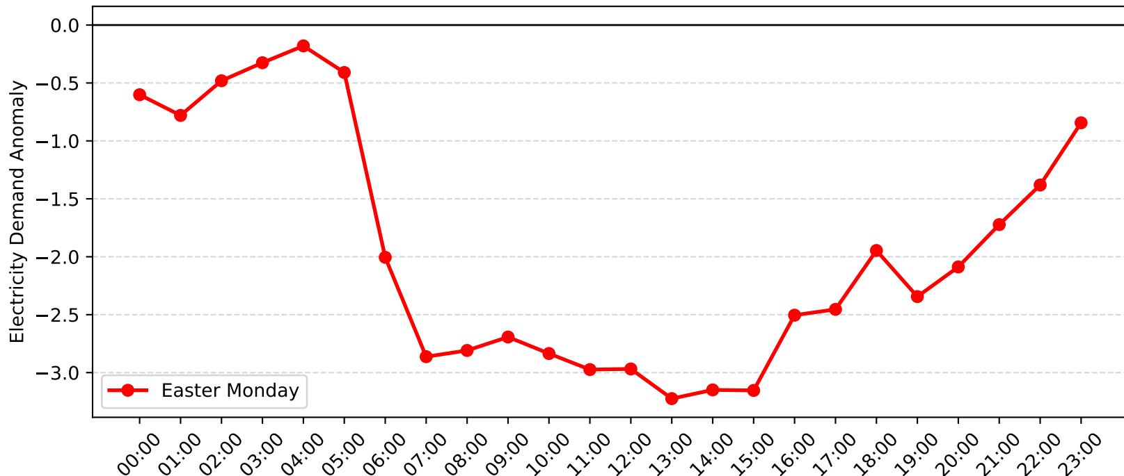
Pymble Demand Anomaly: Easter Monday (2009-2010)
