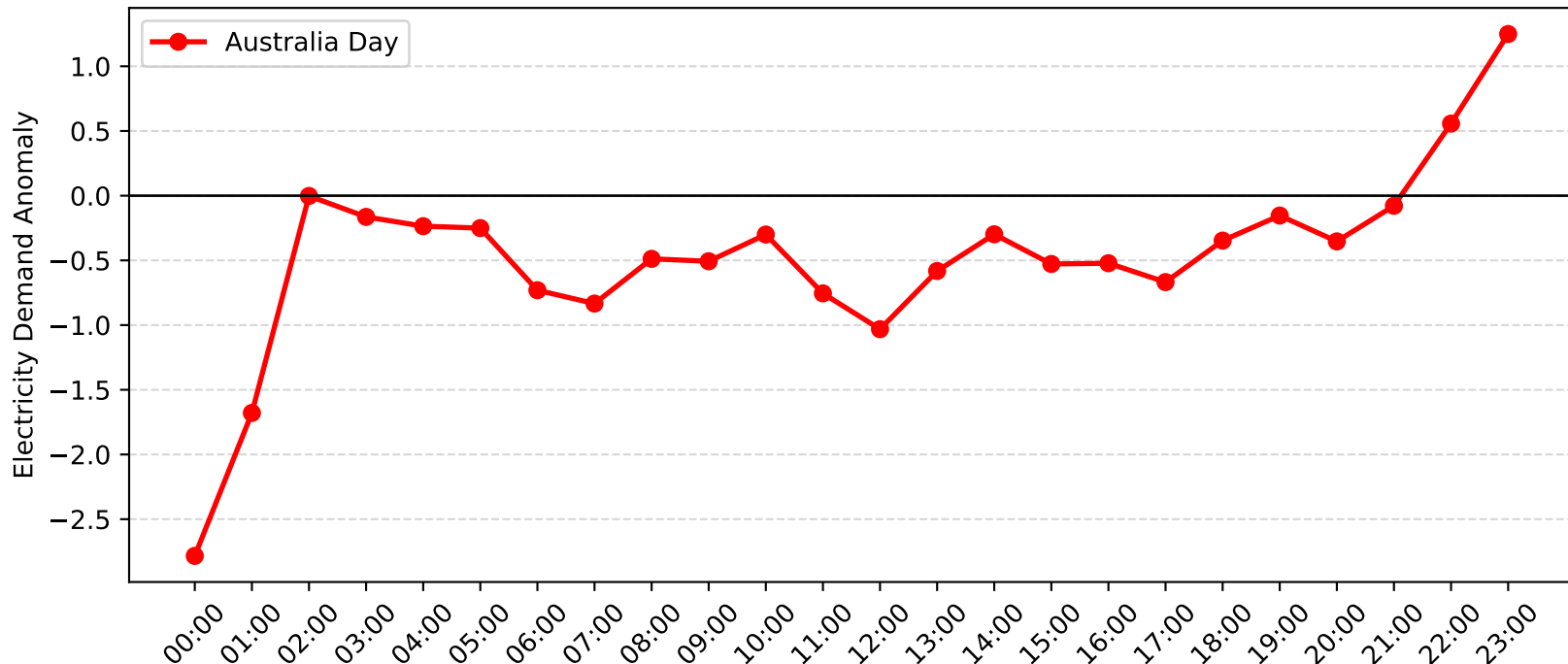
Woy Woy Demand Anomaly: Australia Day (2006-2007)
