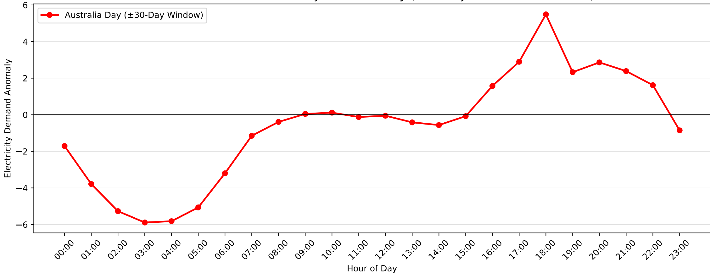
Blakehurst Demand Anomaly: Australia Day ( \pm 30 -Day Window, 2004–2005)
