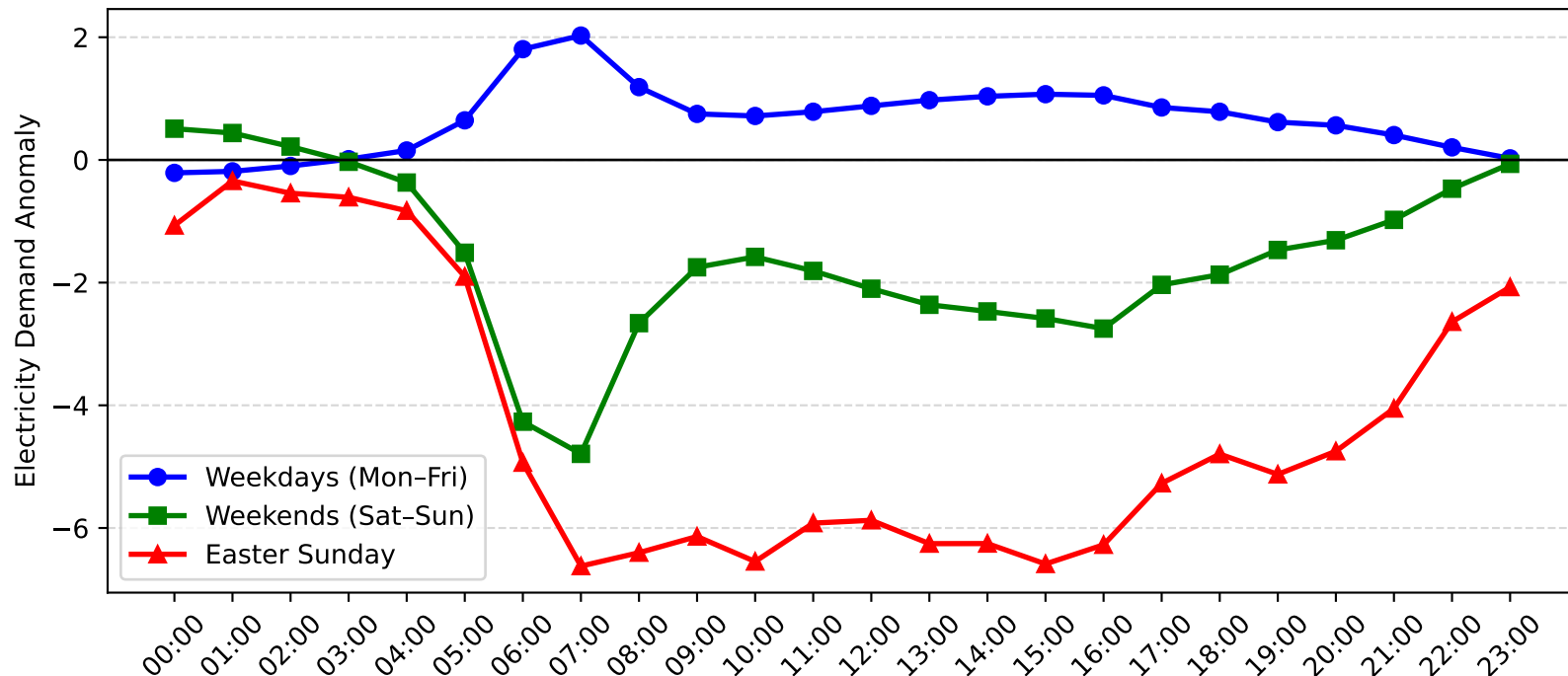
Dulwich Hill Demand Anomaly: Easter Sunday vs Weekday/Weekend (2005-2006)
