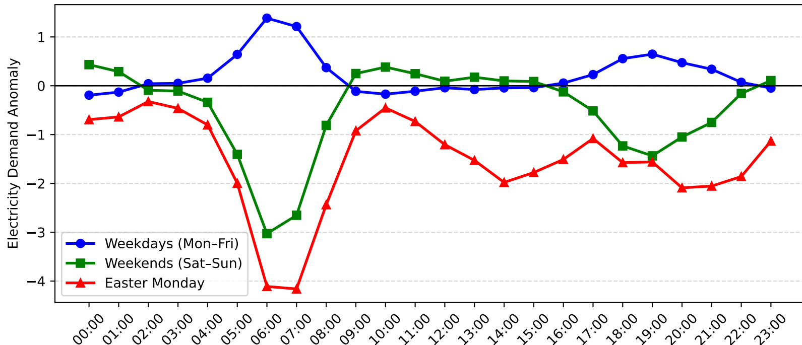
Cronulla Demand Anomaly: Easter Monday vs Weekday/Weekend (2016-2017)
