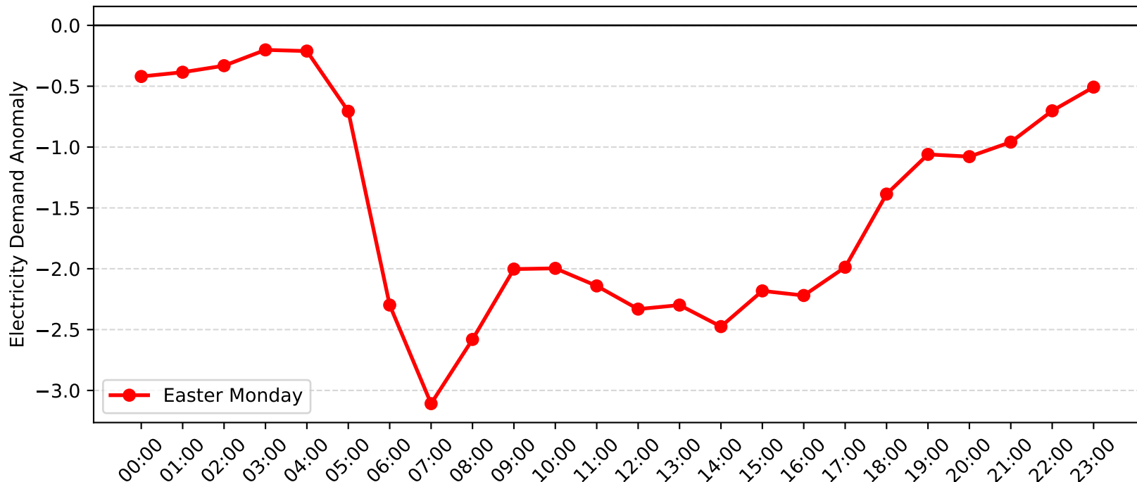
Pymble Demand Anomaly: Easter Monday (2013-2014)
