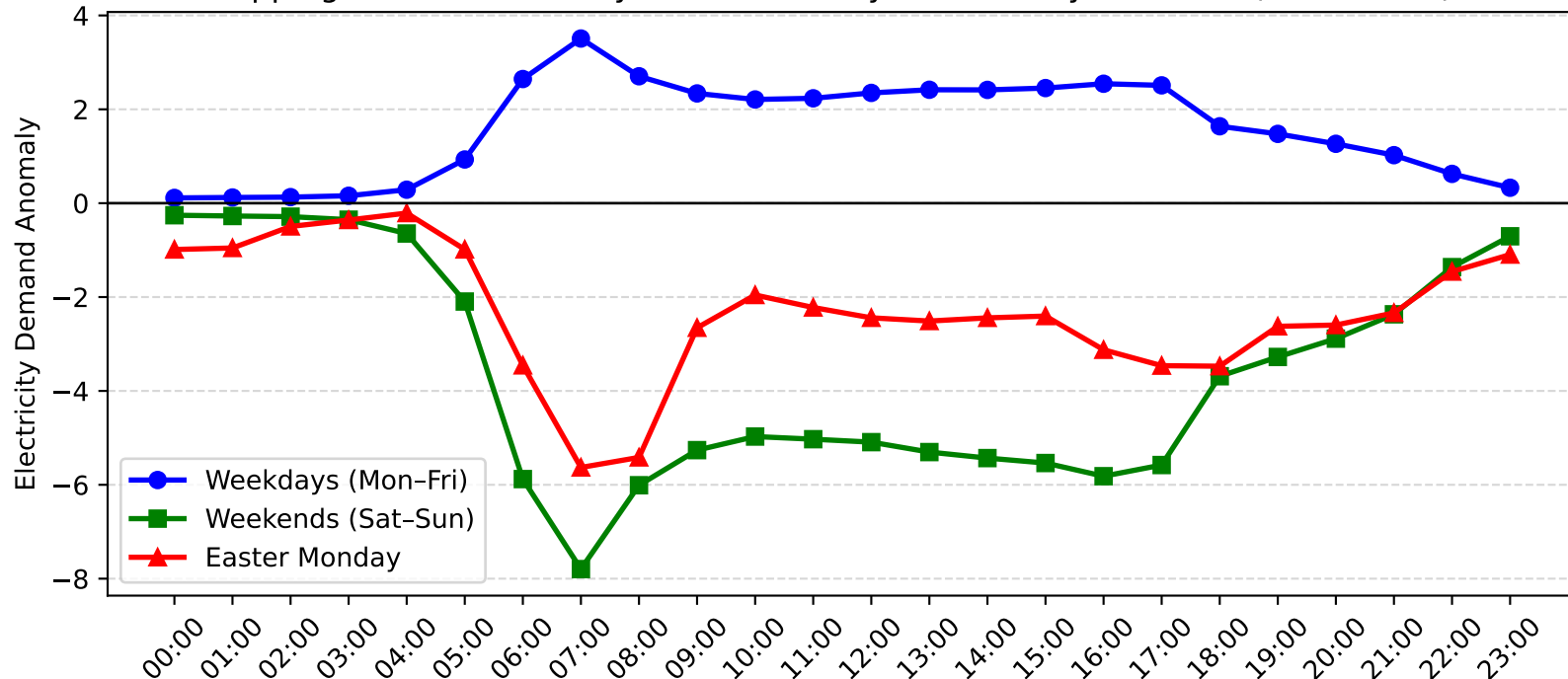
Epping Demand Anomaly: Easter Monday vs Weekday/Weekend (2008-2009)
