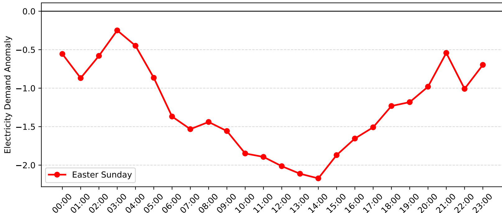
Gateshead Demand Anomaly: Easter Sunday (2015-2016)
