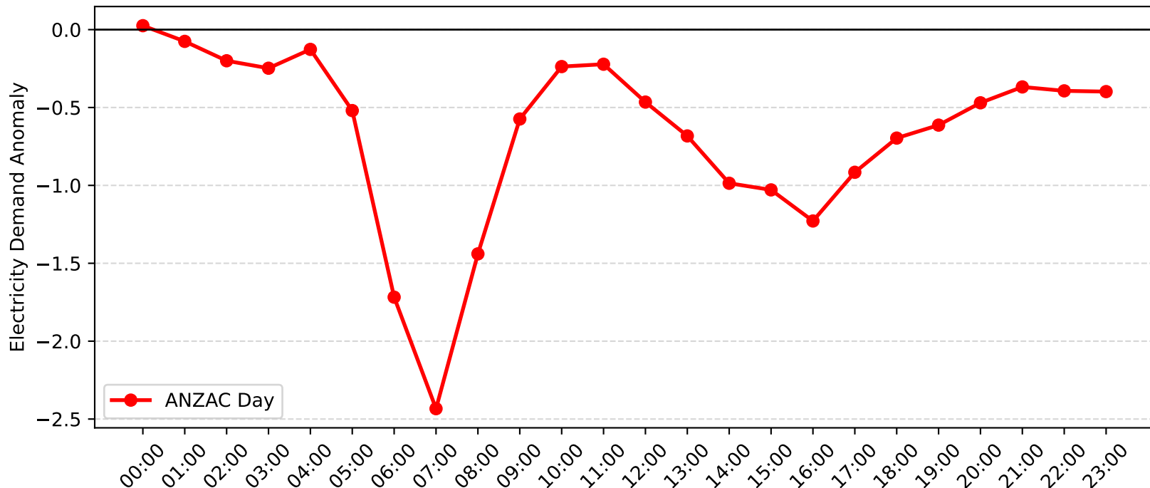
Blakehurst Demand Anomaly: ANZAC Day (2012-2013)
