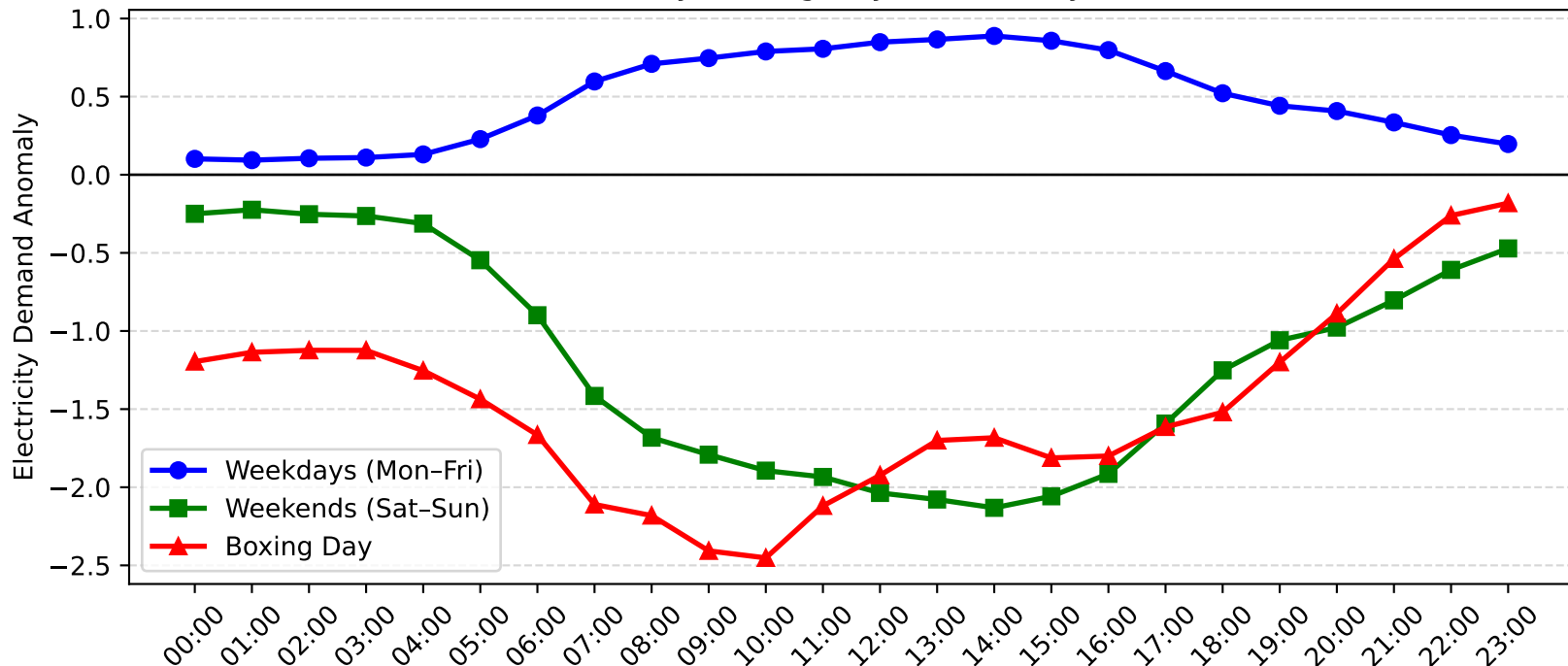
Lidcombe Demand Anomaly: Boxing Day vs Weekday/Weekend (2015-2016)
