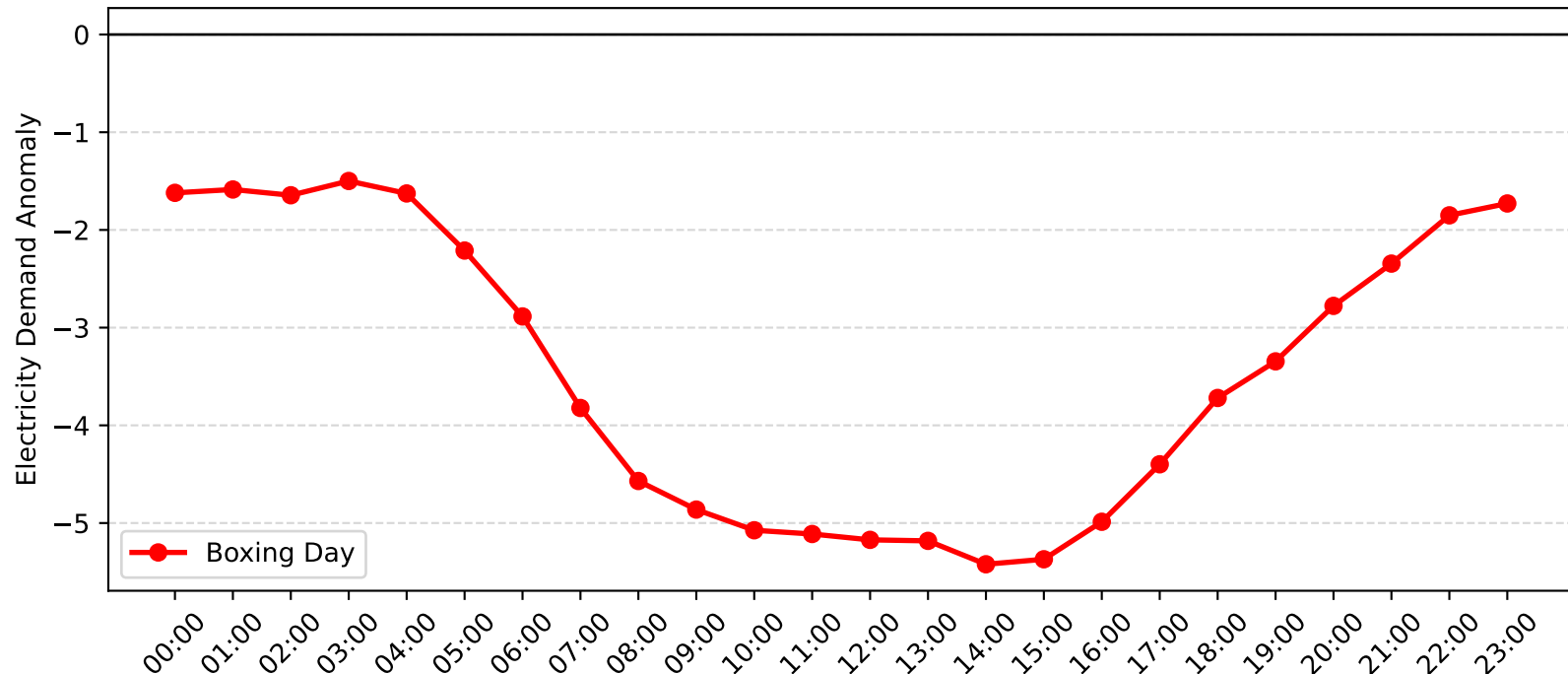
Lidcombe Demand Anomaly: Boxing Day (2005-2006)
