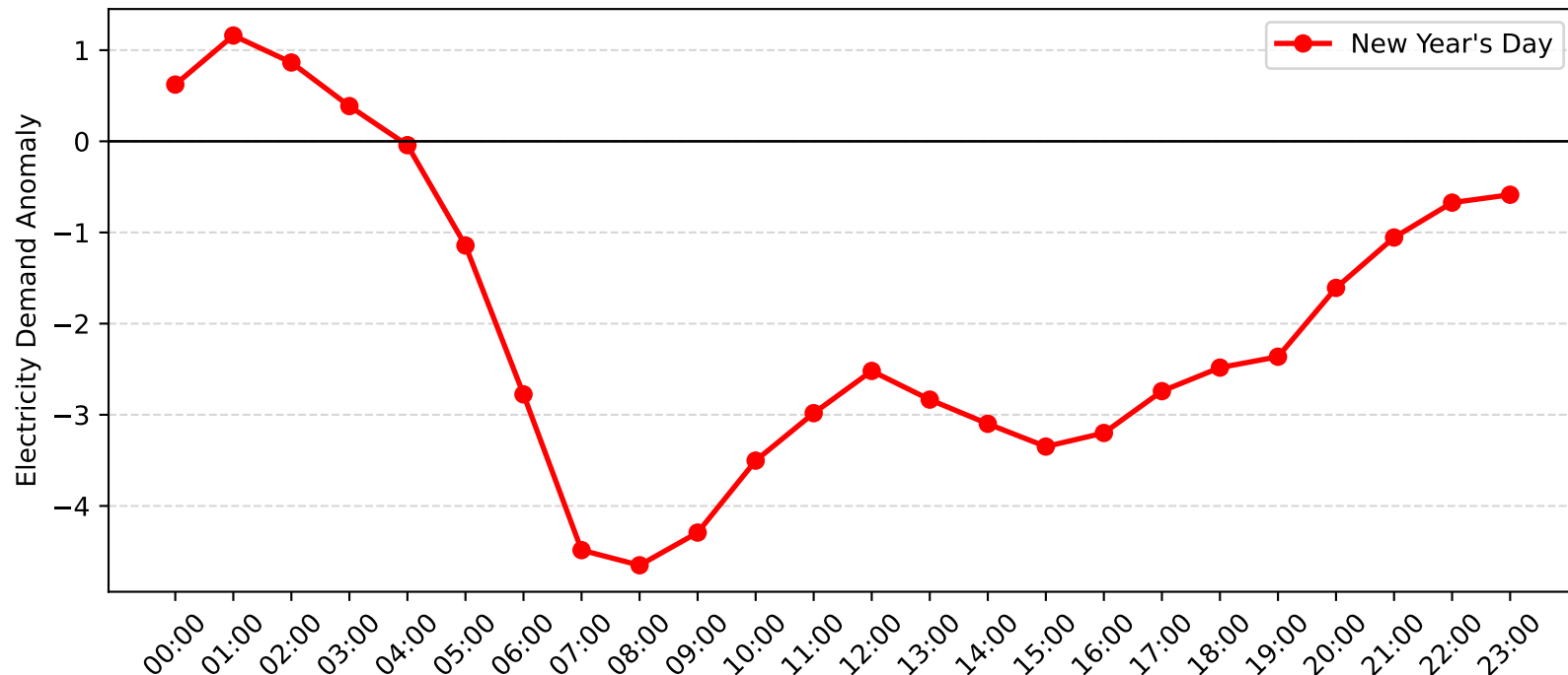
Five Dock Demand Anomaly: New Year's Day (2012-2013)
