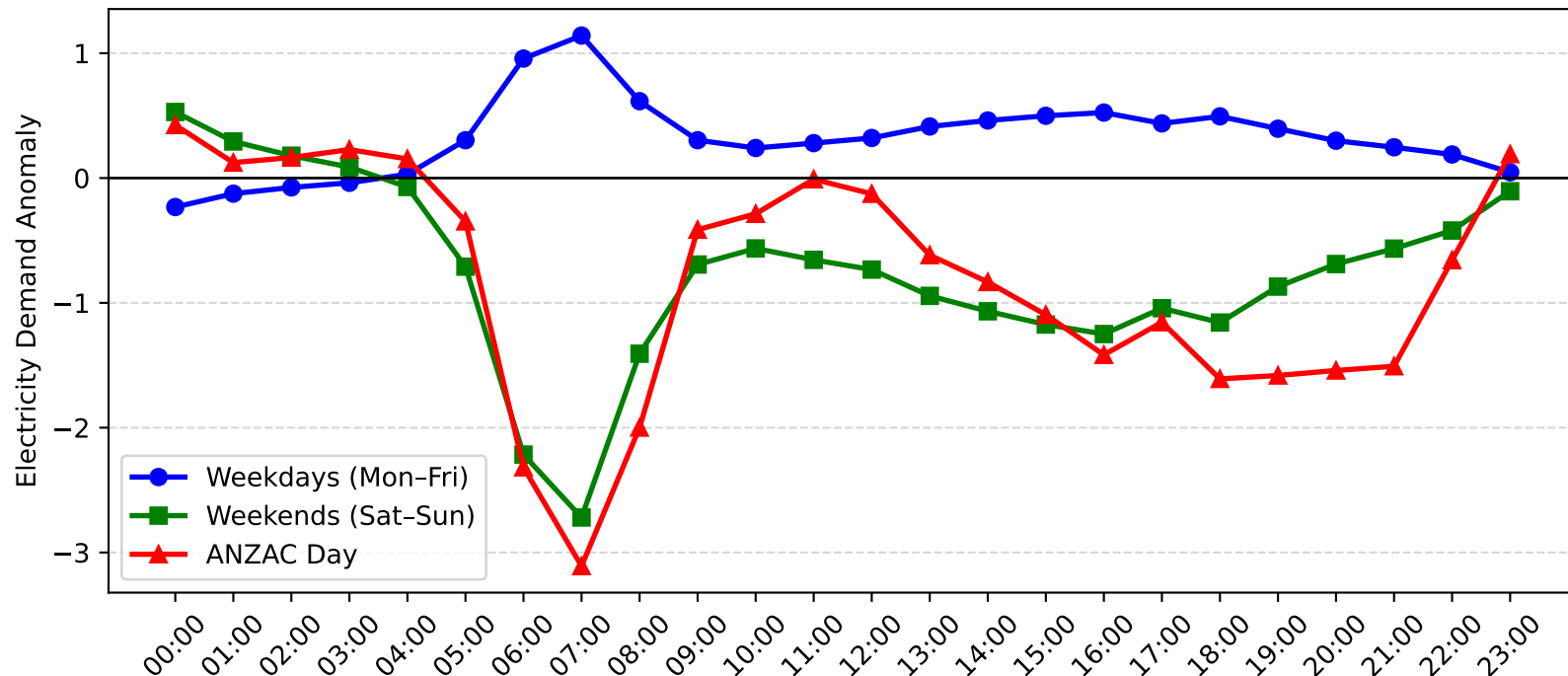
Blakehurst Demand Anomaly: ANZAC Day vs Weekday/Weekend (2008-2009)
