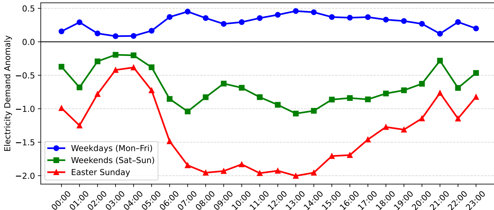
Gateshead Demand Anomaly: Easter Sunday vs Weekday/Weekend (2011-2012)
