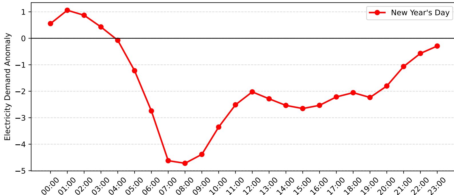
Five Dock Demand Anomaly: New Year's Day (2011-2012)
