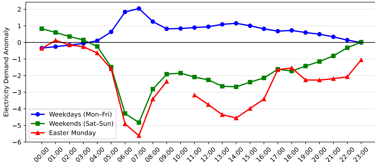
Mortdale Demand Anomaly: Easter Monday vs Weekday/Weekend (2005-2006)
