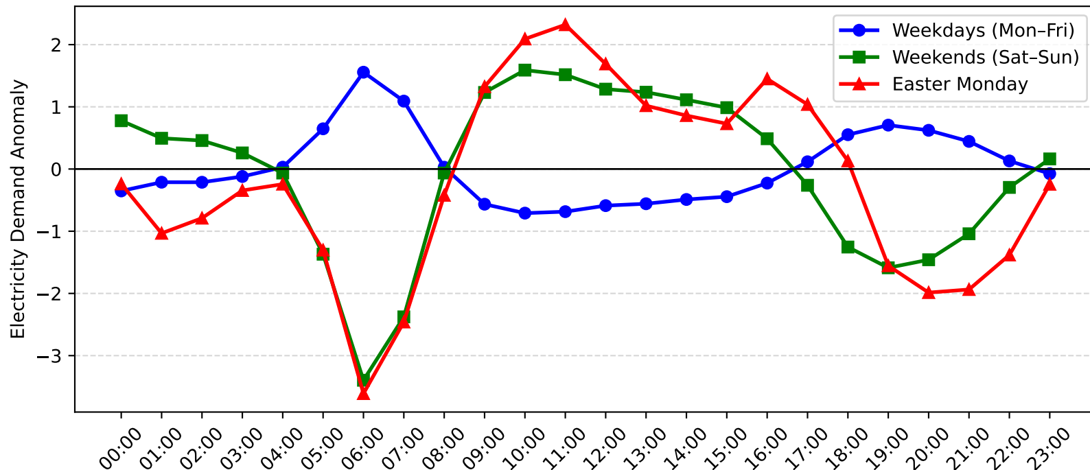
Cronulla Demand Anomaly: Easter Monday vs Weekday/Weekend (2009-2010)
