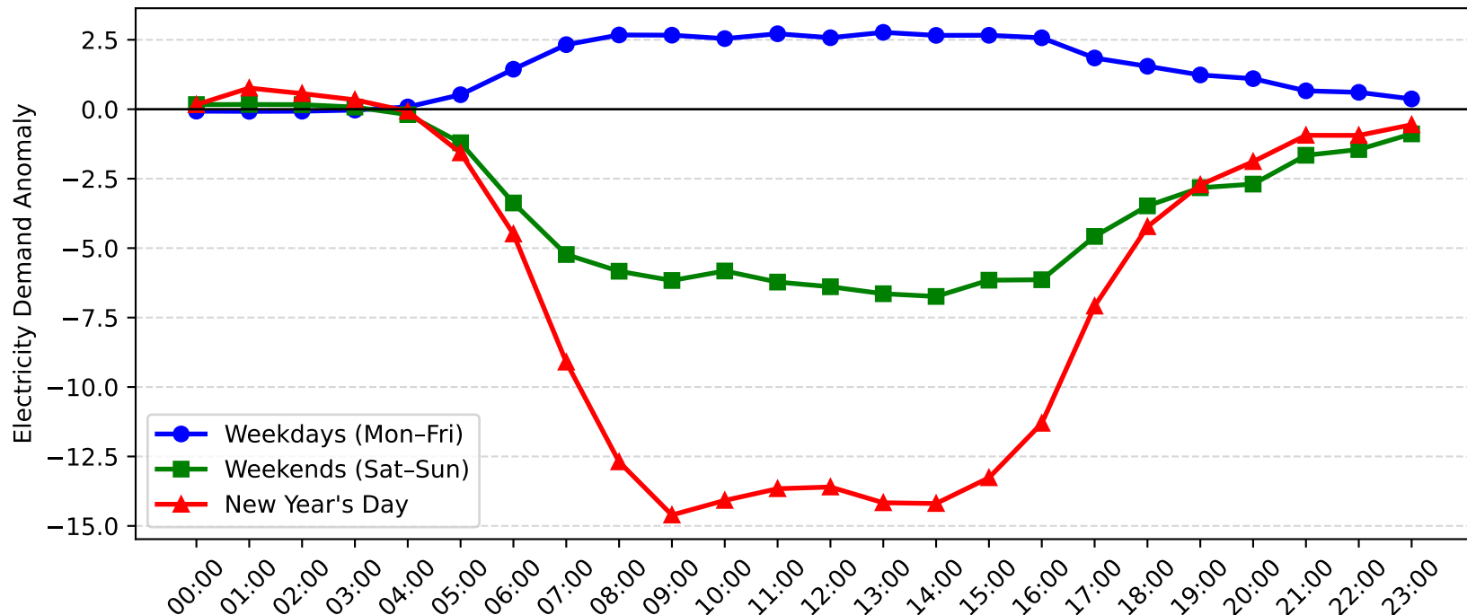
Brookvale Demand Anomaly: New Year's Day vs Weekday/Weekend (2006-2007)
