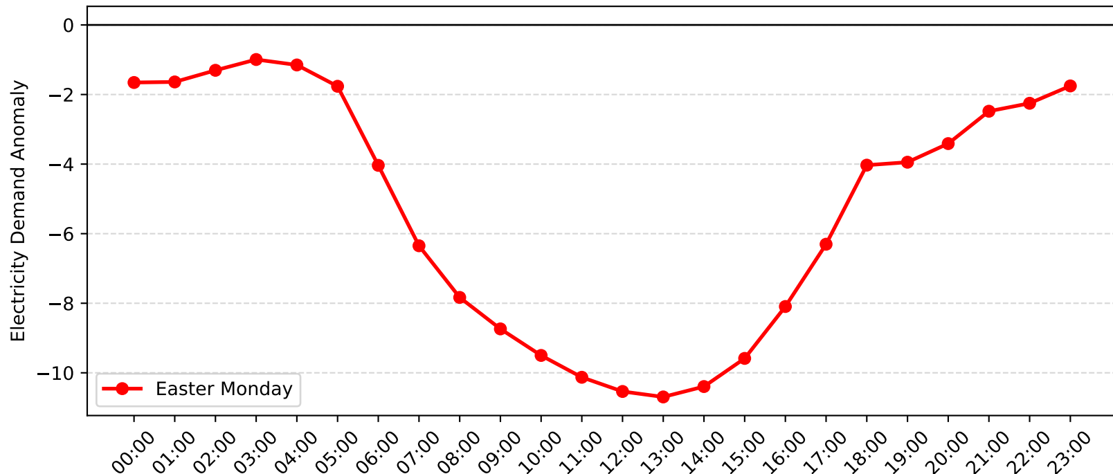
Mascot Demand Anomaly: Easter Monday (2009-2010)
