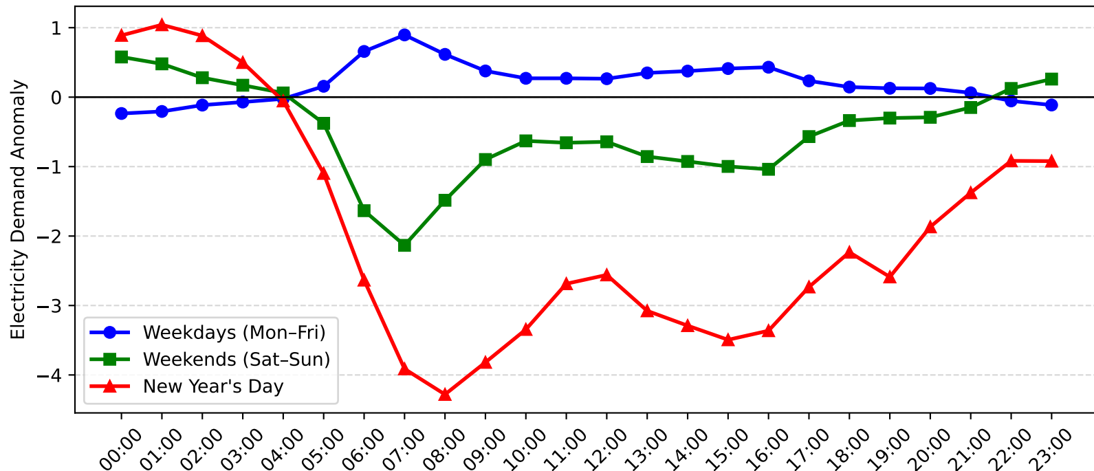
Five Dock Demand Anomaly: New Year's Day vs Weekday/Weekend (2007-2008)
