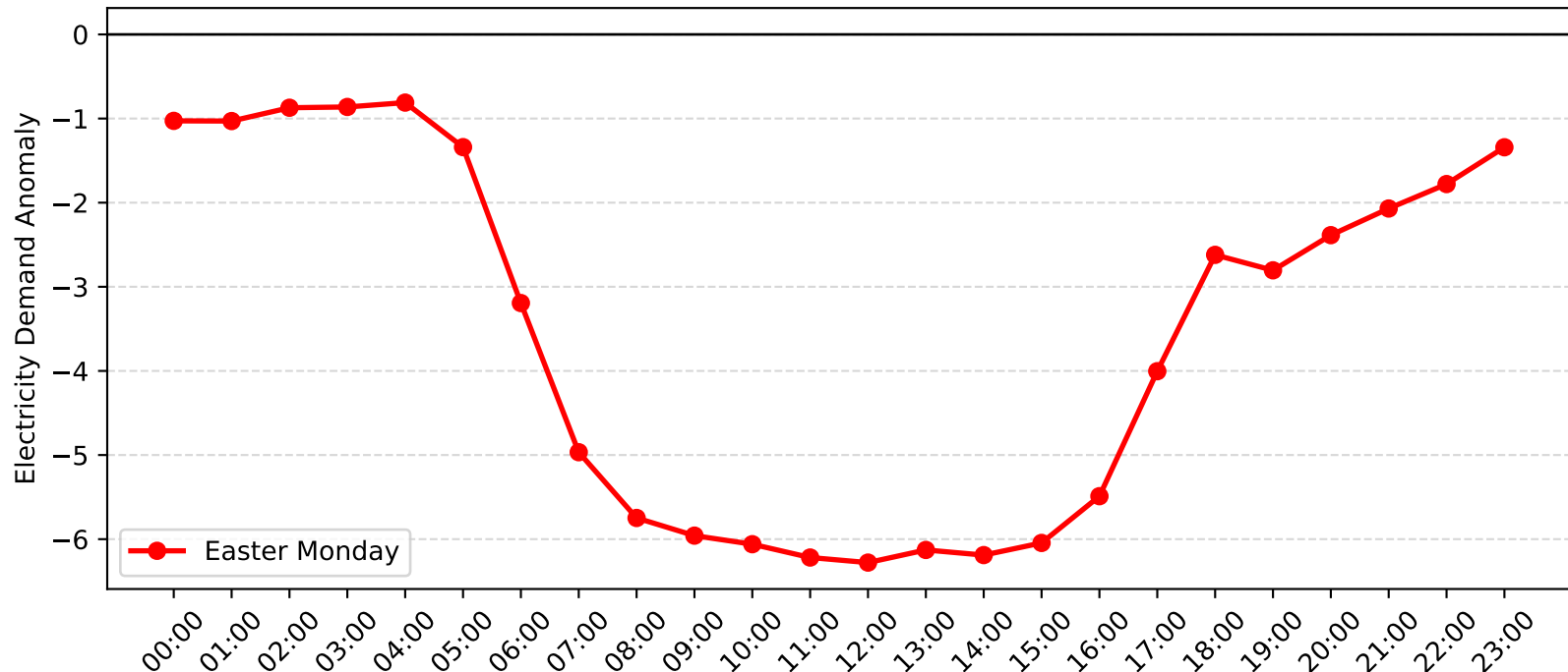
Mascot Demand Anomaly: Easter Monday (2014-2015)
