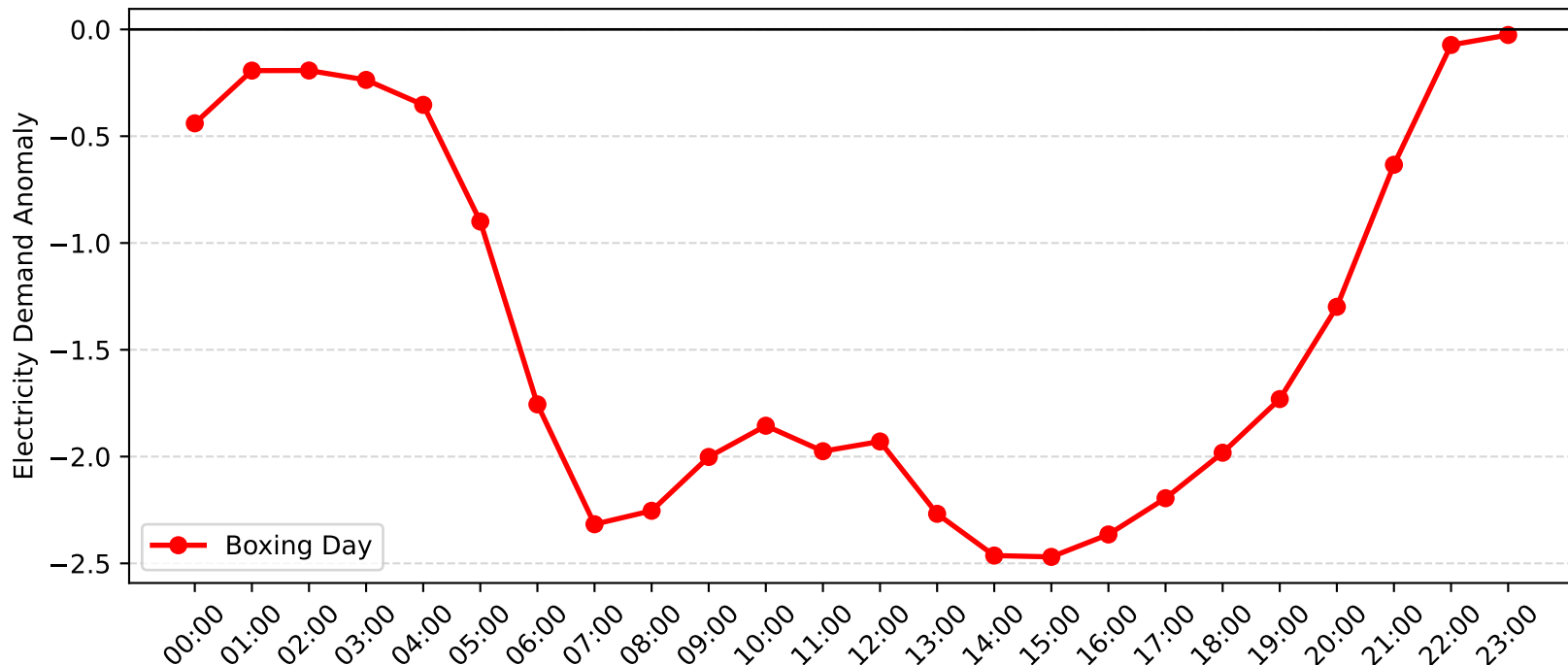
Narrabeen Demand Anomaly: Boxing Day (2005-2006)
