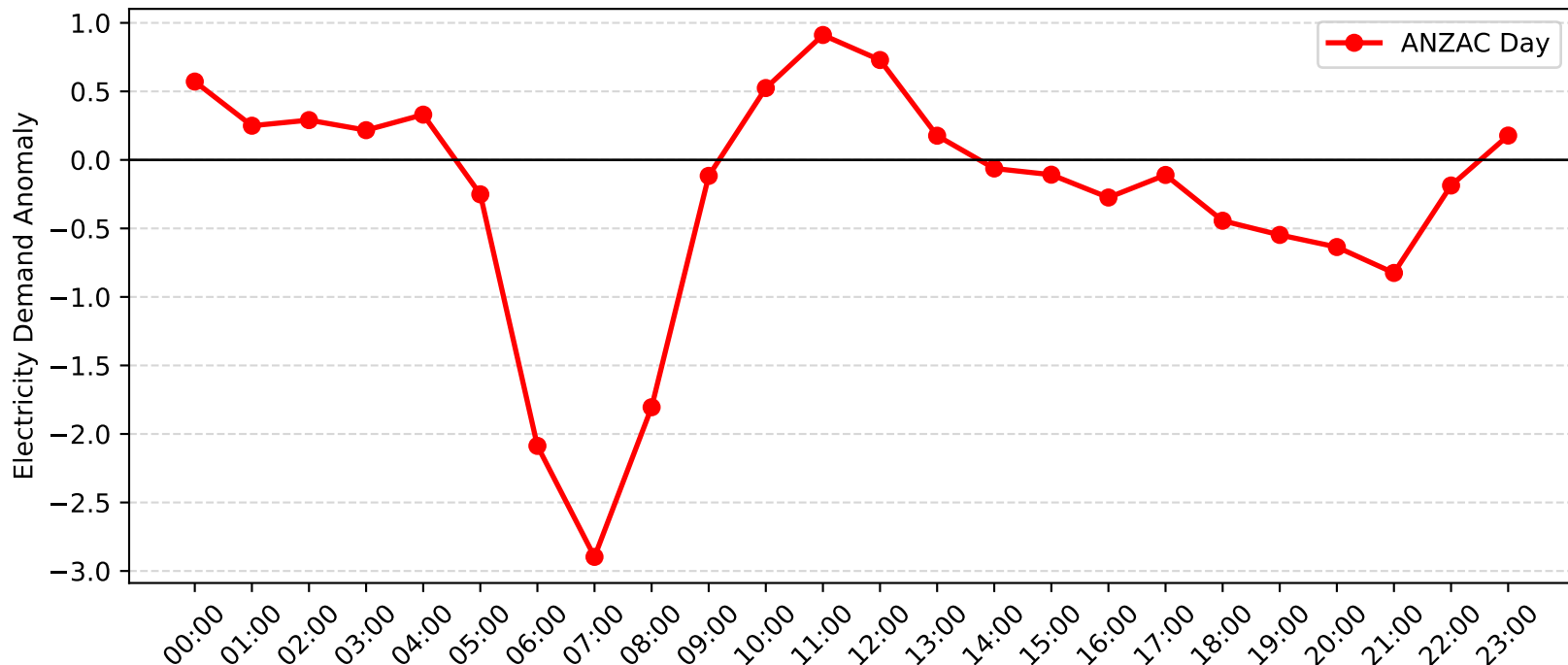
Blakehurst Demand Anomaly: ANZAC Day (2007-2008)
