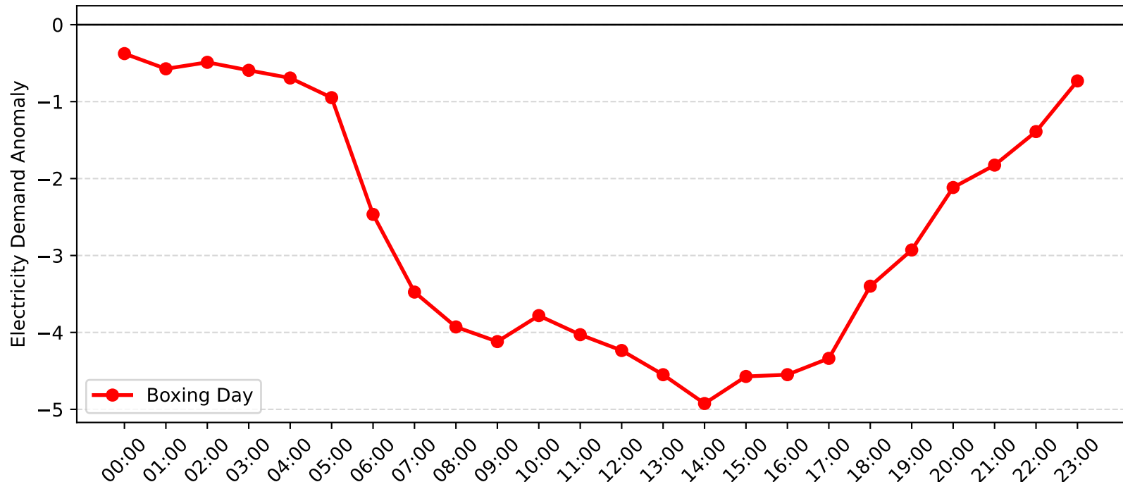
Pymble Demand Anomaly: Boxing Day (2005-2006)
