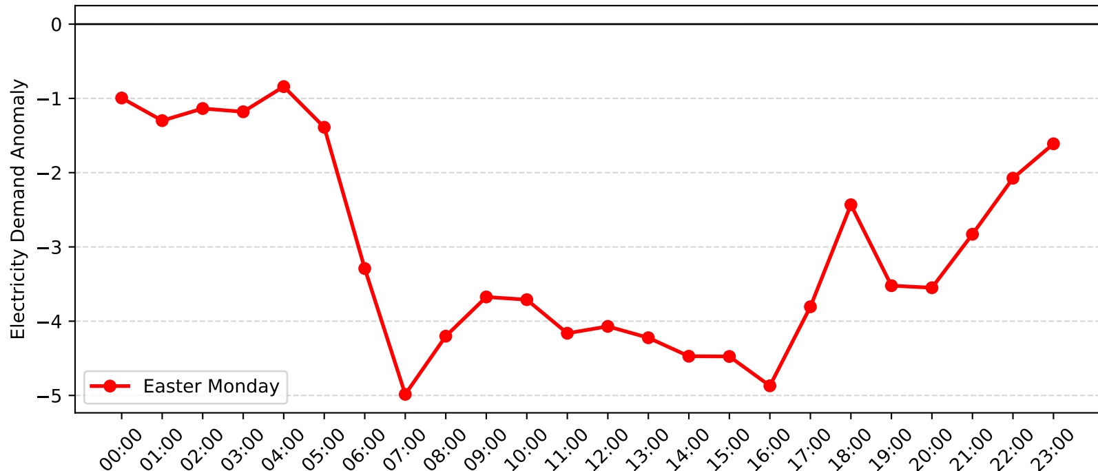
Epping Demand Anomaly: Easter Monday (2014-2015)
