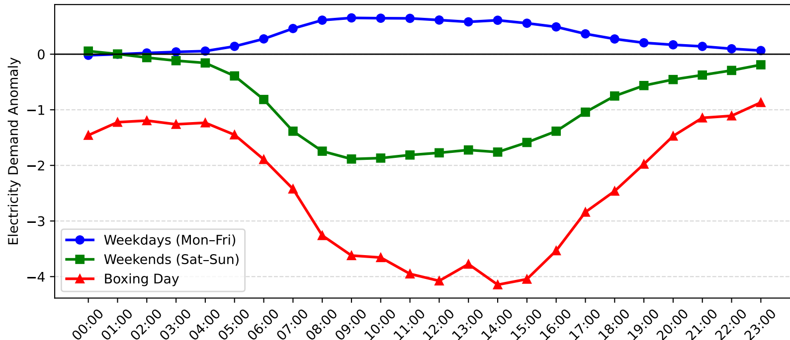
Lidcombe Demand Anomaly: Boxing Day vs Weekday/Weekend (2013-2014)
