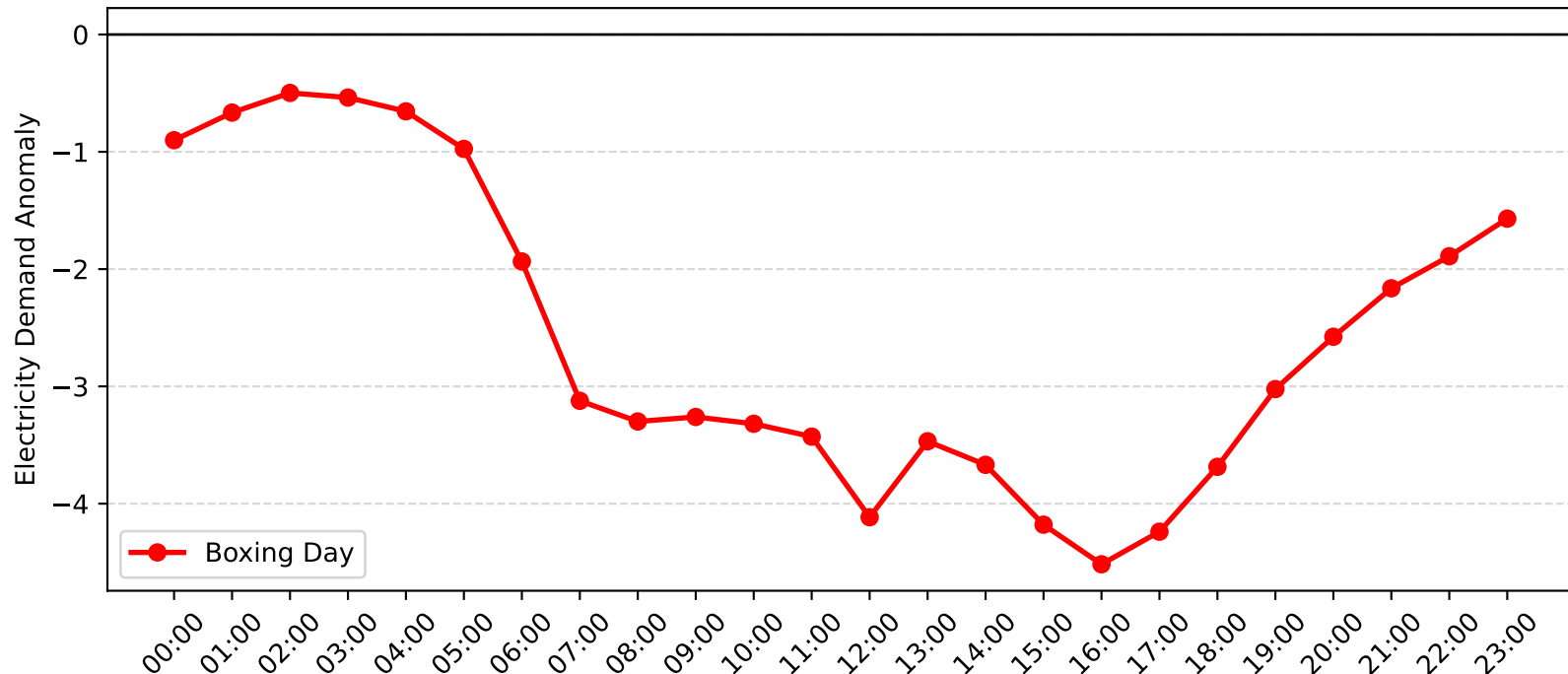
Pymble Demand Anomaly: Boxing Day (2012-2013)
