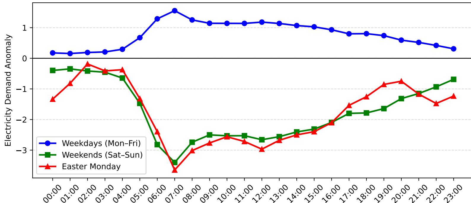
Matraverse Demand Anomaly: Easter Monday vs Weekday/Weekend (2016-2017)
