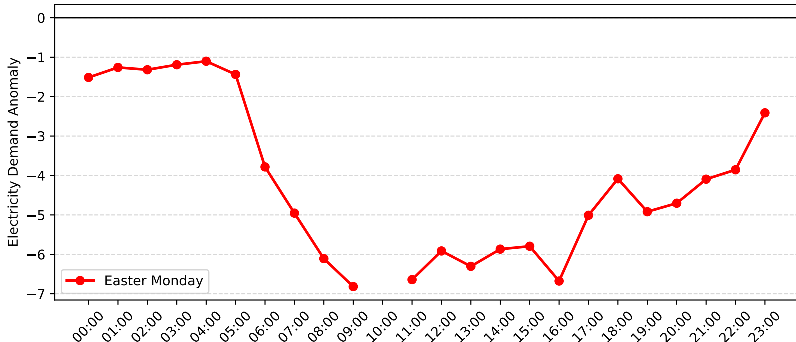
Epping Demand Anomaly: Easter Monday (2005-2006)
