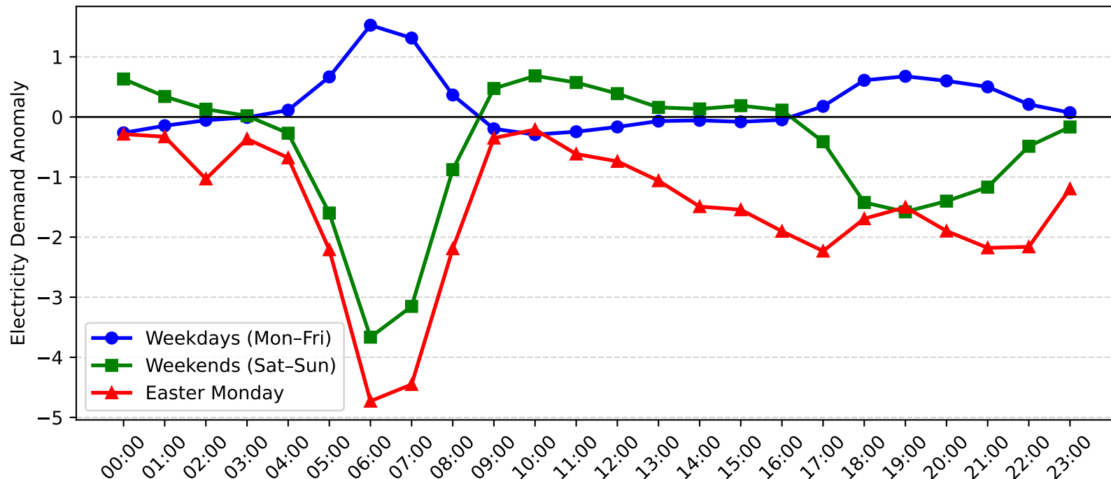
Cronulla Demand Anomaly: Easter Monday vs Weekday/Weekend (2012-2013)
