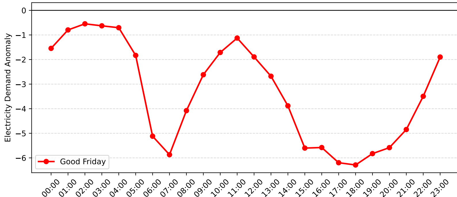
Pennant Hills Demand Anomaly: Good Friday (2015-2016)
