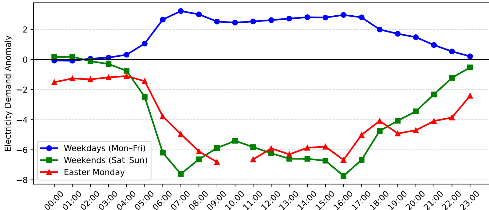
Epping Demand Anomaly: Easter Monday vs Weekday/Weekend (2005-2006)
