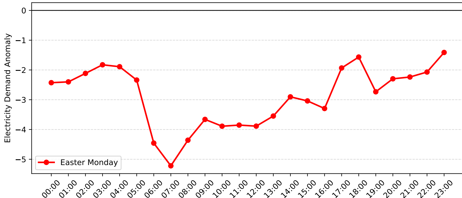
Matraverse Demand Anomaly: Easter Monday (2014-2015)
