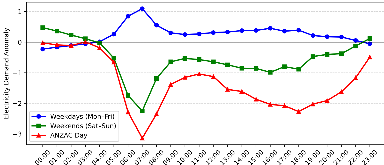
Blakehurst Demand Anomaly: ANZAC Day vs Weekday/Weekend (2009-2010)
