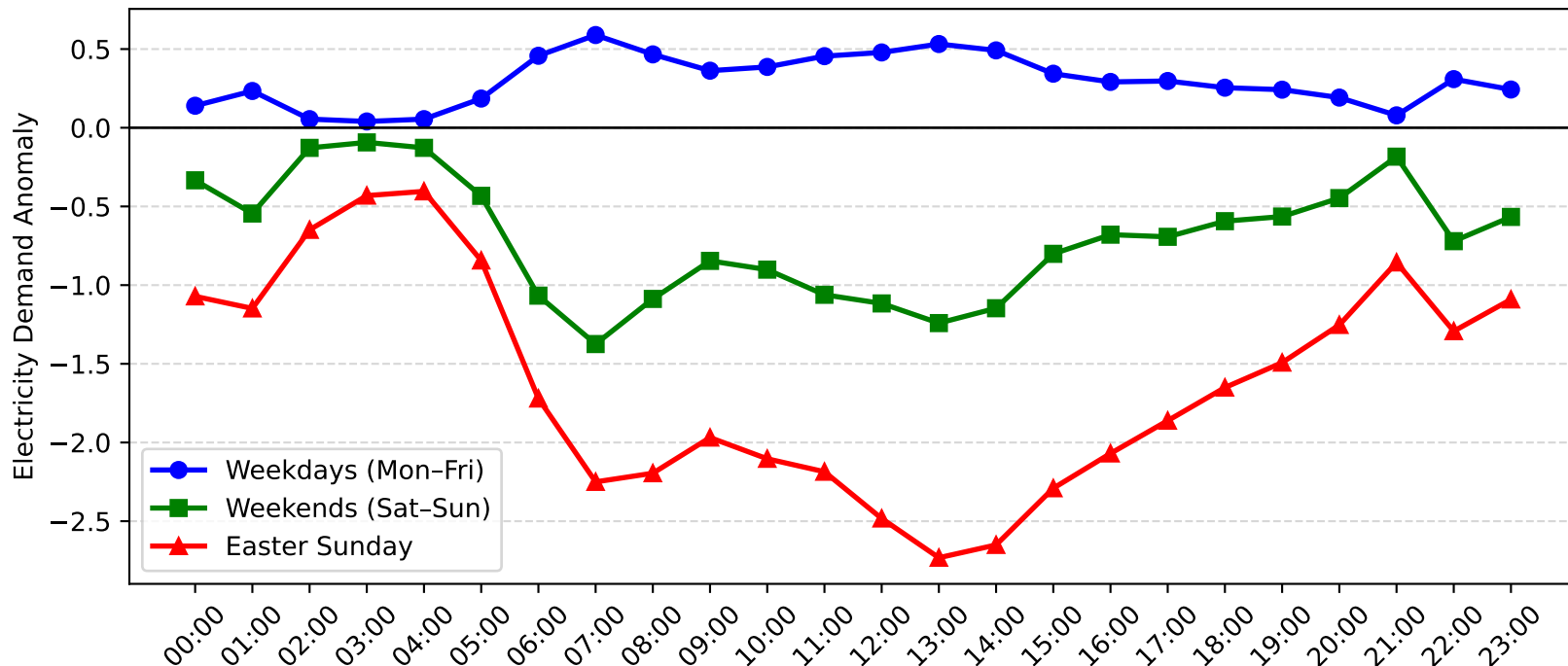
Gateshead Demand Anomaly: Easter Sunday vs Weekday/Weekend (2013-2014)
