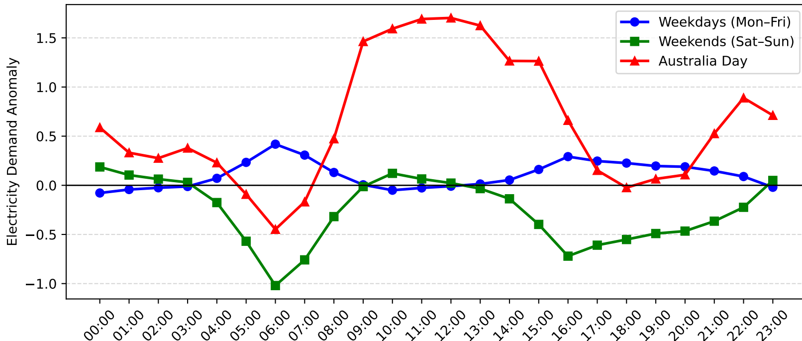
Woy Woy Demand Anomaly: Australia Day vs Weekday/Weekend (2012-2013)
