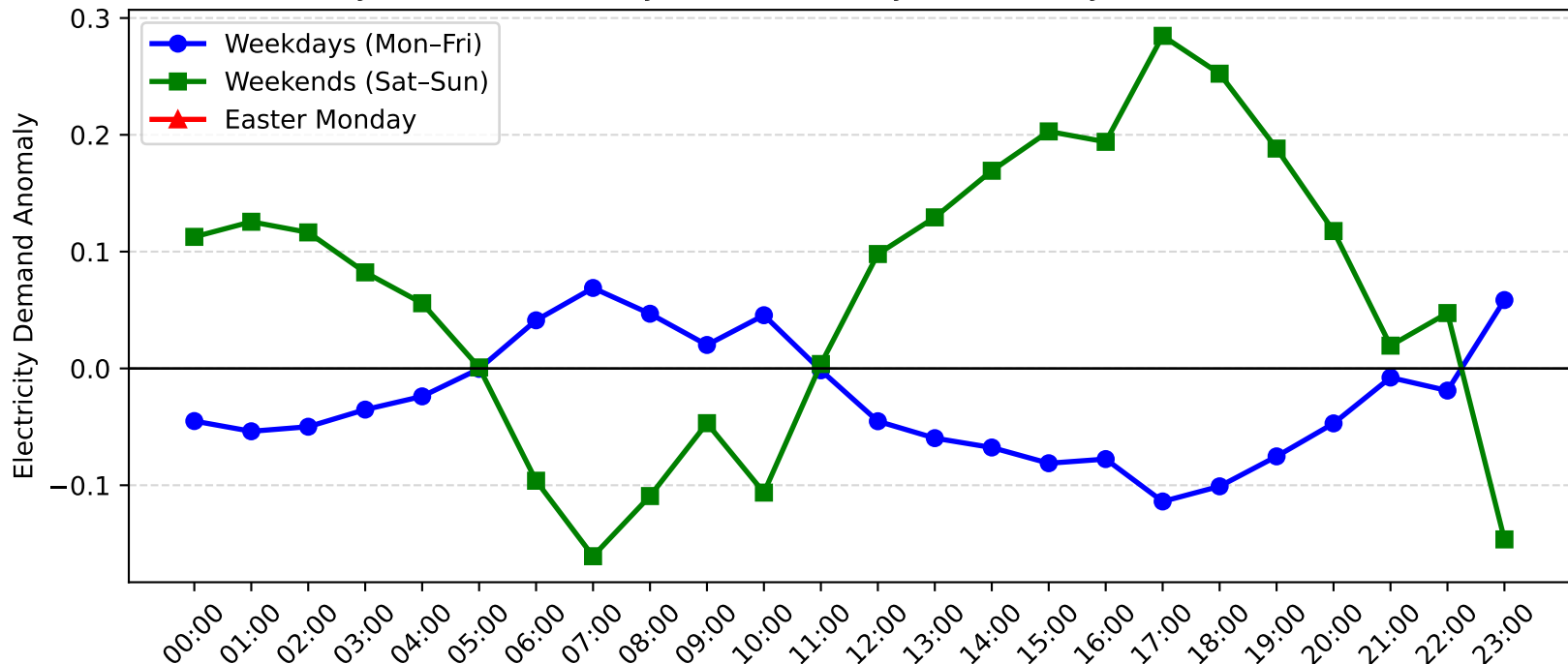
Rothbury Demand Anomaly: Easter Monday vs Weekday/Weekend (2006-2007)
