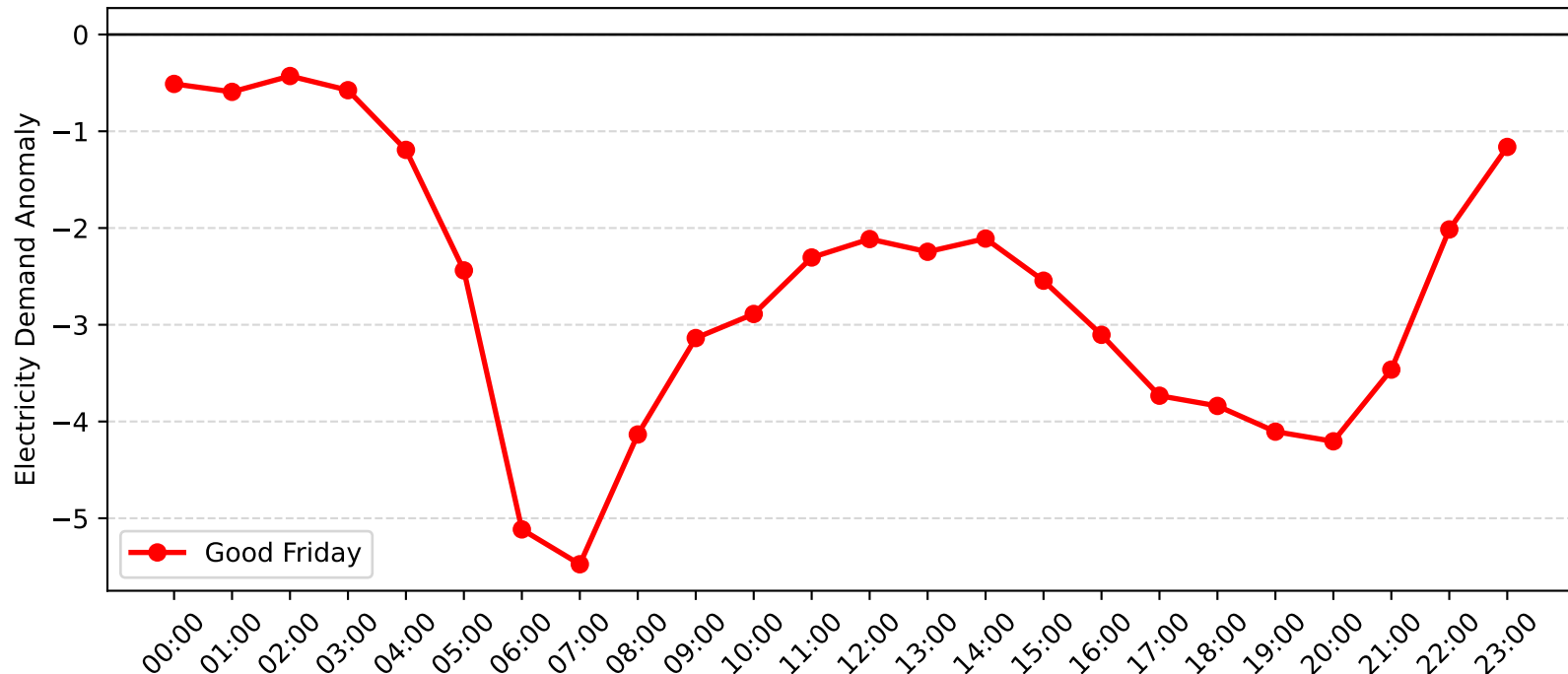
Revesby Demand Anomaly: Good Friday (2011-2012)
