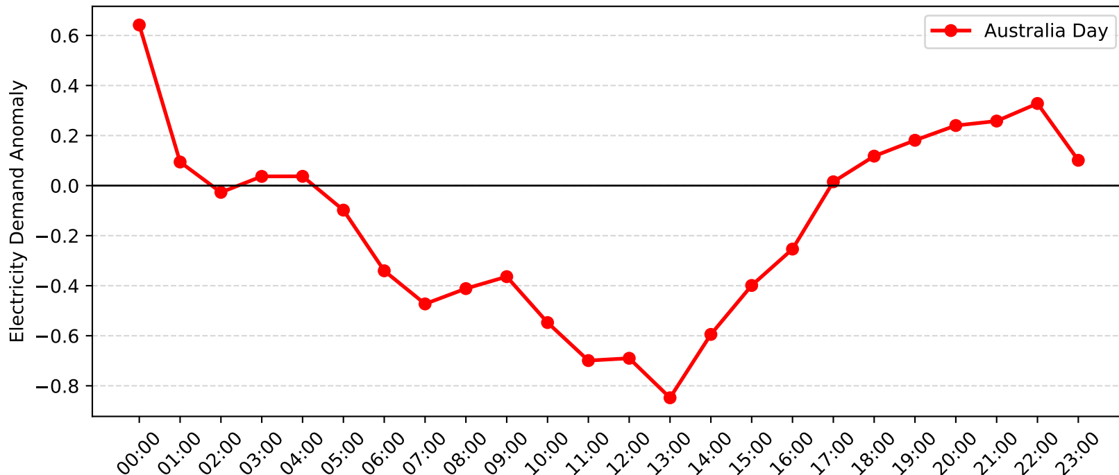
Telarah Demand Anomaly: Australia Day (2007-2008)
