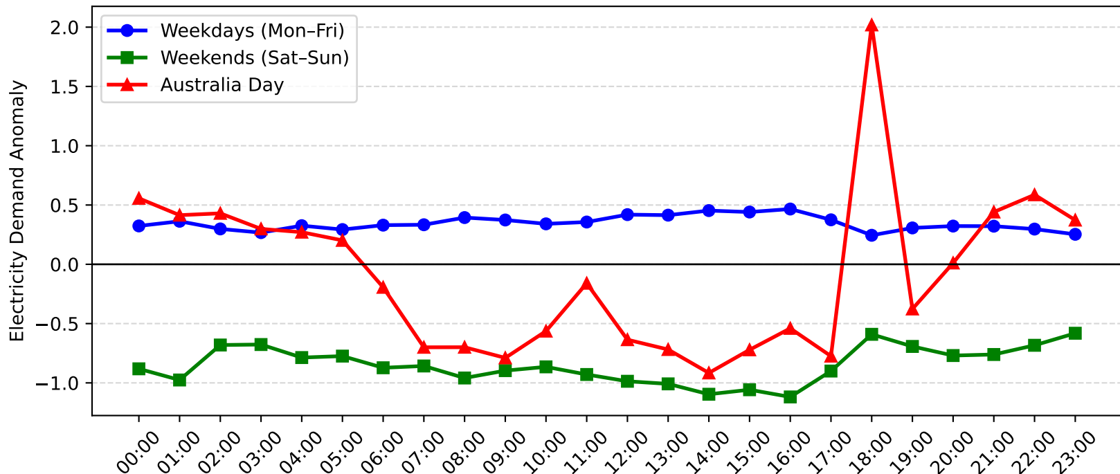
Lisarow Demand Anomaly: Australia Day vs Weekday/Weekend (2004-2005)
