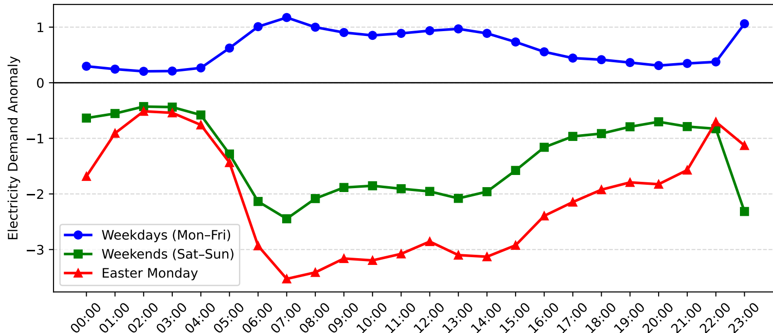
Rutherford Demand Anomaly: Easter Monday vs Weekday/Weekend (2009-2010)
