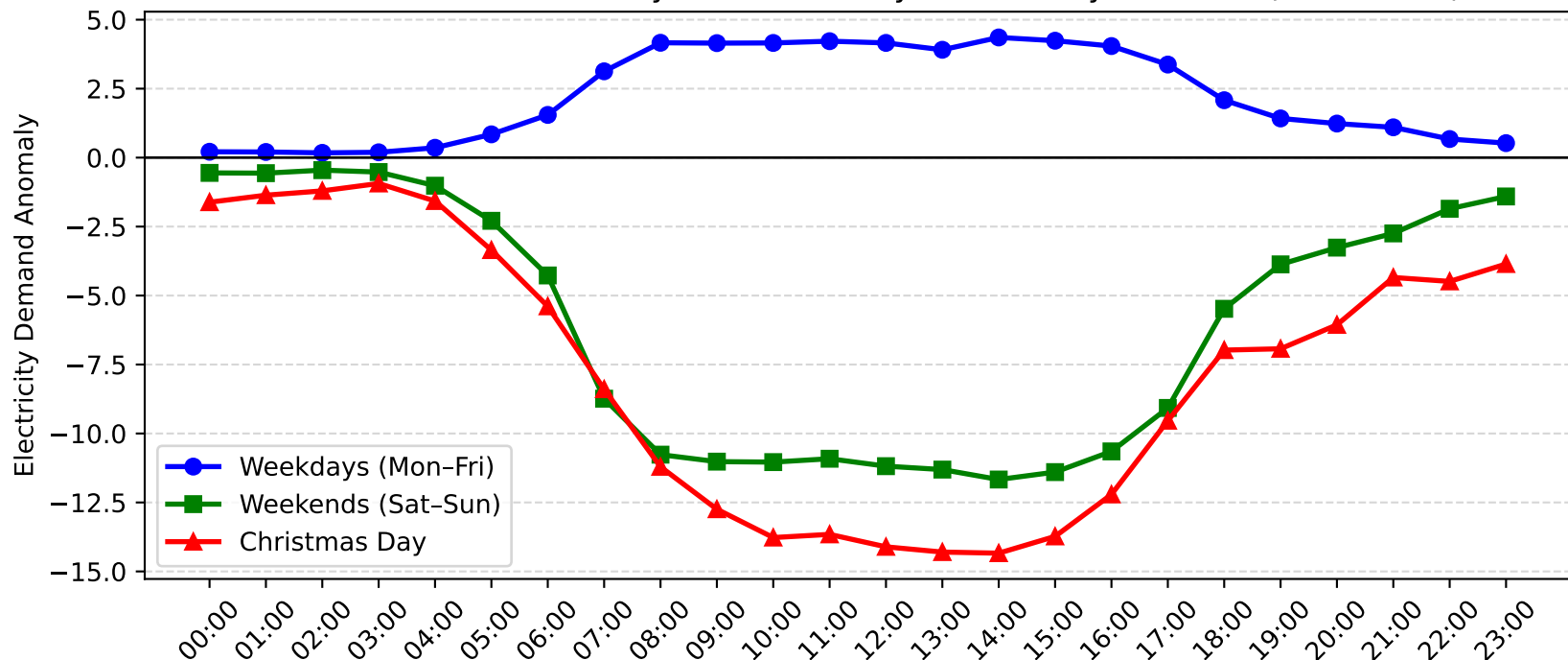
Gore Hill Demand Anomaly: Christmas Day vs Weekday/Weekend (2014-2015)
