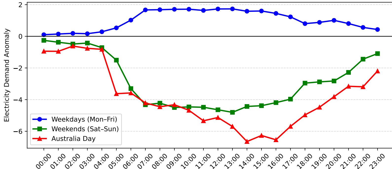
Potts Hill Demand Anomaly: Australia Day vs Weekday/Weekend (2016-2017)
