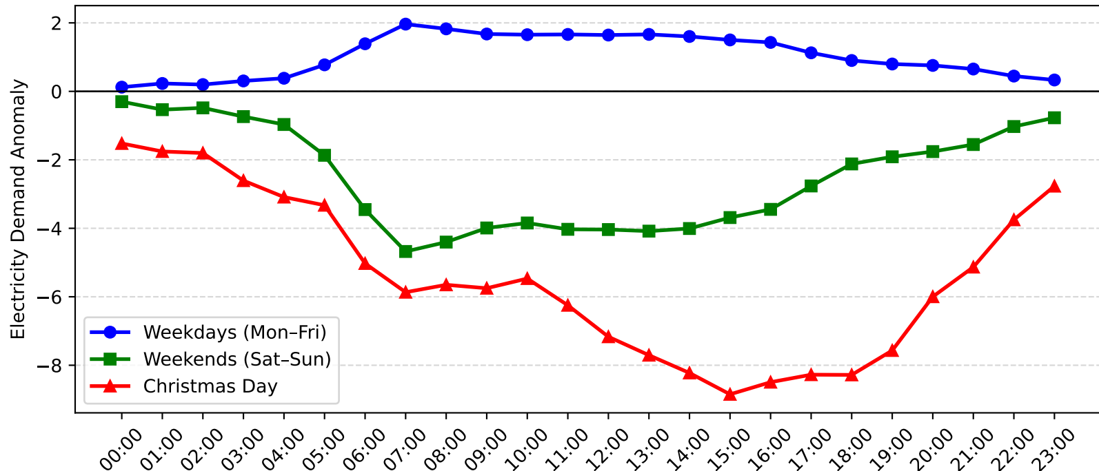
Matraverse Demand Anomaly: Christmas Day vs Weekday/Weekend (2006-2007)
