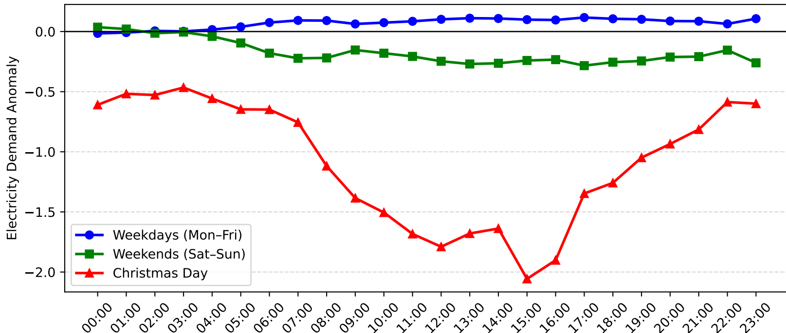
Rothbury Demand Anomaly: Christmas Day vs Weekday/Weekend (2015-2016)
