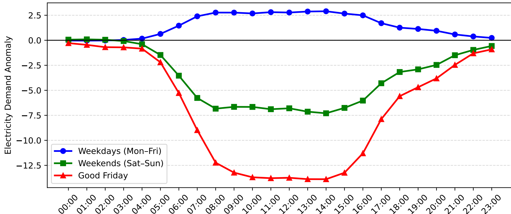
Brookvale Demand Anomaly: Good Friday vs Weekday/Weekend (2010-2011)
