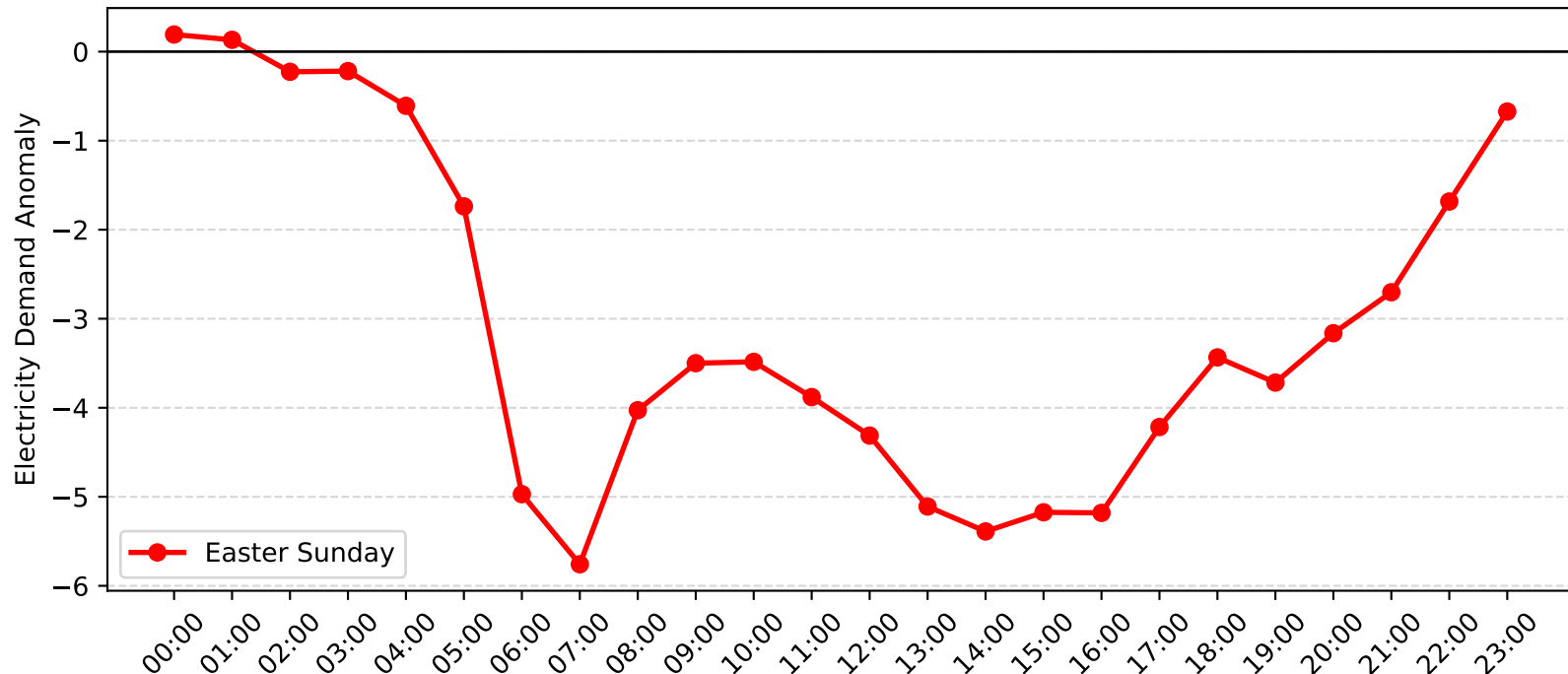
Mortdale Demand Anomaly: Easter Sunday (2005-2006)
