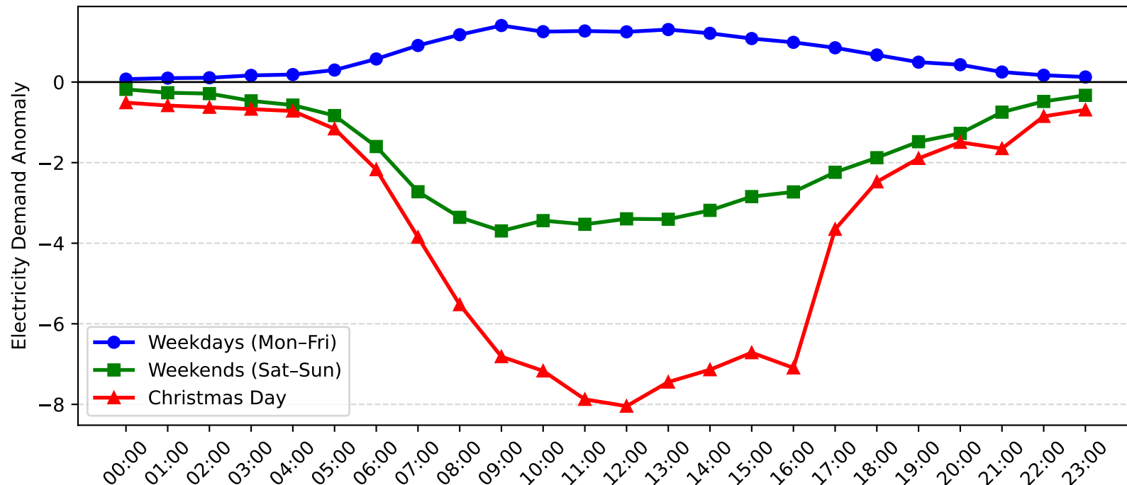
Auburn Demand Anomaly: Christmas Day vs Weekday/Weekend (2007-2008)
