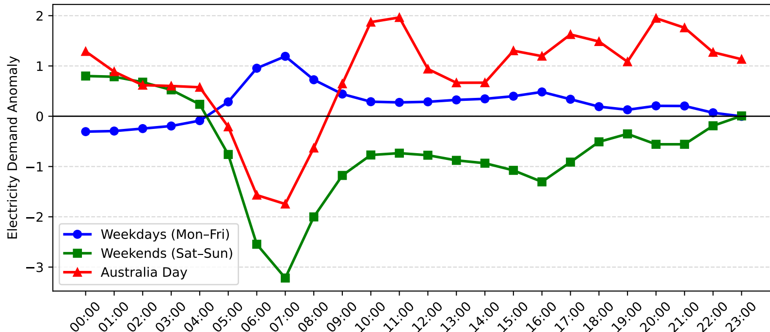
Dulwich Hill Demand Anomaly: Australia Day vs Weekday/Weekend (2011-2012)
