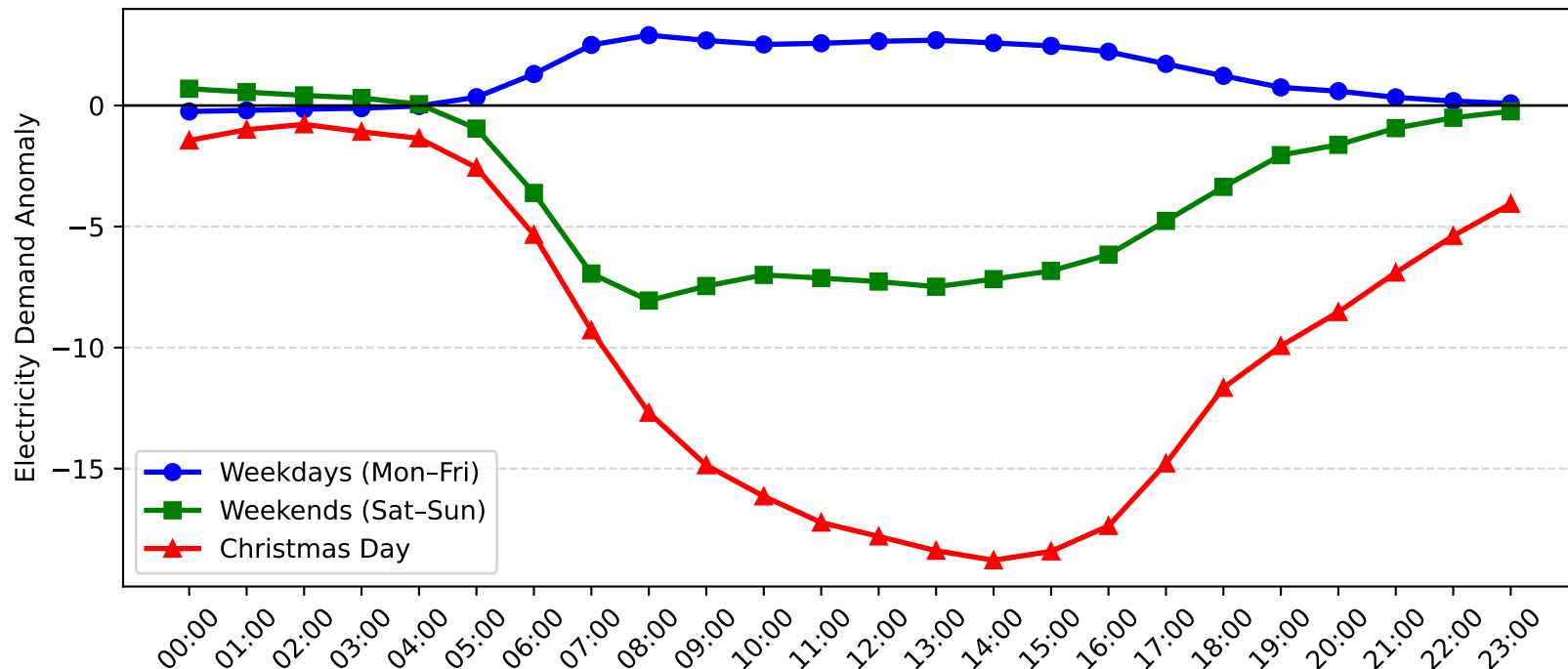
Zetland Demand Anomaly: Christmas Day vs Weekday/Weekend (2012-2013)
