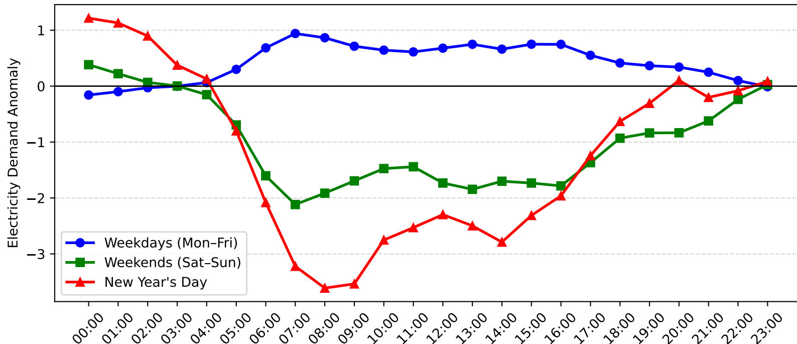
Rockdale Demand Anomaly: New Year's Day vs Weekday/Weekend (2006-2007)
