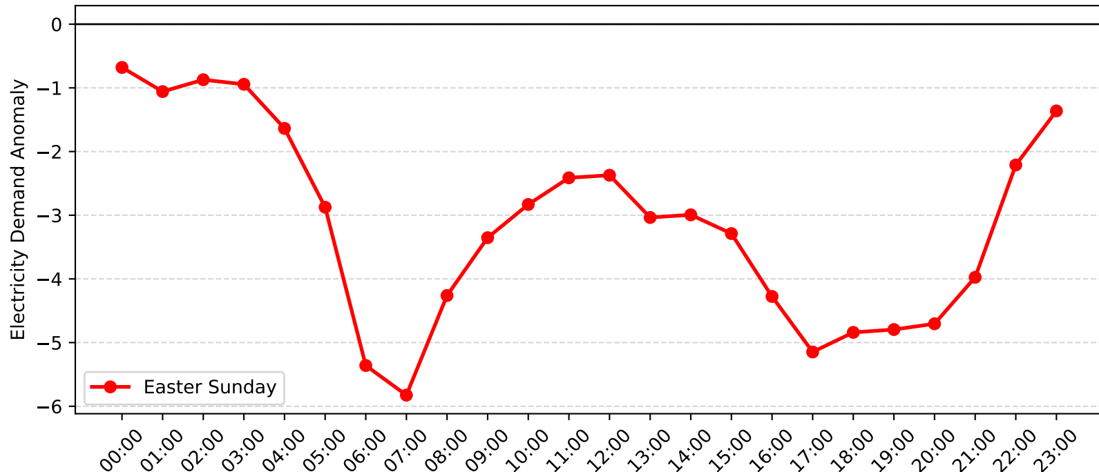
Revesby Demand Anomaly: Easter Sunday (2011-2012)
