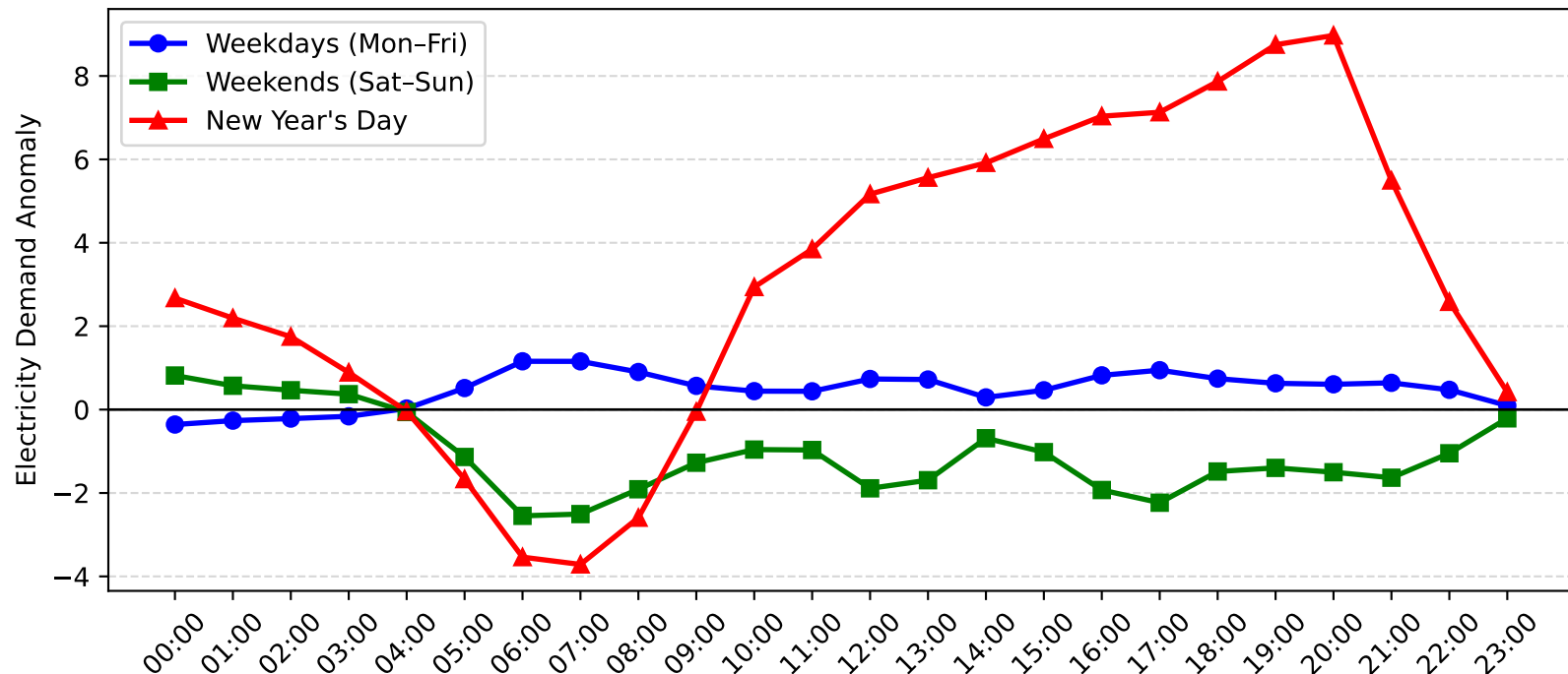
Revesby Demand Anomaly: New Year's Day vs Weekday/Weekend (2005-2006)
