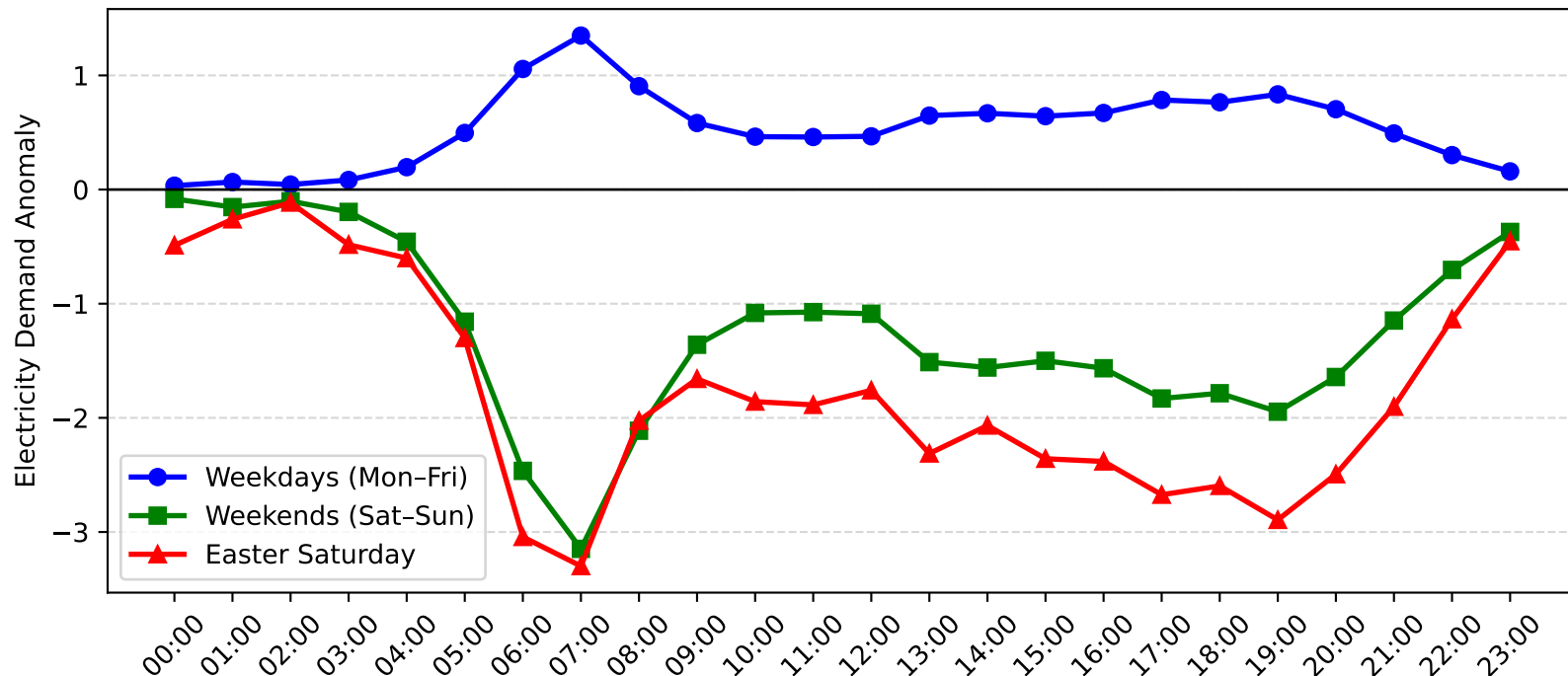
Maroubra Demand Anomaly: Easter Saturday vs Weekday/Weekend (2014-2015)
