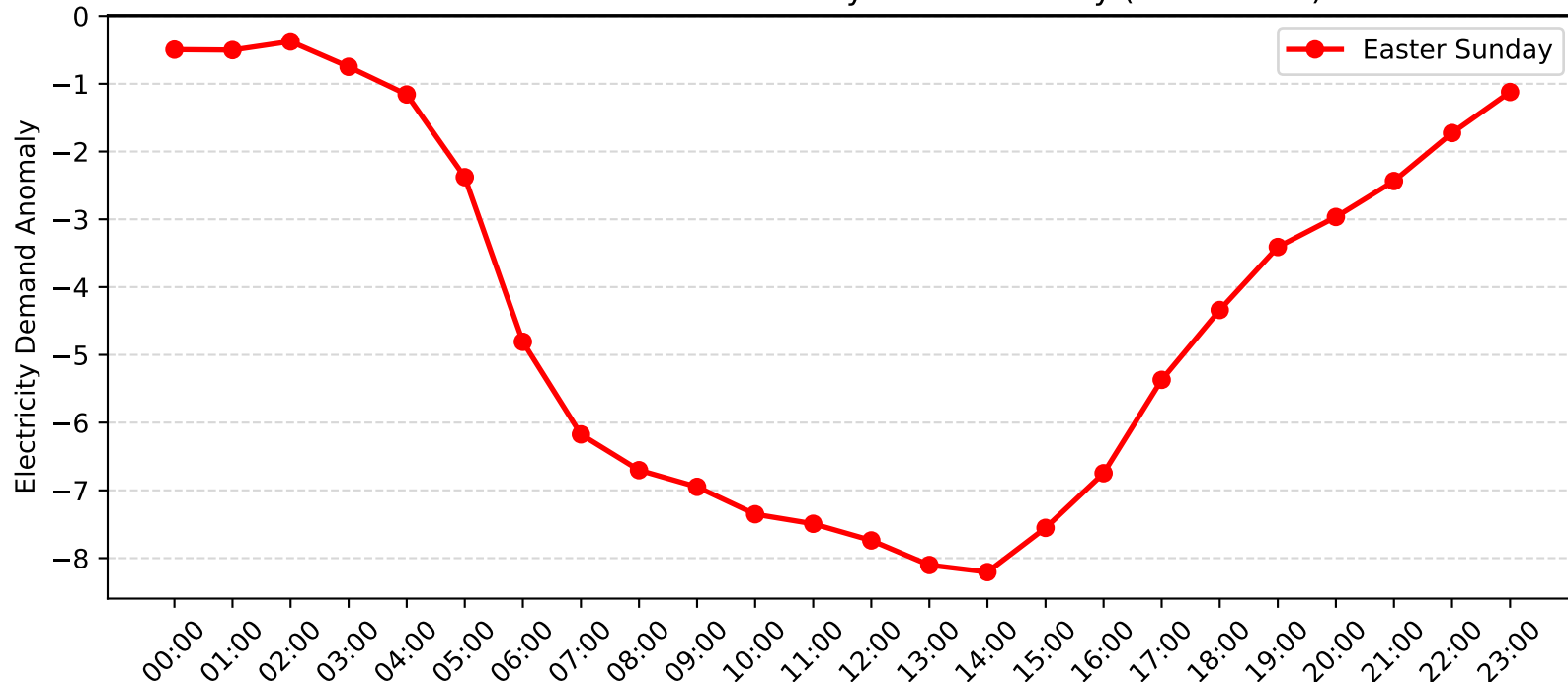
West Gosford Demand Anomaly: Easter Sunday (2013-2014)
