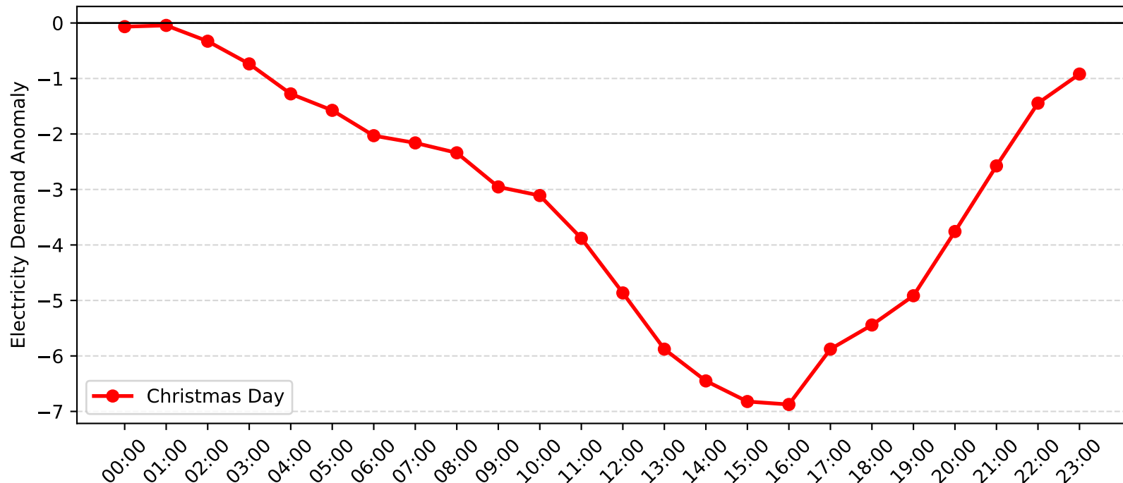
Charmhaven Demand Anomaly: Christmas Day (2015-2016)
