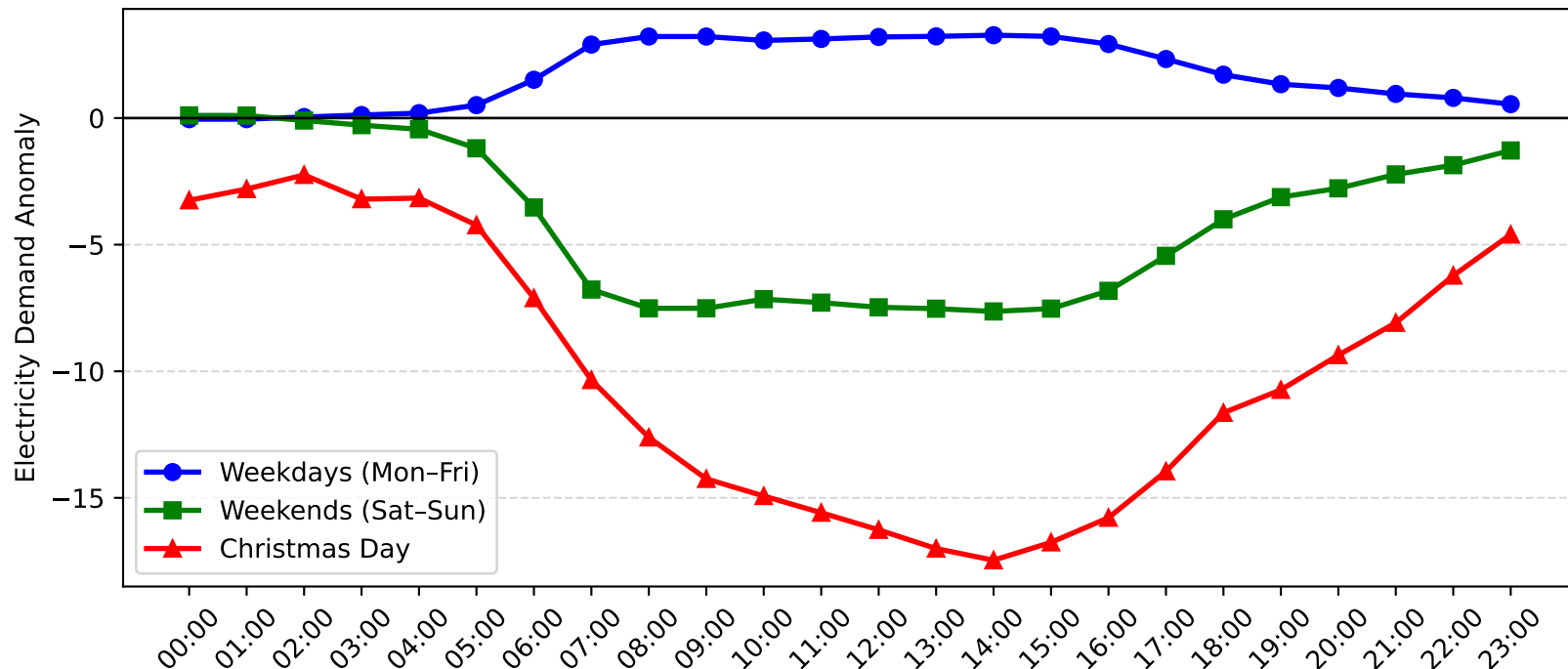
Zetland Demand Anomaly: Christmas Day vs Weekday/Weekend (2016-2017)
