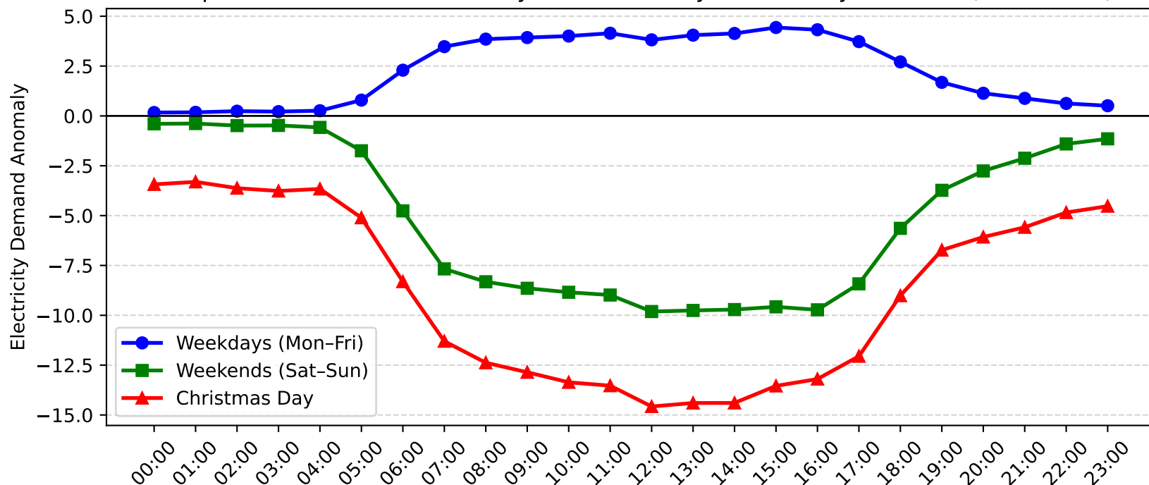
Macquarie Park Demand Anomaly: Christmas Day vs Weekday/Weekend (2004-2005)
