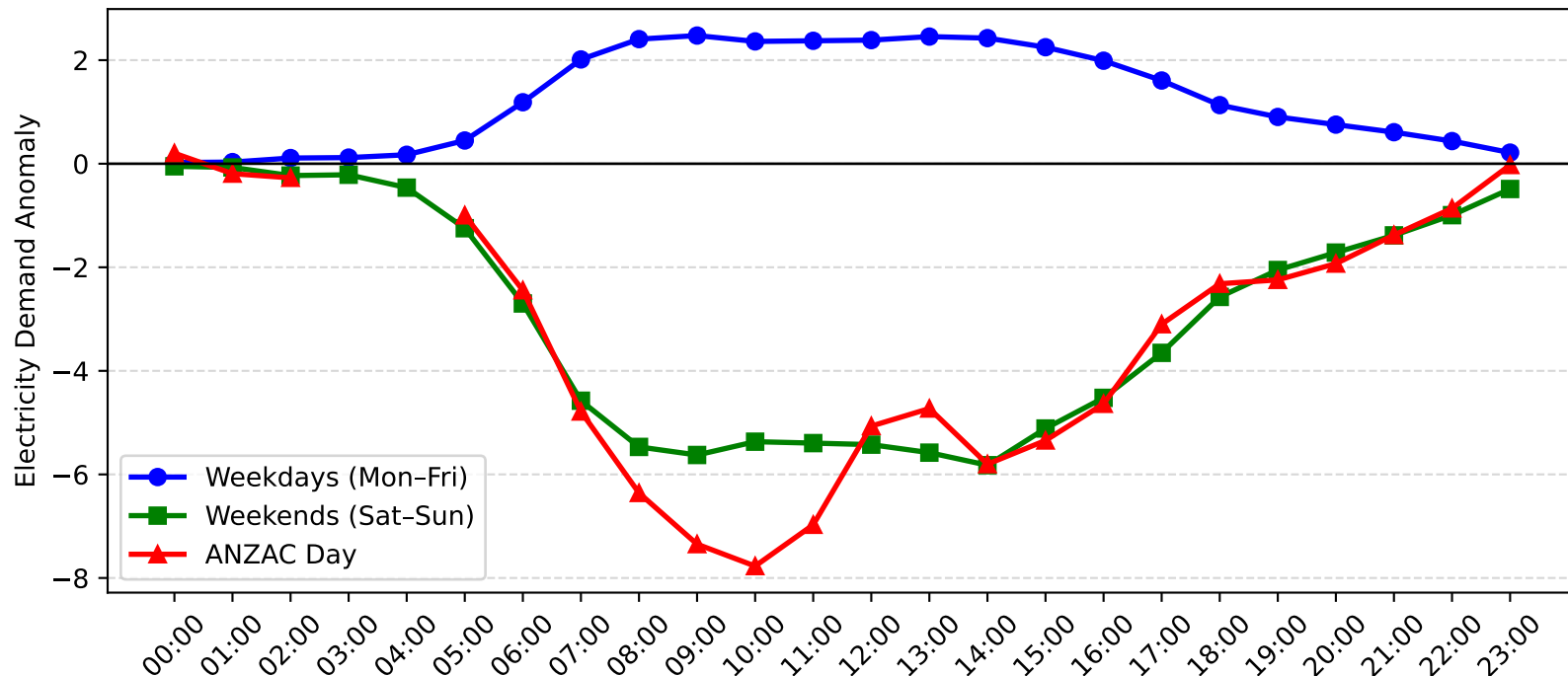
Green Square Demand Anomaly: ANZAC Day vs Weekday/Weekend (2017-2018)
