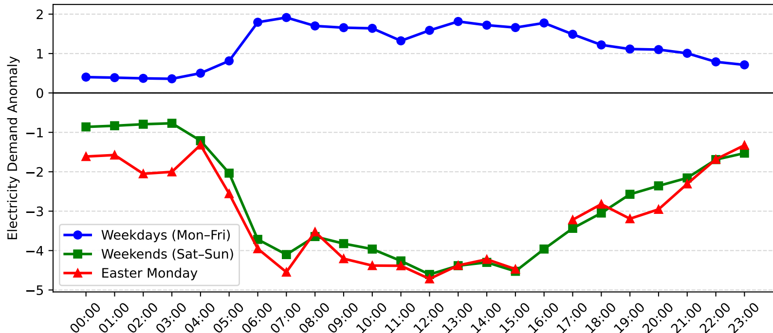
Potts Hill Demand Anomaly: Easter Monday vs Weekday/Weekend (2017-2018)
