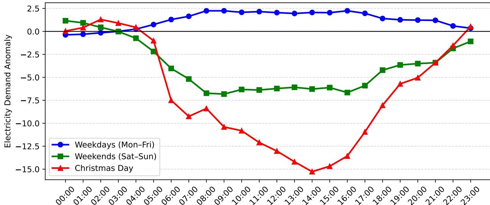
Greenacre Park Demand Anomaly: Christmas Day vs Weekday/Weekend (2013-2014)
