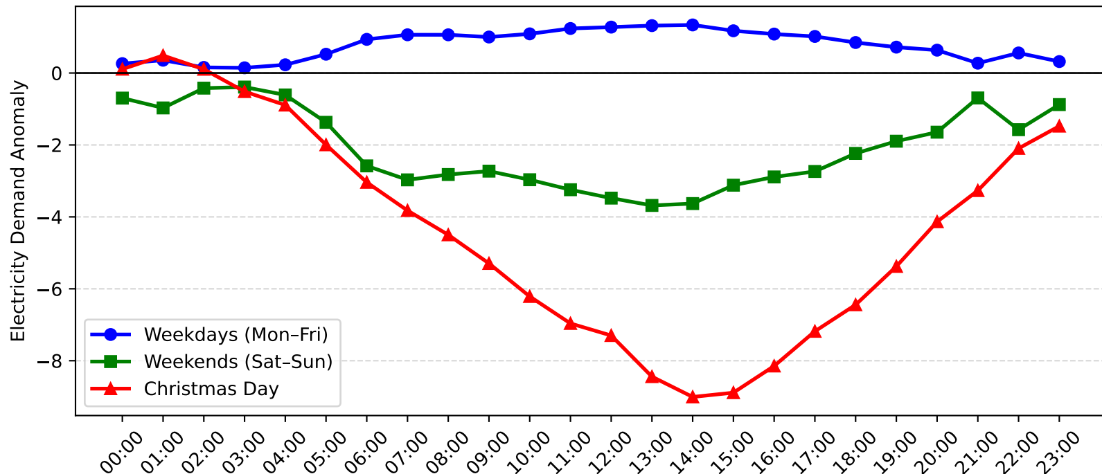
Argenton Demand Anomaly: Christmas Day vs Weekday/Weekend (2014-2015)
