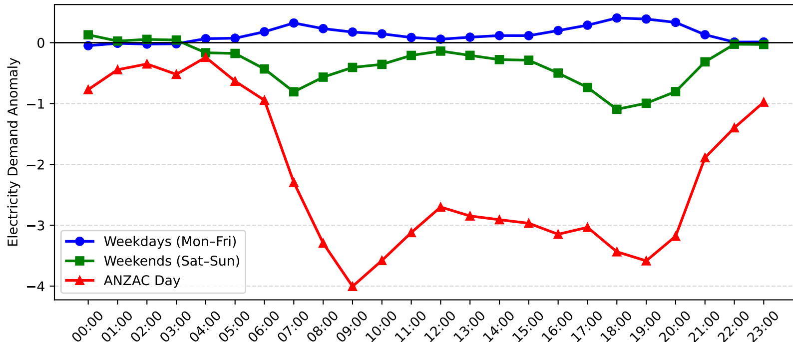
Erina Demand Anomaly: ANZAC Day vs Weekday/Weekend (2004-2005)
