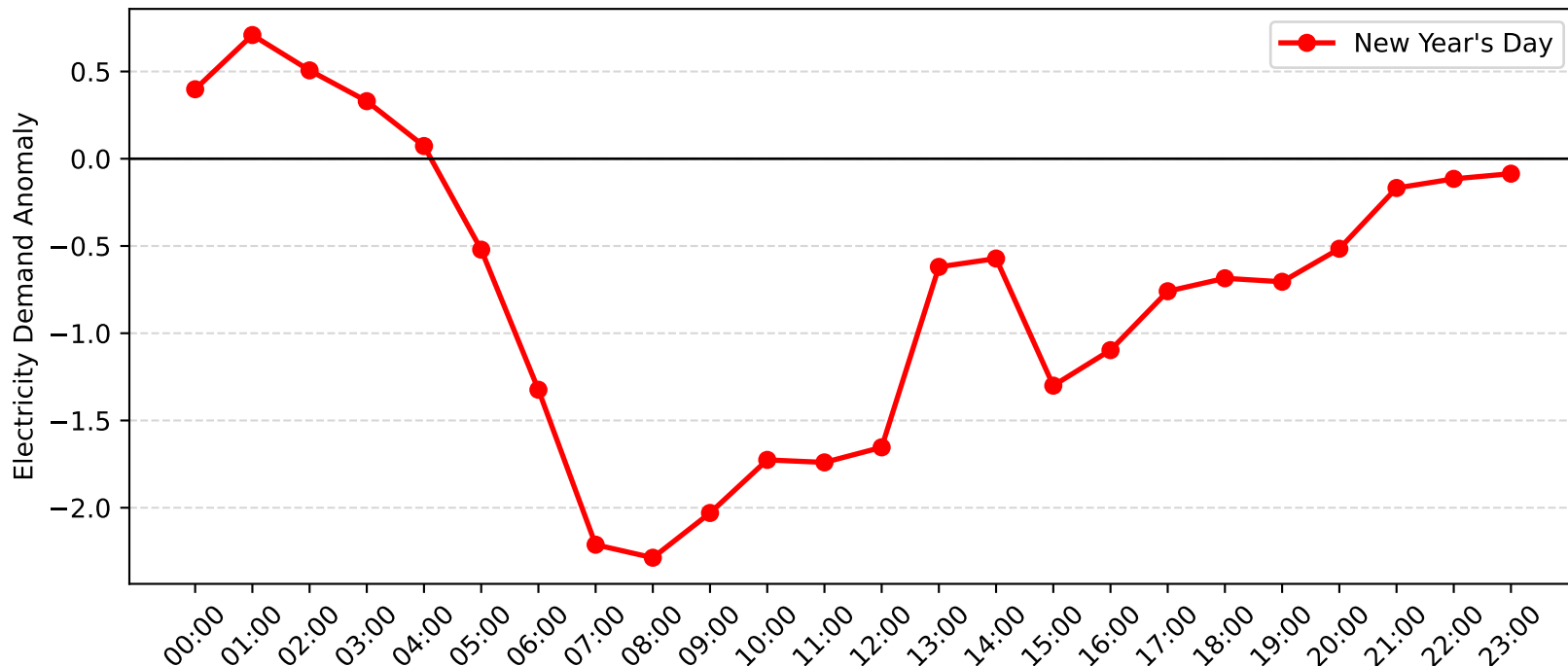
Arncliffe Demand Anomaly: New Year's Day (2013-2014)
