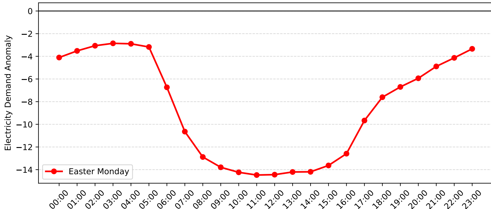
Gore Hill Demand Anomaly: Easter Monday (2010-2011)
