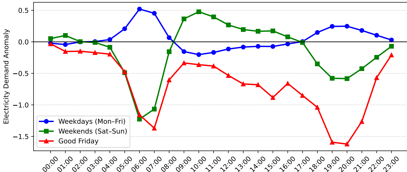
Harbord Demand Anomaly: Good Friday vs Weekday/Weekend (2017-2018)
