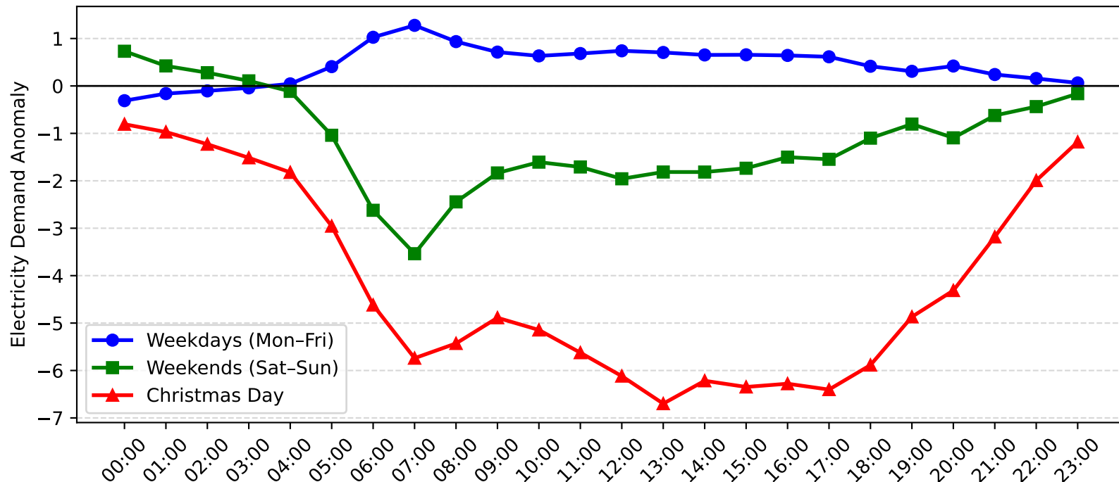
Dulwich Hill Demand Anomaly: Christmas Day vs Weekday/Weekend (2009-2010)
