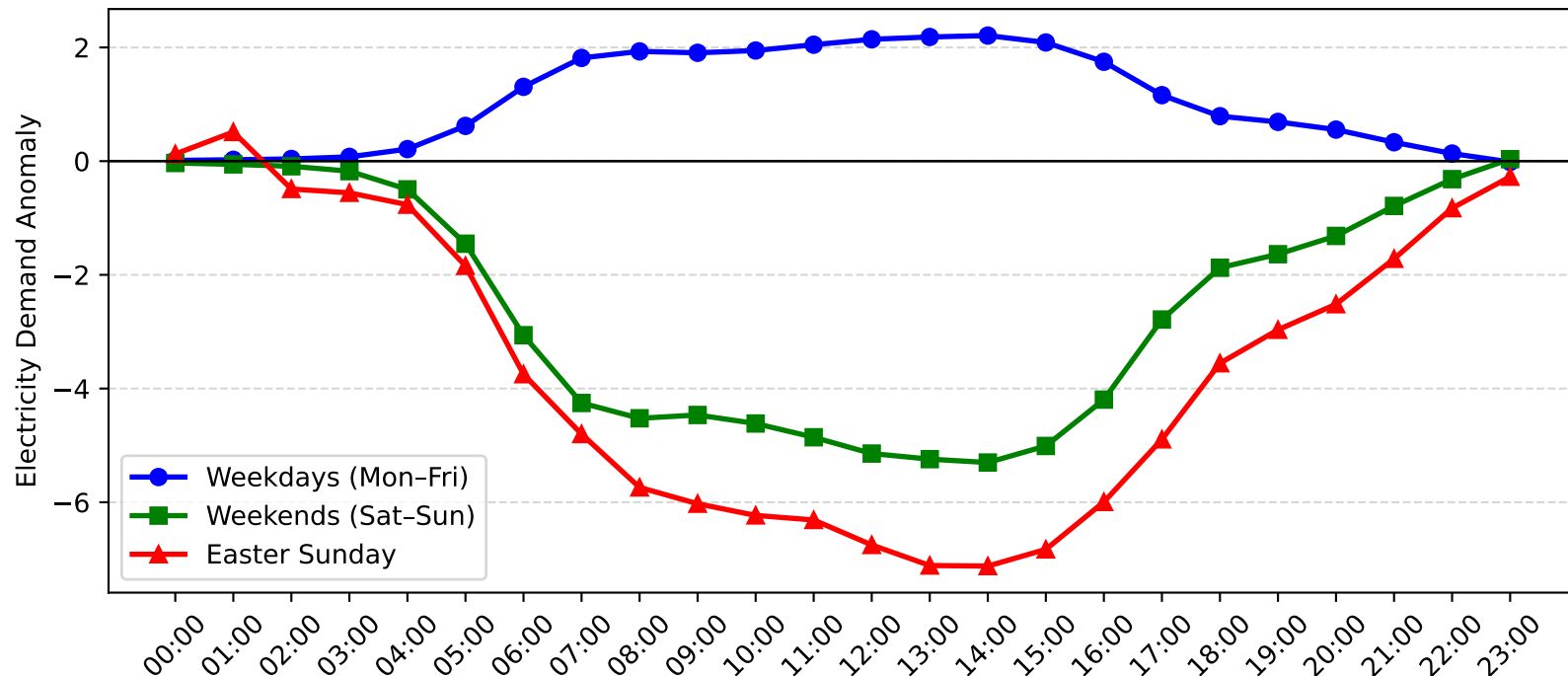
West Gosford Demand Anomaly: Easter Sunday vs Weekday/Weekend (2015-2016)
