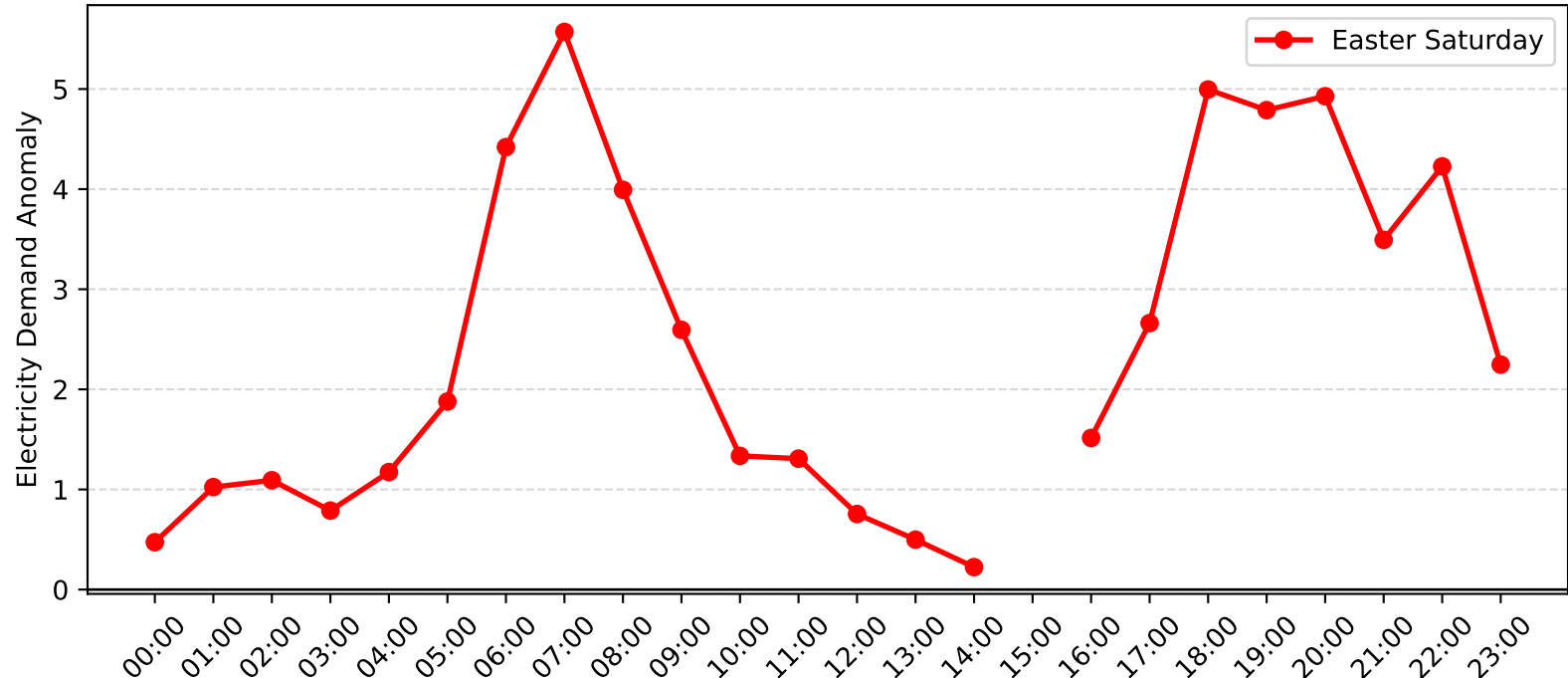
Lisarow Demand Anomaly: Easter Saturday (2004-2005)
