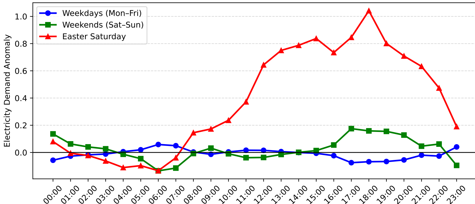
Rothbury Demand Anomaly: Easter Saturday vs Weekday/Weekend (2011-2021)
