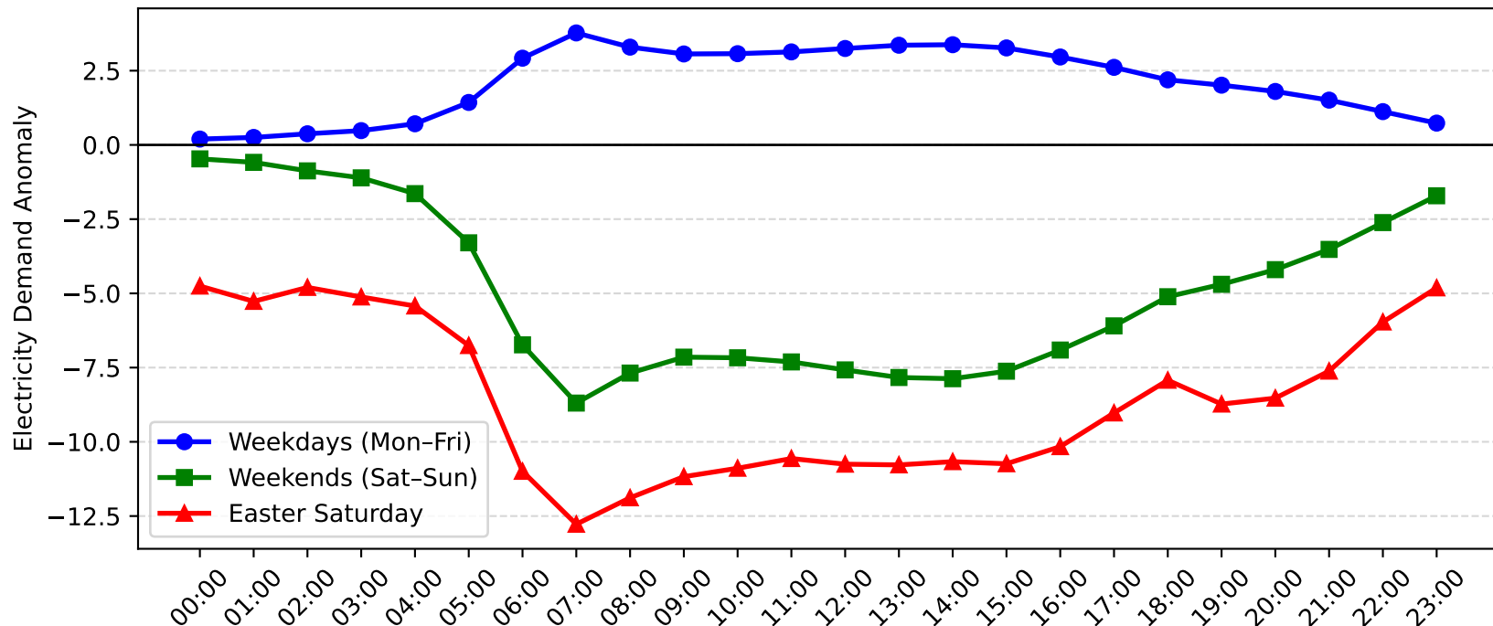
Sefton Demand Anomaly: Easter Saturday vs Weekday/Weekend (2011-2012)
