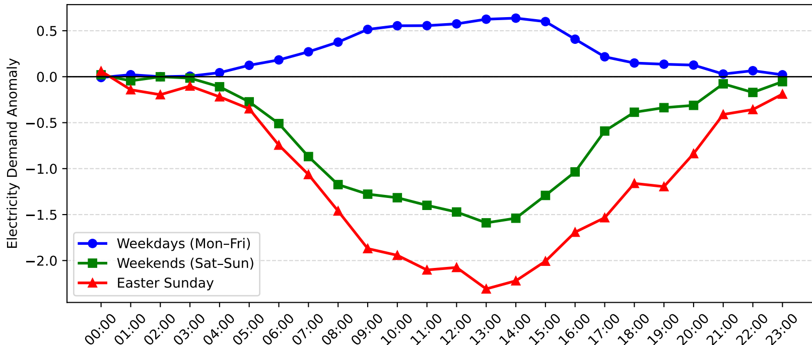
Broadmeadow Demand Anomaly: Easter Sunday vs Weekday/Weekend (2014-2015)
