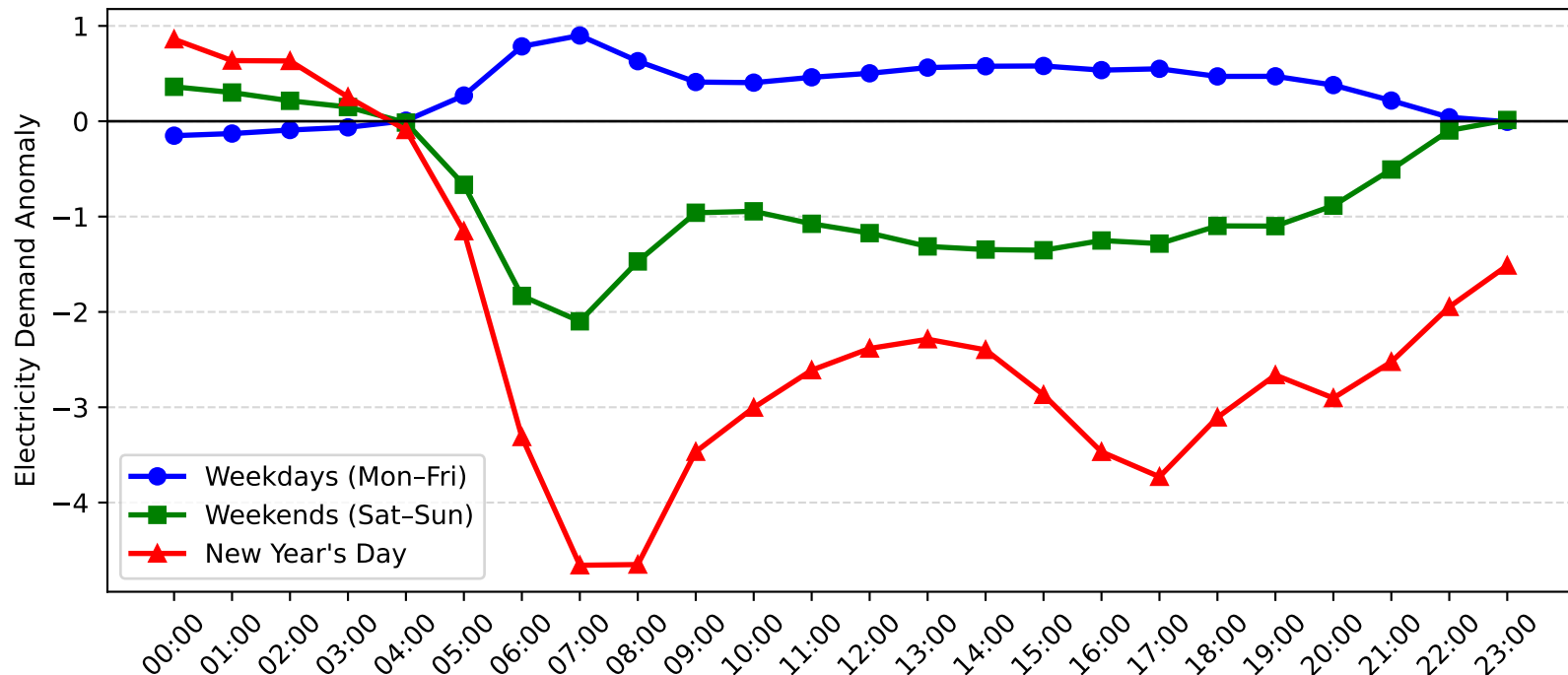
Dee Why West Demand Anomaly: New Year's Day vs Weekday/Weekend (2017-2018)
