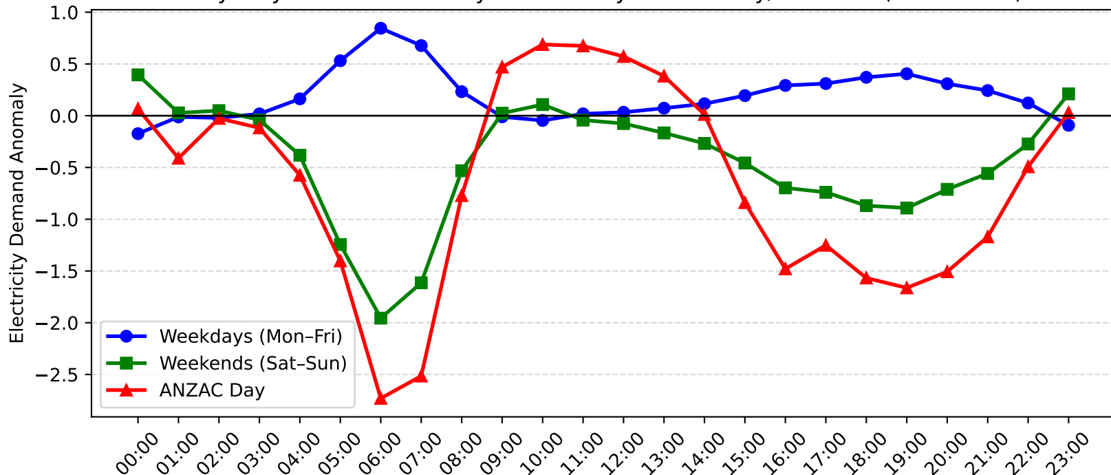
Woy Woy Demand Anomaly: ANZAC Day vs Weekday/Weekend (2008-2009)
