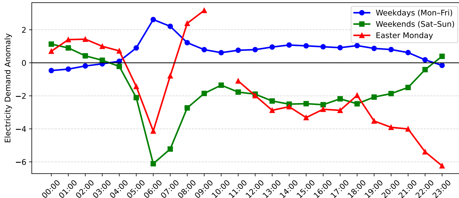
Pennant Hills Demand Anomaly: Easter Monday vs Weekday/Weekend (2005-2006)
