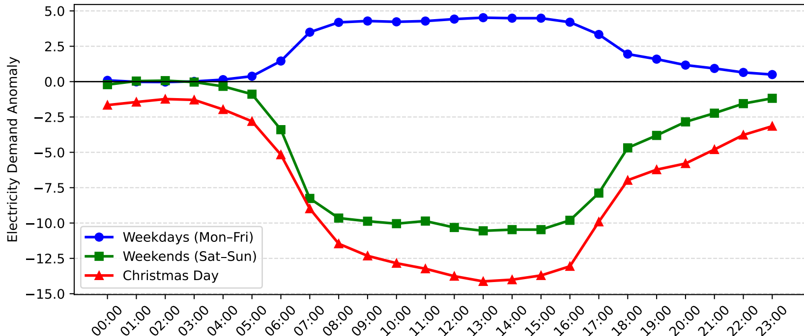
Gore Hill Demand Anomaly: Christmas Day vs Weekday/Weekend (2011-2012)
