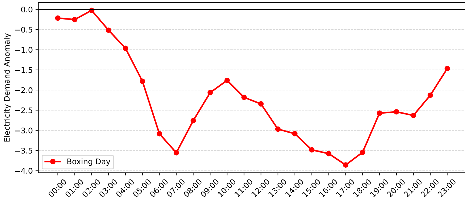
Revesby Demand Anomaly: Boxing Day (2011-2012)
