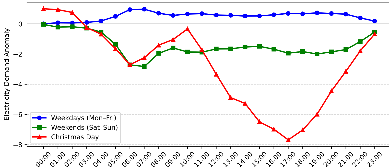
Revesby Demand Anomaly: Christmas Day vs Weekday/Weekend (2014-2015)
