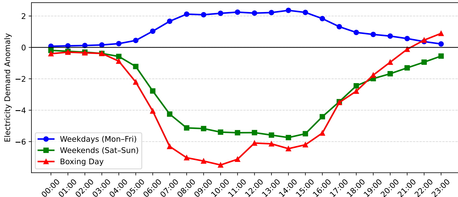
Bankstown Demand Anomaly: Boxing Day vs Weekday/Weekend (2014-2015)
