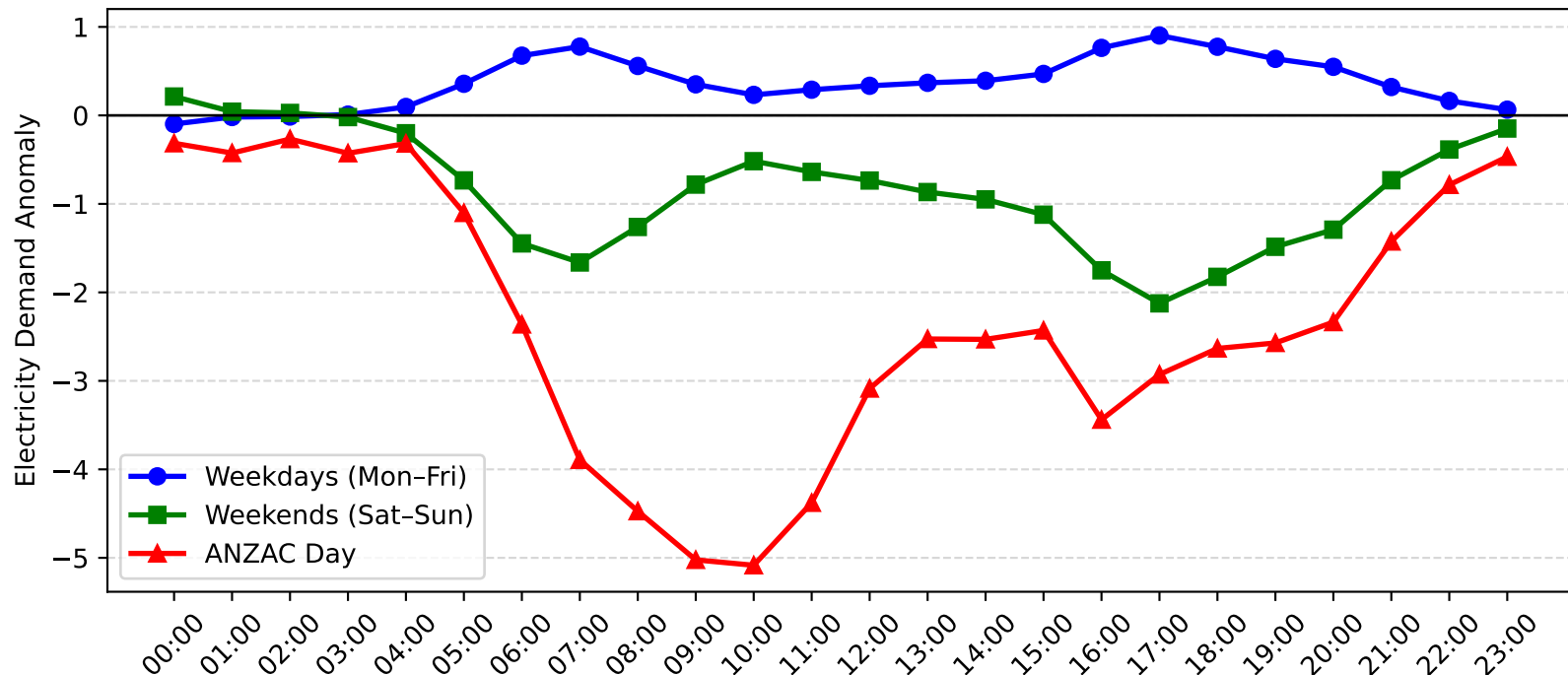
Erina Demand Anomaly: ANZAC Day vs Weekday/Weekend (2010-2011)
