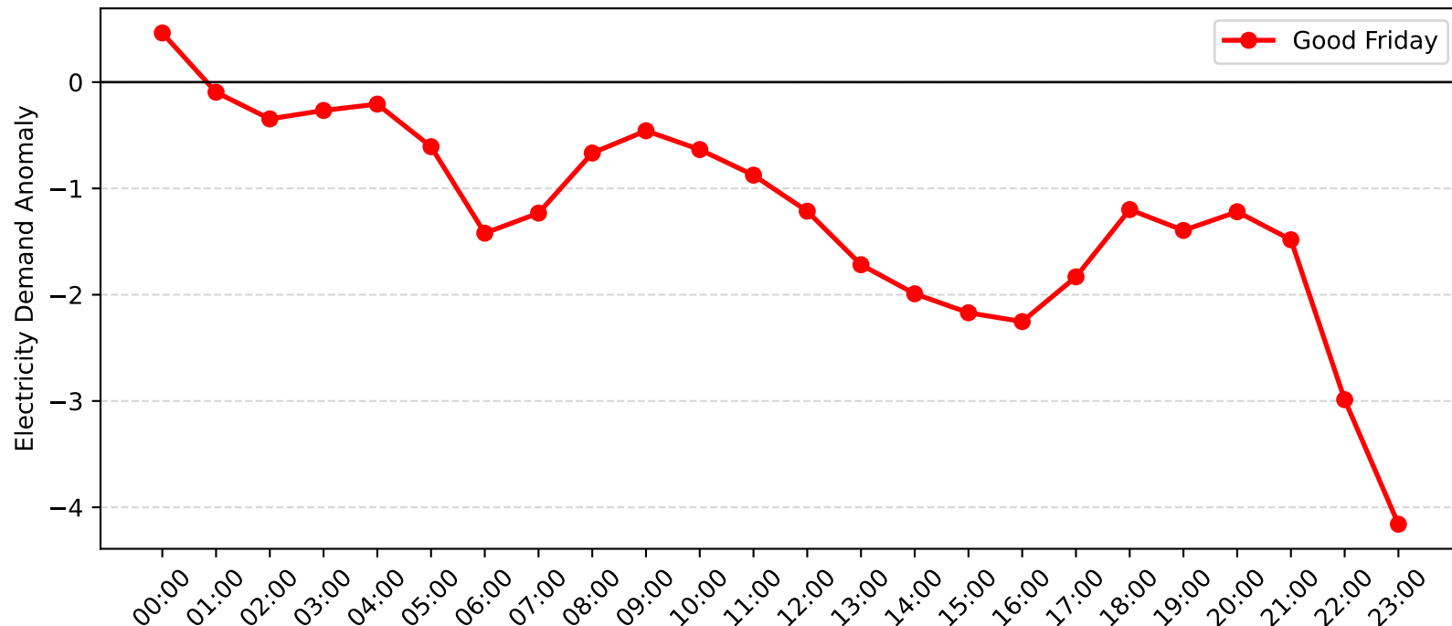
Muswellbrook Demand Anomaly: Good Friday (2006-2007)
