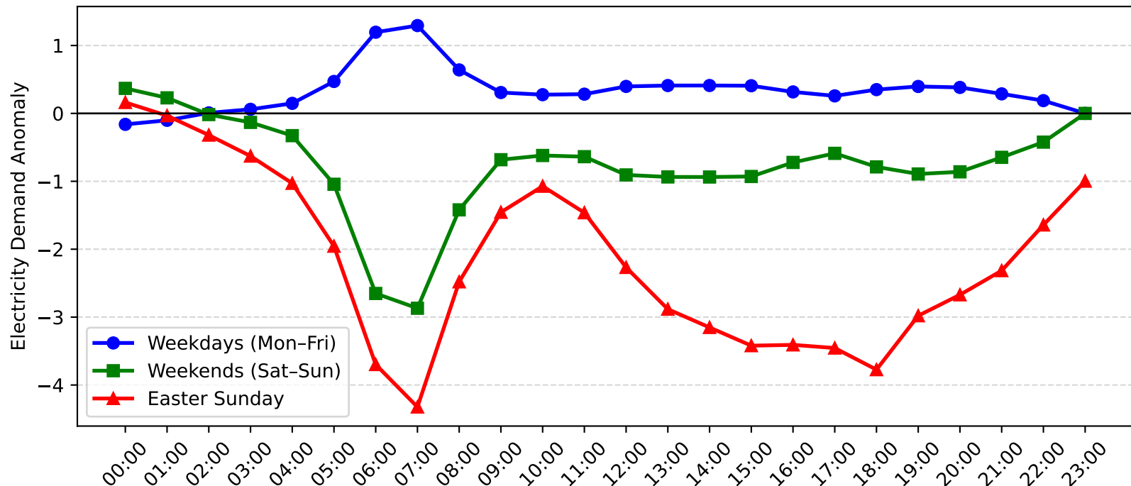
Mortdale Demand Anomaly: Easter Sunday vs Weekday/Weekend (2016-2017)
