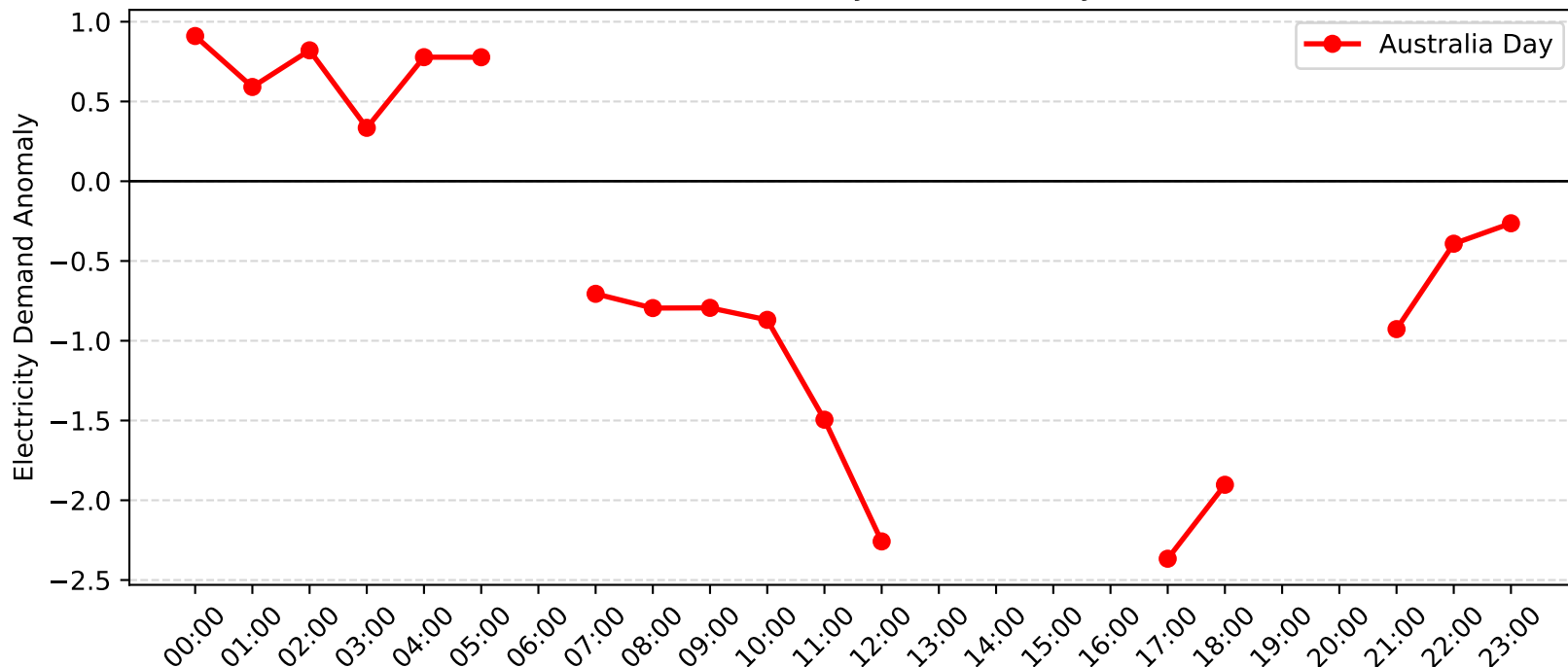
Adamstown Demand Anomaly: Australia Day (2015-2016)
