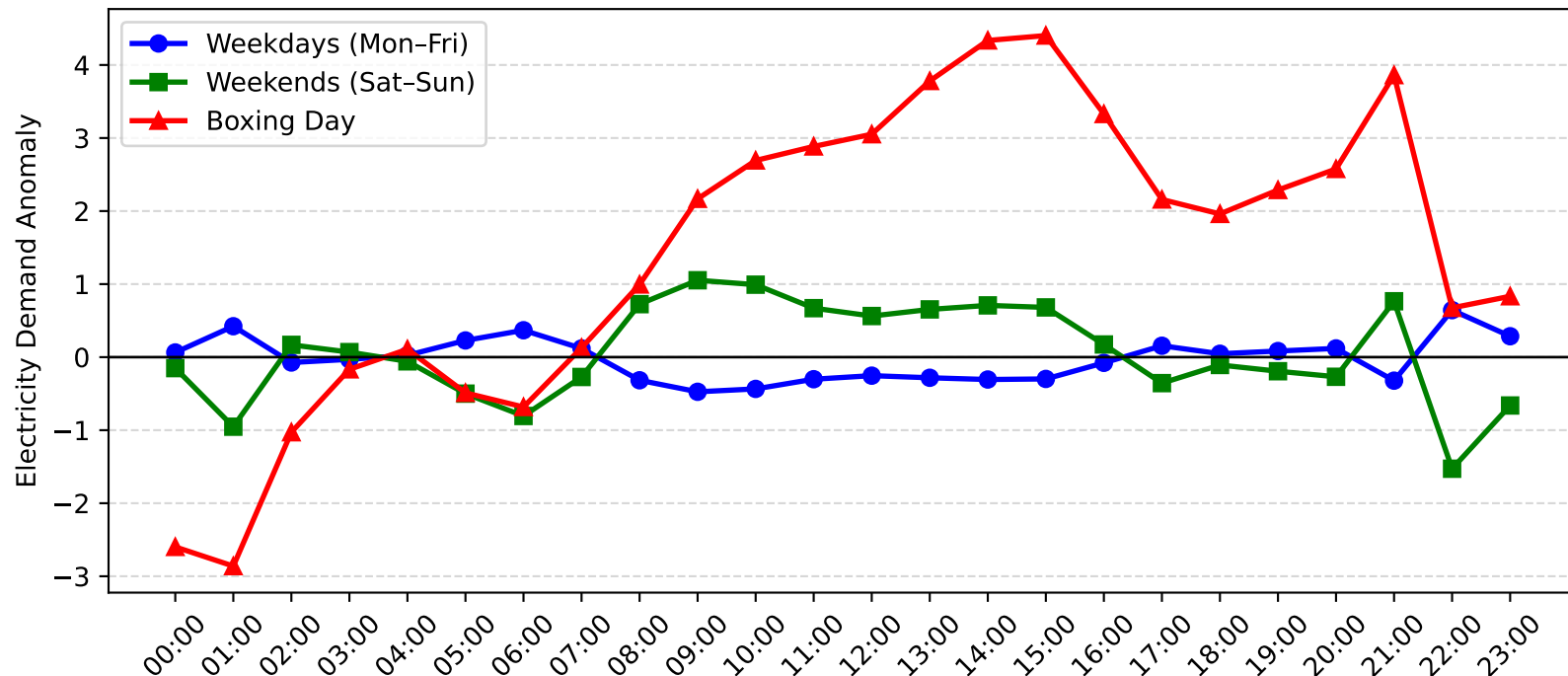
Nelson Bay Demand Anomaly: Boxing Day vs Weekday/Weekend (2010-2011)
