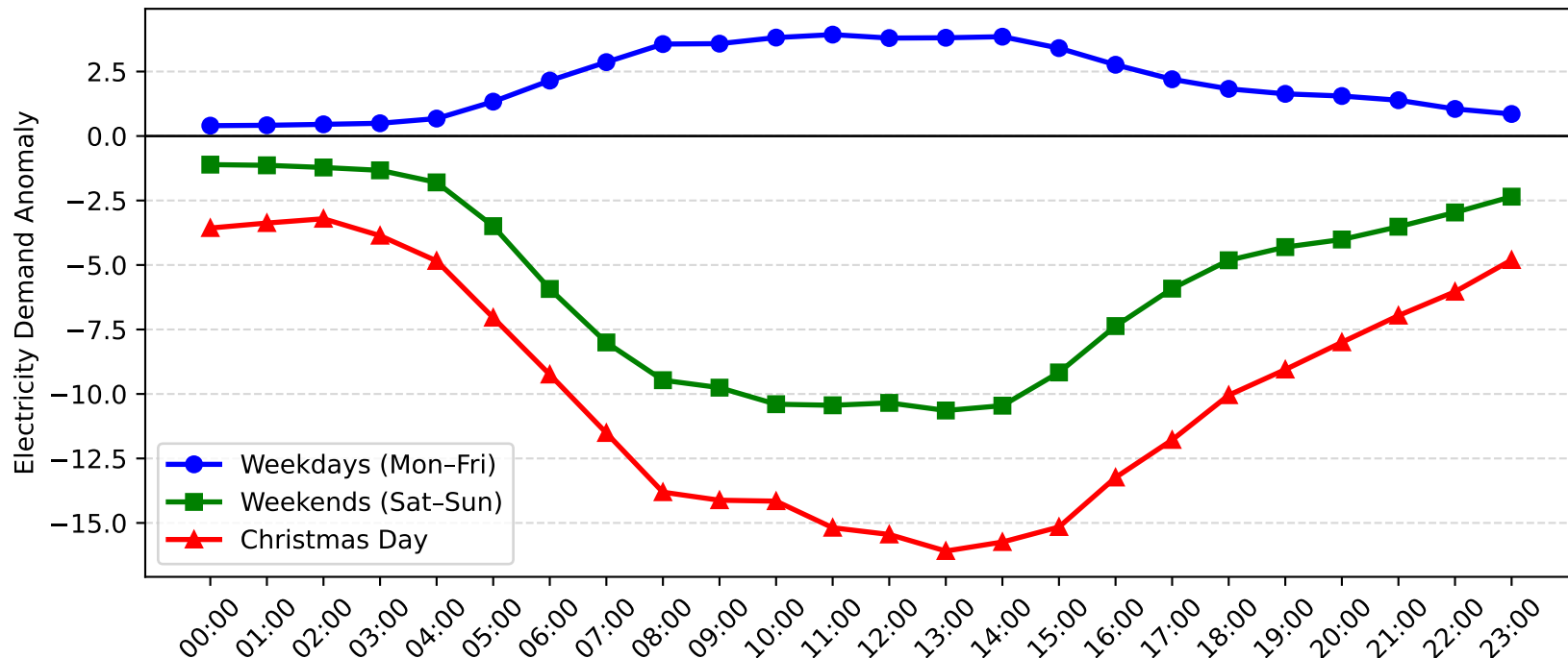
Milperra Demand Anomaly: Christmas Day vs Weekday/Weekend (2014-2015)
