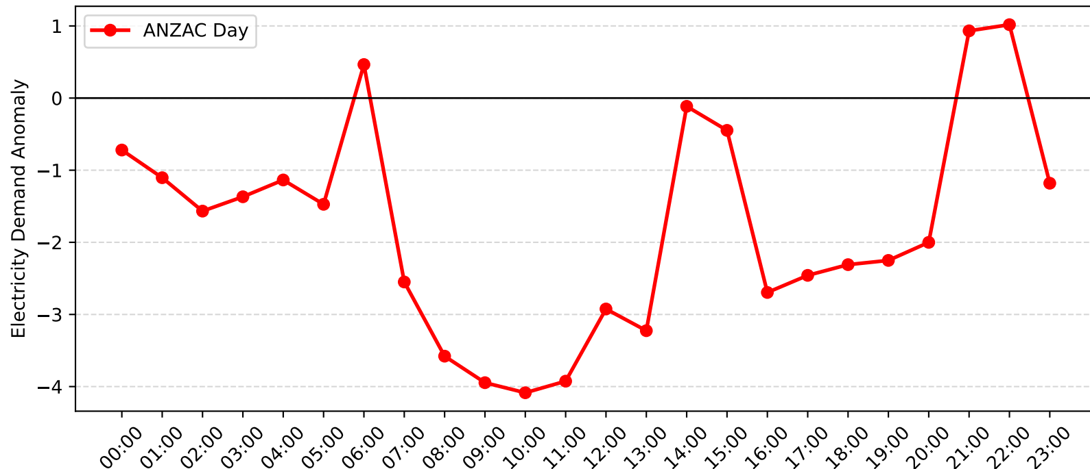
Green Square Demand Anomaly: ANZAC Day (2007-2008)
