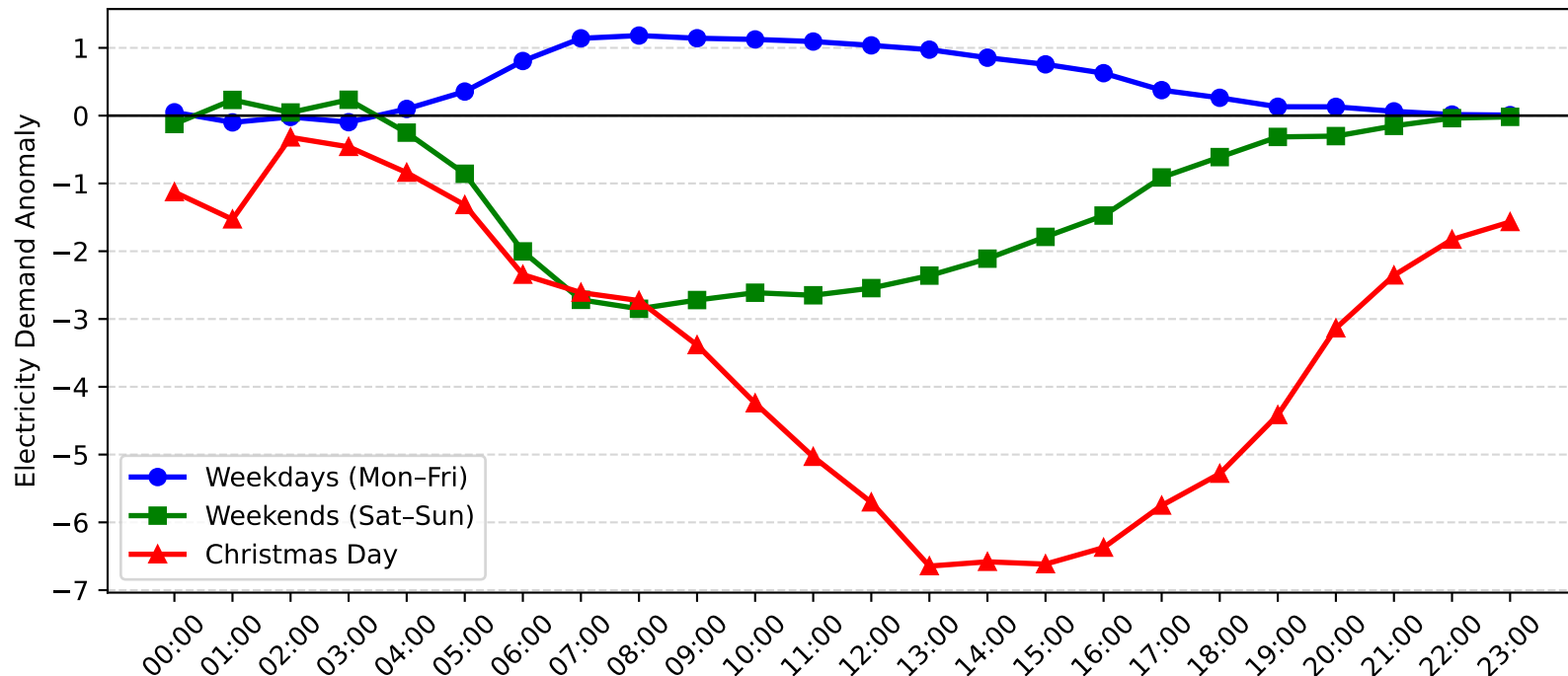
Wyong Demand Anomaly: Christmas Day vs Weekday/Weekend (2006-2007)
