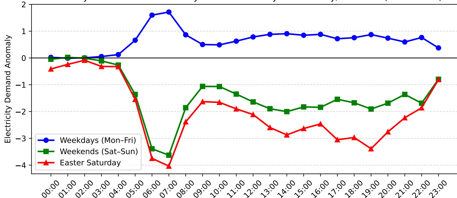
Dee Why West Demand Anomaly: Easter Saturday vs Weekday/Weekend (2009-2010)
