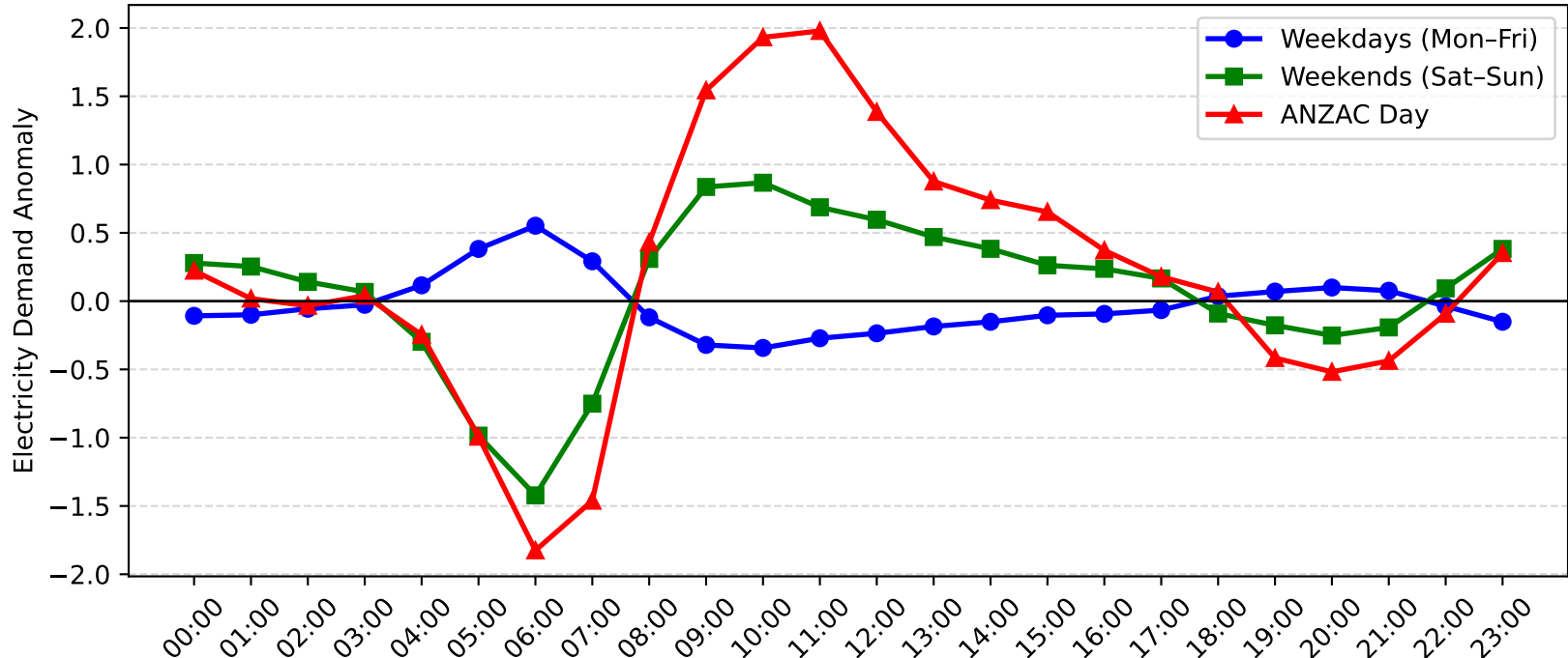
Umina Demand Anomaly: ANZAC Day vs Weekday/Weekend (2011-2012)
