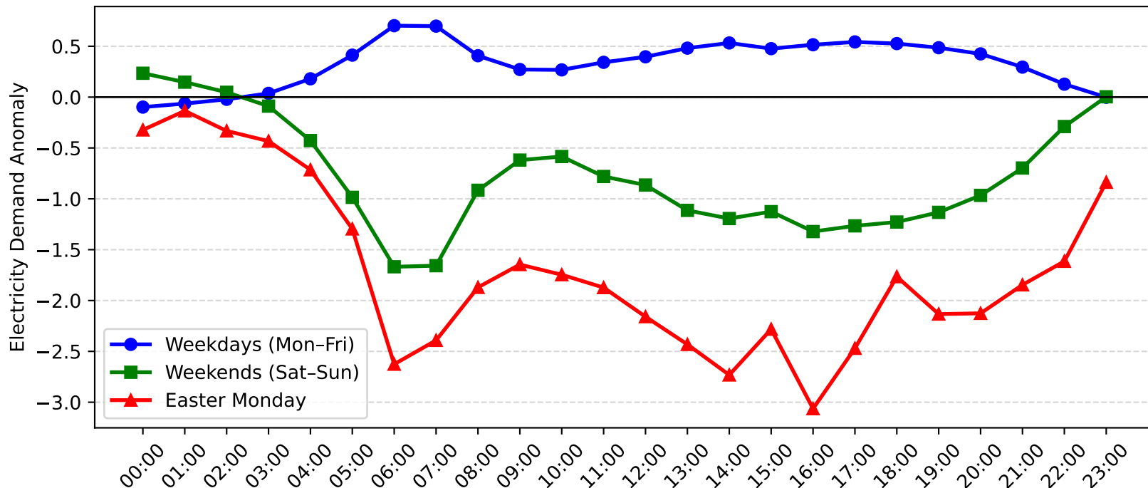
Charmhaven Demand Anomaly: Easter Monday vs Weekday/Weekend (2006-2007)
