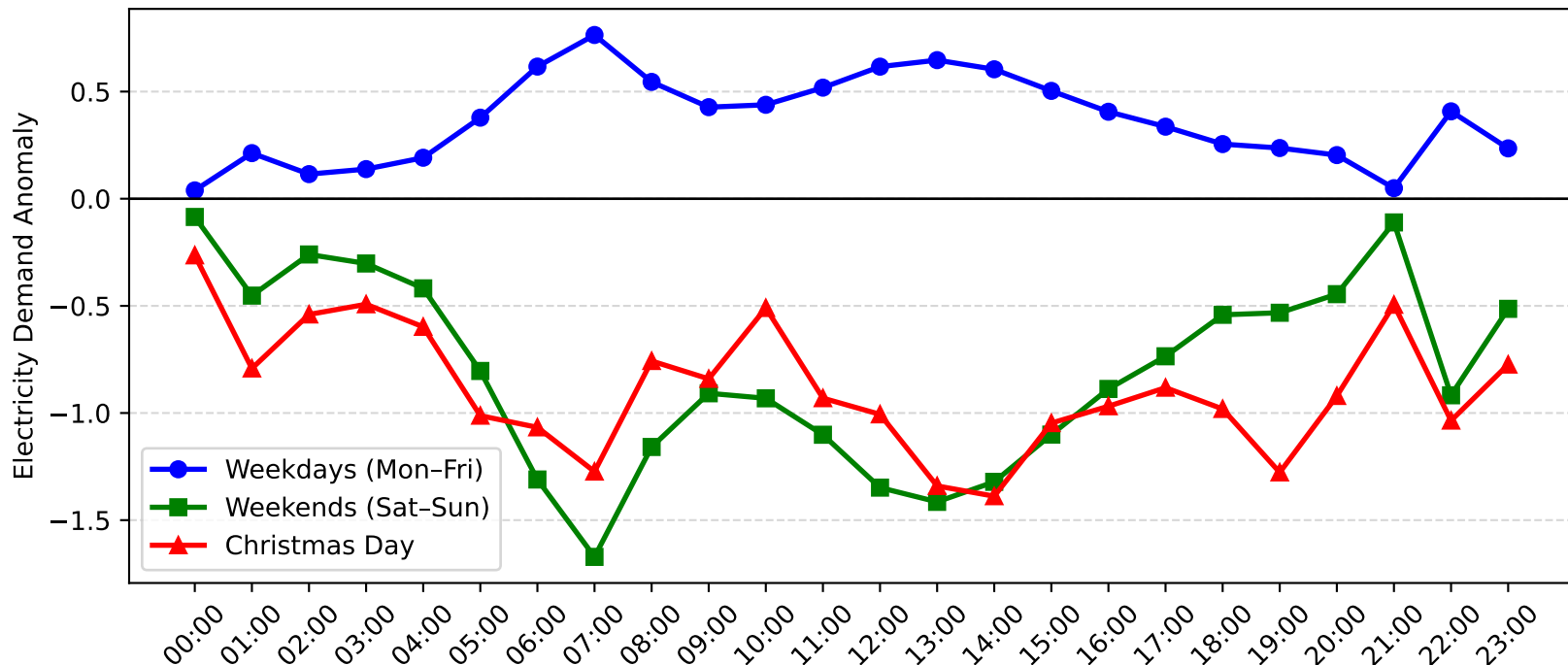
Cardiff Demand Anomaly: Christmas Day vs Weekday/Weekend (2010-2011)
