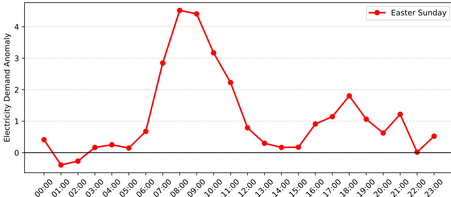
Nelson Bay Demand Anomaly: Easter Sunday (2015-2016)
