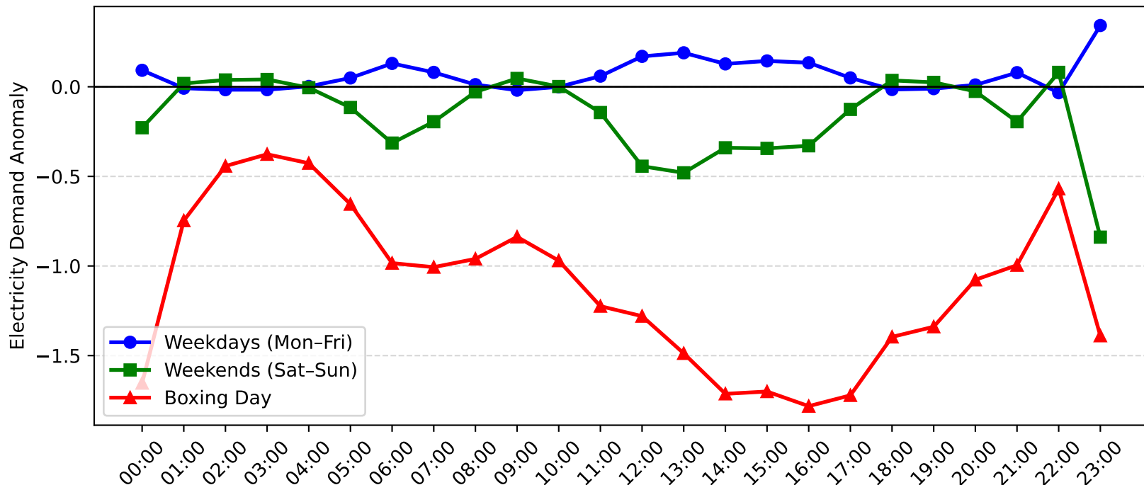
Telarah Demand Anomaly: Boxing Day vs Weekday/Weekend (2005-2006)
