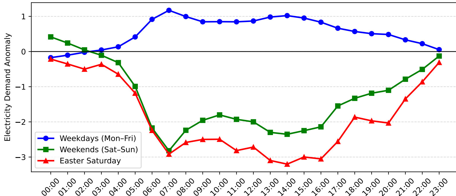
Rockdale Demand Anomaly: Easter Saturday vs Weekday/Weekend (2006-2007)
