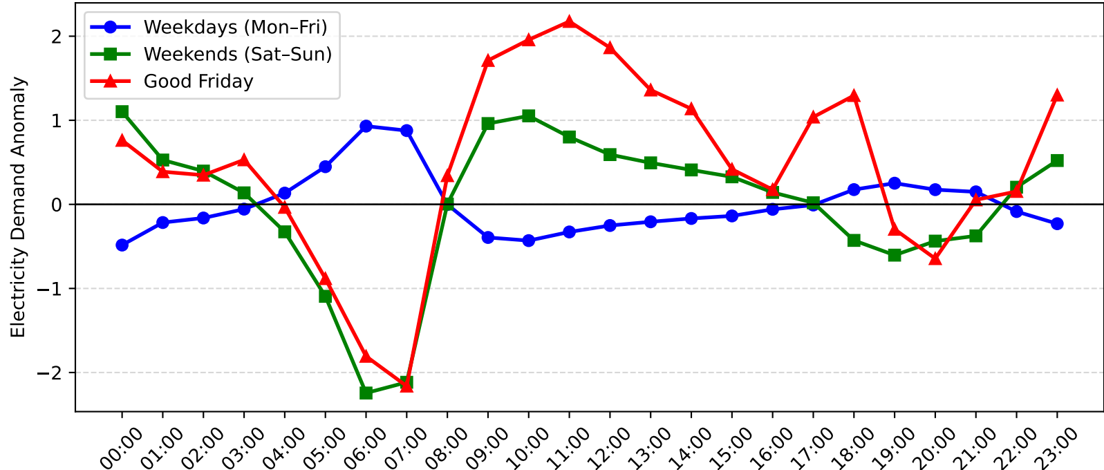
Avoca Demand Anomaly: Good Friday vs Weekday/Weekend (2008-2009)
