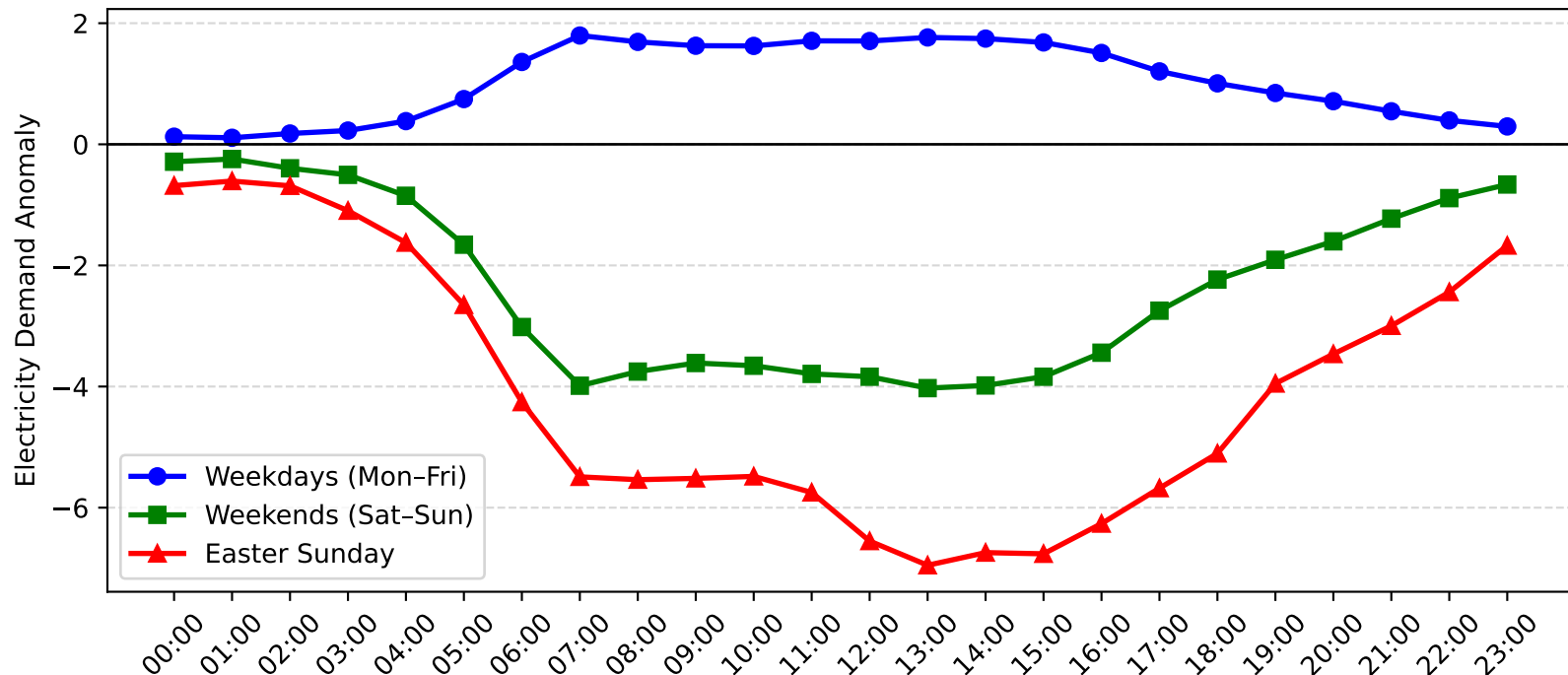
Sefton Demand Anomaly: Easter Sunday vs Weekday/Weekend (2016-2017)
