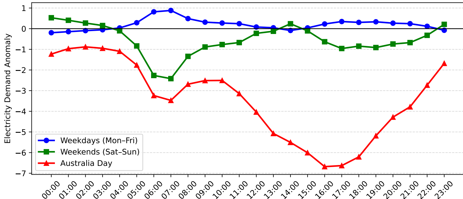
Revesby Demand Anomaly: Australia Day vs Weekday/Weekend (2016-2017)
