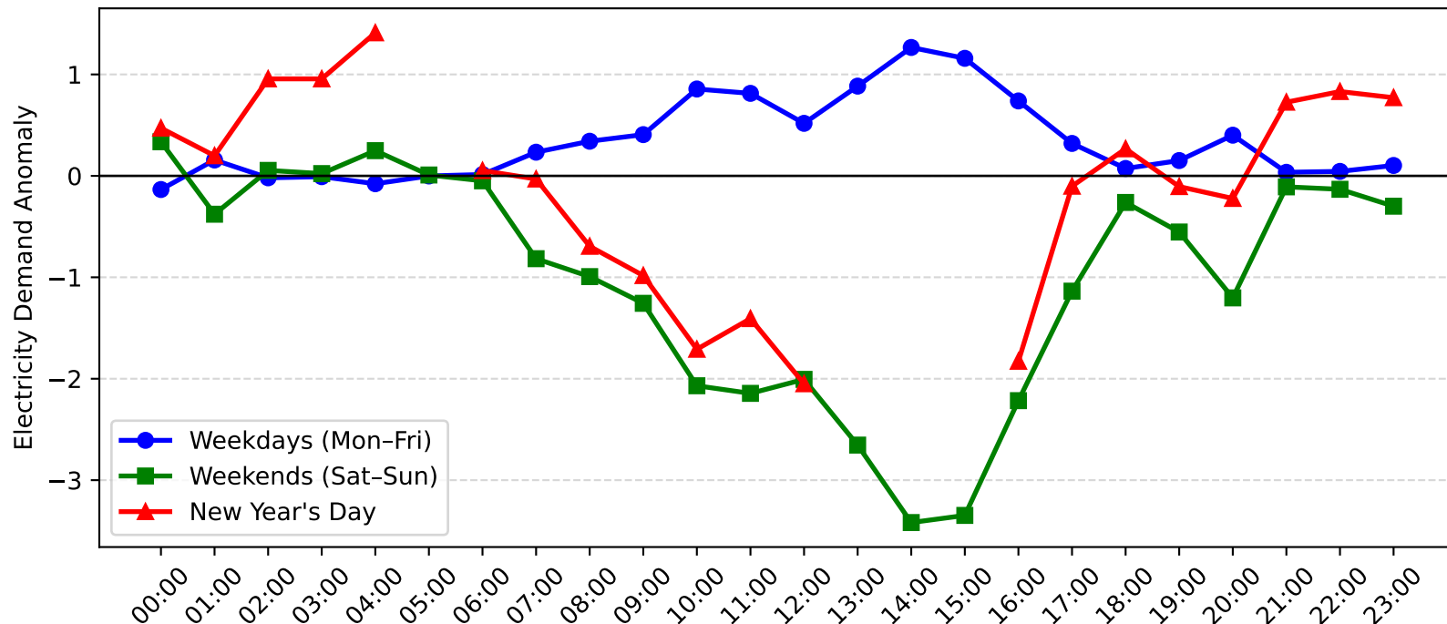
Kogarah Demand Anomaly: New Year's Day vs Weekday/Weekend (2009-2010)
