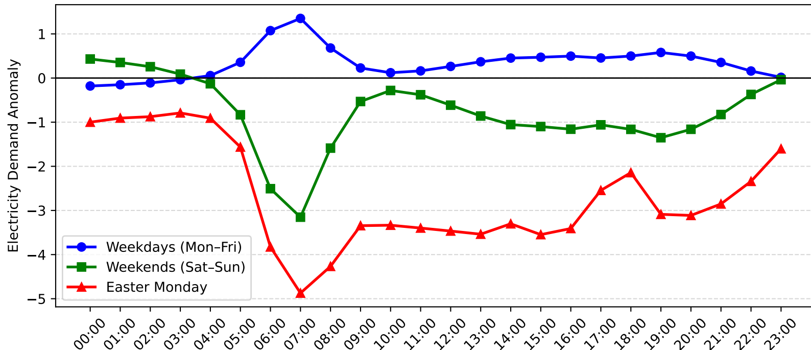
Five Dock Demand Anomaly: Easter Monday vs Weekday/Weekend (2014-2015)
