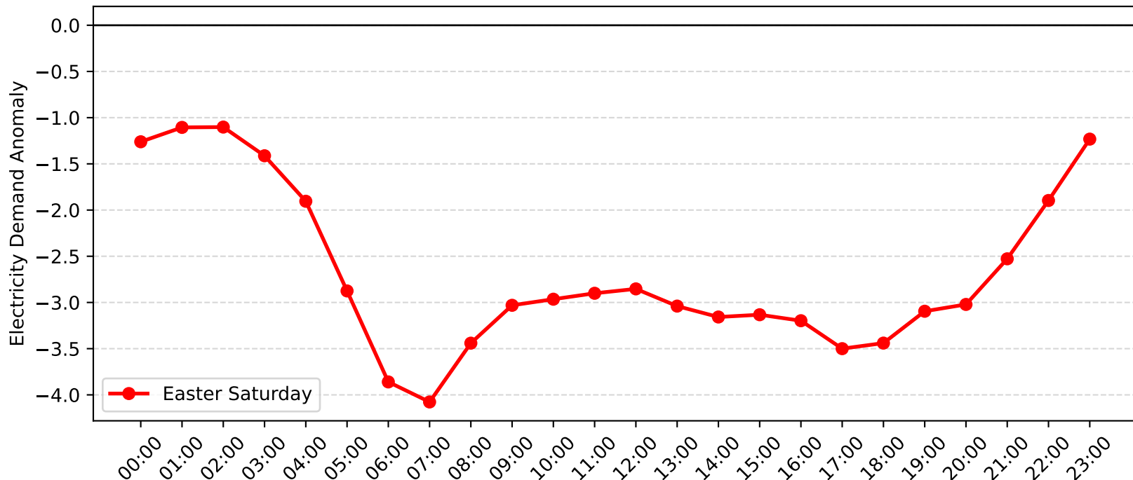
Lisarow Demand Anomaly: Easter Saturday (2010-2011)
