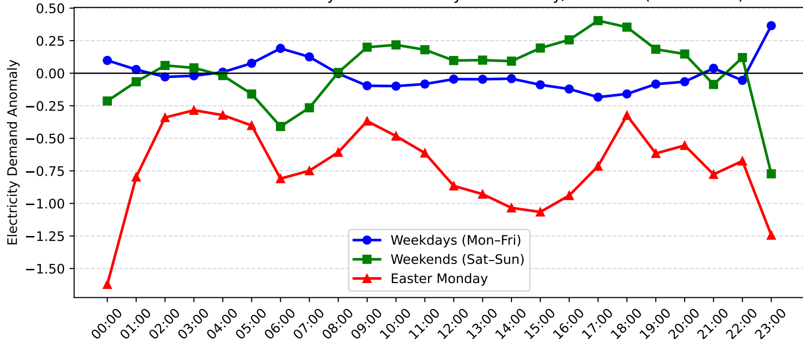
Telarah Demand Anomaly: Easter Monday vs Weekday/Weekend (2009-2010)
