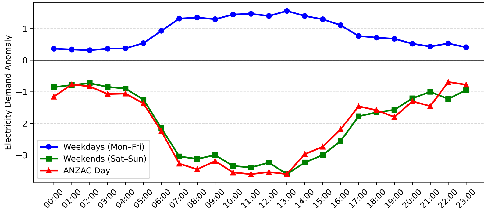
Mayfield West Demand Anomaly: ANZAC Day vs Weekday/Weekend (2016-2017)
