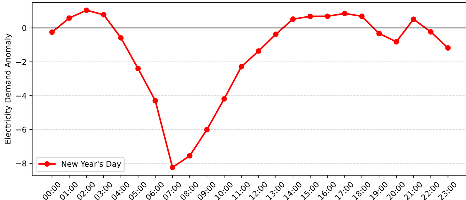
Meadowbank Demand Anomaly: New Year's Day (2011-2012)
