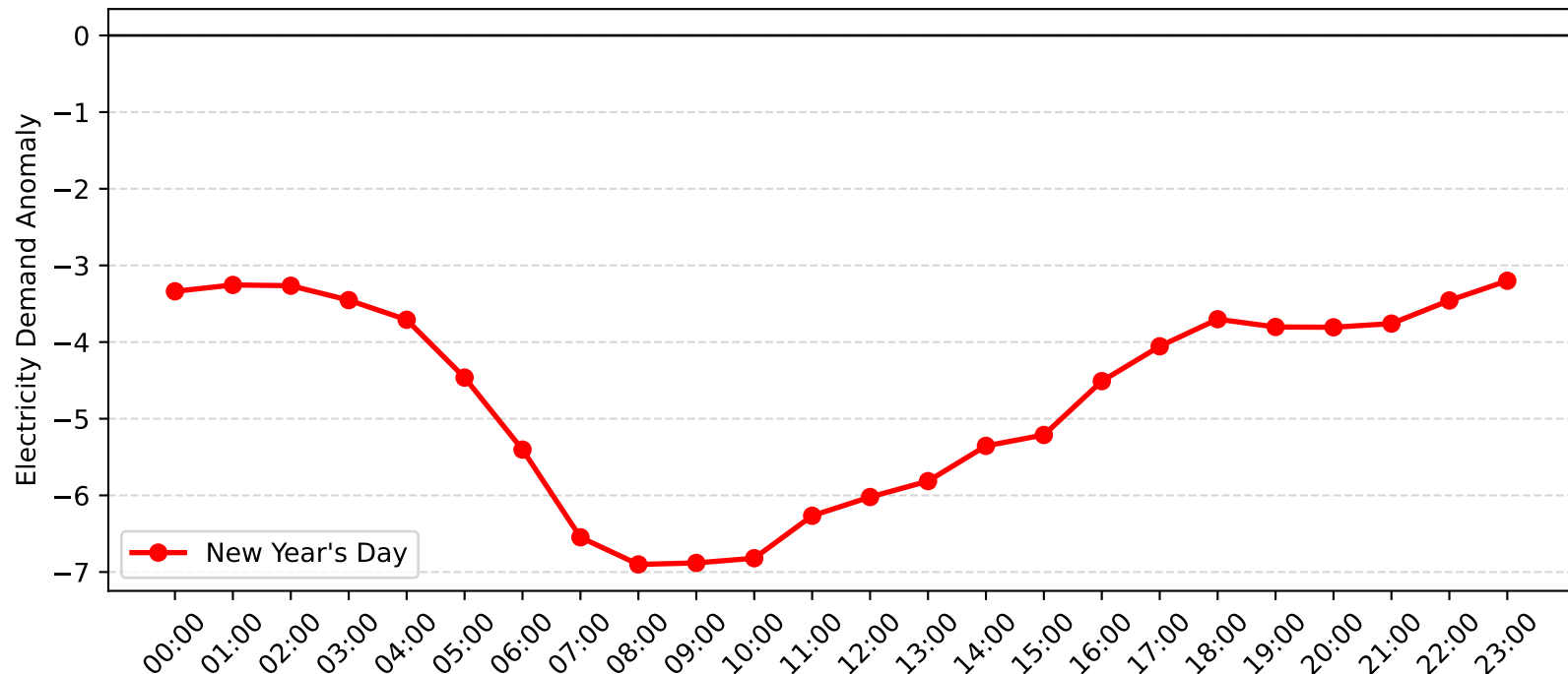
Leightonfield Demand Anomaly: New Year's Day (2010-2011)
