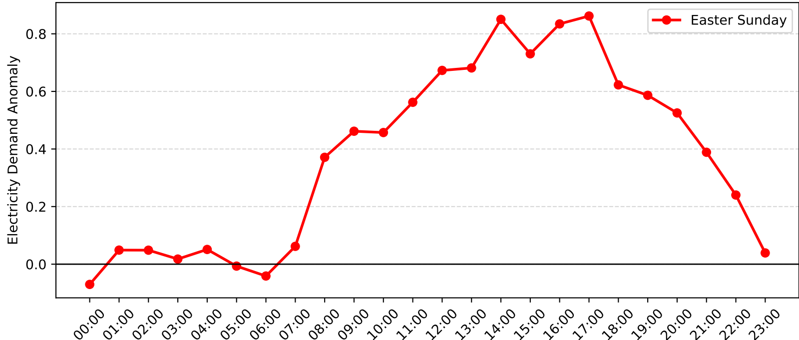
Rothbury Demand Anomaly: Easter Sunday (2011-2012)
