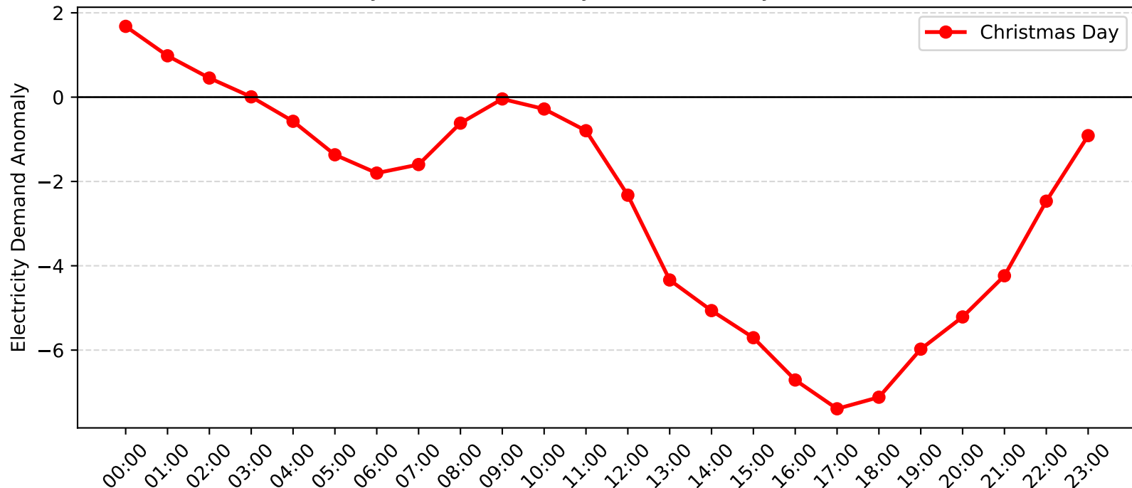
Revesby Demand Anomaly: Christmas Day (2012-2013)
