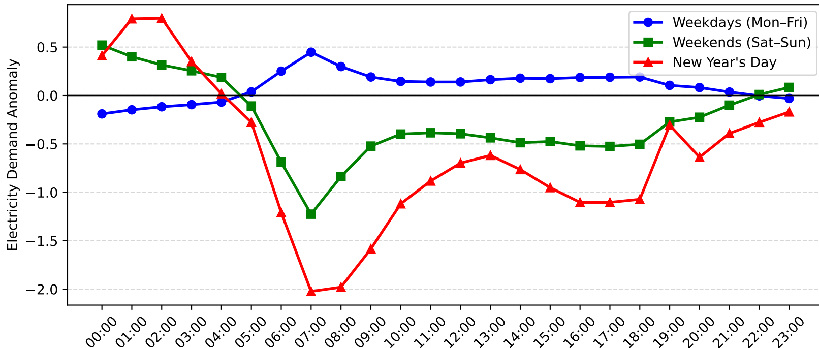
Blakehurst Demand Anomaly: New Year's Day vs Weekday/Weekend (2013-2014)
