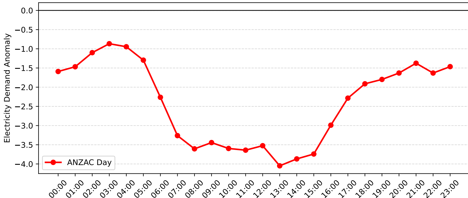
Mayfield West Demand Anomaly: ANZAC Day (2009-2010)
