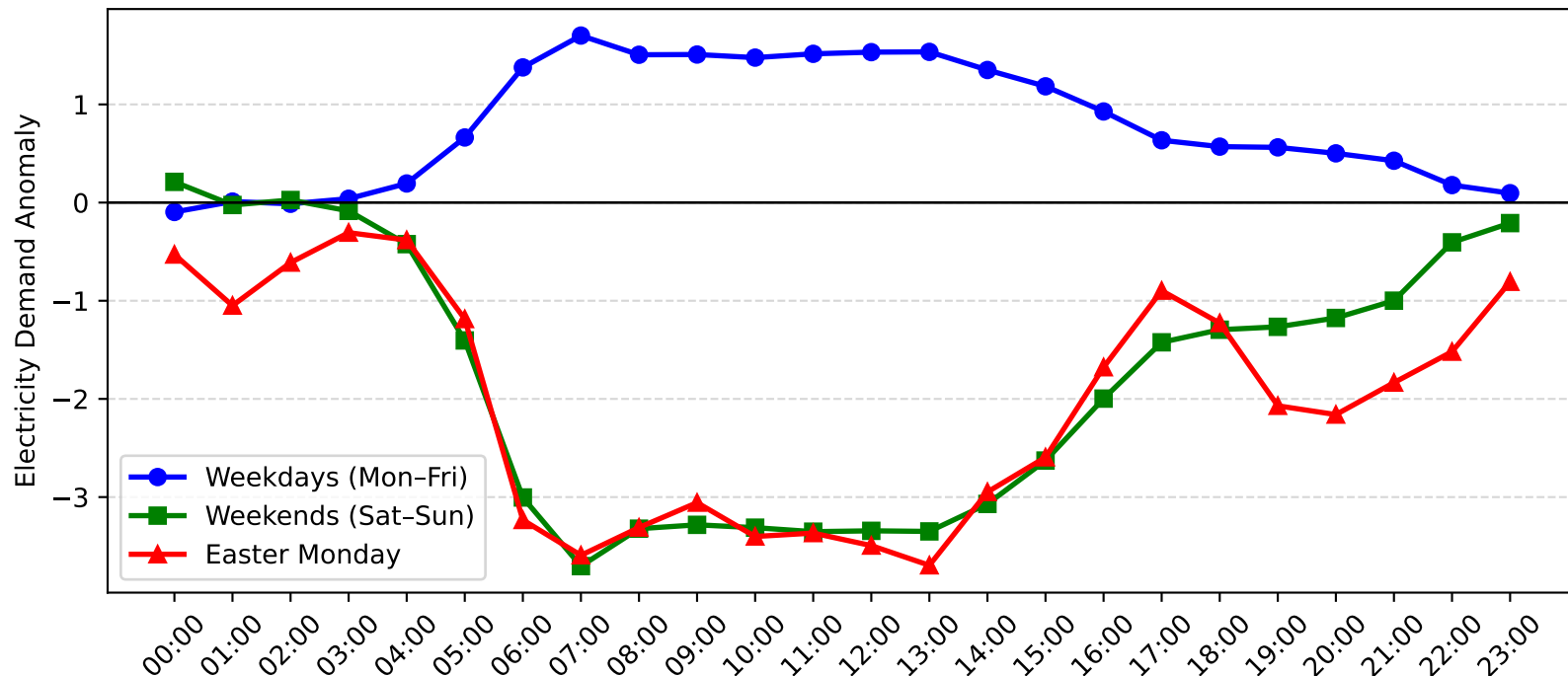
Wyong Demand Anomaly: Easter Monday vs Weekday/Weekend (2009-2010)
