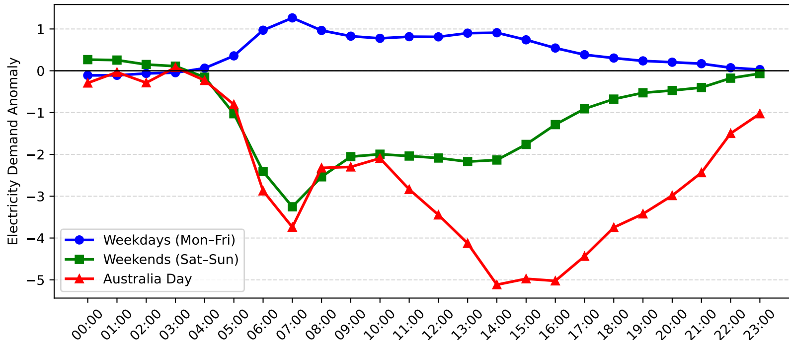
Kirrawee Demand Anomaly: Australia Day vs Weekday/Weekend (2014-2015)
