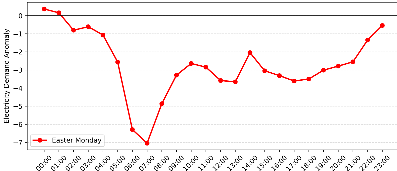
Pennant Hills Demand Anomaly: Easter Monday (2013-2014)
