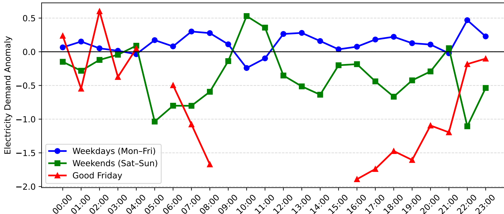
Adamstown Demand Anomaly: Good Friday vs Weekday/Weekend (2017-2018)
