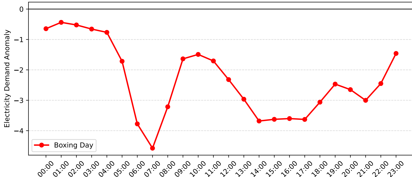
Dee Why West Demand Anomaly: Boxing Day (2009-2010)
