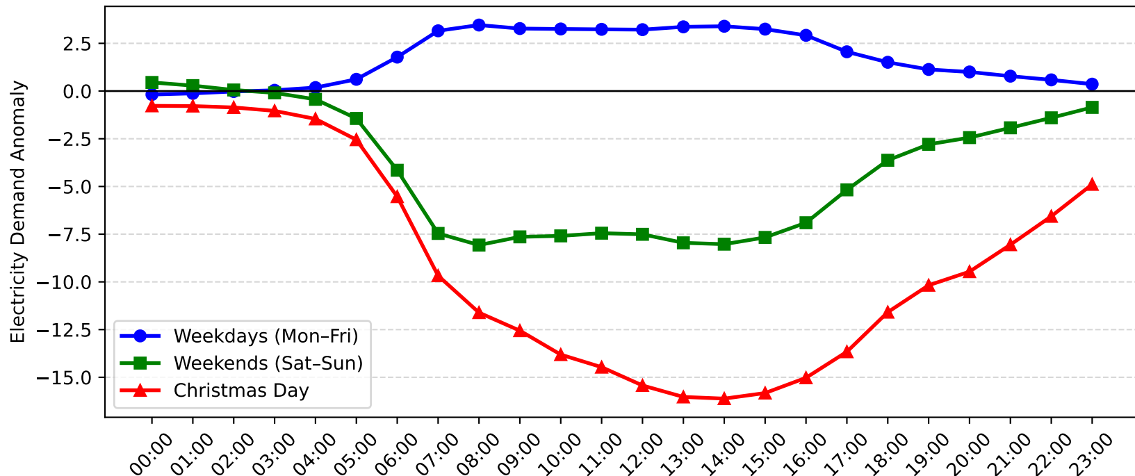
St. Peters Demand Anomaly: Christmas Day vs Weekday/Weekend (2011-2012)
