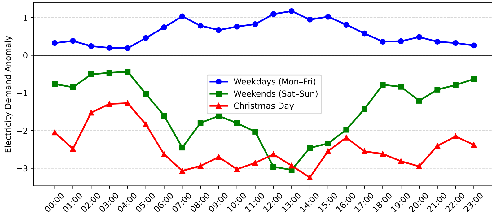
Rutherford Demand Anomaly: Christmas Day vs Weekday/Weekend (2004-2005)
