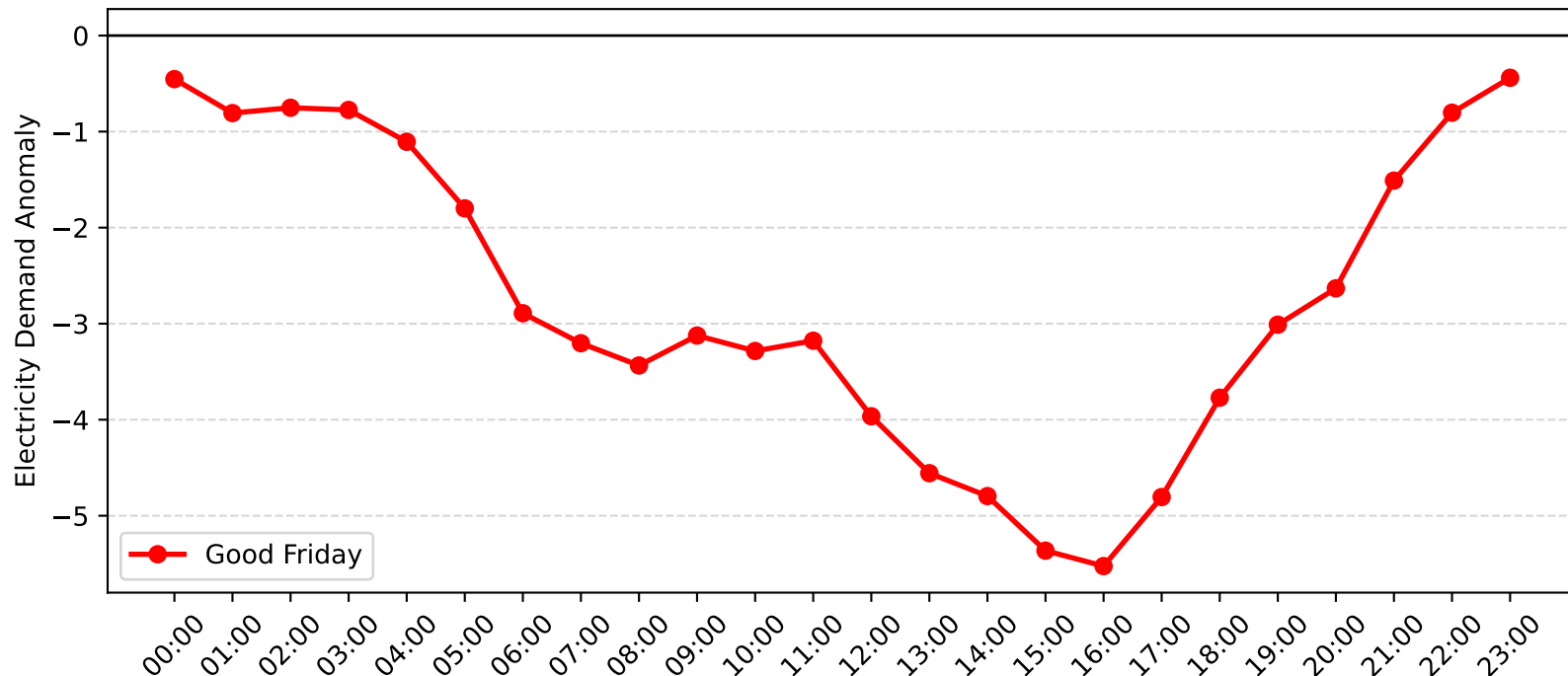
Charmhaven Demand Anomaly: Good Friday (2016-2017)
