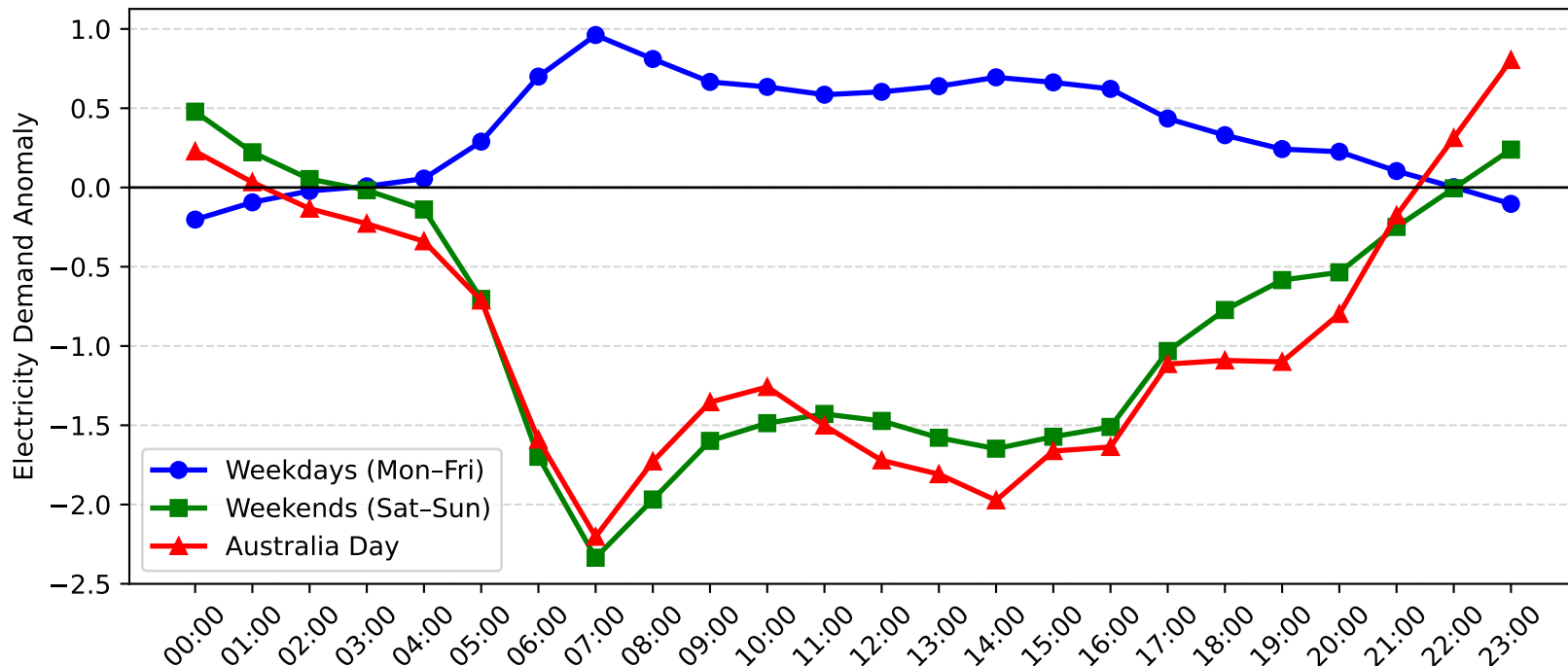
Rockdale Demand Anomaly: Australia Day vs Weekday/Weekend (2007-2008)
