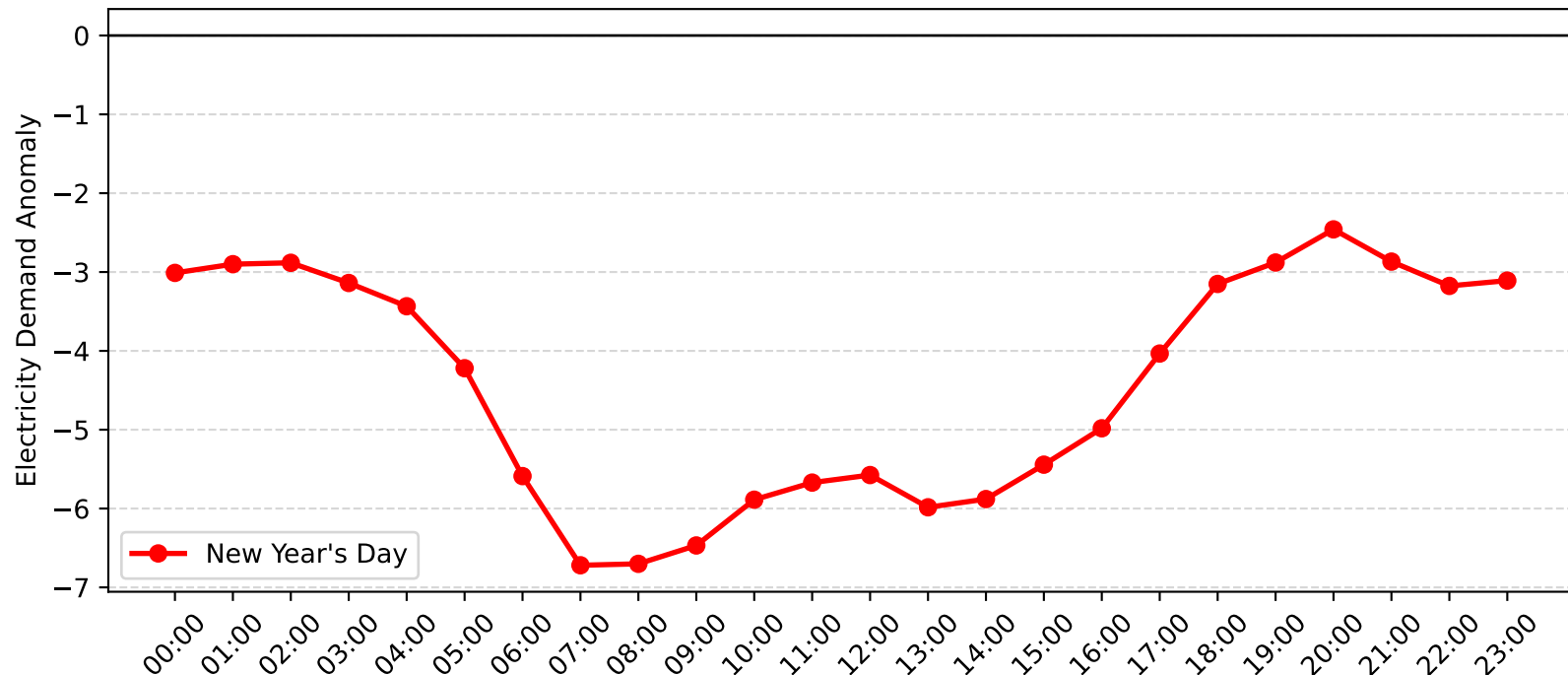
Leightonfield Demand Anomaly: New Year's Day (2006-2007)
