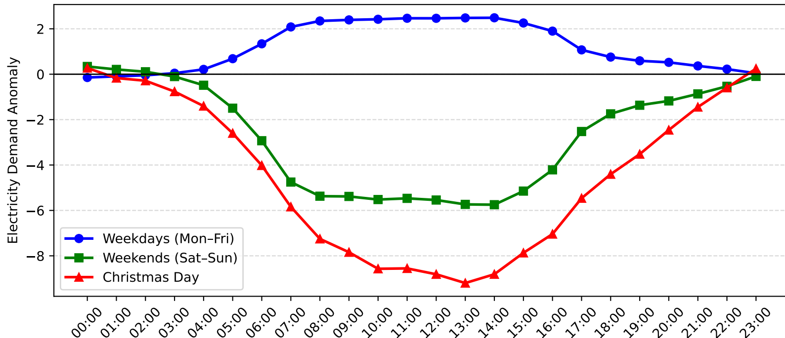
West Gosford Demand Anomaly: Christmas Day vs Weekday/Weekend (2010-2011)
