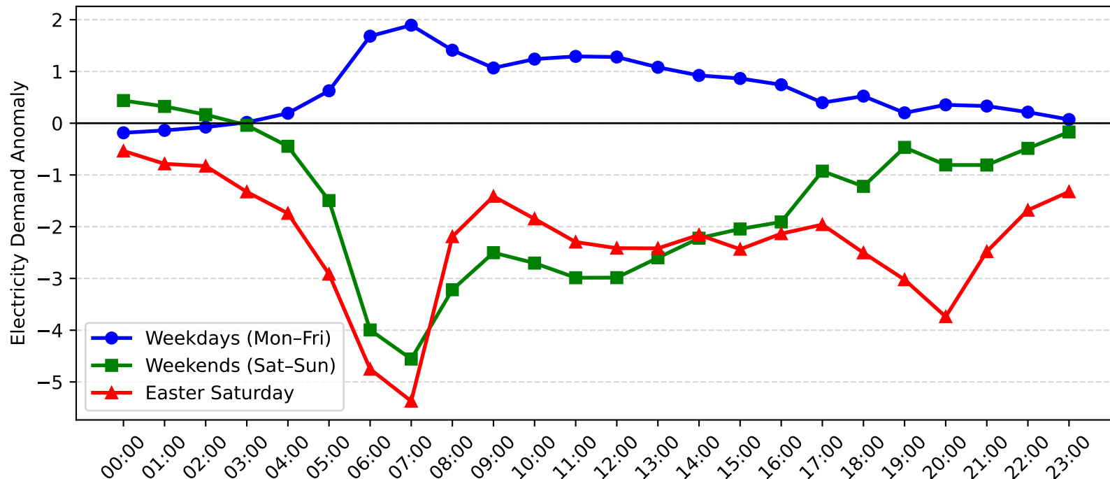
Meadowbank Demand Anomaly: Easter Saturday vs Weekday/Weekend (2006-2007)
