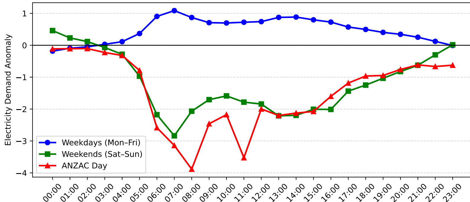
Rockdale Demand Anomaly: ANZAC Day vs Weekday/Weekend (2005-2006)
