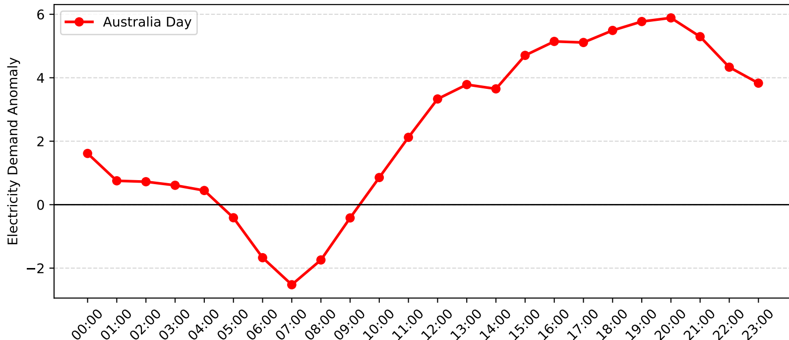
Rutherford Demand Anomaly: Australia Day (2010-2011)
