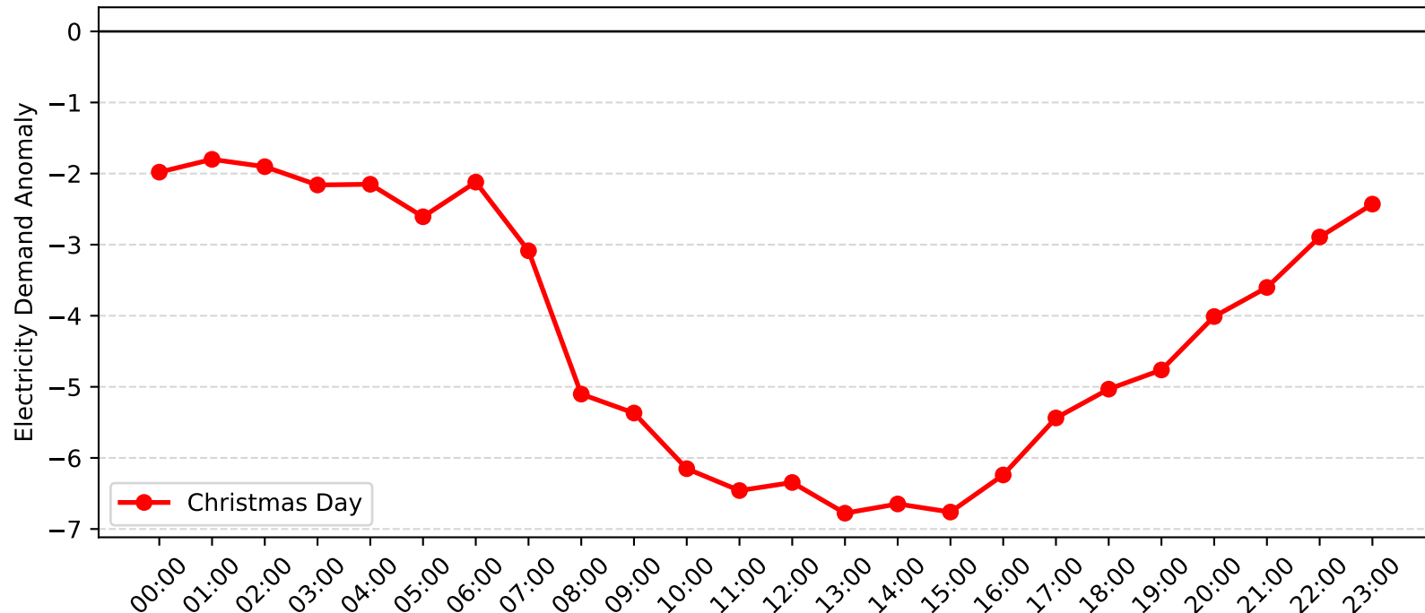
Mayfield West Demand Anomaly: Christmas Day (2014-2015)
