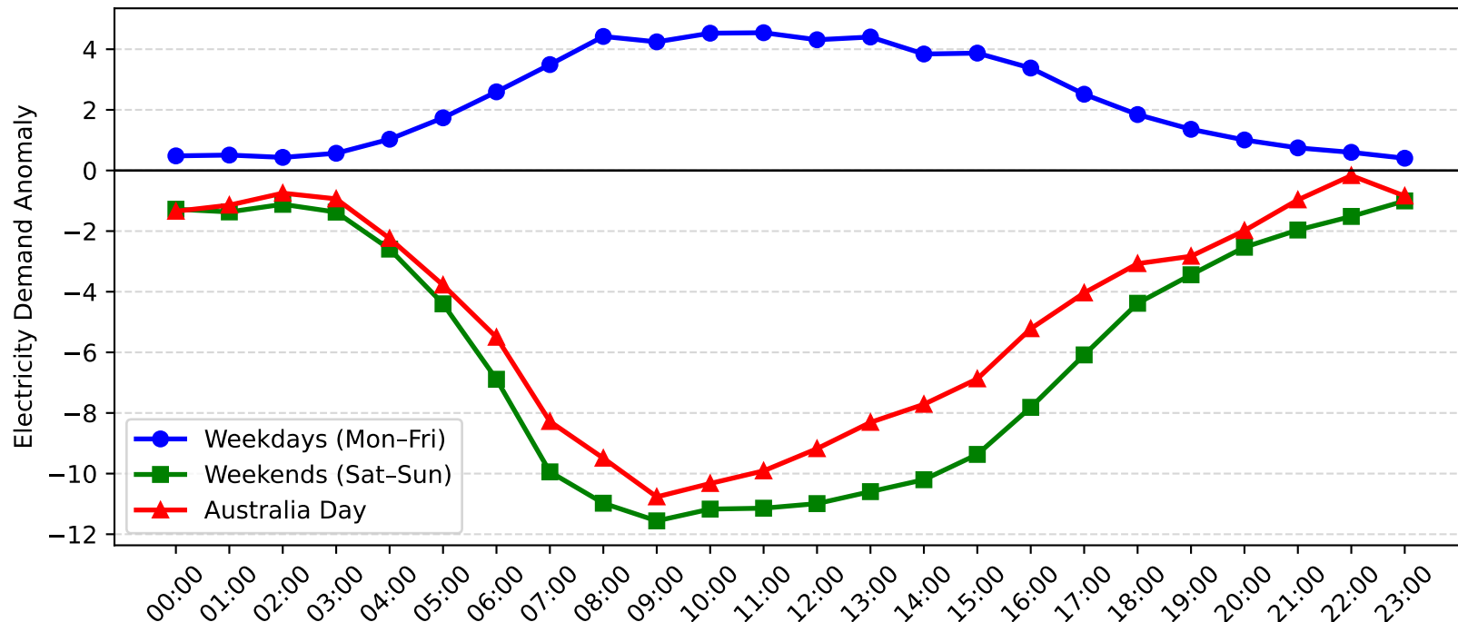
Homebush Bay Demand Anomaly: Australia Day vs Weekday/Weekend (2009-2010)
