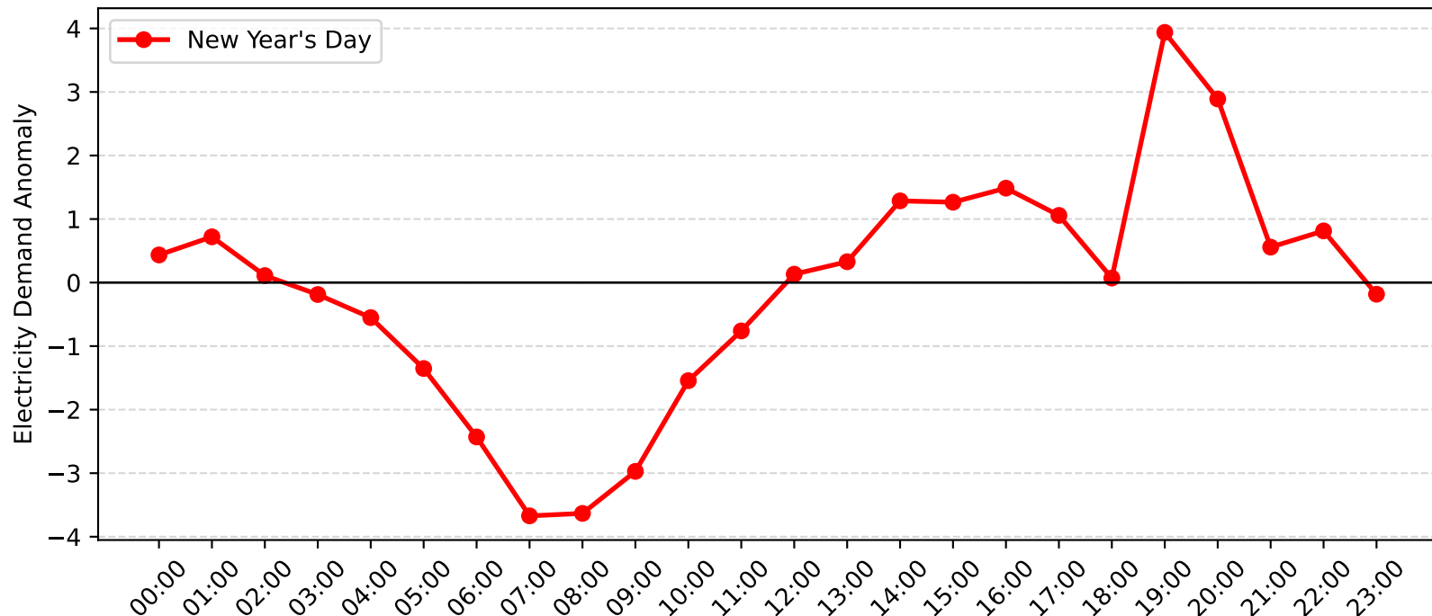
Charmhaven Demand Anomaly: New Year's Day (2008-2009)
