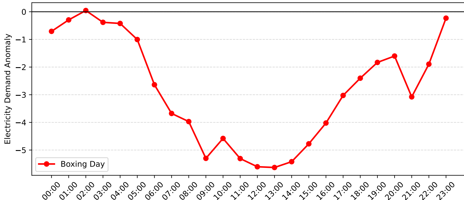
Wyong Demand Anomaly: Boxing Day (2008-2009)
