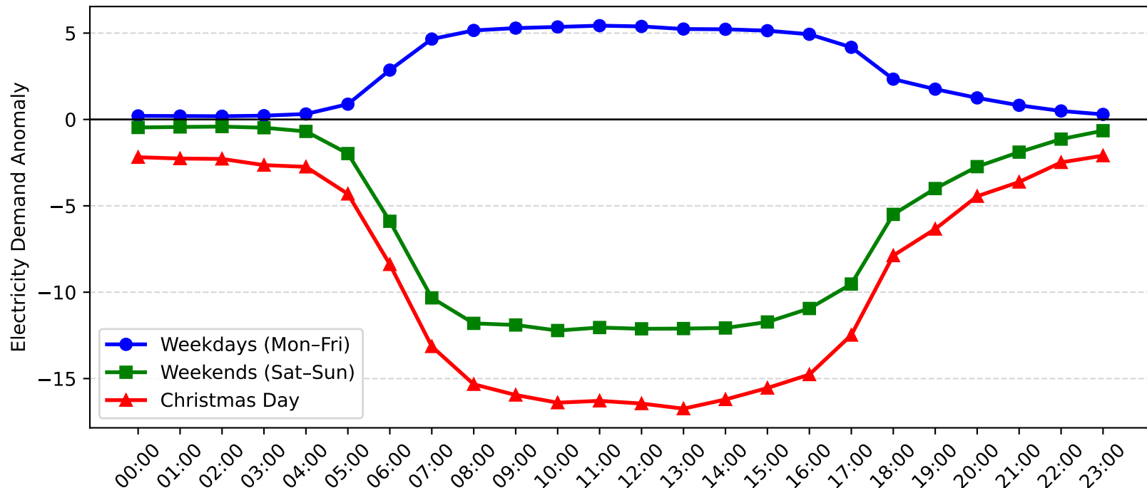
Macquarie Park Demand Anomaly: Christmas Day vs Weekday/Weekend (2010-2011)
