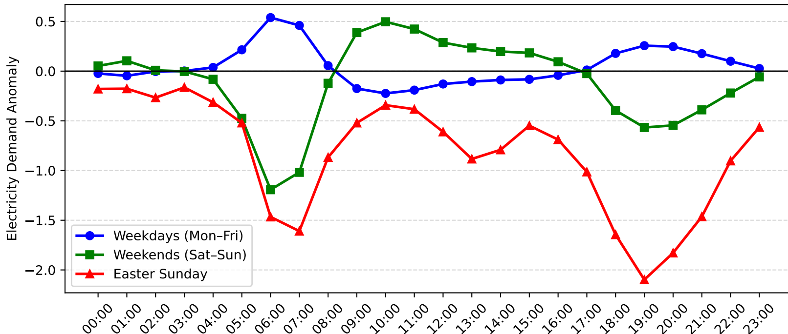
Harbord Demand Anomaly: Easter Sunday vs Weekday/Weekend (2017-2018)
