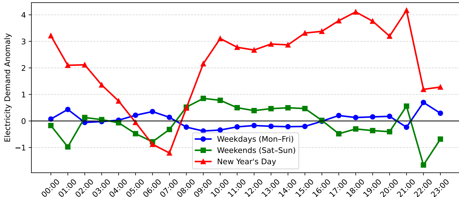
Nelson Bay Demand Anomaly: New Year's Day vs Weekday/Weekend (2011-2012)
