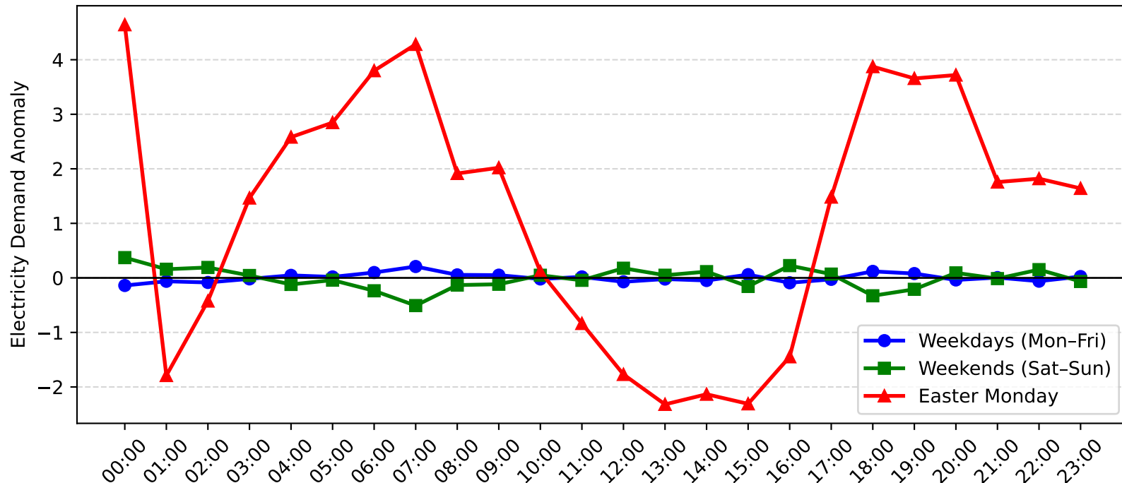
Charmhaven Demand Anomaly: Easter Monday vs Weekday/Weekend (2004-2005)
