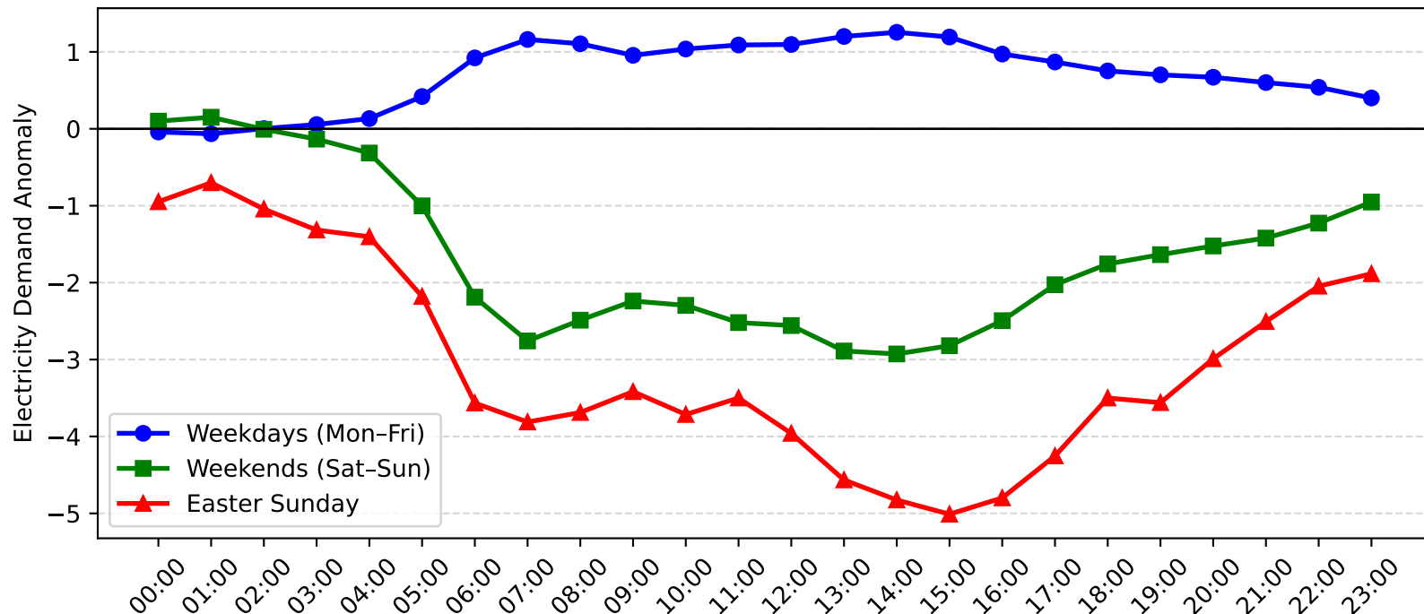
Bass Hill Demand Anomaly: Easter Sunday vs Weekday/Weekend (2006-2007)
