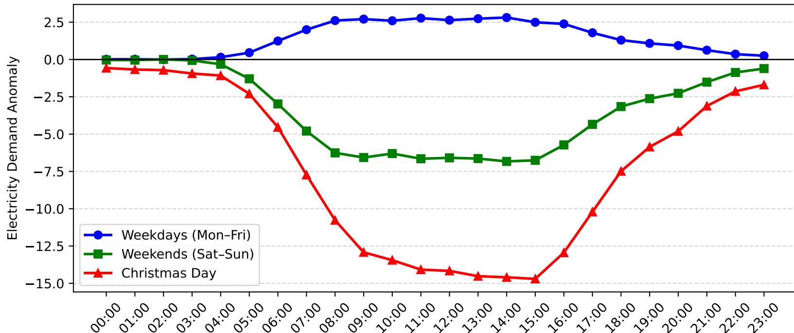
Brookvale Demand Anomaly: Christmas Day vs Weekday/Weekend (2015-2016)
