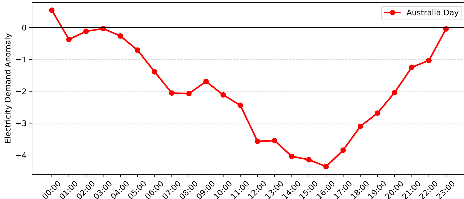
Erina Demand Anomaly: Australia Day (2008-2009)
