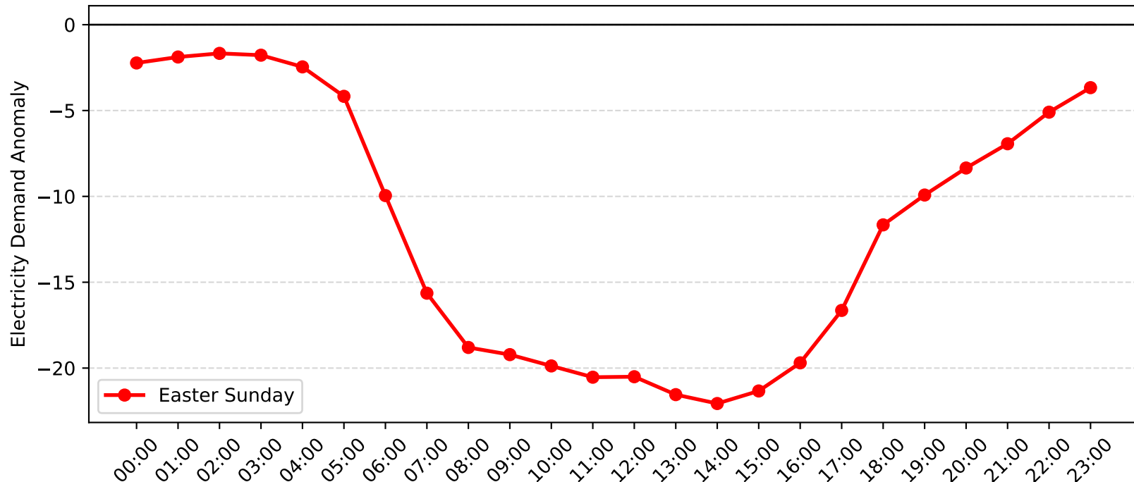
Gore Hill Demand Anomaly: Easter Sunday (2006-2007)
