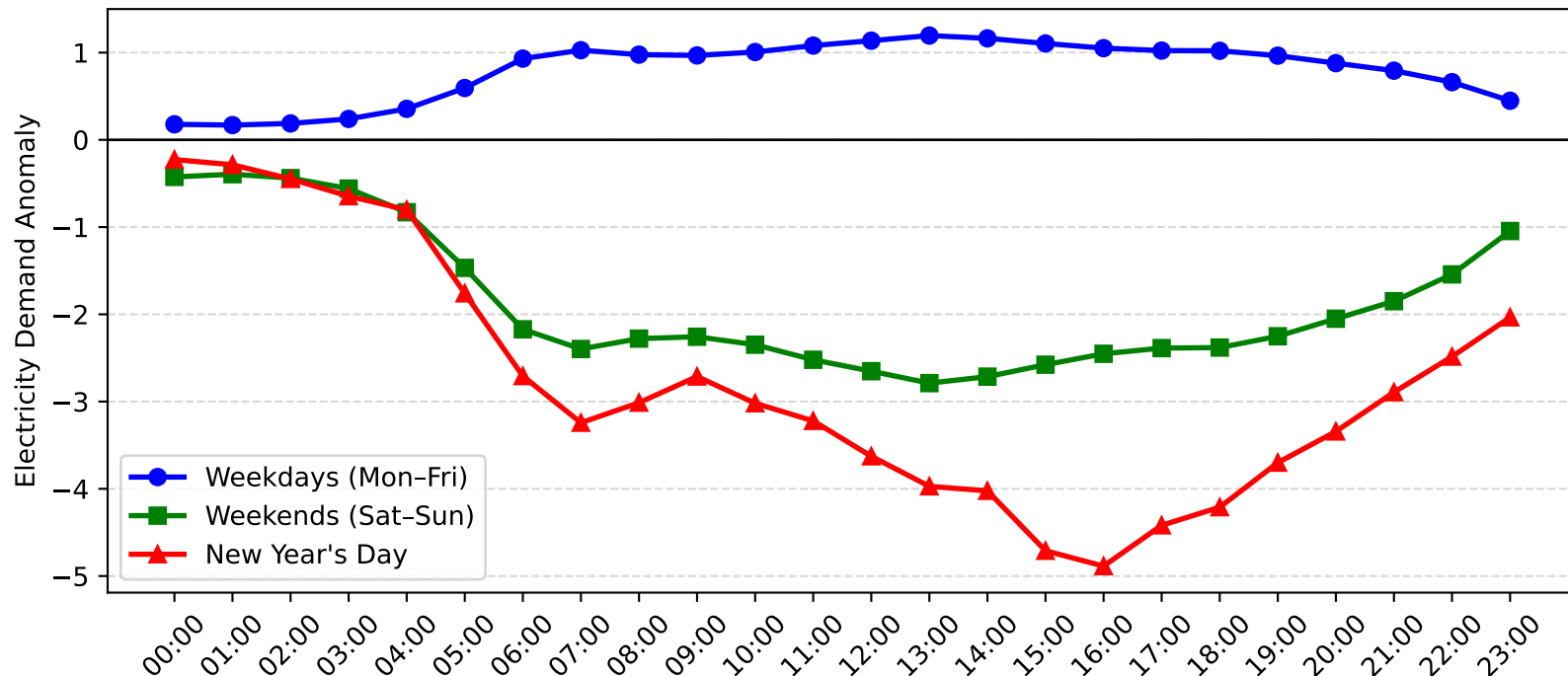
Lisarow Demand Anomaly: New Year's Day vs Weekday/Weekend (2017-2018)
