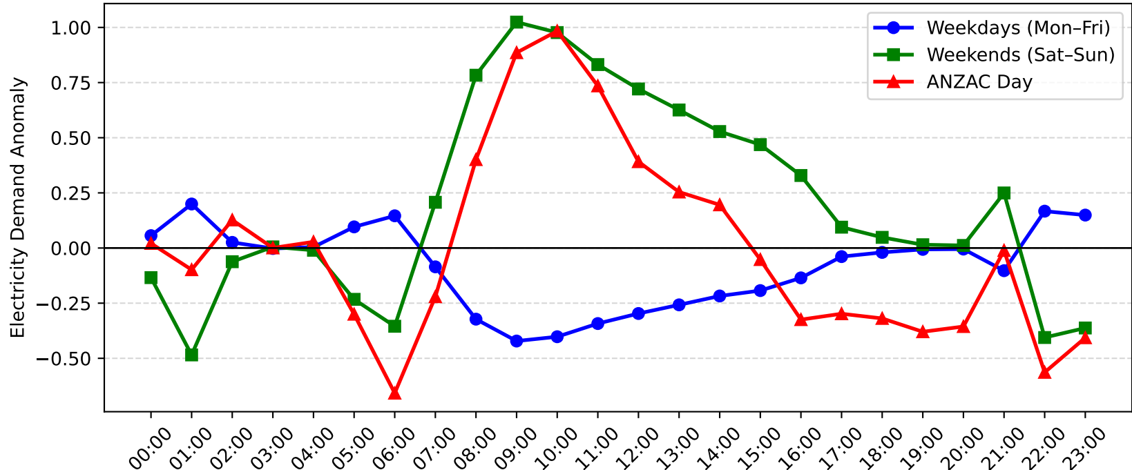
Swansea Demand Anomaly: ANZAC Day vs Weekday/Weekend (2014-2015)
