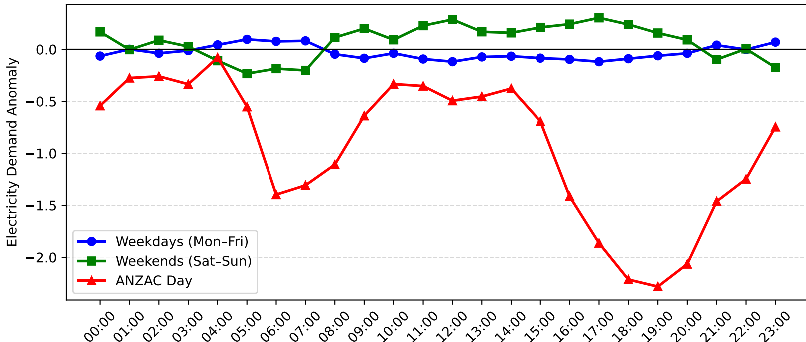
Umina Demand Anomaly: ANZAC Day vs Weekday/Weekend (2004-2005)
