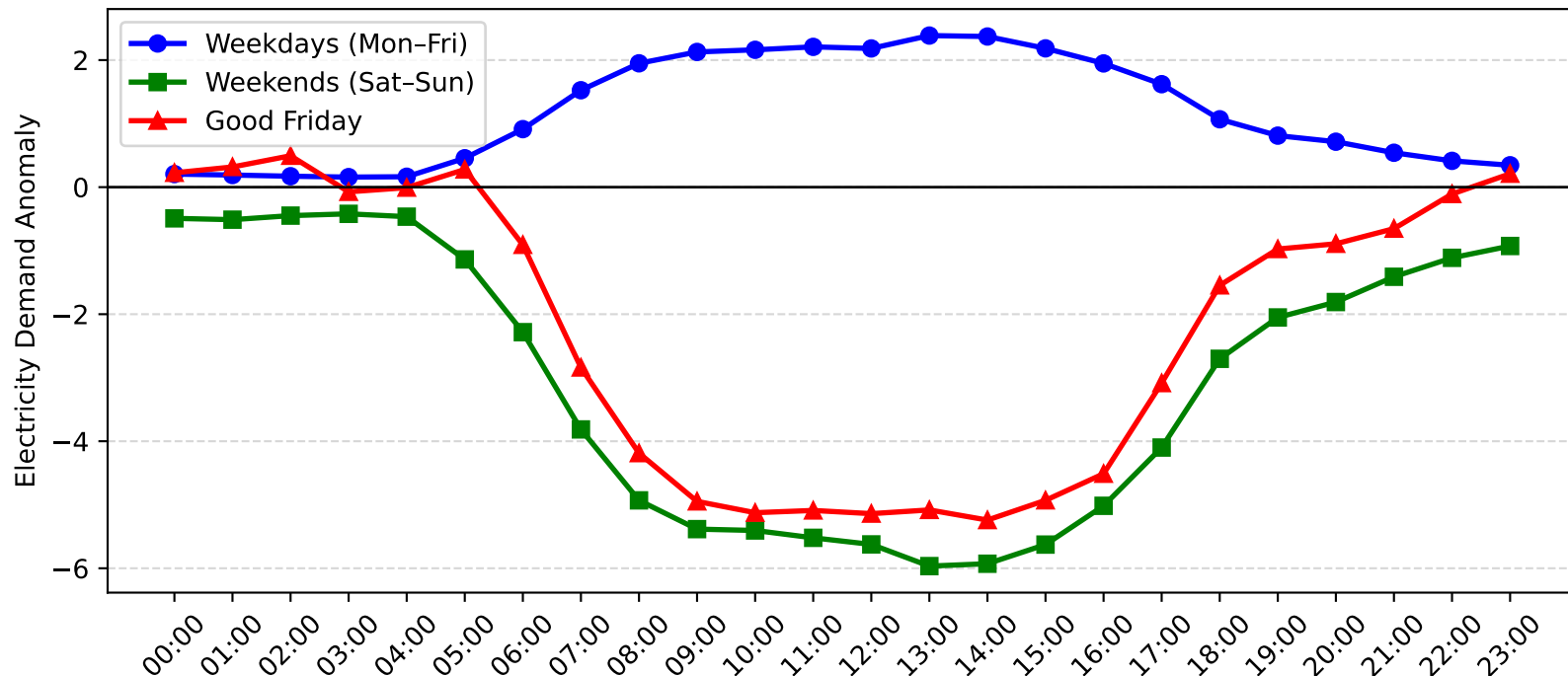
Green Square Demand Anomaly: Good Friday vs Weekday/Weekend (2011-2012)
