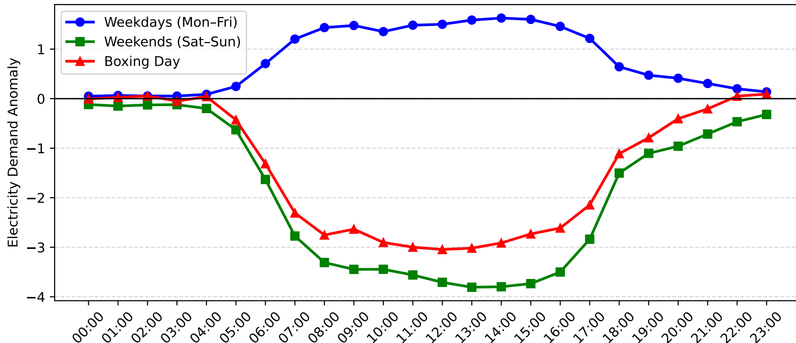
Beacon Hill Demand Anomaly: Boxing Day vs Weekday/Weekend (2015-2016)
