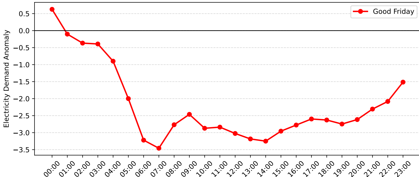
Lisarow Demand Anomaly: Good Friday (2017-2018)
