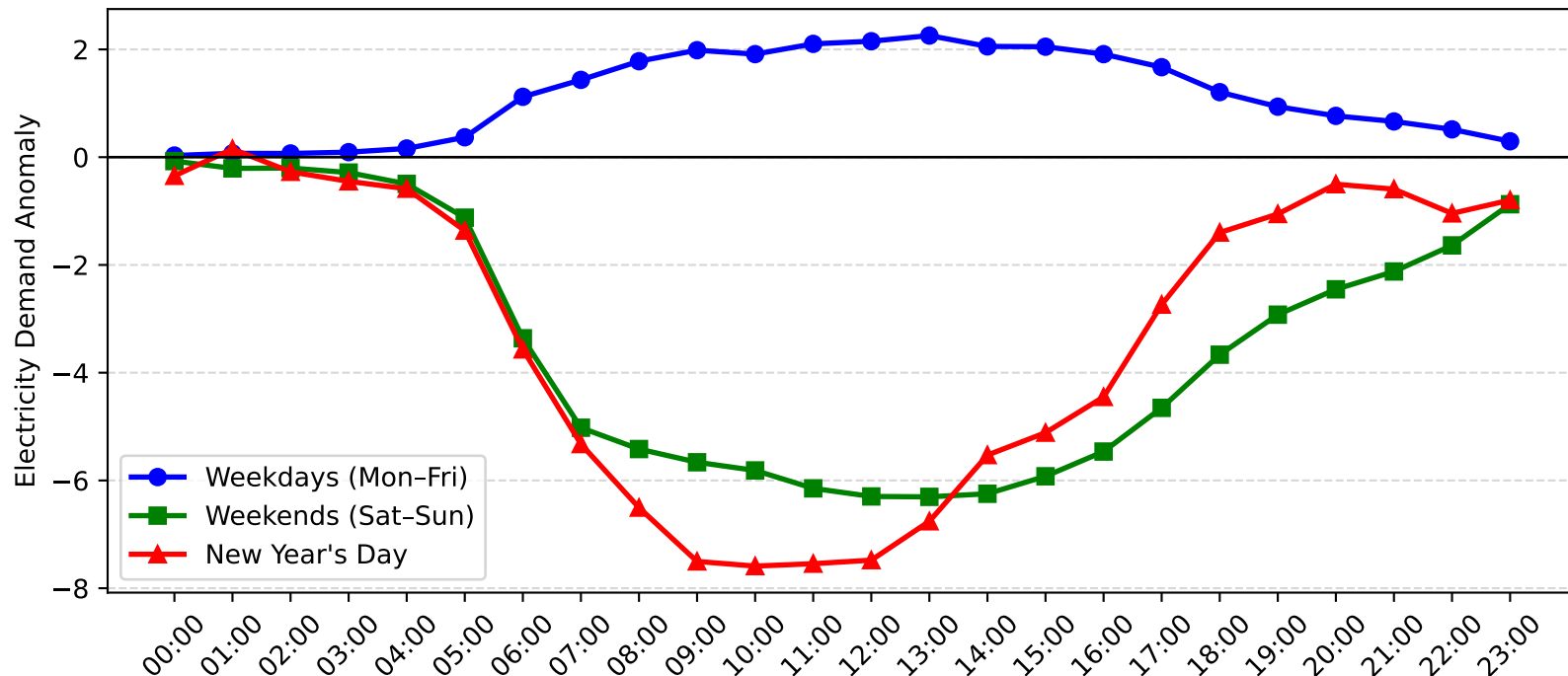
Concord Demand Anomaly: New Year's Day vs Weekday/Weekend (2009-2010)
