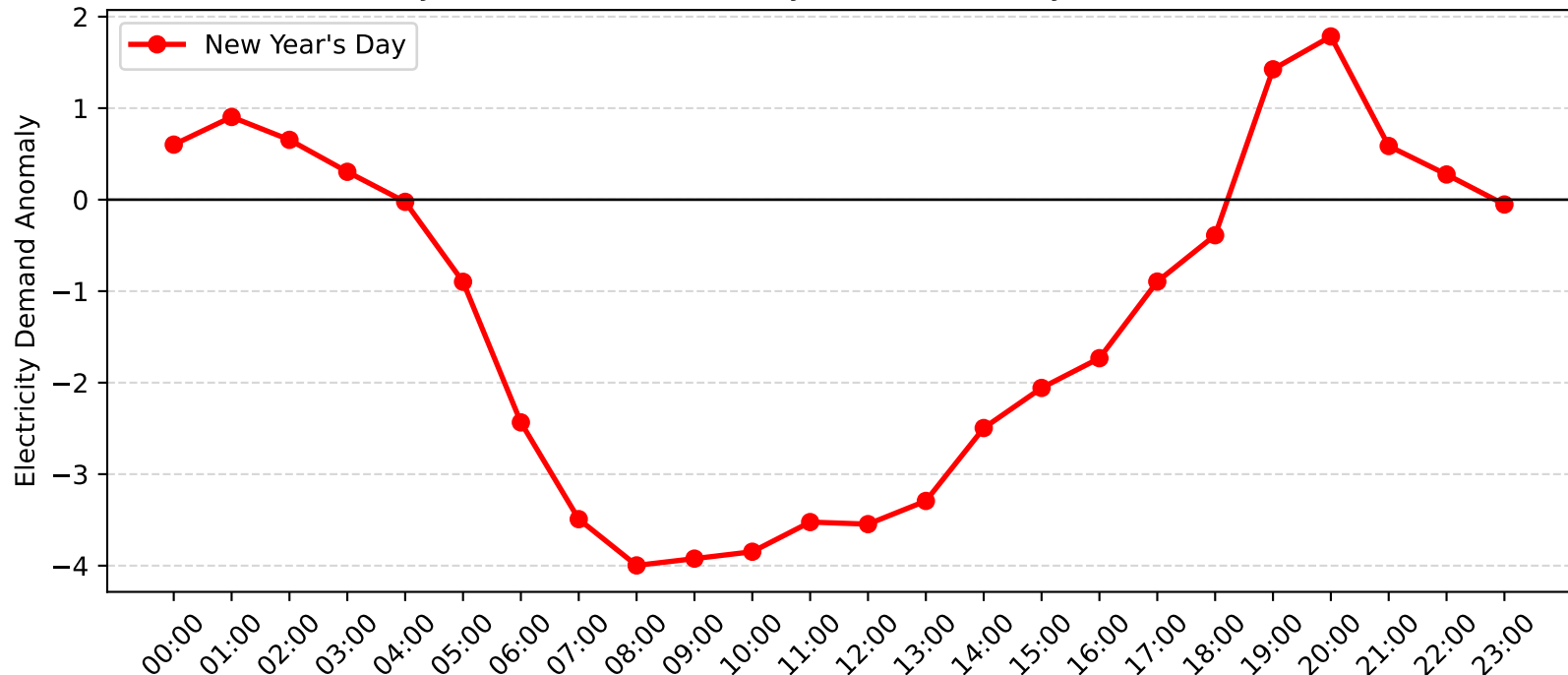
Pymble Demand Anomaly: New Year's Day (2008-2009)
