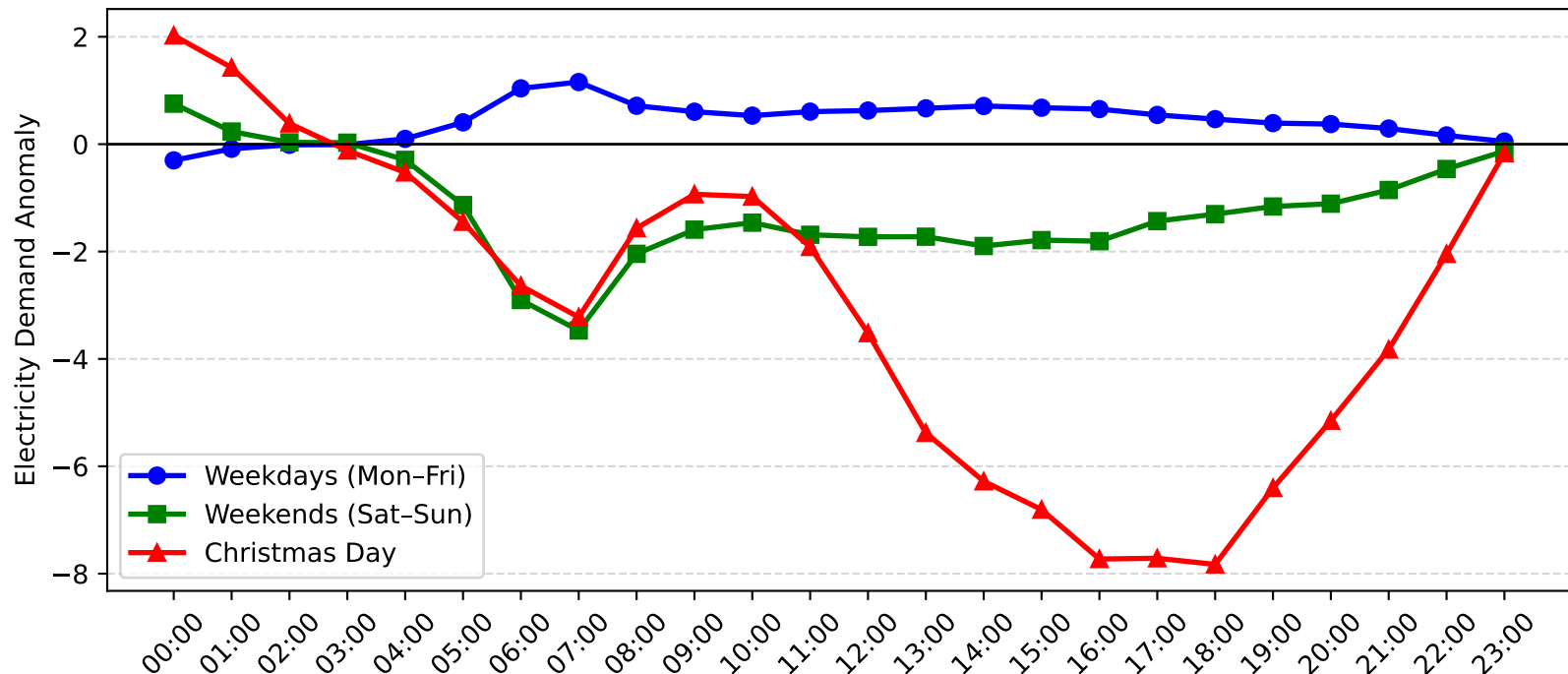
Mortdale Demand Anomaly: Christmas Day vs Weekday/Weekend (2007-2008)
