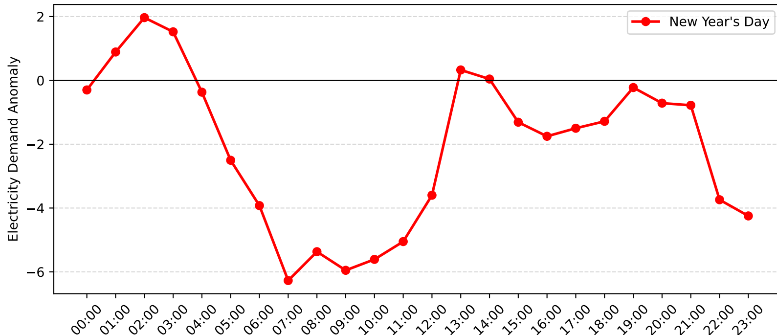
Meadowbank Demand Anomaly: New Year's Day (2014-2015)
