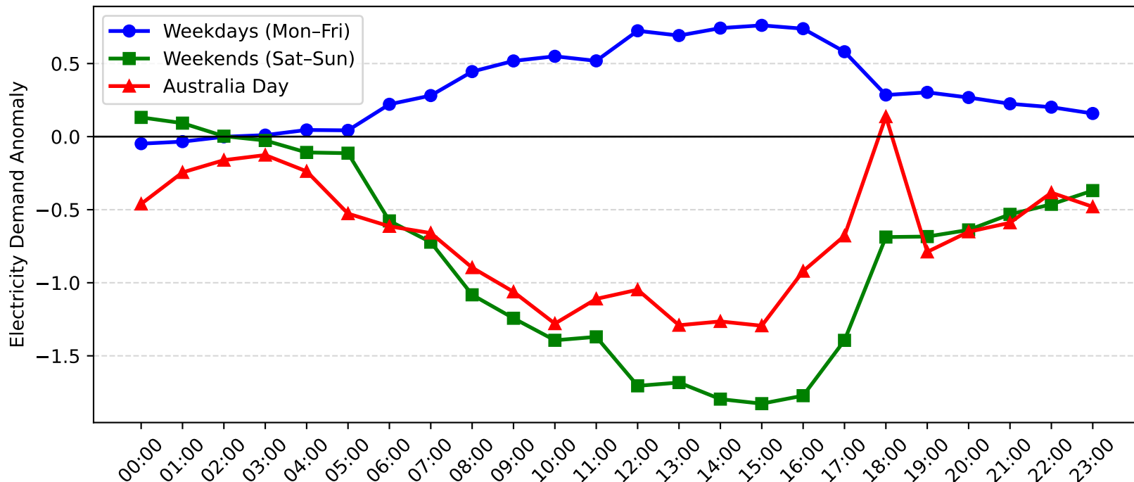
Lidcombe Demand Anomaly: Australia Day vs Weekday/Weekend (2004-2005)
