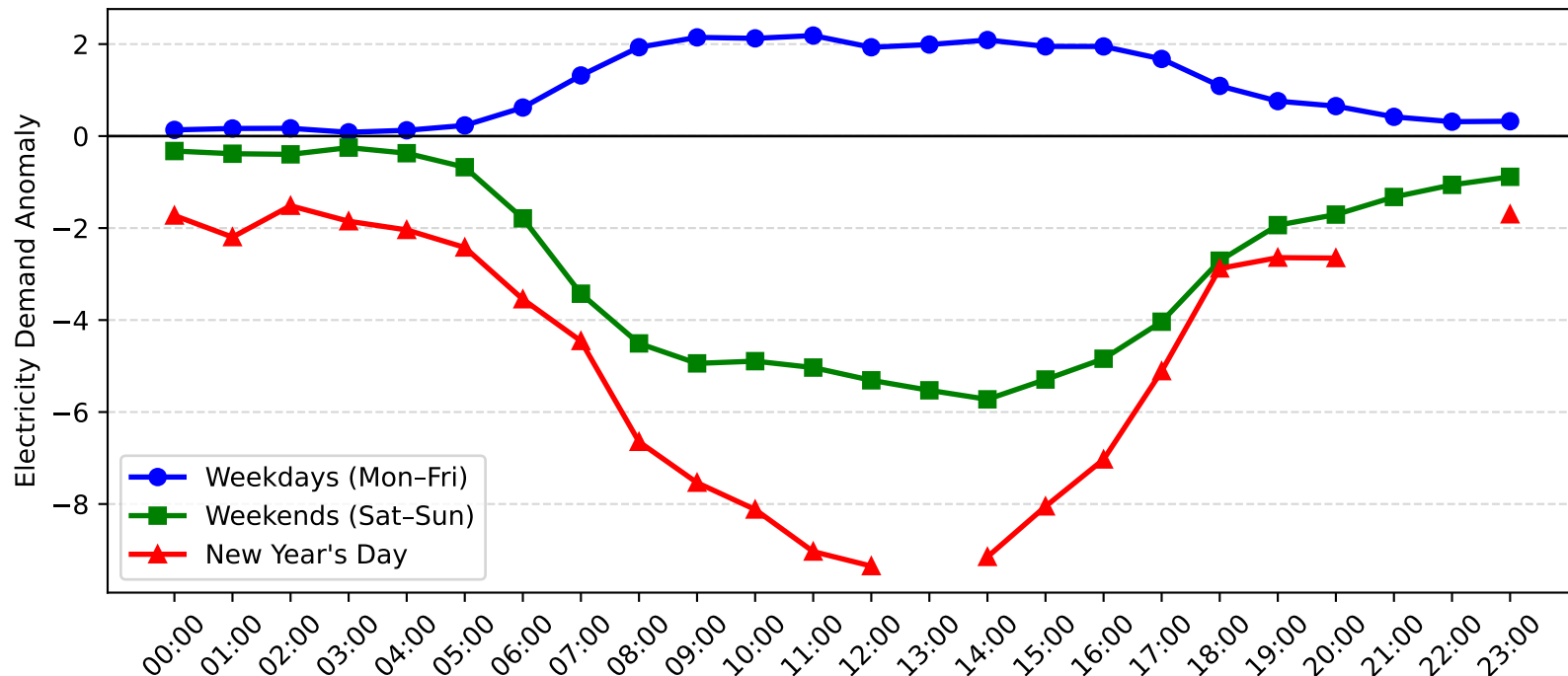
Green Square Demand Anomaly: New Year's Day vs Weekday/Weekend (2012-2013)
