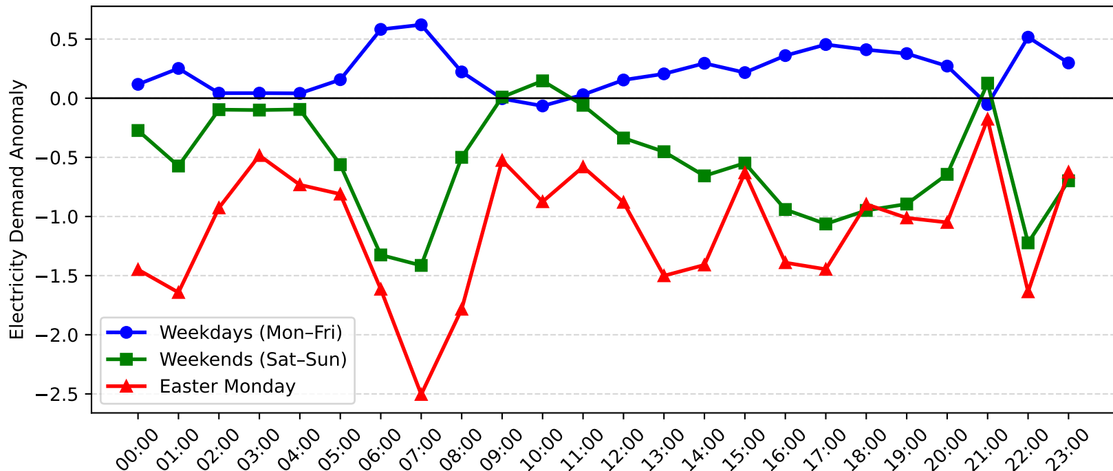
Charlestown Demand Anomaly: Easter Monday vs Weekday/Weekend (2013-2014)
