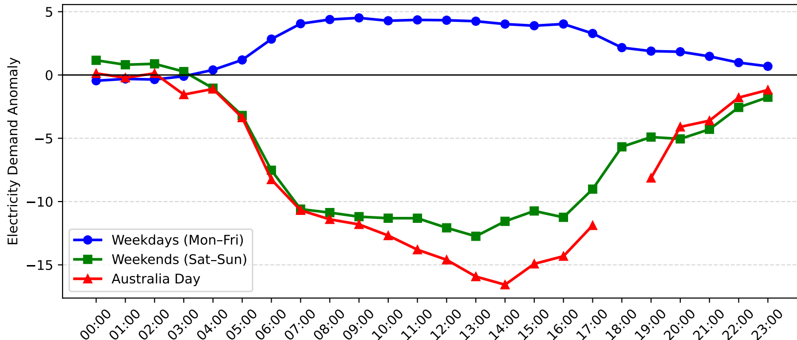
Greenacre Park Demand Anomaly: Australia Day vs Weekday/Weekend (2005-2006)
