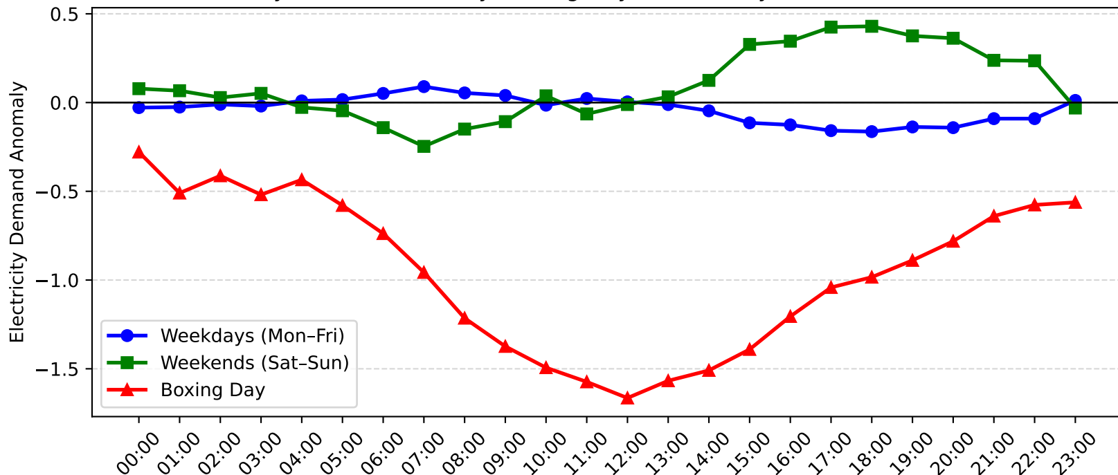
Rothbury Demand Anomaly: Boxing Day vs Weekday/Weekend (2006-2007)
