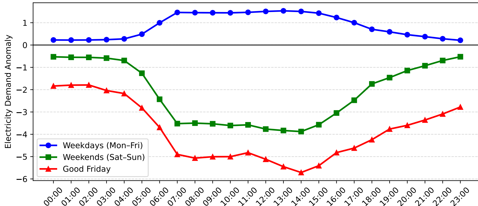
Botany Demand Anomaly: Good Friday vs Weekday/Weekend (2015-2016)
