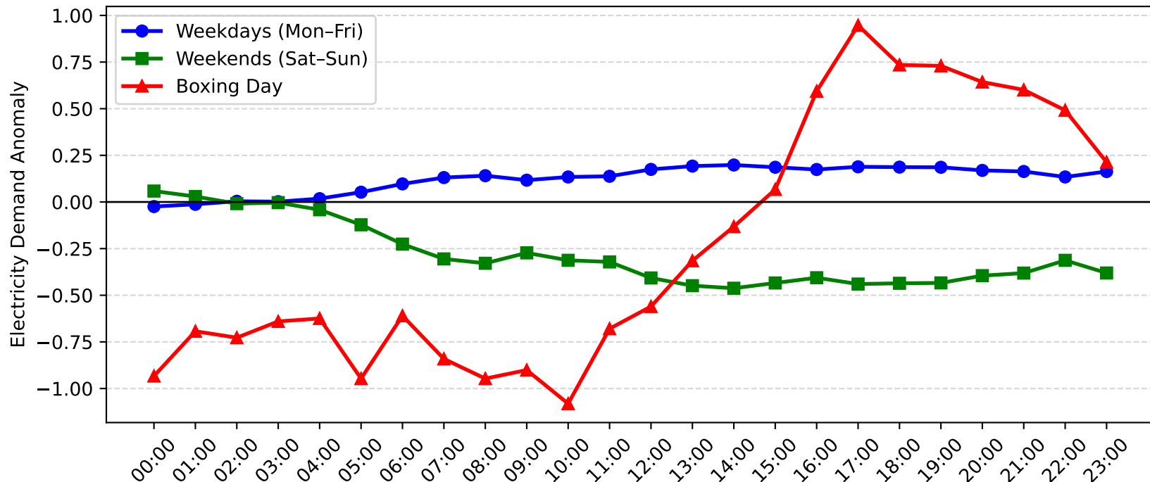
Rothbury Demand Anomaly: Boxing Day vs Weekday/Weekend (2016-2017)
