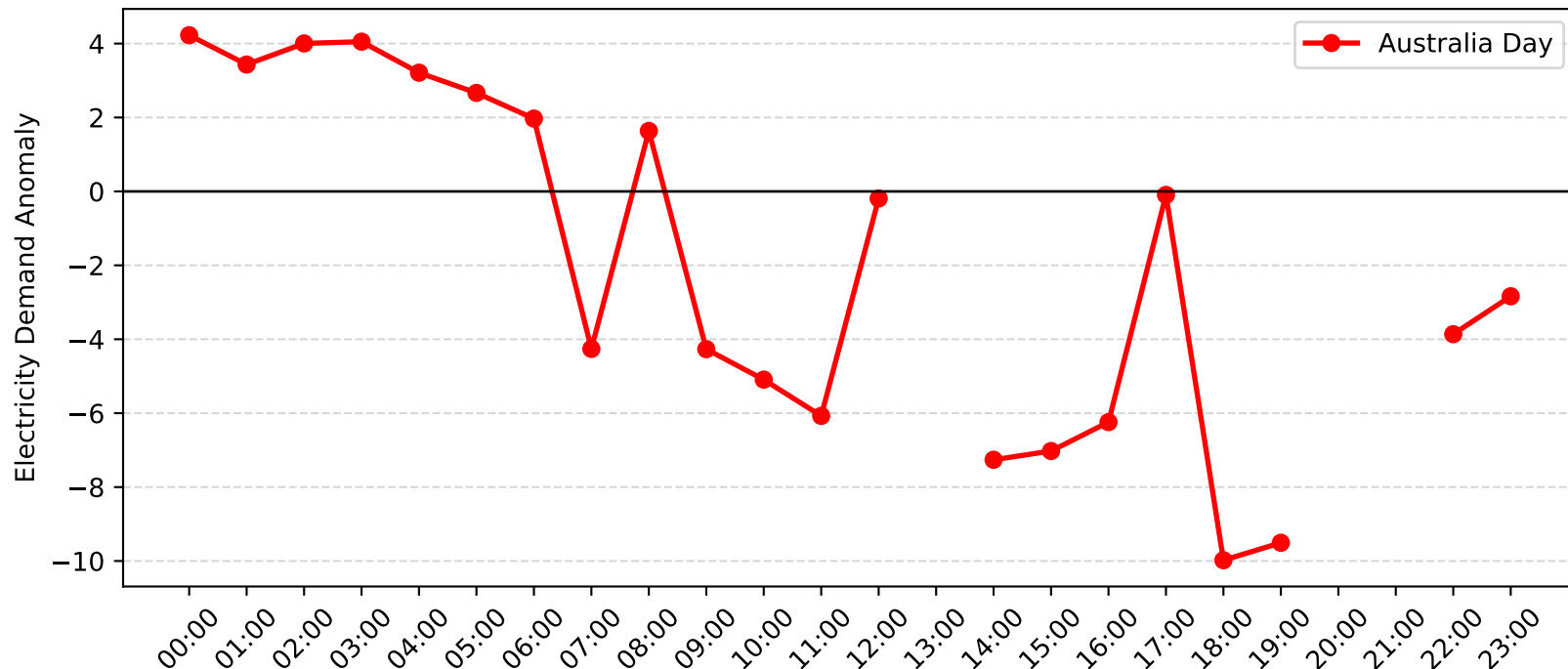
Potts Hill Demand Anomaly: Australia Day (2014-2015)
