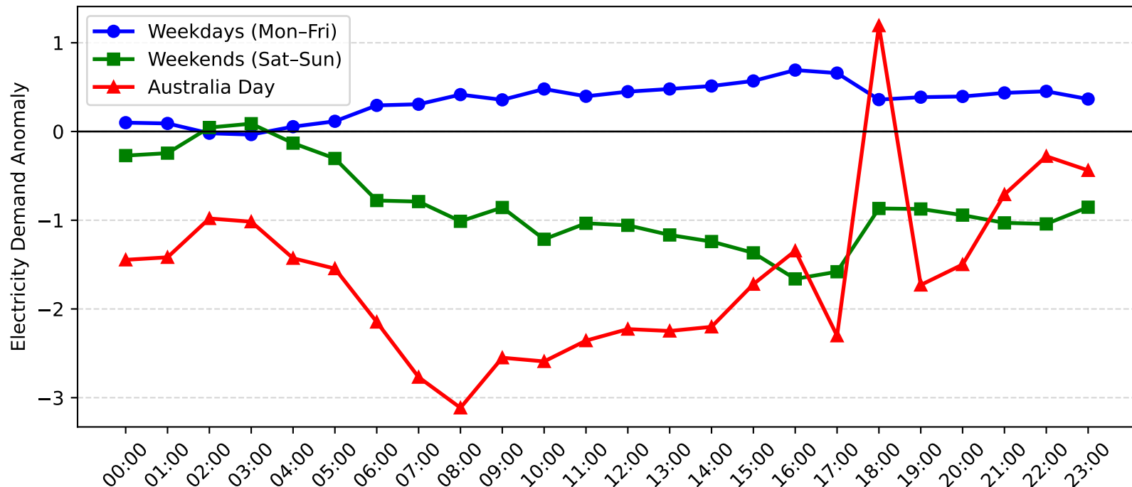
Revesby Demand Anomaly: Australia Day vs Weekday/Weekend (2004-2005)
