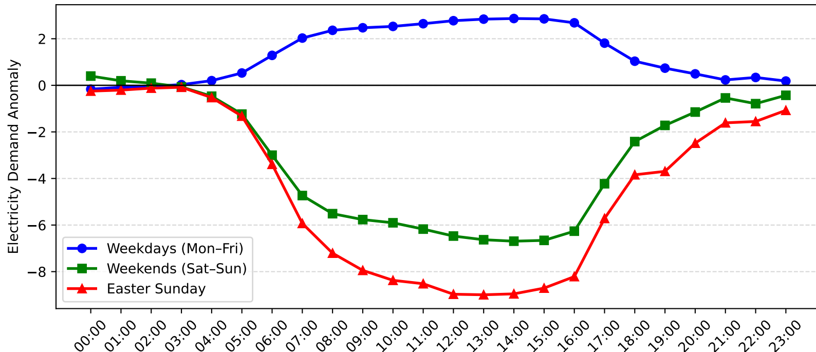
Newcastle Cbd Demand Anomaly: Easter Sunday vs Weekday/Weekend (2012-2013)
