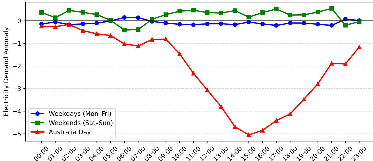
Morisset Demand Anomaly: Australia Day vs Weekday/Weekend (2017-2018)
