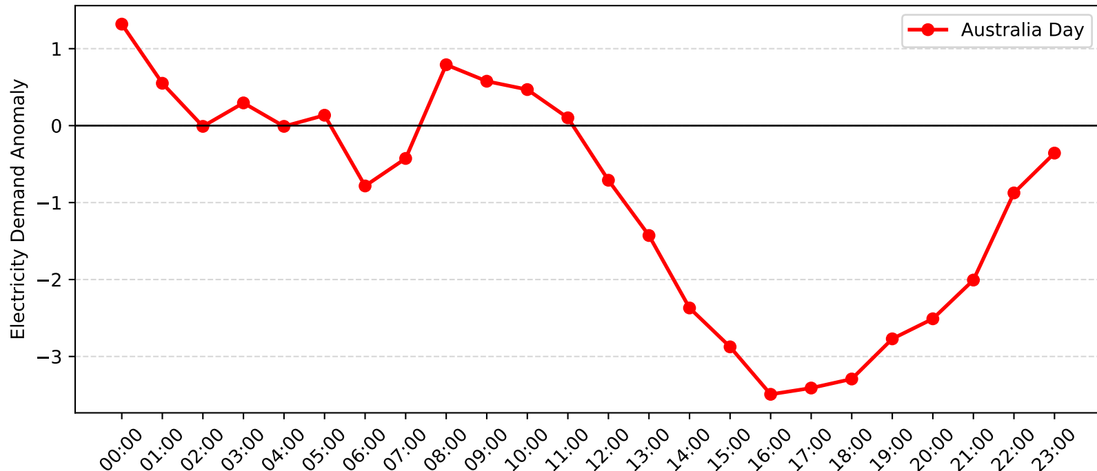
Umina Demand Anomaly: Australia Day (2014-2015)
