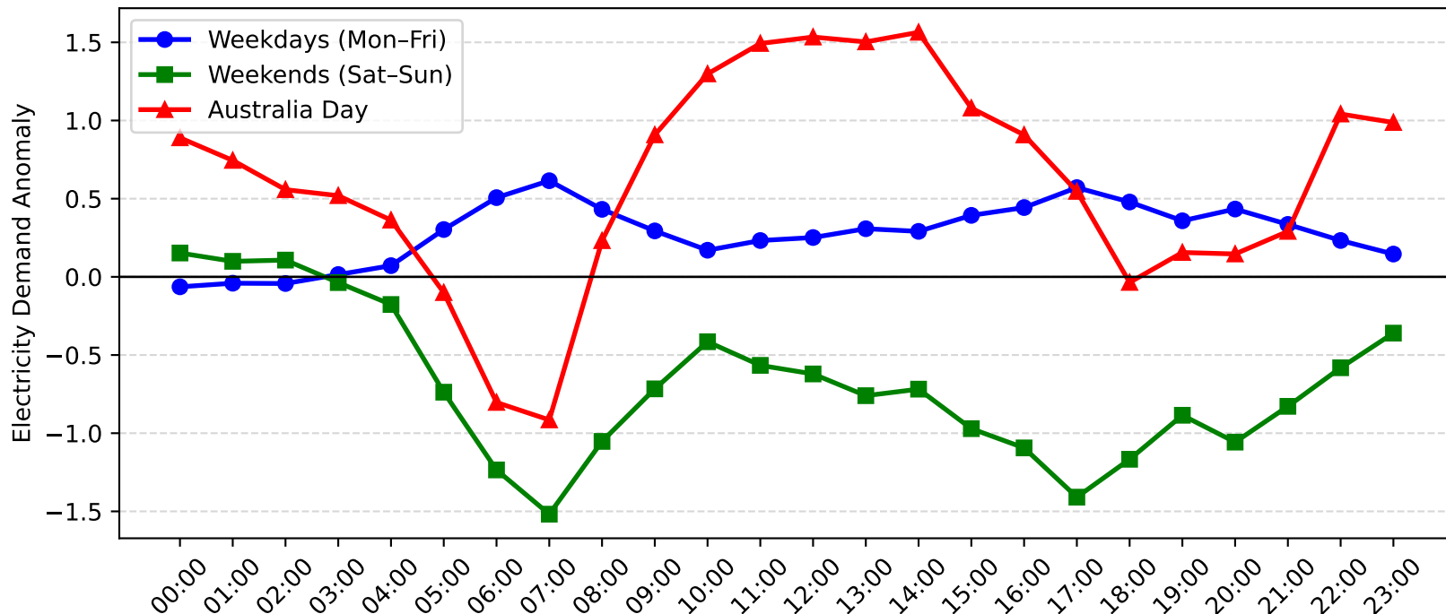
Charmhaven Demand Anomaly: Australia Day vs Weekday/Weekend (2012-2013)
