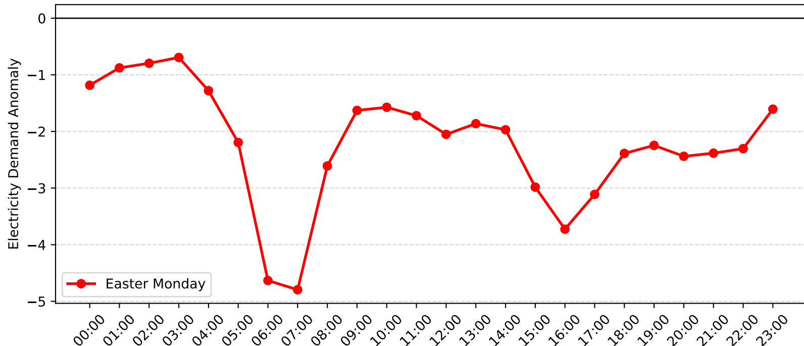
Pennant Hills Demand Anomaly: Easter Monday (2015-2016)
