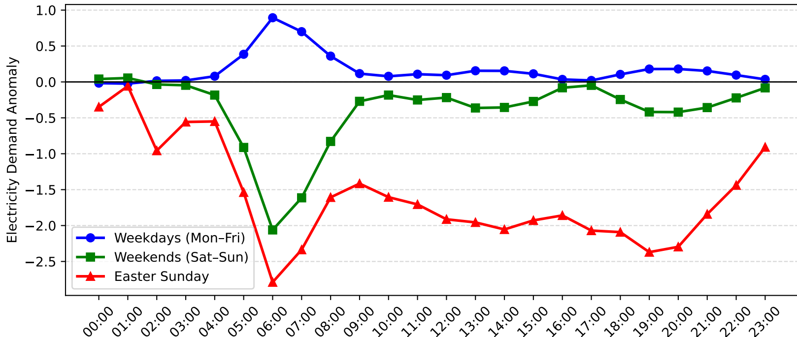
Berowra Demand Anomaly: Easter Sunday vs Weekday/Weekend (2014-2015)
