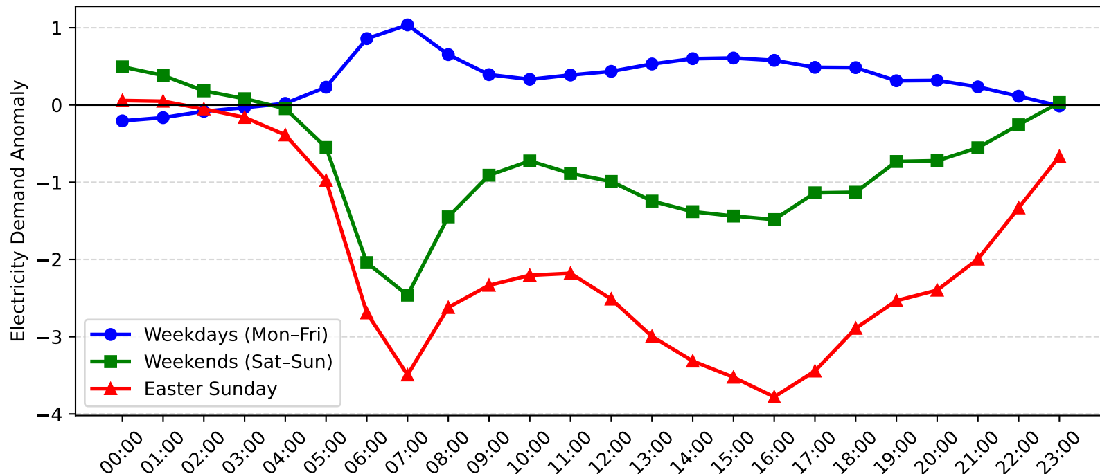
Blakehurst Demand Anomaly: Easter Sunday vs Weekday/Weekend (2006-2007)
