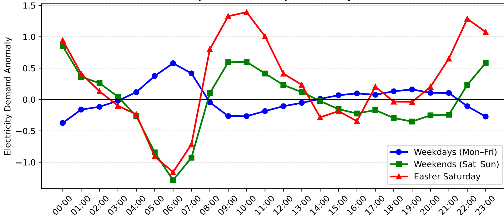
Umina Demand Anomaly: Easter Saturday vs Weekday/Weekend (2008-2009)
