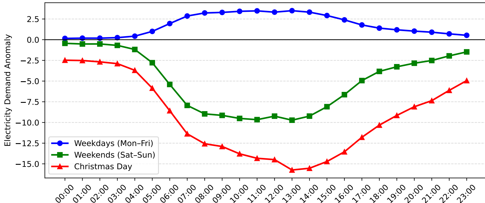
Milperra Demand Anomaly: Christmas Day vs Weekday/Weekend (2012-2013)
