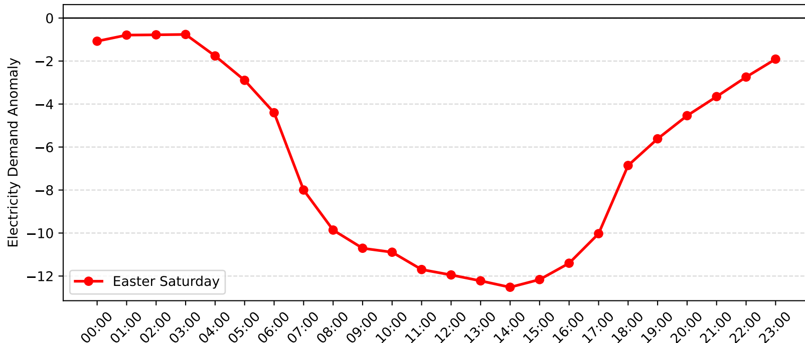
Gore Hill Demand Anomaly: Easter Saturday (2016-2017)
