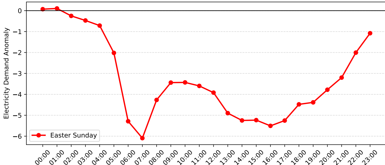
Mortdale Demand Anomaly: Easter Sunday (2006-2007)
