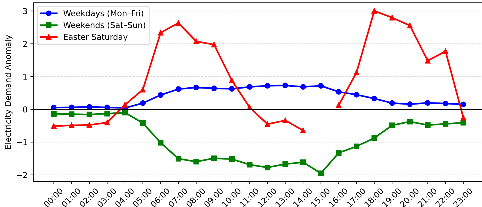
Concord Demand Anomaly: Easter Saturday vs Weekday/Weekend (2004-2005)
