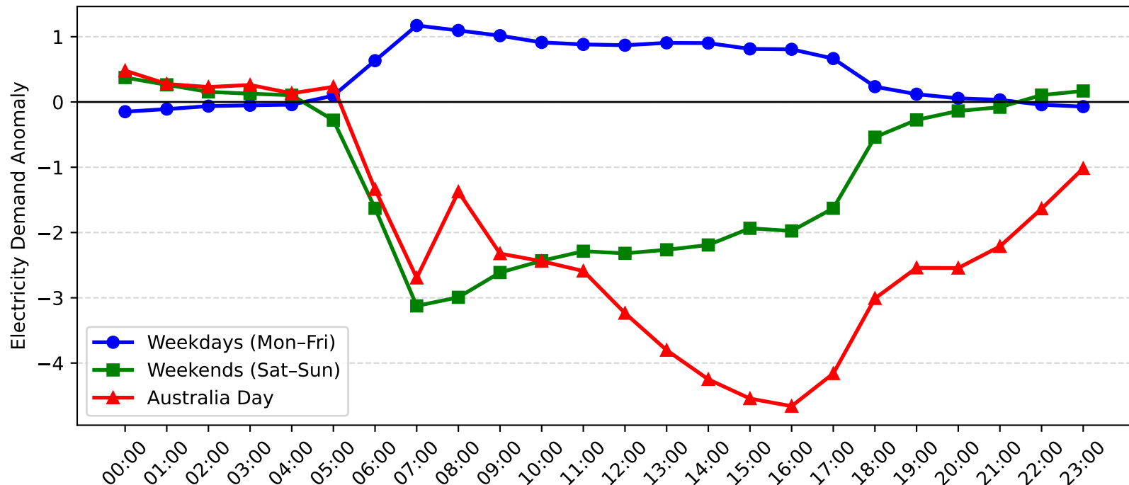
Pymble Demand Anomaly: Australia Day vs Weekday/Weekend (2014-2015)
