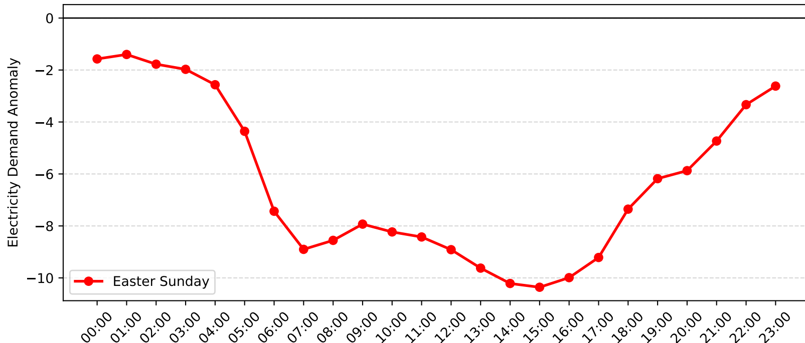
Sefton Demand Anomaly: Easter Sunday (2007-2008)
