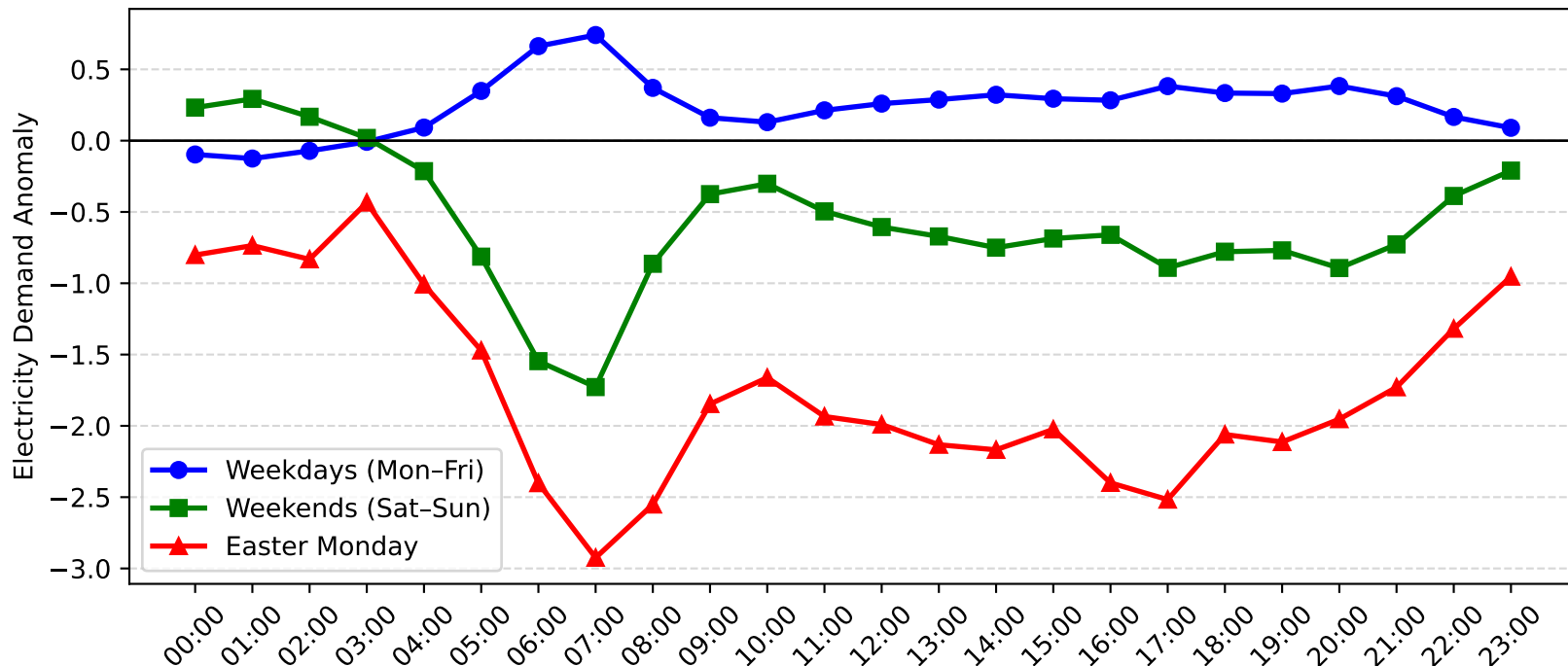
Charmhaven Demand Anomaly: Easter Monday vs Weekday/Weekend (2013-2014)
