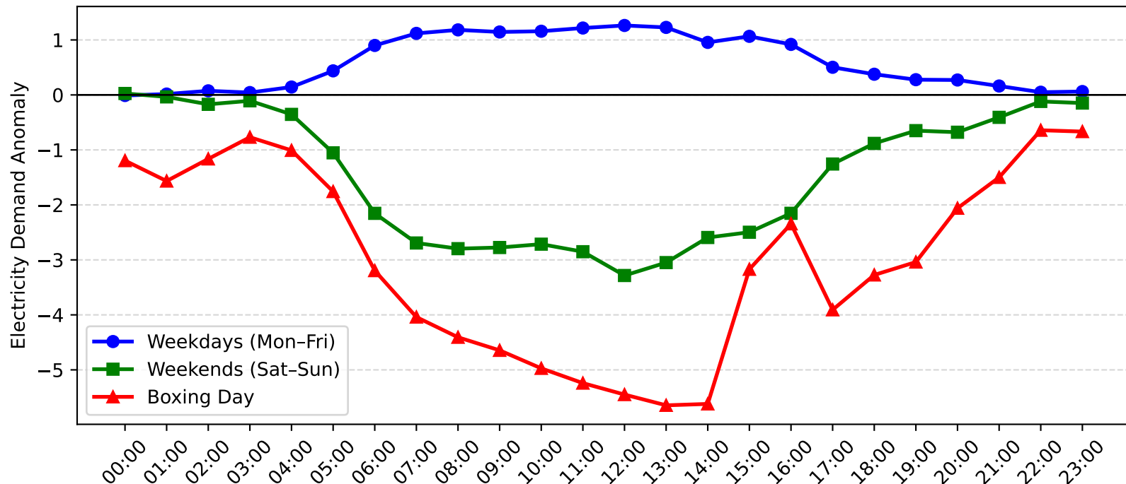
Wyong Demand Anomaly: Boxing Day vs Weekday/Weekend (2005-2006)
