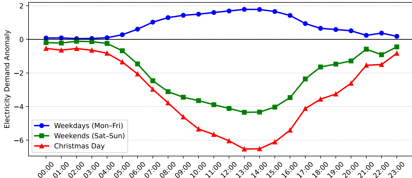
Broadmeadow Demand Anomaly: Christmas Day vs Weekday/Weekend (2015-2016)
