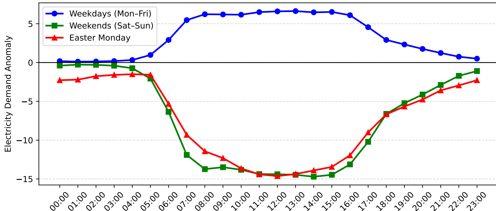
Gore Hill Demand Anomaly: Easter Monday vs Weekday/Weekend (2009-2010)
