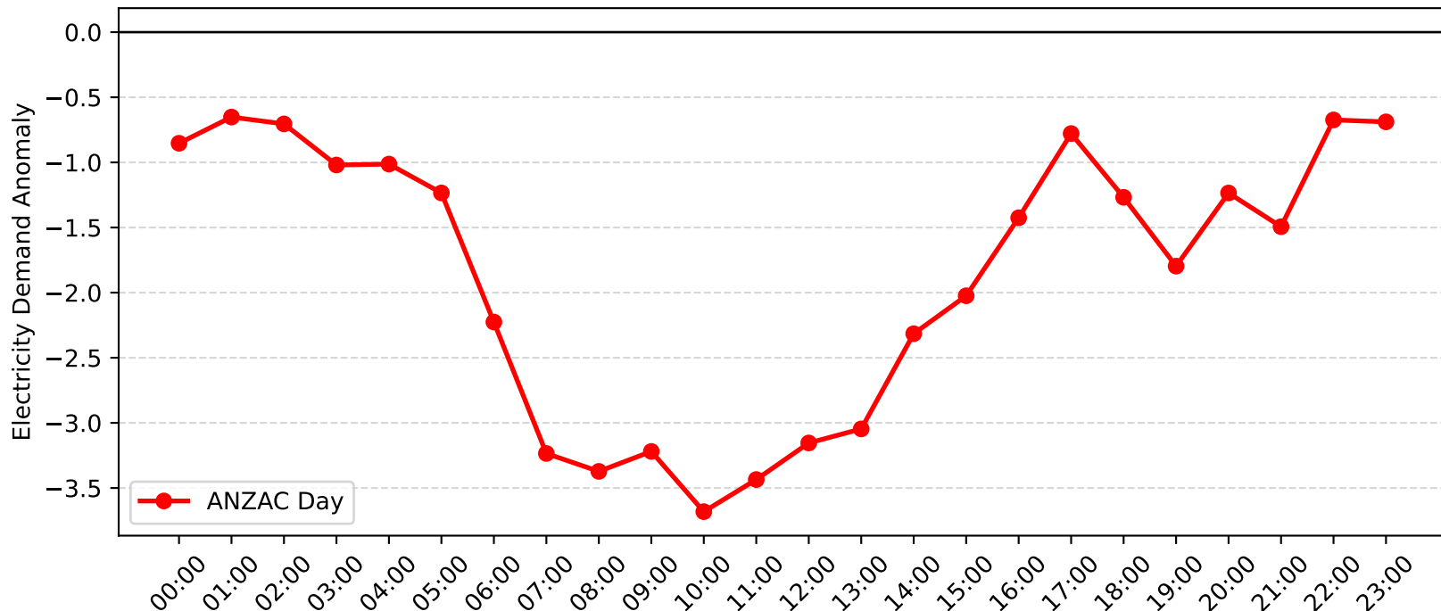
Mayfield West Demand Anomaly: ANZAC Day (2017-2018)
