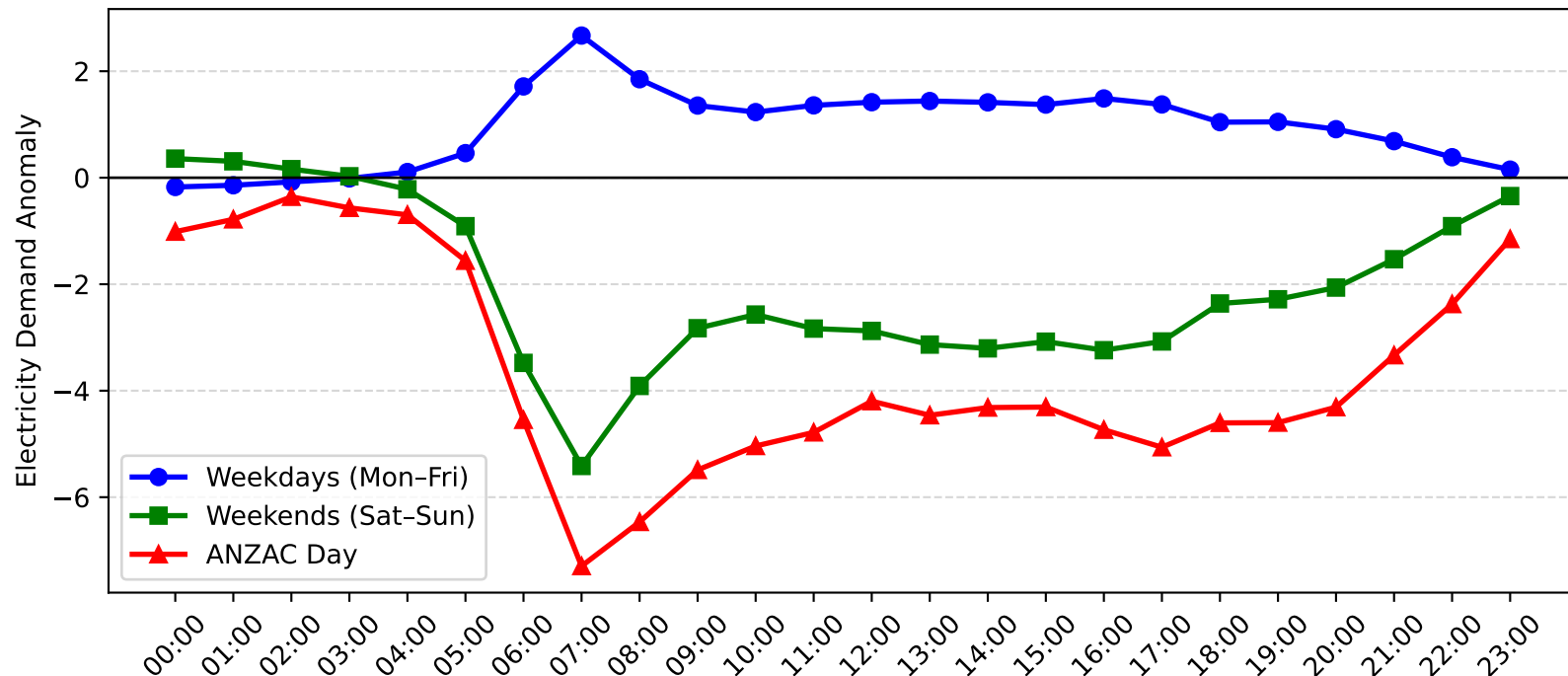
Chatswood Demand Anomaly: ANZAC Day vs Weekday/Weekend (2009-2010)
