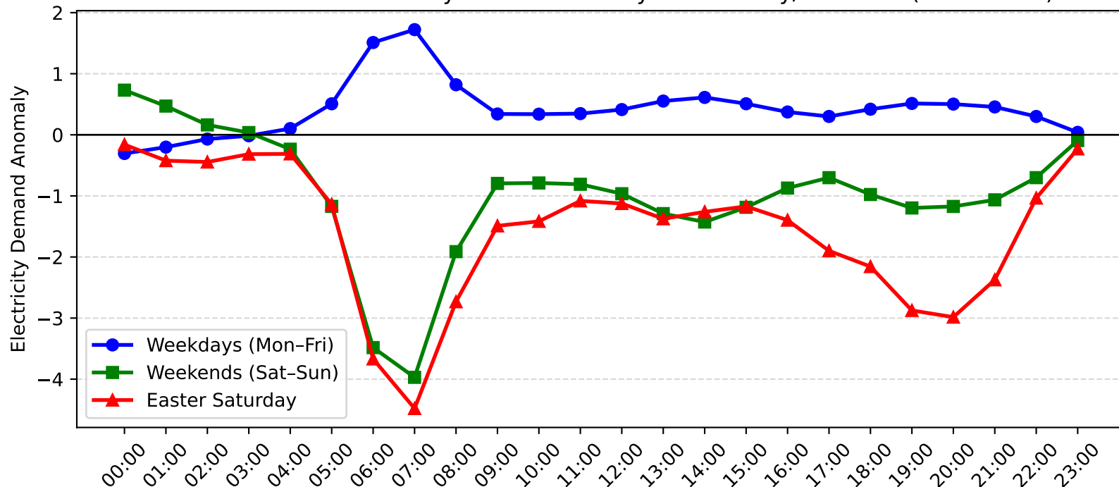
Mortdale Demand Anomaly: Easter Saturday vs Weekday/Weekend (2011-2012)
