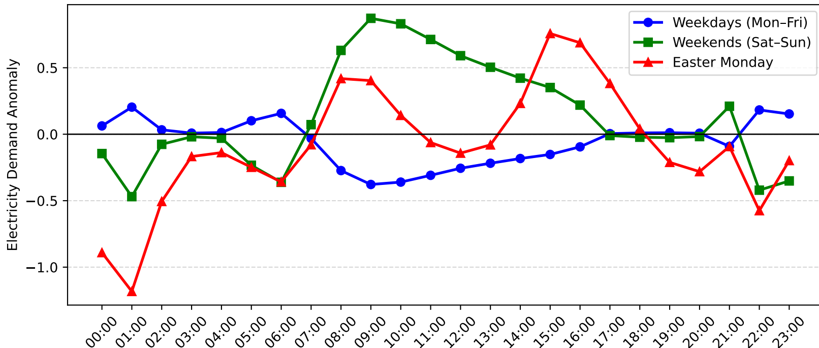
Swansea Demand Anomaly: Easter Monday vs Weekday/Weekend (2014-2015)
