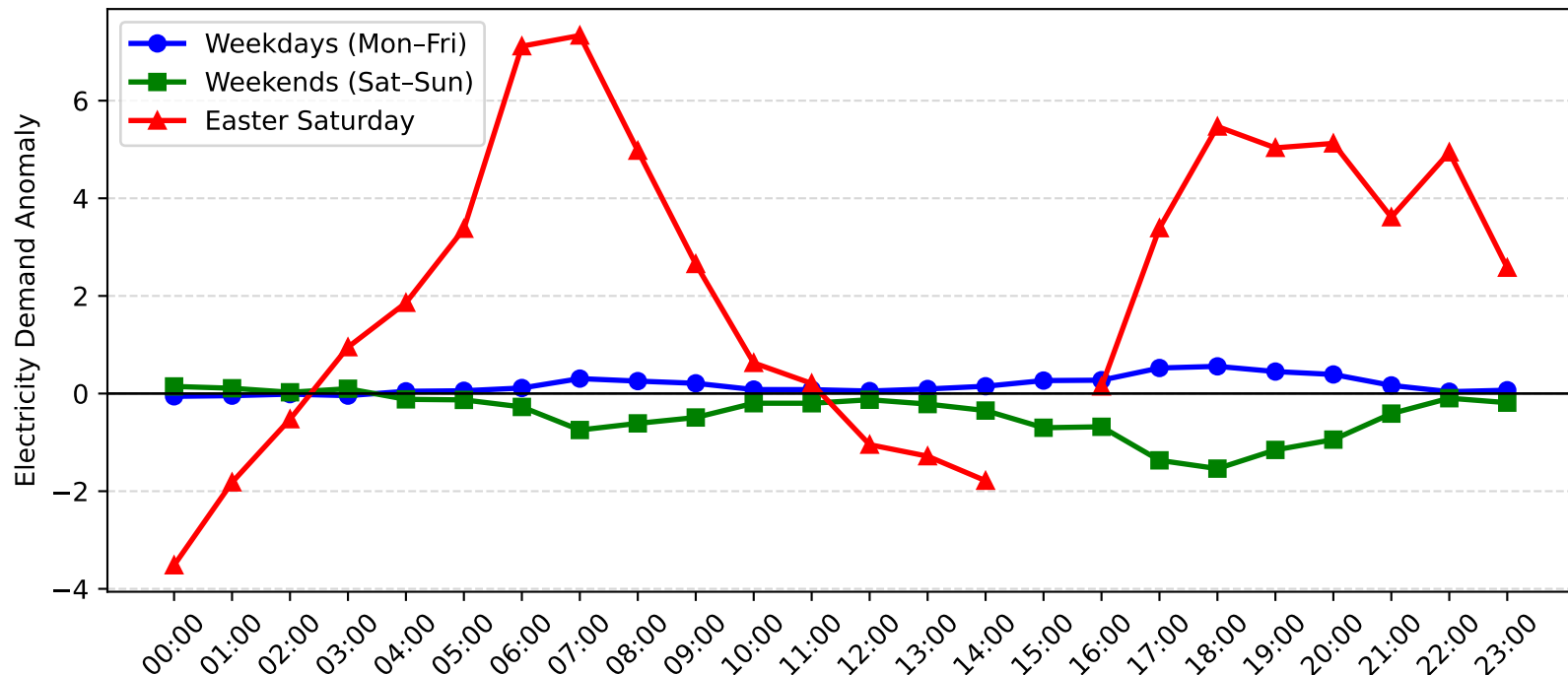
Erina Demand Anomaly: Easter Saturday vs Weekday/Weekend (2004-2005)
