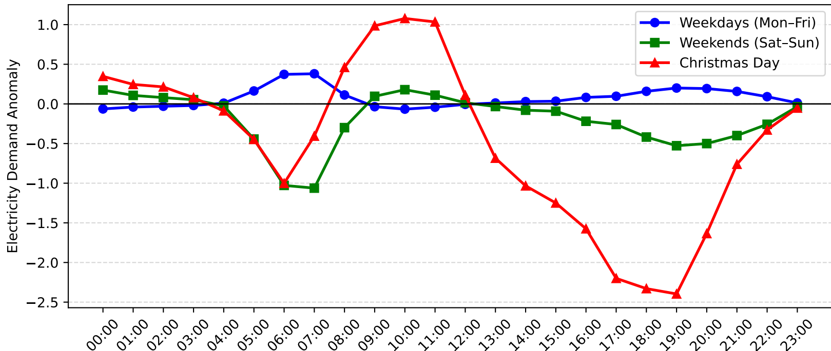
Harbord Demand Anomaly: Christmas Day vs Weekday/Weekend (2014-2015)
