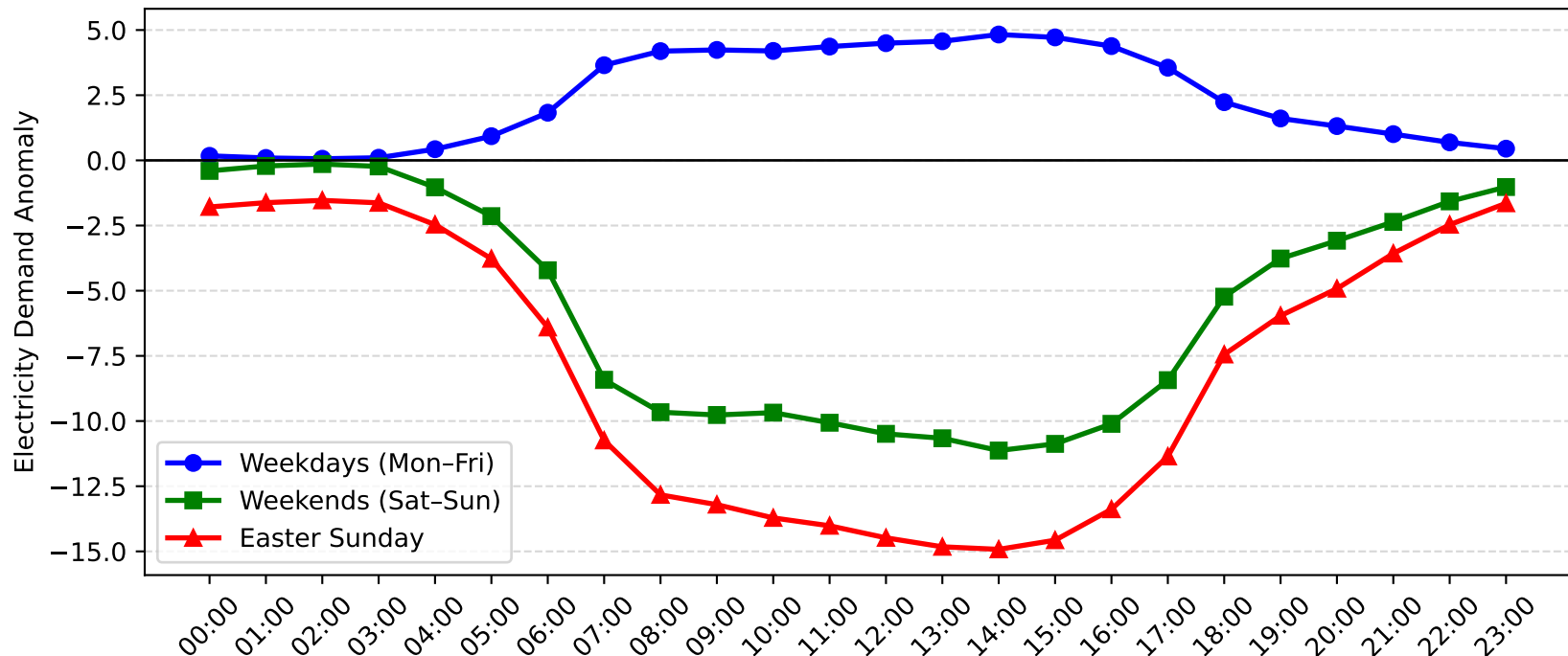
Gore Hill Demand Anomaly: Easter Sunday vs Weekday/Weekend (2015-2016)
