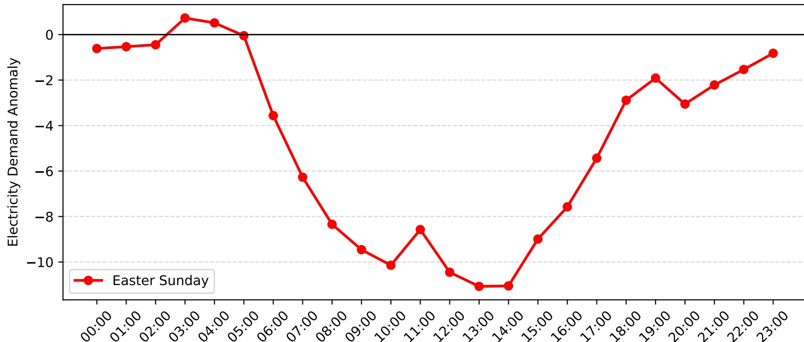
Green Square Demand Anomaly: Easter Sunday (2016-2017)
