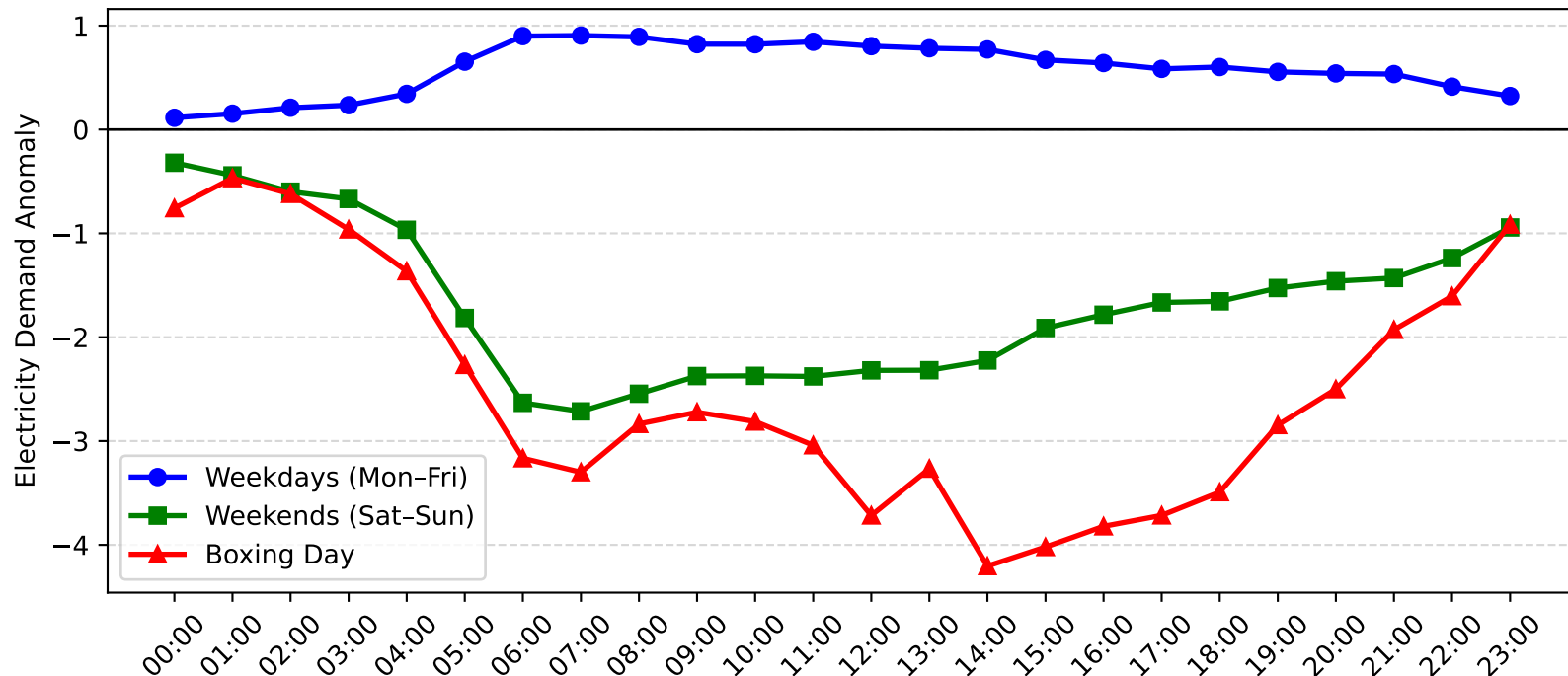
Lisarow Demand Anomaly: Boxing Day vs Weekday/Weekend (2013-2014)
