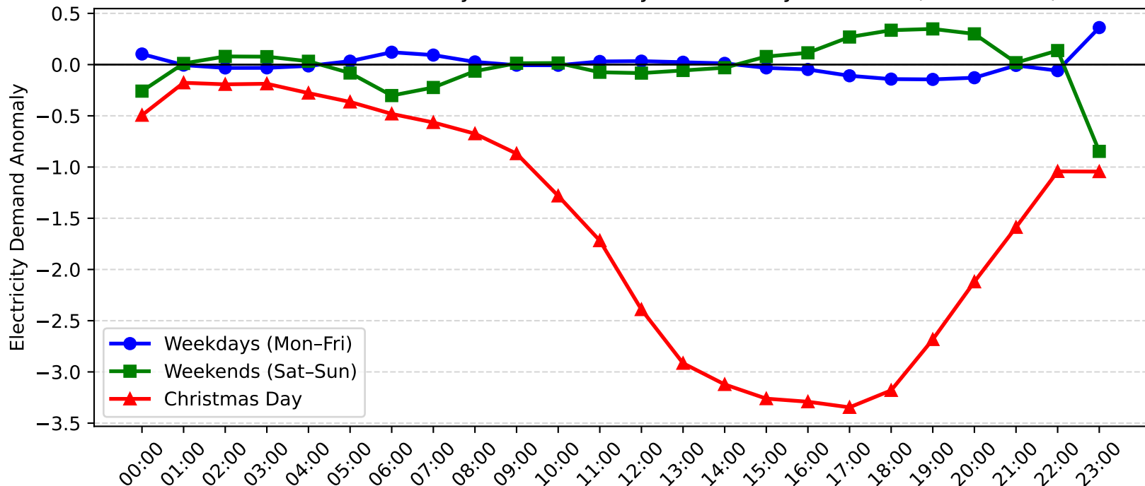
Telarah Demand Anomaly: Christmas Day vs Weekday/Weekend (2006-2007)
