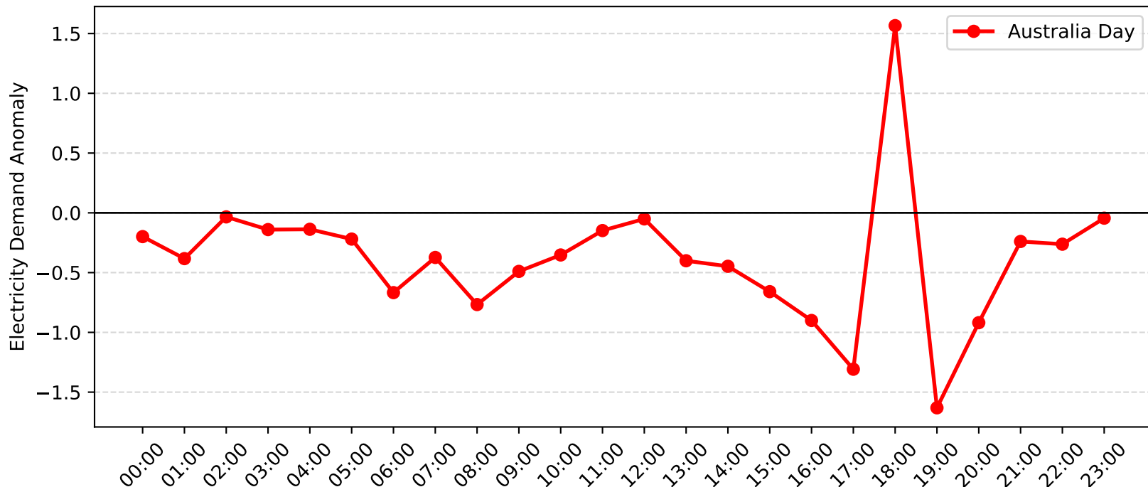
Charmhaven Demand Anomaly: Australia Day (2004-2005)
