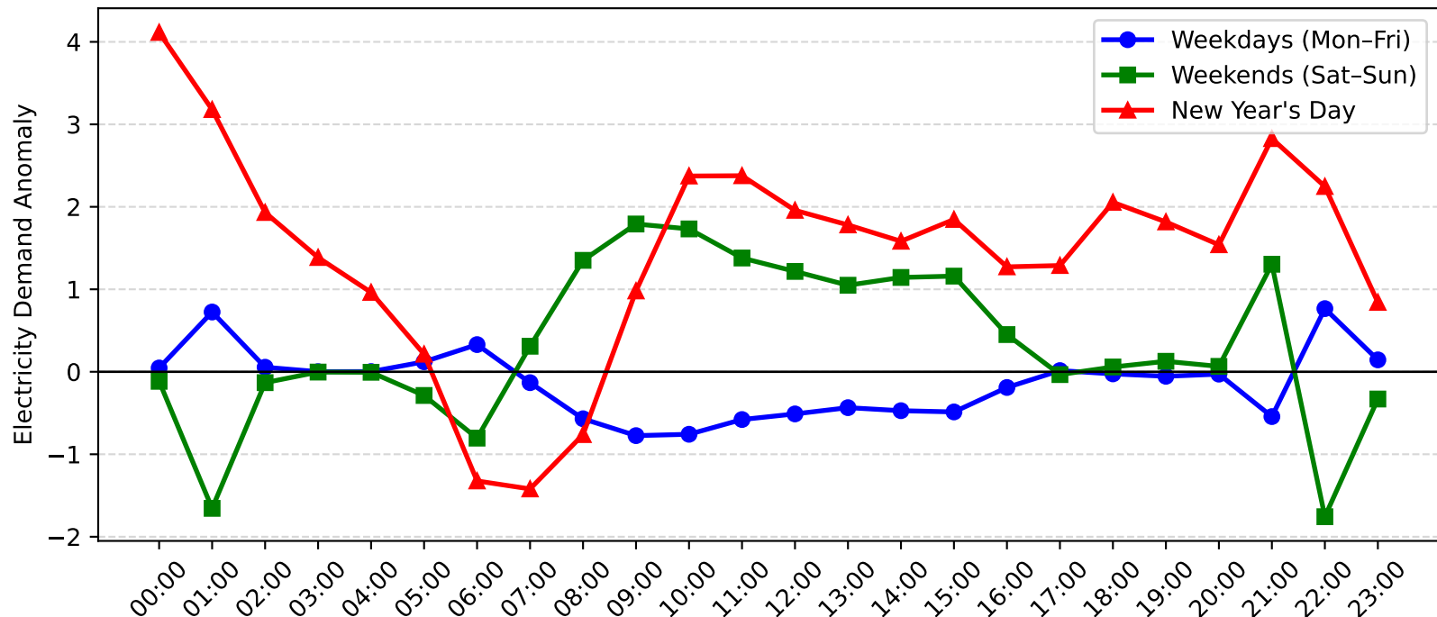
Nelson Bay Demand Anomaly: New Year's Day vs Weekday/Weekend (2007-2008)
