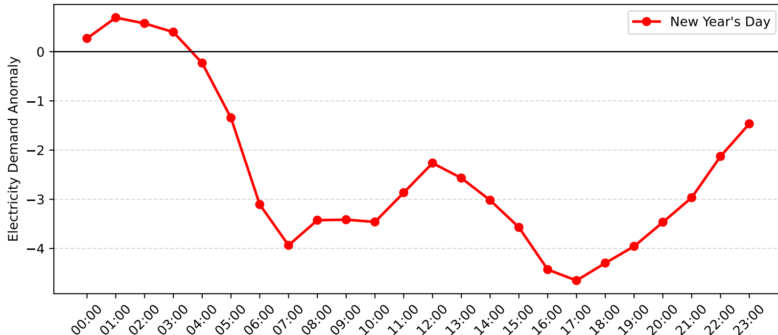
Revesby Demand Anomaly: New Year's Day (2016-2017)
