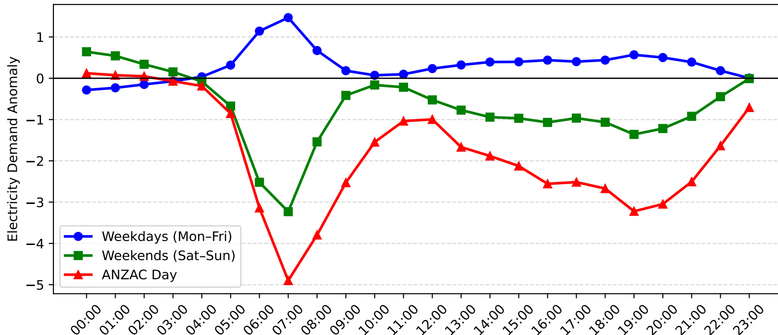
Five Dock Demand Anomaly: ANZAC Day vs Weekday/Weekend (2010-2011)
