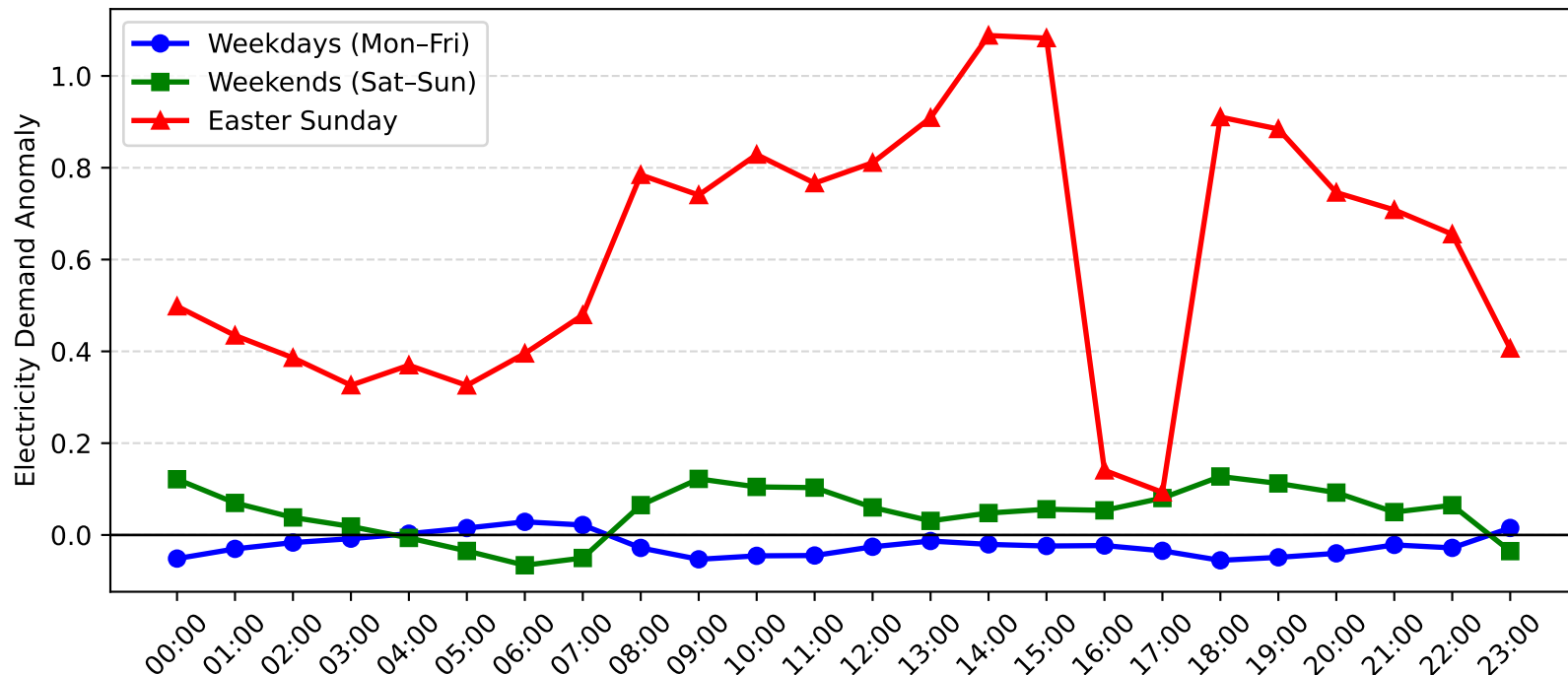
Rothbury Demand Anomaly: Easter Sunday vs Weekday/Weekend (2015-2016)
