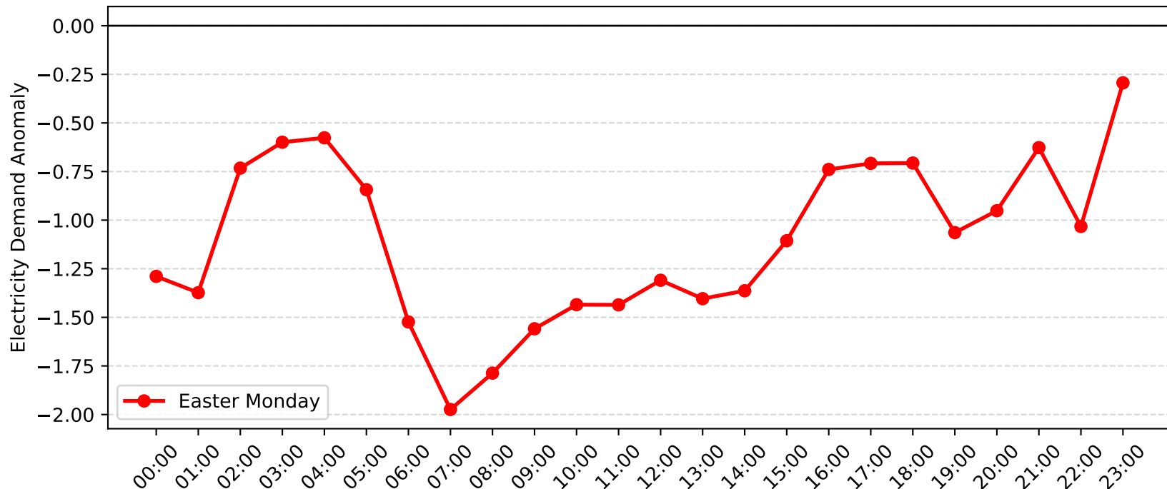
Gateshead Demand Anomaly: Easter Monday (2017-2018)
