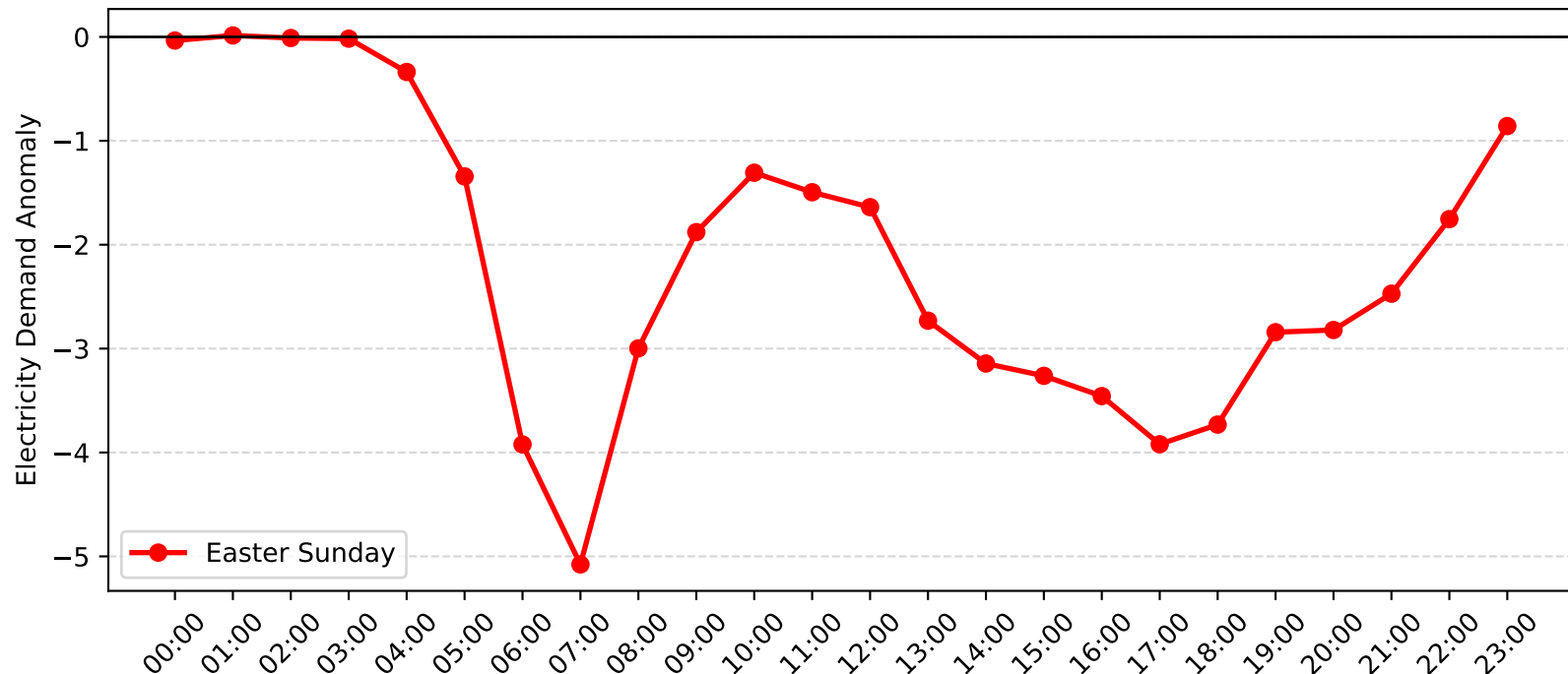
Mortdale Demand Anomaly: Easter Sunday (2012-2013)
