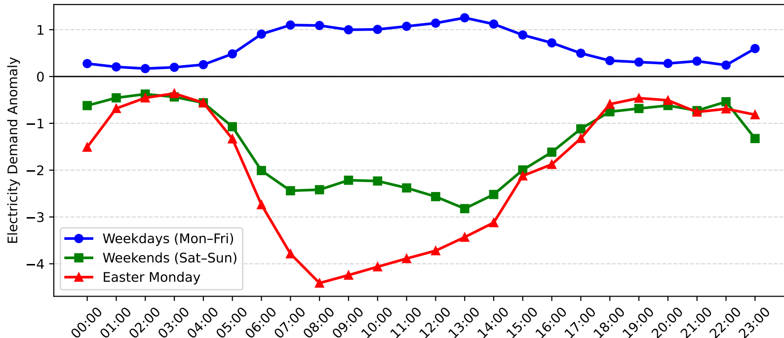
Rutherford Demand Anomaly: Easter Monday vs Weekday/Weekend (2016-2017)
