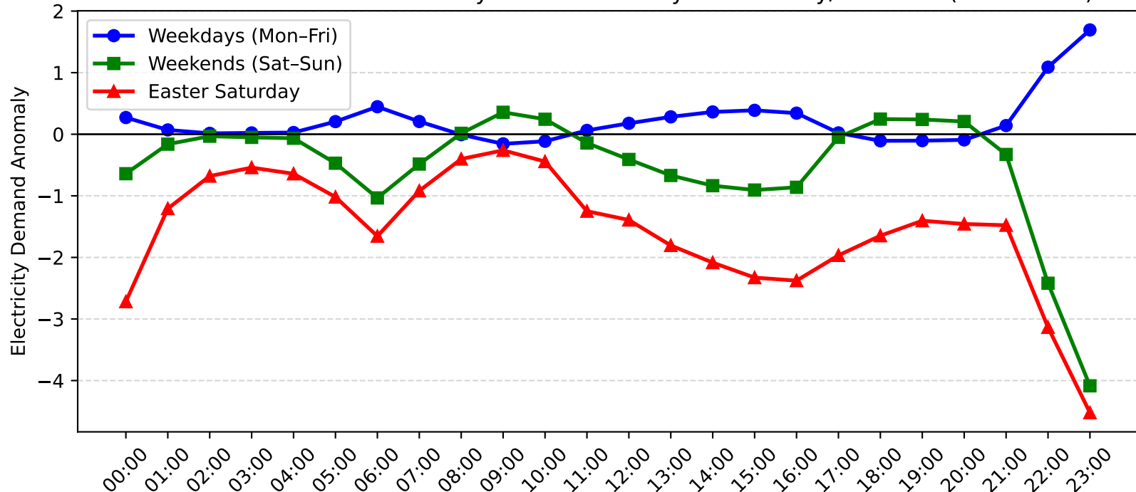
Muswellbrook Demand Anomaly: Easter Saturday vs Weekday/Weekend (2005-2006)
