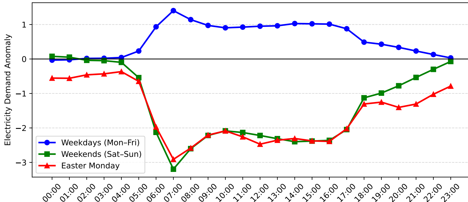
Pymble Demand Anomaly: Easter Monday vs Weekday/Weekend (2015-2016)
