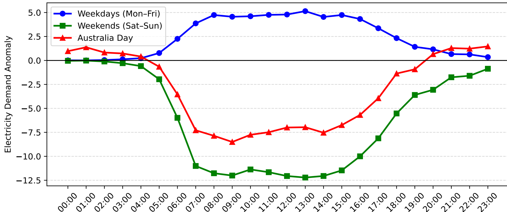
Zetland Demand Anomaly: Australia Day vs Weekday/Weekend (2009-2010)
