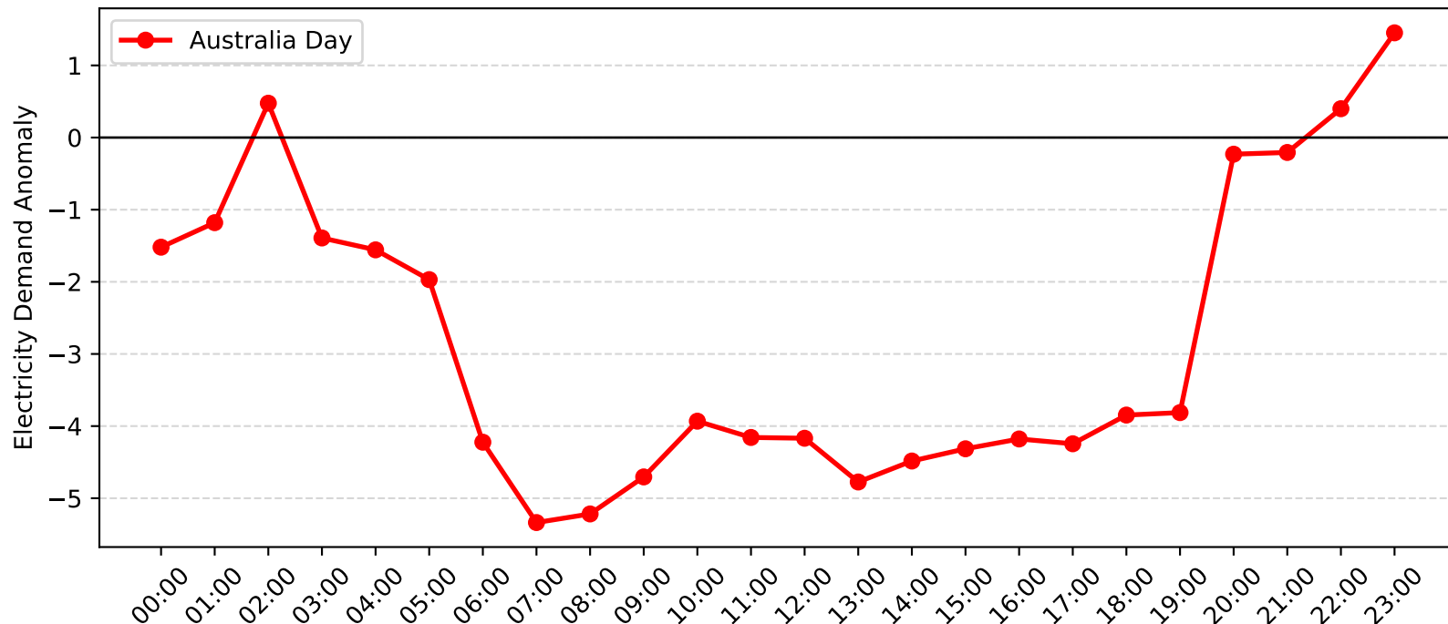
Chatswood Demand Anomaly: Australia Day (2006-2007)
