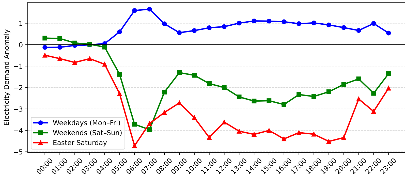
Dee Why West Demand Anomaly: Easter Saturday vs Weekday/Weekend (2005-2006)
