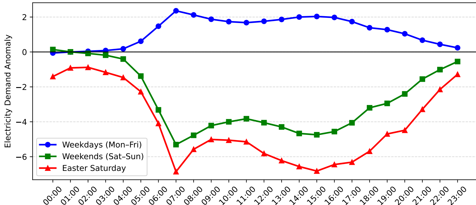
Burwood Demand Anomaly: Easter Saturday vs Weekday/Weekend (2015-2016)
