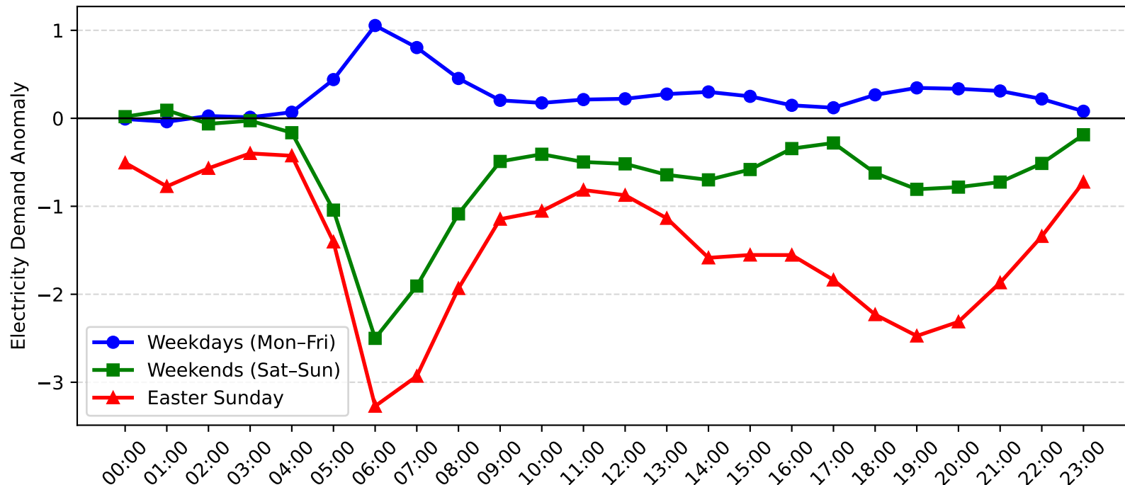
Berowra Demand Anomaly: Easter Sunday vs Weekday/Weekend (2011-2012)
