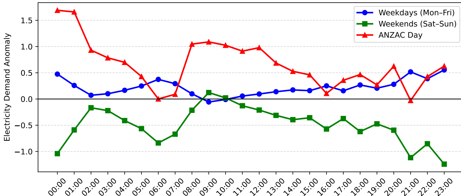
Morisset Demand Anomaly: ANZAC Day vs Weekday/Weekend (2008-2009)
