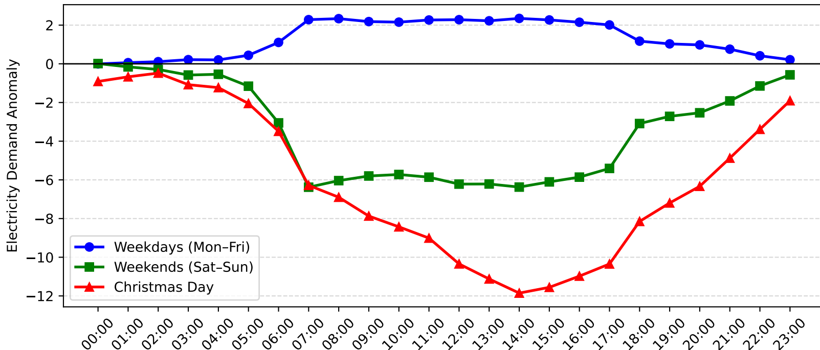
Epping Demand Anomaly: Christmas Day vs Weekday/Weekend (2014-2015)
