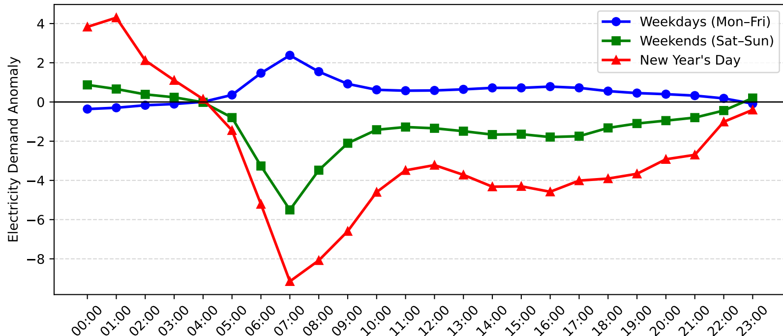
Mosman Demand Anomaly: New Year's Day vs Weekday/Weekend (2011-2012)
