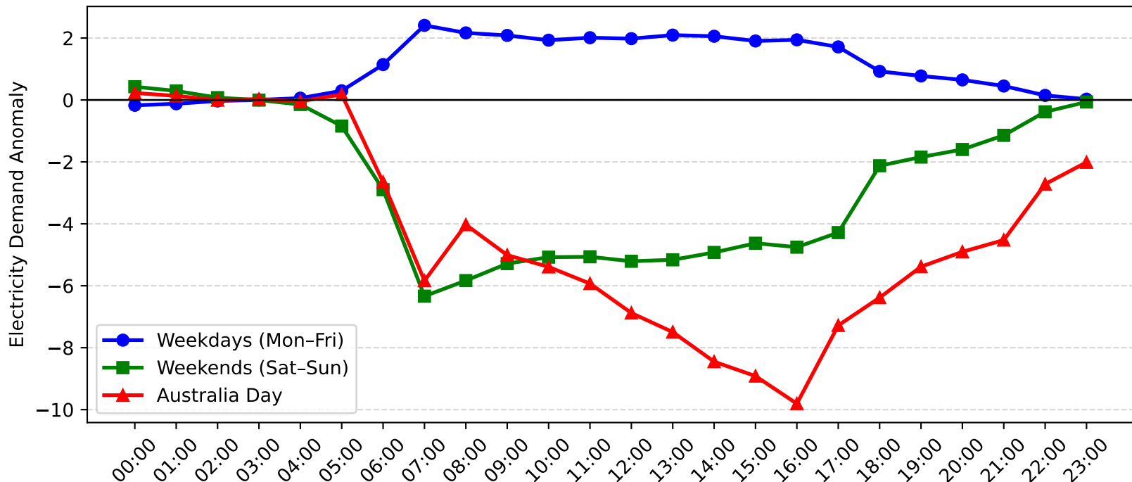
Epping Demand Anomaly: Australia Day vs Weekday/Weekend (2014-2015)
