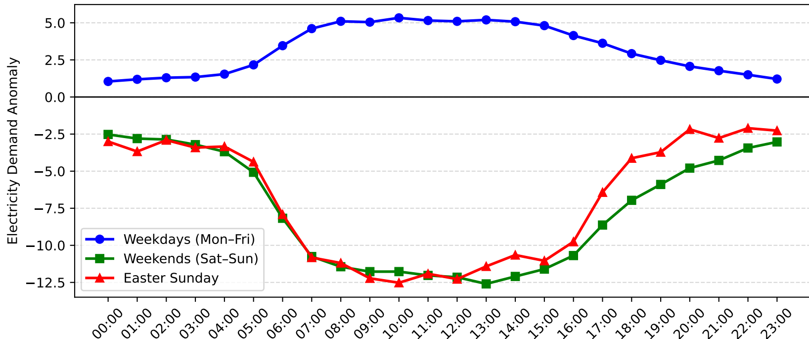
Flemington Demand Anomaly: Easter Sunday vs Weekday/Weekend (2005-2006)
