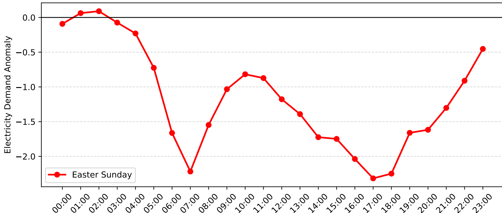
Blakehurst Demand Anomaly: Easter Sunday (2013-2014)
