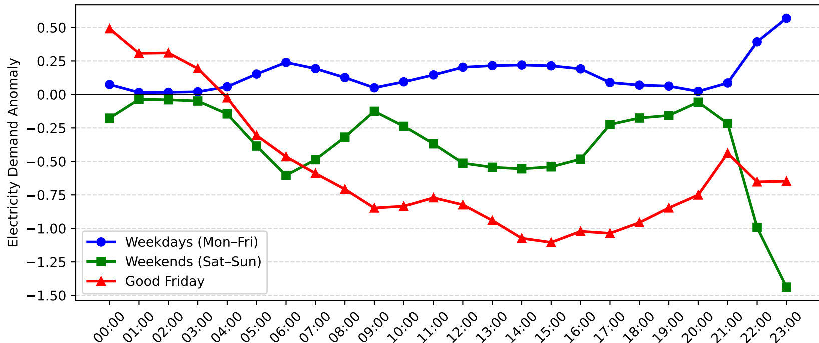
Muswellbrook Demand Anomaly: Good Friday vs Weekday/Weekend (2012-2013)
