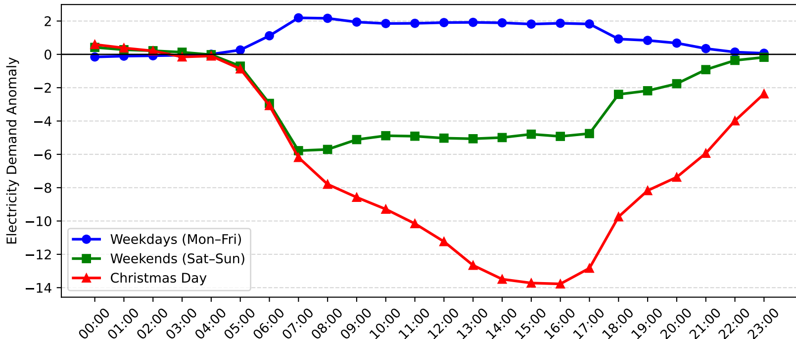
Epping Demand Anomaly: Christmas Day vs Weekday/Weekend (2012-2013)
