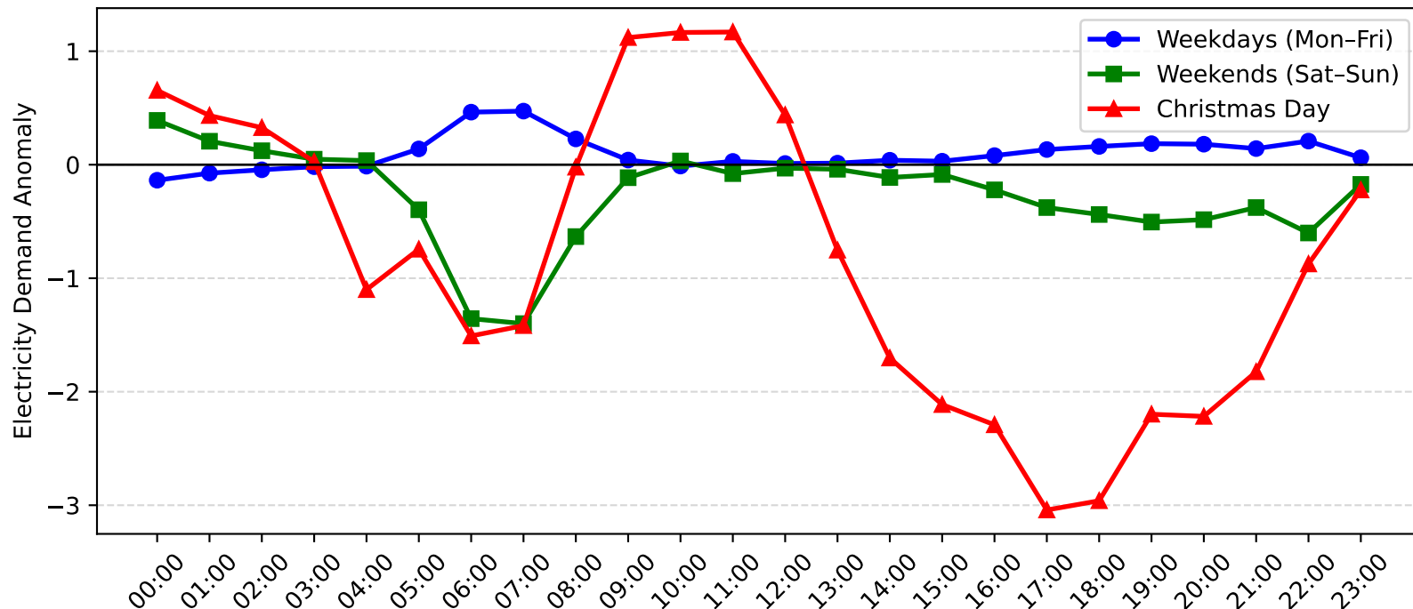
Balgowlah North Demand Anomaly: Christmas Day vs Weekday/Weekend (2013-2014)
