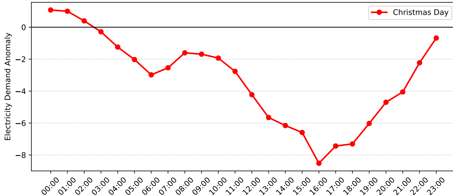
Revesby Demand Anomaly: Christmas Day (2007-2008)
