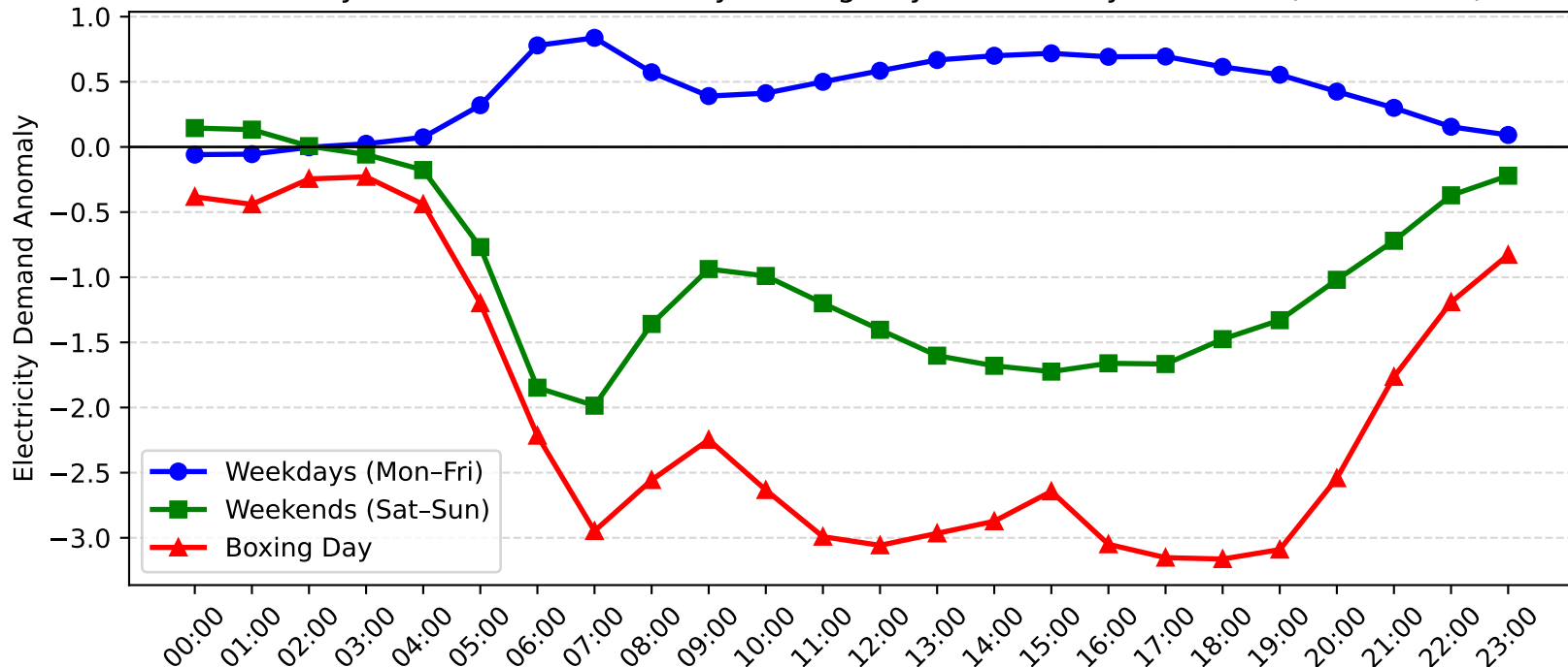
Dee Why West Demand Anomaly: Boxing Day vs Weekday/Weekend (2015-2016)
