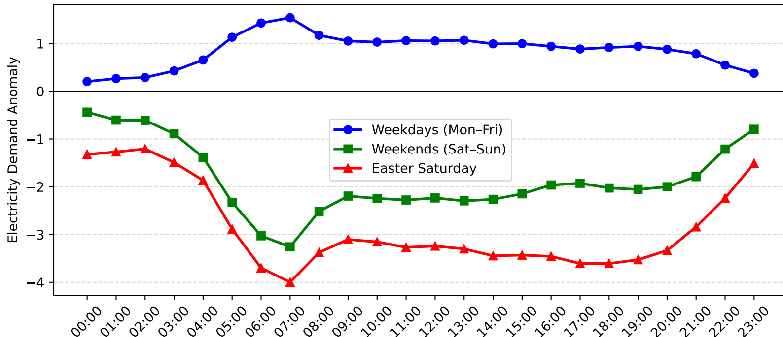
Lisarow Demand Anomaly: Easter Saturday vs Weekday/Weekend (2009-2010)
