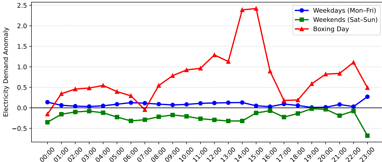
Telarah Demand Anomaly: Boxing Day vs Weekday/Weekend (2014-2015)
