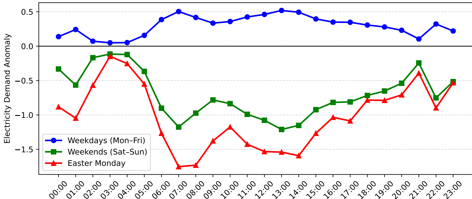
Gateshead Demand Anomaly: Easter Monday vs Weekday/Weekend (2012-2013)
