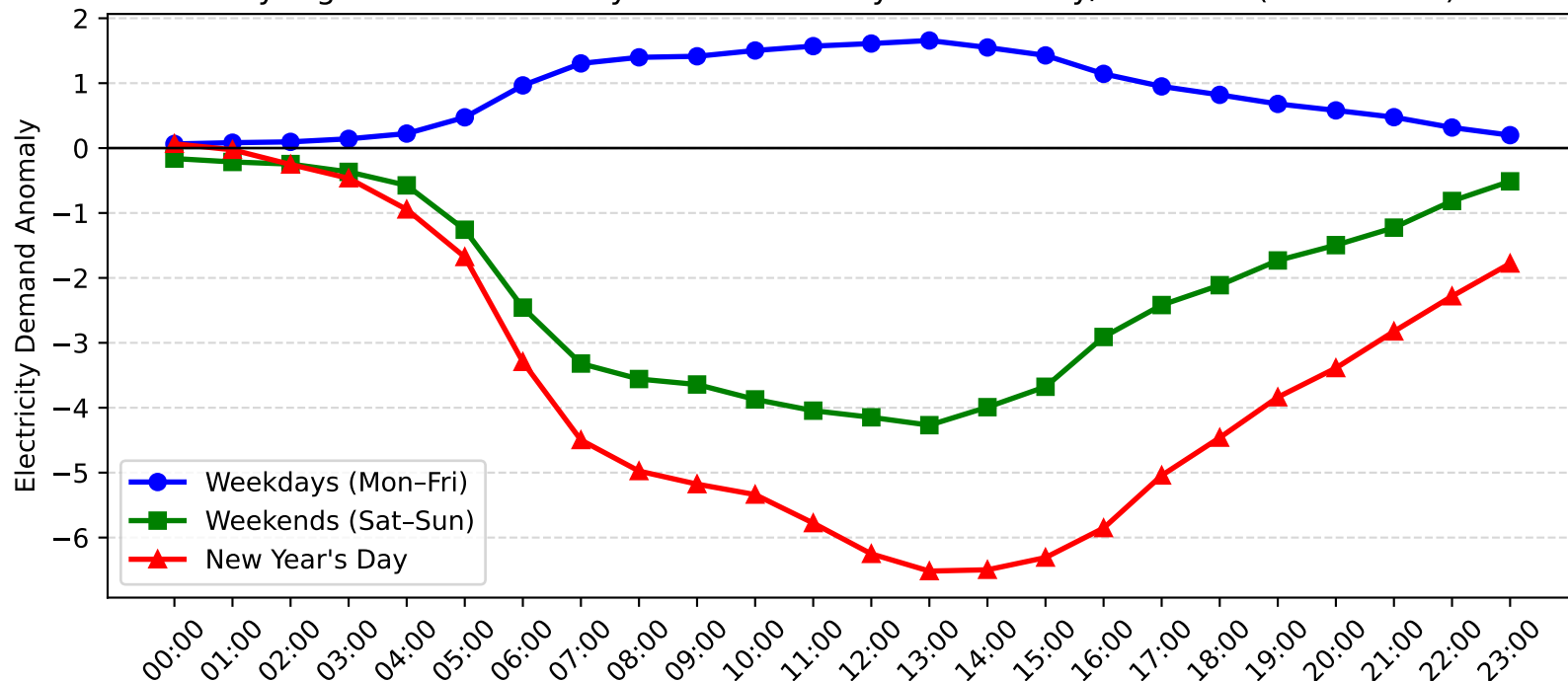
Wyong Demand Anomaly: New Year's Day vs Weekday/Weekend (2016-2017)
