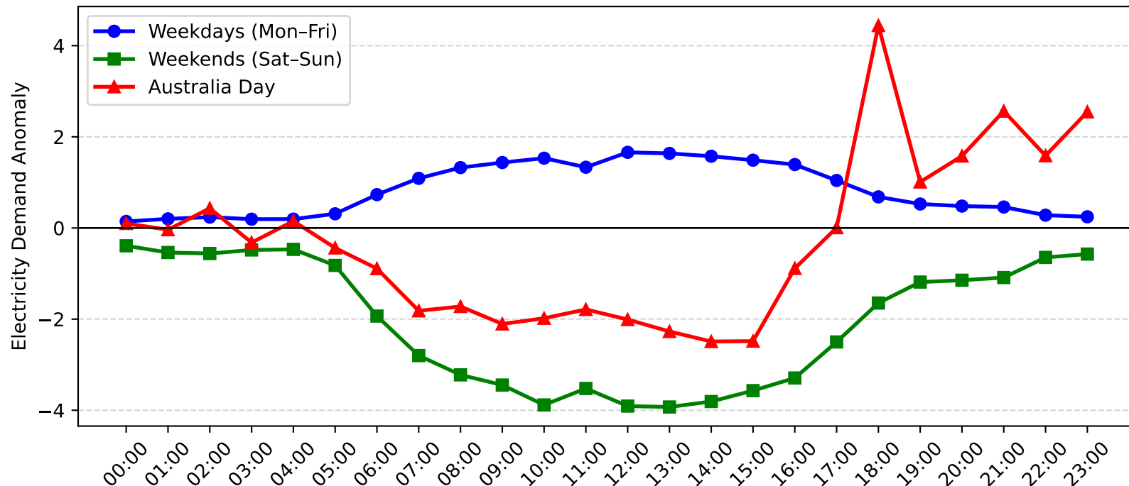
Homebush Bay Demand Anomaly: Australia Day vs Weekday/Weekend (2004-2005)
