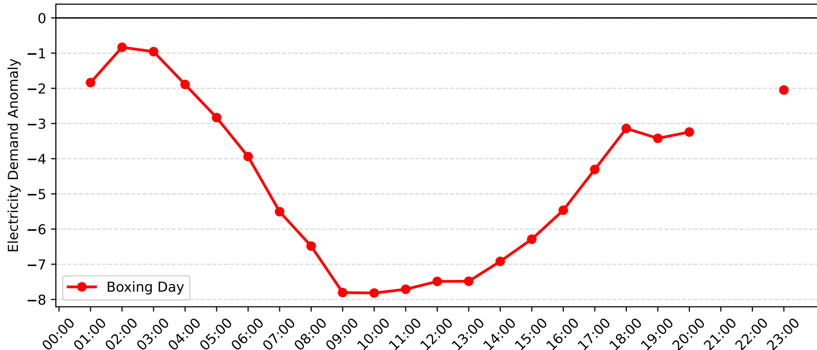
Auburn Demand Anomaly: Boxing Day (2008-2009)
