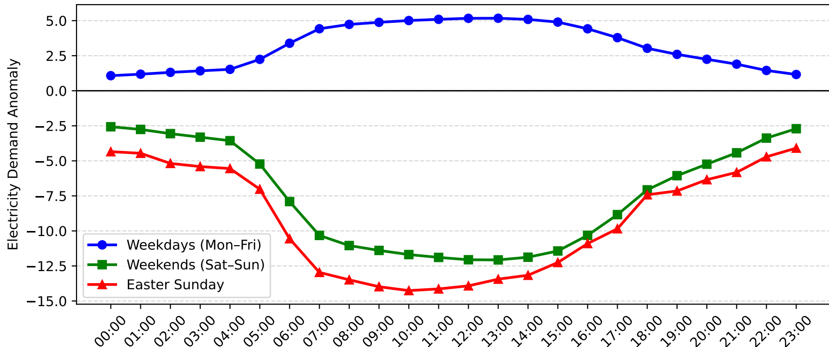
Flemington Demand Anomaly: Easter Sunday vs Weekday/Weekend (2014-2015)
