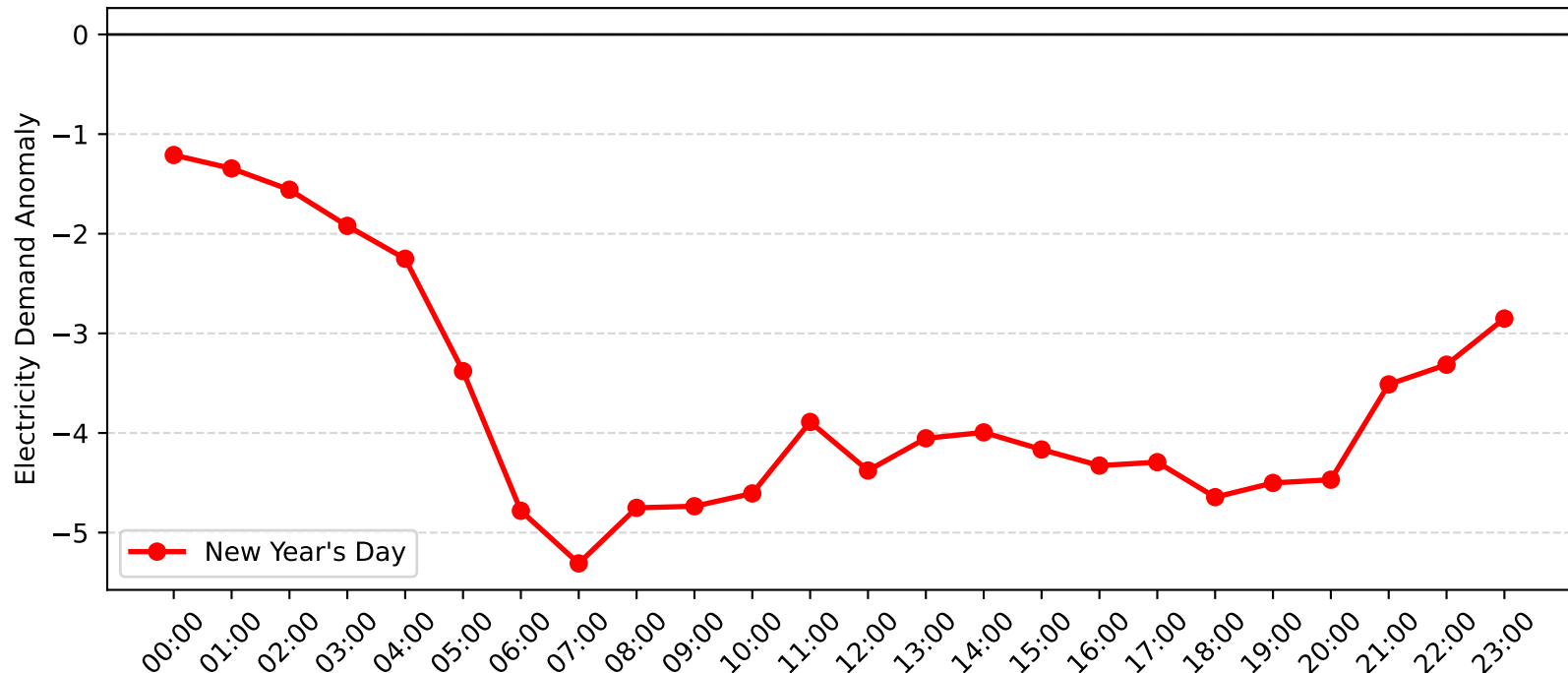
Enfield Demand Anomaly: New Year's Day (2004-2005)
