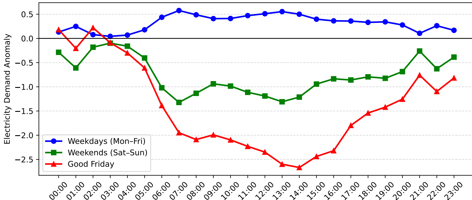
Gateshead Demand Anomaly: Good Friday vs Weekday/Weekend (2009-2010)
