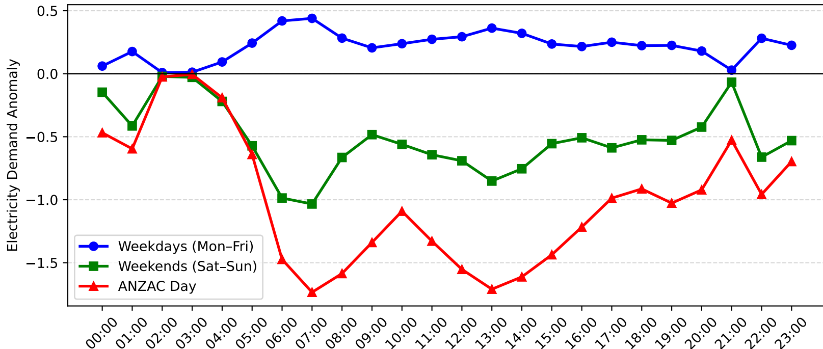
Gateshead Demand Anomaly: ANZAC Day vs Weekday/Weekend (2015-2016)
