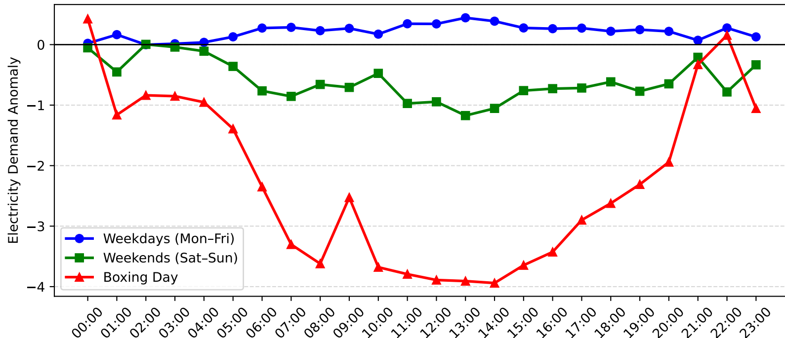
Gateshead Demand Anomaly: Boxing Day vs Weekday/Weekend (2007-2008)
