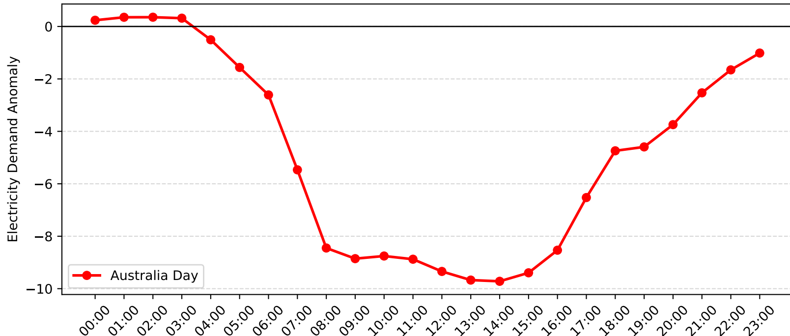
Gore Hill Demand Anomaly: Australia Day (2016-2017)
