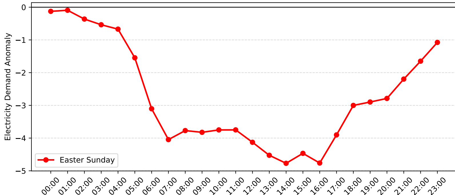
Rockdale Demand Anomaly: Easter Sunday (2006-2007)
