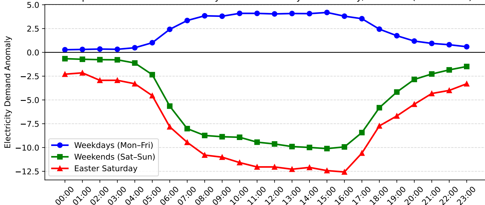
Macquarie Park Demand Anomaly: Easter Saturday vs Weekday/Weekend (2005-2006)
