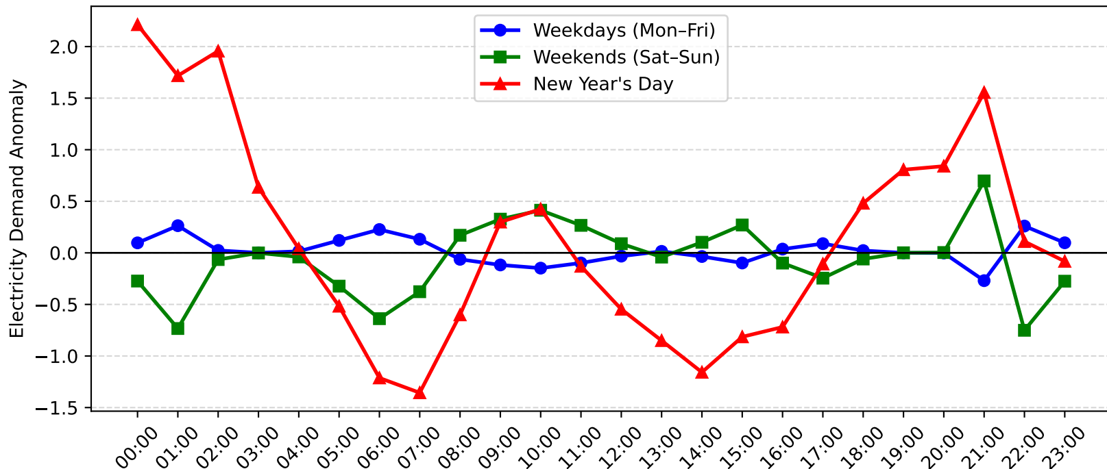
Nelson Bay Demand Anomaly: New Year's Day vs Weekday/Weekend (2015-2016)
