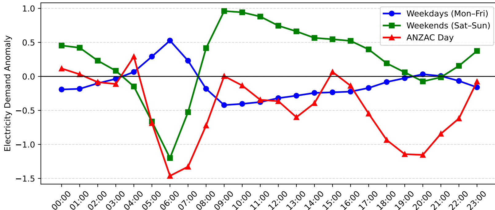
Umina Demand Anomaly: ANZAC Day vs Weekday/Weekend (2015-2016)
