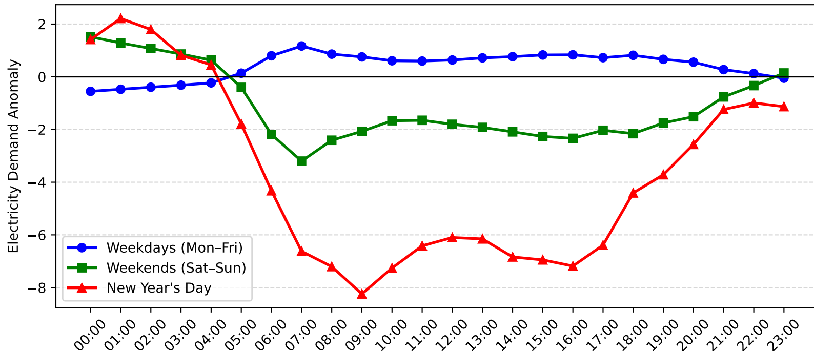
Kogarah Demand Anomaly: New Year's Day vs Weekday/Weekend (2013-2014)
