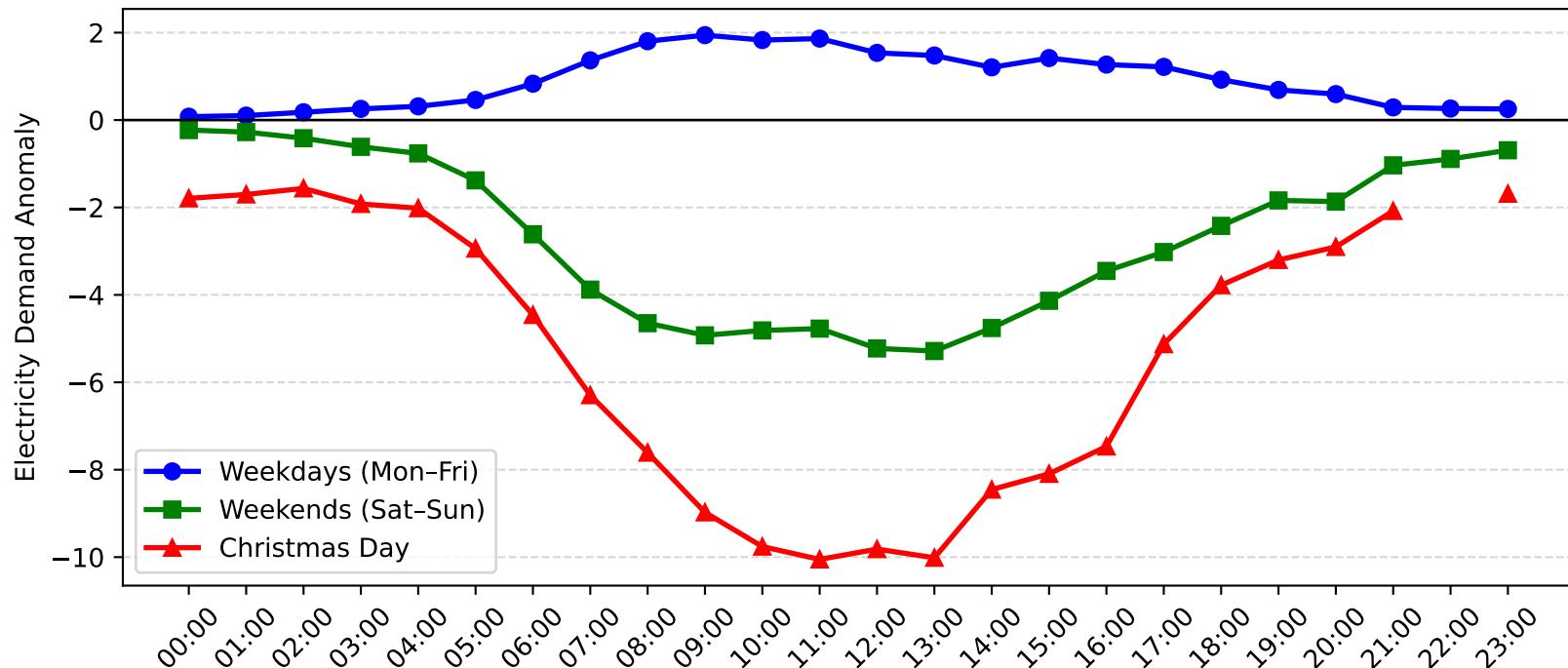
Auburn Demand Anomaly: Christmas Day vs Weekday/Weekend (2009-2010)
