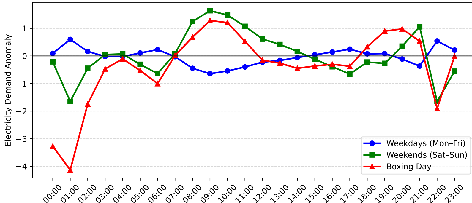
Nelson Bay Demand Anomaly: Boxing Day vs Weekday/Weekend (2008-2009)
