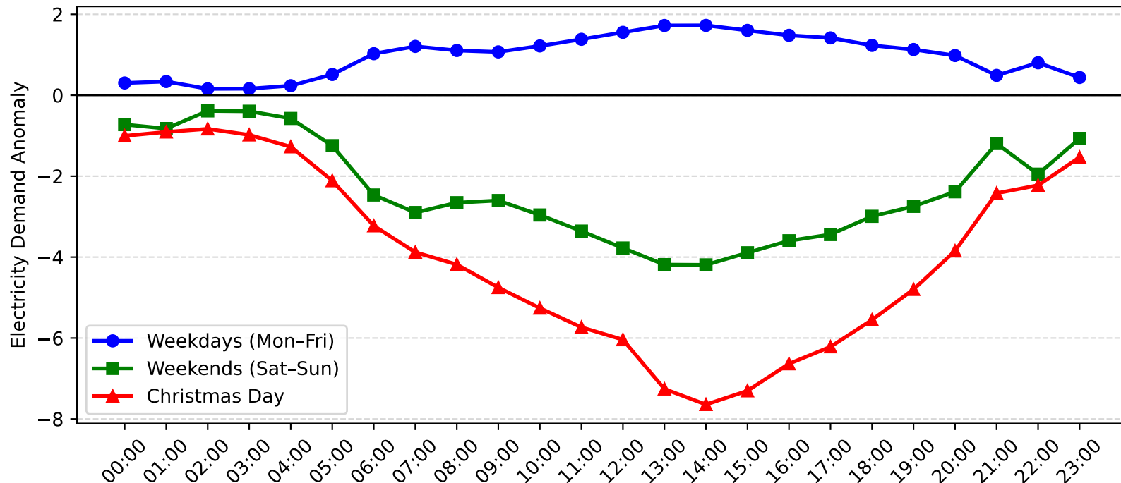
Argenton Demand Anomaly: Christmas Day vs Weekday/Weekend (2015-2016)
