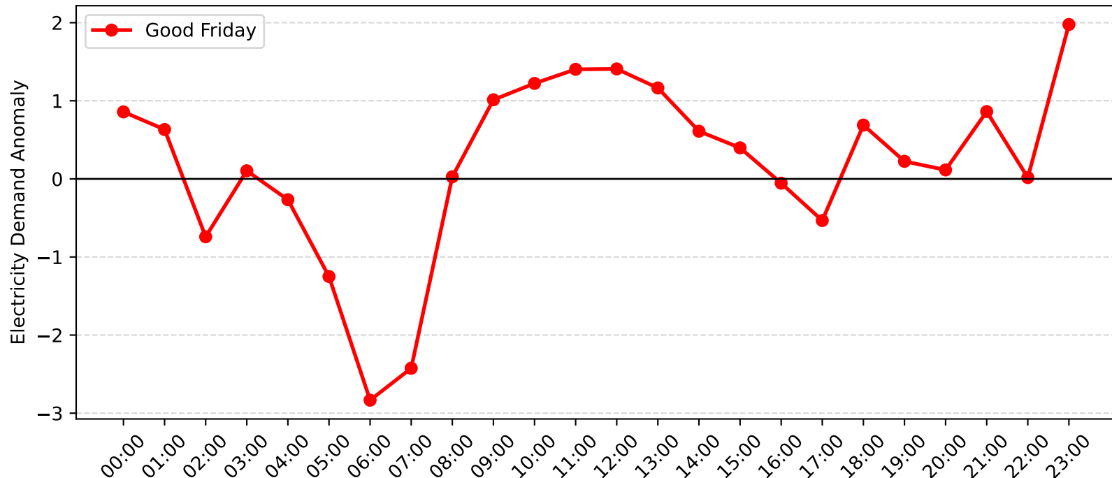
Avoca Demand Anomaly: Good Friday (2005-2006)
