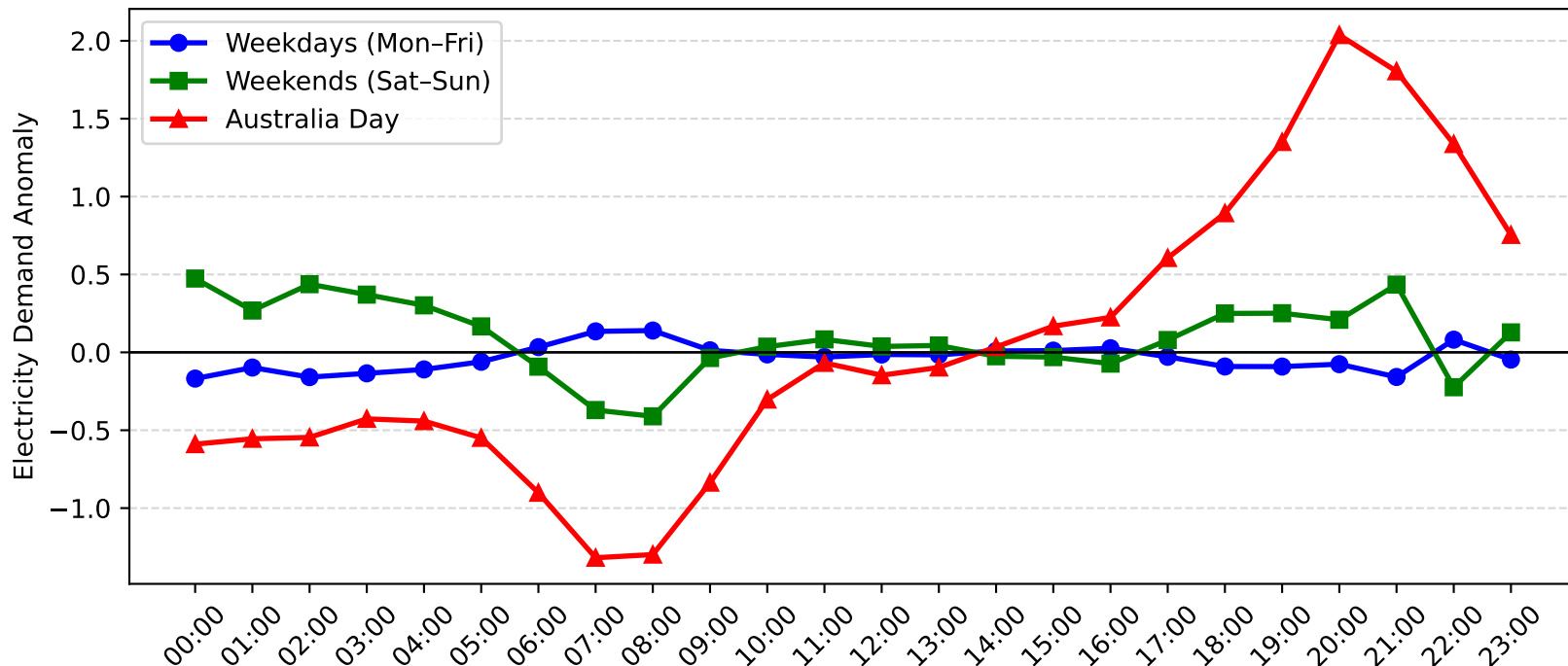
Adamstown Demand Anomaly: Australia Day vs Weekday/Weekend (2010-2011)
