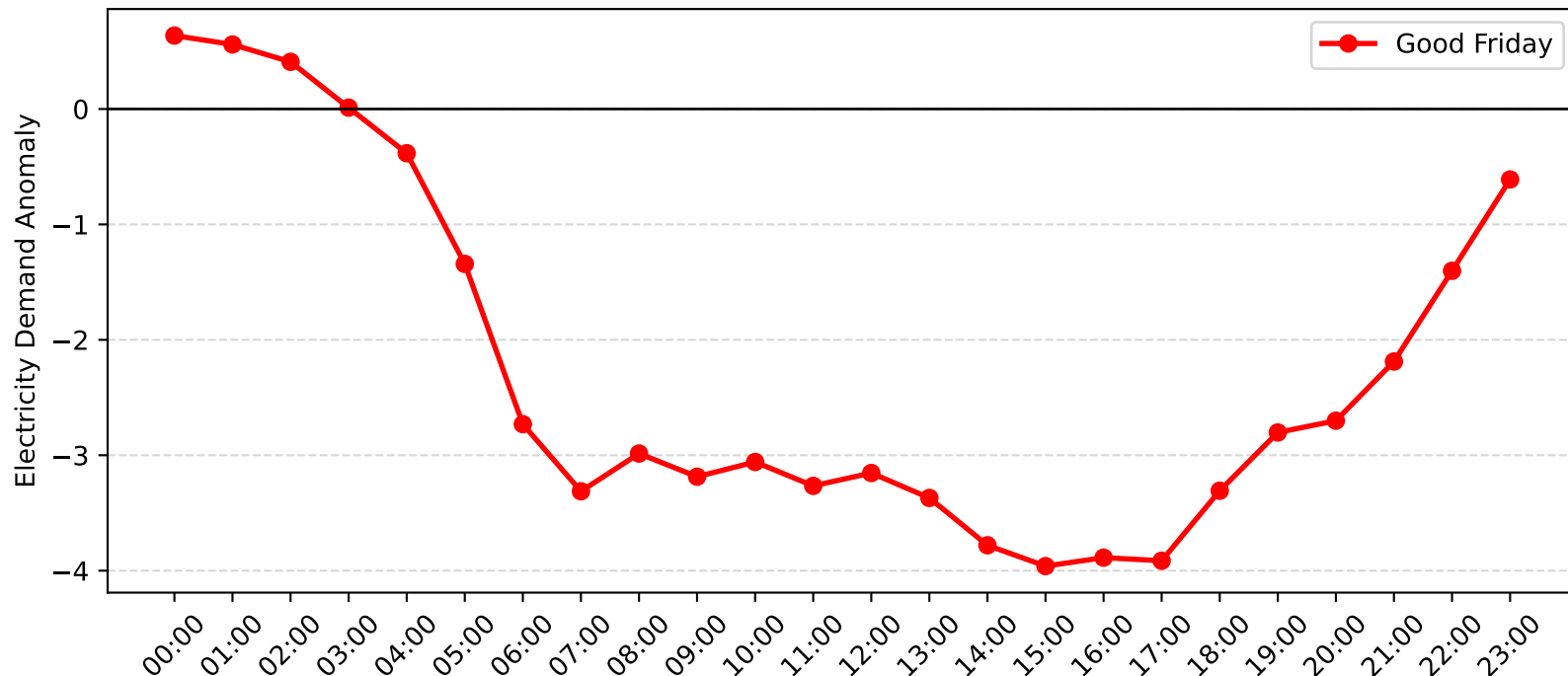
Charmhaven Demand Anomaly: Good Friday (2013-2014)
