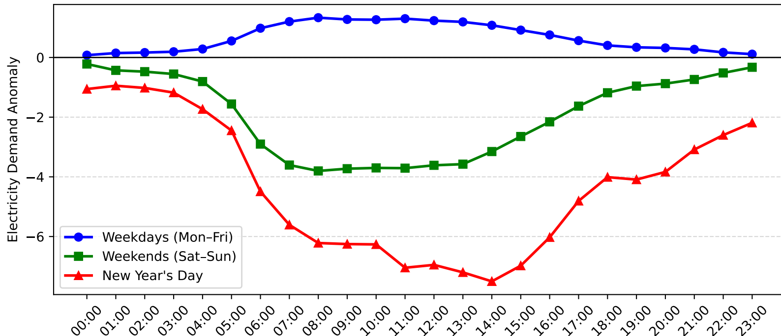
Wyong Demand Anomaly: New Year's Day vs Weekday/Weekend (2015-2016)
