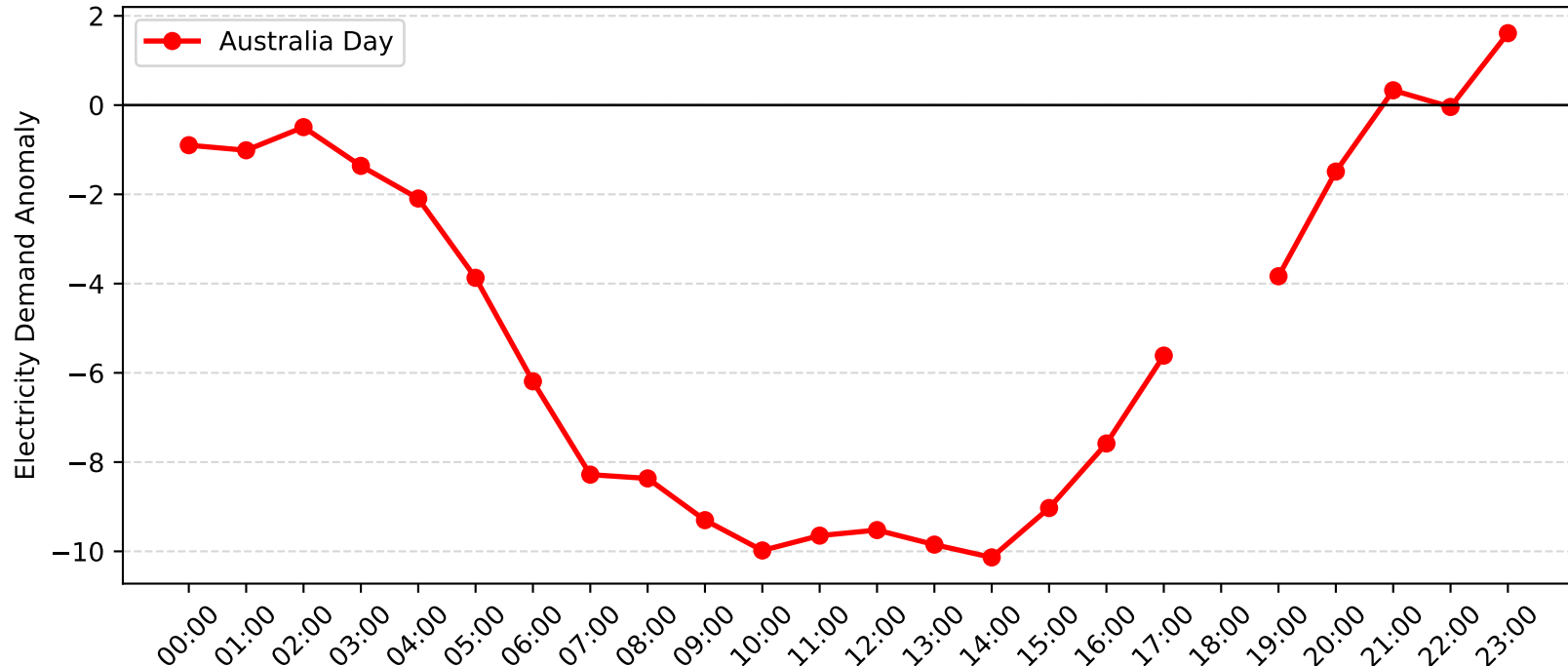
Homebush Bay Demand Anomaly: Australia Day (2005-2006)
