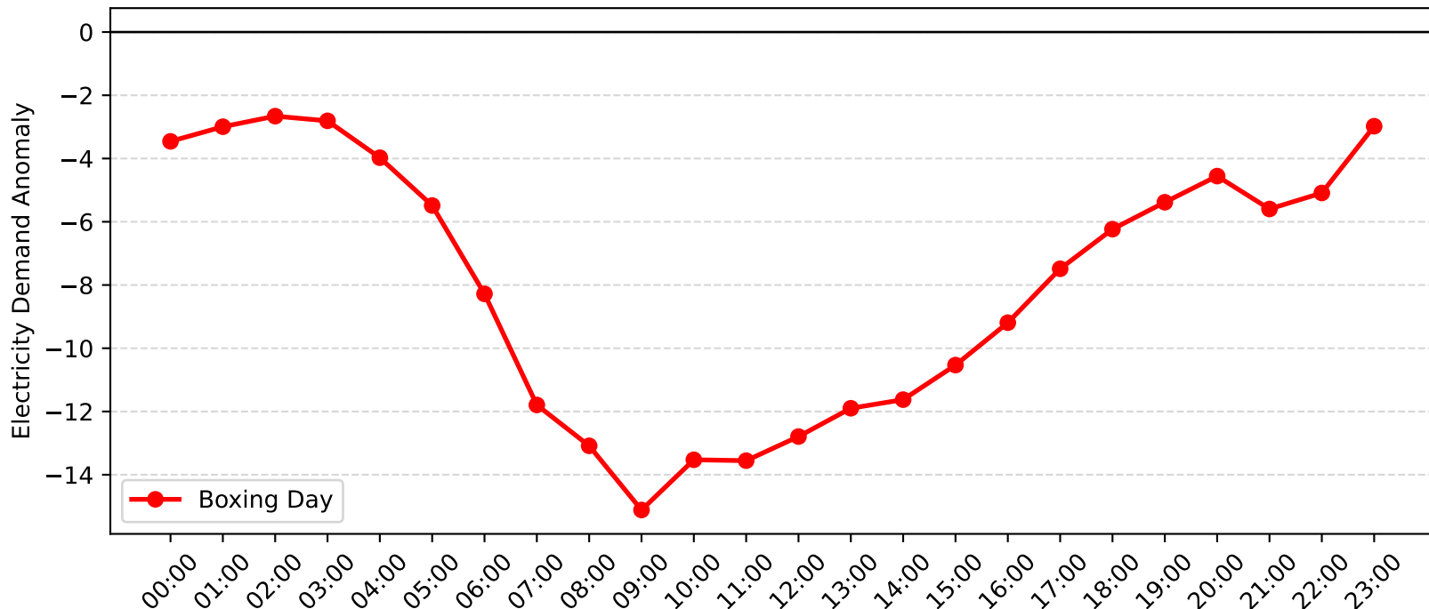
Homebush Bay Demand Anomaly: Boxing Day (2008-2009)
