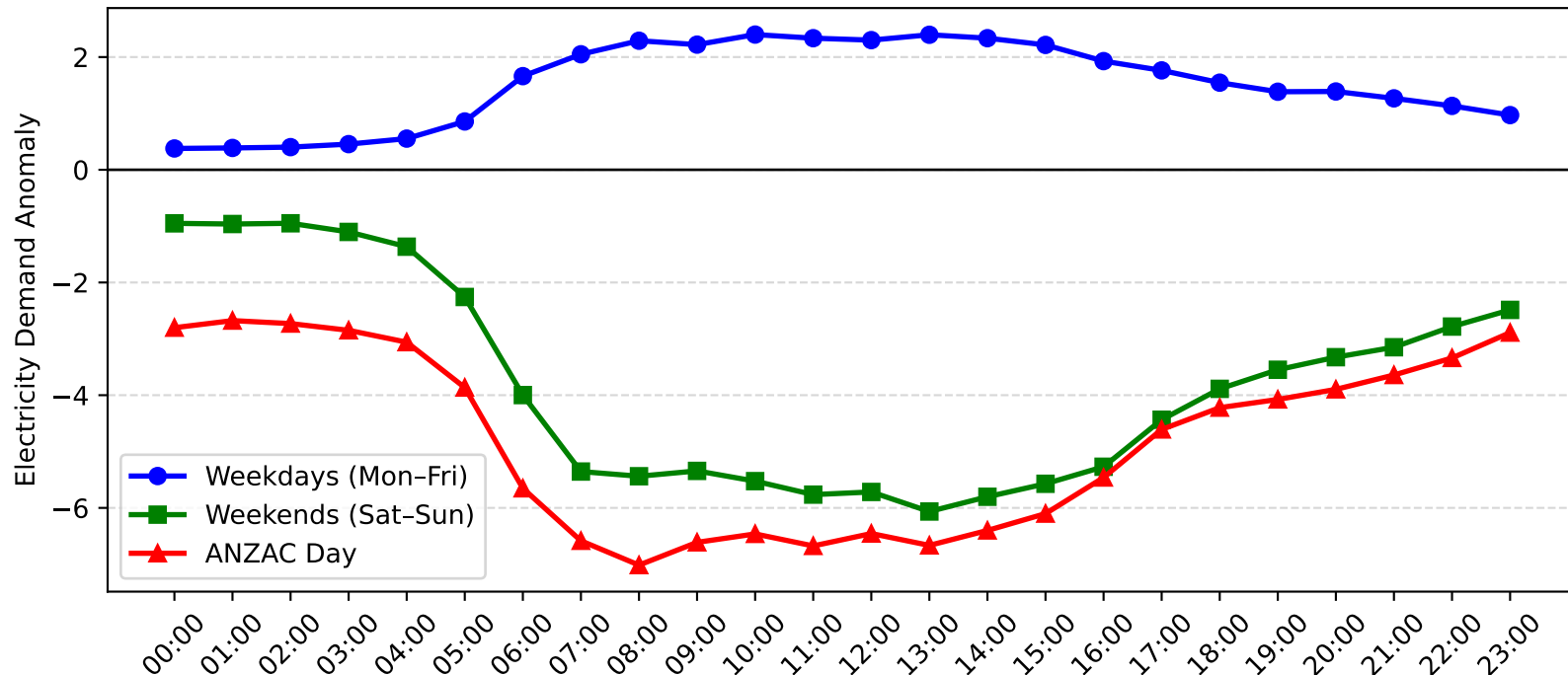
Leightonfield Demand Anomaly: ANZAC Day vs Weekday/Weekend (2005-2006)
