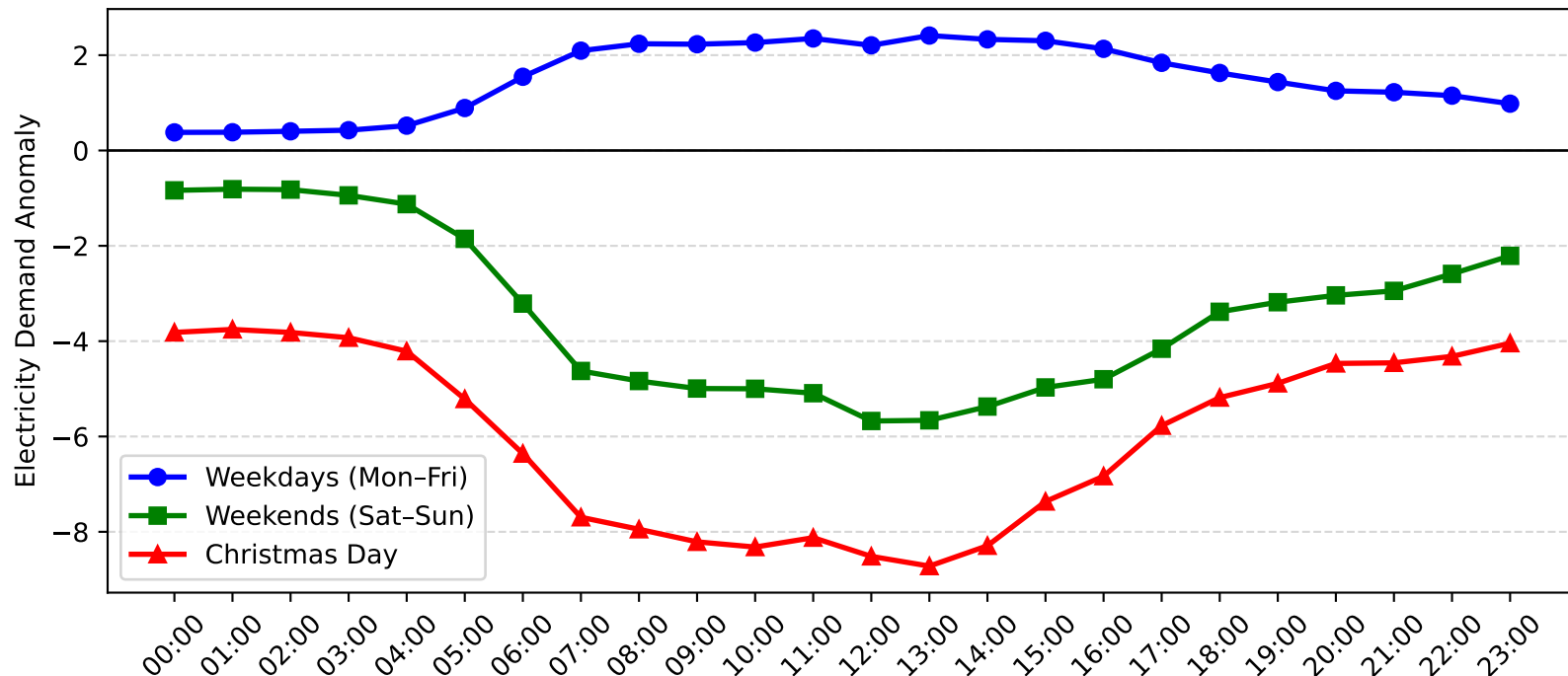
Leightonfield Demand Anomaly: Christmas Day vs Weekday/Weekend (2004-2005)
