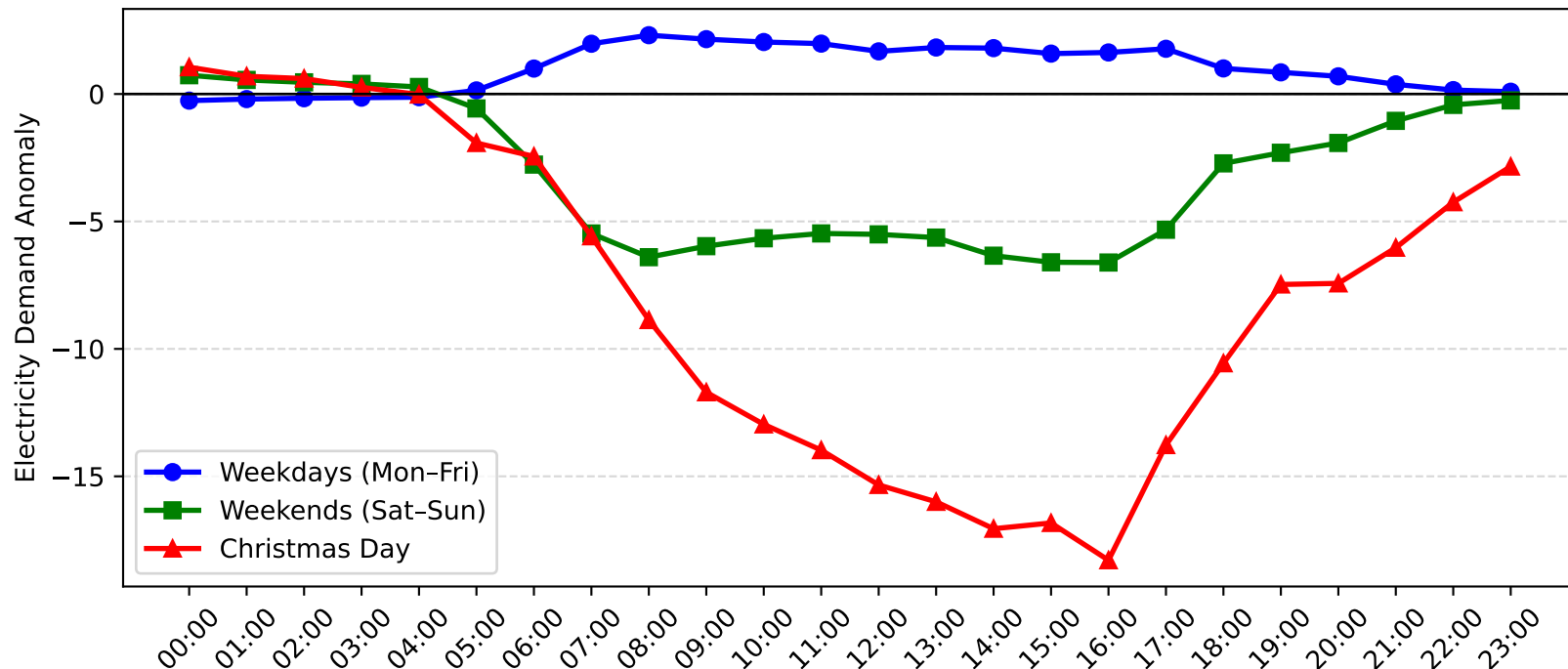
Castle Cove Demand Anomaly: Christmas Day vs Weekday/Weekend (2012-2013)
