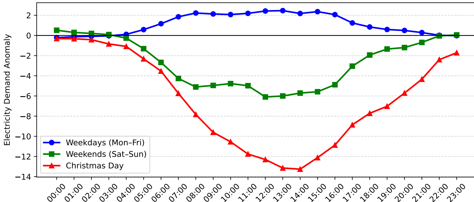
West Gosford Demand Anomaly: Christmas Day vs Weekday/Weekend (2005-2006)
