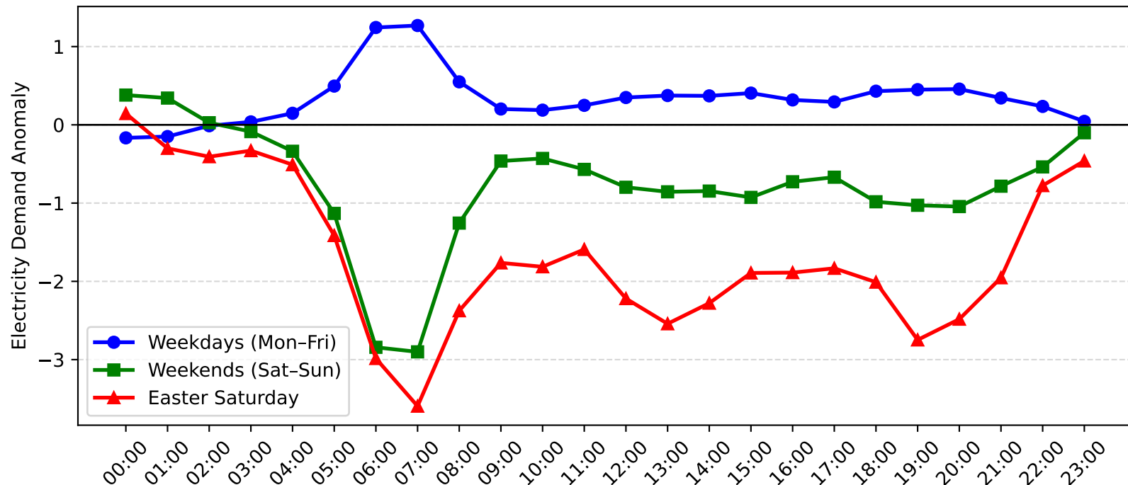
Mortdale Demand Anomaly: Easter Saturday vs Weekday/Weekend (2017-2018)
