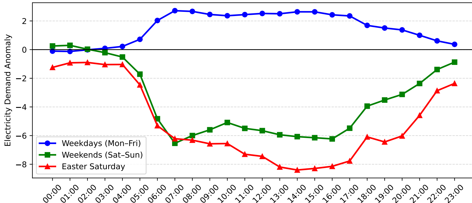
Burwood Demand Anomaly: Easter Saturday vs Weekday/Weekend (2006-2007)
