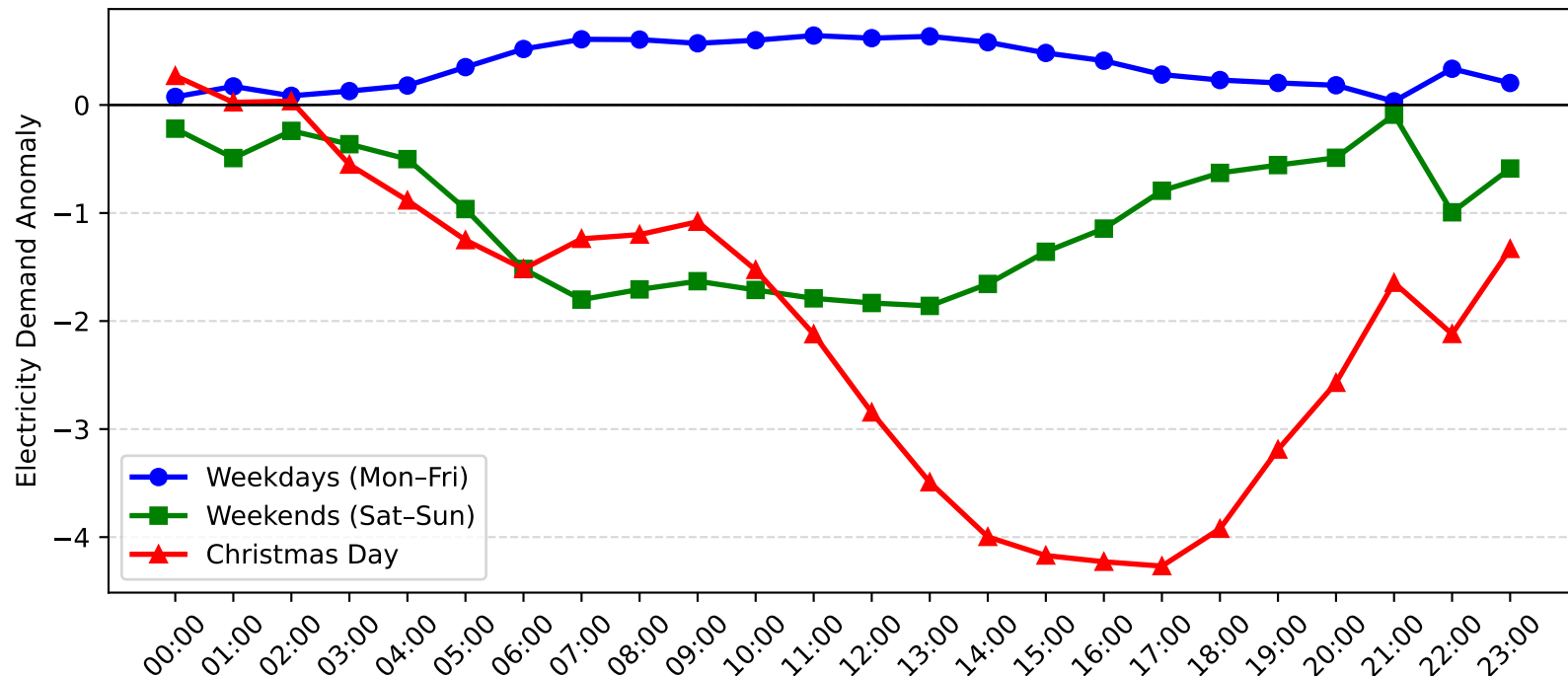
Cardiff Demand Anomaly: Christmas Day vs Weekday/Weekend (2013-2014)
