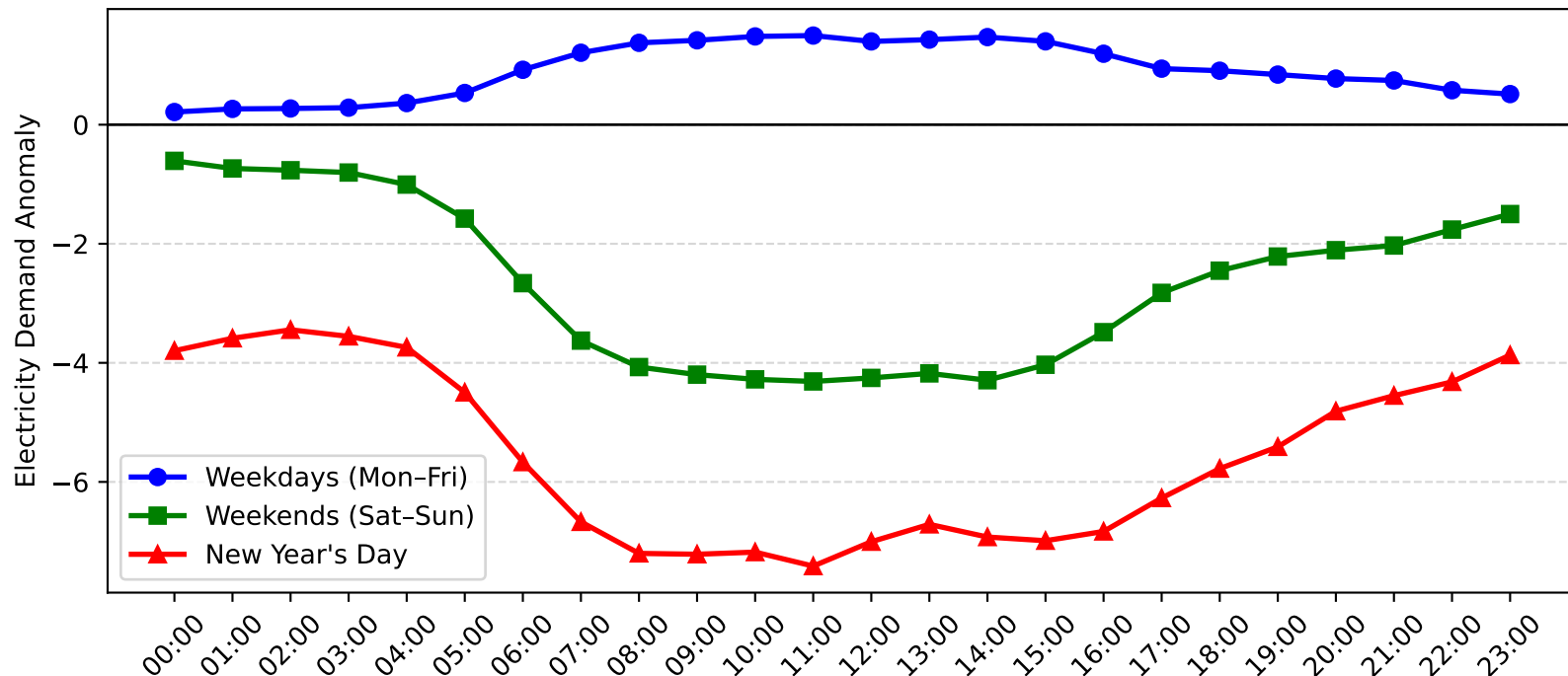
Leightonfield Demand Anomaly: New Year's Day vs Weekday/Weekend (2014-2015)
