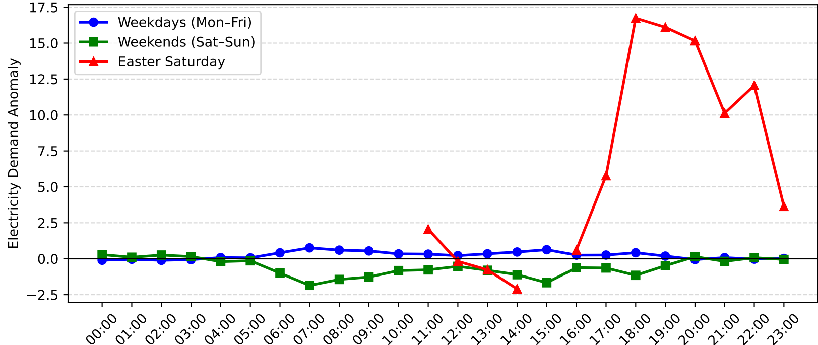
Pennant Hills Demand Anomaly: Easter Saturday vs Weekday/Weekend (2004-2005)
