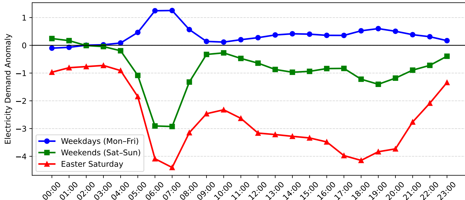
Dee Why West Demand Anomaly: Easter Saturday vs Weekday/Weekend (2013-2014)
