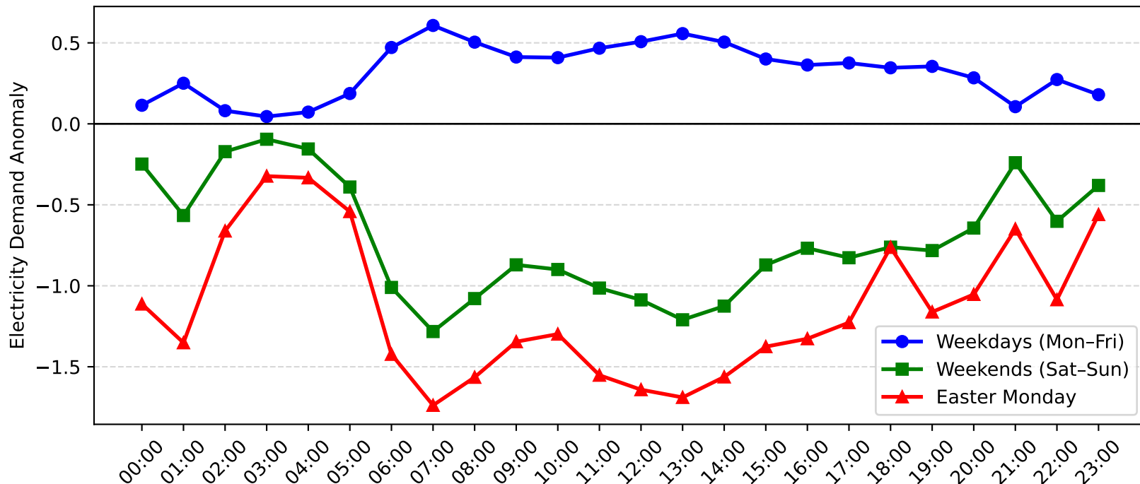
Gateshead Demand Anomaly: Easter Monday vs Weekday/Weekend (2009-2010)
