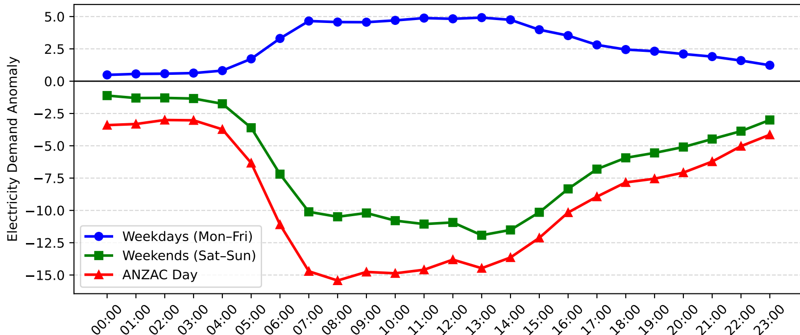
Milperra Demand Anomaly: ANZAC Day vs Weekday/Weekend (2010-2011)
