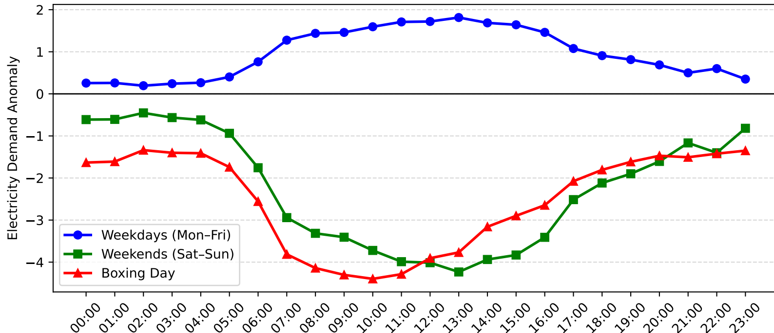
Mayfield West Demand Anomaly: Boxing Day vs Weekday/Weekend (2015-2016)
