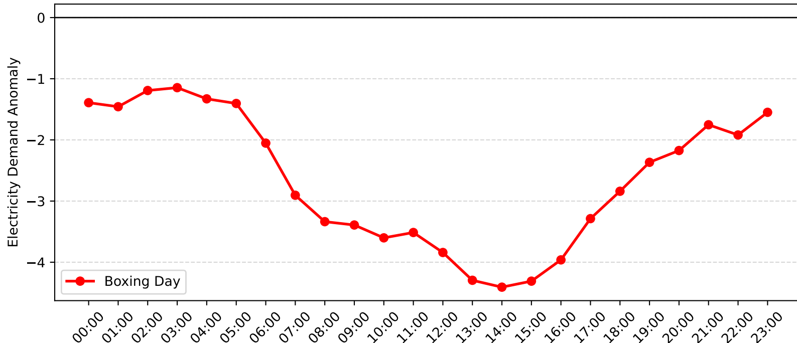
Mayfield West Demand Anomaly: Boxing Day (2009-2010)
