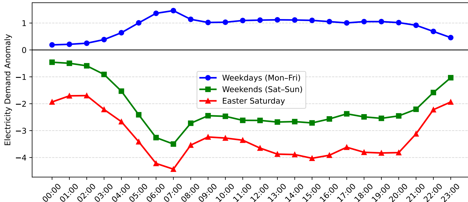
Lisarow Demand Anomaly: Easter Saturday vs Weekday/Weekend (2007-2008)
