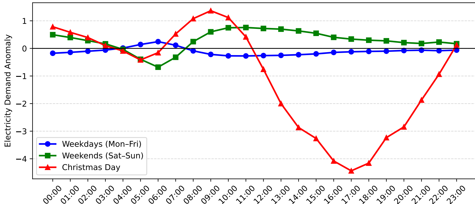
Umina Demand Anomaly: Christmas Day vs Weekday/Weekend (2012-2013)
