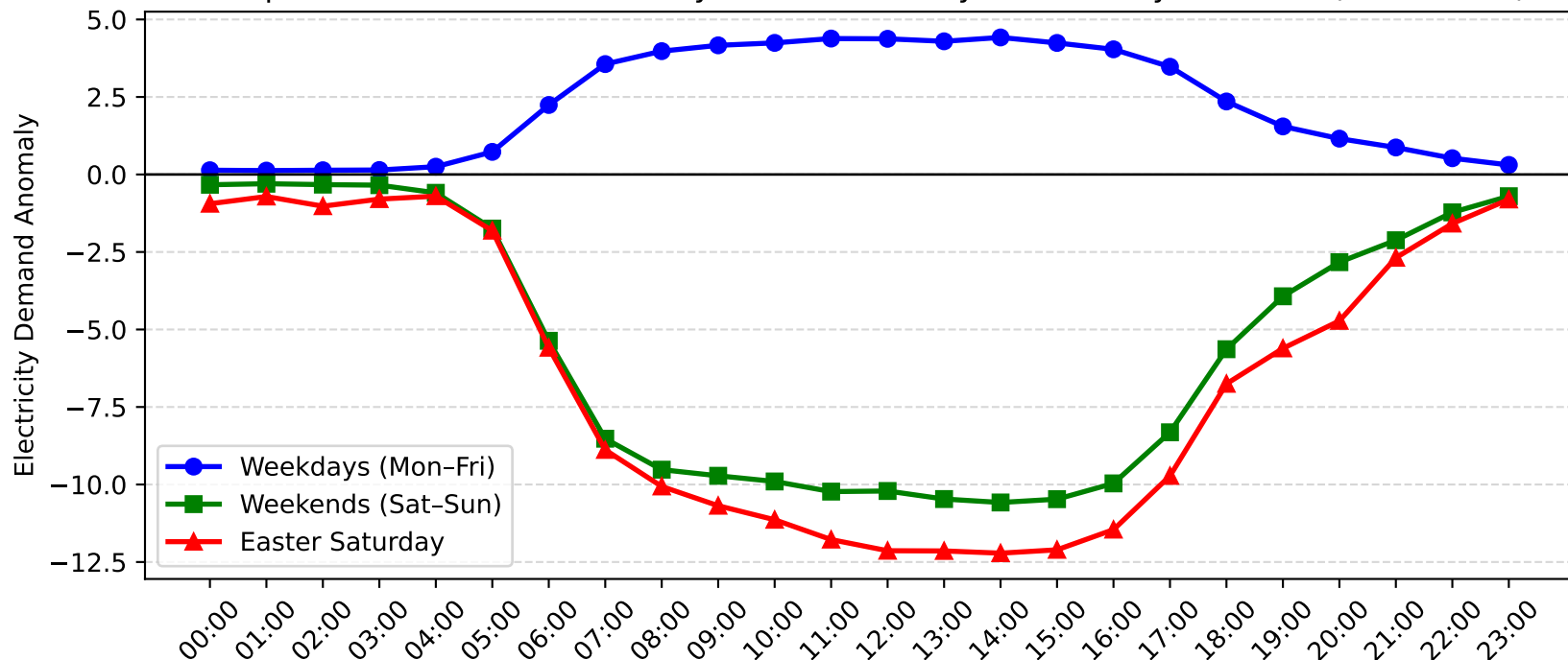
Macquarie Park Demand Anomaly: Easter Saturday vs Weekday/Weekend (2007-2008)
