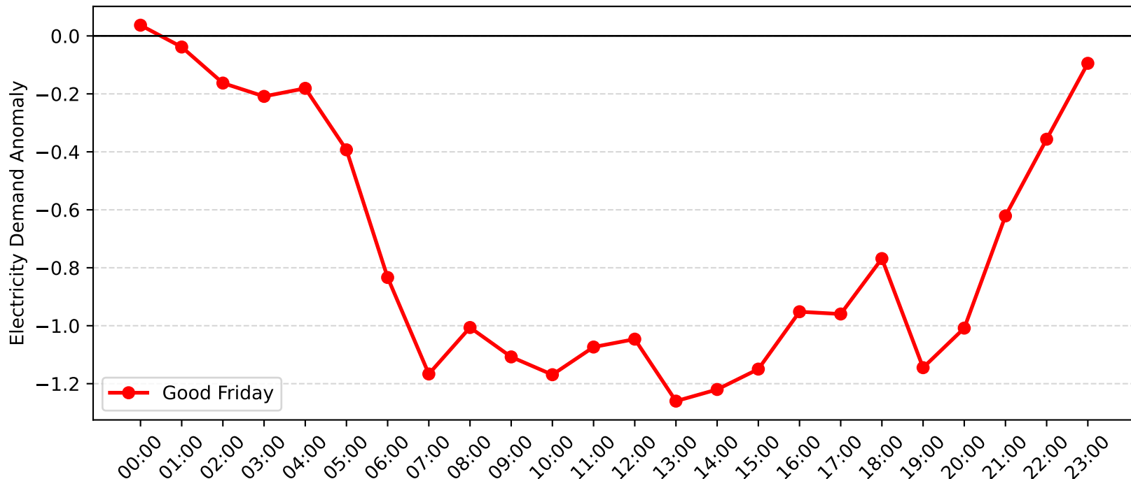
Narrabeen Demand Anomaly: Good Friday (2017-2018)
