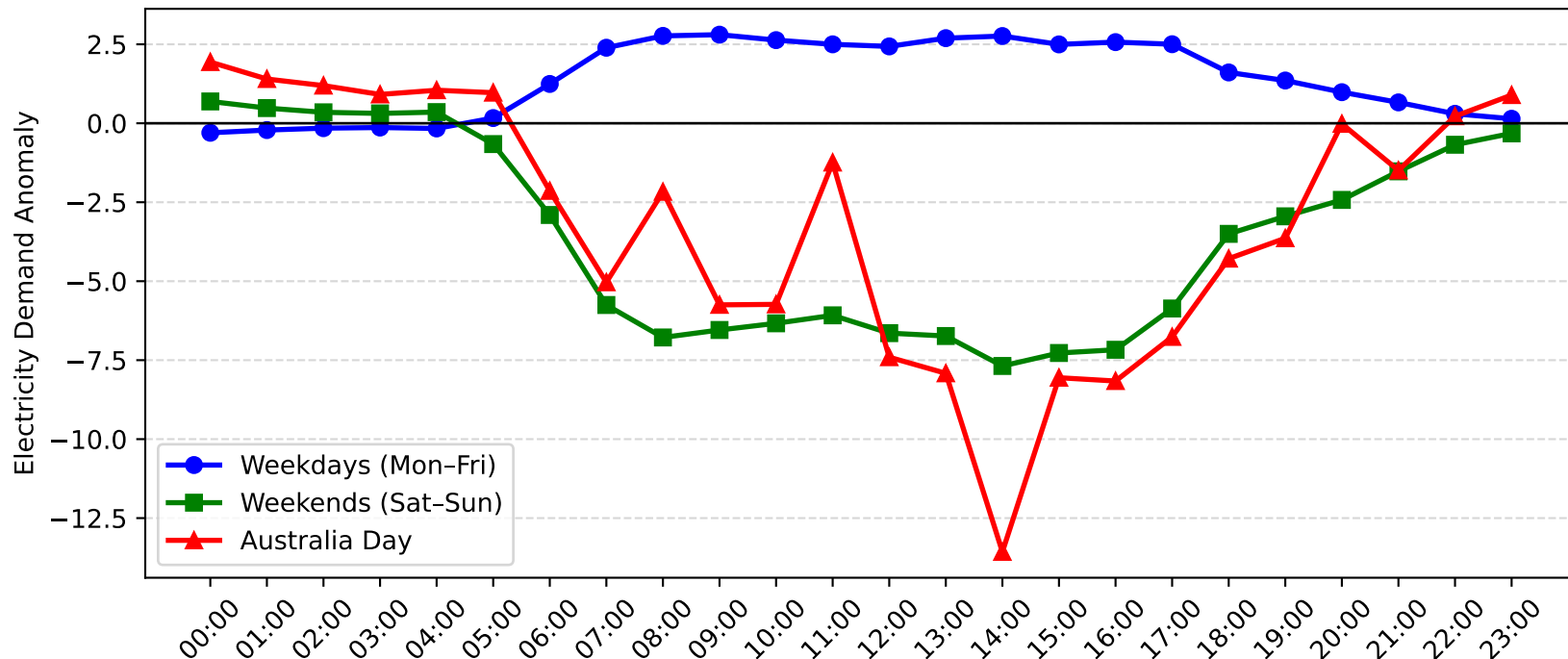
Castle Cove Demand Anomaly: Australia Day vs Weekday/Weekend (2013-2014)
