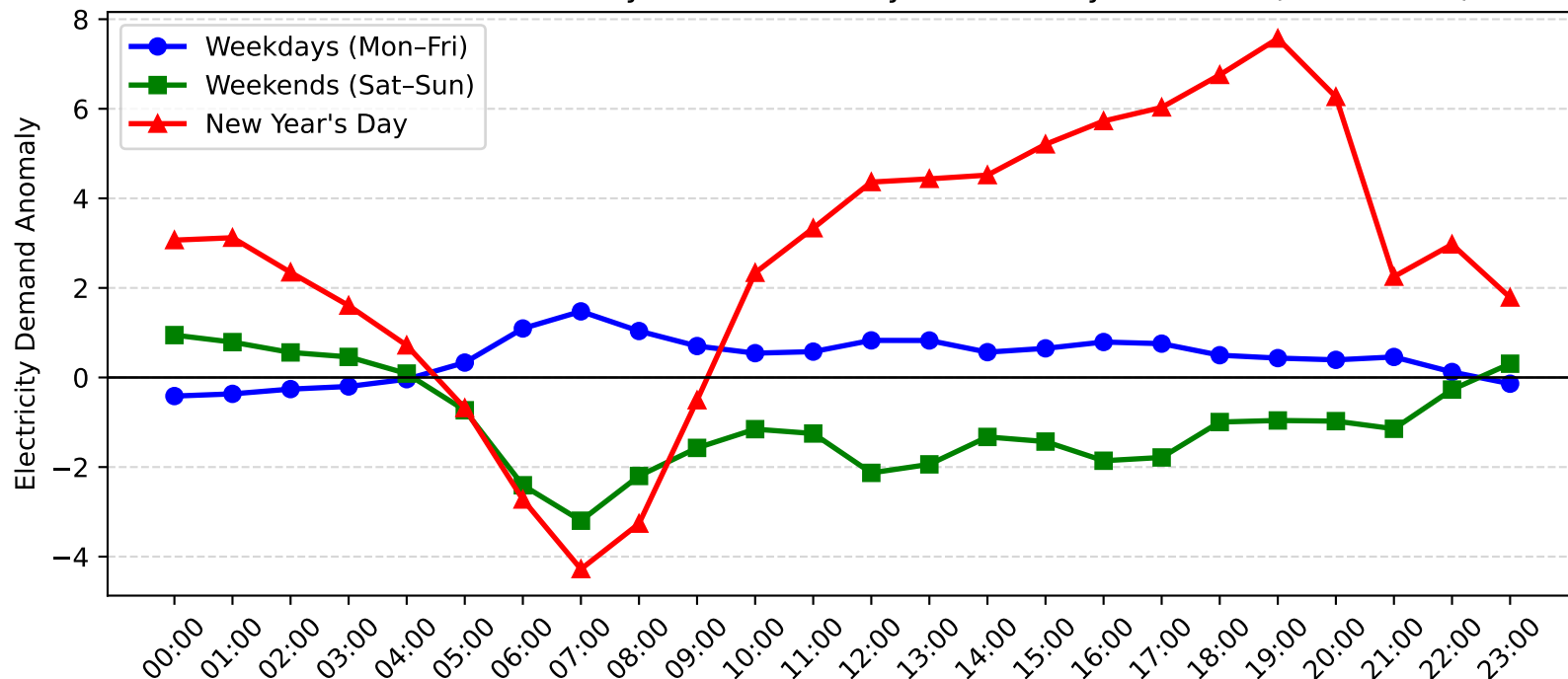
Mortdale Demand Anomaly: New Year's Day vs Weekday/Weekend (2005-2006)
