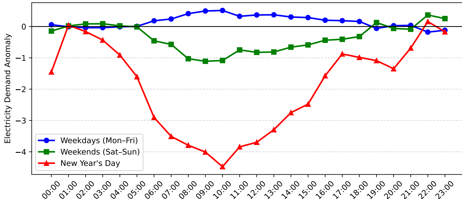
Wyong Demand Anomaly: New Year's Day vs Weekday/Weekend (2004-2005)
