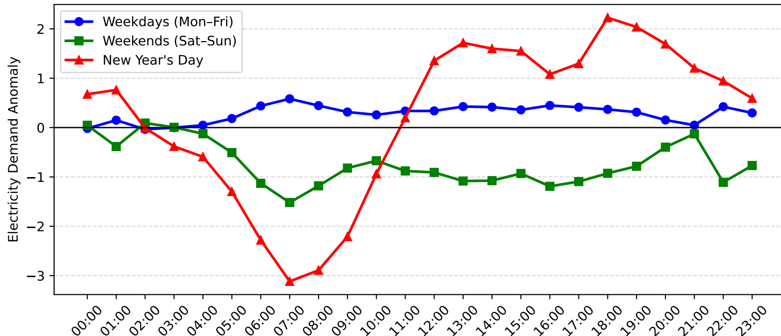
Jesmond Demand Anomaly: New Year's Day vs Weekday/Weekend (2013-2014)
