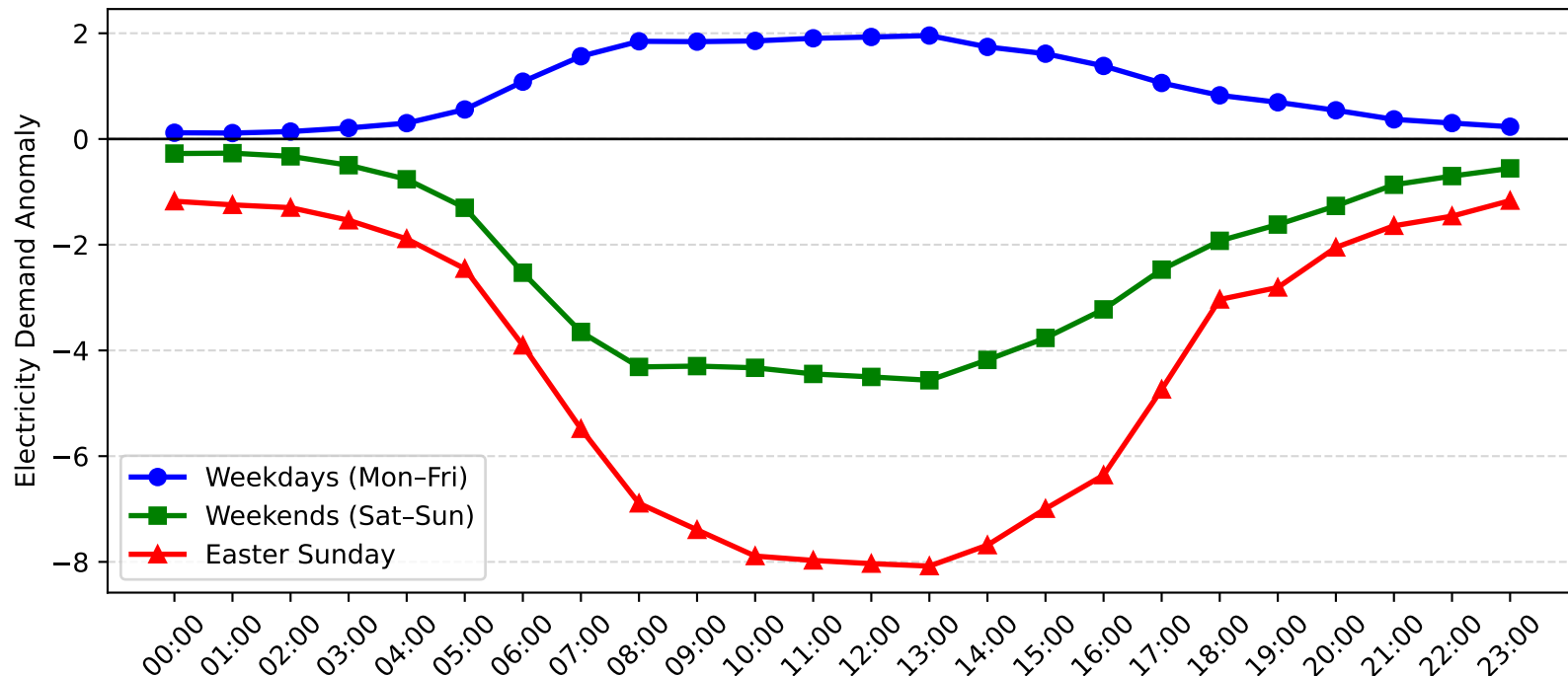
Auburn Demand Anomaly: Easter Sunday vs Weekday/Weekend (2014-2015)
