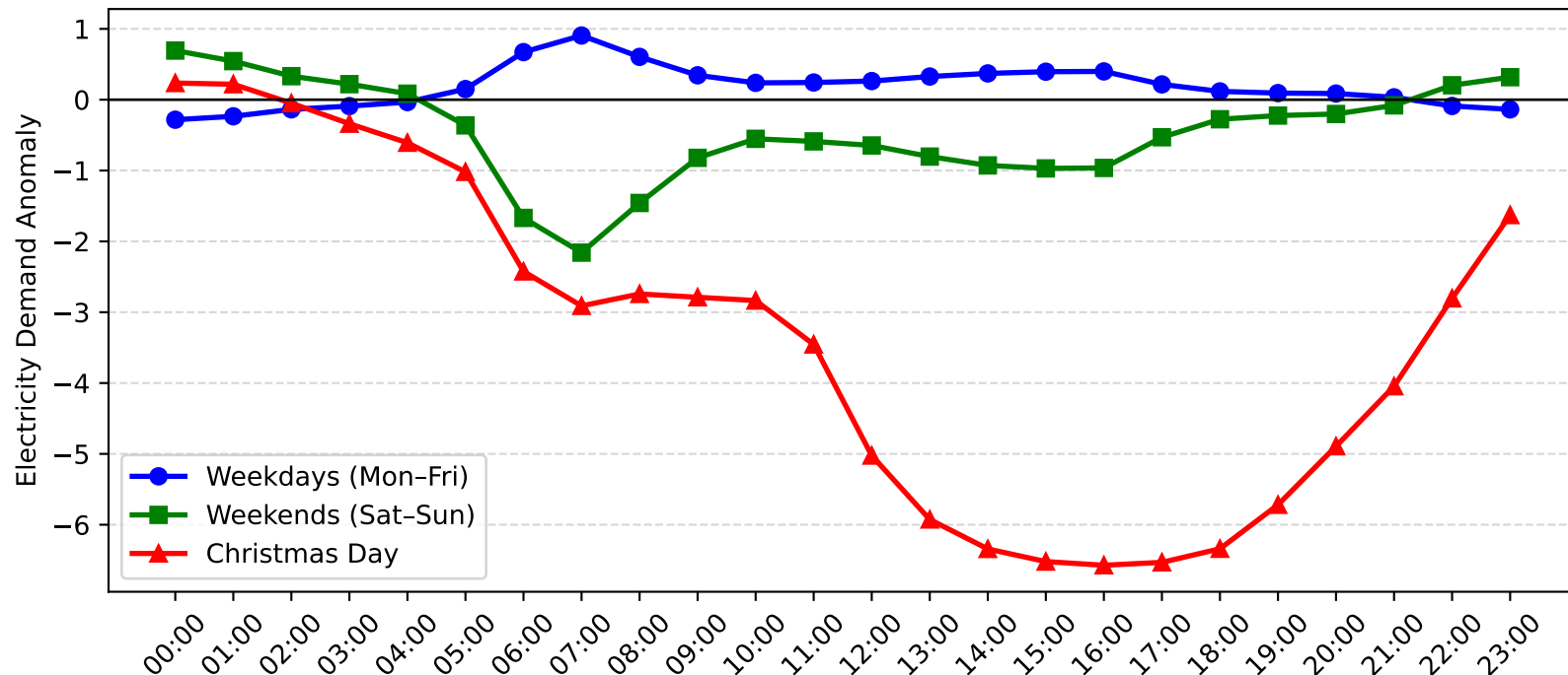
Five Dock Demand Anomaly: Christmas Day vs Weekday/Weekend (2006-2007)
