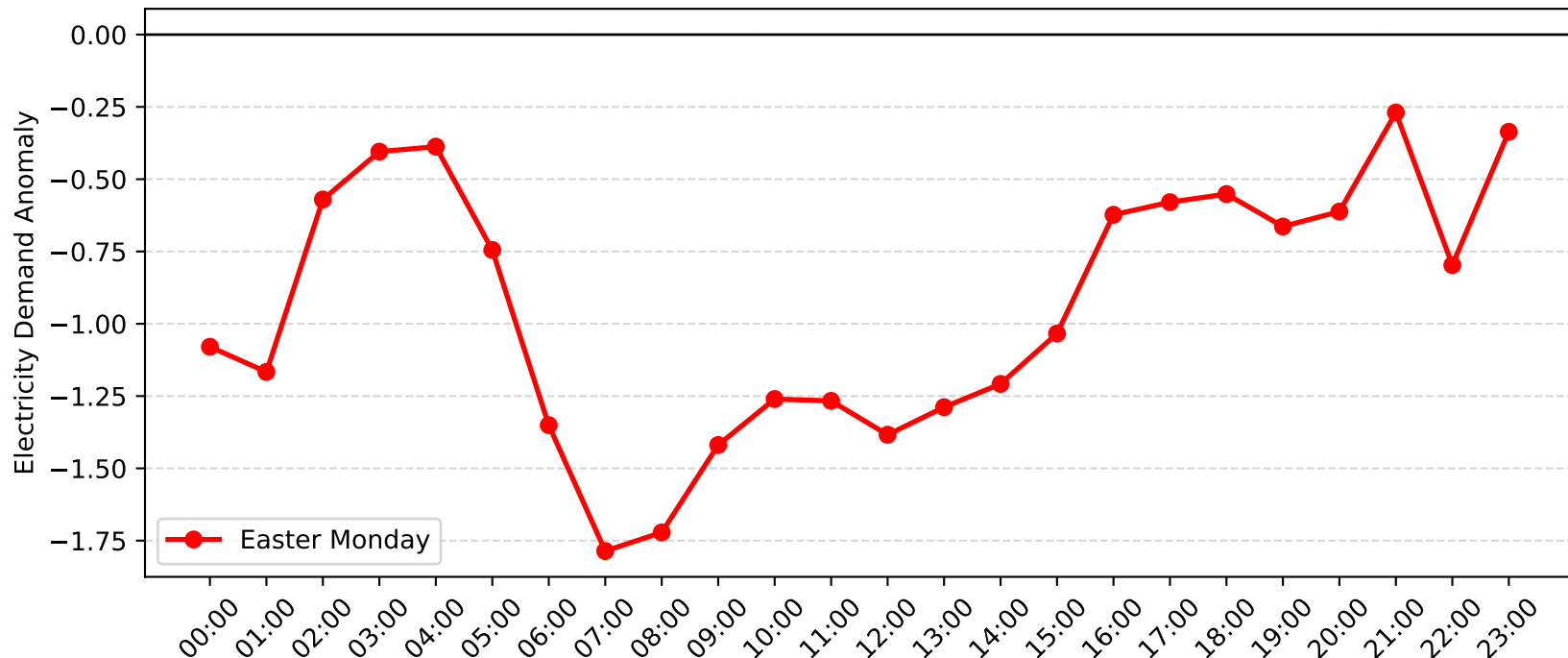
Gateshead Demand Anomaly: Easter Monday (2016-2017)
