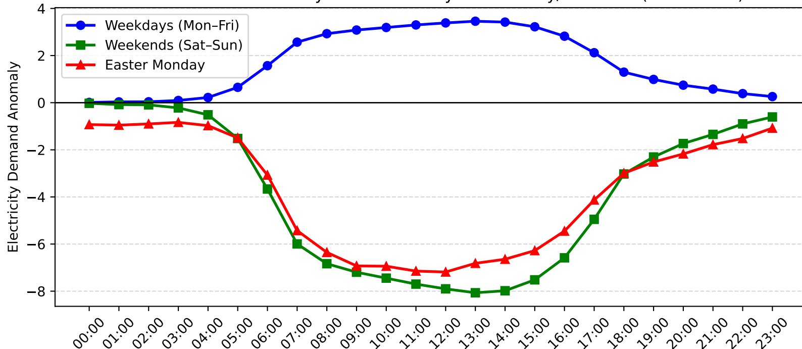
Mascot Demand Anomaly: Easter Monday vs Weekday/Weekend (2013-2014)
