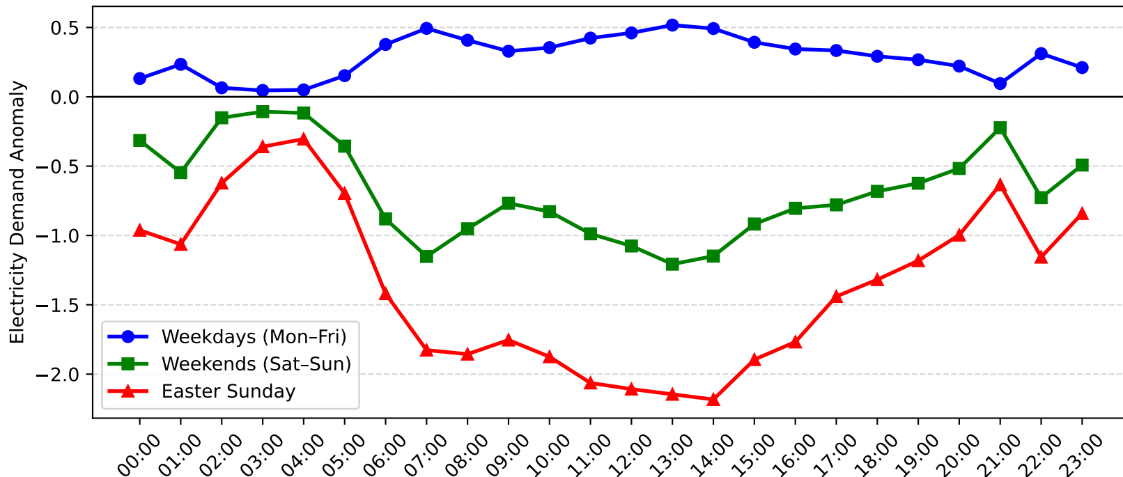
Gateshead Demand Anomaly: Easter Sunday vs Weekday/Weekend (2012-2013)
