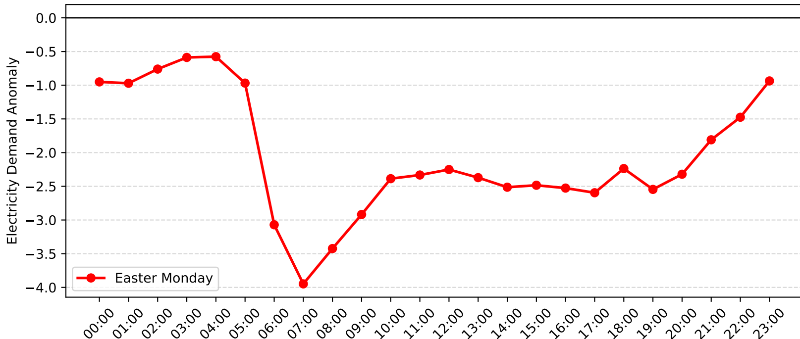
Pymble Demand Anomaly: Easter Monday (2011-2012)
