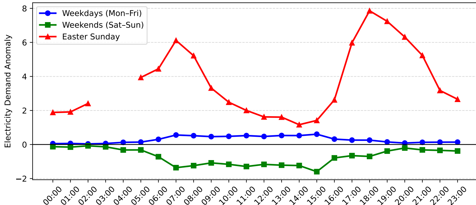
Caringbah Demand Anomaly: Easter Sunday vs Weekday/Weekend (2004-2005)
