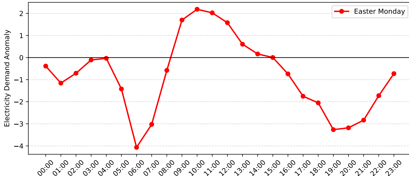
Cronulla Demand Anomaly: Easter Monday (2010-2011)
