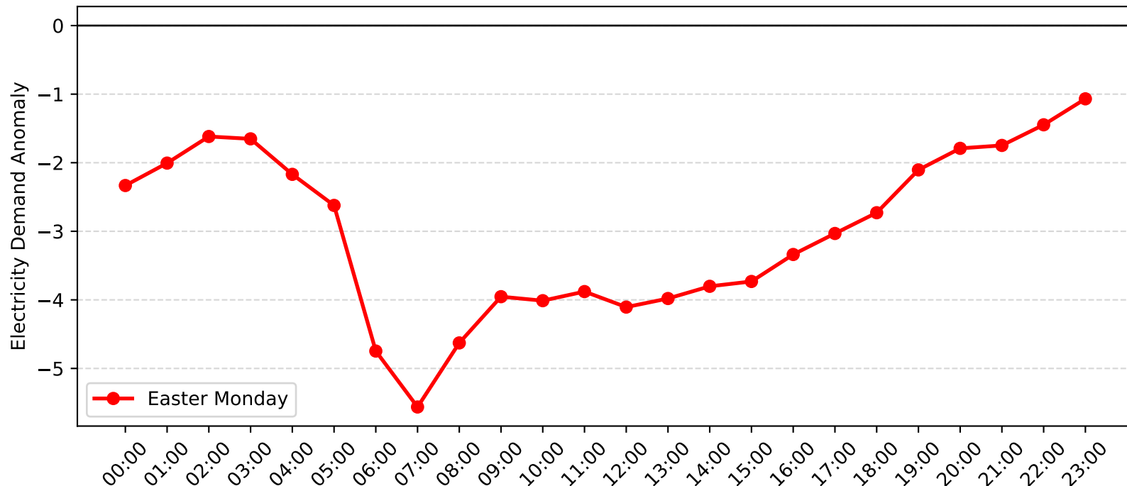
Matraverse Demand Anomaly: Easter Monday (2013-2014)
