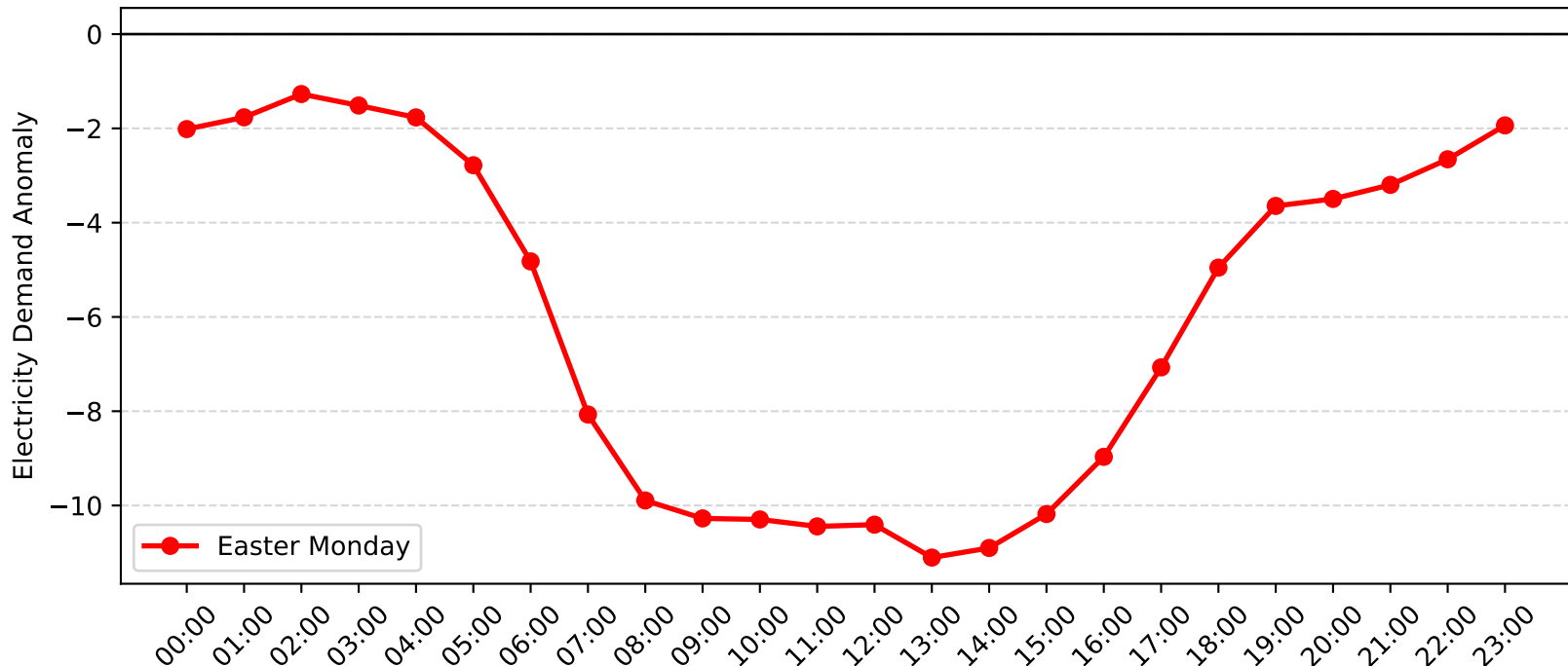
Mascot Demand Anomaly: Easter Monday (2007-2008)
