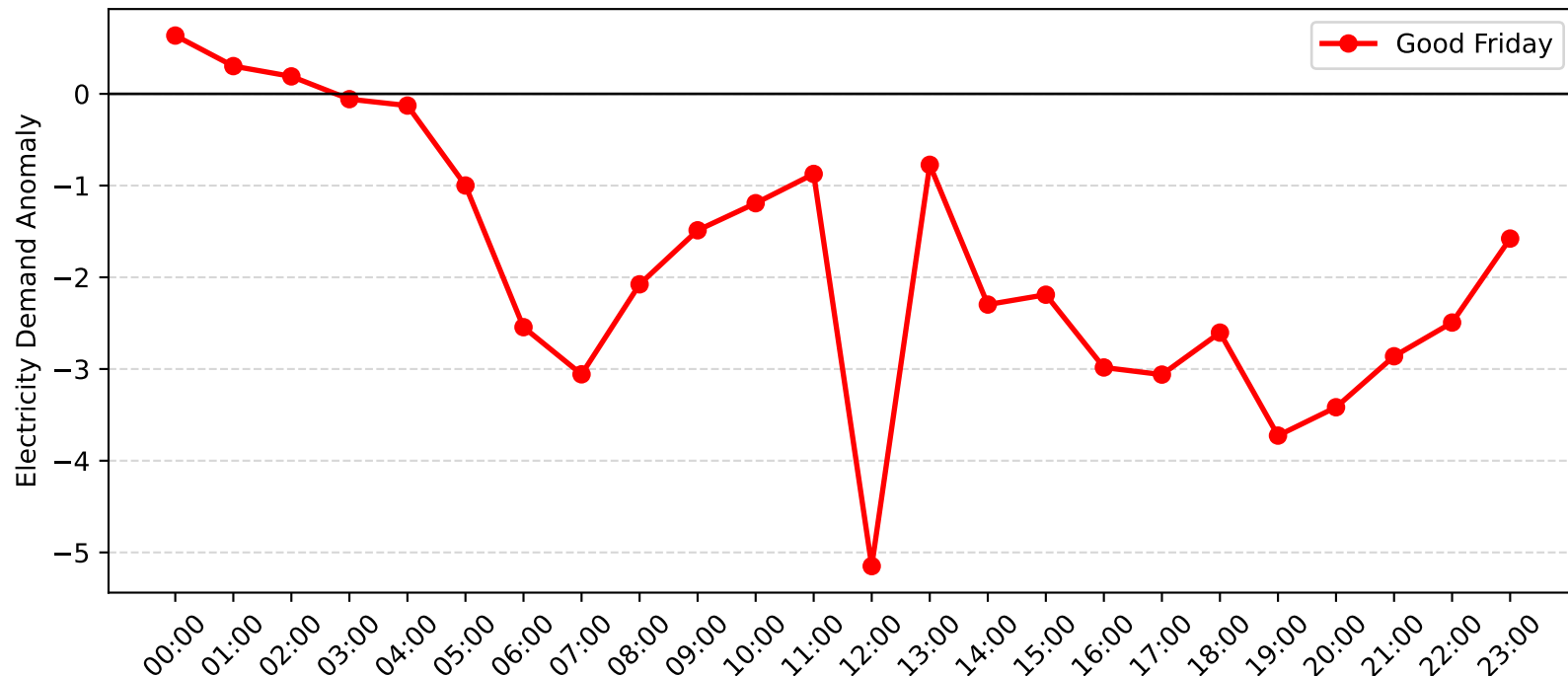
Dulwich Hill Demand Anomaly: Good Friday (2017-2018)
