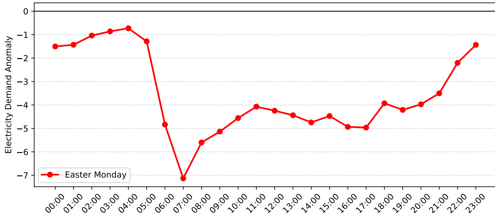
Epping Demand Anomaly: Easter Monday (2010-2011)
