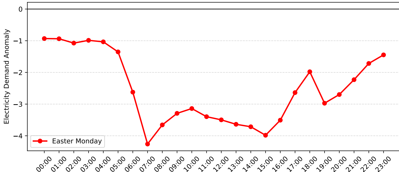
Epping Demand Anomaly: Easter Monday (2017-2018)
