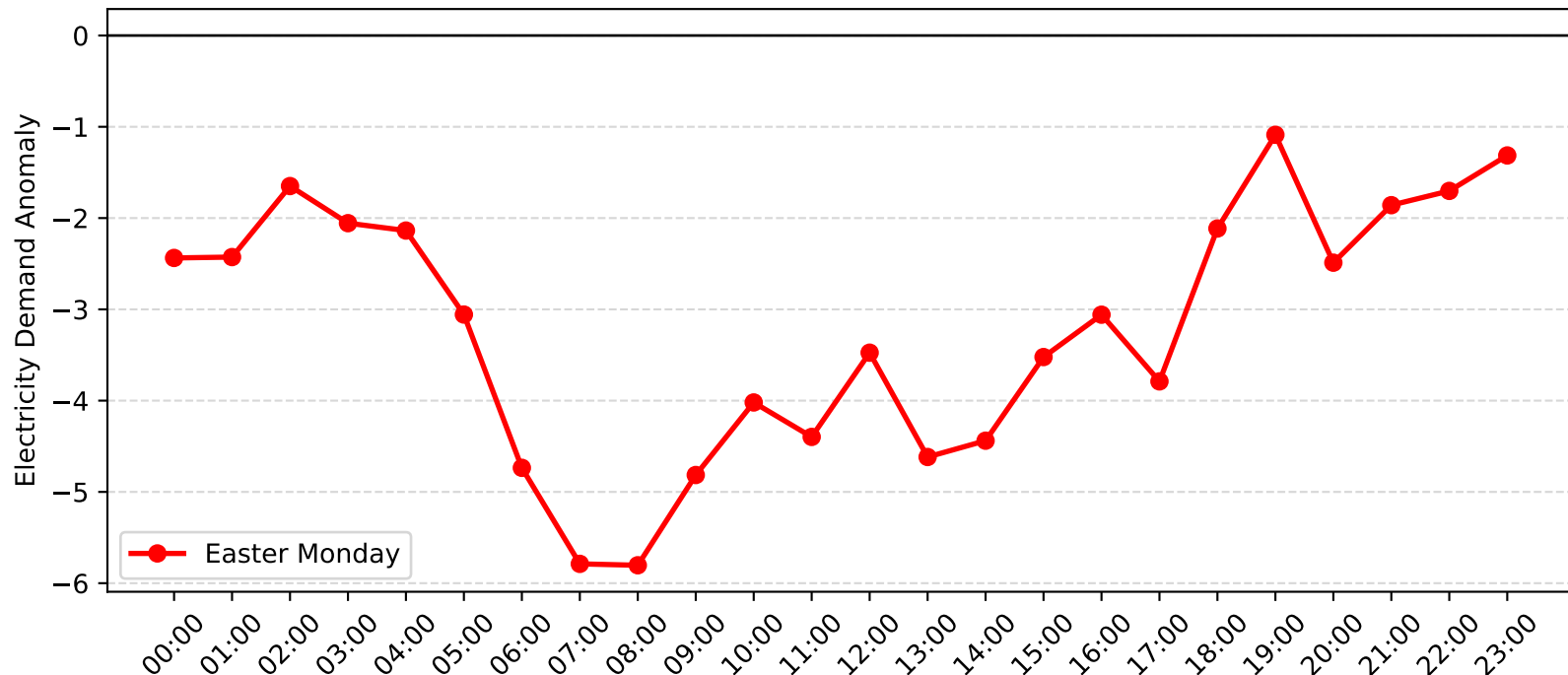
Matraverse Demand Anomaly: Easter Monday (2007-2008)
