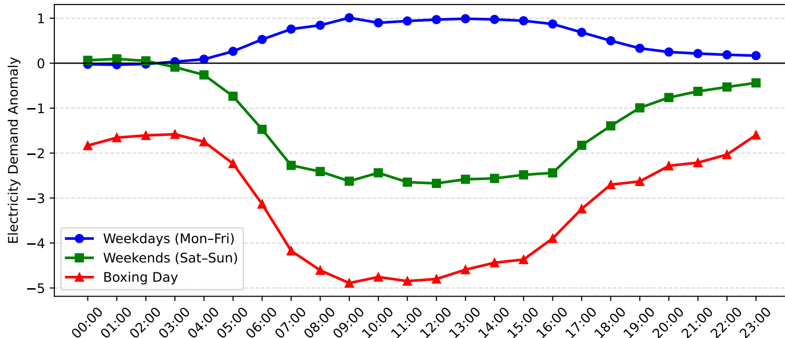
Lidcombe Demand Anomaly: Boxing Day vs Weekday/Weekend (2007-2008)
