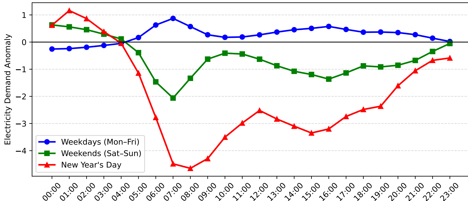
Five Dock Demand Anomaly: New Year's Day vs Weekday/Weekend (2012-2013)
