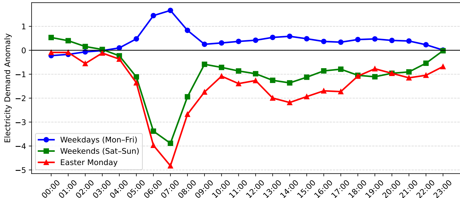
Mortdale Demand Anomaly: Easter Monday vs Weekday/Weekend (2012-2013)
