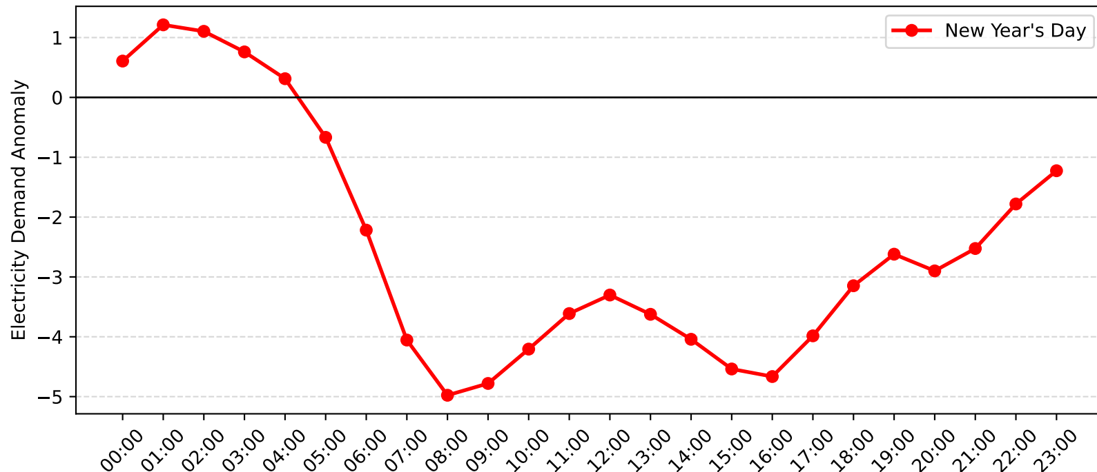
Five Dock Demand Anomaly: New Year's Day (2017-2018)
