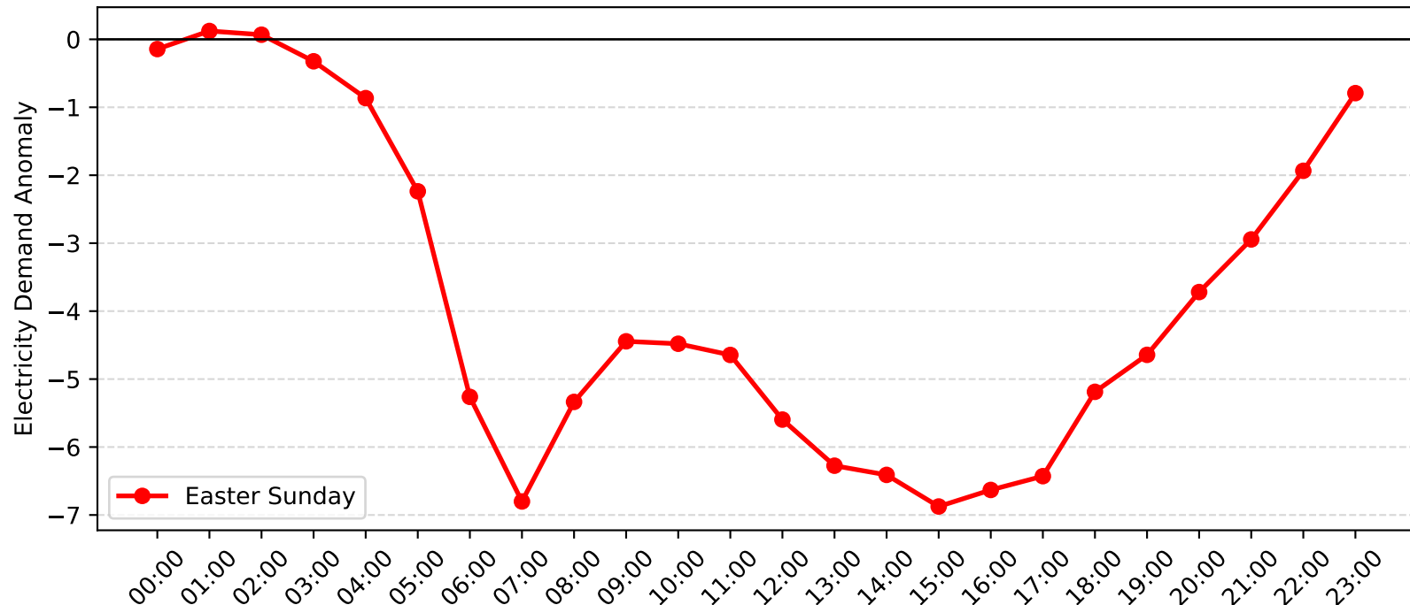
Dulwich Hill Demand Anomaly: Easter Sunday (2007-2008)
