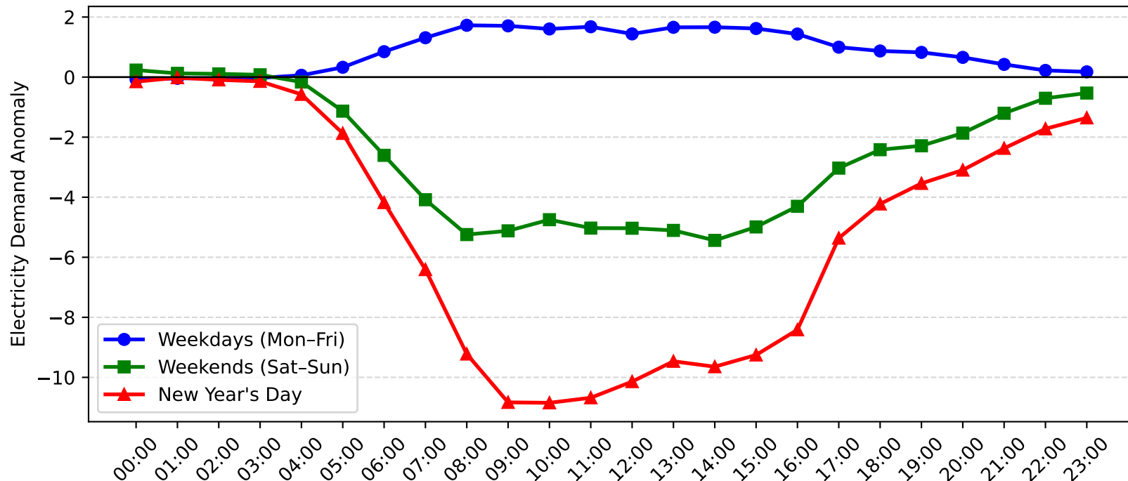
Brookvale Demand Anomaly: New Year's Day vs Weekday/Weekend (2014-2015)
