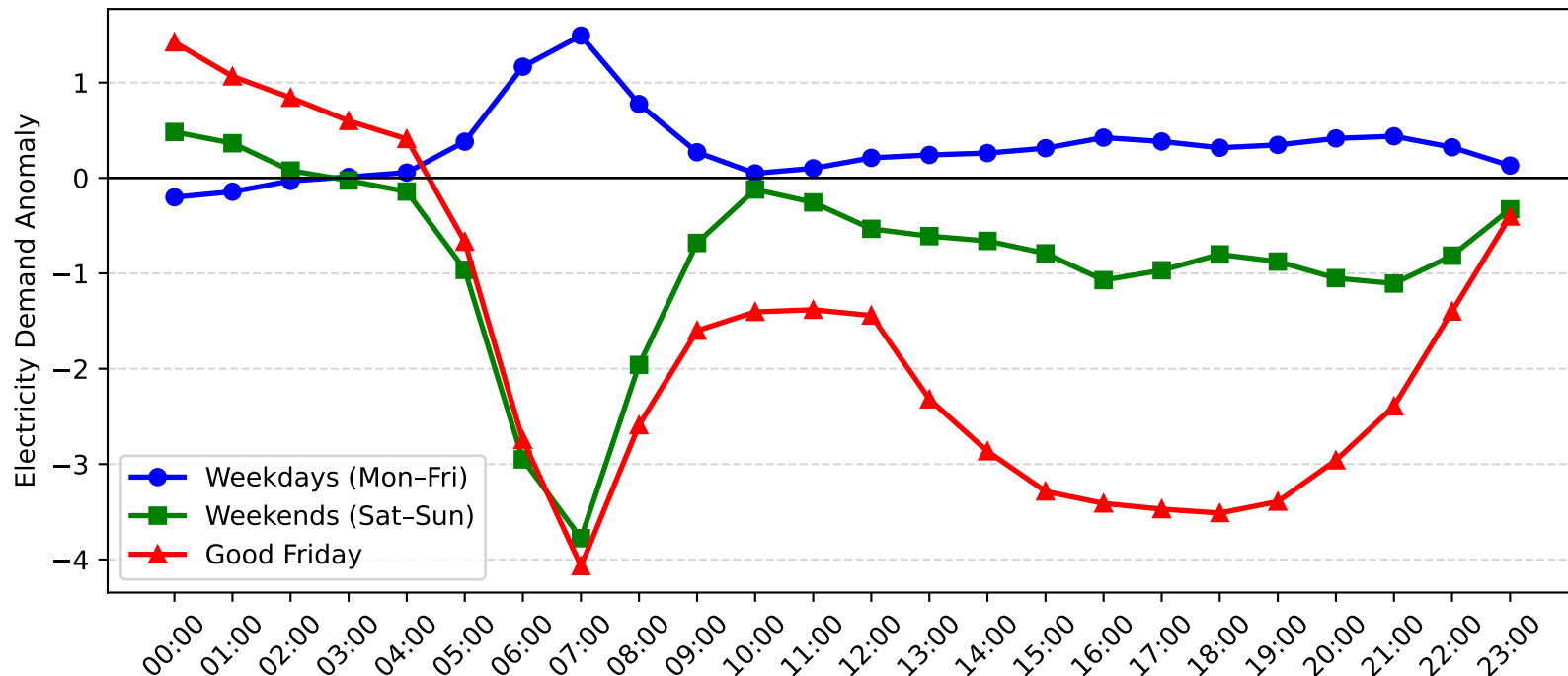
Dulwich Hill Demand Anomaly: Good Friday vs Weekday/Weekend (2013-2014)
