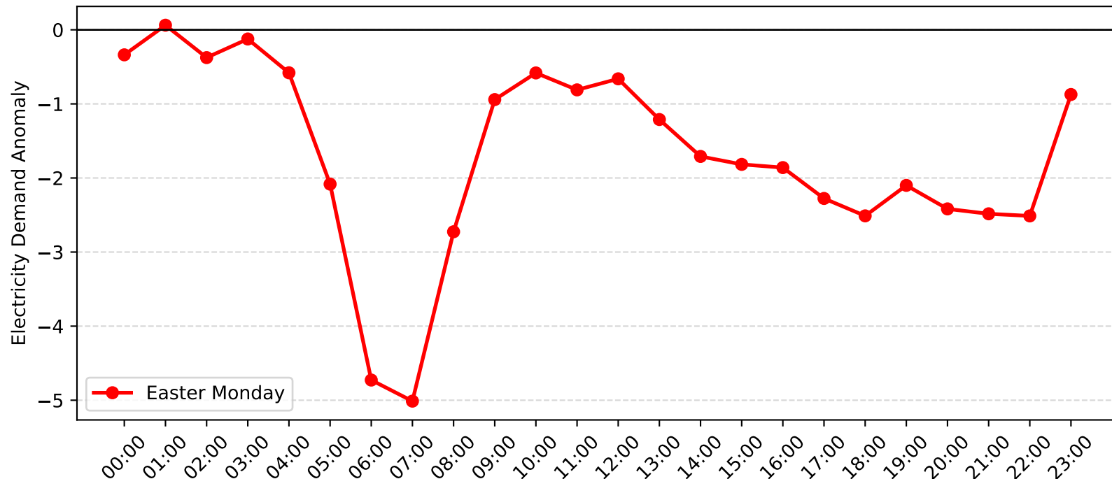
Cronulla Demand Anomaly: Easter Monday (2013-2014)
