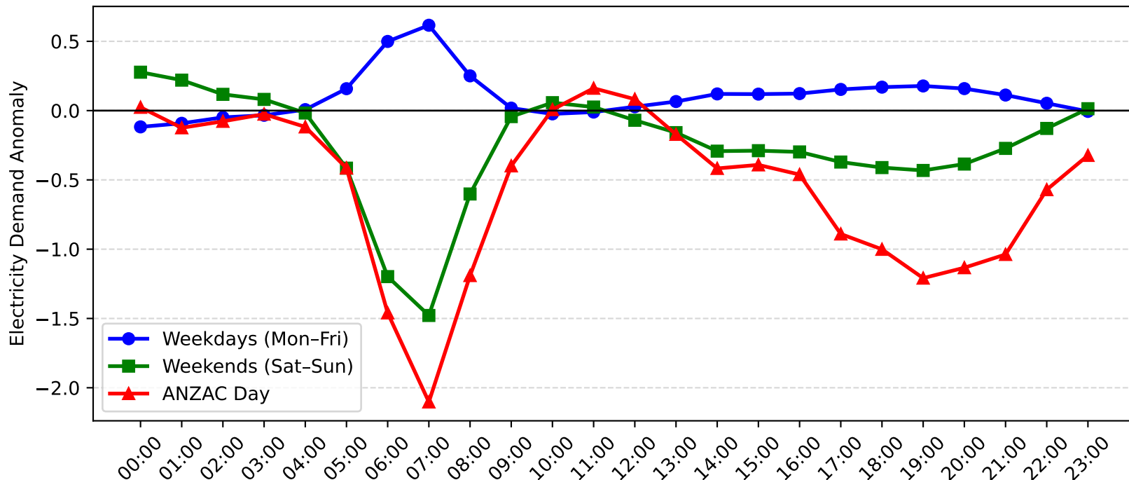
Blakehurst Demand Anomaly: ANZAC Day vs Weekday/Weekend (2014-2015)
