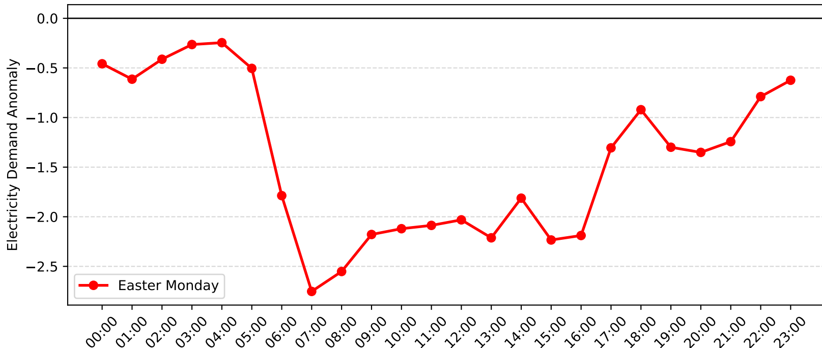
Pymble Demand Anomaly: Easter Monday (2017-2018)
