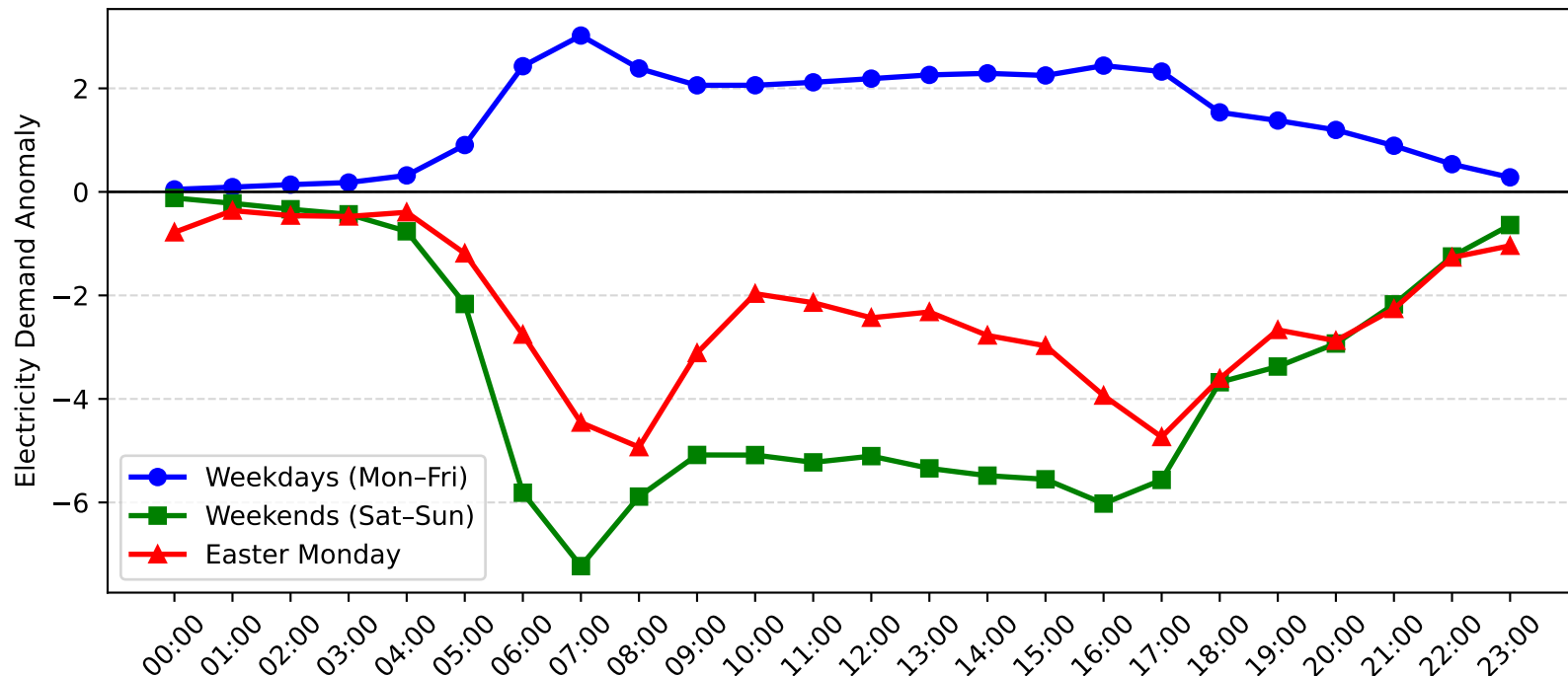
Epping Demand Anomaly: Easter Monday vs Weekday/Weekend (2007-2008)
