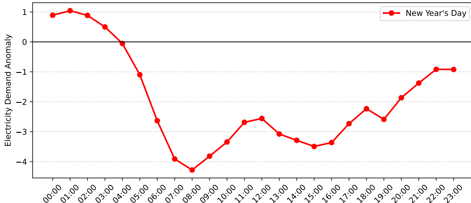
Five Dock Demand Anomaly: New Year's Day (2007-2008)
