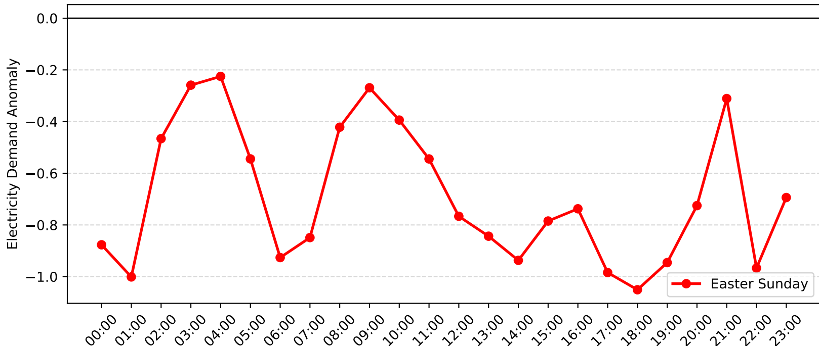
Jewells Demand Anomaly: Easter Sunday (2016-2017)
