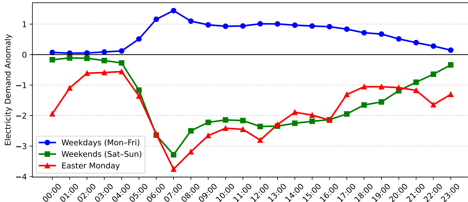
Matraverse Demand Anomaly: Easter Monday vs Weekday/Weekend (2015-2016)
