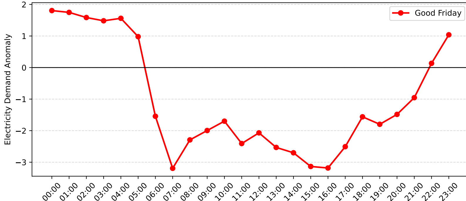
Chatswood Demand Anomaly: Good Friday (2006-2007)
