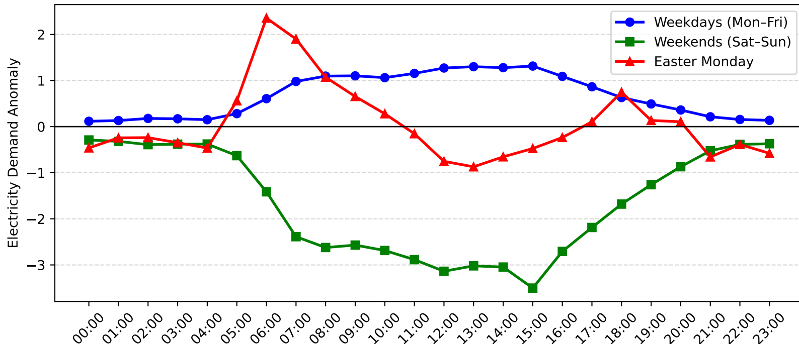
Mascot Demand Anomaly: Easter Monday vs Weekday/Weekend (2004-2005)
