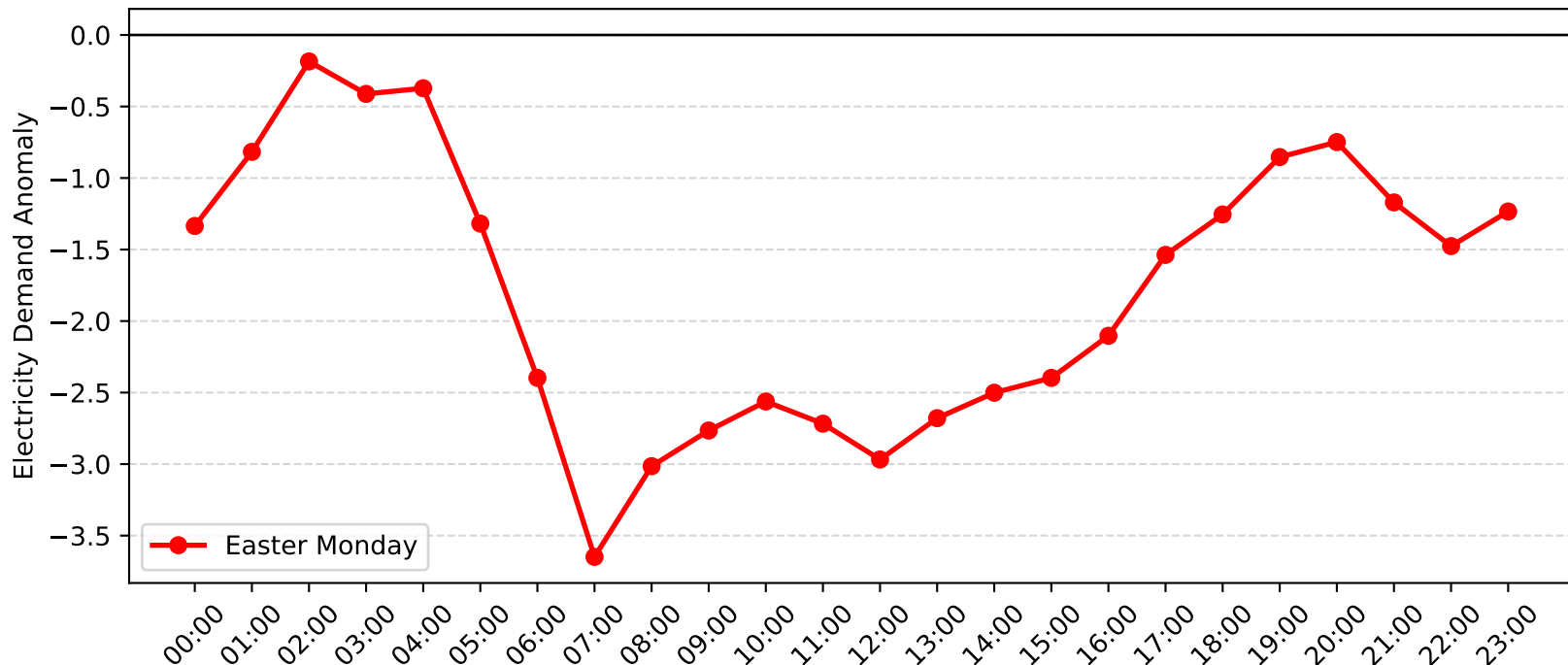
Matraville Demand Anomaly: Easter Monday (2016-2017)
