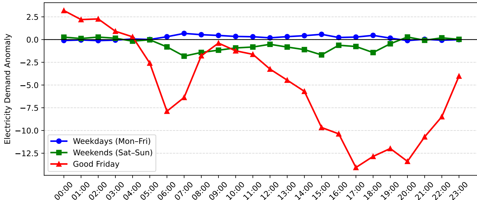
Pennant Hills Demand Anomaly: Good Friday vs Weekday/Weekend (2004-2005)
