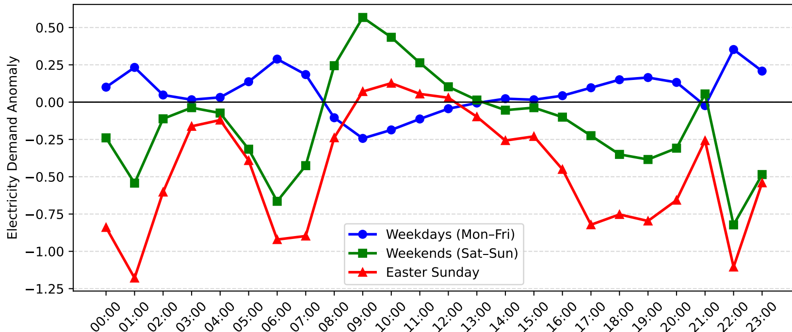
Jewells Demand Anomaly: Easter Sunday vs Weekday/Weekend (2011-2012)
