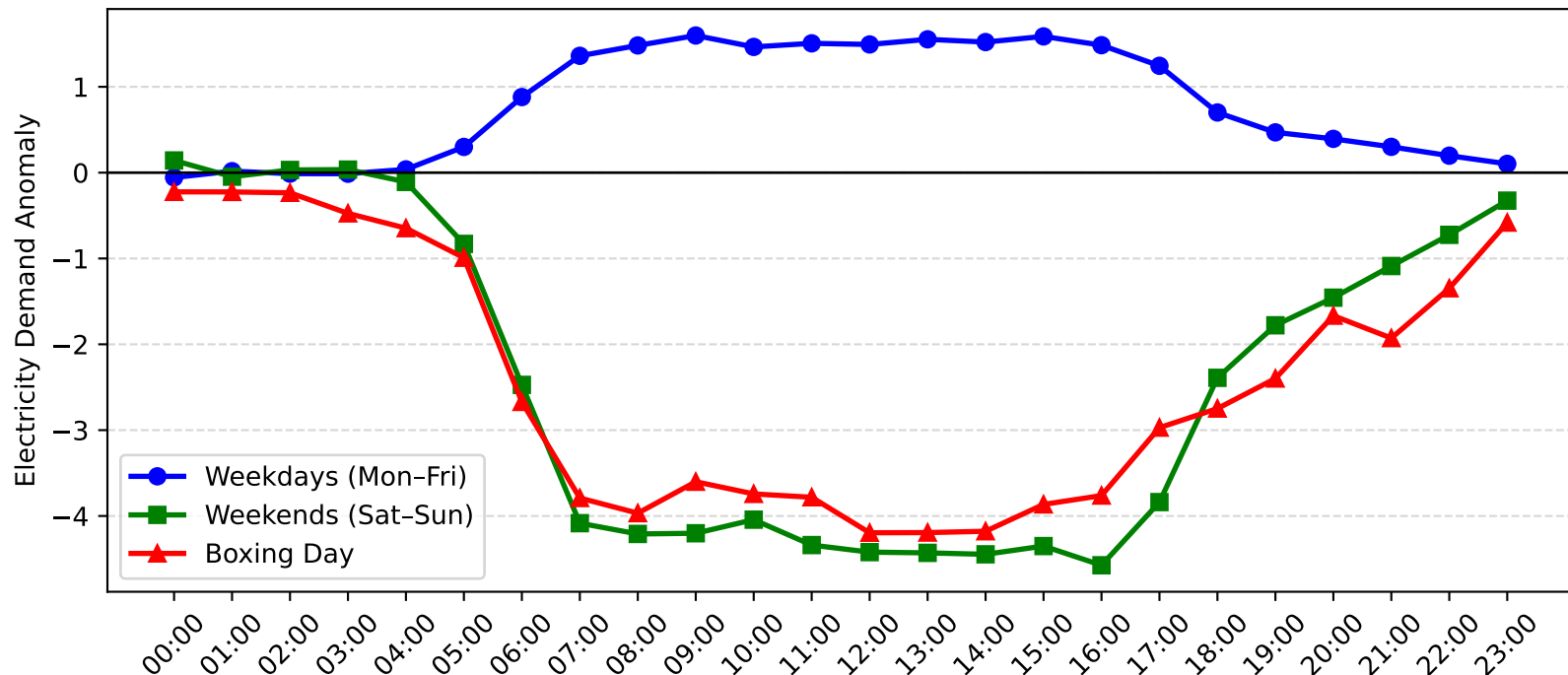
Pymble Demand Anomaly: Boxing Day vs Weekday/Weekend (2007-2008)
