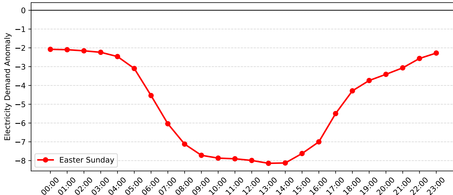
Caringbah Demand Anomaly: Easter Sunday (2008-2009)
