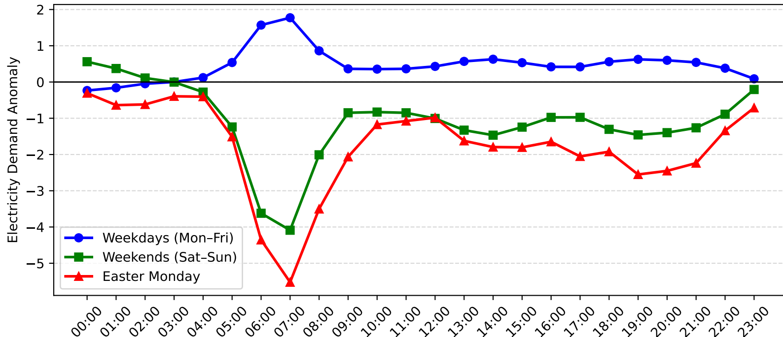
Mortdale Demand Anomaly: Easter Monday vs Weekday/Weekend (2011-2012)
