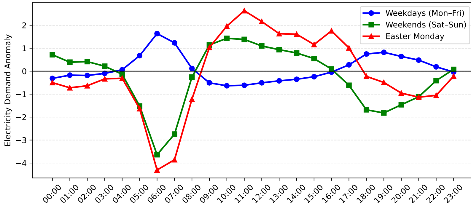
Cronulla Demand Anomaly: Easter Monday vs Weekday/Weekend (2008-2009)
