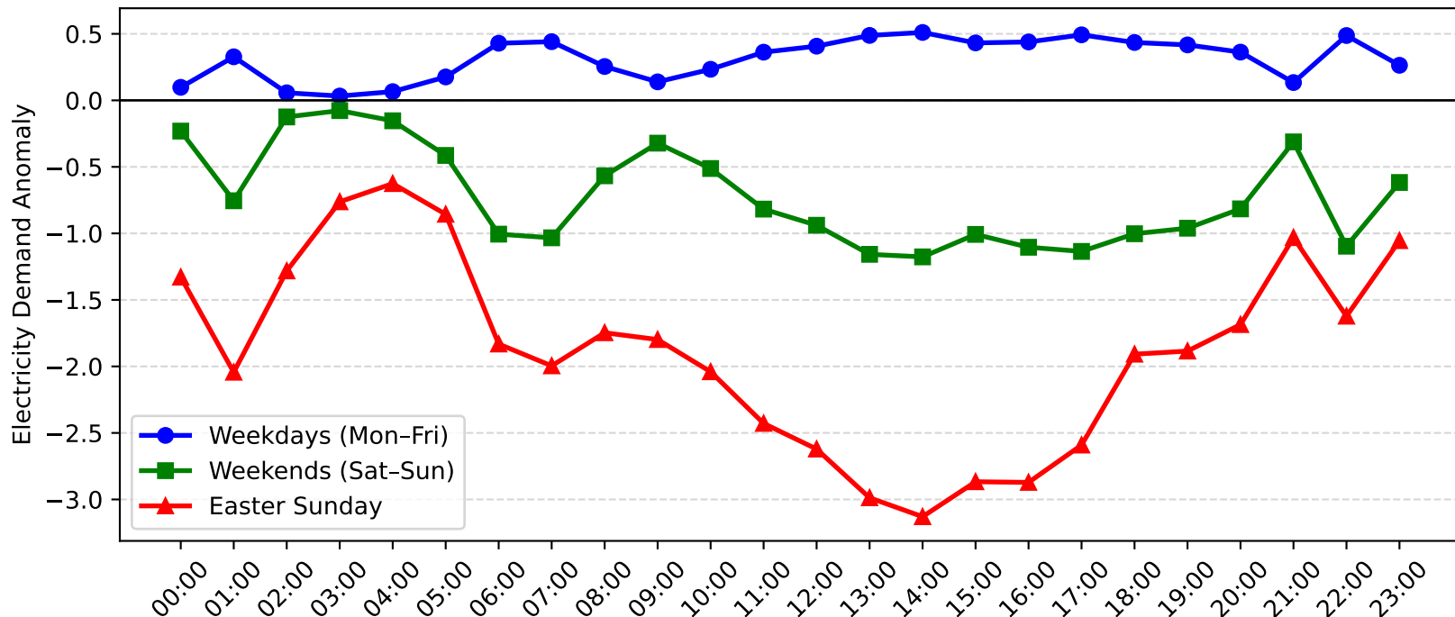
Gateshead Demand Anomaly: Easter Sunday vs Weekday/Weekend (2006-2007)
