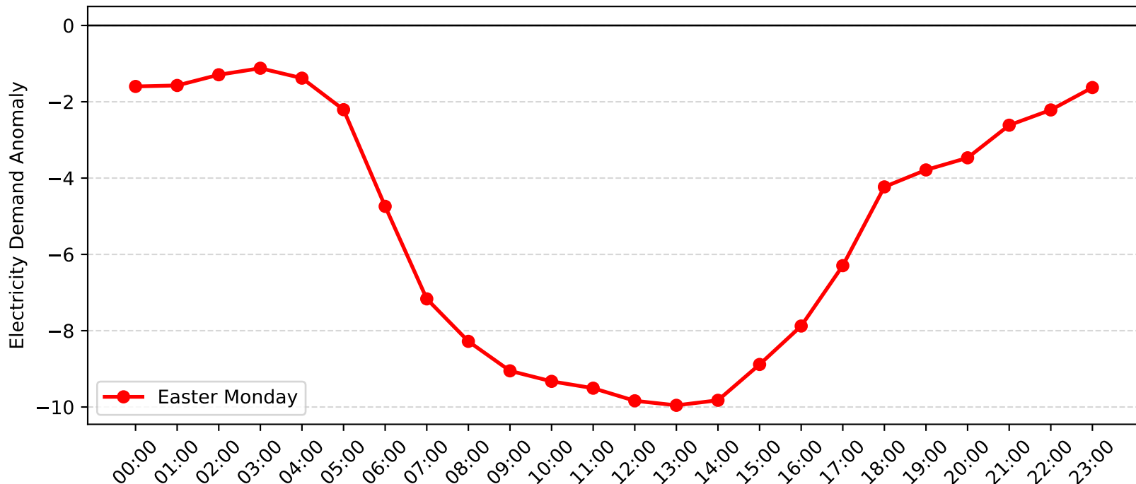
Mascot Demand Anomaly: Easter Monday (2010-2011)
