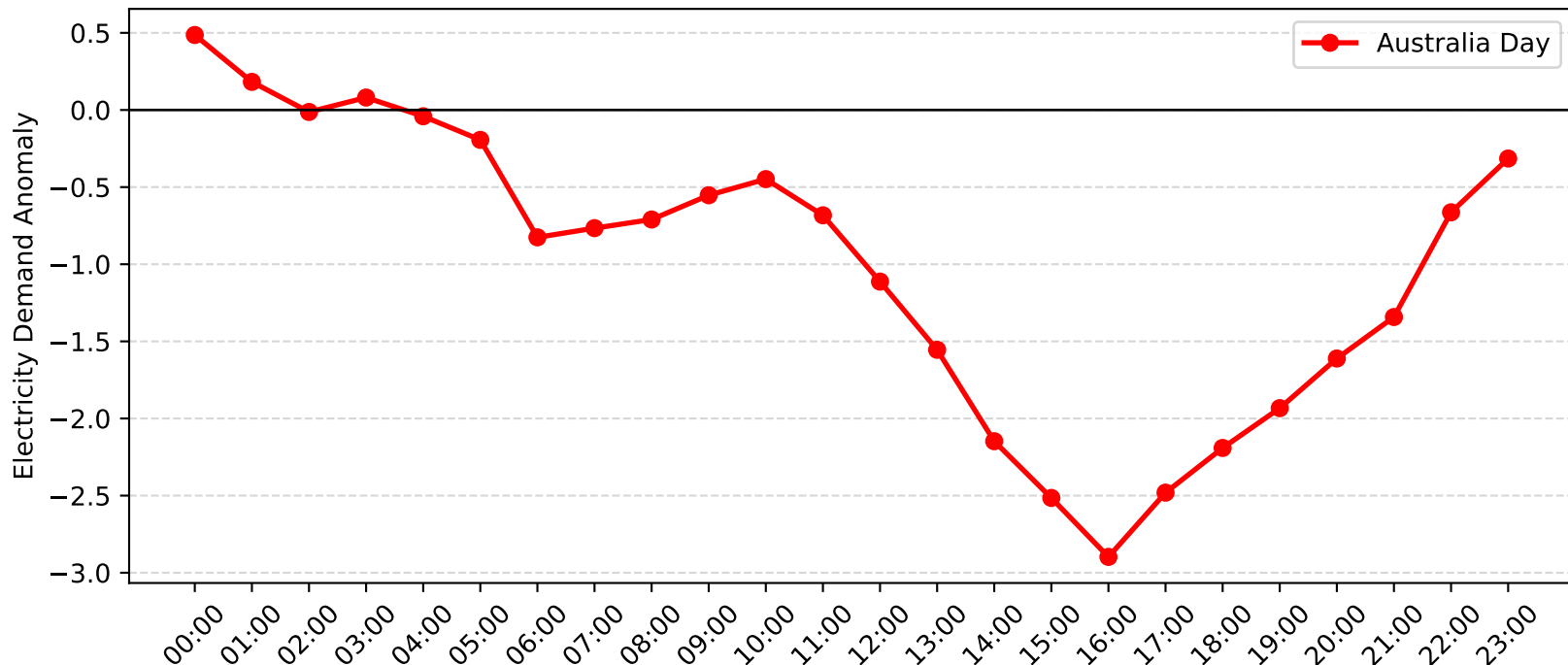
Woy Woy Demand Anomaly: Australia Day (2014-2015)
