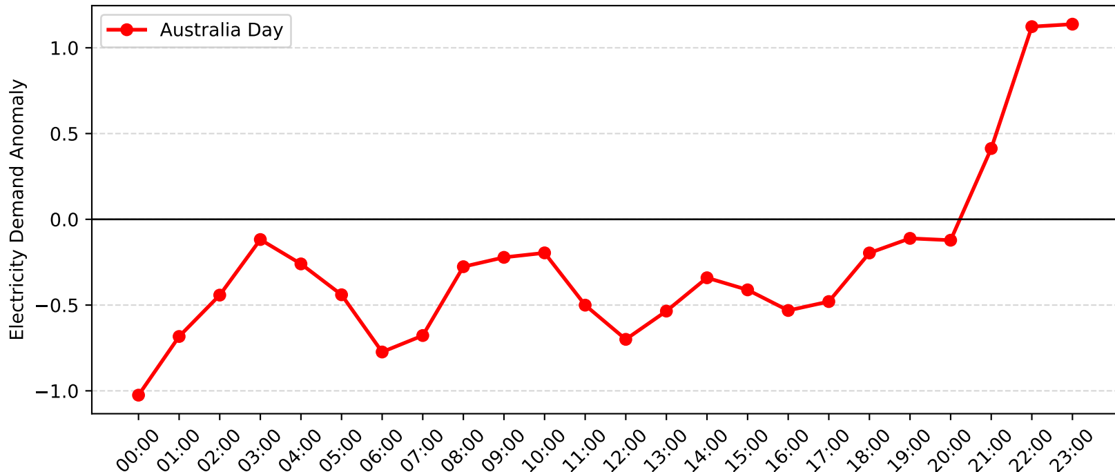
Woy Woy Demand Anomaly: Australia Day (2007-2008)
