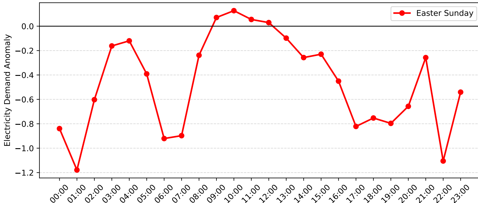
Jewells Demand Anomaly: Easter Sunday (2011-2012)
