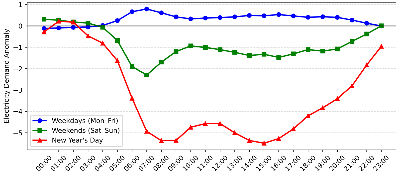
Five Dock Demand Anomaly: New Year's Day vs Weekday/Weekend (2015-2016)
