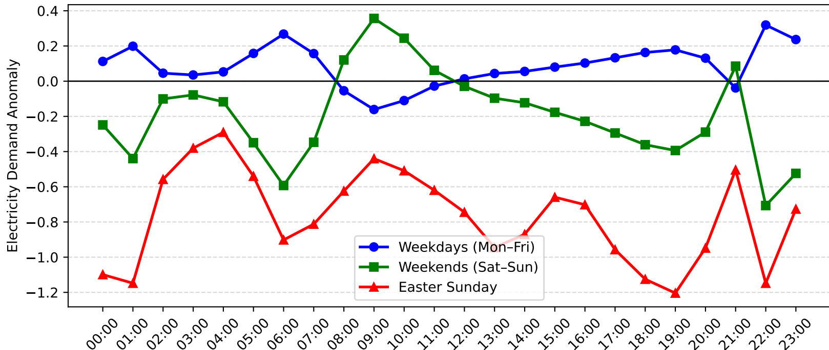
Jewells Demand Anomaly: Easter Sunday vs Weekday/Weekend (2017-2018)
