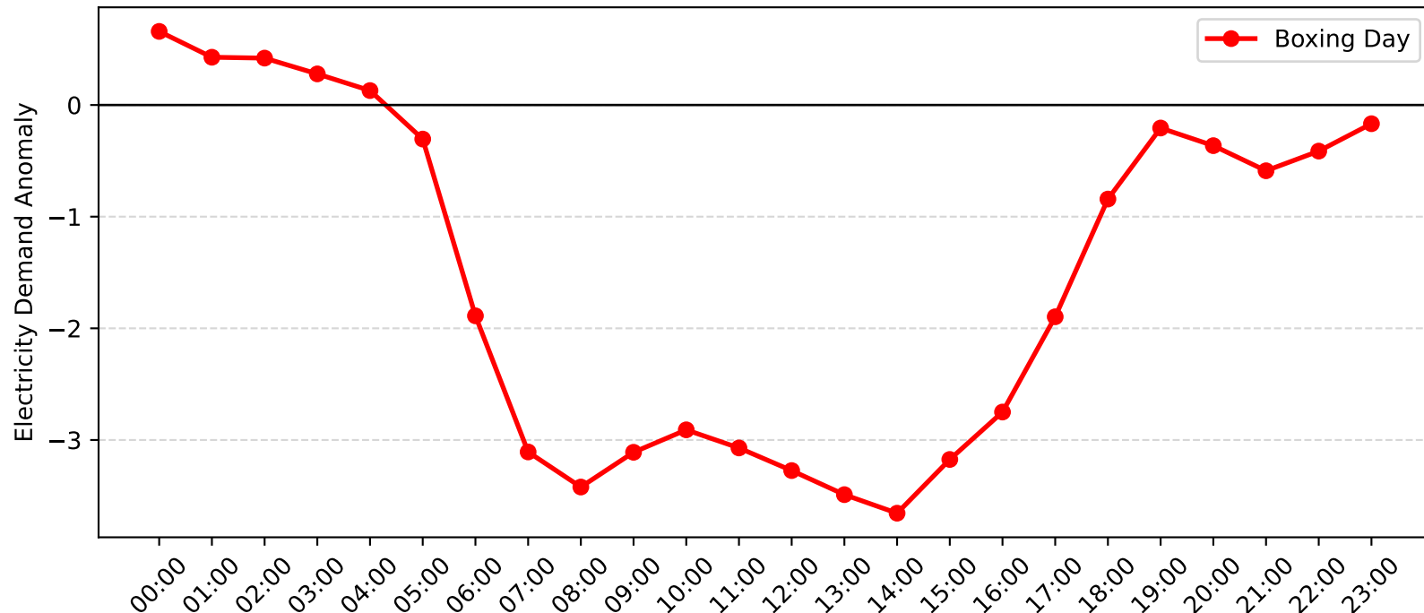
Pymble Demand Anomaly: Boxing Day (2010-2011)
