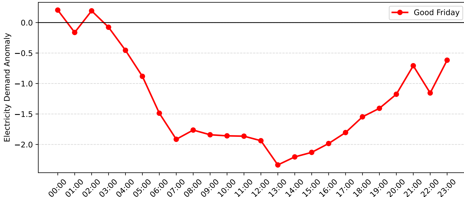
Gateshead Demand Anomaly: Good Friday (2016-2017)
