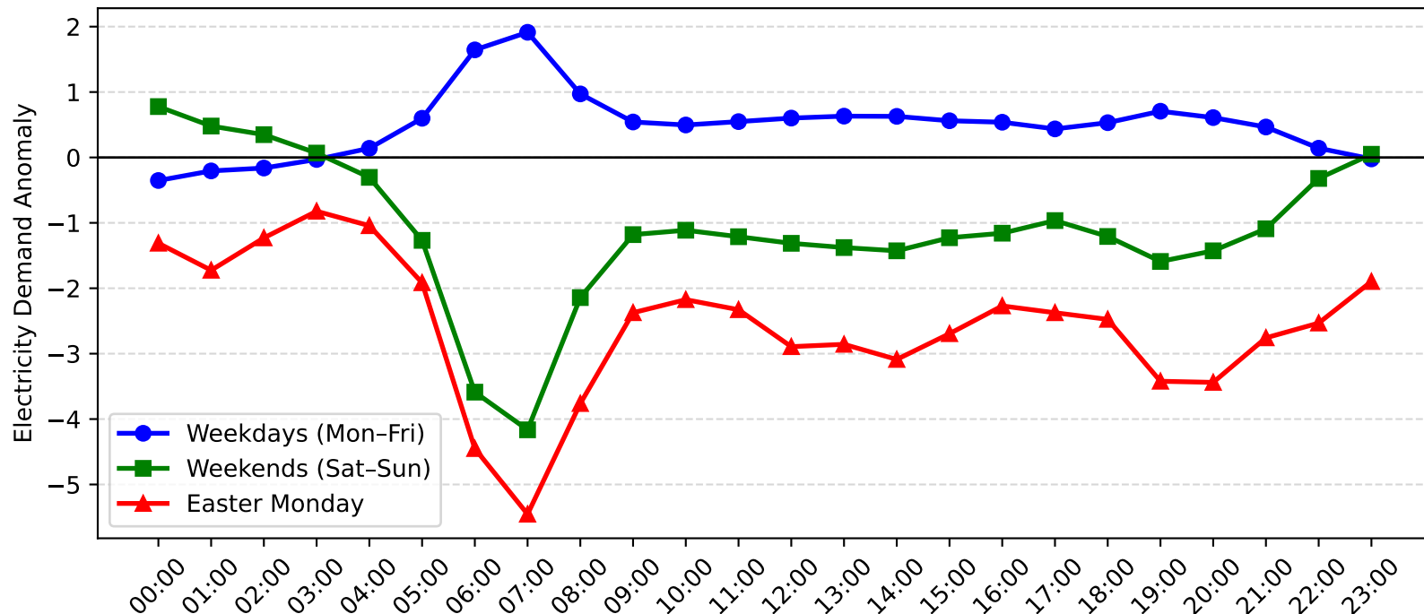
Mortdale Demand Anomaly: Easter Monday vs Weekday/Weekend (2009-2010)
