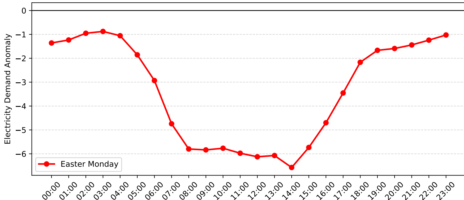
Mascot Demand Anomaly: Easter Monday (2016-2017)
