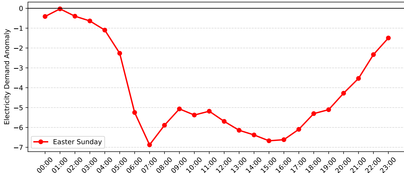
Dulwich Hill Demand Anomaly: Easter Sunday (2006-2007)
