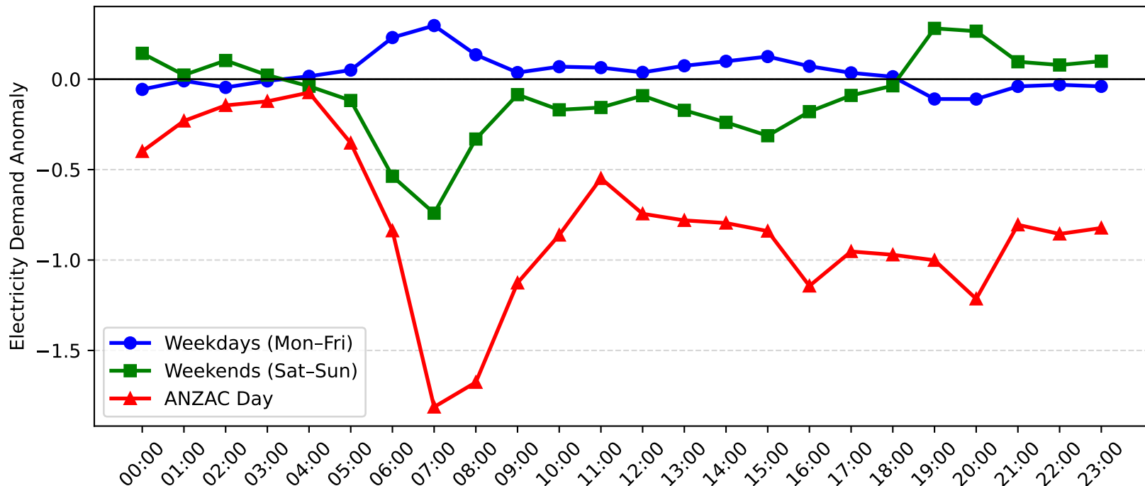
Blakehurst Demand Anomaly: ANZAC Day vs Weekday/Weekend (2004-2005)
