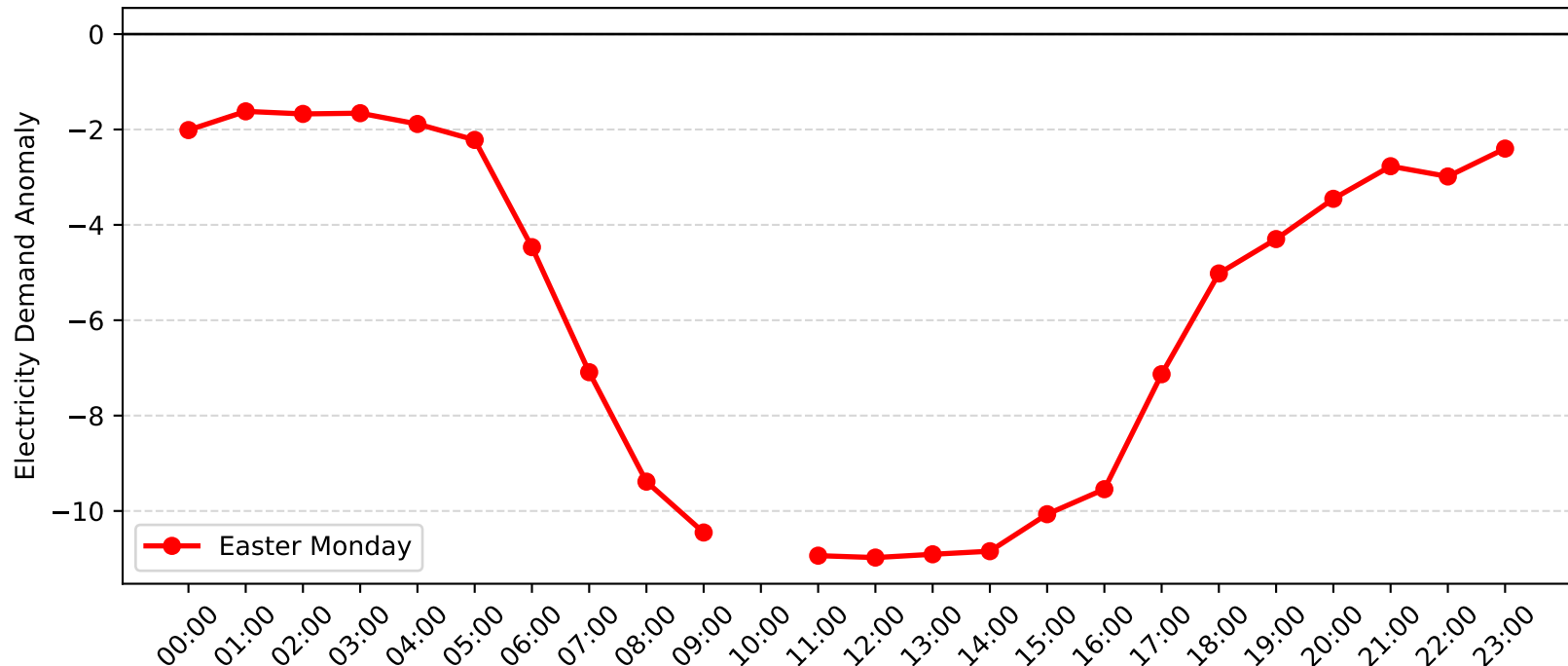
Mascot Demand Anomaly: Easter Monday (2005-2006)
