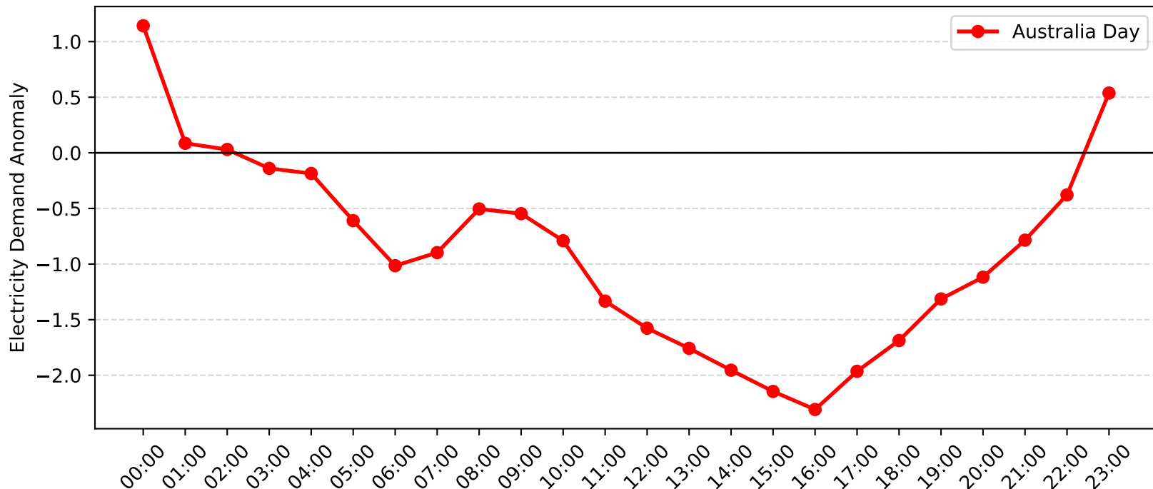
Woy Woy Demand Anomaly: Australia Day (2008-2009)
