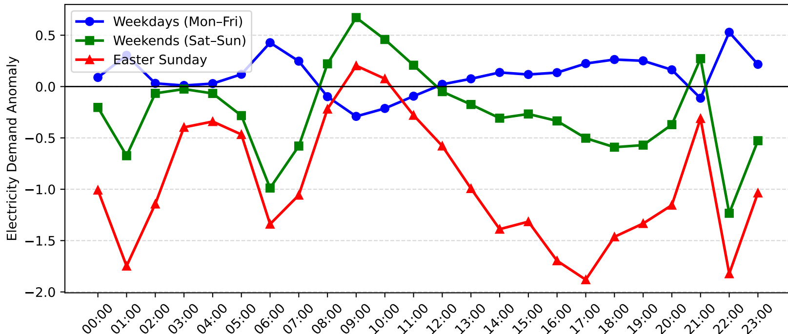
Jewells Demand Anomaly: Easter Sunday vs Weekday/Weekend (2006-2007)
