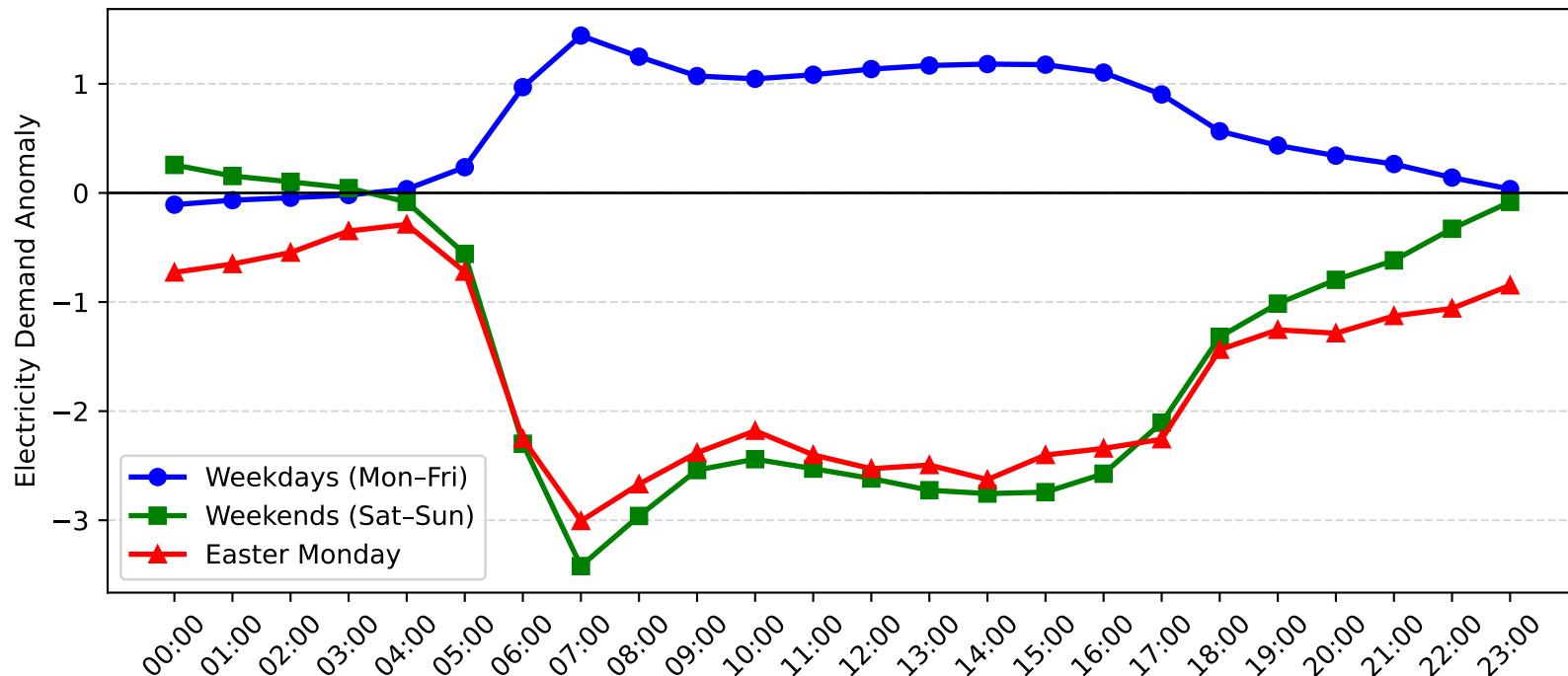
Pymble Demand Anomaly: Easter Monday vs Weekday/Weekend (2012-2013)
