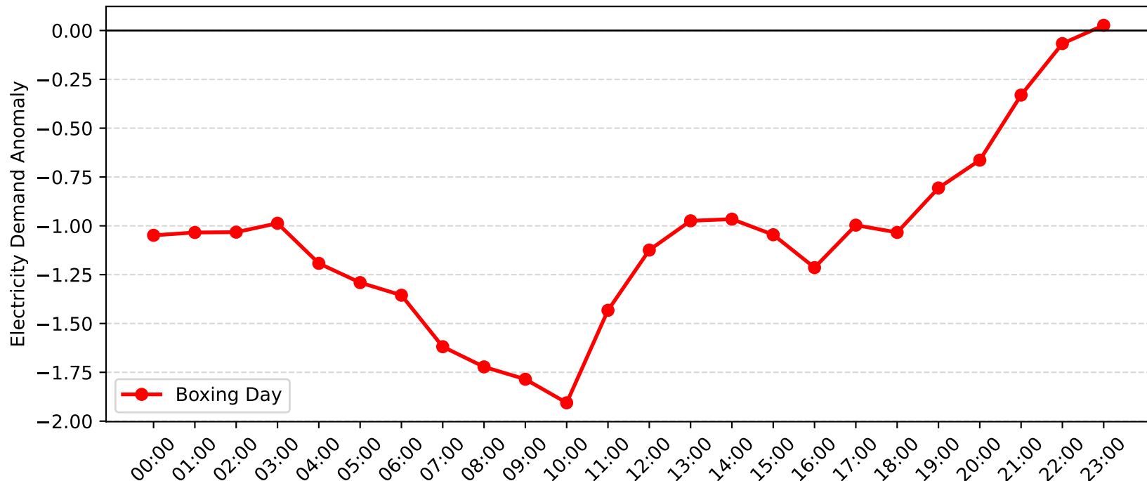
Lidcombe Demand Anomaly: Boxing Day (2016-2017)
