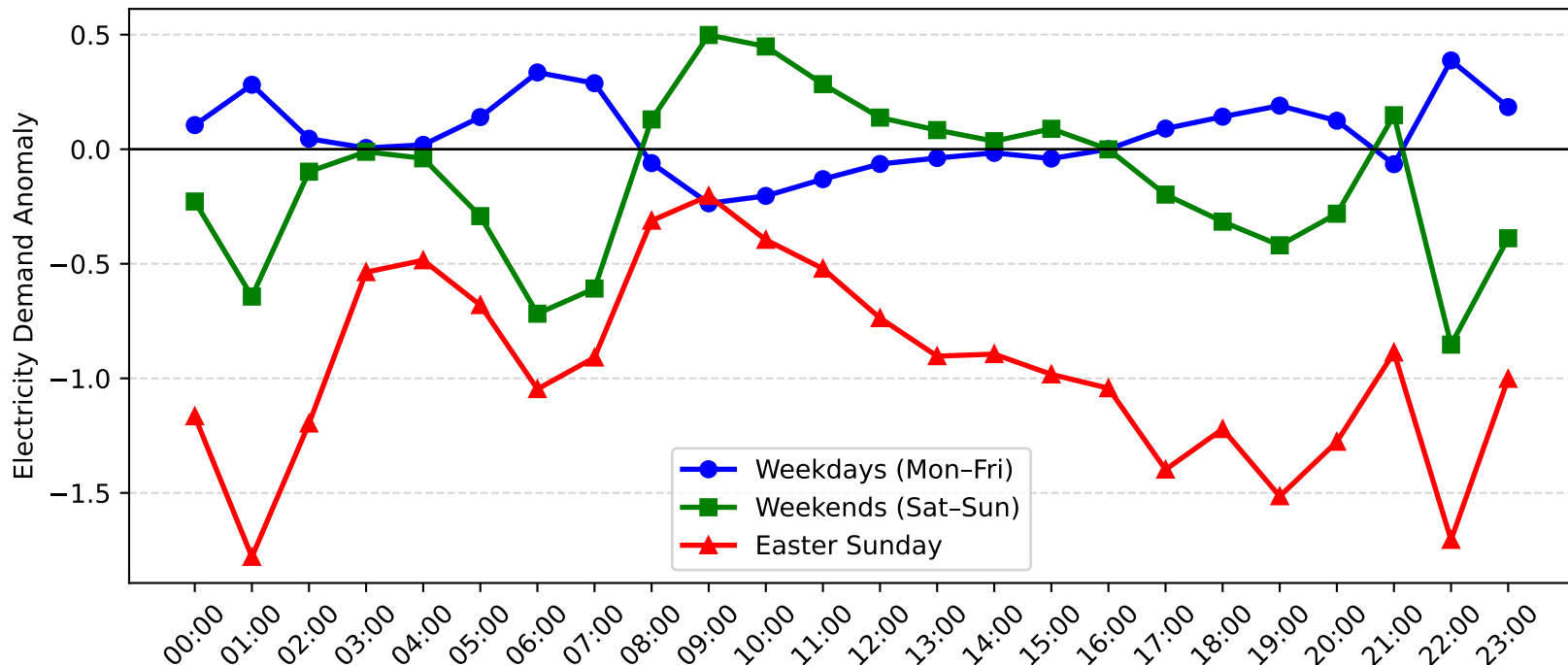
Jewells Demand Anomaly: Easter Sunday vs Weekday/Weekend (2009-2010)
