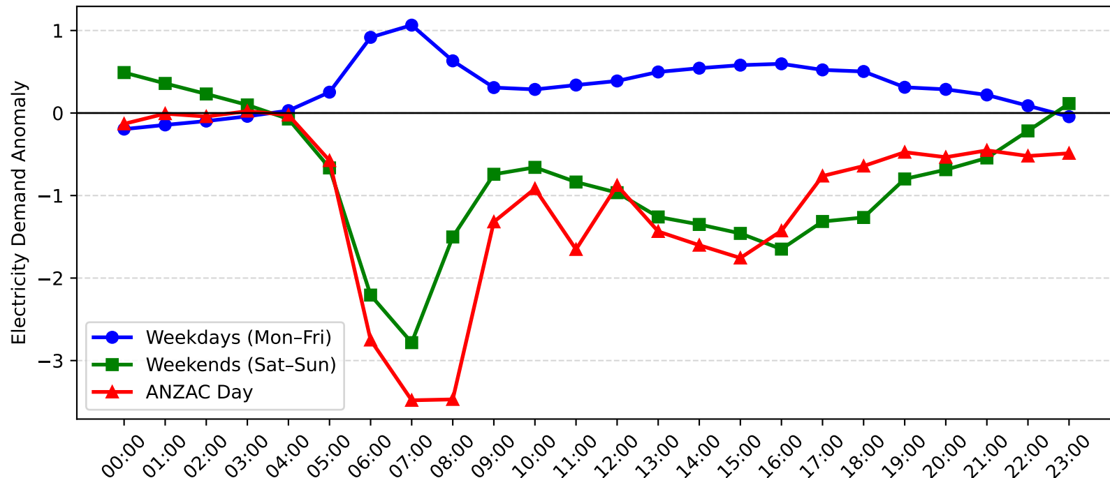
Blakehurst Demand Anomaly: ANZAC Day vs Weekday/Weekend (2005-2006)
