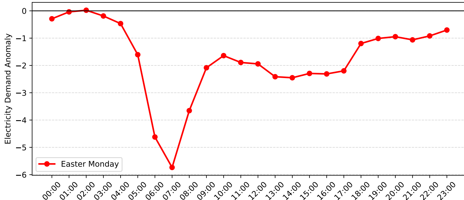
Mortdale Demand Anomaly: Easter Monday (2007-2008)
