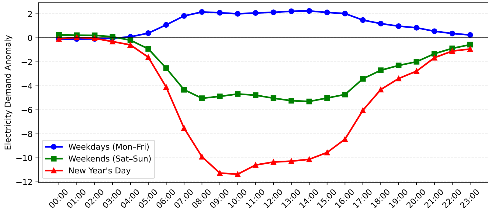
Brookvale Demand Anomaly: New Year's Day vs Weekday/Weekend (2012-2013)
