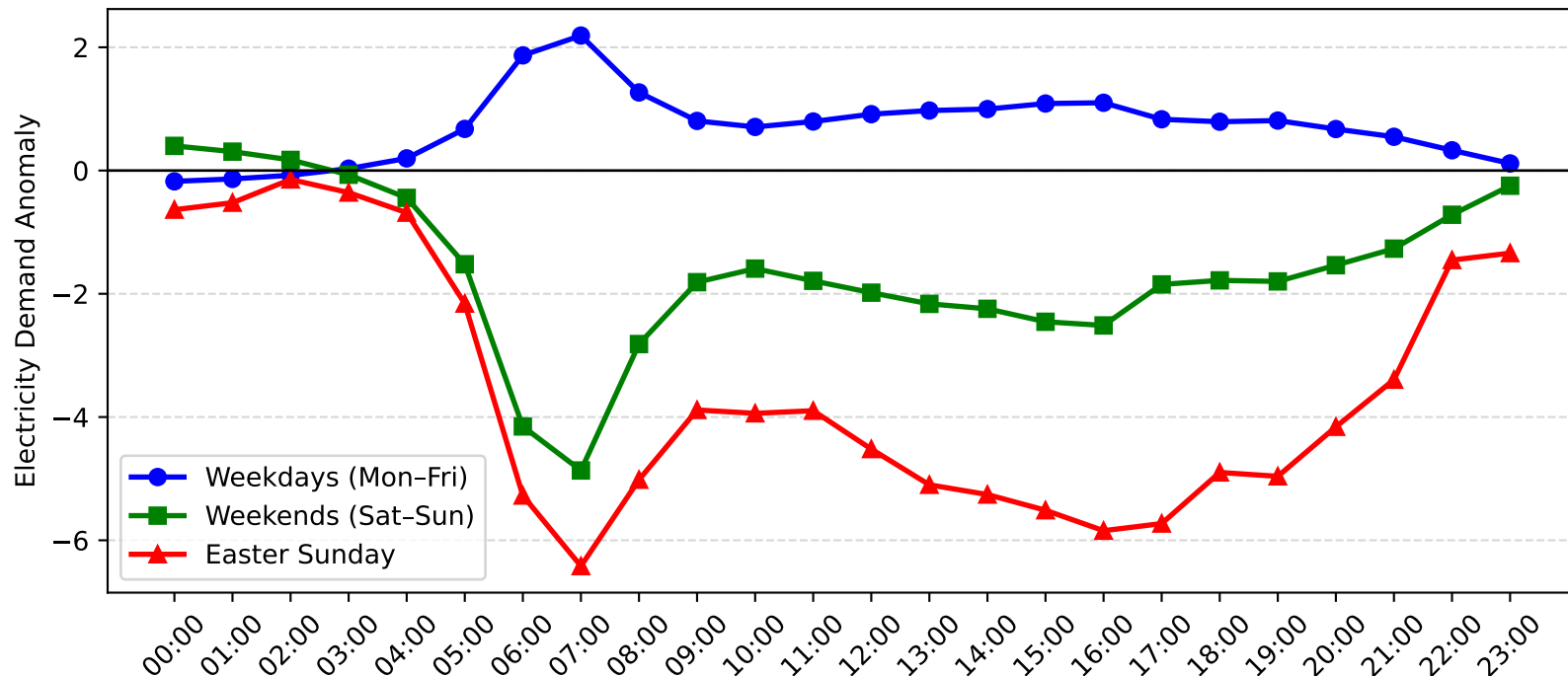
Dulwich Hill Demand Anomaly: Easter Sunday vs Weekday/Weekend (2008-2009)
