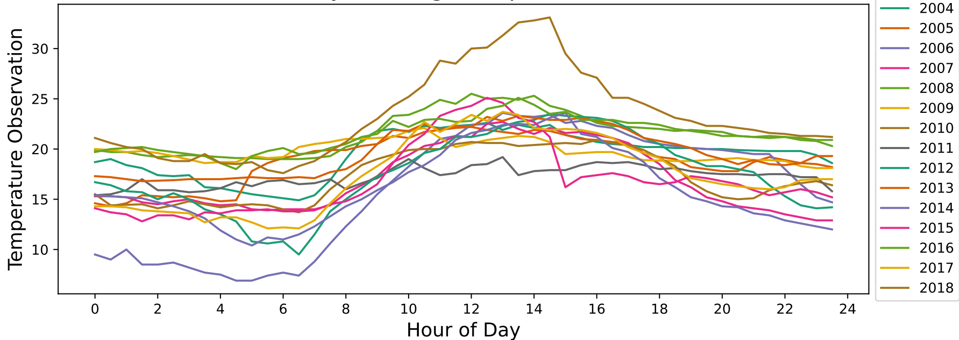
Easter Monday – Average Temperature (2004-2018)
