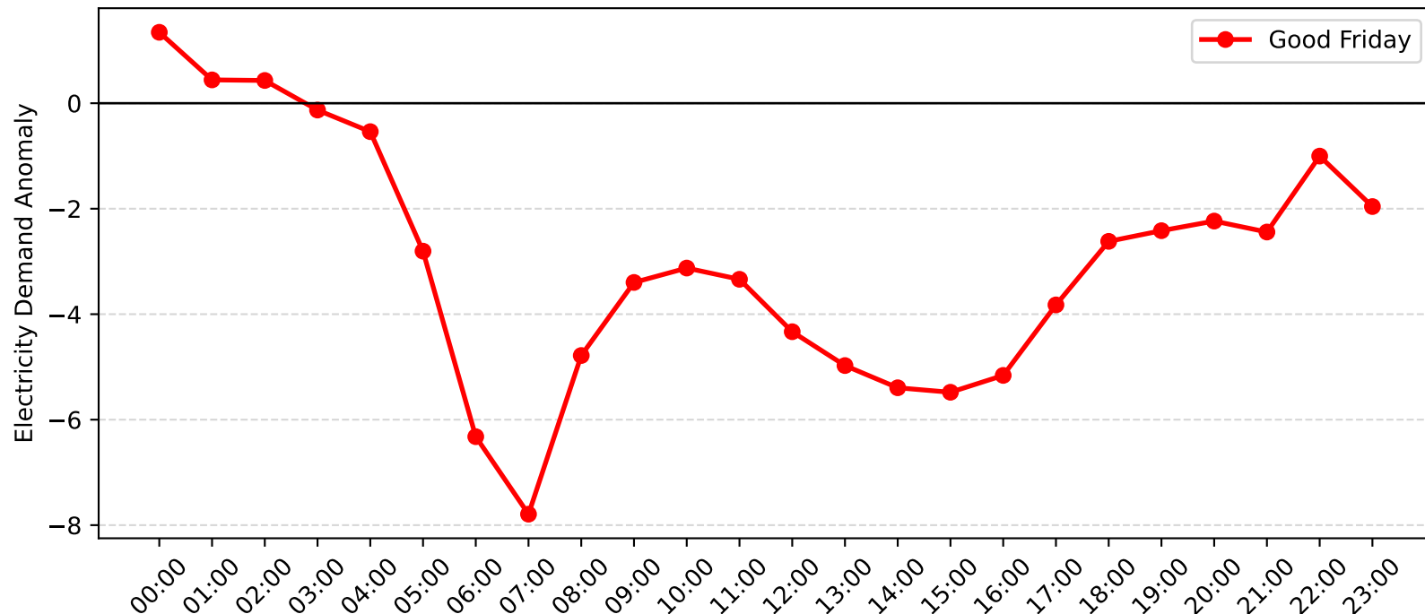
Dulwich Hill Demand Anomaly: Good Friday (2004-2005)
