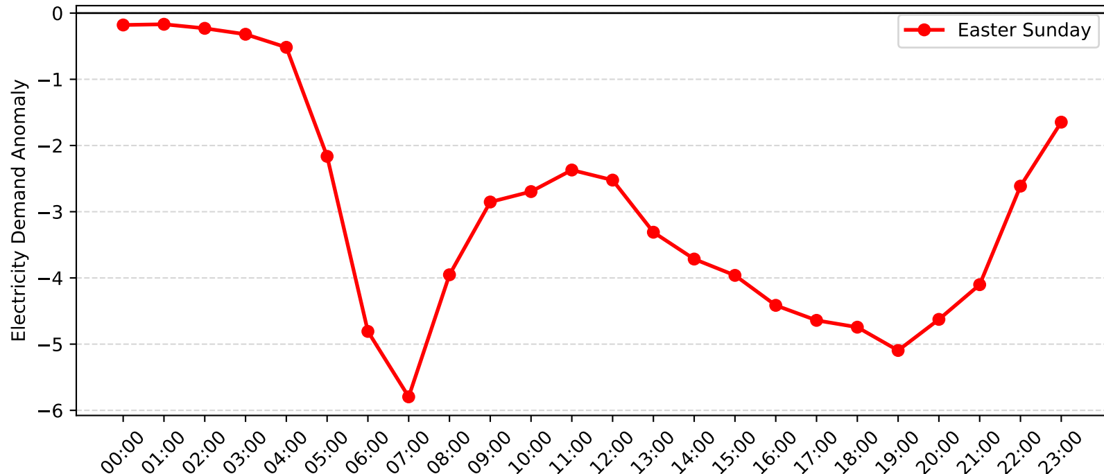
Dulwich Hill Demand Anomaly: Easter Sunday (2011-2012)
