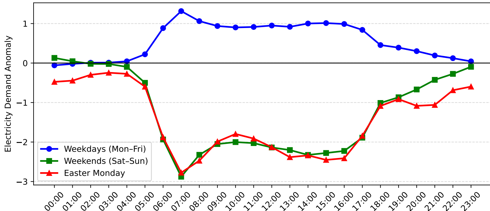
Pymble Demand Anomaly: Easter Monday vs Weekday/Weekend (2016-2017)
