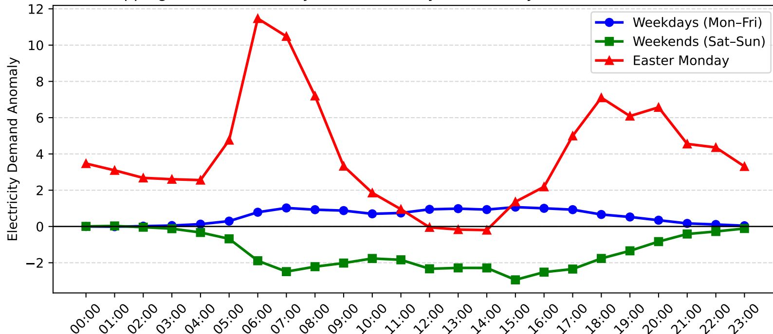
Epping Demand Anomaly: Easter Monday vs Weekday/Weekend (2004-2005)
