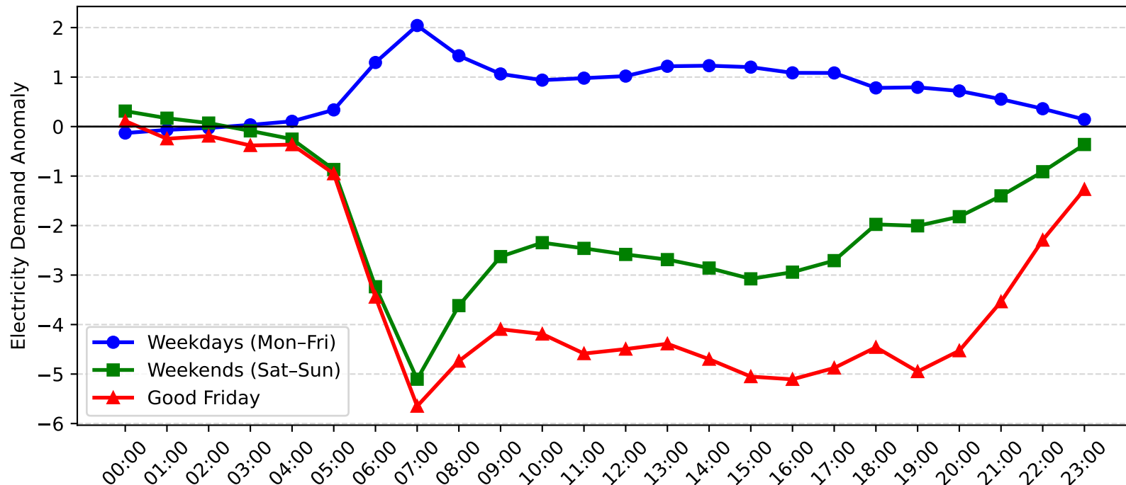
Chatswood Demand Anomaly: Good Friday vs Weekday/Weekend (2011-2012)
