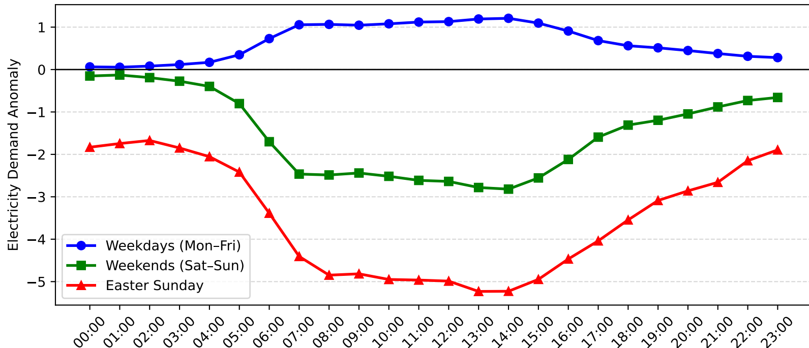
Caringbah Demand Anomaly: Easter Sunday vs Weekday/Weekend (2013-2014)
