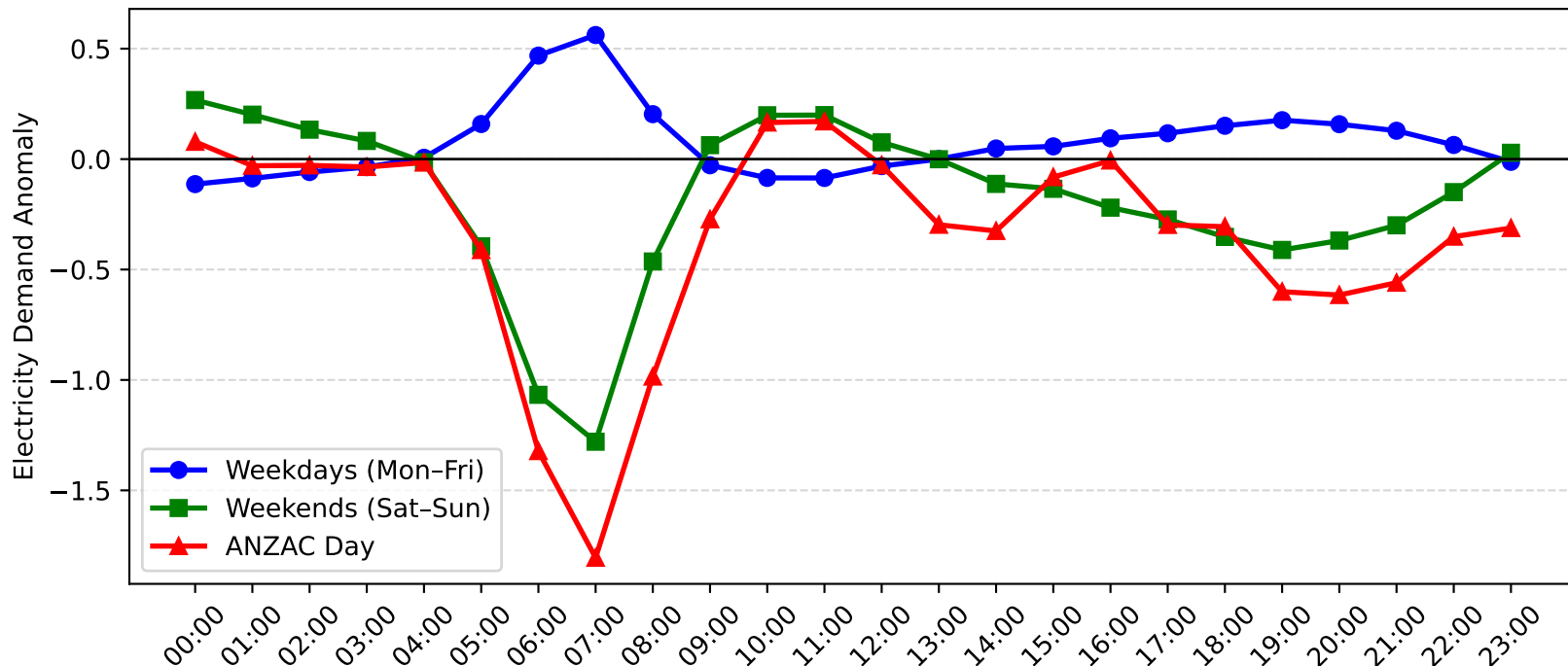
Blakehurst Demand Anomaly: ANZAC Day vs Weekday/Weekend (2015-2016)
