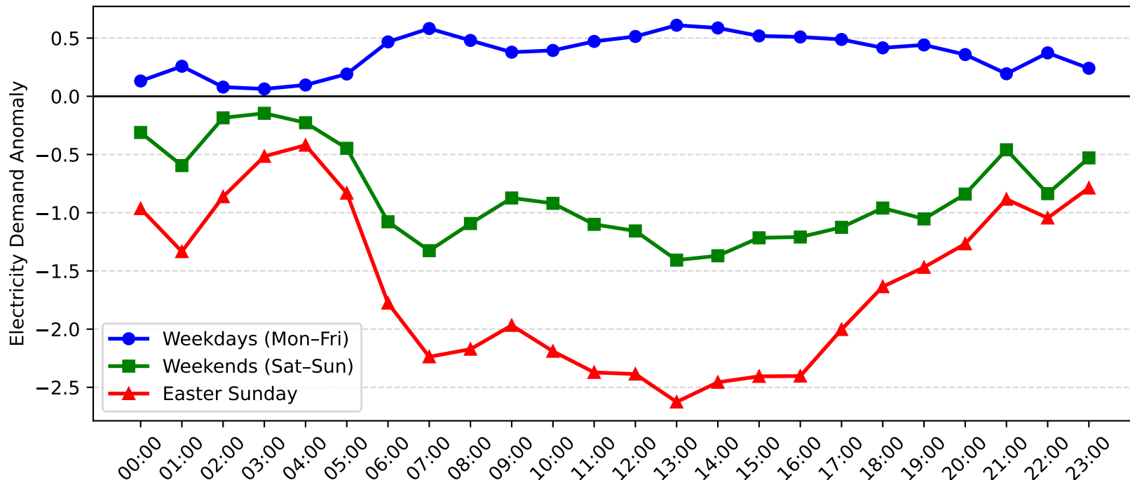
Gateshead Demand Anomaly: Easter Sunday vs Weekday/Weekend (2008-2009)
