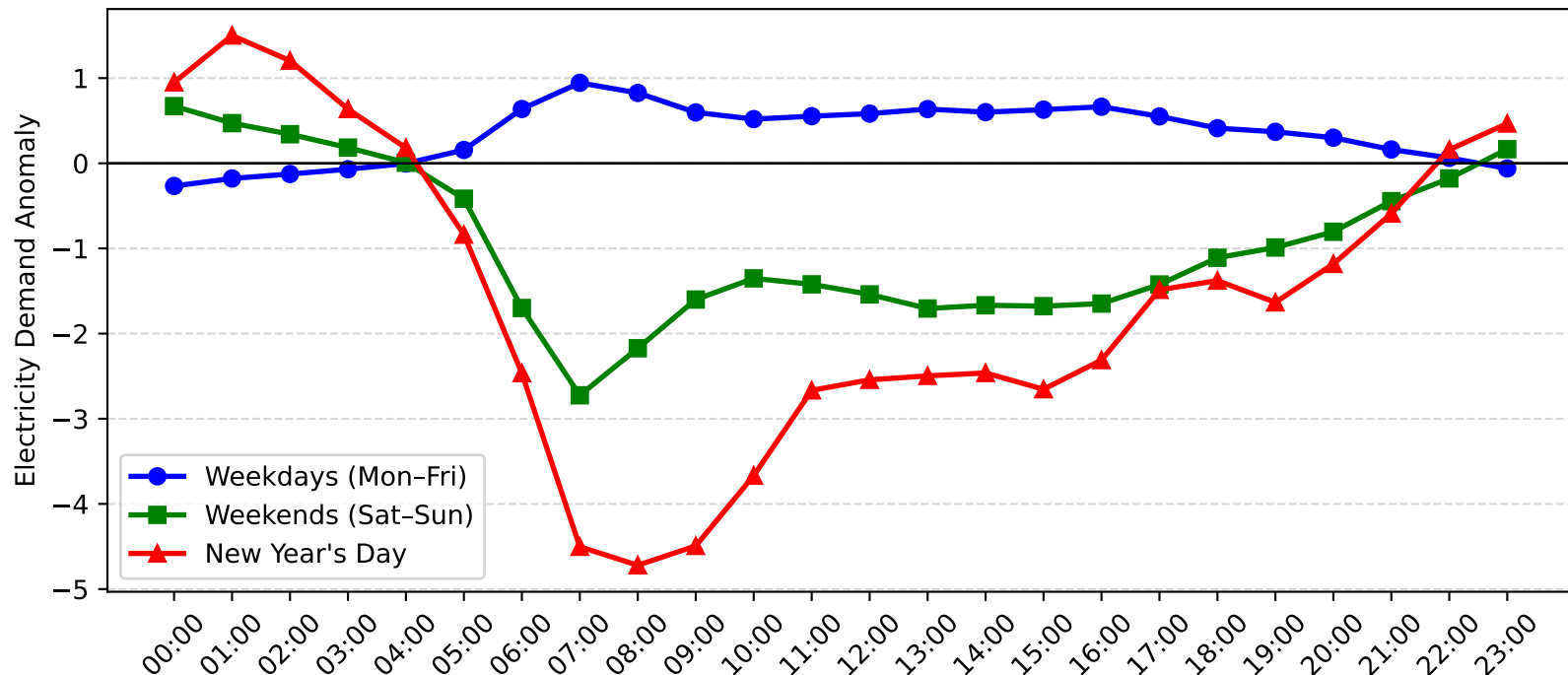
Five Dock Demand Anomaly: New Year's Day vs Weekday/Weekend (2010-2011)
