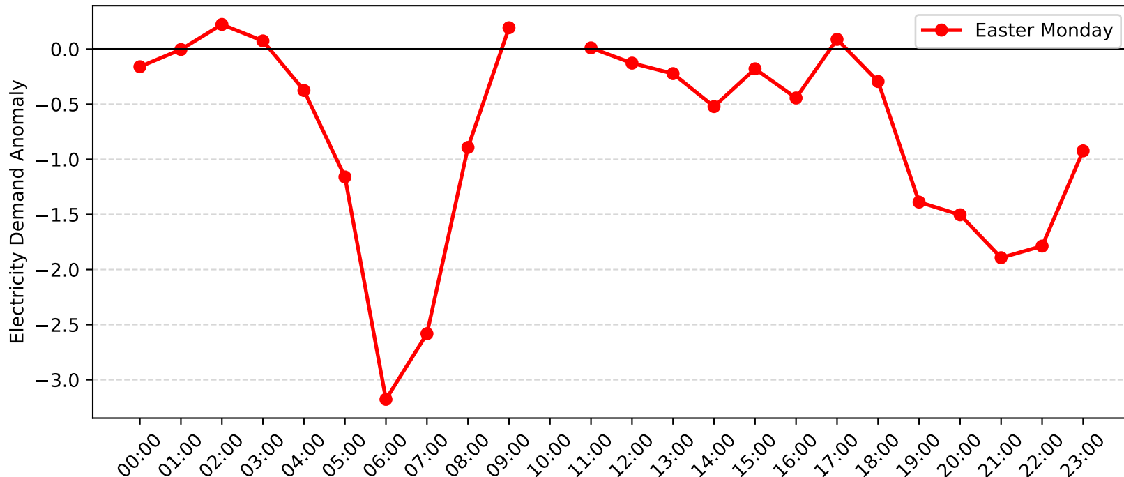
Cronulla Demand Anomaly: Easter Monday (2005-2006)
