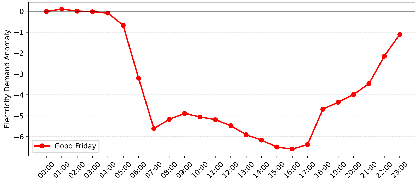
Chatswood Demand Anomaly: Good Friday (2009-2010)
