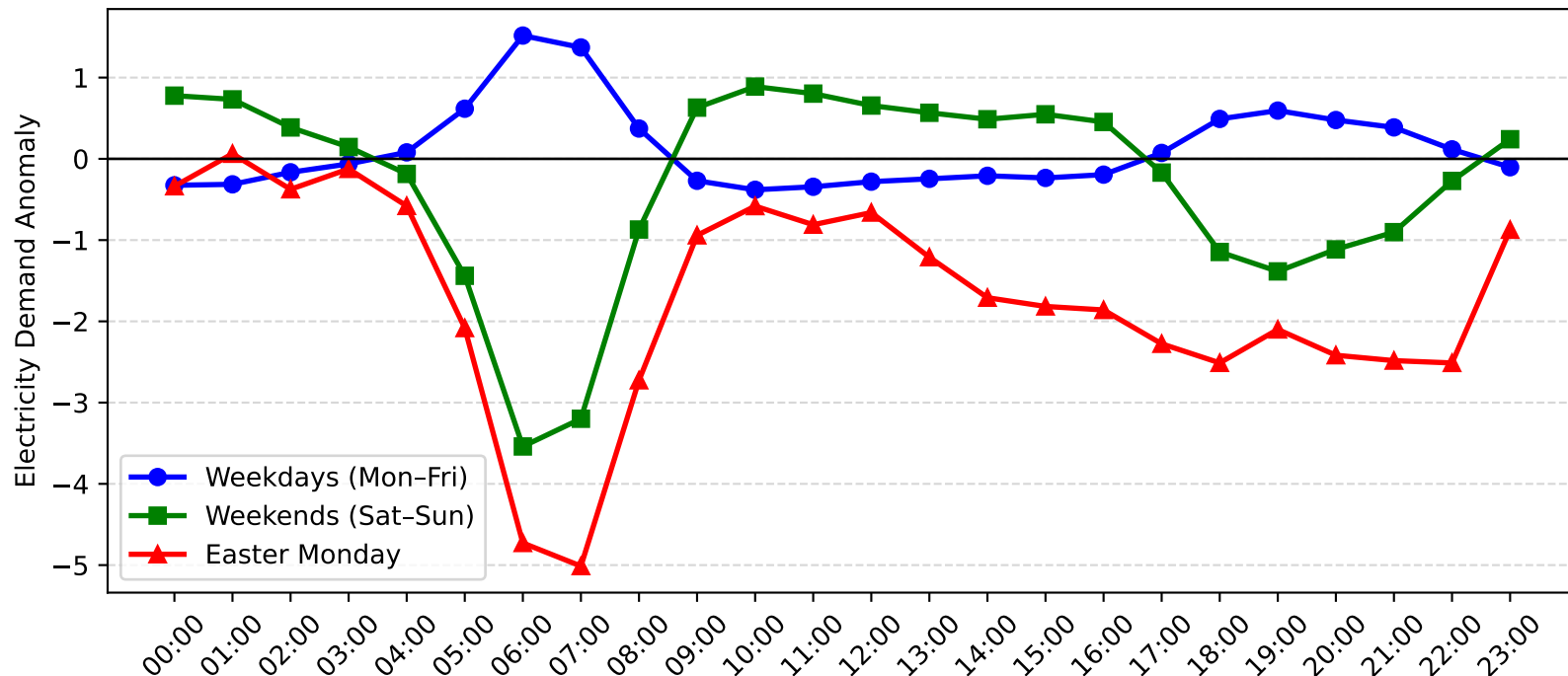
Cronulla Demand Anomaly: Easter Monday vs Weekday/Weekend (2013-2014)
