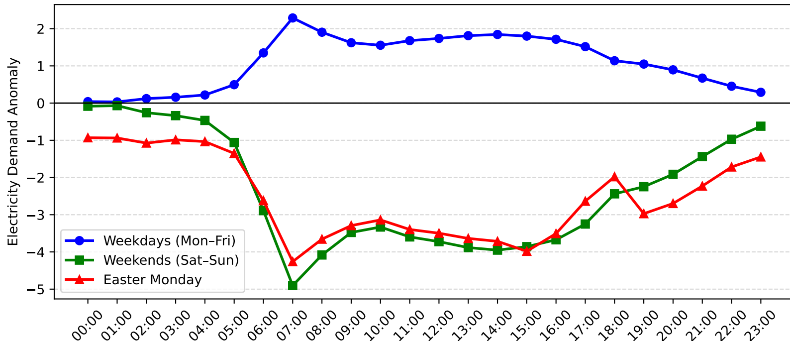
Epping Demand Anomaly: Easter Monday vs Weekday/Weekend (2017-2018)
