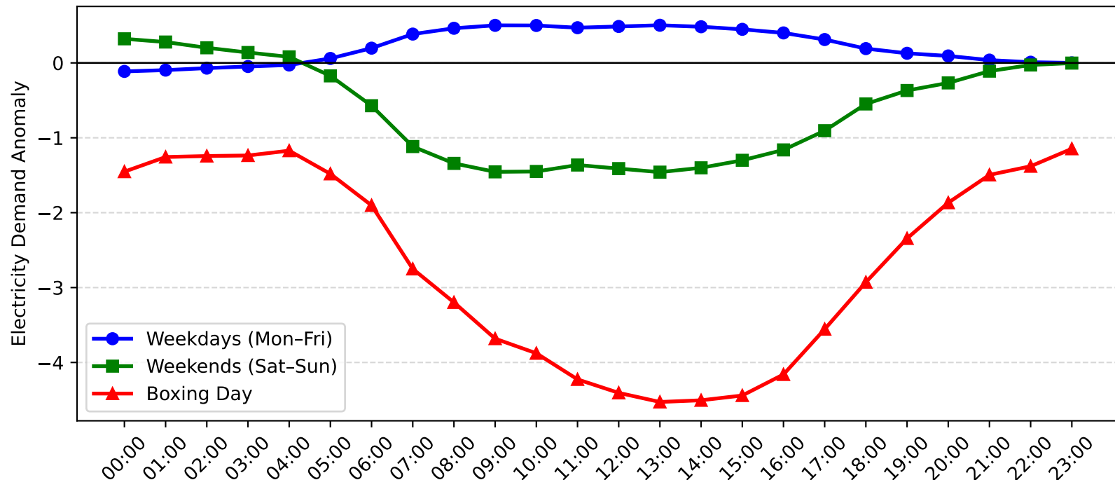
Lidcombe Demand Anomaly: Boxing Day vs Weekday/Weekend (2012-2013)
