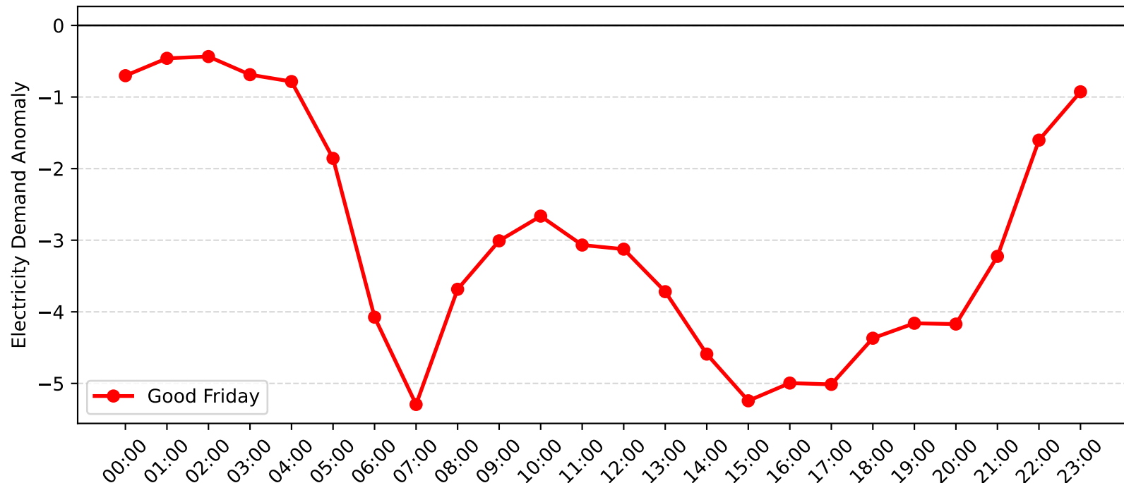
Dulwich Hill Demand Anomaly: Good Friday (2009-2010)
