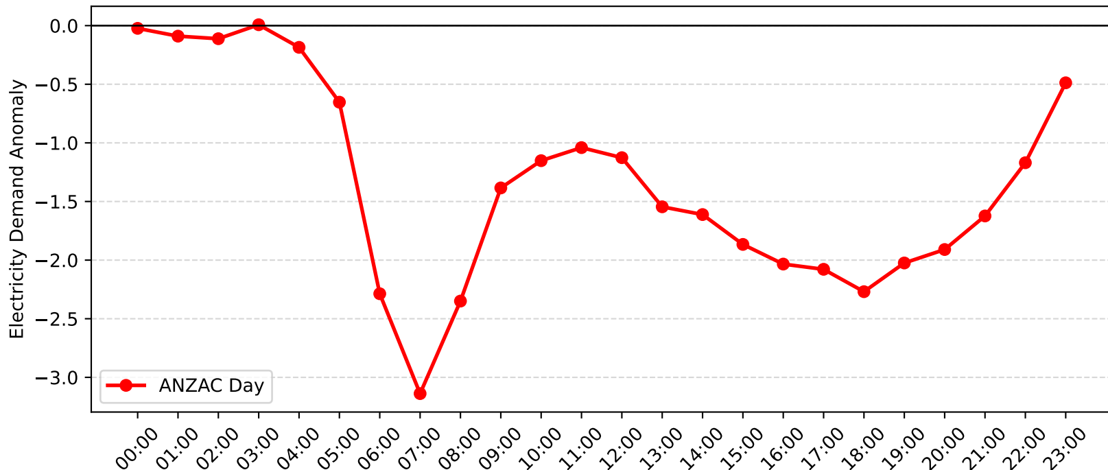
Blakehurst Demand Anomaly: ANZAC Day (2009-2010)
