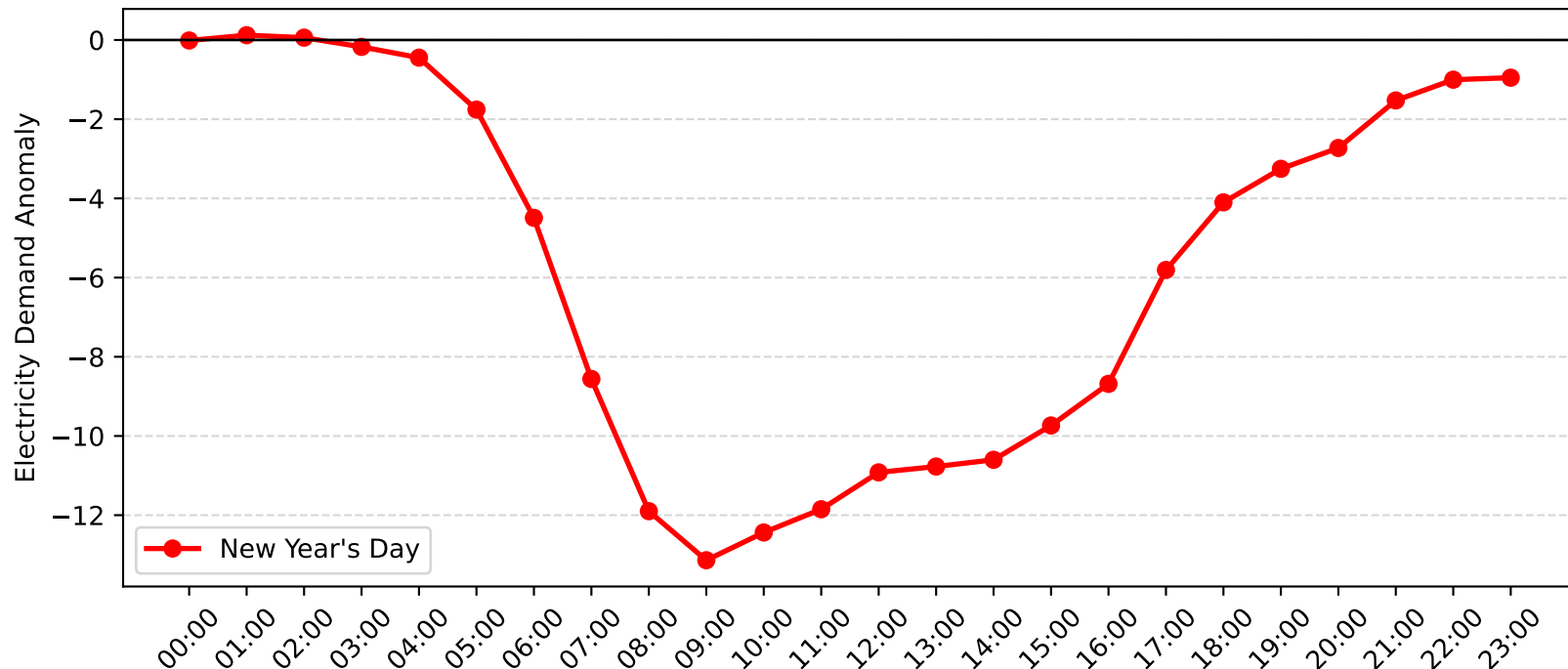
Brookvale Demand Anomaly: New Year's Day (2009-2010)
