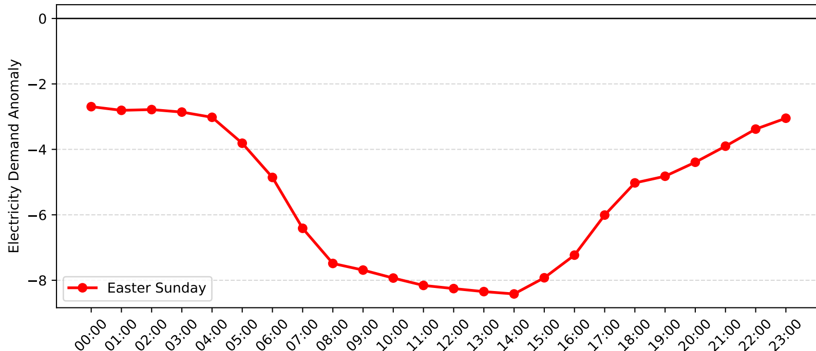
Caringbah Demand Anomaly: Easter Sunday (2010-2011)
