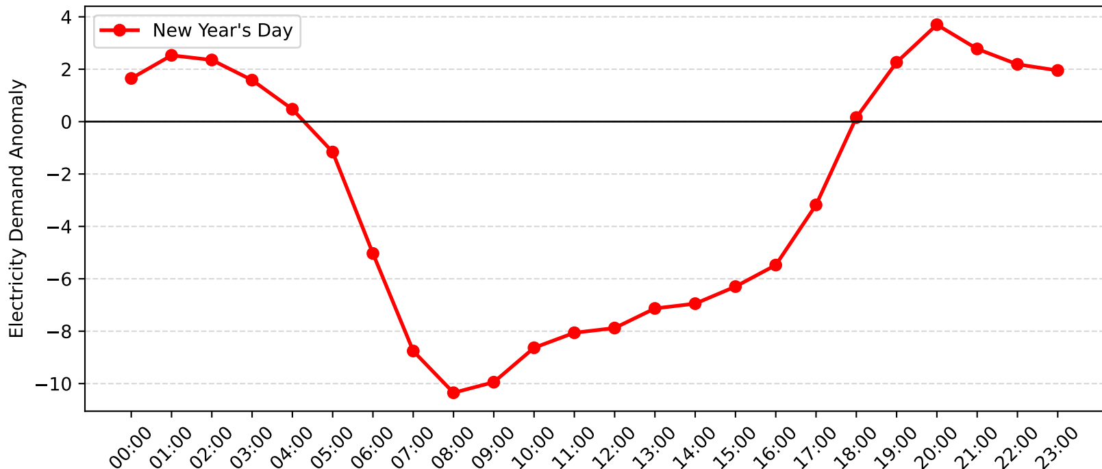
Burwood Demand Anomaly: New Year's Day (2005-2006)
