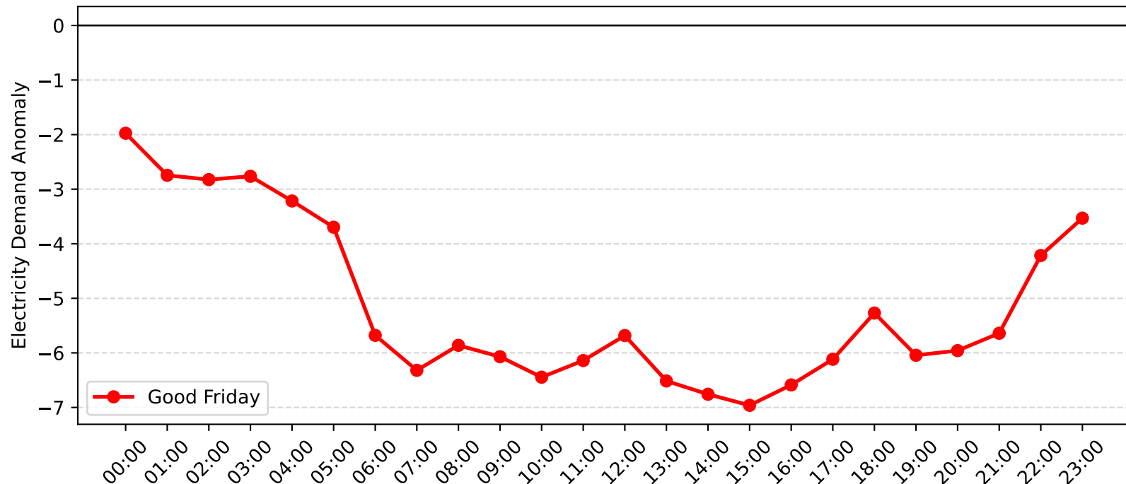
Pennant Hills Demand Anomaly: Good Friday (2017-2018)
