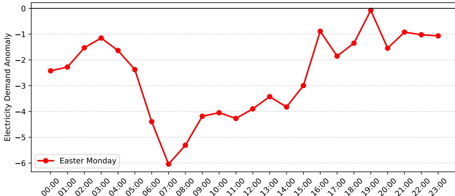
Matraville Demand Anomaly: Easter Monday (2008-2009)
