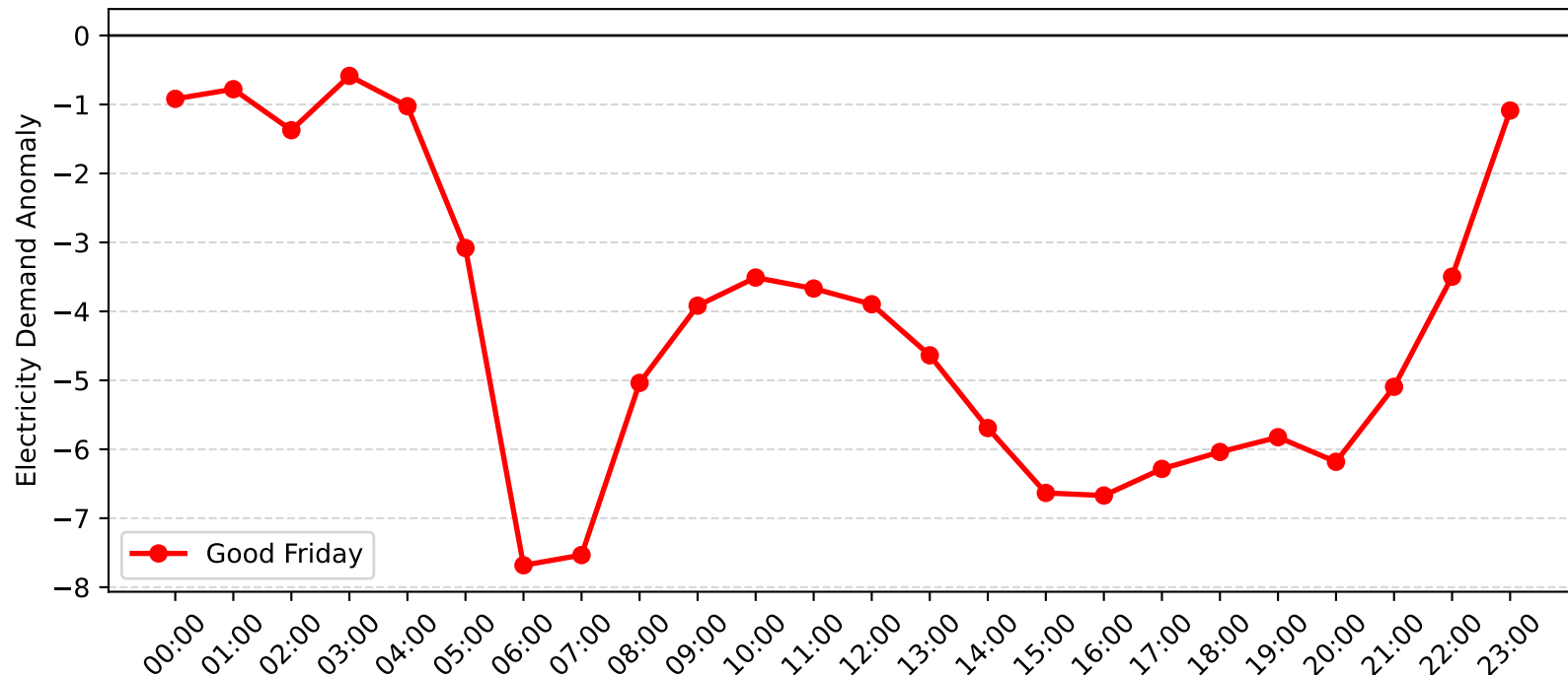
Pennant Hills Demand Anomaly: Good Friday (2005-2006)
