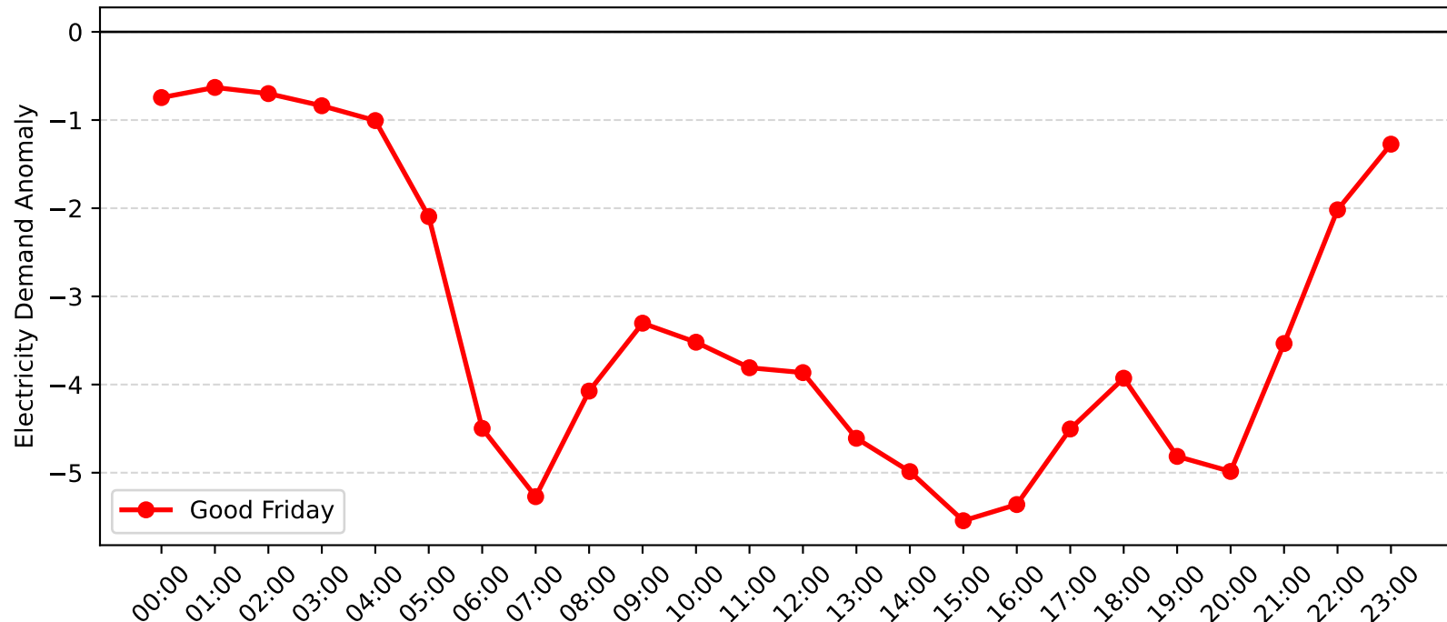
Dulwich Hill Demand Anomaly: Good Friday (2008-2009)
