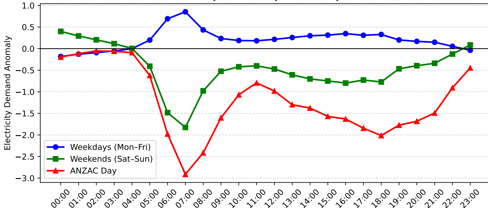
Blakehurst Demand Anomaly: ANZAC Day vs Weekday/Weekend (2010-2011)
