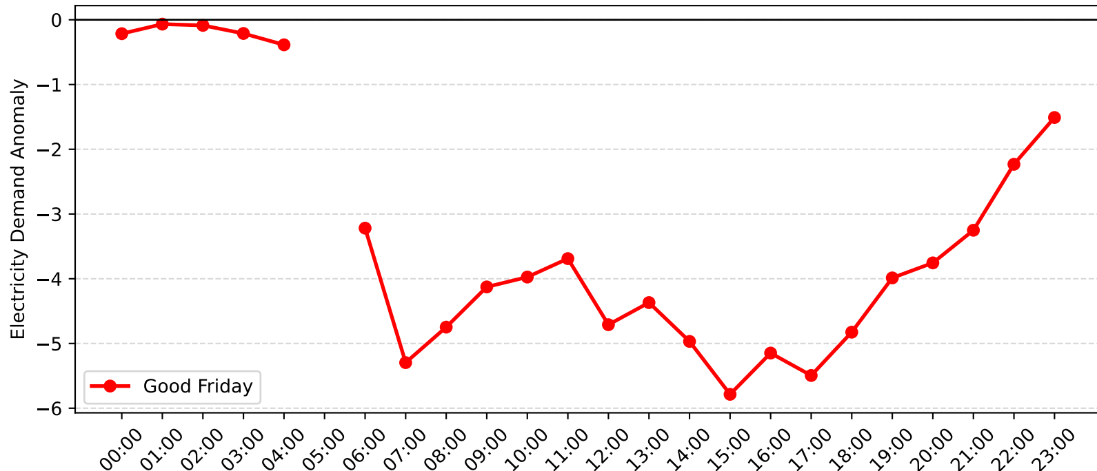
Chatswood Demand Anomaly: Good Friday (2015-2016)
