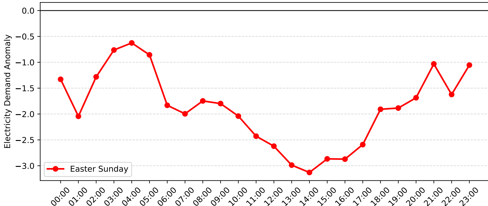
Gateshead Demand Anomaly: Easter Sunday (2006-2007)
