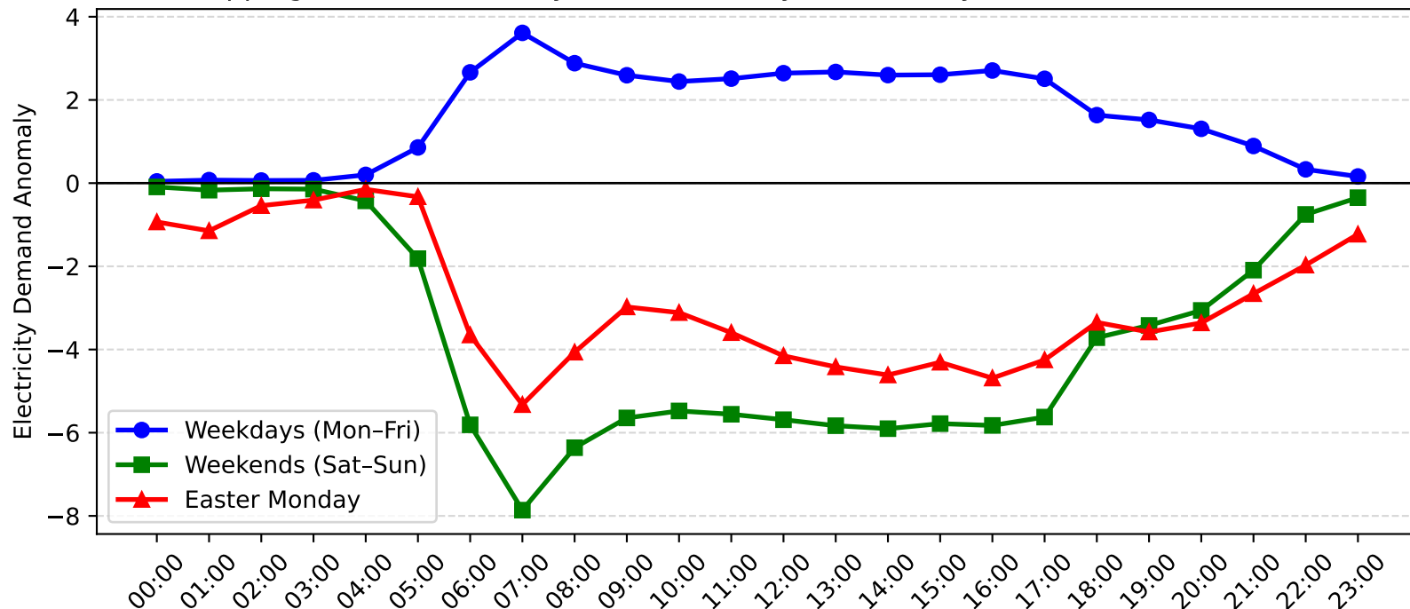
Epping Demand Anomaly: Easter Monday vs Weekday/Weekend (2009-2010)
