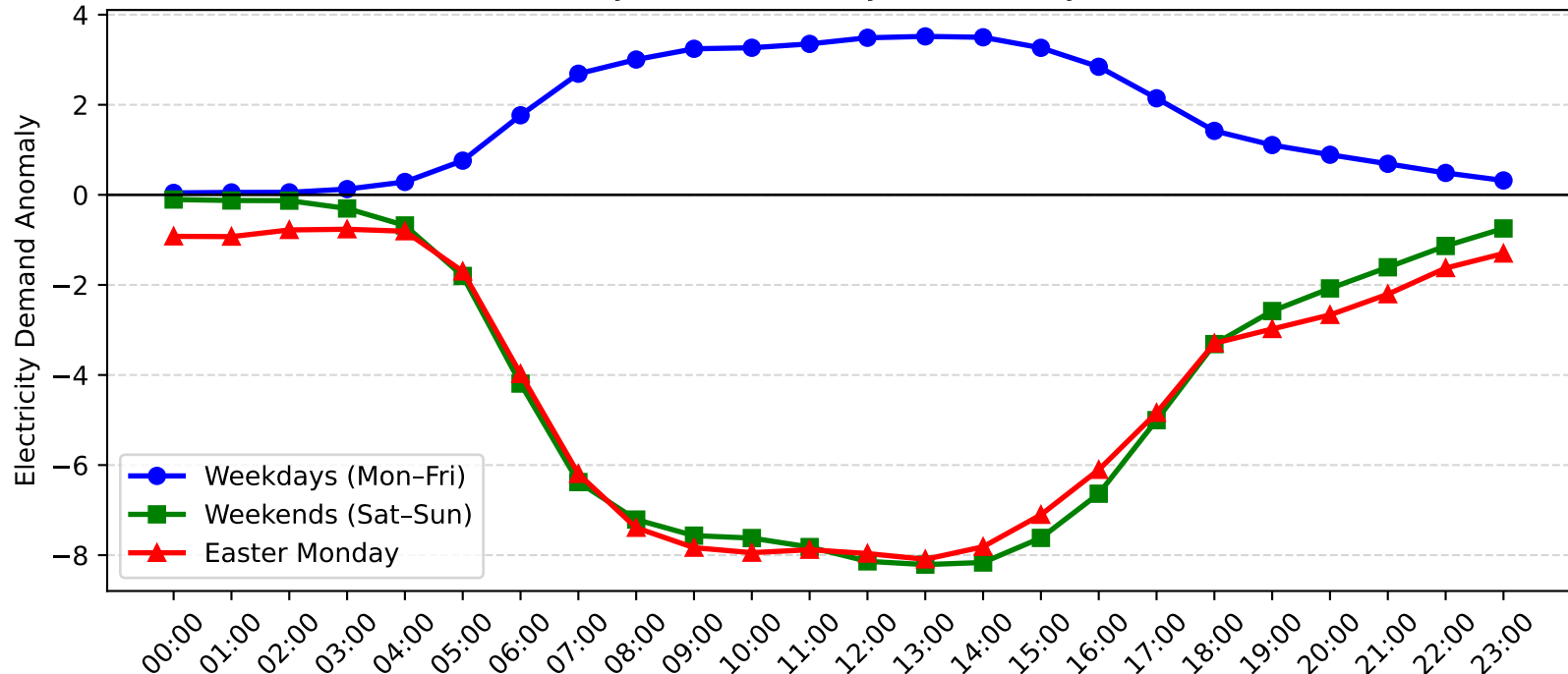
Mascot Demand Anomaly: Easter Monday vs Weekday/Weekend (2011-2012)
