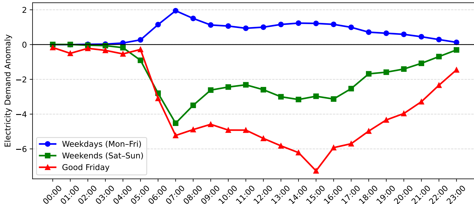
Chatswood Demand Anomaly: Good Friday vs Weekday/Weekend (2016-2017)
