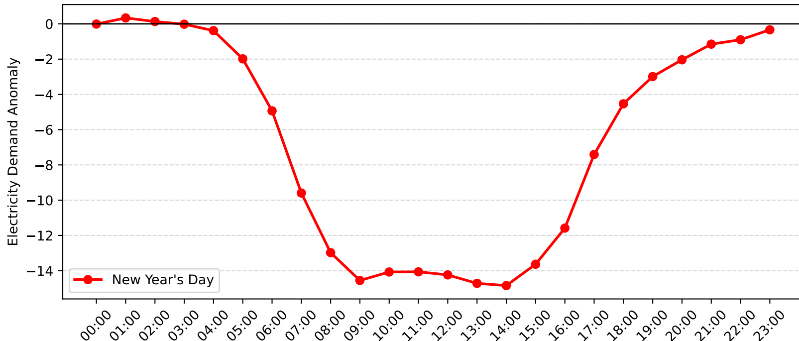
Brookvale Demand Anomaly: New Year's Day (2005-2006)
