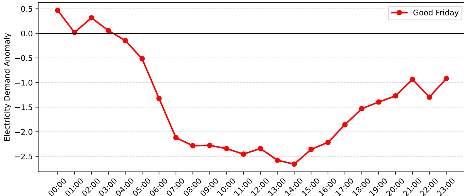
Gateshead Demand Anomaly: Good Friday (2013-2014)
