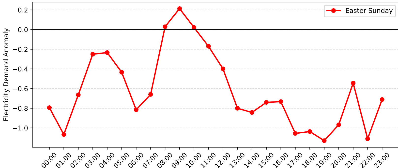
Jewells Demand Anomaly: Easter Sunday (2014-2015)
