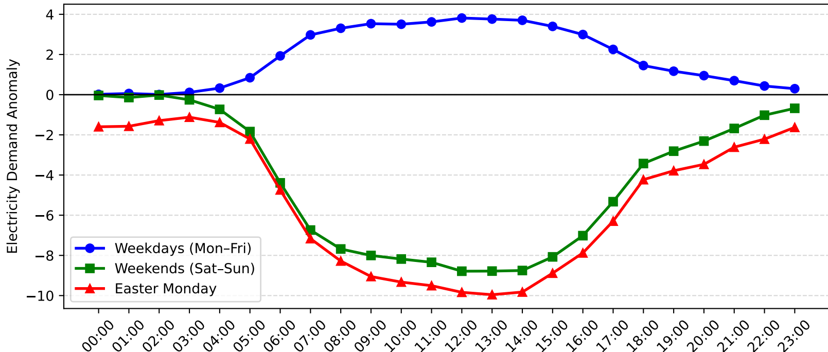
Mascot Demand Anomaly: Easter Monday vs Weekday/Weekend (2010-2011)
