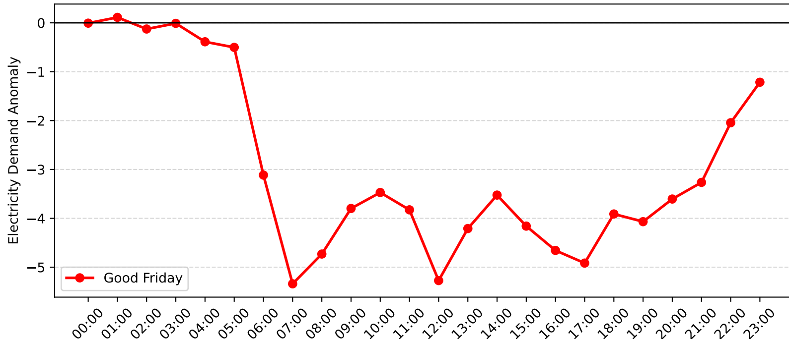
Chatswood Demand Anomaly: Good Friday (2014-2015)
