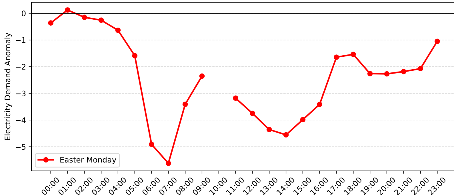
Mortdale Demand Anomaly: Easter Monday (2005-2006)
