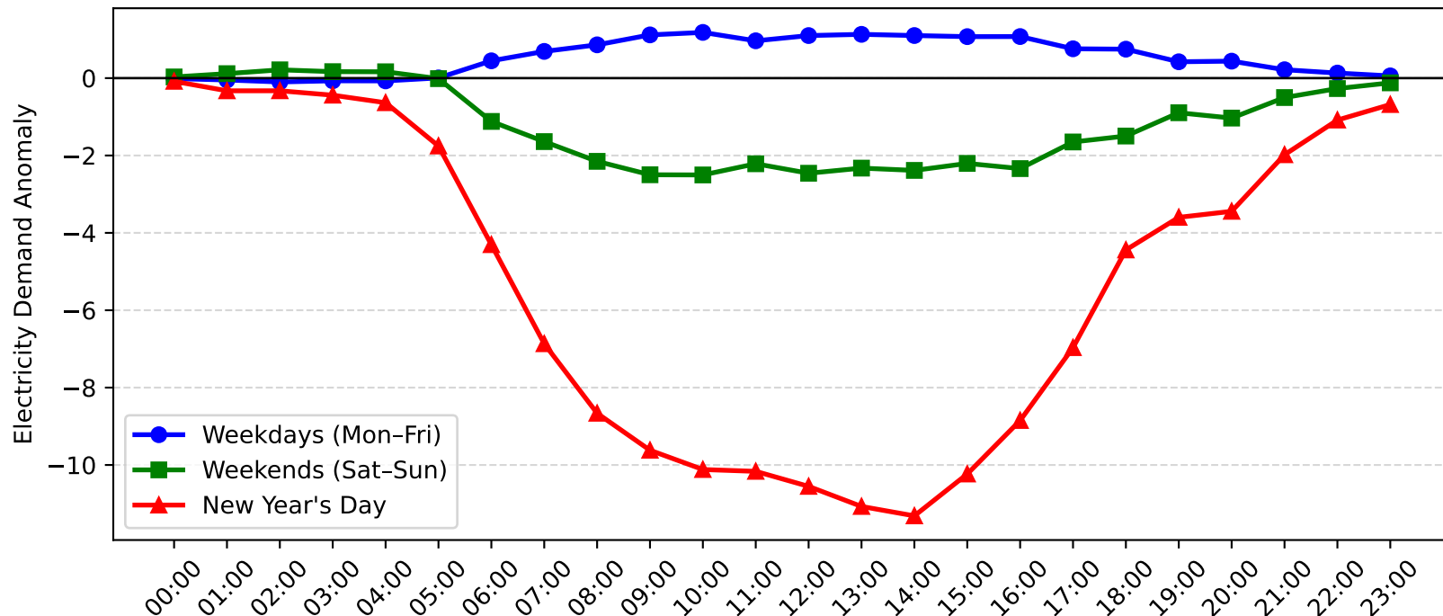
Brookvale Demand Anomaly: New Year's Day vs Weekday/Weekend (2004-2005)
