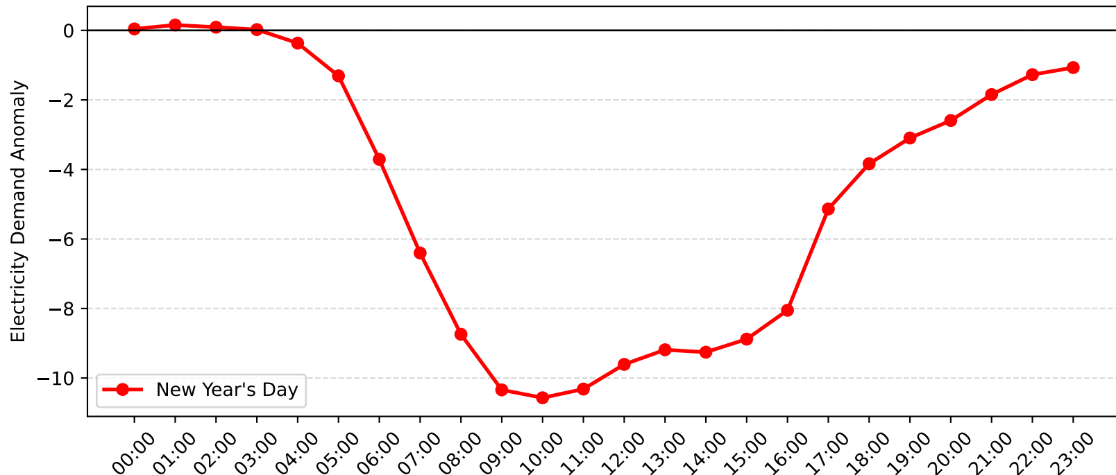
Brookvale Demand Anomaly: New Year's Day (2013-2014)
