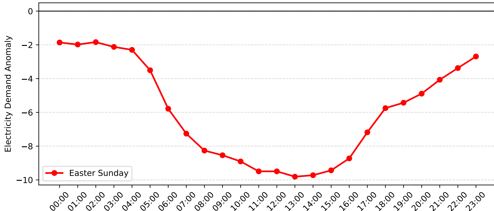
Caringbah Demand Anomaly: Easter Sunday (2005-2006)
