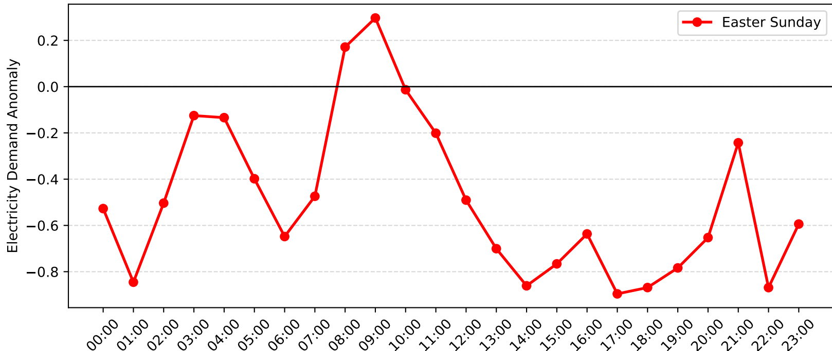
Jewells Demand Anomaly: Easter Sunday (2015-2016)
