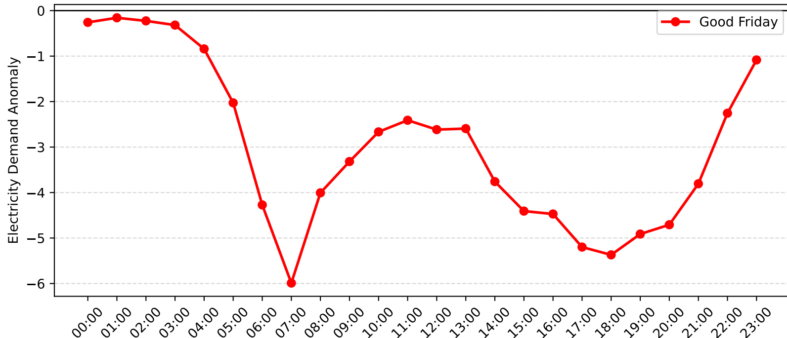
Dulwich Hill Demand Anomaly: Good Friday (2010-2011)
