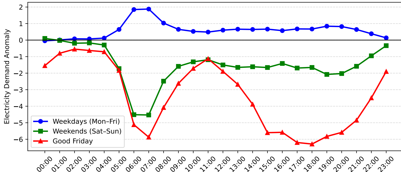
Pennant Hills Demand Anomaly: Good Friday vs Weekday/Weekend (2015-2016)
