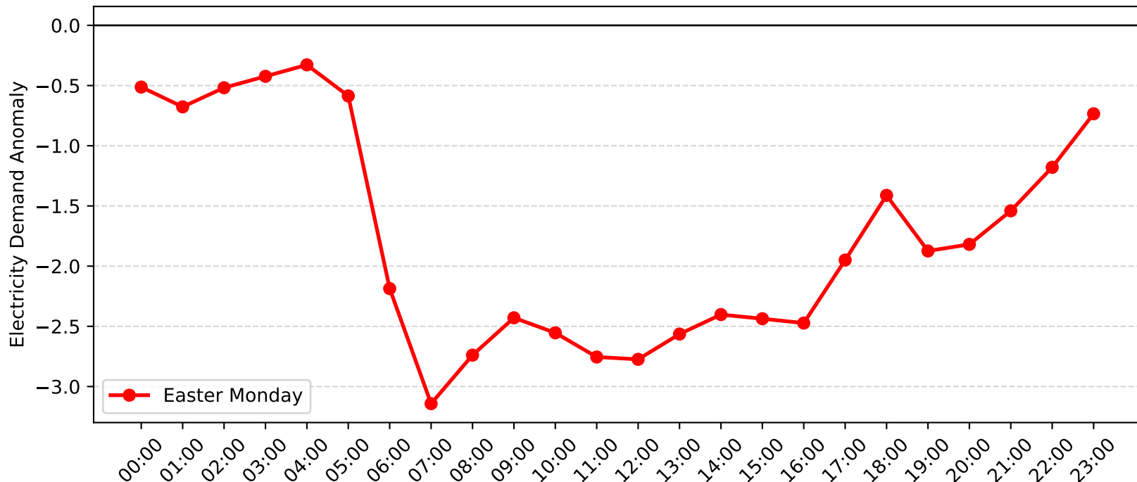
Pymble Demand Anomaly: Easter Monday (2014-2015)
