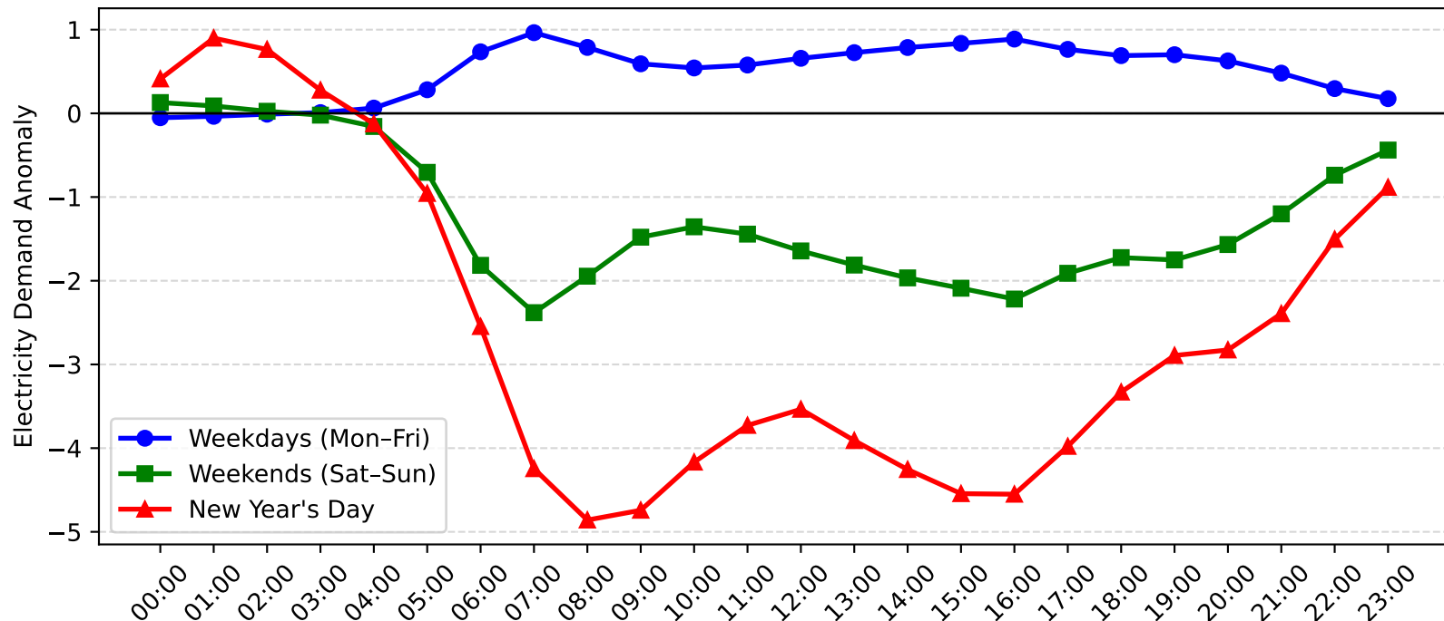
Five Dock Demand Anomaly: New Year's Day vs Weekday/Weekend (2016-2017)
