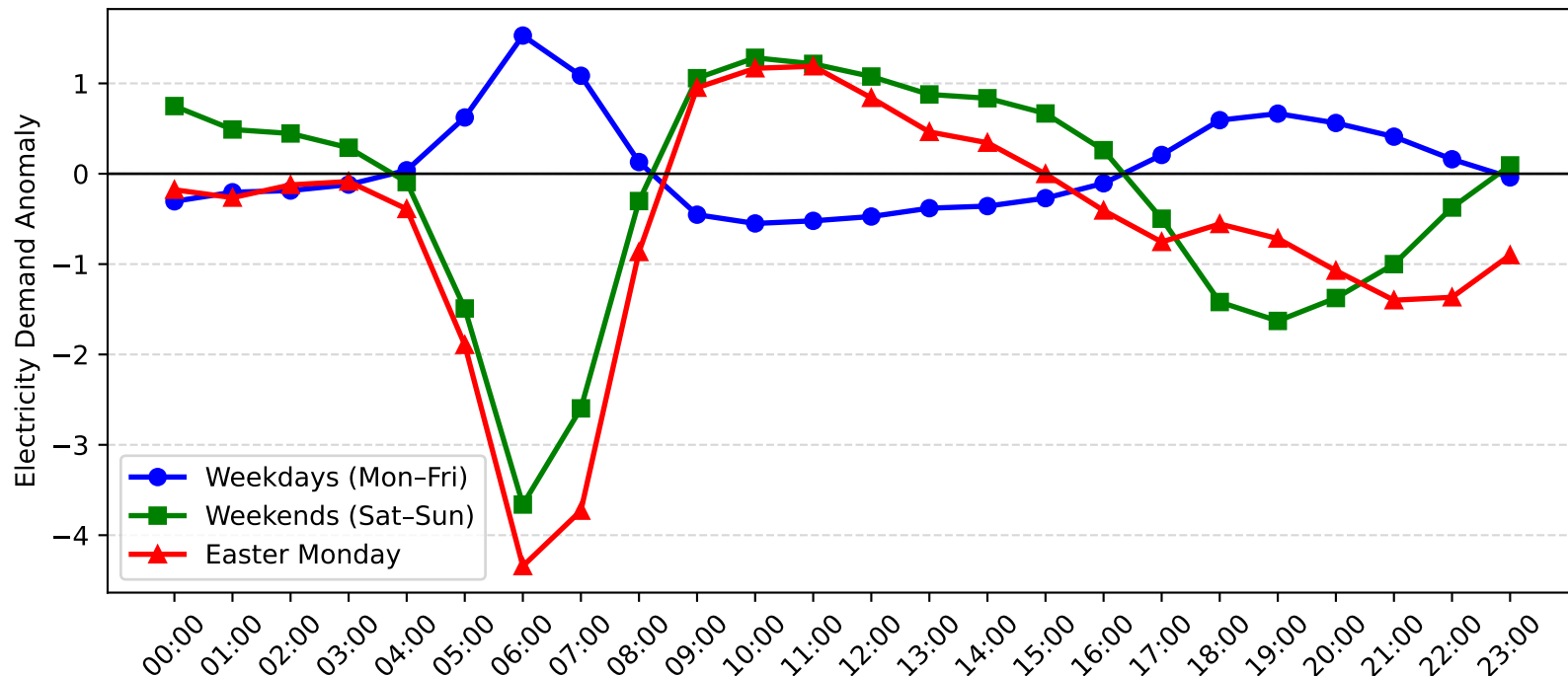
Cronulla Demand Anomaly: Easter Monday vs Weekday/Weekend (2007-2008)
