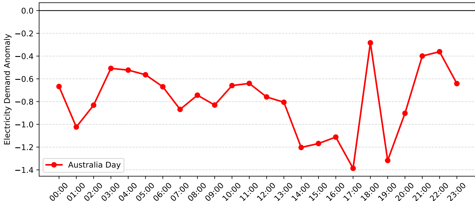
Woy Woy Demand Anomaly: Australia Day (2004-2005)
