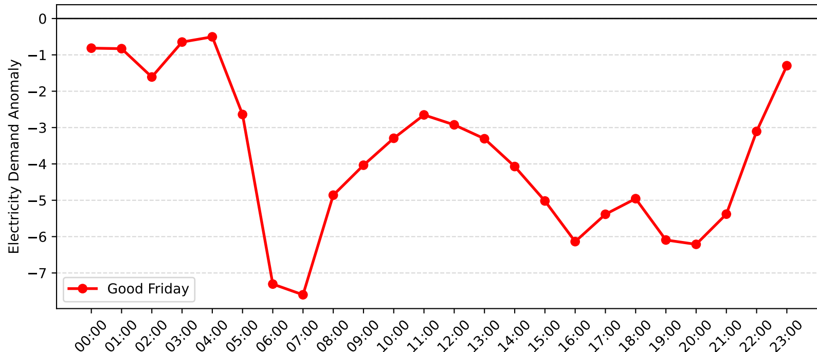
Pennant Hills Demand Anomaly: Good Friday (2006-2007)
