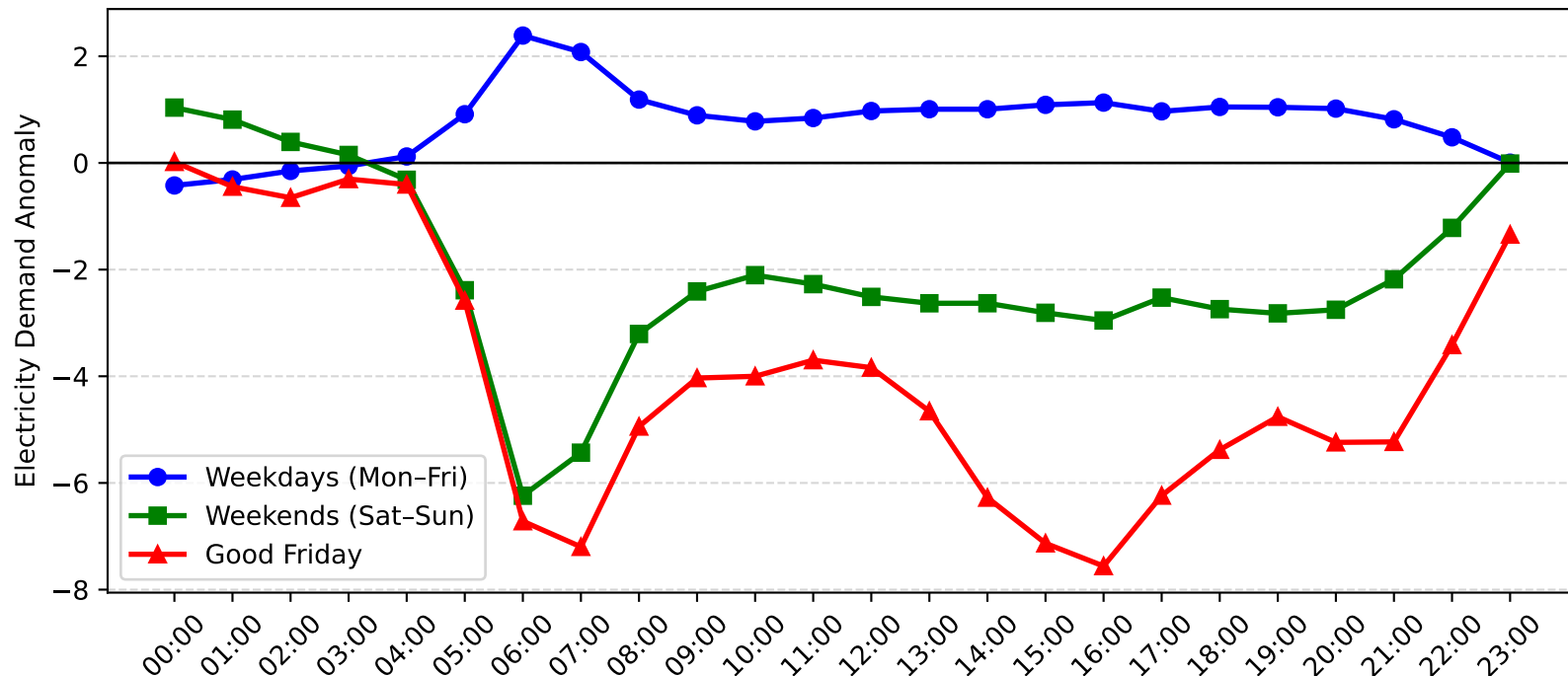
Pennant Hills Demand Anomaly: Good Friday vs Weekday/Weekend (2007-2008)
