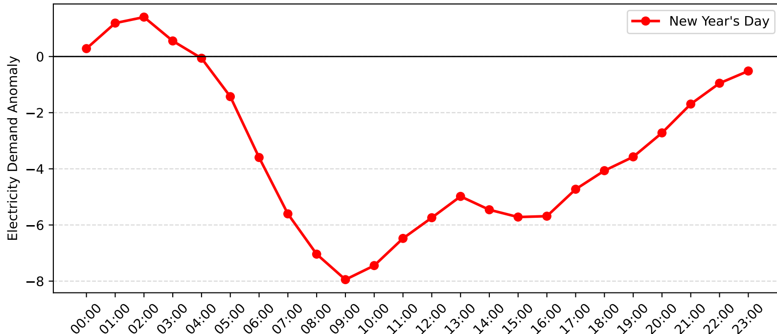
Burwood Demand Anomaly: New Year's Day (2013-2014)
