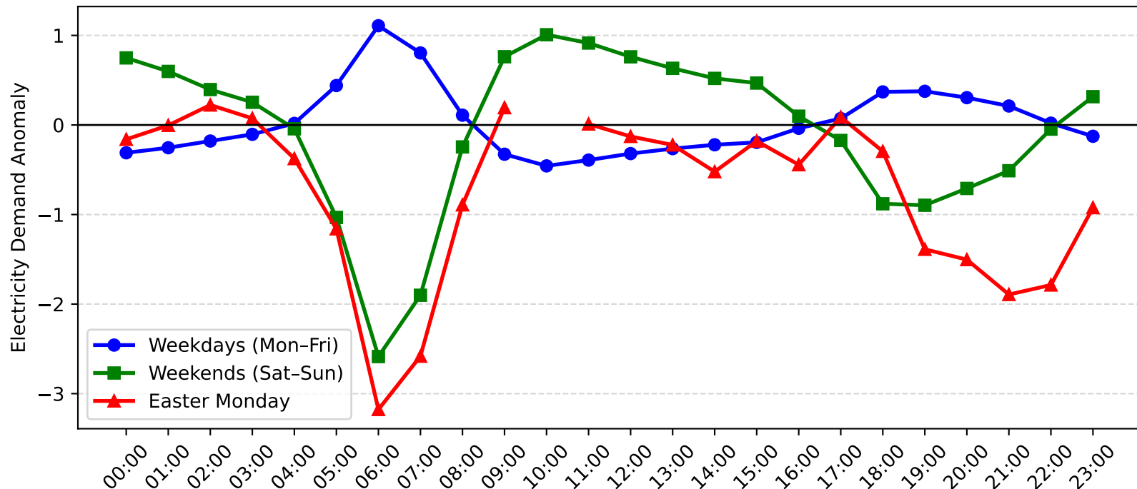
Cronulla Demand Anomaly: Easter Monday vs Weekday/Weekend (2005-2006)
