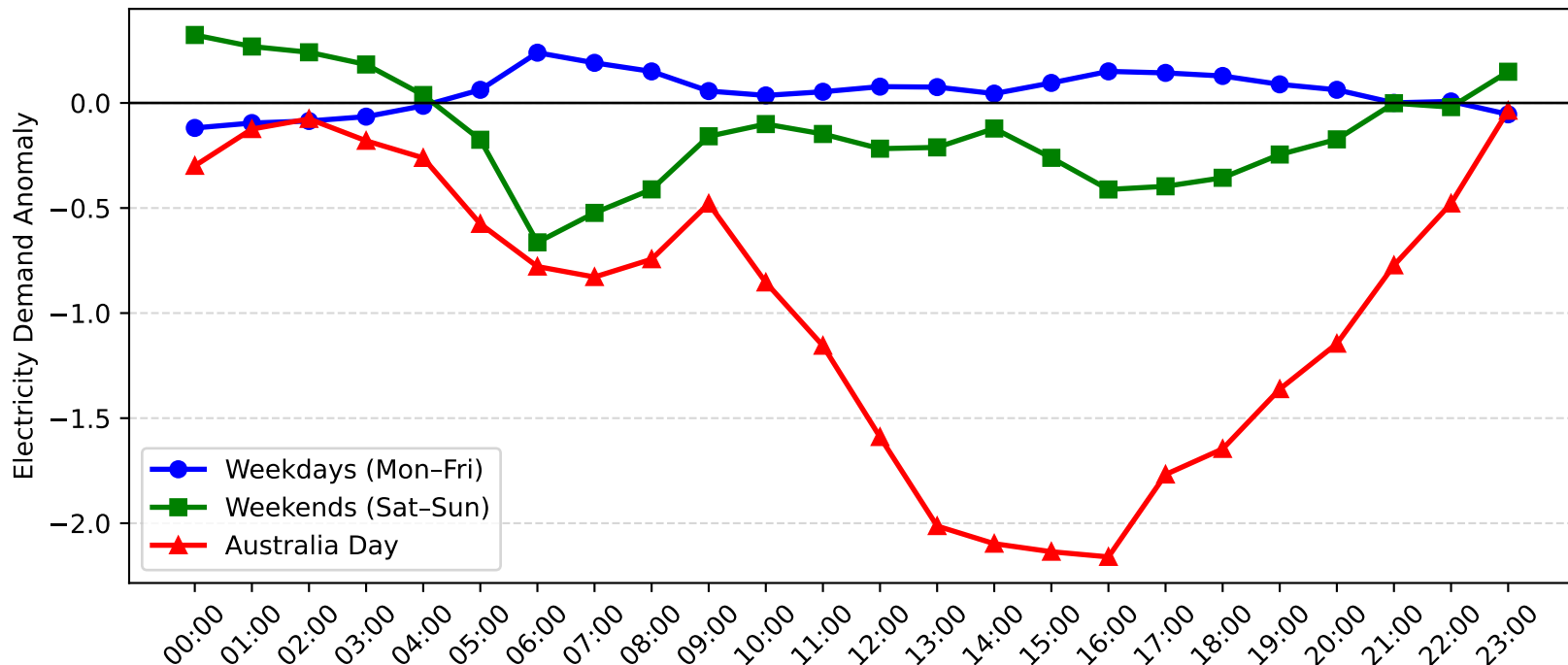
Woy Woy Demand Anomaly: Australia Day vs Weekday/Weekend (2016-2017)
