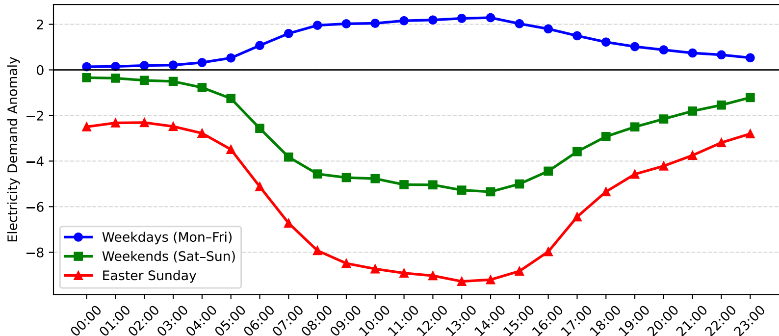
Caringbah Demand Anomaly: Easter Sunday vs Weekday/Weekend (2007-2008)
