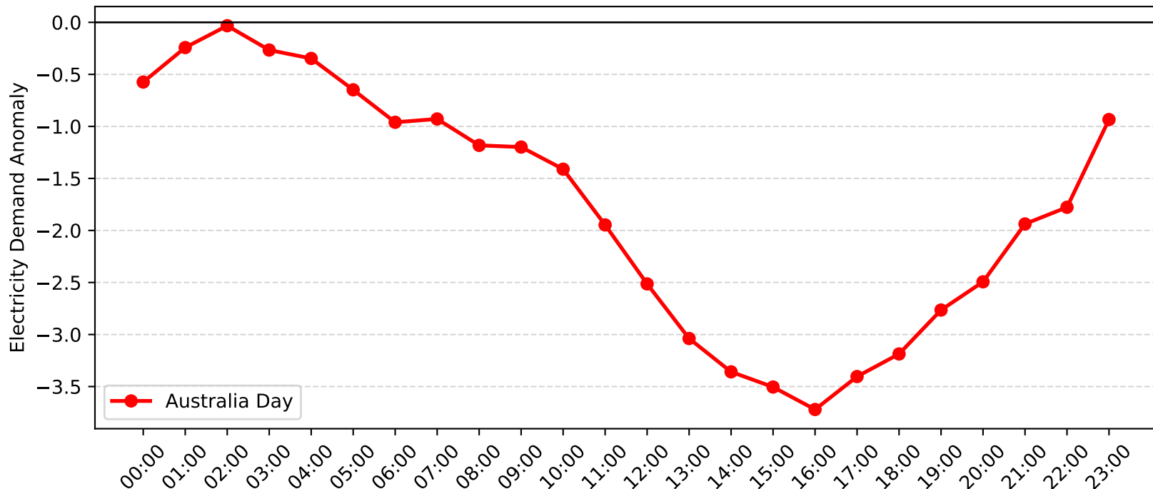
Woy Woy Demand Anomaly: Australia Day (2017-2018)
