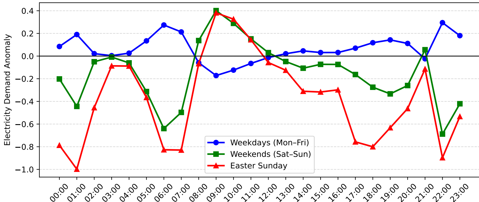
Jewells Demand Anomaly: Easter Sunday vs Weekday/Weekend (2012-2013)
