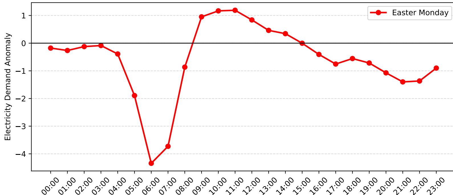
Cronulla Demand Anomaly: Easter Monday (2007-2008)
