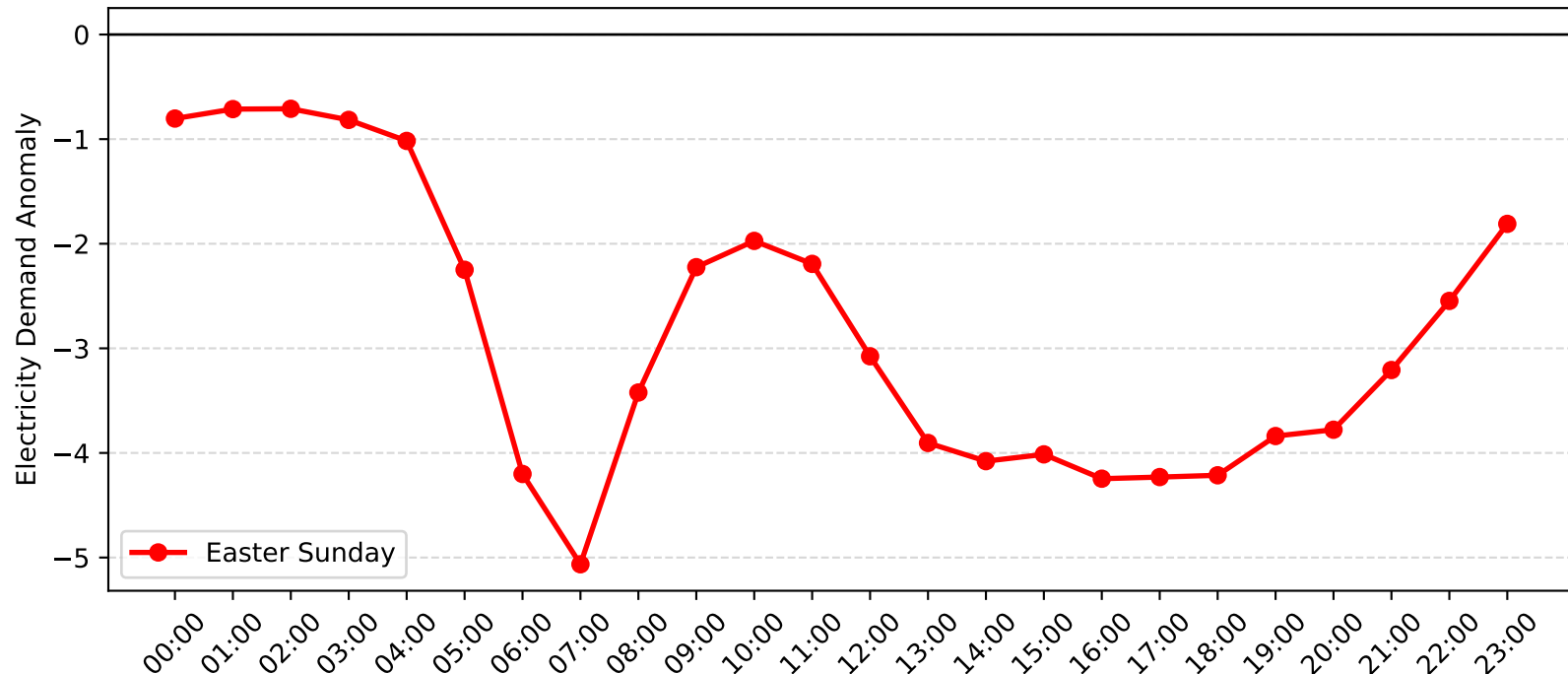
Dulwich Hill Demand Anomaly: Easter Sunday (2016-2017)
