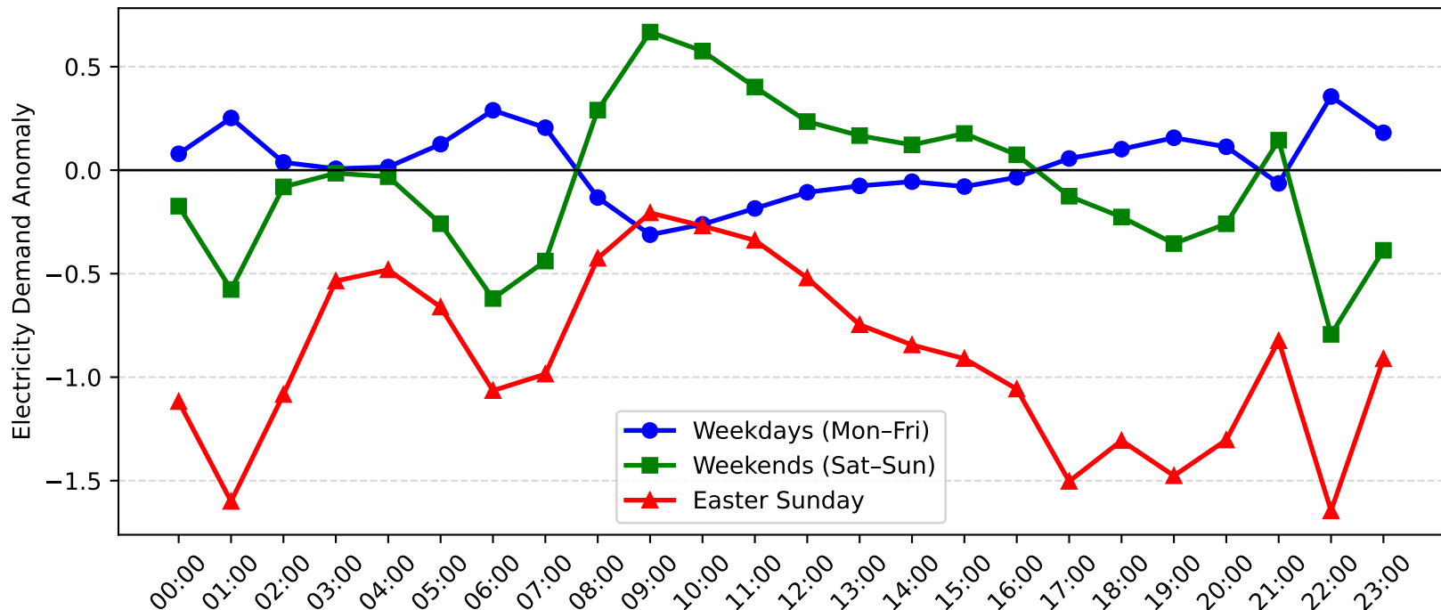
Jewells Demand Anomaly: Easter Sunday vs Weekday/Weekend (2010-2011)
