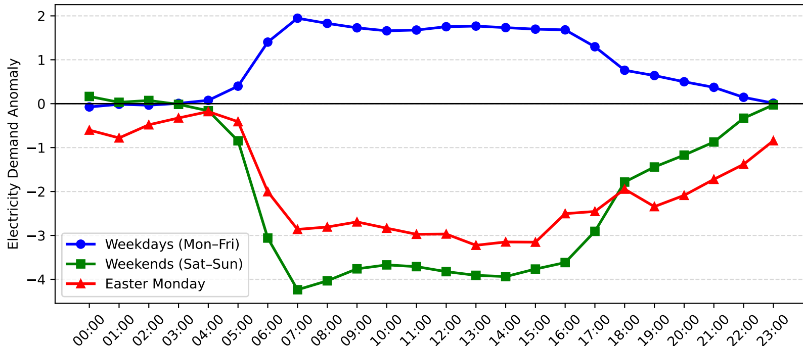
Pymble Demand Anomaly: Easter Monday vs Weekday/Weekend (2009-2010)
