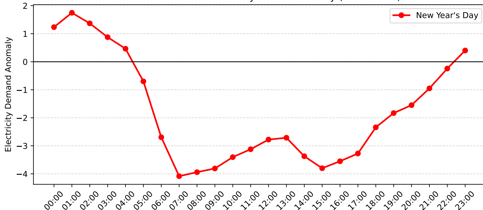
Five Dock Demand Anomaly: New Year's Day (2014-2015)
