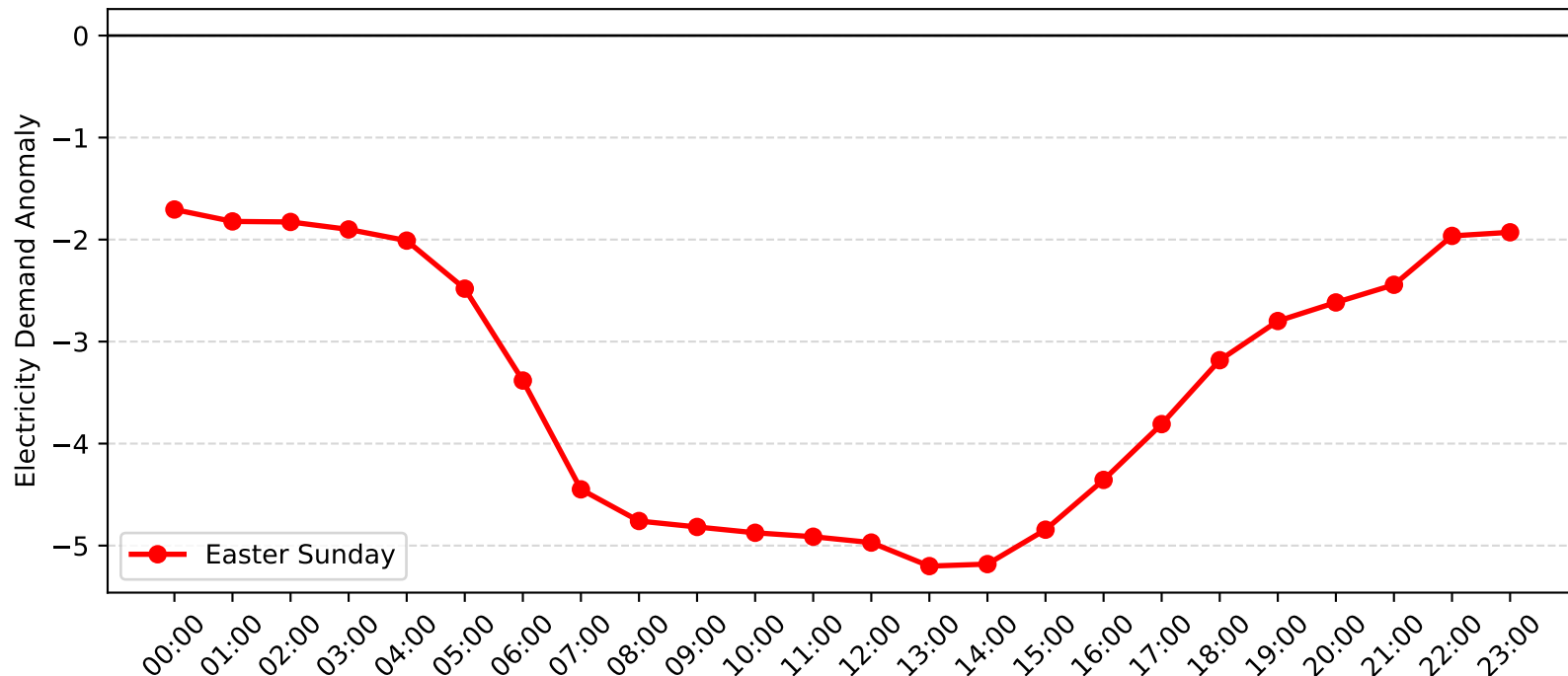
Caringbah Demand Anomaly: Easter Sunday (2012-2013)
