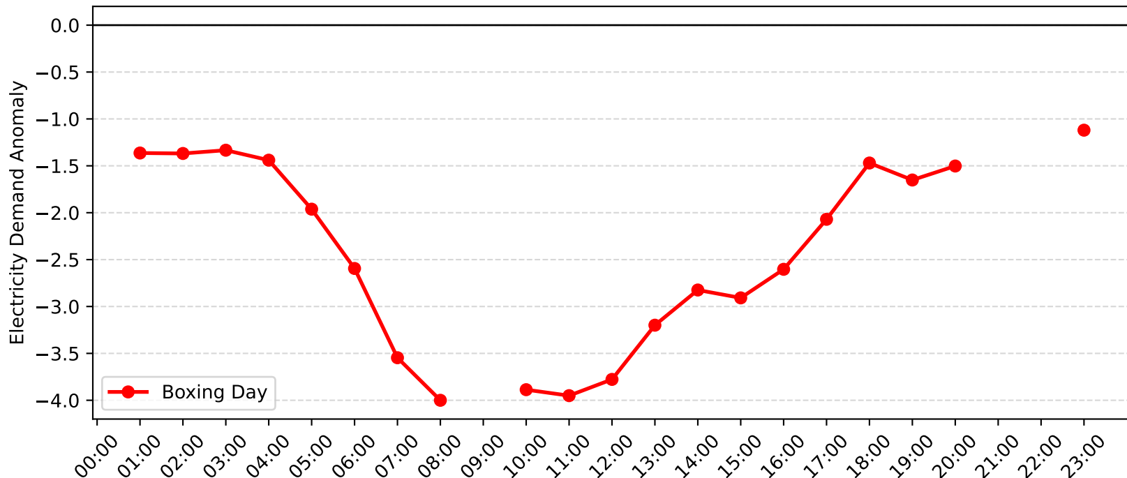
Lidcombe Demand Anomaly: Boxing Day (2008-2009)
