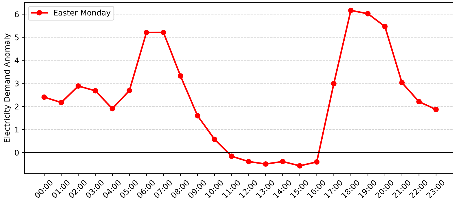
Cronulla Demand Anomaly: Easter Monday (2004-2005)
