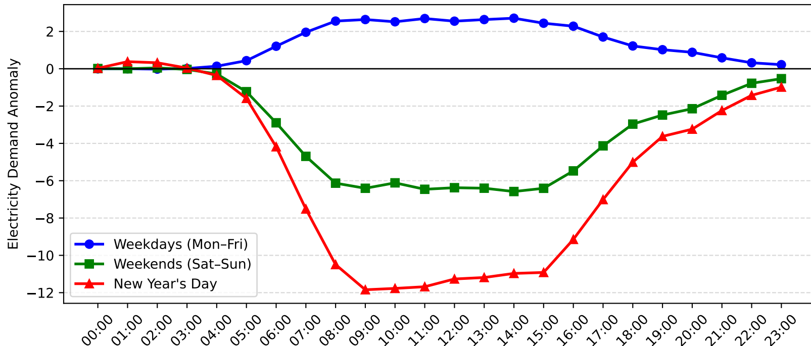
Brookvale Demand Anomaly: New Year's Day vs Weekday/Weekend (2016-2017)
