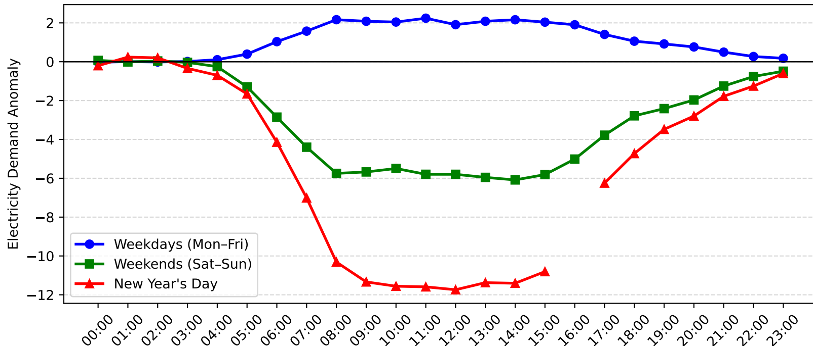
Brookvale Demand Anomaly: New Year's Day vs Weekday/Weekend (2015-2016)
