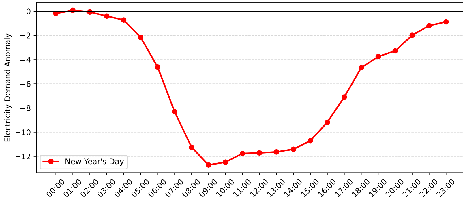
Brookvale Demand Anomaly: New Year's Day (2011-2012)
