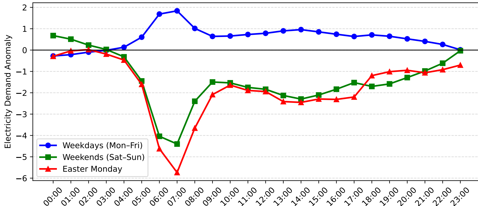
Mortdale Demand Anomaly: Easter Monday vs Weekday/Weekend (2007-2008)
