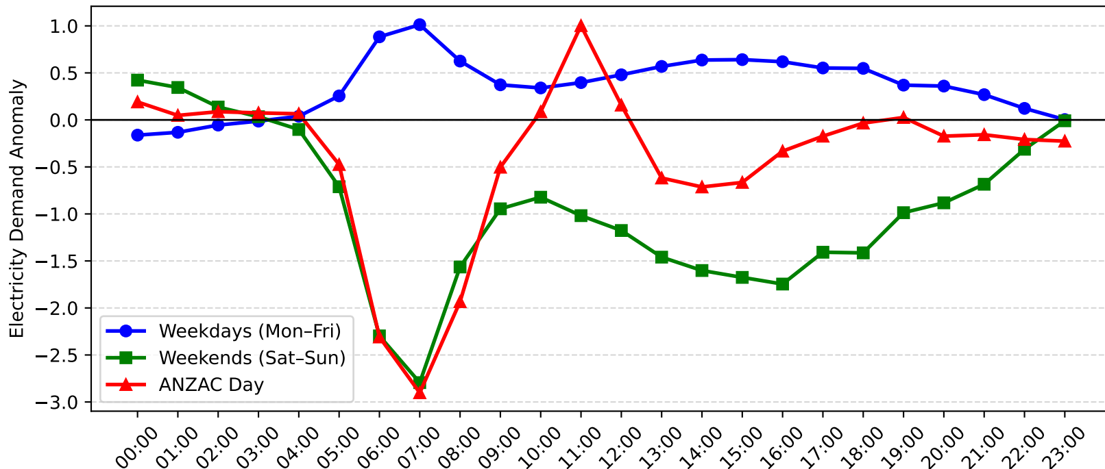
Blakehurst Demand Anomaly: ANZAC Day vs Weekday/Weekend (2006-2007)
