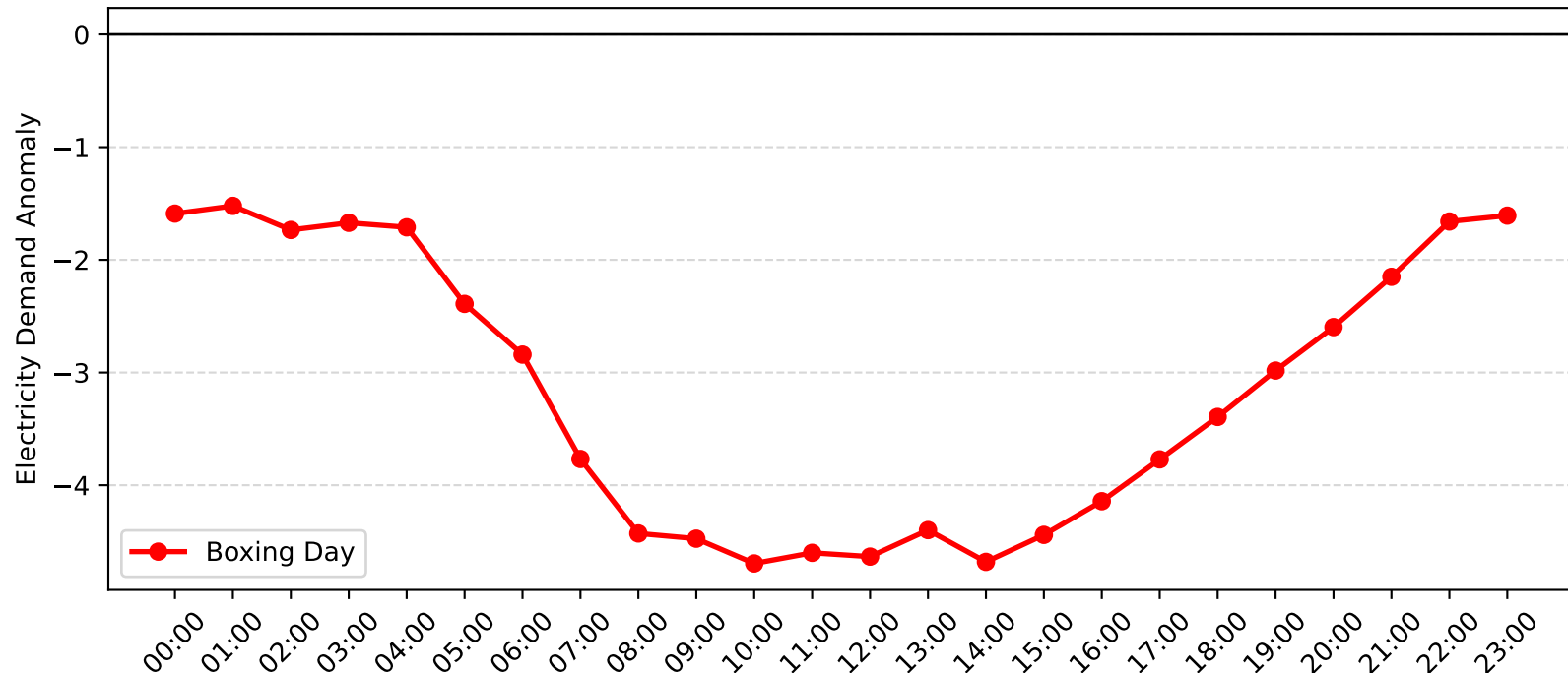
Lidcombe Demand Anomaly: Boxing Day (2004-2005)
