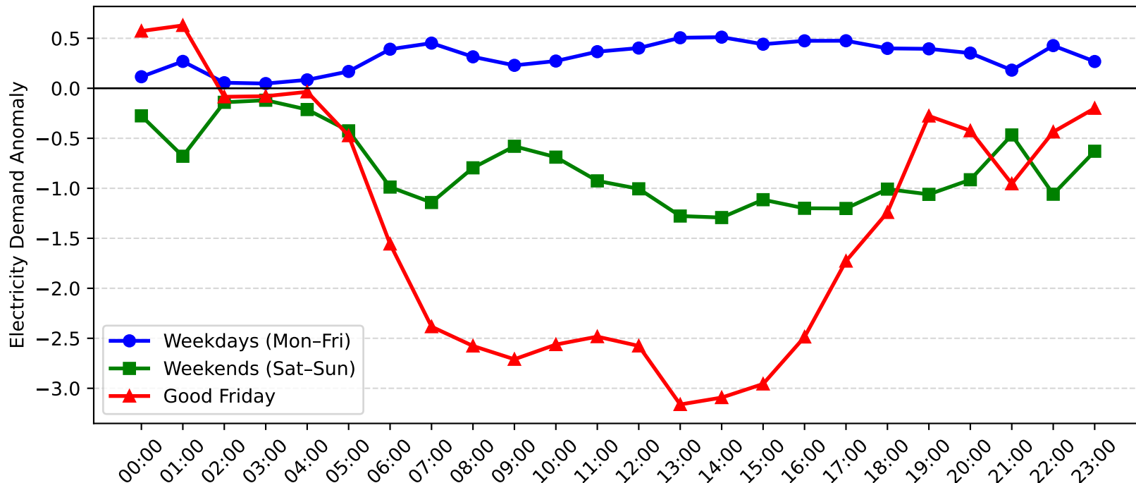
Gateshead Demand Anomaly: Good Friday vs Weekday/Weekend (2007-2008)
