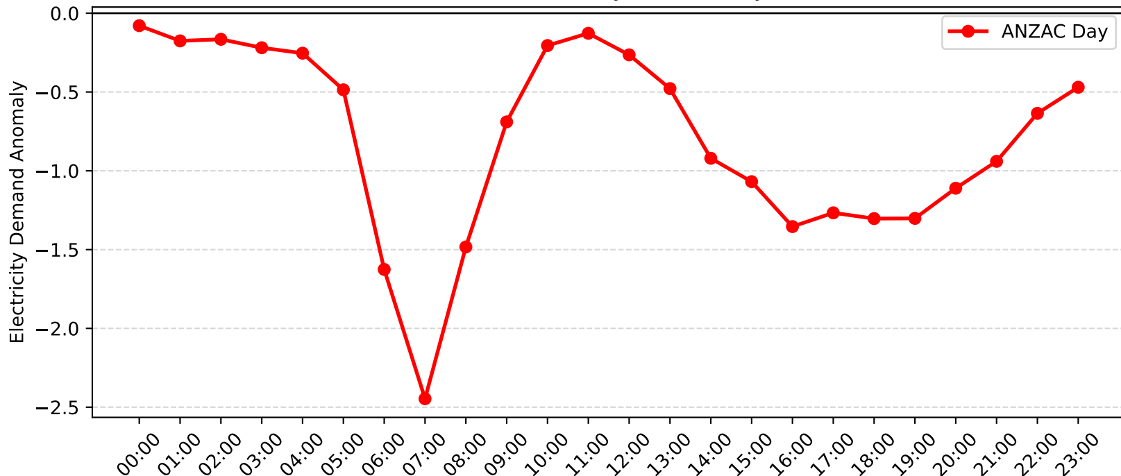
Blakehurst Demand Anomaly: ANZAC Day (2013-2014)
