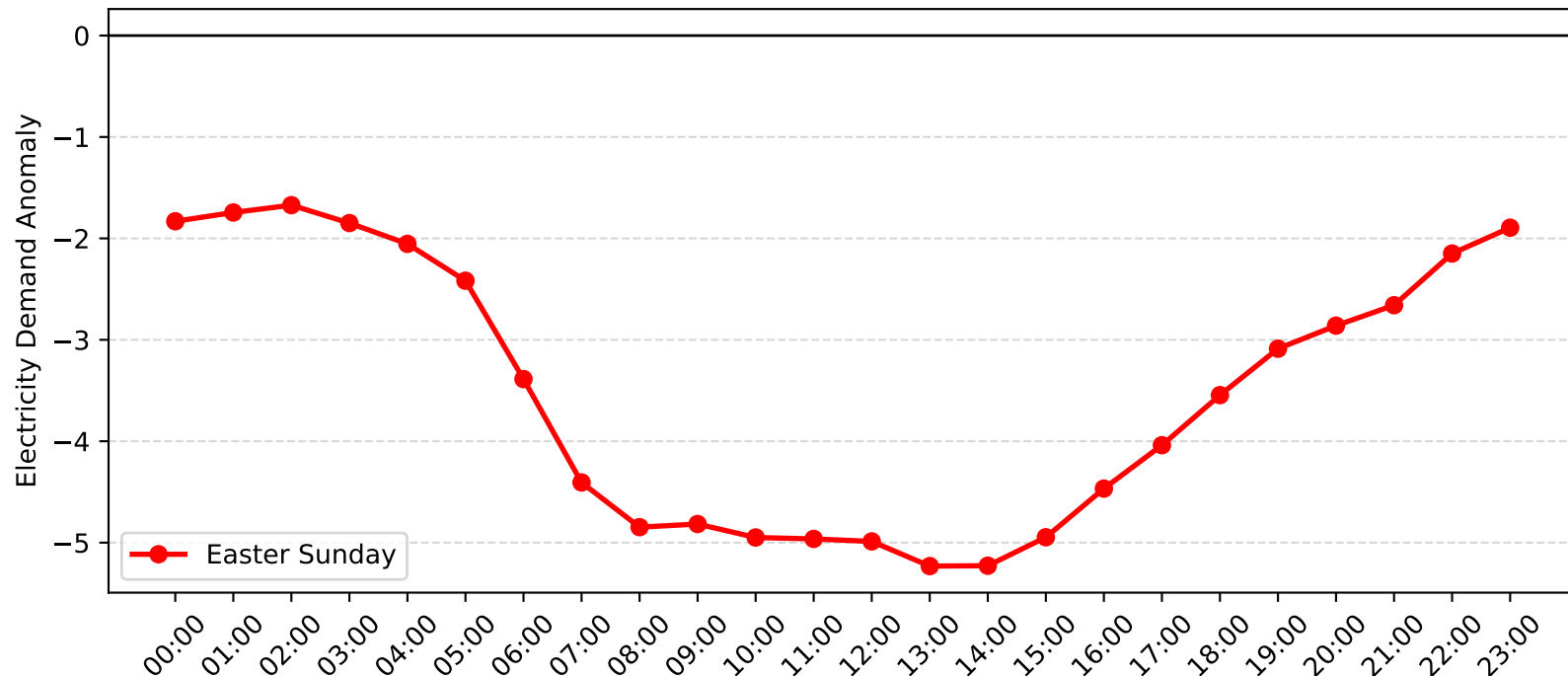
Caringbah Demand Anomaly: Easter Sunday (2013-2014)
