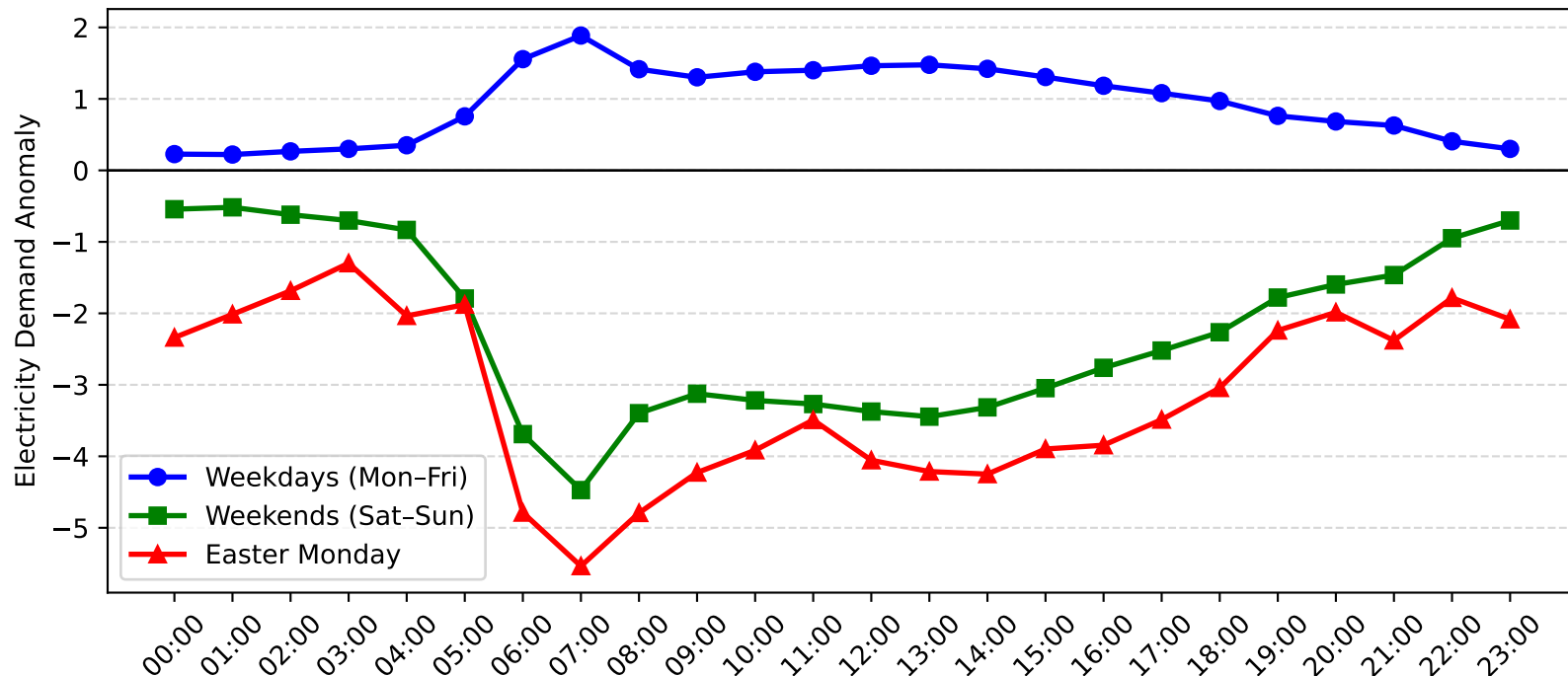
Matravlle Demand Anomaly: Easter Monday vs Weekday/Weekend (2012-2013)
