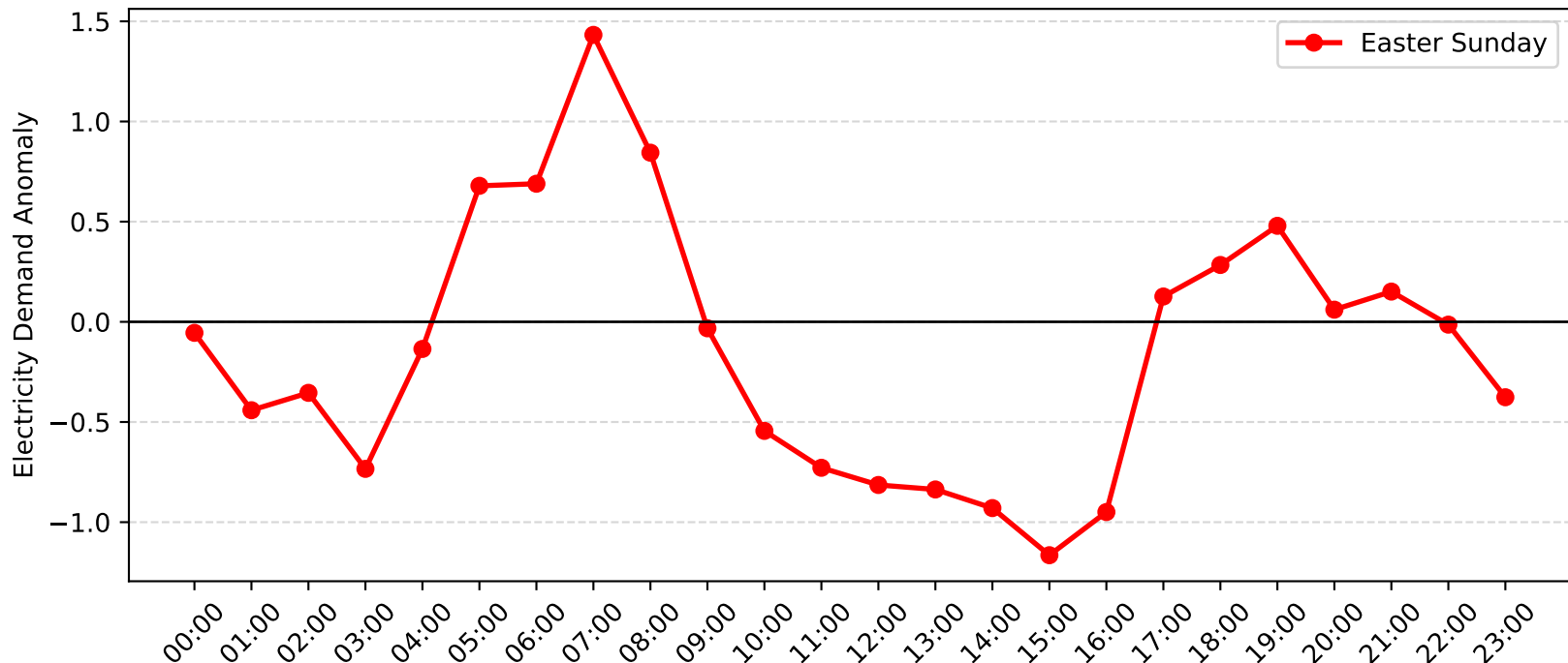
Jewells Demand Anomaly: Easter Sunday (2004-2005)
