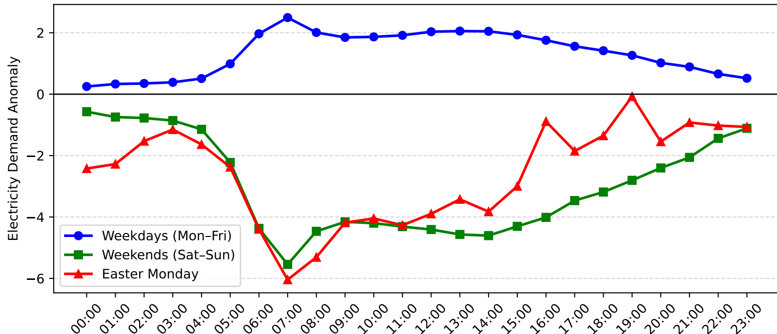
Matraverse Demand Anomaly: Easter Monday vs Weekday/Weekend (2008-2009)
