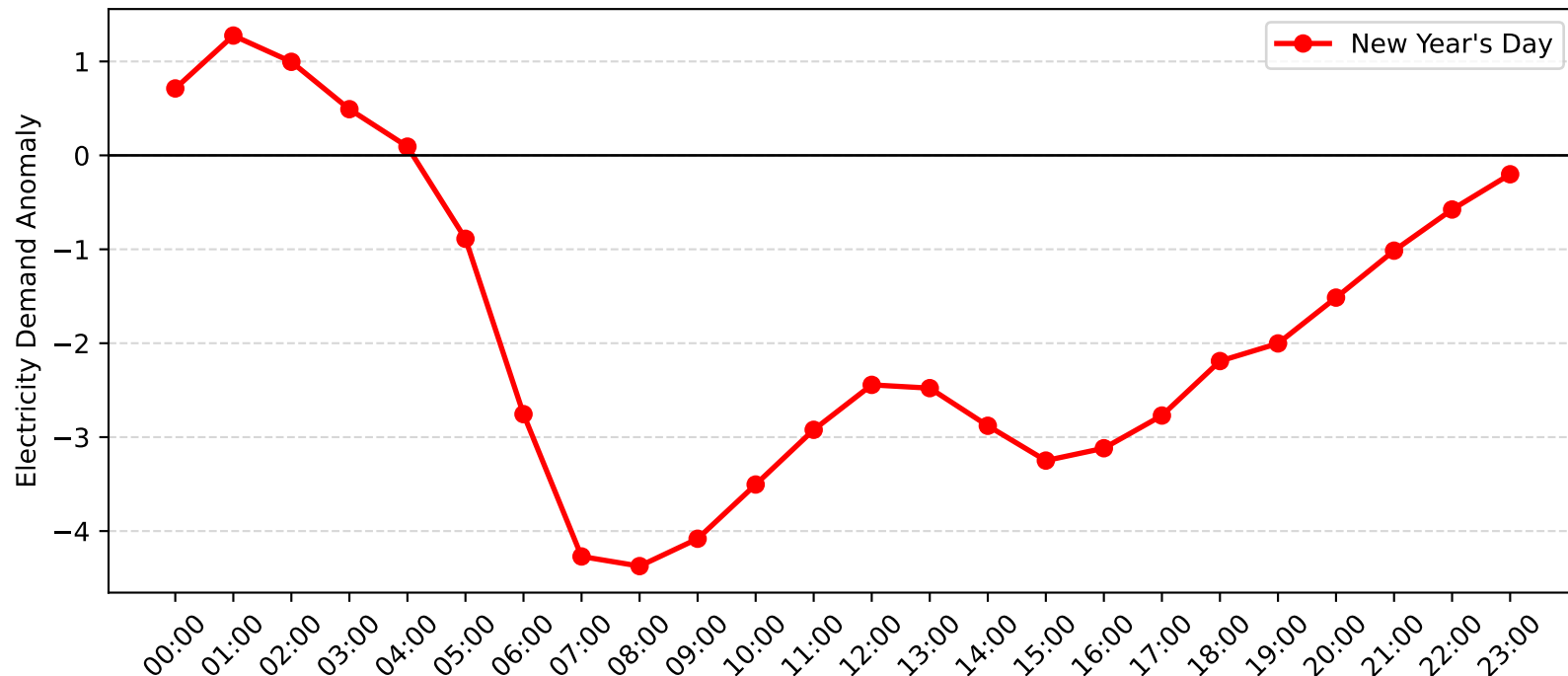
Five Dock Demand Anomaly: New Year's Day (2013-2014)
