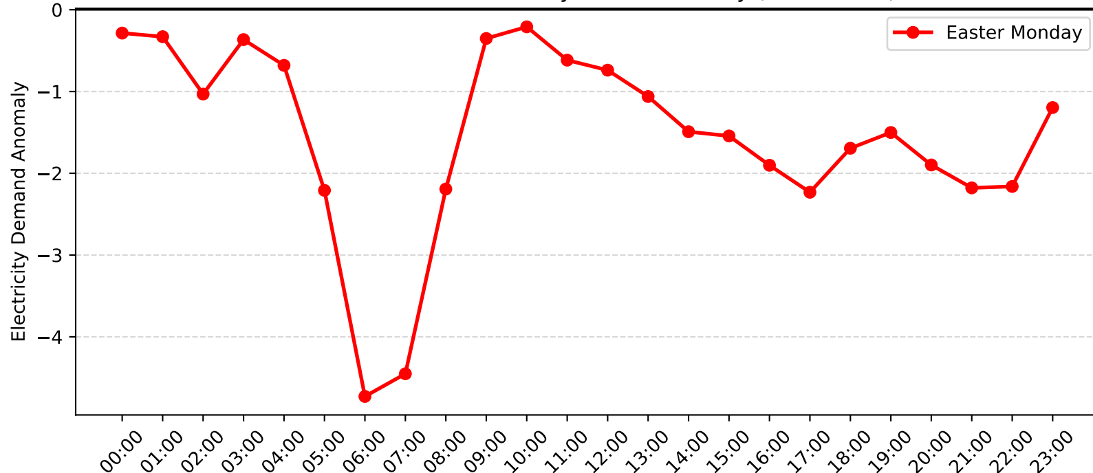
Cronulla Demand Anomaly: Easter Monday (2012-2013)
