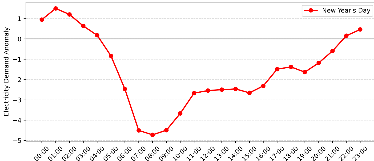
Five Dock Demand Anomaly: New Year's Day (2010-2011)
