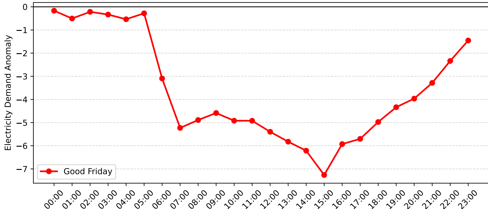
Chatswood Demand Anomaly: Good Friday (2016-2017)
