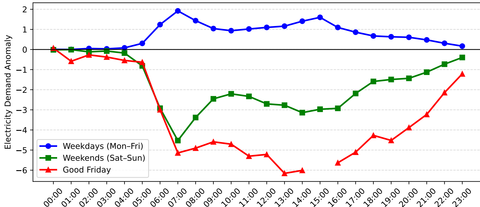
Chatswood Demand Anomaly: Good Friday vs Weekday/Weekend (2017-2018)
