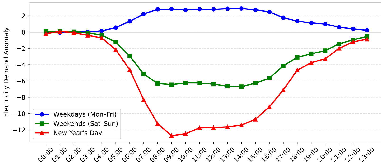
Brookvale Demand Anomaly: New Year's Day vs Weekday/Weekend (2011-2012)
