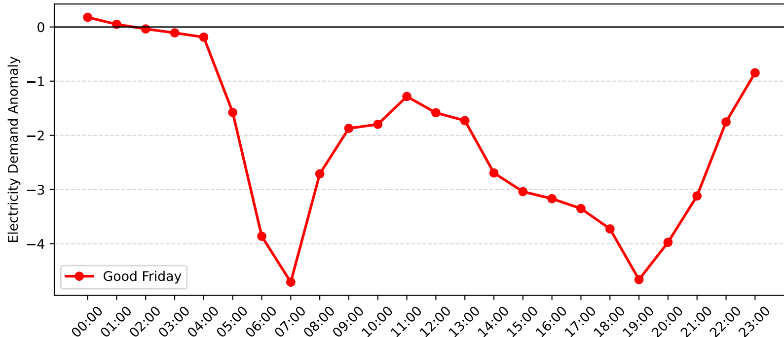
Dulwich Hill Demand Anomaly: Good Friday (2011-2012)
