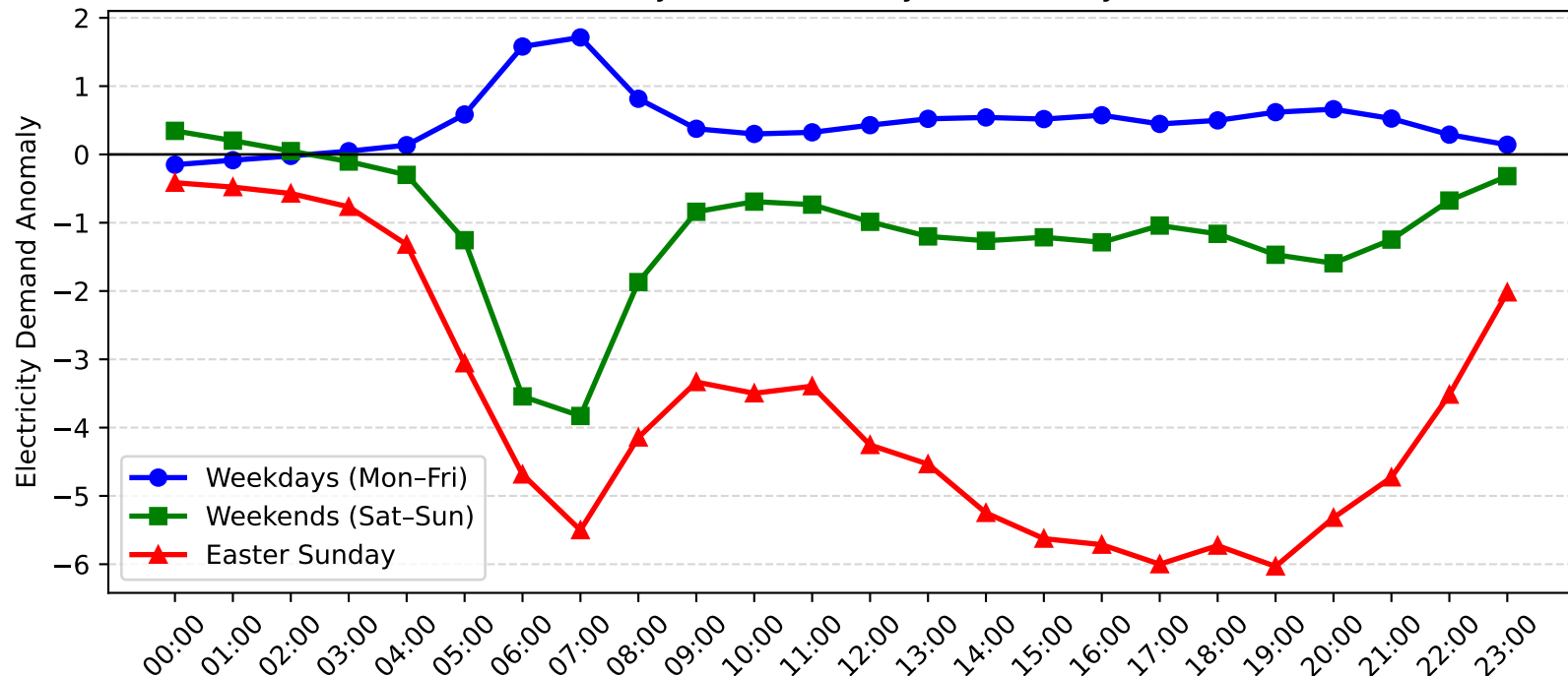
Dulwich Hill Demand Anomaly: Easter Sunday vs Weekday/Weekend (2010-2011)
