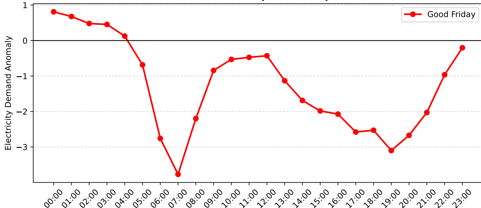
Dulwich Hill Demand Anomaly: Good Friday (2014-2015)
