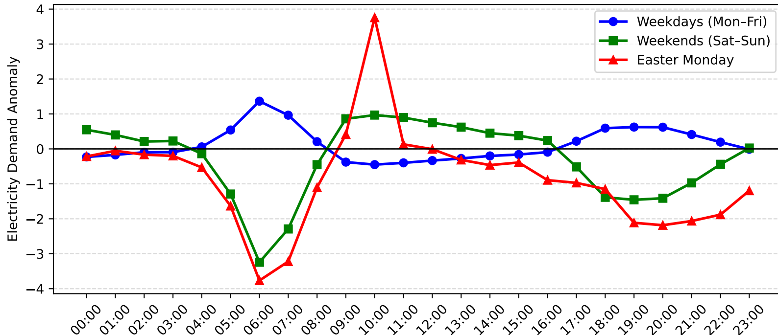
Cronulla Demand Anomaly: Easter Monday vs Weekday/Weekend (2006-2007)
