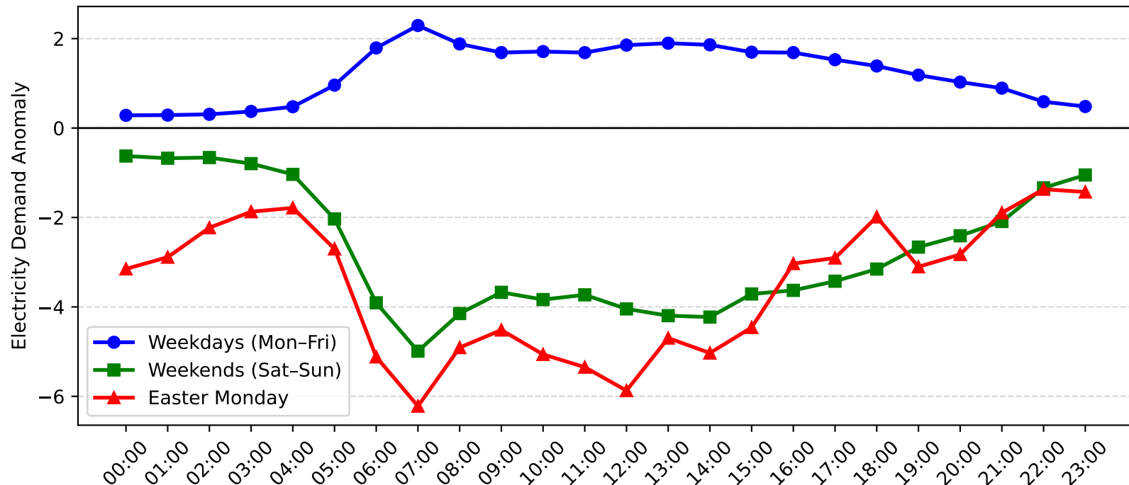
Matraverse Demand Anomaly: Easter Monday vs Weekday/Weekend (2009-2010)
