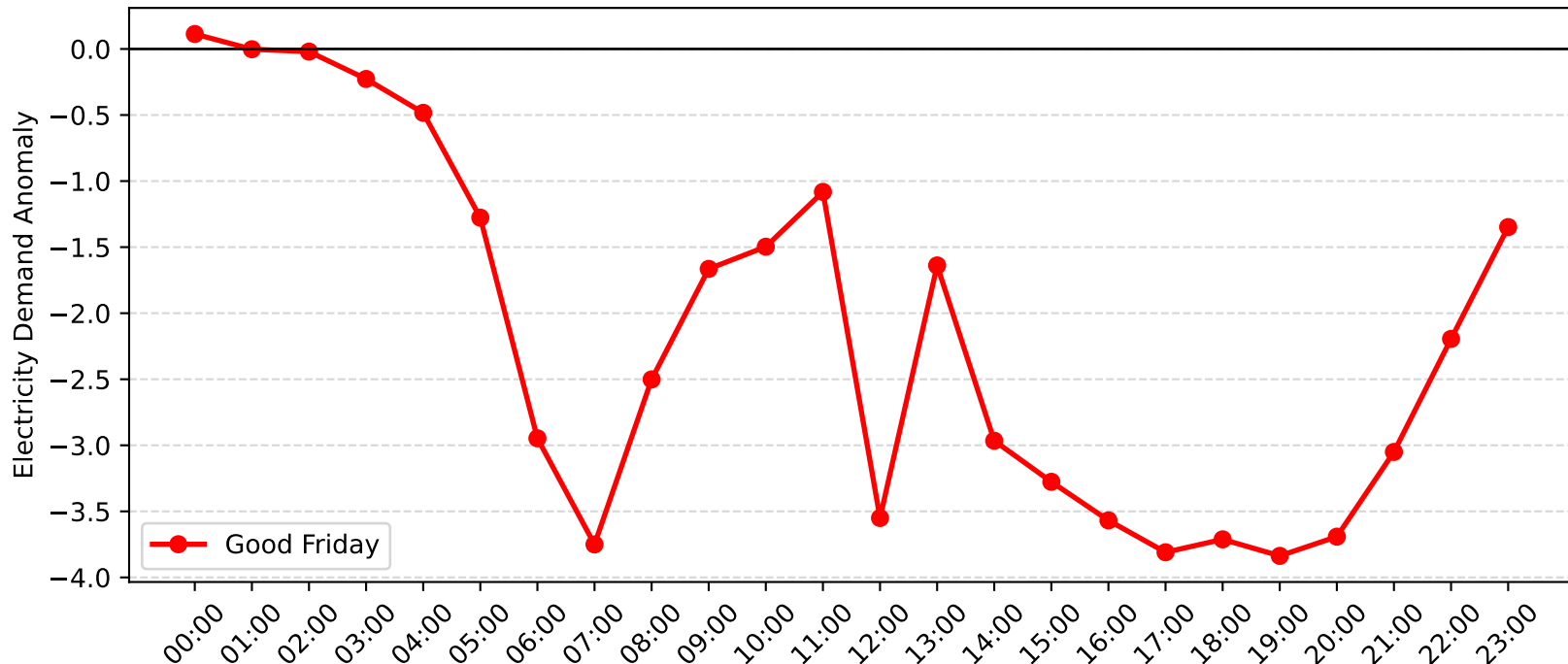
Dulwich Hill Demand Anomaly: Good Friday (2016-2017)
