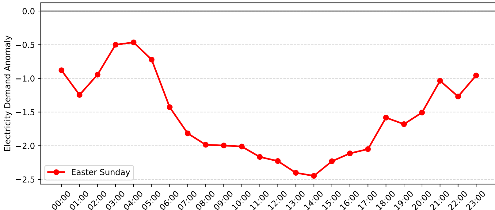
Gateshead Demand Anomaly: Easter Sunday (2010-2011)
