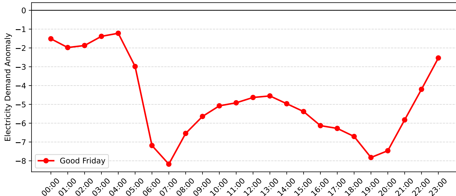
Pennant Hills Demand Anomaly: Good Friday (2011-2012)
