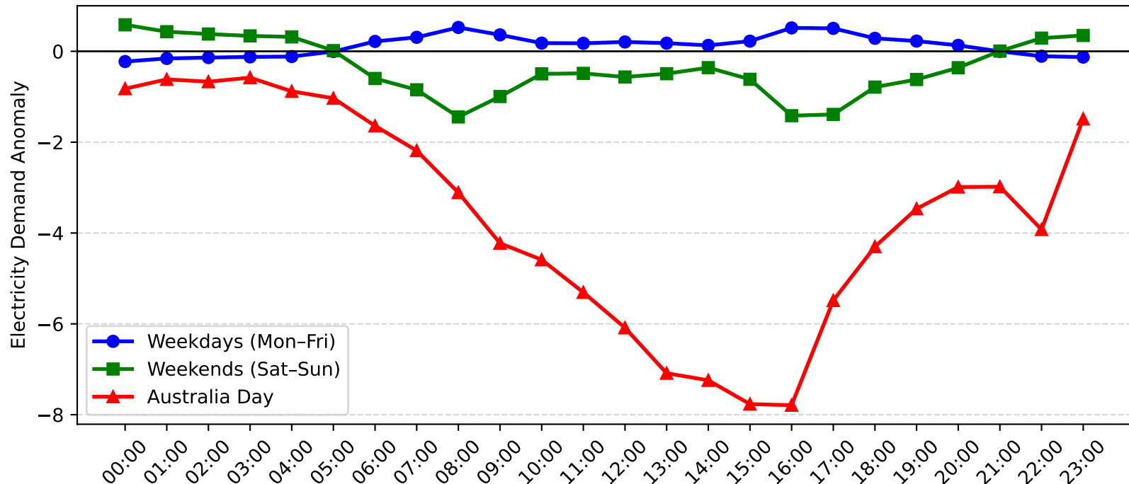
Erina Demand Anomaly: Australia Day vs Weekday/Weekend (2017-2018)
