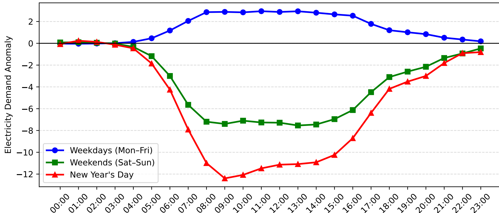
Brookvale Demand Anomaly: New Year's Day vs Weekday/Weekend (2010-2011)
