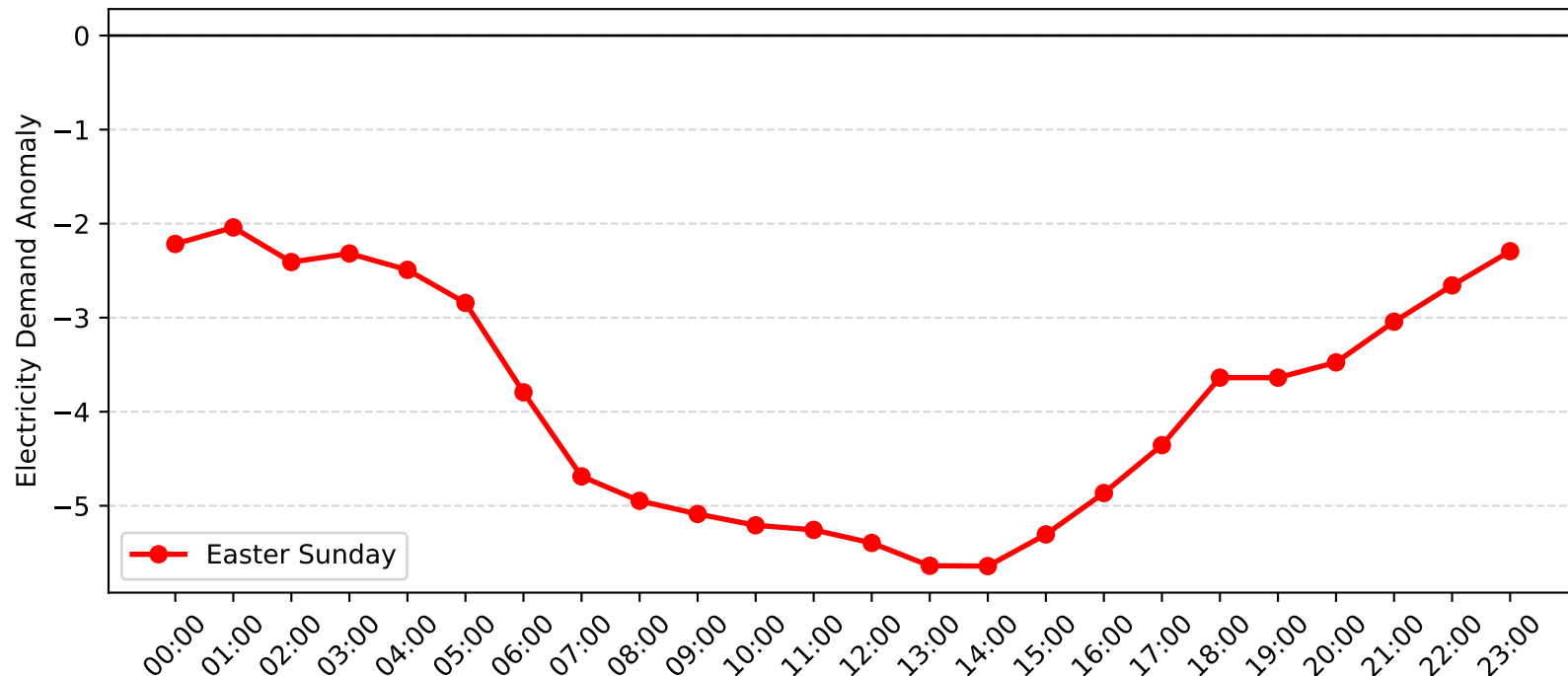
Caringbah Demand Anomaly: Easter Sunday (2014-2015)
