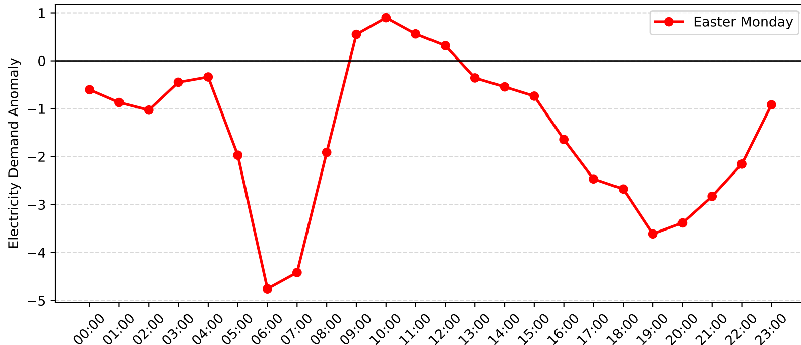
Cronulla Demand Anomaly: Easter Monday (2011-2012)
