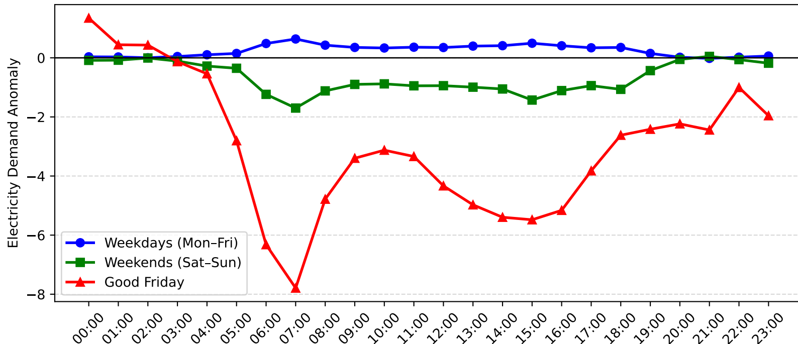
Dulwich Hill Demand Anomaly: Good Friday vs Weekday/Weekend (2004-2005)
