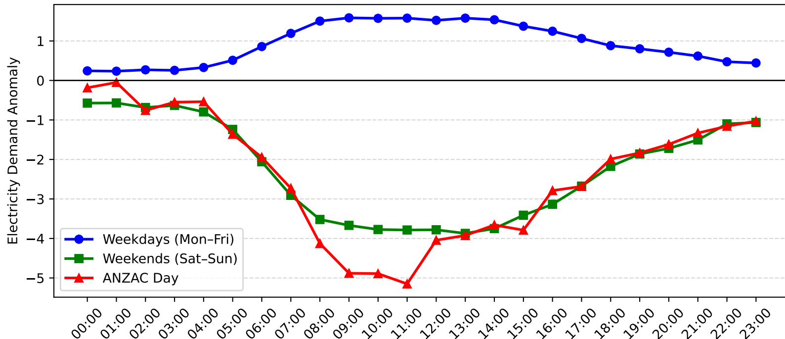
Green Square Demand Anomaly: ANZAC Day vs Weekday/Weekend (2008-2009)
