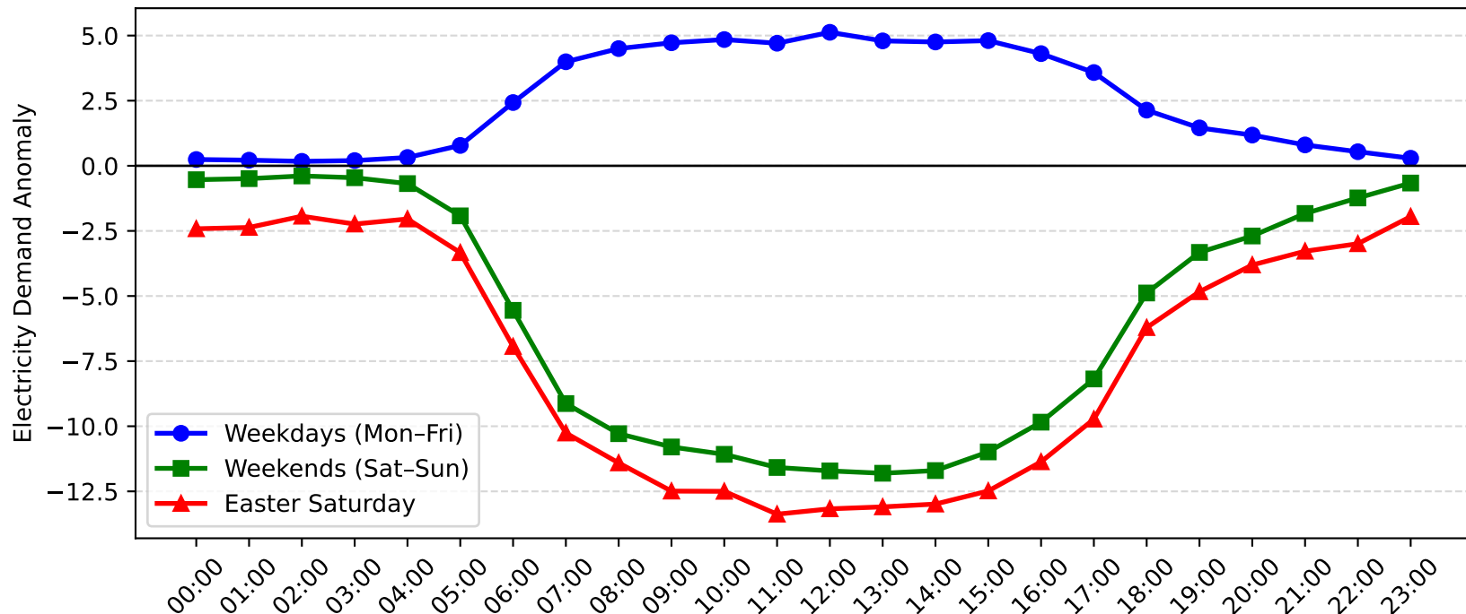
Macquarie Park Demand Anomaly: Easter Saturday vs Weekday/Weekend (2017-2018)
