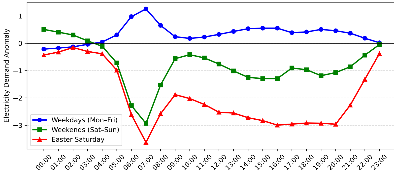
Five Dock Demand Anomaly: Easter Saturday vs Weekday/Weekend (2012-2013)
