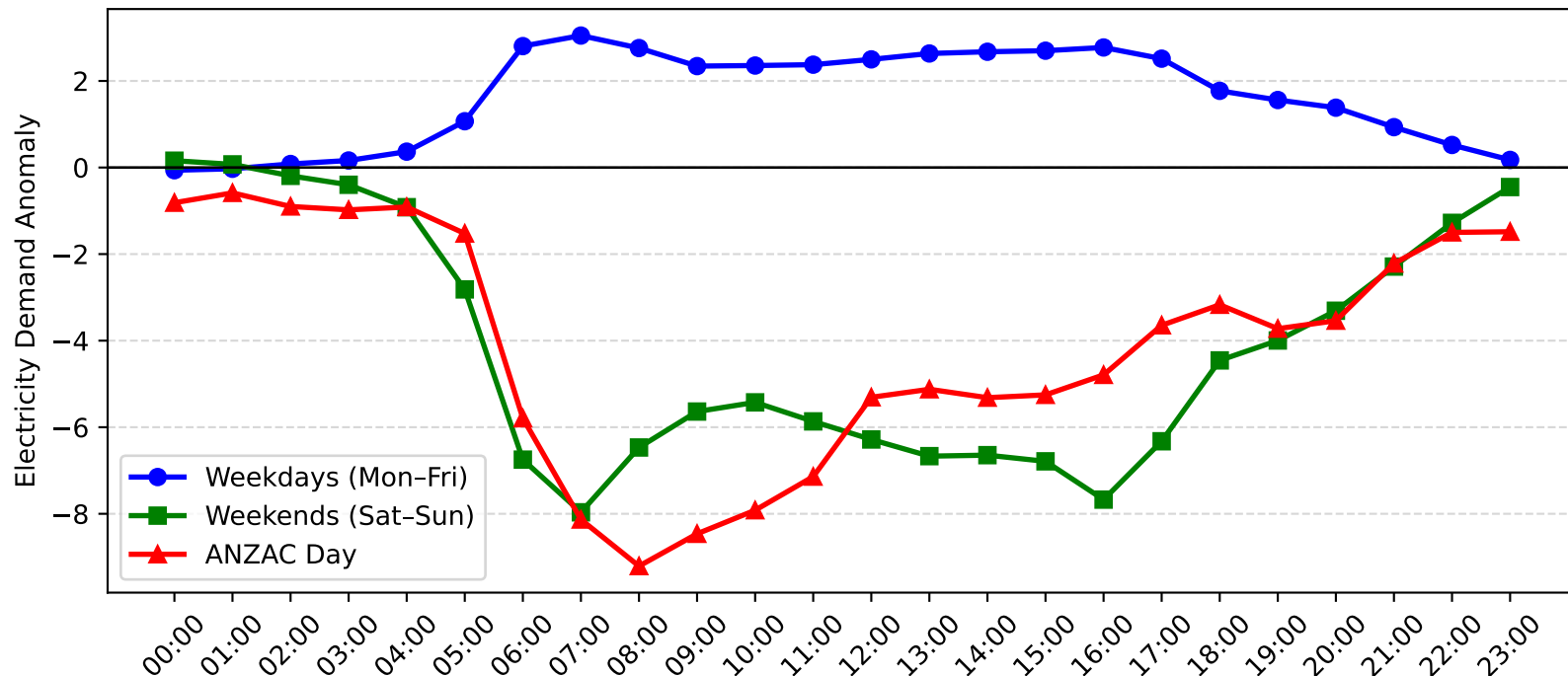
Epping Demand Anomaly: ANZAC Day vs Weekday/Weekend (2005-2006)
