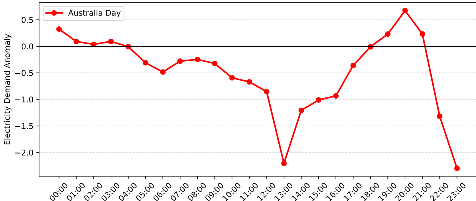
Muswellbrook Demand Anomaly: Australia Day (2007-2008)
