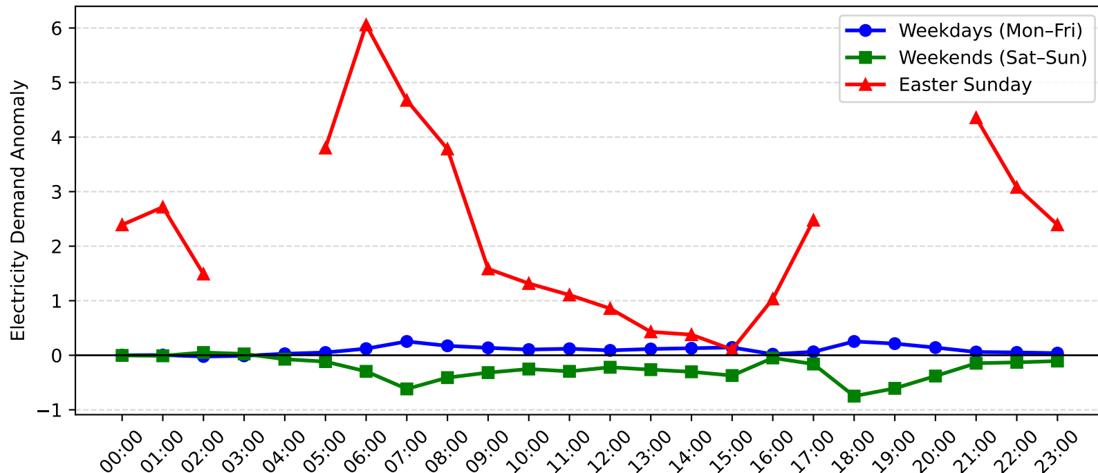
Berowra Demand Anomaly: Easter Sunday vs Weekday/Weekend (2004-2005)
