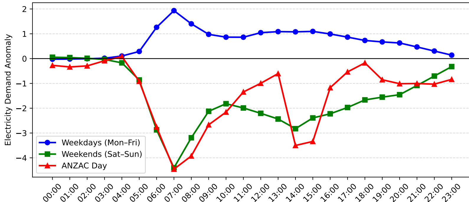
Chatswood Demand Anomaly: ANZAC Day vs Weekday/Weekend (2016-2017)
