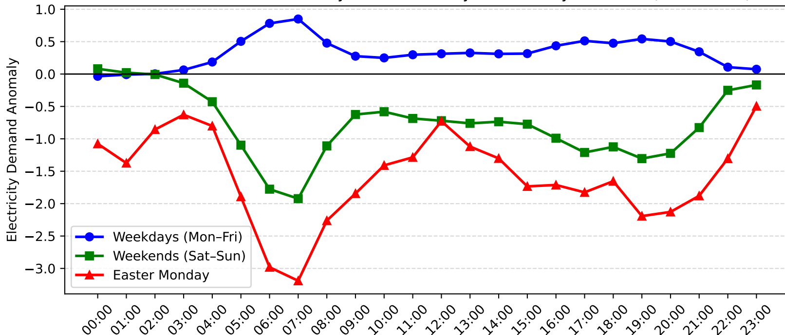
Charmhaven Demand Anomaly: Easter Monday vs Weekday/Weekend (2010-2011)
