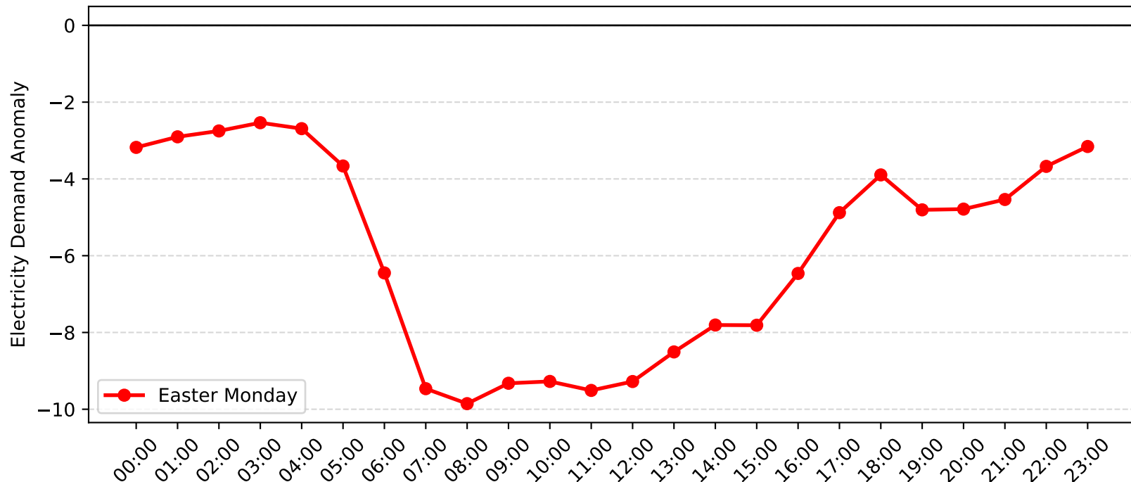
Marrickville Demand Anomaly: Easter Monday (2014-2015)
