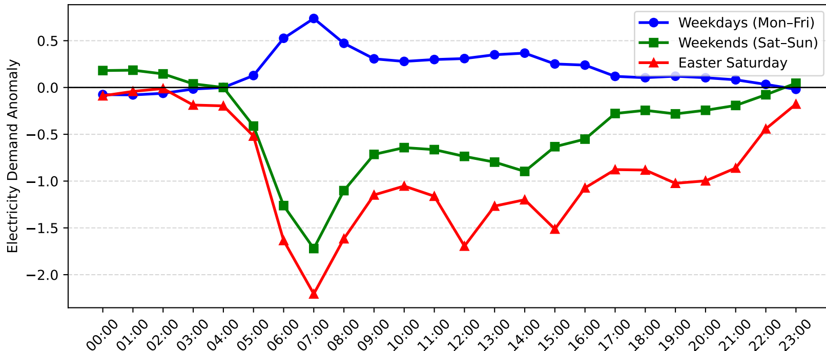
Arncliffe Demand Anomaly: Easter Saturday vs Weekday/Weekend (2014-2015)
