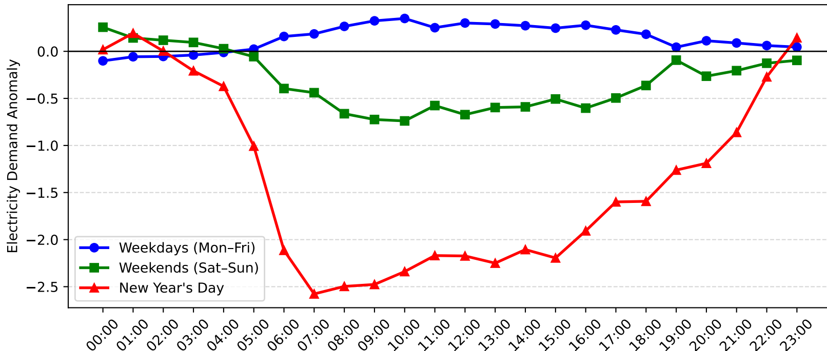
Rockdale Demand Anomaly: New Year's Day vs Weekday/Weekend (2004-2005)
