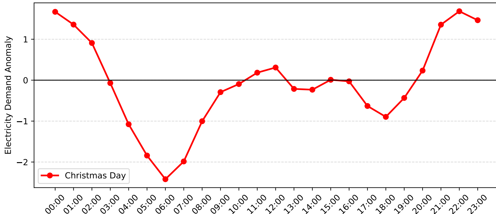
Revesby Demand Anomaly: Christmas Day (2010-2011)
