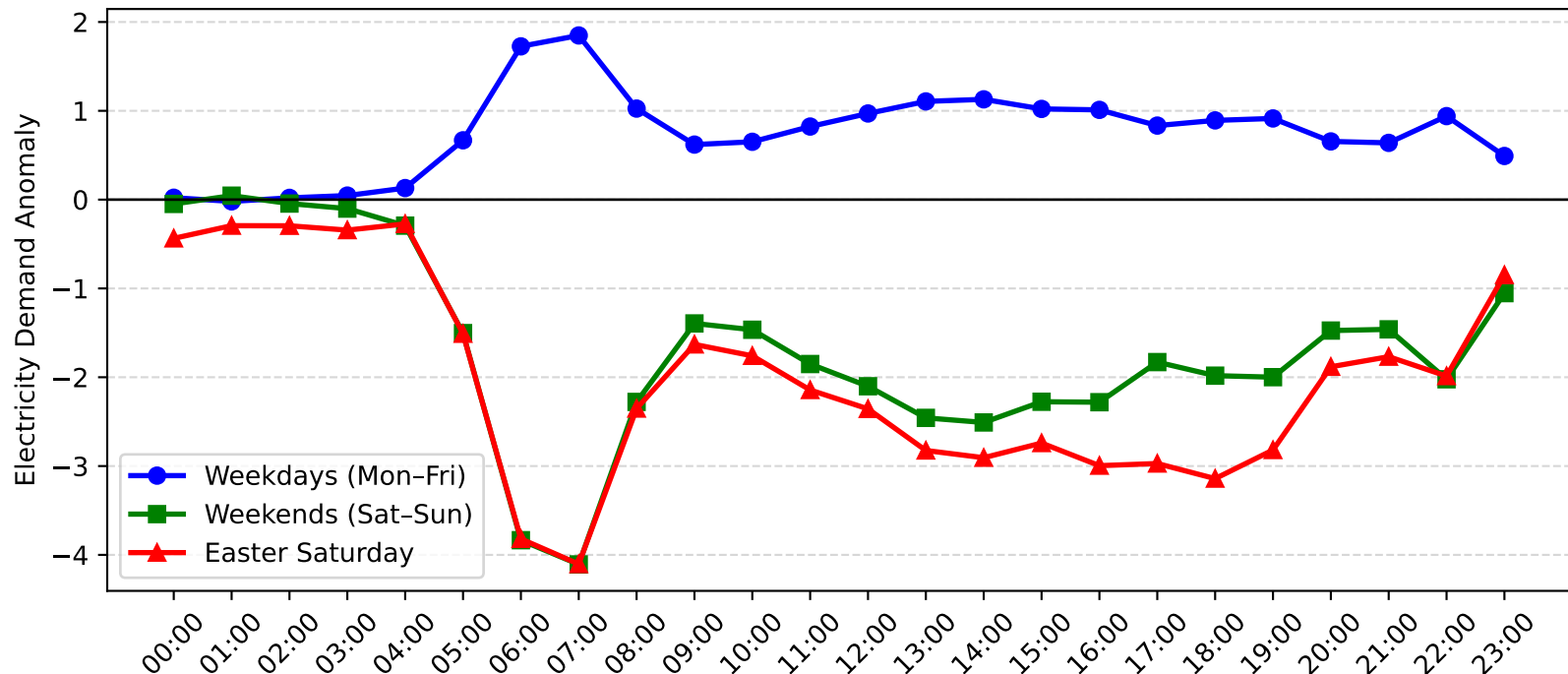
Dee Why West Demand Anomaly: Easter Saturday vs Weekday/Weekend (2008-2009)
