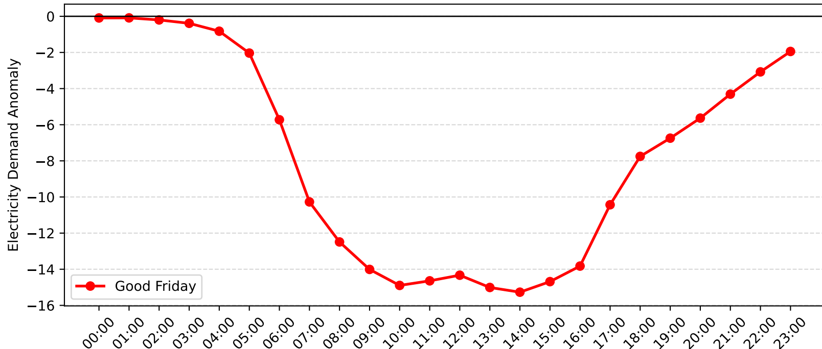
Zetland Demand Anomaly: Good Friday (2006-2007)
