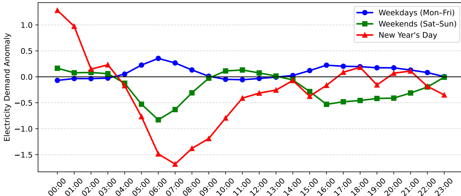
Woy Woy Demand Anomaly: New Year's Day vs Weekday/Weekend (2012-2013)
