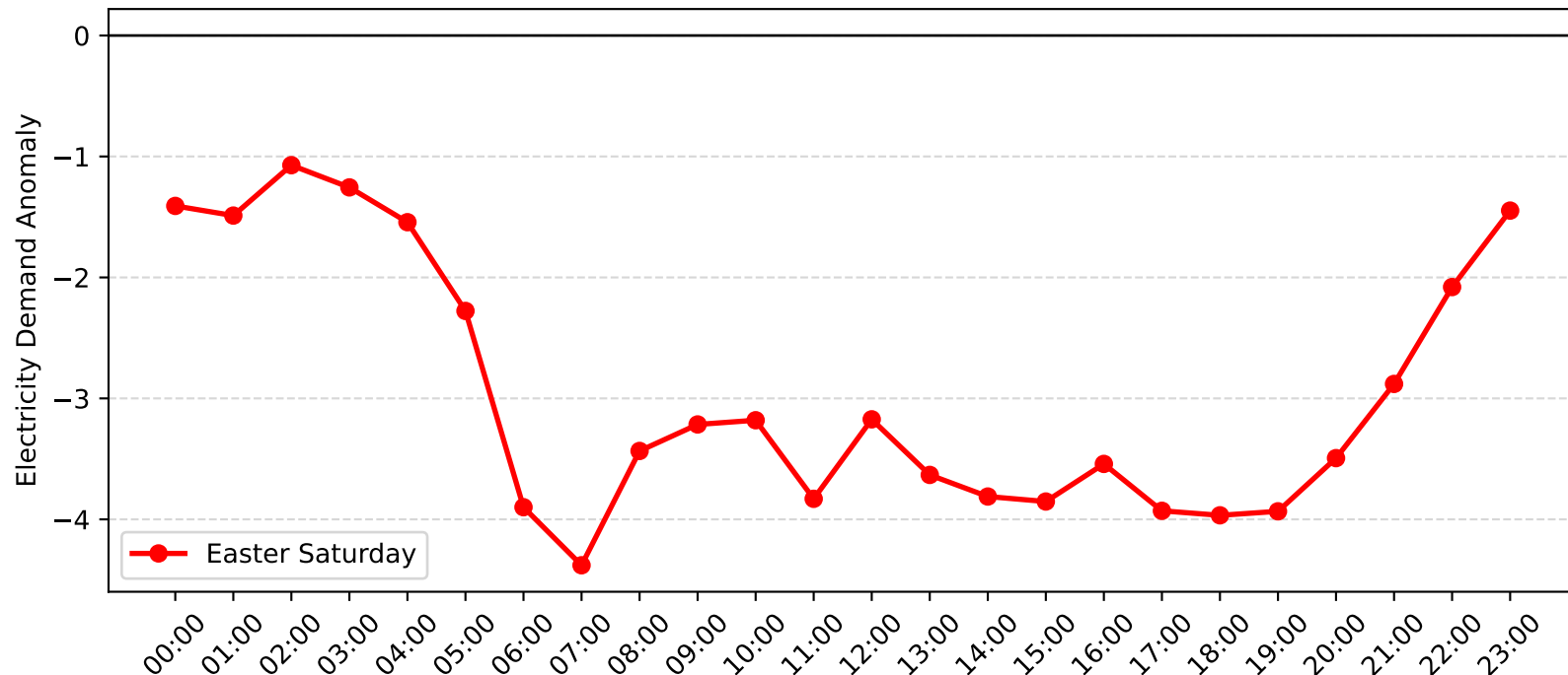
Maroubra Demand Anomaly: Easter Saturday (2013-2014)
