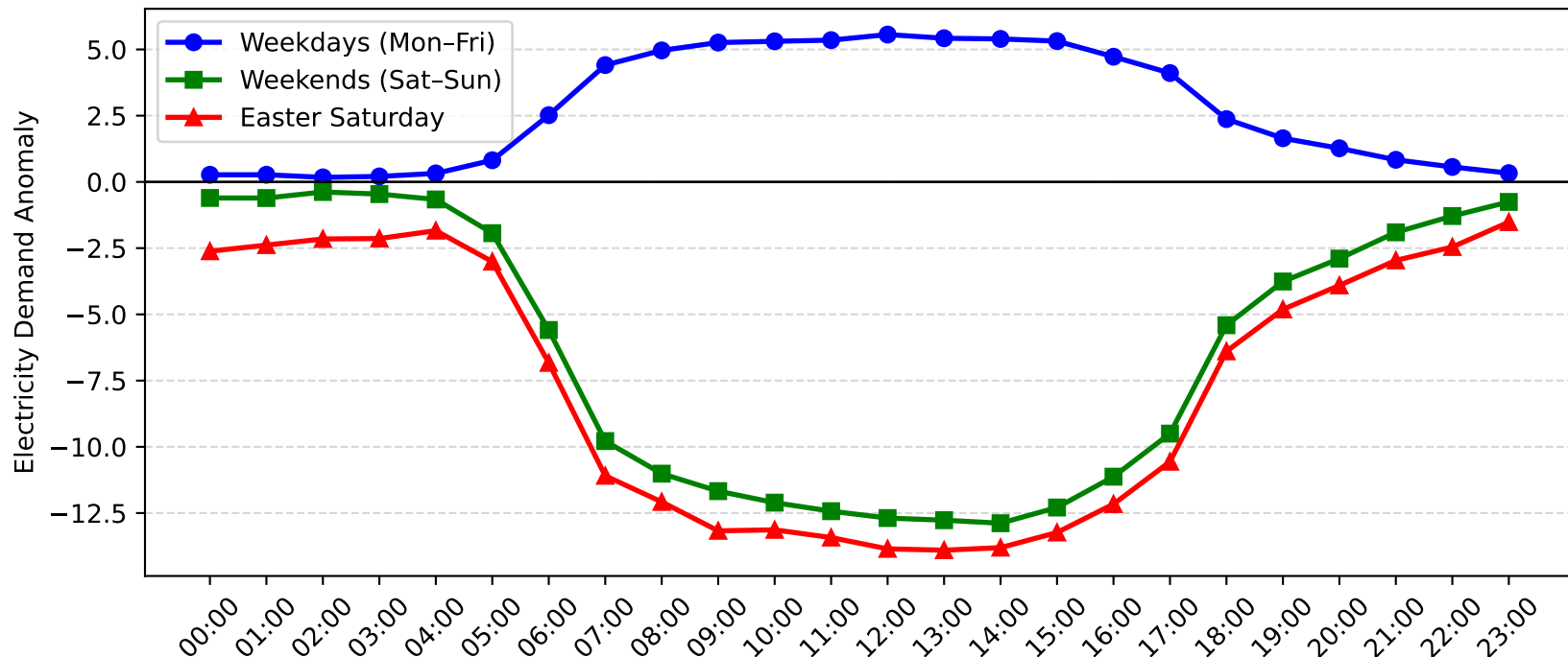
Macquarie Park Demand Anomaly: Easter Saturday vs Weekday/Weekend (2016-2017)
