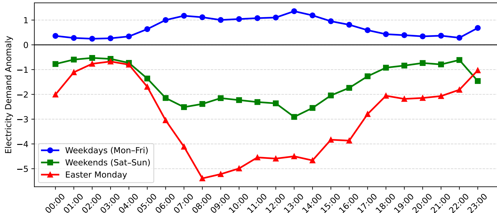
Rutherford Demand Anomaly: Easter Monday vs Weekday/Weekend (2017-2018)
