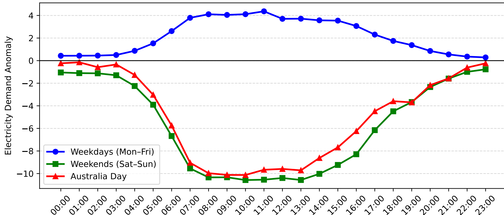
Homebush Bay Demand Anomaly: Australia Day vs Weekday/Weekend (2006-2007)
