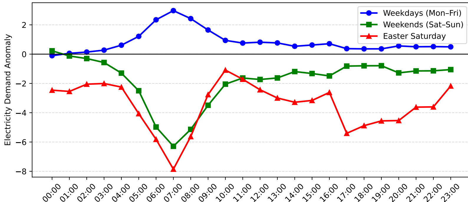
Meadowbank Demand Anomaly: Easter Saturday vs Weekday/Weekend (2009-2010)
