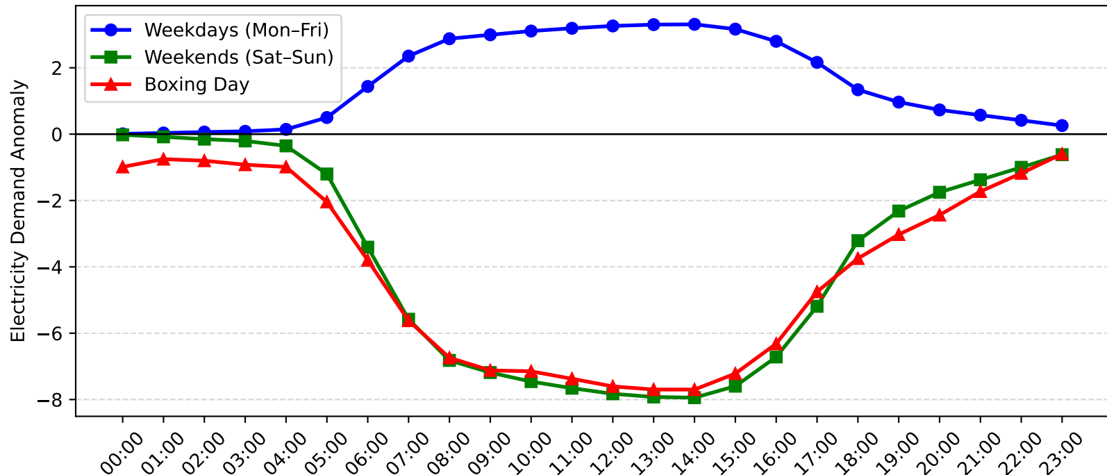
Mascot Demand Anomaly: Boxing Day vs Weekday/Weekend (2015-2016)
