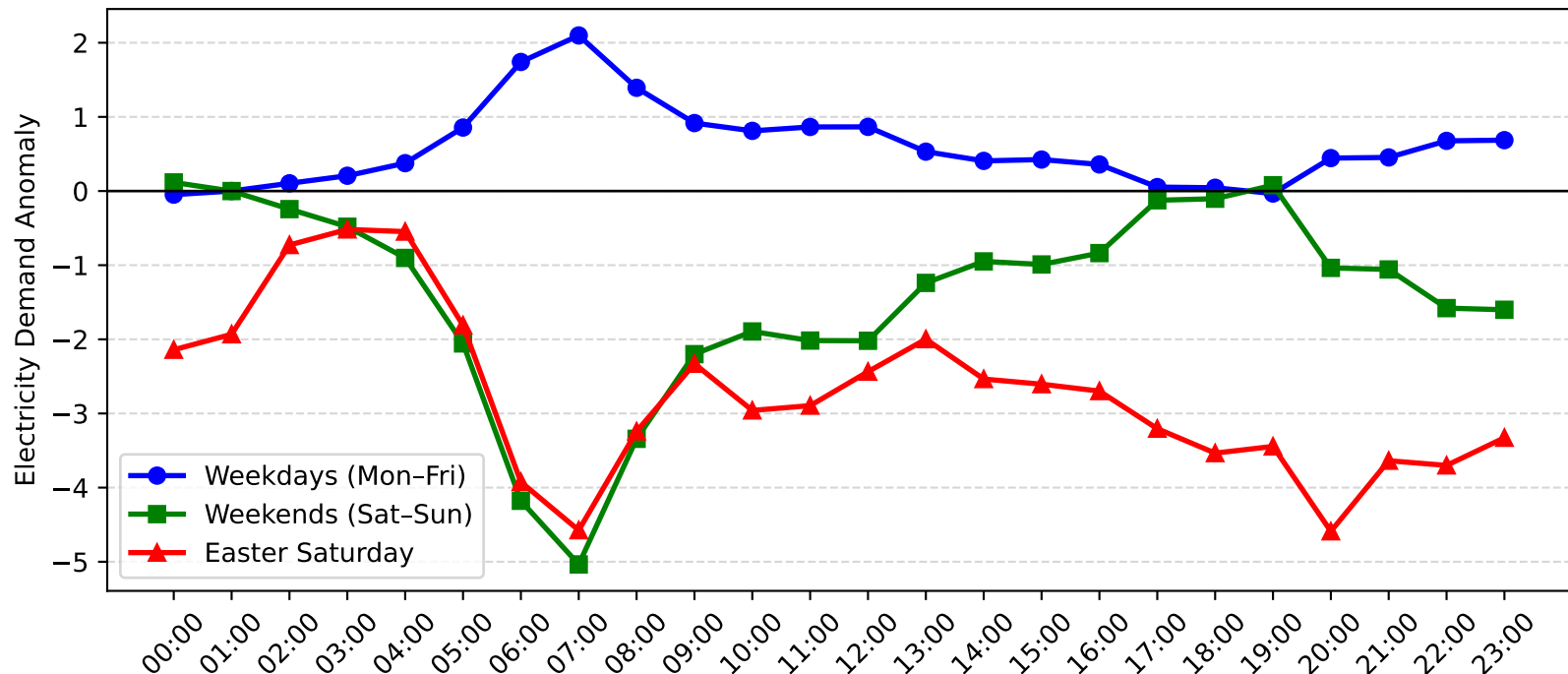
Meadowbank Demand Anomaly: Easter Saturday vs Weekday/Weekend (2012-2013)
