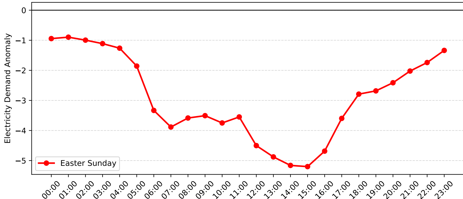
Bass Hill Demand Anomaly: Easter Sunday (2005-2006)
