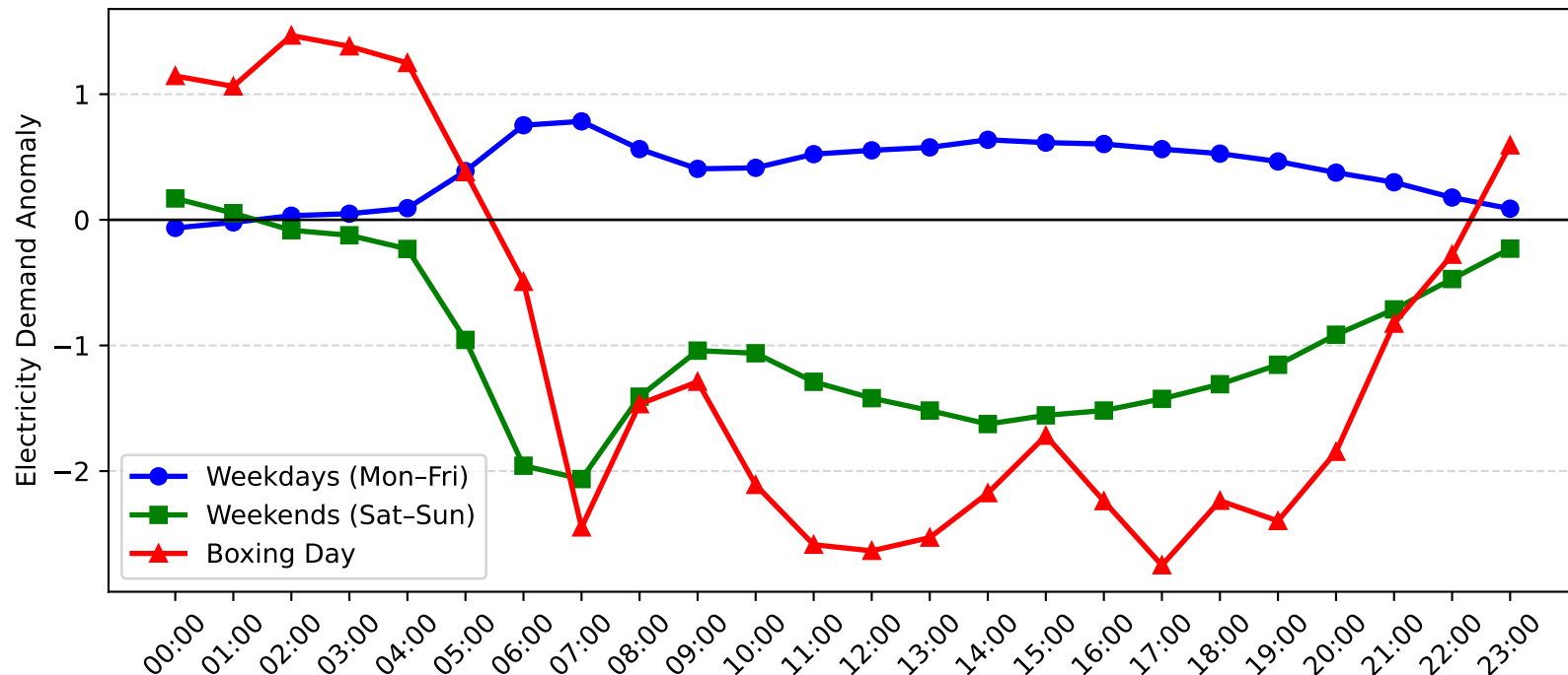
Dee Why West Demand Anomaly: Boxing Day vs Weekday/Weekend (2014-2015)
