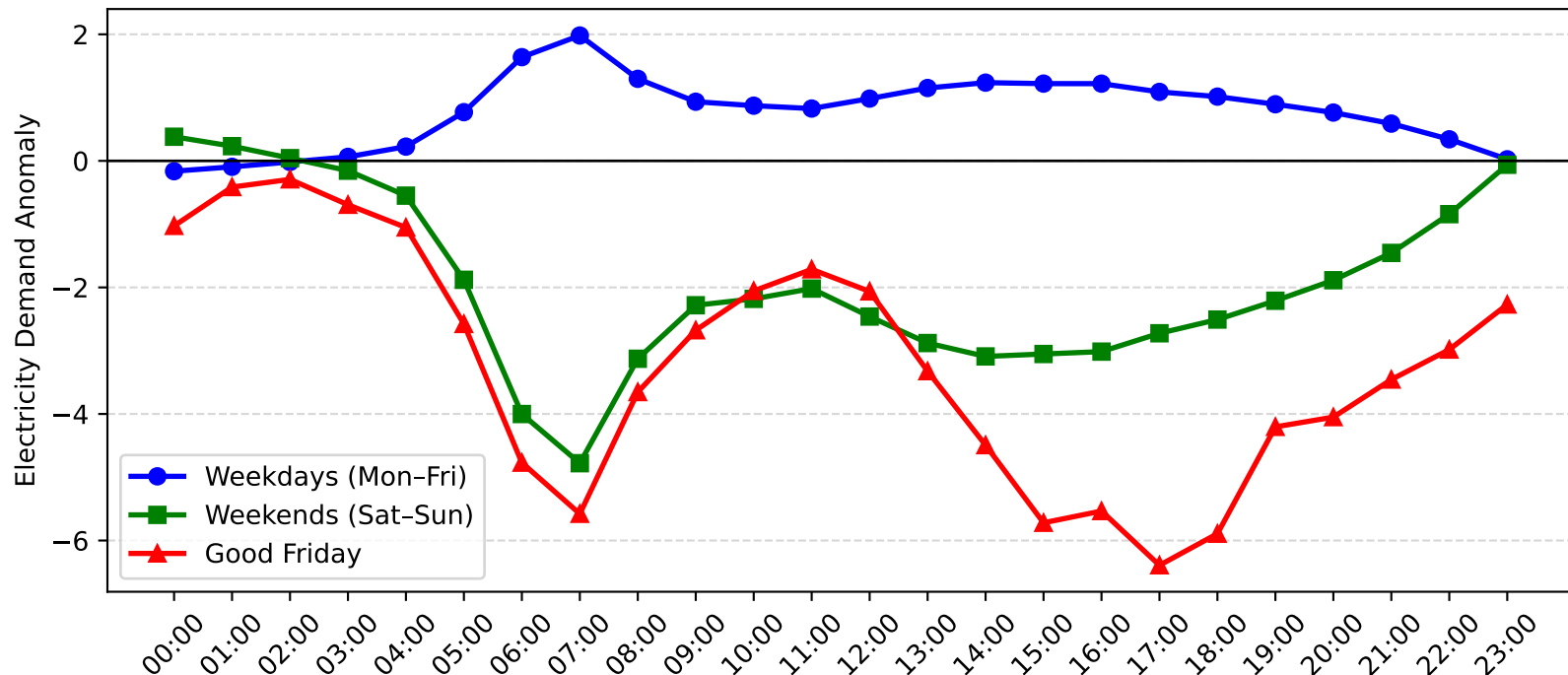
Campsie Demand Anomaly: Good Friday vs Weekday/Weekend (2015-2016)
