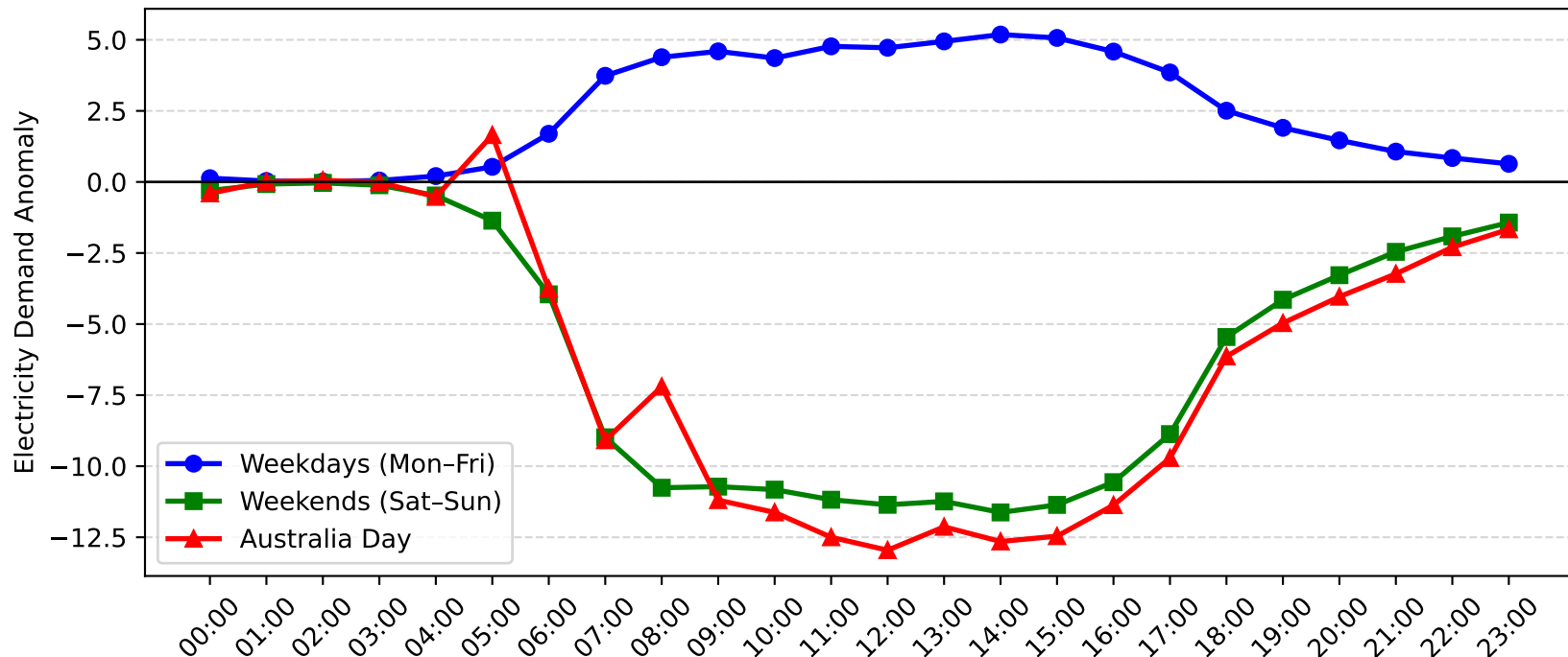
Gore Hill Demand Anomaly: Australia Day vs Weekday/Weekend (2013-2014)
