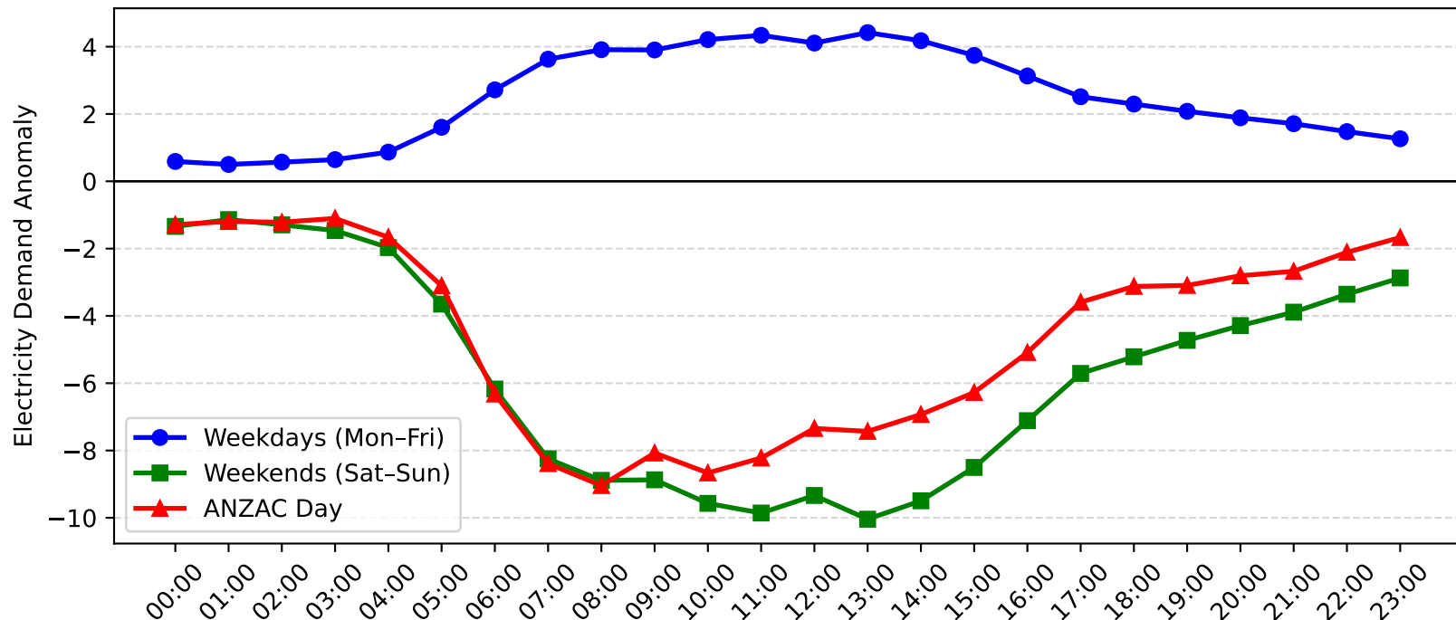
Milperra Demand Anomaly: ANZAC Day vs Weekday/Weekend (2017-2018)
