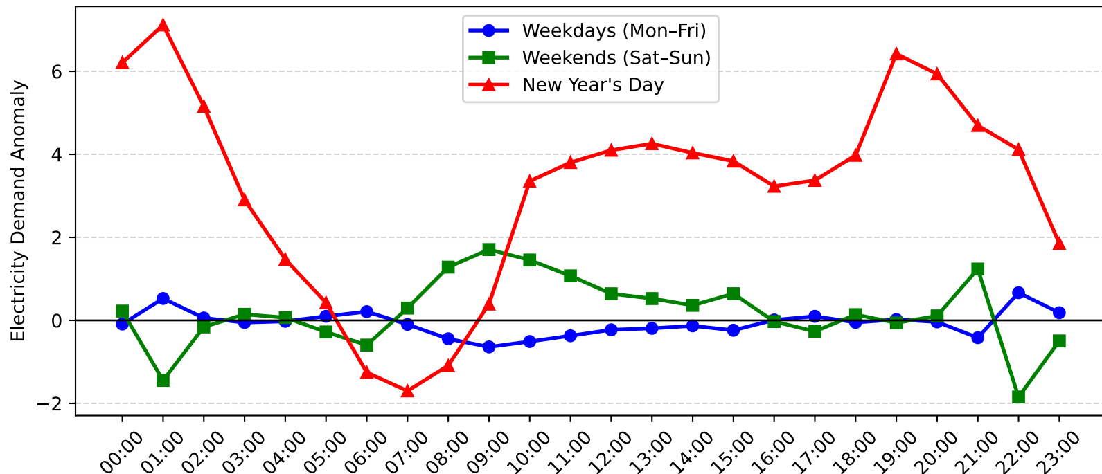
Nelson Bay Demand Anomaly: New Year's Day vs Weekday/Weekend (2008-2009)
