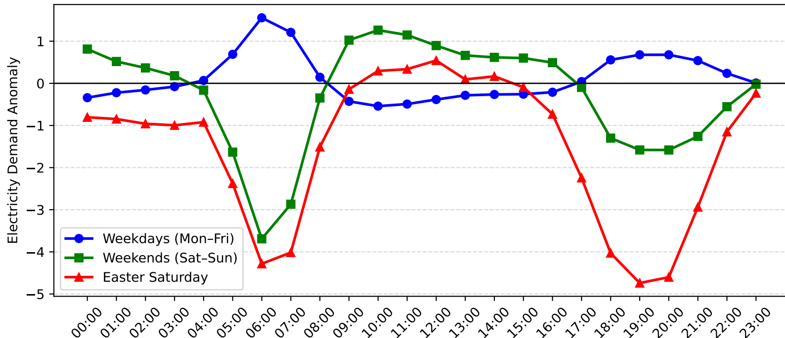
Cronulla Demand Anomaly: Easter Saturday vs Weekday/Weekend (2011-2012)
