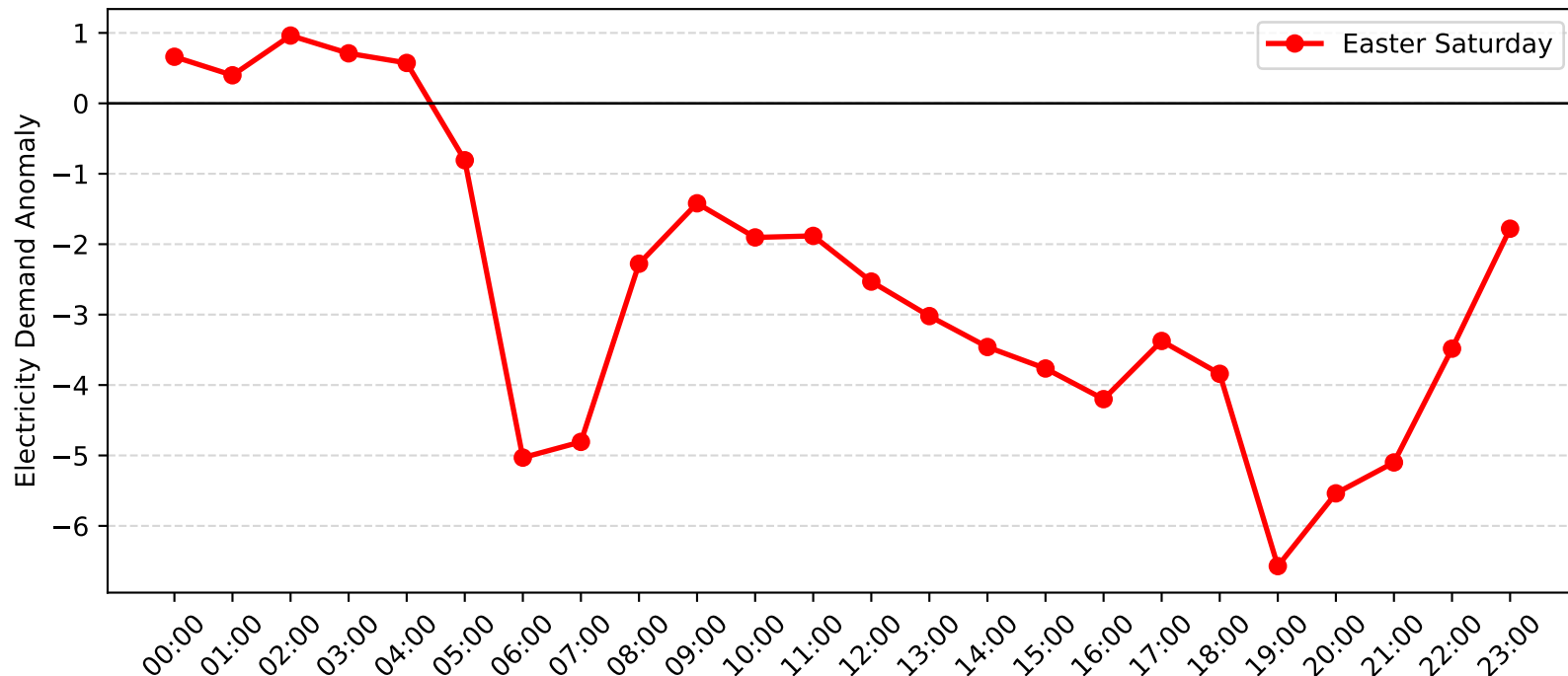
Pennant Hills Demand Anomaly: Easter Saturday (2009-2010)
