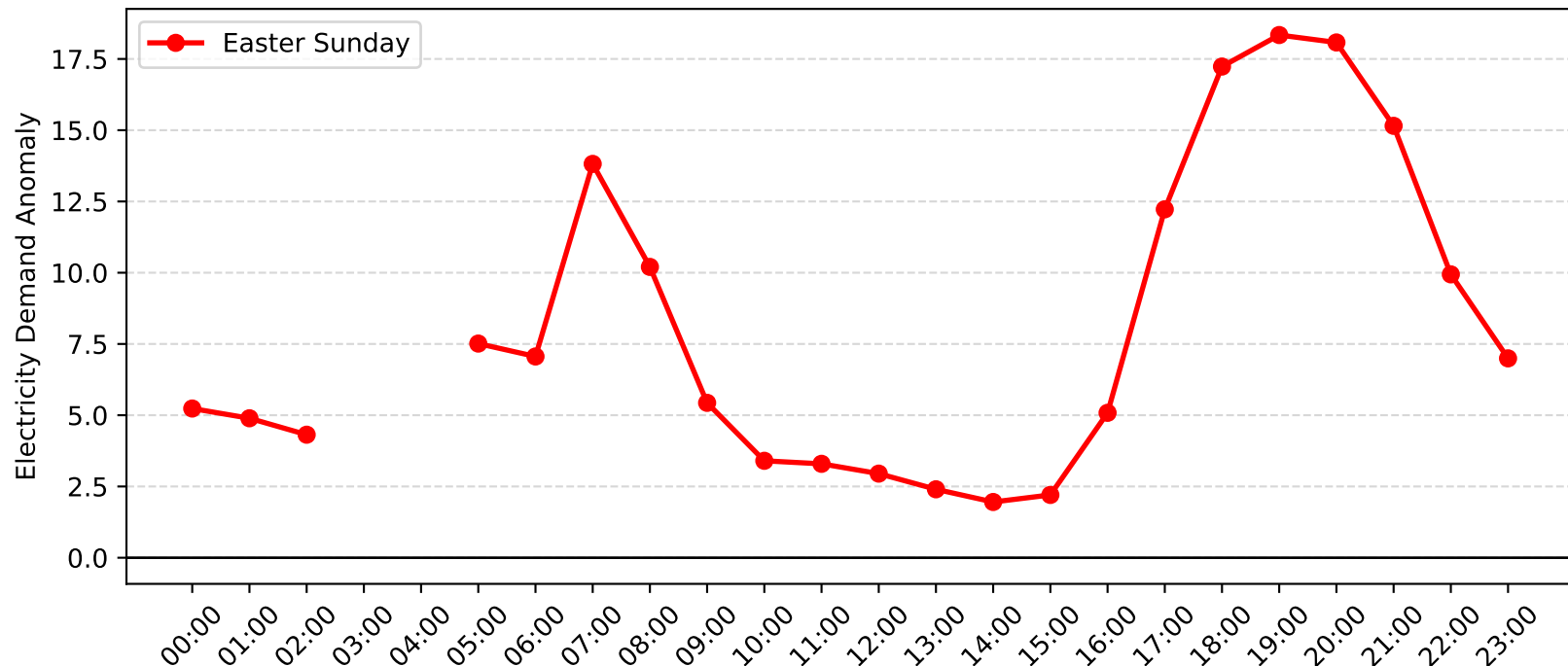
Mosman Demand Anomaly: Easter Sunday (2004-2005)
