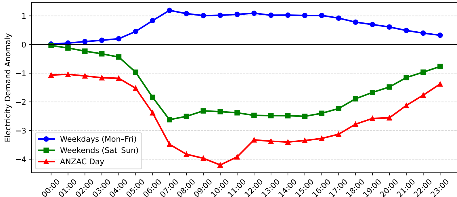
Lidcombe Demand Anomaly: ANZAC Day vs Weekday/Weekend (2010-2011)
