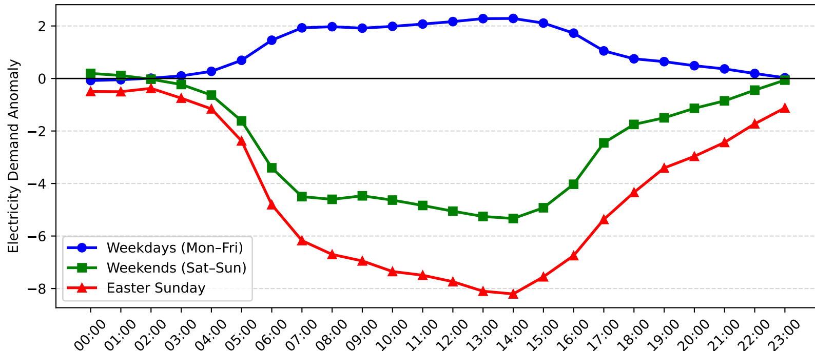
West Gosford Demand Anomaly: Easter Sunday vs Weekday/Weekend (2013-2014)
