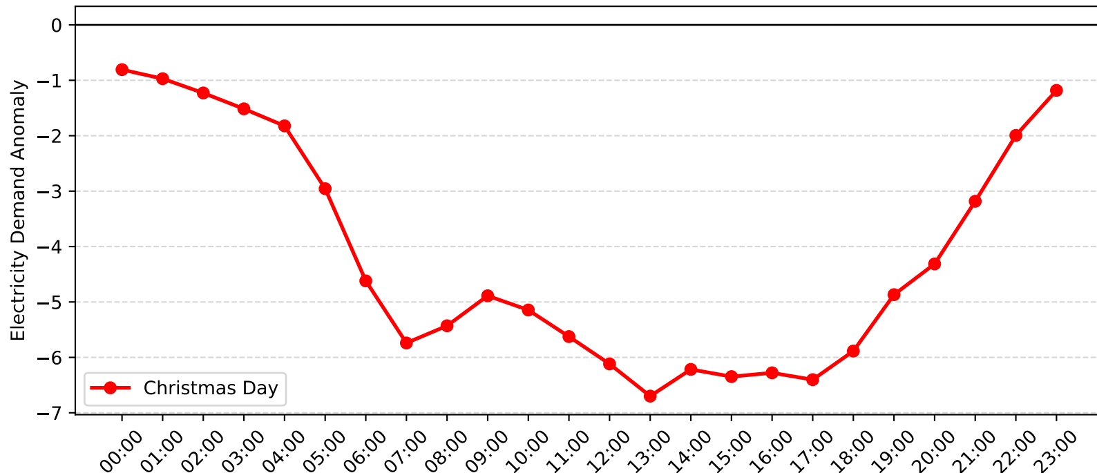
Dulwich Hill Demand Anomaly: Christmas Day (2009-2010)
