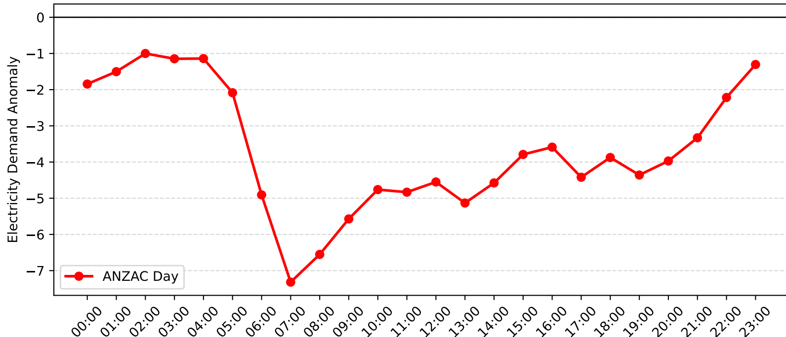
Chatswood Demand Anomaly: ANZAC Day (2010-2011)
