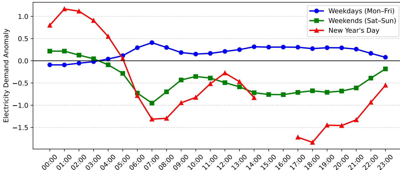
Blakehurst Demand Anomaly: New Year's Day vs Weekday/Weekend (2017-2018)
