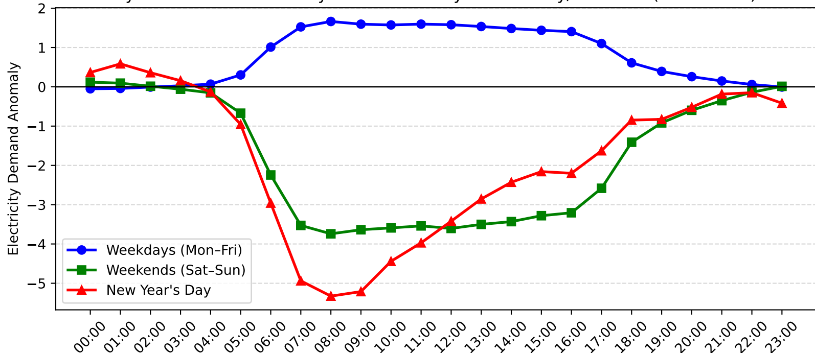
Pymble Demand Anomaly: New Year's Day vs Weekday/Weekend (2011-2012)
