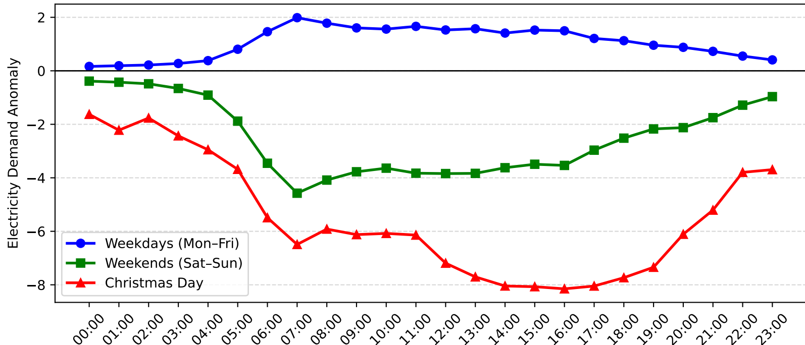
Matraverse Demand Anomaly: Christmas Day vs Weekday/Weekend (2005-2006)
