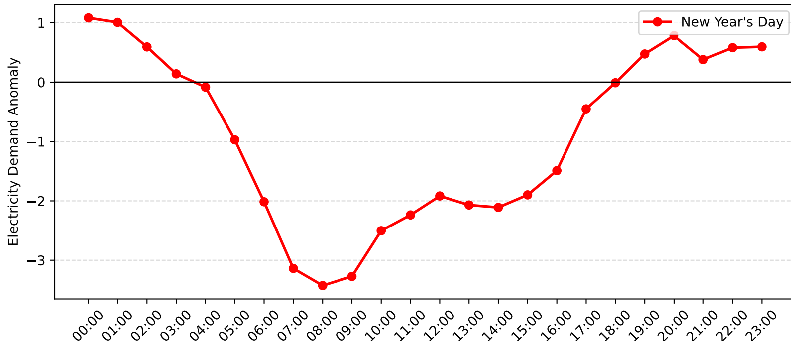
Rockdale Demand Anomaly: New Year's Day (2005-2006)
