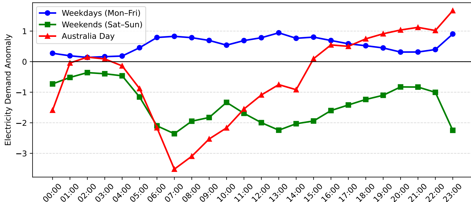
Rutherford Demand Anomaly: Australia Day vs Weekday/Weekend (2009-2010)
