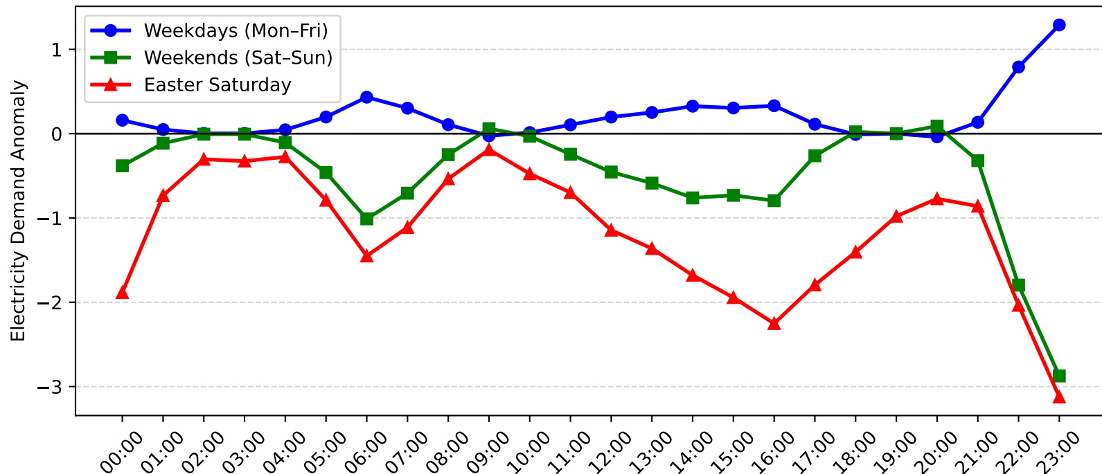
Muswellbrook Demand Anomaly: Easter Saturday vs Weekday/Weekend (2007-2008)
