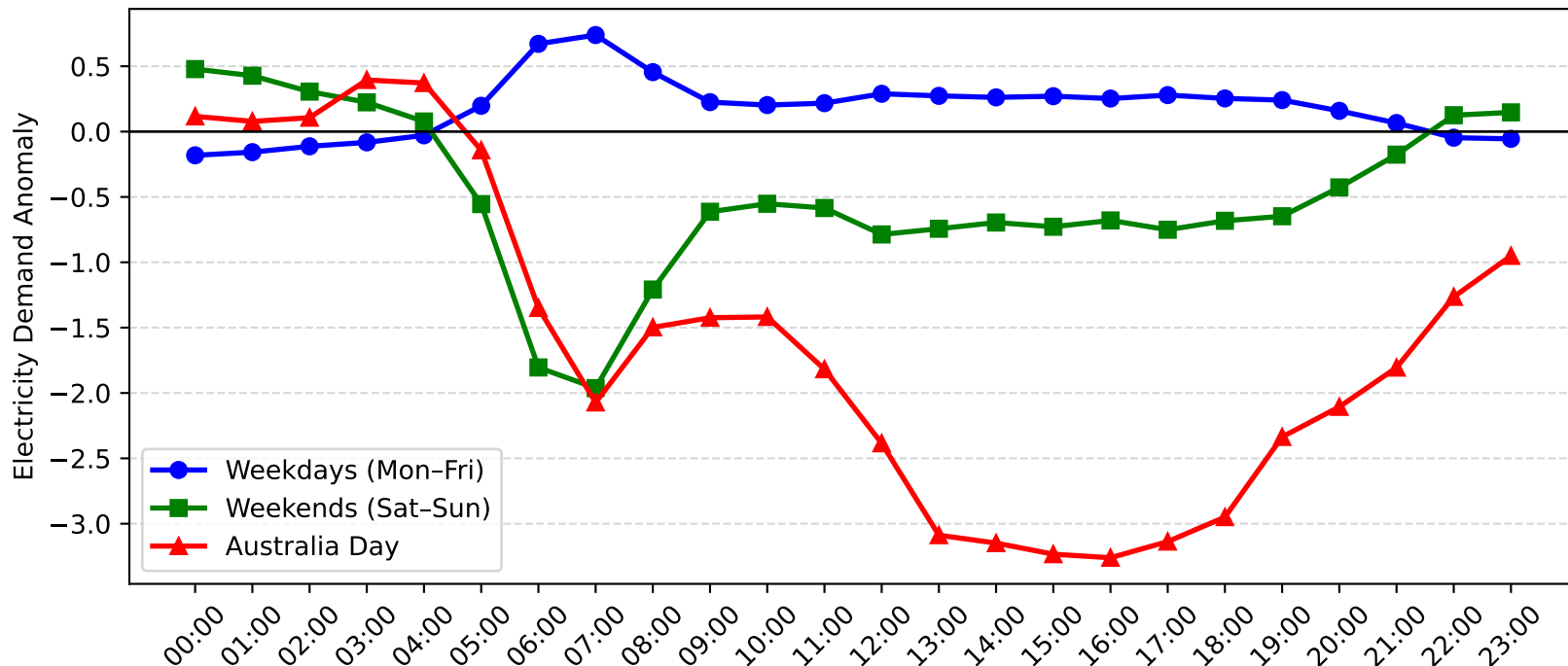
Dee Why West Demand Anomaly: Australia Day vs Weekday/Weekend (2016-2017)
