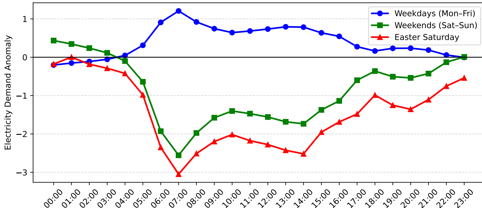
Arncliffe Demand Anomaly: Easter Saturday vs Weekday/Weekend (2009-2010)
