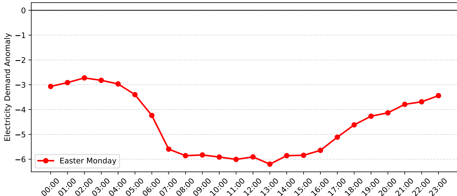
Leightonfield Demand Anomaly: Easter Monday (2016-2017)
