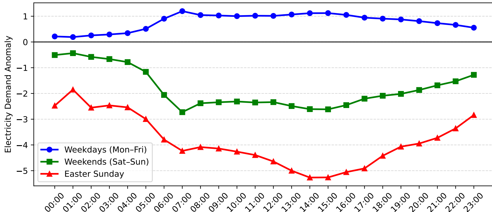
Bass Hill Demand Anomaly: Easter Sunday vs Weekday/Weekend (2015-2016)
