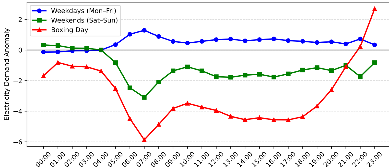
Dee Why West Demand Anomaly: Boxing Day vs Weekday/Weekend (2005-2006)
