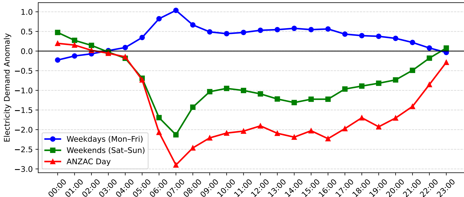
Rockdale Demand Anomaly: ANZAC Day vs Weekday/Weekend (2009-2010)
