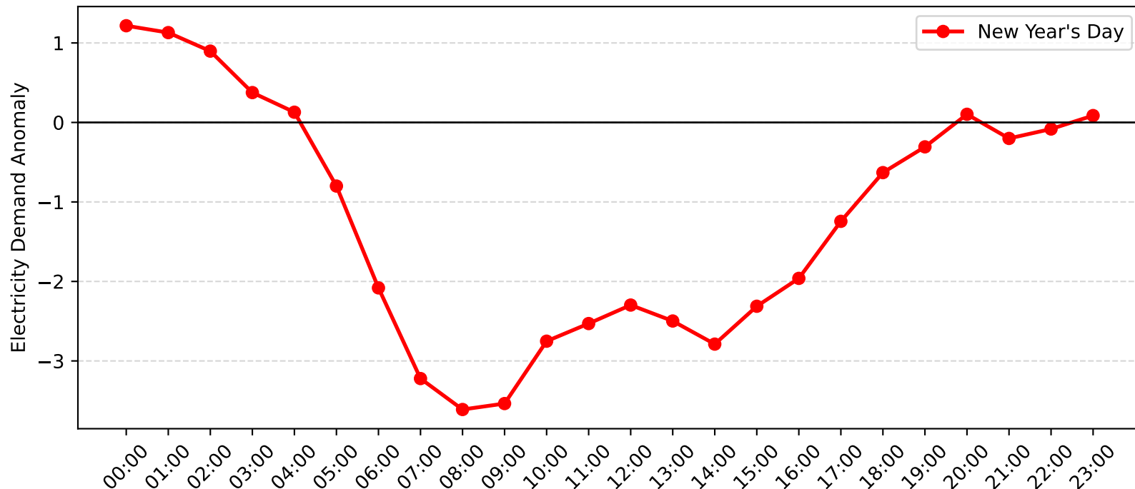
Rockdale Demand Anomaly: New Year's Day (2006-2007)
