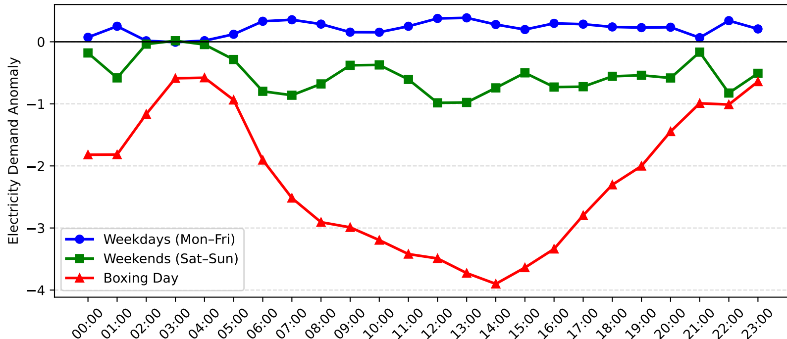
Gateshead Demand Anomaly: Boxing Day vs Weekday/Weekend (2005-2006)
