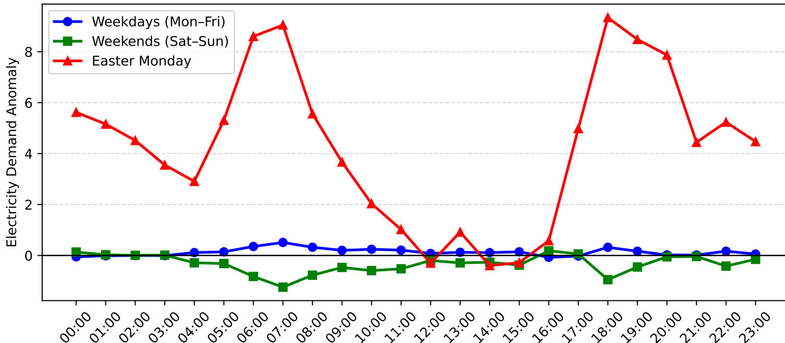
Revesby Demand Anomaly: Easter Monday vs Weekday/Weekend (2004-2005)
