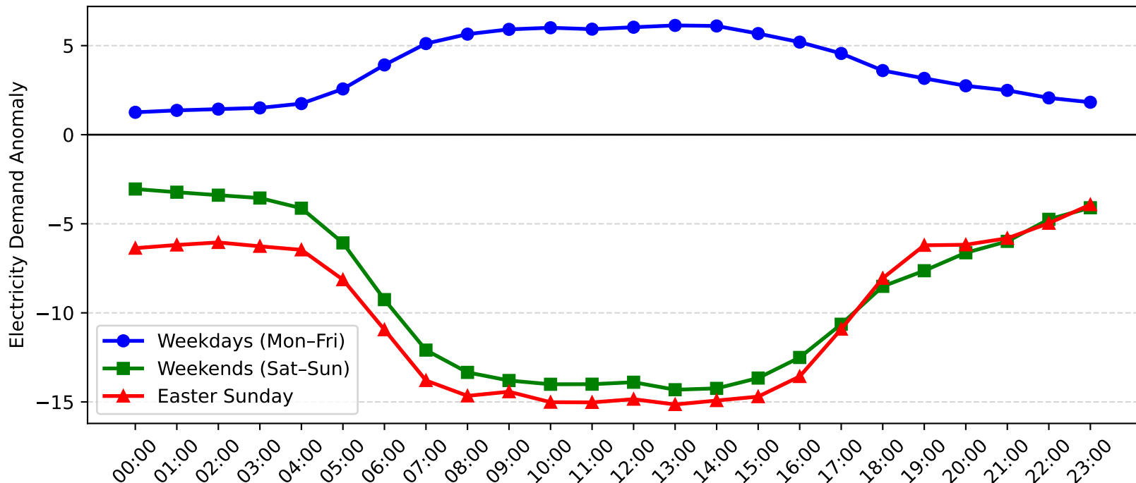
Flemington Demand Anomaly: Easter Sunday vs Weekday/Weekend (2007-2008)
