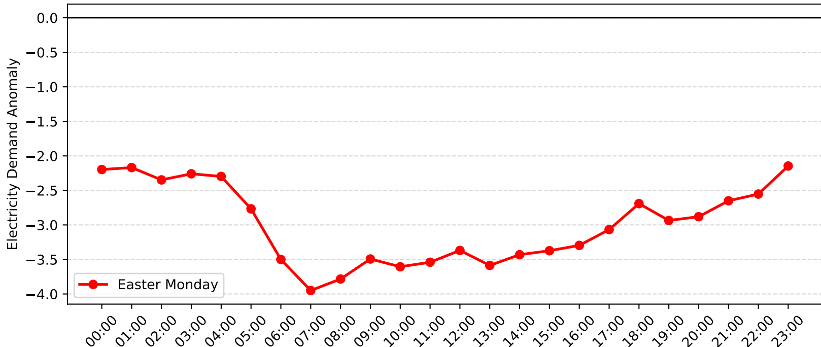
Bass Hill Demand Anomaly: Easter Monday (2014-2015)
