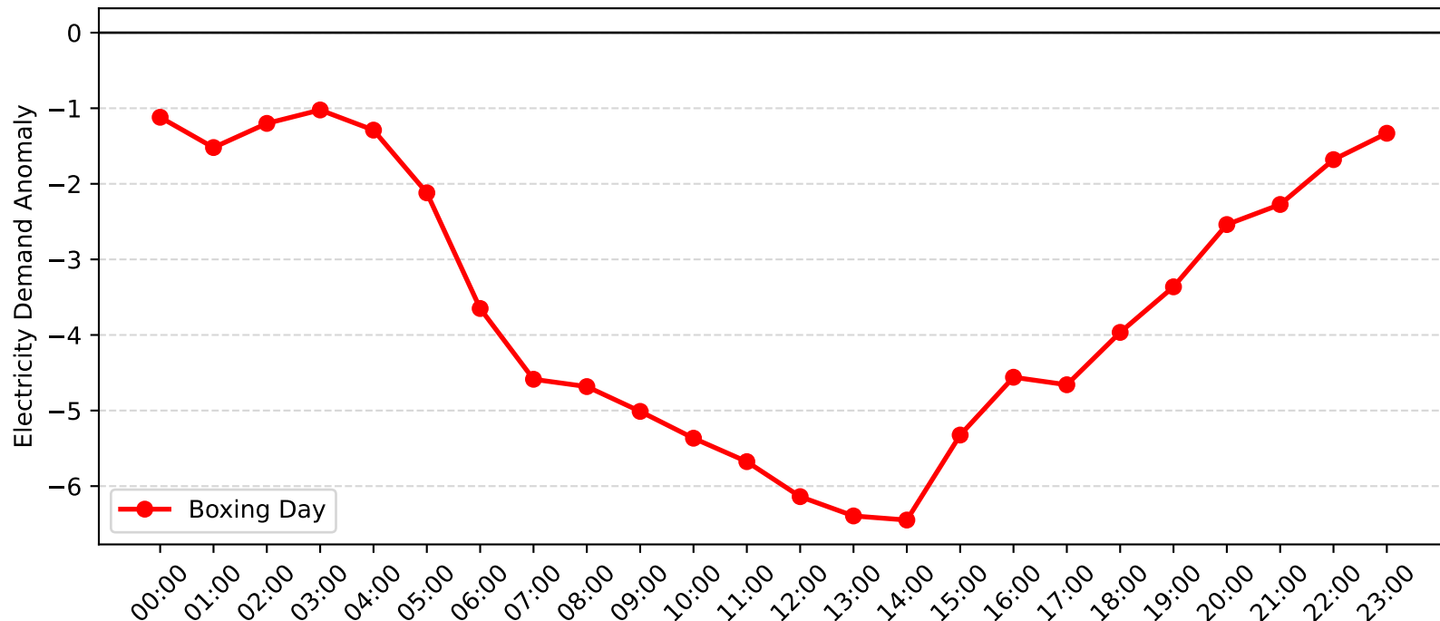
Wyong Demand Anomaly: Boxing Day (2006-2007)
