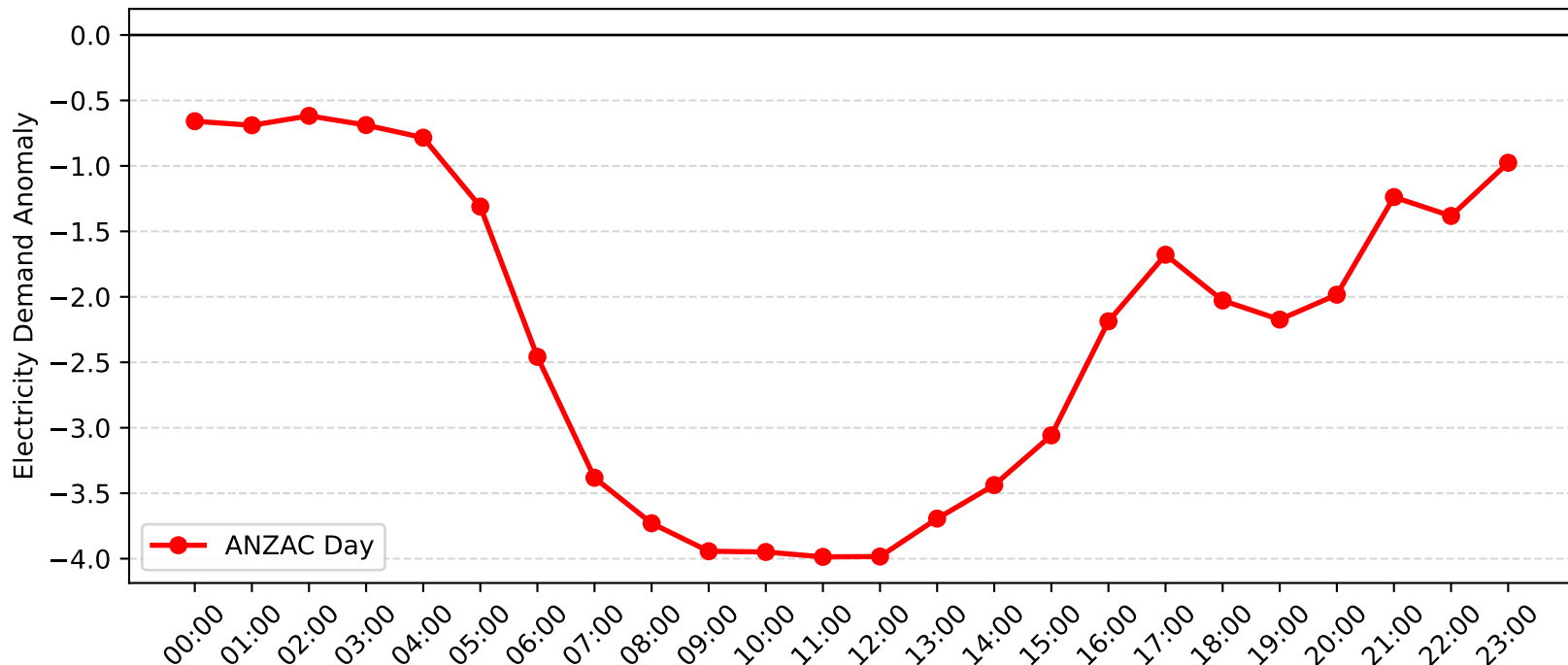
Broadmeadow Demand Anomaly: ANZAC Day (2017-2018)
