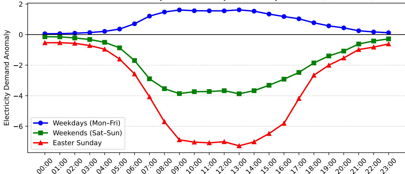
Auburn Demand Anomaly: Easter Sunday vs Weekday/Weekend (2007-2008)
