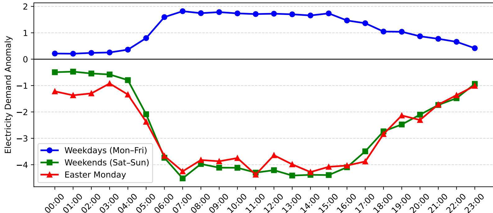
Potts Hill Demand Anomaly: Easter Monday vs Weekday/Weekend (2015-2016)
