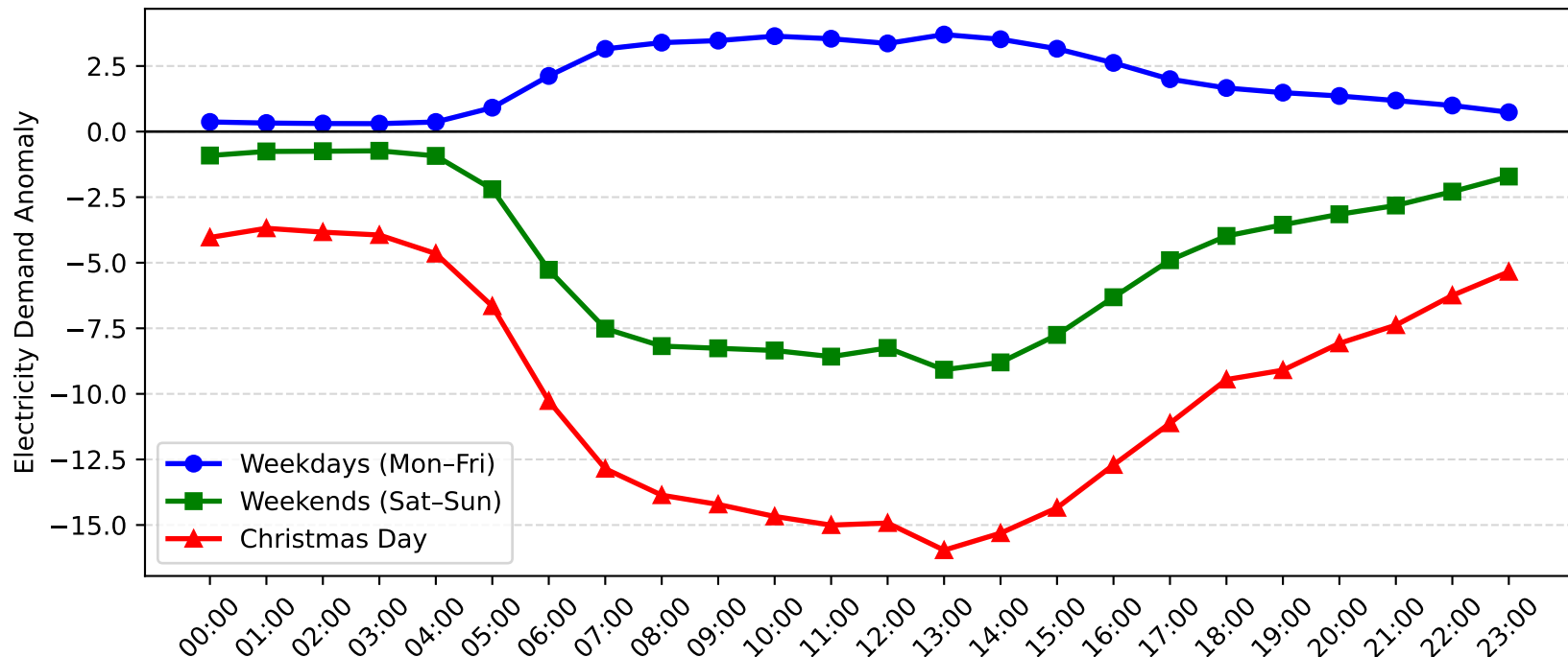
Milperra Demand Anomaly: Christmas Day vs Weekday/Weekend (2006-2007)
