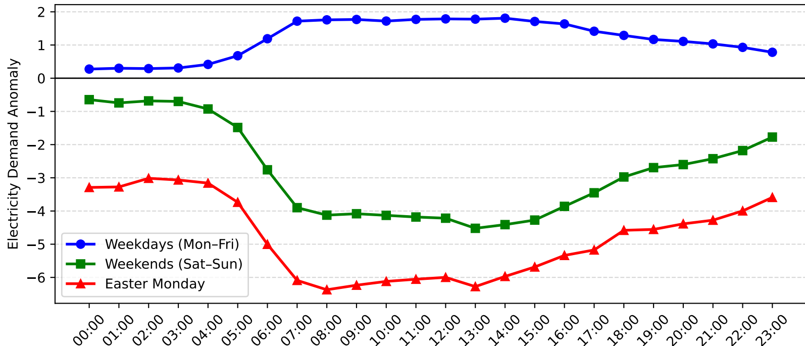
Leightonfield Demand Anomaly: Easter Monday vs Weekday/Weekend (2010-2011)
