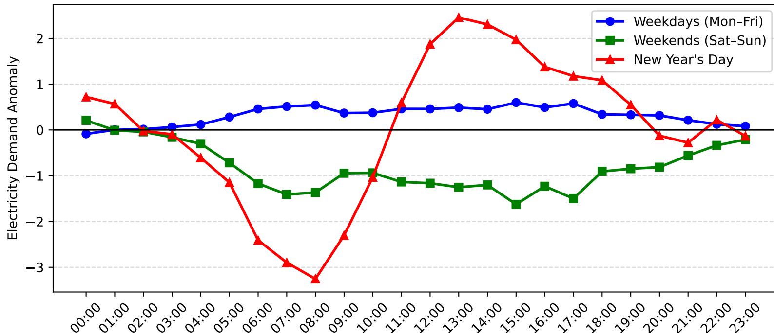
Charmhaven Demand Anomaly: New Year's Day vs Weekday/Weekend (2010-2011)
