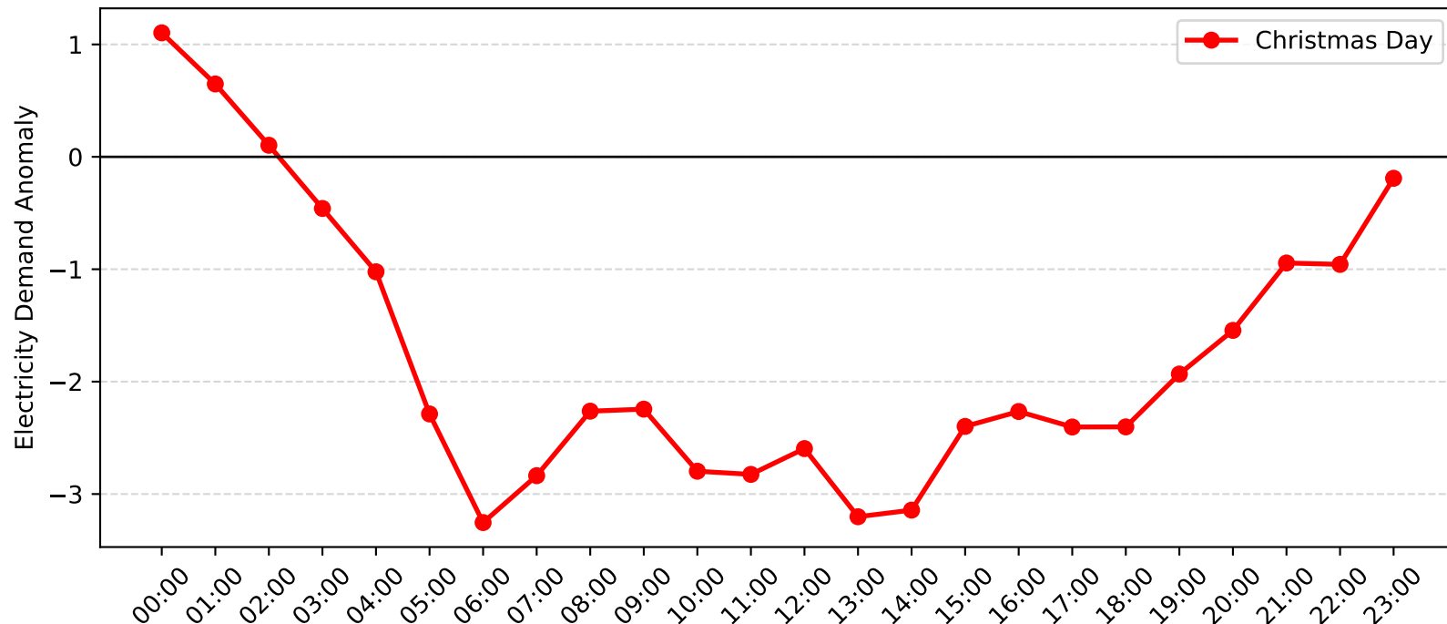
Revesby Demand Anomaly: Christmas Day (2004-2005)
