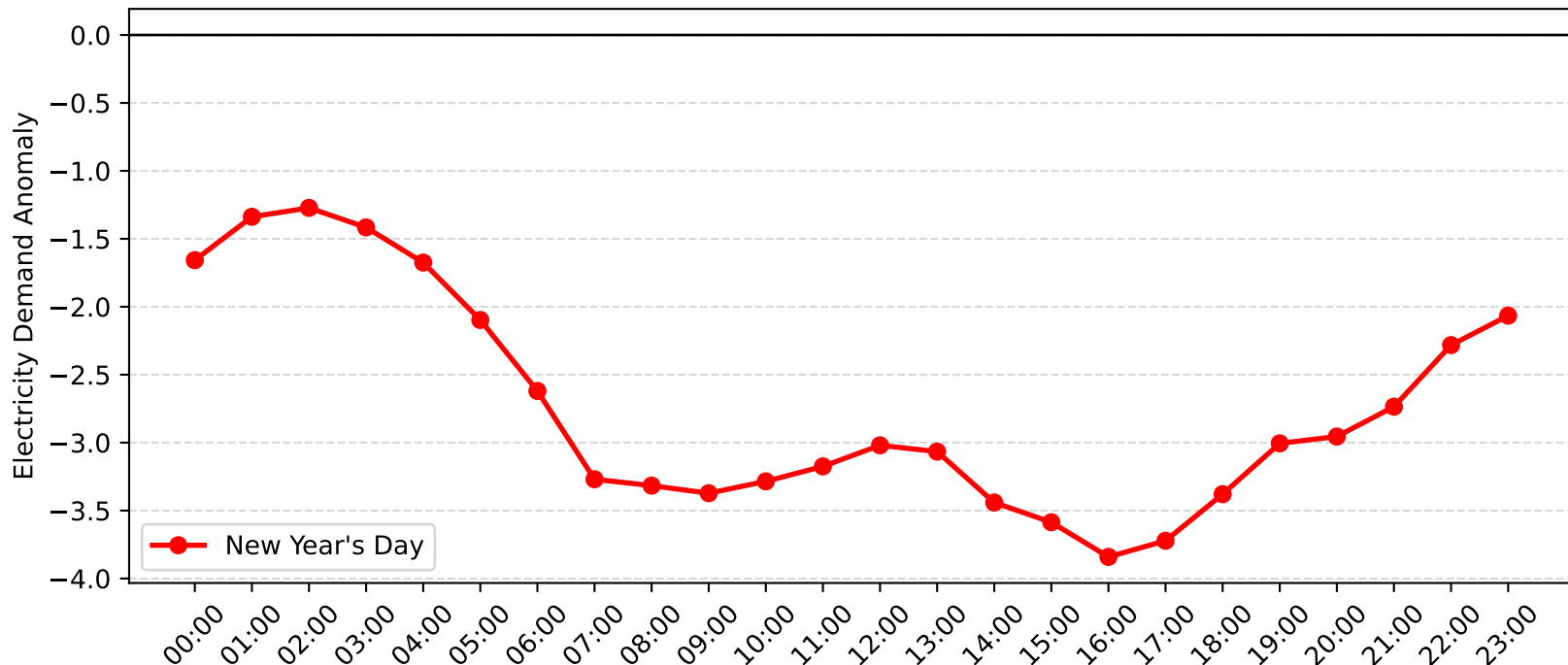
Enfield Demand Anomaly: New Year's Day (2016-2017)
