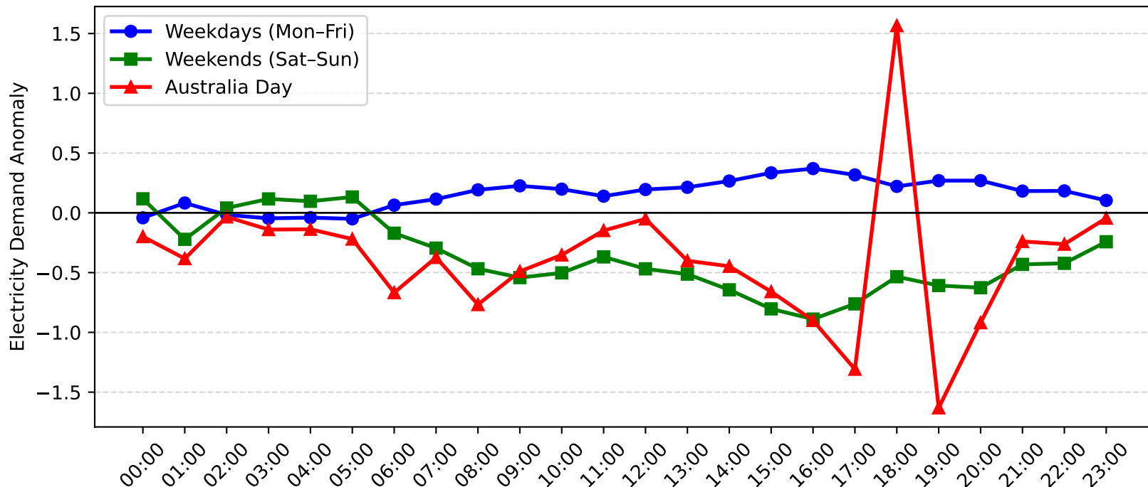
Charmhaven Demand Anomaly: Australia Day vs Weekday/Weekend (2004-2005)
