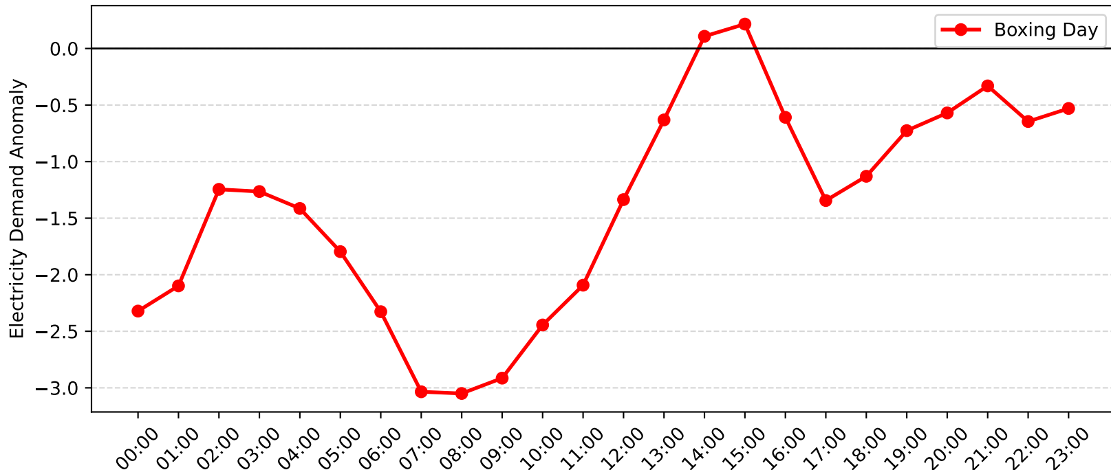
Jesmond Demand Anomaly: Boxing Day (2015-2016)
