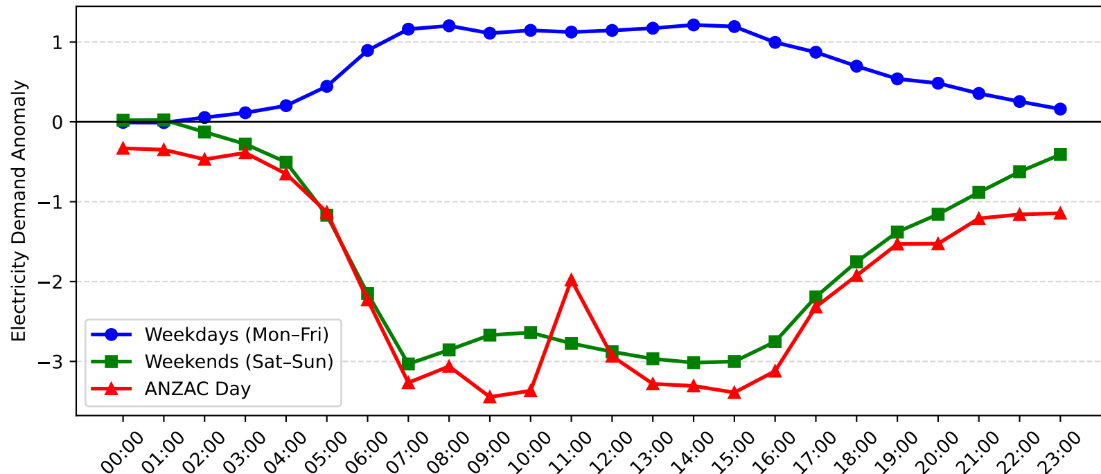
Lidcombe Demand Anomaly: ANZAC Day vs Weekday/Weekend (2005-2006)
