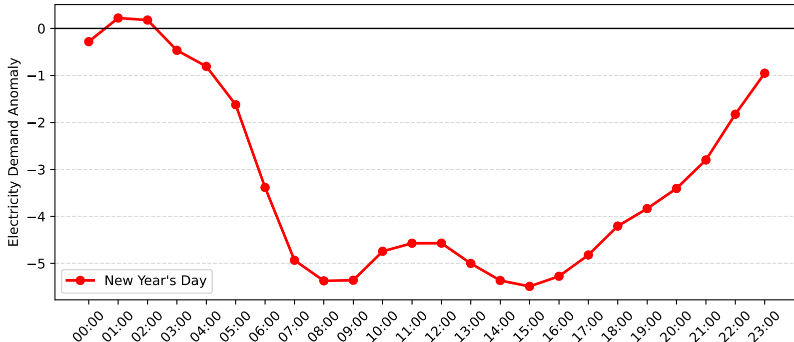
Five Dock Demand Anomaly: New Year's Day (2015-2016)
