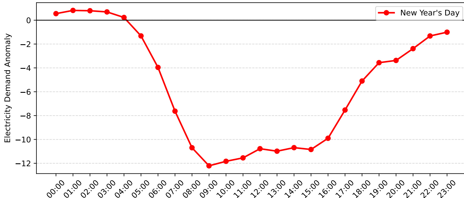
Brookvale Demand Anomaly: New Year's Day (2017-2018)
