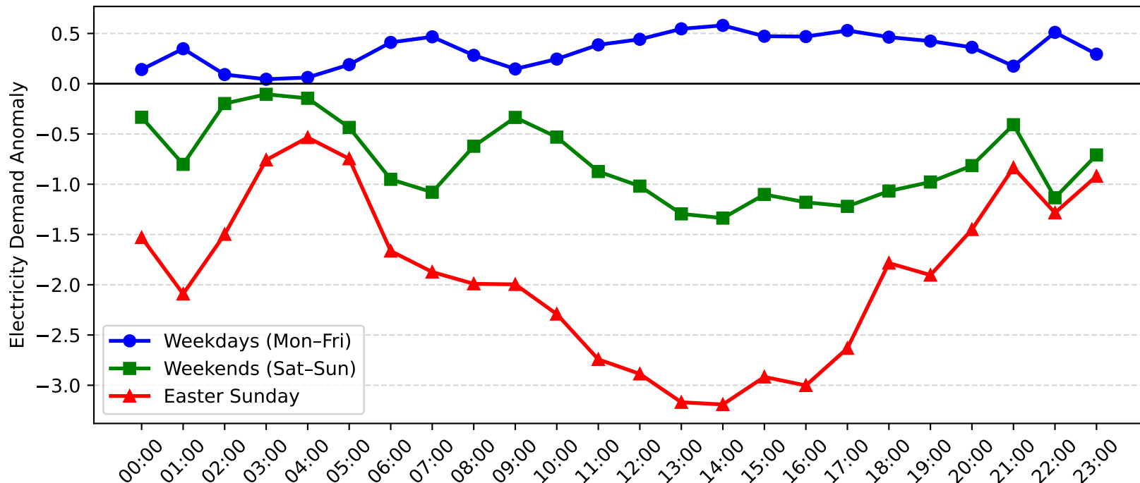
Gateshead Demand Anomaly: Easter Sunday vs Weekday/Weekend (2005-2006)
