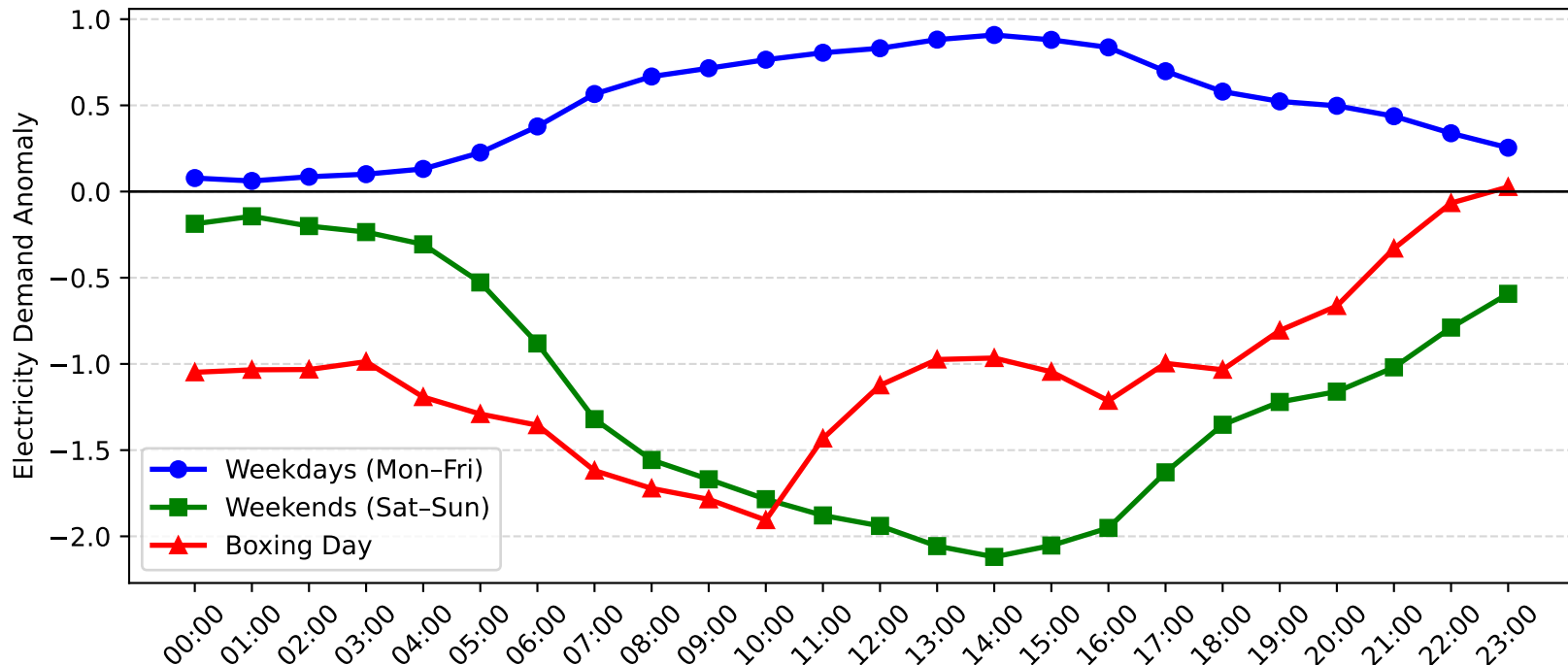
Lidcombe Demand Anomaly: Boxing Day vs Weekday/Weekend (2016-2017)
