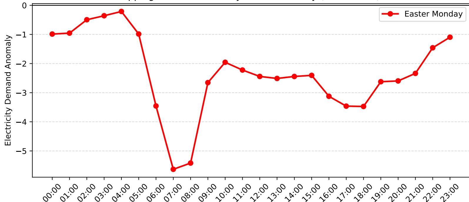
Epping Demand Anomaly: Easter Monday (2008-2009)
