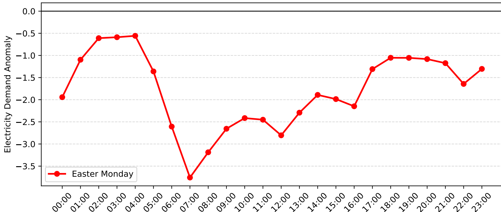
Matraville Demand Anomaly: Easter Monday (2015-2016)
