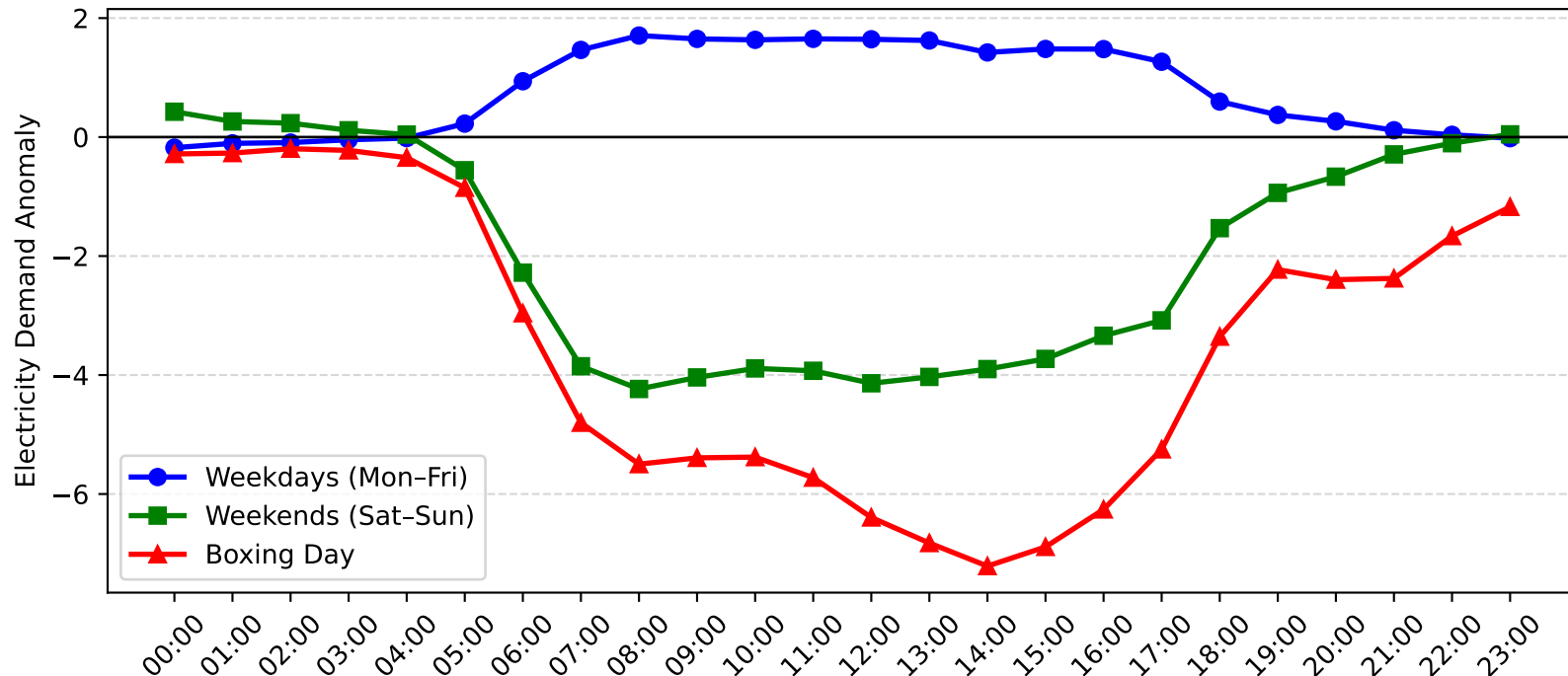
Pymble Demand Anomaly: Boxing Day vs Weekday/Weekend (2009-2010)
