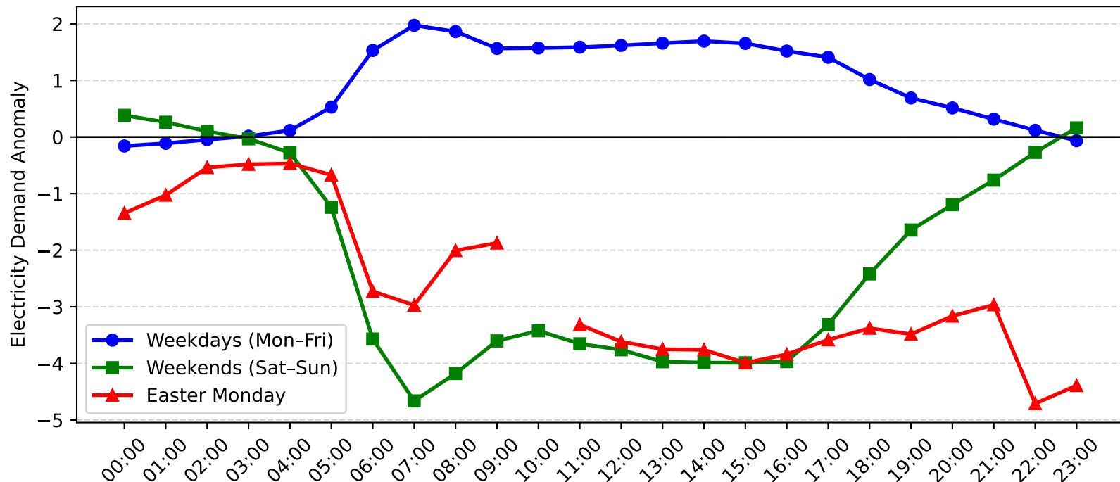
Pymble Demand Anomaly: Easter Monday vs Weekday/Weekend (2005-2006)
