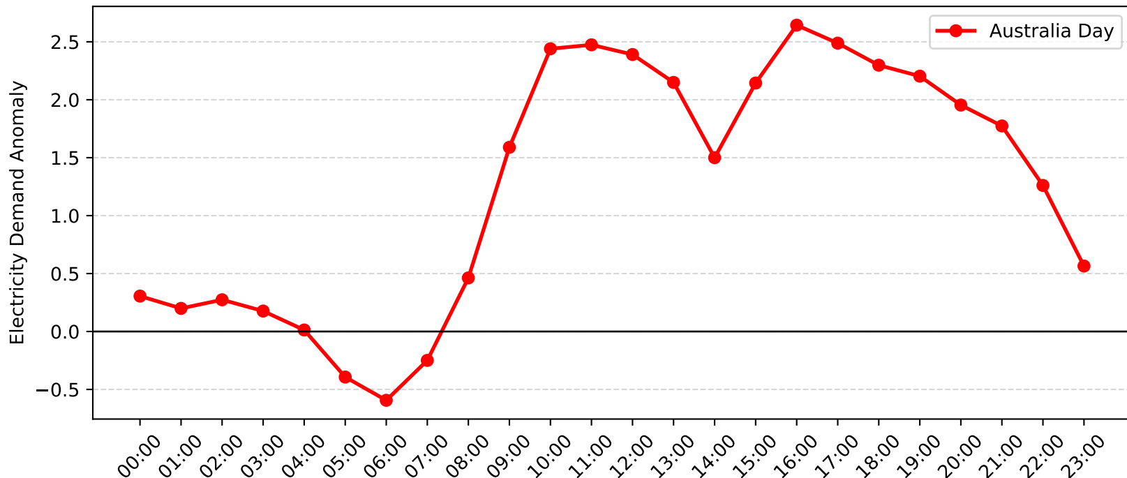
Woy Woy Demand Anomaly: Australia Day (2011-2012)
