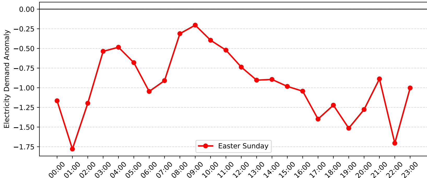
Jewells Demand Anomaly: Easter Sunday (2009-2010)
