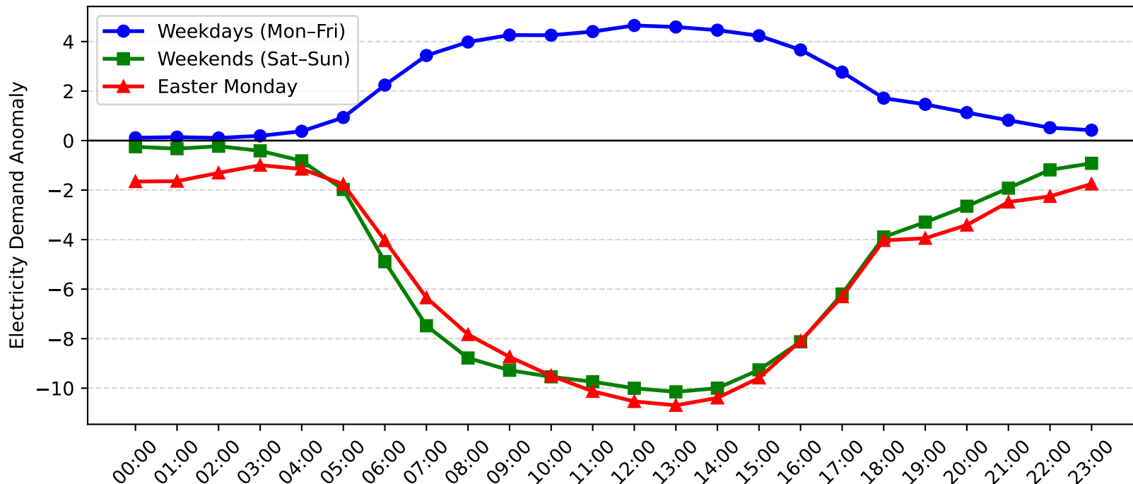
Mascot Demand Anomaly: Easter Monday vs Weekday/Weekend (2009-2010)
