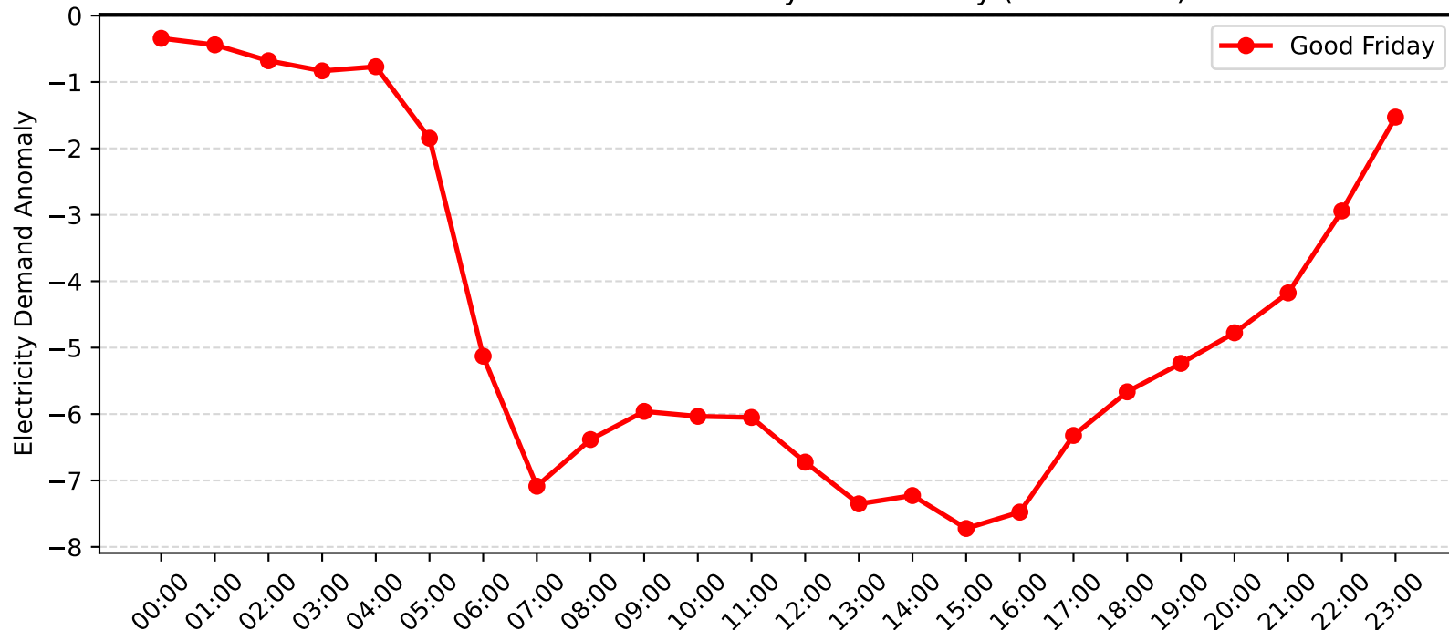
Chatswood Demand Anomaly: Good Friday (2005-2006)
