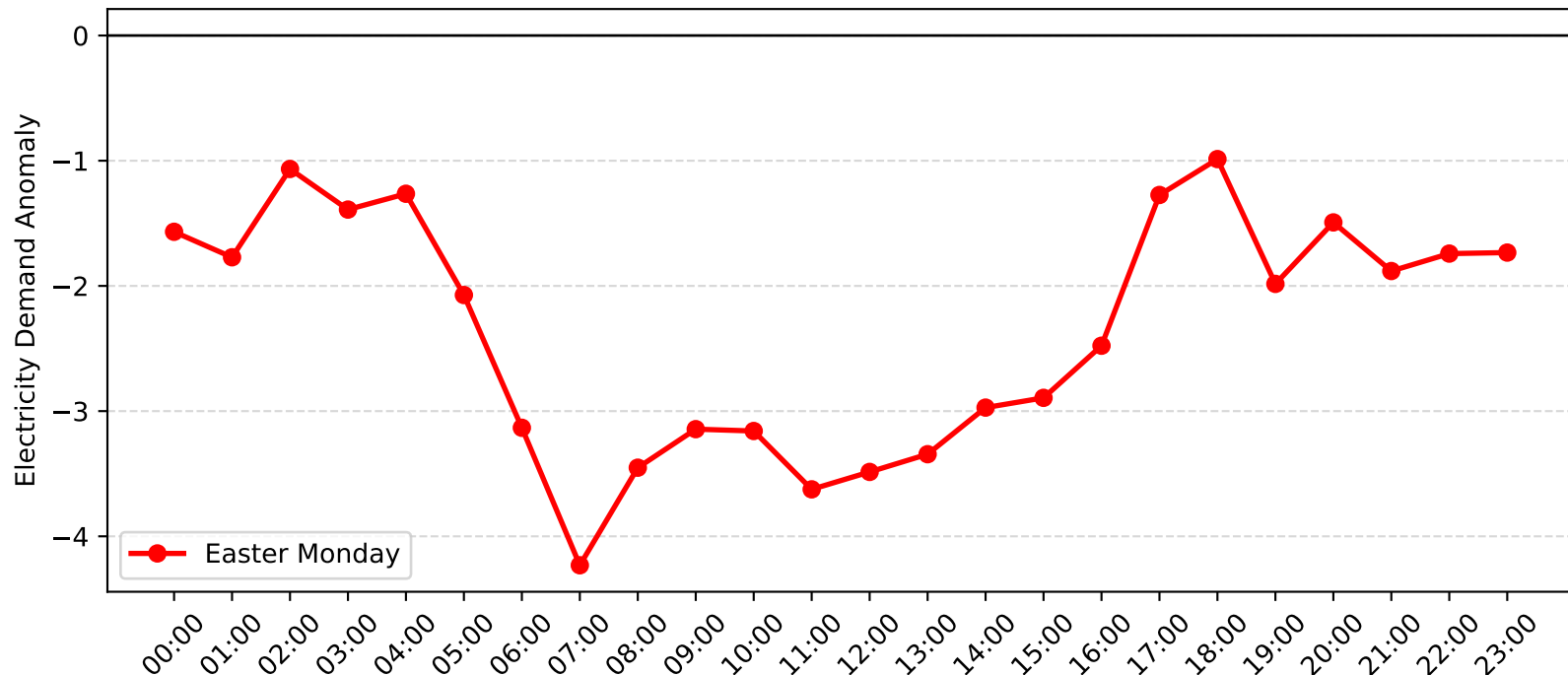
Matraville Demand Anomaly: Easter Monday (2017-2018)
