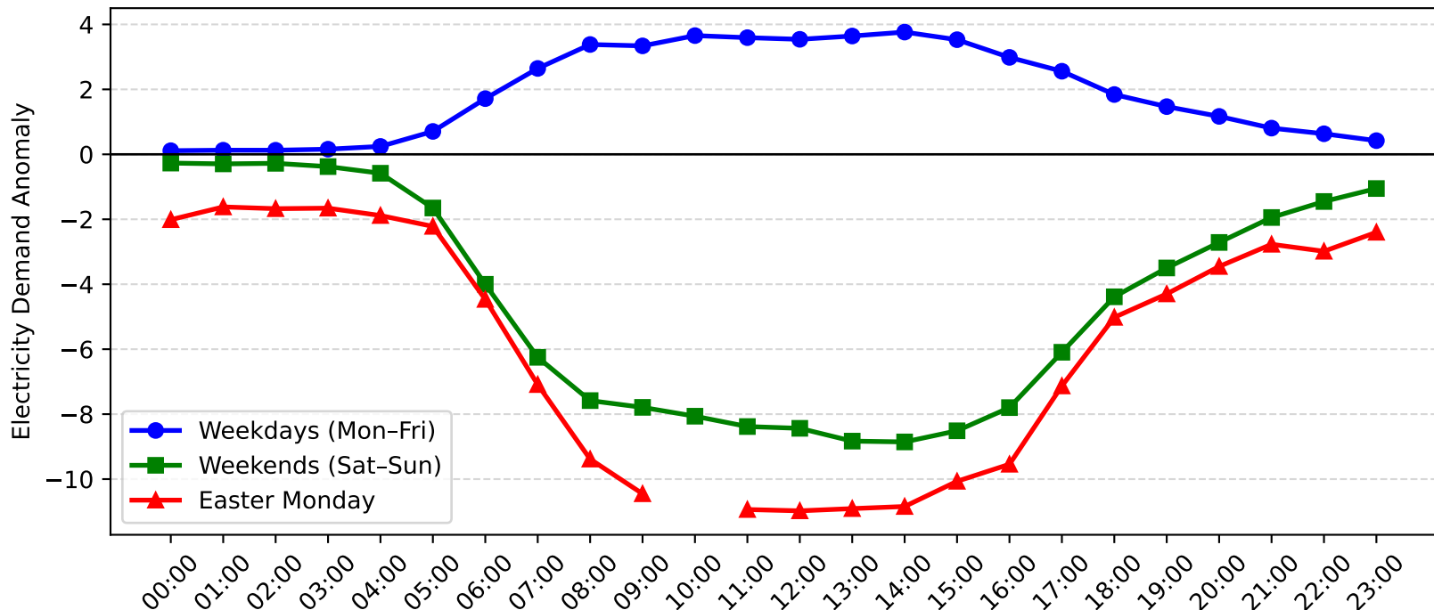
Mascot Demand Anomaly: Easter Monday vs Weekday/Weekend (2005-2006)
