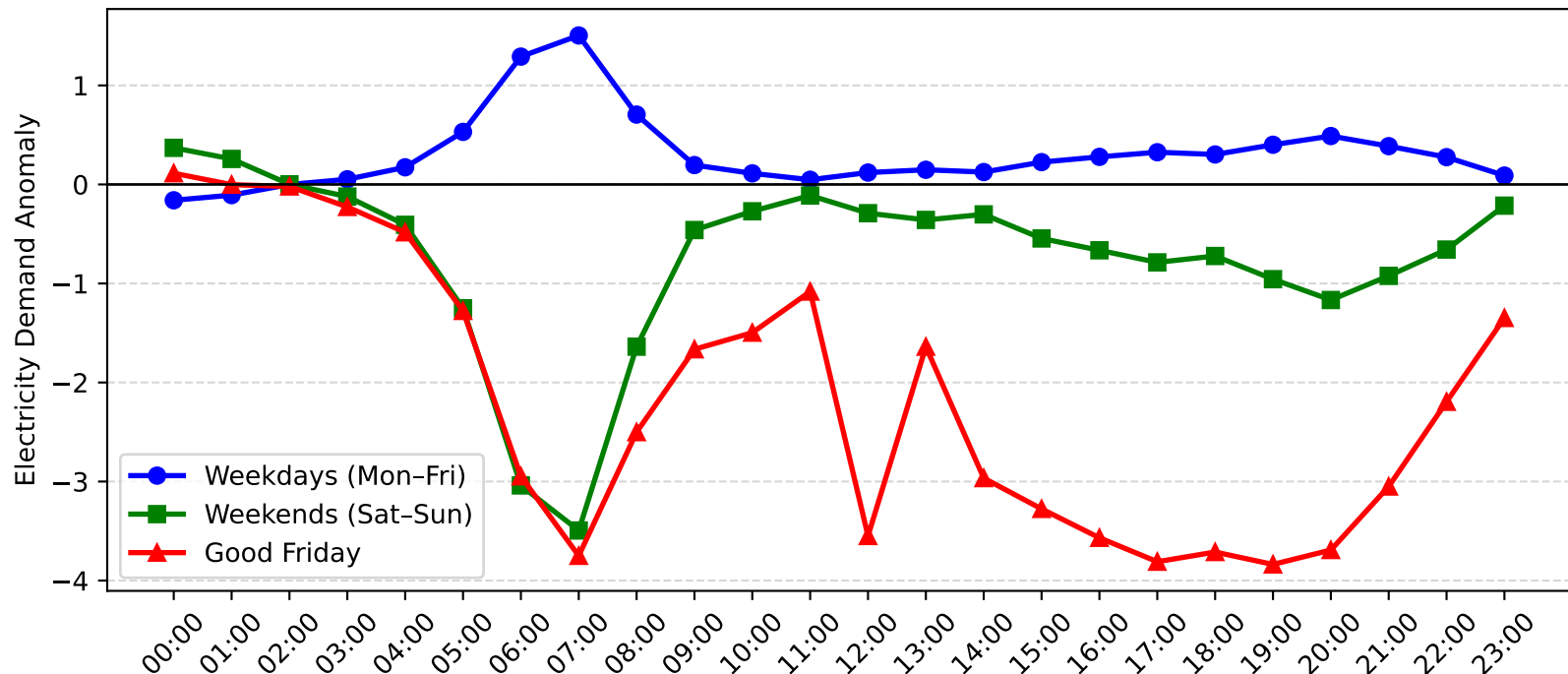
Dulwich Hill Demand Anomaly: Good Friday vs Weekday/Weekend (2016-2017)
