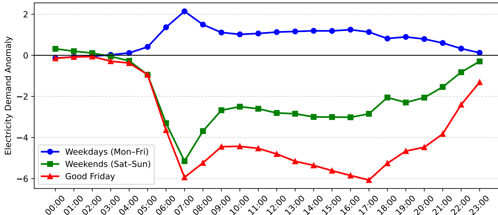
Chatswood Demand Anomaly: Good Friday vs Weekday/Weekend (2010-2011)
