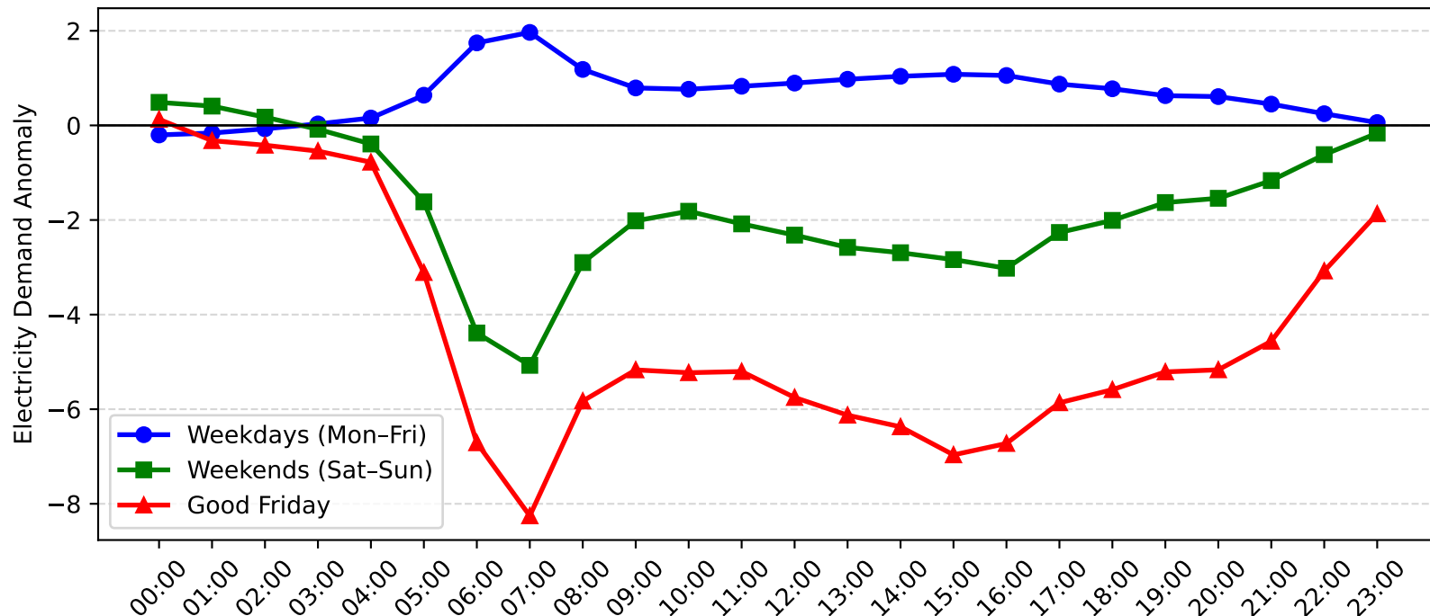
Dulwich Hill Demand Anomaly: Good Friday vs Weekday/Weekend (2005-2006)
