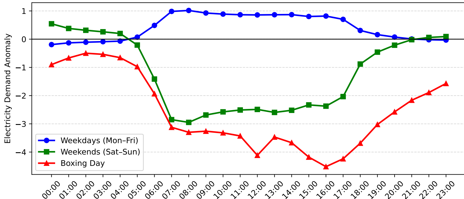
Pymble Demand Anomaly: Boxing Day vs Weekday/Weekend (2012-2013)
