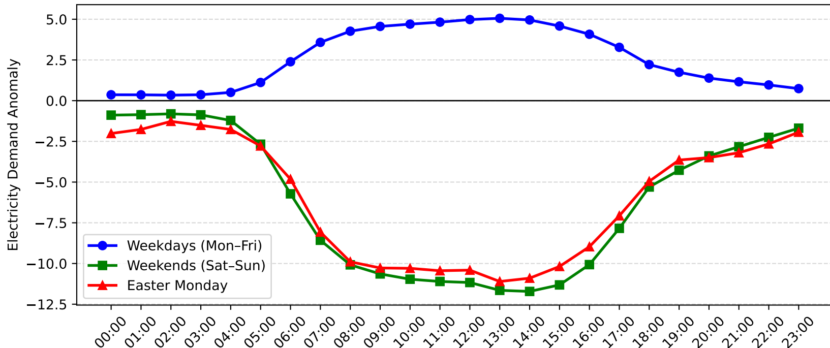
Mascot Demand Anomaly: Easter Monday vs Weekday/Weekend (2007-2008)
