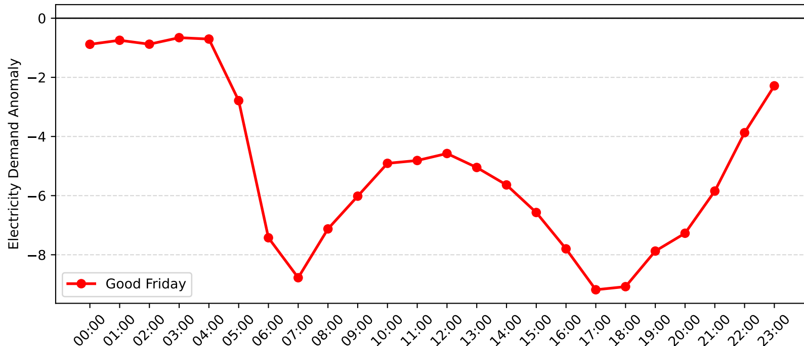
Pennant Hills Demand Anomaly: Good Friday (2010-2011)
