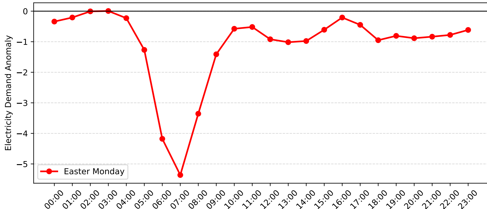
Mortdale Demand Anomaly: Easter Monday (2008-2009)
