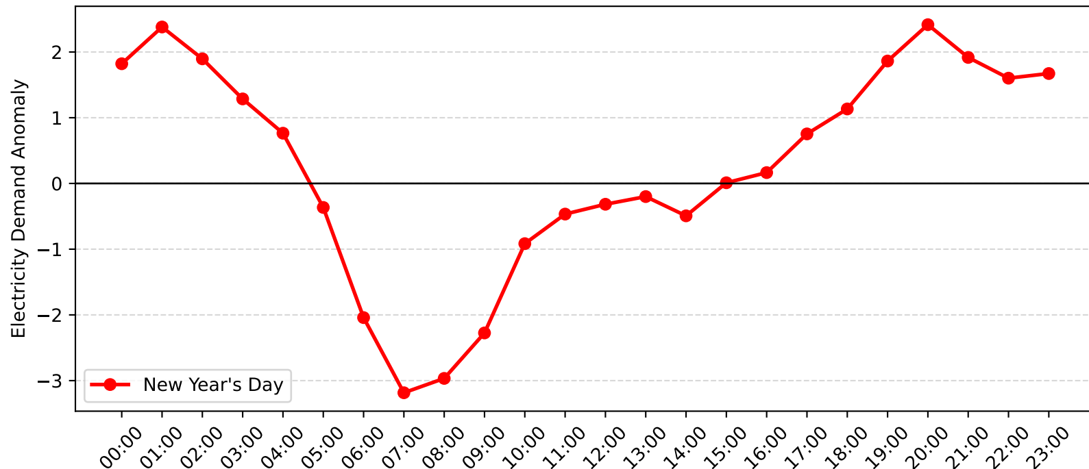
Five Dock Demand Anomaly: New Year's Day (2005-2006)
