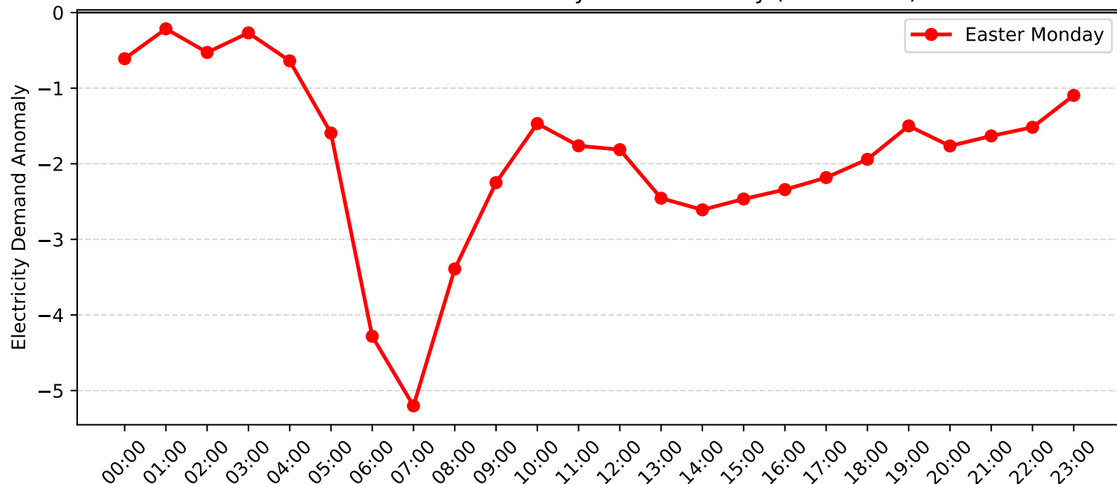
Mortdale Demand Anomaly: Easter Monday (2013-2014)
