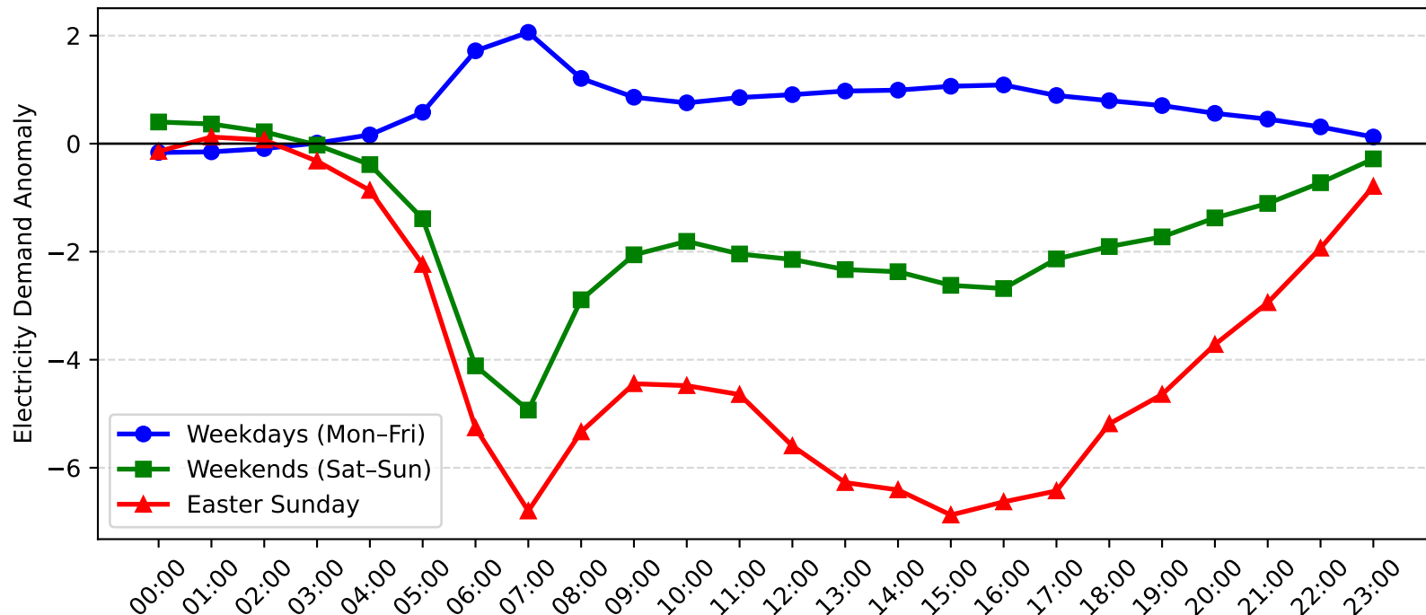
Dulwich Hill Demand Anomaly: Easter Sunday vs Weekday/Weekend (2007-2008)
