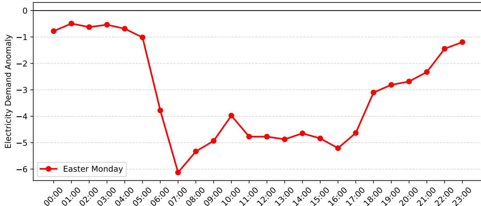
Epping Demand Anomaly: Easter Monday (2012-2013)
