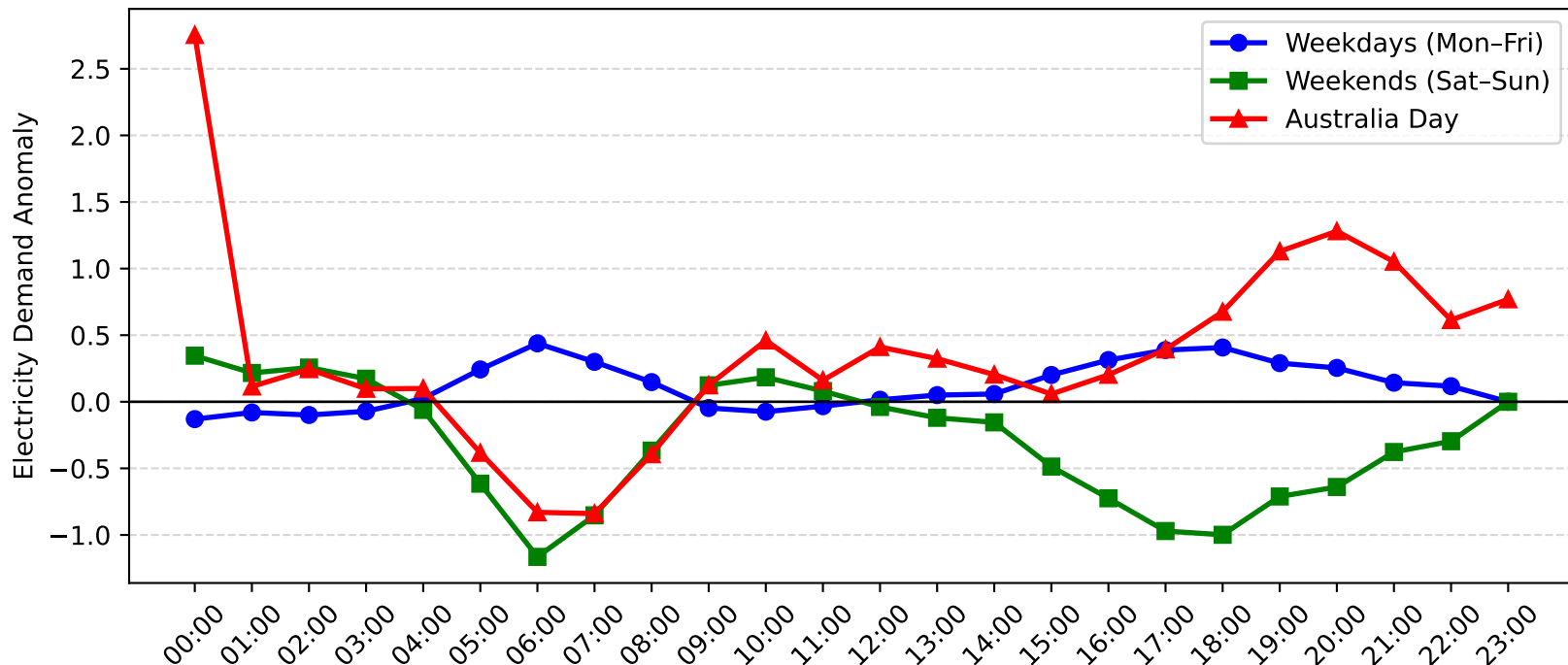
Woy Woy Demand Anomaly: Australia Day vs Weekday/Weekend (2009-2010)
