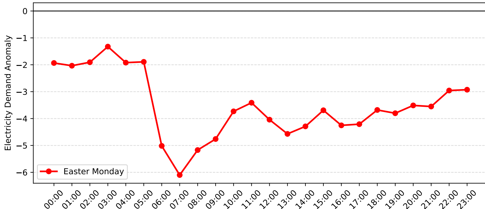
Matraville Demand Anomaly: Easter Monday (2011-2012)
