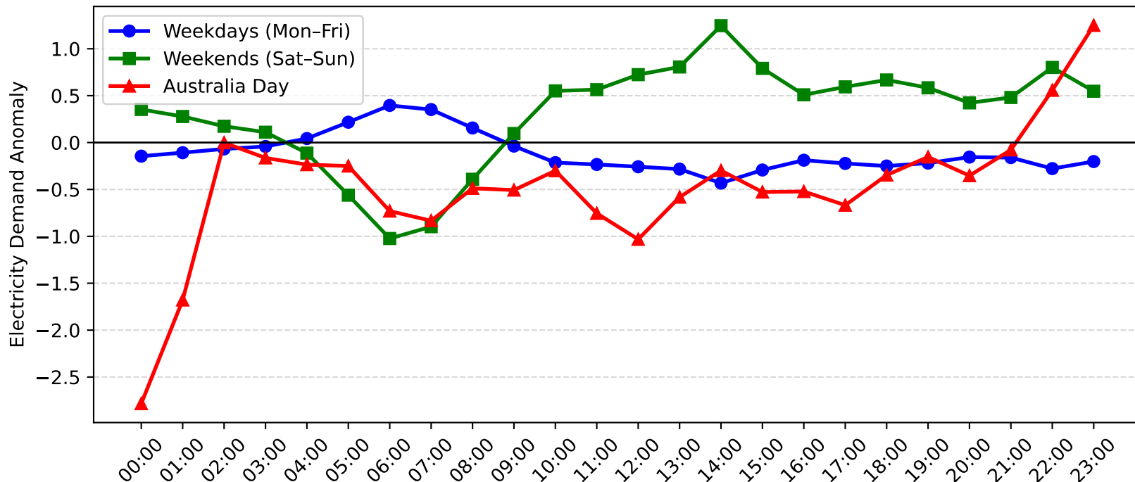
Woy Woy Demand Anomaly: Australia Day vs Weekday/Weekend (2006-2007)
