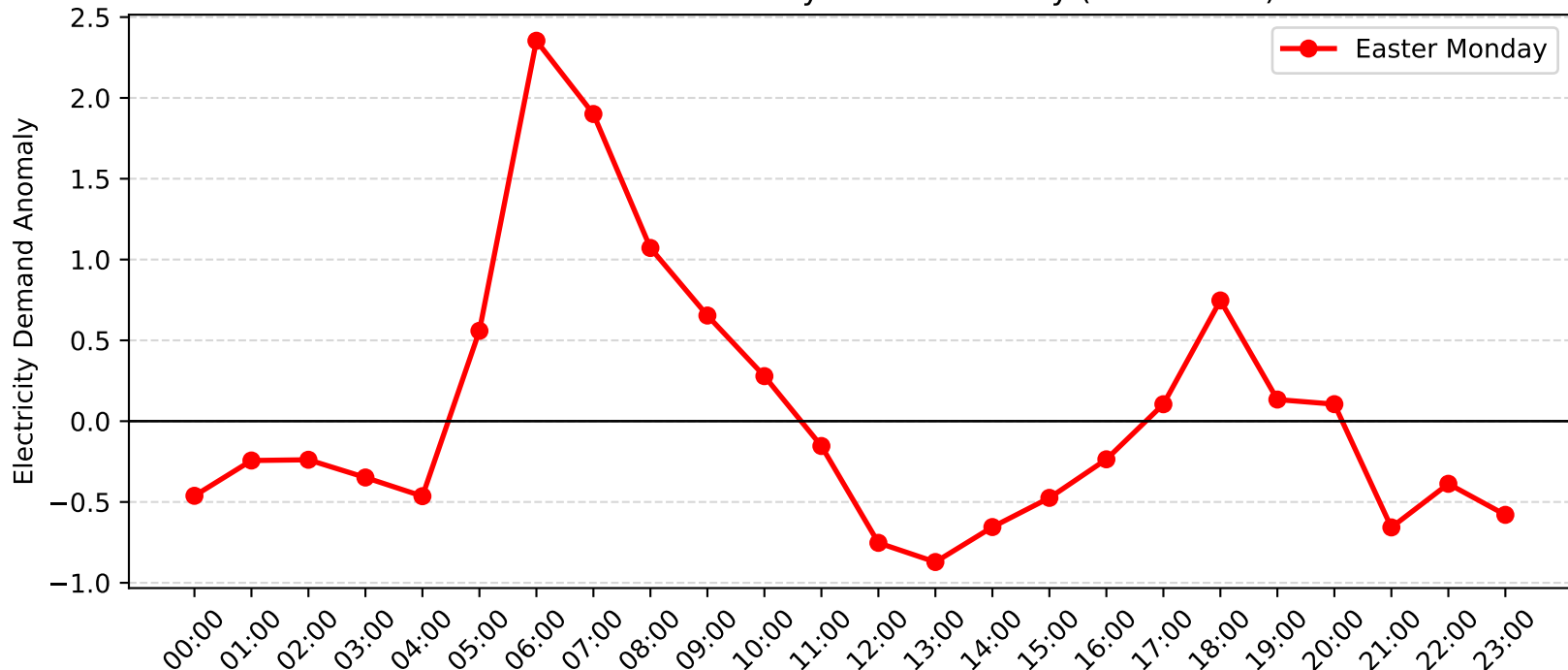
Mascot Demand Anomaly: Easter Monday (2004-2005)
