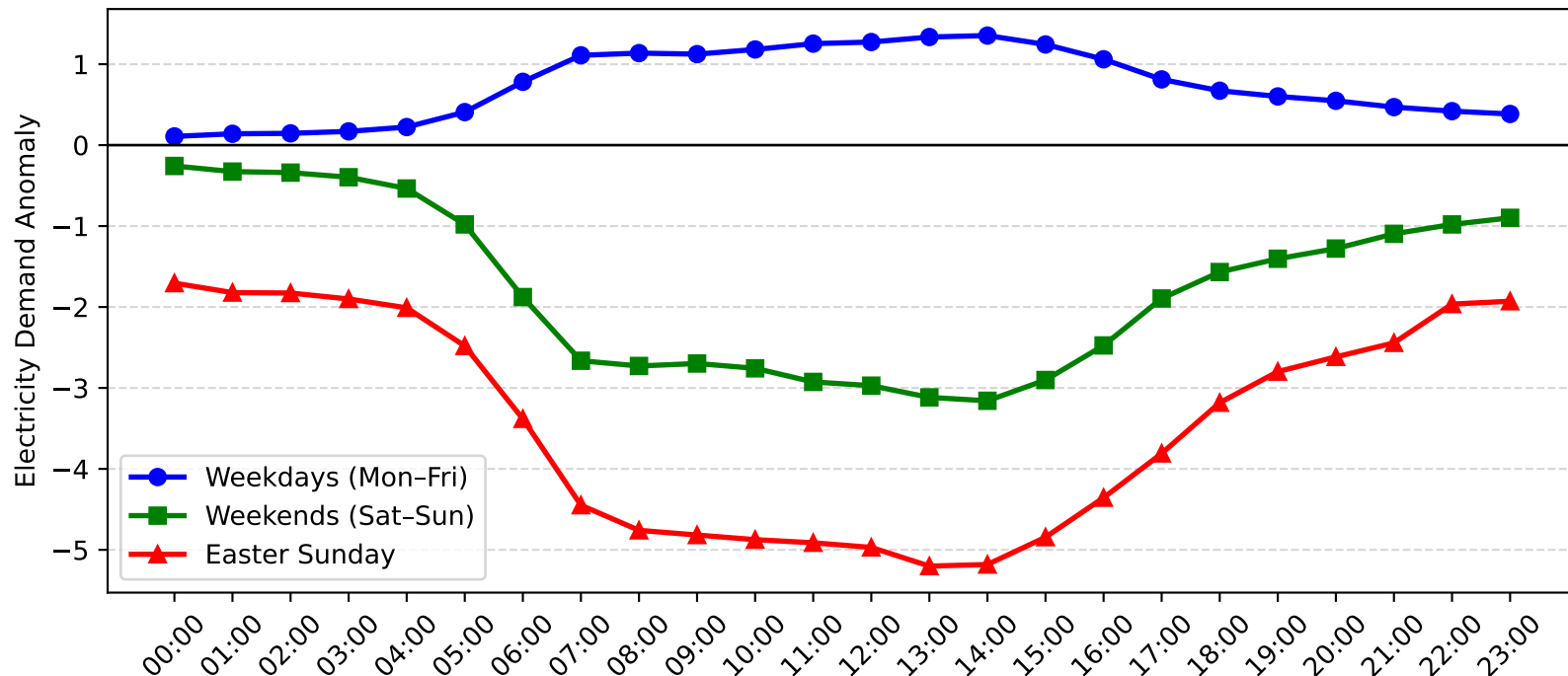
Caringbah Demand Anomaly: Easter Sunday vs Weekday/Weekend (2012-2013)
