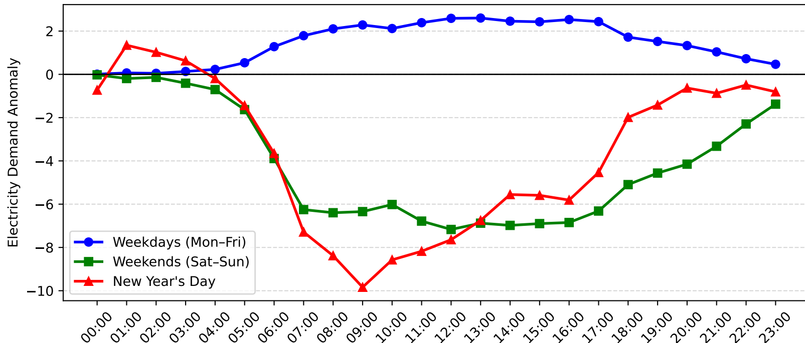
Burwood Demand Anomaly: New Year's Day vs Weekday/Weekend (2009-2010)
