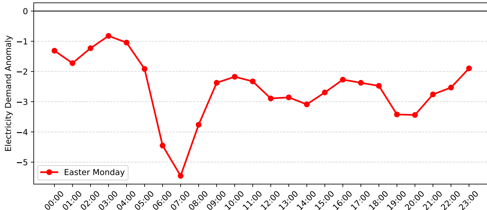
Mortdale Demand Anomaly: Easter Monday (2009-2010)
