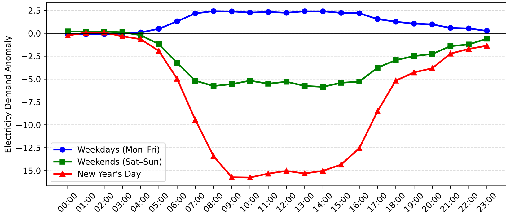
Brookvale Demand Anomaly: New Year's Day vs Weekday/Weekend (2007-2008)
