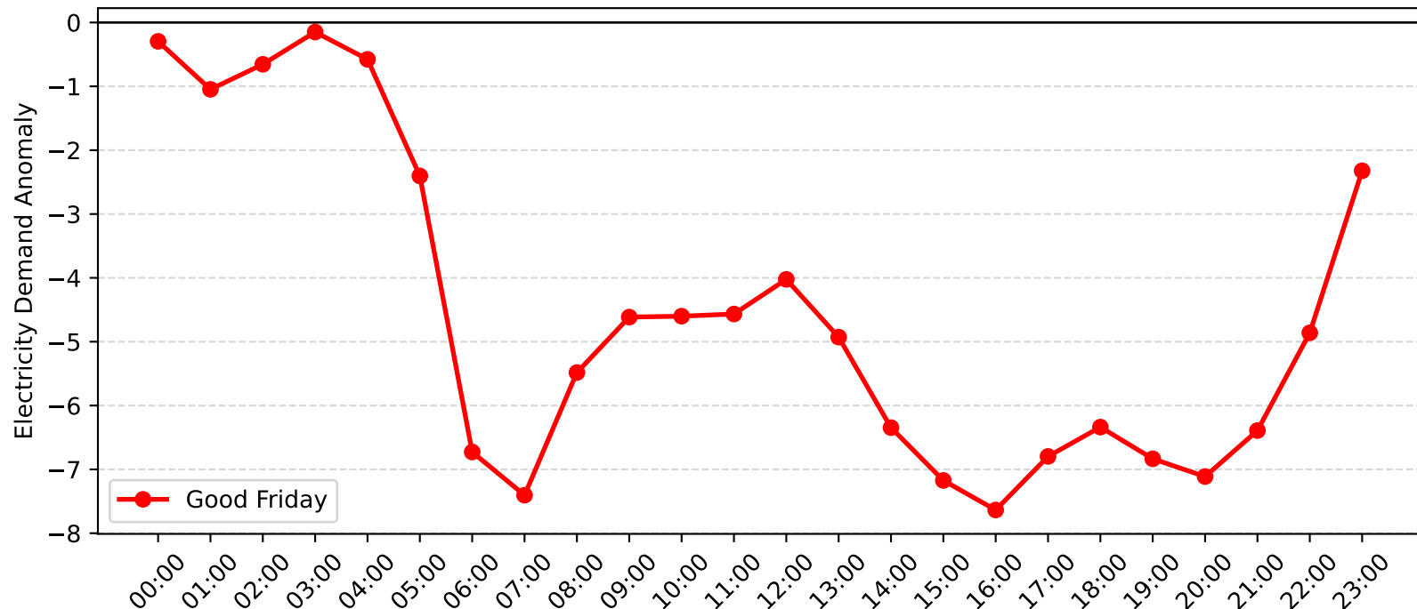
Pennant Hills Demand Anomaly: Good Friday (2008-2009)
