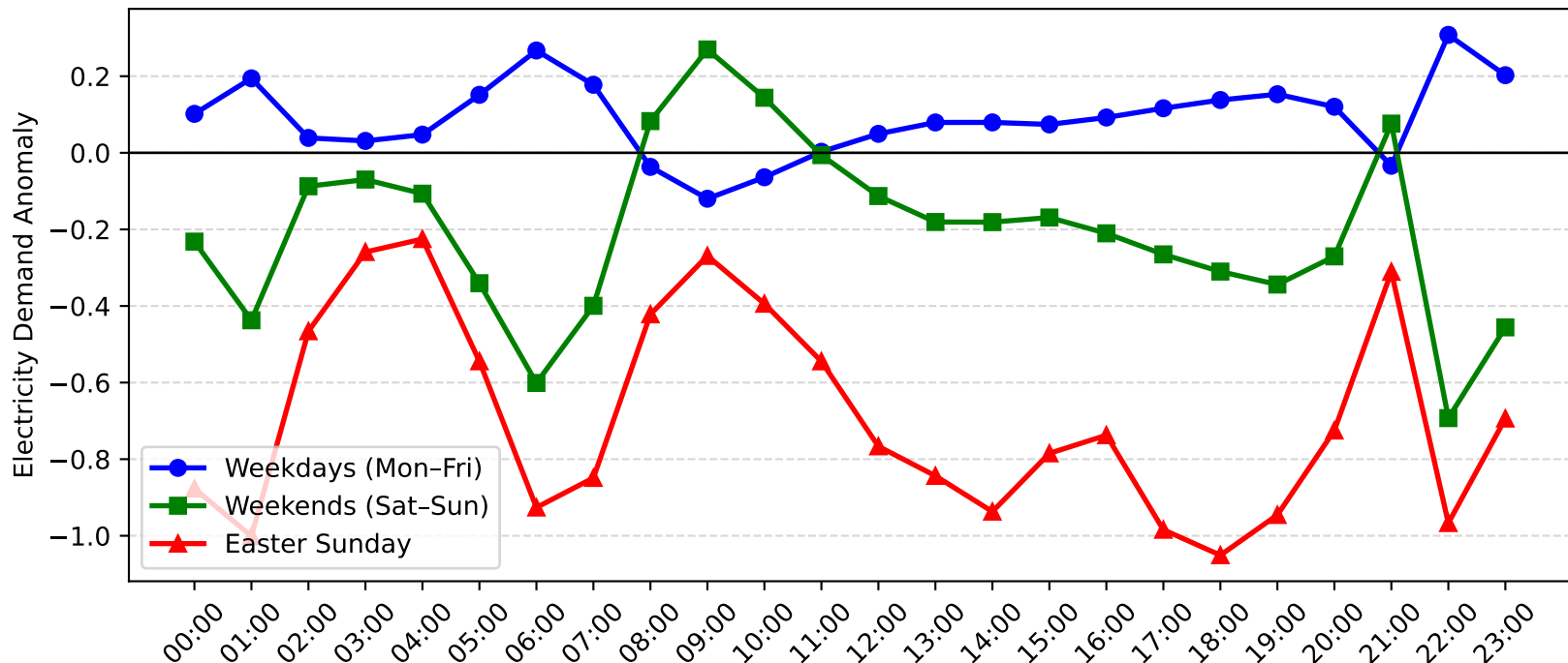
Jewells Demand Anomaly: Easter Sunday vs Weekday/Weekend (2016-2017)
