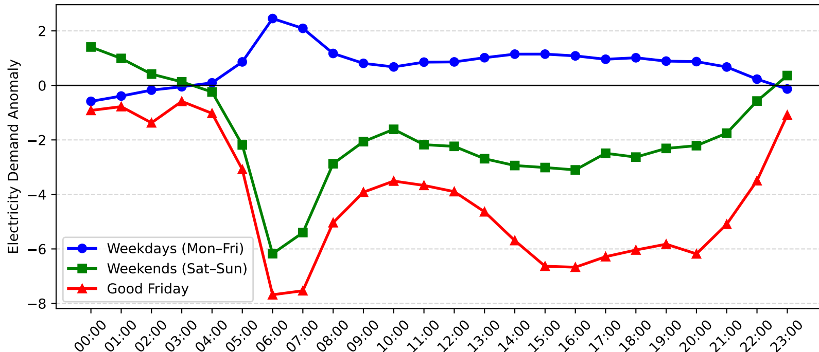
Pennant Hills Demand Anomaly: Good Friday vs Weekday/Weekend (2005-2006)
