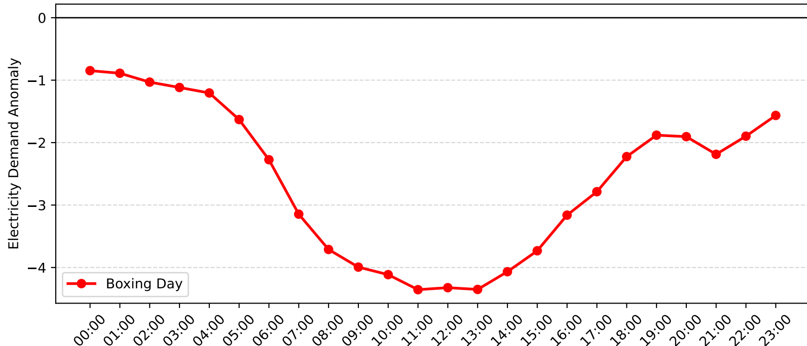
Lidcombe Demand Anomaly: Boxing Day (2010-2011)
