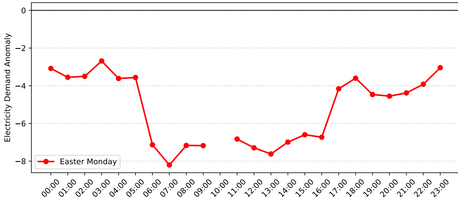
Matraville Demand Anomaly: Easter Monday (2005-2006)
