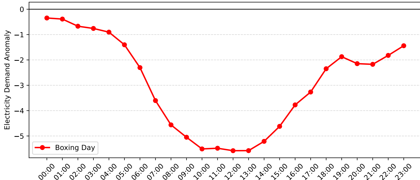
Lidcombe Demand Anomaly: Boxing Day (2009-2010)
