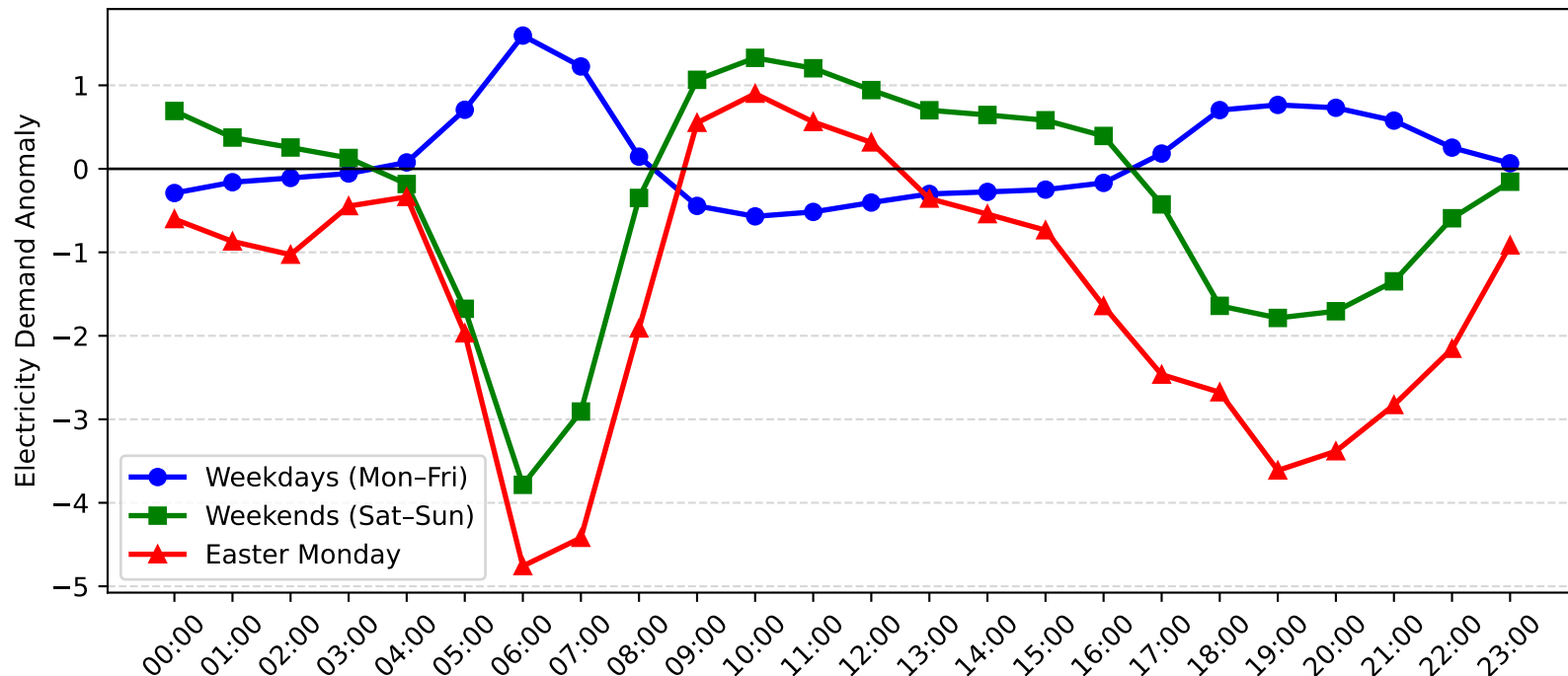
Cronulla Demand Anomaly: Easter Monday vs Weekday/Weekend (2011-2012)
