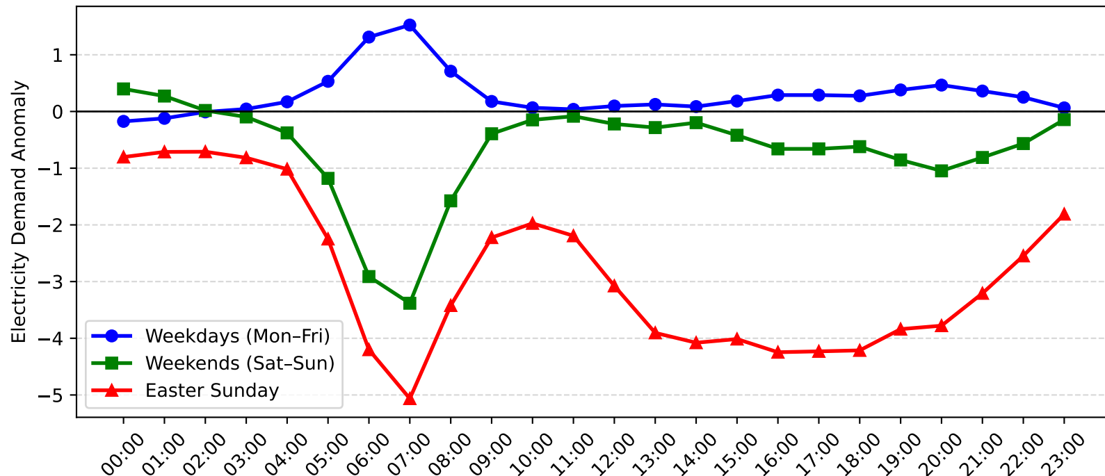
Dulwich Hill Demand Anomaly: Easter Sunday vs Weekday/Weekend (2016-2017)
