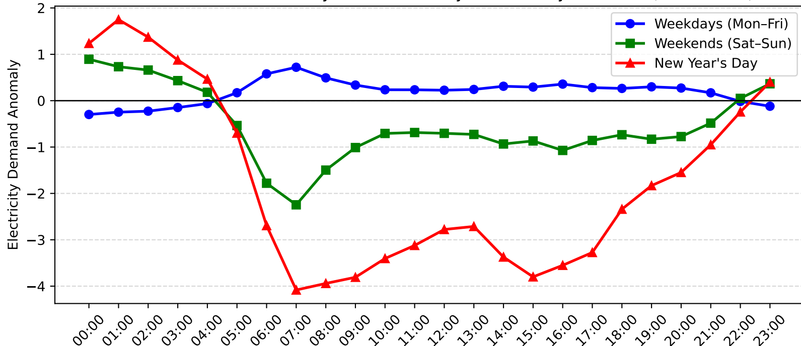
Five Dock Demand Anomaly: New Year's Day vs Weekday/Weekend (2014-2015)
