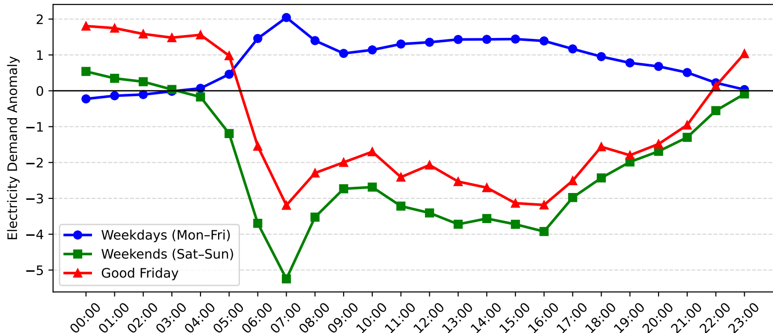
Chatswood Demand Anomaly: Good Friday vs Weekday/Weekend (2006-2007)
