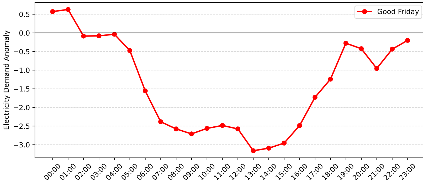
Gateshead Demand Anomaly: Good Friday (2007-2008)
