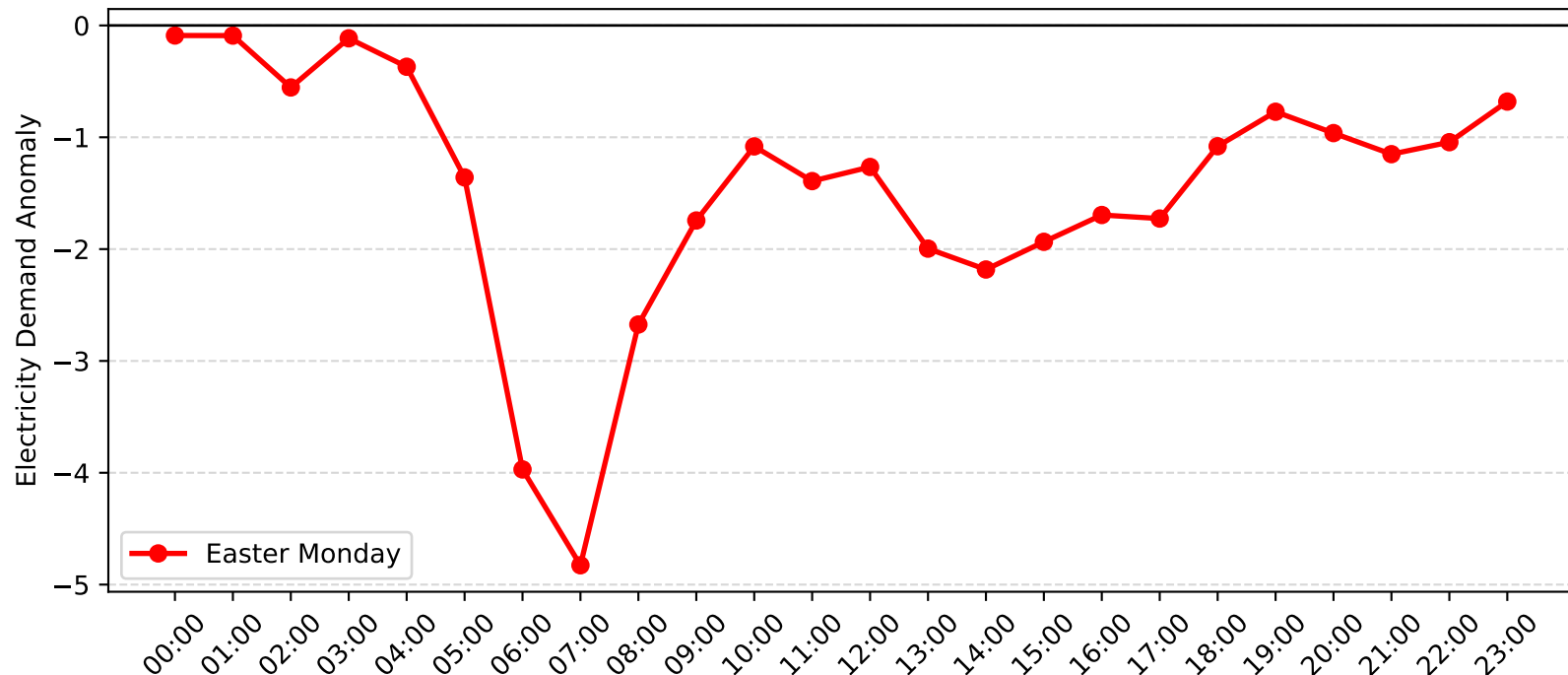
Mortdale Demand Anomaly: Easter Monday (2012-2013)
