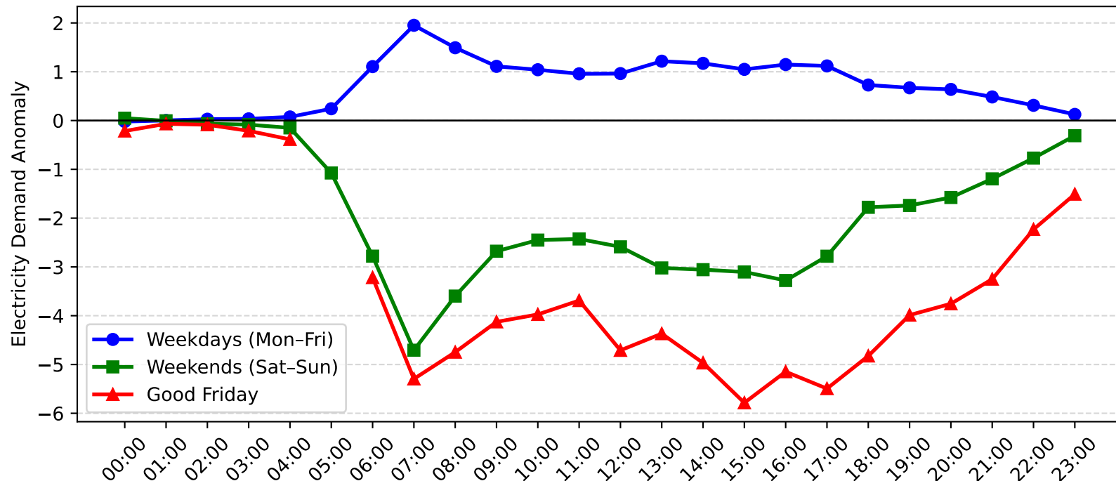
Chatswood Demand Anomaly: Good Friday vs Weekday/Weekend (2015-2016)
