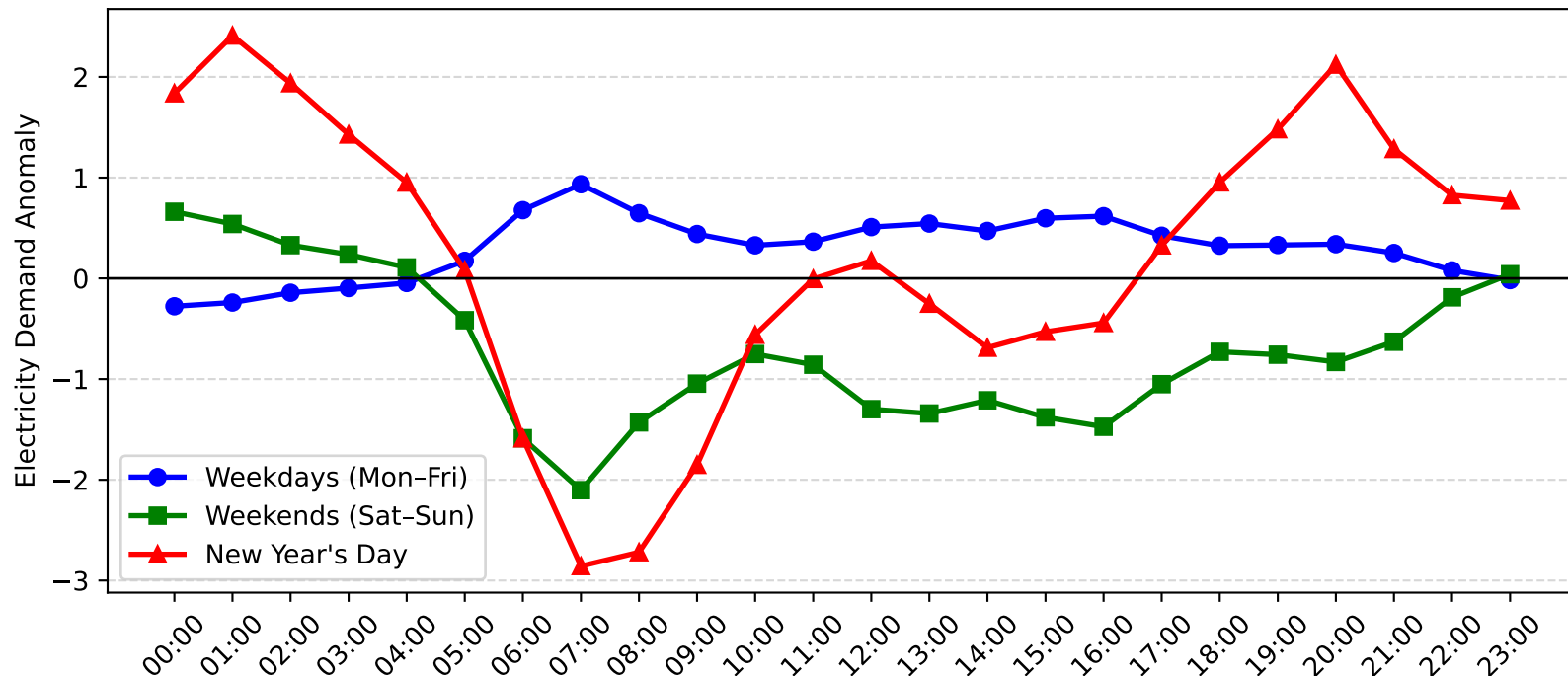
Five Dock Demand Anomaly: New Year's Day vs Weekday/Weekend (2006-2007)
