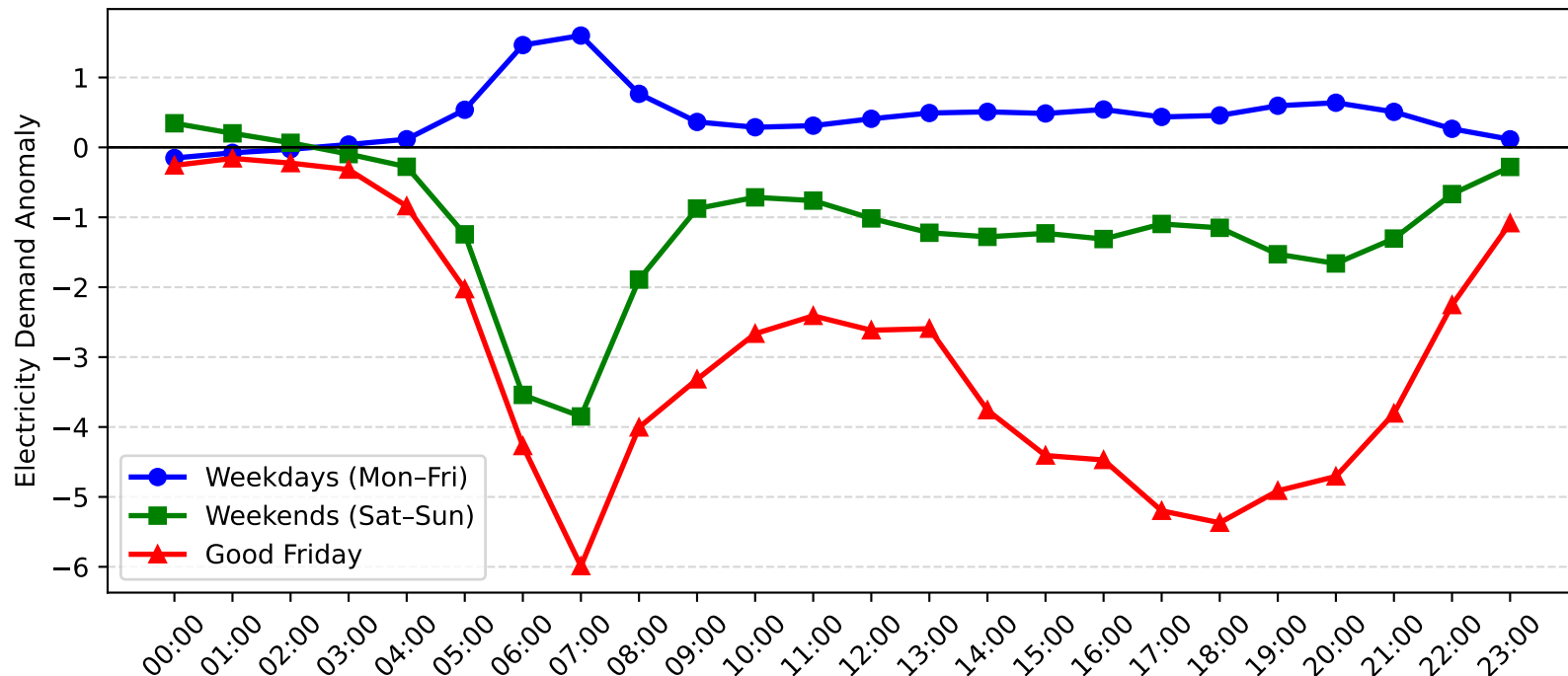
Dulwich Hill Demand Anomaly: Good Friday vs Weekday/Weekend (2010-2011)
