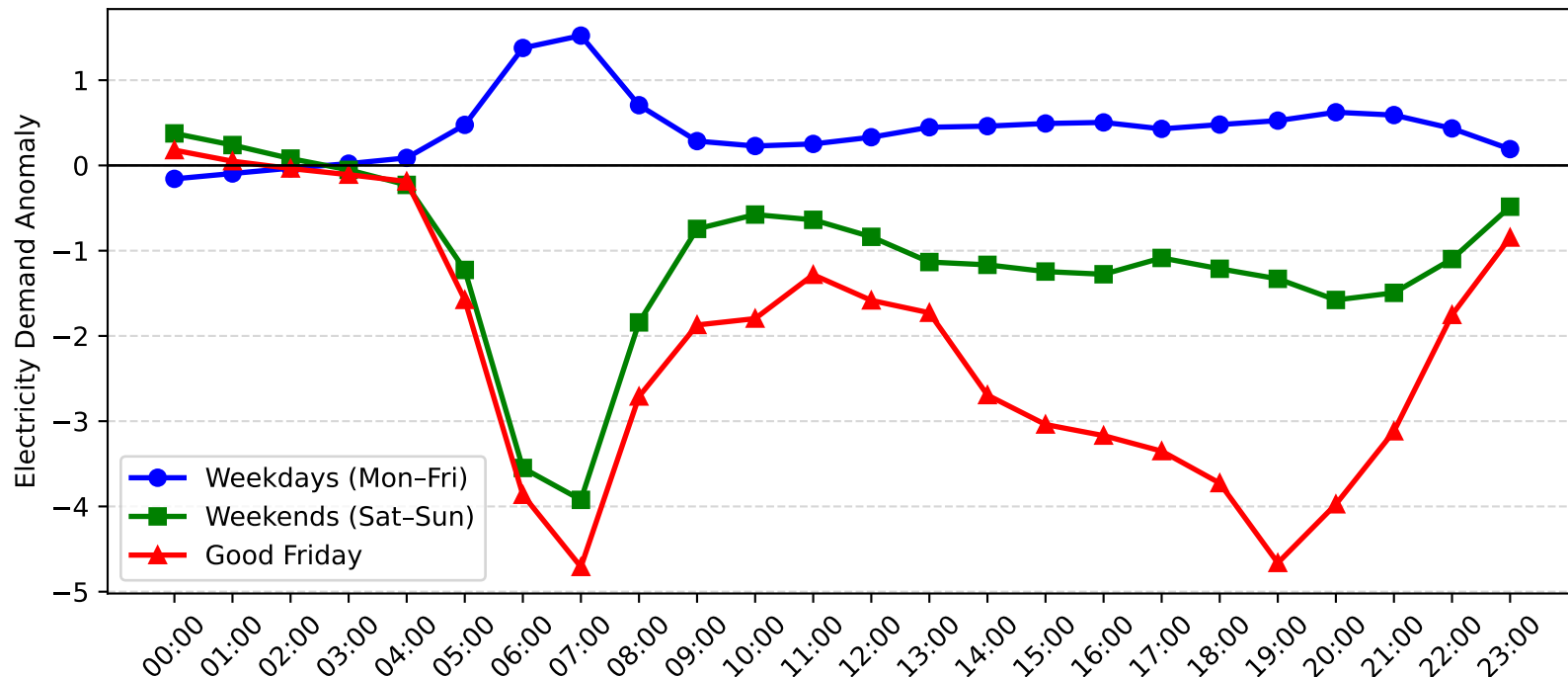
Dulwich Hill Demand Anomaly: Good Friday vs Weekday/Weekend (2011-2012)
