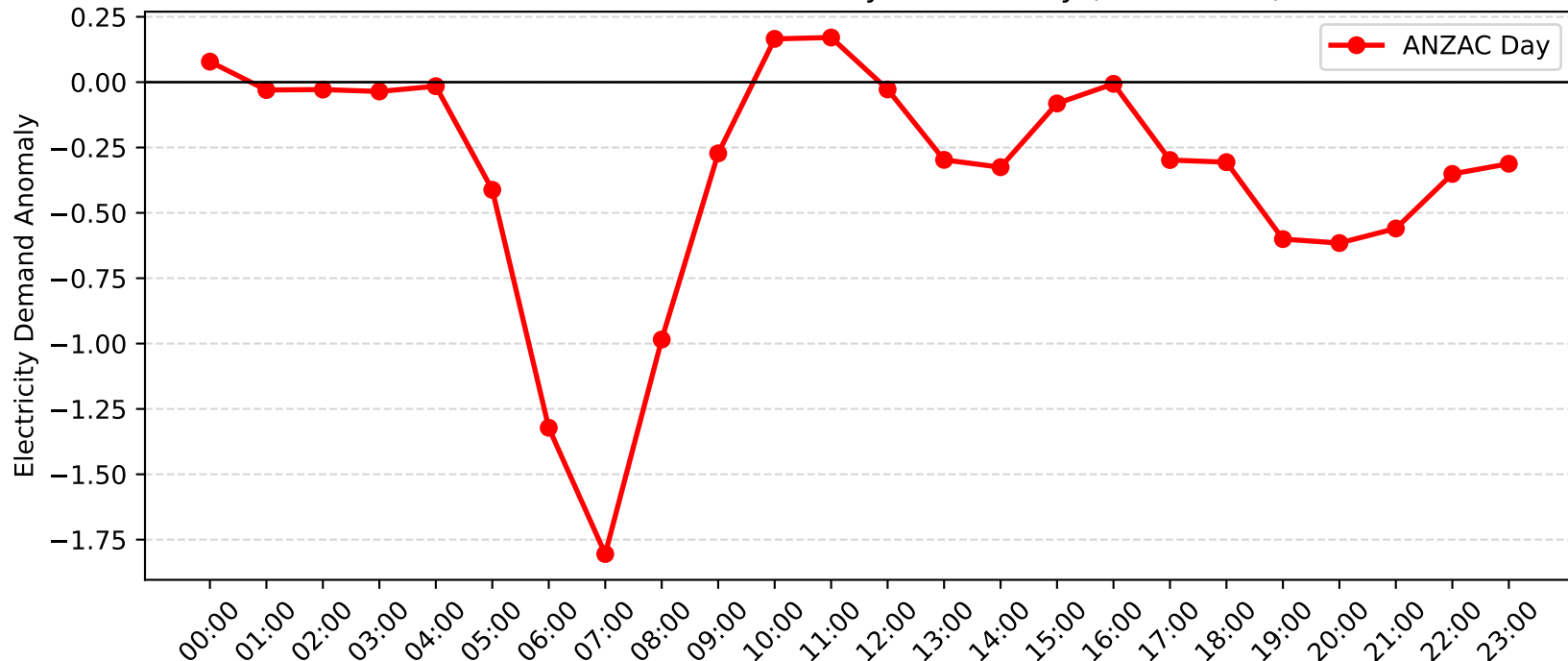
Blakehurst Demand Anomaly: ANZAC Day (2015-2016)
