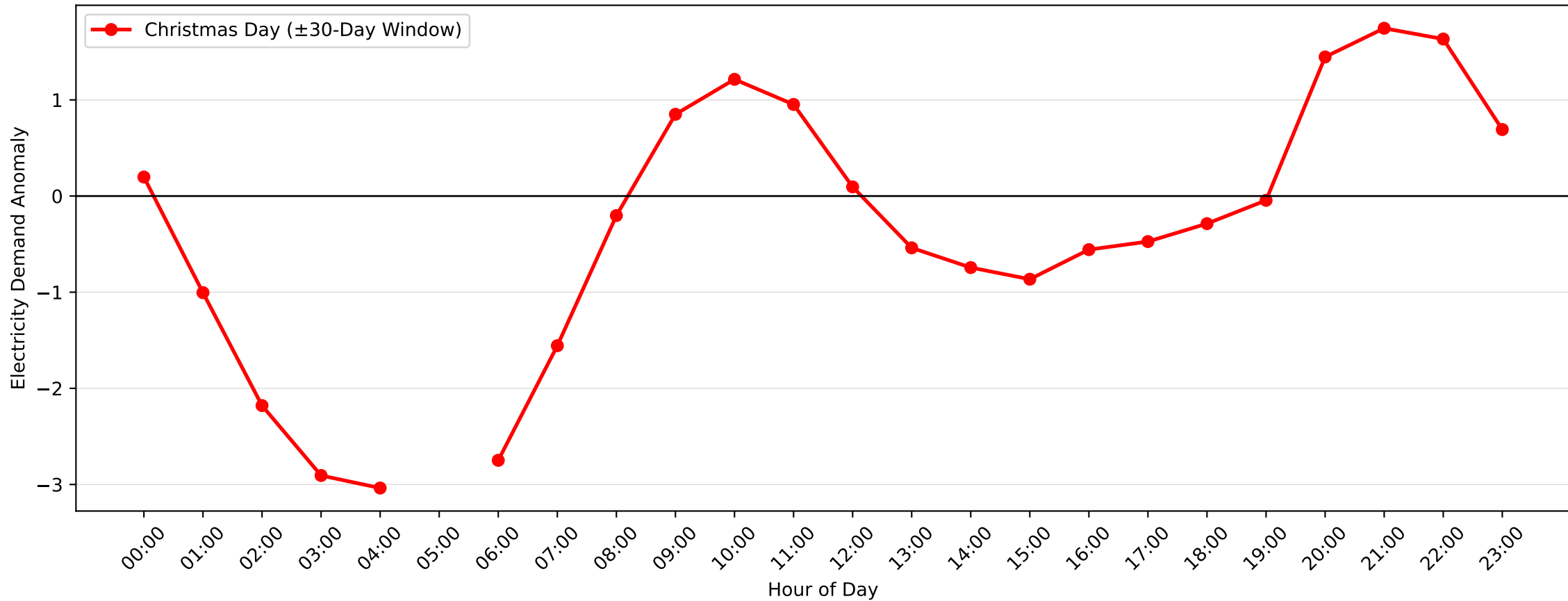
Blakehurst Demand Anomaly: Christmas Day ( \pm 30 -Day Window, 2014-2015)
