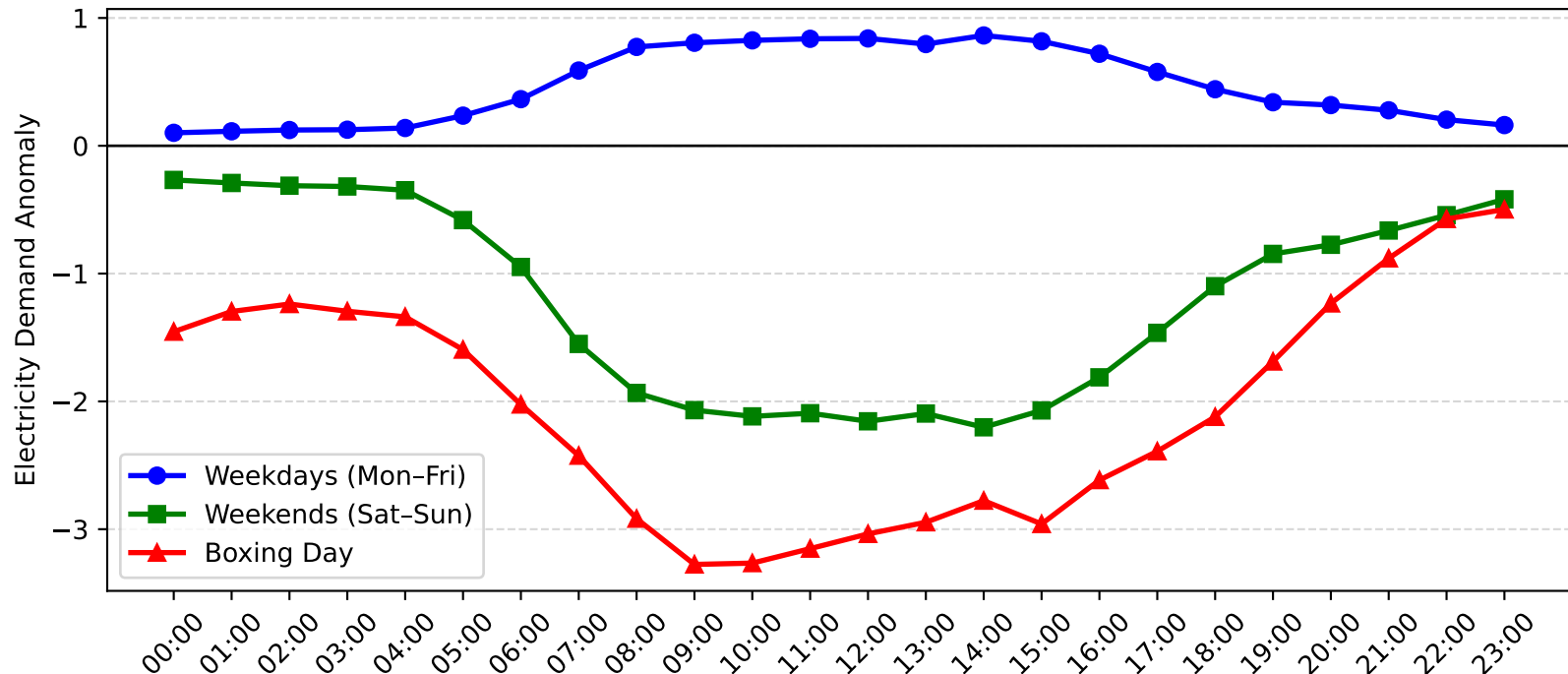
Lidcombe Demand Anomaly: Boxing Day vs Weekday/Weekend (2014-2015)
