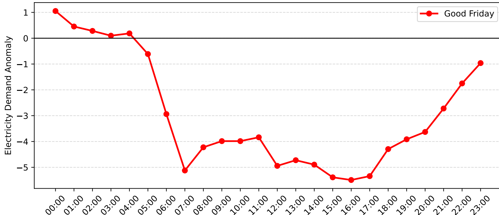
Chatswood Demand Anomaly: Good Friday (2012-2013)
