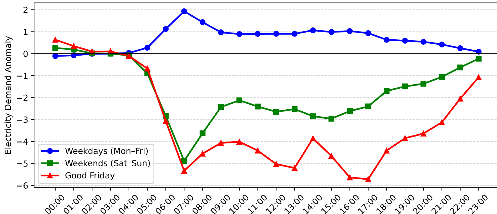
Chatswood Demand Anomaly: Good Friday vs Weekday/Weekend (2013-2014)
