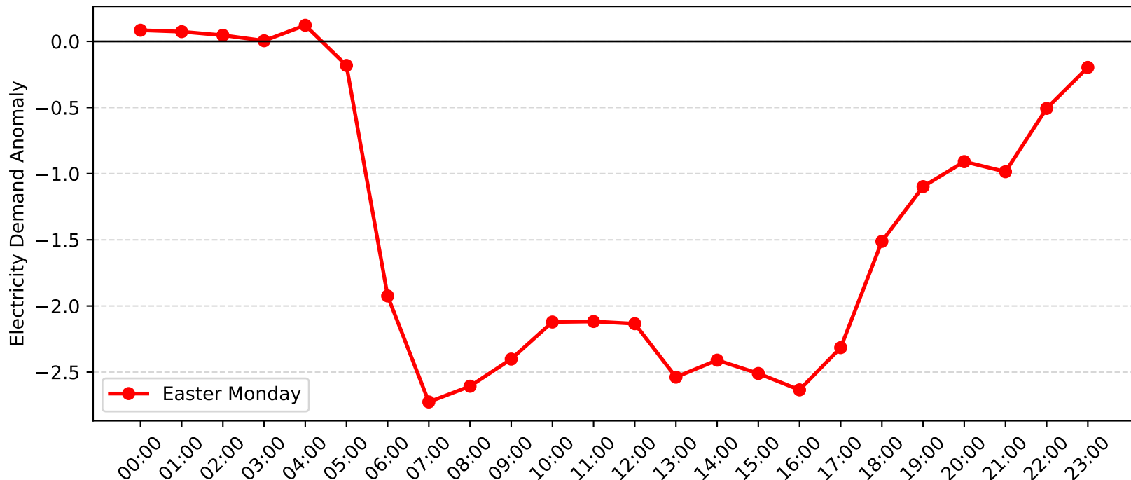
Pymble Demand Anomaly: Easter Monday (2007-2008)
