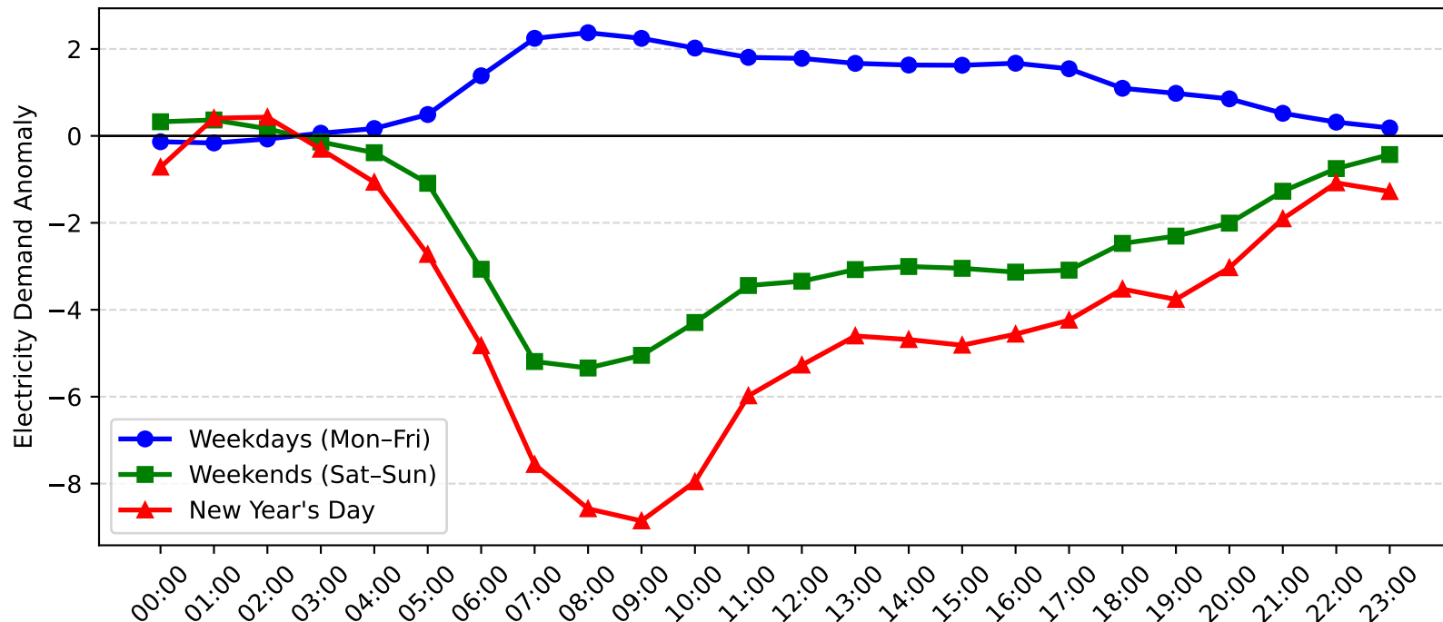
Burwood Demand Anomaly: New Year's Day vs Weekday/Weekend (2011-2012)
