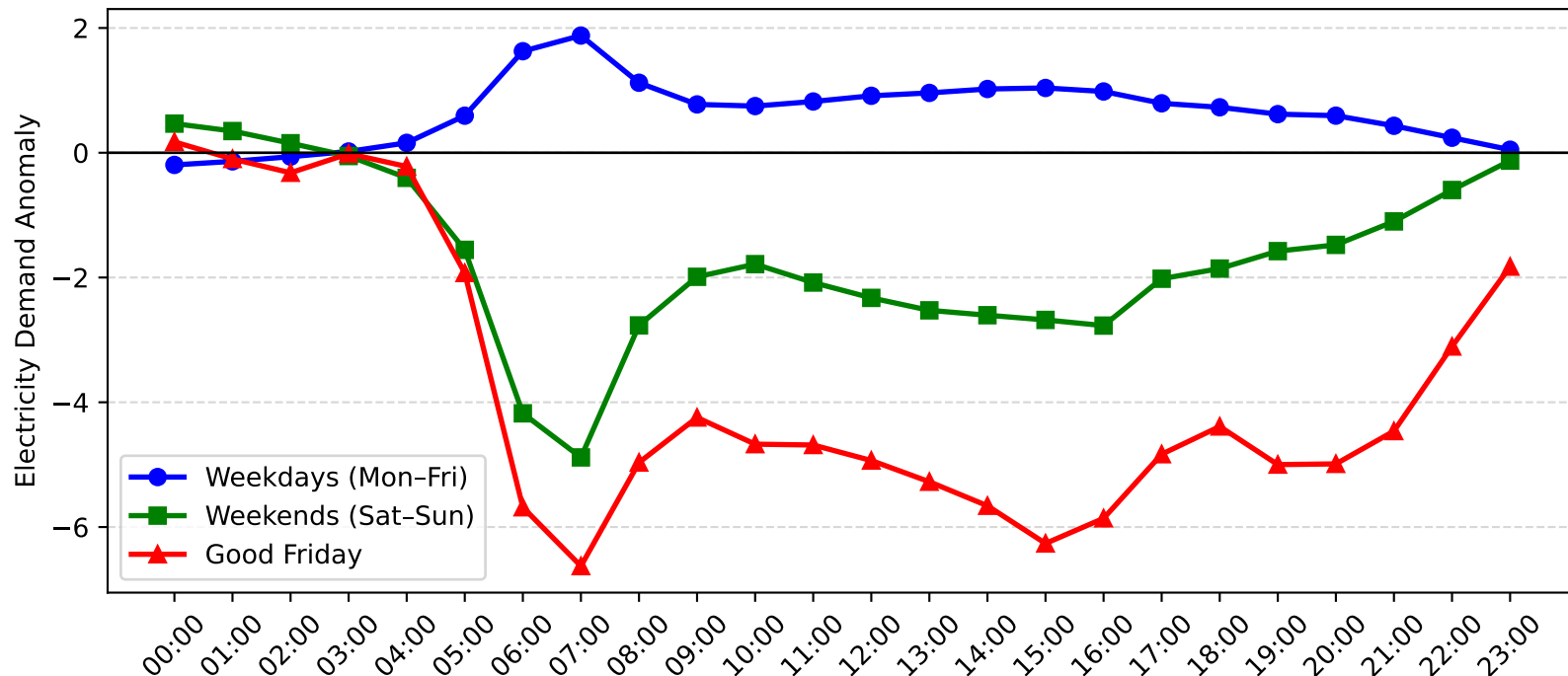
Dulwich Hill Demand Anomaly: Good Friday vs Weekday/Weekend (2006-2007)
