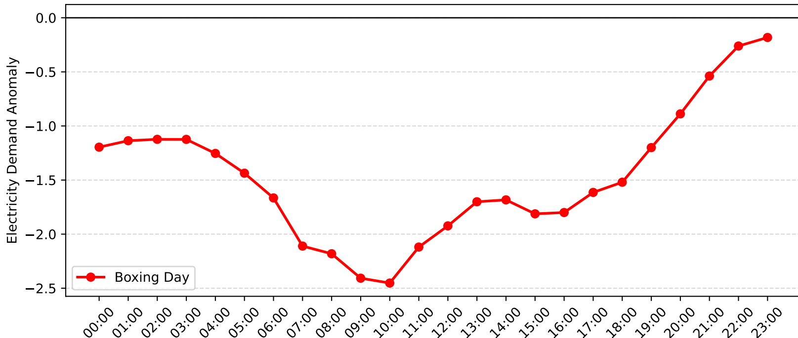
Lidcombe Demand Anomaly: Boxing Day (2015-2016)
