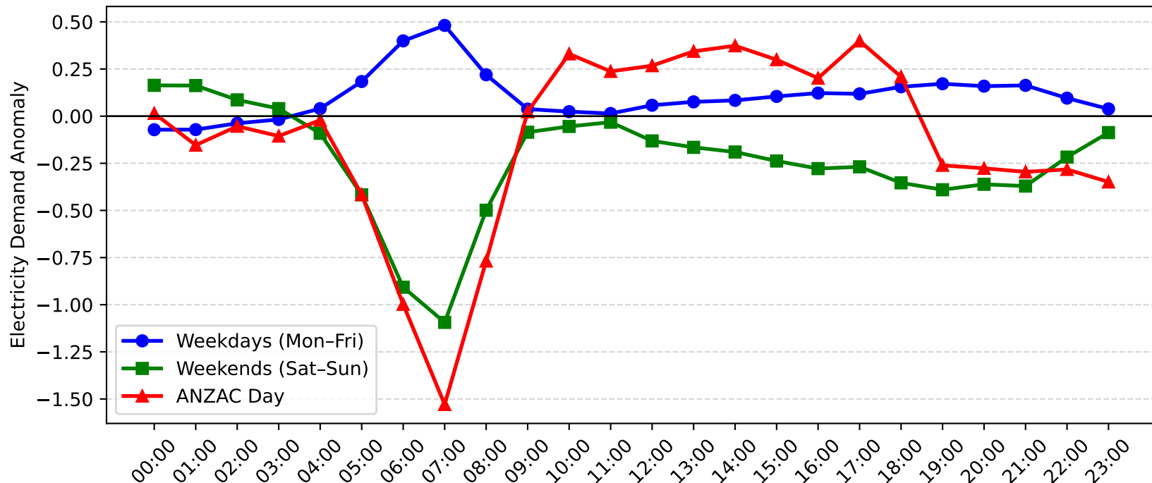
Blakehurst Demand Anomaly: ANZAC Day vs Weekday/Weekend (2017-2018)
