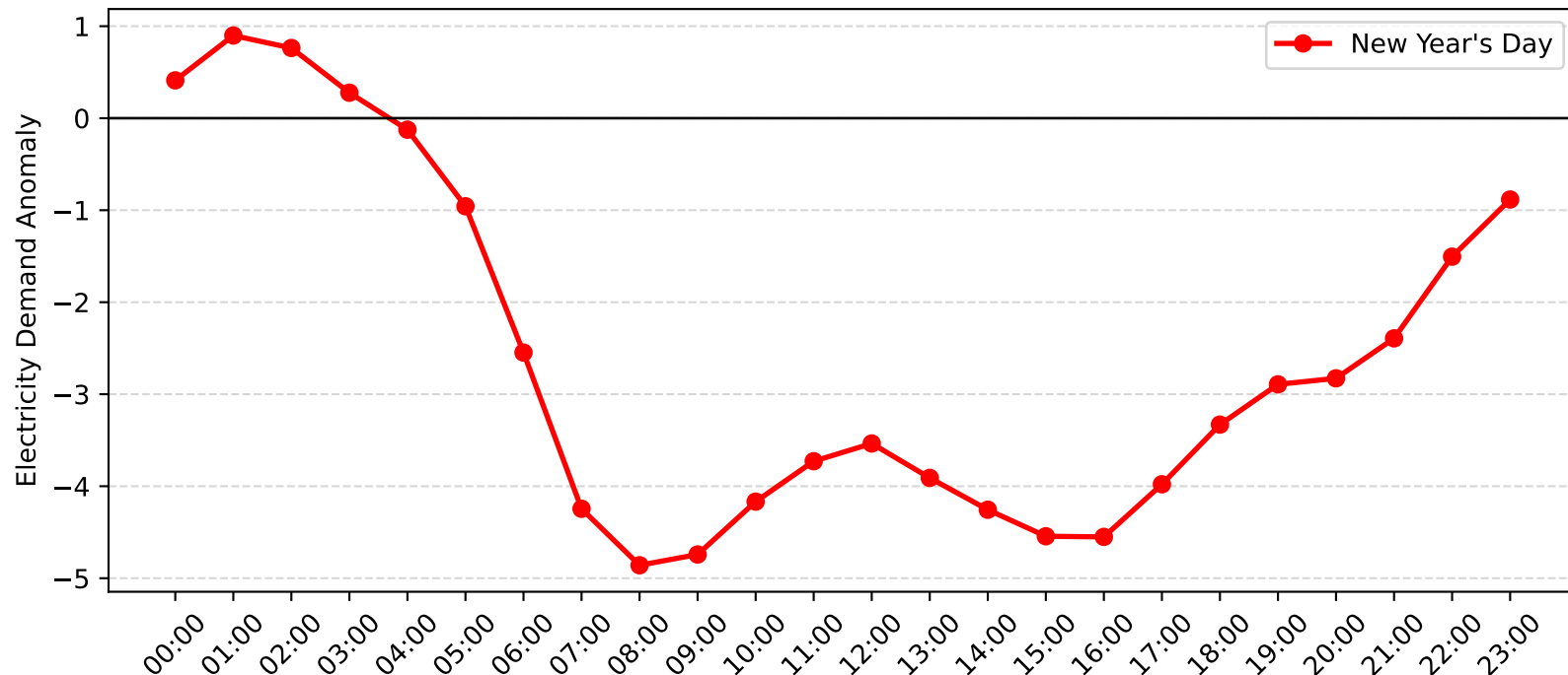
Five Dock Demand Anomaly: New Year's Day (2016-2017)
