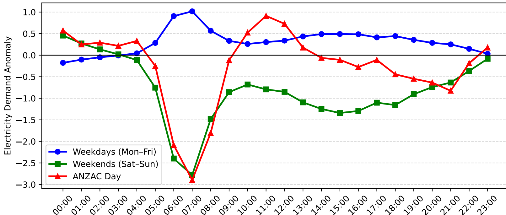
Blakehurst Demand Anomaly: ANZAC Day vs Weekday/Weekend (2007-2008)
