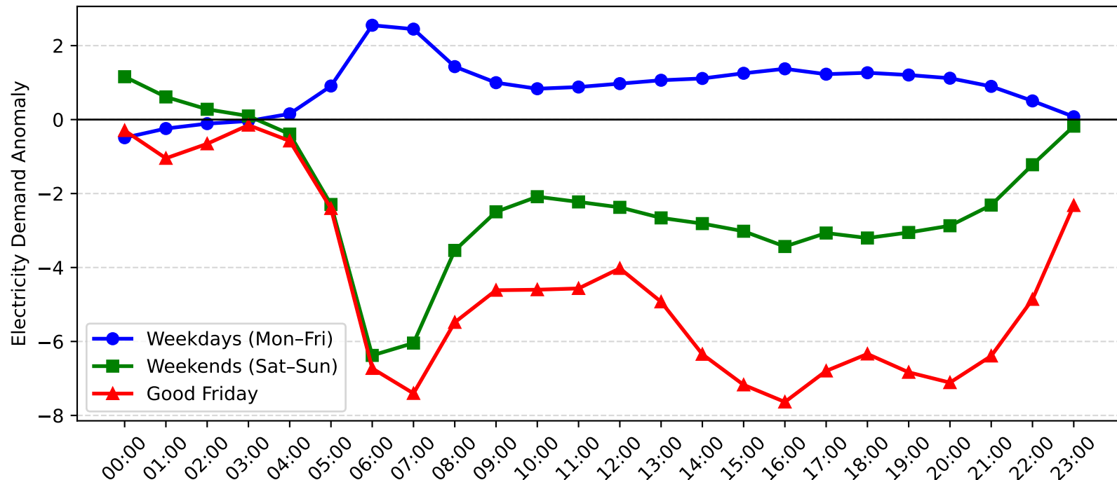
Pennant Hills Demand Anomaly: Good Friday vs Weekday/Weekend (2008-2009)
