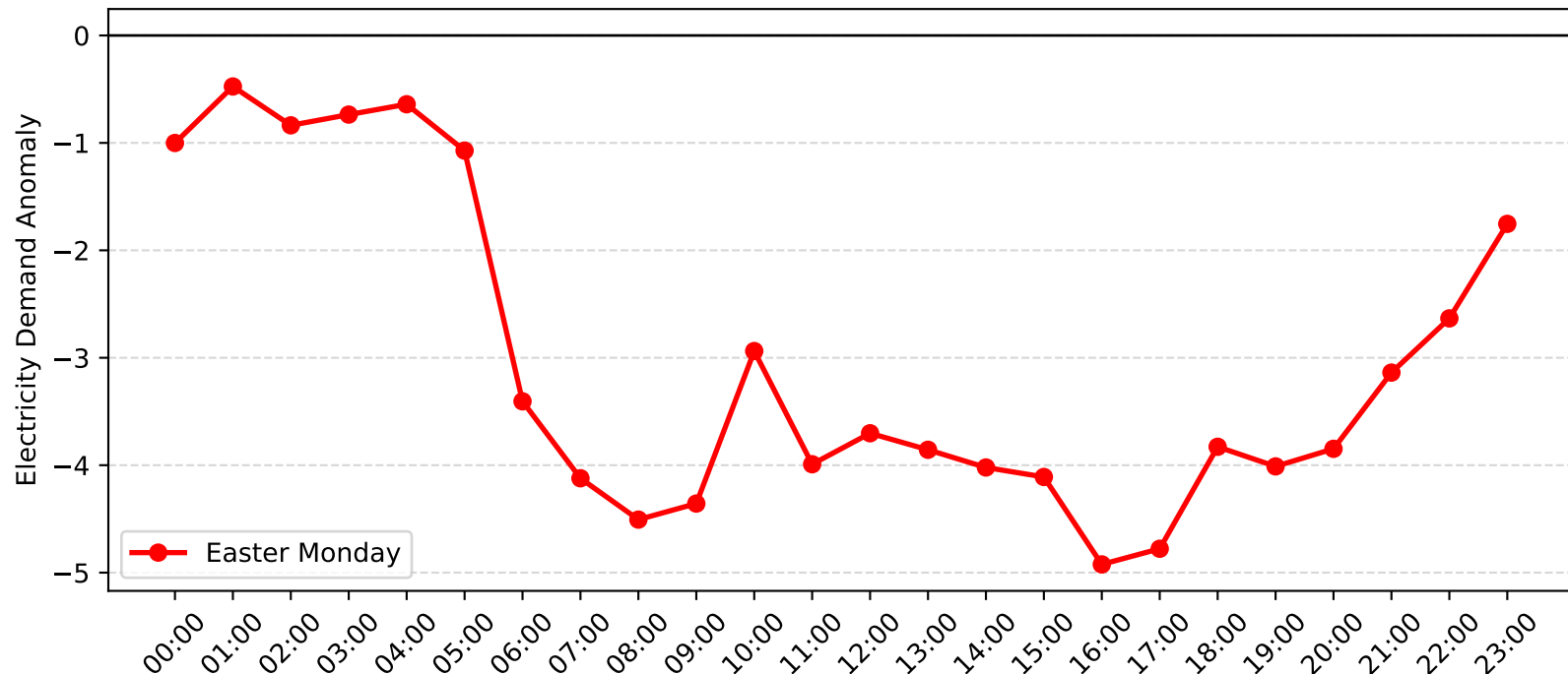
Epping Demand Anomaly: Easter Monday (2006-2007)
