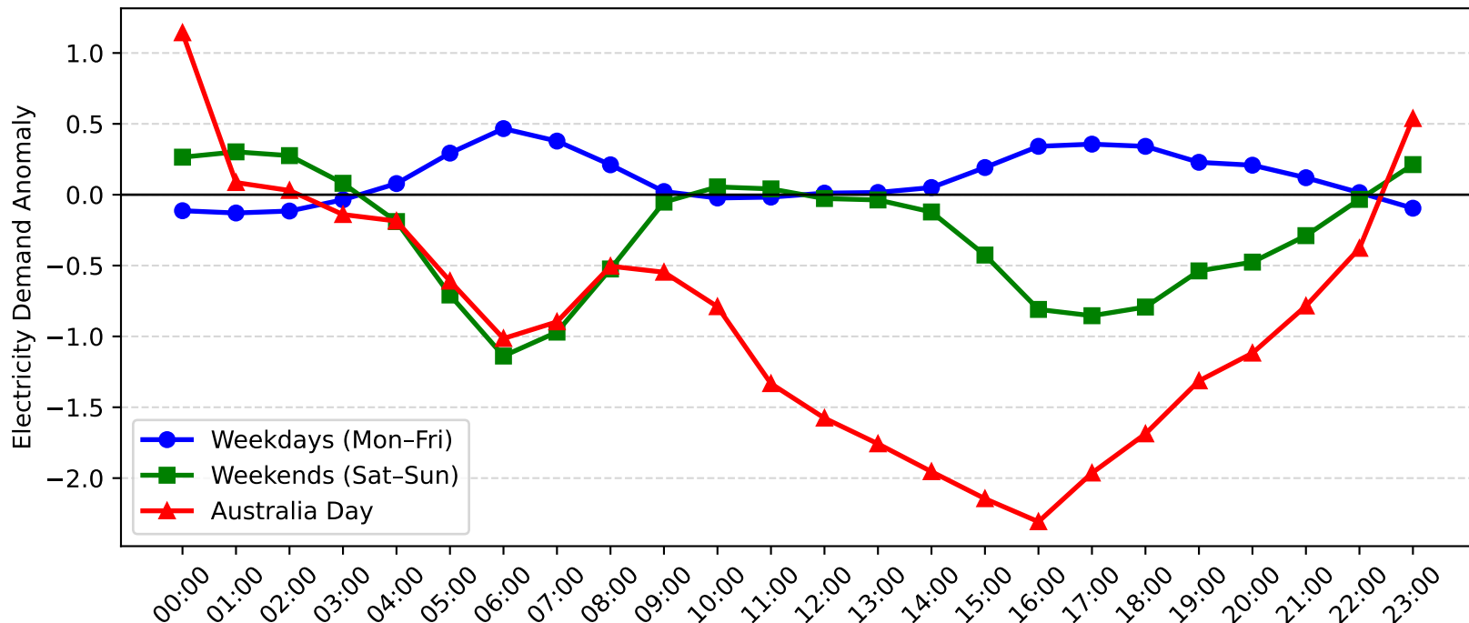
Woy Woy Demand Anomaly: Australia Day vs Weekday/Weekend (2008-2009)
