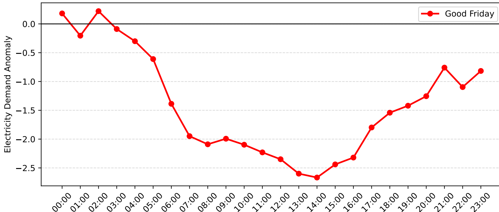
Gateshead Demand Anomaly: Good Friday (2009-2010)
