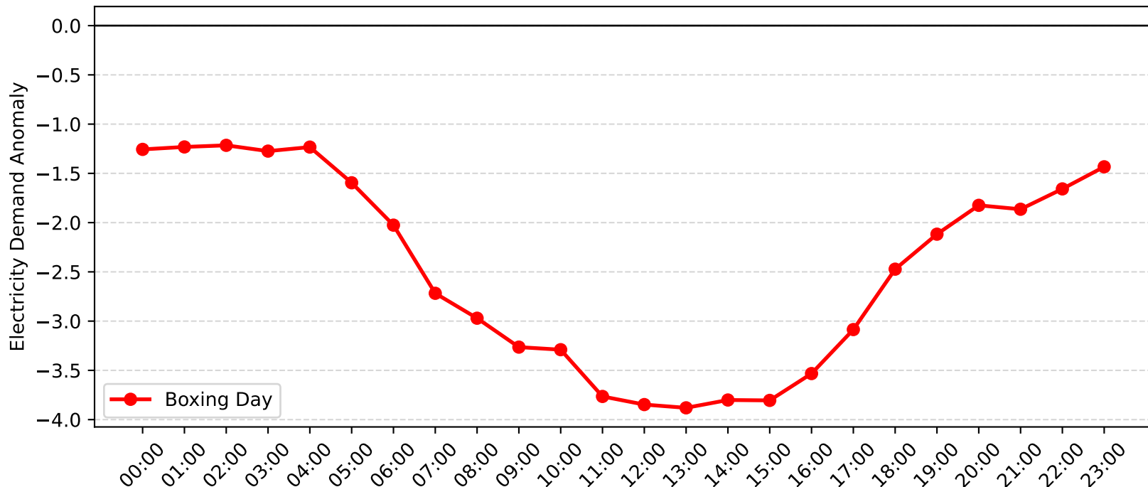
Lidcombe Demand Anomaly: Boxing Day (2011-2012)
