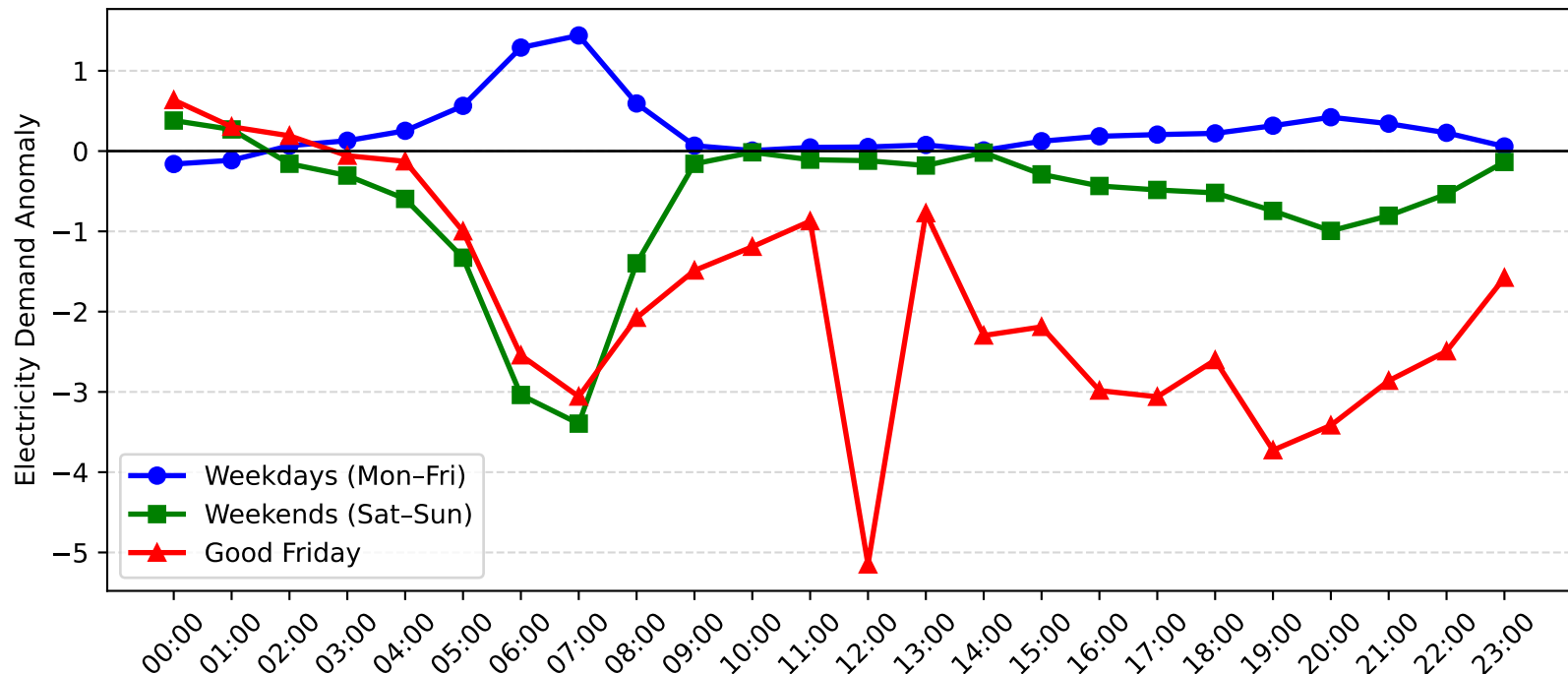
Dulwich Hill Demand Anomaly: Good Friday vs Weekday/Weekend (2017-2018)
