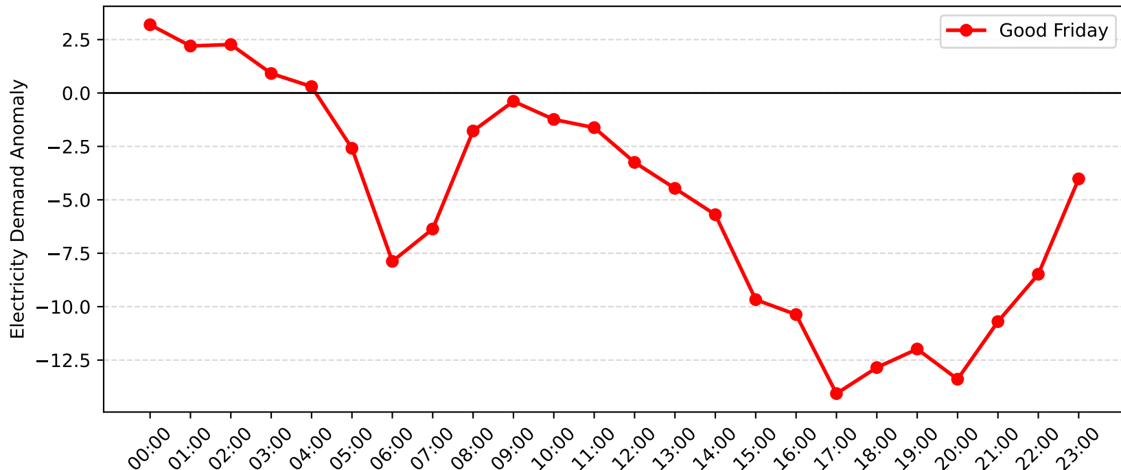
Pennant Hills Demand Anomaly: Good Friday (2004-2005)
