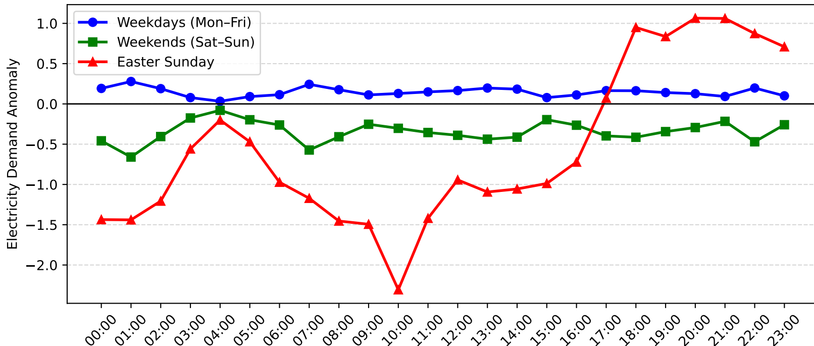
Gateshead Demand Anomaly: Easter Sunday vs Weekday/Weekend (2004-2005)
