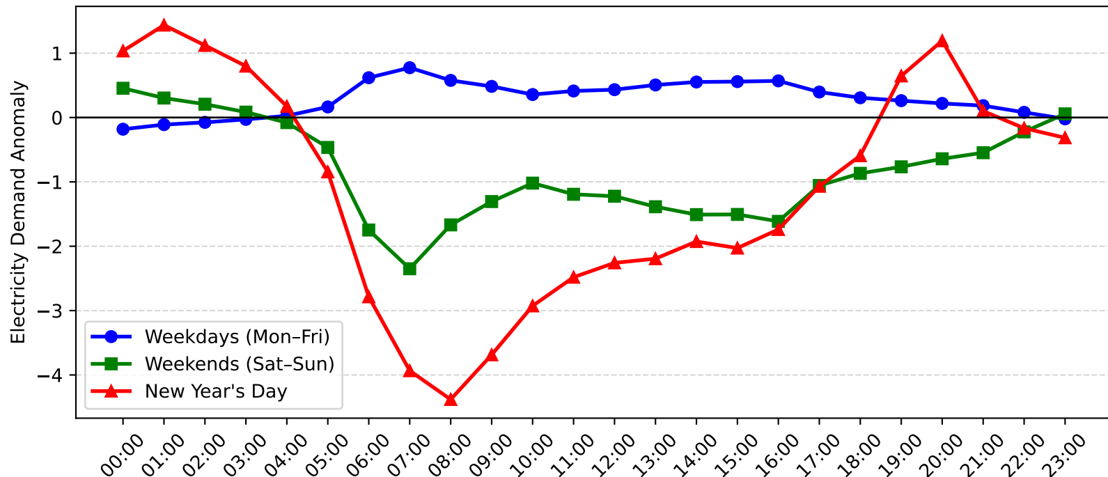
Five Dock Demand Anomaly: New Year's Day vs Weekday/Weekend (2008-2009)
