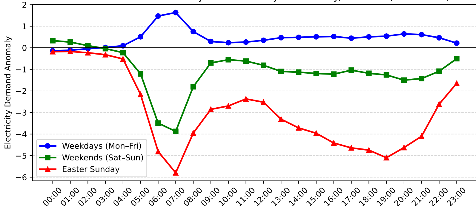
Dulwich Hill Demand Anomaly: Easter Sunday vs Weekday/Weekend (2011-2012)
