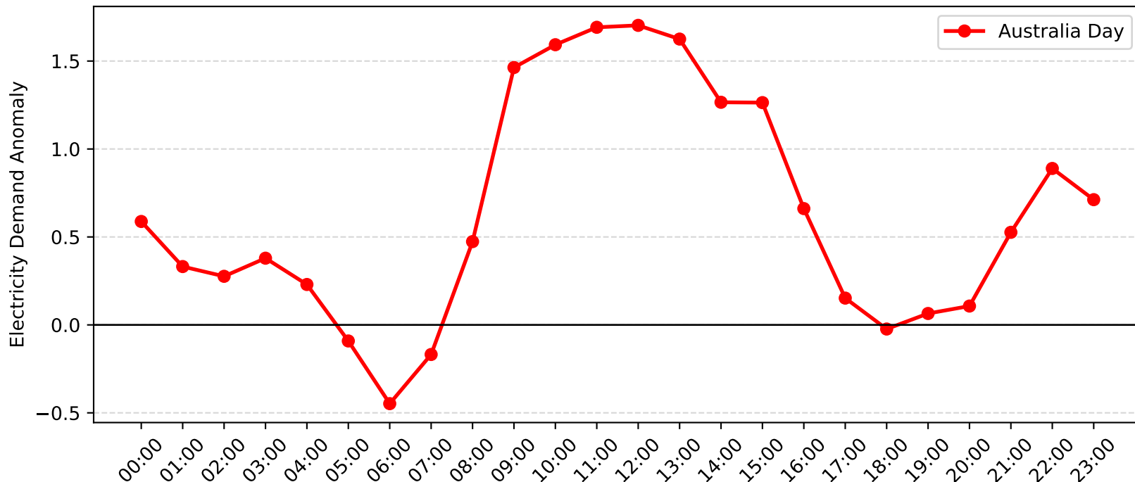
Woy Woy Demand Anomaly: Australia Day (2012-2013)
