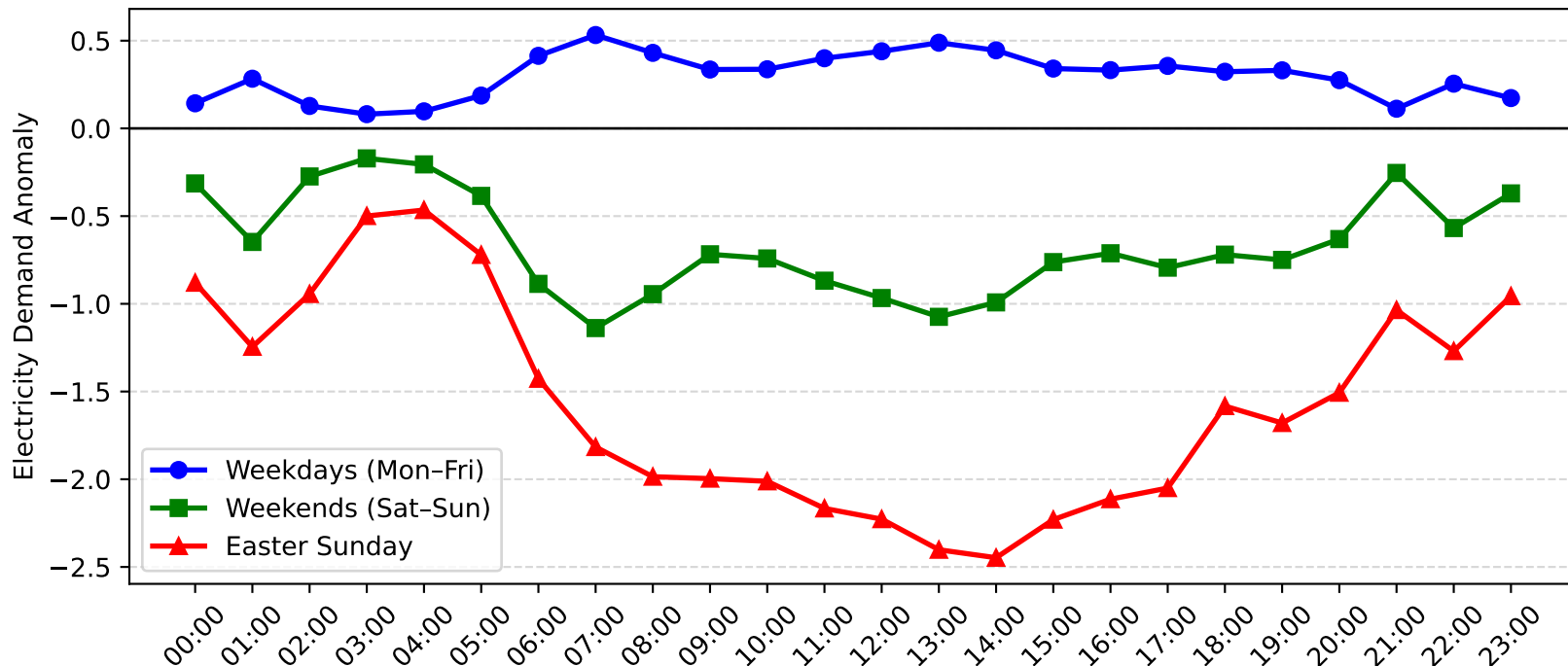
Gateshead Demand Anomaly: Easter Sunday vs Weekday/Weekend (2010-2011)
