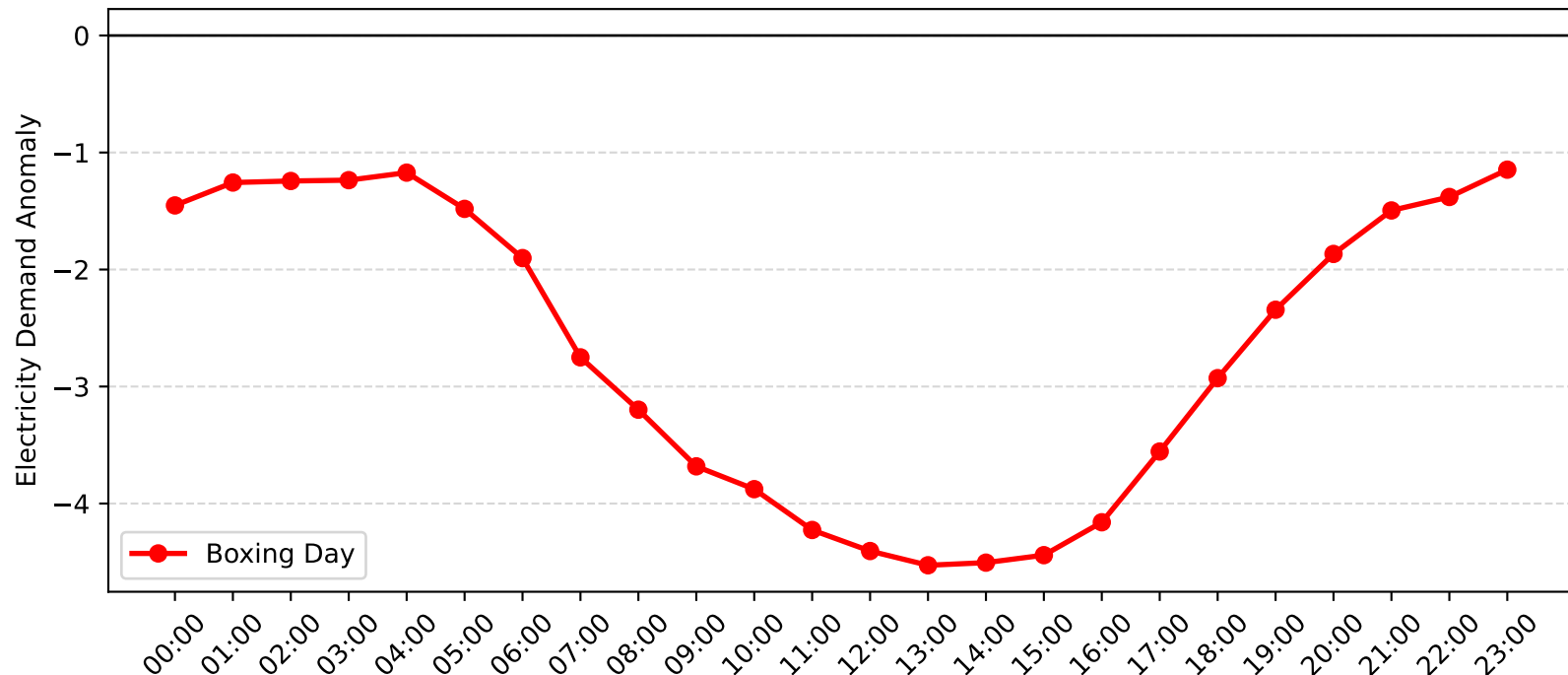
Lidcombe Demand Anomaly: Boxing Day (2012-2013)
