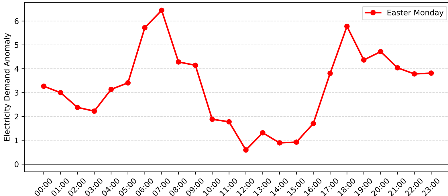
Matraville Demand Anomaly: Easter Monday (2004-2005)
