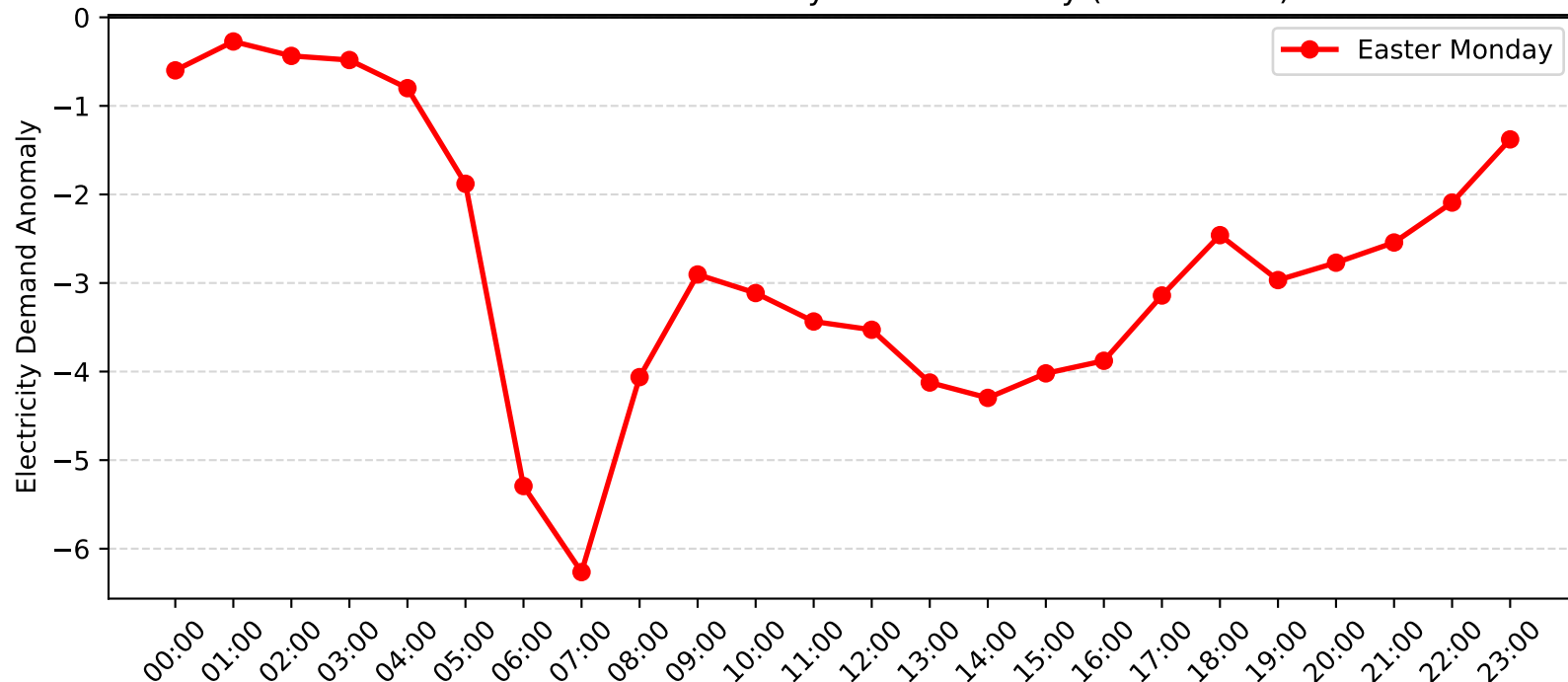
Mortdale Demand Anomaly: Easter Monday (2006-2007)
