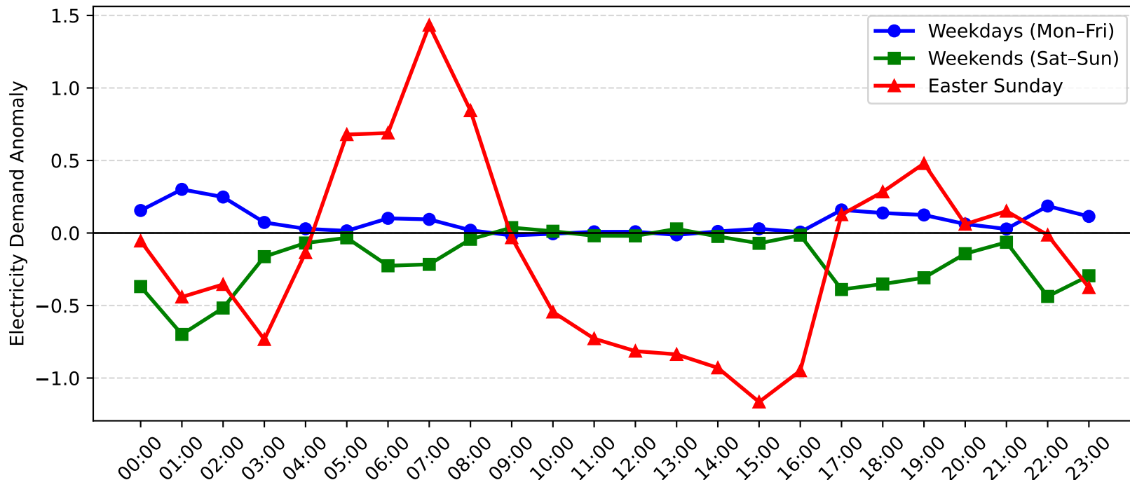
Jewells Demand Anomaly: Easter Sunday vs Weekday/Weekend (2004-2005)
