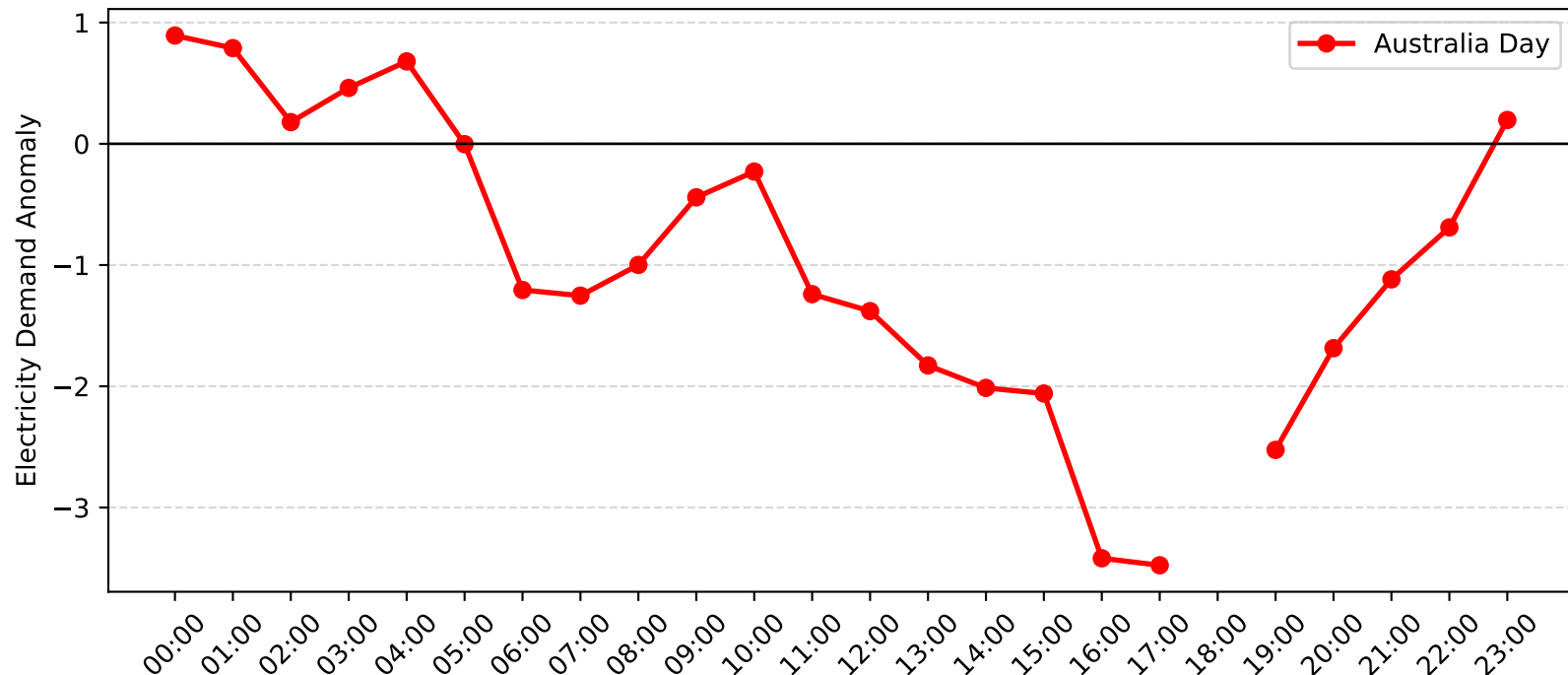
Erina Demand Anomaly: Australia Day (2005-2006)
