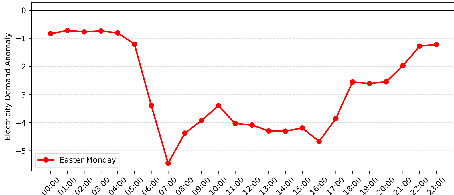
Epping Demand Anomaly: Easter Monday (2013-2014)
