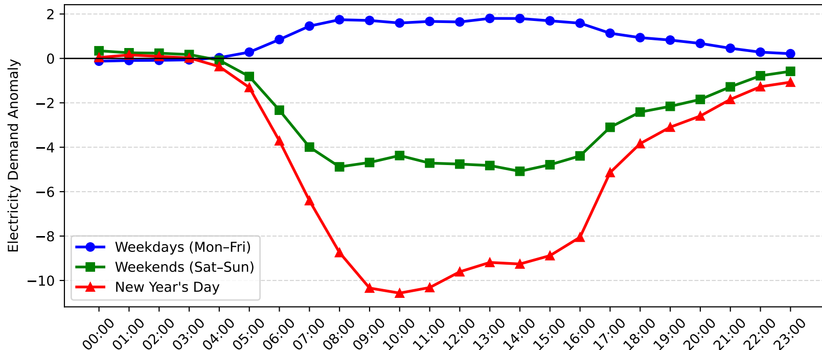
Brookvale Demand Anomaly: New Year's Day vs Weekday/Weekend (2013-2014)
