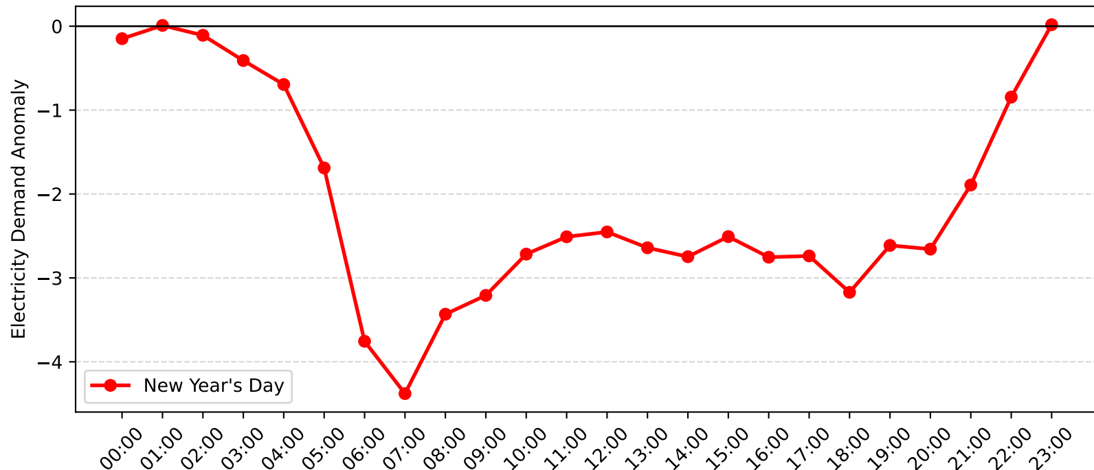
Five Dock Demand Anomaly: New Year's Day (2004-2005)
