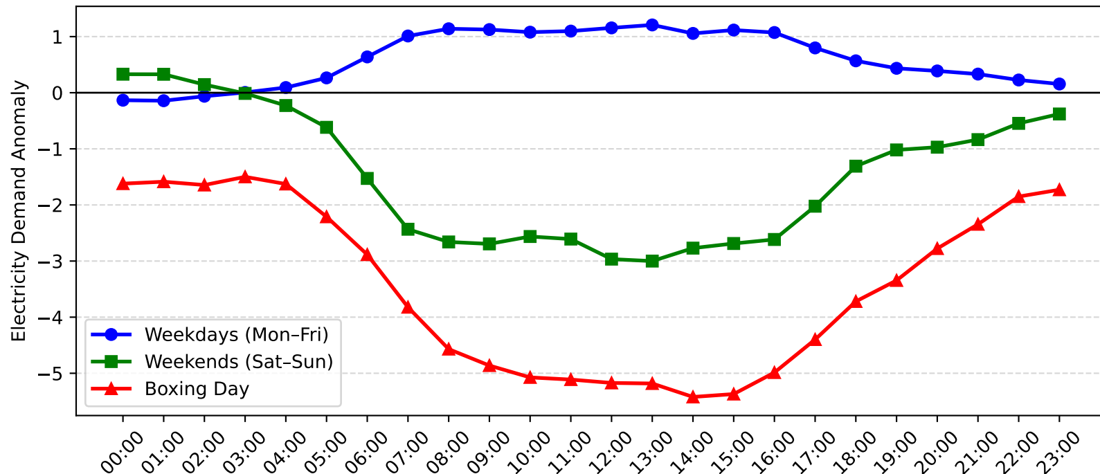
Lidcombe Demand Anomaly: Boxing Day vs Weekday/Weekend (2005-2006)
