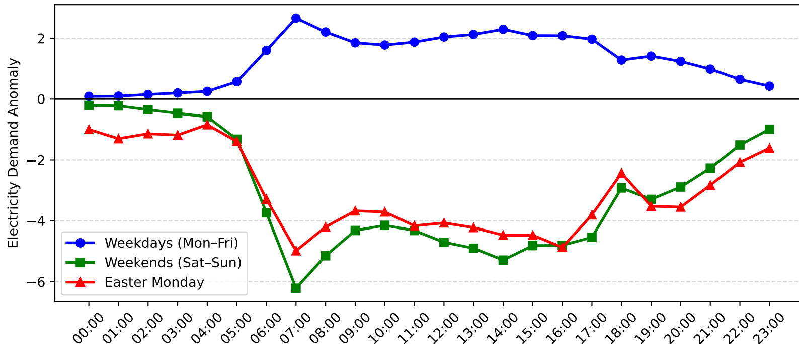
Epping Demand Anomaly: Easter Monday vs Weekday/Weekend (2014-2015)
