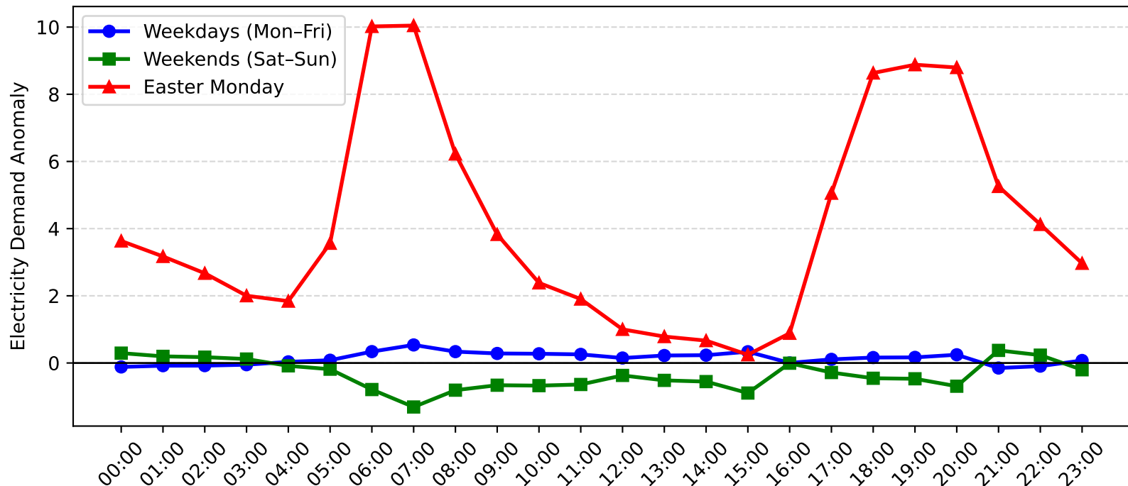
Mortdale Demand Anomaly: Easter Monday vs Weekday/Weekend (2004-2005)
