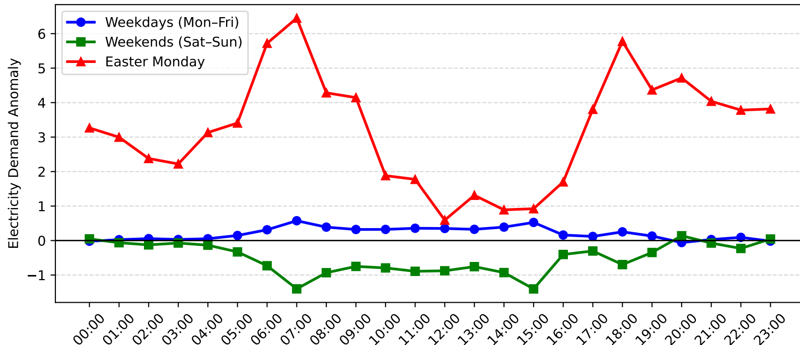
Matraverse Demand Anomaly: Easter Monday vs Weekday/Weekend (2004-2005)
