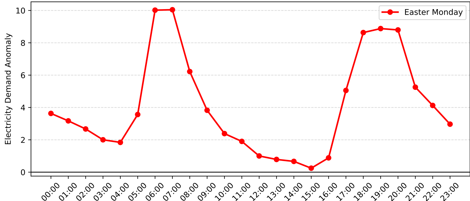
Mortdale Demand Anomaly: Easter Monday (2004-2005)
