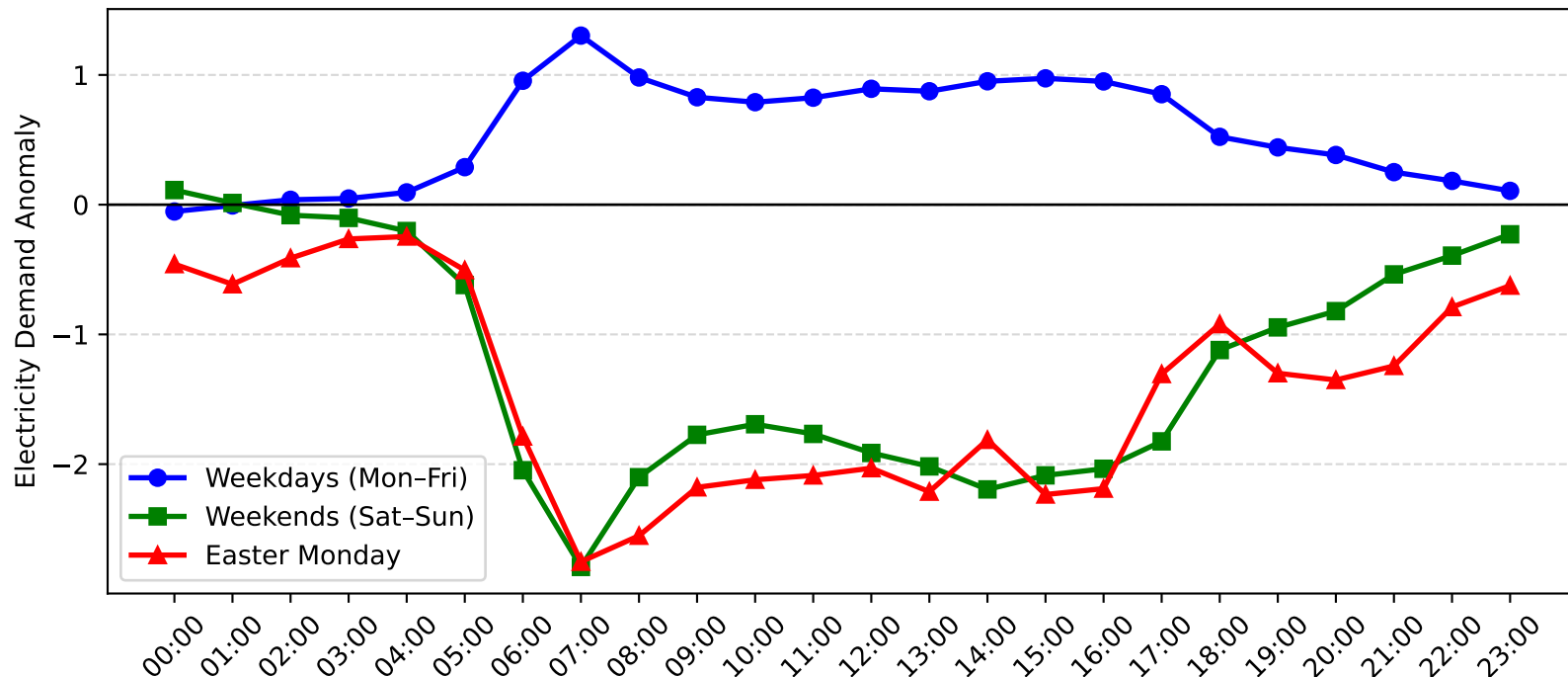
Pymble Demand Anomaly: Easter Monday vs Weekday/Weekend (2017-2018)
