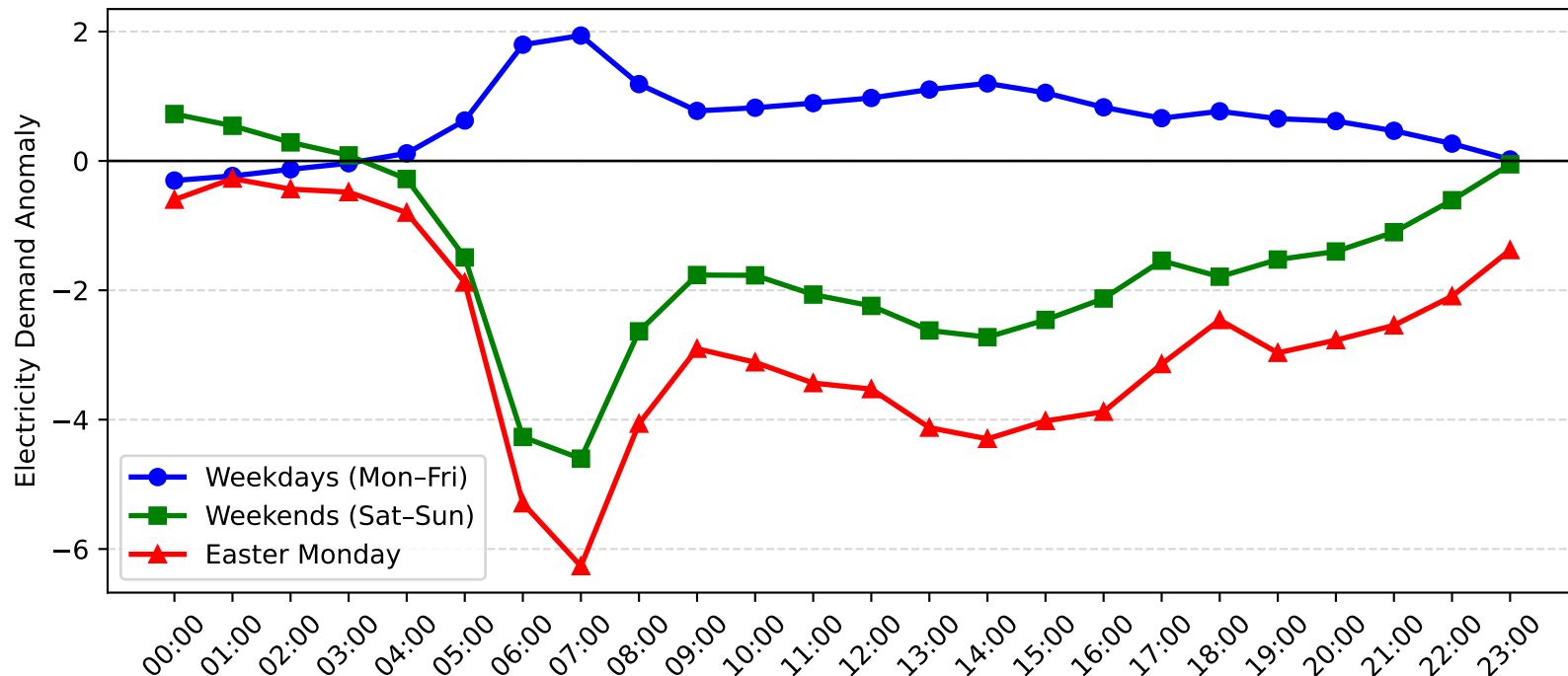
Mortdale Demand Anomaly: Easter Monday vs Weekday/Weekend (2006-2007)
