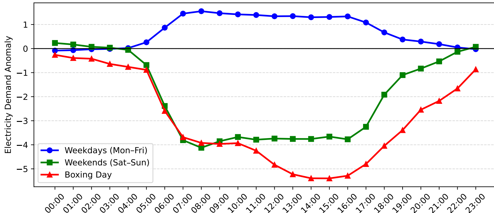
Pymble Demand Anomaly: Boxing Day vs Weekday/Weekend (2006-2007)
