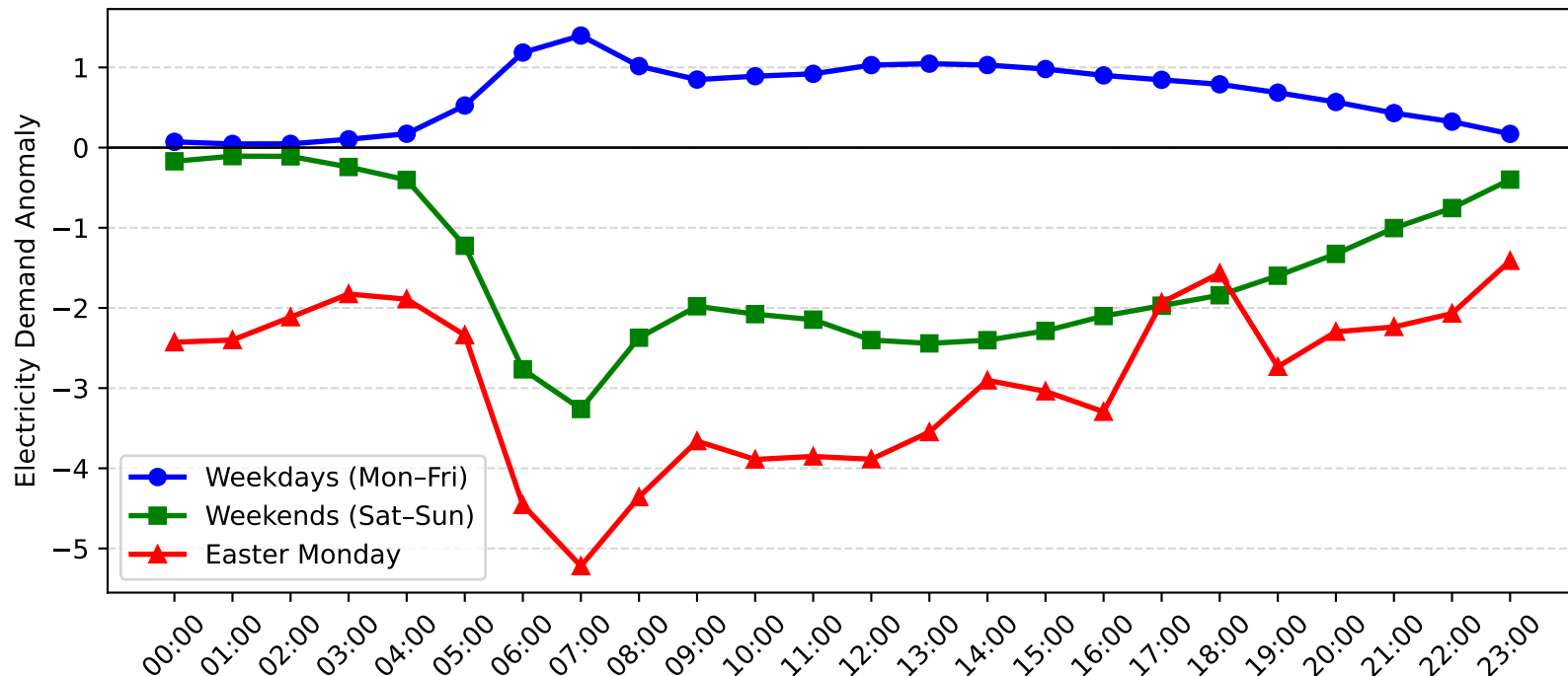
Matraverse Demand Anomaly: Easter Monday vs Weekday/Weekend (2014-2015)
