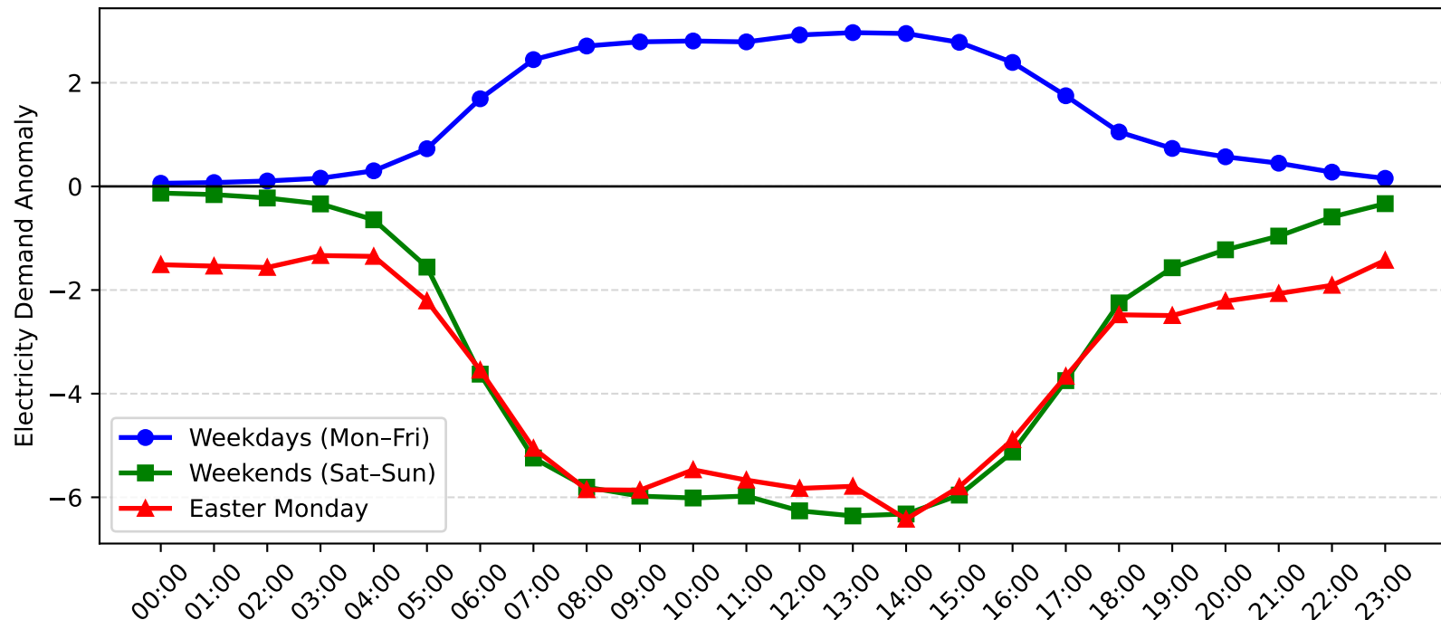
Mascot Demand Anomaly: Easter Monday vs Weekday/Weekend (2017-2018)
