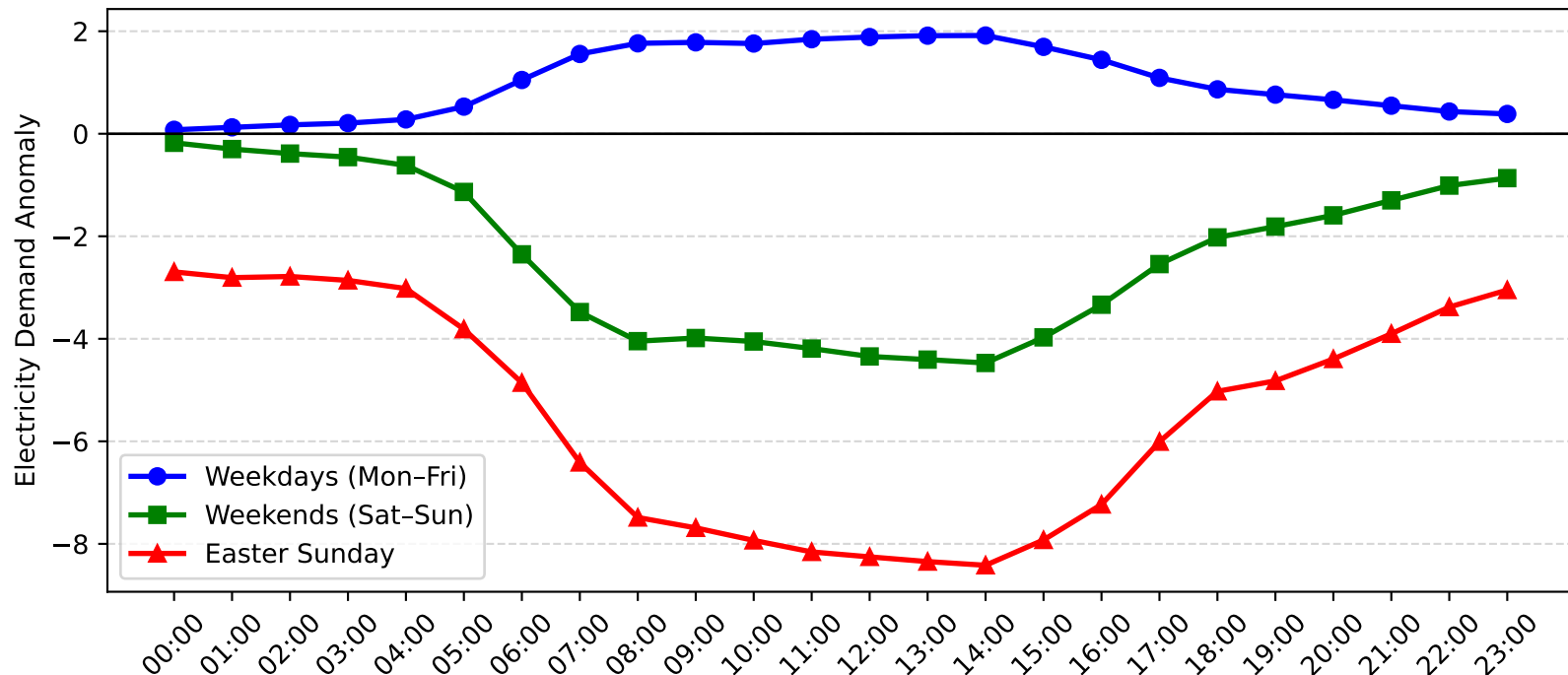
Caringbah Demand Anomaly: Easter Sunday vs Weekday/Weekend (2010-2011)
