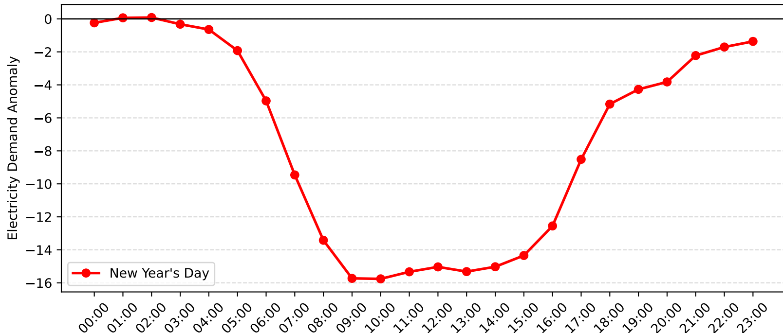
Brookvale Demand Anomaly: New Year's Day (2007-2008)
