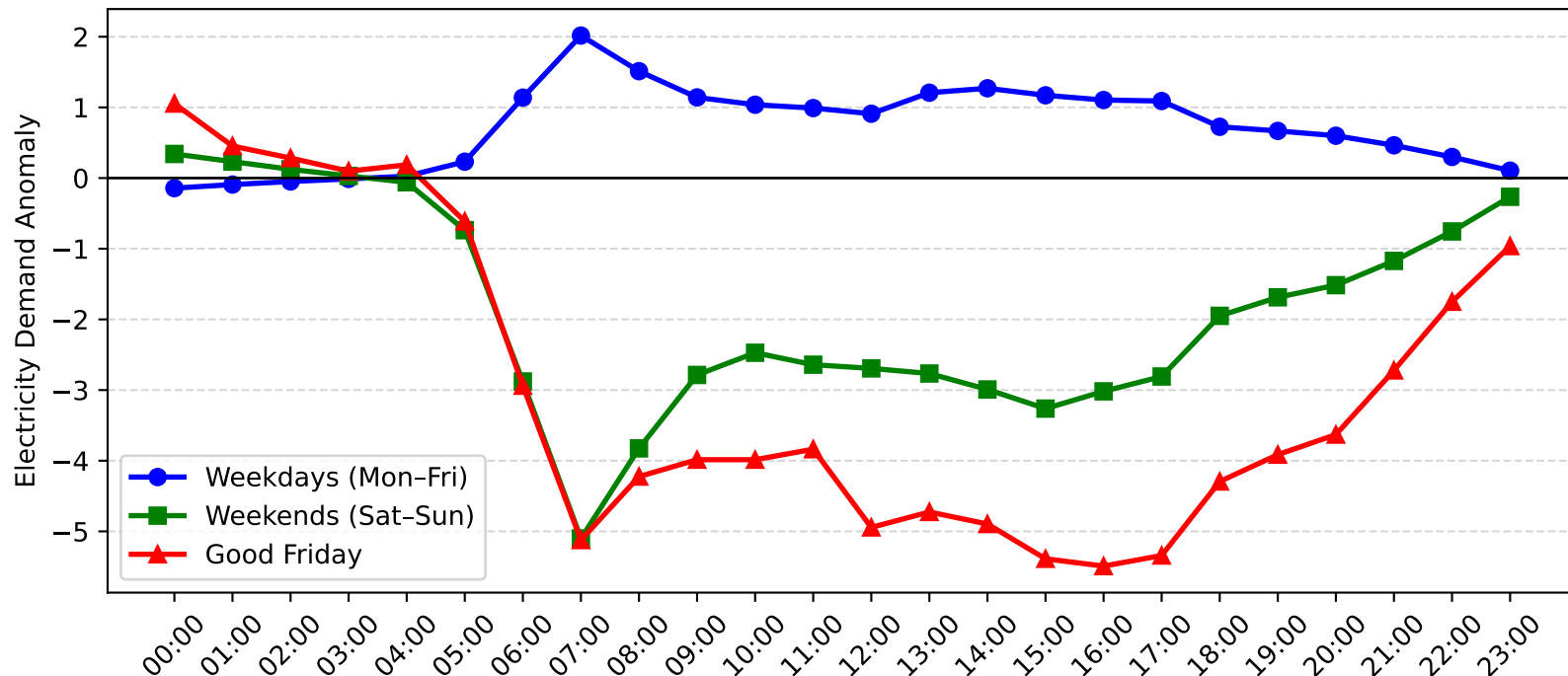
Chatswood Demand Anomaly: Good Friday vs Weekday/Weekend (2012-2013)
