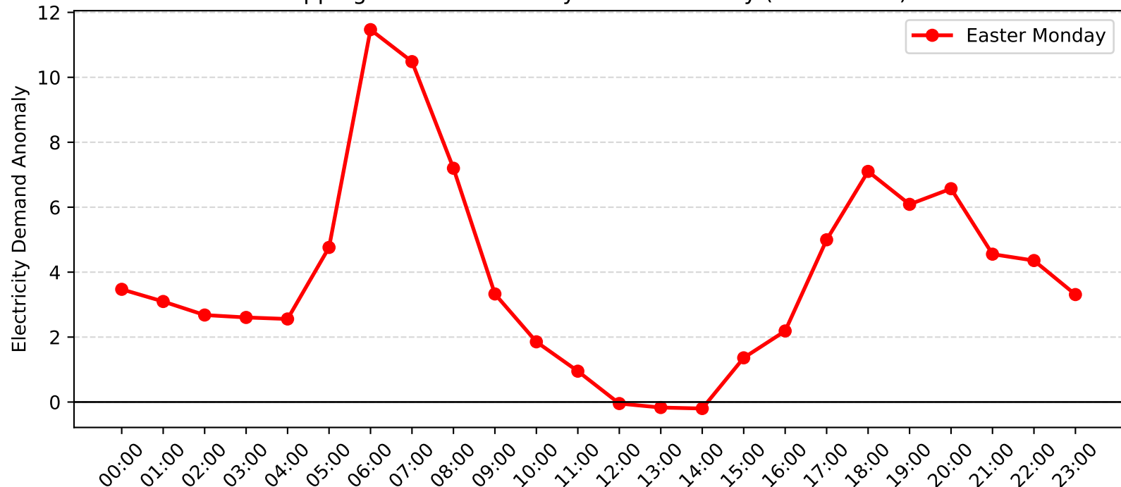
Epping Demand Anomaly: Easter Monday (2004-2005)
