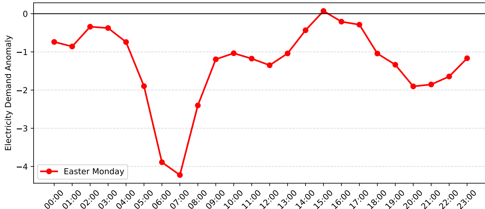
Cronulla Demand Anomaly: Easter Monday (2015-2016)
