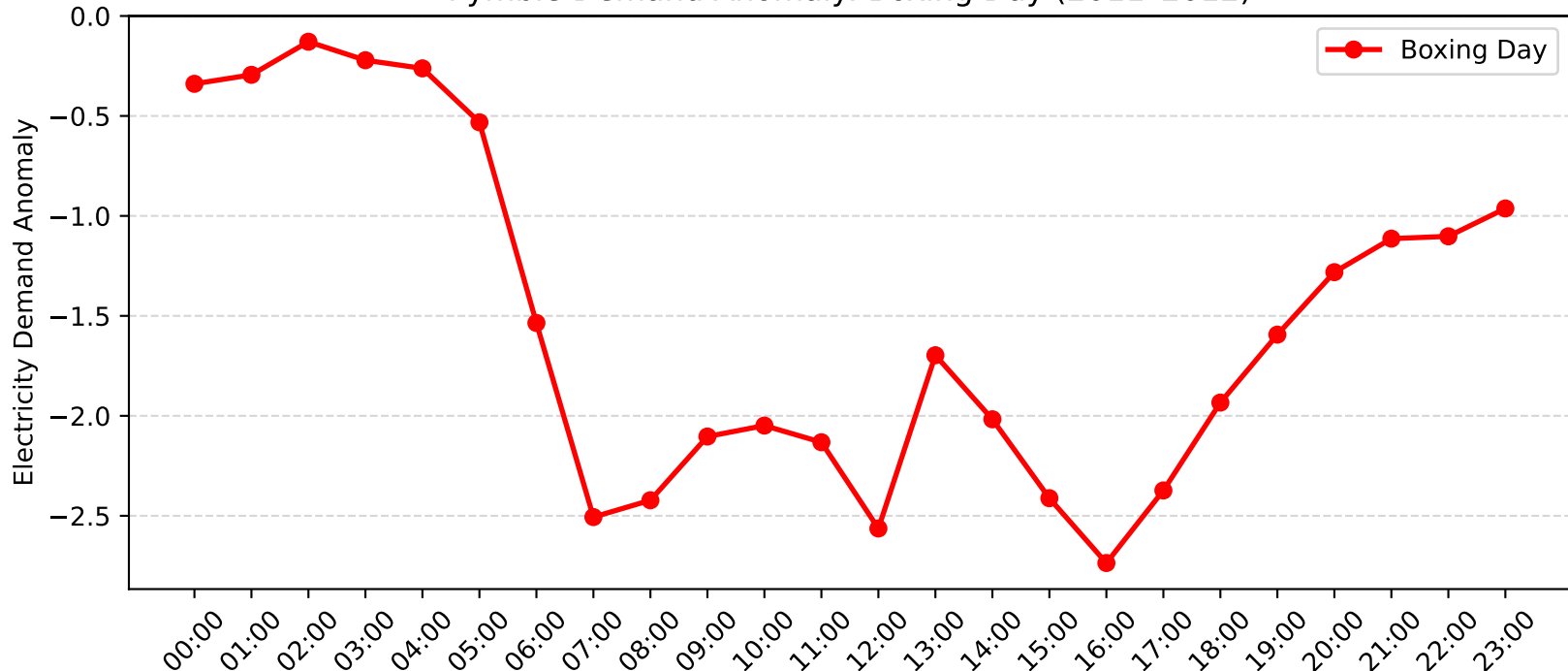
Pymble Demand Anomaly: Boxing Day (2011-2012)
