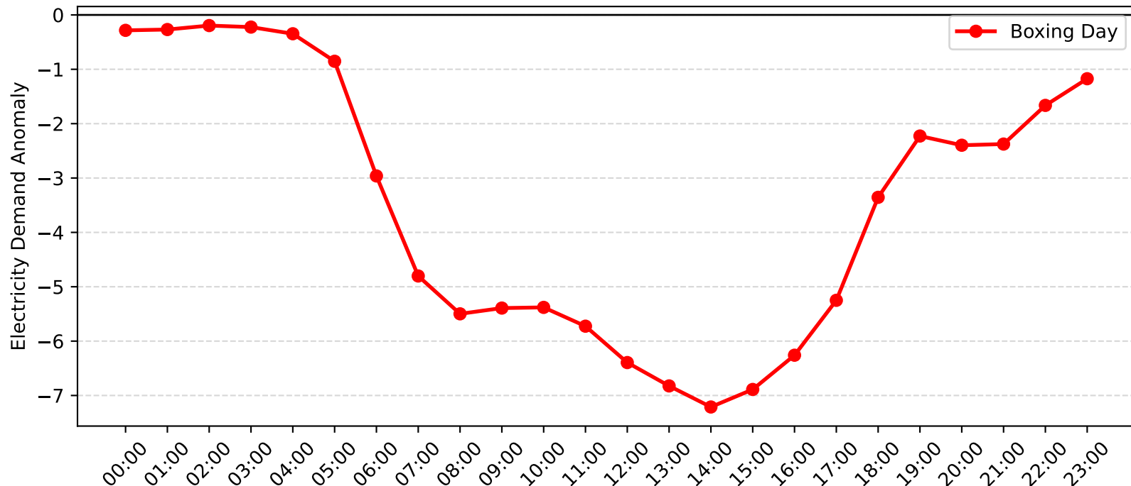
Pymble Demand Anomaly: Boxing Day (2009-2010)
