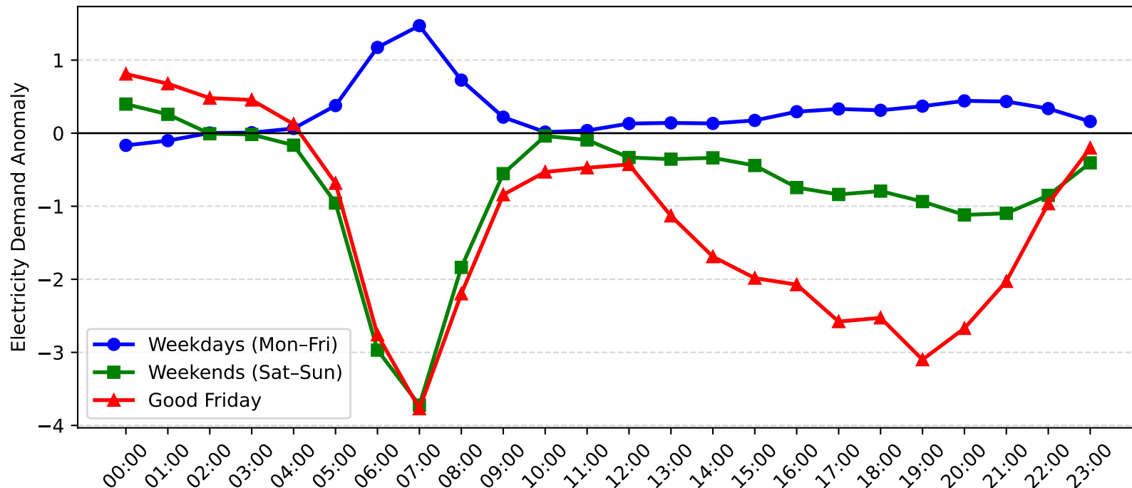
Dulwich Hill Demand Anomaly: Good Friday vs Weekday/Weekend (2014-2015)
