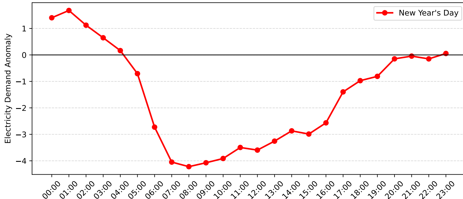
Five Dock Demand Anomaly: New Year's Day (2009-2010)
