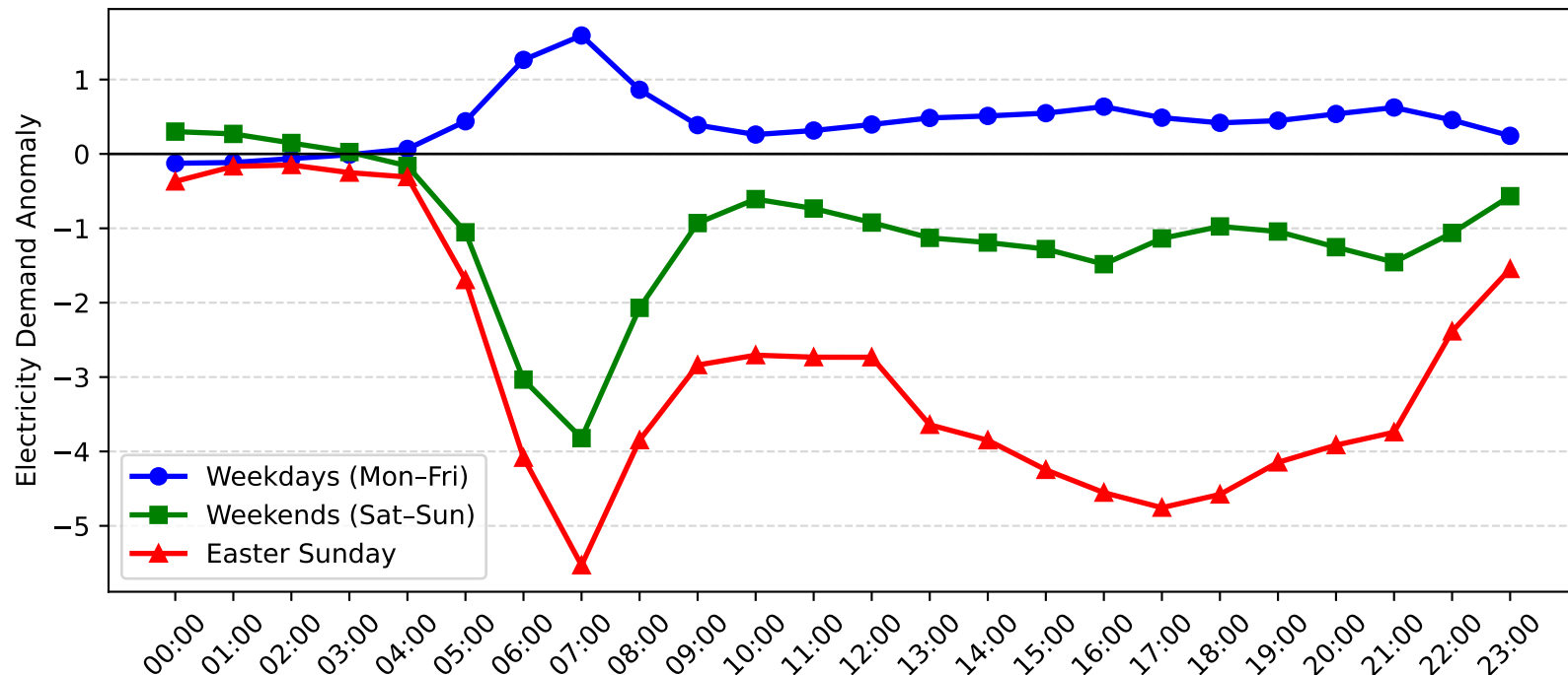
Dulwich Hill Demand Anomaly: Easter Sunday vs Weekday/Weekend (2012-2013)
