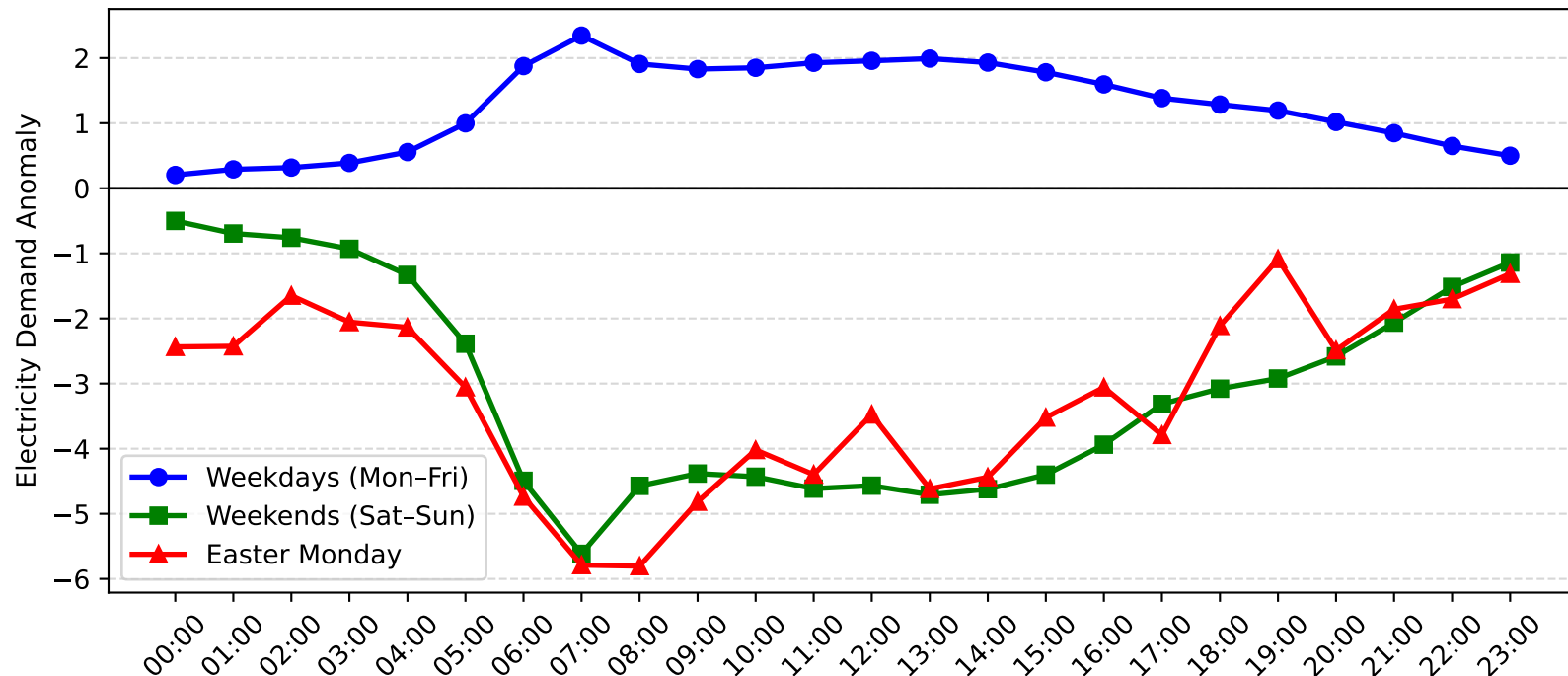
Matraverse Demand Anomaly: Easter Monday vs Weekday/Weekend (2007-2008)
