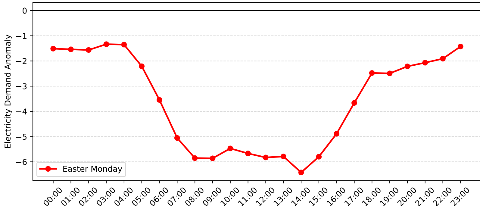
Mascot Demand Anomaly: Easter Monday (2017-2018)
