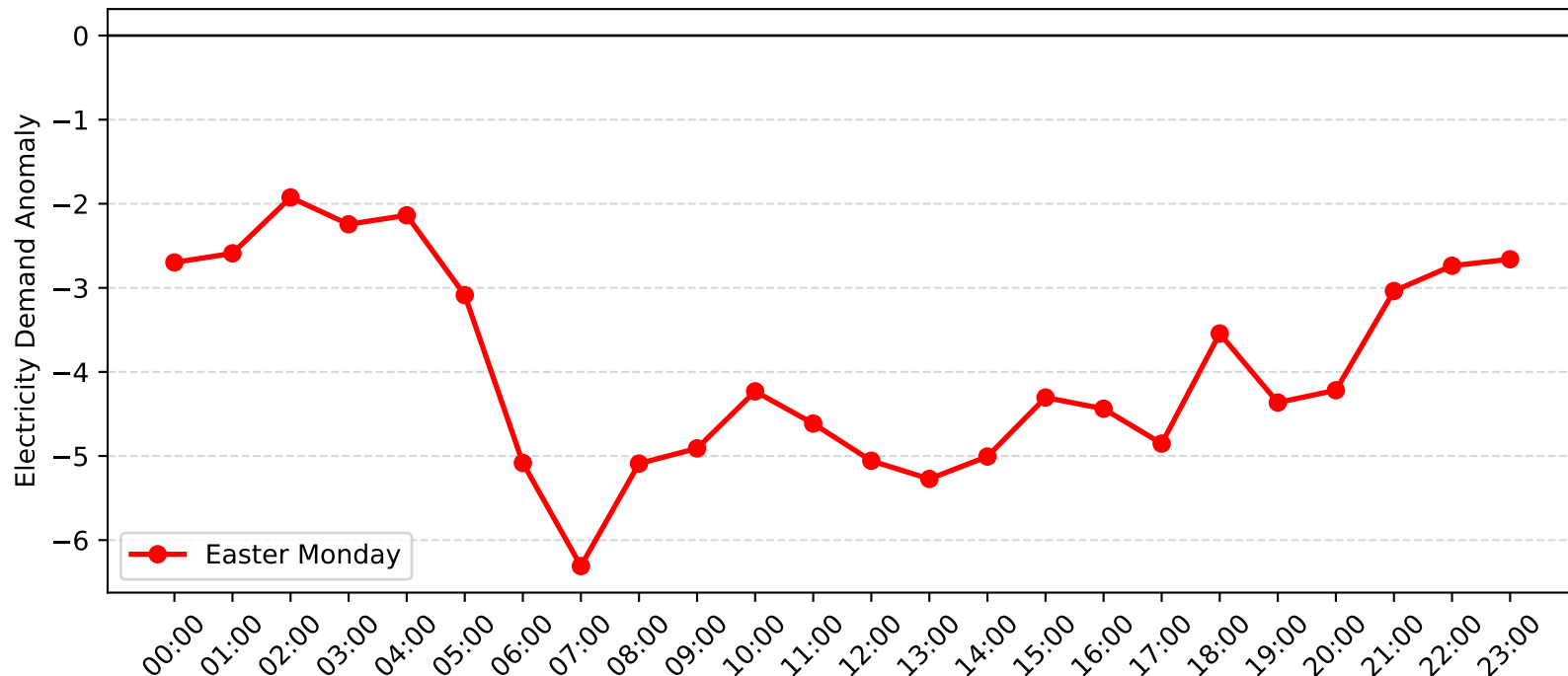
Matraville Demand Anomaly: Easter Monday (2010-2011)
