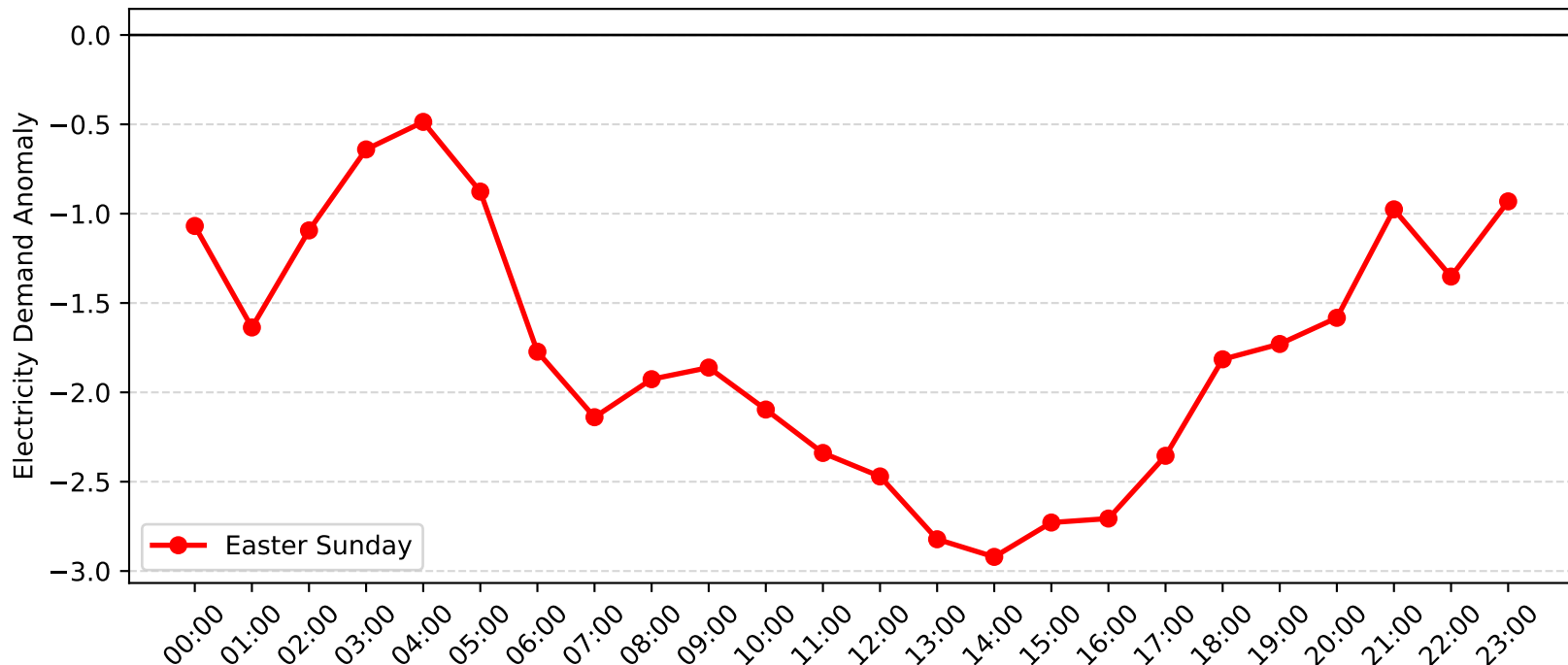
Gateshead Demand Anomaly: Easter Sunday (2007-2008)
