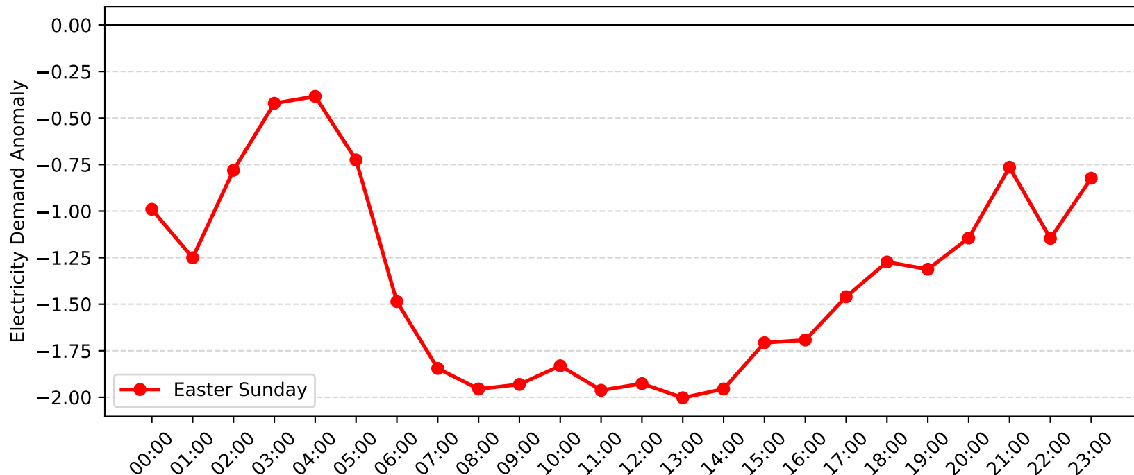
Gateshead Demand Anomaly: Easter Sunday (2011-2012)
