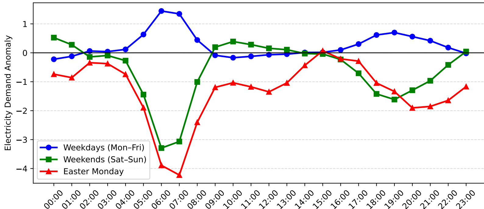
Cronulla Demand Anomaly: Easter Monday vs Weekday/Weekend (2015-2016)
