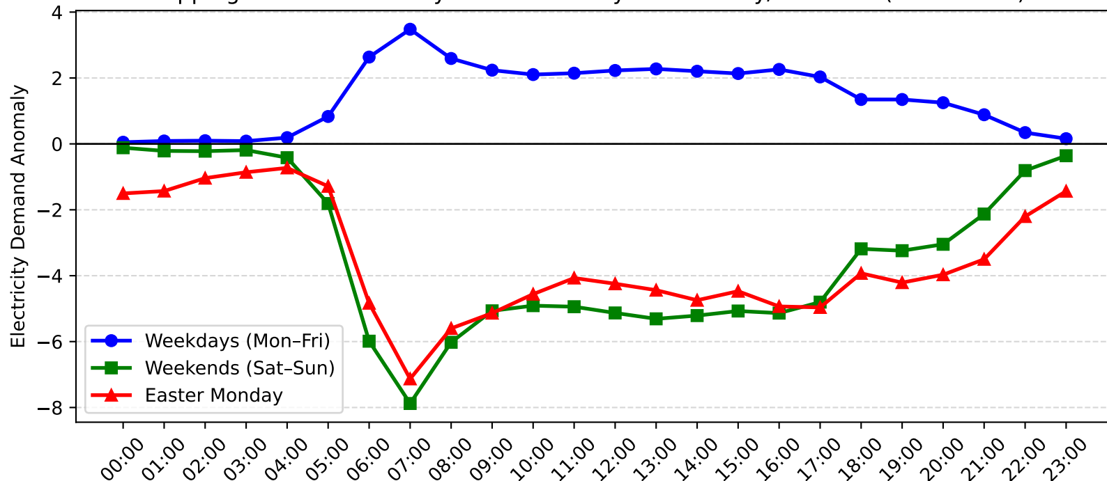
Epping Demand Anomaly: Easter Monday vs Weekday/Weekend (2010-2011)
