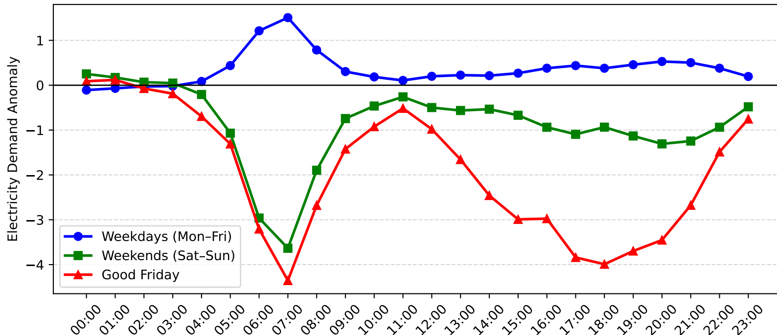
Dulwich Hill Demand Anomaly: Good Friday vs Weekday/Weekend (2015-2016)
