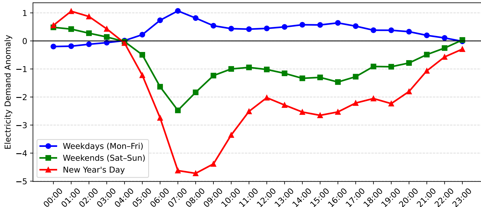
Five Dock Demand Anomaly: New Year's Day vs Weekday/Weekend (2011-2012)
