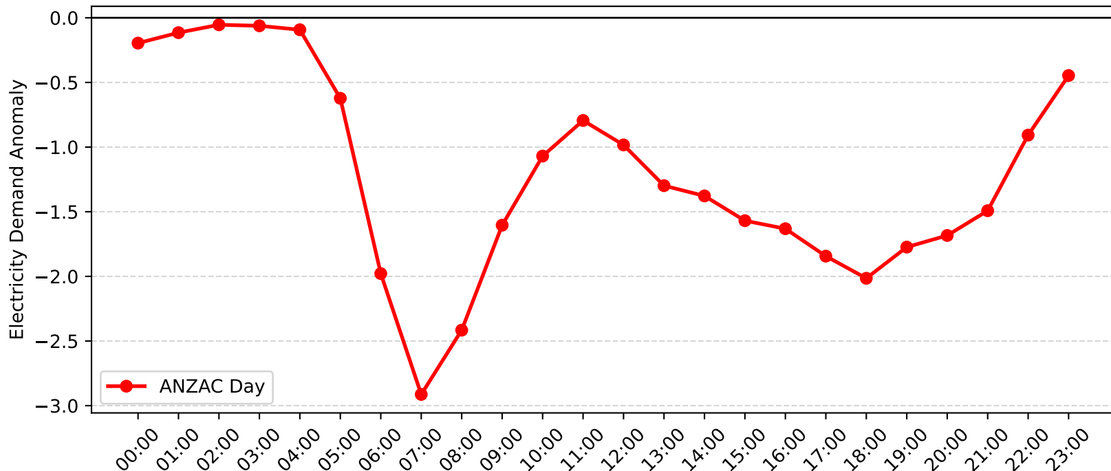
Blakehurst Demand Anomaly: ANZAC Day (2010-2011)
