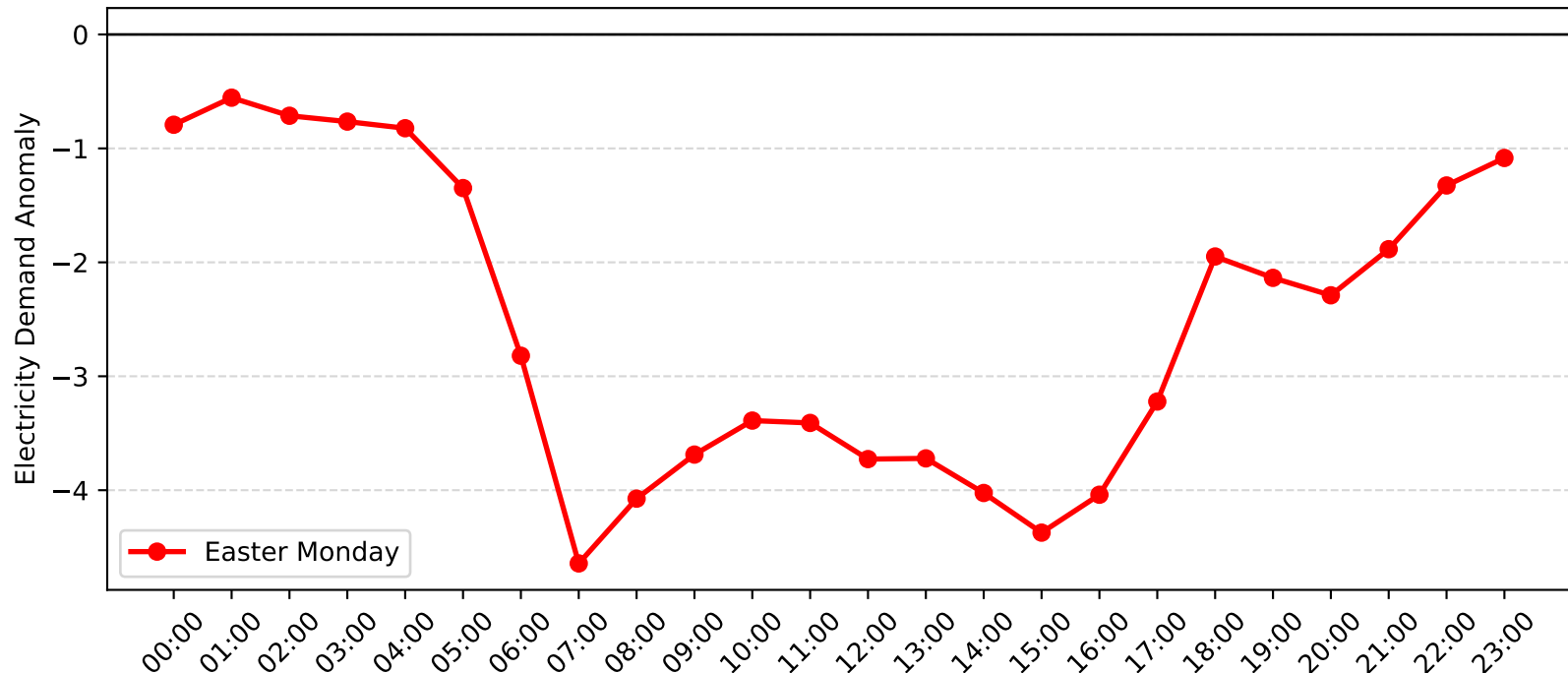
Epping Demand Anomaly: Easter Monday (2016-2017)
