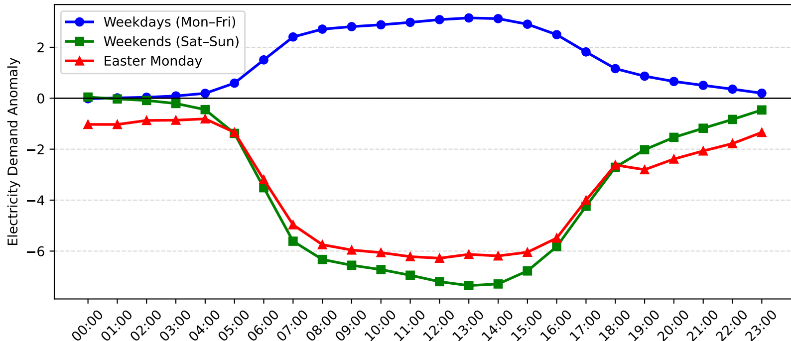
Mascot Demand Anomaly: Easter Monday vs Weekday/Weekend (2014-2015)
