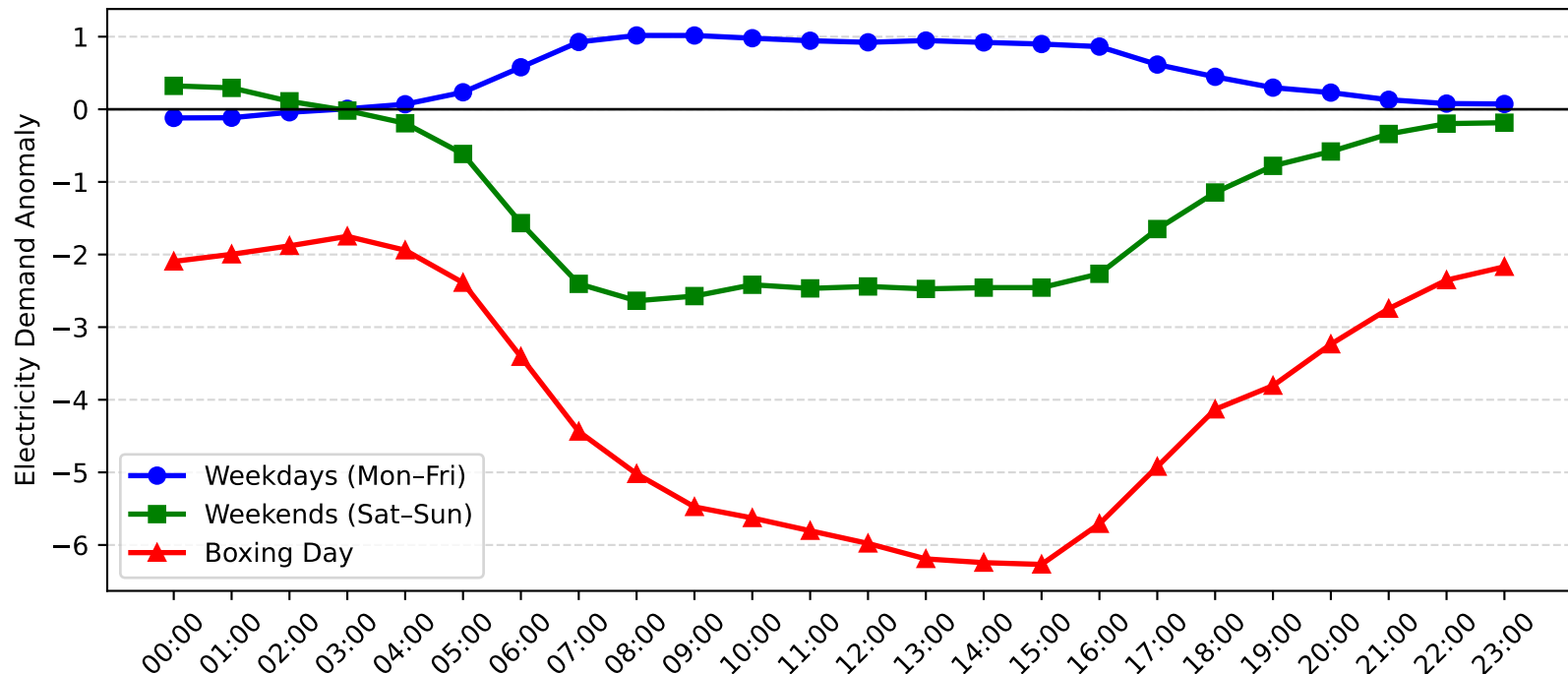
Lidcombe Demand Anomaly: Boxing Day vs Weekday/Weekend (2006-2007)
