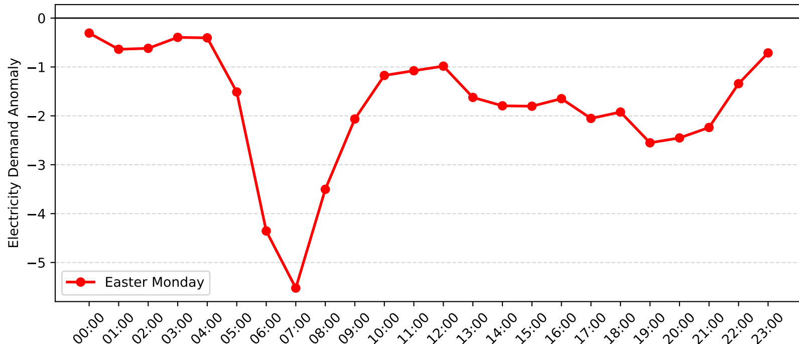
Mortdale Demand Anomaly: Easter Monday (2011-2012)
