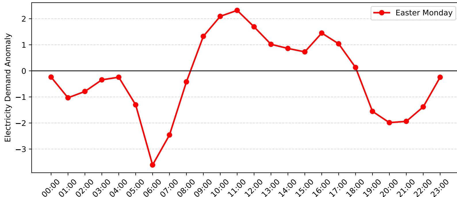
Cronulla Demand Anomaly: Easter Monday (2009-2010)
