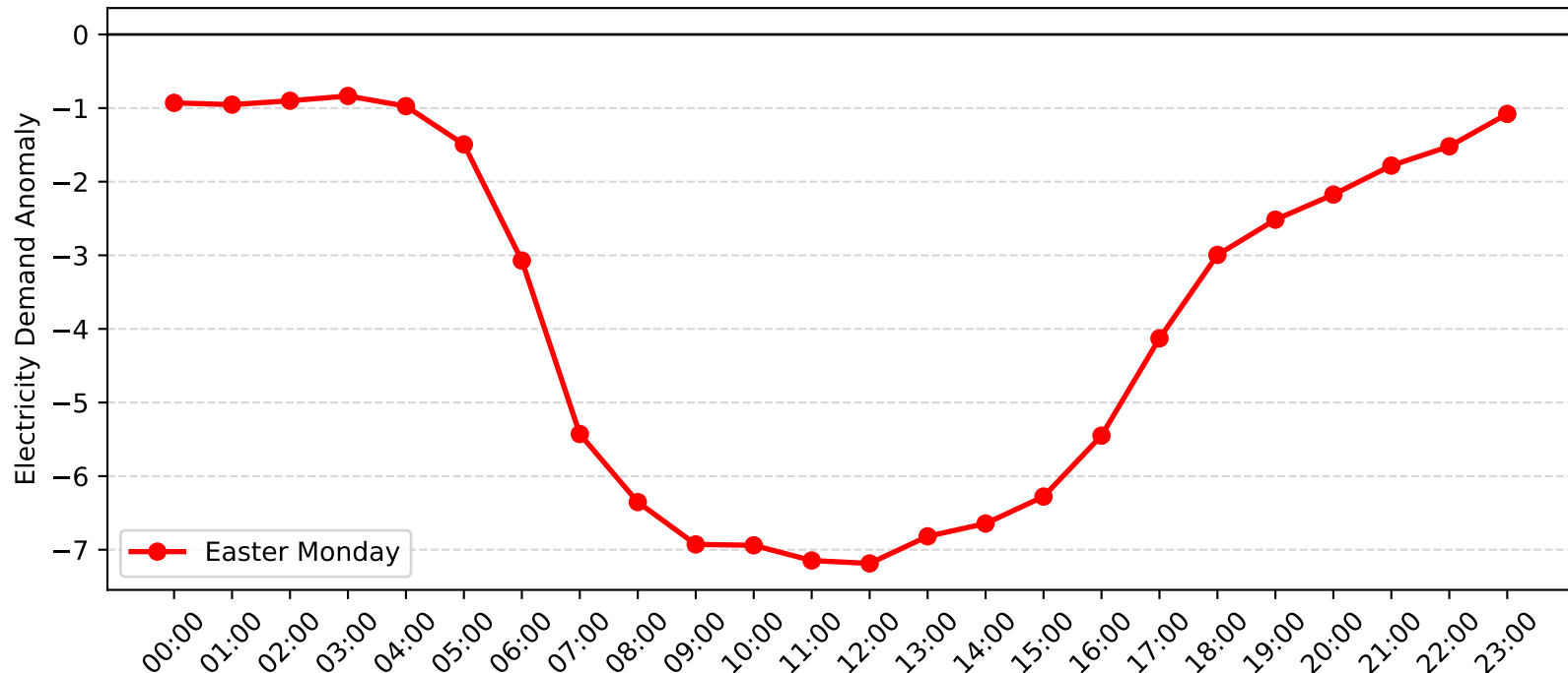
Mascot Demand Anomaly: Easter Monday (2013-2014)
