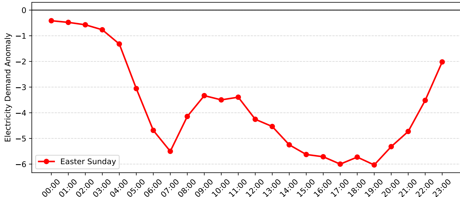
Dulwich Hill Demand Anomaly: Easter Sunday (2010-2011)
