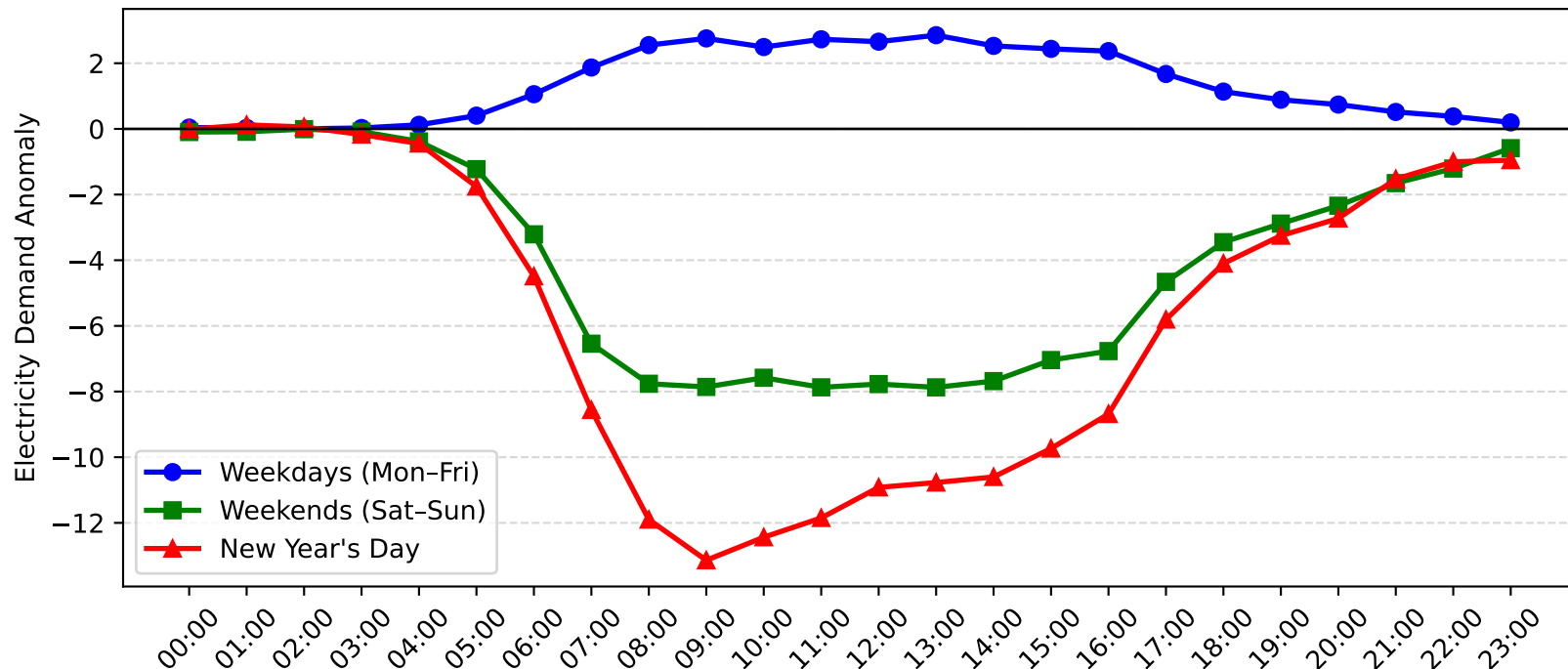
Brookvale Demand Anomaly: New Year's Day vs Weekday/Weekend (2009-2010)
