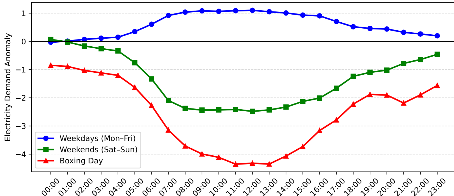
Lidcombe Demand Anomaly: Boxing Day vs Weekday/Weekend (2010-2011)
