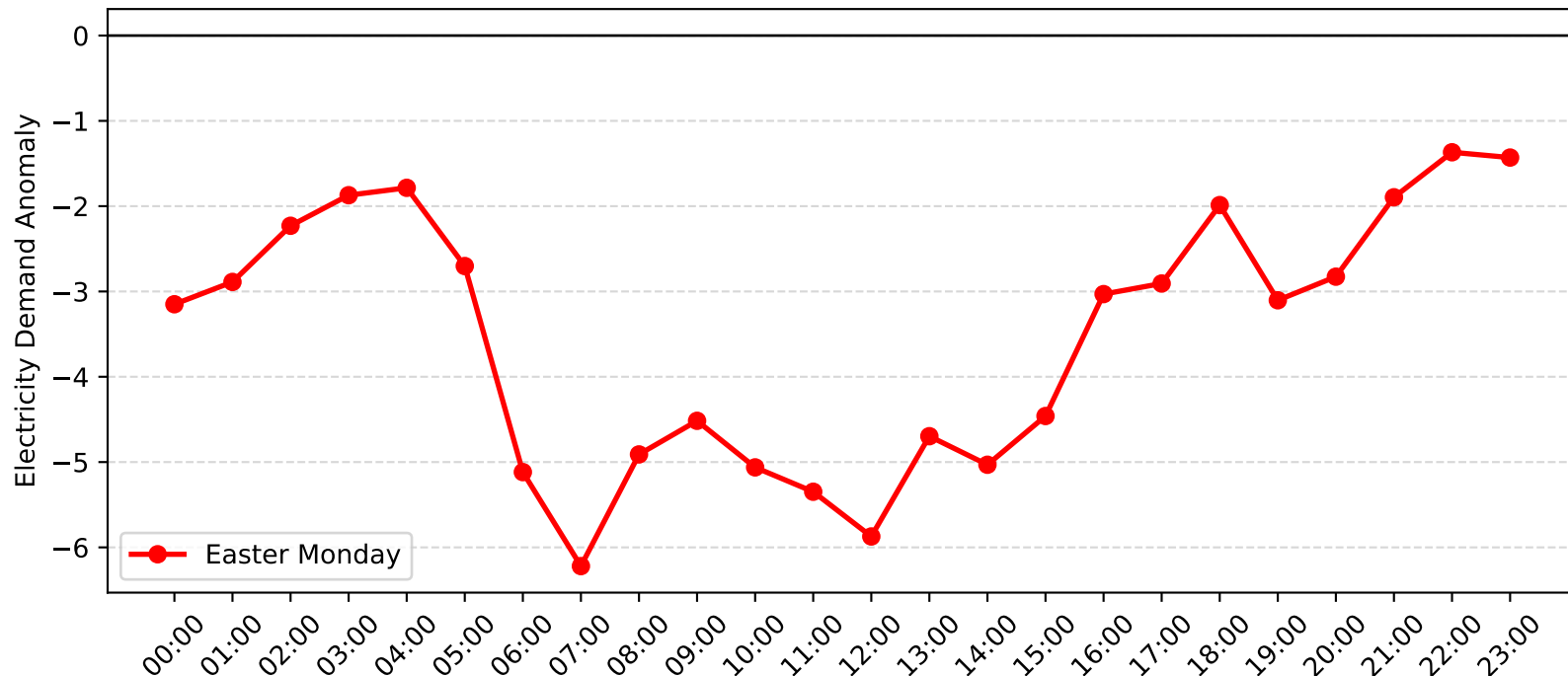
Matraville Demand Anomaly: Easter Monday (2009-2010)
