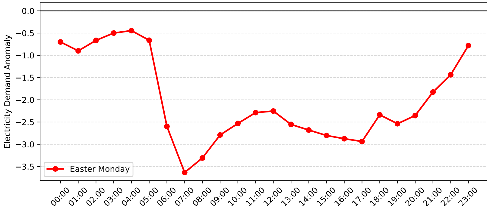
Pymble Demand Anomaly: Easter Monday (2010-2011)
