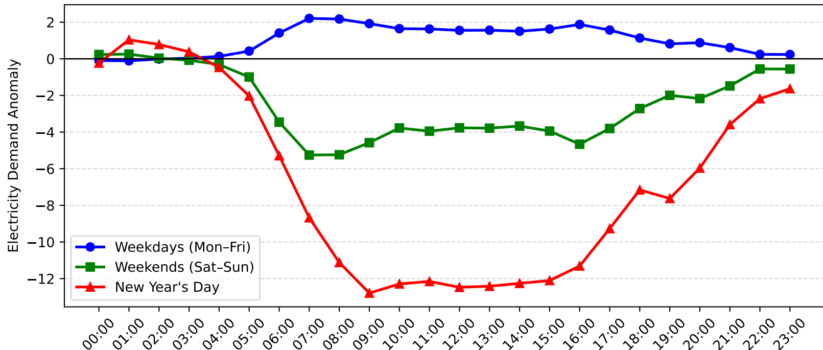
Burwood Demand Anomaly: New Year's Day vs Weekday/Weekend (2007-2008)
