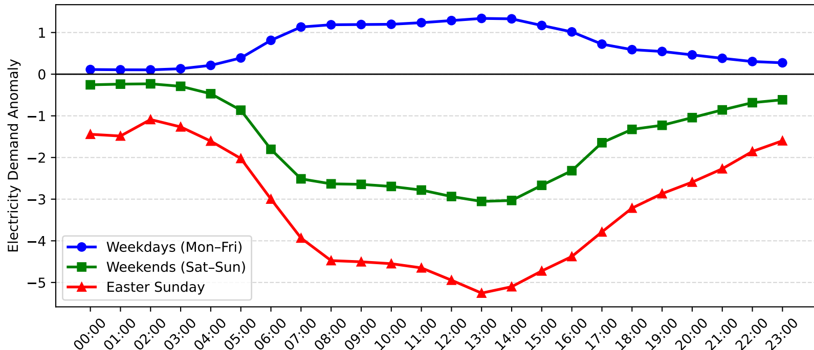
Caringbah Demand Anomaly: Easter Sunday vs Weekday/Weekend (2016-2017)
