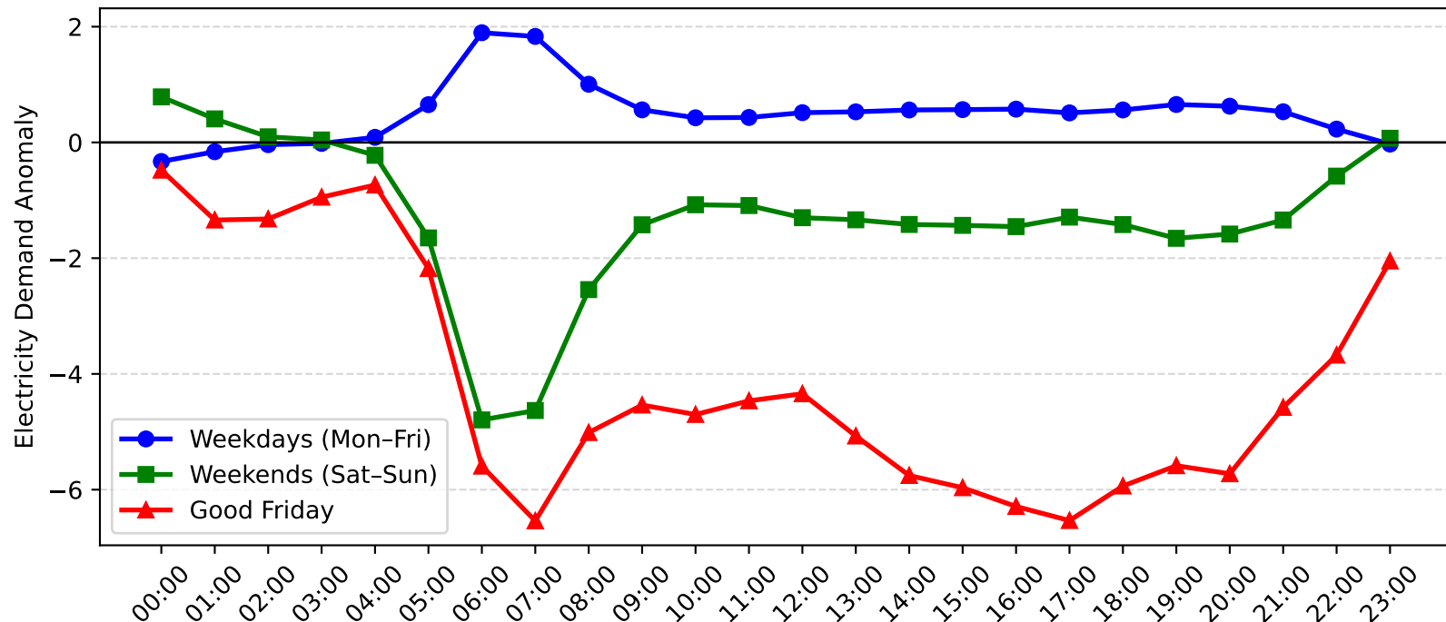
Pennant Hills Demand Anomaly: Good Friday vs Weekday/Weekend (2012-2013)
