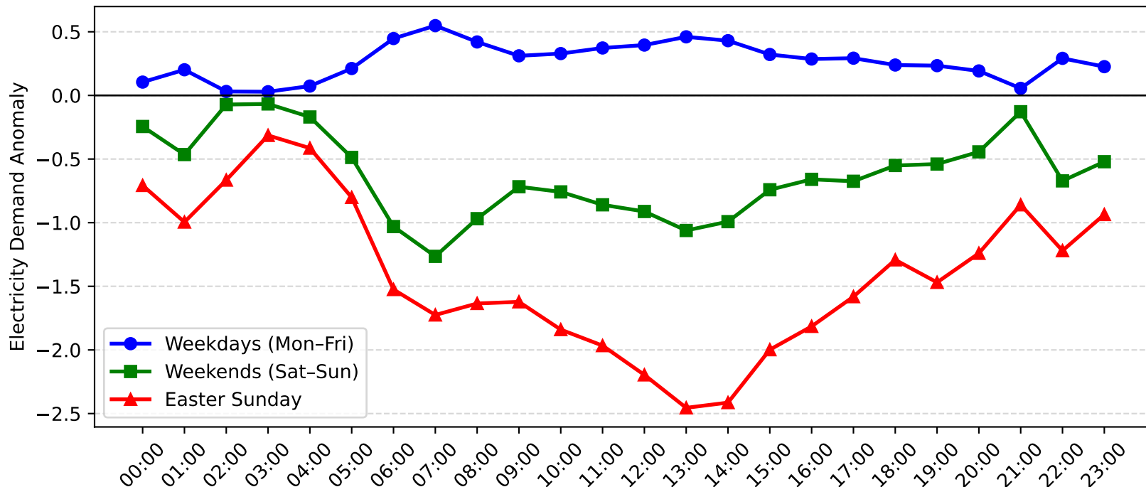
Gateshead Demand Anomaly: Easter Sunday vs Weekday/Weekend (2014-2015)
