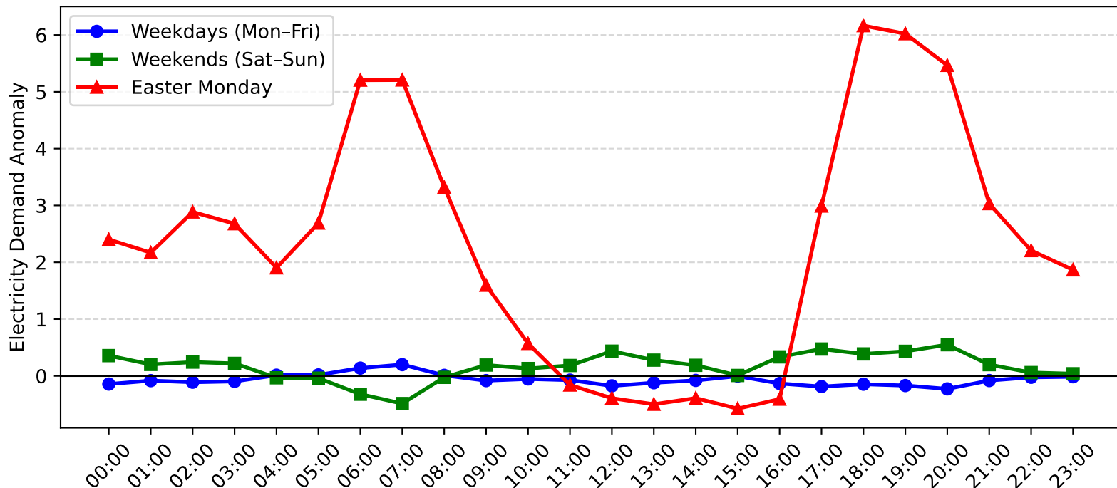
Cronulla Demand Anomaly: Easter Monday vs Weekday/Weekend (2004-2005)
