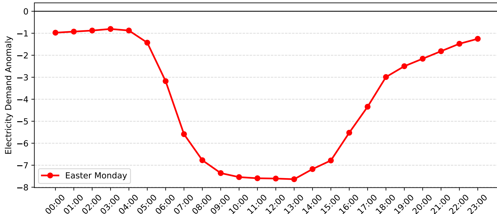
Mascot Demand Anomaly: Easter Monday (2012-2013)
