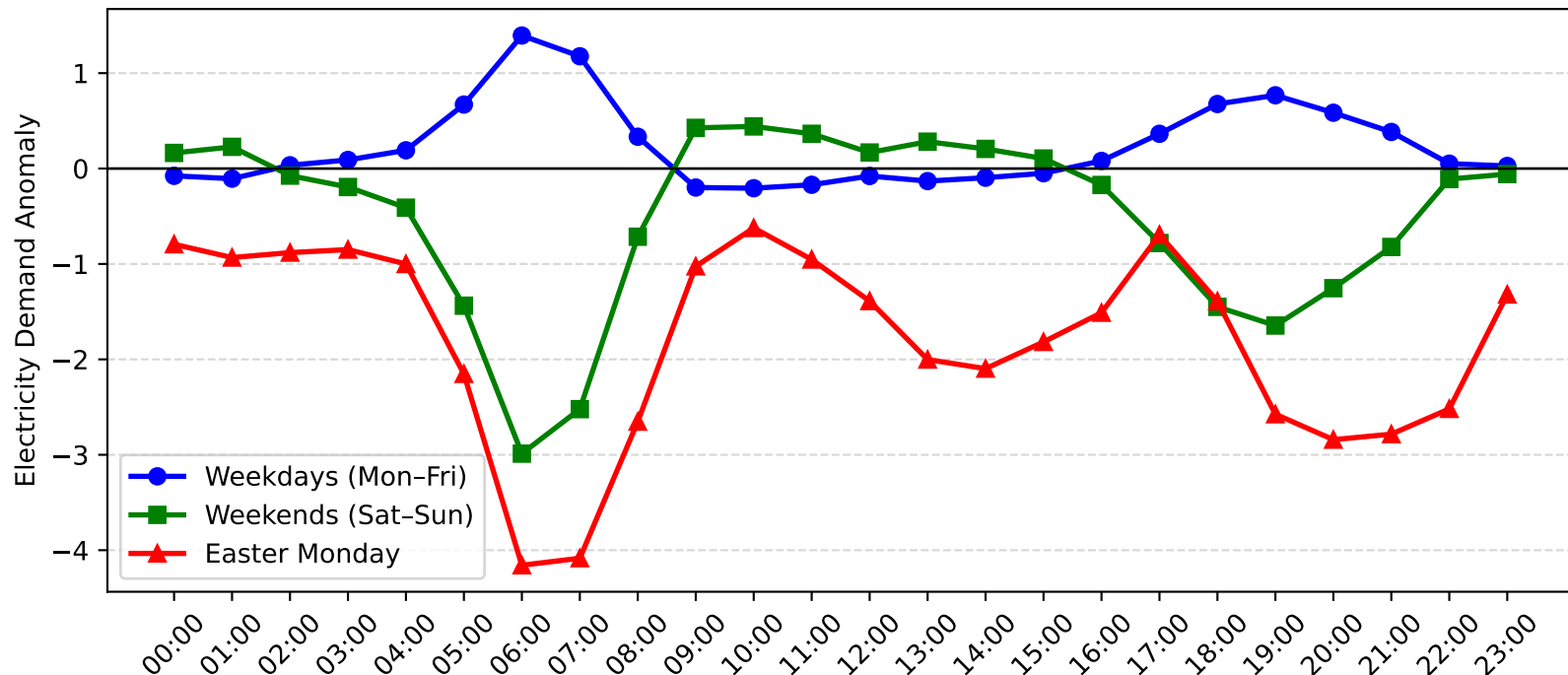
Cronulla Demand Anomaly: Easter Monday vs Weekday/Weekend (2017-2018)
