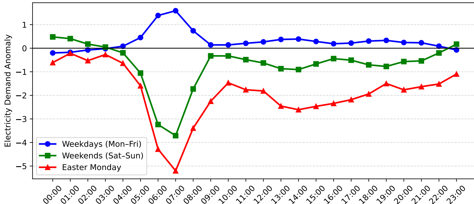
Mortdale Demand Anomaly: Easter Monday vs Weekday/Weekend (2013-2014)
