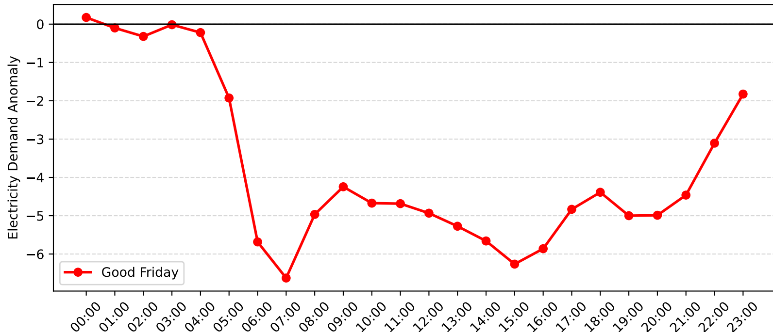
Dulwich Hill Demand Anomaly: Good Friday (2006-2007)
