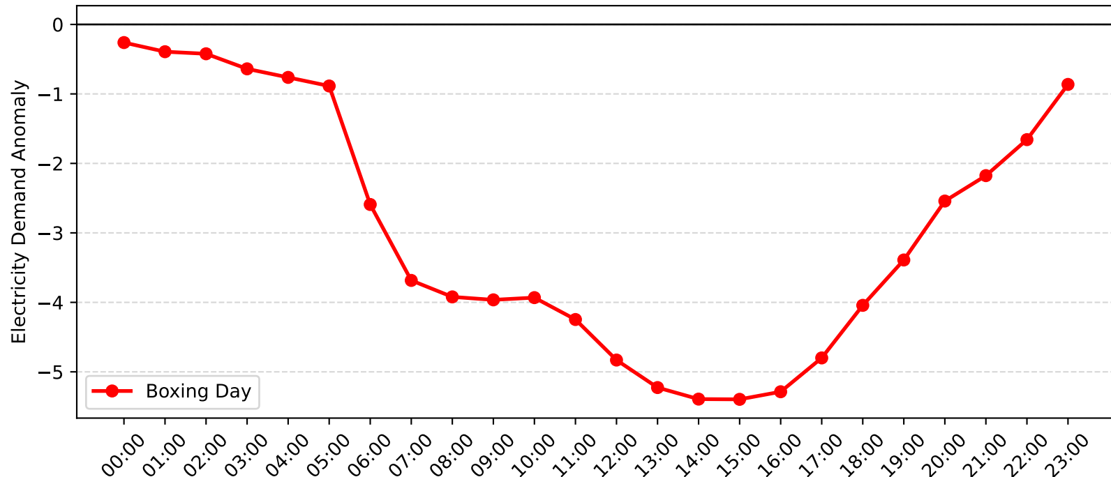
Pymble Demand Anomaly: Boxing Day (2006-2007)
