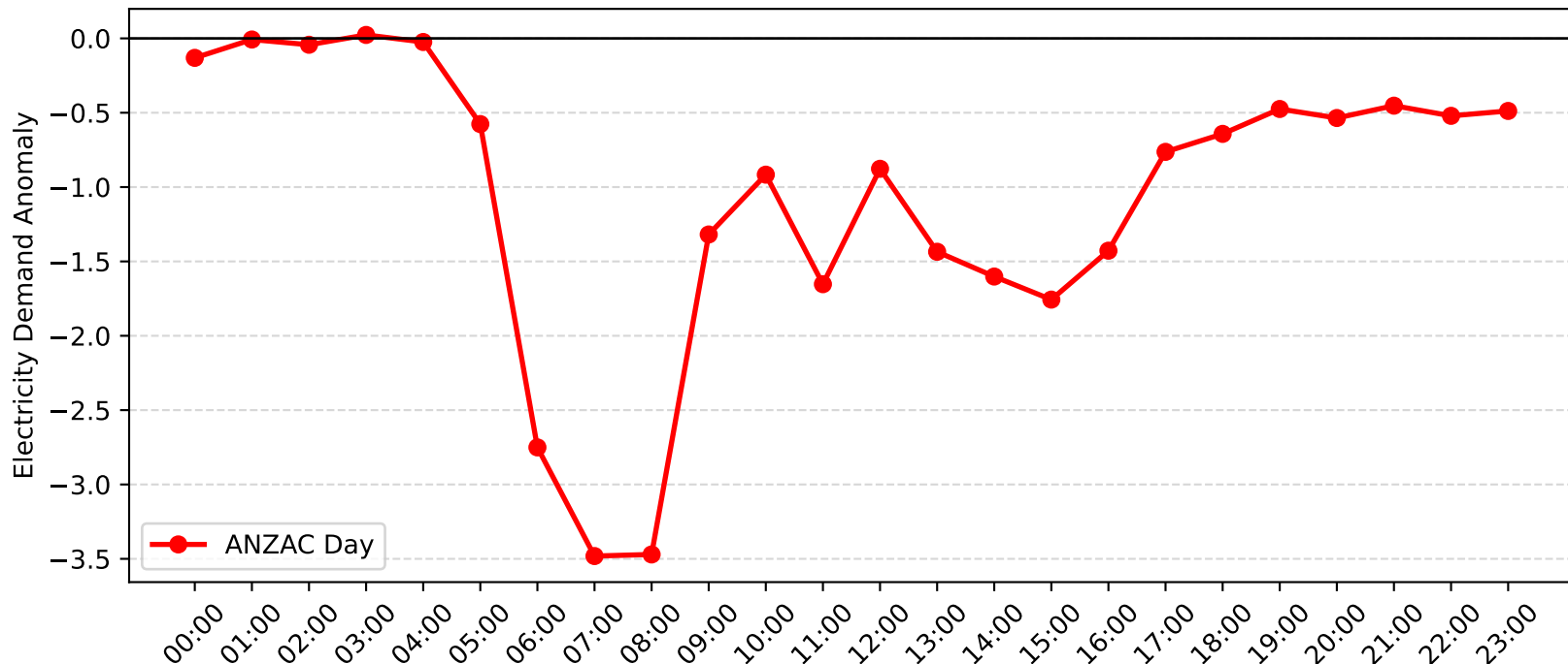
Blakehurst Demand Anomaly: ANZAC Day (2005-2006)
