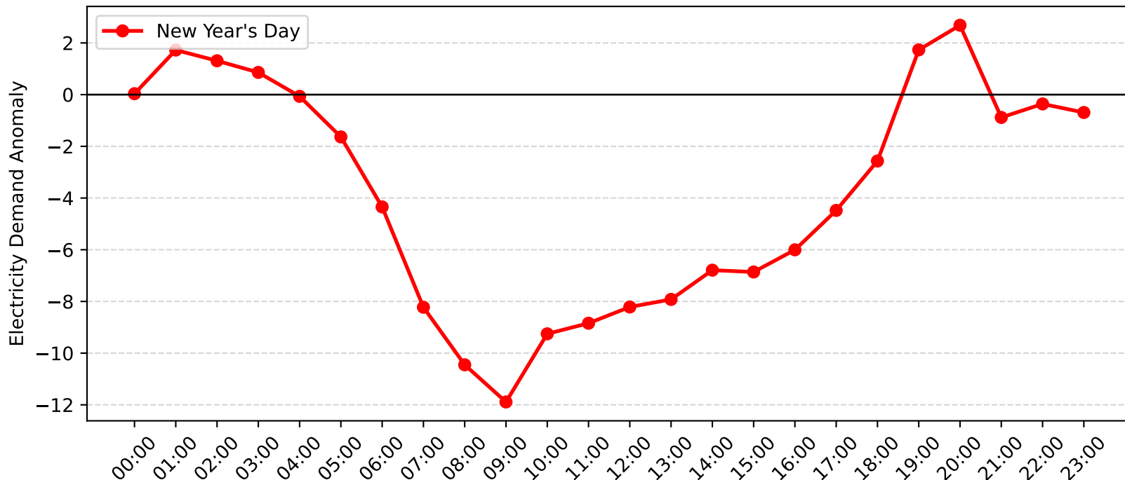
Burwood Demand Anomaly: New Year's Day (2008-2009)
