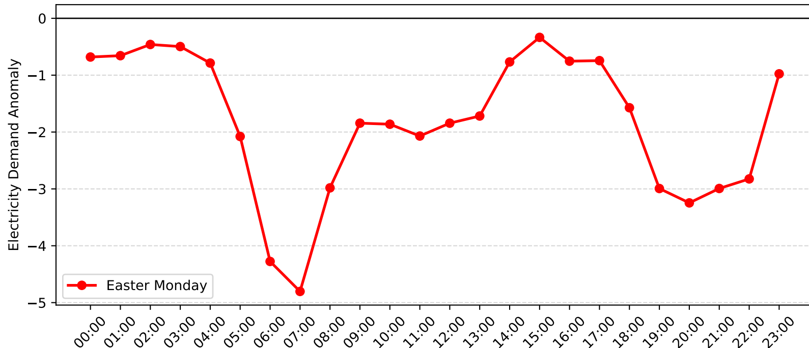
Cronulla Demand Anomaly: Easter Monday (2014-2015)
