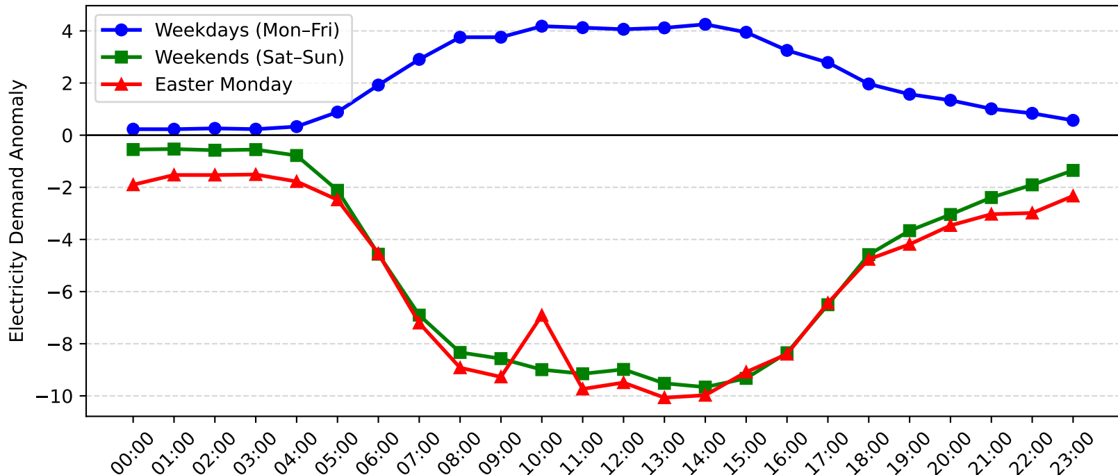
Mascot Demand Anomaly: Easter Monday vs Weekday/Weekend (2006-2007)
