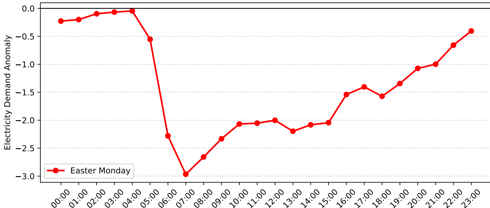
Pymble Demand Anomaly: Easter Monday (2008-2009)
