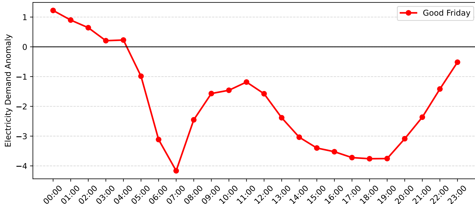
Dulwich Hill Demand Anomaly: Good Friday (2012-2013)
