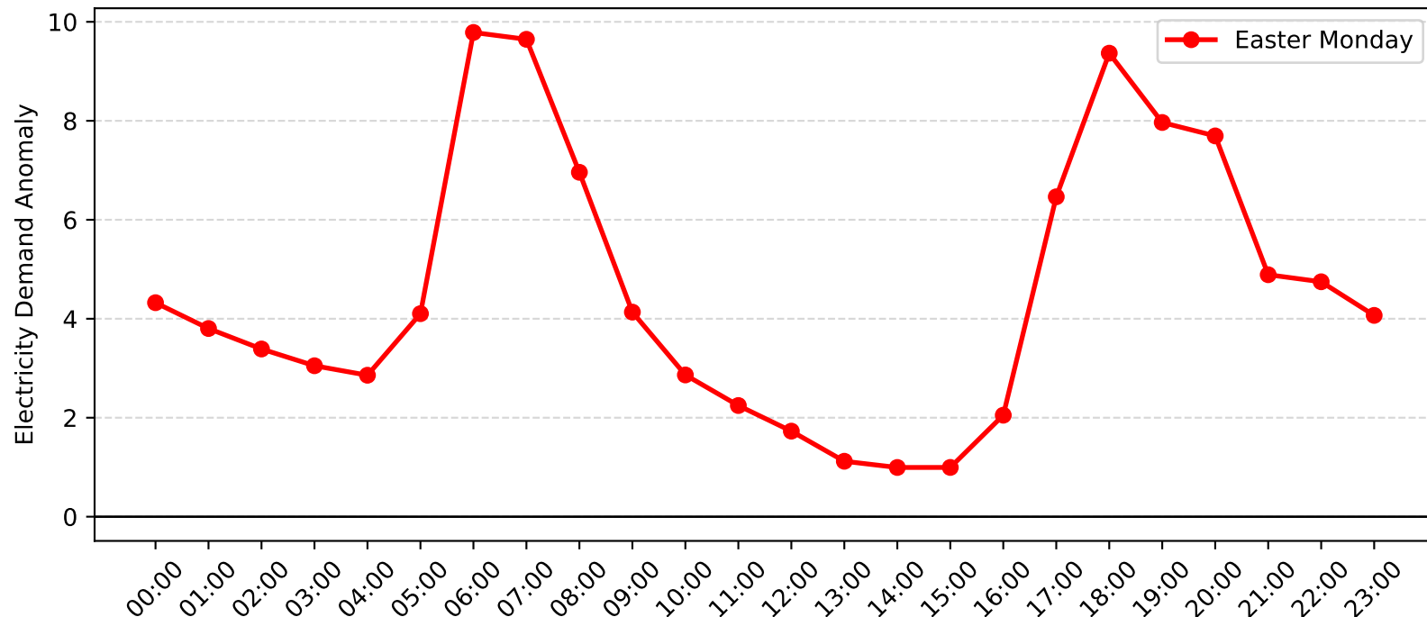
Pymble Demand Anomaly: Easter Monday (2004-2005)
