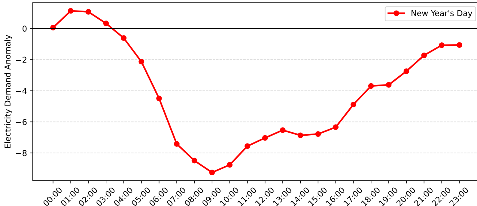
Burwood Demand Anomaly: New Year's Day (2012-2013)
