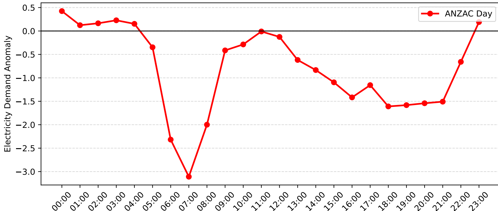
Blakehurst Demand Anomaly: ANZAC Day (2008-2009)
