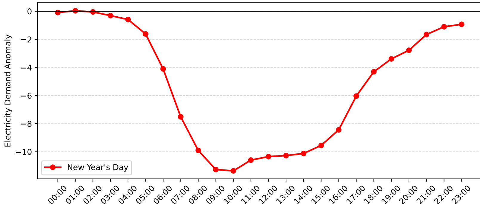
Brookvale Demand Anomaly: New Year's Day (2012-2013)
