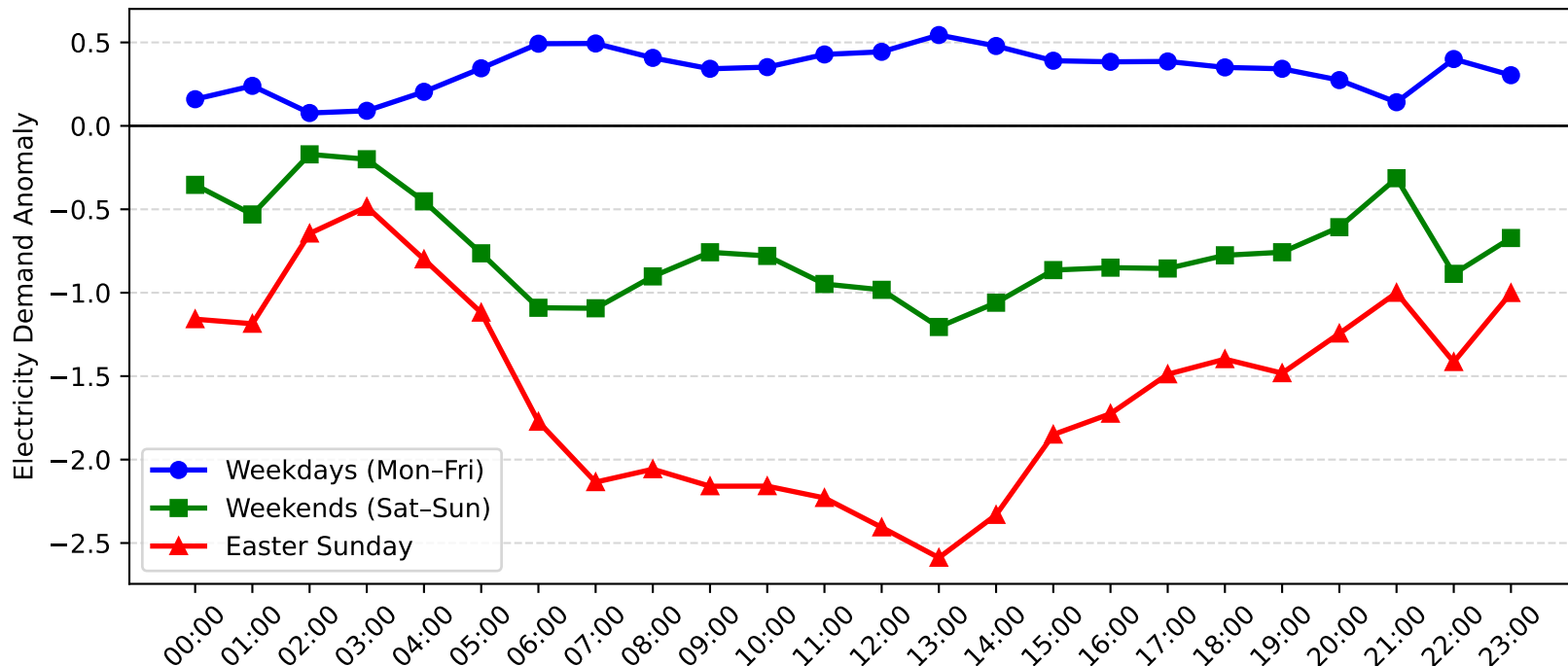
Gateshead Demand Anomaly: Easter Sunday vs Weekday/Weekend (2017-2018)
