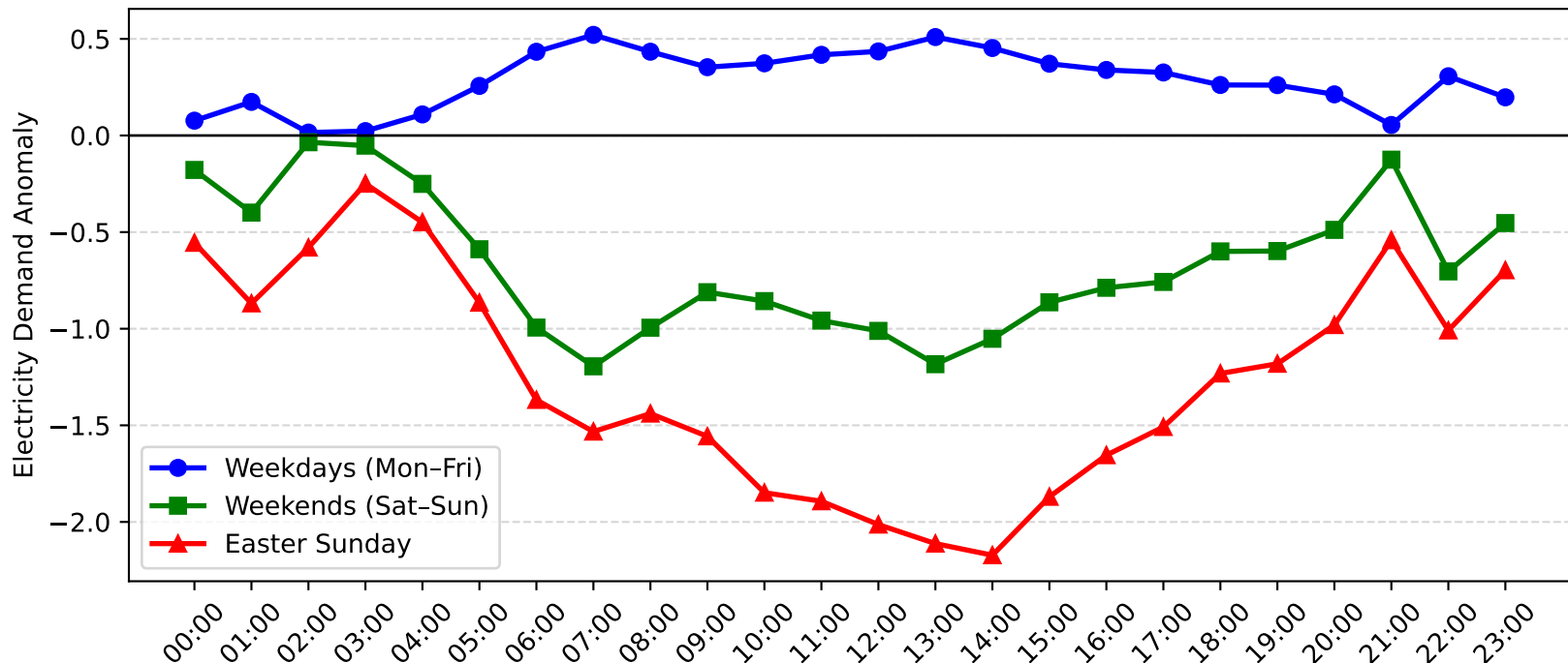
Gateshead Demand Anomaly: Easter Sunday vs Weekday/Weekend (2015-2016)
