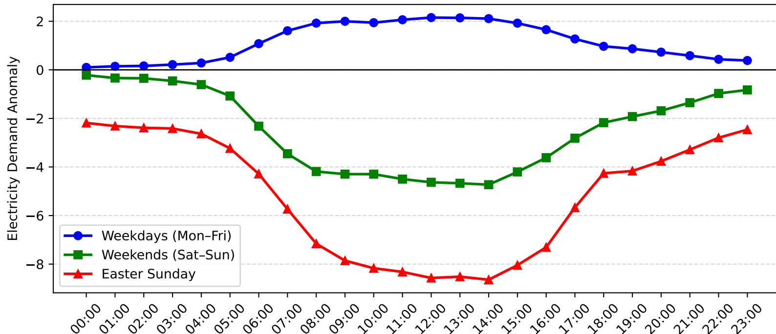
Caringbah Demand Anomaly: Easter Sunday vs Weekday/Weekend (2009-2010)
