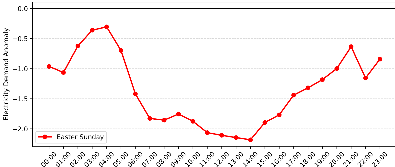
Gateshead Demand Anomaly: Easter Sunday (2012-2013)
