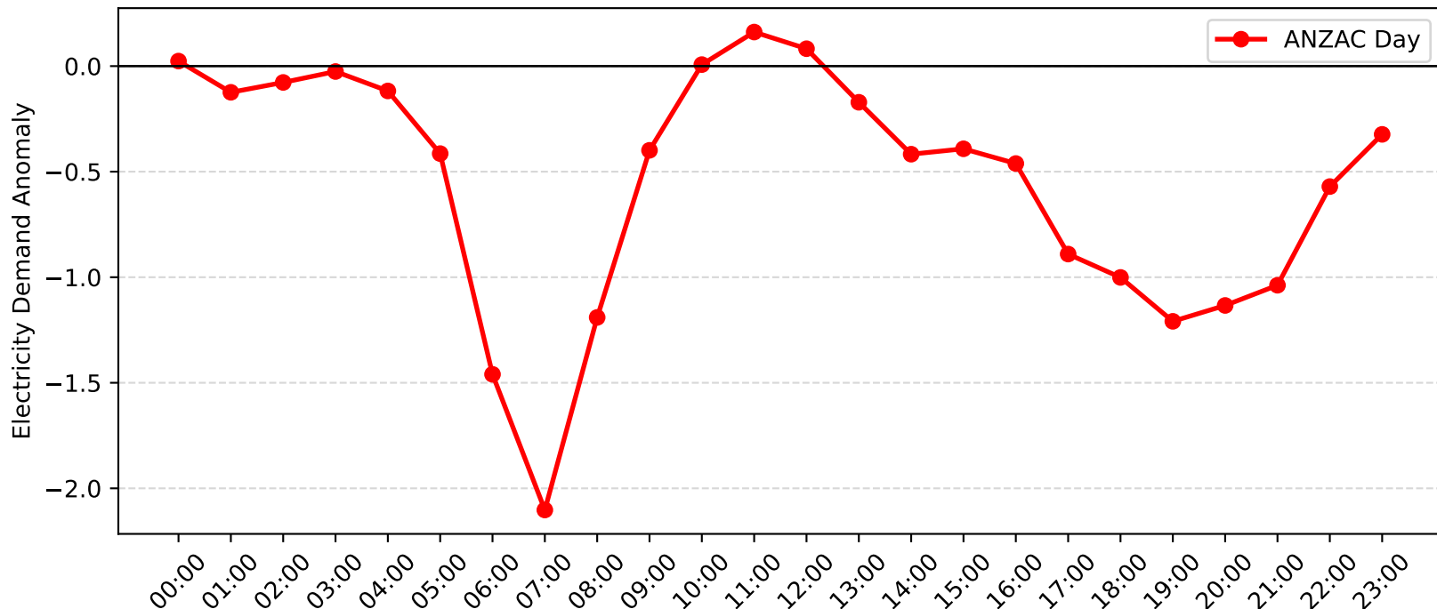
Blakehurst Demand Anomaly: ANZAC Day (2014-2015)
