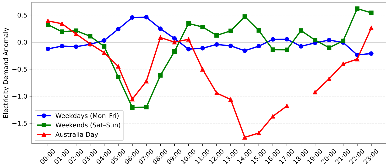
Woy Woy Demand Anomaly: Australia Day vs Weekday/Weekend (2005-2006)
