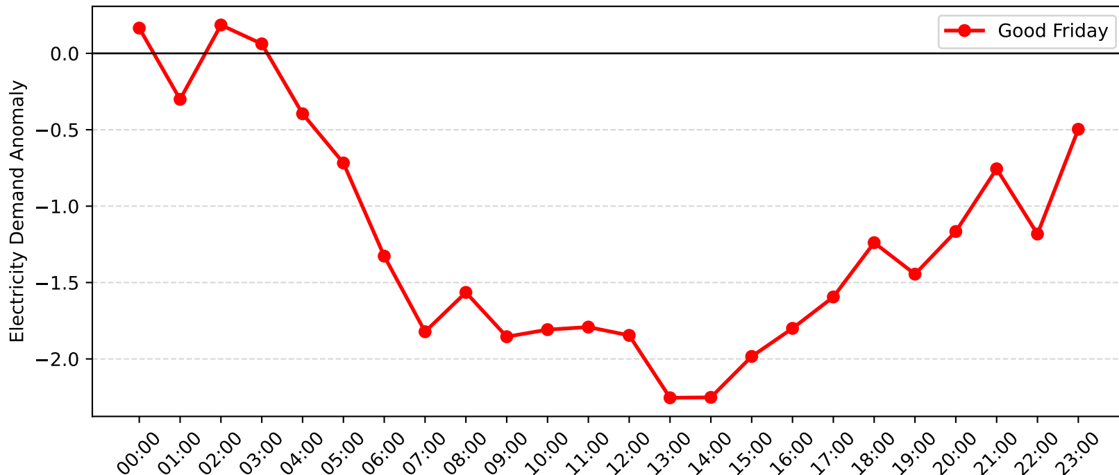
Gateshead Demand Anomaly: Good Friday (2017-2018)
