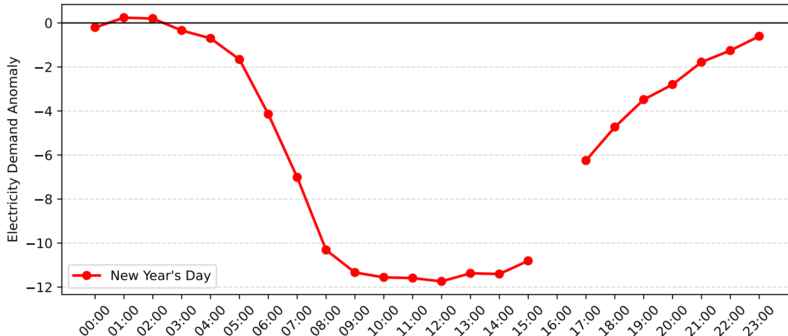
Brookvale Demand Anomaly: New Year's Day (2015-2016)
