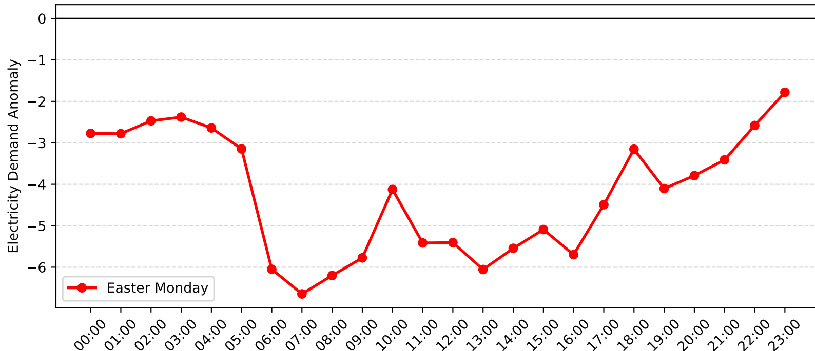
Matraverse Demand Anomaly: Easter Monday (2006-2007)
