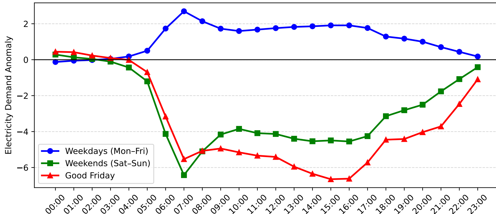
Chatswood Demand Anomaly: Good Friday vs Weekday/Weekend (2008-2009)
