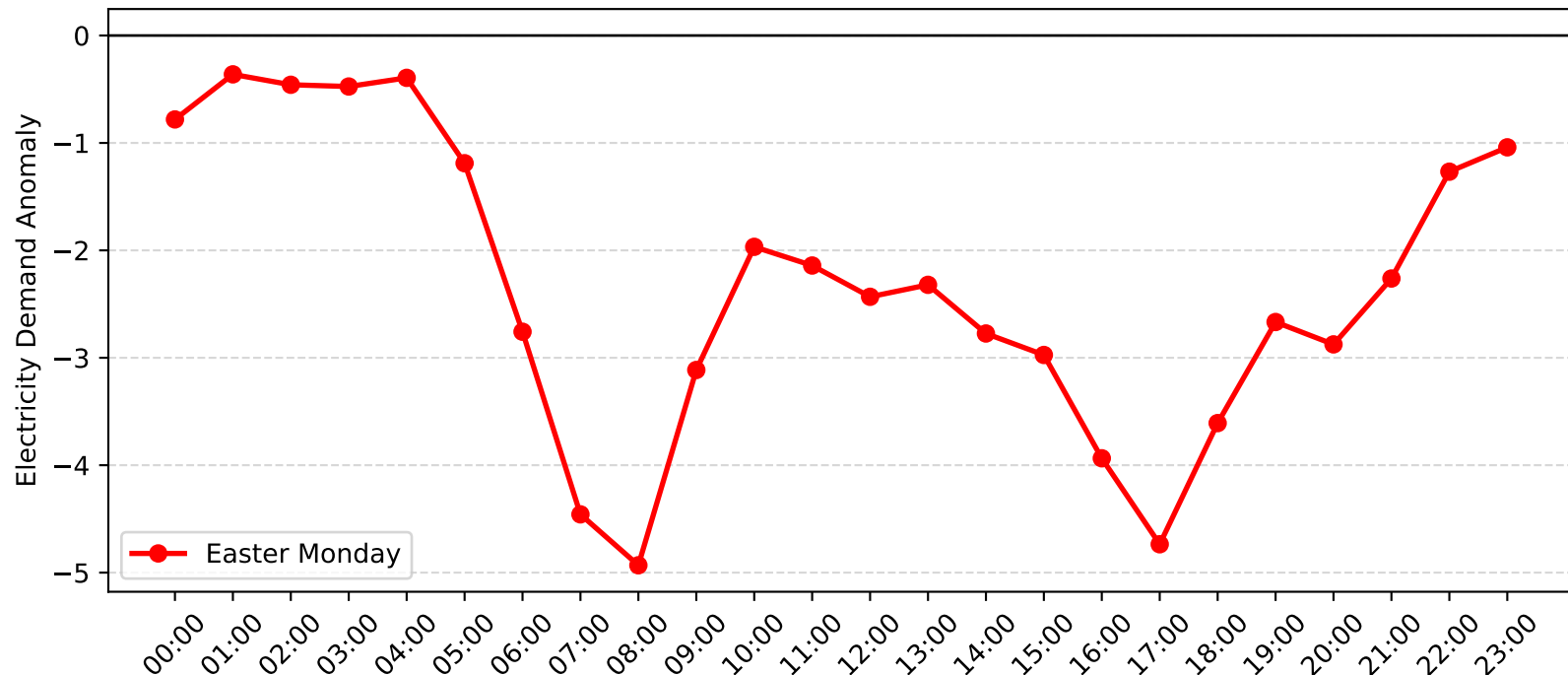
Epping Demand Anomaly: Easter Monday (2007-2008)
