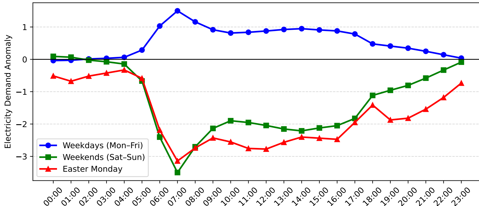
Pymble Demand Anomaly: Easter Monday vs Weekday/Weekend (2014-2015)
