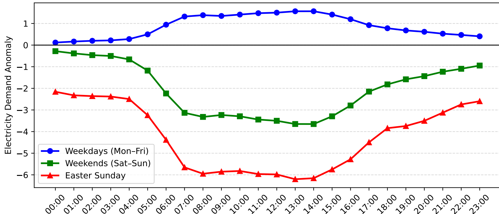
Caringbah Demand Anomaly: Easter Sunday vs Weekday/Weekend (2011-2012)
