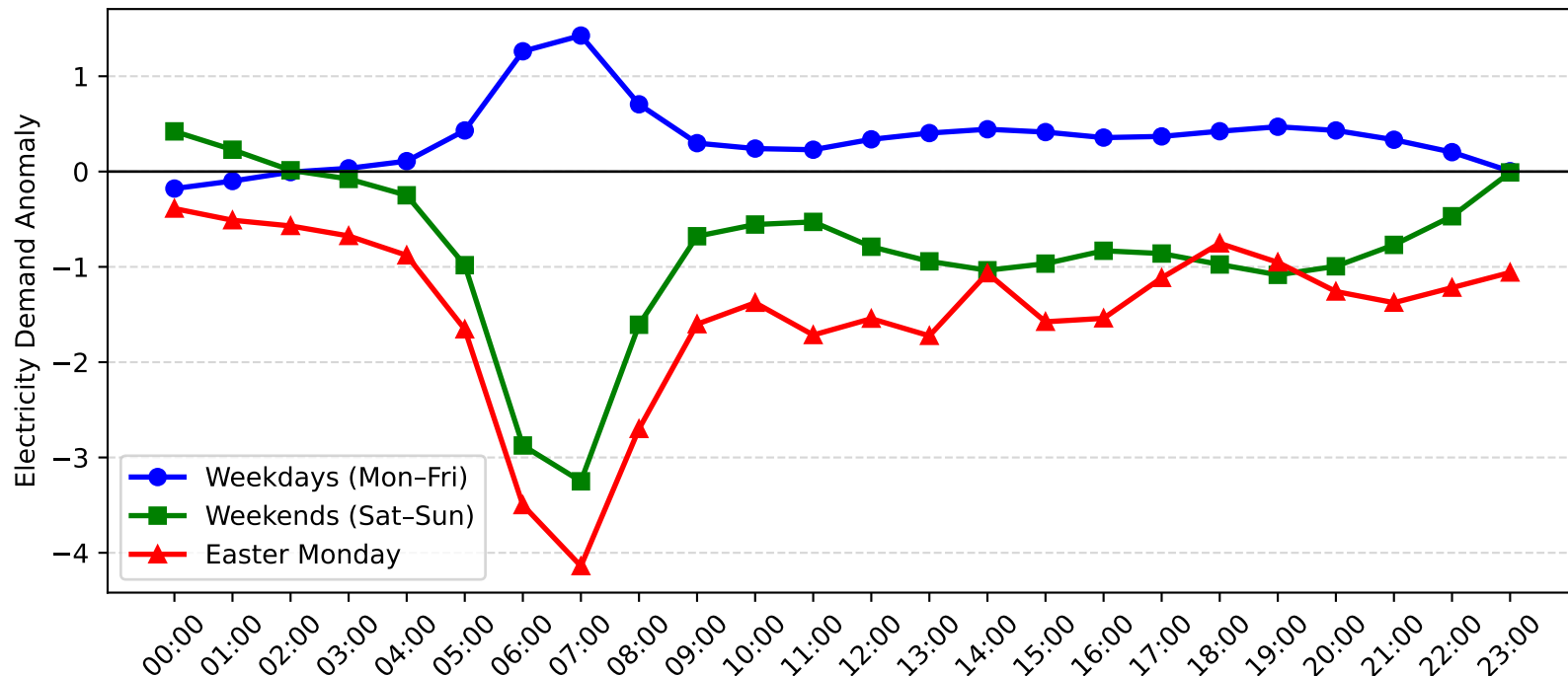
Mortdale Demand Anomaly: Easter Monday vs Weekday/Weekend (2015-2016)
