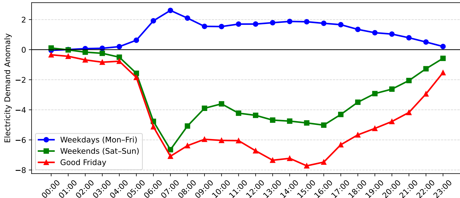
Chatswood Demand Anomaly: Good Friday vs Weekday/Weekend (2005-2006)
