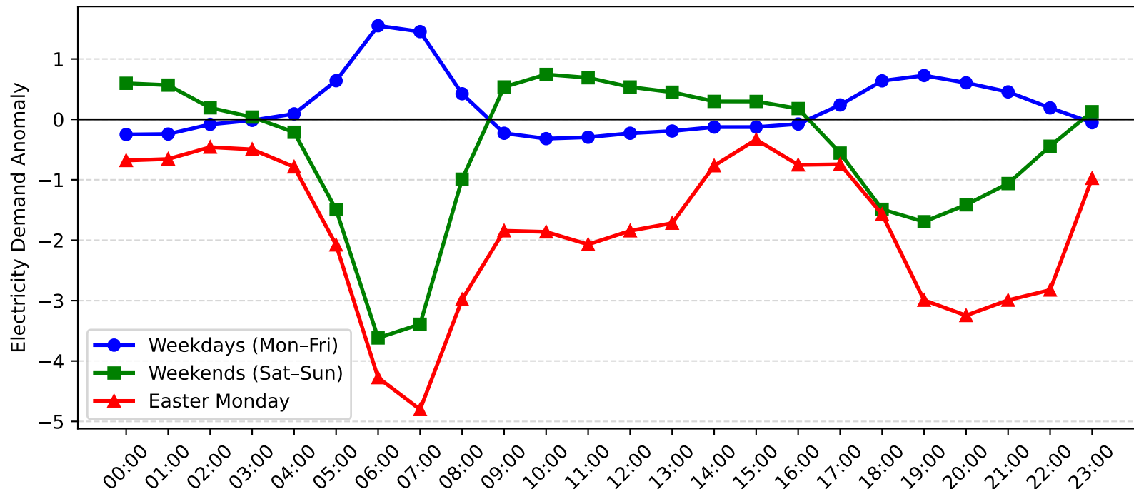
Cronulla Demand Anomaly: Easter Monday vs Weekday/Weekend (2014-2015)
