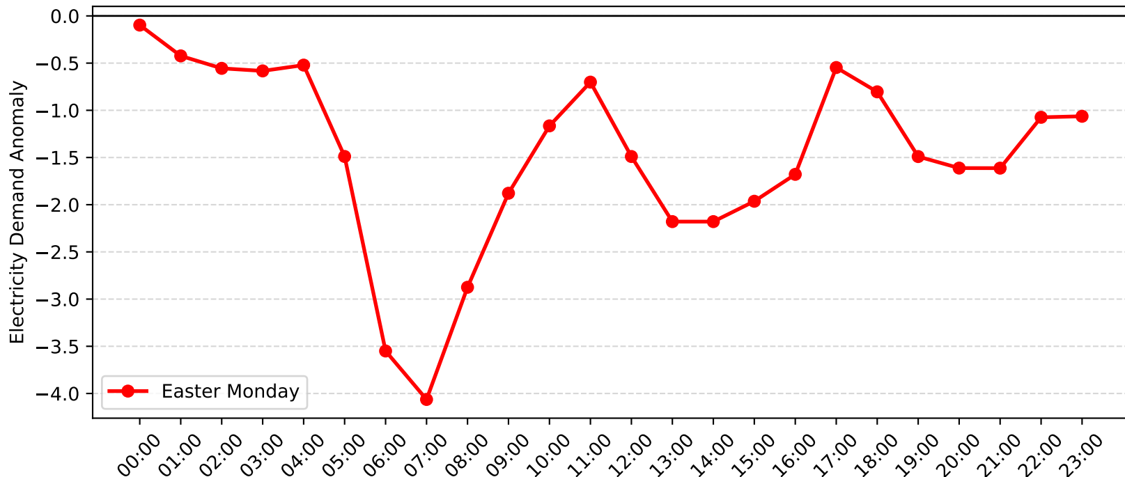
Mortdale Demand Anomaly: Easter Monday (2017-2018)
