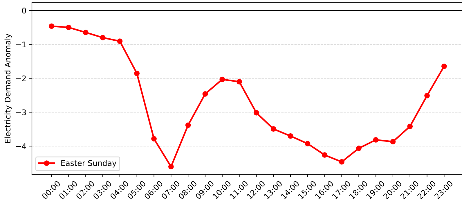
Dulwich Hill Demand Anomaly: Easter Sunday (2015-2016)
