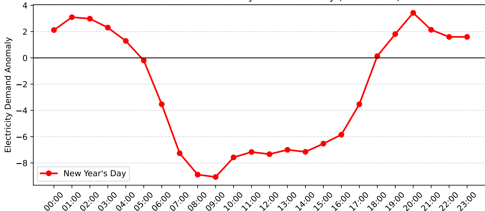
Burwood Demand Anomaly: New Year's Day (2006-2007)
