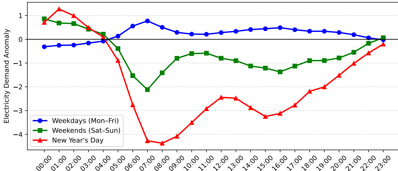
Five Dock Demand Anomaly: New Year's Day vs Weekday/Weekend (2013-2014)
