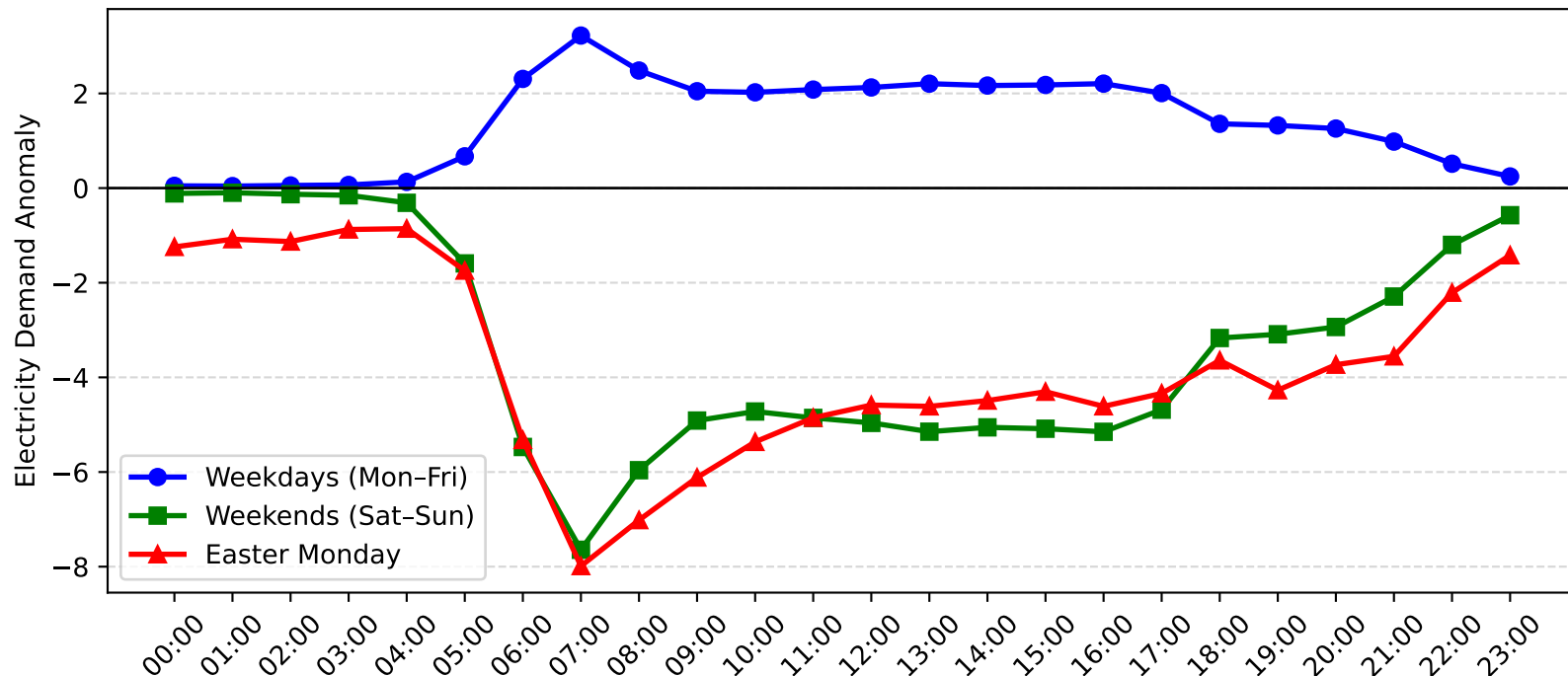
Epping Demand Anomaly: Easter Monday vs Weekday/Weekend (2011-2012)
