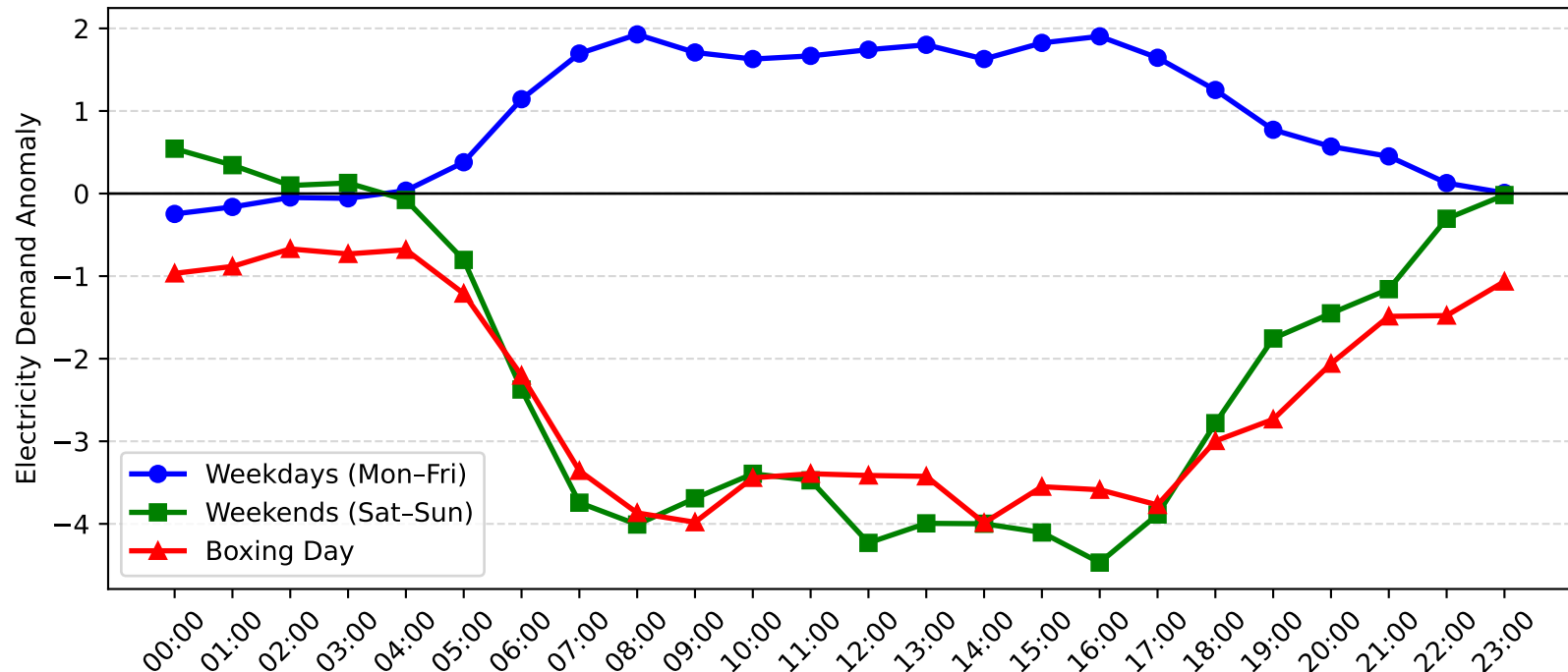
Pymble Demand Anomaly: Boxing Day vs Weekday/Weekend (2004-2005)
