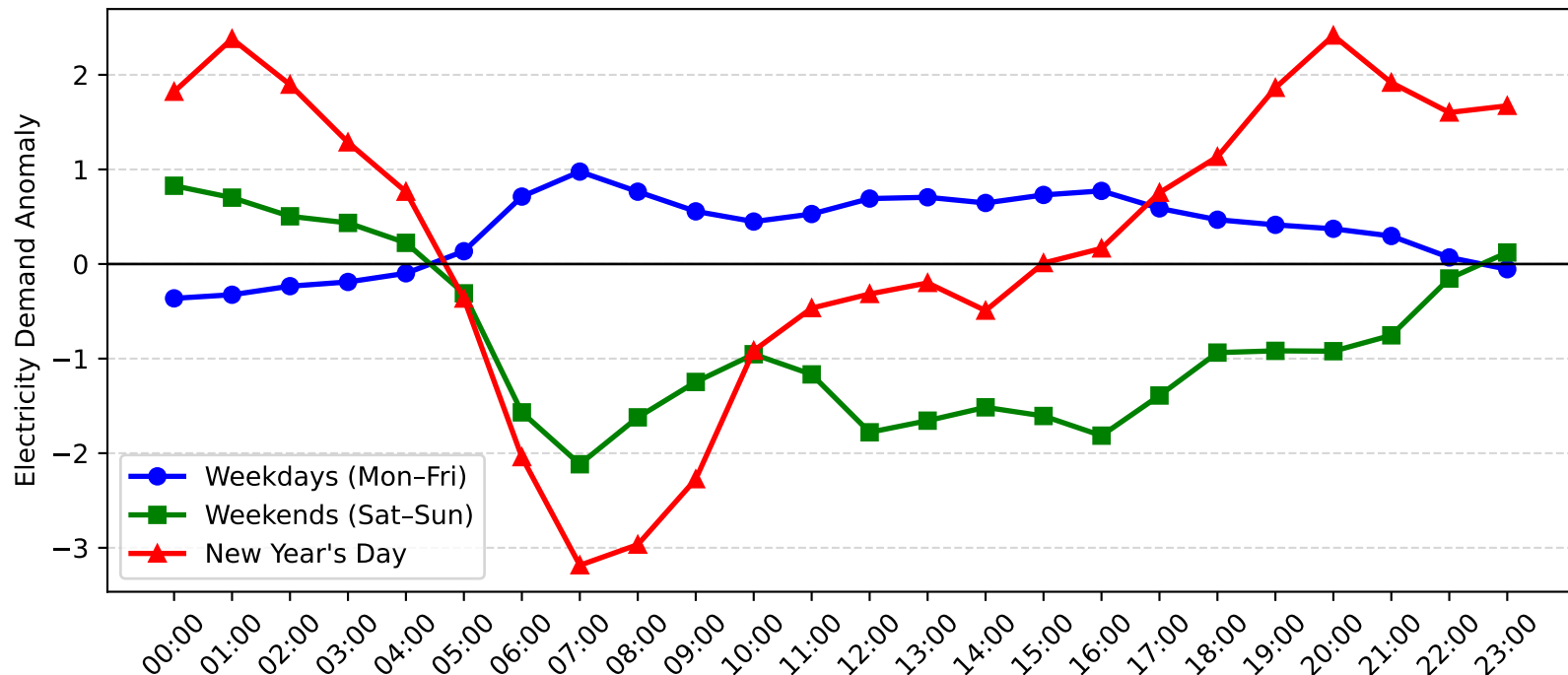
Five Dock Demand Anomaly: New Year's Day vs Weekday/Weekend (2005-2006)
