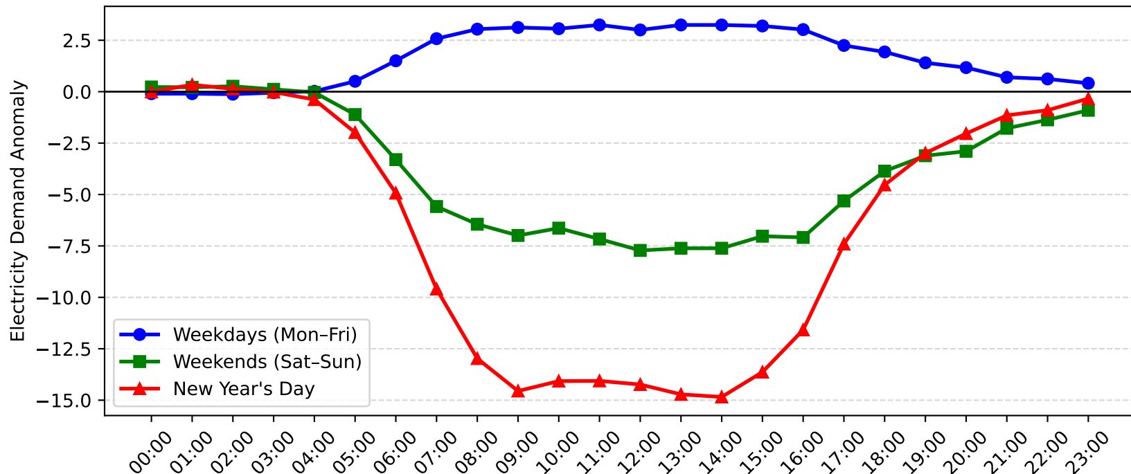
Brookvale Demand Anomaly: New Year's Day vs Weekday/Weekend (2005-2006)
