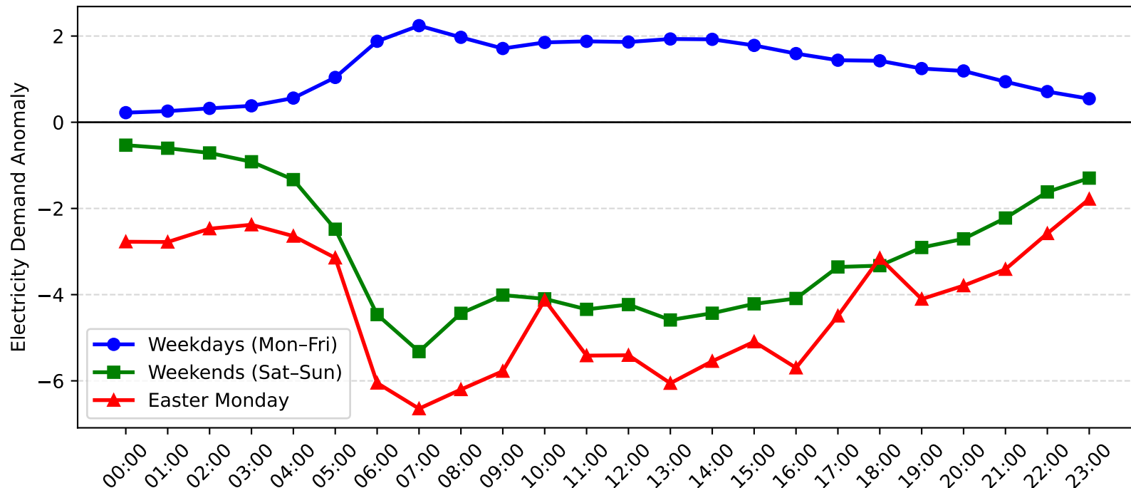
Matraverse Demand Anomaly: Easter Monday vs Weekday/Weekend (2006-2007)
