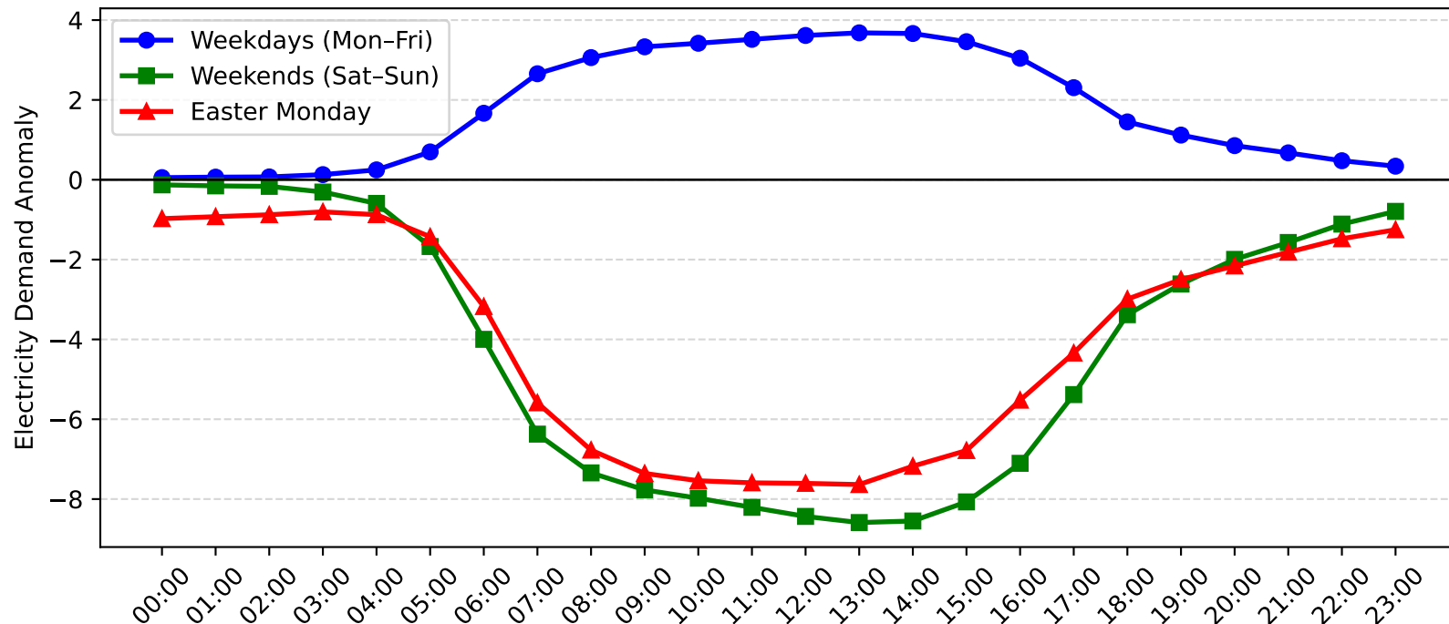
Mascot Demand Anomaly: Easter Monday vs Weekday/Weekend (2012-2013)
