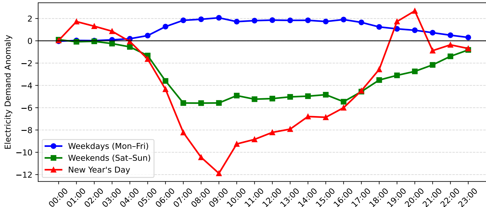
Burwood Demand Anomaly: New Year's Day vs Weekday/Weekend (2008-2009)
