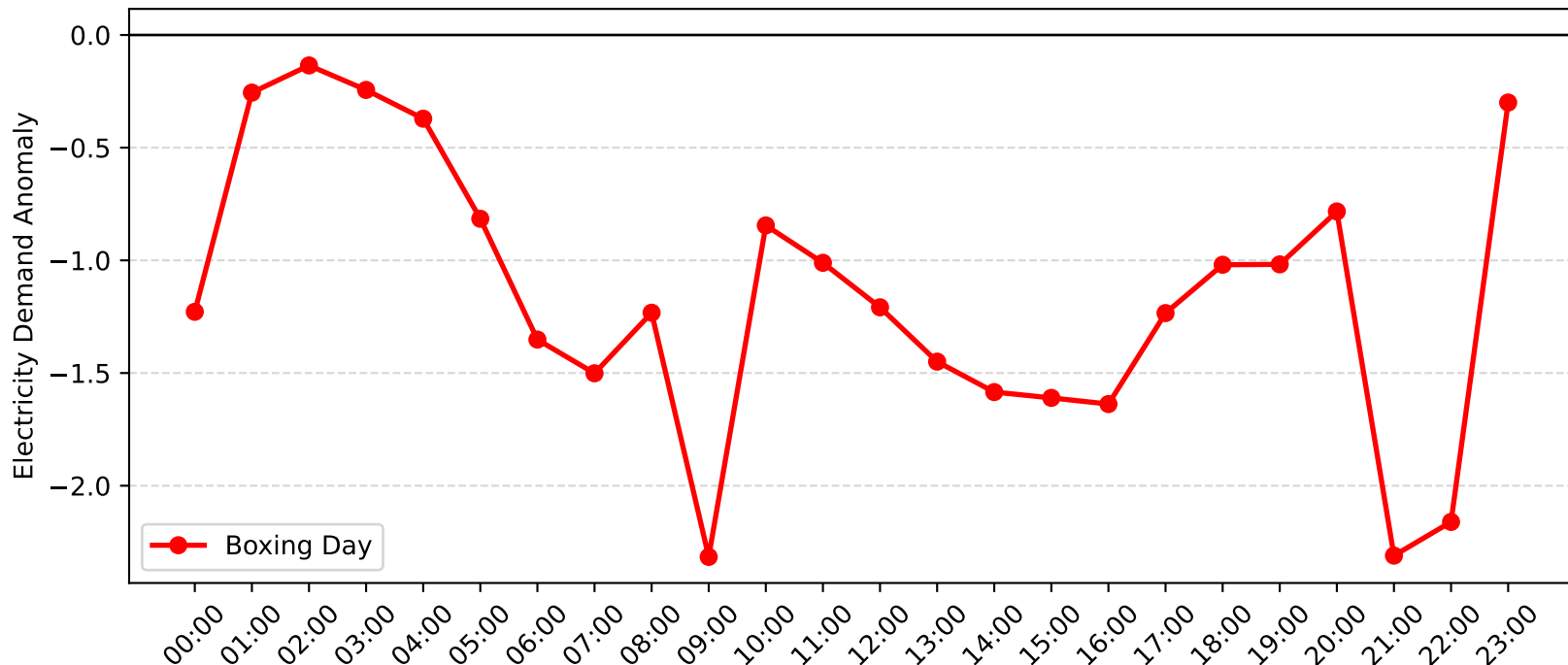
Narrabeen Demand Anomaly: Boxing Day (2008-2009)
