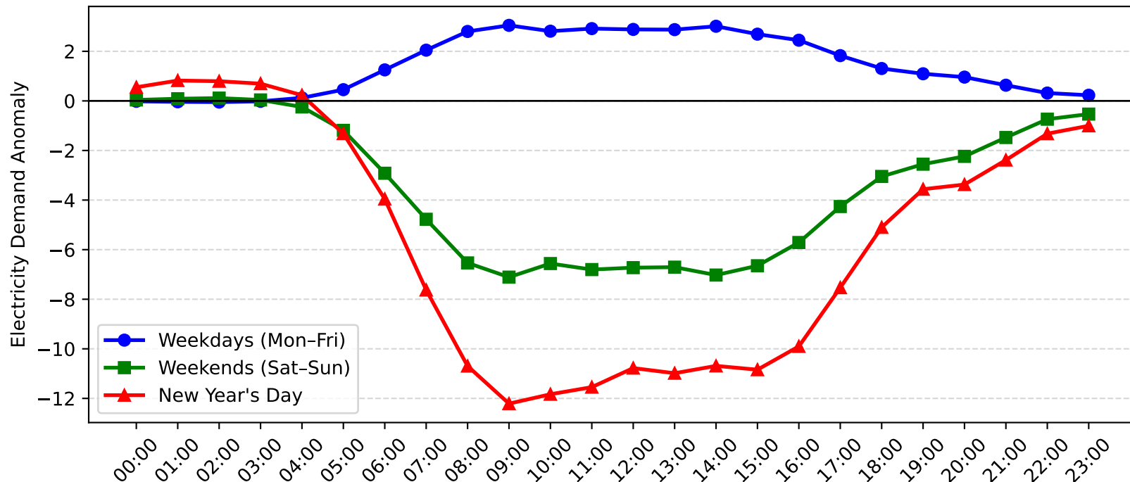
Brookvale Demand Anomaly: New Year's Day vs Weekday/Weekend (2017-2018)
