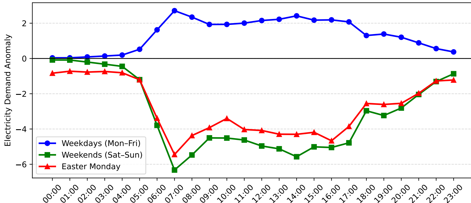
Epping Demand Anomaly: Easter Monday vs Weekday/Weekend (2013-2014)
