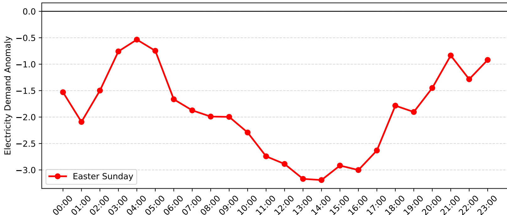
Gateshead Demand Anomaly: Easter Sunday (2005-2006)
