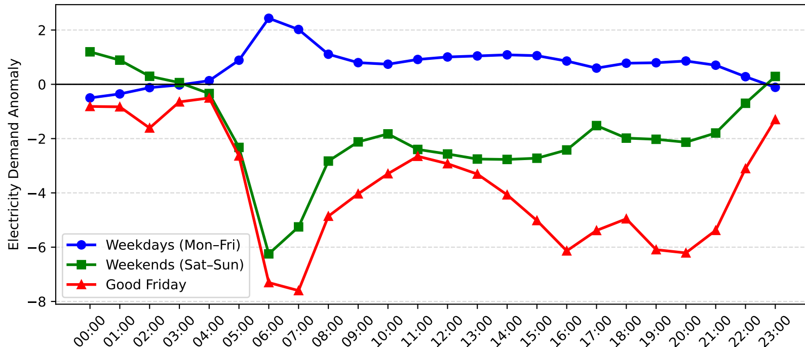
Pennant Hills Demand Anomaly: Good Friday vs Weekday/Weekend (2006-2007)
