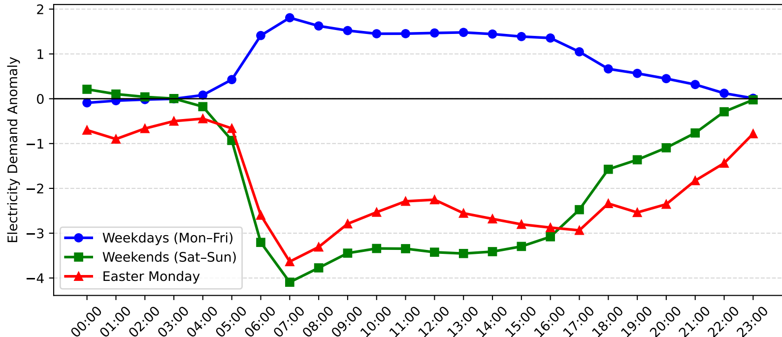
Pymble Demand Anomaly: Easter Monday vs Weekday/Weekend (2010-2011)
