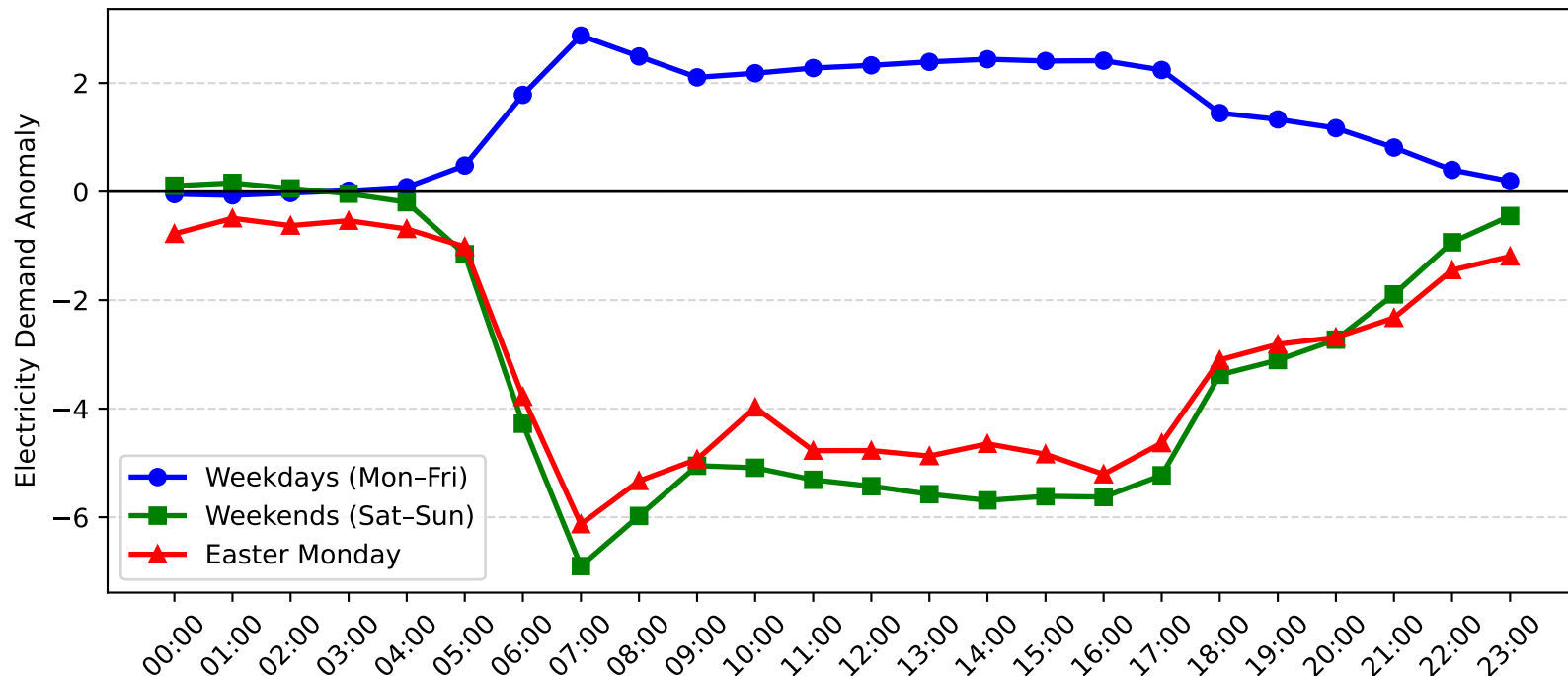
Epping Demand Anomaly: Easter Monday vs Weekday/Weekend (2012-2013)
