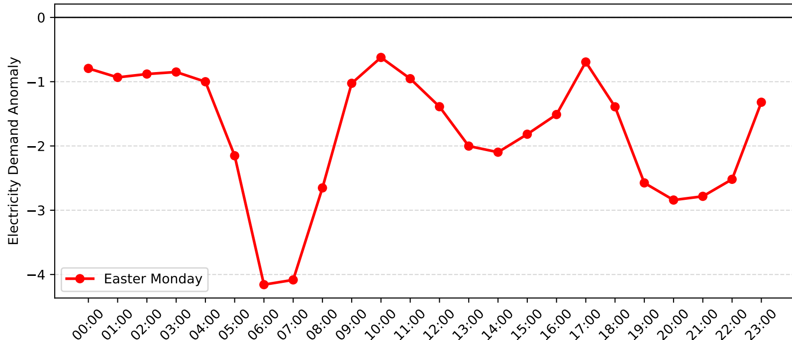
Cronulla Demand Anomaly: Easter Monday (2017-2018)
