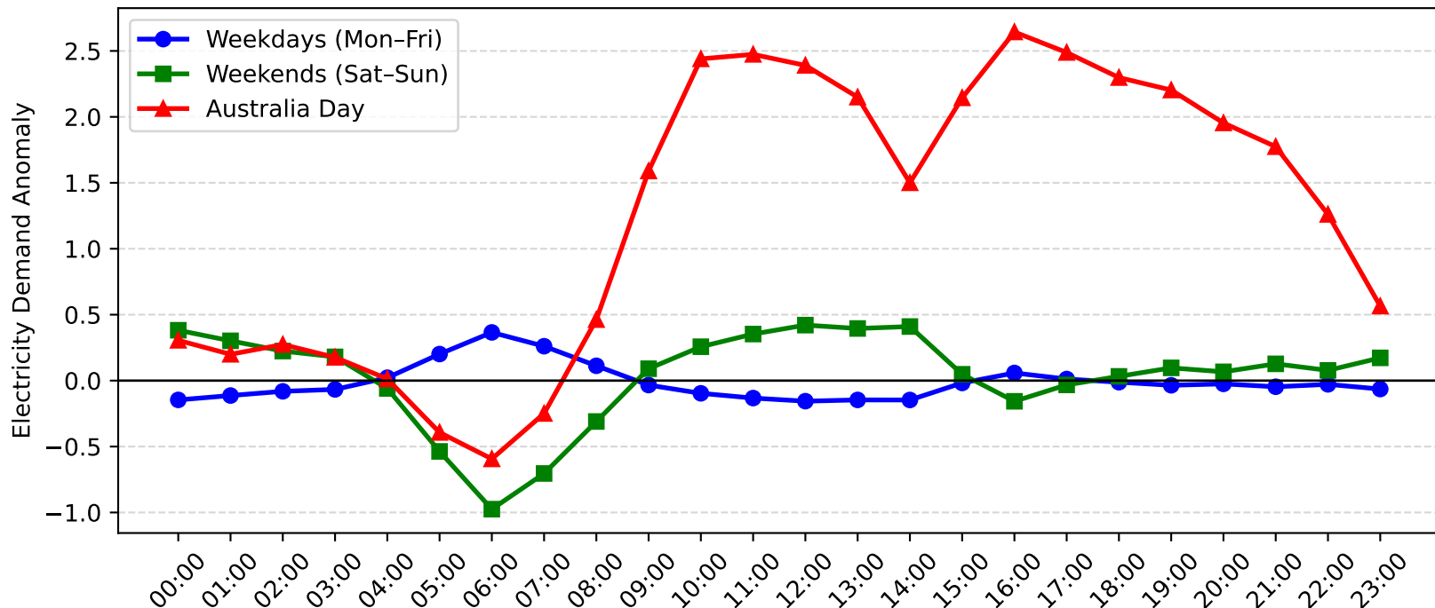
Woy Woy Demand Anomaly: Australia Day vs Weekday/Weekend (2011-2012)
