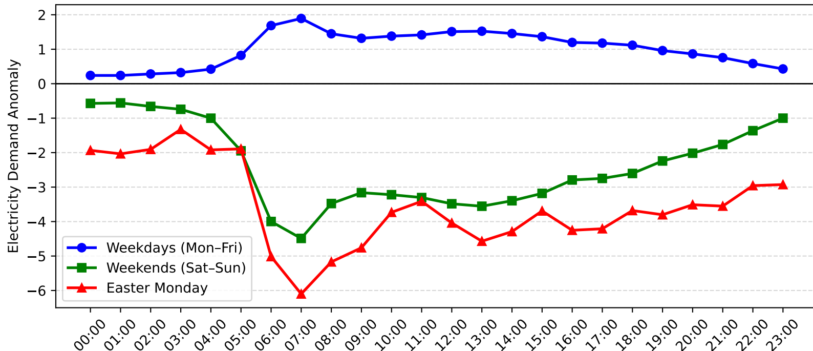
Matraverse Demand Anomaly: Easter Monday vs Weekday/Weekend (2011-2012)
