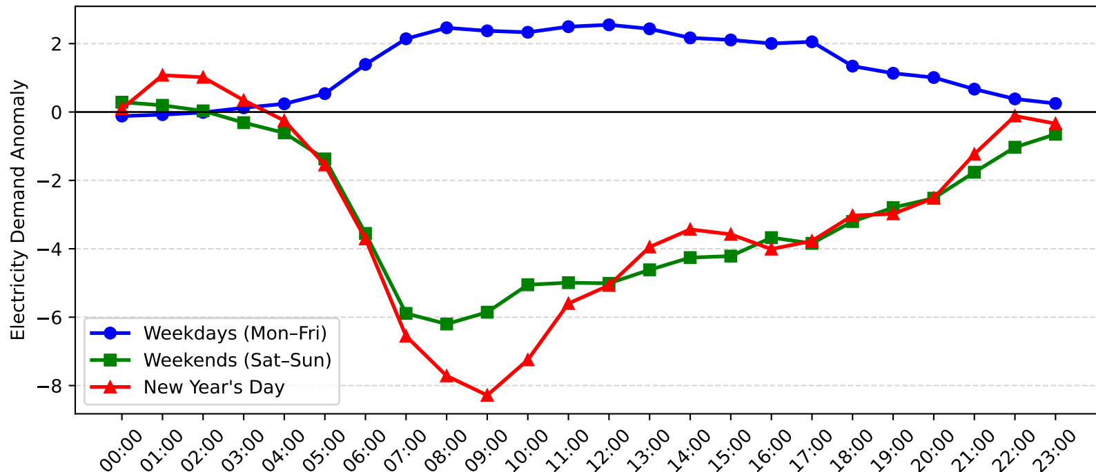
Burwood Demand Anomaly: New Year's Day vs Weekday/Weekend (2010-2011)
