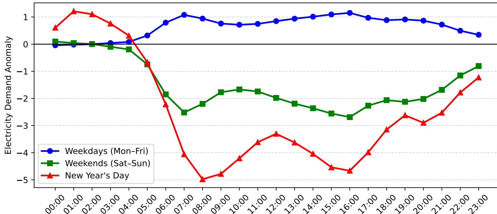
Five Dock Demand Anomaly: New Year's Day vs Weekday/Weekend (2017-2018)
