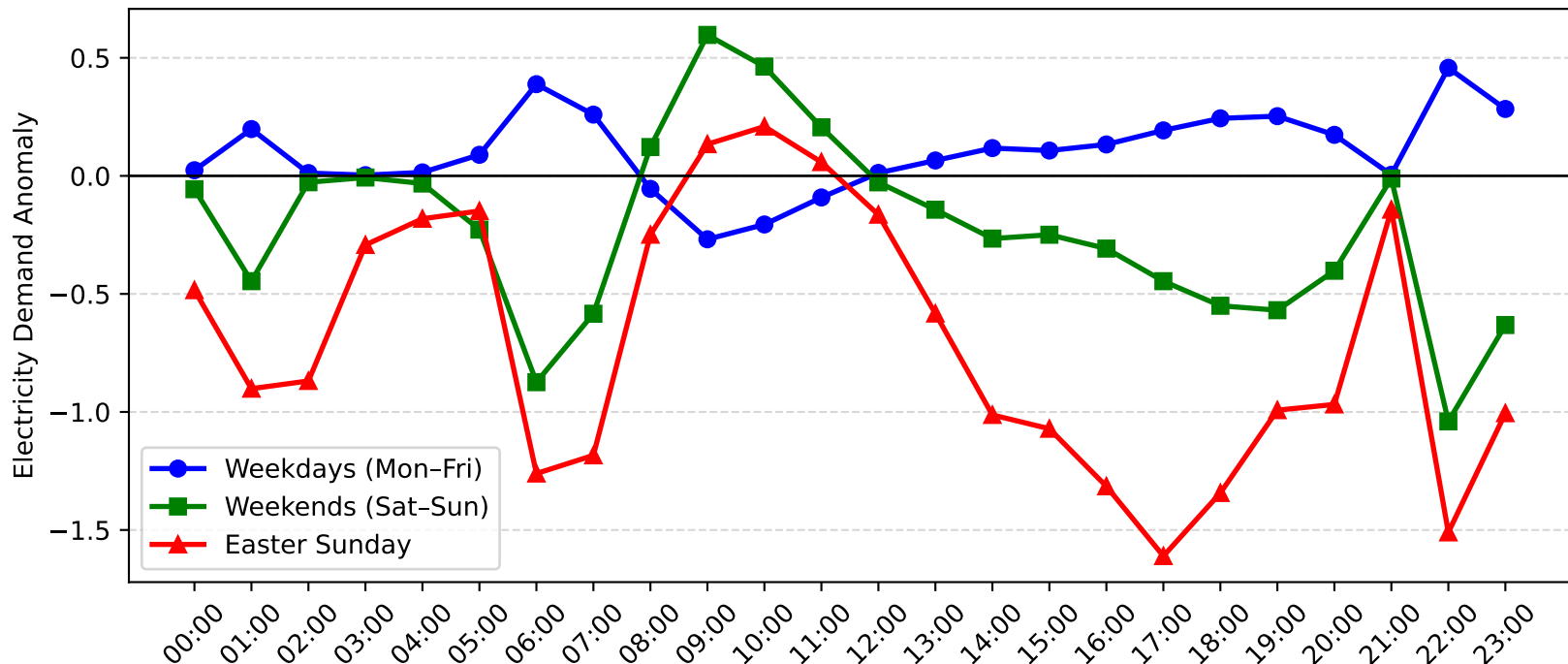
Jewells Demand Anomaly: Easter Sunday vs Weekday/Weekend (2007-2008)
