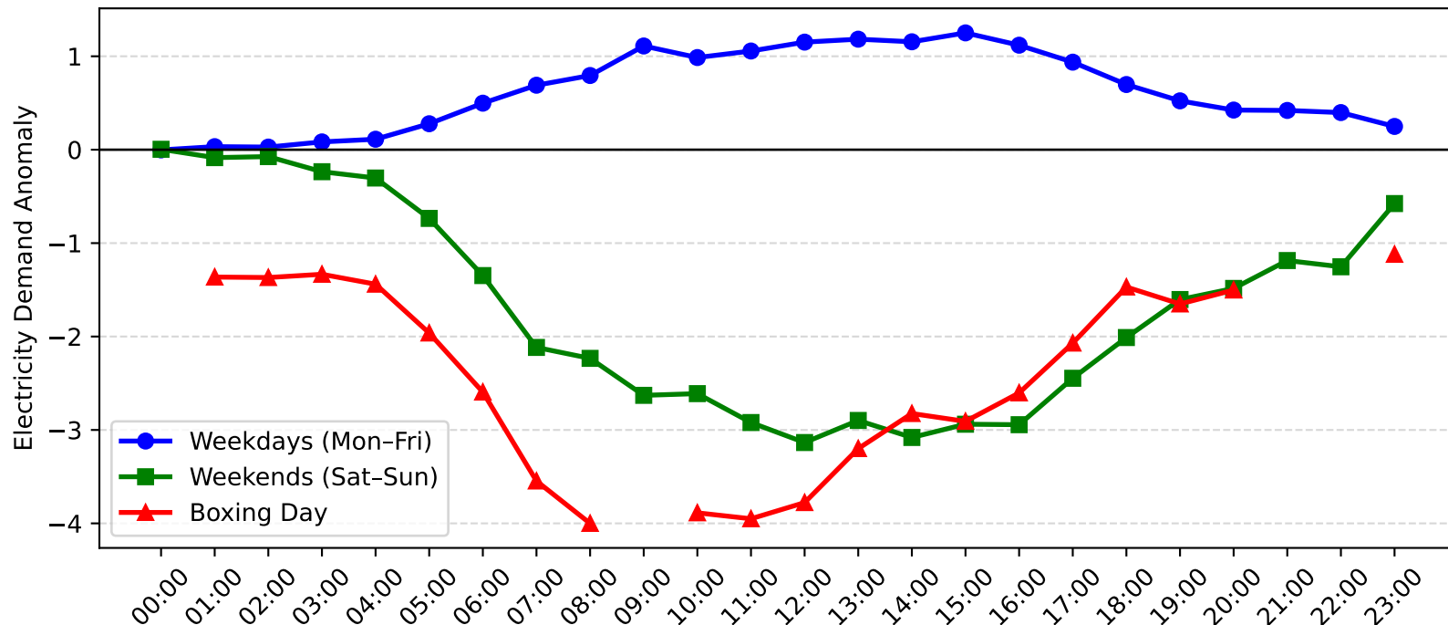
Lidcombe Demand Anomaly: Boxing Day vs Weekday/Weekend (2008-2009)
