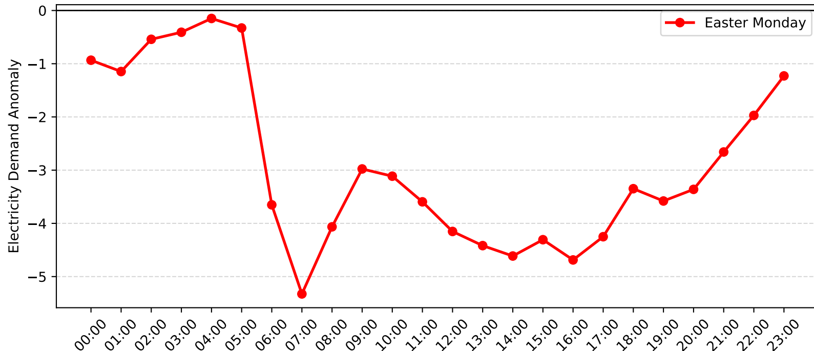
Epping Demand Anomaly: Easter Monday (2009-2010)
