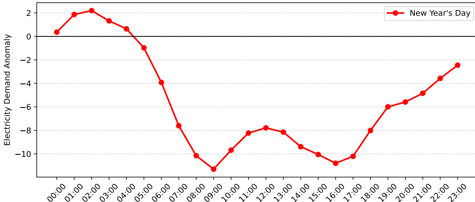
Burwood Demand Anomaly: New Year's Day (2017-2018)
