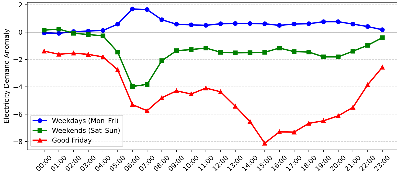
Pennant Hills Demand Anomaly: Good Friday vs Weekday/Weekend (2016-2017)
