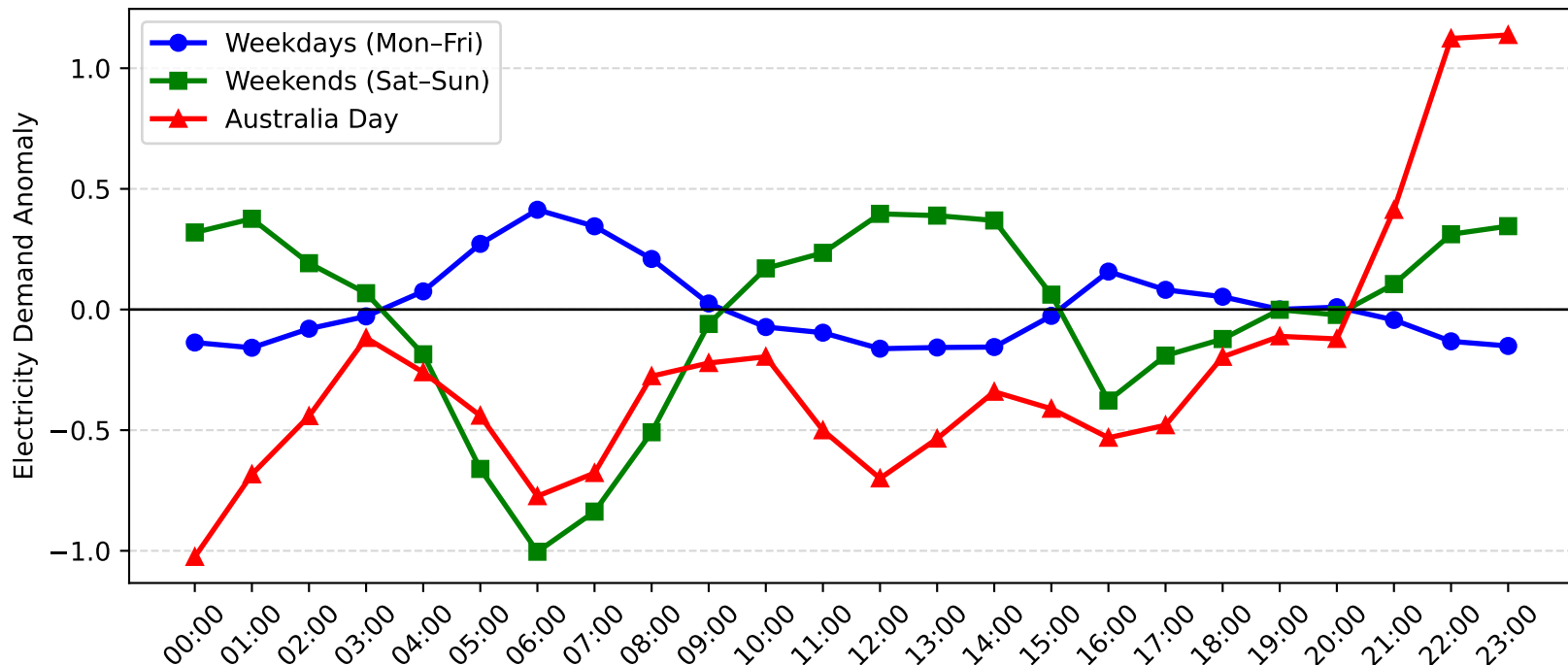
Woy Woy Demand Anomaly: Australia Day vs Weekday/Weekend (2007-2008)
