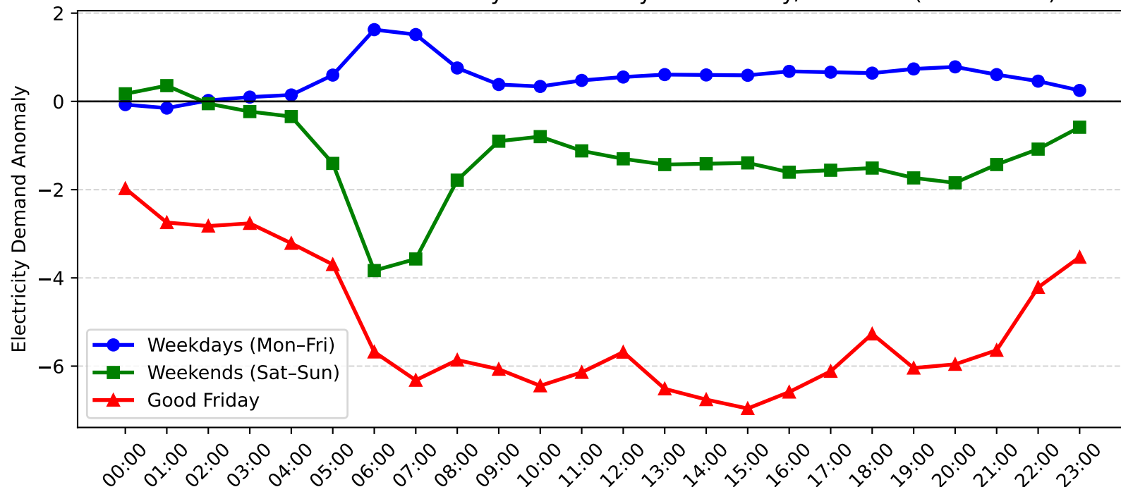
Pennant Hills Demand Anomaly: Good Friday vs Weekday/Weekend (2017-2018)
