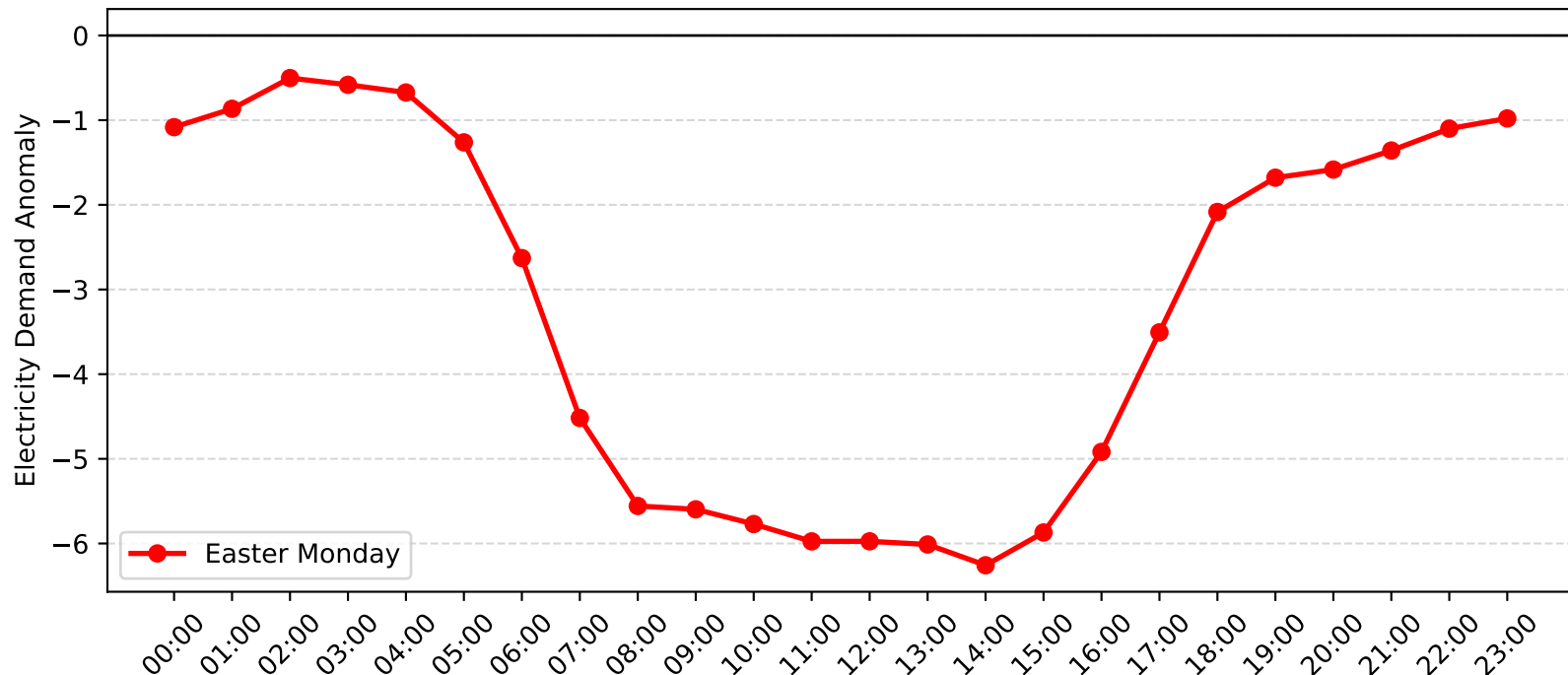
Mascot Demand Anomaly: Easter Monday (2015-2016)
