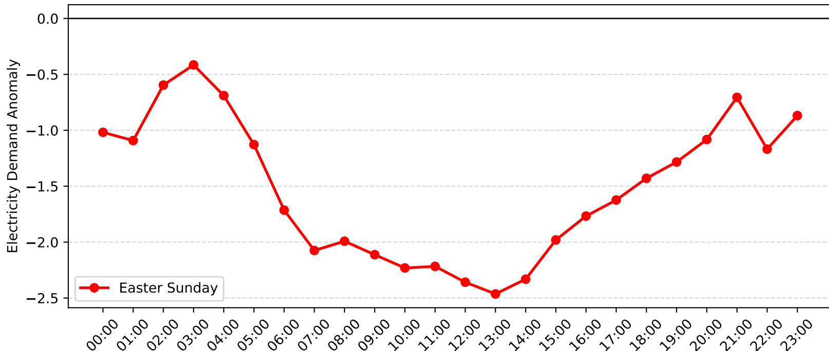
Gateshead Demand Anomaly: Easter Sunday (2016-2017)
