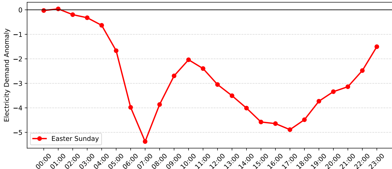
Dulwich Hill Demand Anomaly: Easter Sunday (2013-2014)
