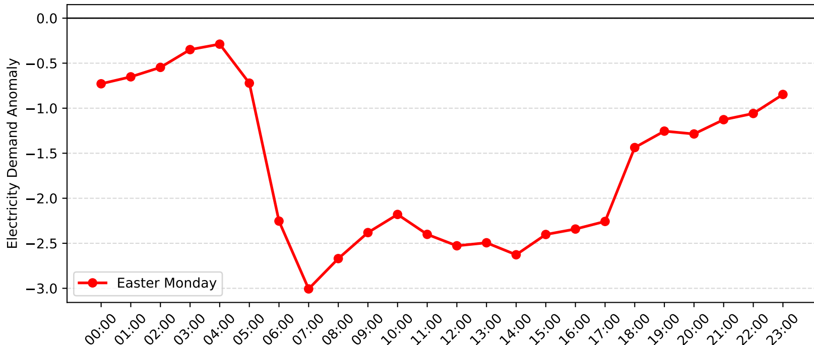
Pymble Demand Anomaly: Easter Monday (2012-2013)
