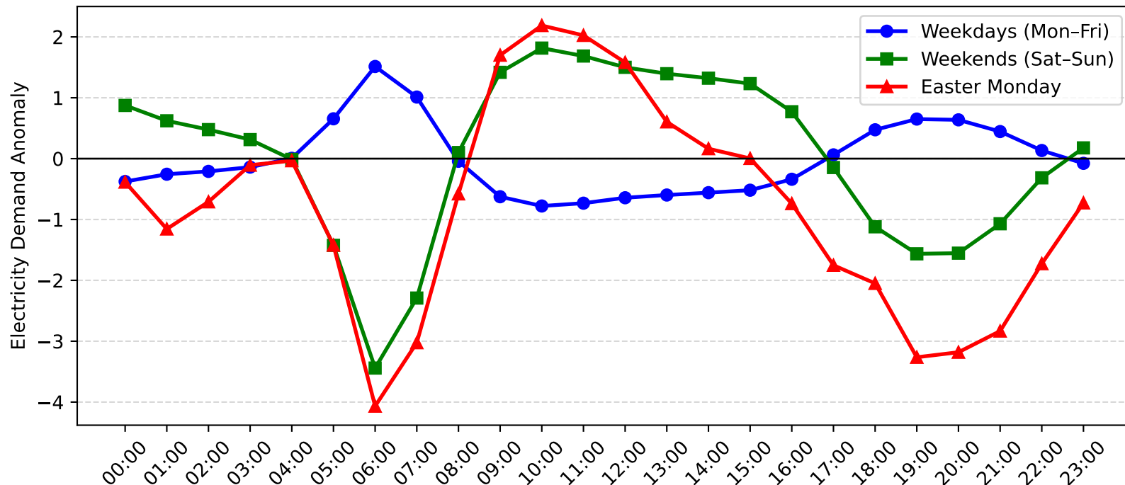
Cronulla Demand Anomaly: Easter Monday vs Weekday/Weekend (2010-2011)
