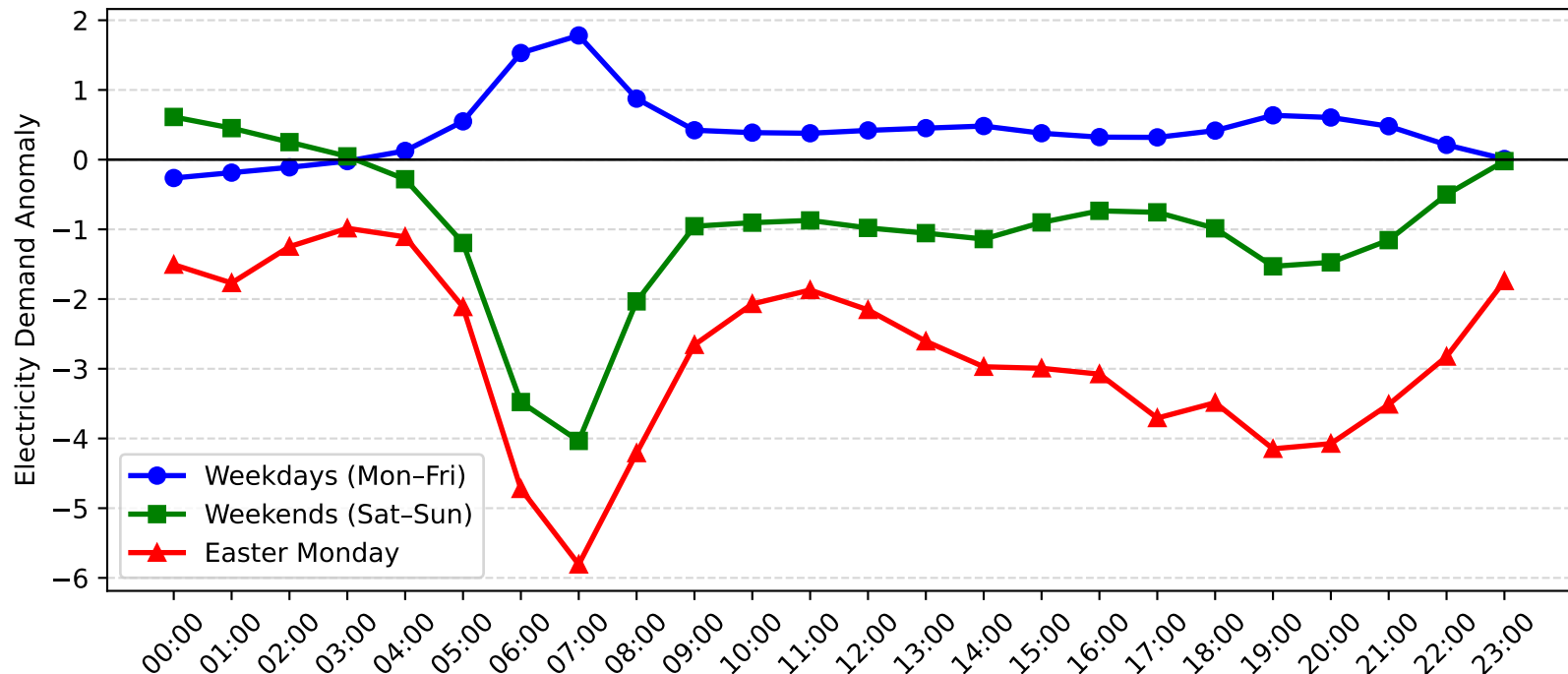
Mortdale Demand Anomaly: Easter Monday vs Weekday/Weekend (2010-2011)
