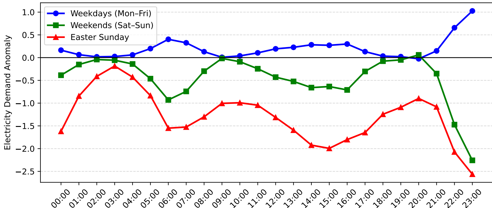
Muswellbrook Demand Anomaly: Easter Sunday vs Weekday/Weekend (2008-2009)
