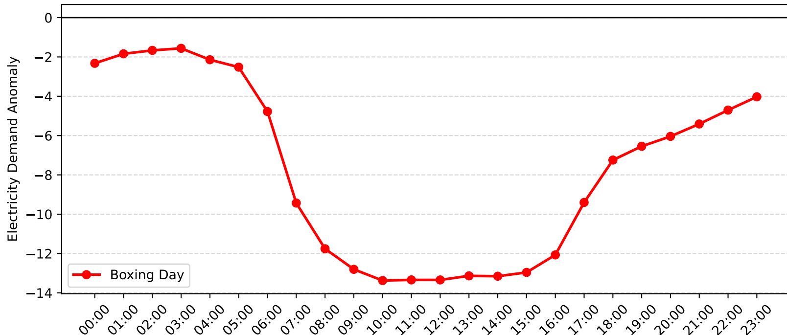
Gore Hill Demand Anomaly: Boxing Day (2012-2013)
