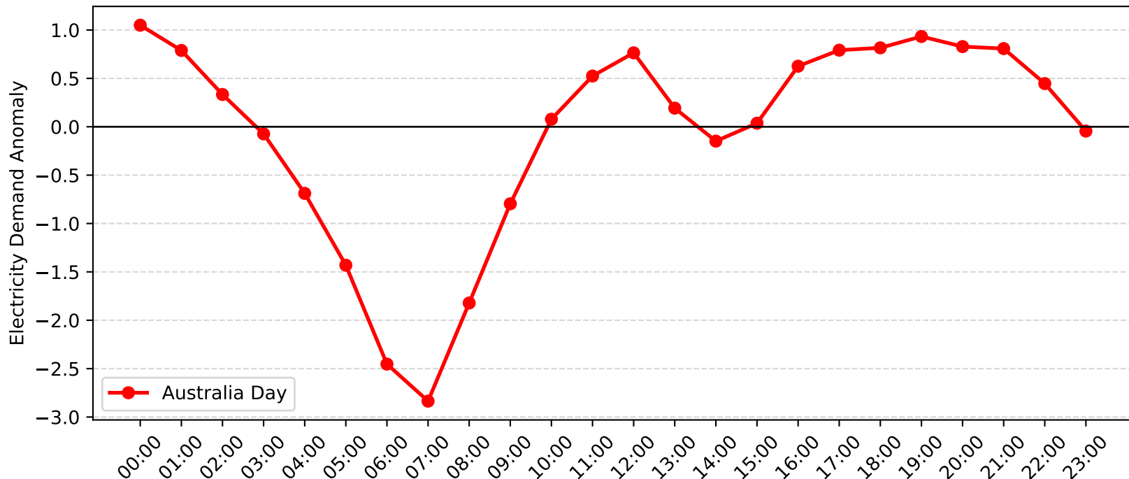
Lisarow Demand Anomaly: Australia Day (2011-2012)
