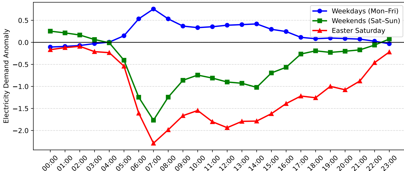
Arncliffe Demand Anomaly: Easter Saturday vs Weekday/Weekend (2013-2014)
