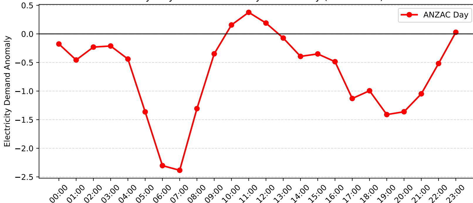
Woy Woy Demand Anomaly: ANZAC Day (2010-2011)
