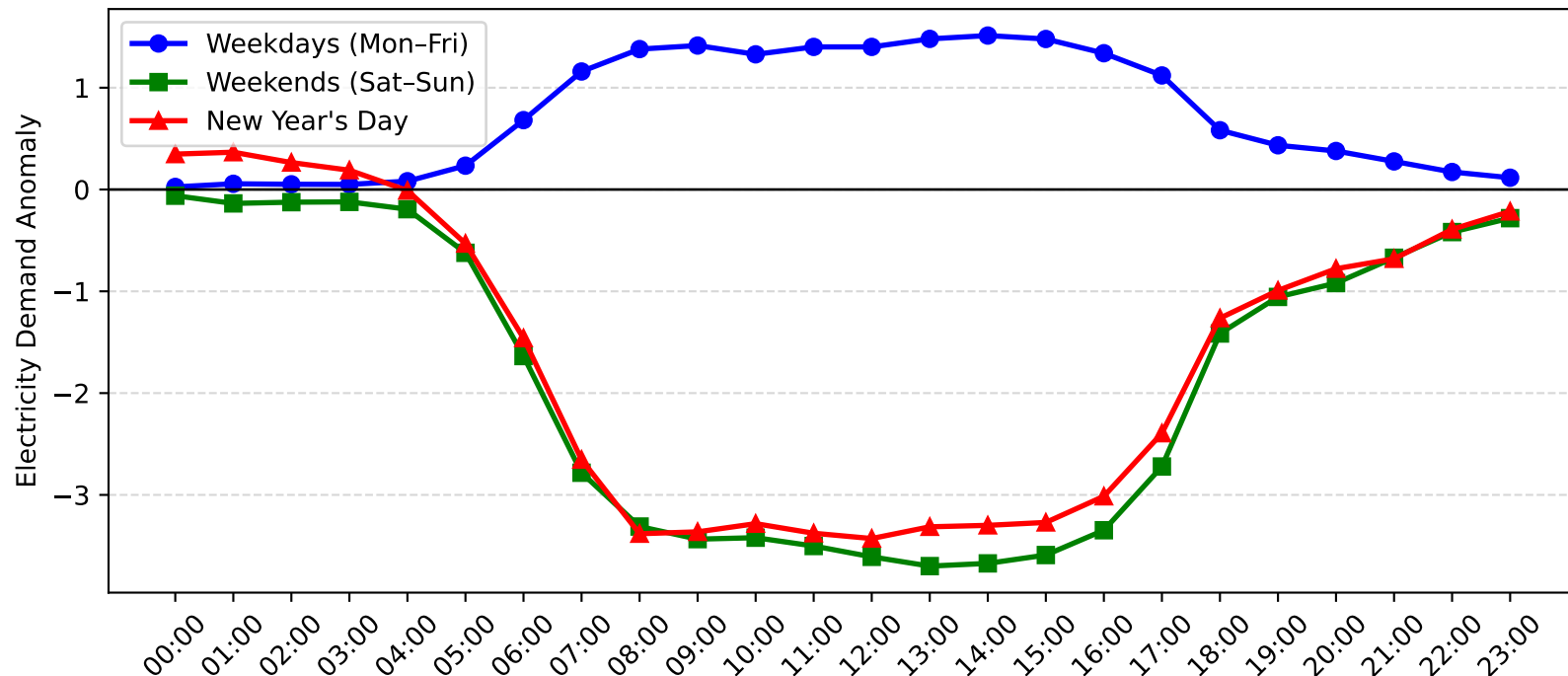
Beacon Hill Demand Anomaly: New Year's Day vs Weekday/Weekend (2016-2017)
