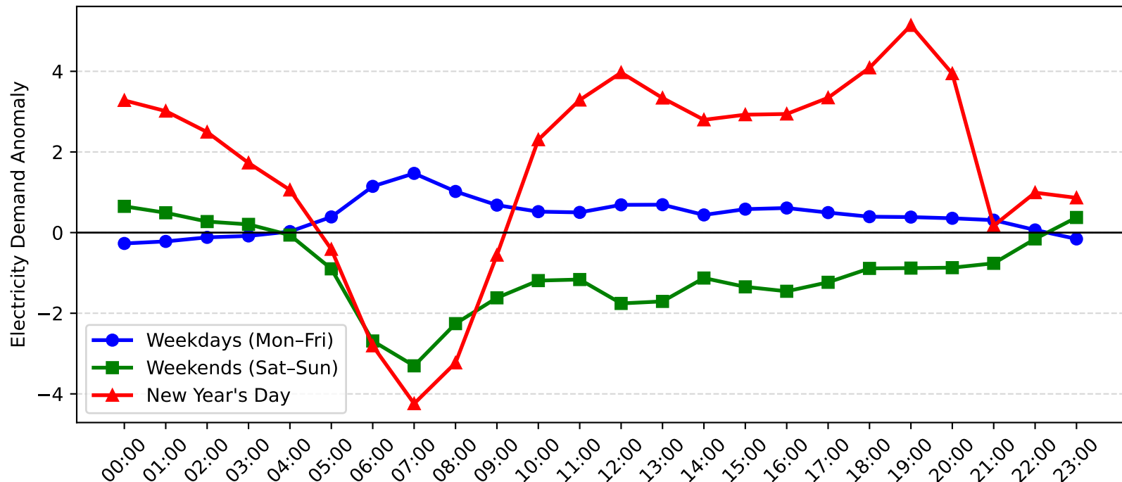
Mortdale Demand Anomaly: New Year's Day vs Weekday/Weekend (2006-2007)
