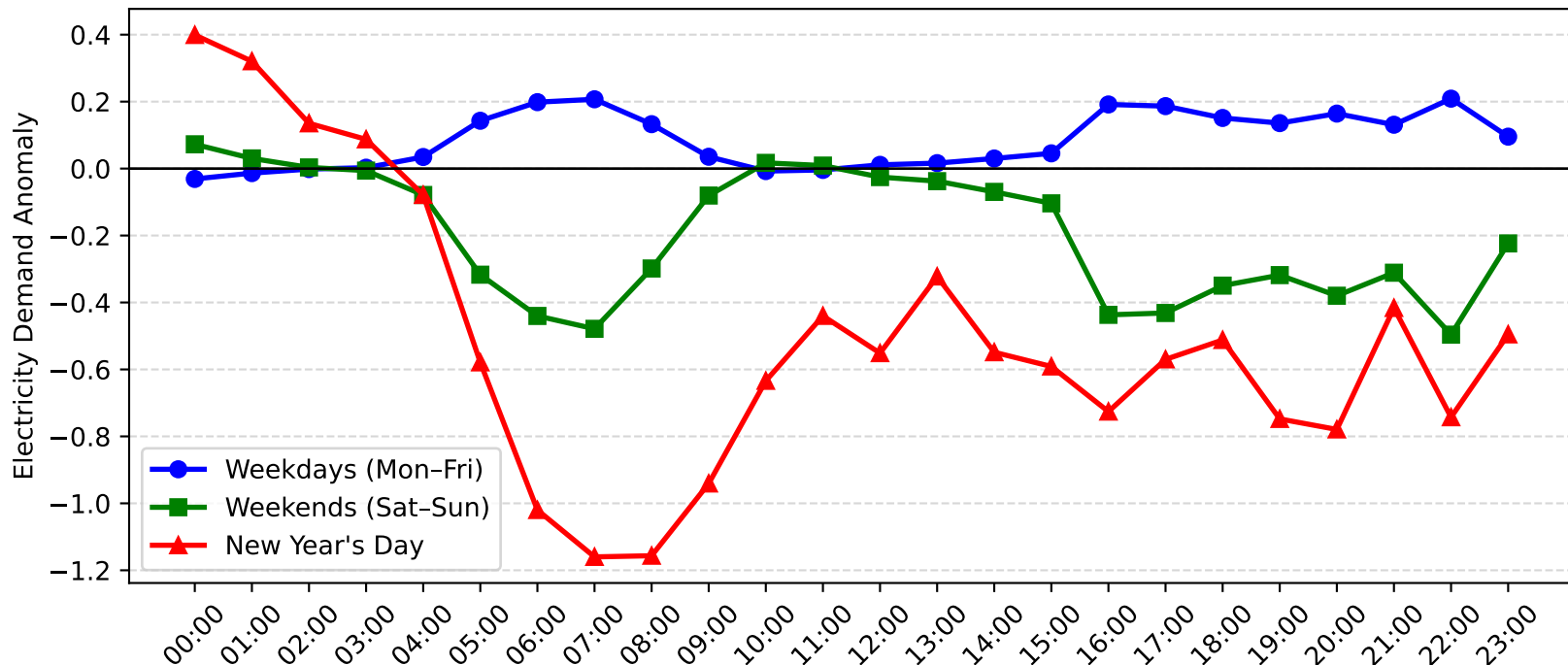
Narrabeen Demand Anomaly: New Year's Day vs Weekday/Weekend (2011-2012)
