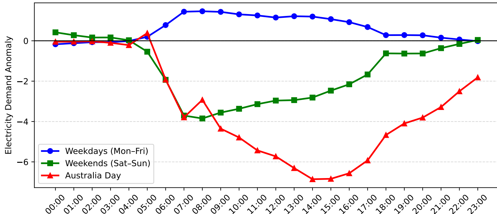
Concord Demand Anomaly: Australia Day vs Weekday/Weekend (2014-2015)
