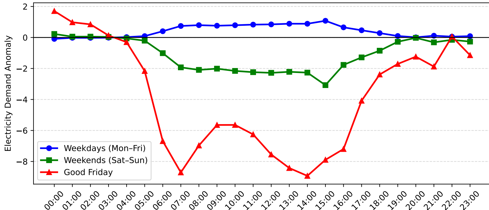
Hunters Hill Demand Anomaly: Good Friday vs Weekday/Weekend (2004-2005)
