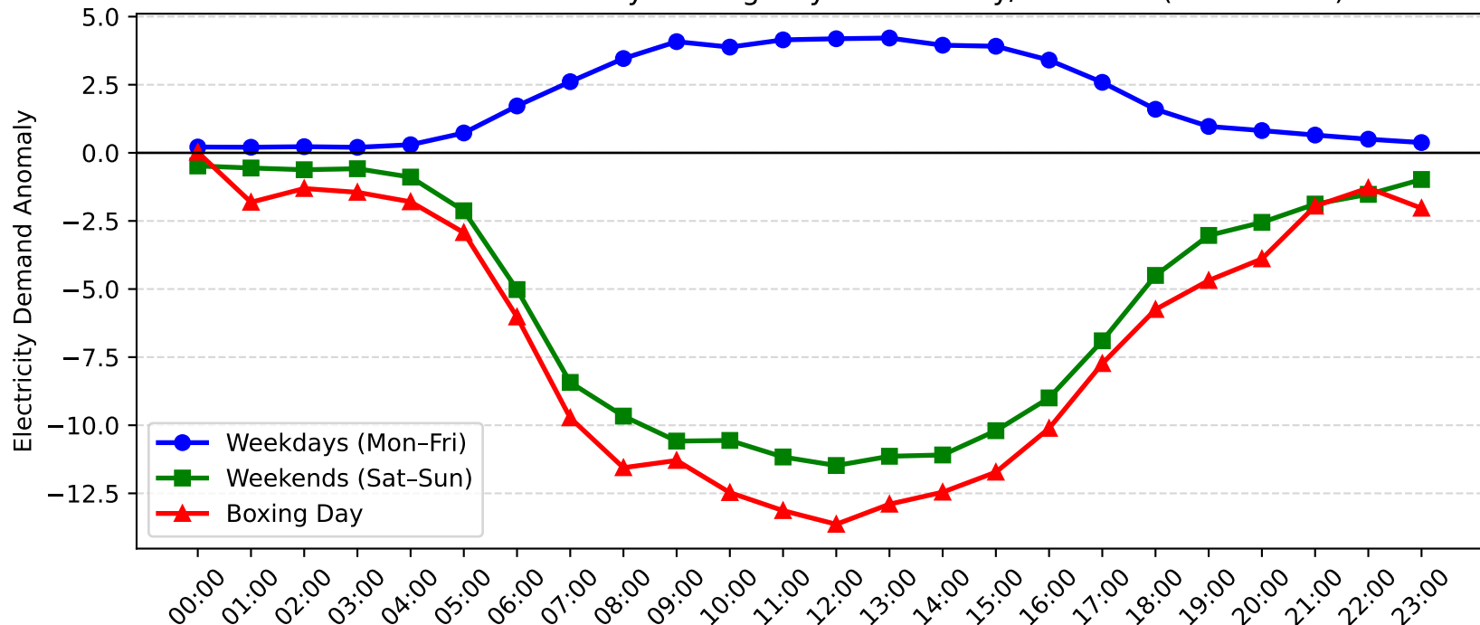
Mascot Demand Anomaly: Boxing Day vs Weekday/Weekend (2008-2009)
