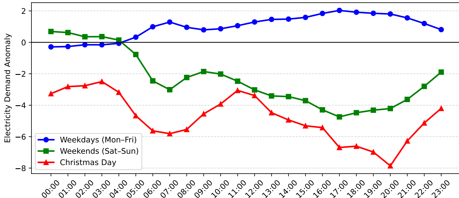
Pennant Hills Demand Anomaly: Christmas Day vs Weekday/Weekend (2016-2017)
