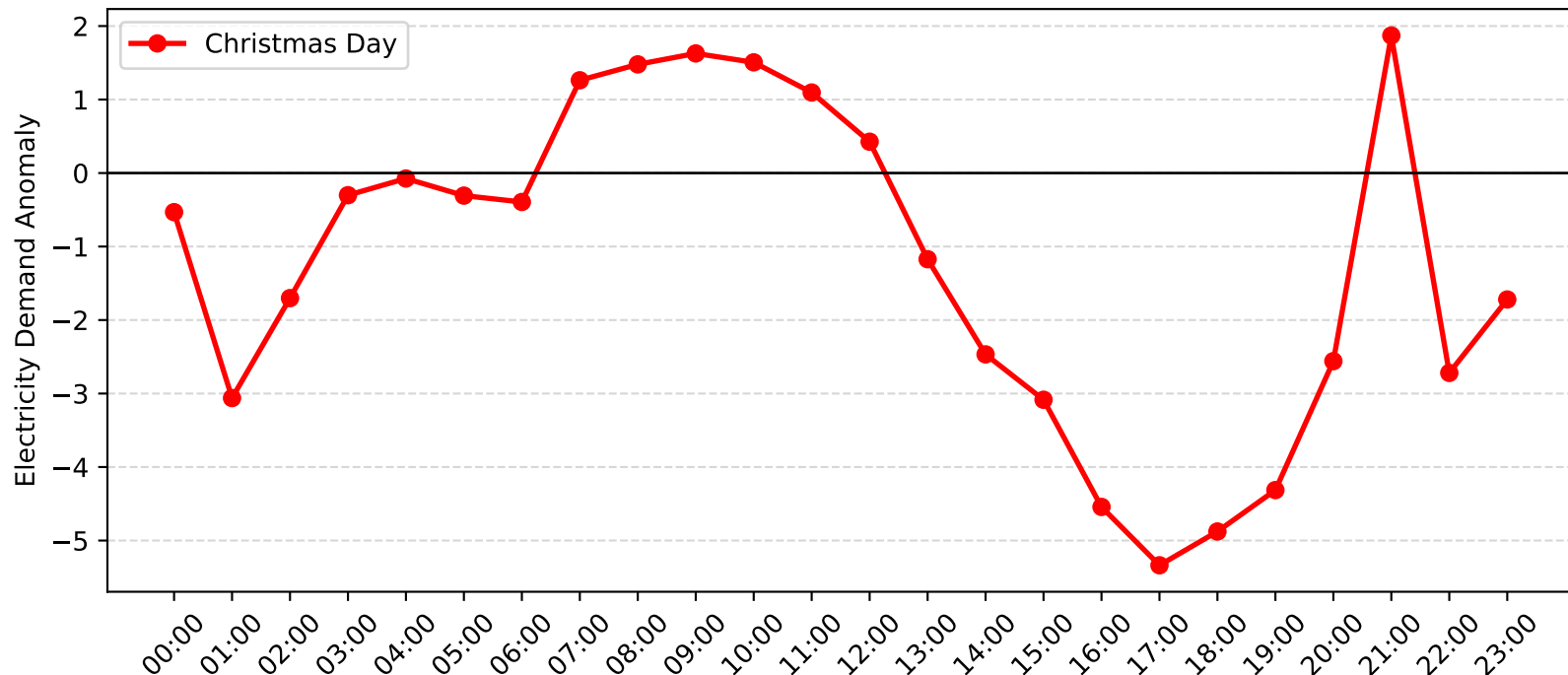
Nelson Bay Demand Anomaly: Christmas Day (2005-2006)
