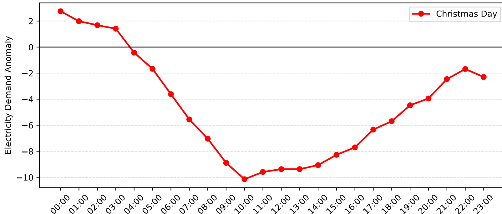
Meadowbank Demand Anomaly: Christmas Day (2004-2005)
