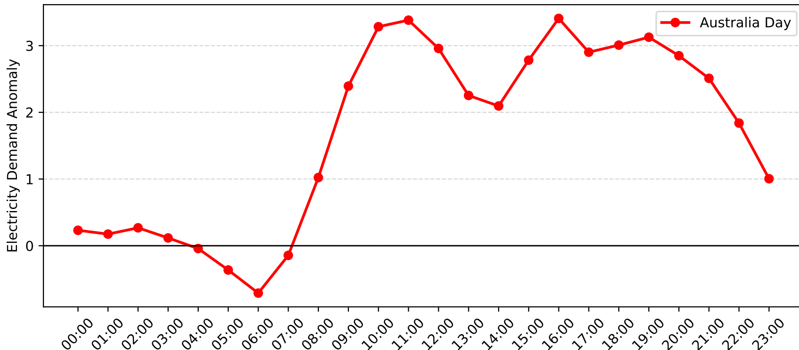
Umina Demand Anomaly: Australia Day (2011-2012)
