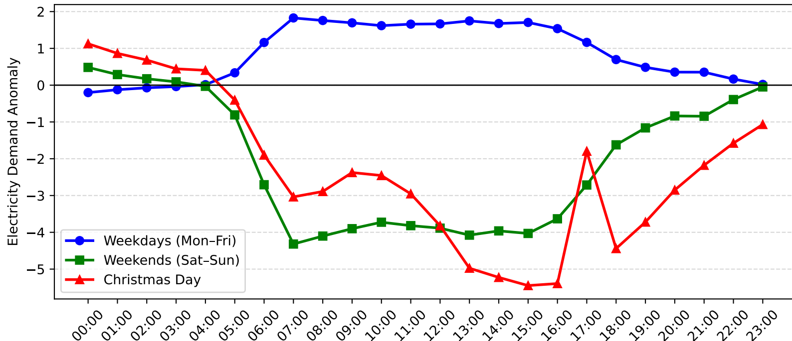
Hunters Hill Demand Anomaly: Christmas Day vs Weekday/Weekend (2011-2012)
