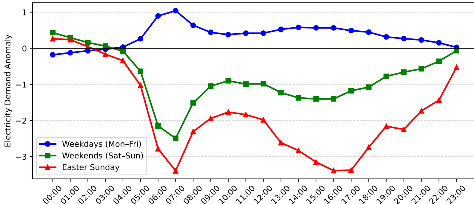
Blakehurst Demand Anomaly: Easter Sunday vs Weekday/Weekend (2007-2008)
