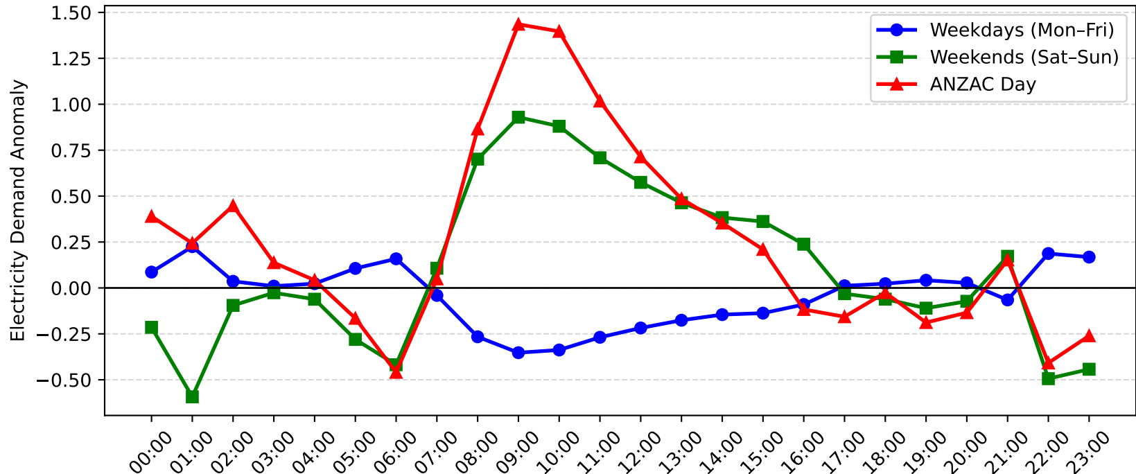
Swansea Demand Anomaly: ANZAC Day vs Weekday/Weekend (2013-2014)
