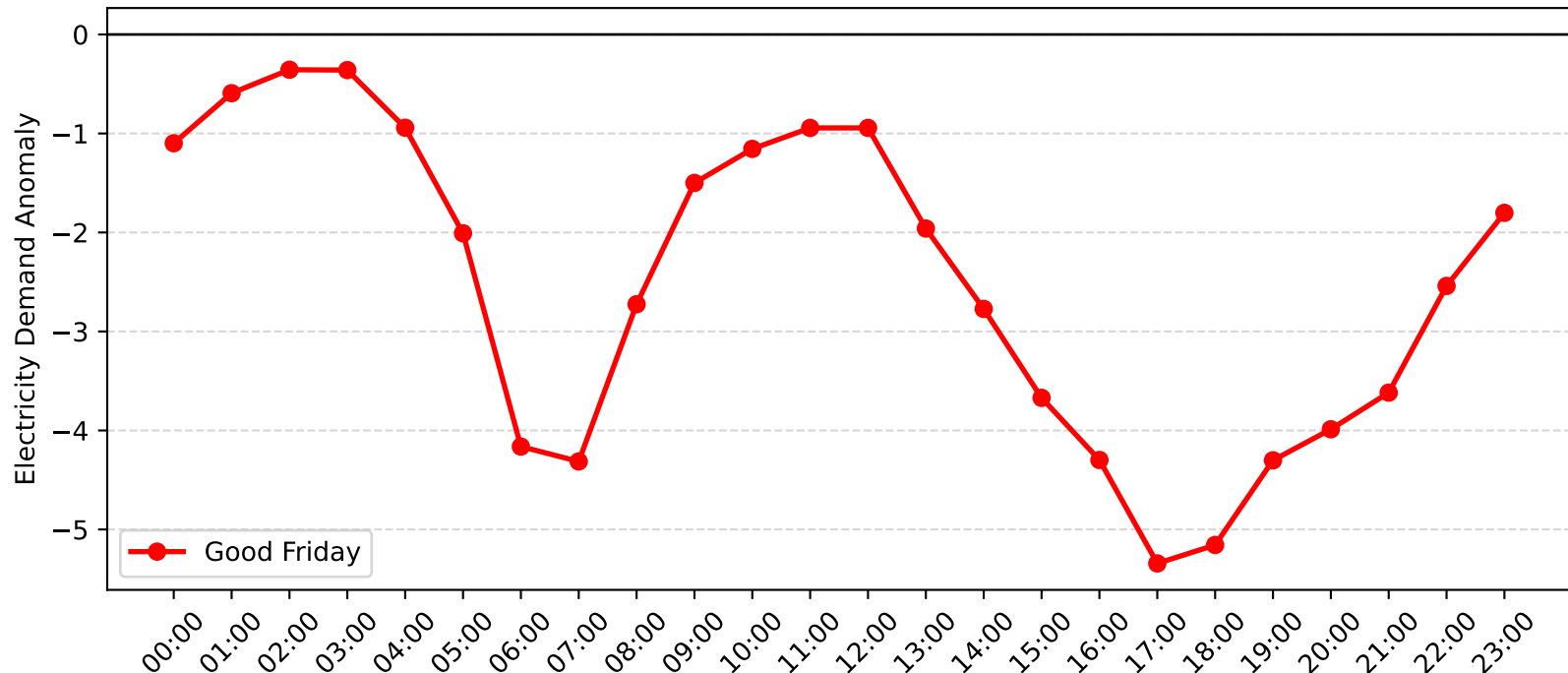
Revesby Demand Anomaly: Good Friday (2015-2016)
