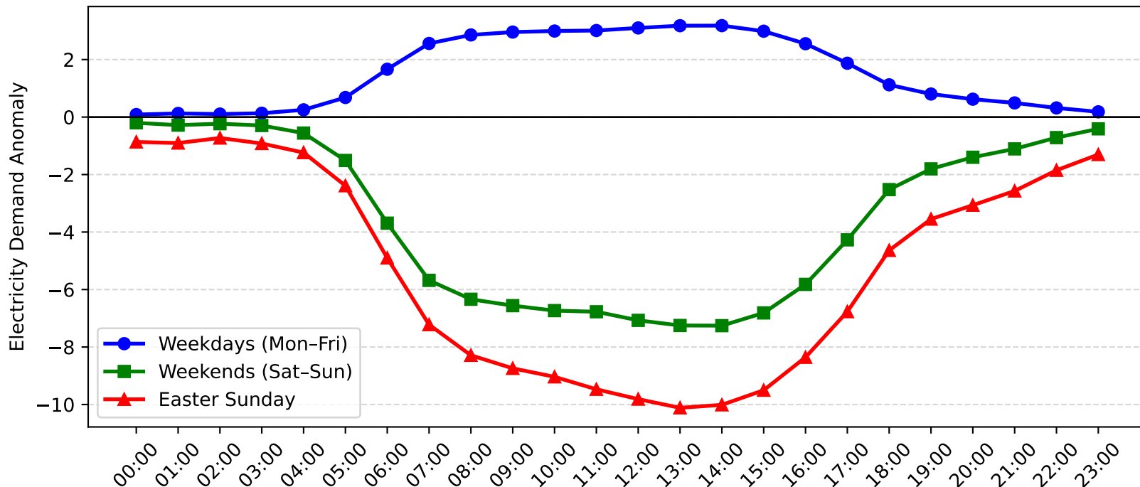
Mascot Demand Anomaly: Easter Sunday vs Weekday/Weekend (2016-2017)
