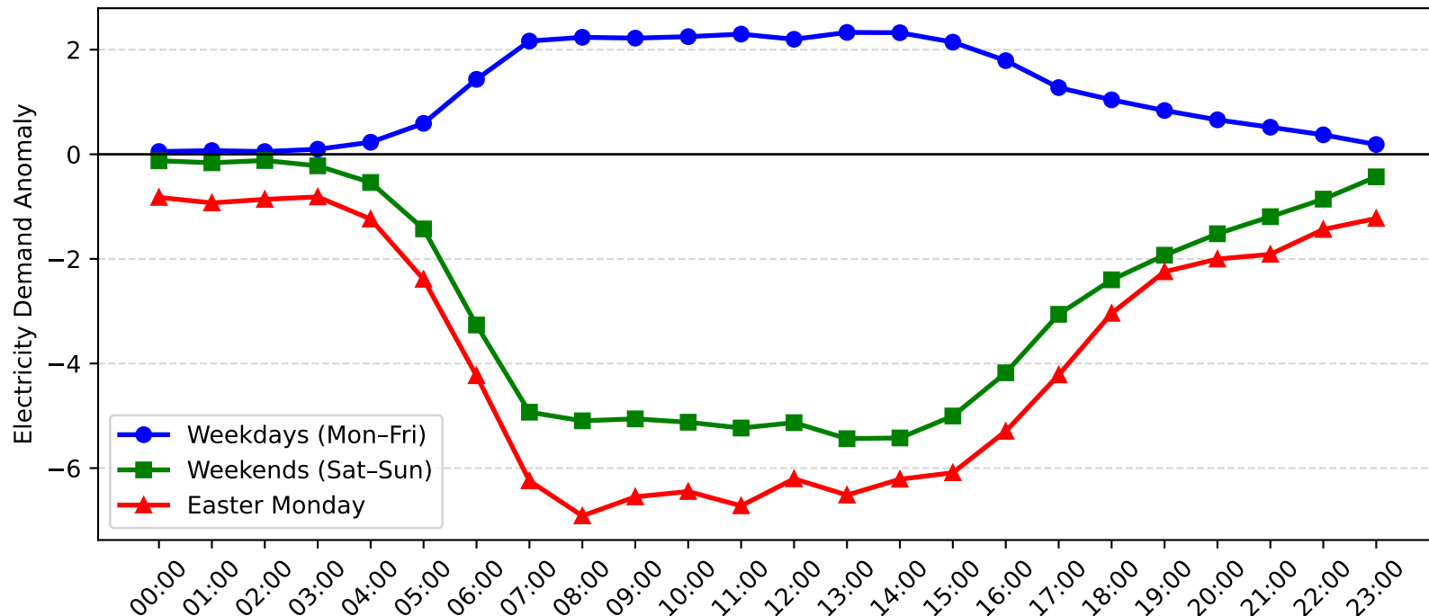
Bankstown Demand Anomaly: Easter Monday vs Weekday/Weekend (2015-2016)
