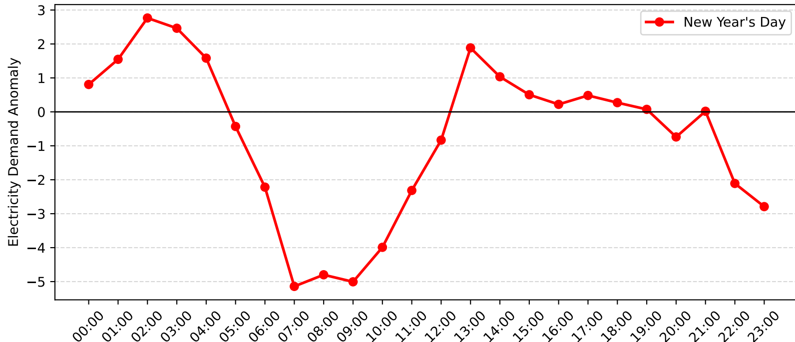
Meadowbank Demand Anomaly: New Year's Day (2013-2014)
