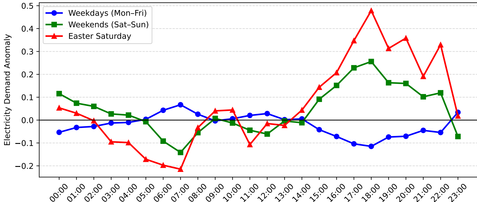
Rothbury Demand Anomaly: Easter Saturday vs Weekday/Weekend (2009-2010)
