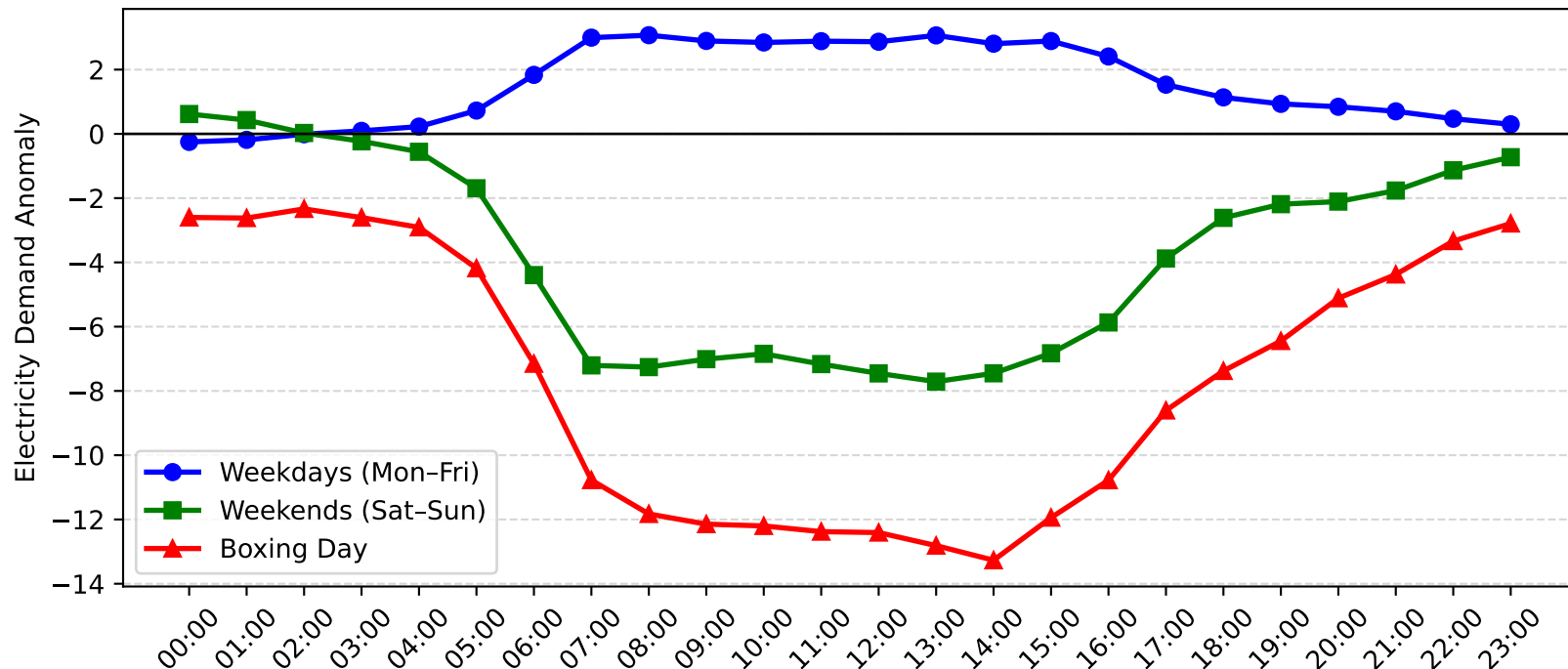
Marrickville Demand Anomaly: Boxing Day vs Weekday/Weekend (2005-2006)
