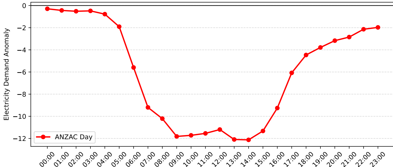
Zetland Demand Anomaly: ANZAC Day (2006-2007)
