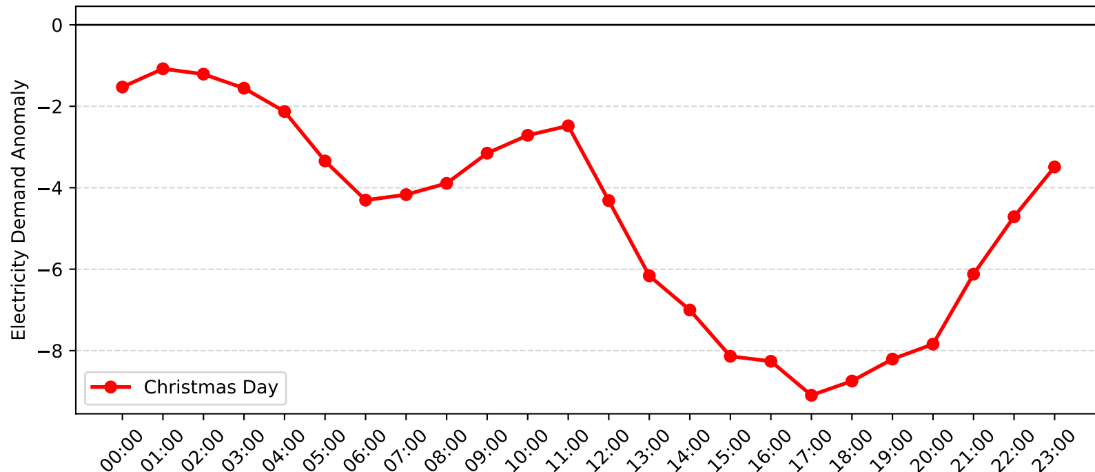
Pennant Hills Demand Anomaly: Christmas Day (2015-2016)
