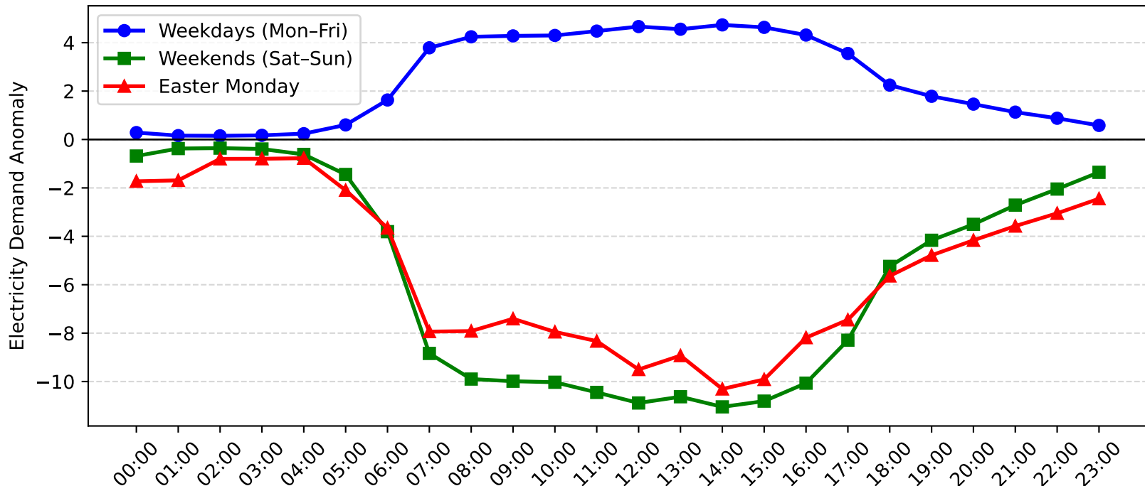
Gore Hill Demand Anomaly: Easter Monday vs Weekday/Weekend (2013-2014)
