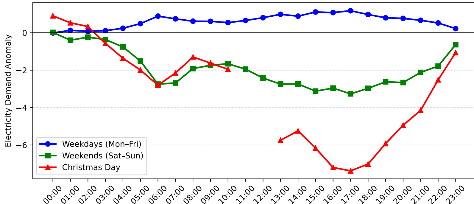
Revesby Demand Anomaly: Christmas Day vs Weekday/Weekend (2008-2009)
