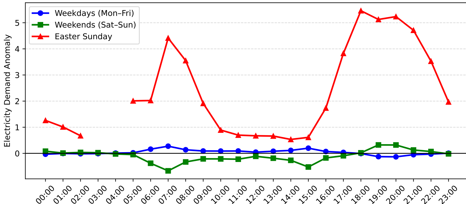
Blakehurst Demand Anomaly: Easter Sunday vs Weekday/Weekend (2004-2005)
