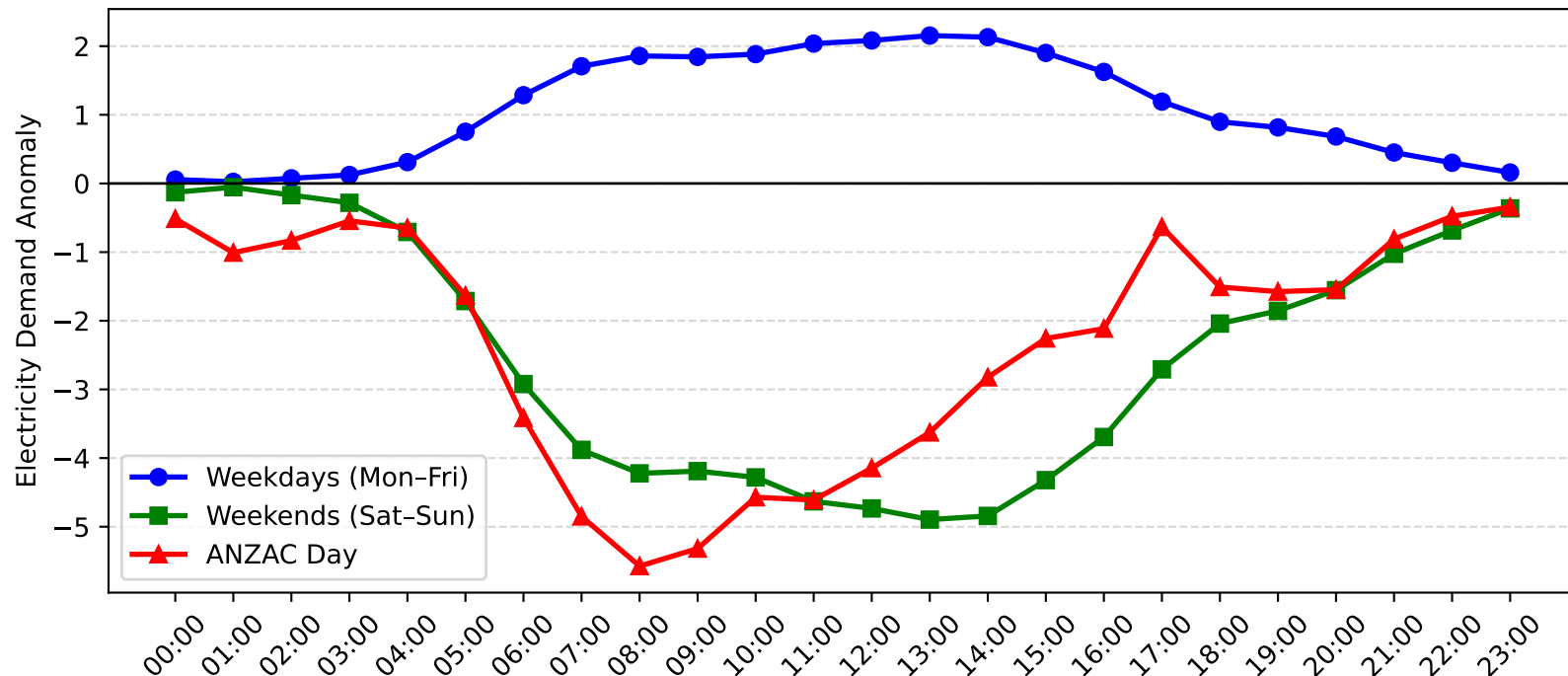
West Gosford Demand Anomaly: ANZAC Day vs Weekday/Weekend (2017-2018)
