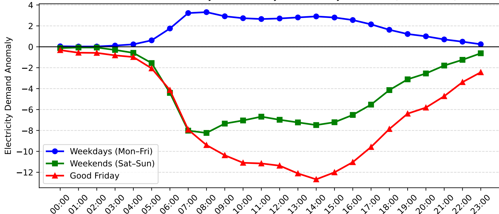
Zetland Demand Anomaly: Good Friday vs Weekday/Weekend (2015-2016)
