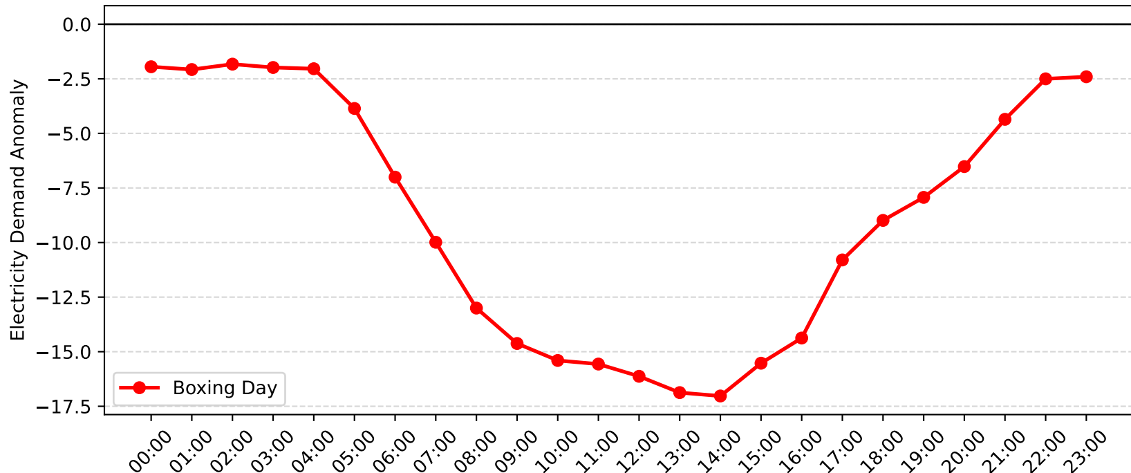
Zetland Demand Anomaly: Boxing Day (2004-2005)
