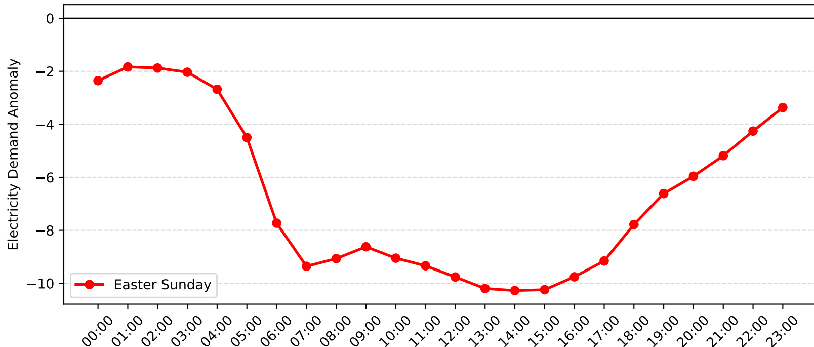
Sefton Demand Anomaly: Easter Sunday (2013-2014)
