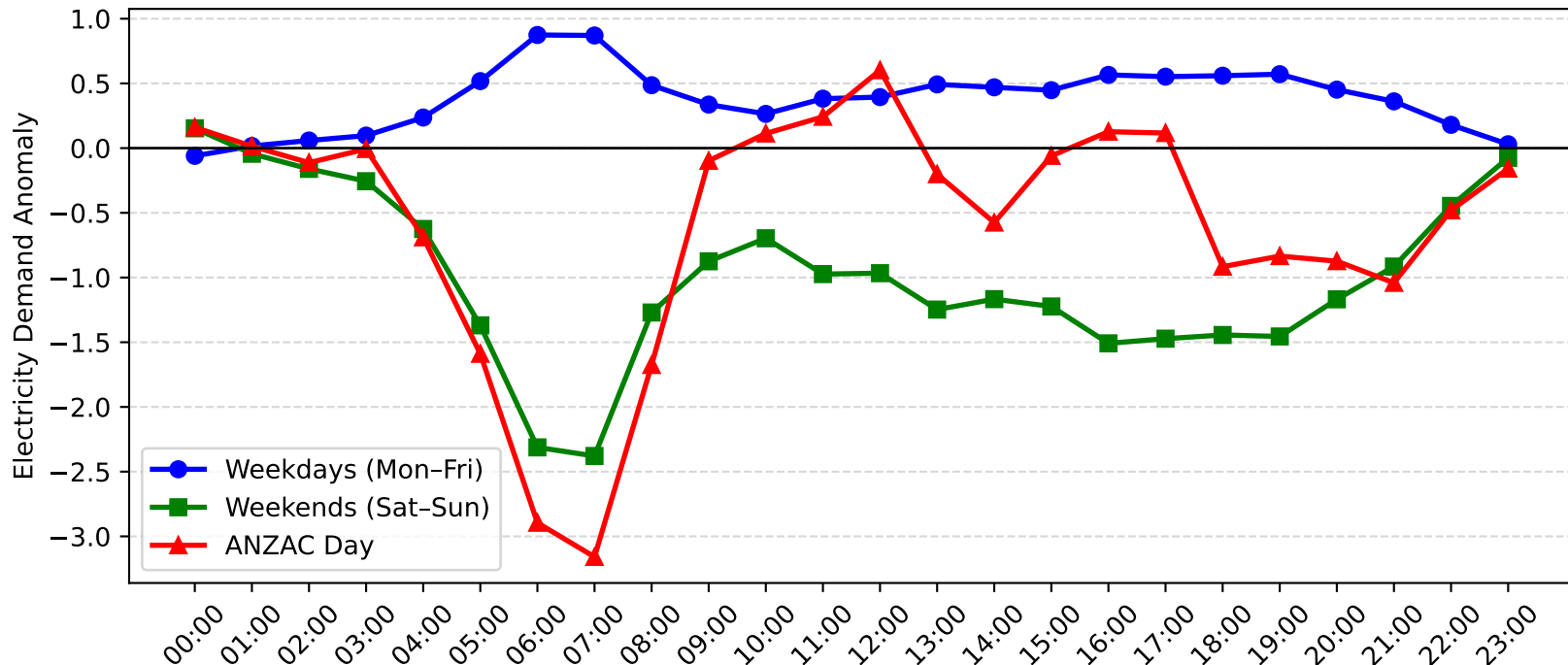
Charmhaven Demand Anomaly: ANZAC Day vs Weekday/Weekend (2007-2008)
