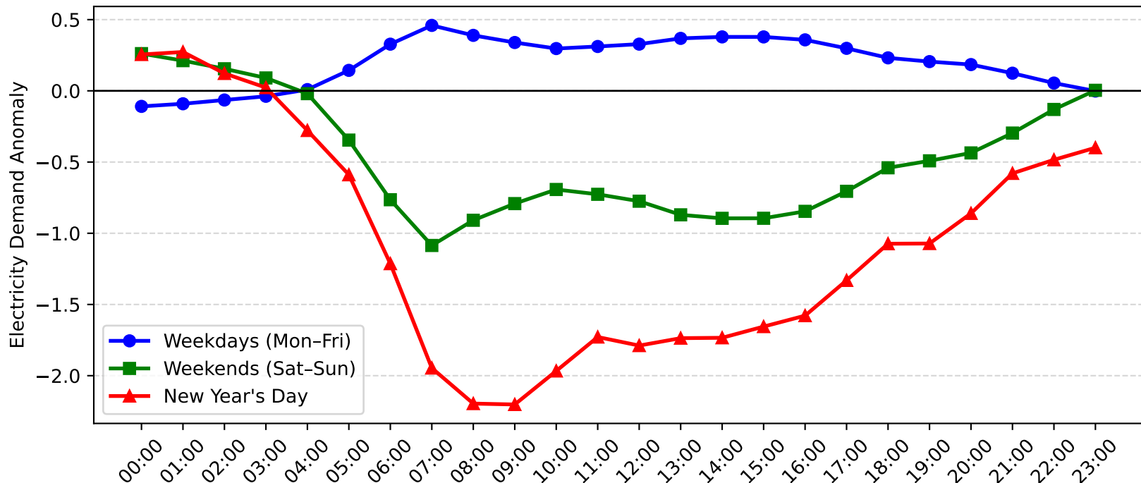
Rockdale Demand Anomaly: New Year's Day vs Weekday/Weekend (2012-2013)
