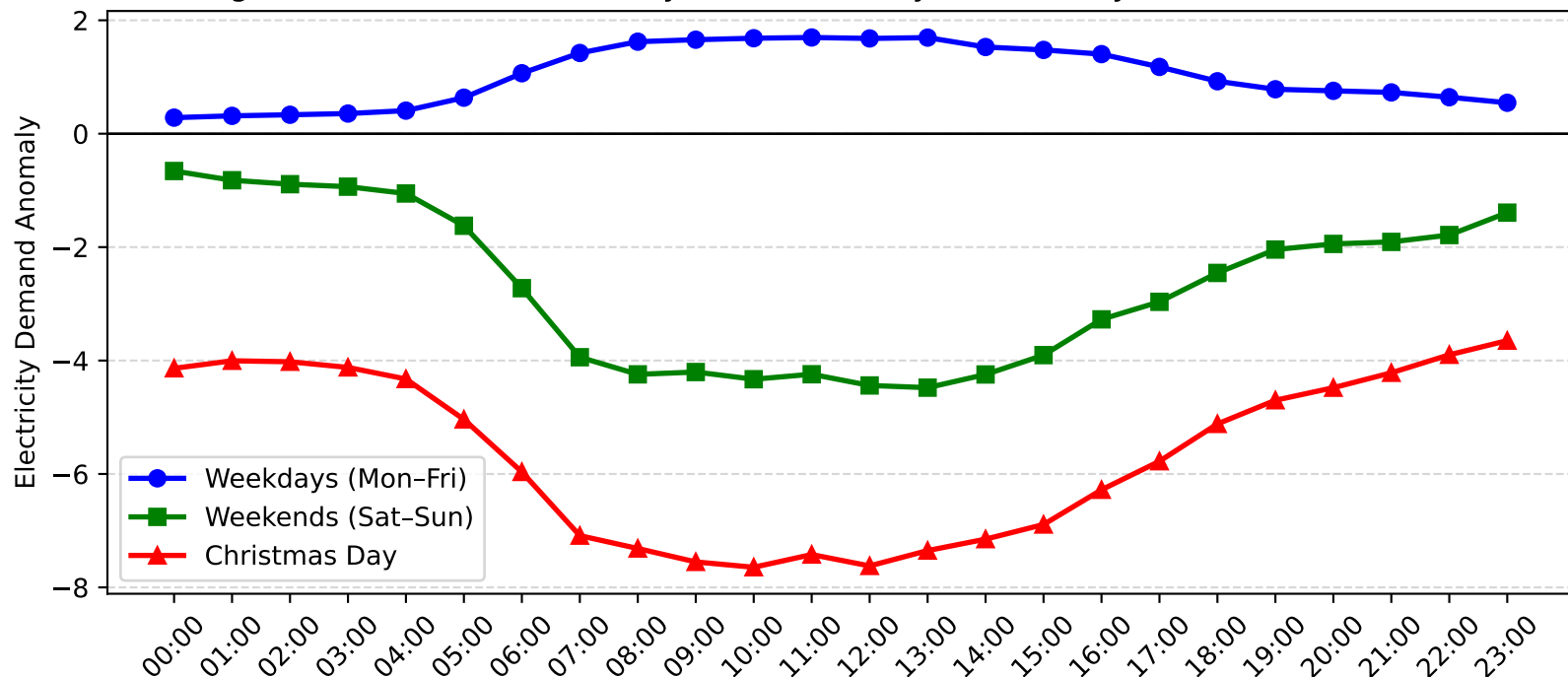
Leightonfield Demand Anomaly: Christmas Day vs Weekday/Weekend (2009-2010)
