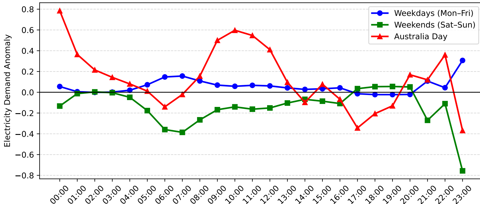
Telarah Demand Anomaly: Australia Day vs Weekday/Weekend (2012-2013)
