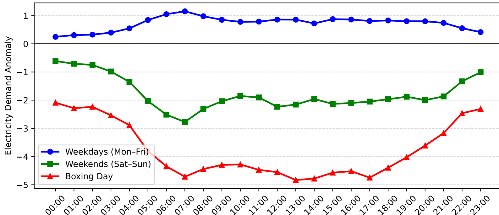
Lisarow Demand Anomaly: Boxing Day vs Weekday/Weekend (2005-2006)
