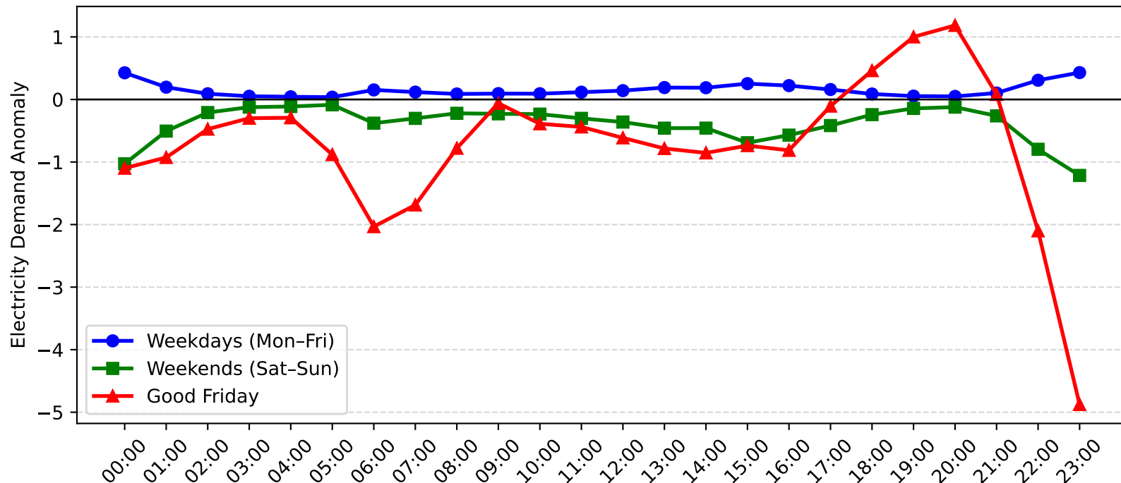
Muswellbrook Demand Anomaly: Good Friday vs Weekday/Weekend (2004-2005)
