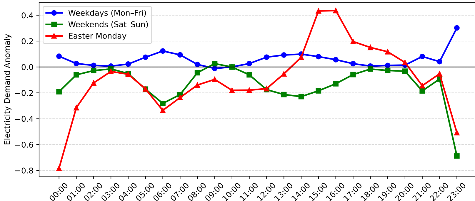
Telarah Demand Anomaly: Easter Monday vs Weekday/Weekend (2015-2016)
