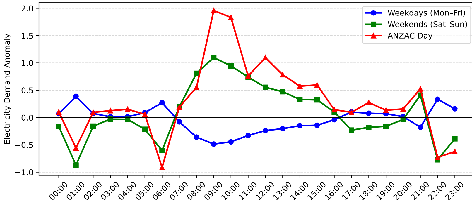
Swansea Demand Anomaly: ANZAC Day vs Weekday/Weekend (2005-2006)
