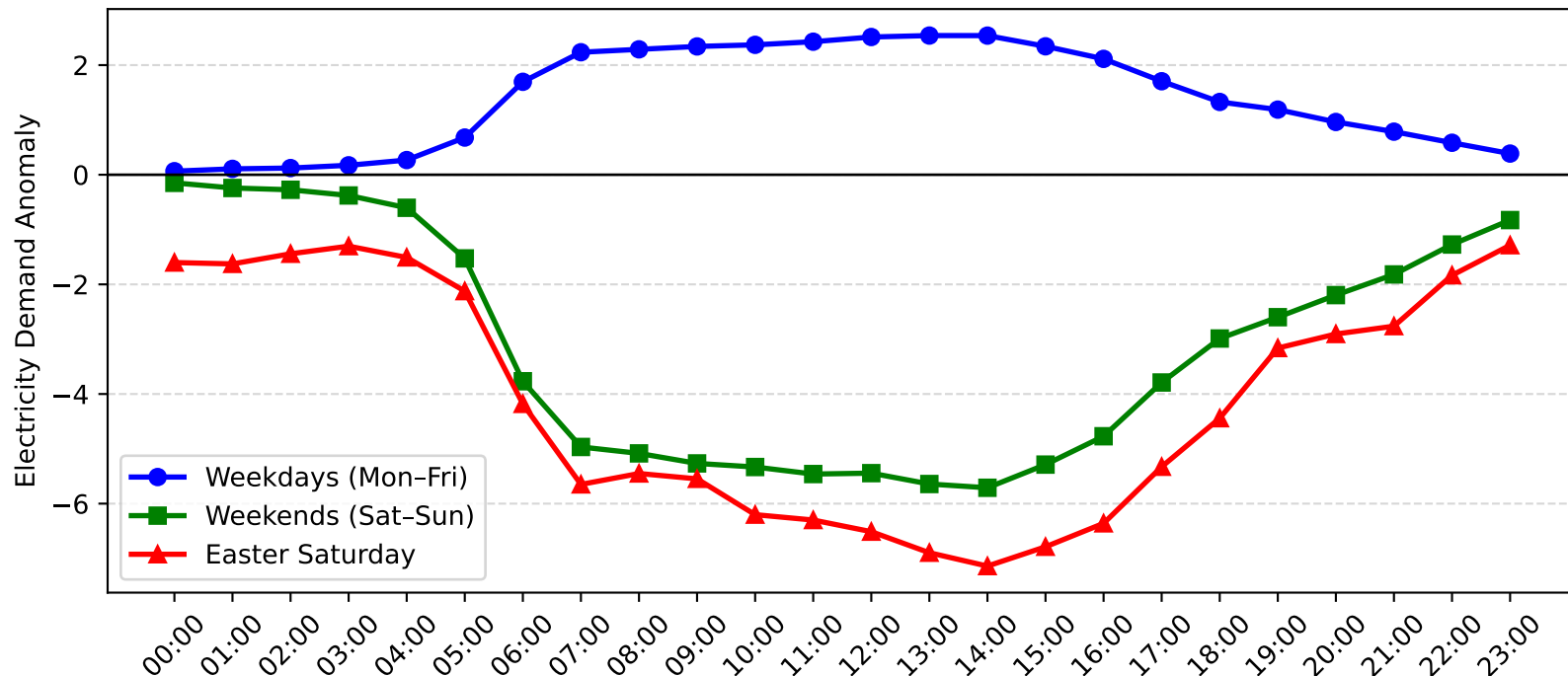
Concord Demand Anomaly: Easter Saturday vs Weekday/Weekend (2008-2009)
