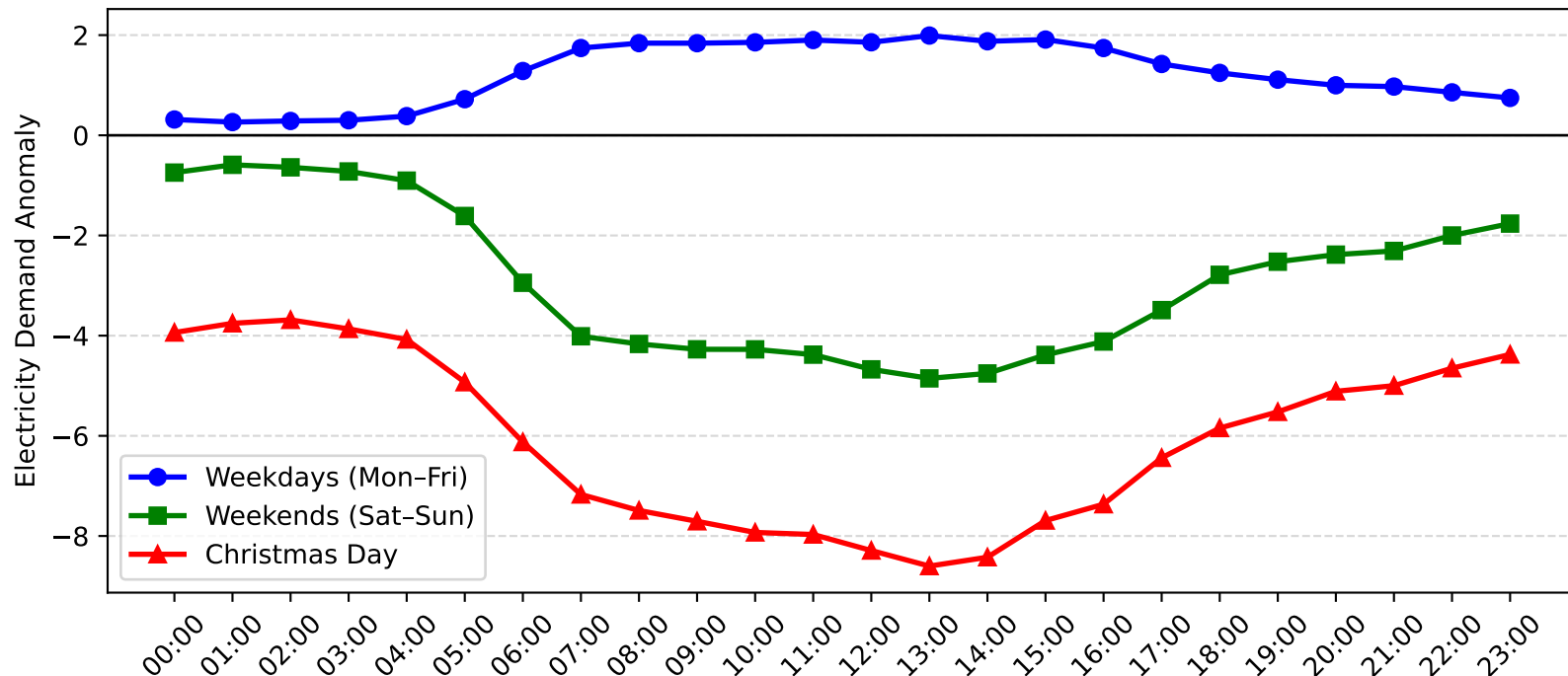
Leightonfield Demand Anomaly: Christmas Day vs Weekday/Weekend (2005-2006)
