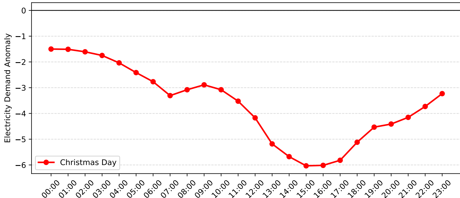
Bass Hill Demand Anomaly: Christmas Day (2012-2013)
