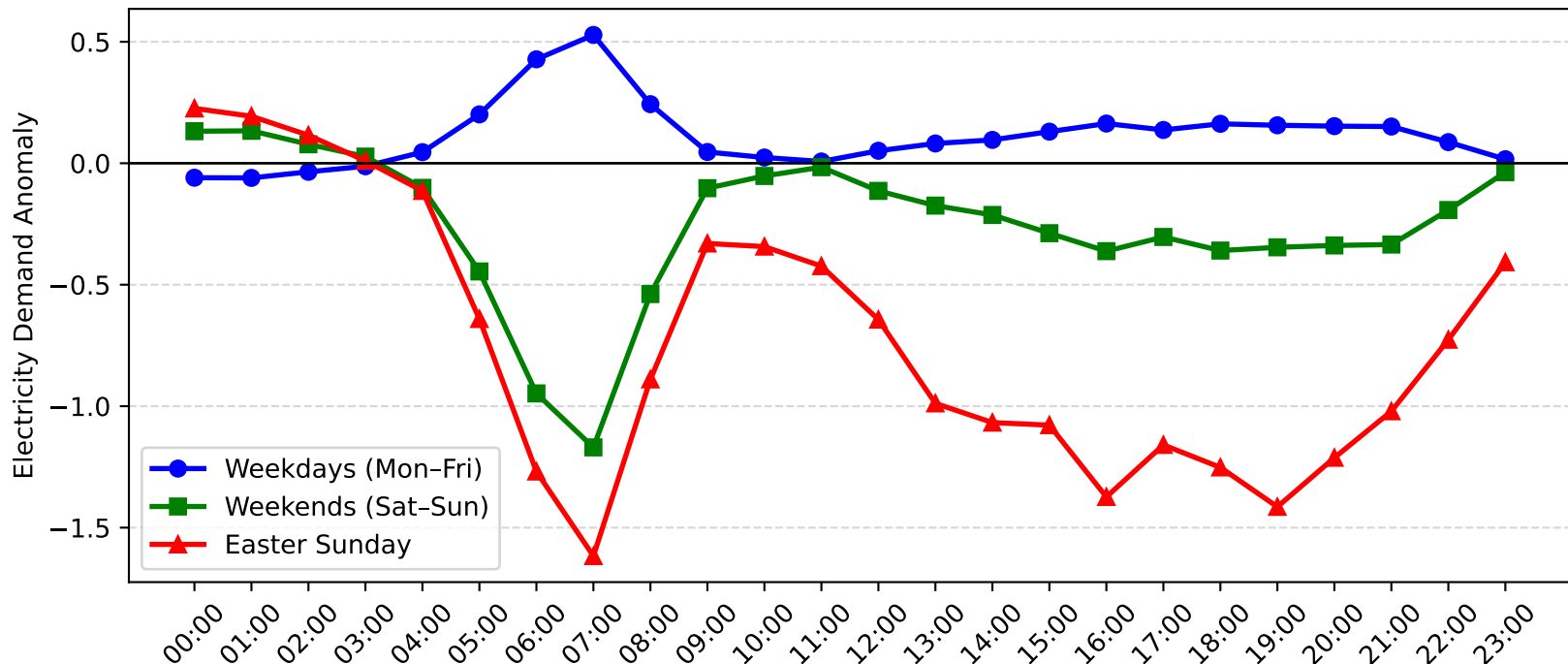
Blakehurst Demand Anomaly: Easter Sunday vs Weekday/Weekend (2017-2018)
