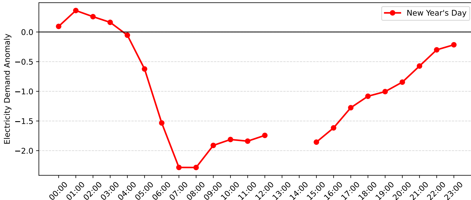
Arncliffe Demand Anomaly: New Year's Day (2014-2015)
