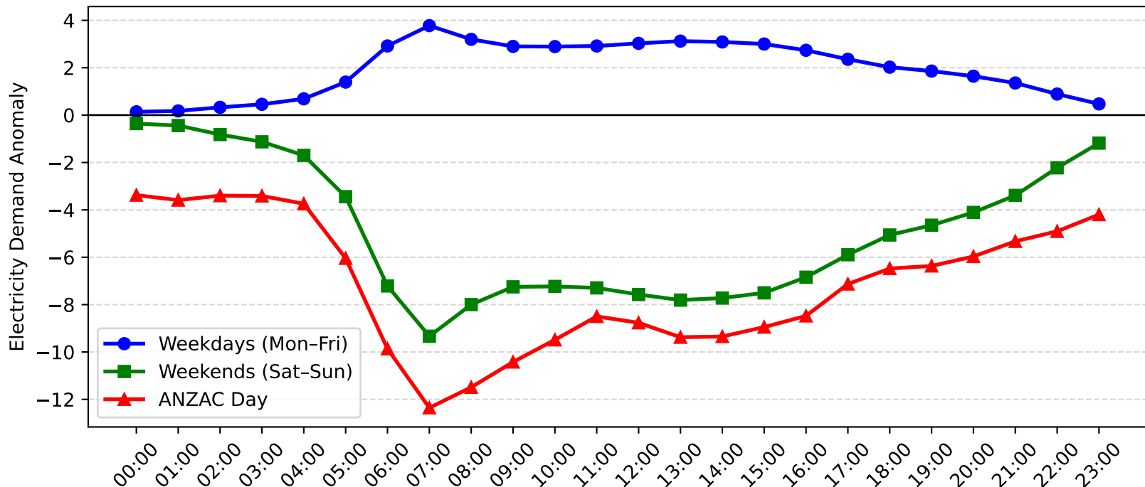
Sefton Demand Anomaly: ANZAC Day vs Weekday/Weekend (2011-2012)
