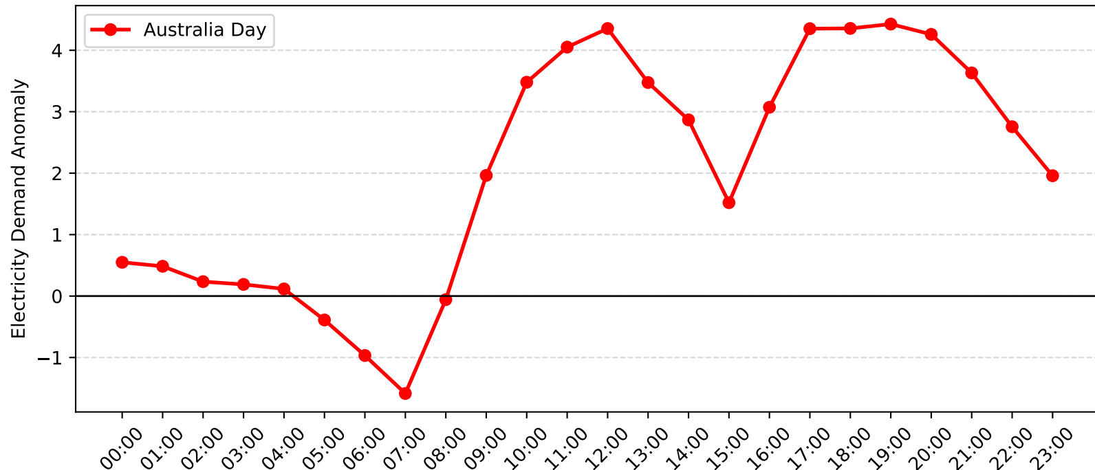
Charmhaven Demand Anomaly: Australia Day (2011-2012)
