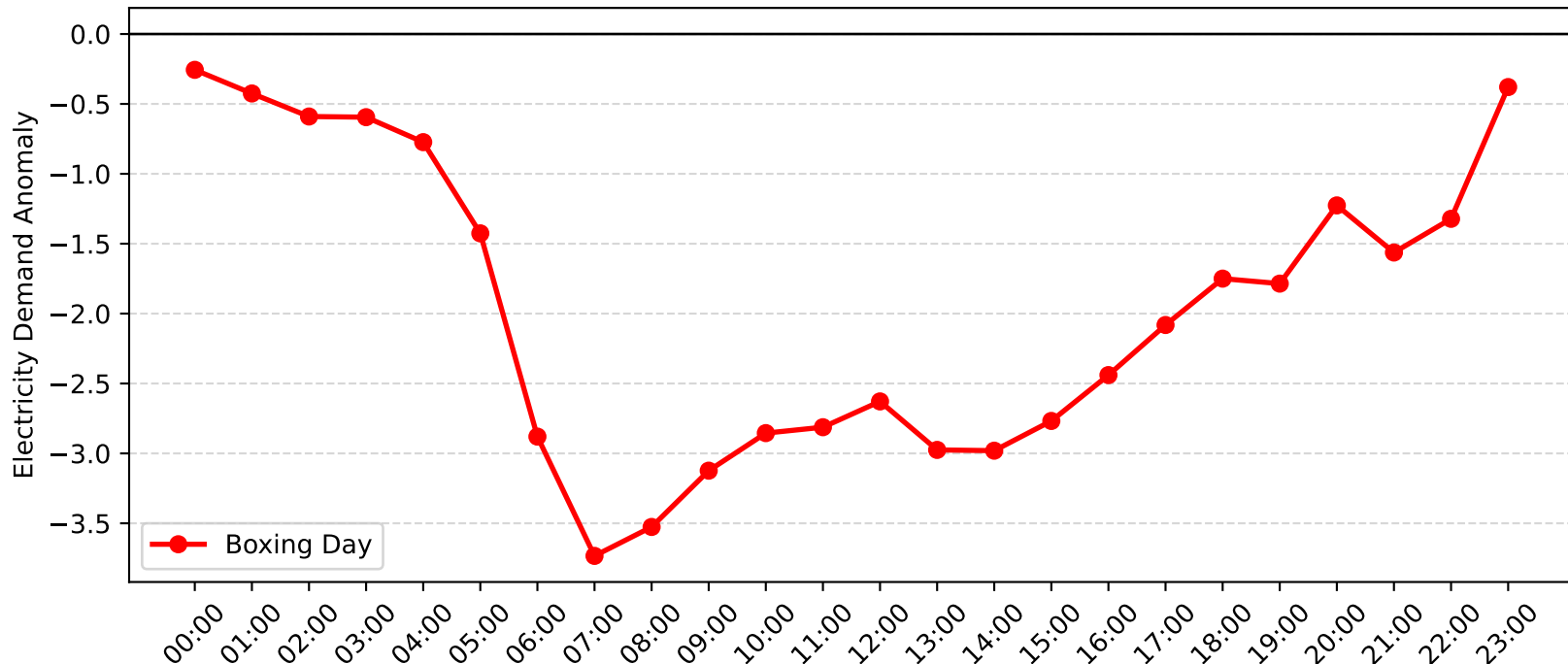
Arncliffe Demand Anomaly: Boxing Day (2007-2008)
