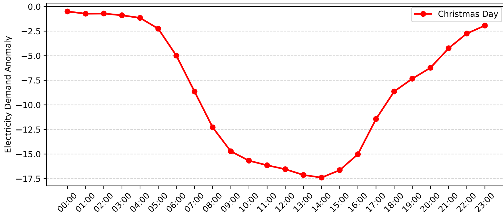
Brookvale Demand Anomaly: Christmas Day (2006-2007)
