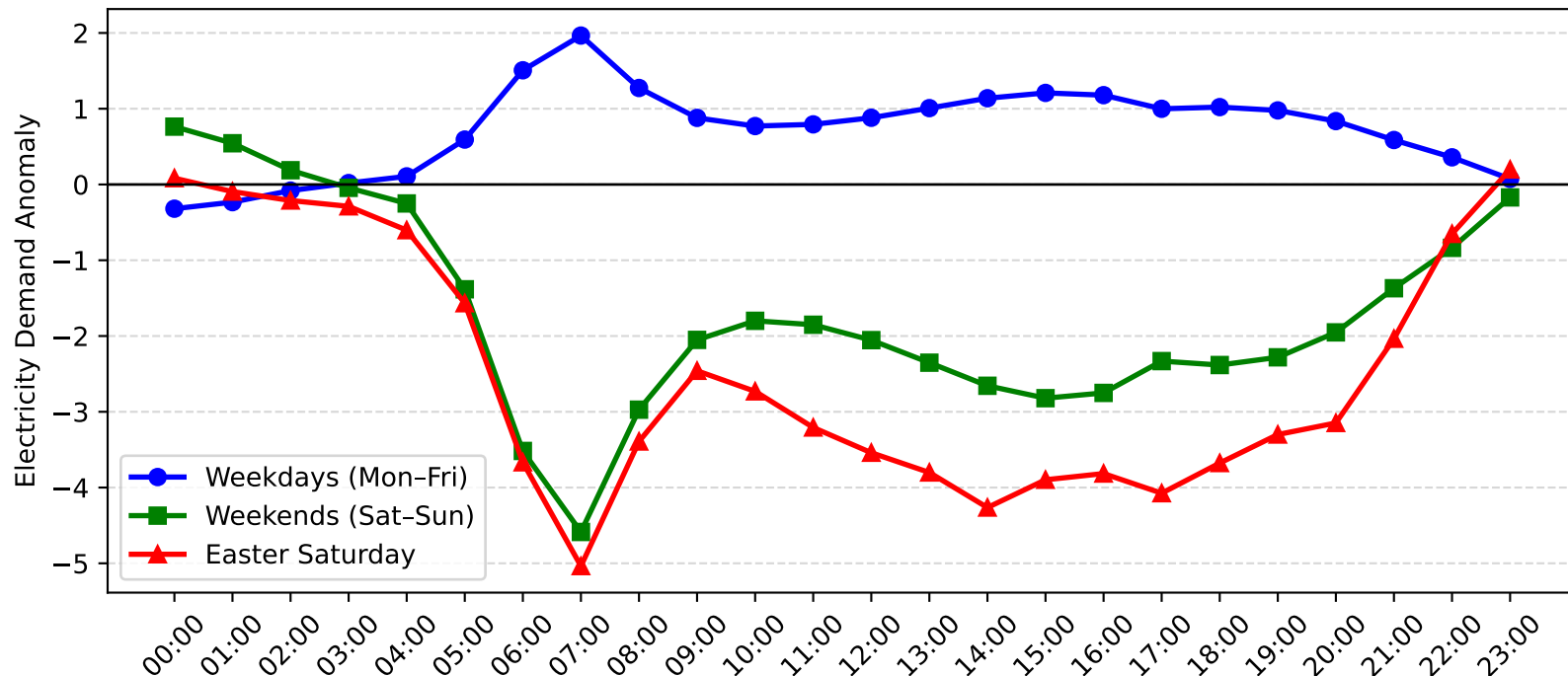
Kogarah Demand Anomaly: Easter Saturday vs Weekday/Weekend (2013-2014)
