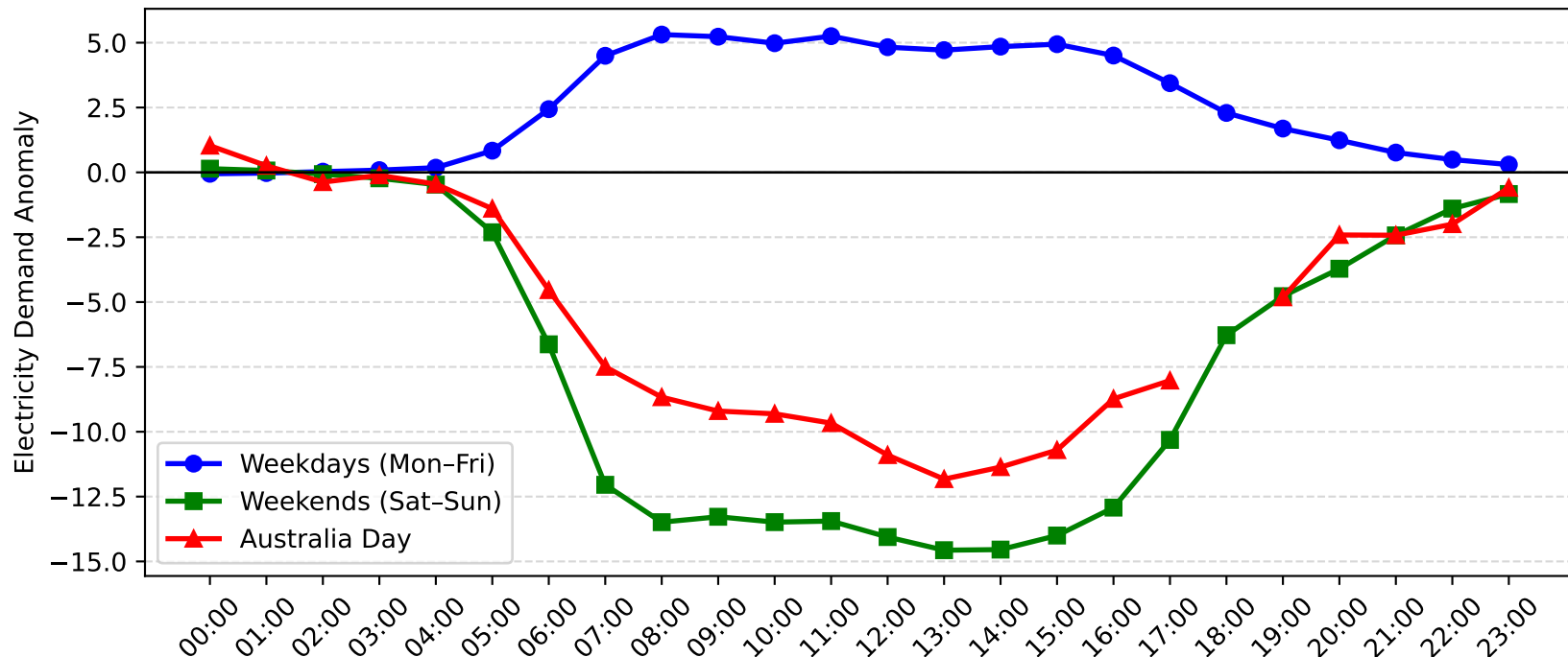
Zetland Demand Anomaly: Australia Day vs Weekday/Weekend (2005-2006)
