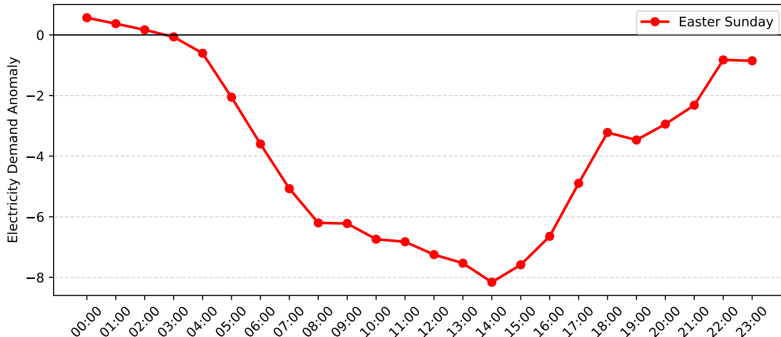
West Gosford Demand Anomaly: Easter Sunday (2009-2010)
