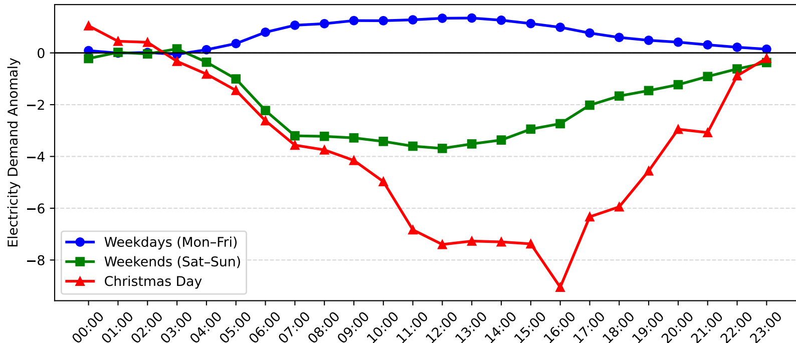
Wyong Demand Anomaly: Christmas Day vs Weekday/Weekend (2007-2008)
