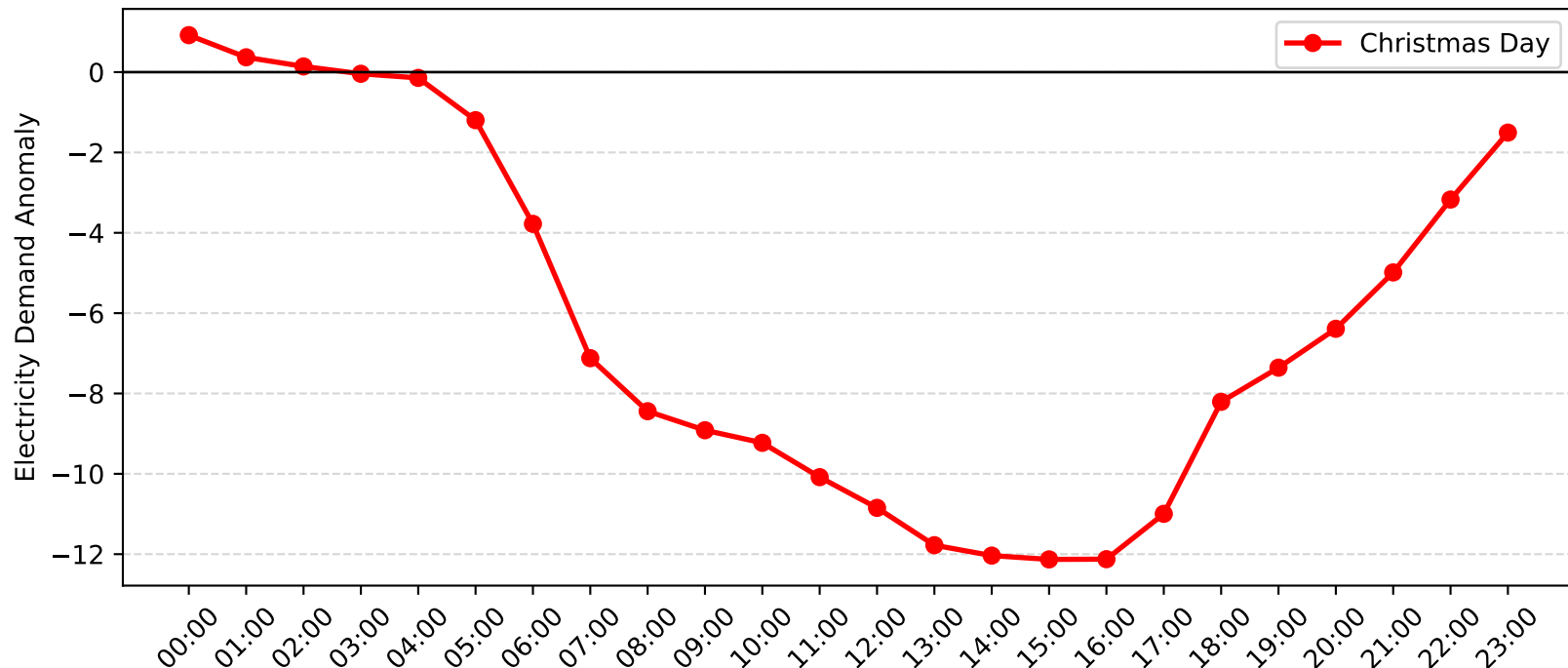
Epping Demand Anomaly: Christmas Day (2011-2012)
