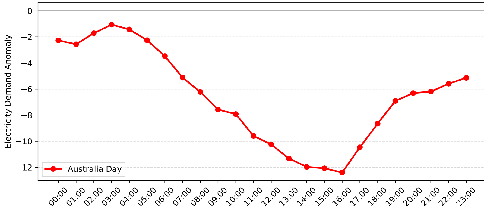
Greenacre Park Demand Anomaly: Australia Day (2017-2018)
