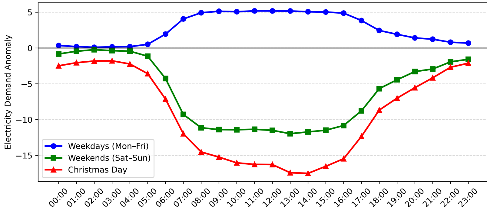
Gore Hill Demand Anomaly: Christmas Day vs Weekday/Weekend (2010-2011)
