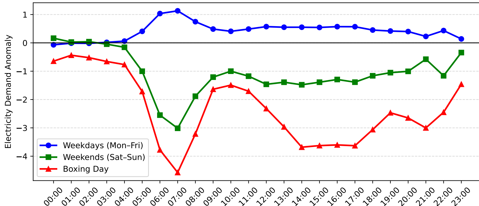
Dee Why West Demand Anomaly: Boxing Day vs Weekday/Weekend (2009-2010)
