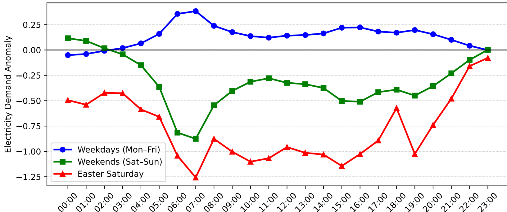
Rockdale Demand Anomaly: Easter Saturday vs Weekday/Weekend (2017-2018)
