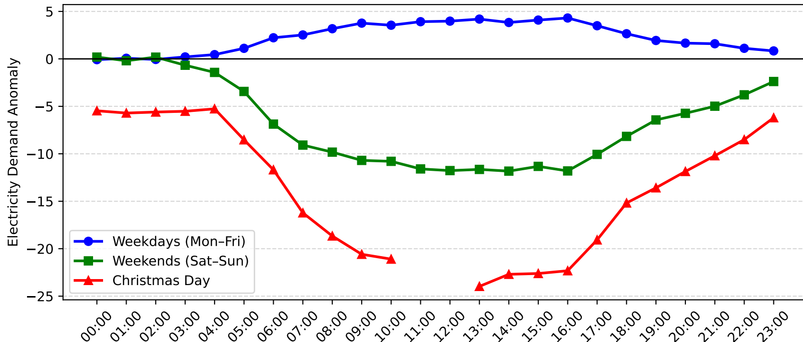
Greenacre Park Demand Anomaly: Christmas Day vs Weekday/Weekend (2008-2009)
