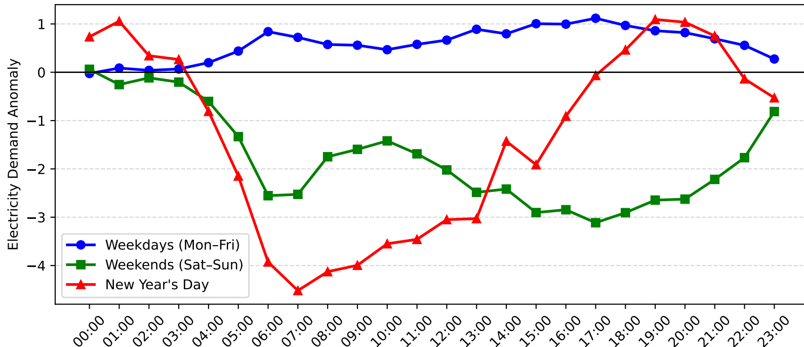
Revesby Demand Anomaly: New Year's Day vs Weekday/Weekend (2009-2010)
