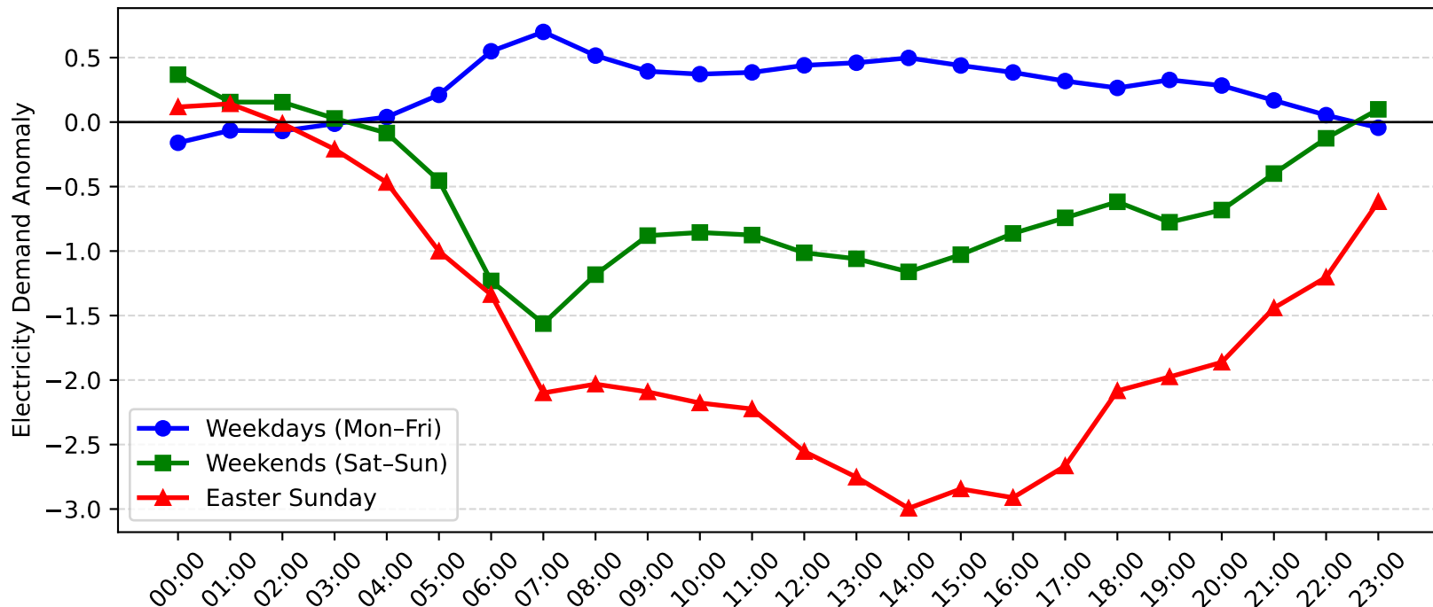
Rockdale Demand Anomaly: Easter Sunday vs Weekday/Weekend (2010-2011)
