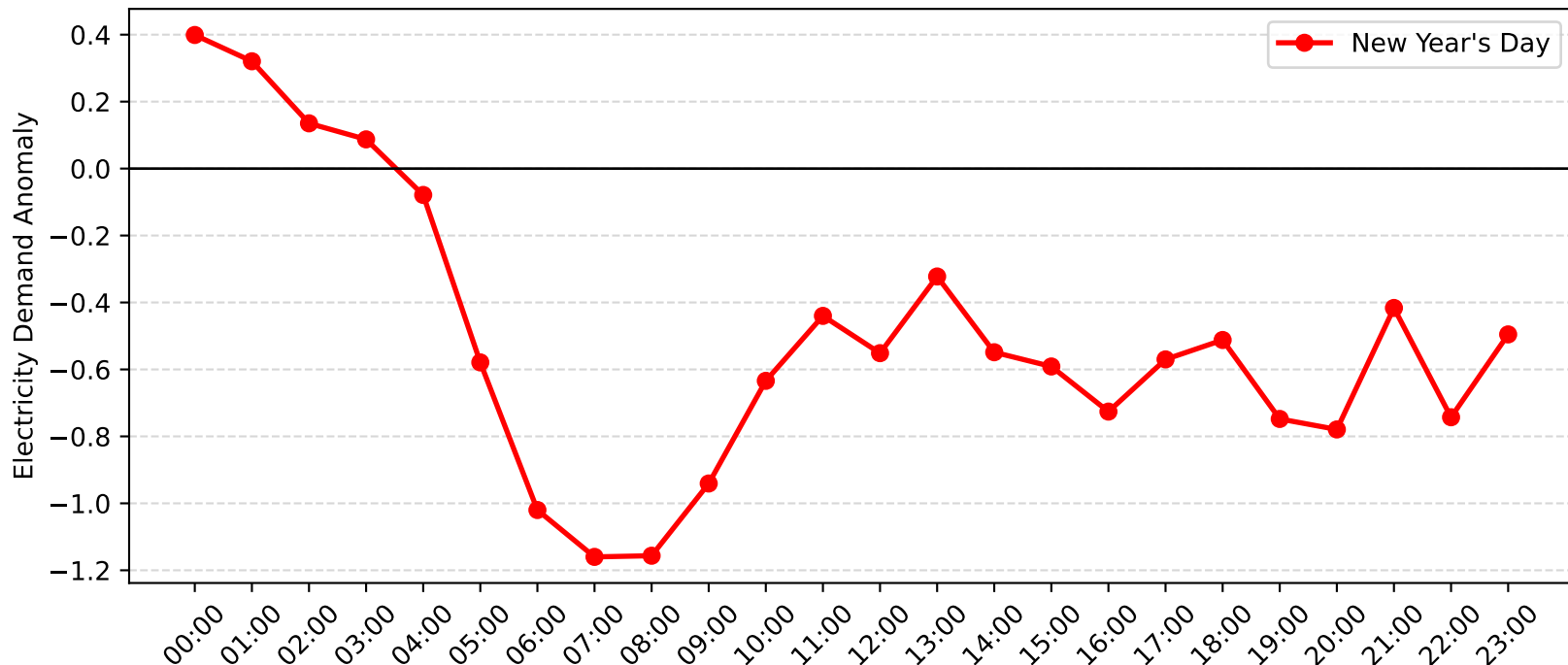
Narrabeen Demand Anomaly: New Year's Day (2011-2012)
