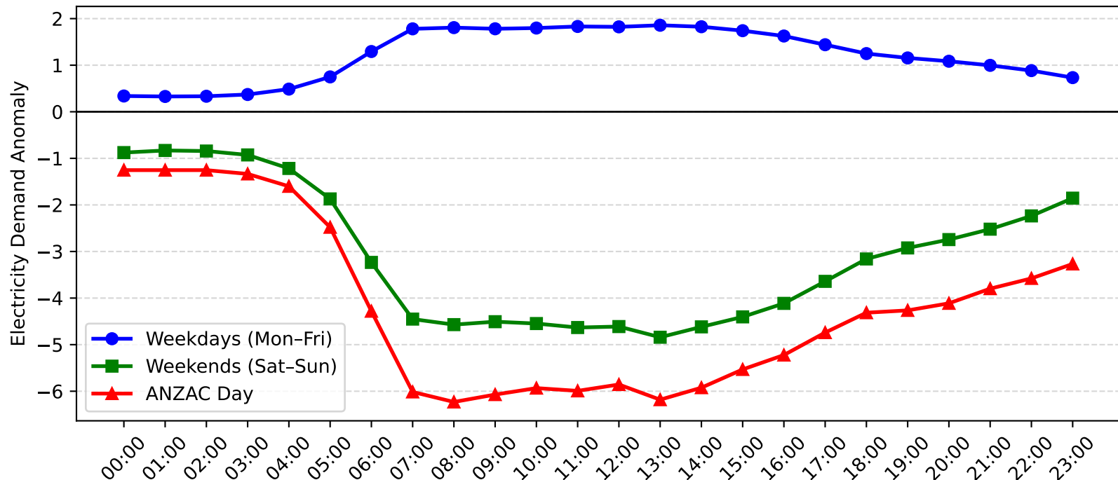
Leightonfield Demand Anomaly: ANZAC Day vs Weekday/Weekend (2011-2012)
