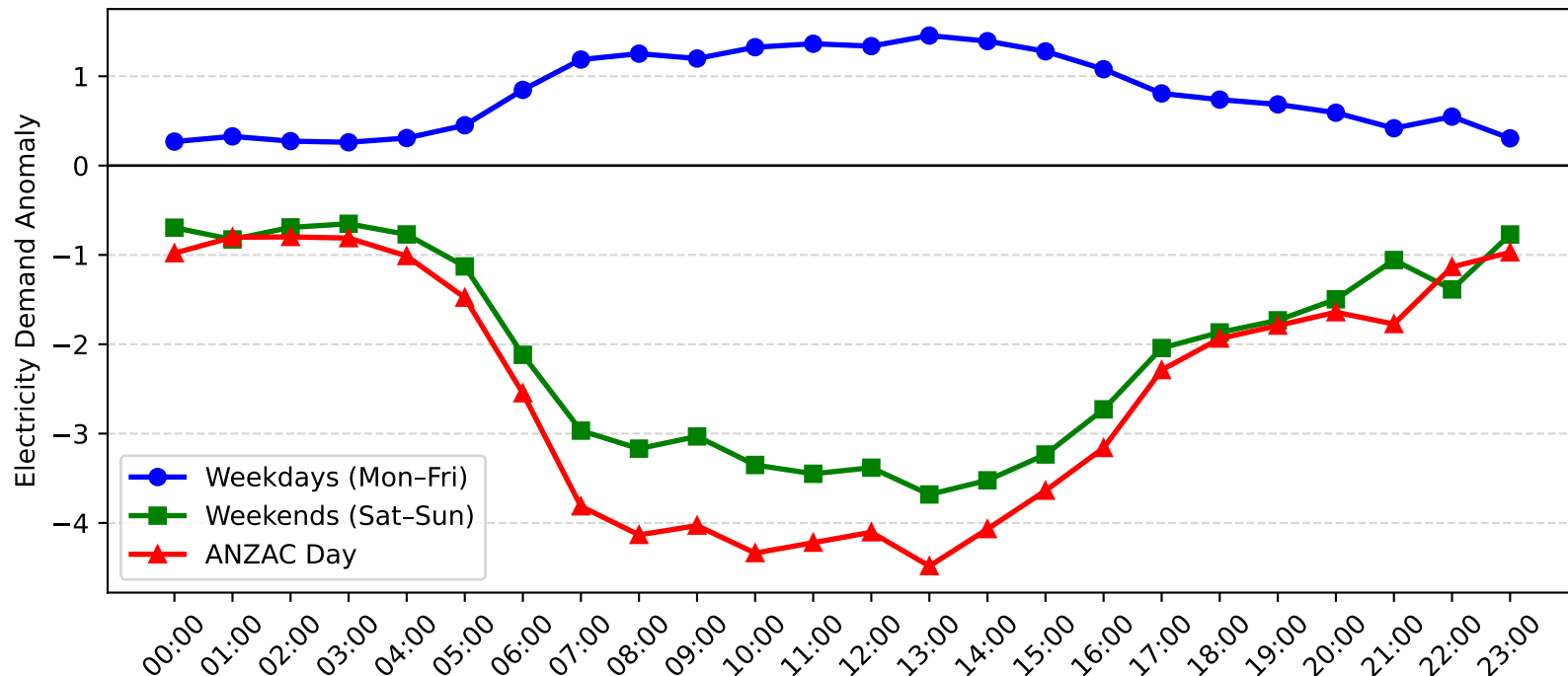
Mayfield West Demand Anomaly: ANZAC Day vs Weekday/Weekend (2011-2012)
