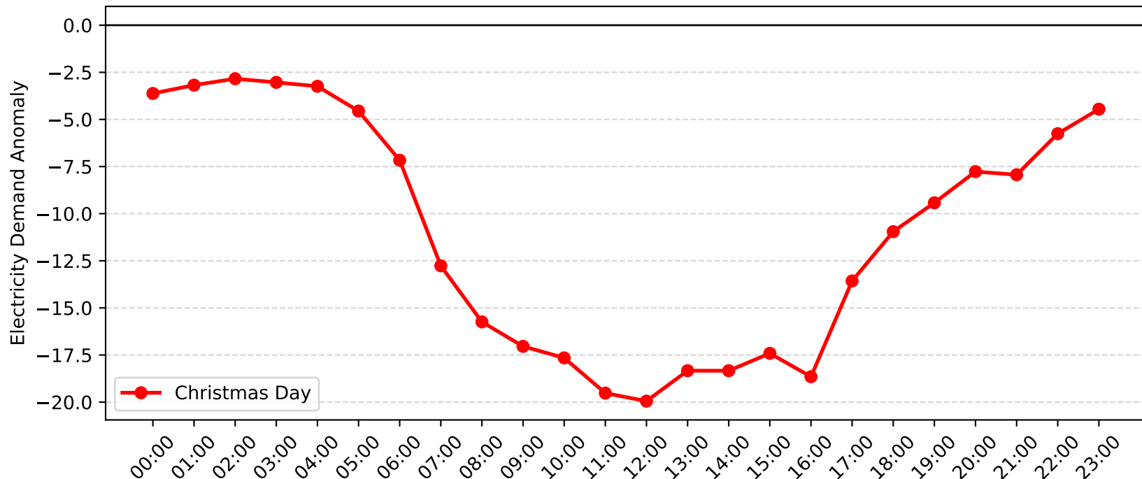
Gore Hill Demand Anomaly: Christmas Day (2007-2008)
