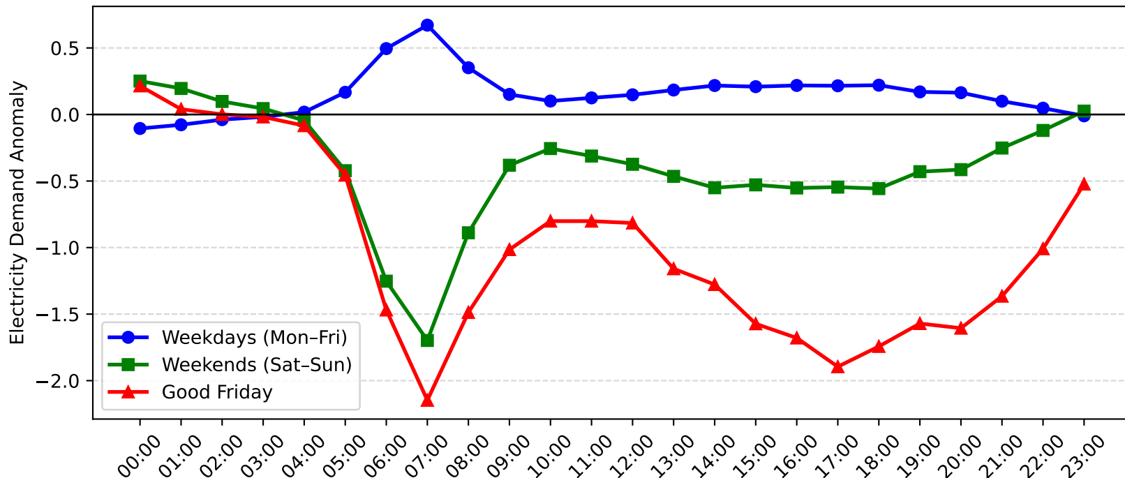
Blakehurst Demand Anomaly: Good Friday vs Weekday/Weekend (2013-2014)
