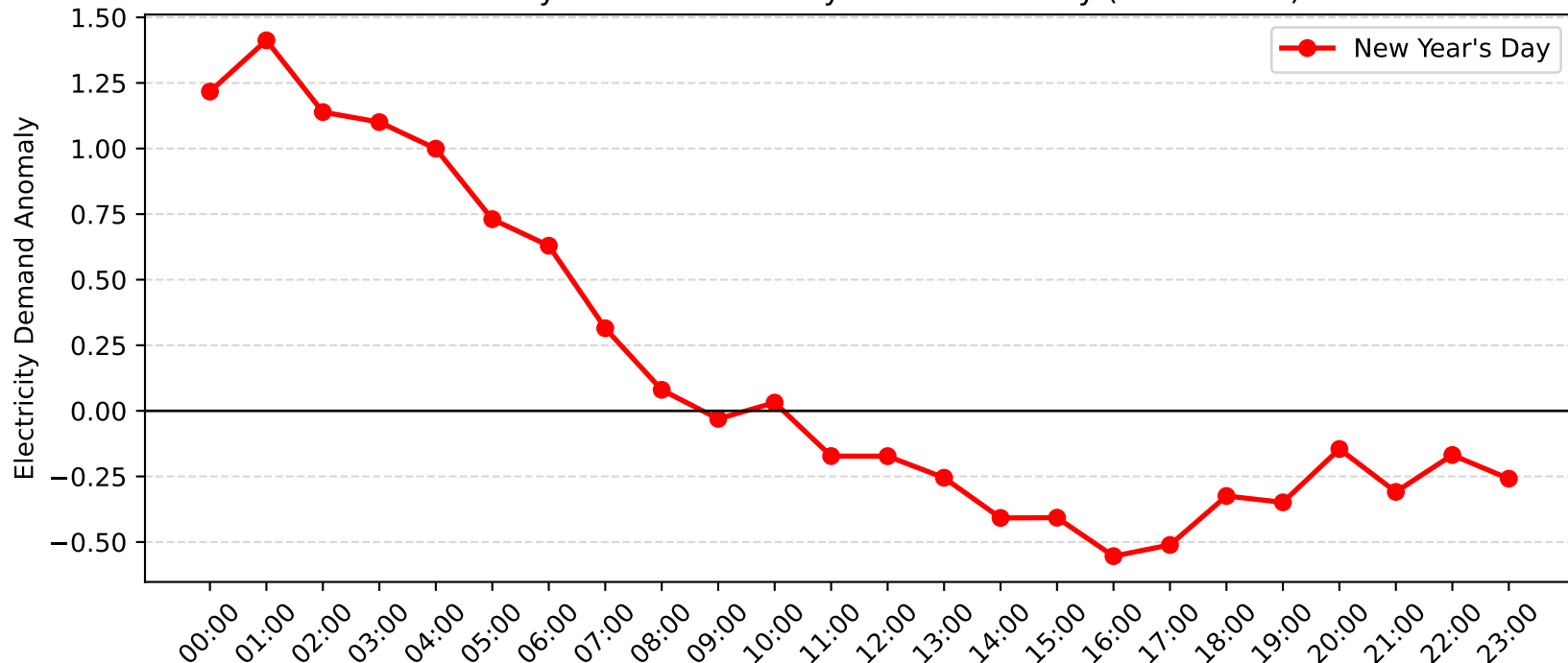
Rothbury Demand Anomaly: New Year's Day (2017-2018)
