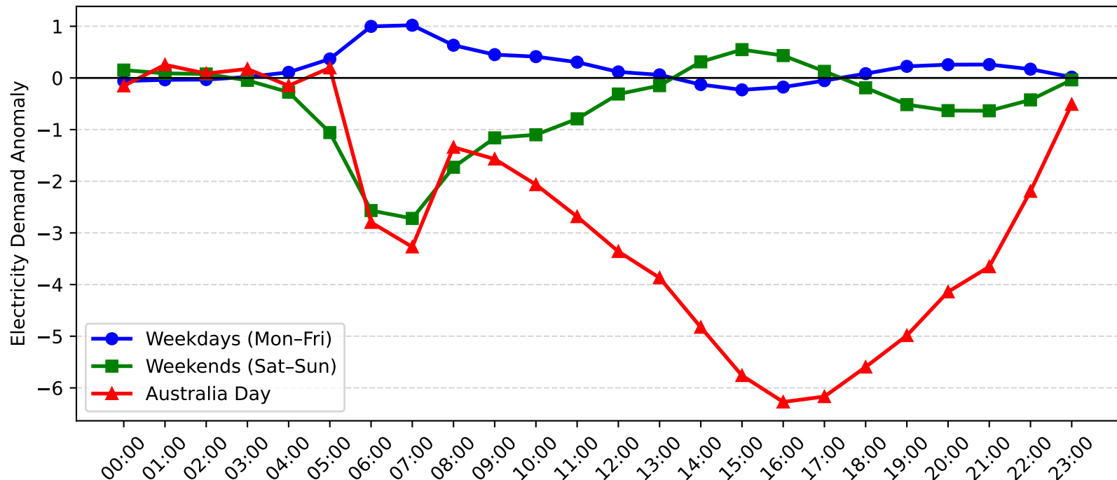
Revesby Demand Anomaly: Australia Day vs Weekday/Weekend (2014-2015)
