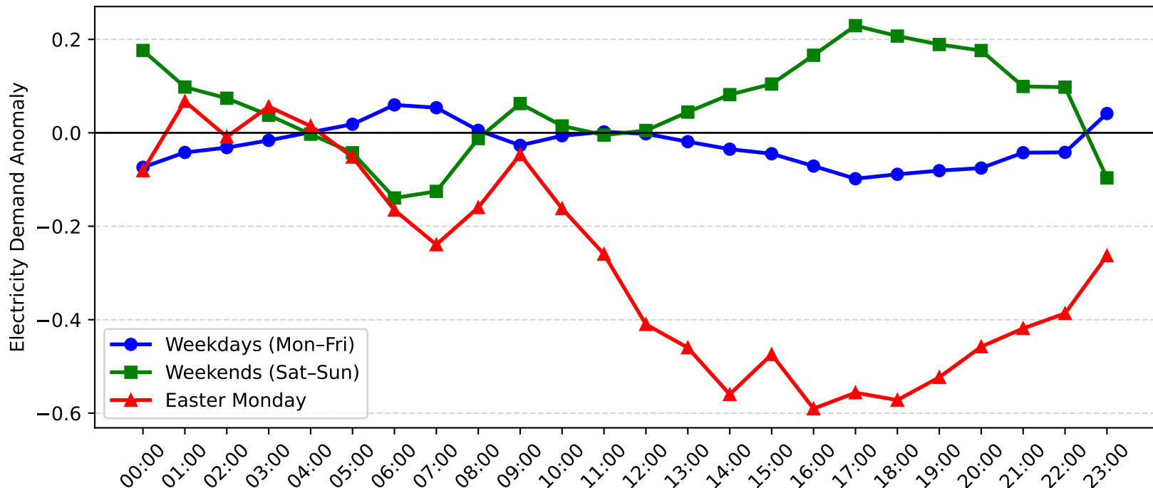
Rothbury Demand Anomaly: Easter Monday vs Weekday/Weekend (2012-2013)
