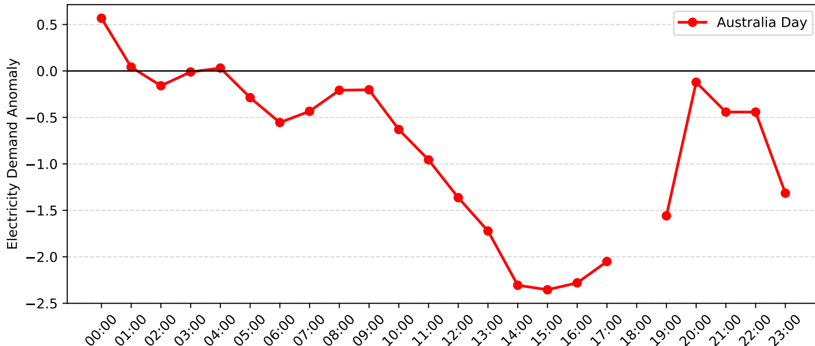
Telarah Demand Anomaly: Australia Day (2005-2006)
