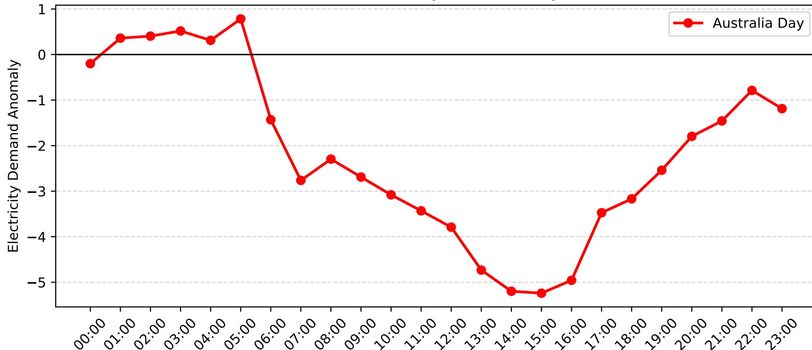
Rutherford Demand Anomaly: Australia Day (2014-2015)
