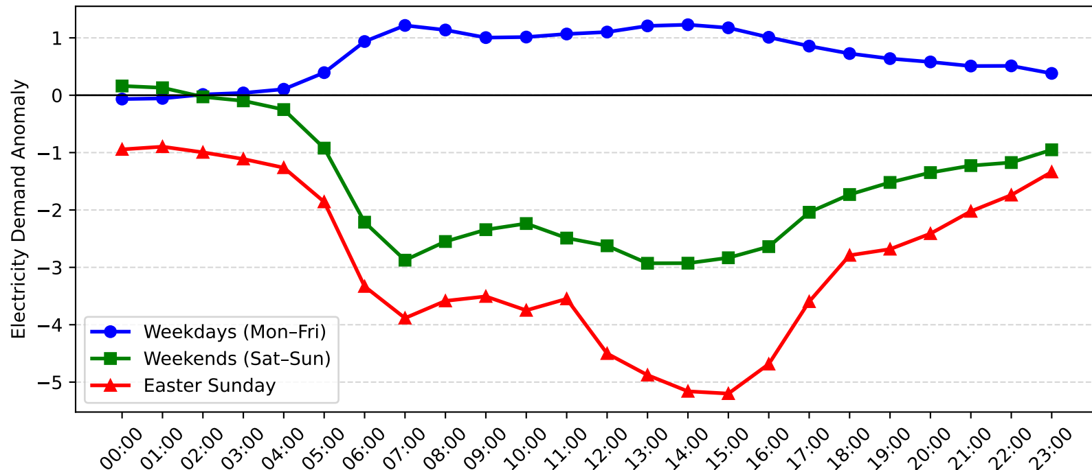
Bass Hill Demand Anomaly: Easter Sunday vs Weekday/Weekend (2005-2006)
