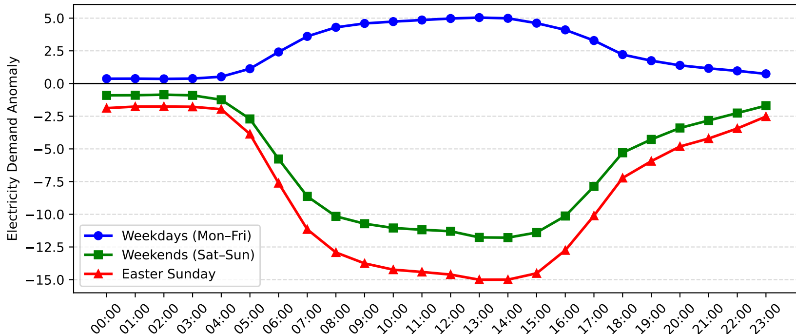
Mascot Demand Anomaly: Easter Sunday vs Weekday/Weekend (2007-2008)
