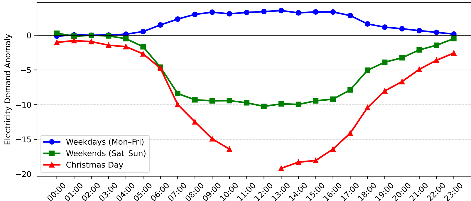
Castle Cove Demand Anomaly: Christmas Day vs Weekday/Weekend (2008-2009)
