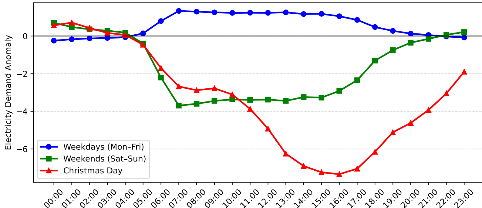
Hunters Hill Demand Anomaly: Christmas Day vs Weekday/Weekend (2012-2013)
