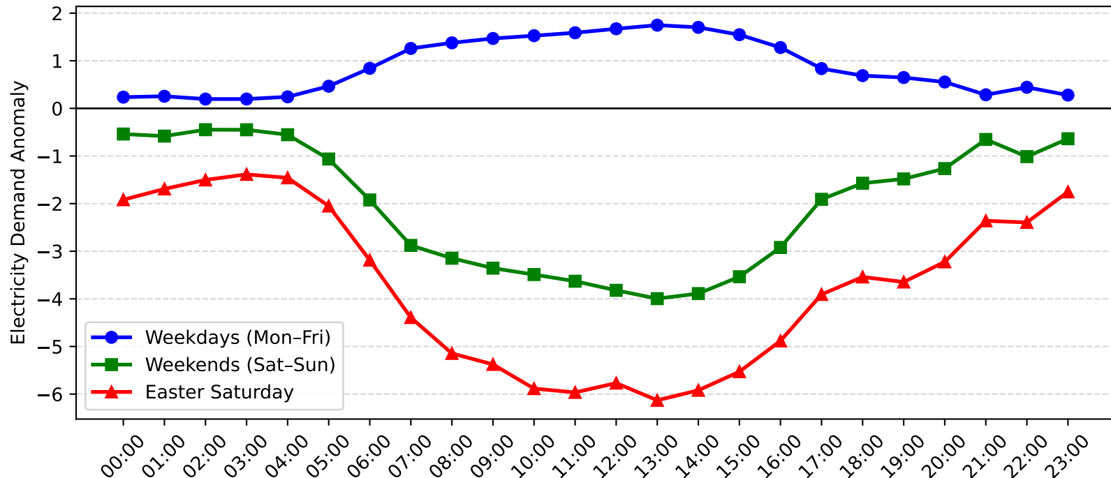
Broadmeadow Demand Anomaly: Easter Saturday vs Weekday/Weekend (2017-2018)
