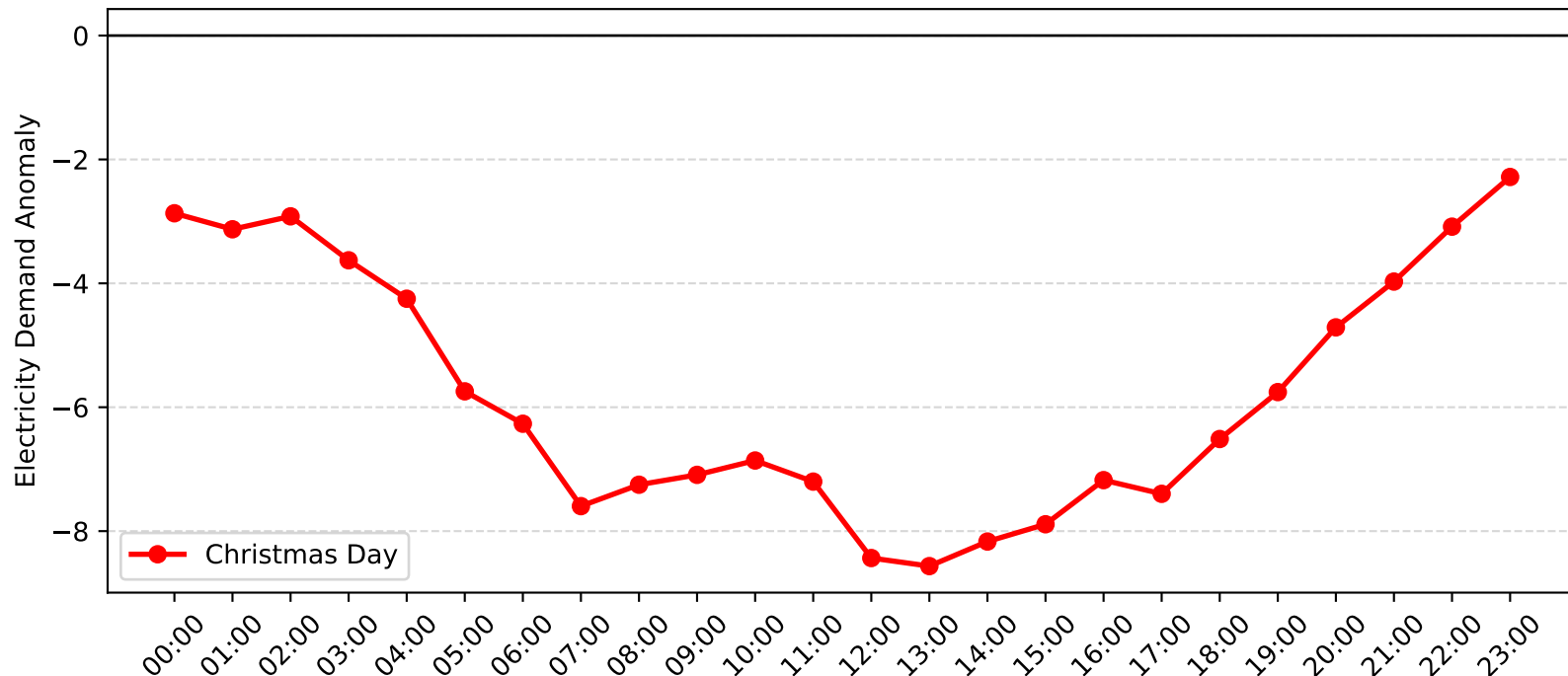
Matraverse Demand Anomaly: Christmas Day (2009-2010)
