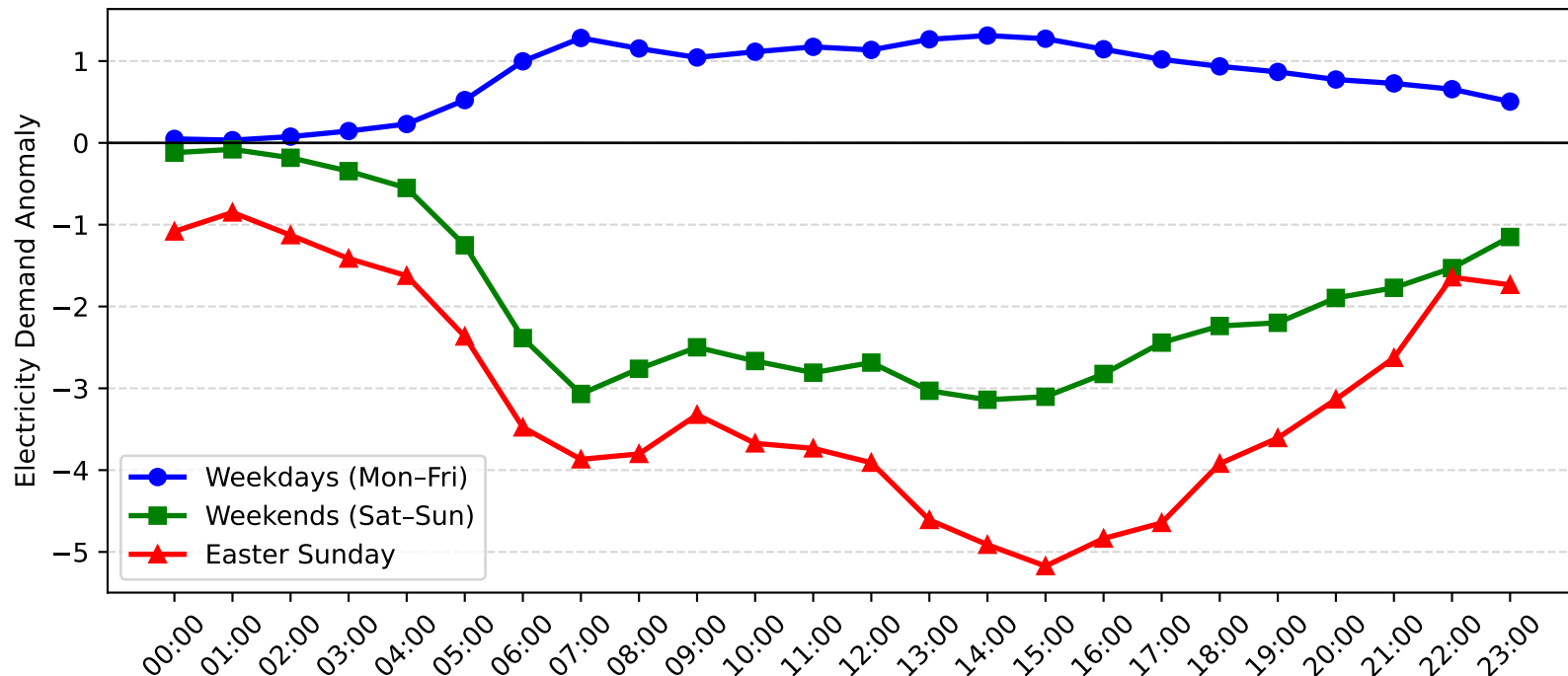
Bass Hill Demand Anomaly: Easter Sunday vs Weekday/Weekend (2007-2008)
