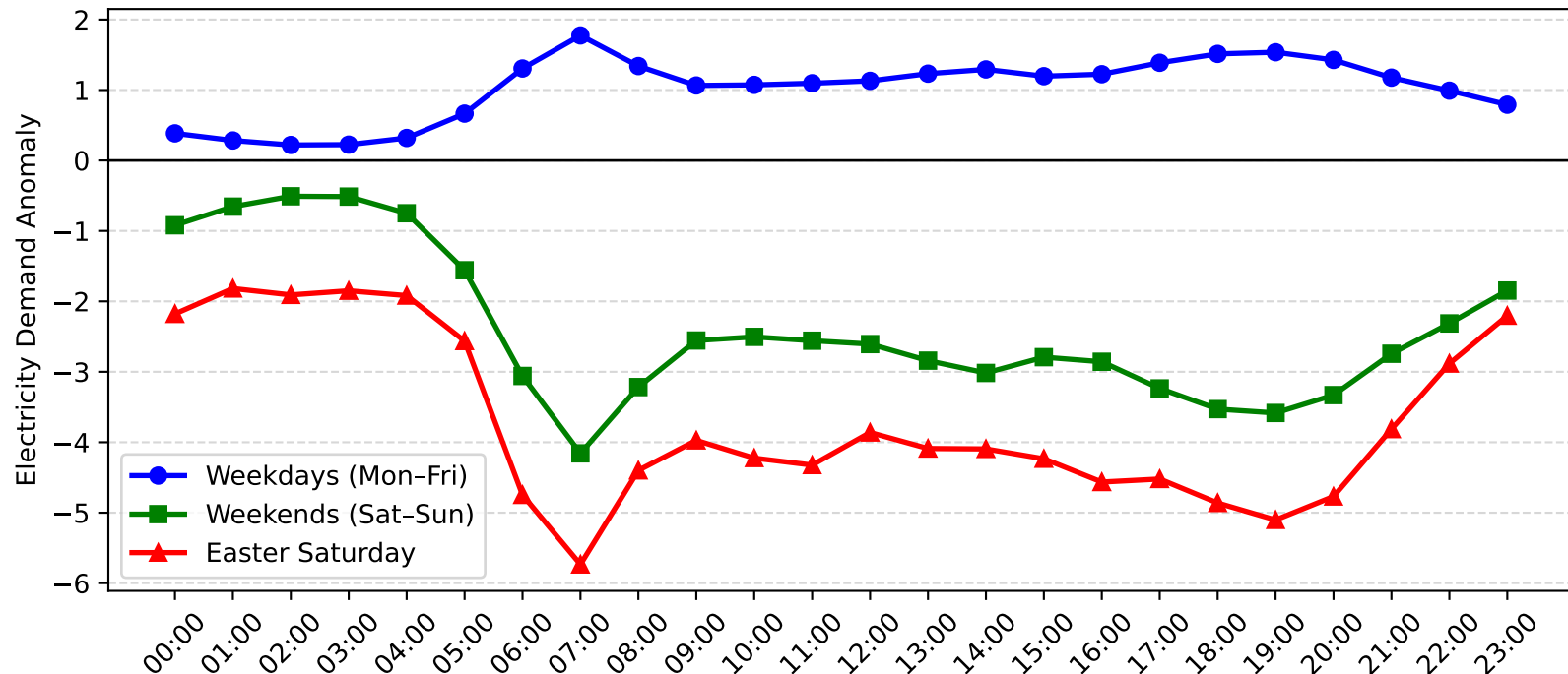
Maroubra Demand Anomaly: Easter Saturday vs Weekday/Weekend (2011-2012)
