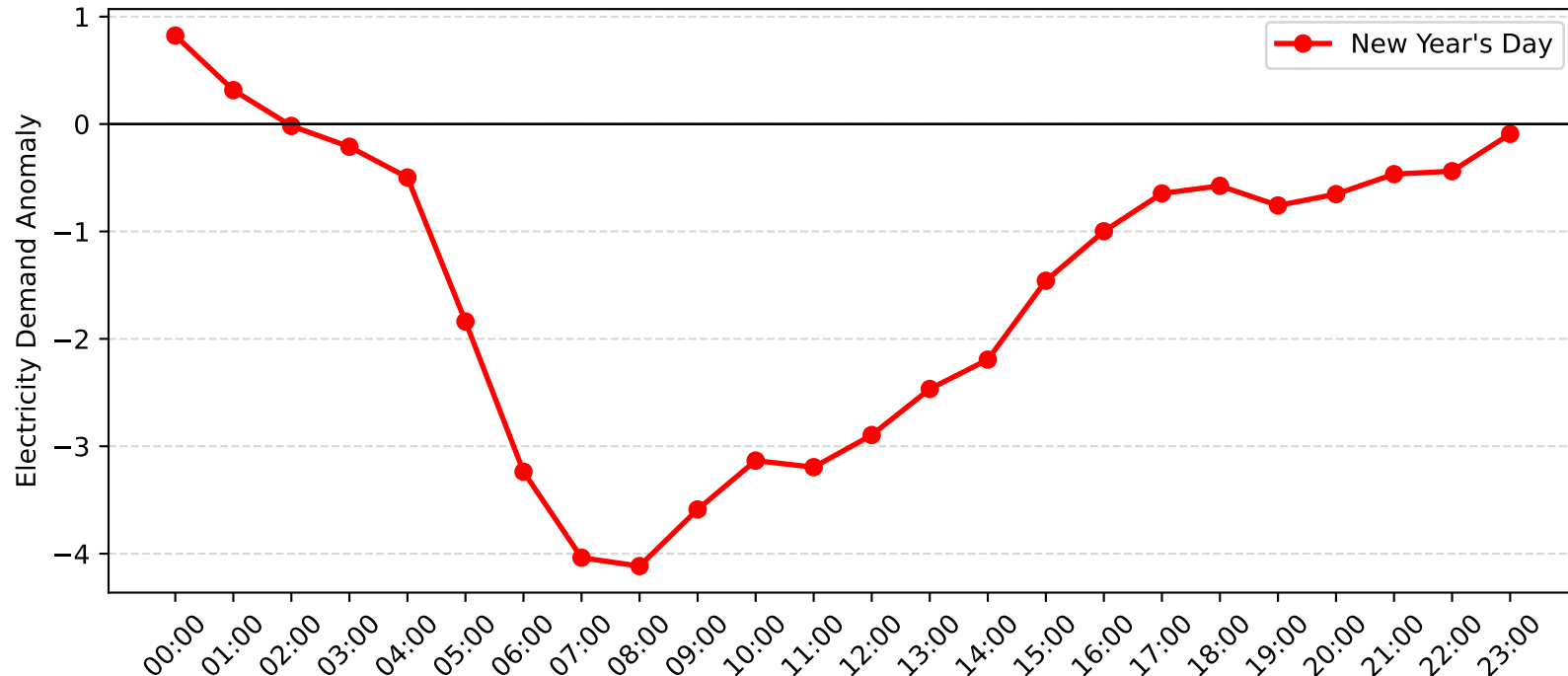
Wyong Demand Anomaly: New Year's Day (2013-2014)
