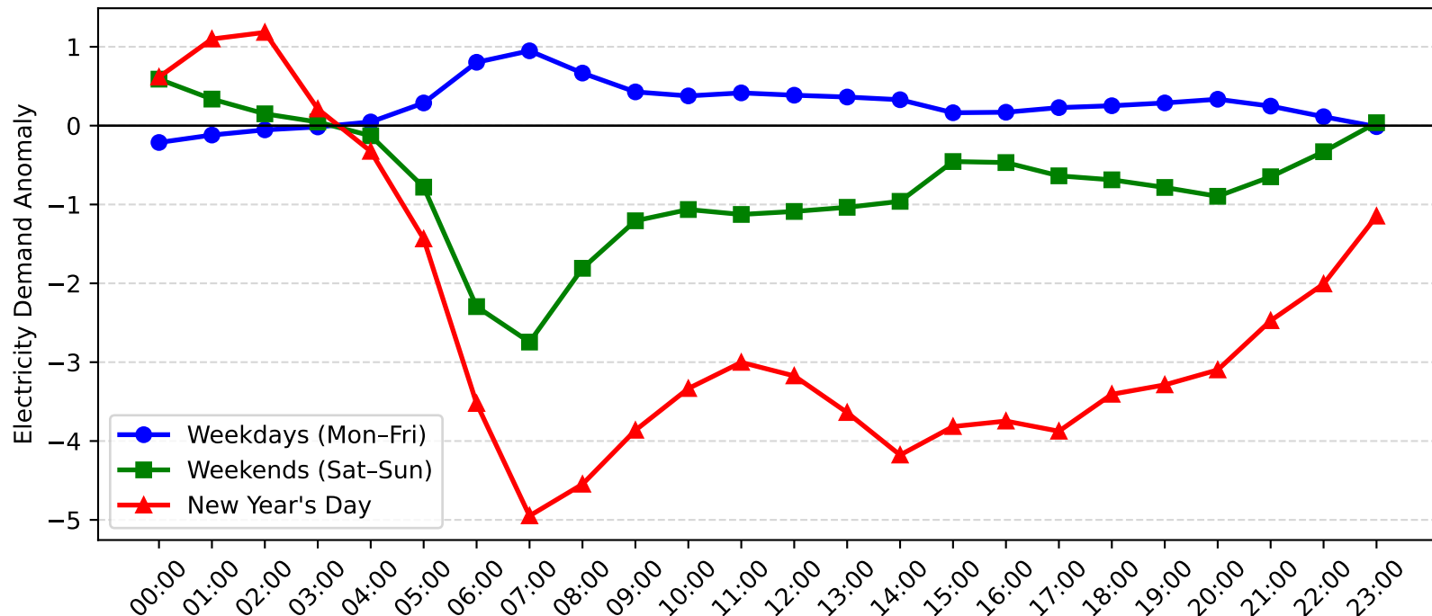
Mortdale Demand Anomaly: New Year's Day vs Weekday/Weekend (2015-2016)
