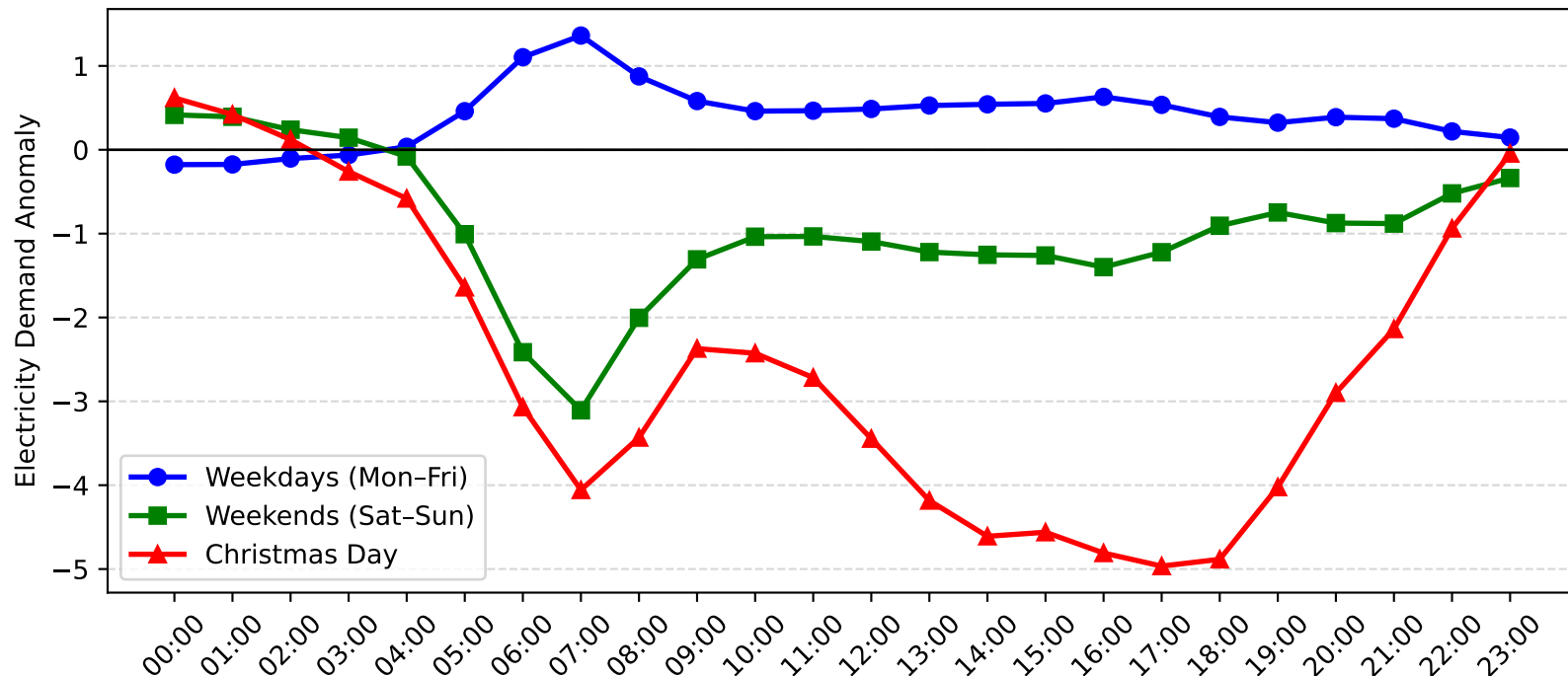
Dulwich Hill Demand Anomaly: Christmas Day vs Weekday/Weekend (2010-2011)
