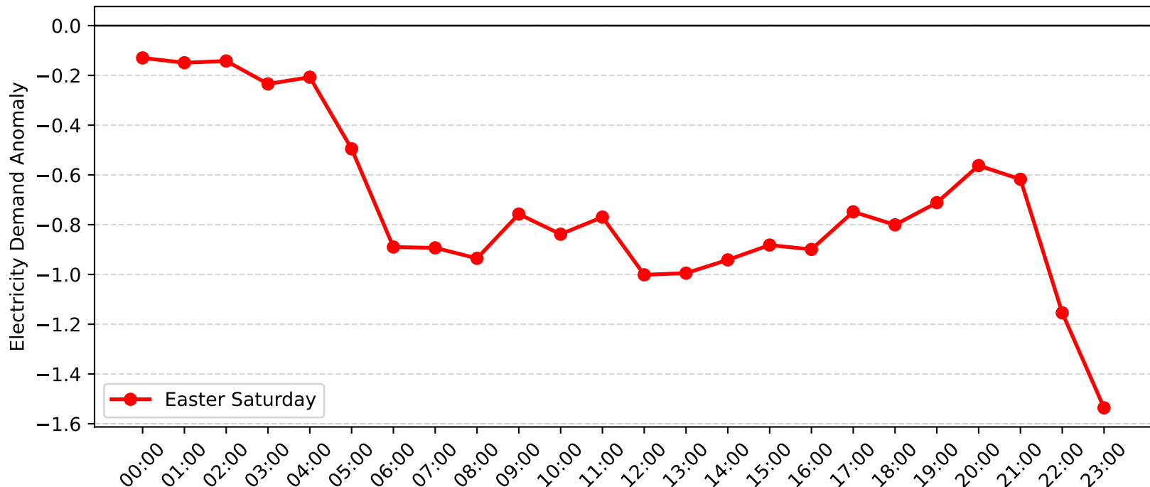
Muswellbrook Demand Anomaly: Easter Saturday (2013-2014)
