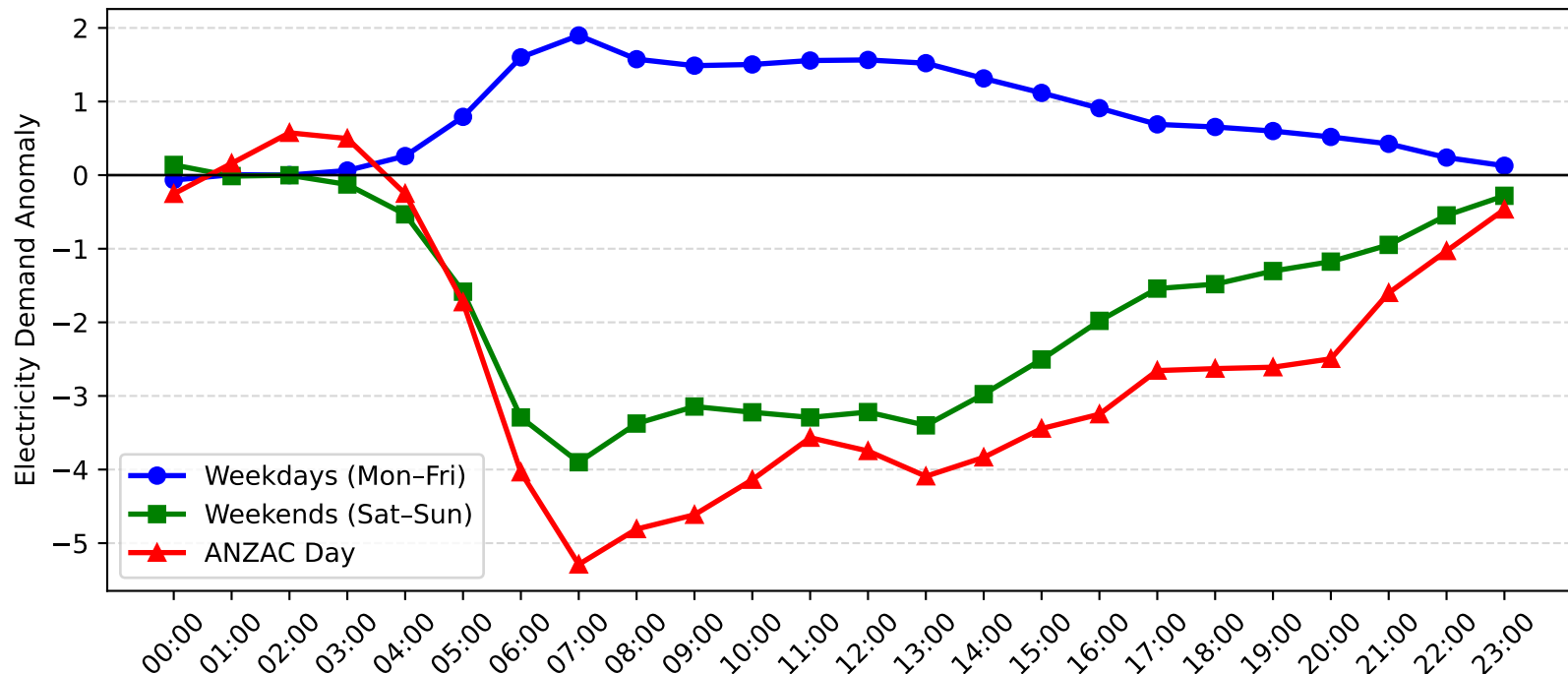
Wyong Demand Anomaly: ANZAC Day vs Weekday/Weekend (2009-2010)
