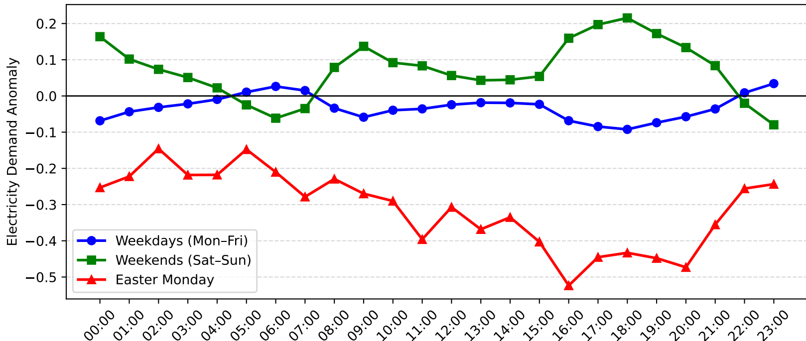
Rothbury Demand Anomaly: Easter Monday vs Weekday/Weekend (2014-2015)
