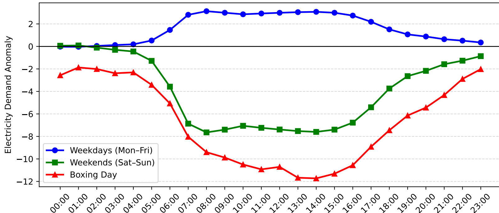
Zetland Demand Anomaly: Boxing Day vs Weekday/Weekend (2015-2016)
