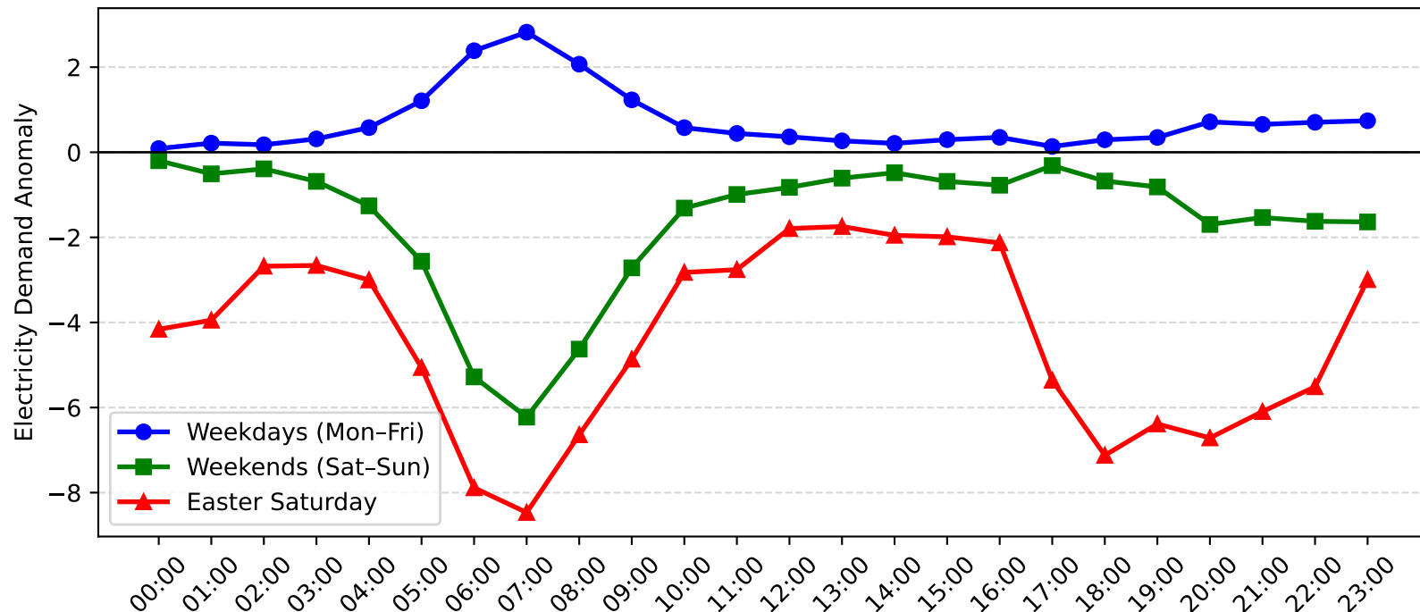
Meadowbank Demand Anomaly: Easter Saturday vs Weekday/Weekend (2010-2011)
