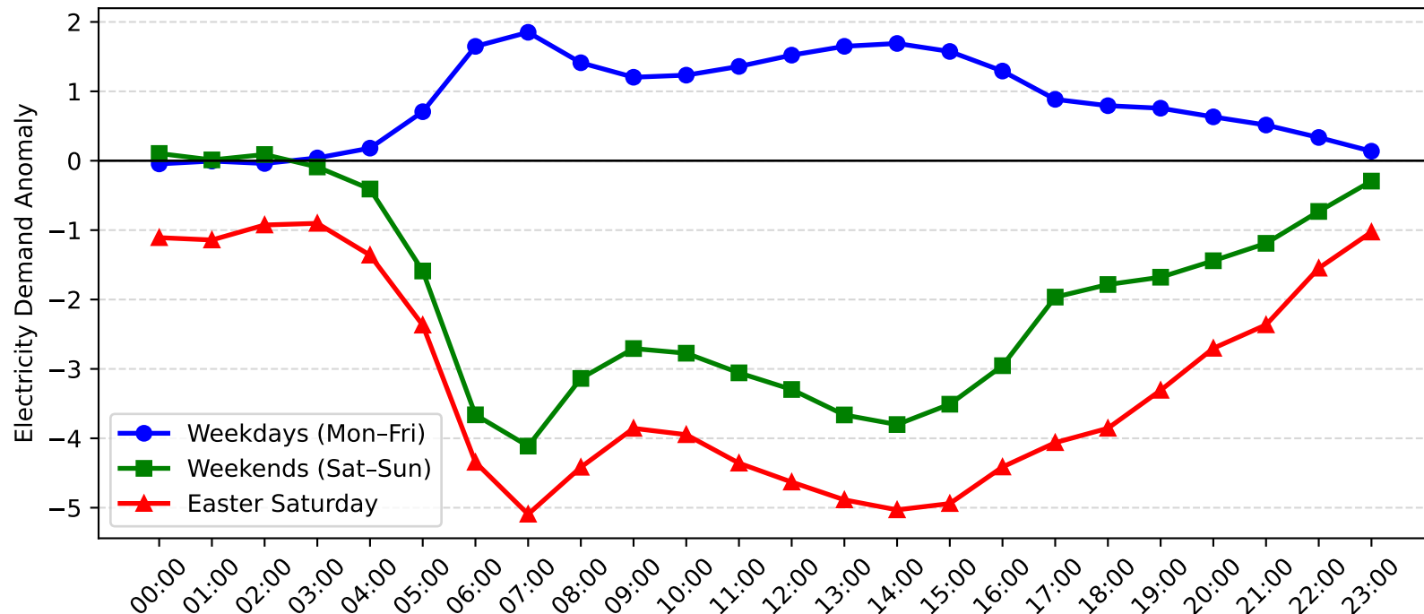
Kirrawee Demand Anomaly: Easter Saturday vs Weekday/Weekend (2008-2009)
