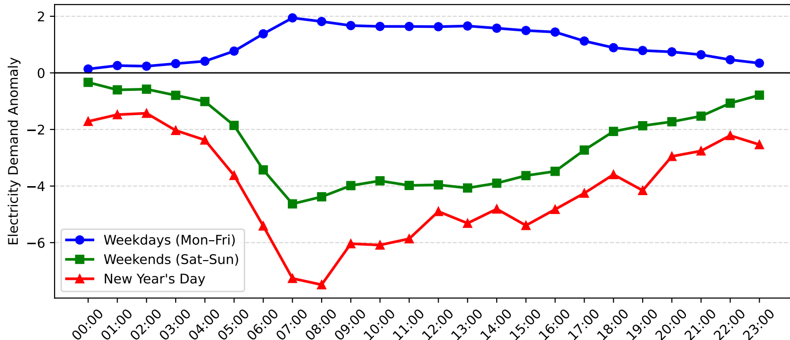
Matraverse Demand Anomaly: New Year's Day vs Weekday/Weekend (2007-2008)
