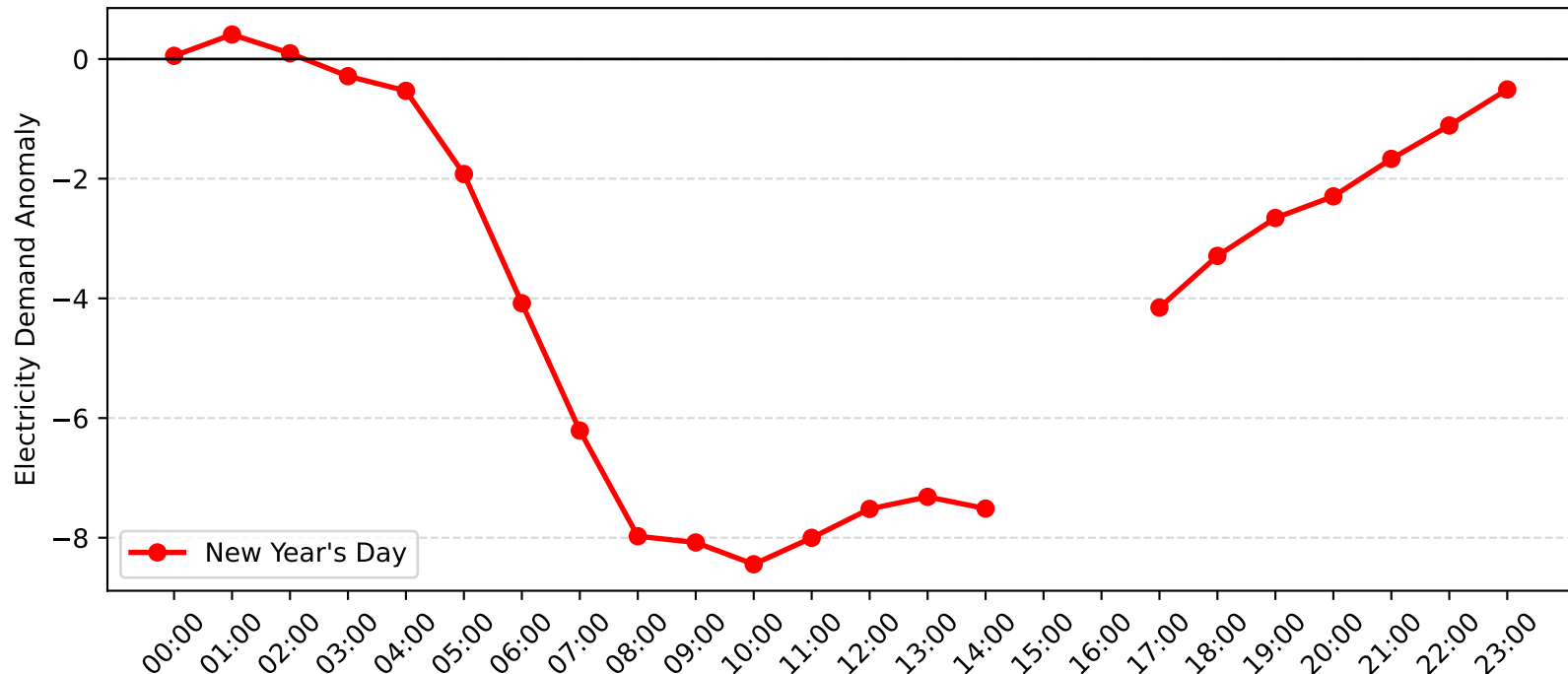
Bankstown Demand Anomaly: New Year's Day (2015-2016)
