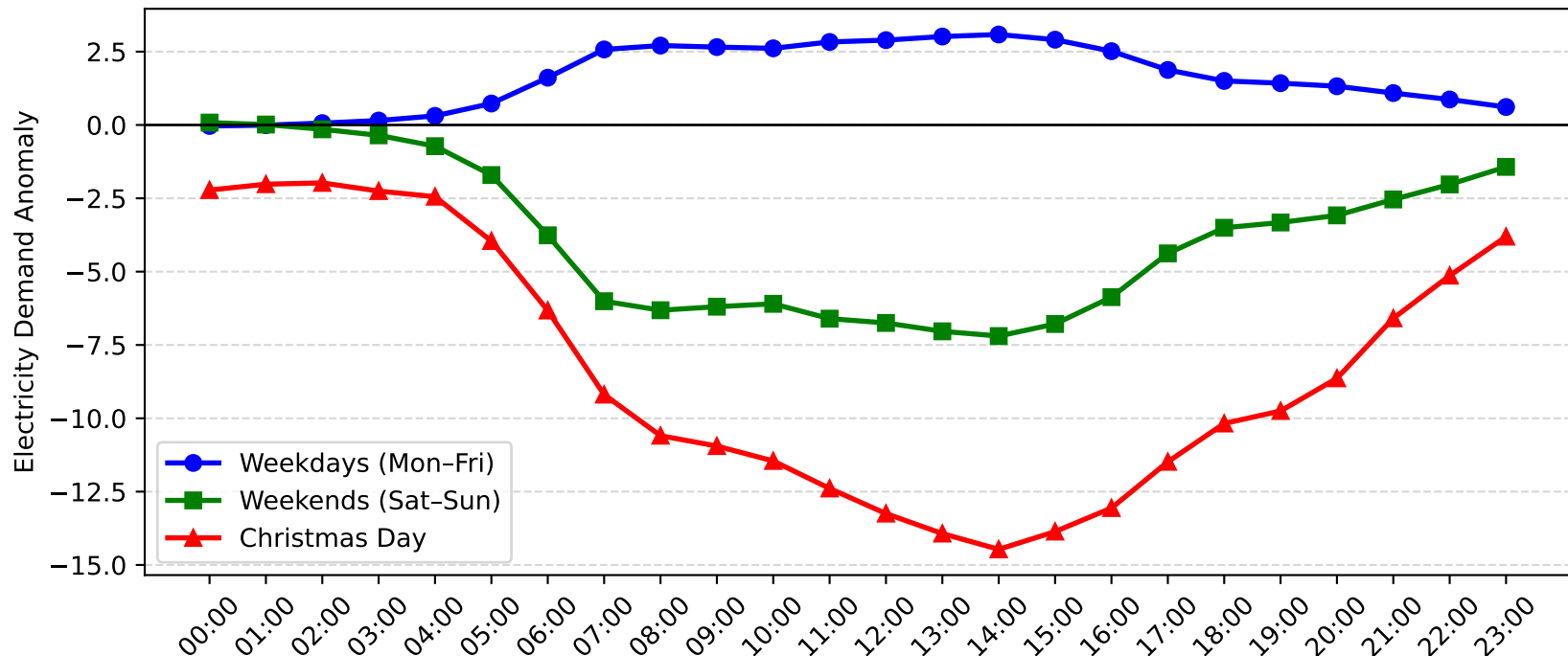
Marrickville Demand Anomaly: Christmas Day vs Weekday/Weekend (2016-2017)
