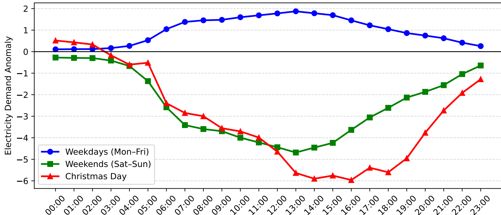
Wyong Demand Anomaly: Christmas Day vs Weekday/Weekend (2015-2016)
