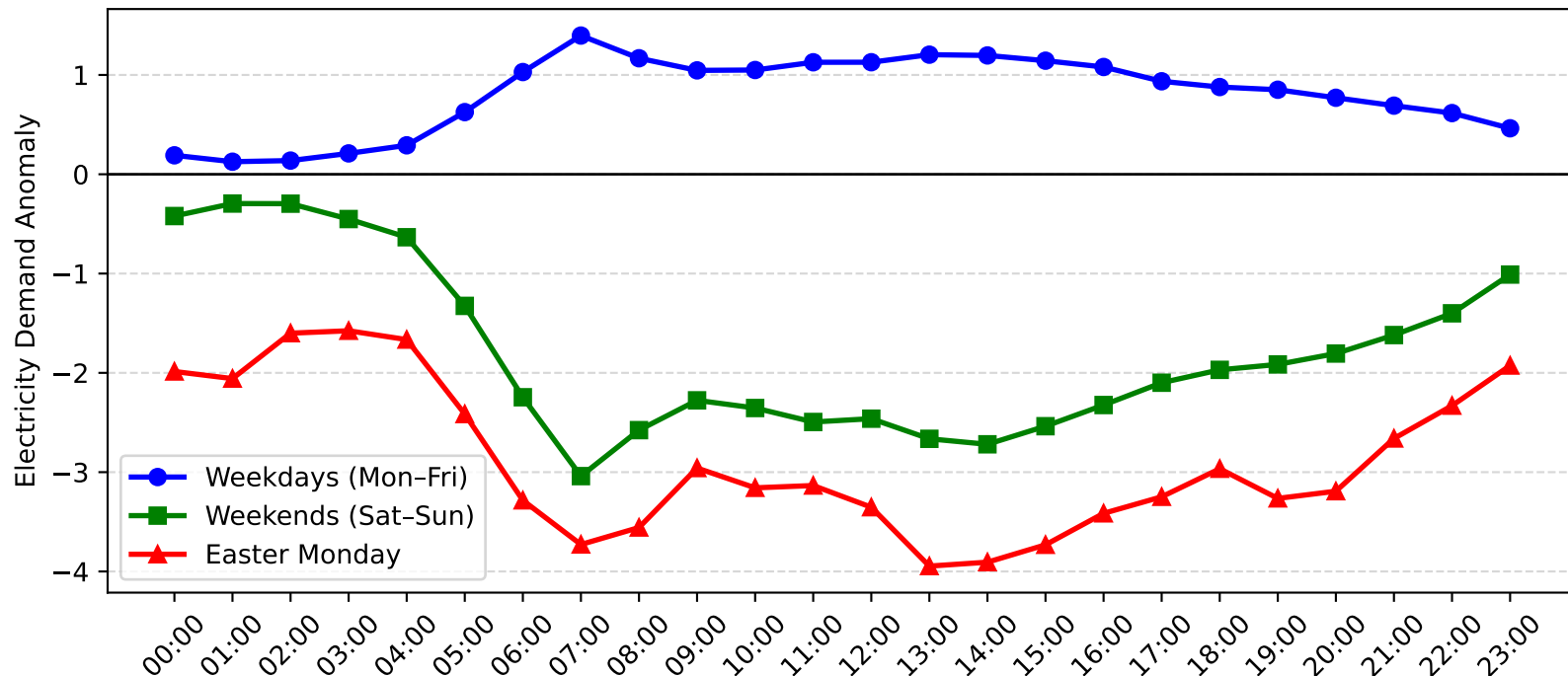
Bass Hill Demand Anomaly: Easter Monday vs Weekday/Weekend (2009-2010)
