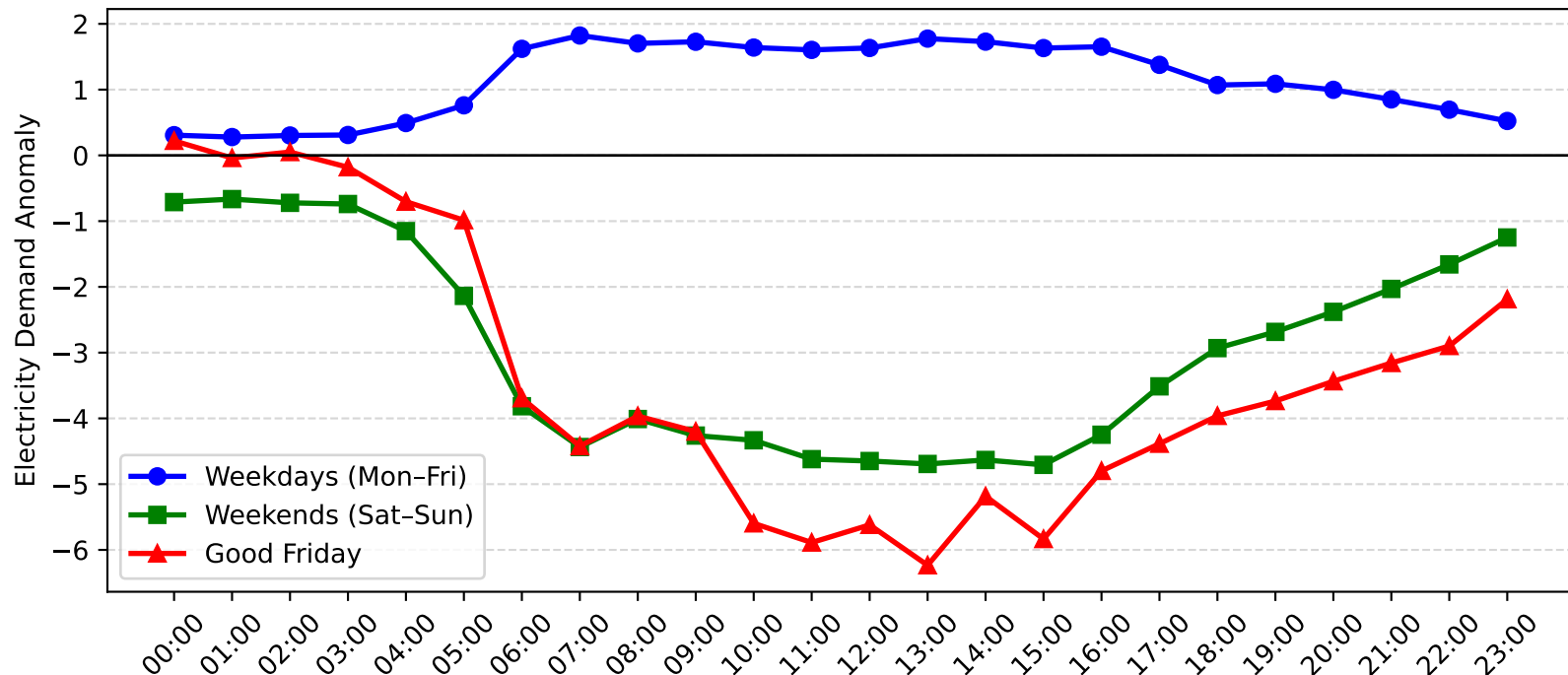
Potts Hill Demand Anomaly: Good Friday vs Weekday/Weekend (2016-2017)
