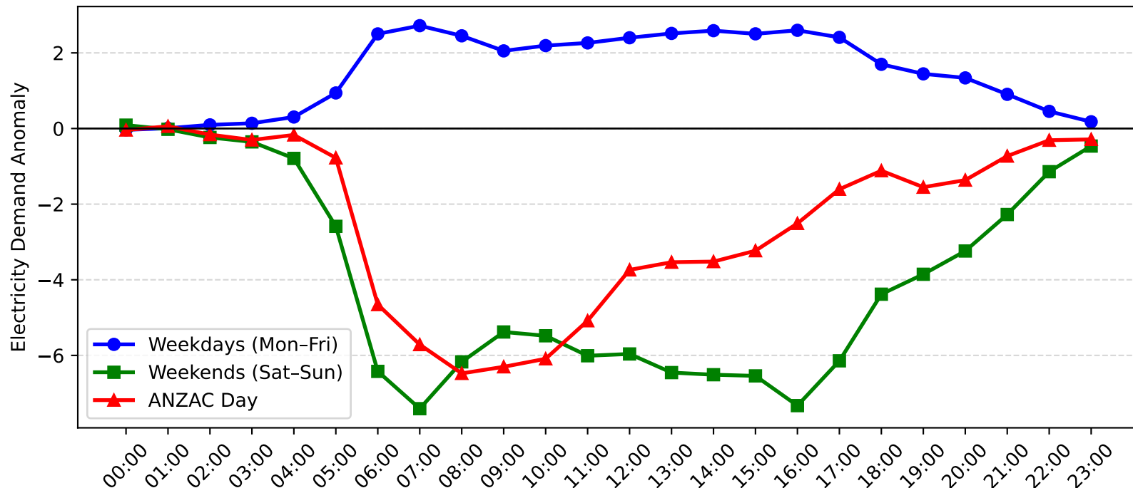
Epping Demand Anomaly: ANZAC Day vs Weekday/Weekend (2006-2007)
