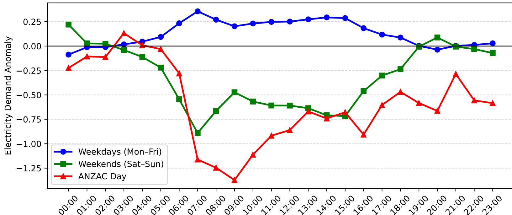
Rockdale Demand Anomaly: ANZAC Day vs Weekday/Weekend (2004-2005)
