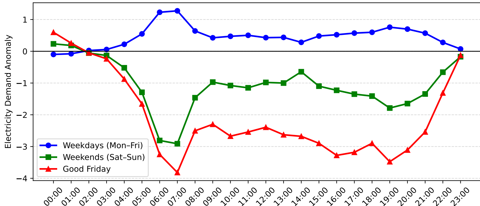
Revesby Demand Anomaly: Good Friday vs Weekday/Weekend (2017-2018)
