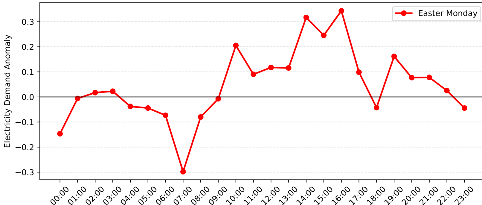
Rothbury Demand Anomaly: Easter Monday (2007-2008)
