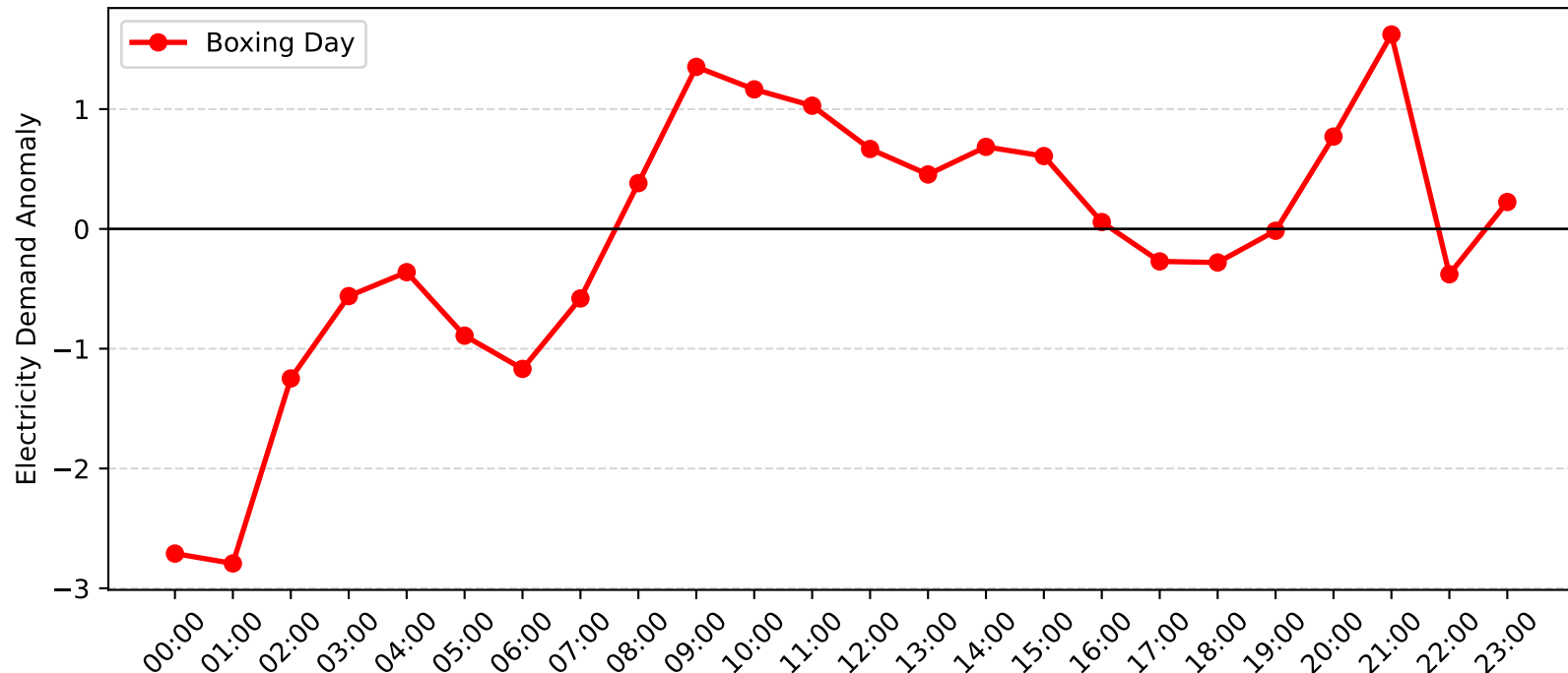
Nelson Bay Demand Anomaly: Boxing Day (2011-2012)
