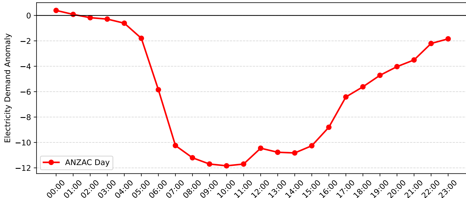
Zetland Demand Anomaly: ANZAC Day (2007-2008)
