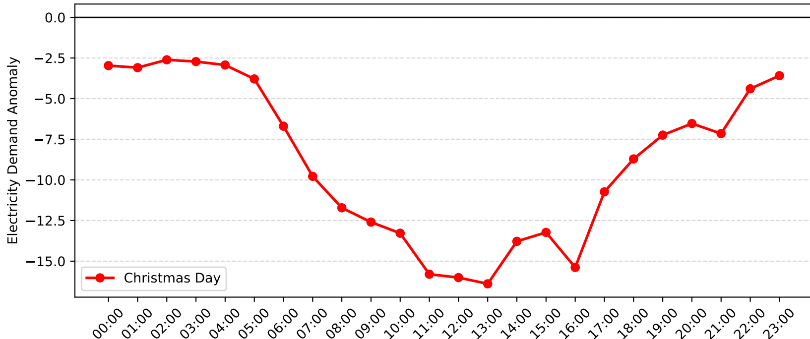
Macquarie Park Demand Anomaly: Christmas Day (2007-2008)
