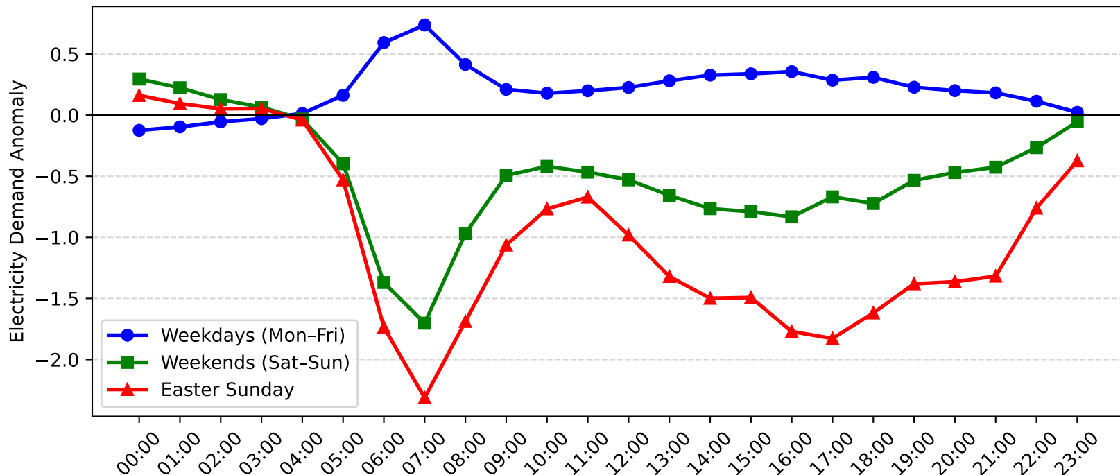
Blakehurst Demand Anomaly: Easter Sunday vs Weekday/Weekend (2011-2012)
