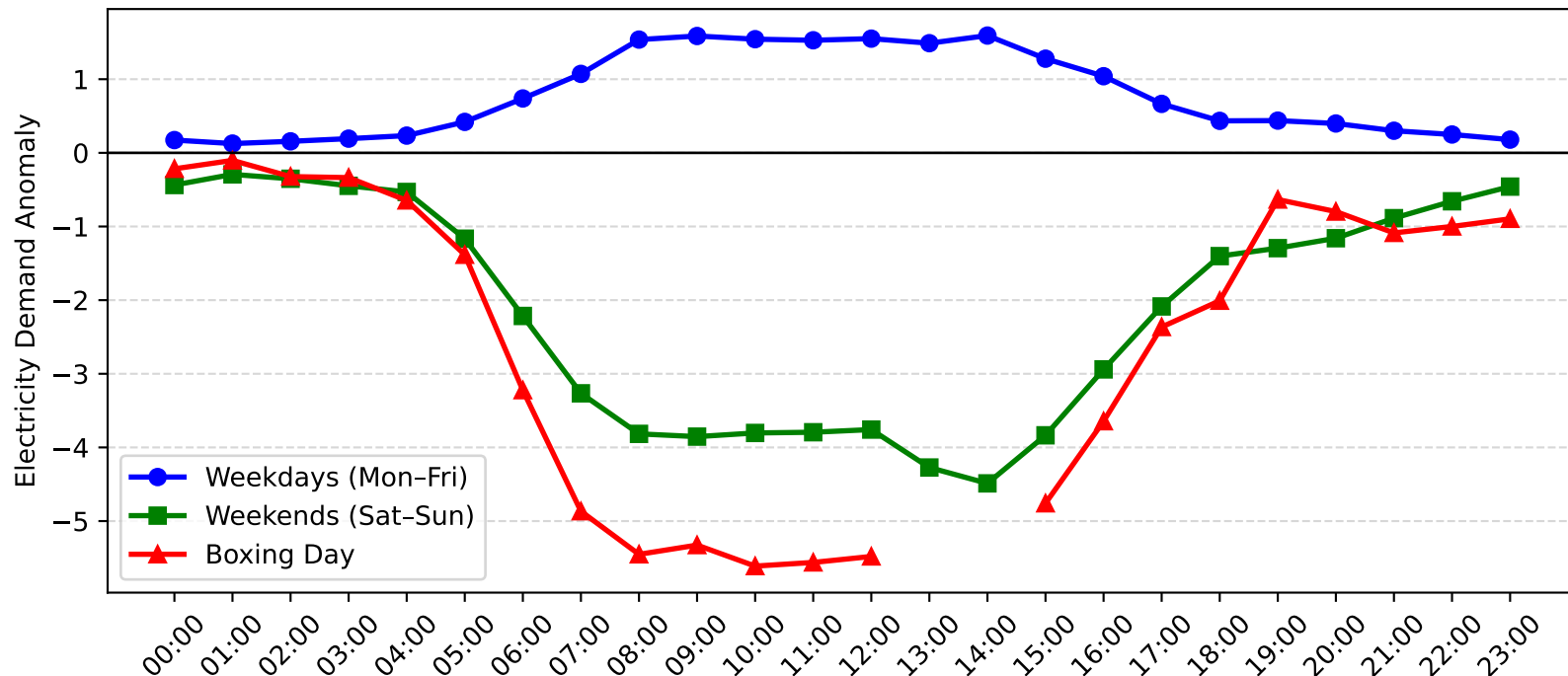
Bankstown Demand Anomaly: Boxing Day vs Weekday/Weekend (2010-2011)
