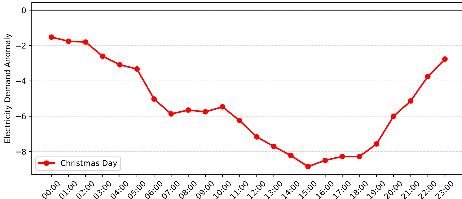
Matraville Demand Anomaly: Christmas Day (2006-2007)
