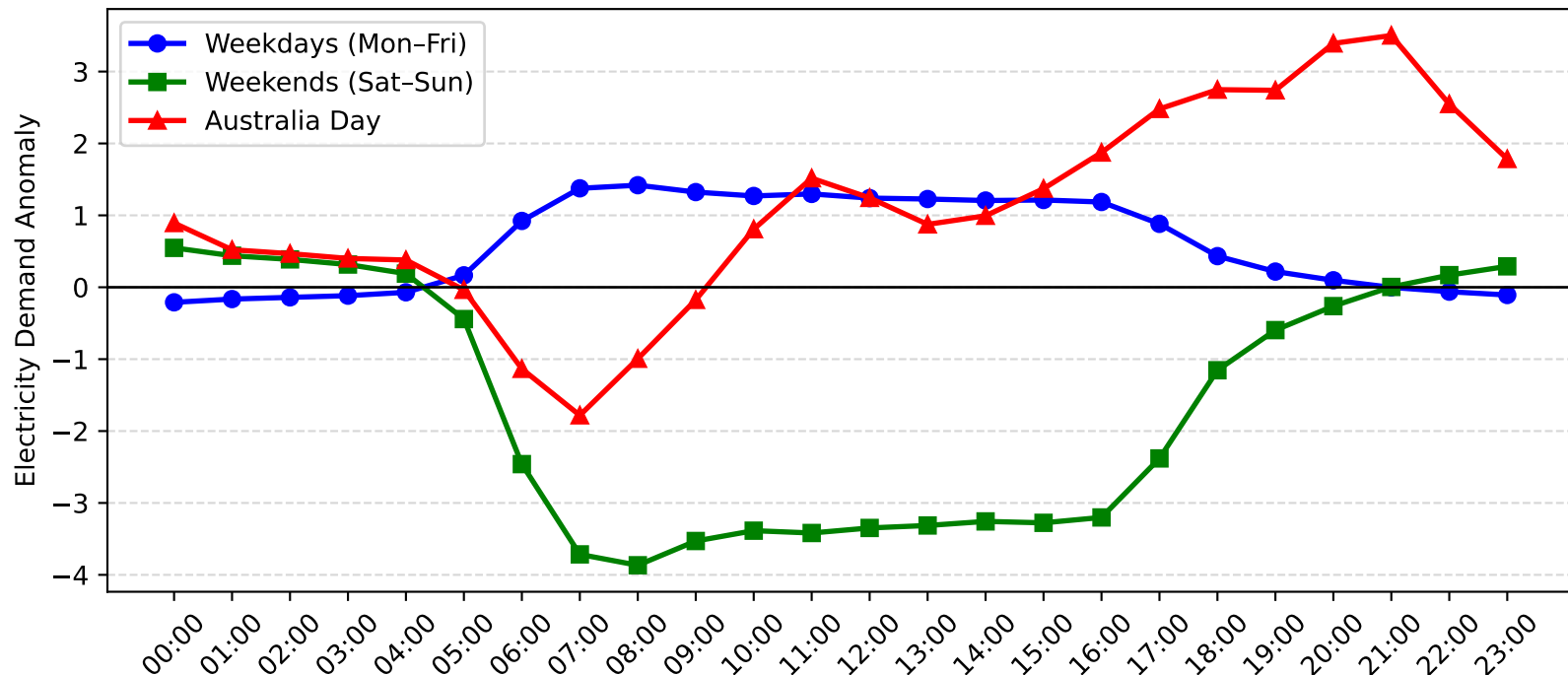
Pymble Demand Anomaly: Australia Day vs Weekday/Weekend (2011-2012)
