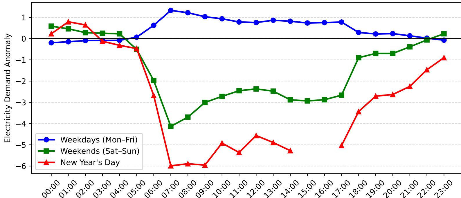
Chatswood Demand Anomaly: New Year's Day vs Weekday/Weekend (2014-2015)
