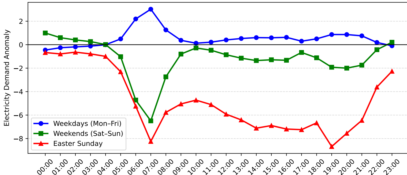
Mosman Demand Anomaly: Easter Sunday vs Weekday/Weekend (2009-2010)
