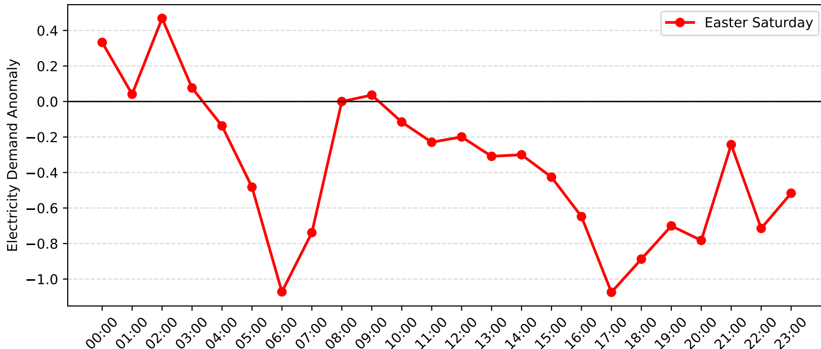
Morisset Demand Anomaly: Easter Saturday (2012-2013)
