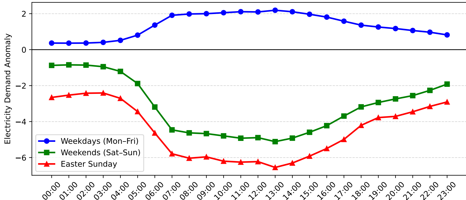
Leightonfield Demand Anomaly: Easter Sunday vs Weekday/Weekend (2012-2013)
