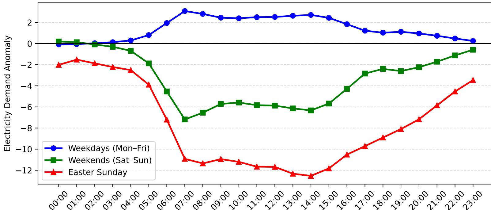
Marrickville Demand Anomaly: Easter Sunday vs Weekday/Weekend (2013-2014)
