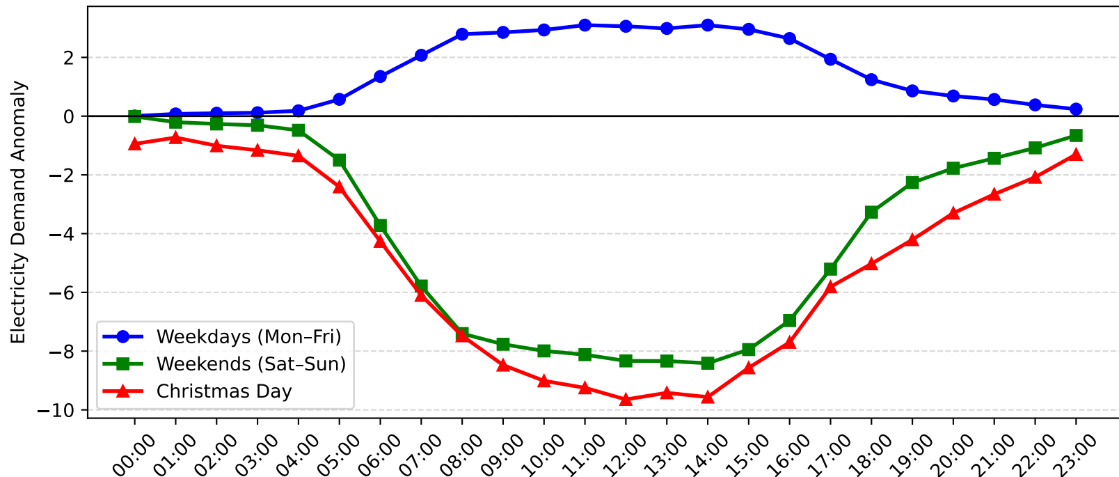
Mascot Demand Anomaly: Christmas Day vs Weekday/Weekend (2014-2015)
