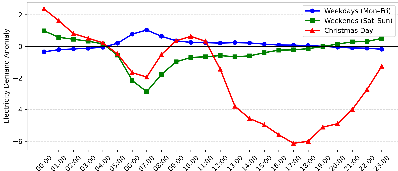
Mortdale Demand Anomaly: Christmas Day vs Weekday/Weekend (2012-2013)
