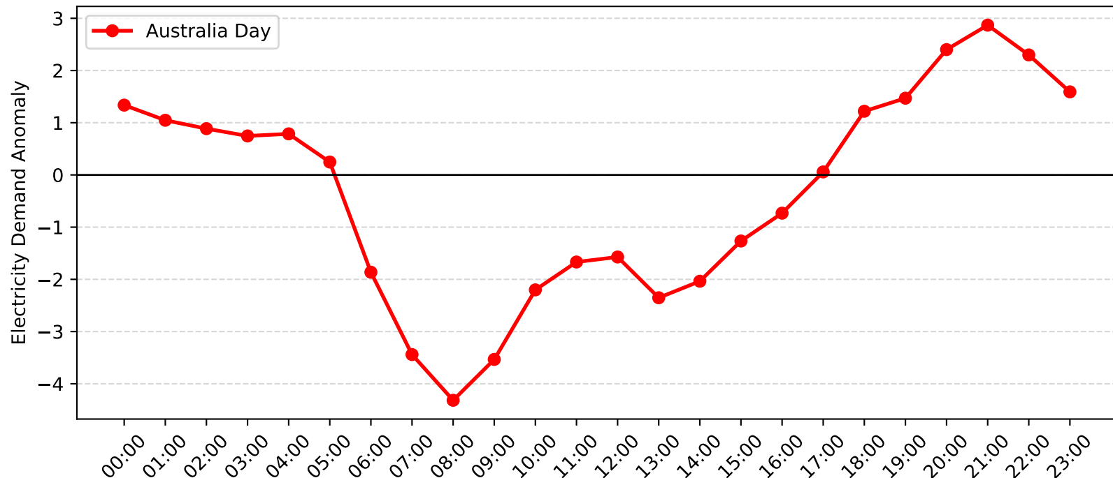
Castle Cove Demand Anomaly: Australia Day (2011-2012)
