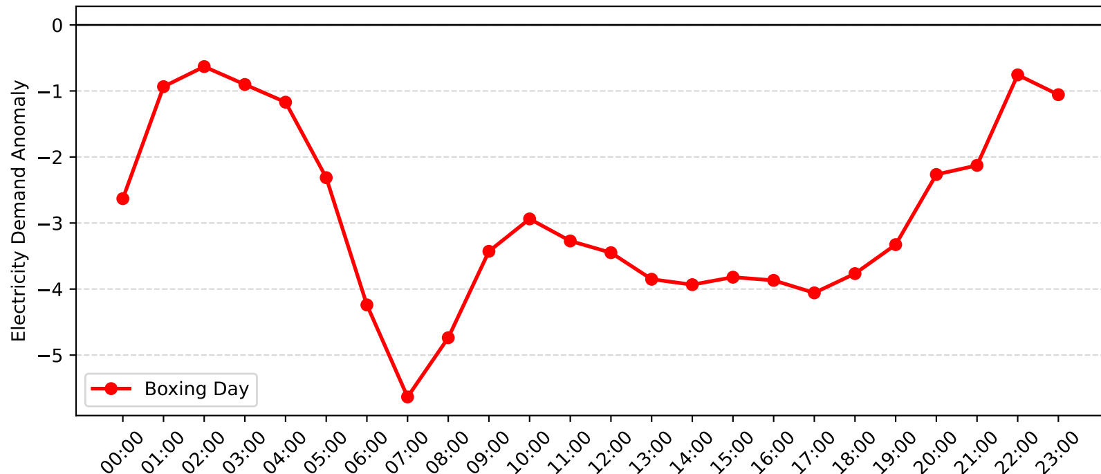
Dee Why West Demand Anomaly: Boxing Day (2007-2008)
