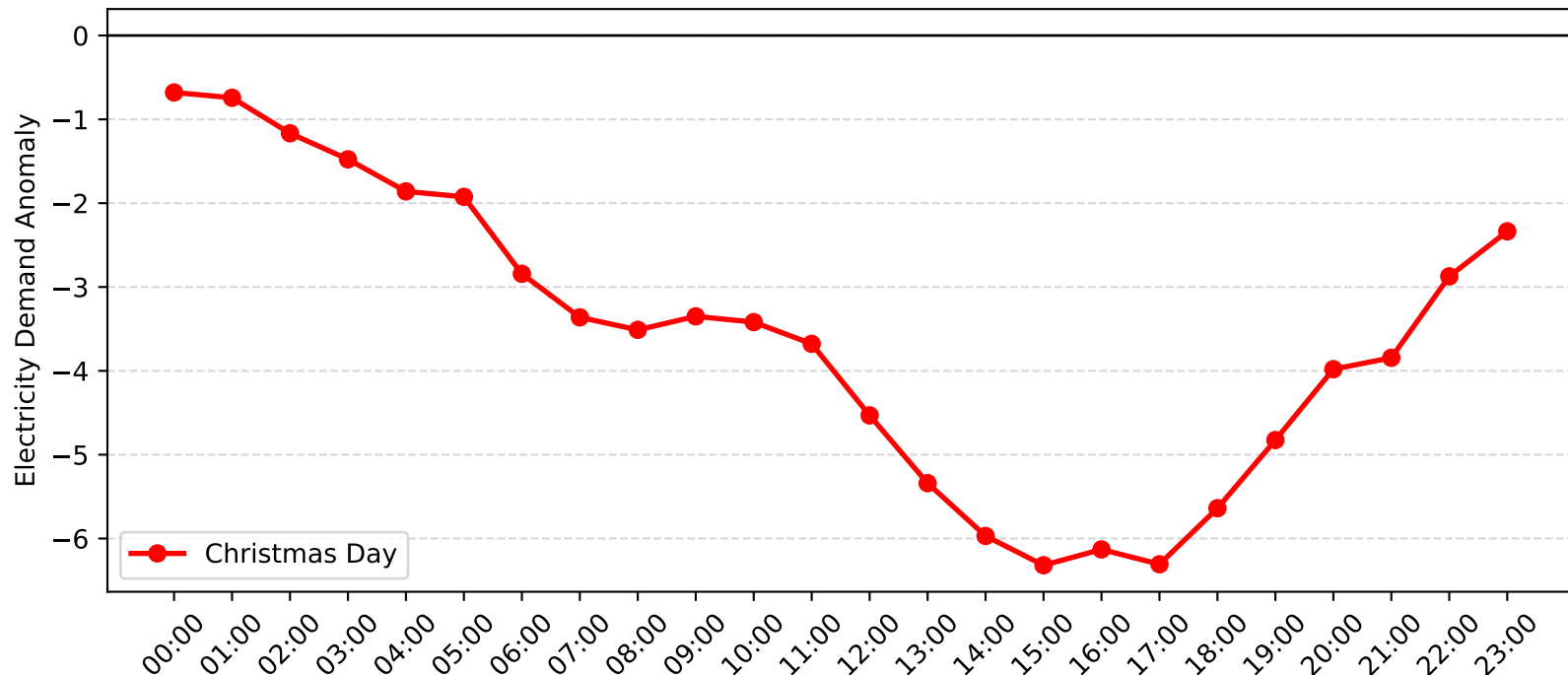
Bass Hill Demand Anomaly: Christmas Day (2006-2007)
