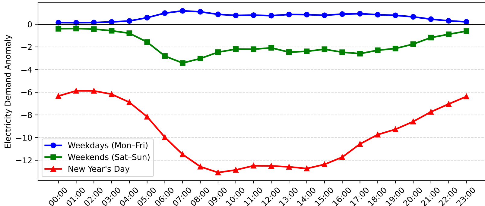
Maroubra Demand Anomaly: New Year's Day vs Weekday/Weekend (2015-2016)
