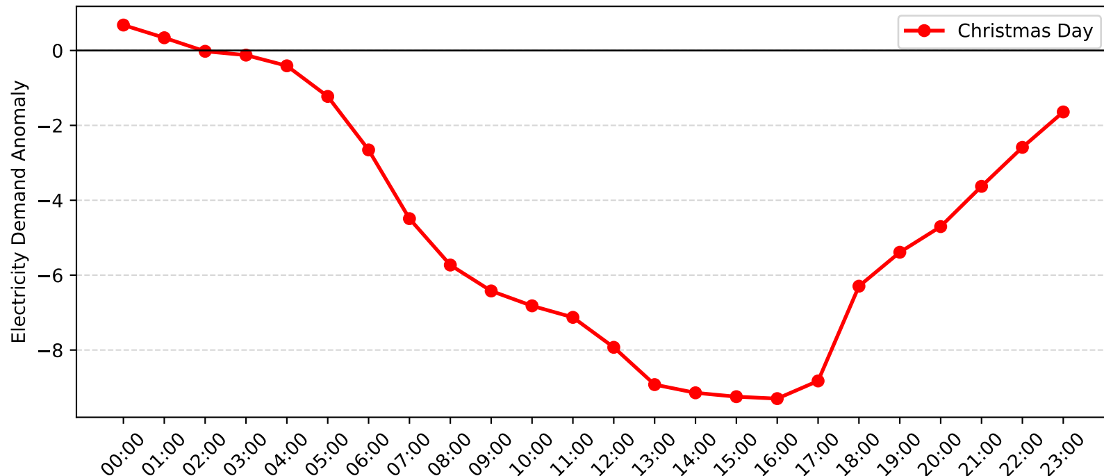
Top Ryde Demand Anomaly: Christmas Day (2011-2012)
