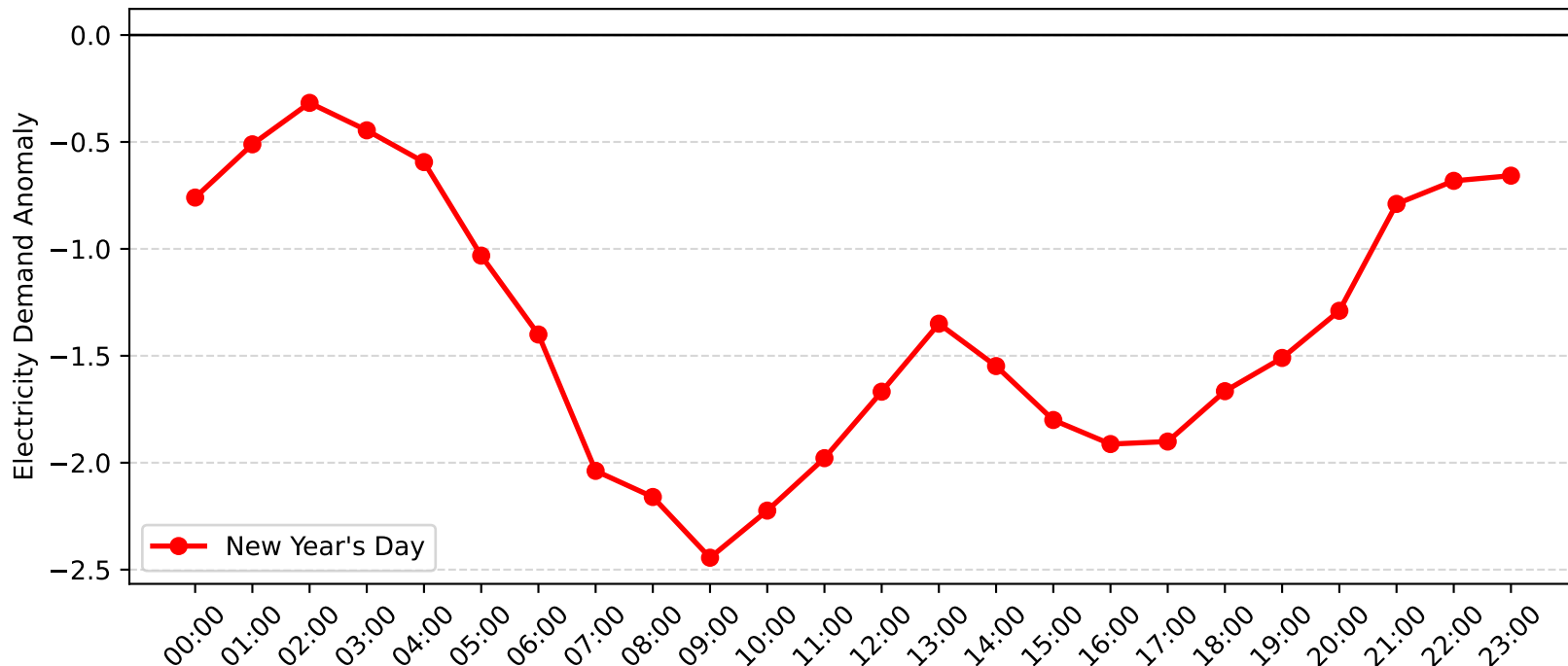
Lidcombe Demand Anomaly: New Year's Day (2013-2014)
