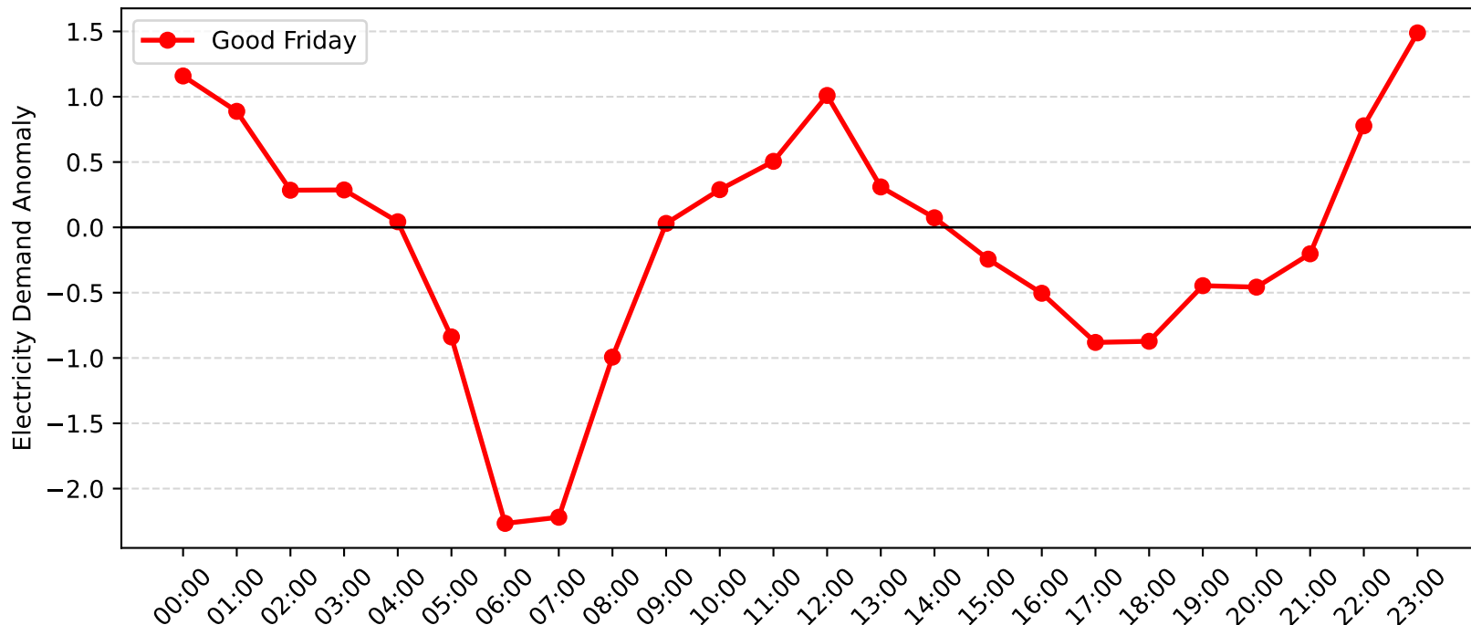
Avoca Demand Anomaly: Good Friday (2012-2013)
