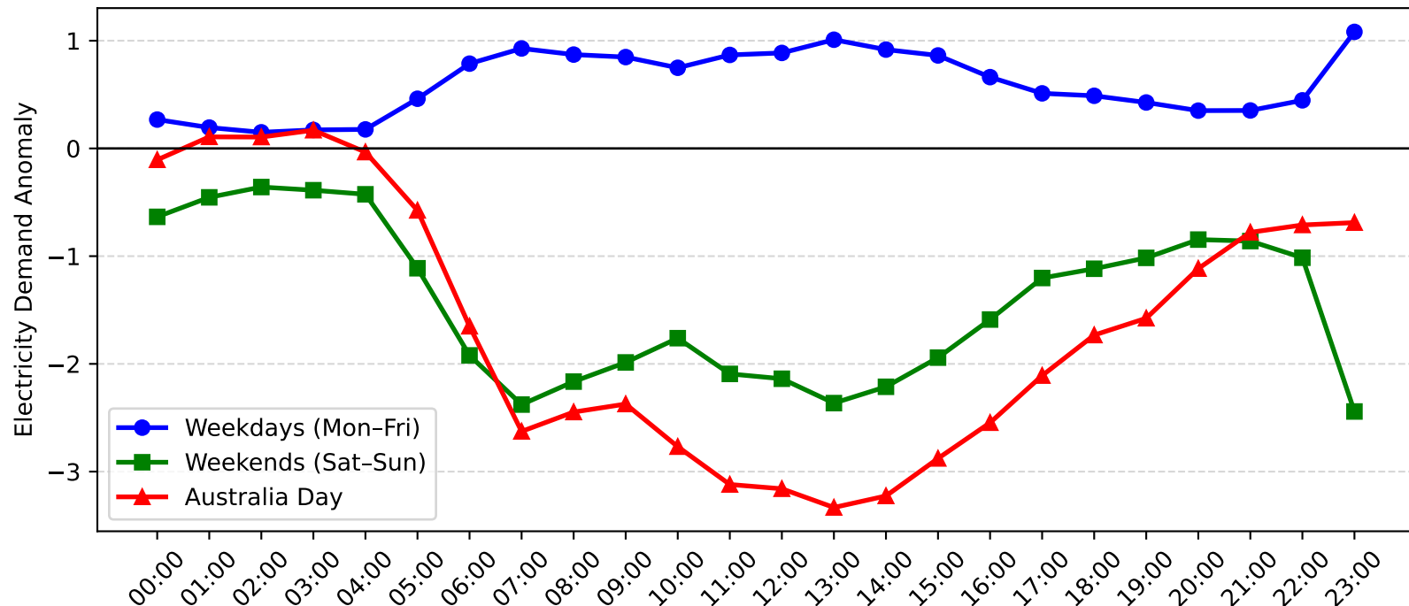
Rutherford Demand Anomaly: Australia Day vs Weekday/Weekend (2008-2009)
