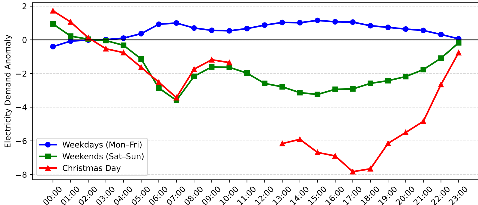
Mortdale Demand Anomaly: Christmas Day vs Weekday/Weekend (2008-2009)
