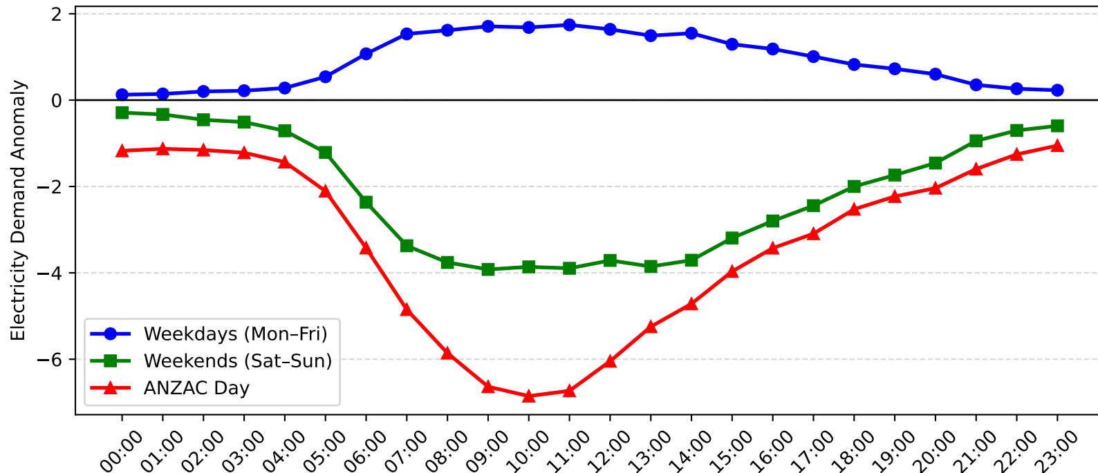
Auburn Demand Anomaly: ANZAC Day vs Weekday/Weekend (2010-2011)
