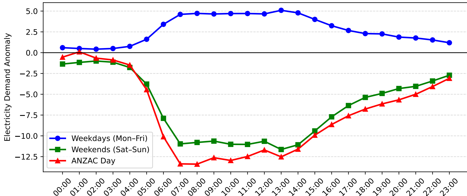
Milperra Demand Anomaly: ANZAC Day vs Weekday/Weekend (2008-2009)
