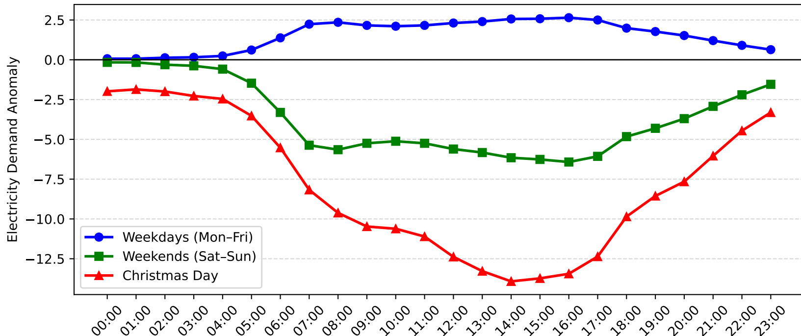
Burwood Demand Anomaly: Christmas Day vs Weekday/Weekend (2015-2016)
