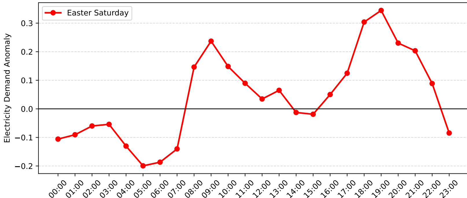
Rothbury Demand Anomaly: Easter Saturday (2014-2015)
