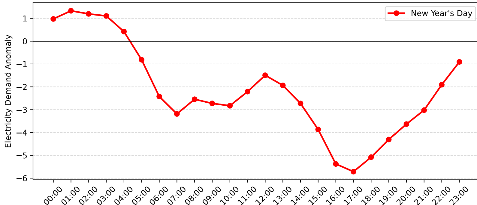
Revesby Demand Anomaly: New Year's Day (2017-2018)
