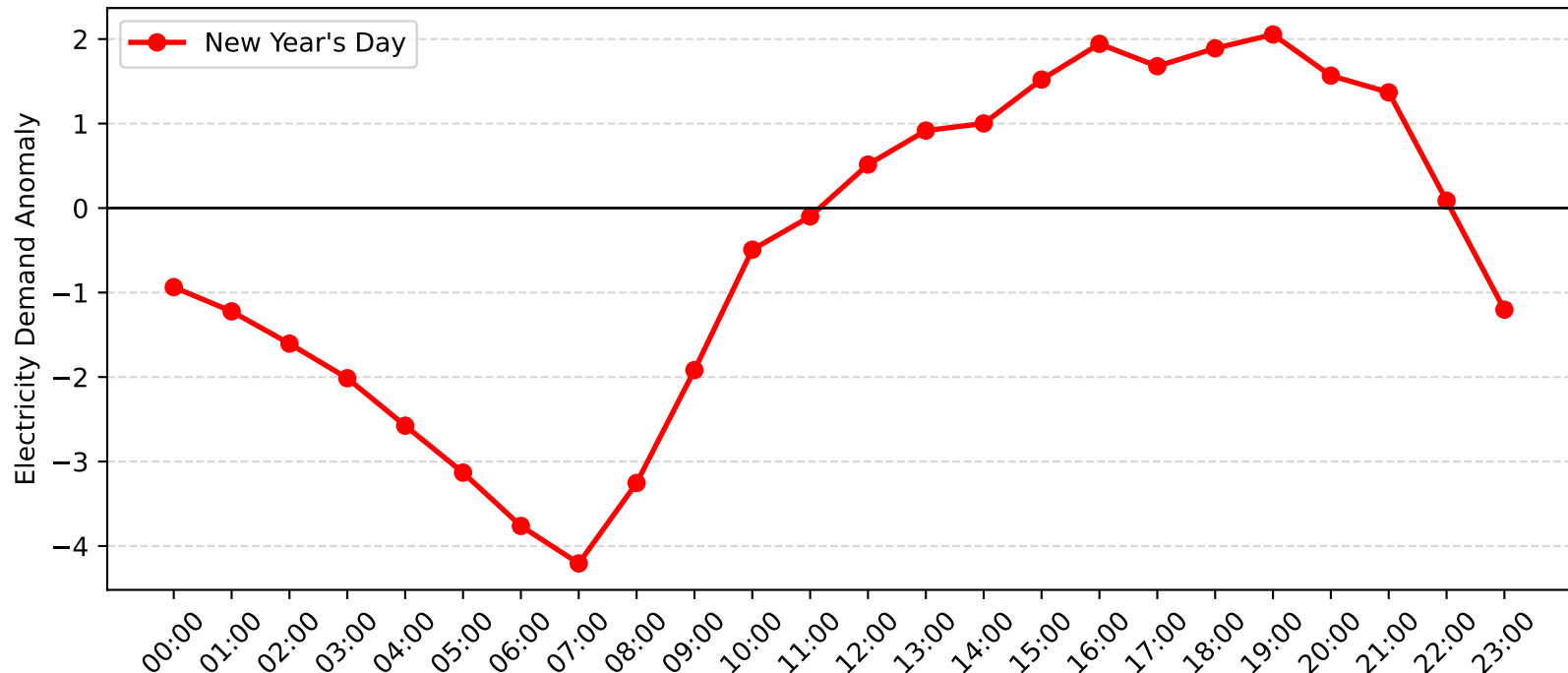
Lisarow Demand Anomaly: New Year's Day (2005-2006)
