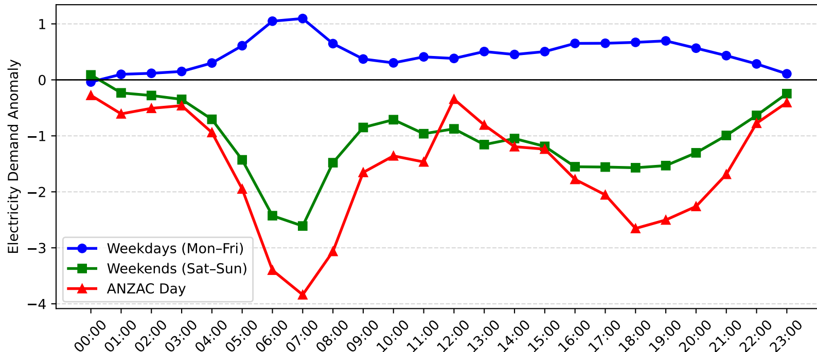
Charmhaven Demand Anomaly: ANZAC Day vs Weekday/Weekend (2008-2009)
