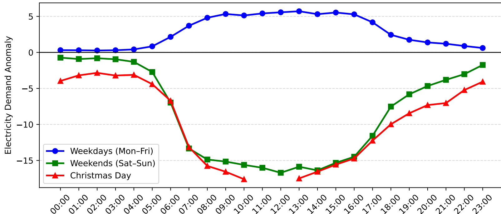
Gore Hill Demand Anomaly: Christmas Day vs Weekday/Weekend (2008-2009)
