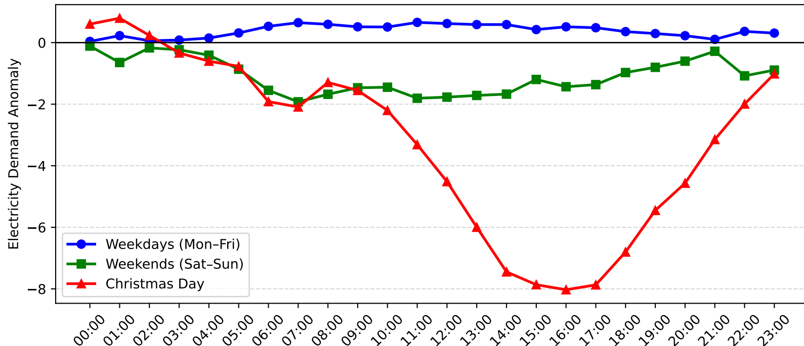
Jesmond Demand Anomaly: Christmas Day vs Weekday/Weekend (2013-2014)
