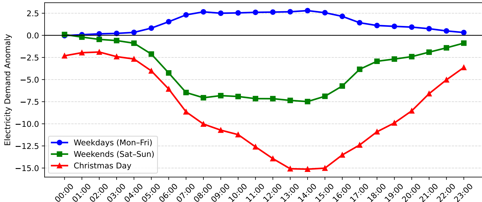
Marrickville Demand Anomaly: Christmas Day vs Weekday/Weekend (2014-2015)
