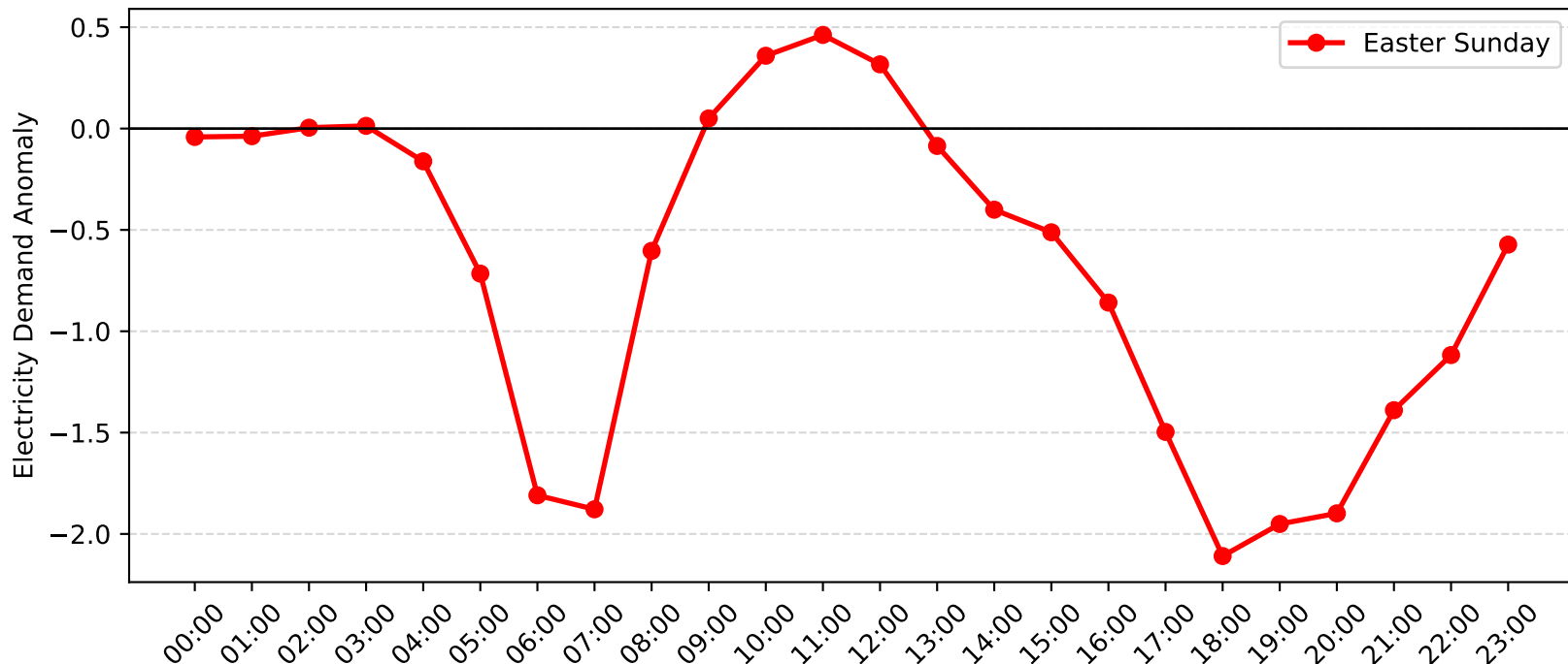
Harbord Demand Anomaly: Easter Sunday (2012-2013)
