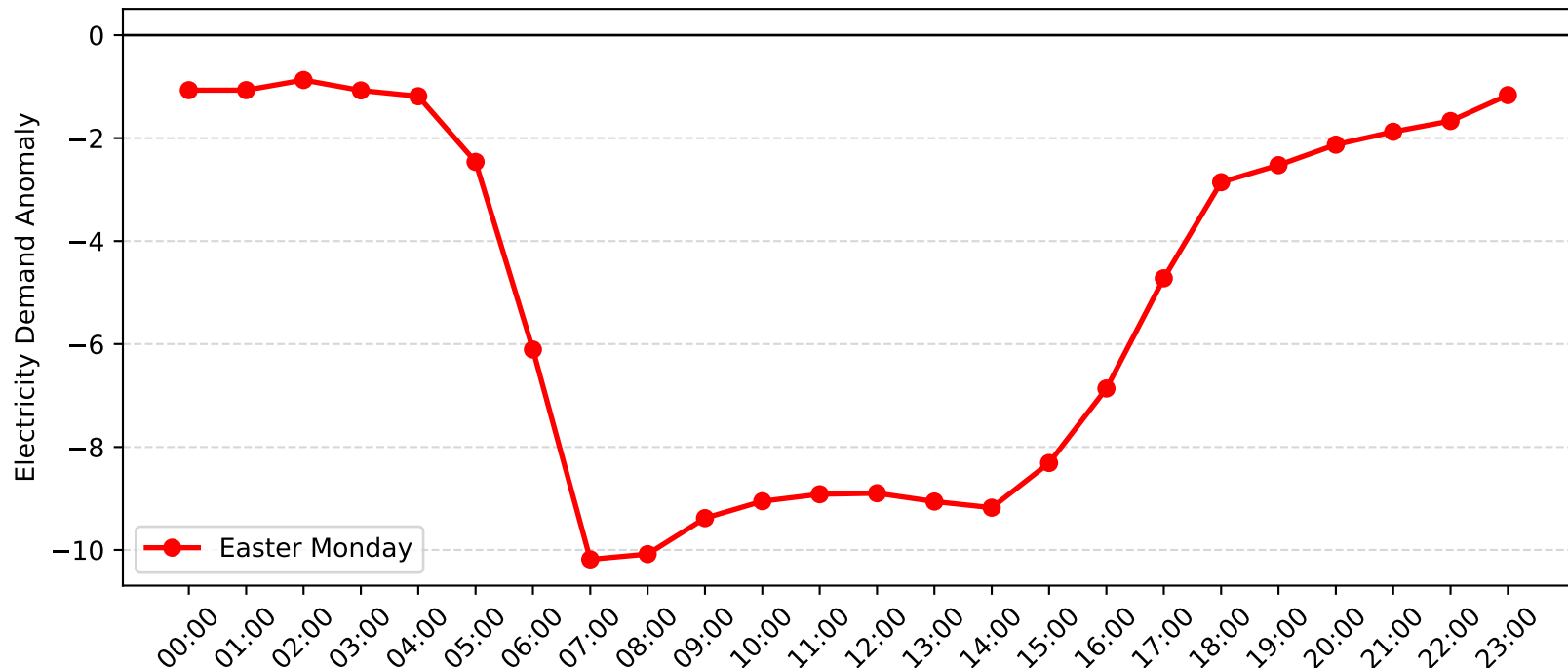
Marrickville Demand Anomaly: Easter Monday (2007-2008)
