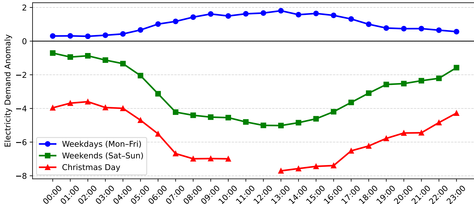
Leightonfield Demand Anomaly: Christmas Day vs Weekday/Weekend (2008-2009)
