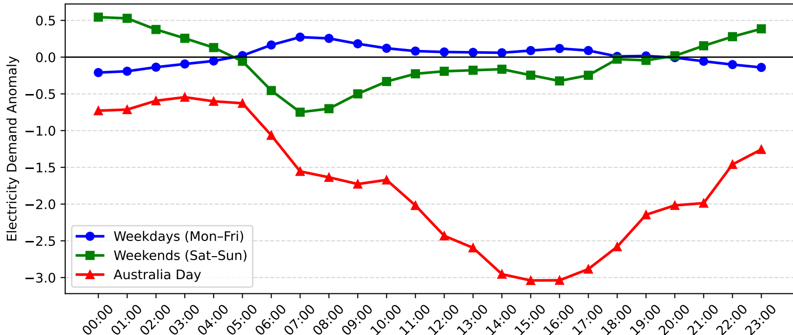
Rockdale Demand Anomaly: Australia Day vs Weekday/Weekend (2017-2018)
