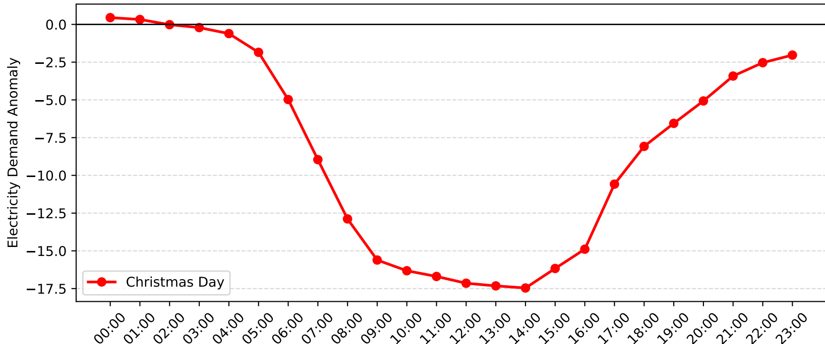
Brookvale Demand Anomaly: Christmas Day (2004-2005)
