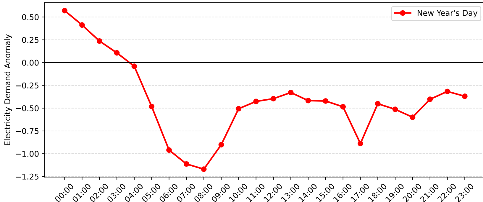
Narrabeen Demand Anomaly: New Year's Day (2010-2011)
