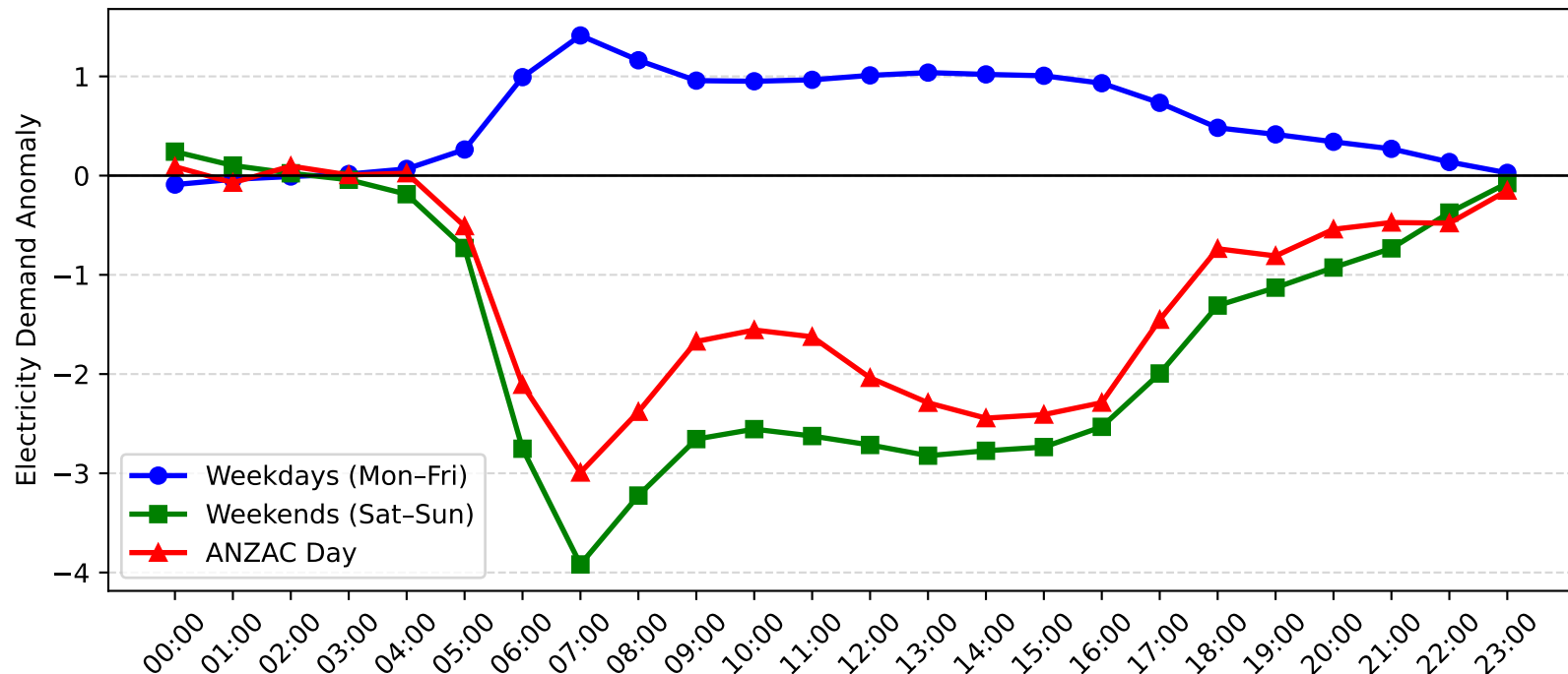
Pymble Demand Anomaly: ANZAC Day vs Weekday/Weekend (2012-2013)
