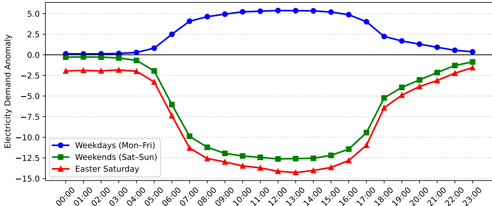
Macquarie Park Demand Anomaly: Easter Saturday vs Weekday/Weekend (2012-2013)
