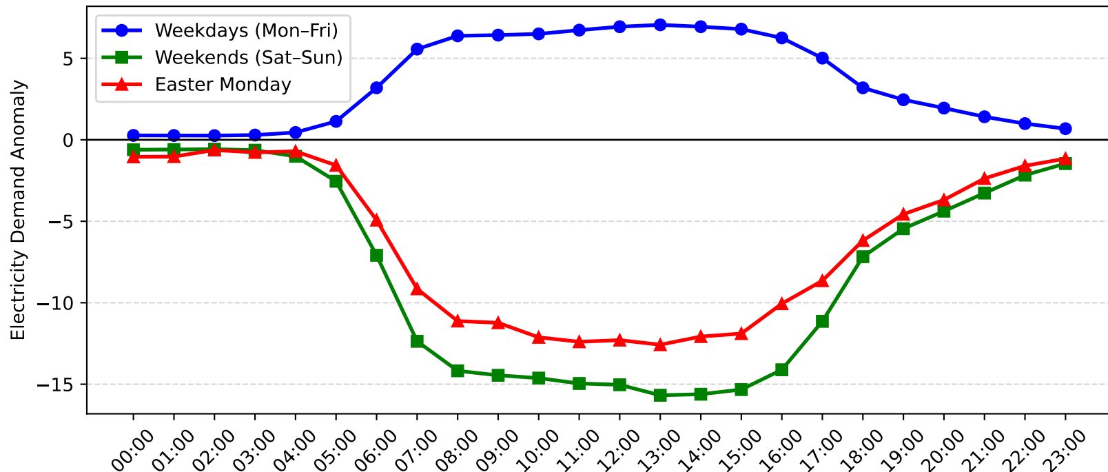
Gore Hill Demand Anomaly: Easter Monday vs Weekday/Weekend (2008-2009)
