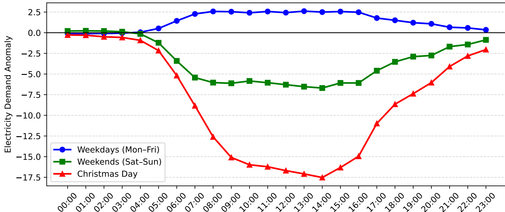
Brookvale Demand Anomaly: Christmas Day vs Weekday/Weekend (2005-2006)
