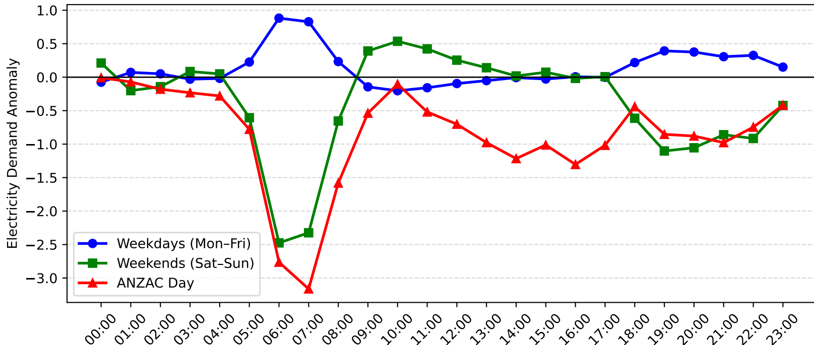
Balgowlah North Demand Anomaly: ANZAC Day vs Weekday/Weekend (2012-2013)
