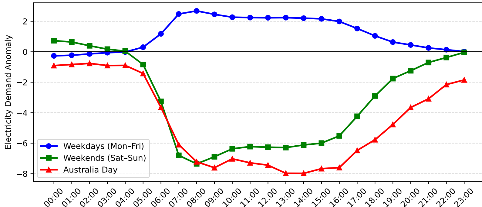
Zetland Demand Anomaly: Australia Day vs Weekday/Weekend (2016-2017)
