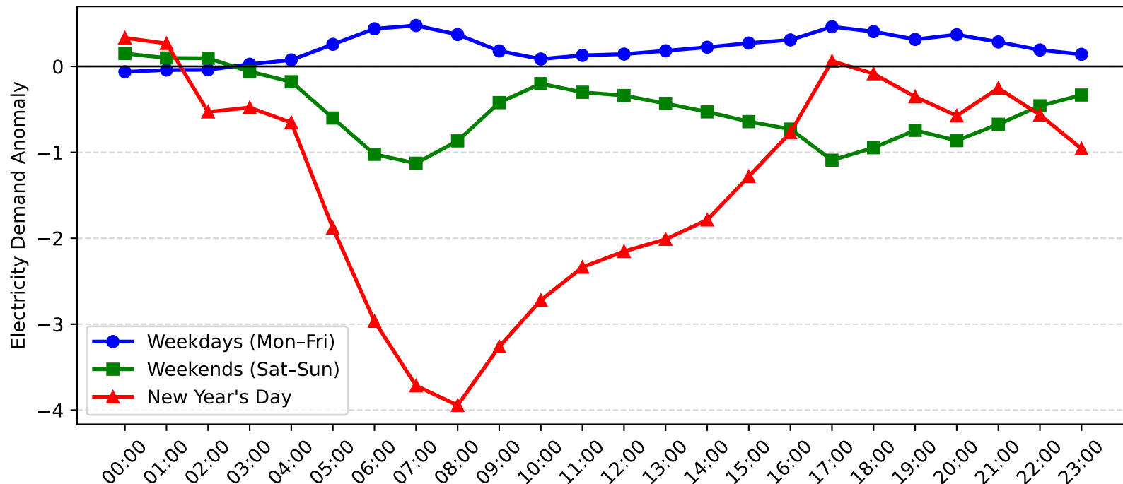
Charmhaven Demand Anomaly: New Year's Day vs Weekday/Weekend (2012-2013)
