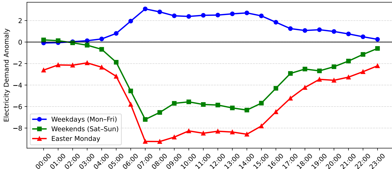
Marrickville Demand Anomaly: Easter Monday vs Weekday/Weekend (2013-2014)
