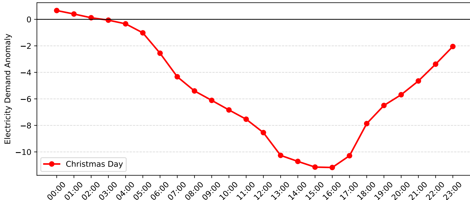
Top Ryde Demand Anomaly: Christmas Day (2012-2013)
