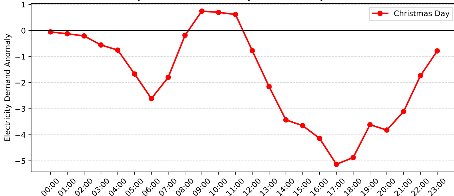
Dee Why West Demand Anomaly: Christmas Day (2013-2014)
