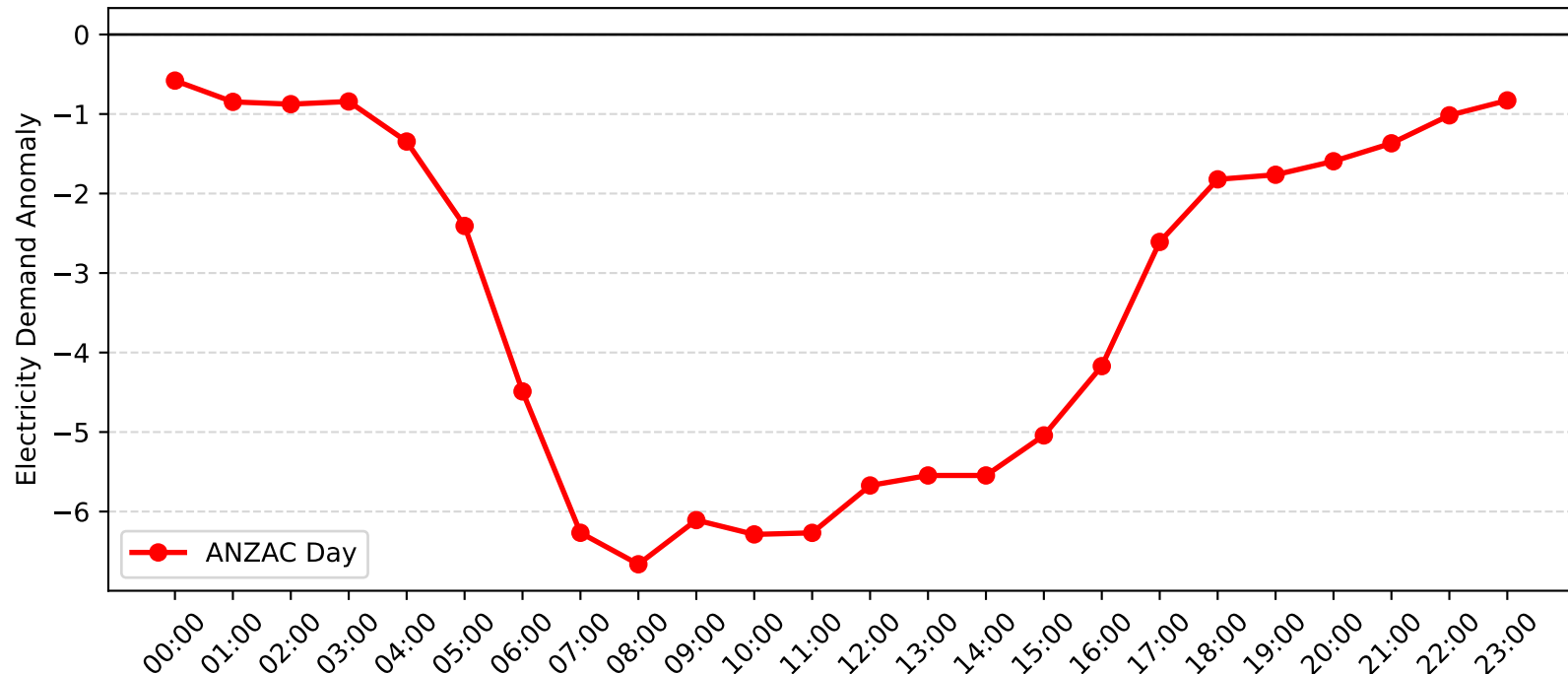
Bankstown Demand Anomaly: ANZAC Day (2016-2017)
