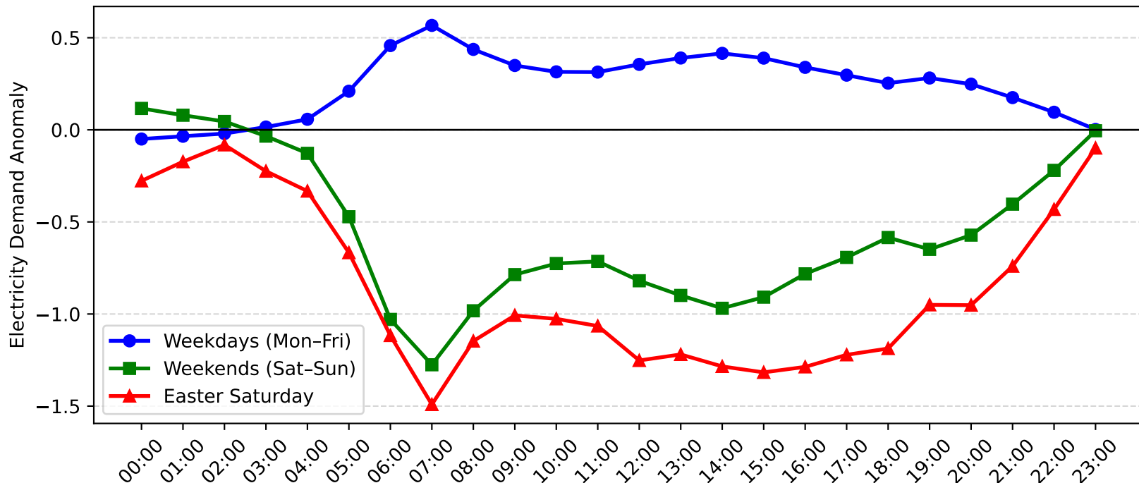
Rockdale Demand Anomaly: Easter Saturday vs Weekday/Weekend (2015-2016)
