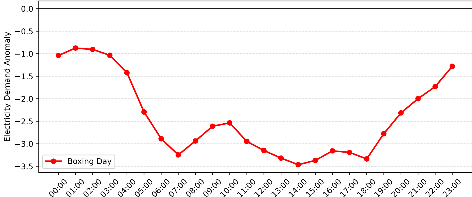
Lisarow Demand Anomaly: Boxing Day (2011-2012)
