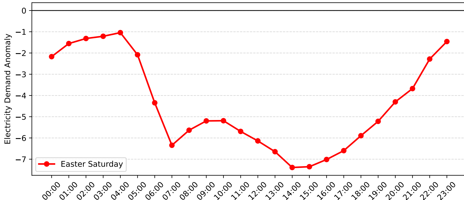
Burwood Demand Anomaly: Easter Saturday (2008-2009)
