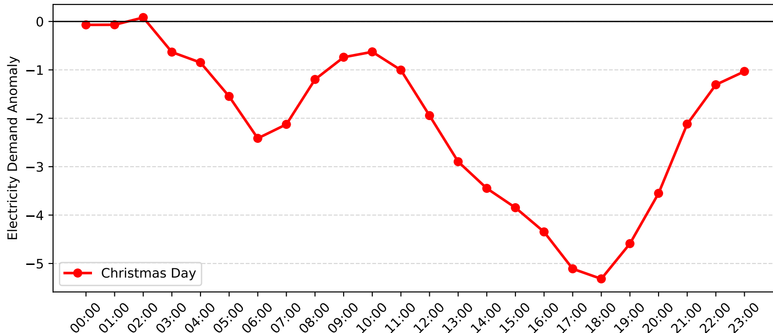
Dee Why West Demand Anomaly: Christmas Day (2015-2016)
