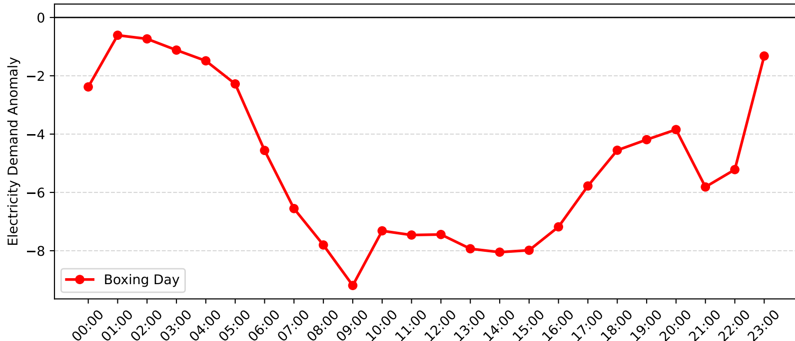
Punchbowl Demand Anomaly: Boxing Day (2008-2009)
