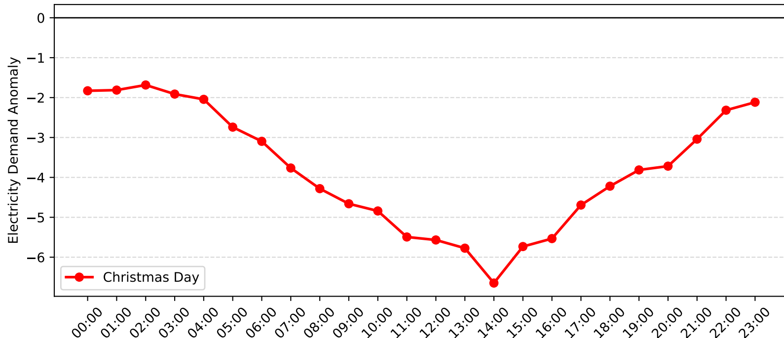
Caringbah Demand Anomaly: Christmas Day (2015-2016)
