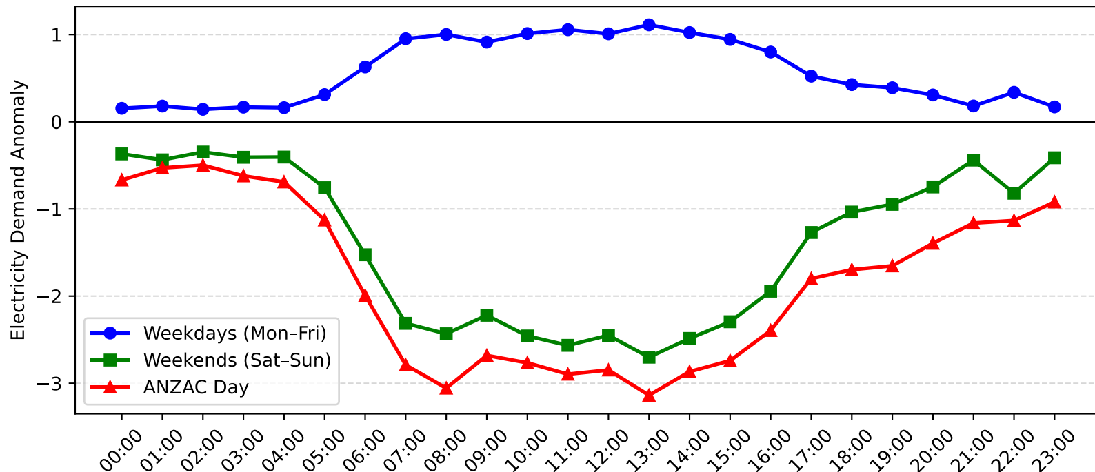
Mayfield West Demand Anomaly: ANZAC Day vs Weekday/Weekend (2014-2015)
