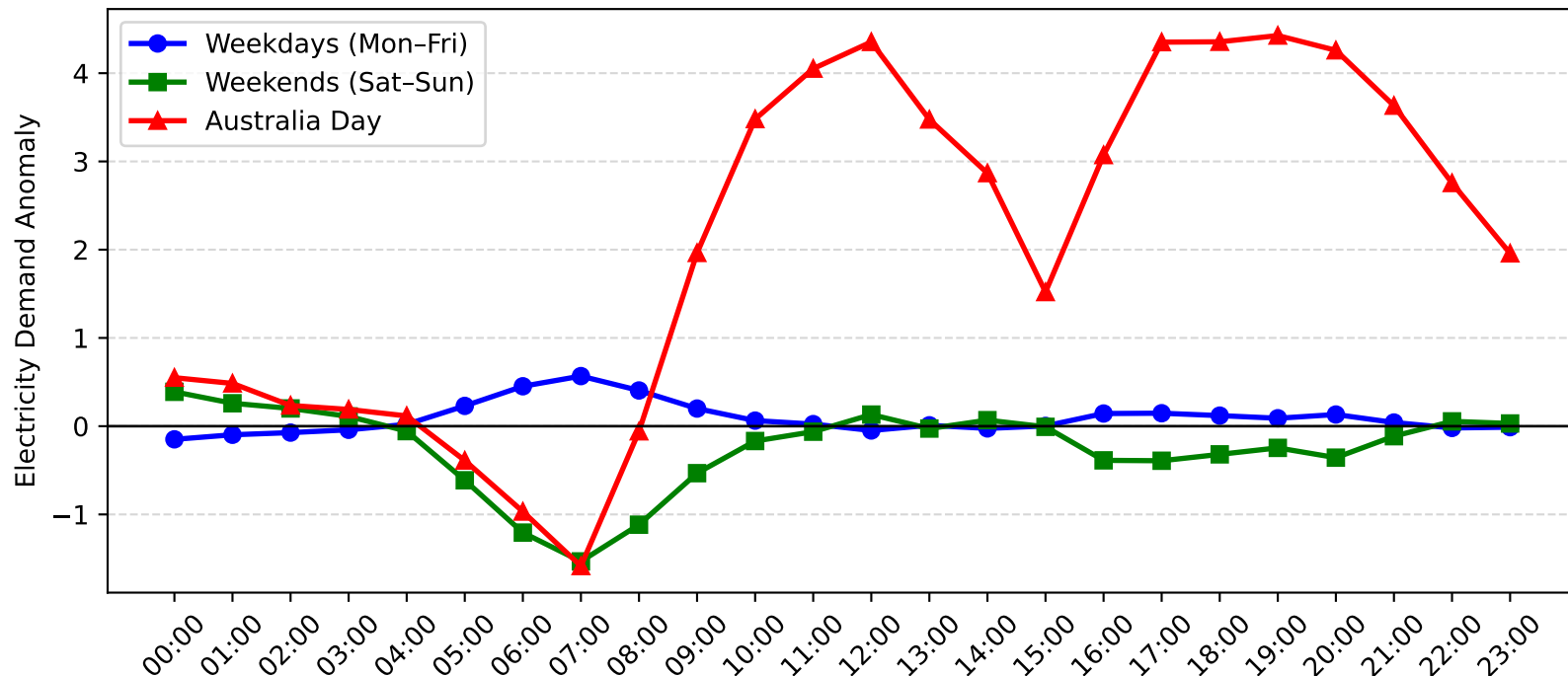
Charmhaven Demand Anomaly: Australia Day vs Weekday/Weekend (2011-2012)
