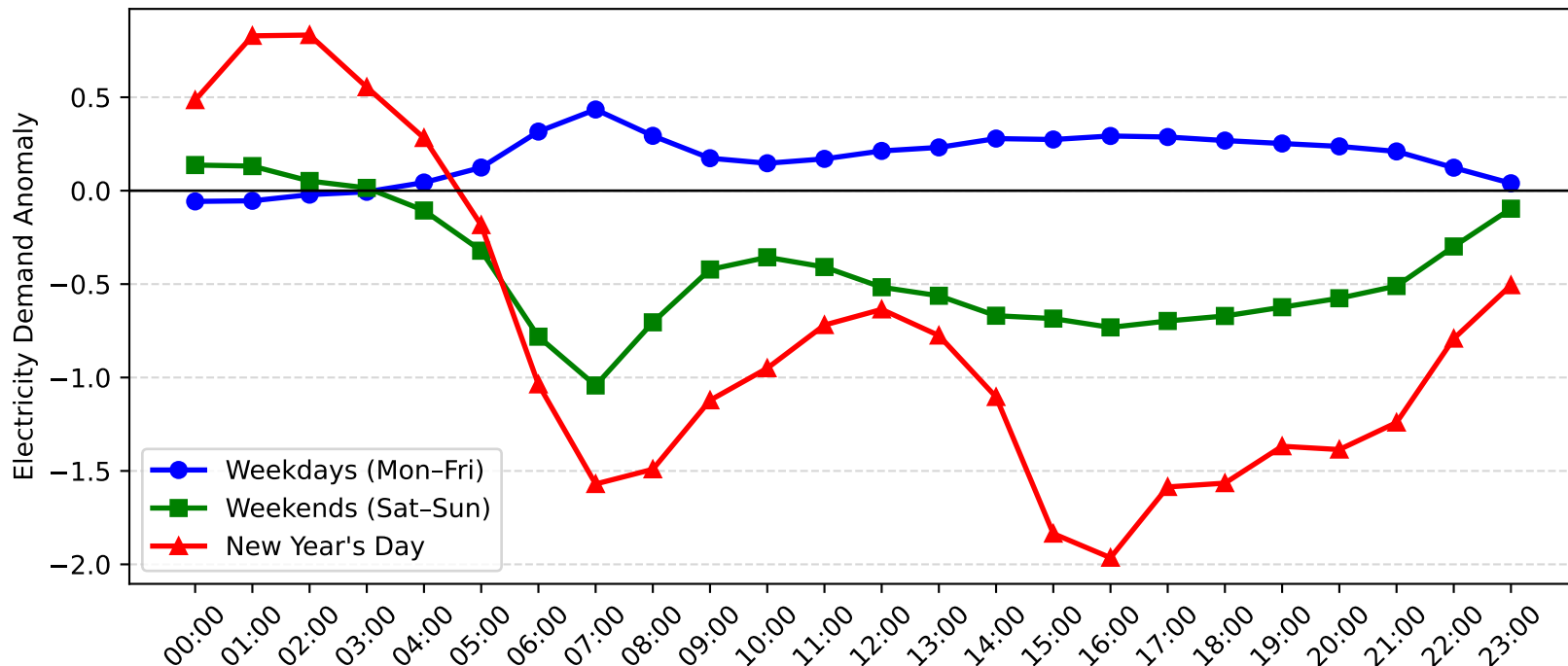
Blakehurst Demand Anomaly: New Year's Day vs Weekday/Weekend (2016-2017)
