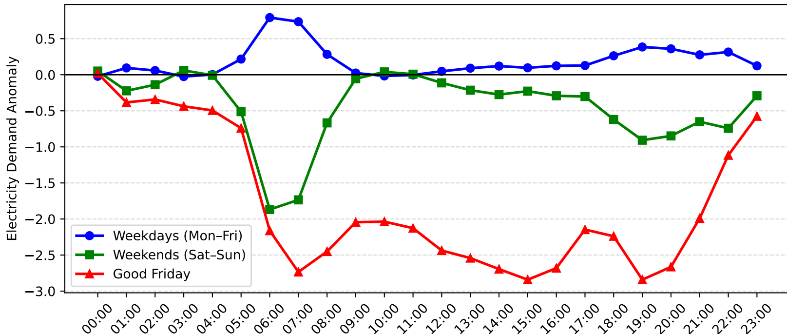
Balgowlah North Demand Anomaly: Good Friday vs Weekday/Weekend (2017-2018)
