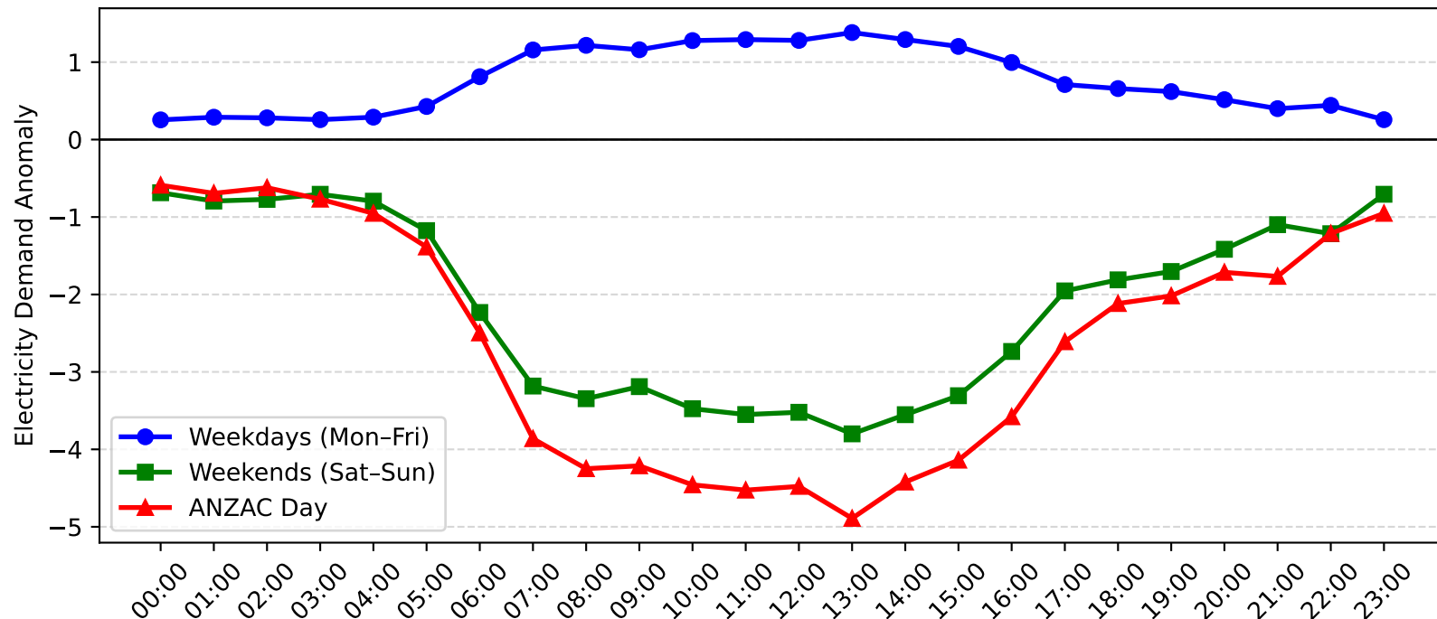
Mayfield West Demand Anomaly: ANZAC Day vs Weekday/Weekend (2012-2013)
