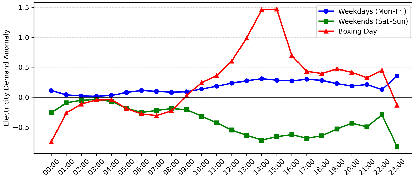
Telarah Demand Anomaly: Boxing Day vs Weekday/Weekend (2015-2016)
