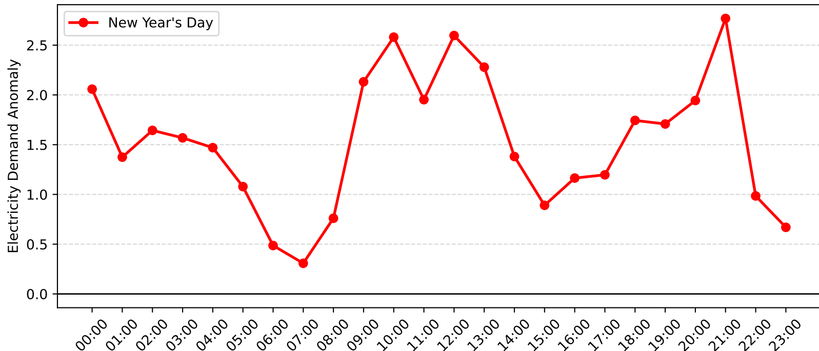
Nelson Bay Demand Anomaly: New Year's Day (2017-2018)
