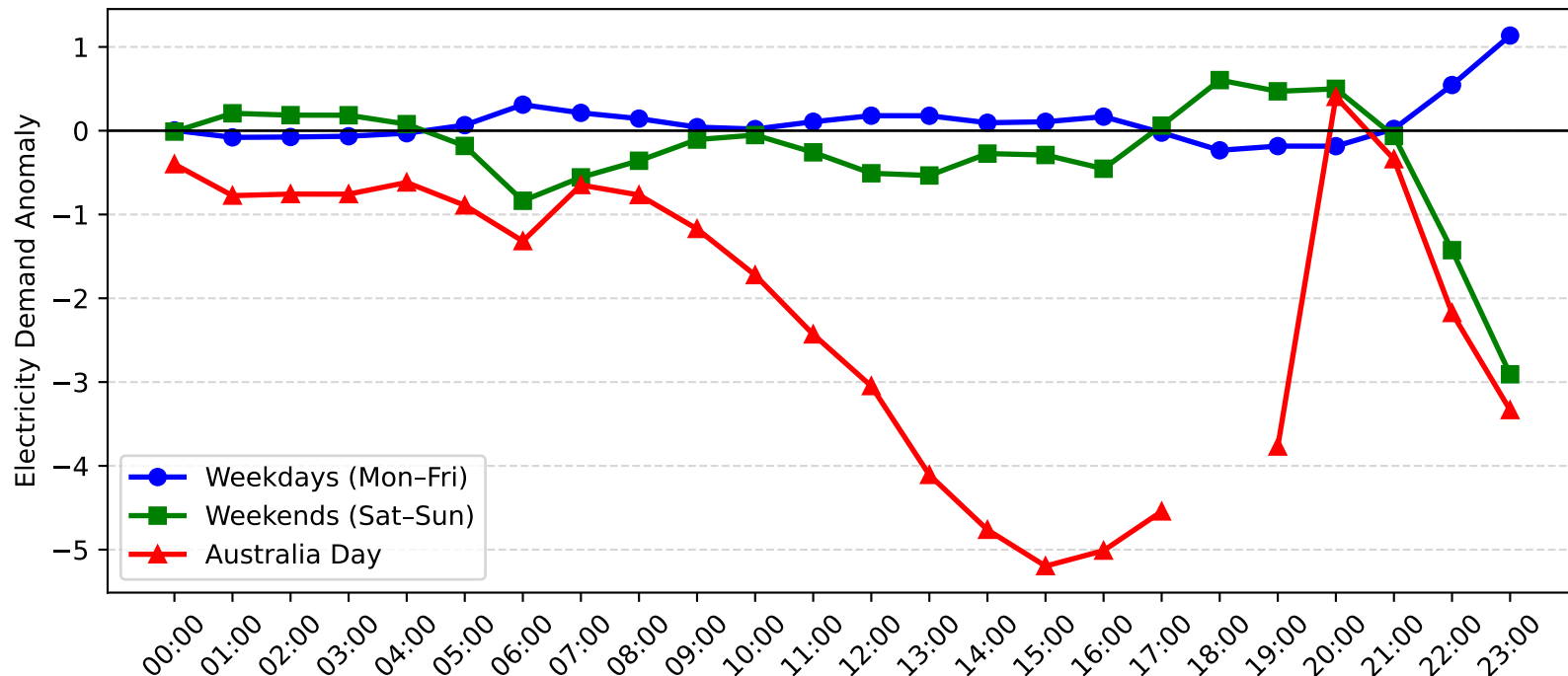
Muswellbrook Demand Anomaly: Australia Day vs Weekday/Weekend (2005-2006)
