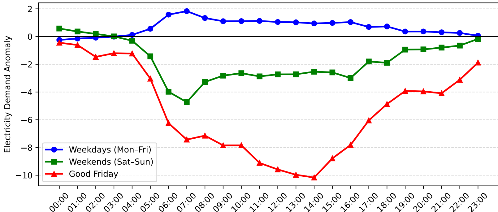
Meadowbank Demand Anomaly: Good Friday vs Weekday/Weekend (2005-2006)
