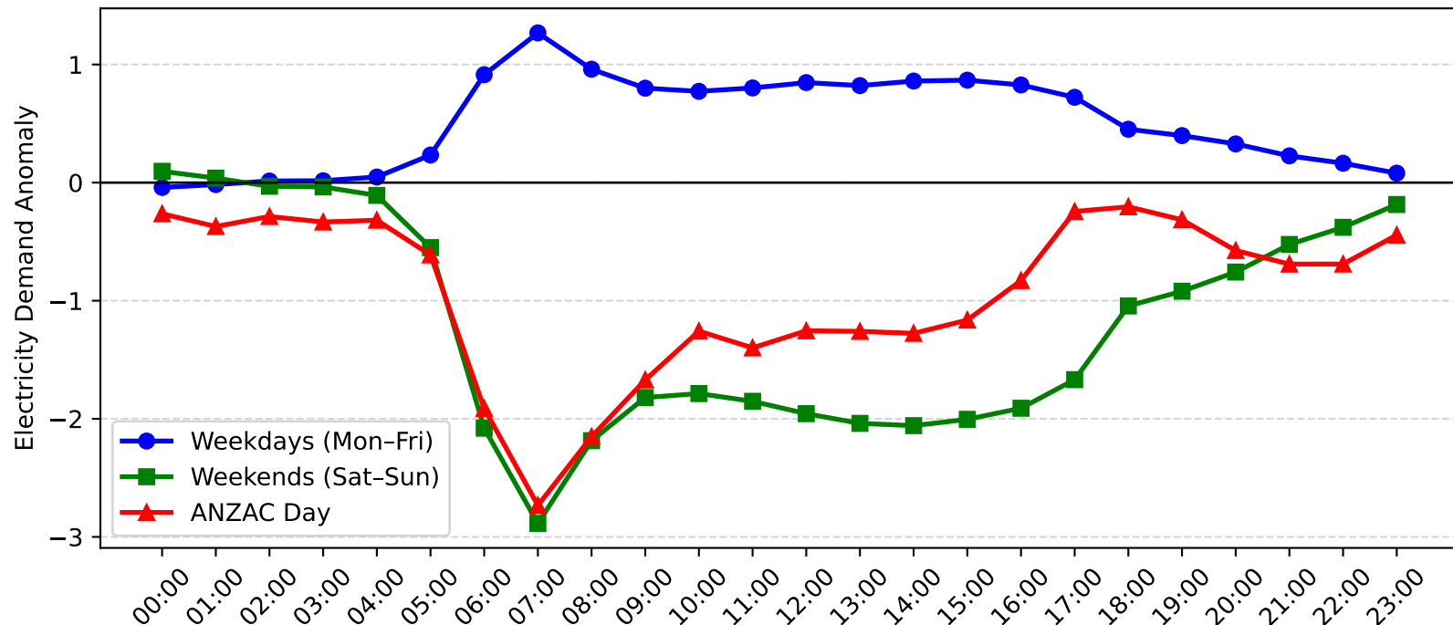
Pymble Demand Anomaly: ANZAC Day vs Weekday/Weekend (2016-2017)
