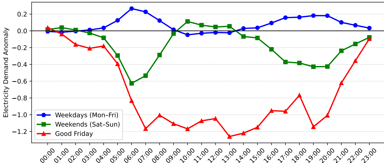
Narrabeen Demand Anomaly: Good Friday vs Weekday/Weekend (2017-2018)
