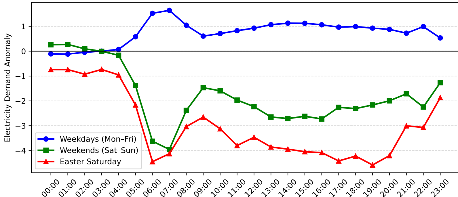
Dee Why West Demand Anomaly: Easter Saturday vs Weekday/Weekend (2006-2007)
