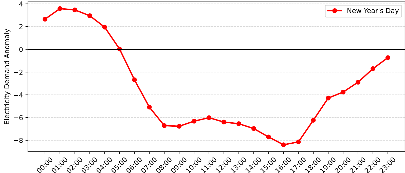
Kogarah Demand Anomaly: New Year's Day (2017-2018)
