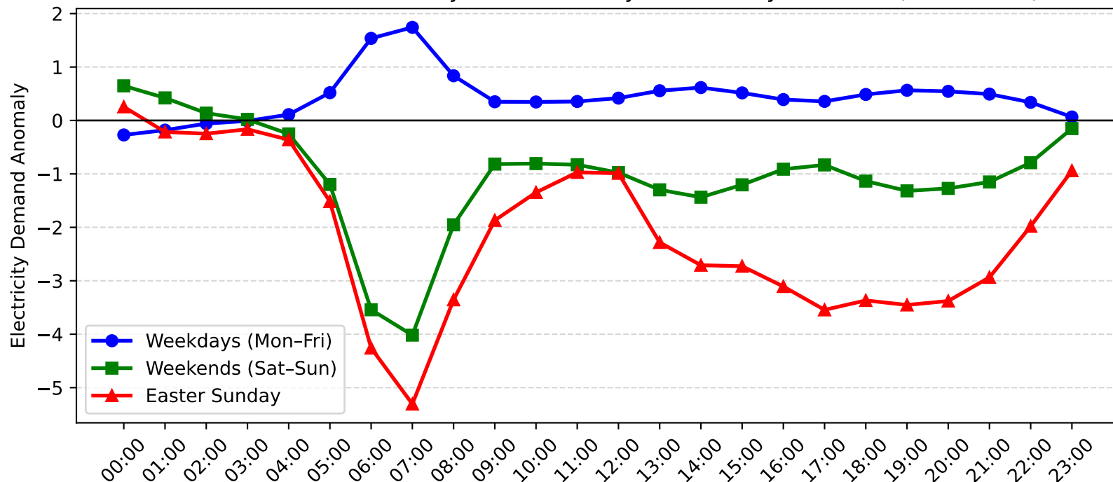
Mortdale Demand Anomaly: Easter Sunday vs Weekday/Weekend (2011-2012)
