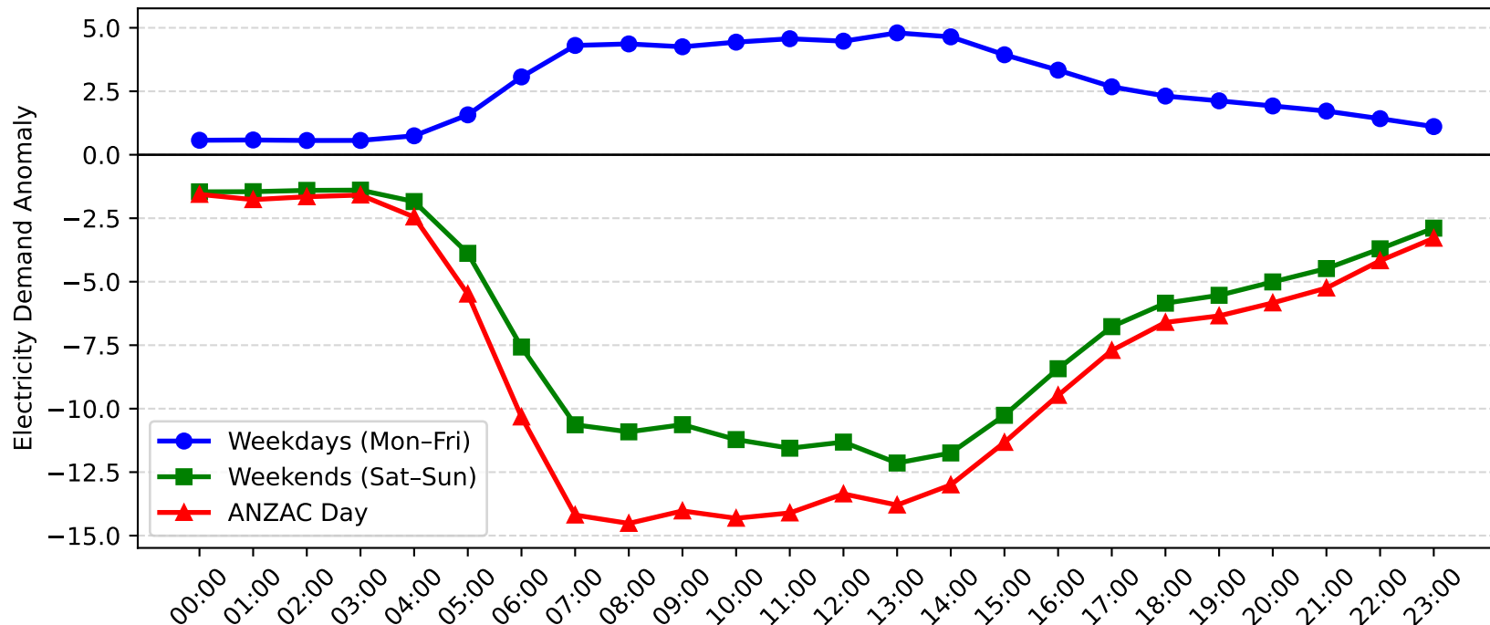
Milperra Demand Anomaly: ANZAC Day vs Weekday/Weekend (2011-2012)
