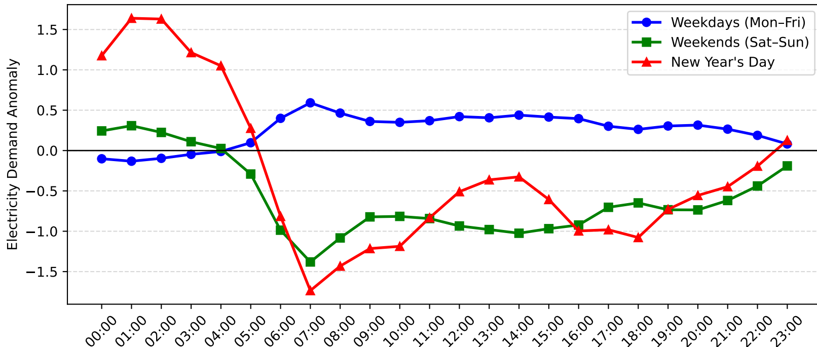
Arnccliffe Demand Anomaly: New Year's Day vs Weekday/Weekend (2017-2018)
