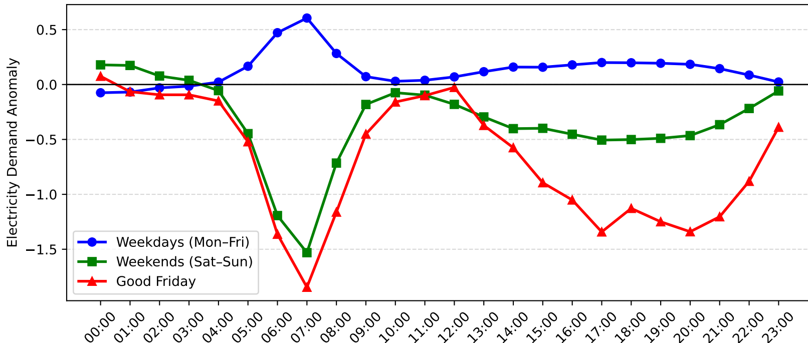
Blakehurst Demand Anomaly: Good Friday vs Weekday/Weekend (2014-2015)
