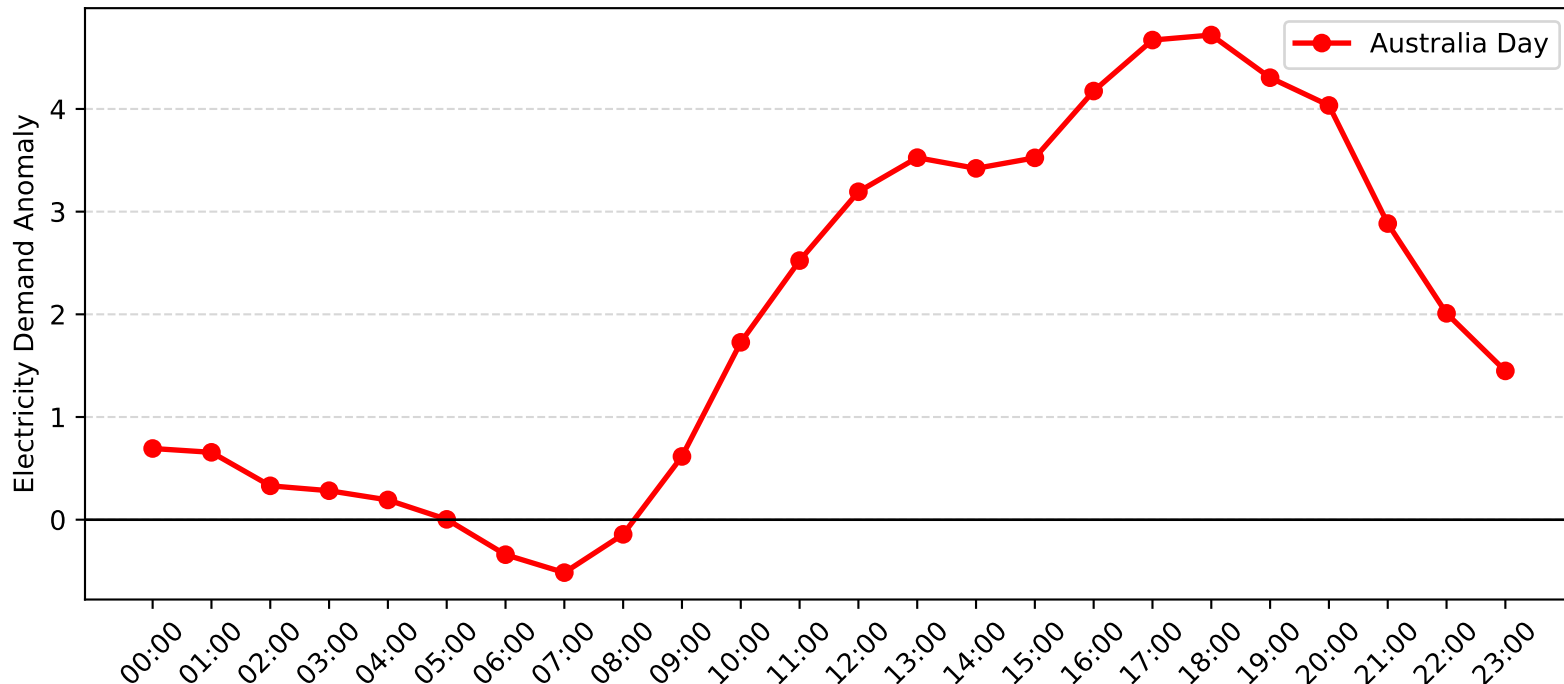
Morisset Demand Anomaly: Australia Day (2010-2011)
