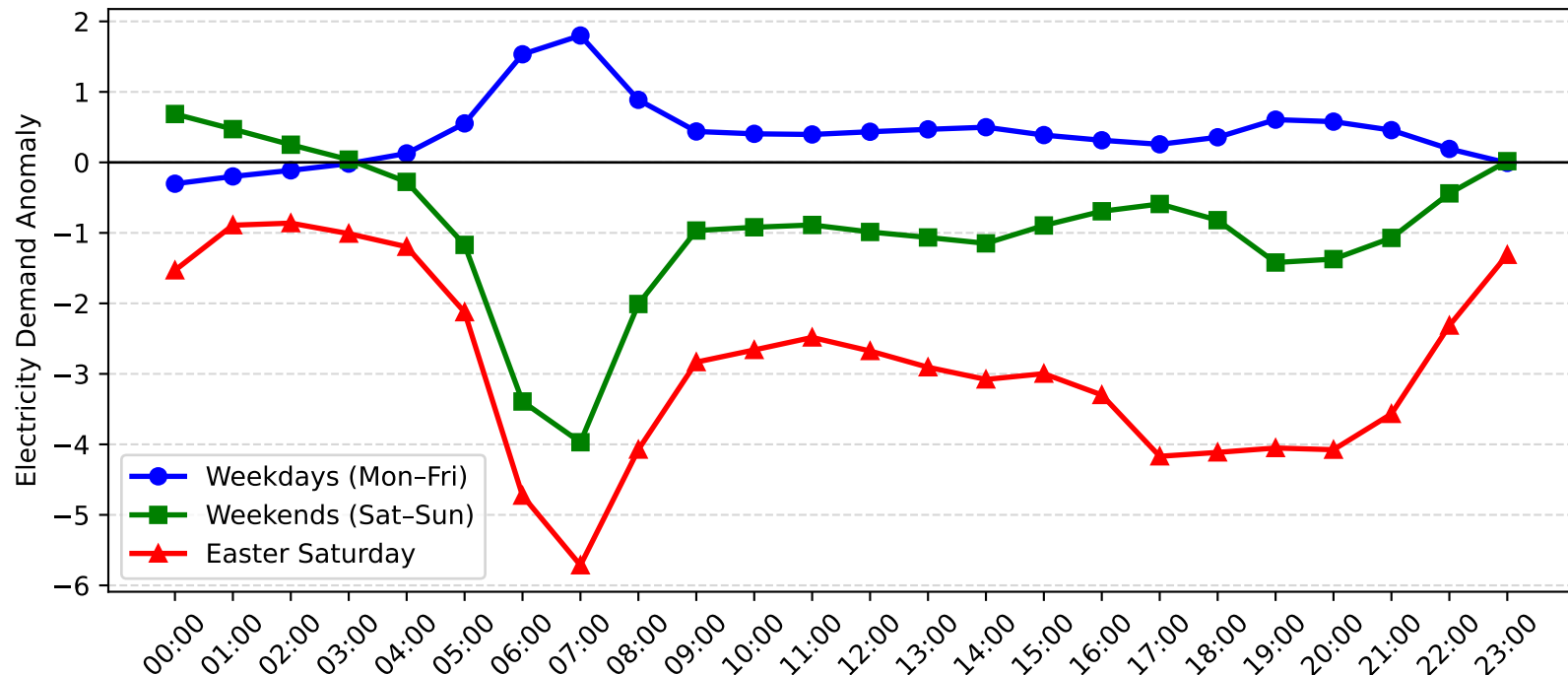
Mortdale Demand Anomaly: Easter Saturday vs Weekday/Weekend (2010-2011)
