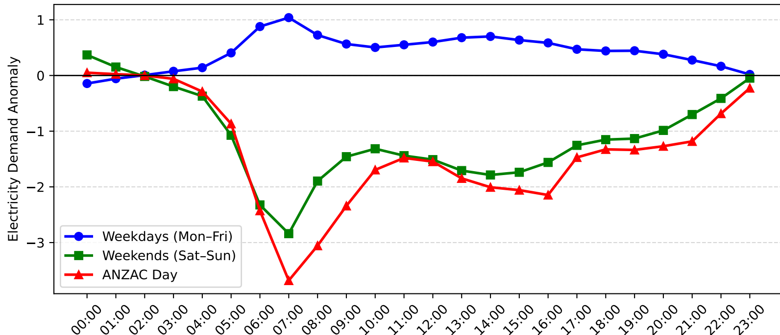
Rockdale Demand Anomaly: ANZAC Day vs Weekday/Weekend (2007-2008)
