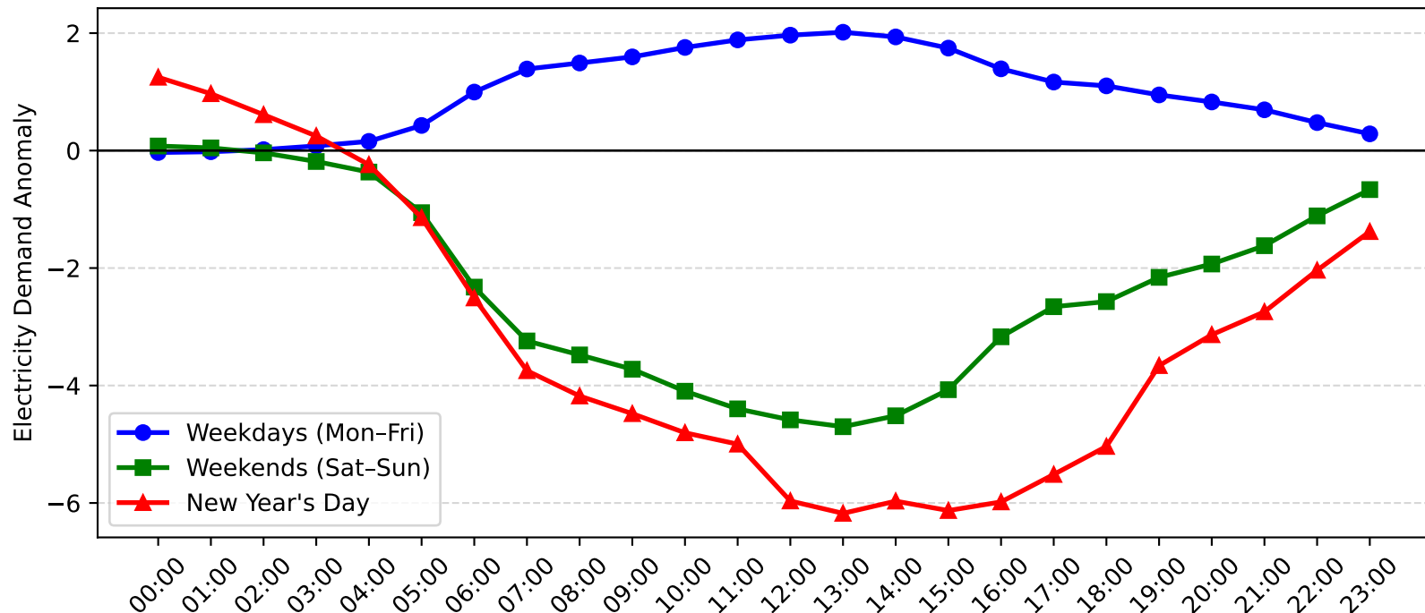
Wyong Demand Anomaly: New Year's Day vs Weekday/Weekend (2017-2018)
