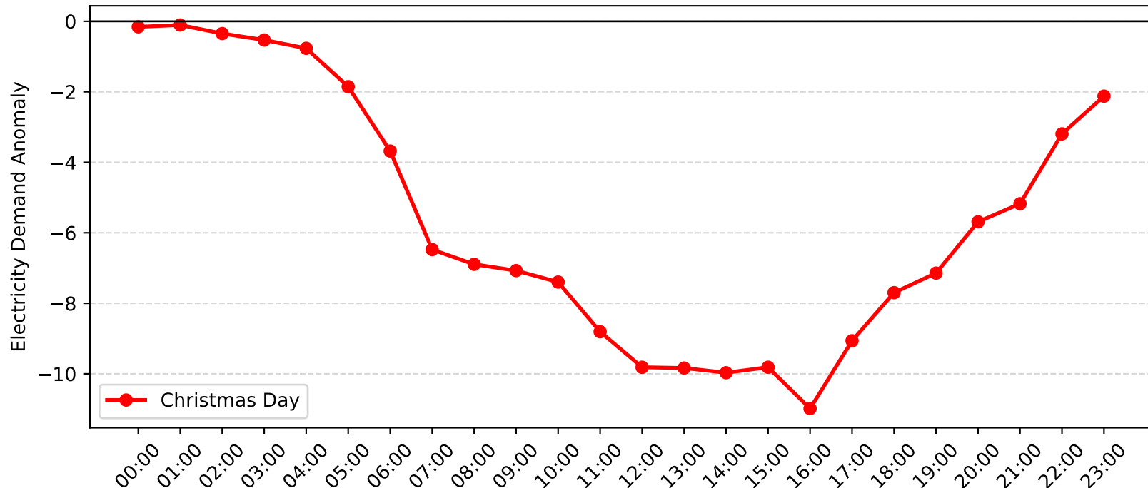
Chatswood Demand Anomaly: Christmas Day (2007-2008)
