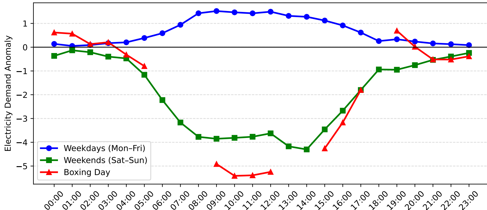
Bankstown Demand Anomaly: Boxing Day vs Weekday/Weekend (2009-2010)
