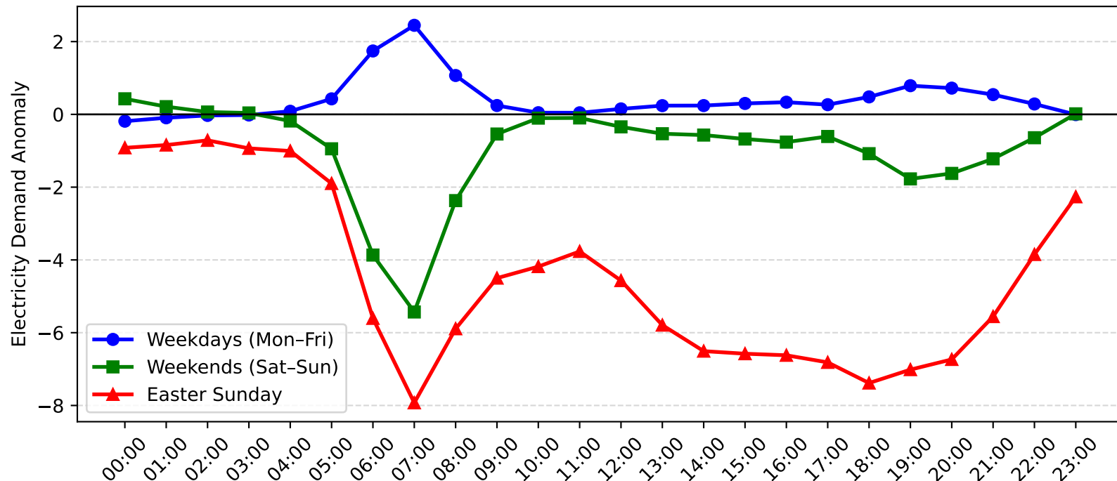
Mosman Demand Anomaly: Easter Sunday vs Weekday/Weekend (2016-2017)
