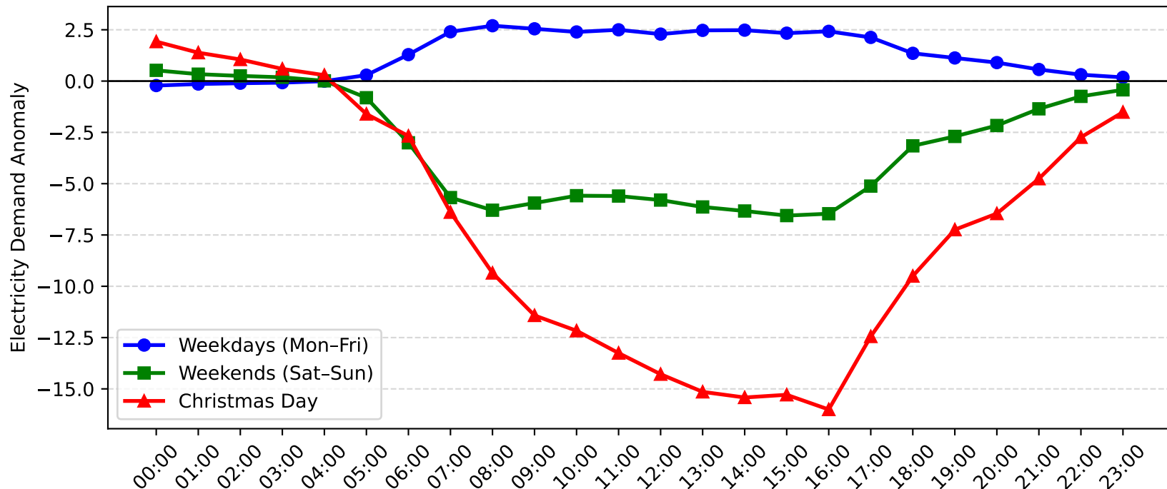
Castle Cove Demand Anomaly: Christmas Day vs Weekday/Weekend (2011-2012)
