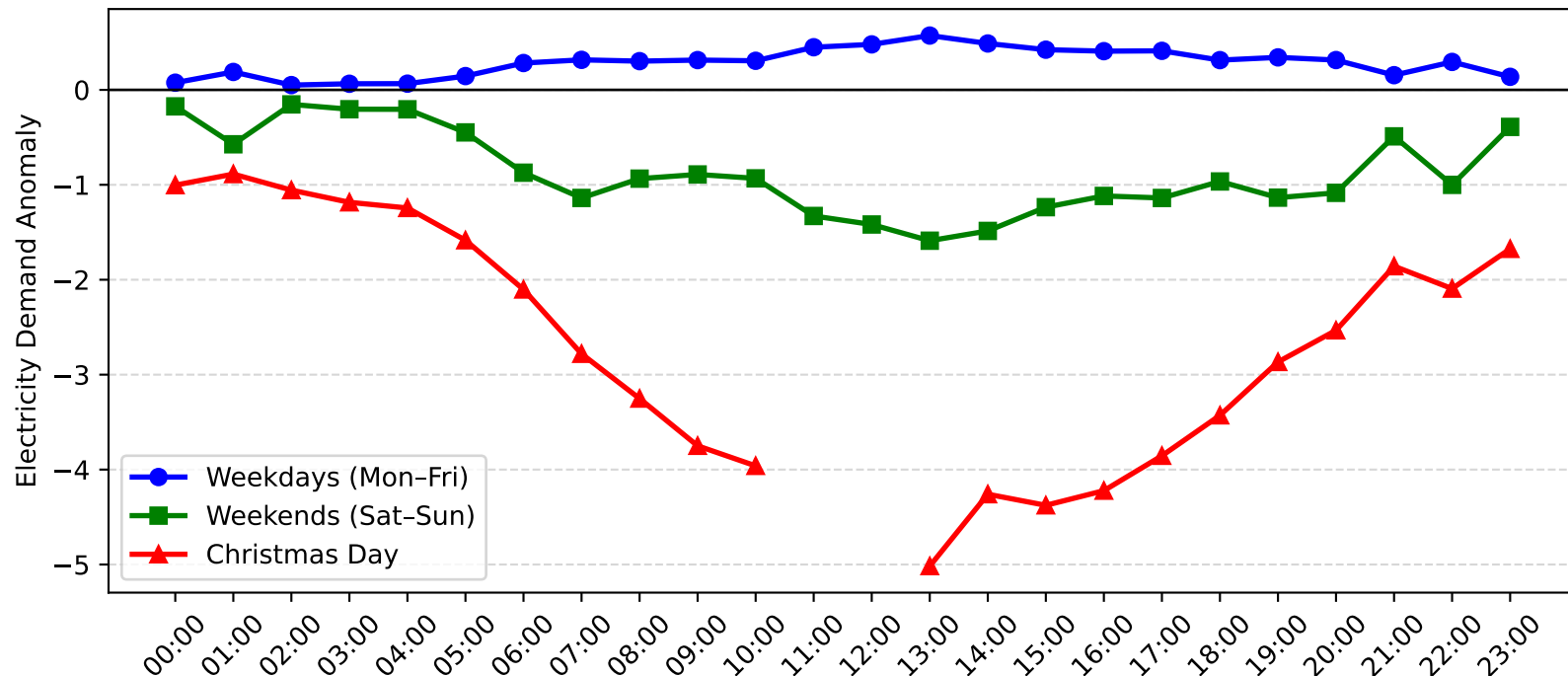
Gateshead Demand Anomaly: Christmas Day vs Weekday/Weekend (2008-2009)
