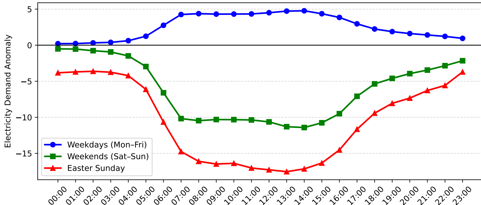
St. Peters Demand Anomaly: Easter Sunday vs Weekday/Weekend (2007-2008)
