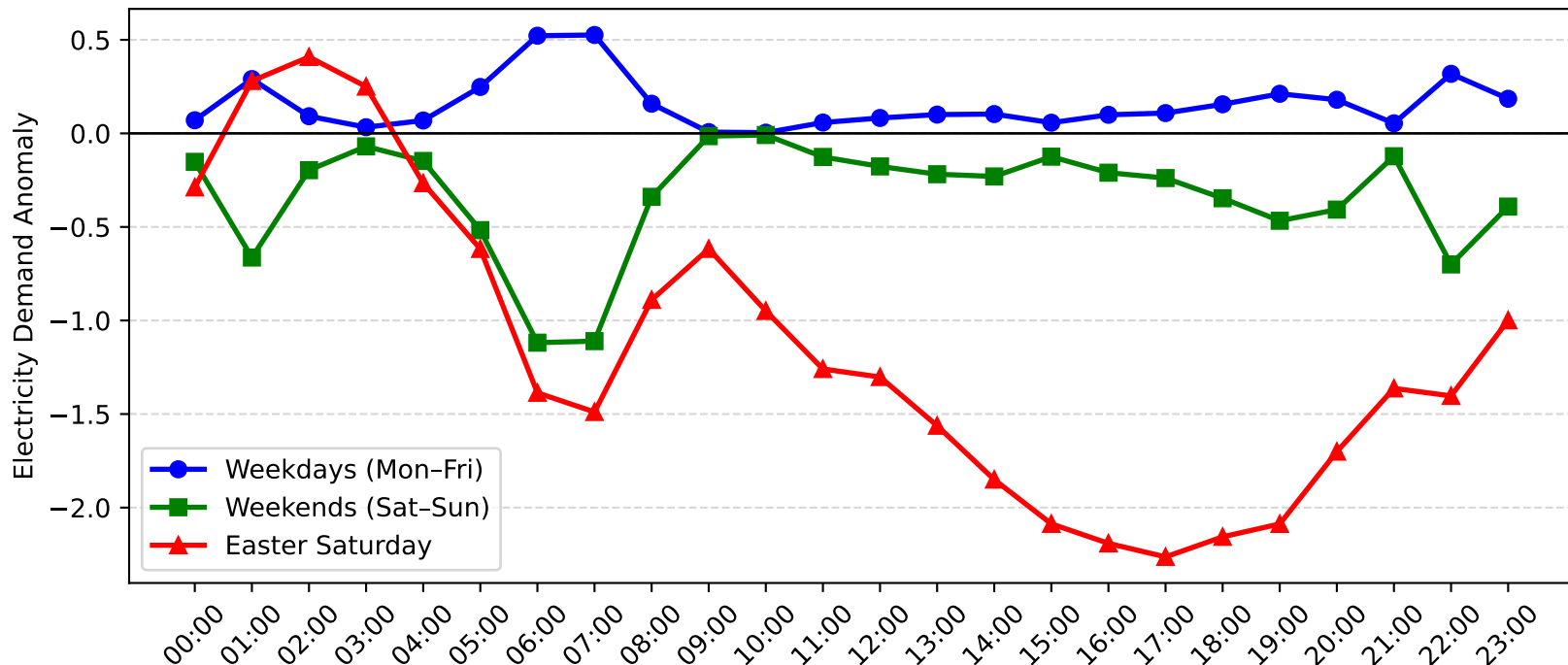
Maryland Demand Anomaly: Easter Saturday vs Weekday/Weekend (2009-2010)
