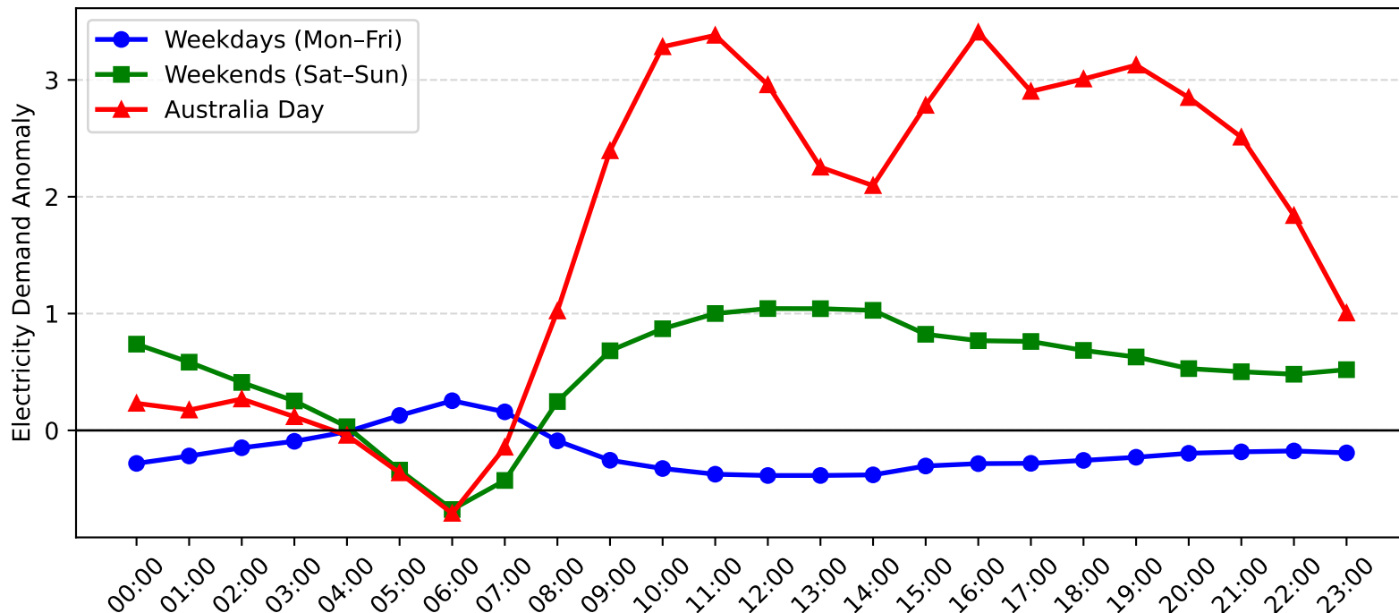
Umina Demand Anomaly: Australia Day vs Weekday/Weekend (2011-2012)
