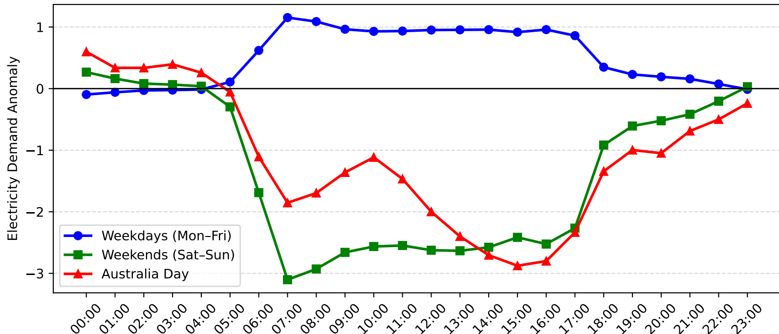
Pymble Demand Anomaly: Australia Day vs Weekday/Weekend (2015-2016)
