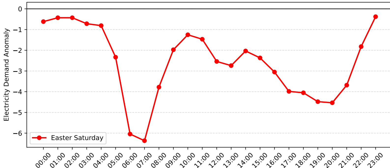
Pennant Hills Demand Anomaly: Easter Saturday (2014-2015)
