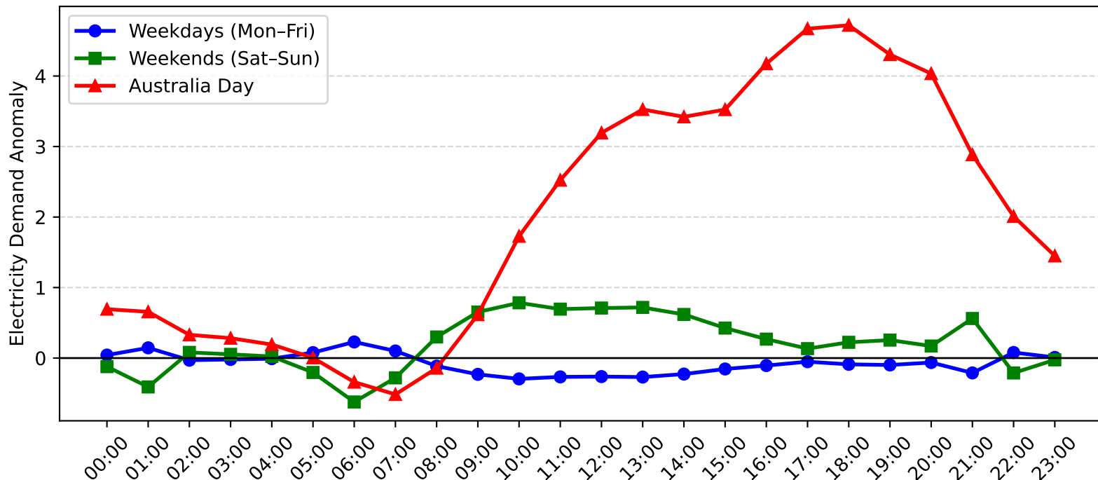
Morisset Demand Anomaly: Australia Day vs Weekday/Weekend (2010-2011)
