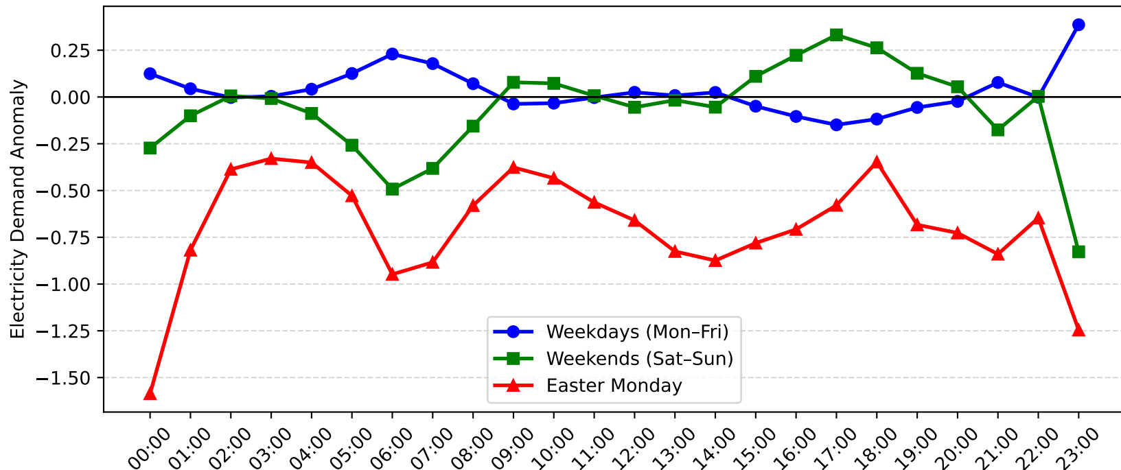
Telarah Demand Anomaly: Easter Monday vs Weekday/Weekend (2010-2011)
