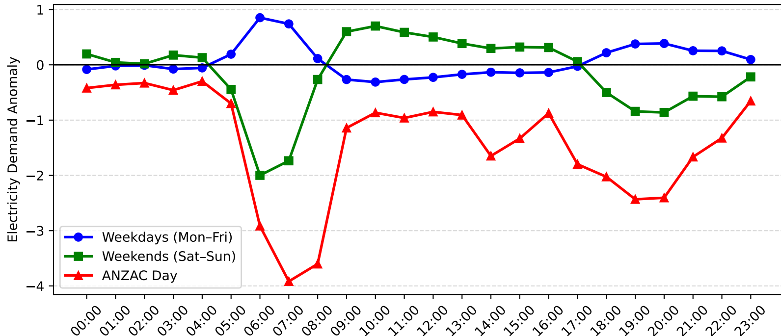
Balgowlah North Demand Anomaly: ANZAC Day vs Weekday/Weekend (2015-2016)
