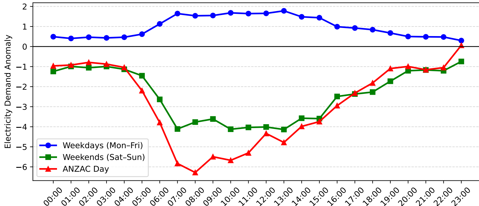
Milperra Demand Anomaly: ANZAC Day vs Weekday/Weekend (2004-2005)
