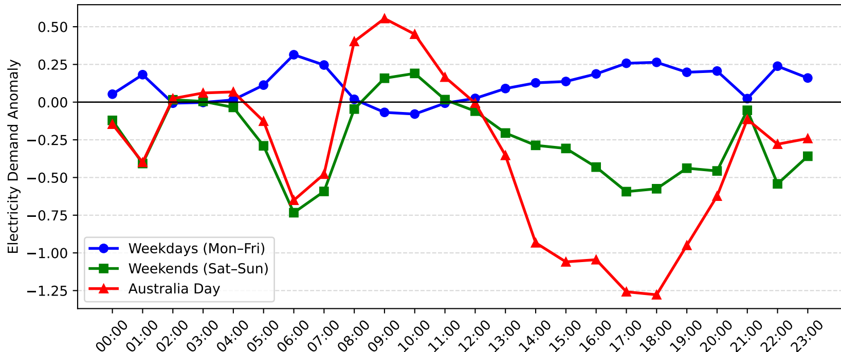
Morisset Demand Anomaly: Australia Day vs Weekday/Weekend (2013-2014)
