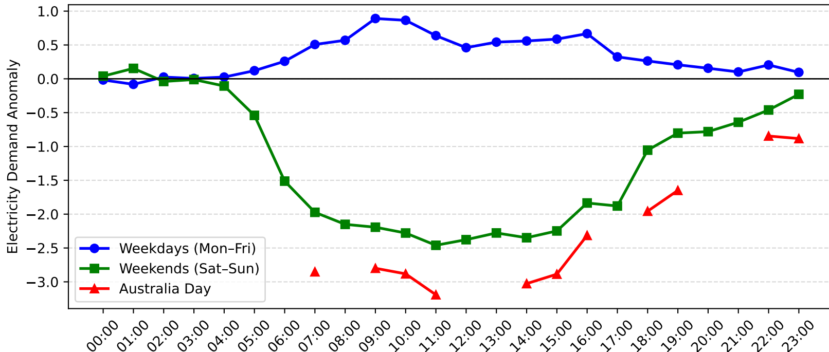
Potts Hill Demand Anomaly: Australia Day vs Weekday/Weekend (2013-2014)
