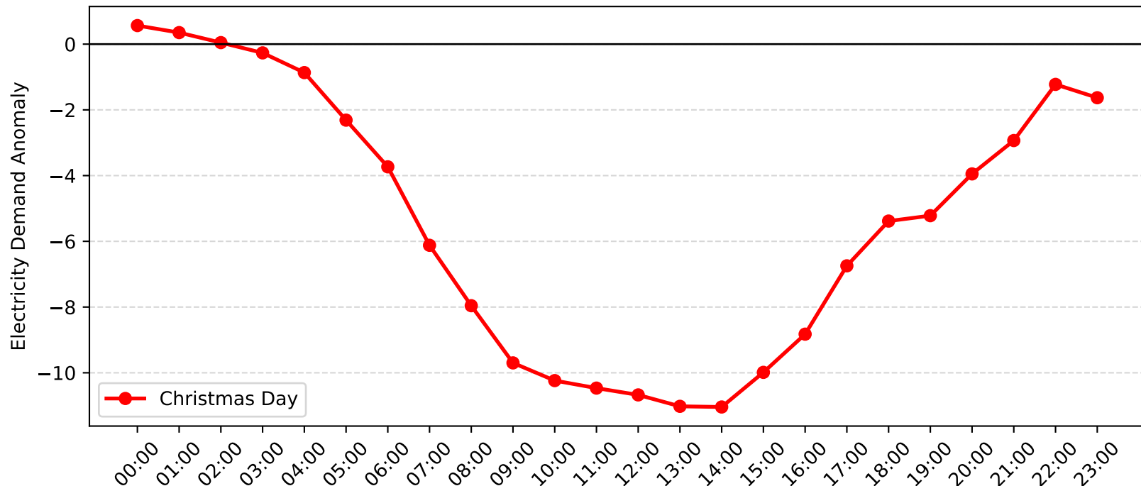
West Gosford Demand Anomaly: Christmas Day (2004-2005)
