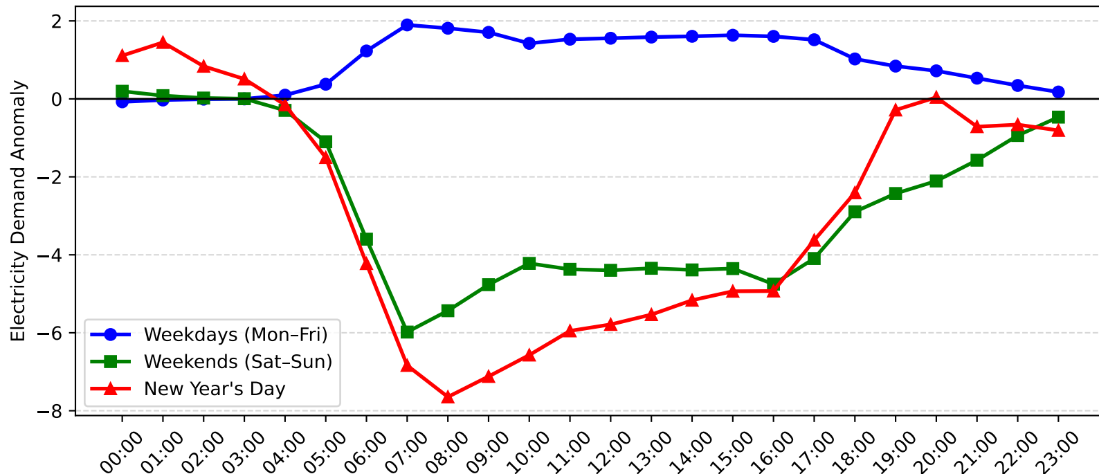
Chatswood Demand Anomaly: New Year's Day vs Weekday/Weekend (2008-2009)
