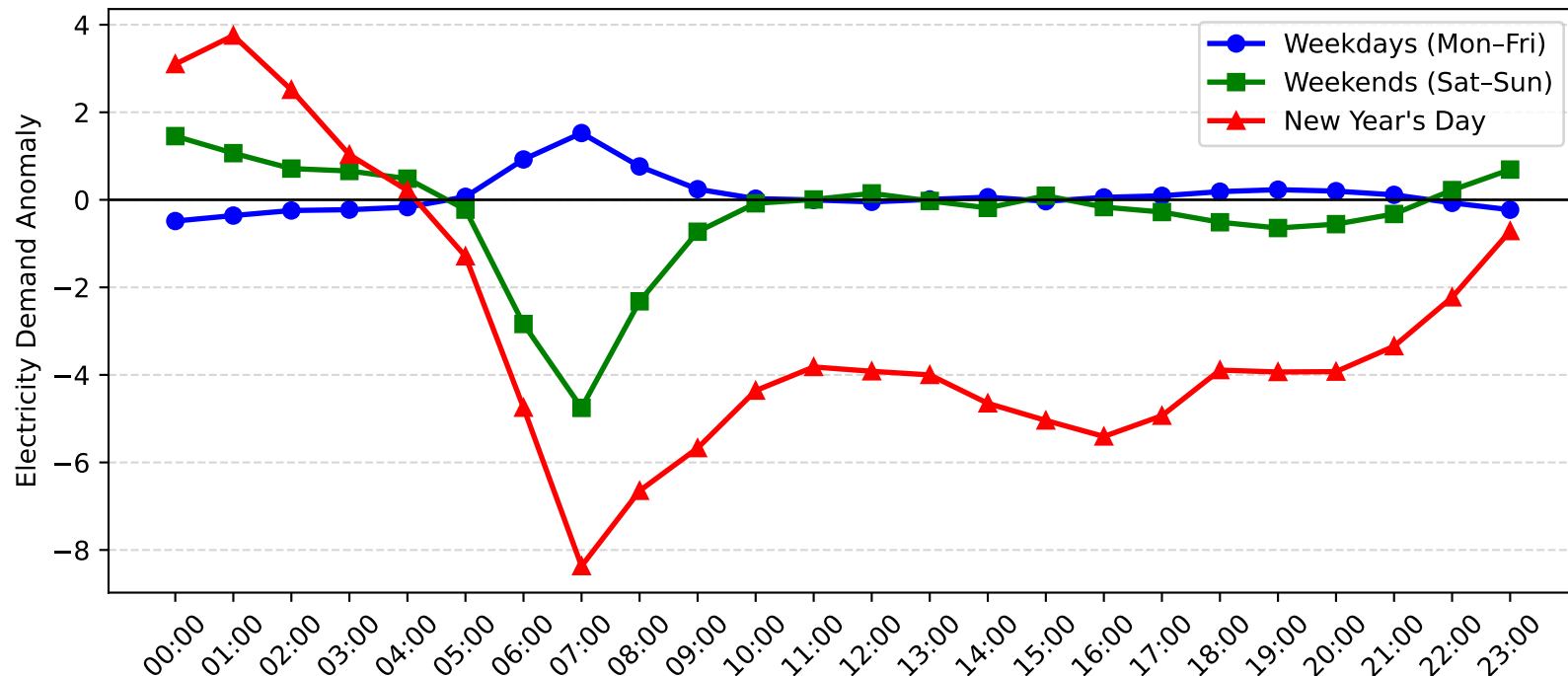
Mosman Demand Anomaly: New Year's Day vs Weekday/Weekend (2014-2015)
