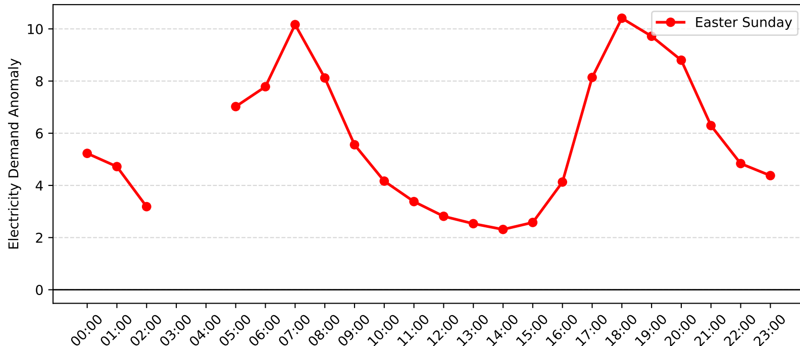
Sefton Demand Anomaly: Easter Sunday (2004-2005)
