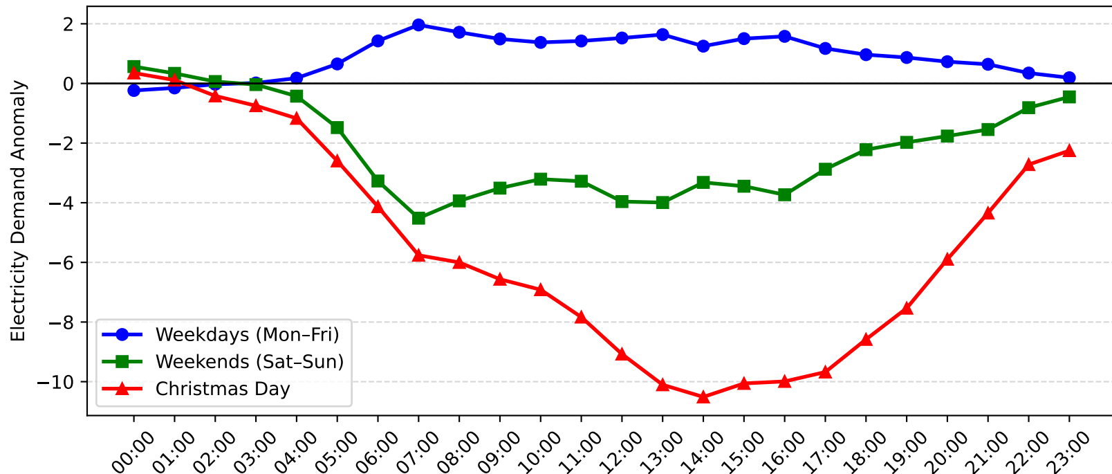
Campsie Demand Anomaly: Christmas Day vs Weekday/Weekend (2005-2006)
