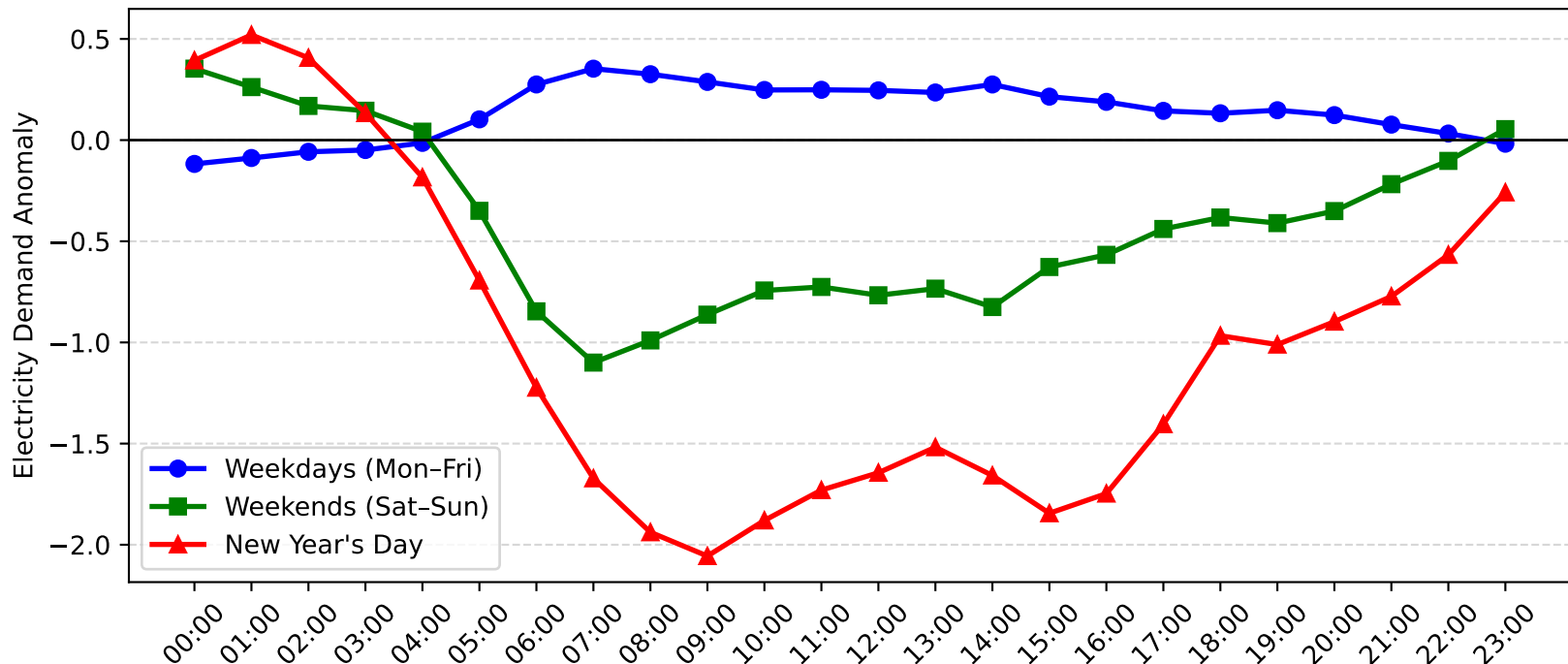
Rockdale Demand Anomaly: New Year's Day vs Weekday/Weekend (2014-2015)
