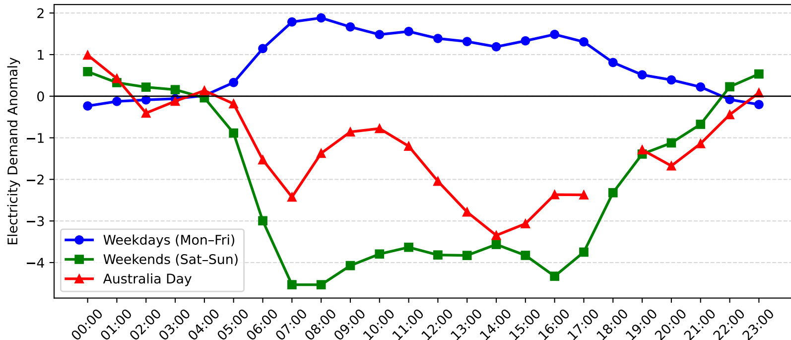
Pymble Demand Anomaly: Australia Day vs Weekday/Weekend (2005-2006)
