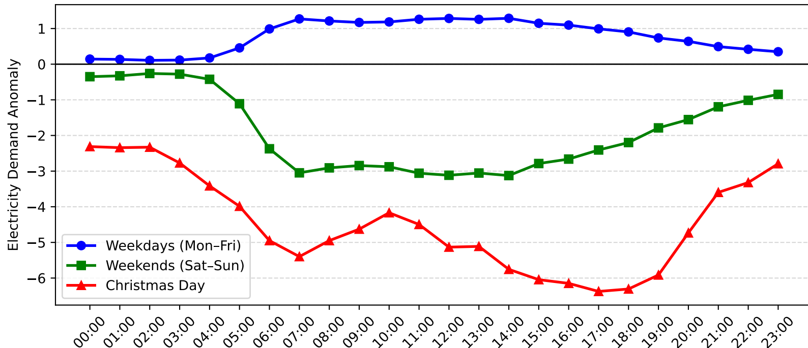
Matravlle Demand Anomaly: Christmas Day vs Weekday/Weekend (2015-2016)
