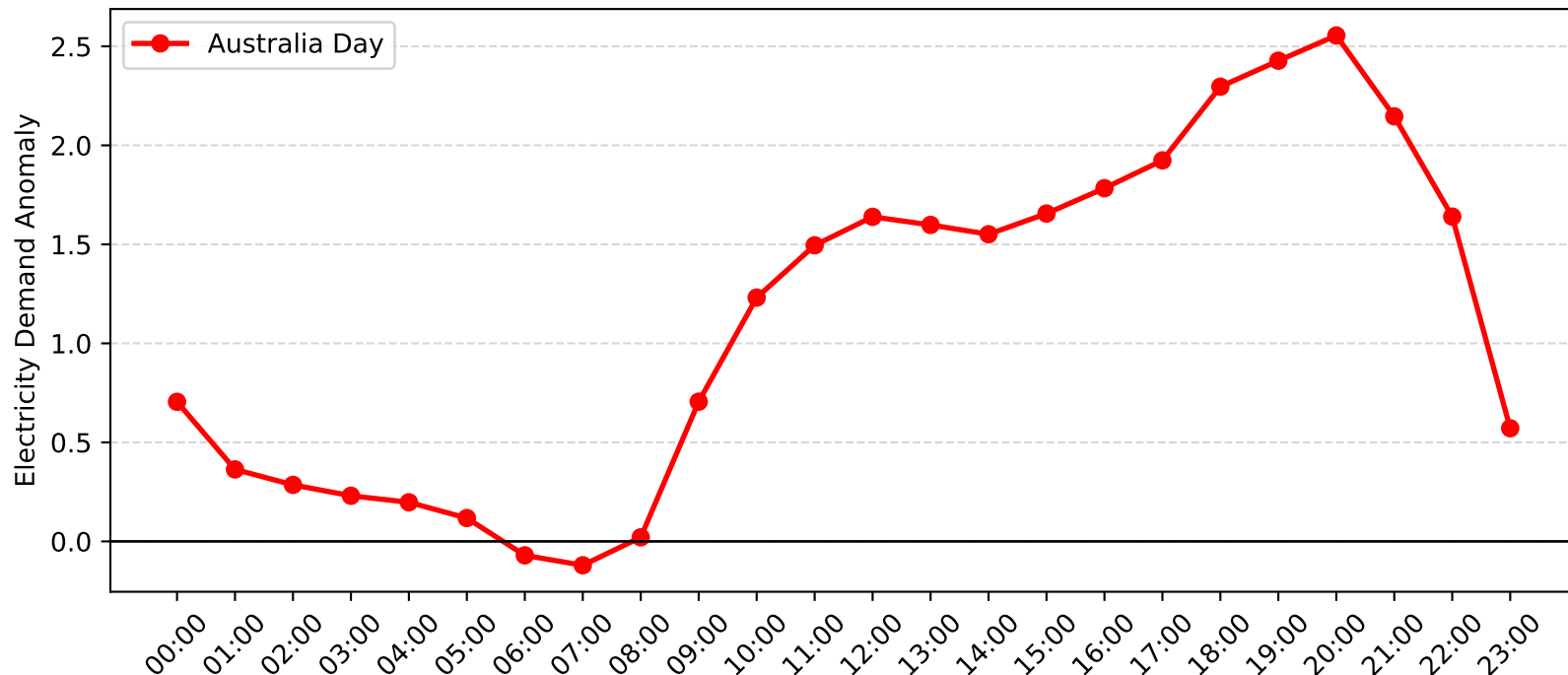
Telarah Demand Anomaly: Australia Day (2011-2012)
