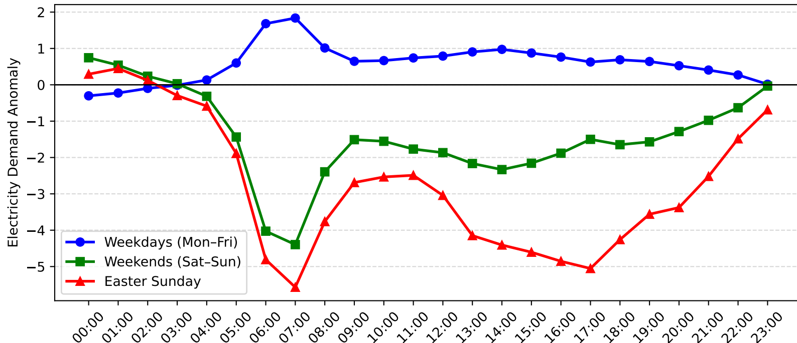
Mortdale Demand Anomaly: Easter Sunday vs Weekday/Weekend (2007-2008)
