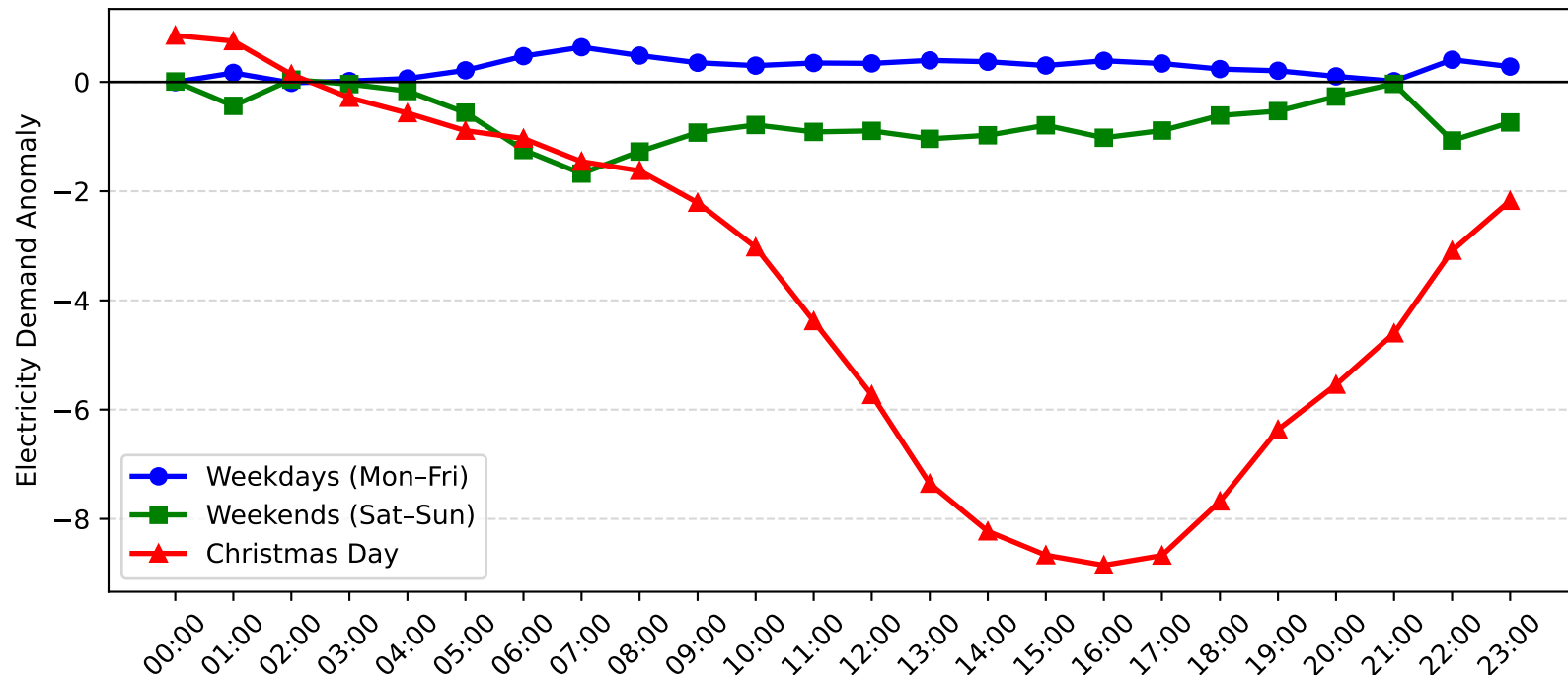
Jesmond Demand Anomaly: Christmas Day vs Weekday/Weekend (2012-2013)
