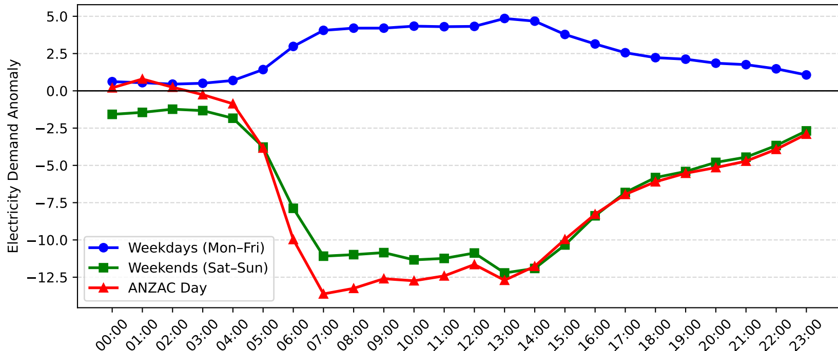
Milperra Demand Anomaly: ANZAC Day vs Weekday/Weekend (2007-2008)
