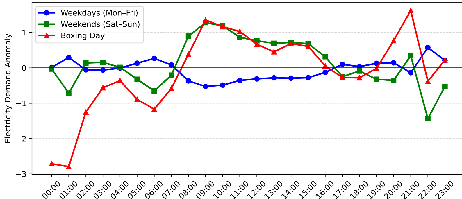
Nelson Bay Demand Anomaly: Boxing Day vs Weekday/Weekend (2011-2012)
