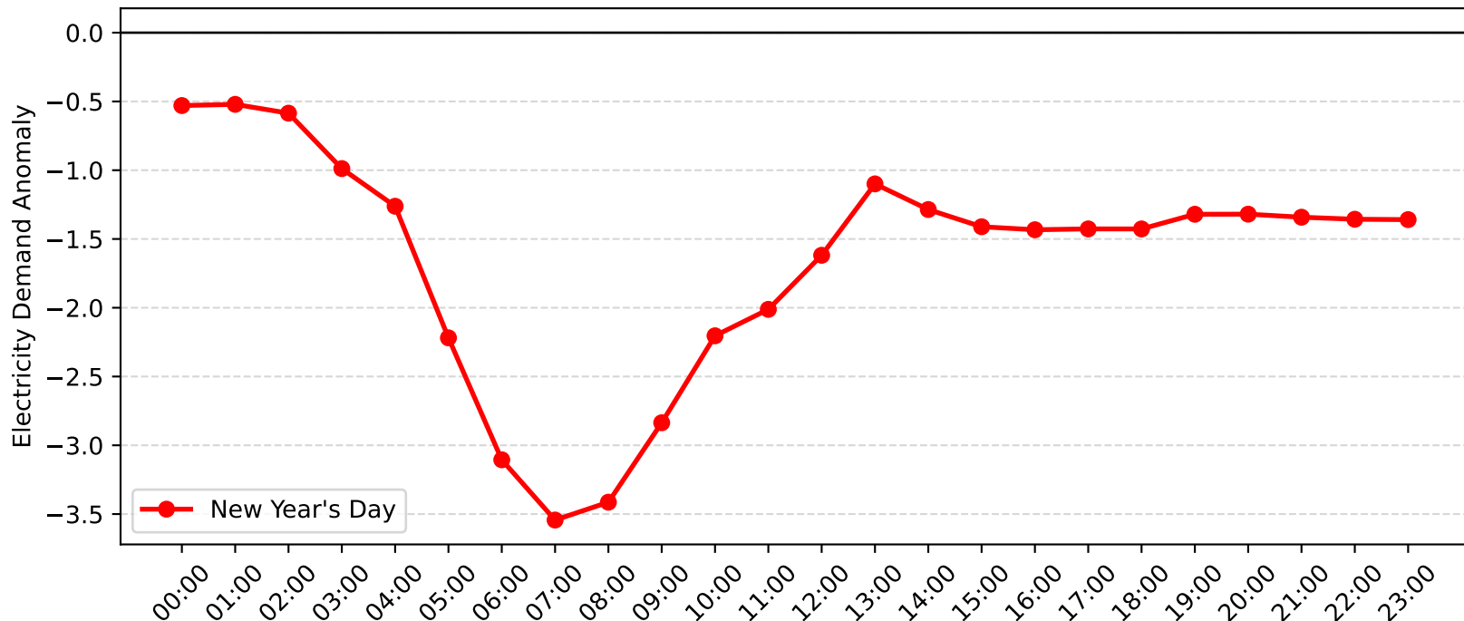
Lisarow Demand Anomaly: New Year's Day (2013-2014)
