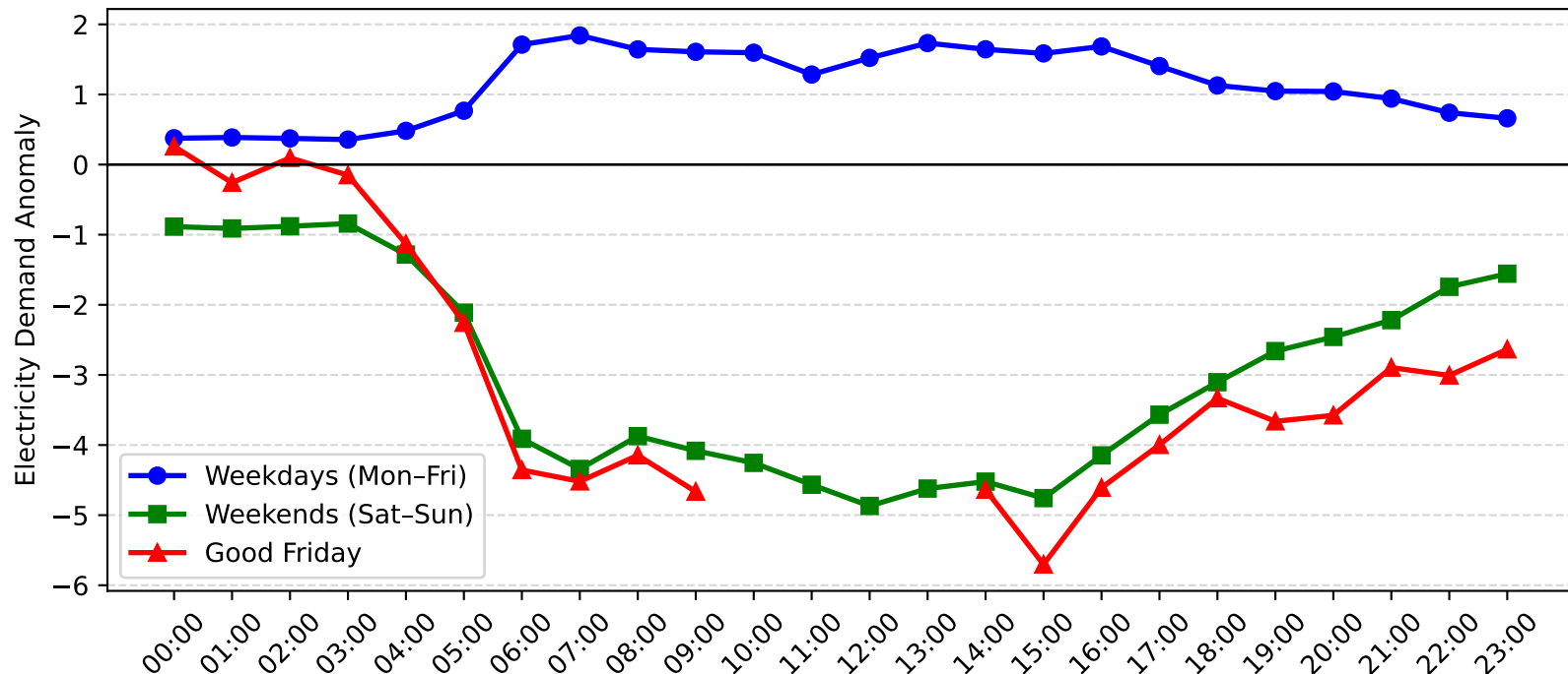
Potts Hill Demand Anomaly: Good Friday vs Weekday/Weekend (2017-2018)
