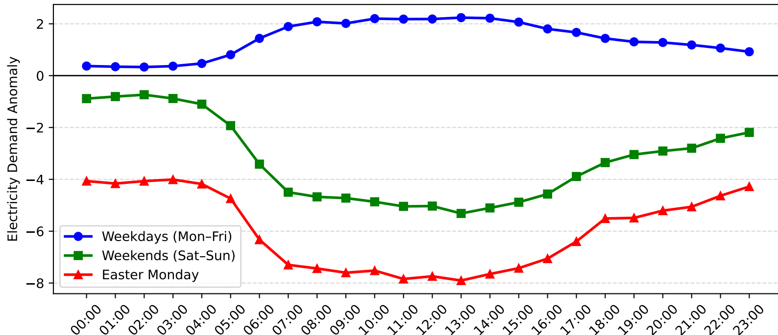
Leightonfield Demand Anomaly: Easter Monday vs Weekday/Weekend (2006-2007)
