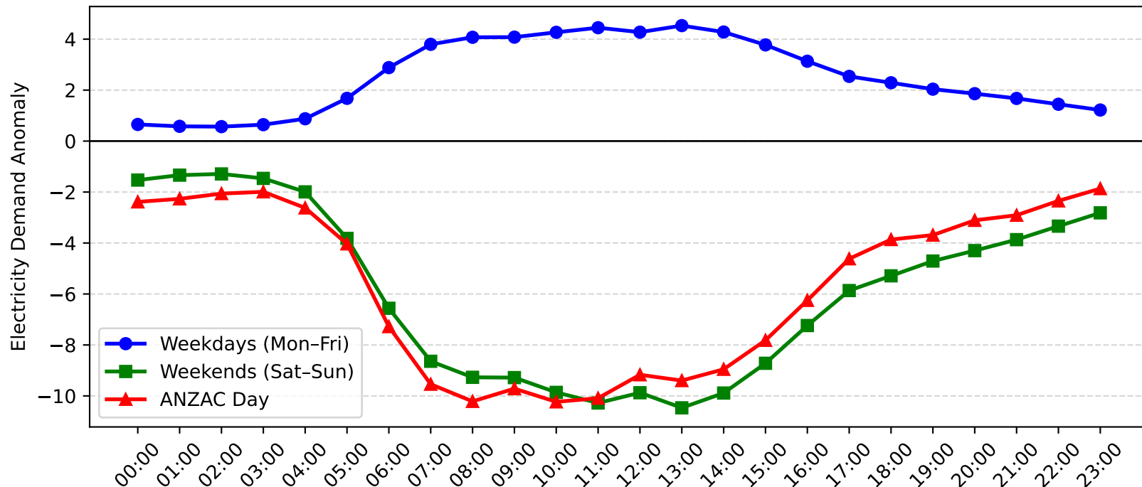
Milperra Demand Anomaly: ANZAC Day vs Weekday/Weekend (2016-2017)
