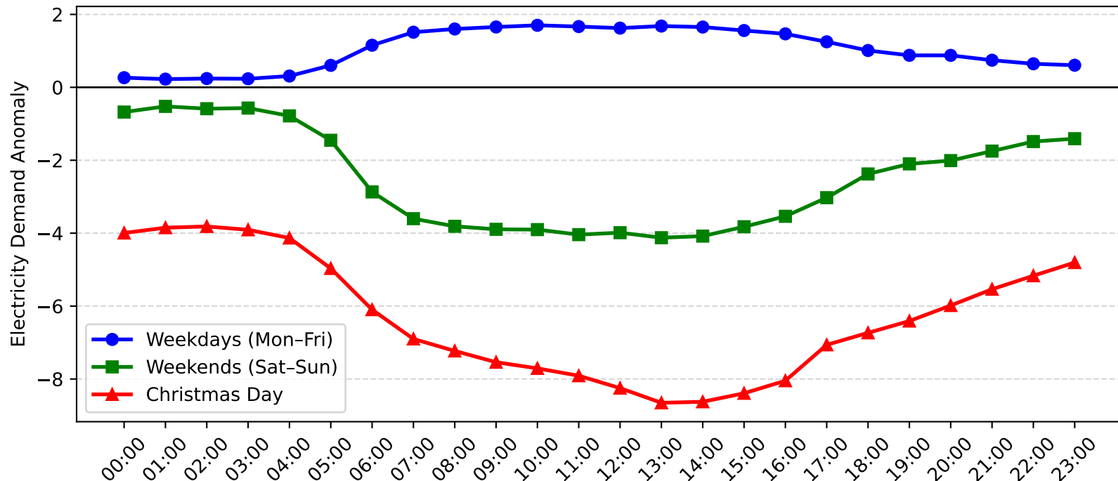
Leightonfield Demand Anomaly: Christmas Day vs Weekday/Weekend (2006-2007)
