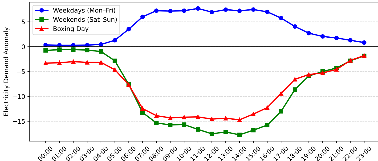
Gore Hill Demand Anomaly: Boxing Day vs Weekday/Weekend (2004-2005)
