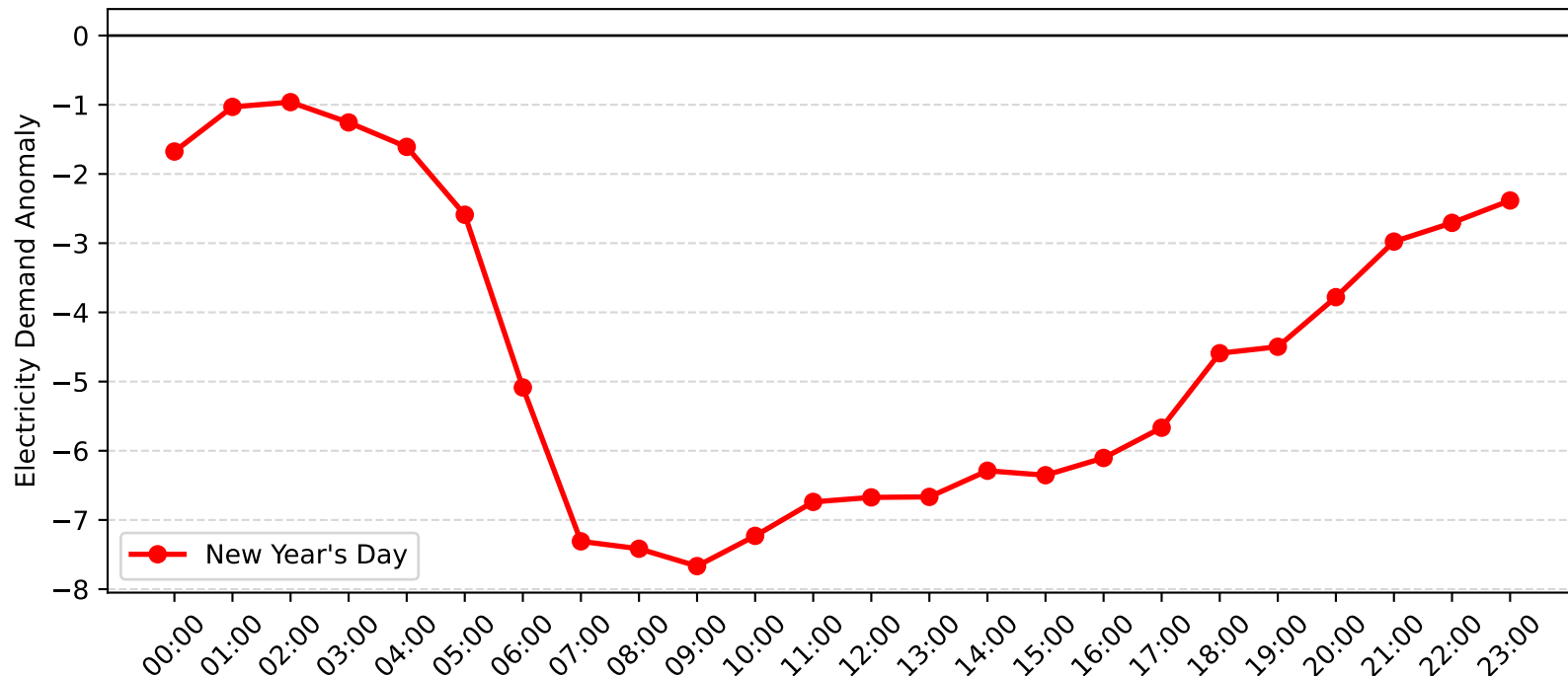
Maroubra Demand Anomaly: New Year's Day (2012-2013)
