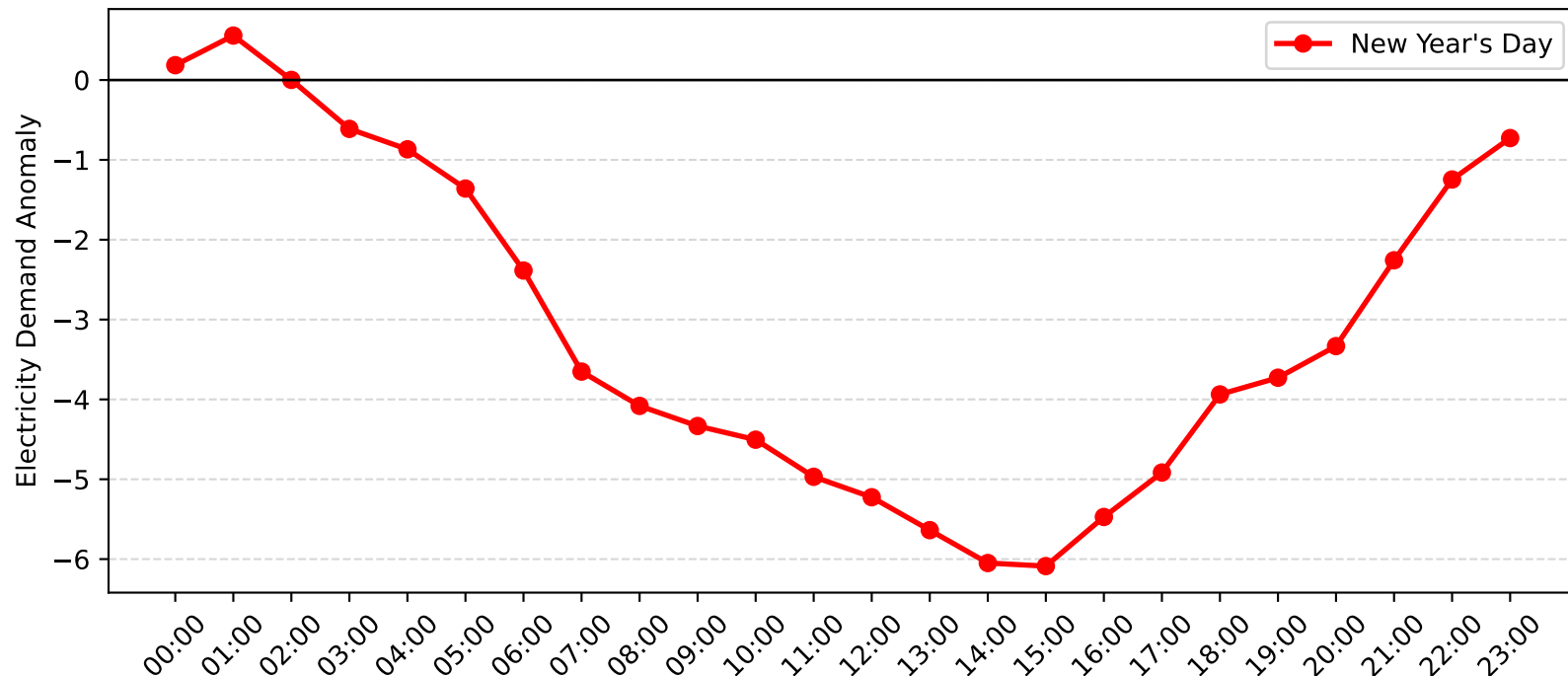
Jesmond Demand Anomaly: New Year's Day (2015-2016)
