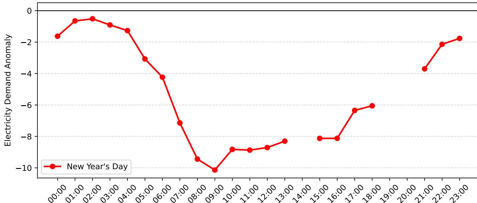
Maroubra Demand Anomaly: New Year's Day (2008-2009)
