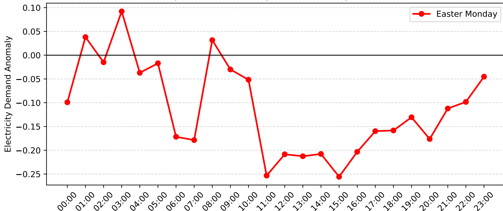
Rothbury Demand Anomaly: Easter Monday (2011-2012)
