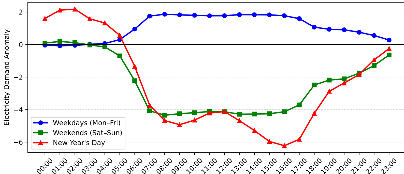
Concord Demand Anomaly: New Year's Day vs Weekday/Weekend (2017-2018)
