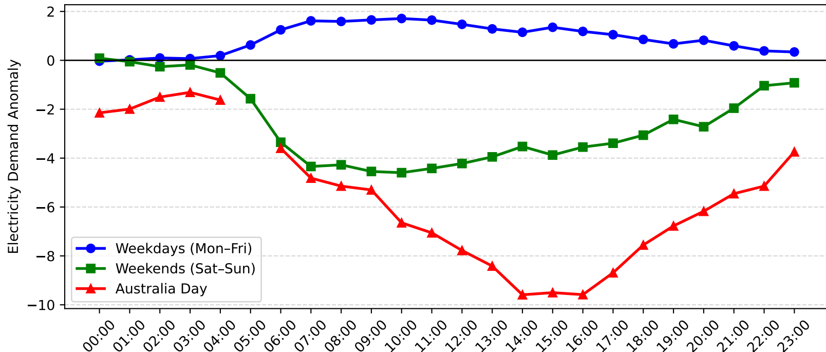
Potts Hill Demand Anomaly: Australia Day vs Weekday/Weekend (2017-2018)
