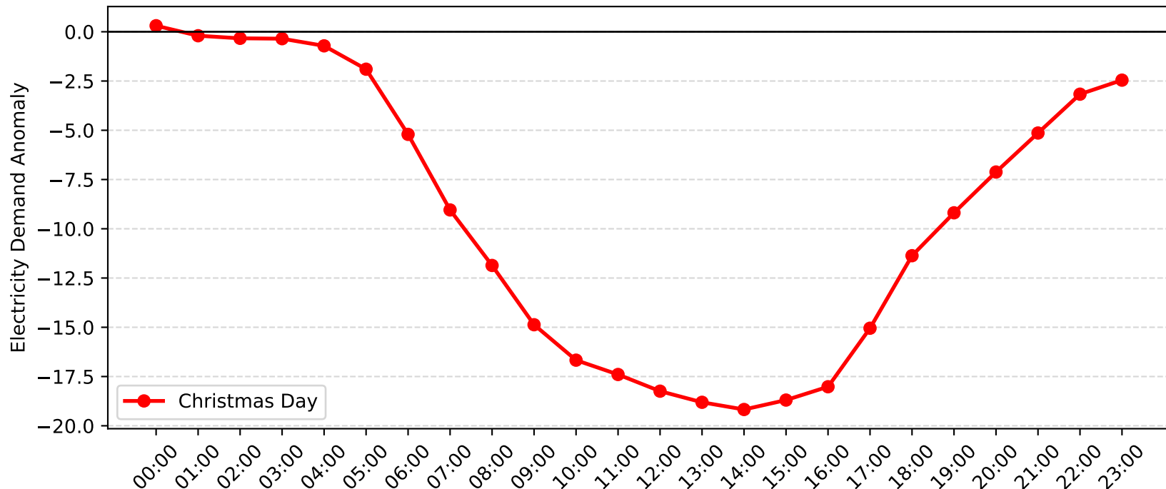
Castle Cove Demand Anomaly: Christmas Day (2005-2006)
