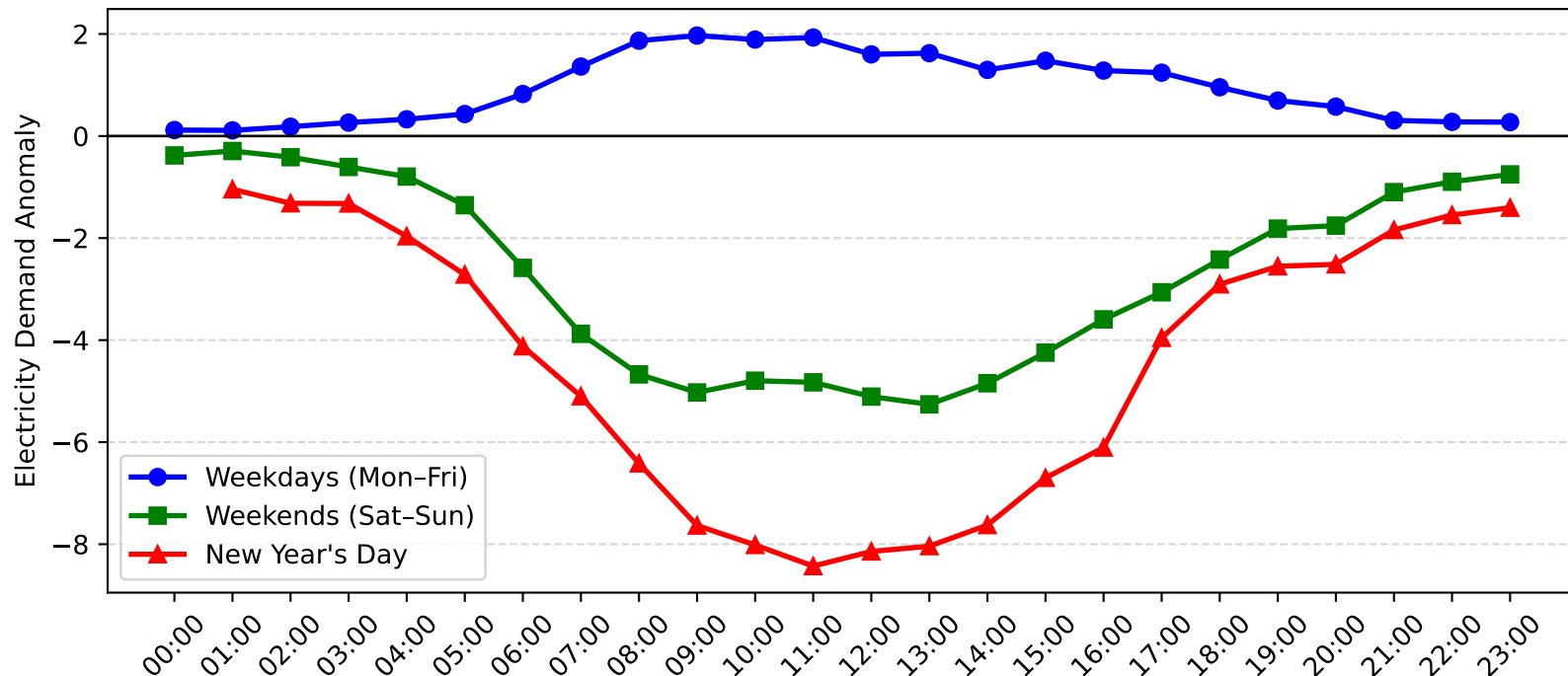
Auburn Demand Anomaly: New Year's Day vs Weekday/Weekend (2010-2011)
