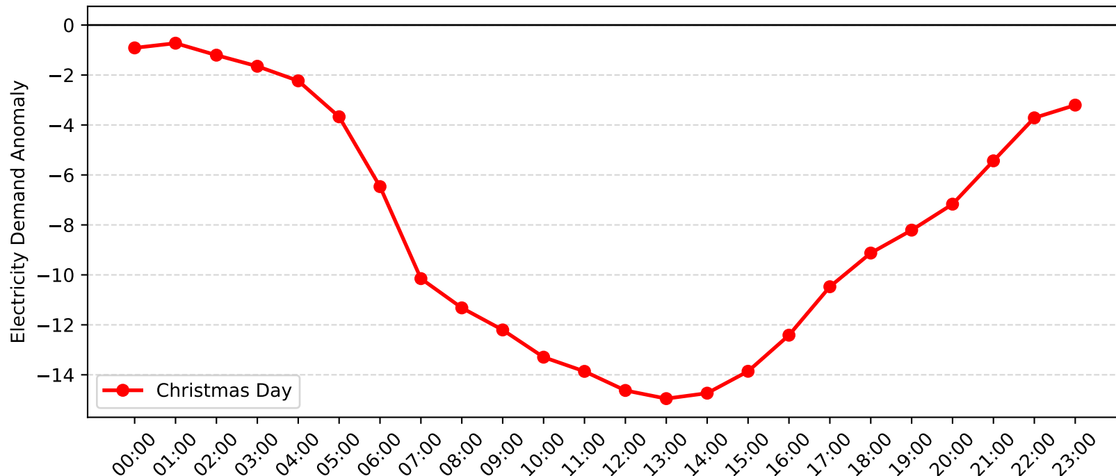
Marrickville Demand Anomaly: Christmas Day (2004-2005)
