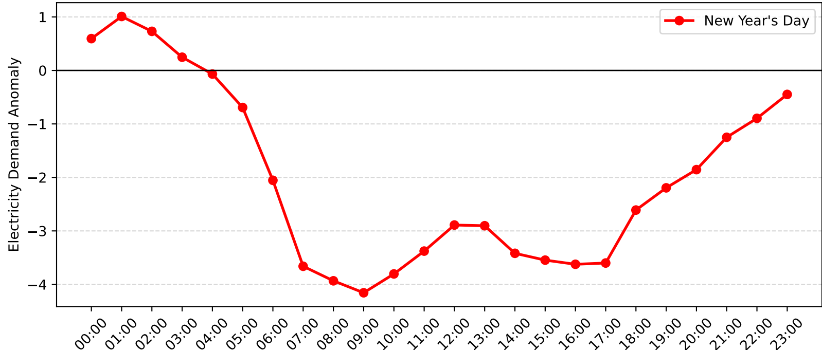
Concord Demand Anomaly: New Year's Day (2013-2014)
