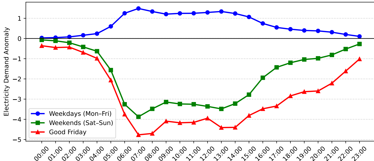
Wyong Demand Anomaly: Good Friday vs Weekday/Weekend (2014-2015)
