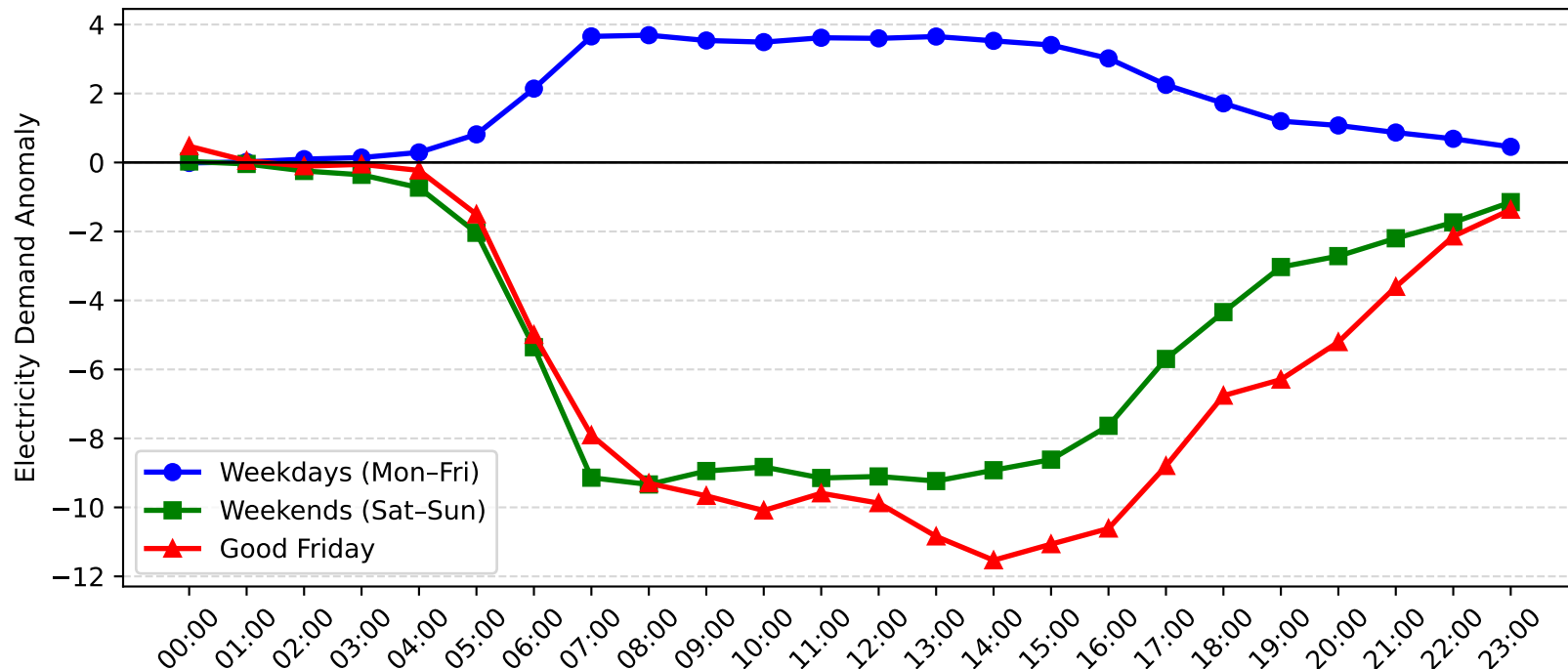
Zetland Demand Anomaly: Good Friday vs Weekday/Weekend (2011-2012)
