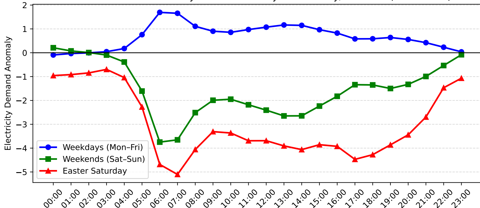
Kirrawee Demand Anomaly: Easter Saturday vs Weekday/Weekend (2010-2011)
