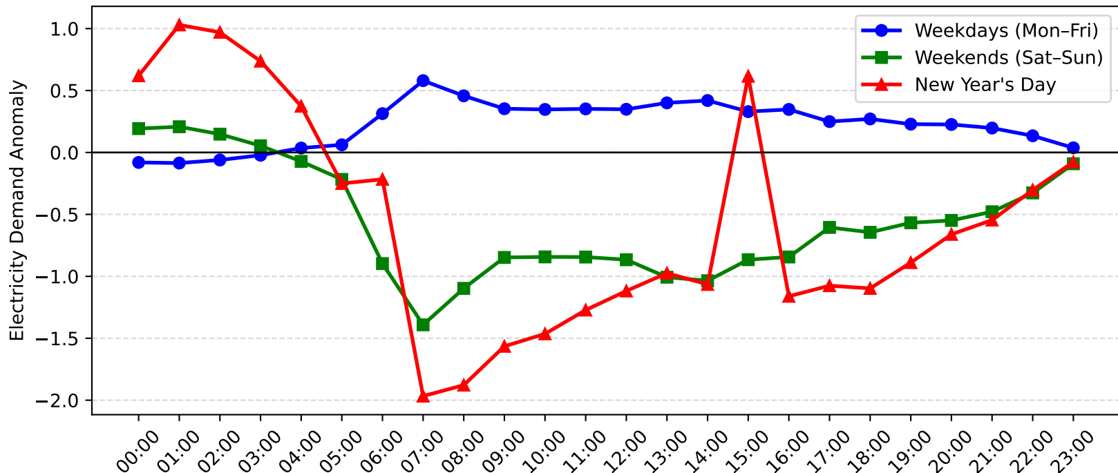
Arnccliffe Demand Anomaly: New Year's Day vs Weekday/Weekend (2016-2017)
