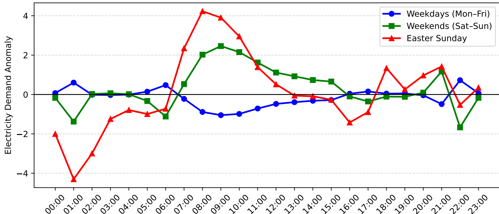
Nelson Bay Demand Anomaly: Easter Sunday vs Weekday/Weekend (2005-2006)
