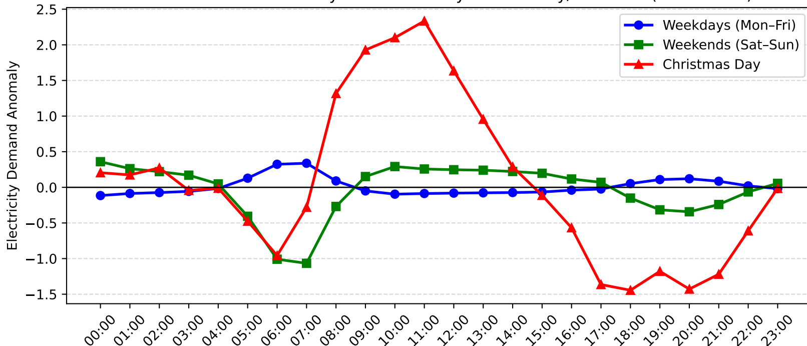
Harbord Demand Anomaly: Christmas Day vs Weekday/Weekend (2013-2014)
