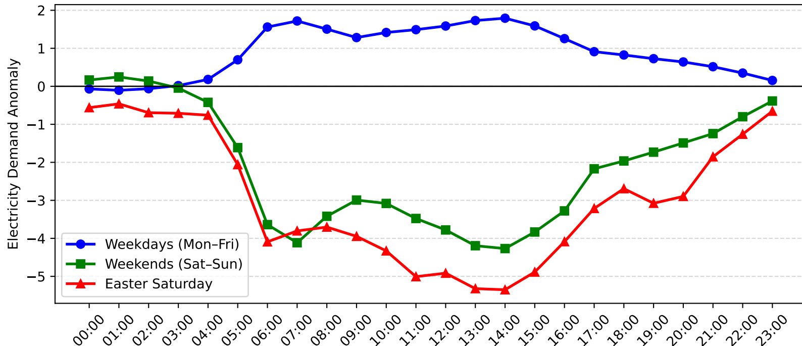
Kirrawee Demand Anomaly: Easter Saturday vs Weekday/Weekend (2005-2006)
