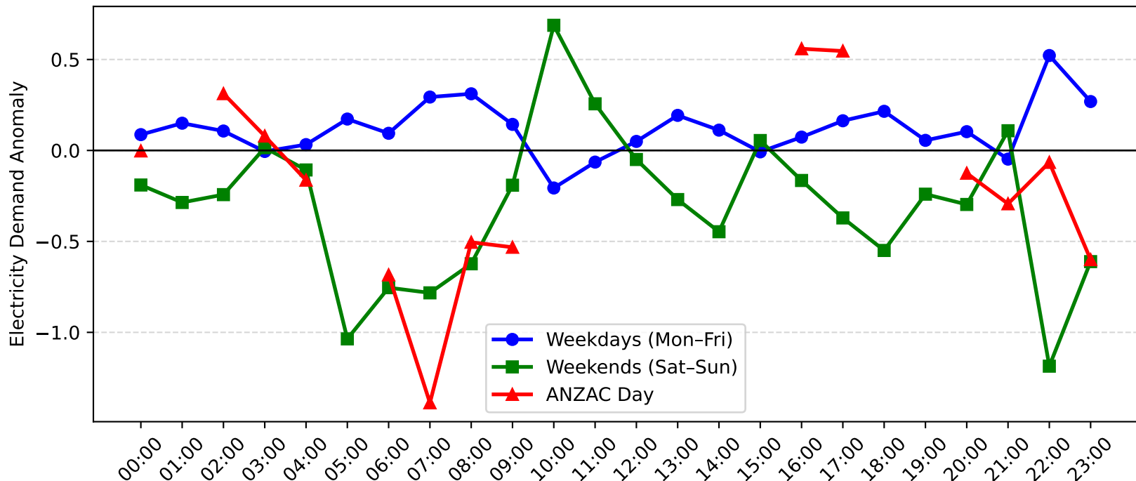
Adamstown Demand Anomaly: ANZAC Day vs Weekday/Weekend (2017-2018)
