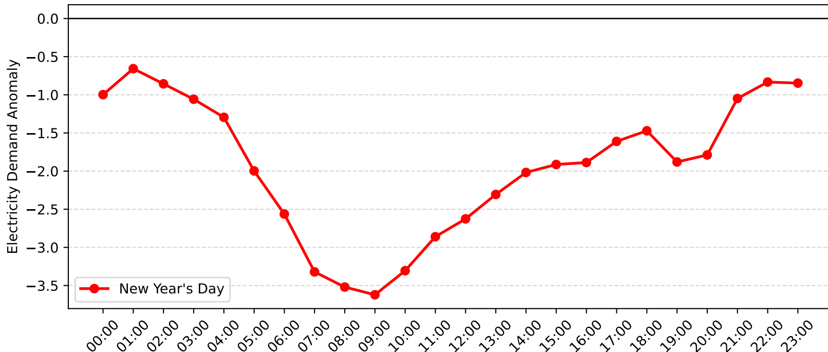
Lidcombe Demand Anomaly: New Year's Day (2011-2012)
