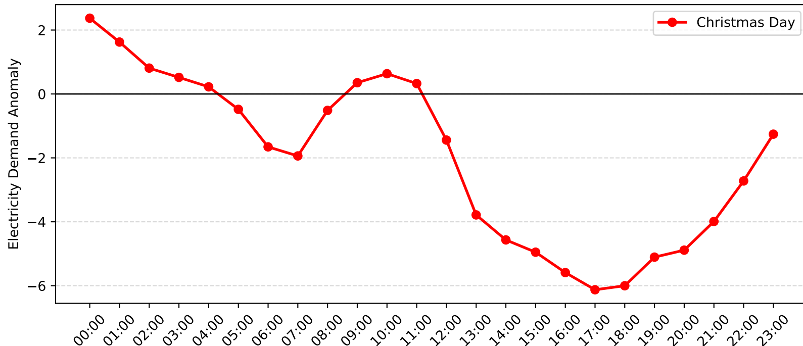
Mortdale Demand Anomaly: Christmas Day (2012-2013)
