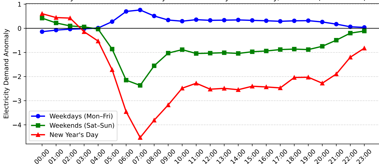
Dee Why West Demand Anomaly: New Year's Day vs Weekday/Weekend (2014-2015)
