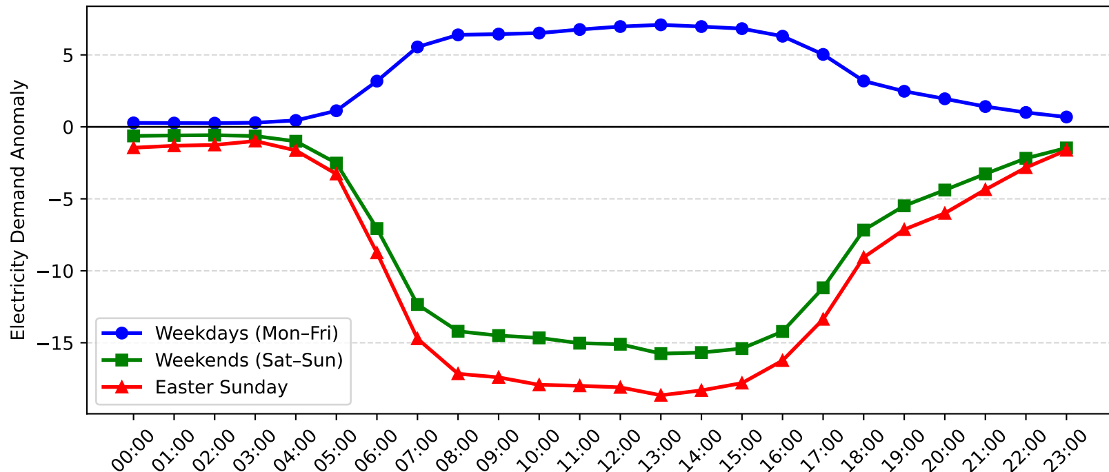
Gore Hill Demand Anomaly: Easter Sunday vs Weekday/Weekend (2008-2009)
