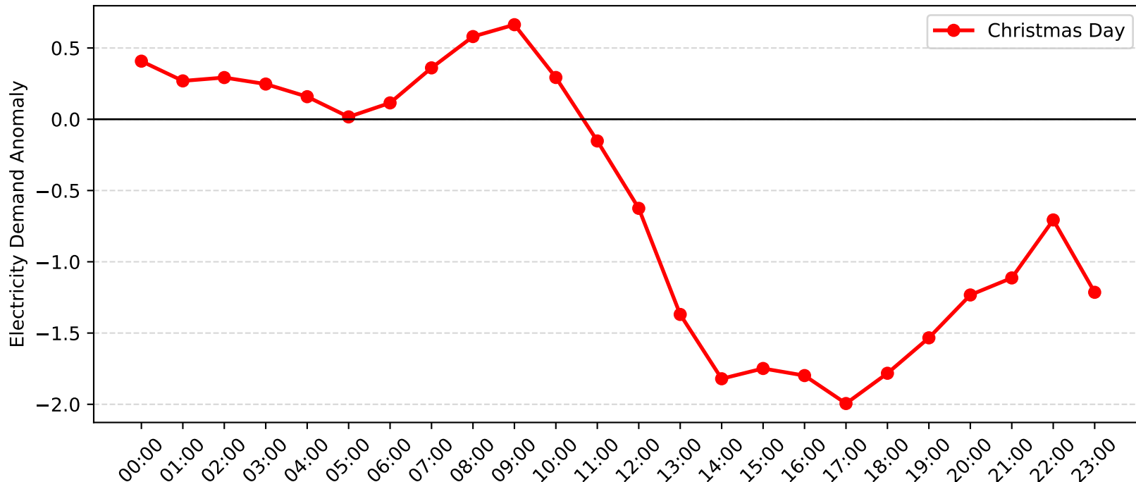
Telarah Demand Anomaly: Christmas Day (2011-2012)
