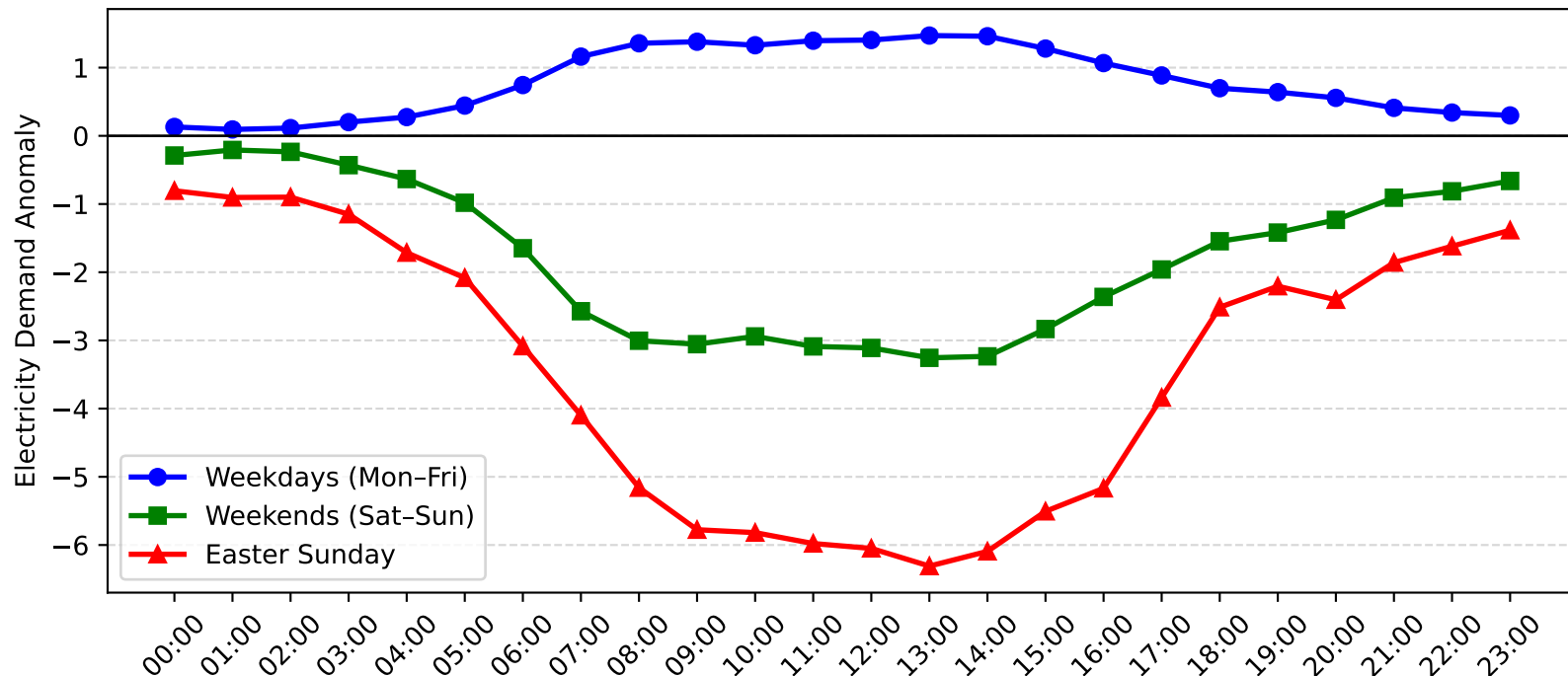
Auburn Demand Anomaly: Easter Sunday vs Weekday/Weekend (2017-2018)
