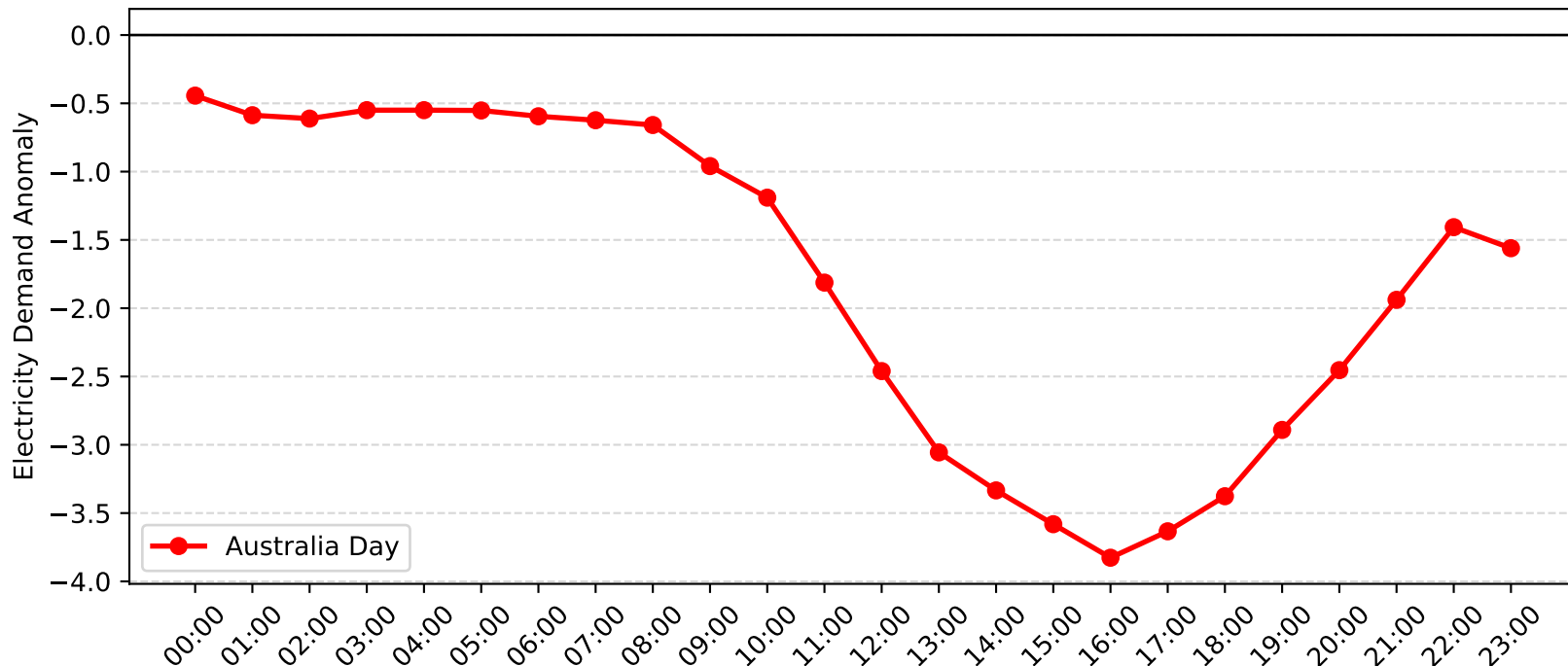
Telarah Demand Anomaly: Australia Day (2017-2018)
