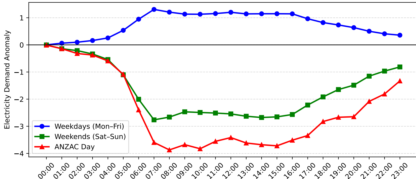
Lidcombe Demand Anomaly: ANZAC Day vs Weekday/Weekend (2009-2010)
