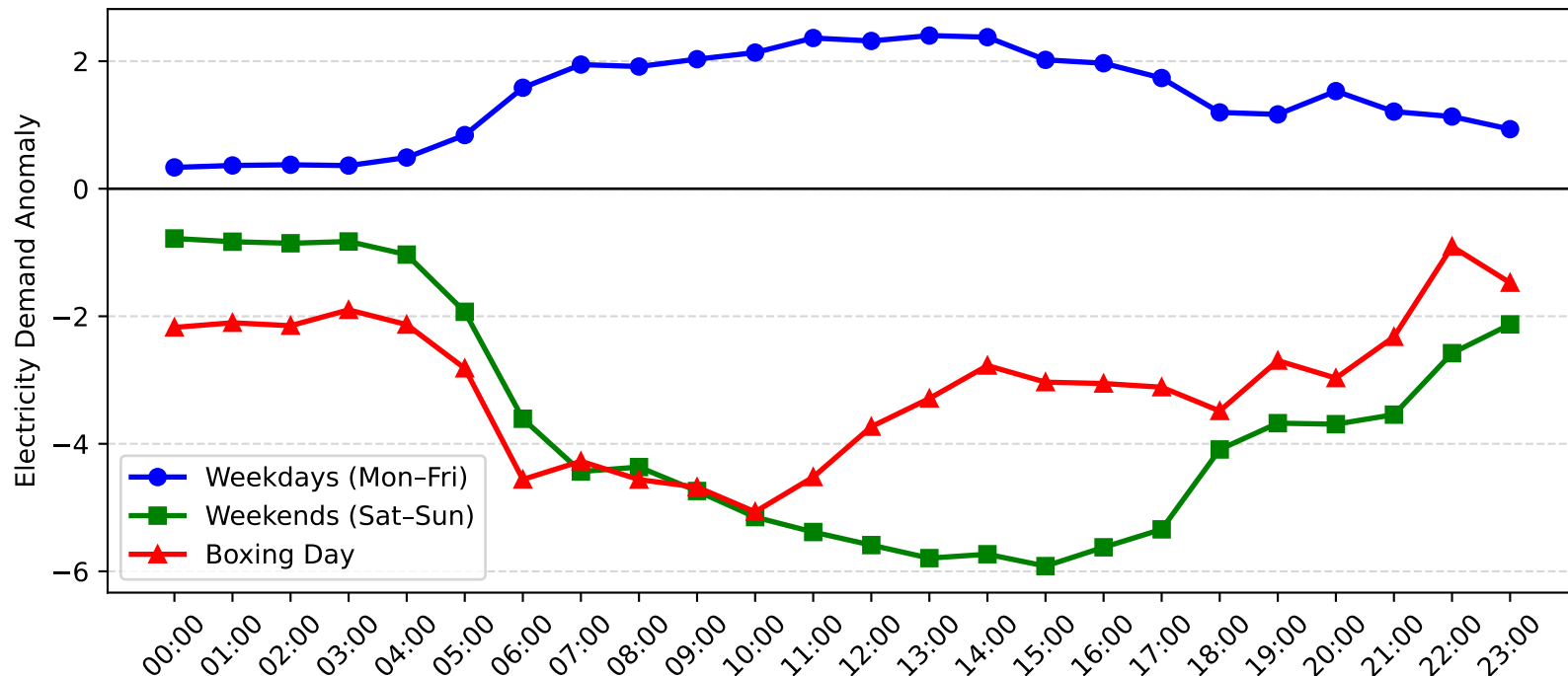
Potts Hill Demand Anomaly: Boxing Day vs Weekday/Weekend (2016-2017)
