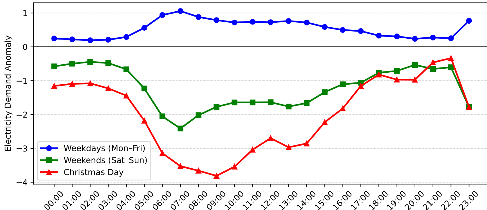
Rutherford Demand Anomaly: Christmas Day vs Weekday/Weekend (2010-2011)
