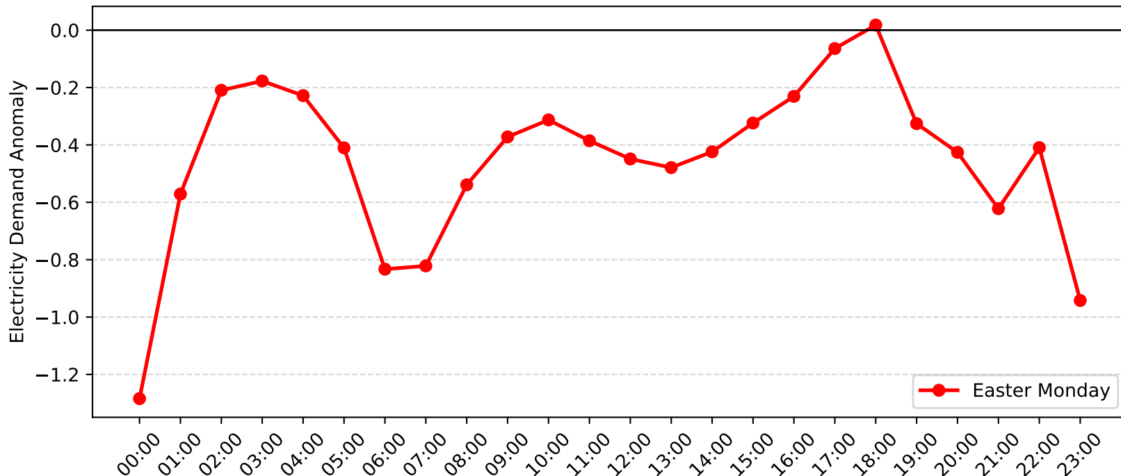
Telarah Demand Anomaly: Easter Monday (2011-2012)
