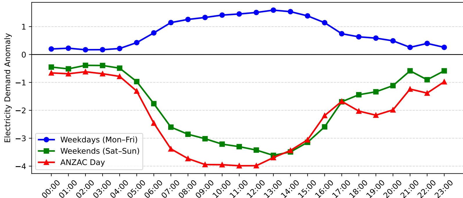
Broadmeadow Demand Anomaly: ANZAC Day vs Weekday/Weekend (2017-2018)
