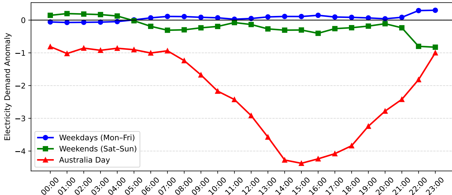
Muswellbrook Demand Anomaly: Australia Day vs Weekday/Weekend (2017-2018)
