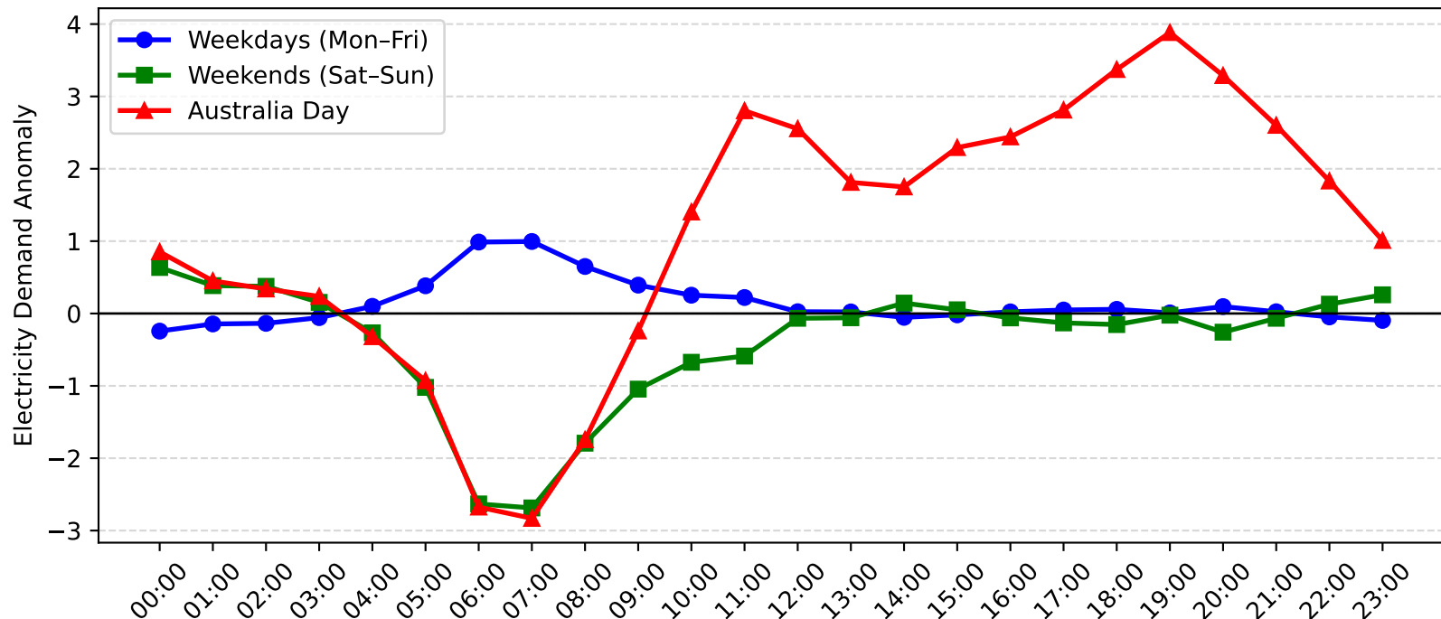
Revesby Demand Anomaly: Australia Day vs Weekday/Weekend (2011-2012)
