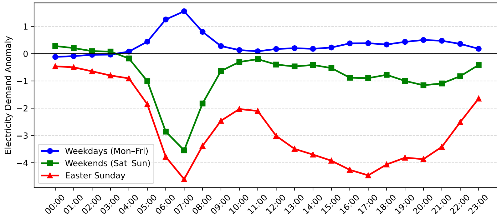
Dulwich Hill Demand Anomaly: Easter Sunday vs Weekday/Weekend (2015-2016)
