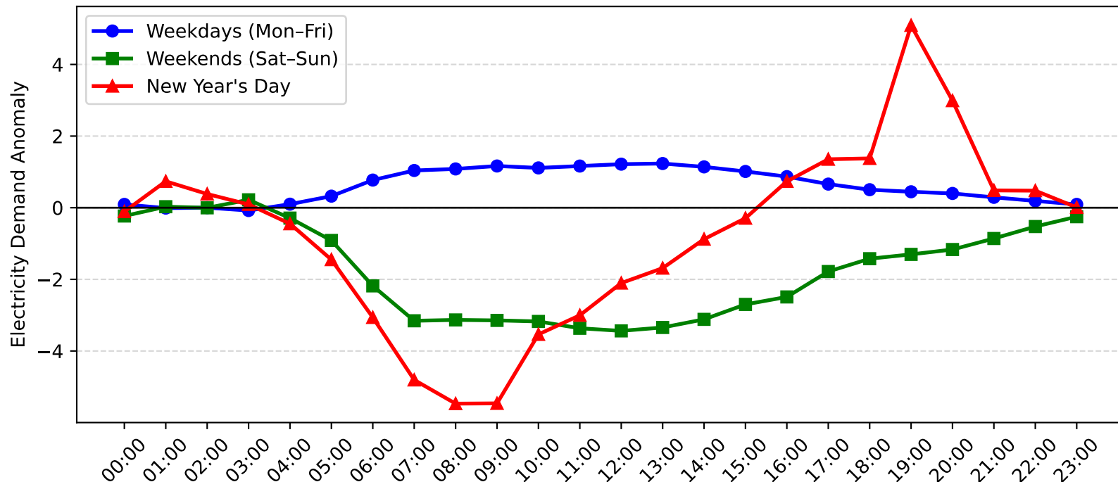
Wyong Demand Anomaly: New Year's Day vs Weekday/Weekend (2008-2009)
