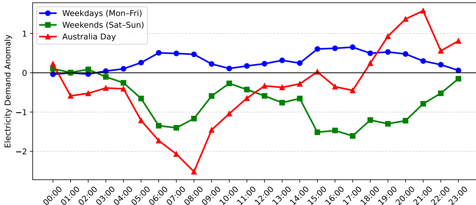
Charmhaven Demand Anomaly: Australia Day vs Weekday/Weekend (2009-2010)
