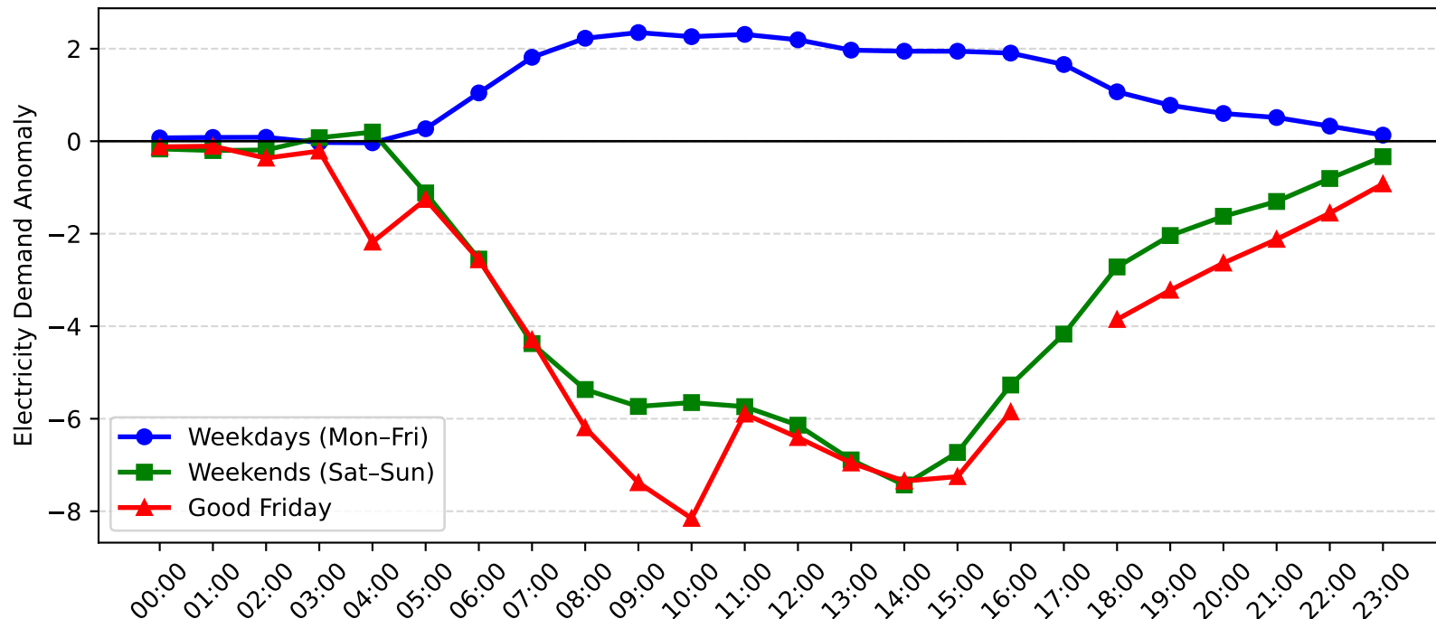
Green Square Demand Anomaly: Good Friday vs Weekday/Weekend (2015-2016)
