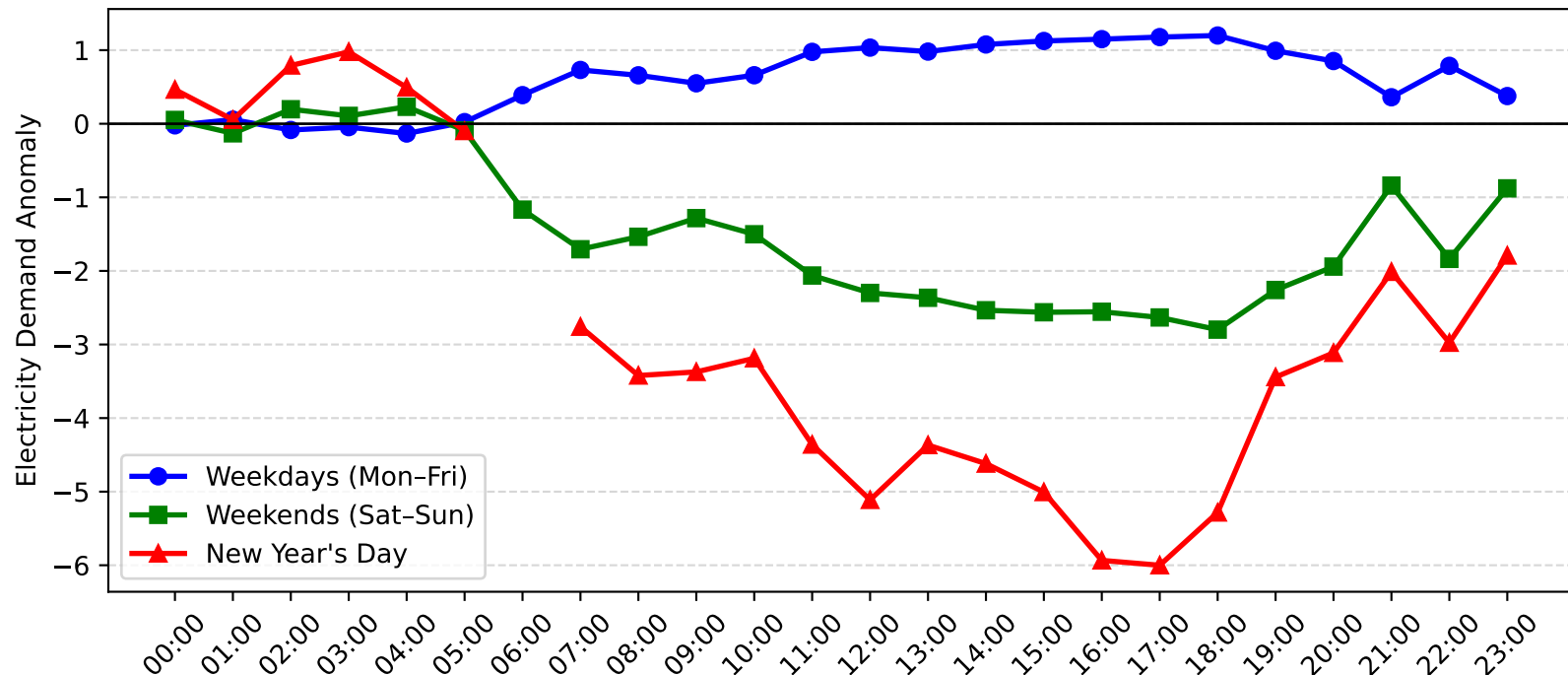
Charlestown Demand Anomaly: New Year's Day vs Weekday/Weekend (2017-2018)
