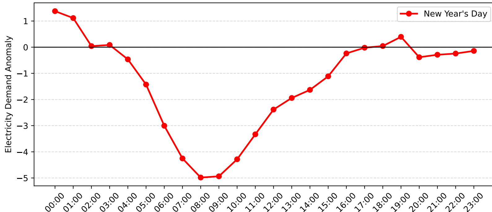
Wyong Demand Anomaly: New Year's Day (2009-2010)
