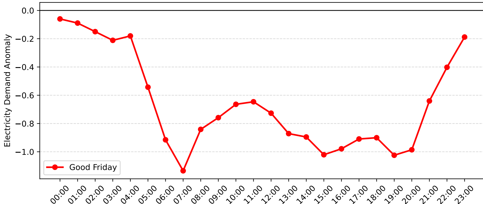
Narrabeen Demand Anomaly: Good Friday (2016-2017)
