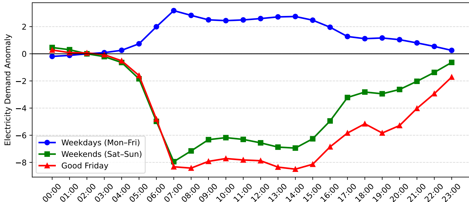
Marrickville Demand Anomaly: Good Friday vs Weekday/Weekend (2011-2012)
