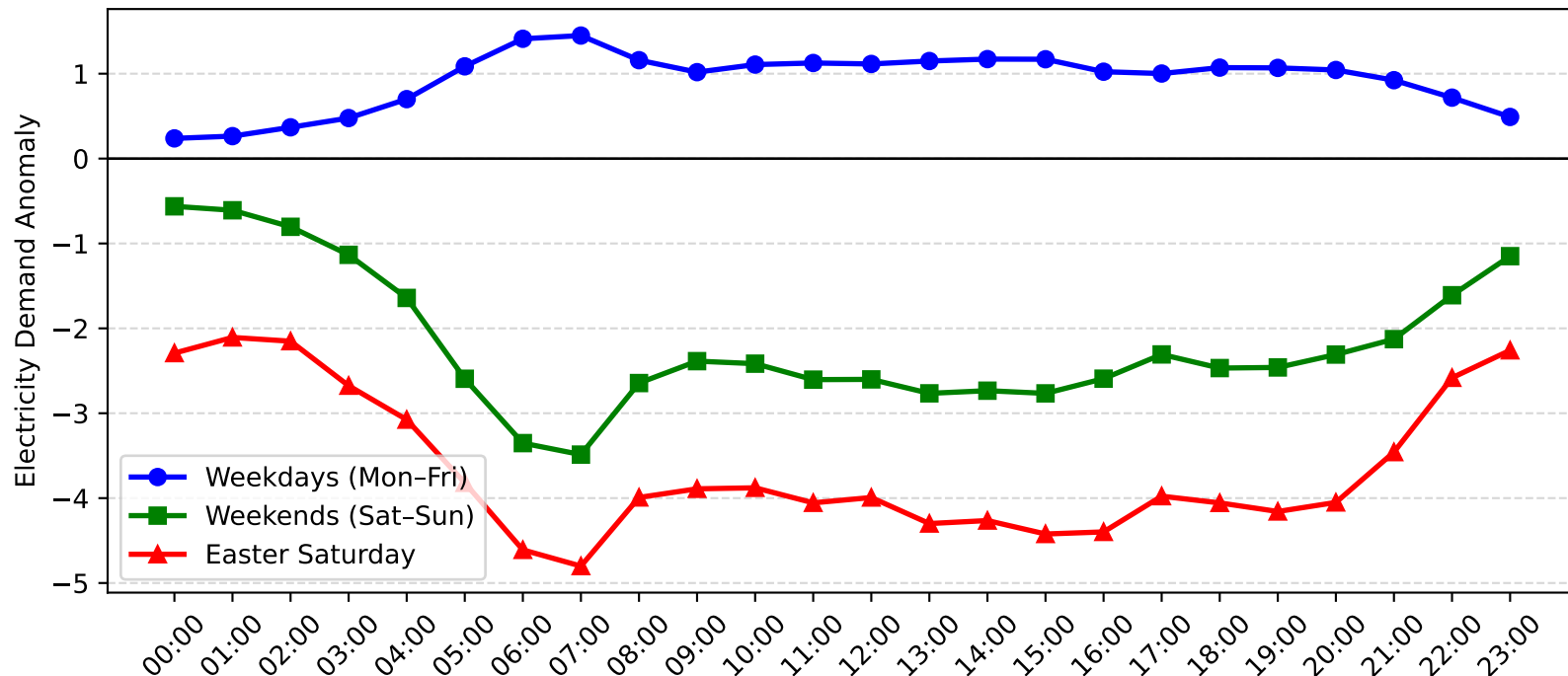
Lisarow Demand Anomaly: Easter Saturday vs Weekday/Weekend (2006-2007)
