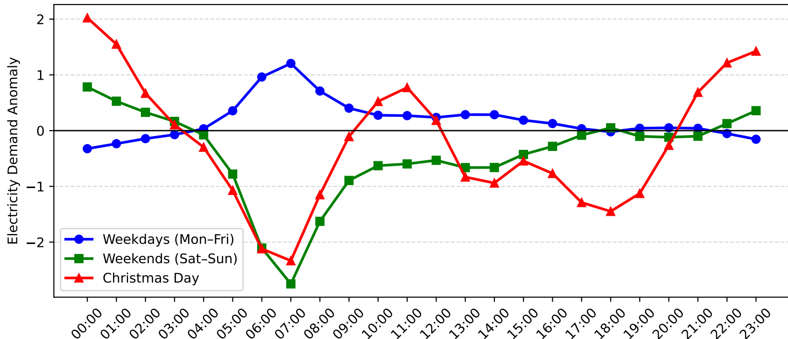
Mortdale Demand Anomaly: Christmas Day vs Weekday/Weekend (2010-2011)
