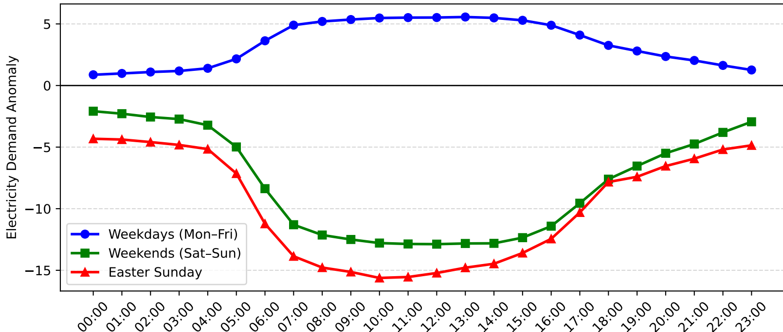
Flemington Demand Anomaly: Easter Sunday vs Weekday/Weekend (2011-2012)
