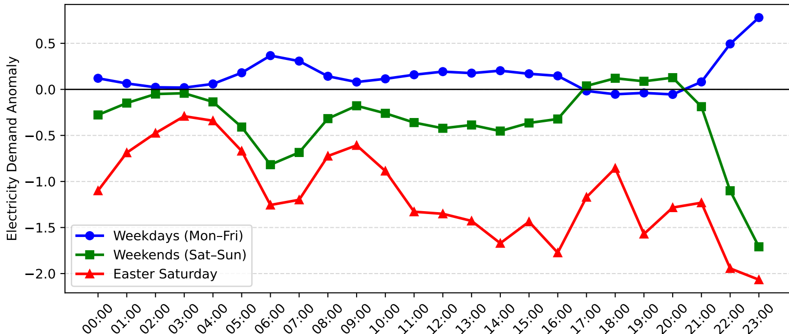
Muswellbrook Demand Anomaly: Easter Saturday vs Weekday/Weekend (2009-2010)
