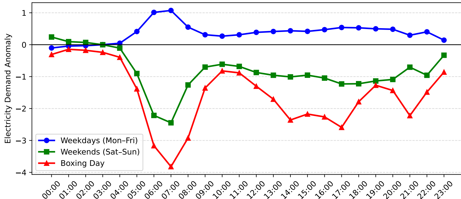
Dee Why West Demand Anomaly: Boxing Day vs Weekday/Weekend (2010-2011)
