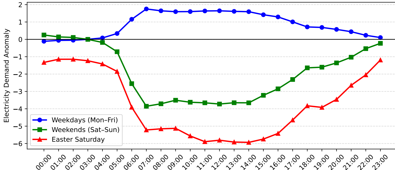
Concord Demand Anomaly: Easter Saturday vs Weekday/Weekend (2010-2011)
