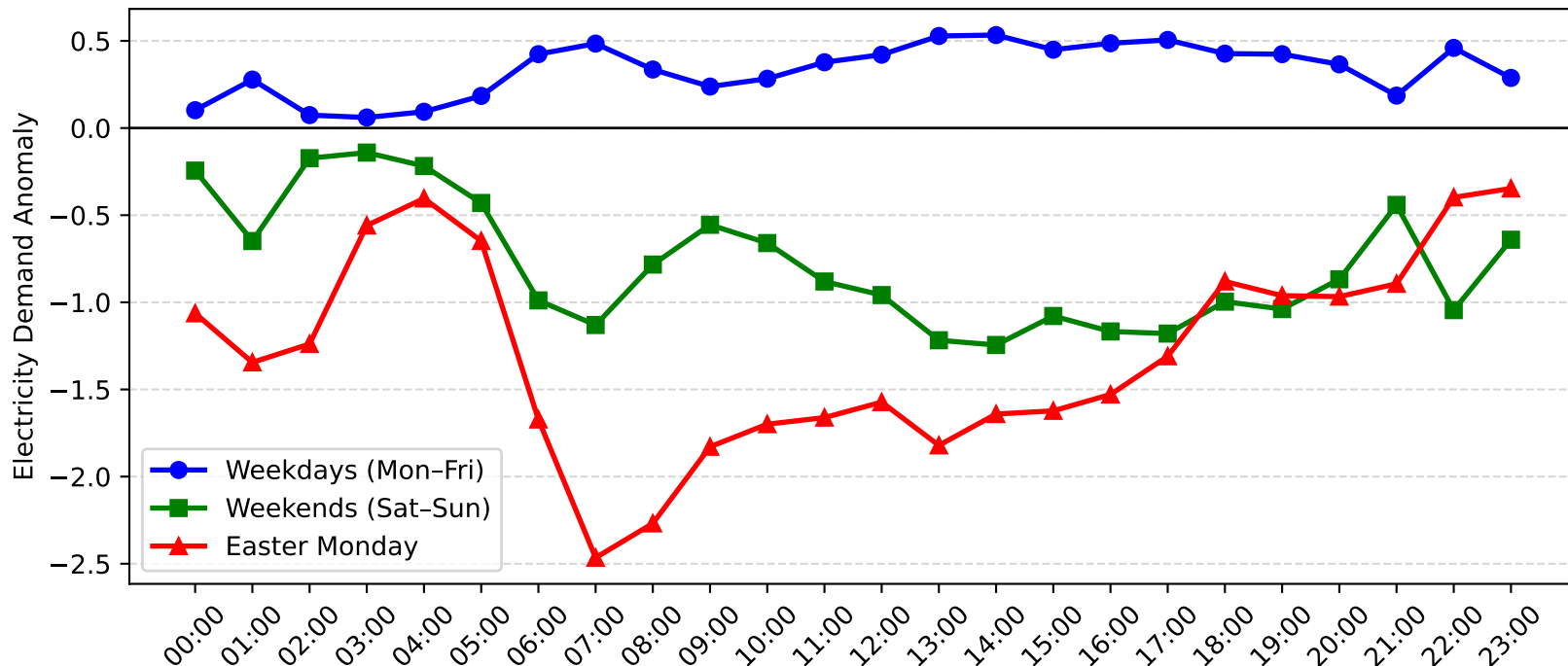
Gateshead Demand Anomaly: Easter Monday vs Weekday/Weekend (2007-2008)
