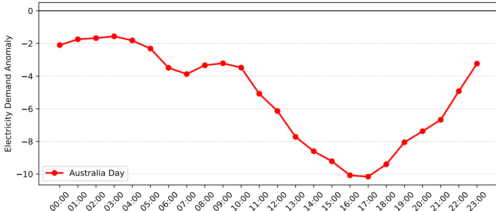
Revesby Demand Anomaly: Australia Day (2017-2018)
