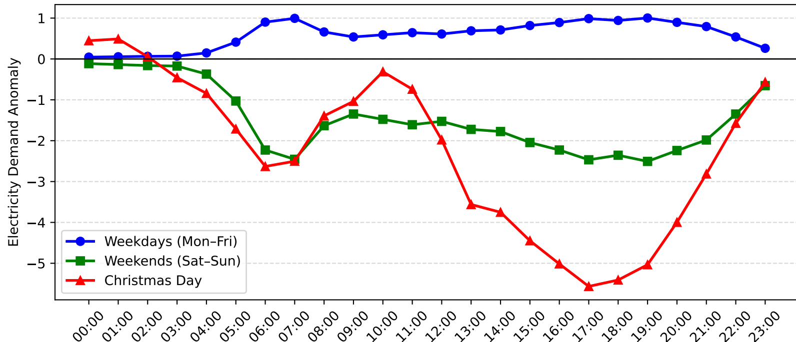
Revesby Demand Anomaly: Christmas Day vs Weekday/Weekend (2015-2016)
