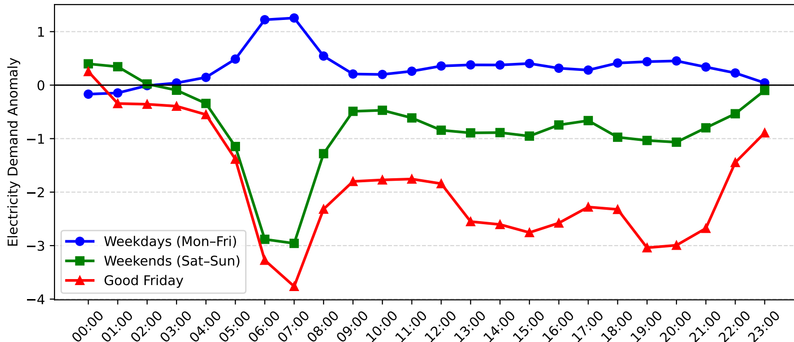
Mortdale Demand Anomaly: Good Friday vs Weekday/Weekend (2017-2018)
