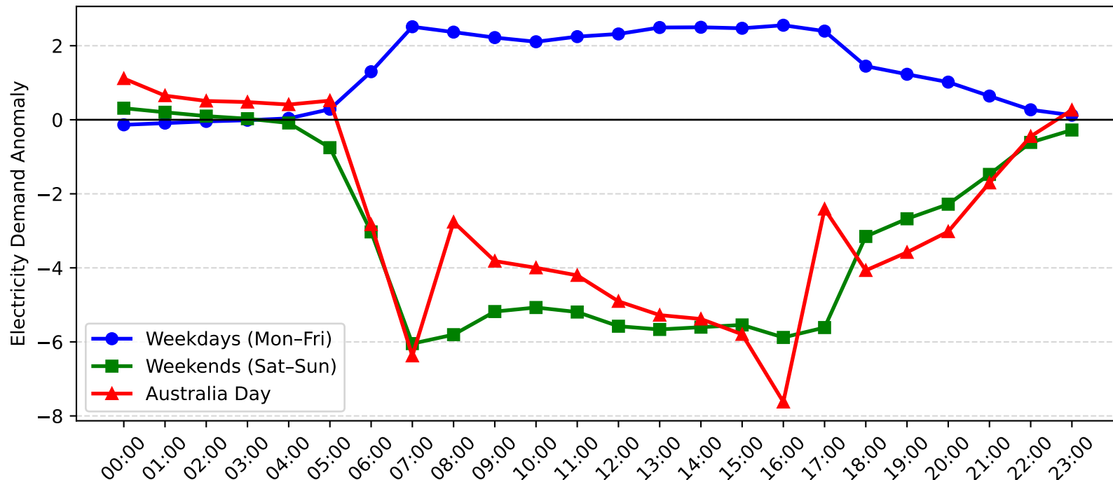
Epping Demand Anomaly: Australia Day vs Weekday/Weekend (2013-2014)
