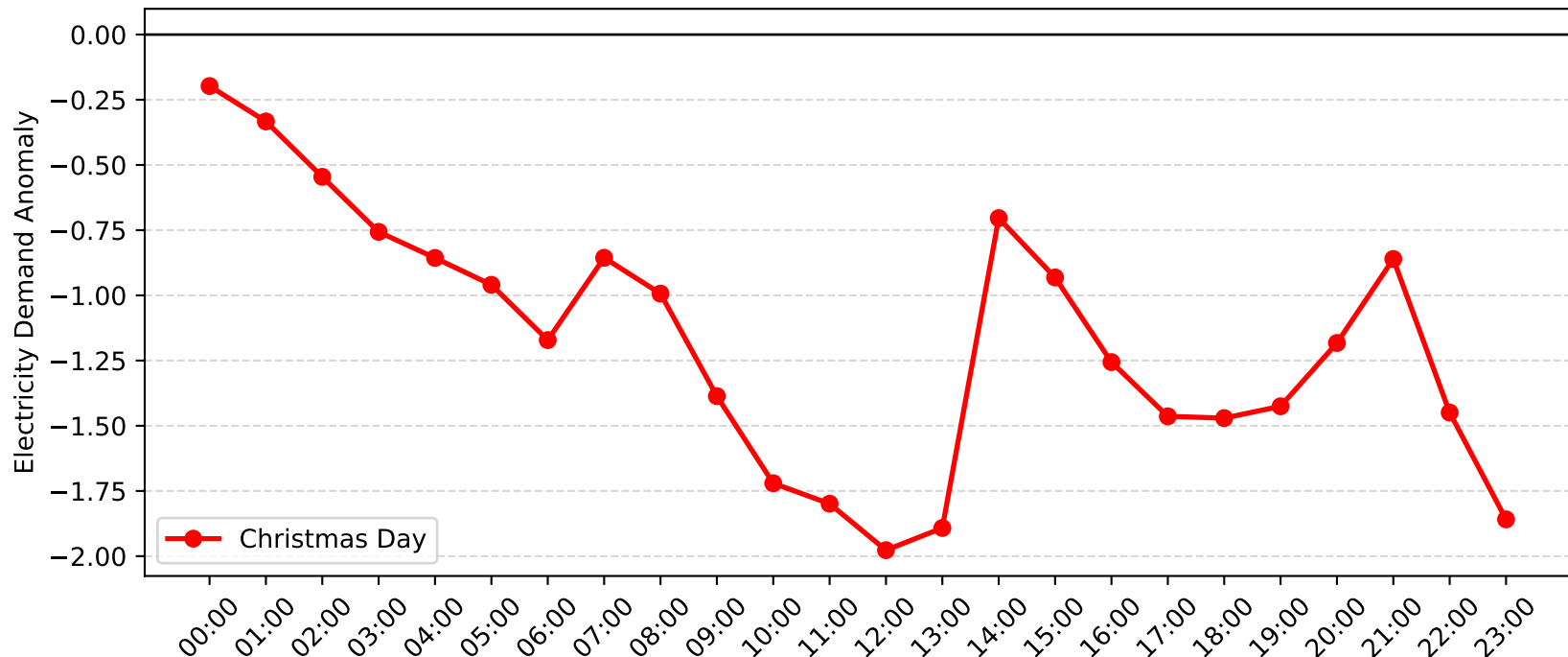
Muswellbrook Demand Anomaly: Christmas Day (2009-2010)
