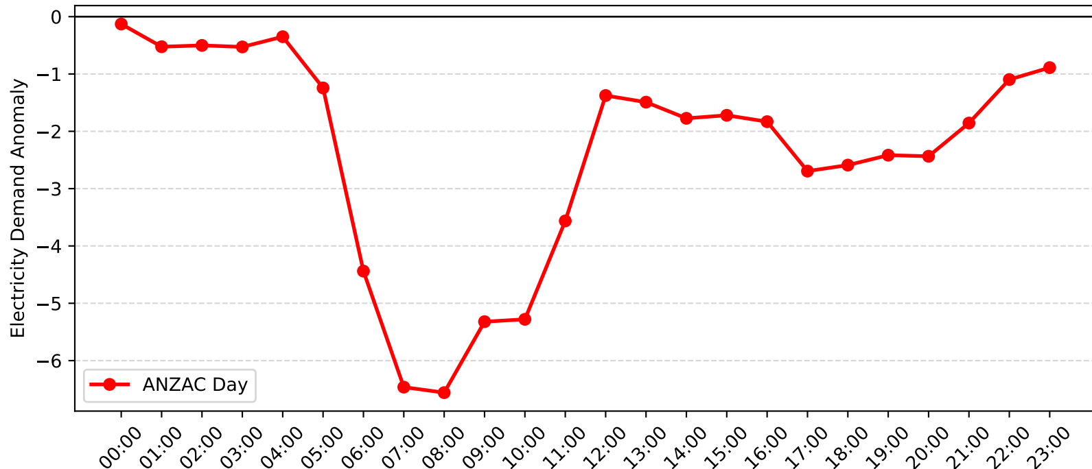
Epping Demand Anomaly: ANZAC Day (2007-2008)
