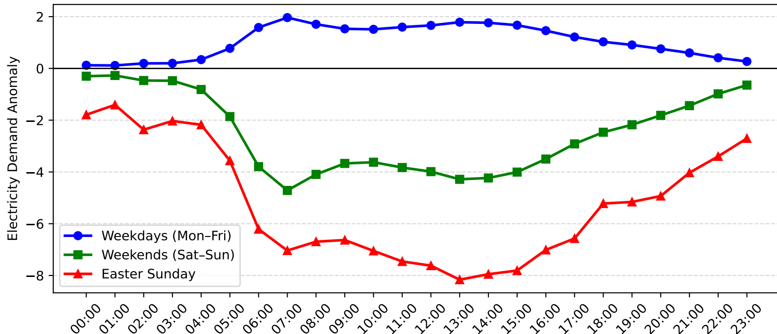
Sefton Demand Anomaly: Easter Sunday vs Weekday/Weekend (2014-2015)
