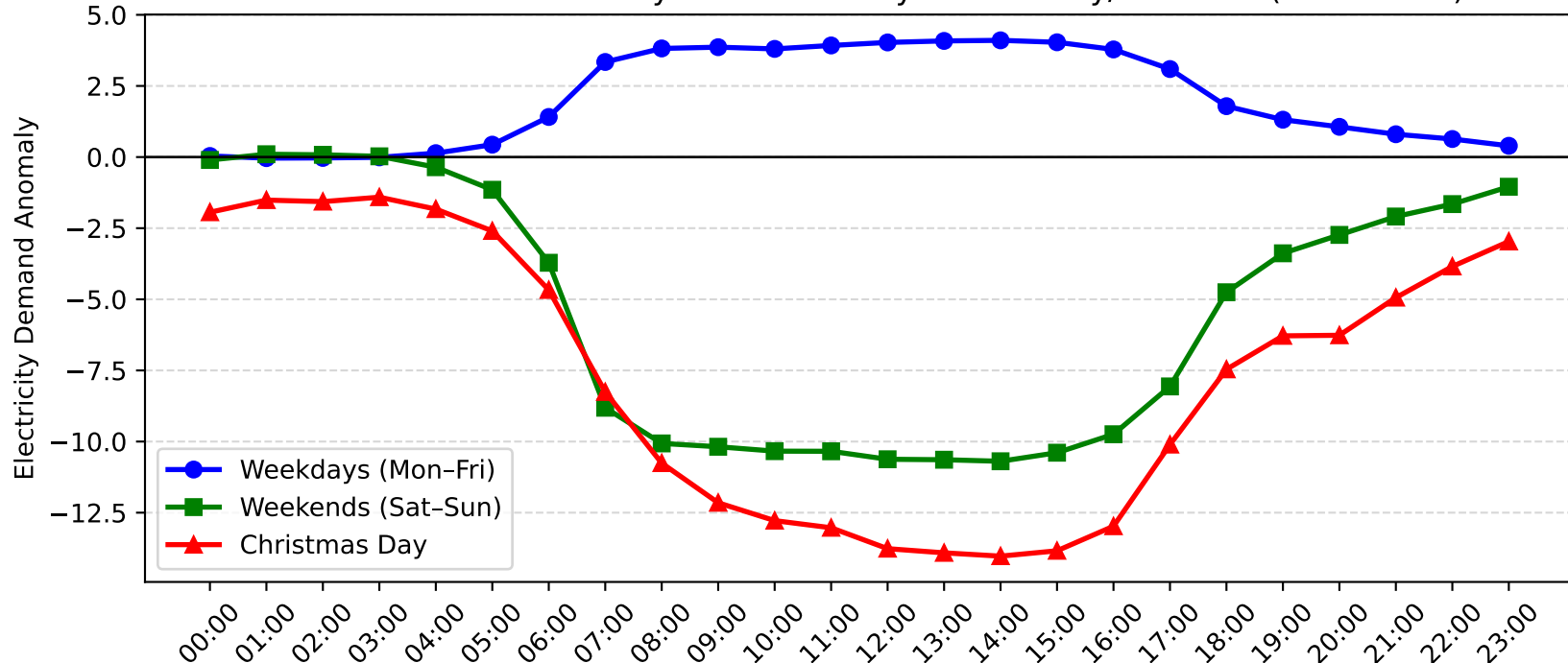
Gore Hill Demand Anomaly: Christmas Day vs Weekday/Weekend (2012-2013)
