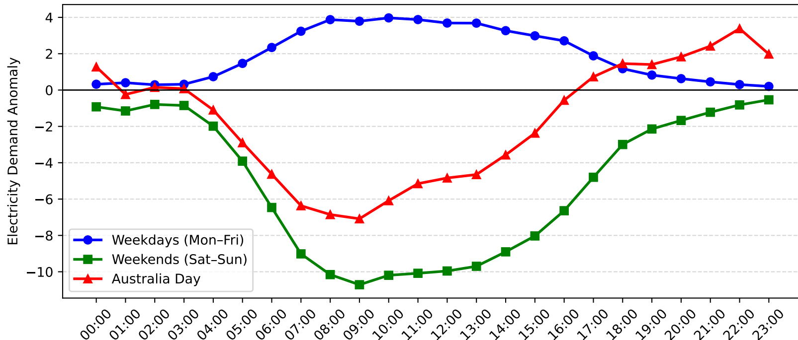
Homebush Bay Demand Anomaly: Australia Day vs Weekday/Weekend (2010-2011)
