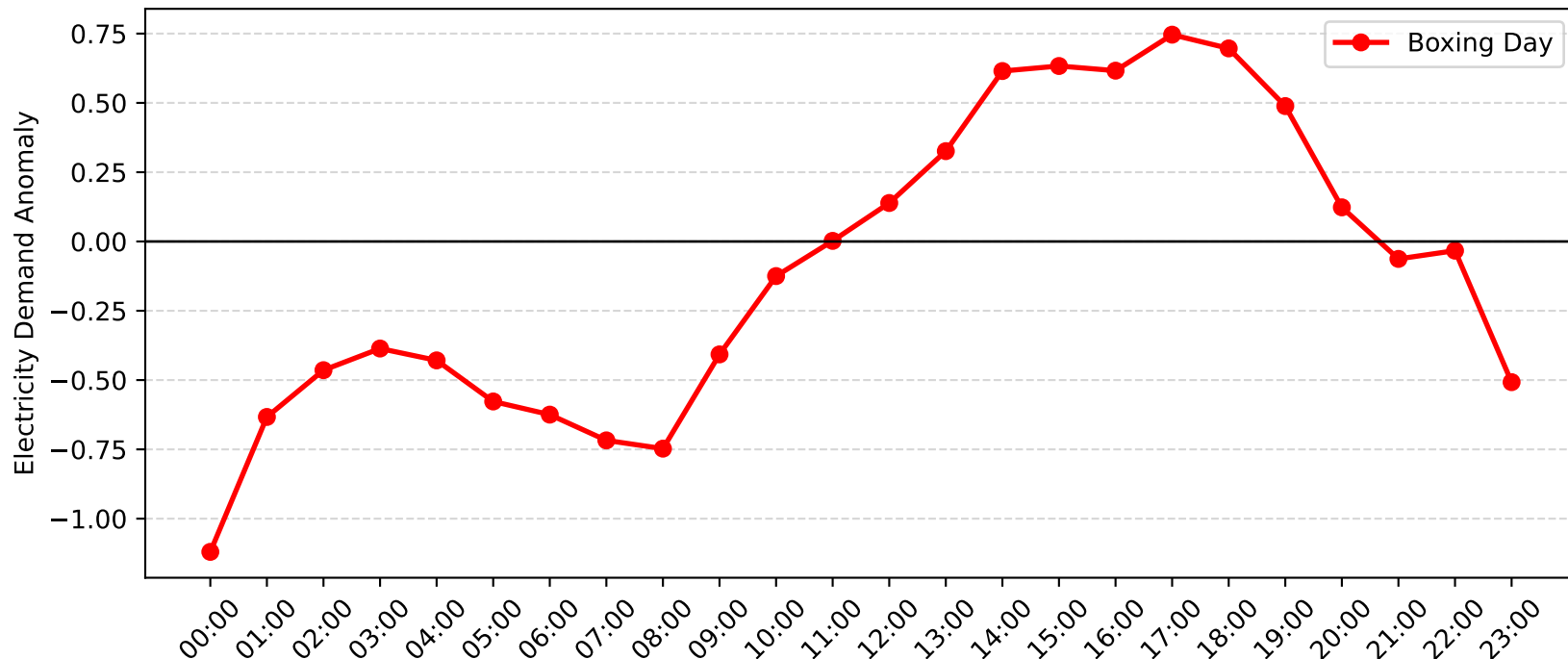
Telarah Demand Anomaly: Boxing Day (2016-2017)
