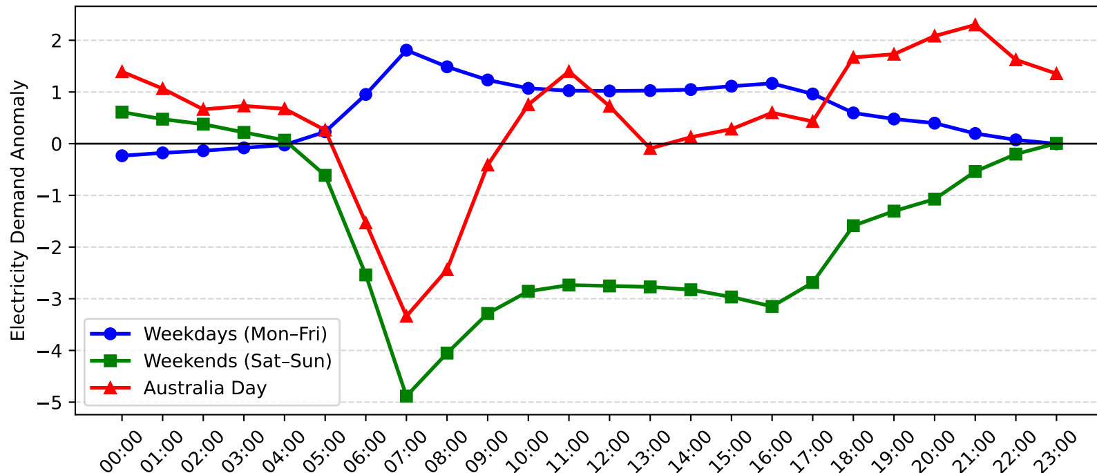
Chatswood Demand Anomaly: Australia Day vs Weekday/Weekend (2011-2012)
