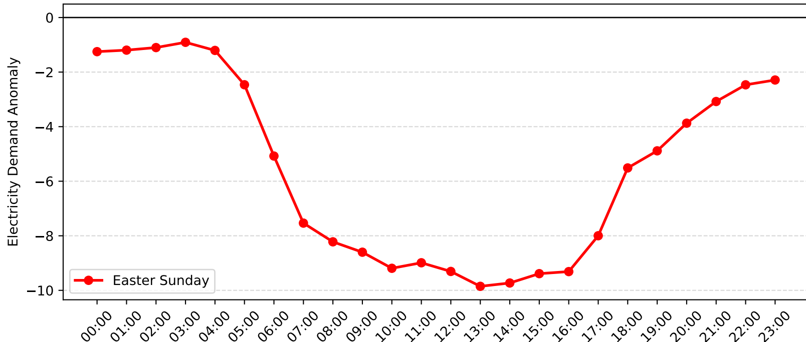
Macquarie Park Demand Anomaly: Easter Sunday (2009-2010)
