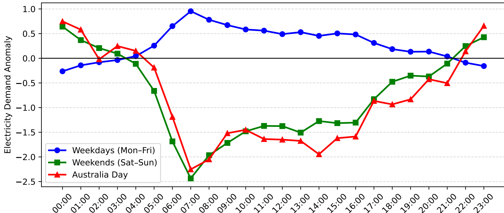
Rockdale Demand Anomaly: Australia Day vs Weekday/Weekend (2006-2007)
