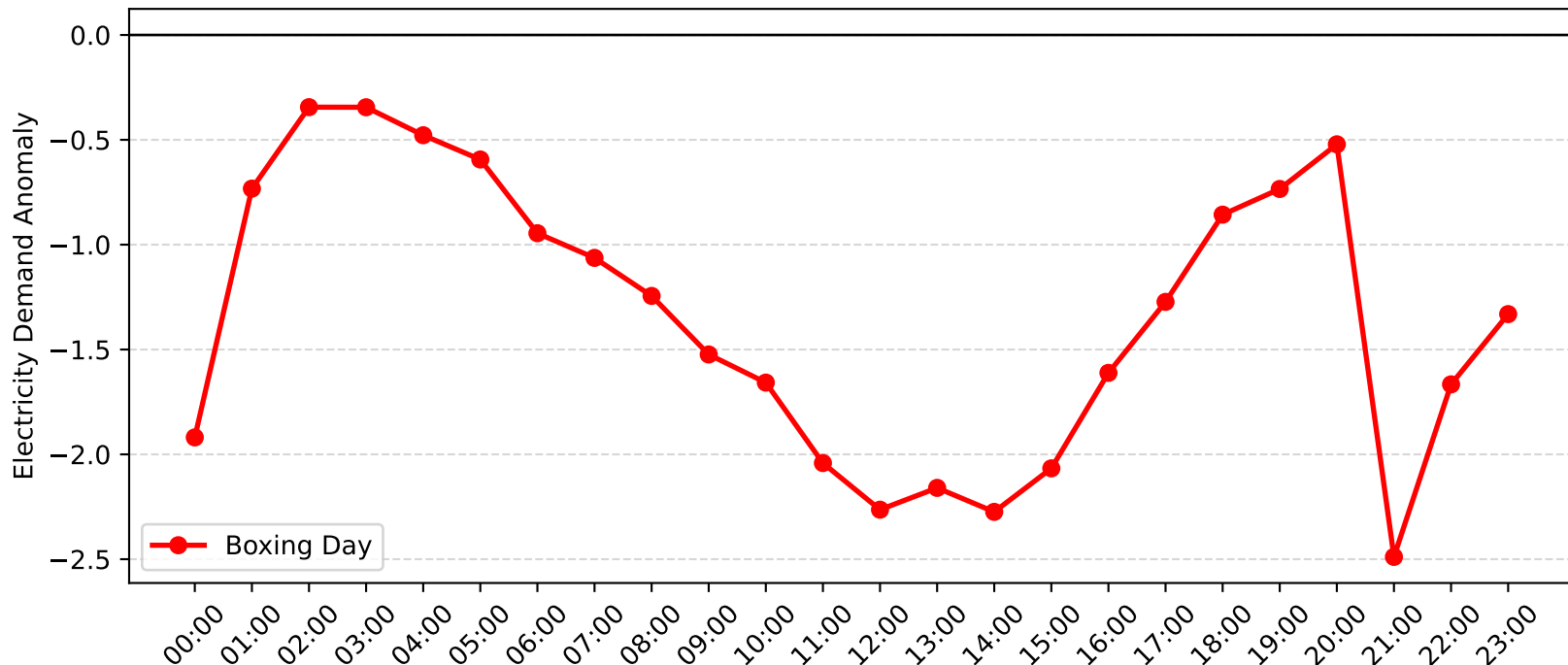
Telarah Demand Anomaly: Boxing Day (2008-2009)
