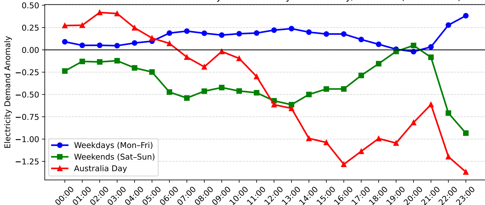
Muswellbrook Demand Anomaly: Australia Day vs Weekday/Weekend (2015-2016)
