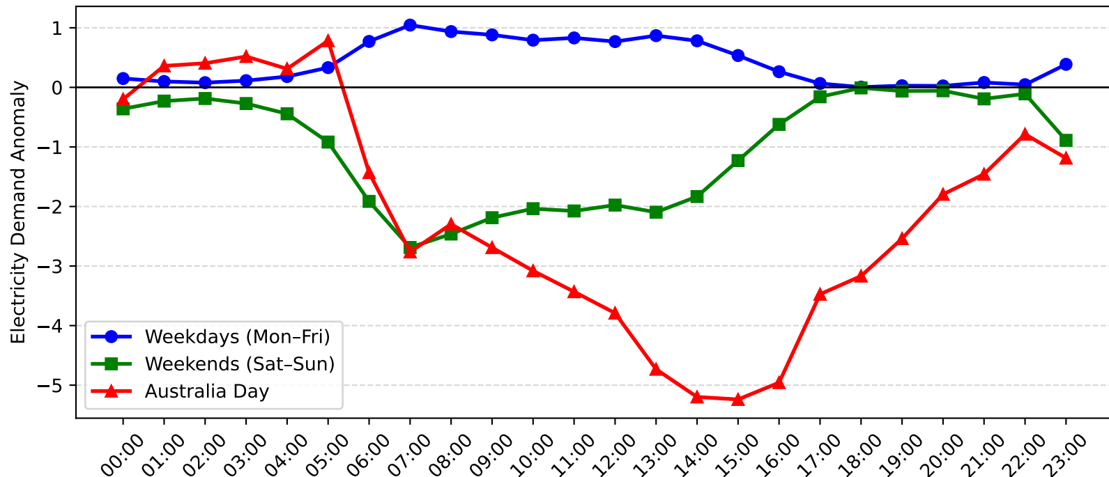
Rutherford Demand Anomaly: Australia Day vs Weekday/Weekend (2014-2015)
