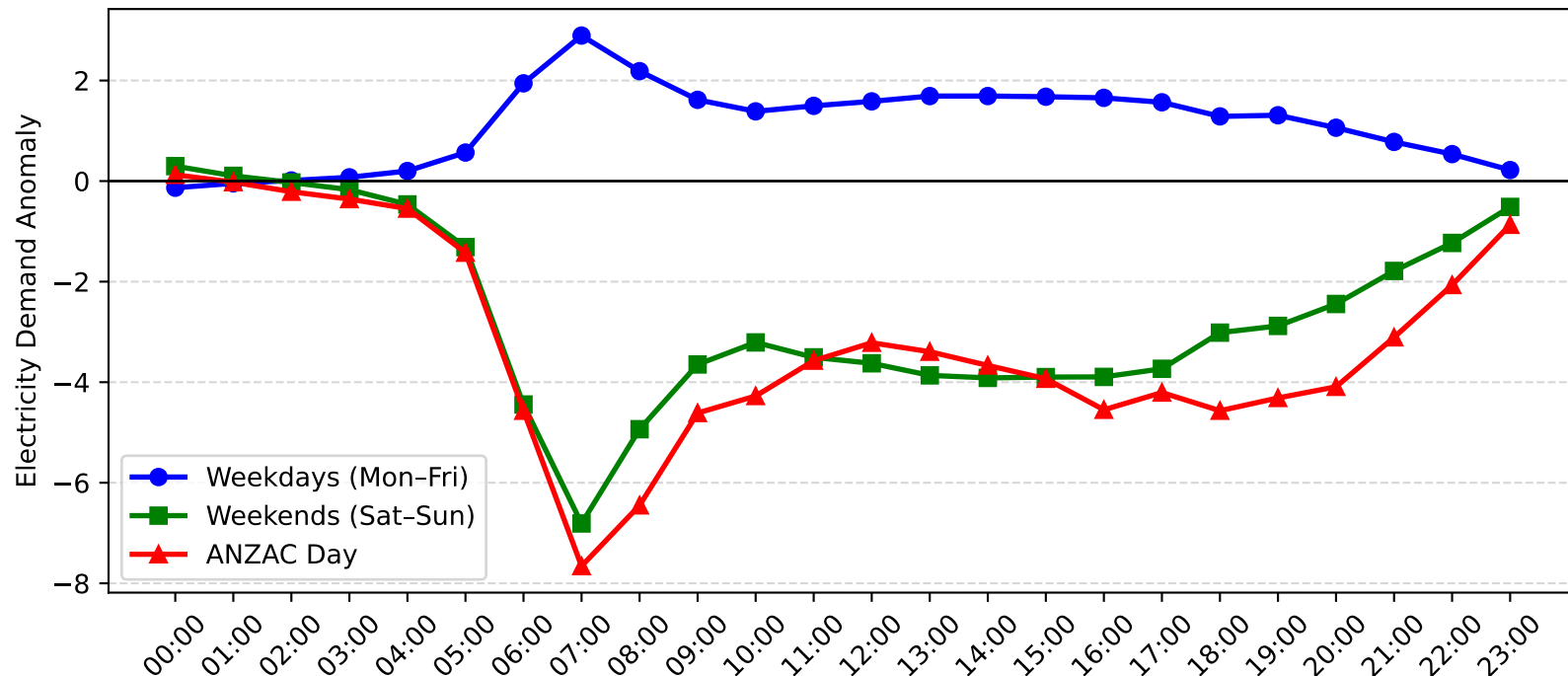
Chatswood Demand Anomaly: ANZAC Day vs Weekday/Weekend (2008-2009)
