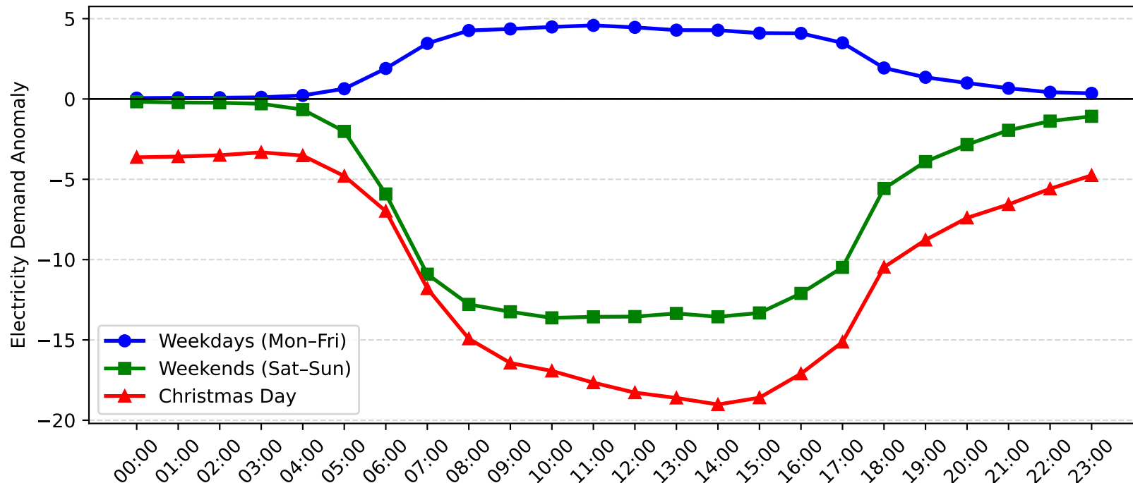
Macquarie Park Demand Anomaly: Christmas Day vs Weekday/Weekend (2013-2014)
