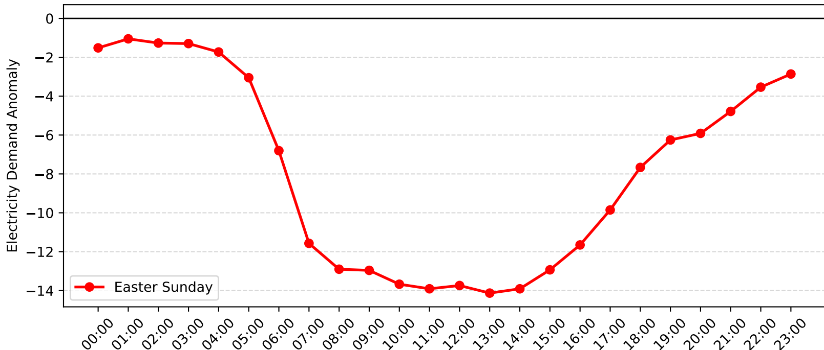
St. Peters Demand Anomaly: Easter Sunday (2012-2013)
