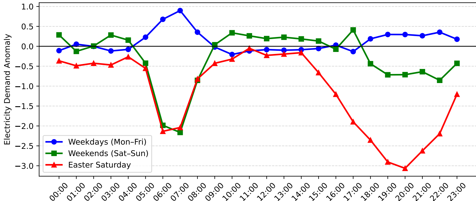
Balgowlah North Demand Anomaly: Easter Saturday vs Weekday/Weekend (2011-2012)
