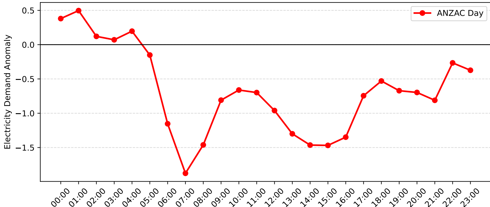
Adamstown Demand Anomaly: ANZAC Day (2012-2013)
