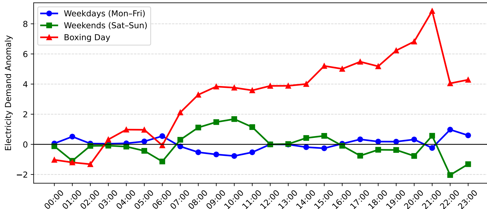
Nelson Bay Demand Anomaly: Boxing Day vs Weekday/Weekend (2004-2005)
