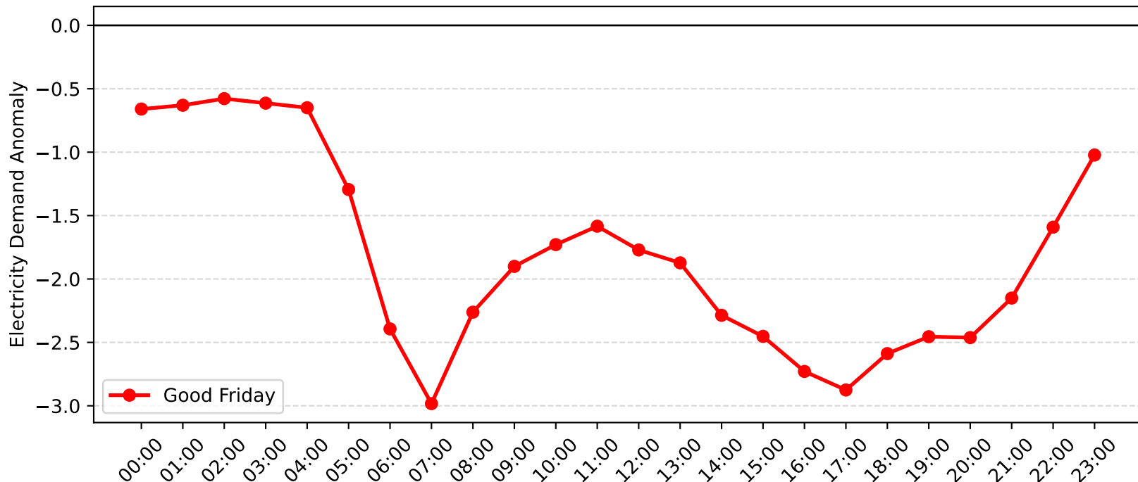
Blakehurst Demand Anomaly: Good Friday (2009-2010)
