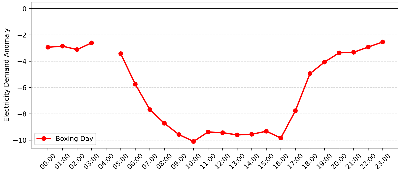
Macquarie Park Demand Anomaly: Boxing Day (2016-2017)
