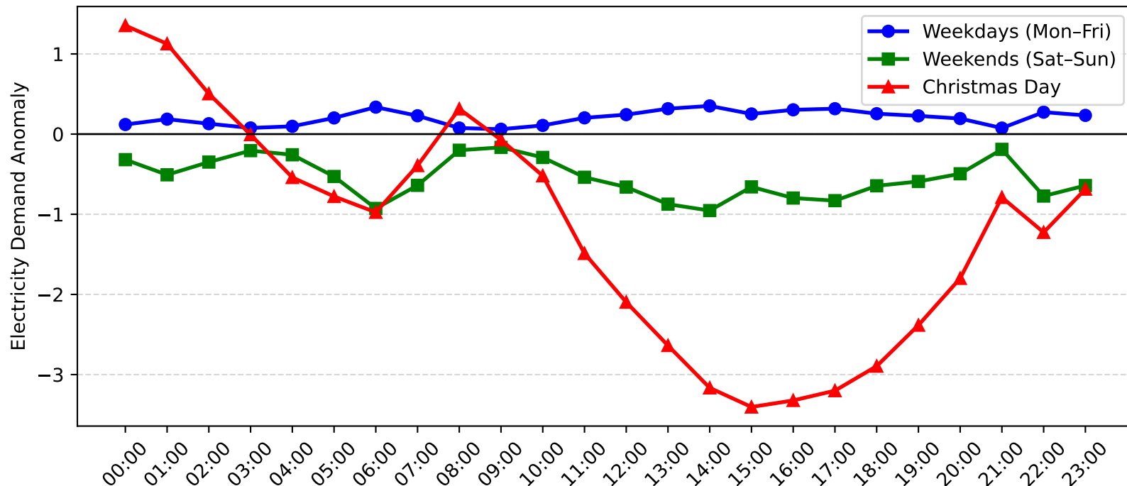
Morisset Demand Anomaly: Christmas Day vs Weekday/Weekend (2014-2015)
