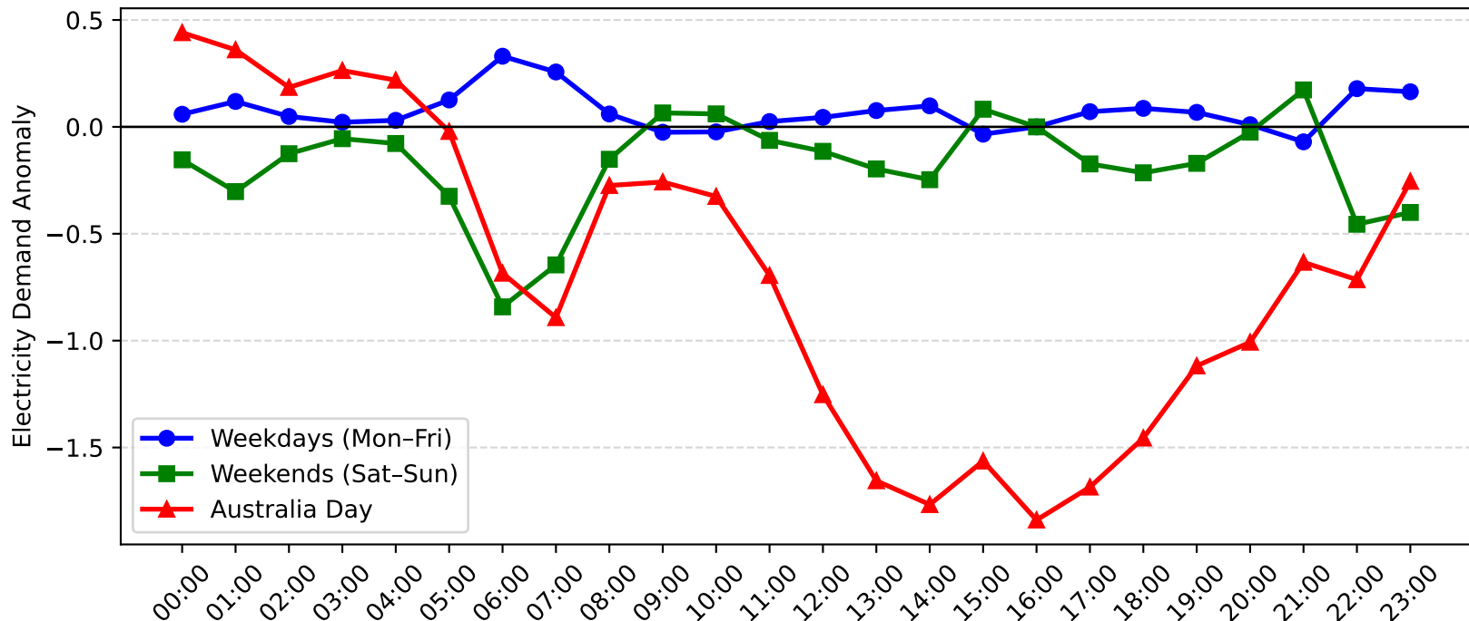
Morisset Demand Anomaly: Australia Day vs Weekday/Weekend (2015-2016)
