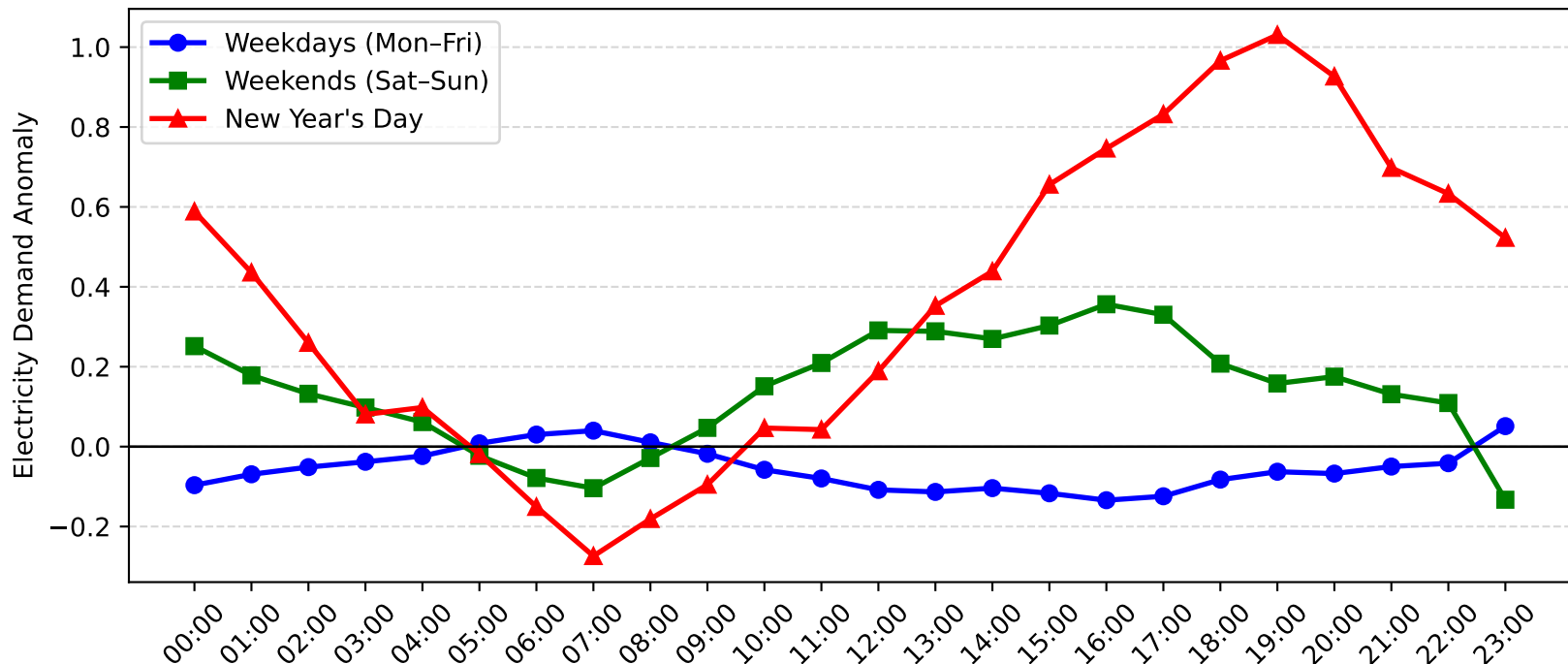
Rothbury Demand Anomaly: New Year's Day vs Weekday/Weekend (2013-2014)
