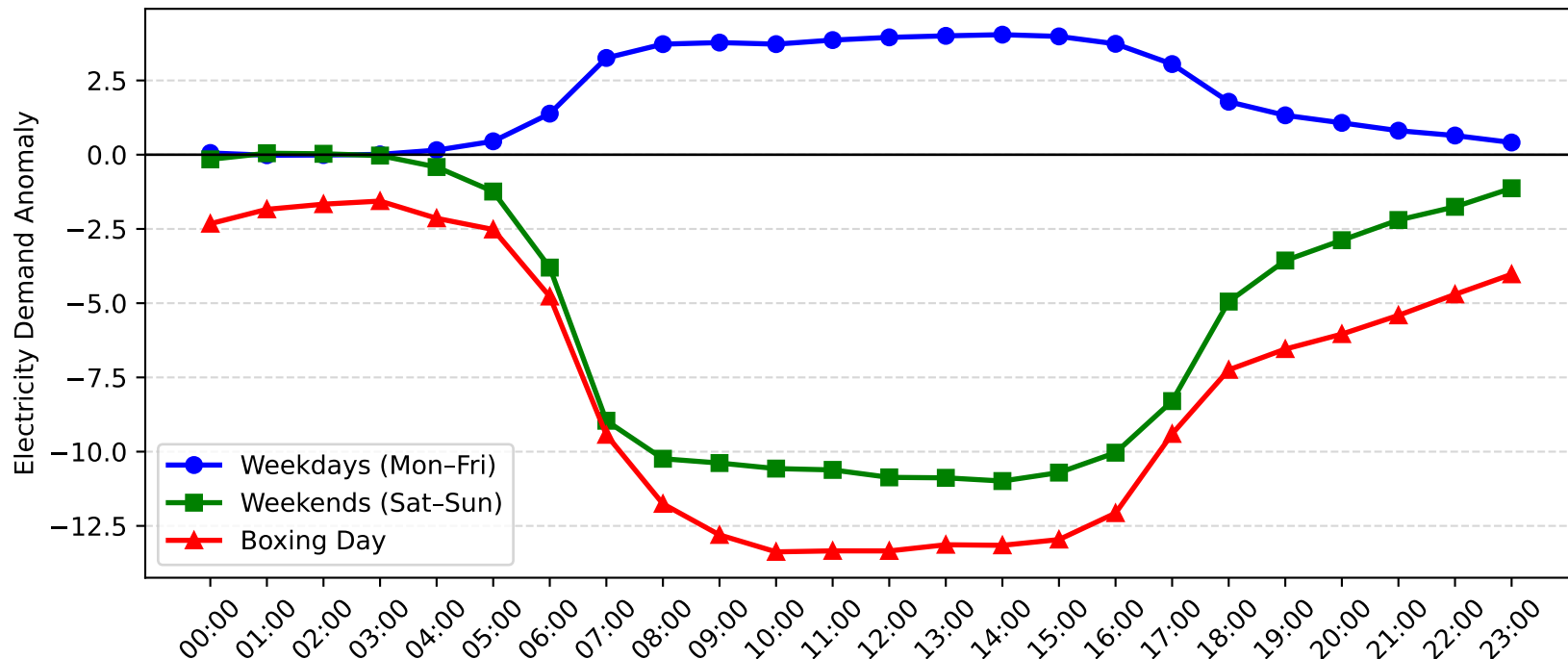
Gore Hill Demand Anomaly: Boxing Day vs Weekday/Weekend (2012-2013)
