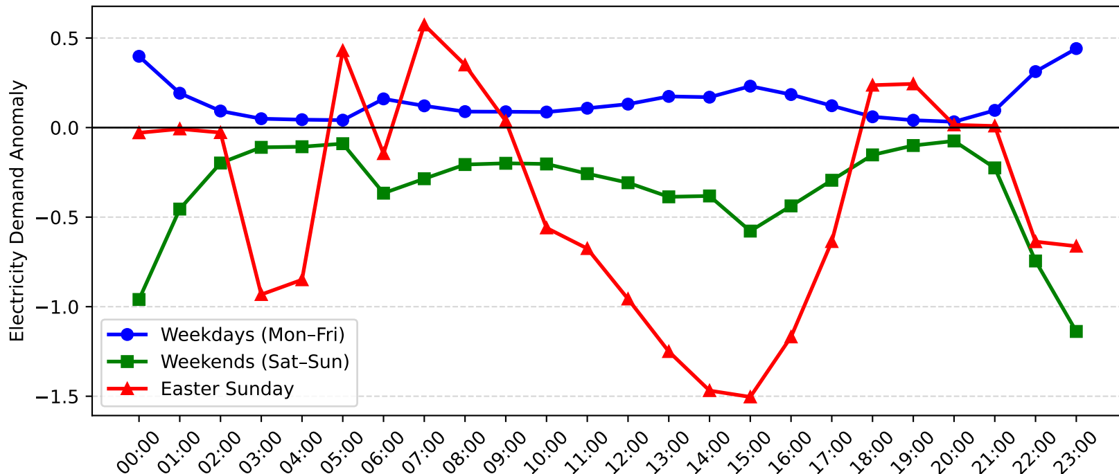
Muswellbrook Demand Anomaly: Easter Sunday vs Weekday/Weekend (2004-2005)
