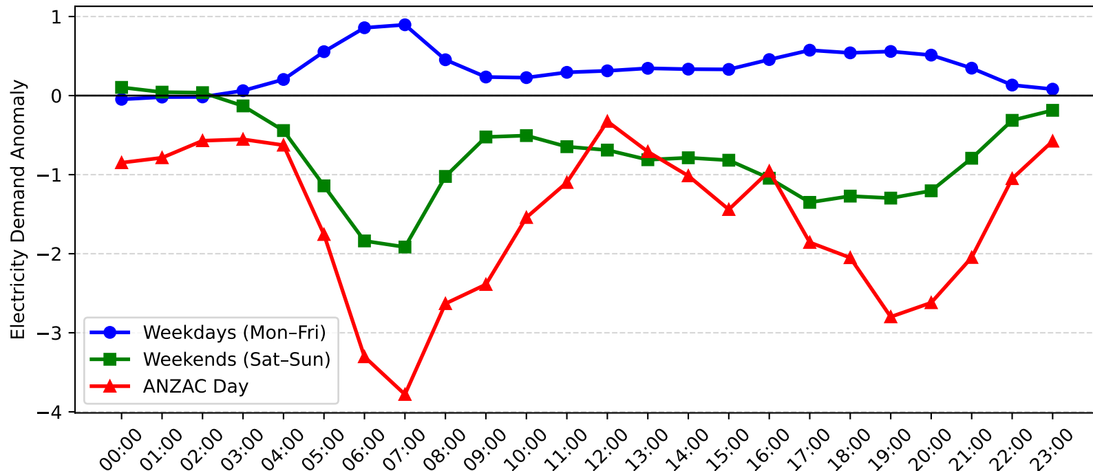
Charmhaven Demand Anomaly: ANZAC Day vs Weekday/Weekend (2010-2011)
