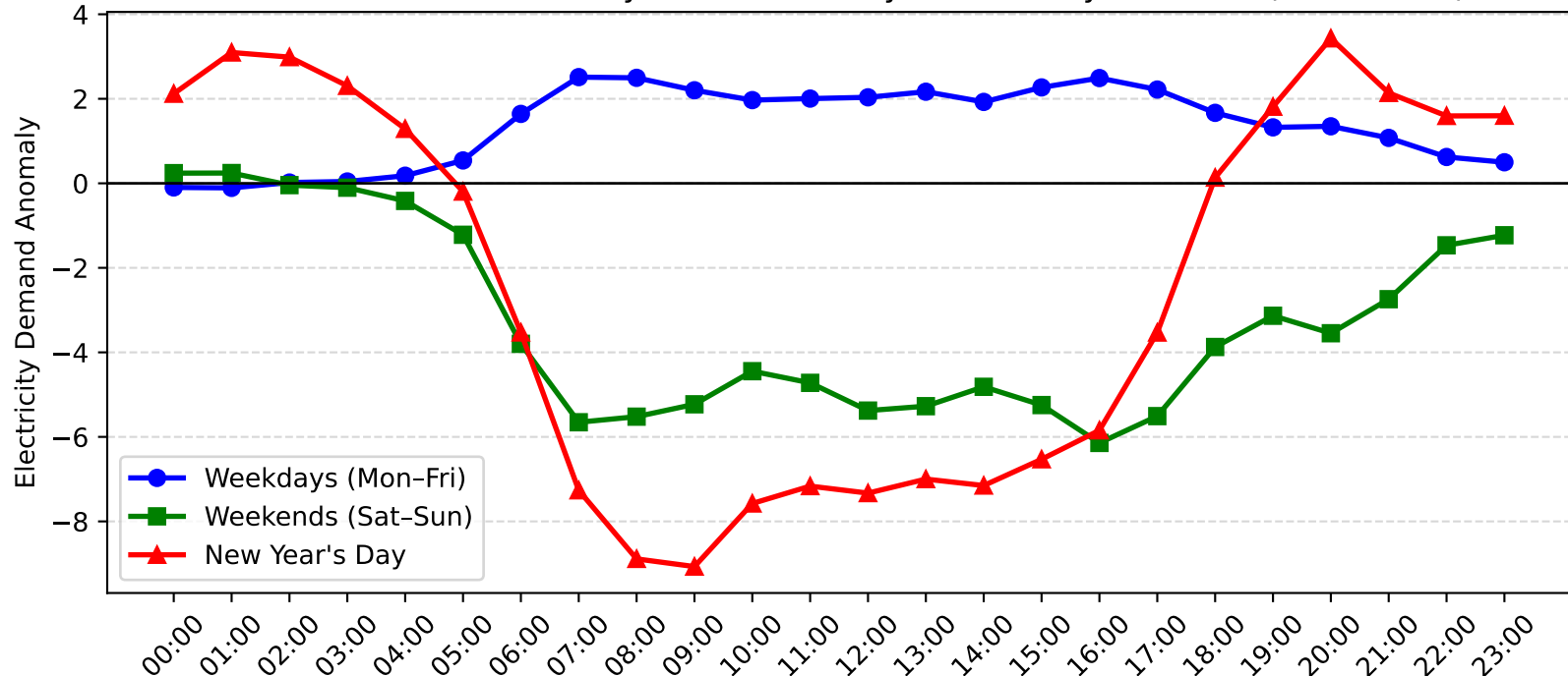
Burwood Demand Anomaly: New Year's Day vs Weekday/Weekend (2006-2007)
