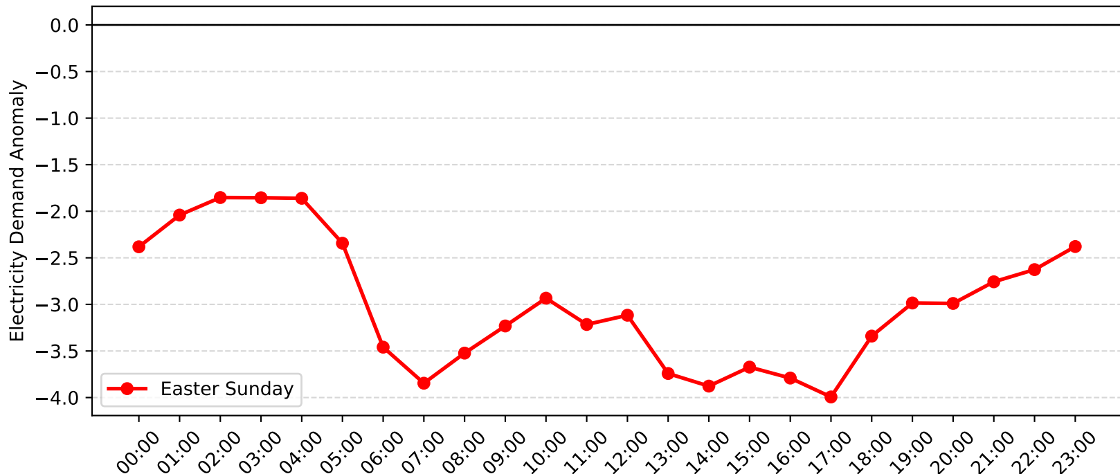
Bass Hill Demand Anomaly: Easter Sunday (2012-2013)
