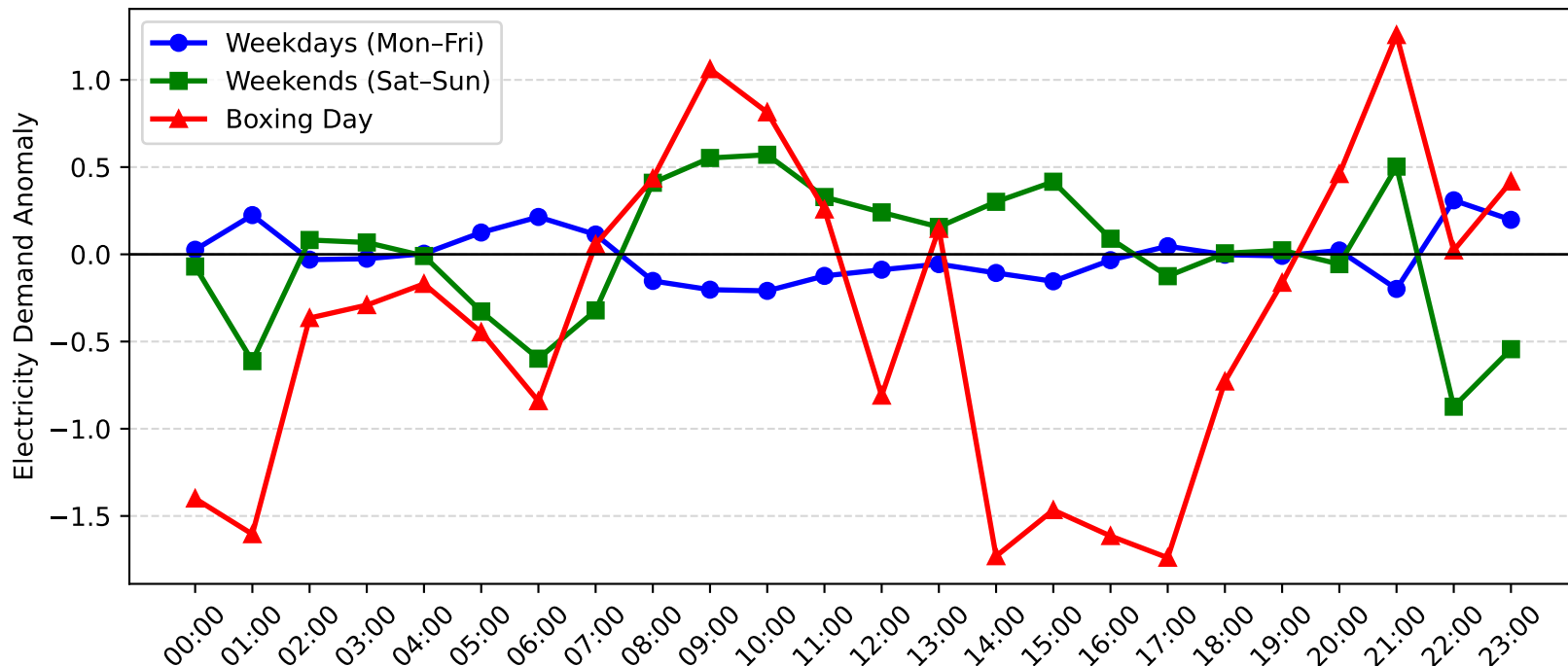
Nelson Bay Demand Anomaly: Boxing Day vs Weekday/Weekend (2013-2014)
