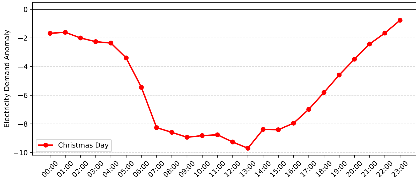
Hunters Hill Demand Anomaly: Christmas Day (2009-2010)
