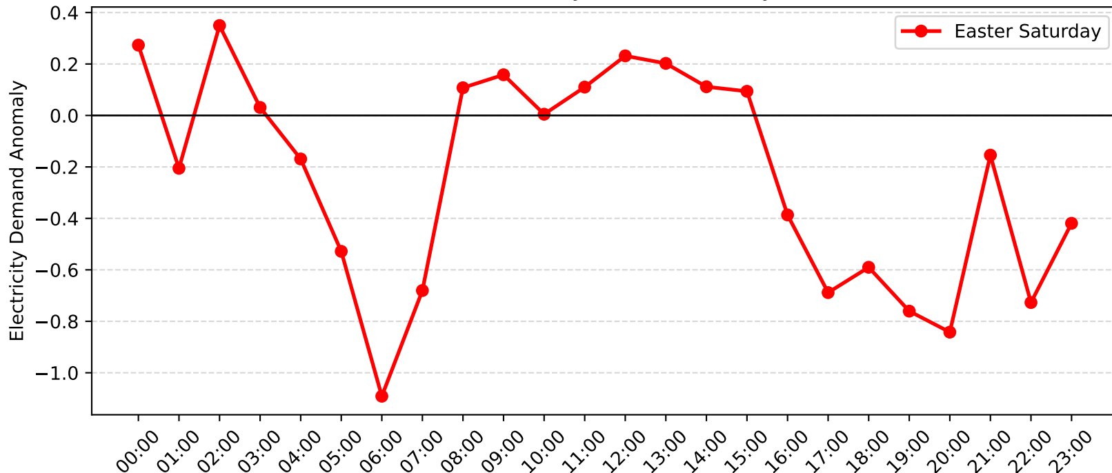
Morisset Demand Anomaly: Easter Saturday (2011-2012)
