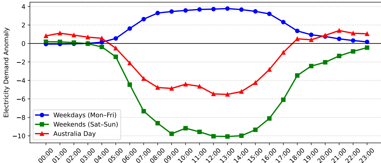
Mascot Demand Anomaly: Australia Day vs Weekday/Weekend (2010-2011)
