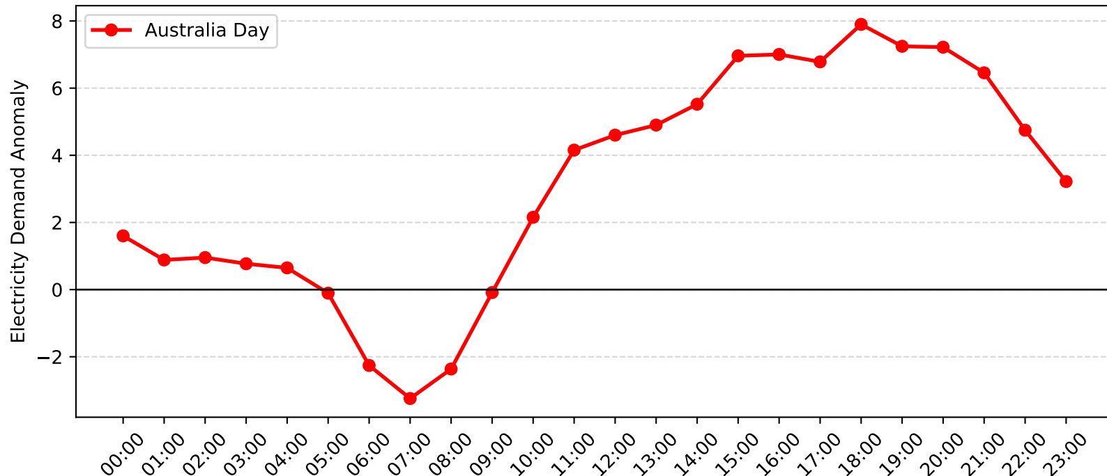
Epping Demand Anomaly: Australia Day (2010-2011)
