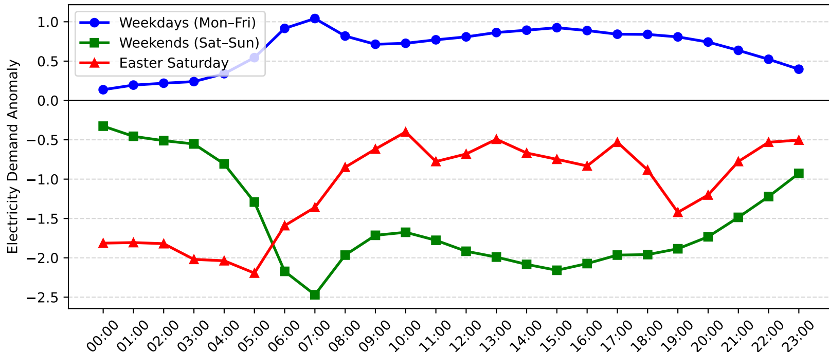
Enfield Demand Anomaly: Easter Saturday vs Weekday/Weekend (2011-2012)
