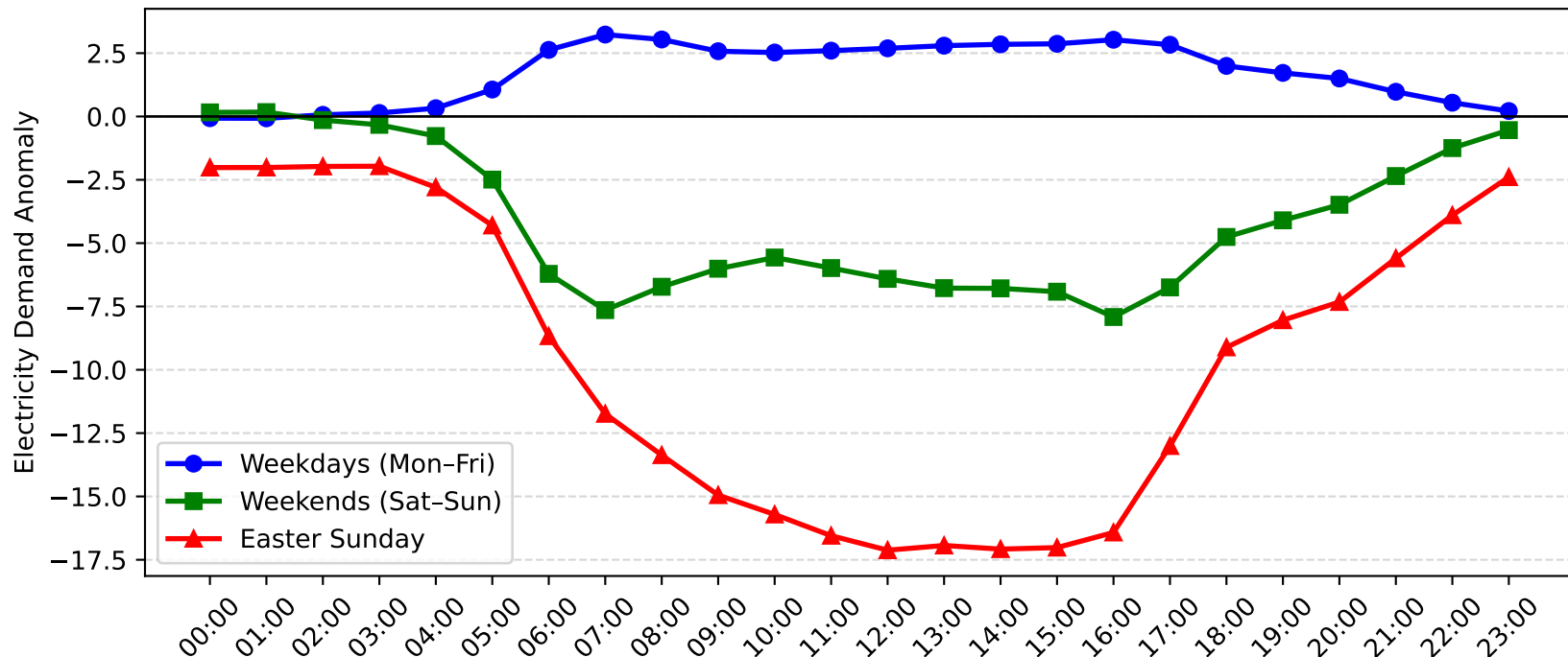
Epping Demand Anomaly: Easter Sunday vs Weekday/Weekend (2005-2006)
