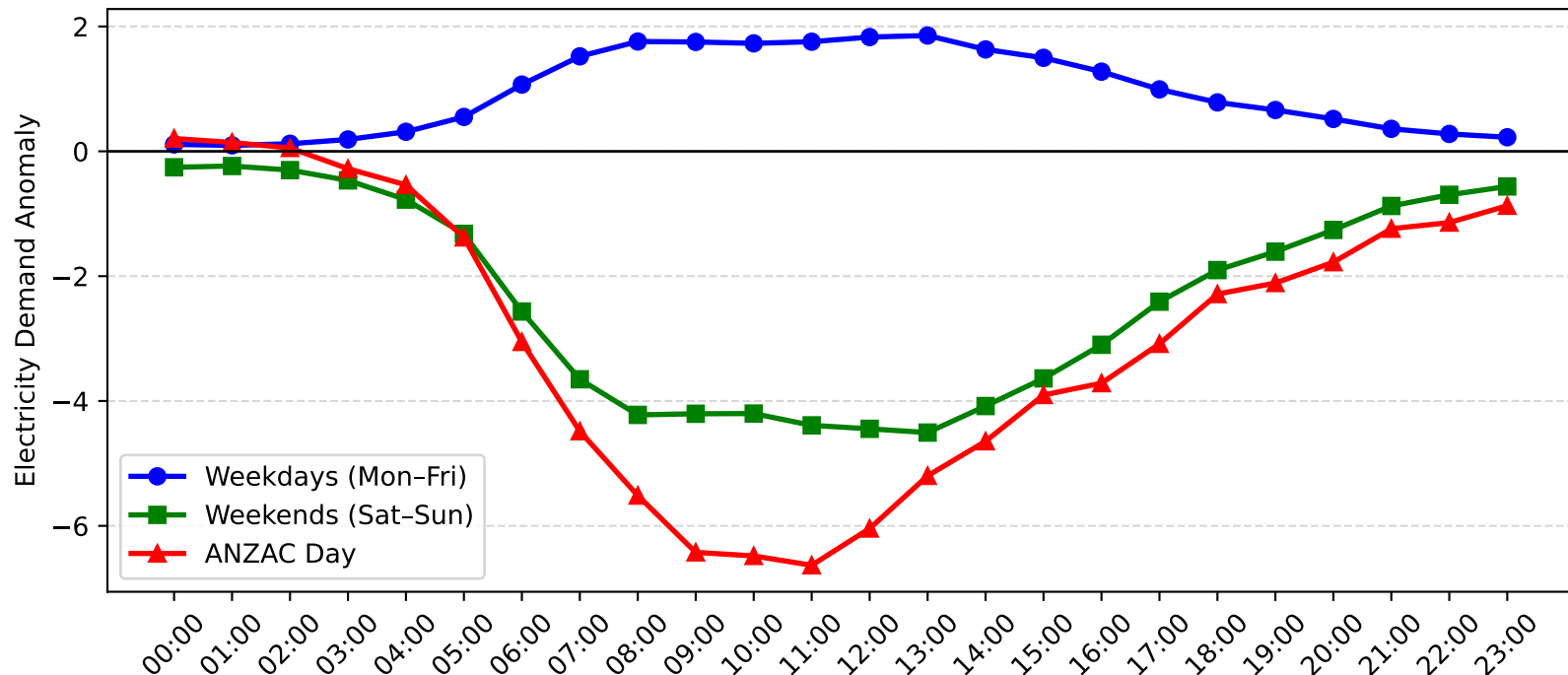
Auburn Demand Anomaly: ANZAC Day vs Weekday/Weekend (2014-2015)
