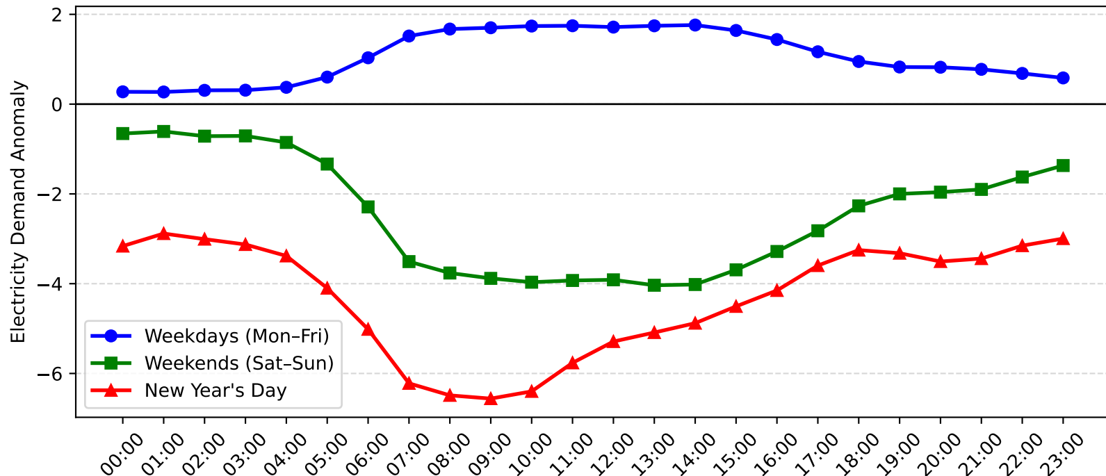
Leightonfield Demand Anomaly: New Year's Day vs Weekday/Weekend (2011-2012)
