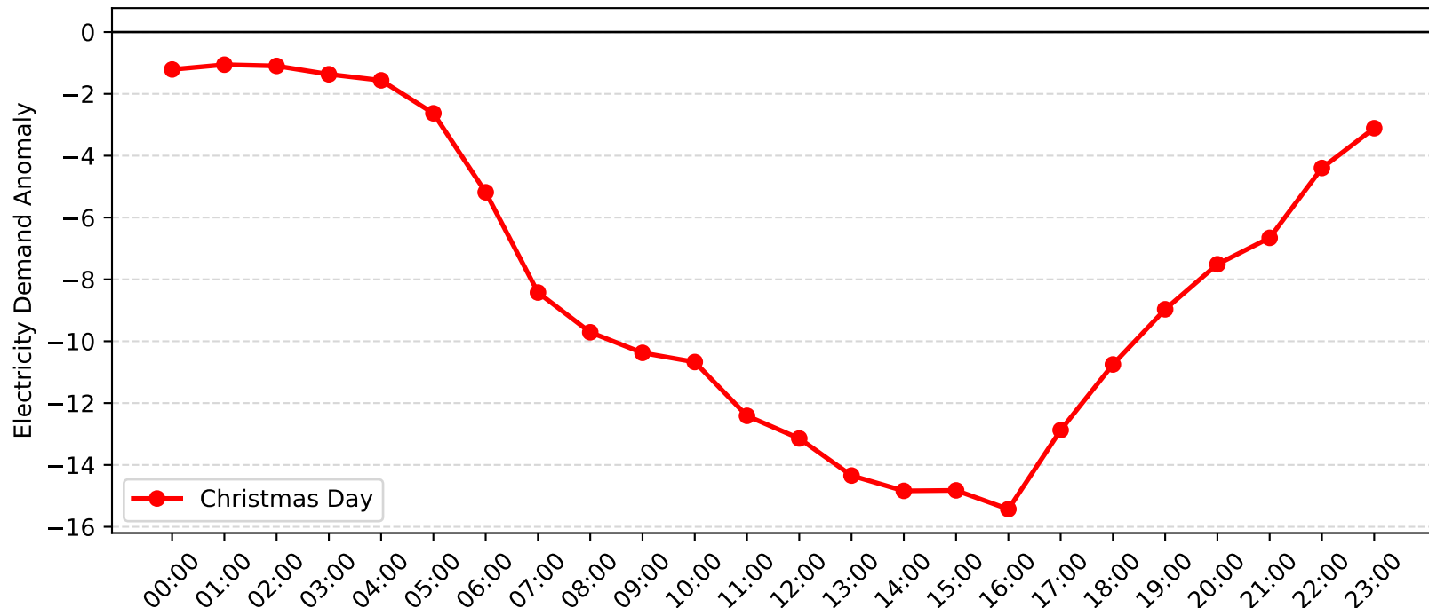
Epping Demand Anomaly: Christmas Day (2007-2008)
