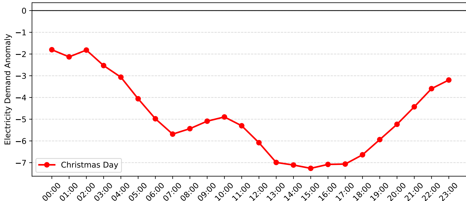
Matraverse Demand Anomaly: Christmas Day (2011-2012)
