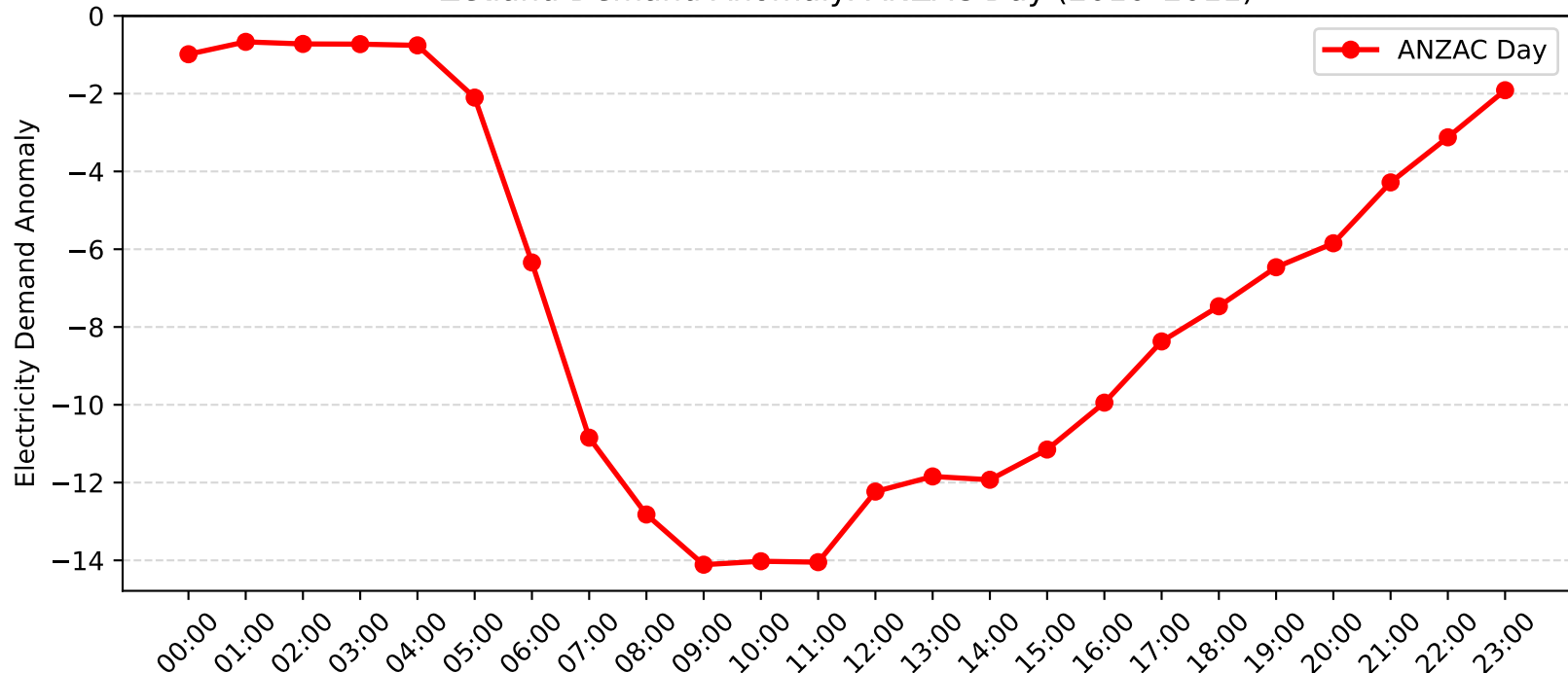
Zetland Demand Anomaly: ANZAC Day (2010-2011)
