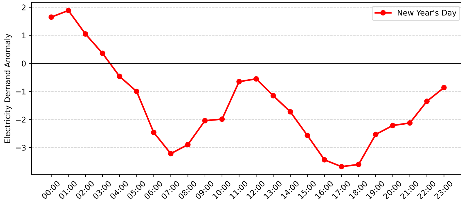
Mortdale Demand Anomaly: New Year's Day (2017-2018)
