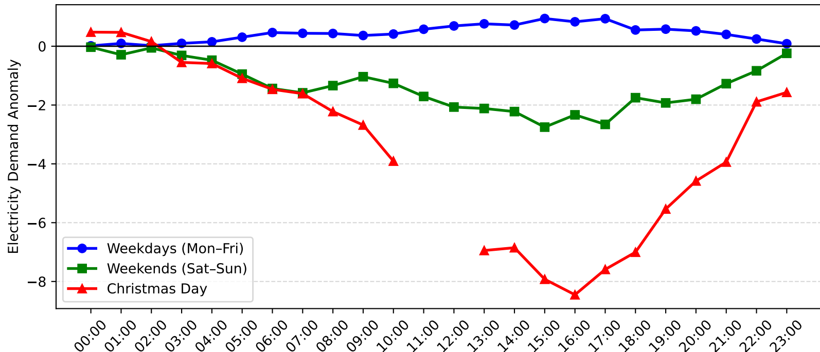
Charmhaven Demand Anomaly: Christmas Day vs Weekday/Weekend (2008-2009)
