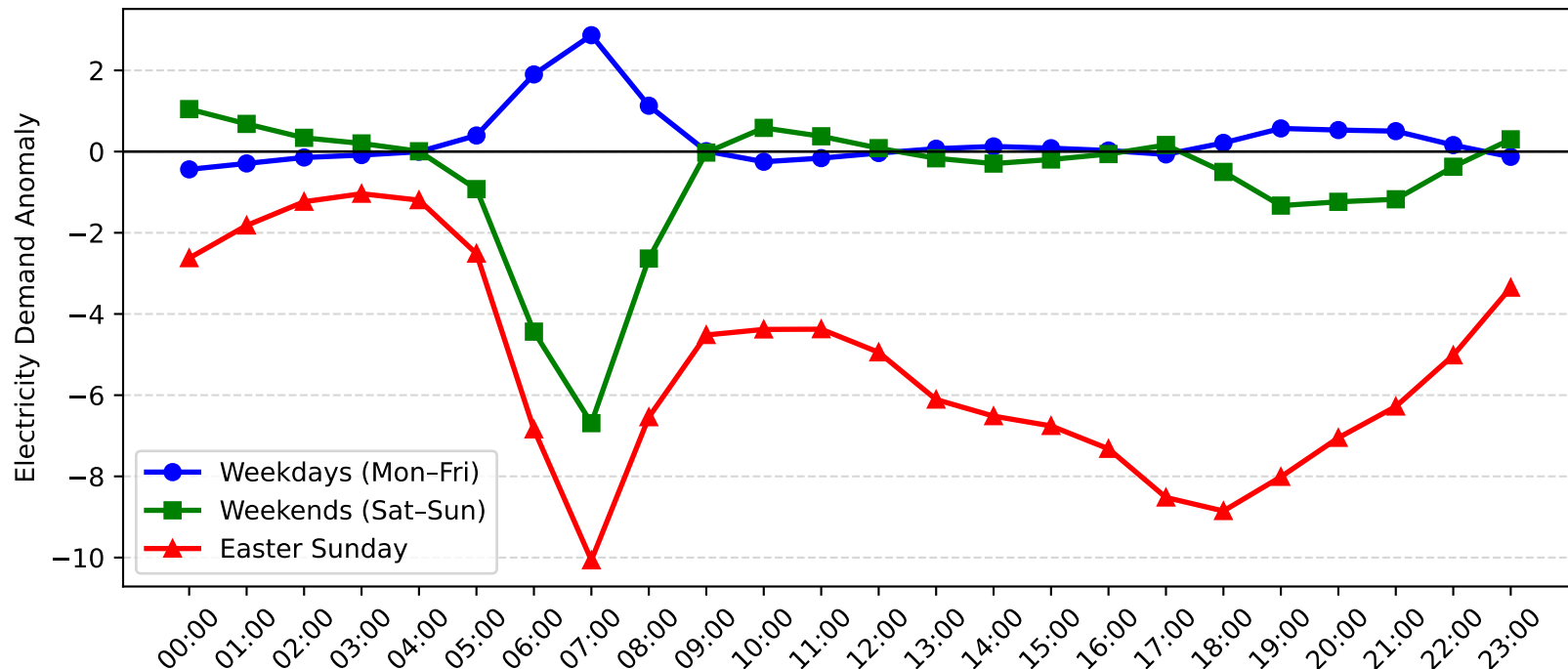
Mosman Demand Anomaly: Easter Sunday vs Weekday/Weekend (2013-2014)
