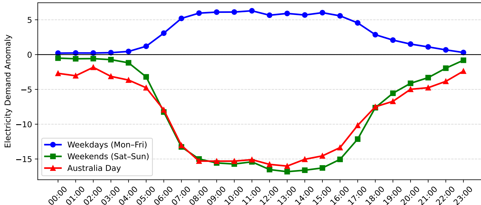
Gore Hill Demand Anomaly: Australia Day vs Weekday/Weekend (2006-2007)
