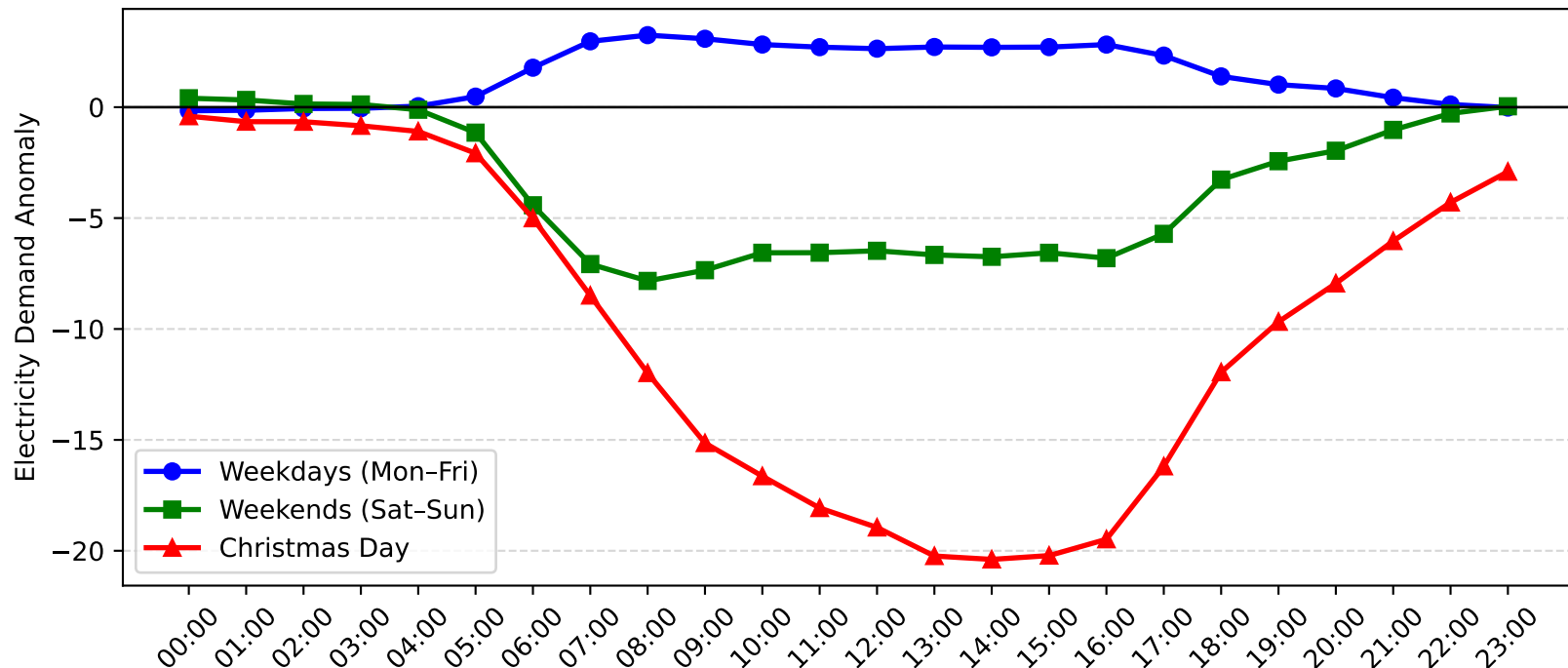
Castle Cove Demand Anomaly: Christmas Day vs Weekday/Weekend (2006-2007)
