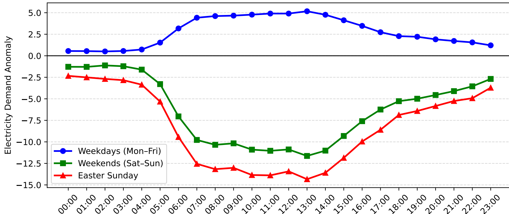
Milperra Demand Anomaly: Easter Sunday vs Weekday/Weekend (2009-2010)
