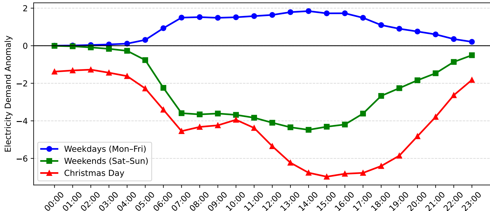
Hunters Hill Demand Anomaly: Christmas Day vs Weekday/Weekend (2015-2016)
