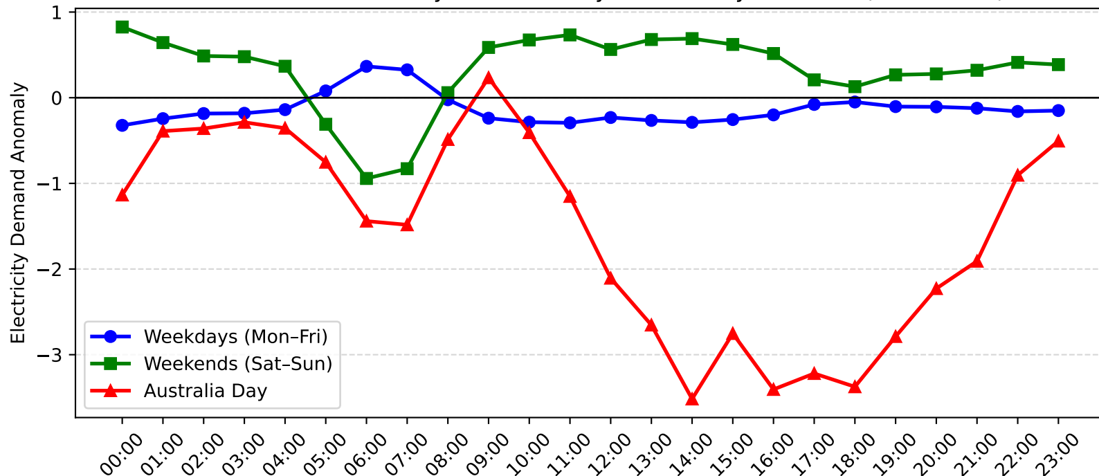
Avoca Demand Anomaly: Australia Day vs Weekday/Weekend (2016-2017)
