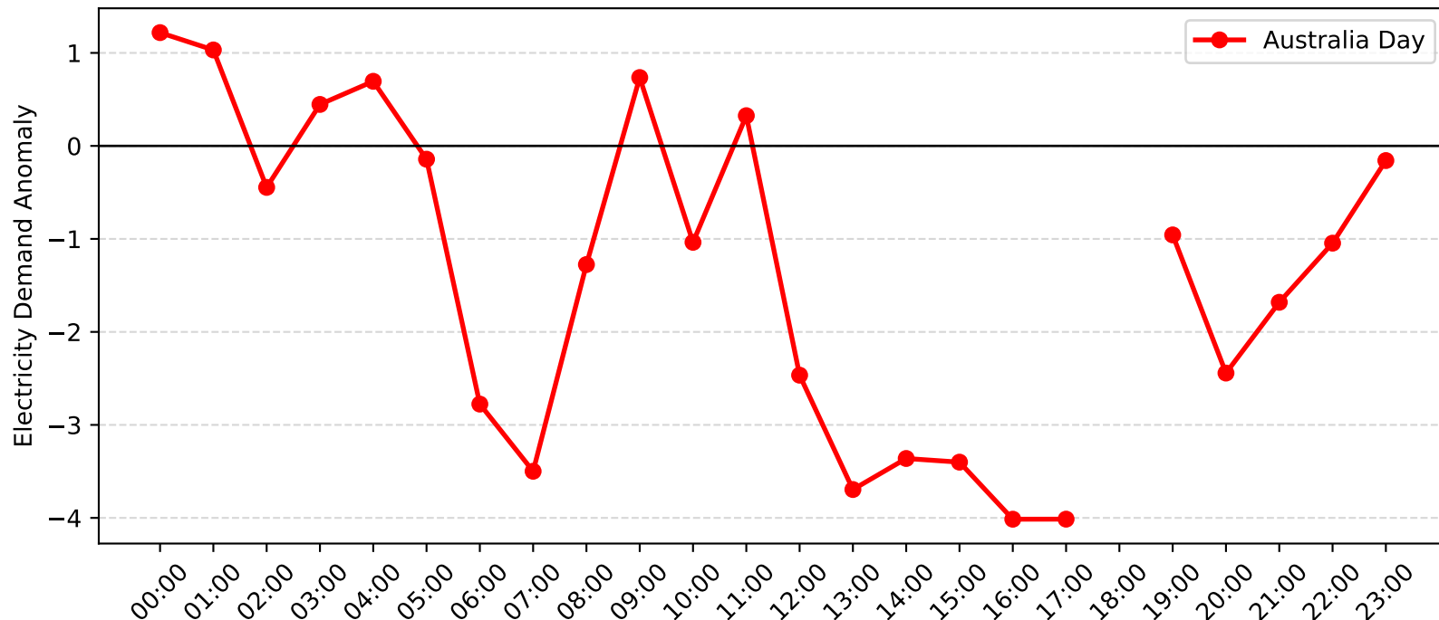
Chatswood Demand Anomaly: Australia Day (2005-2006)
