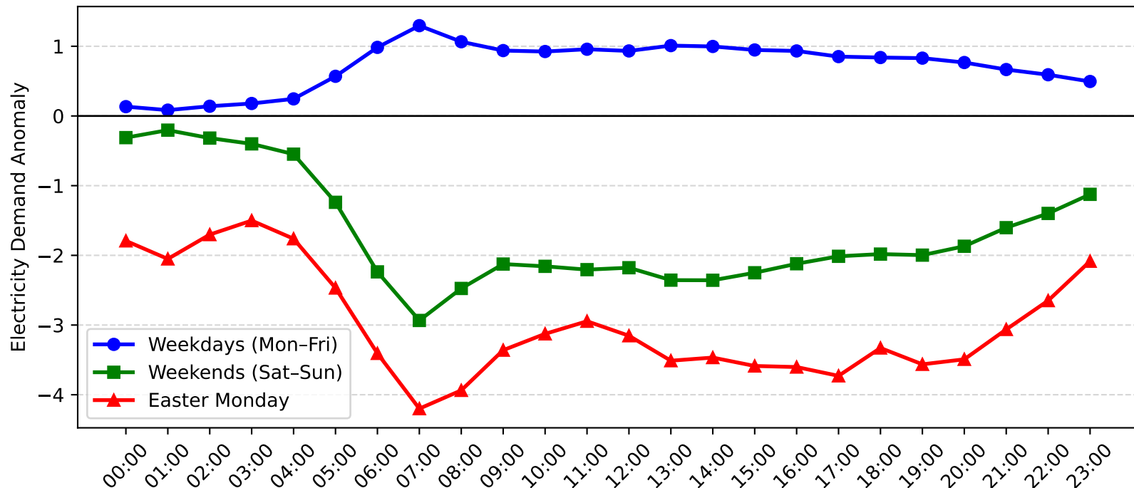
Bass Hill Demand Anomaly: Easter Monday vs Weekday/Weekend (2010-2011)
