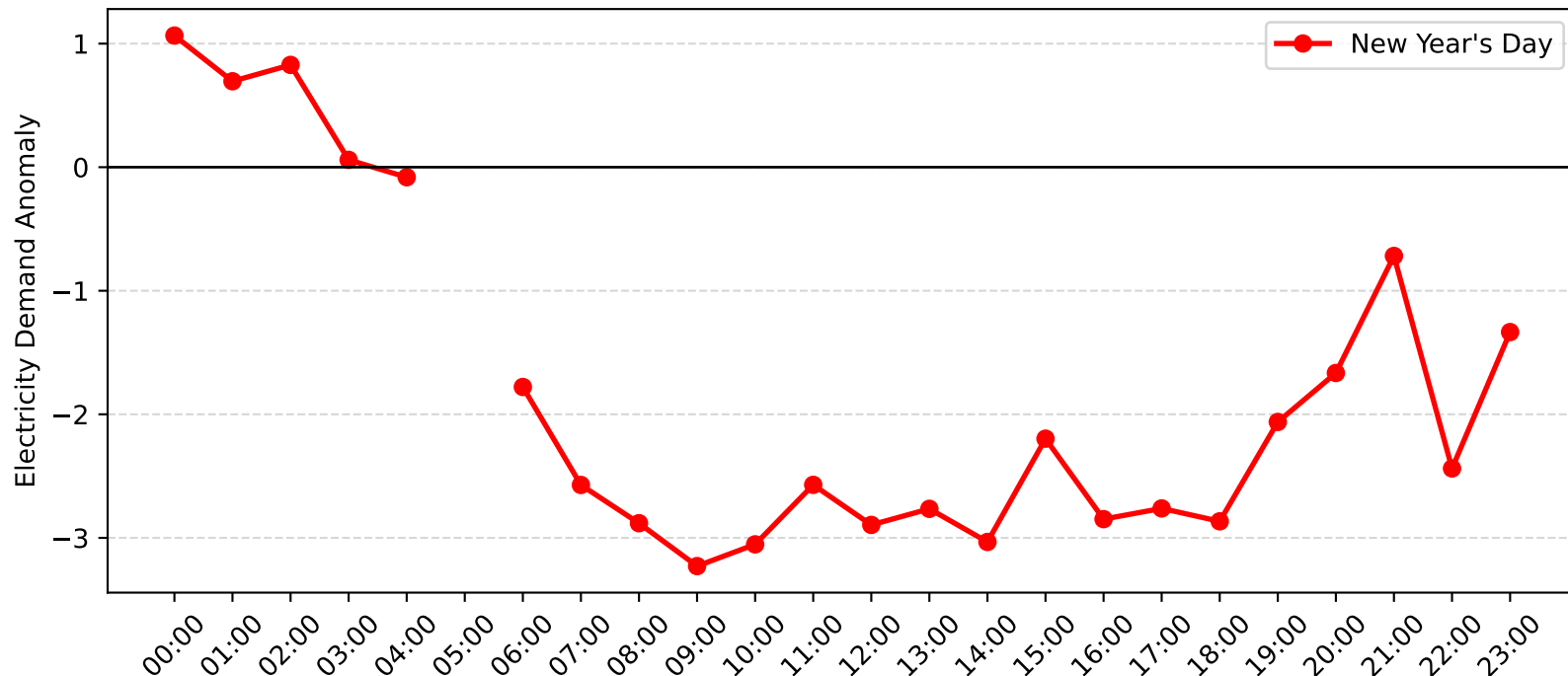
Charlestown Demand Anomaly: New Year's Day (2014-2015)
