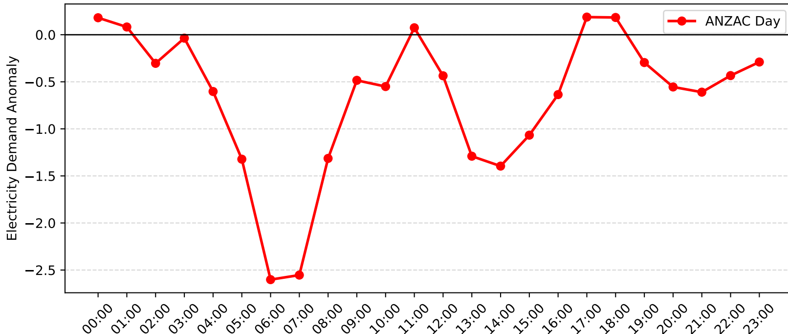
Charmhaven Demand Anomaly: ANZAC Day (2006-2007)
