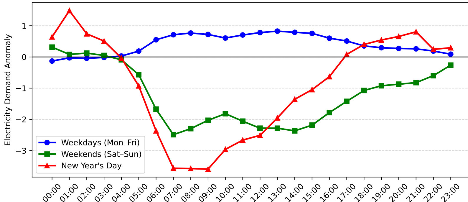
Arnccliffe Demand Anomaly: New Year's Day vs Weekday/Weekend (2009-2010)
