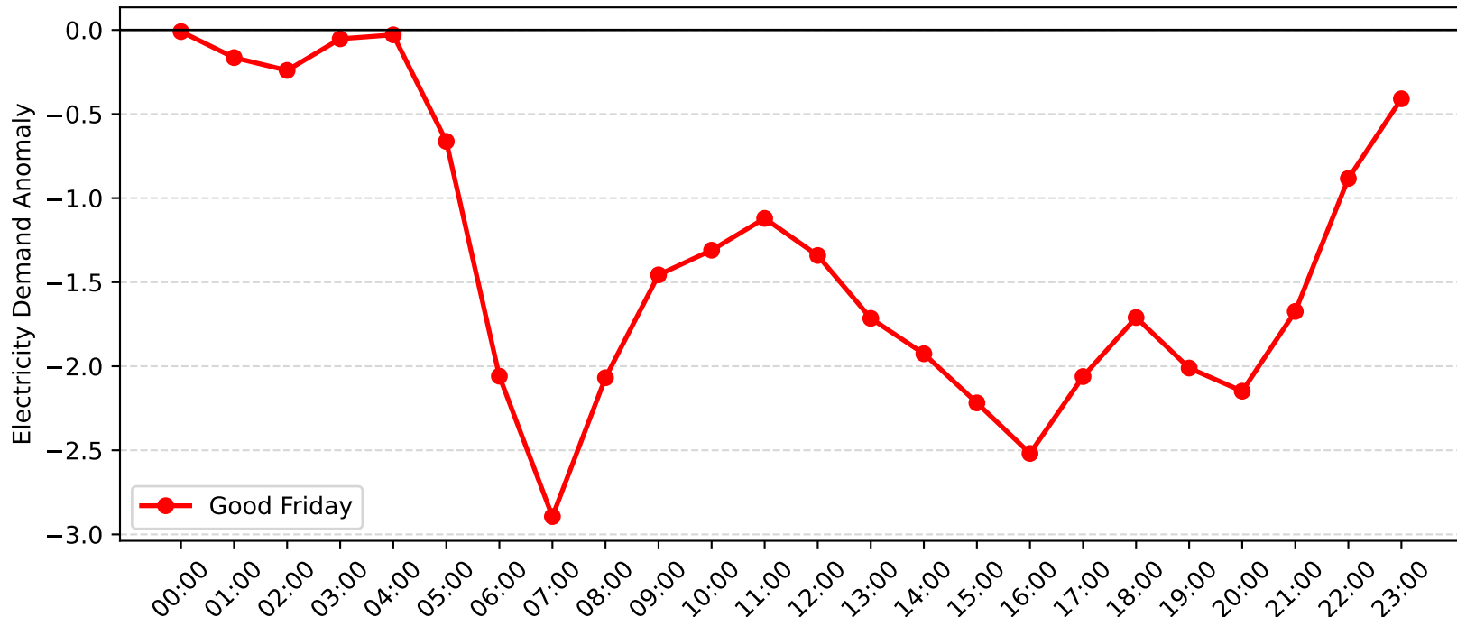
Blakehurst Demand Anomaly: Good Friday (2006-2007)
