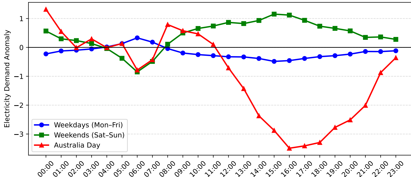
Umina Demand Anomaly: Australia Day vs Weekday/Weekend (2014-2015)
