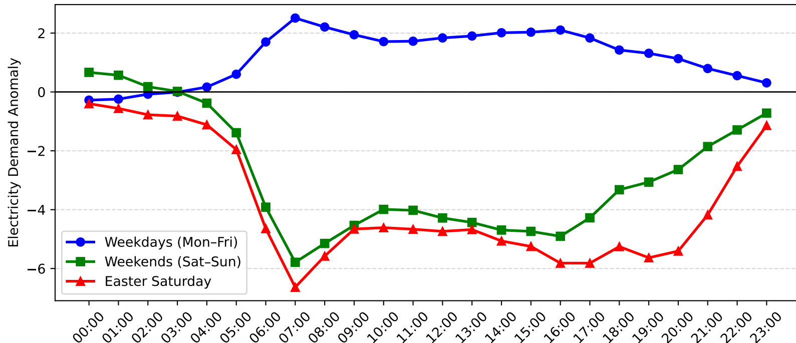
Burwood Demand Anomaly: Easter Saturday vs Weekday/Weekend (2011-2012)
