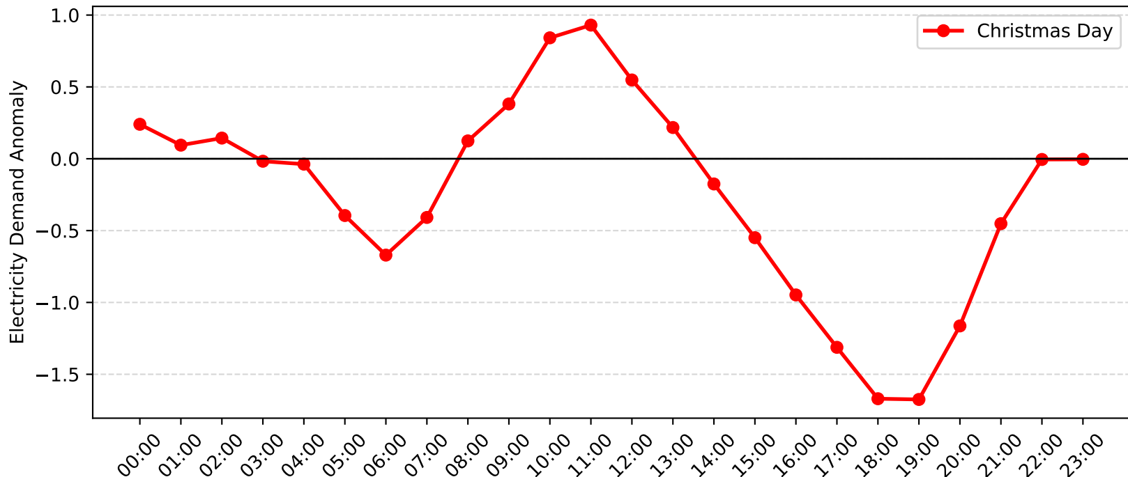
Harbord Demand Anomaly: Christmas Day (2016-2017)
