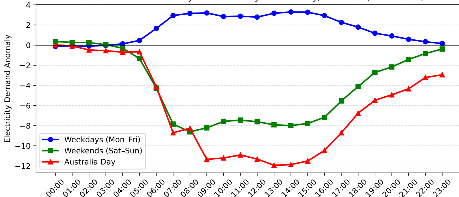
Zetland Demand Anomaly: Australia Day vs Weekday/Weekend (2014-2015)
