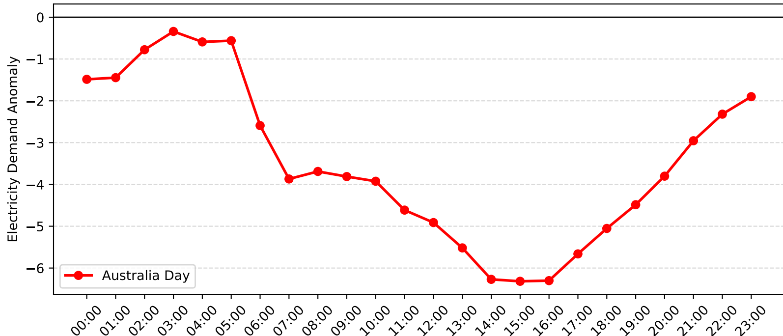
Argenton Demand Anomaly: Australia Day (2014-2015)
