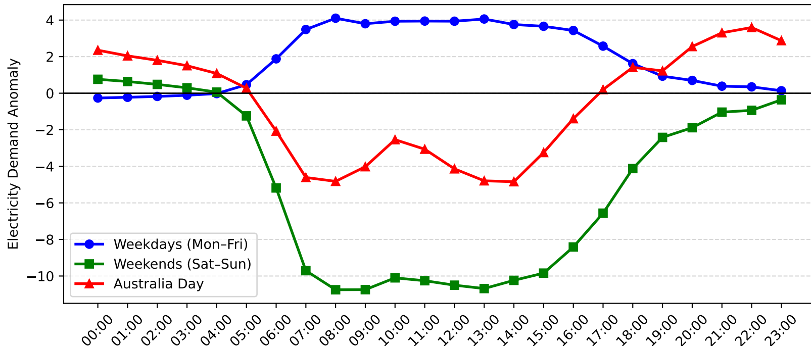
Zetland Demand Anomaly: Australia Day vs Weekday/Weekend (2010-2011)
