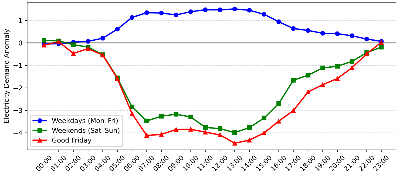
Wyong Demand Anomaly: Good Friday vs Weekday/Weekend (2005-2006)
