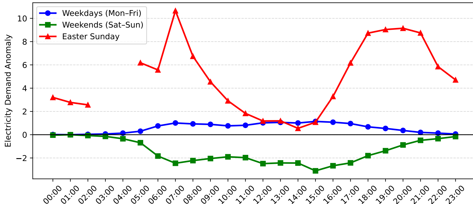
Epping Demand Anomaly: Easter Sunday vs Weekday/Weekend (2004-2005)
