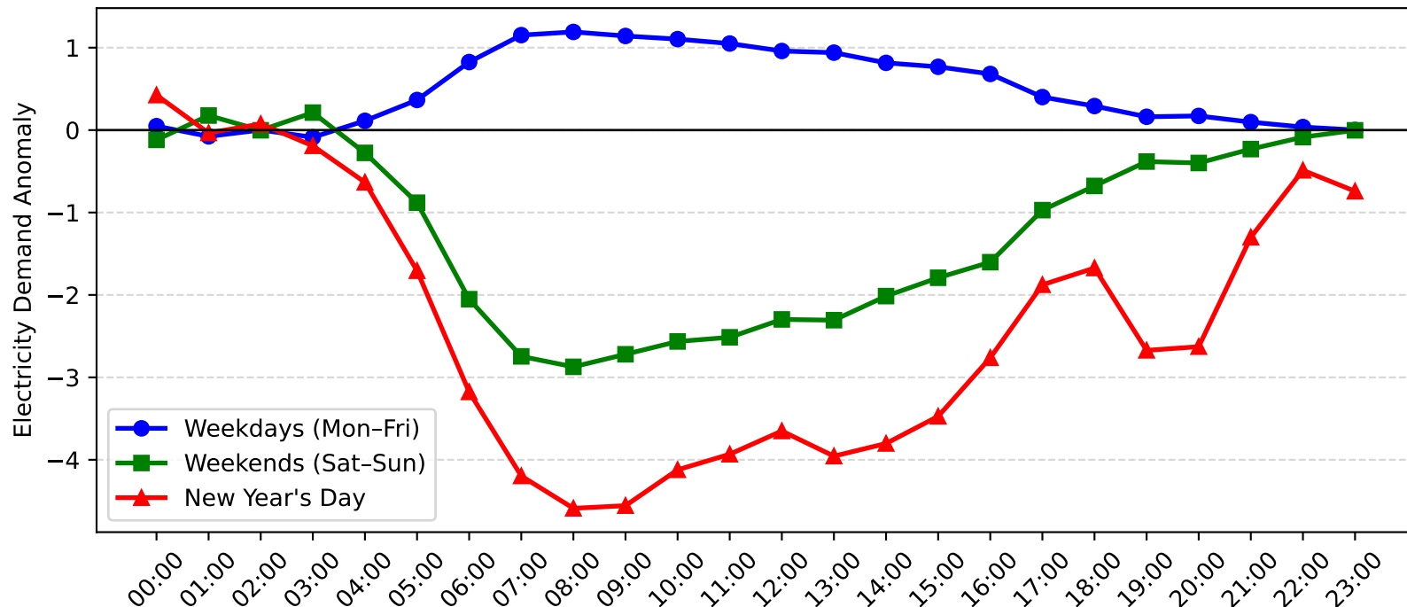
Wyong Demand Anomaly: New Year's Day vs Weekday/Weekend (2007-2008)
