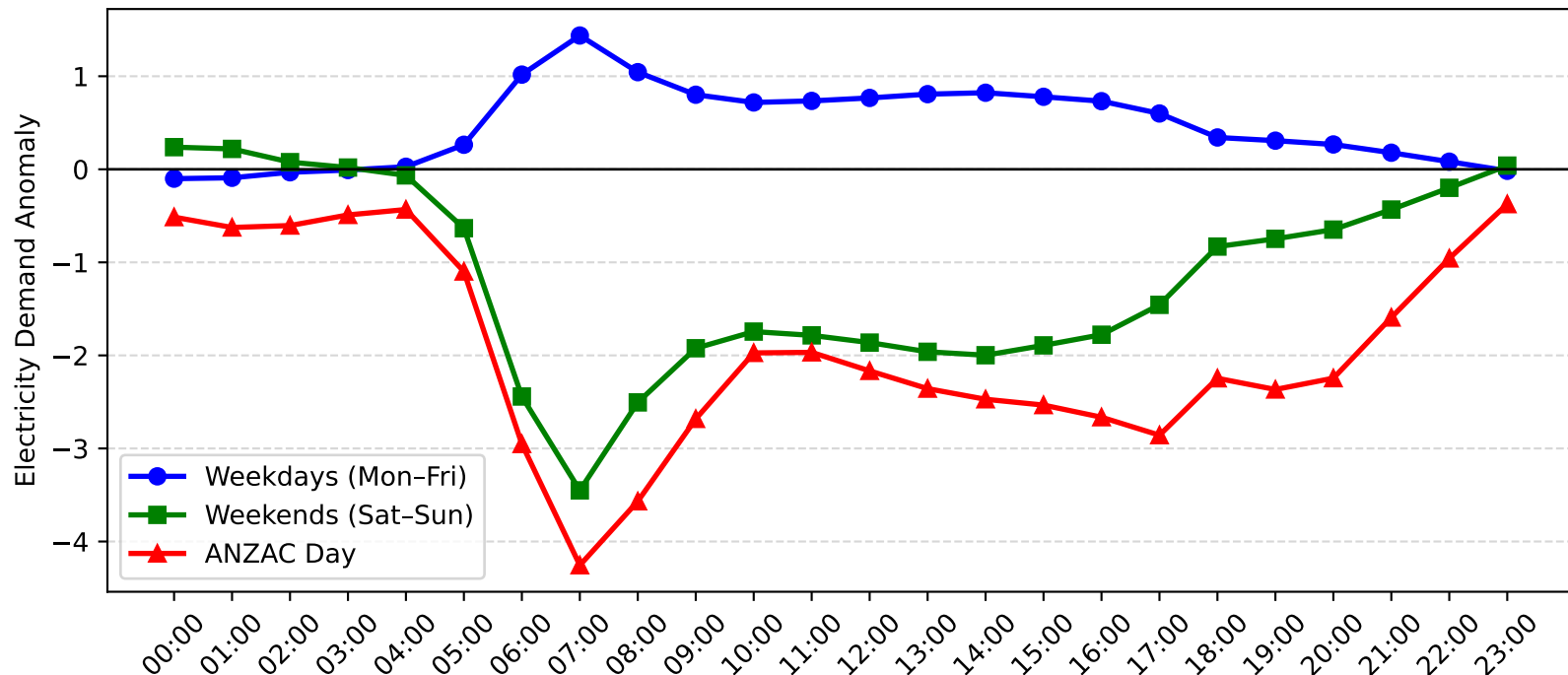
Pymble Demand Anomaly: ANZAC Day vs Weekday/Weekend (2014-2015)
