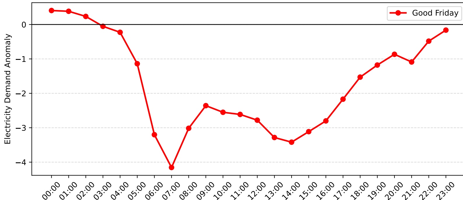
Arncliffe Demand Anomaly: Good Friday (2004-2005)
