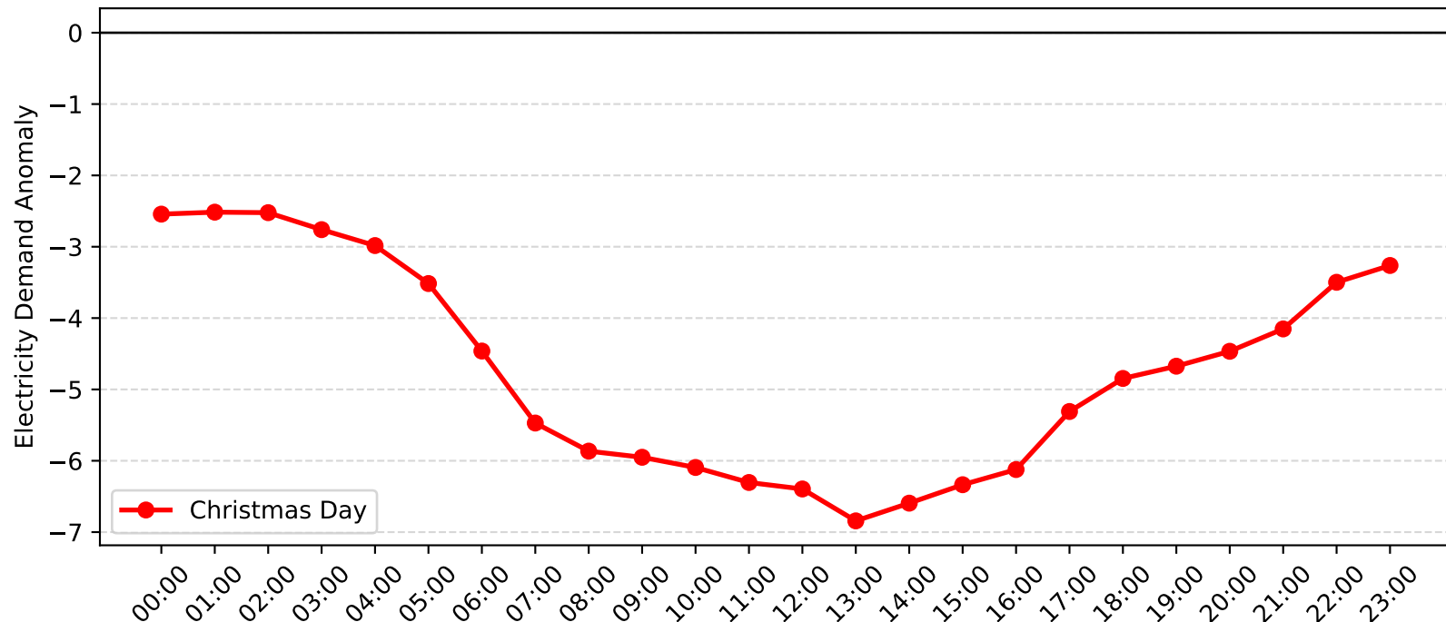
Leightonfield Demand Anomaly: Christmas Day (2011-2012)
