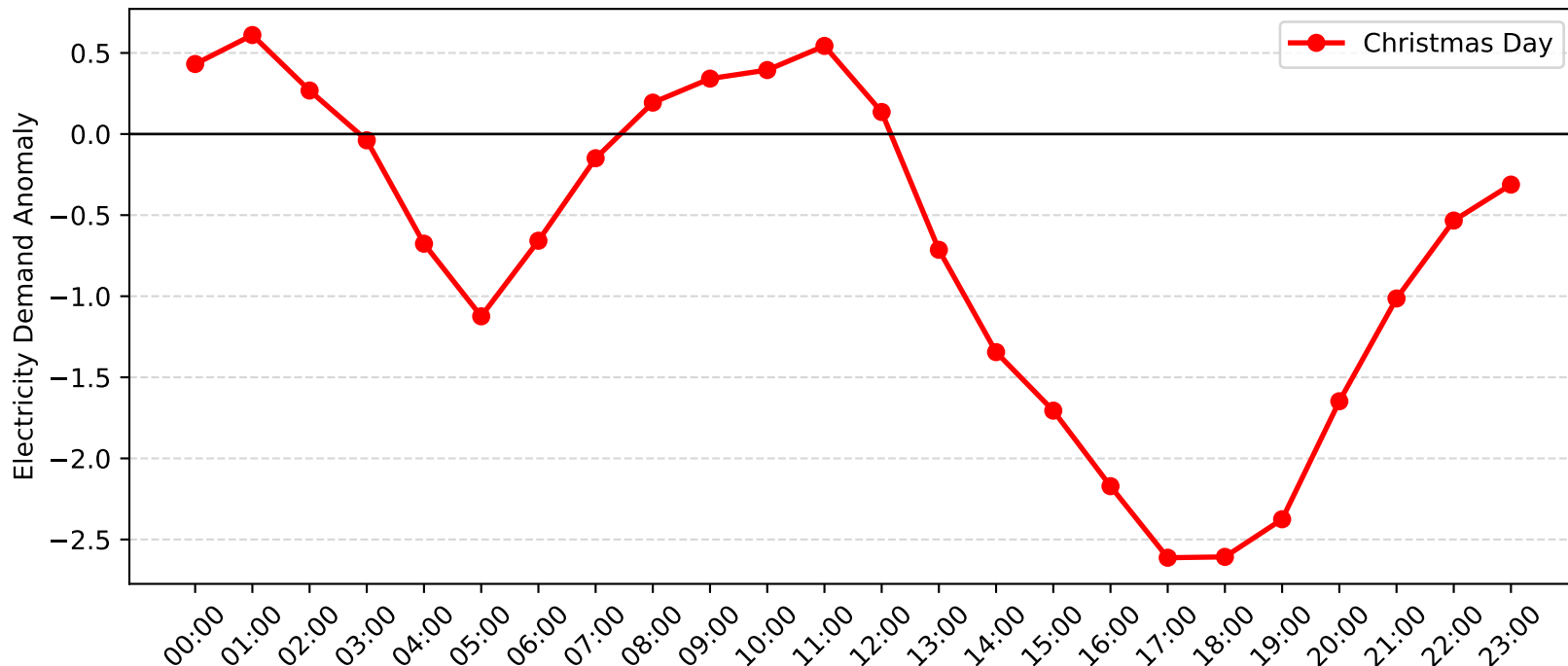
Umina Demand Anomaly: Christmas Day (2016-2017)
