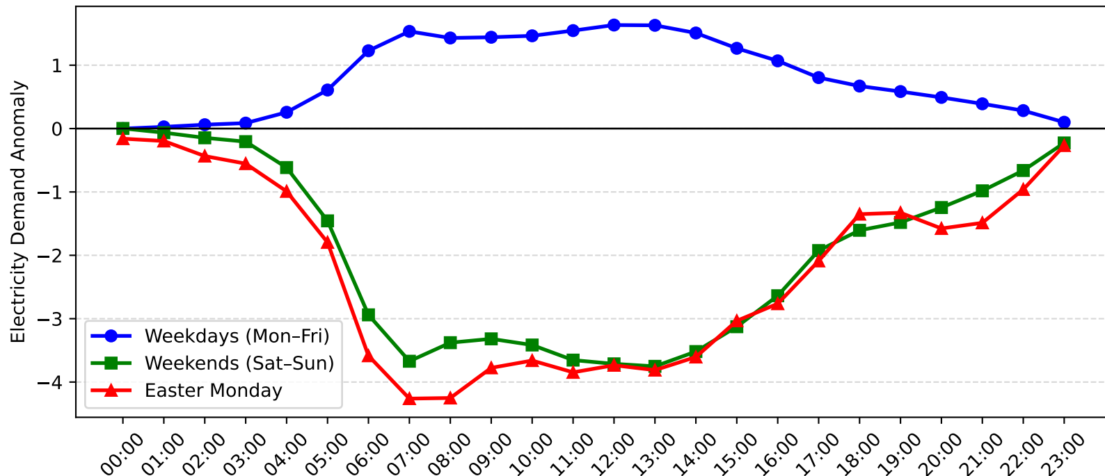
Wyong Demand Anomaly: Easter Monday vs Weekday/Weekend (2007-2008)
