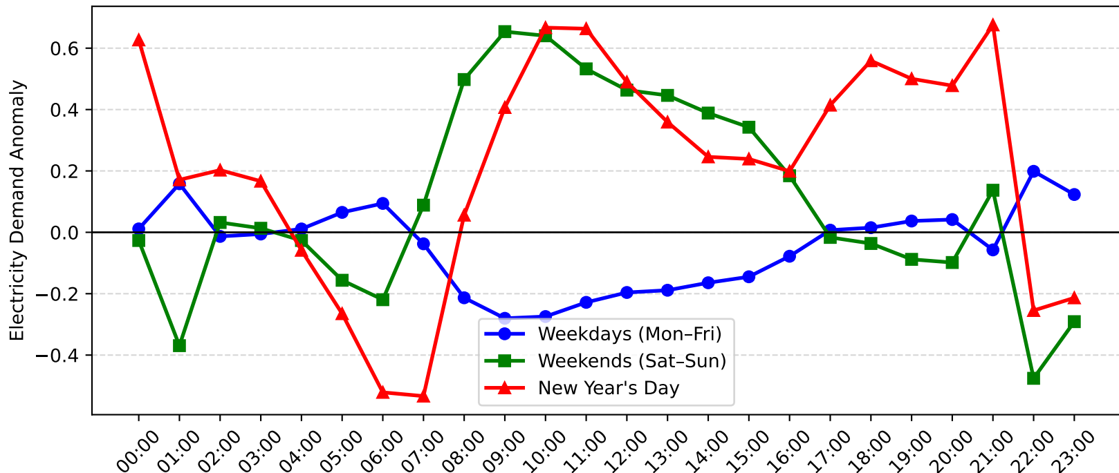
Swansea Demand Anomaly: New Year's Day vs Weekday/Weekend (2012-2013)
