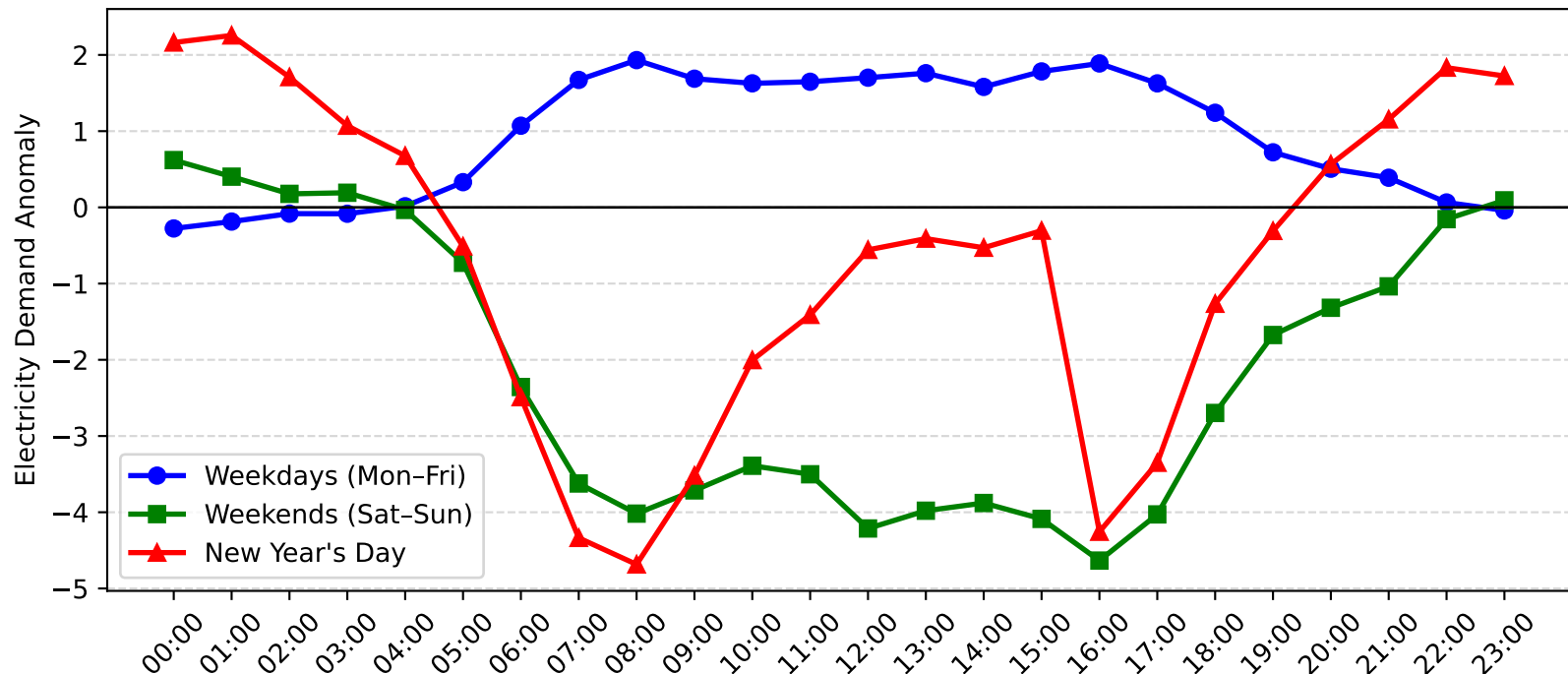
Pymble Demand Anomaly: New Year's Day vs Weekday/Weekend (2005-2006)
