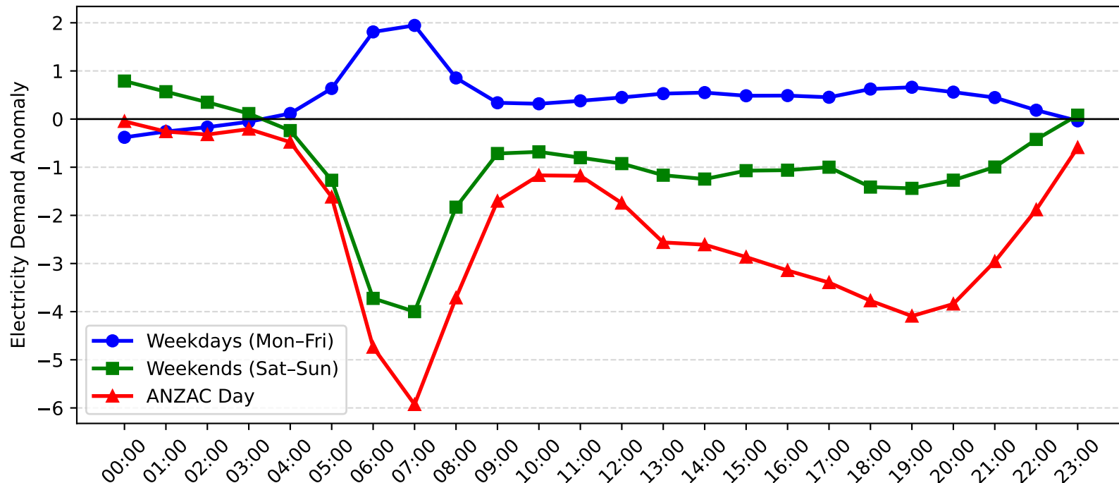
Mortdale Demand Anomaly: ANZAC Day vs Weekday/Weekend (2009-2010)
