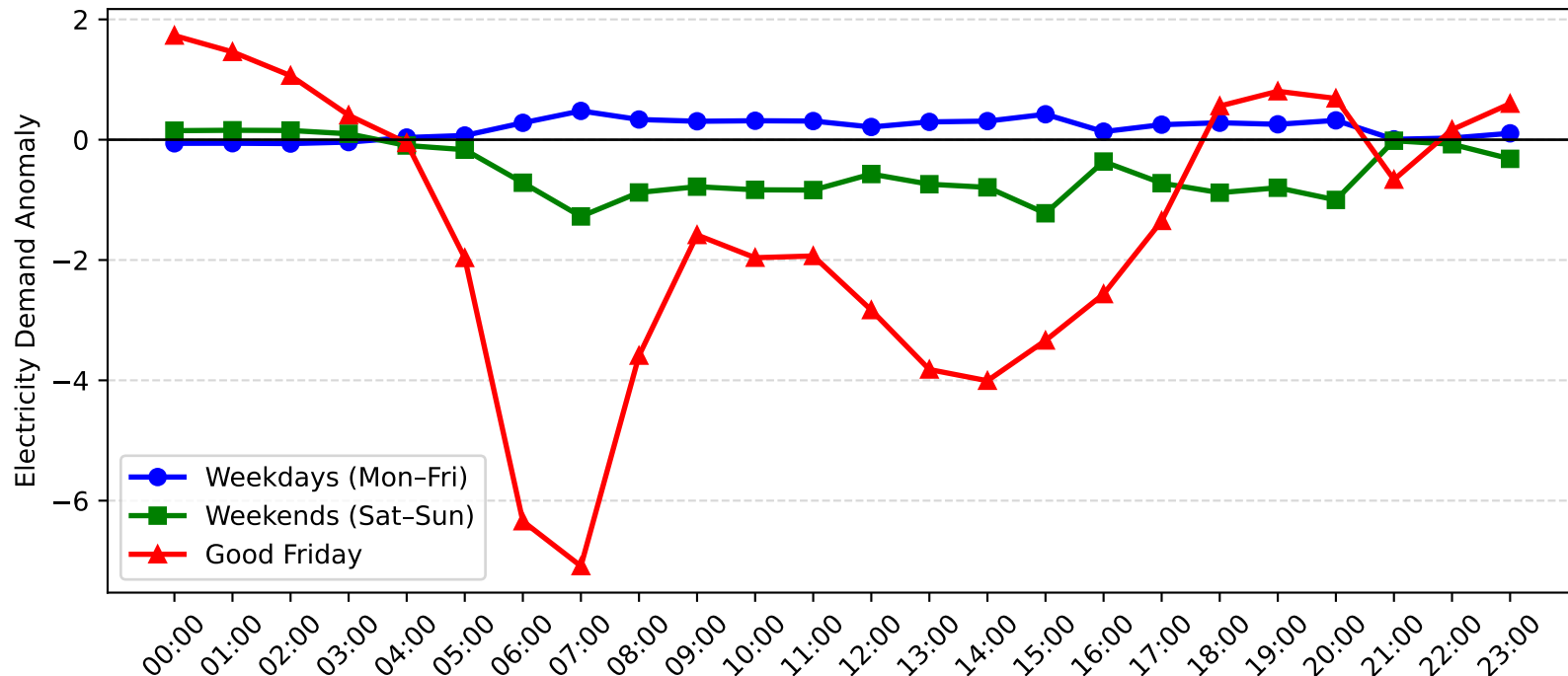
Mortdale Demand Anomaly: Good Friday vs Weekday/Weekend (2004-2005)
