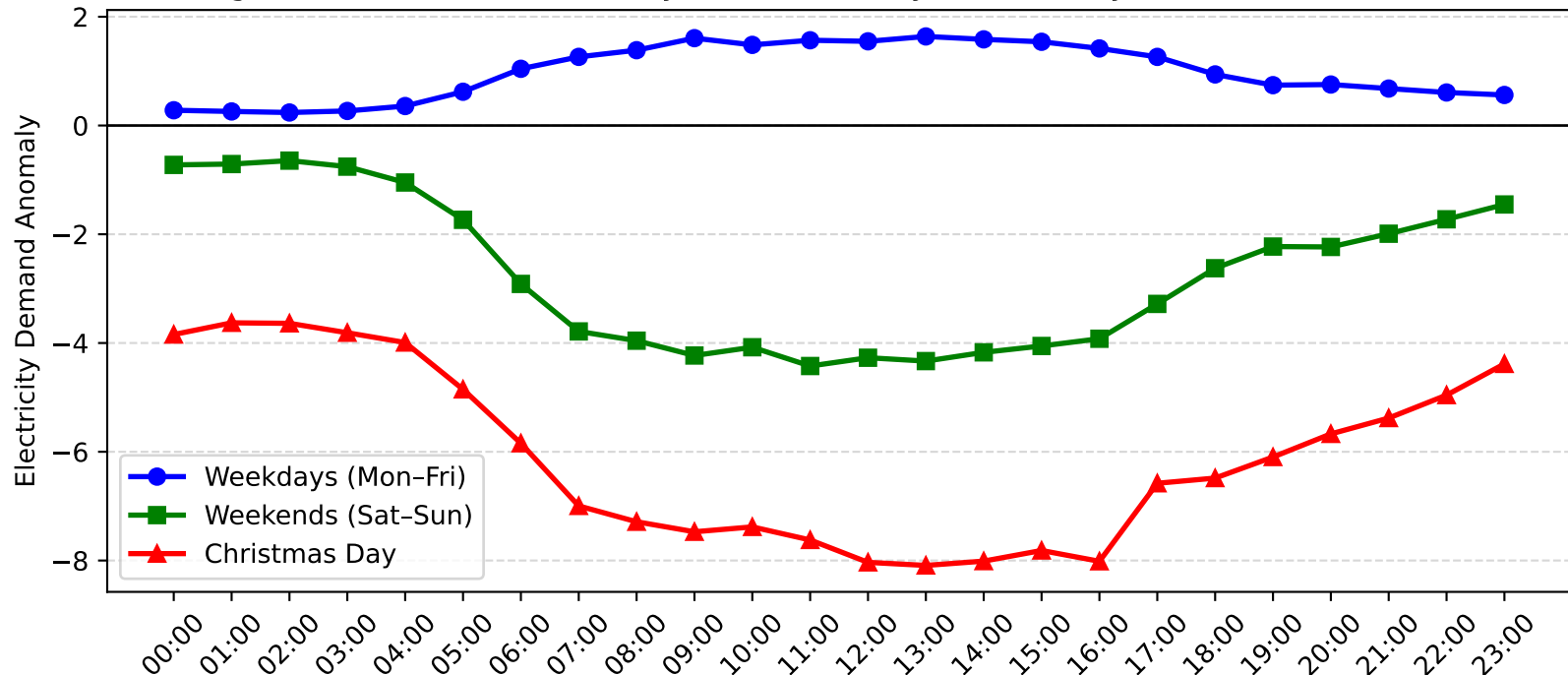
Leightonfield Demand Anomaly: Christmas Day vs Weekday/Weekend (2007-2008)
