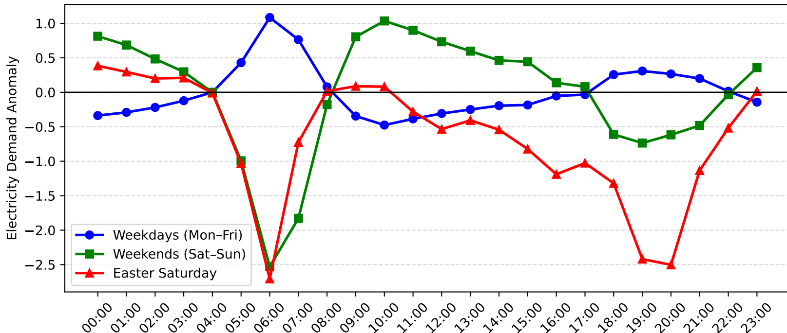
Cronulla Demand Anomaly: Easter Saturday vs Weekday/Weekend (2005-2006)
