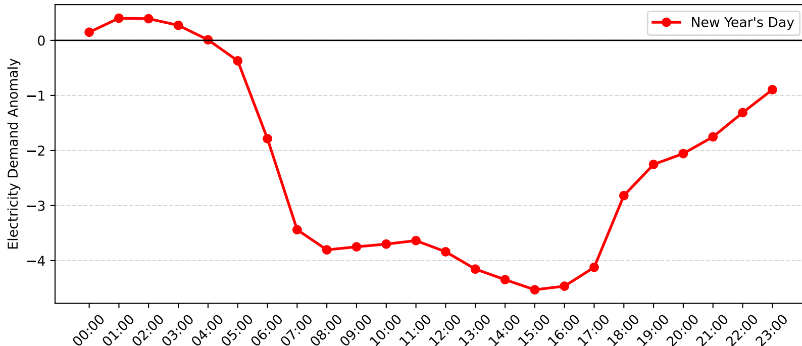
Pymble Demand Anomaly: New Year's Day (2016-2017)
