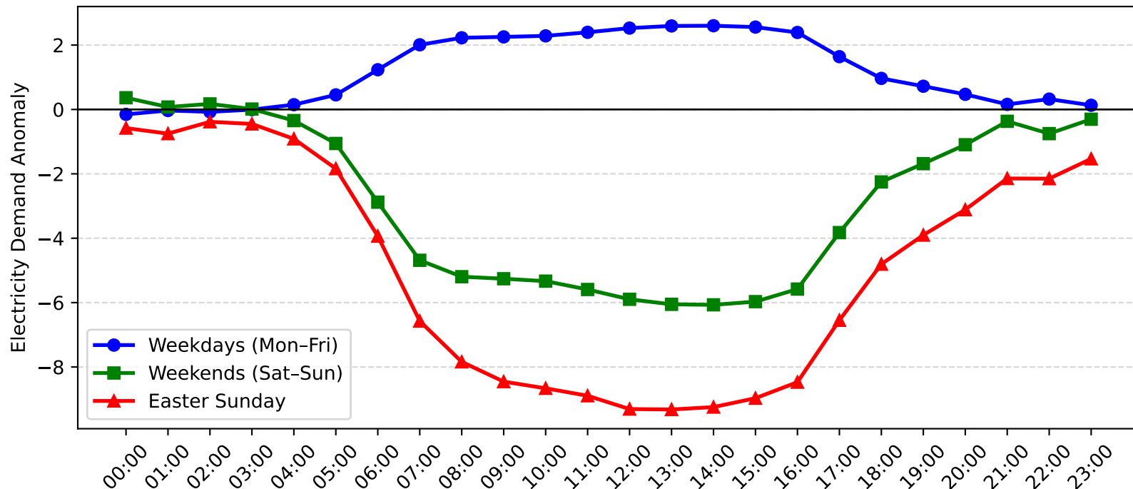
Newcastle Cbd Demand Anomaly: Easter Sunday vs Weekday/Weekend (2013-2014)
