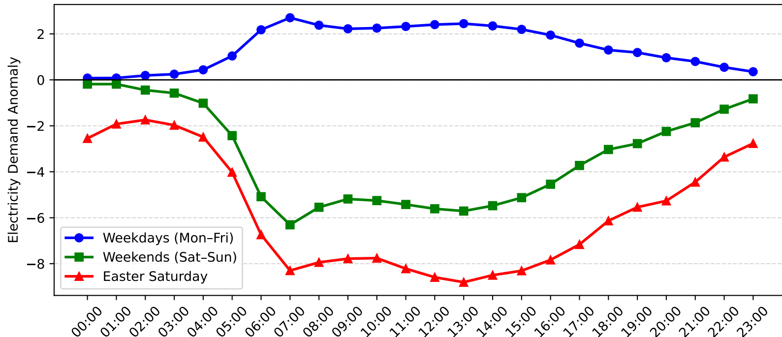
Sefton Demand Anomaly: Easter Saturday vs Weekday/Weekend (2013-2014)
