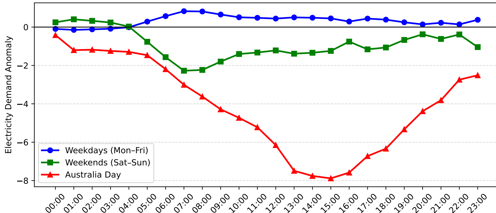
Rutherford Demand Anomaly: Australia Day vs Weekday/Weekend (2017-2018)
