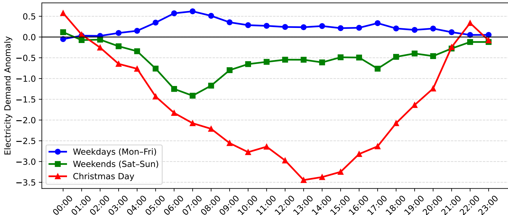
Charmhaven Demand Anomaly: Christmas Day vs Weekday/Weekend (2010-2011)
