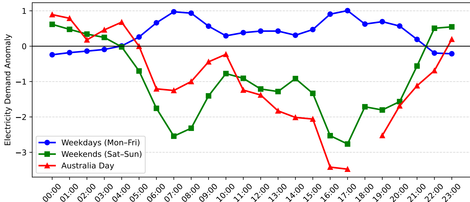
Erina Demand Anomaly: Australia Day vs Weekday/Weekend (2005-2006)
