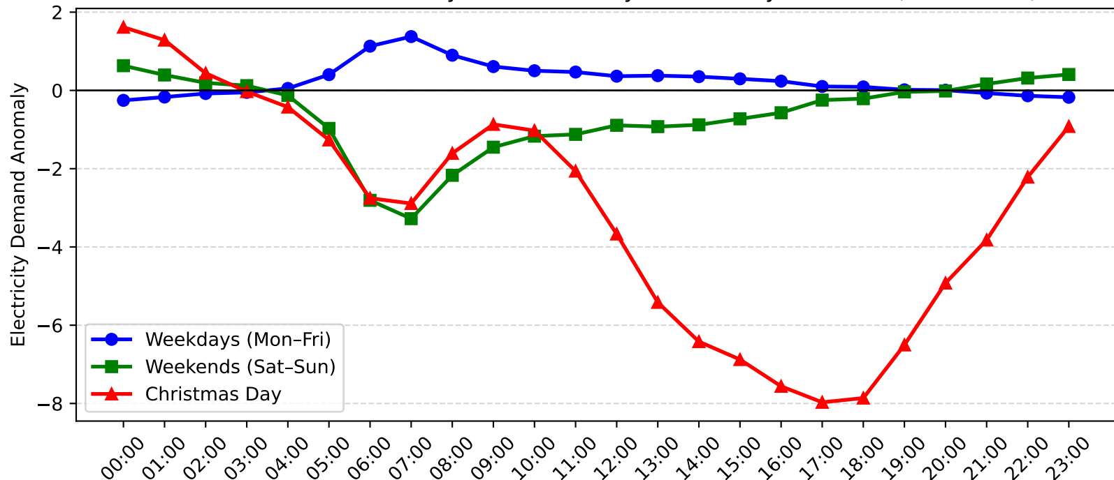
Mortdale Demand Anomaly: Christmas Day vs Weekday/Weekend (2006-2007)
