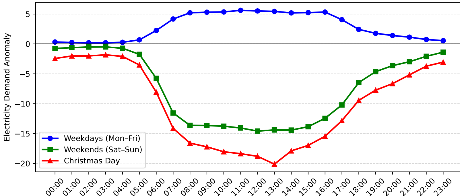
Gore Hill Demand Anomaly: Christmas Day vs Weekday/Weekend (2009-2010)
