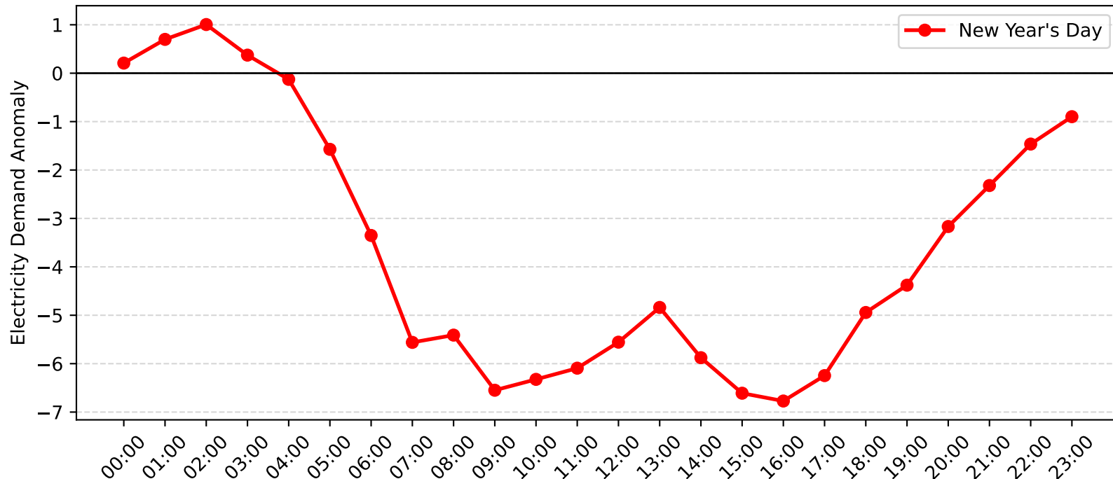
Top Ryde Demand Anomaly: New Year's Day (2014-2015)
