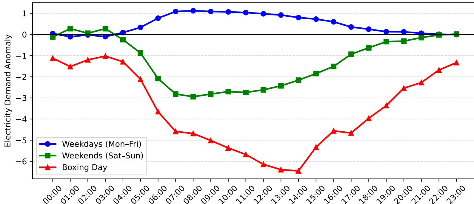
Wyong Demand Anomaly: Boxing Day vs Weekday/Weekend (2006-2007)
