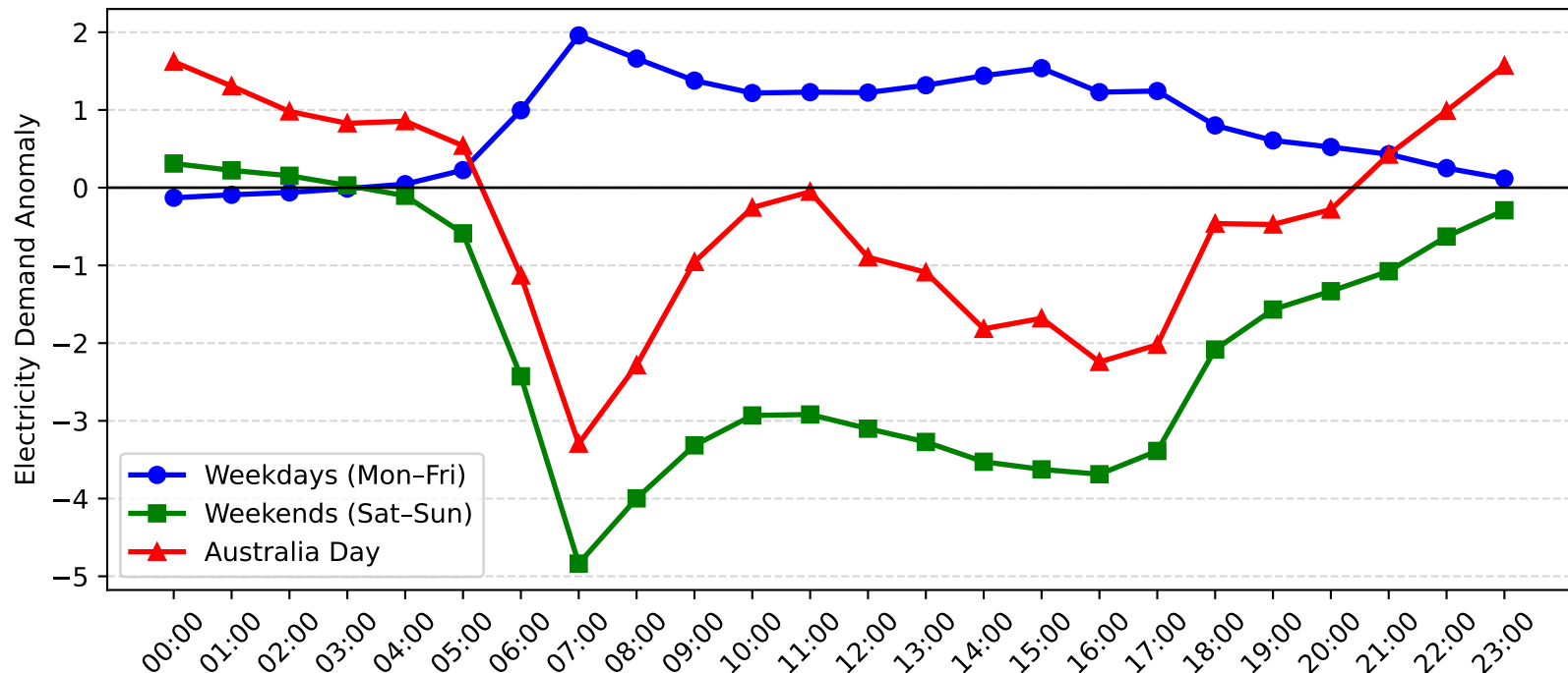
Chatswood Demand Anomaly: Australia Day vs Weekday/Weekend (2012-2013)
