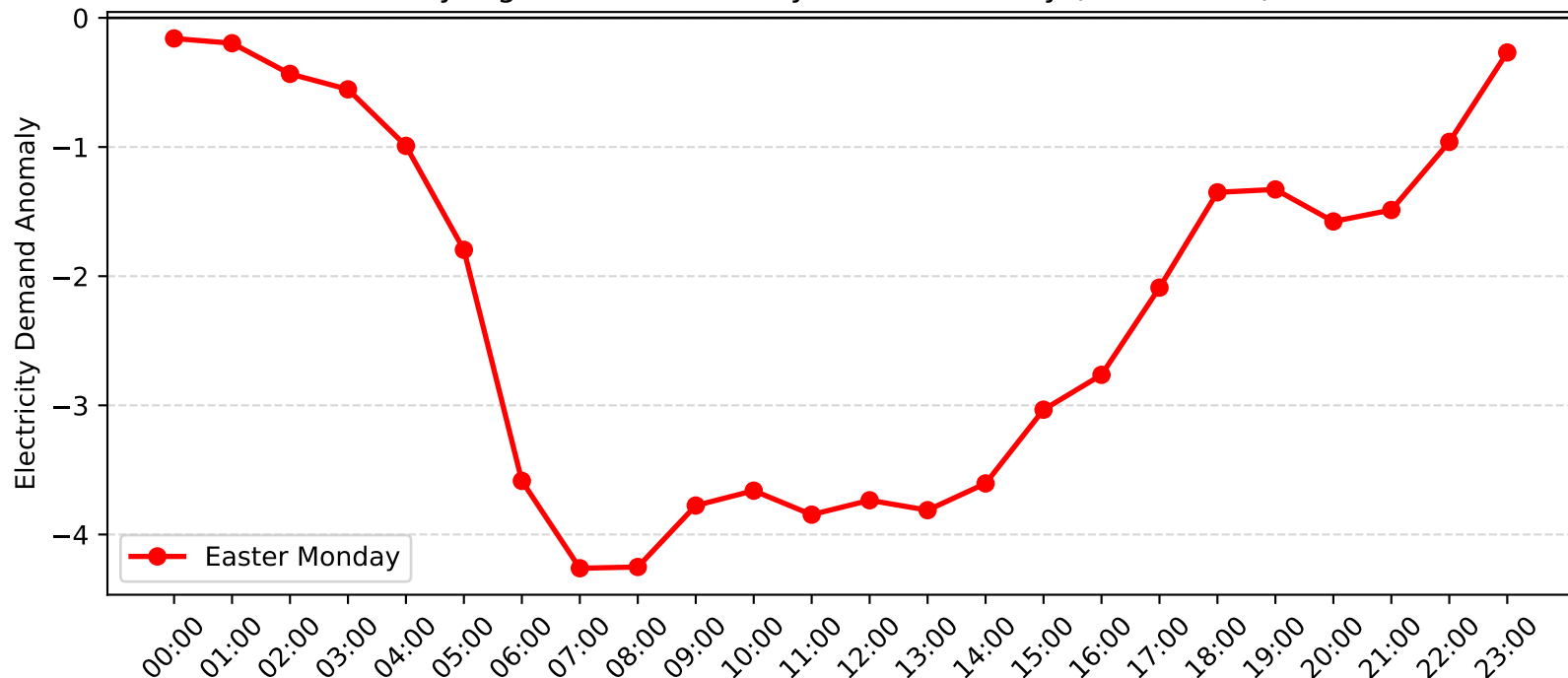
Wyong Demand Anomaly: Easter Monday (2007-2008)
