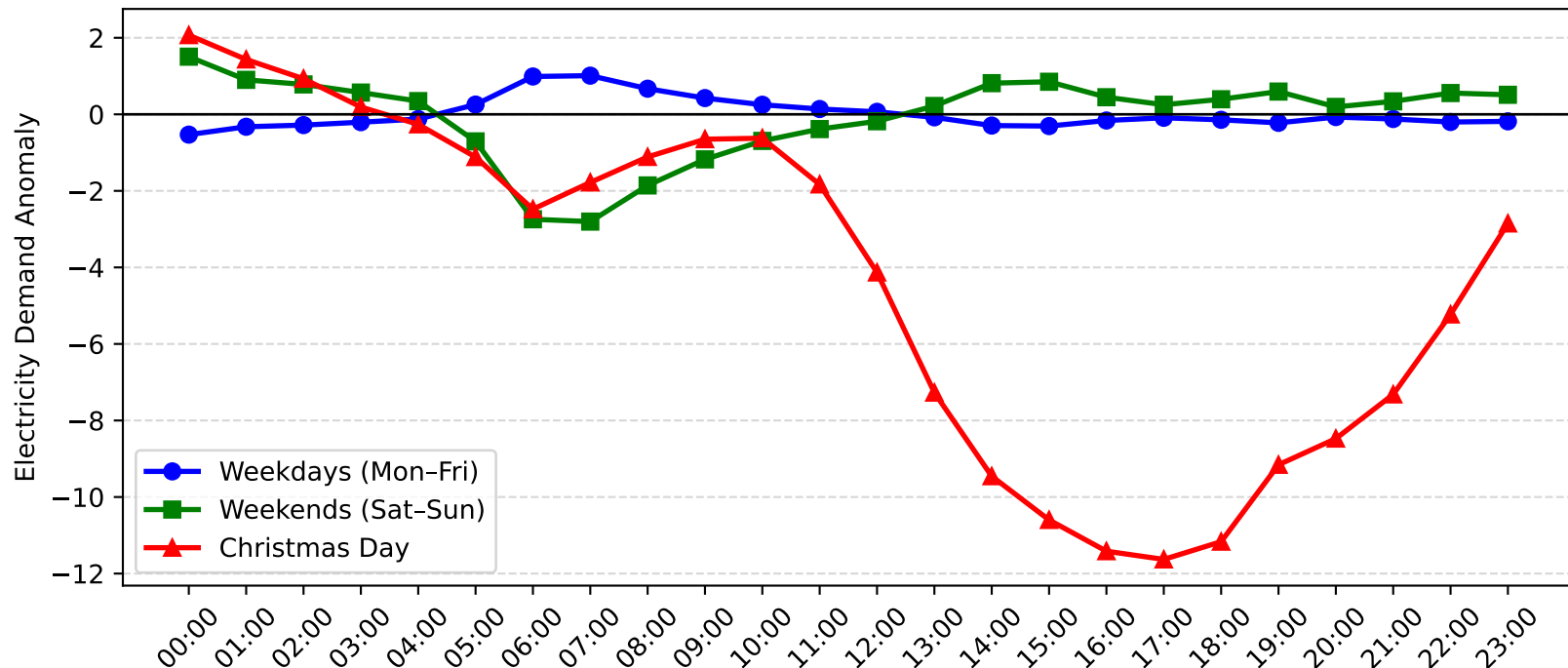
Pennant Hills Demand Anomaly: Christmas Day vs Weekday/Weekend (2012-2013)
