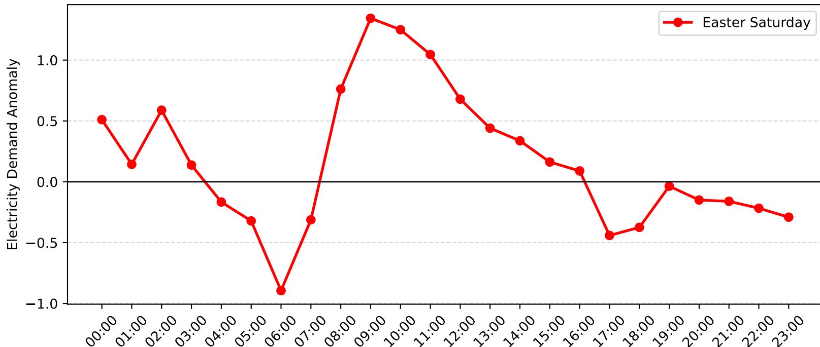
Morisset Demand Anomaly: Easter Saturday (2015-2016)
