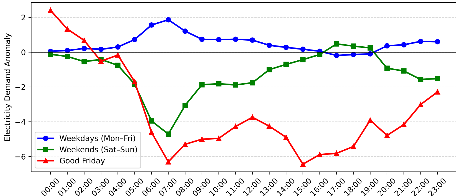
Meadowbank Demand Anomaly: Good Friday vs Weekday/Weekend (2013-2014)
