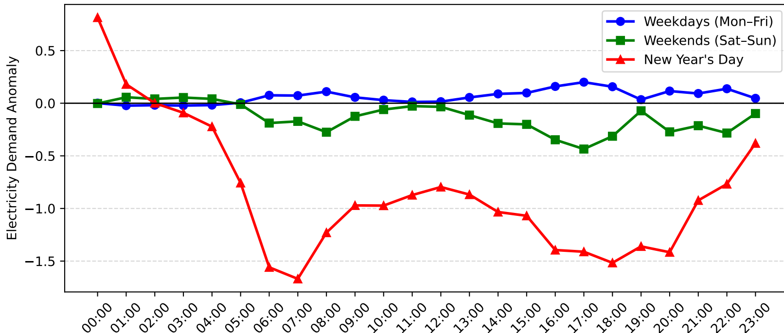
Narrabeen Demand Anomaly: New Year's Day vs Weekday/Weekend (2004-2005)
