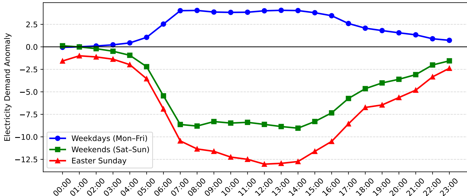
St. Peters Demand Anomaly: Easter Sunday vs Weekday/Weekend (2009-2010)
