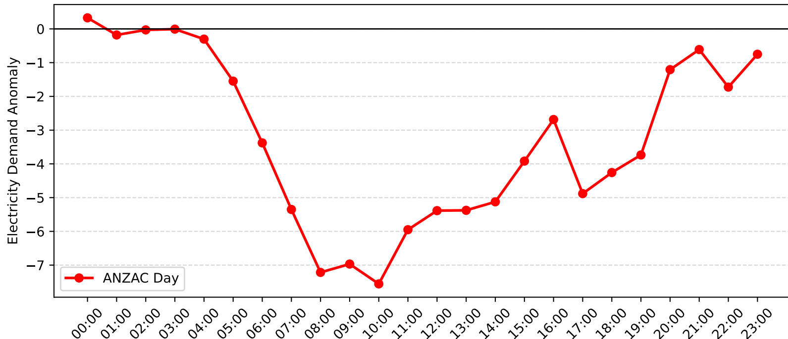
Bankstown Demand Anomaly: ANZAC Day (2014-2015)
