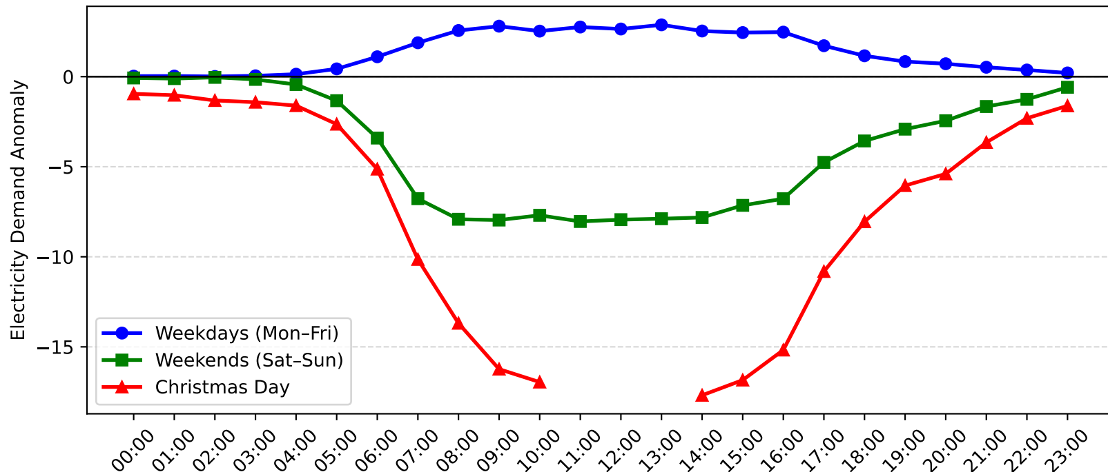
Brookvale Demand Anomaly: Christmas Day vs Weekday/Weekend (2008-2009)
