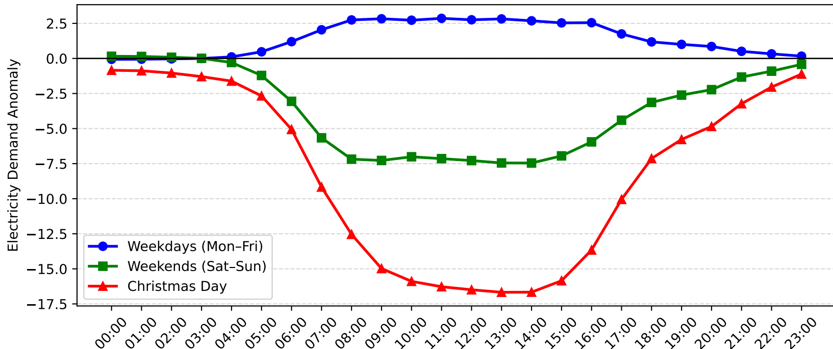
Brookvale Demand Anomaly: Christmas Day vs Weekday/Weekend (2009-2010)
