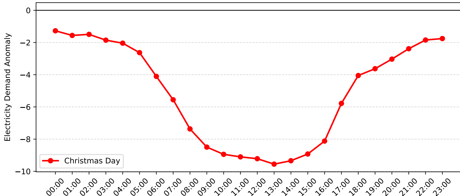
Auburn Demand Anomaly: Christmas Day (2015-2016)
