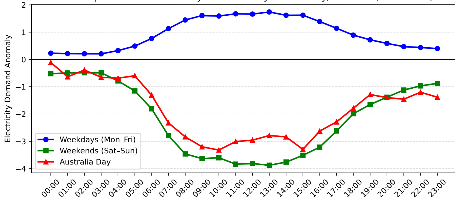
Green Square Demand Anomaly: Australia Day vs Weekday/Weekend (2008-2009)
