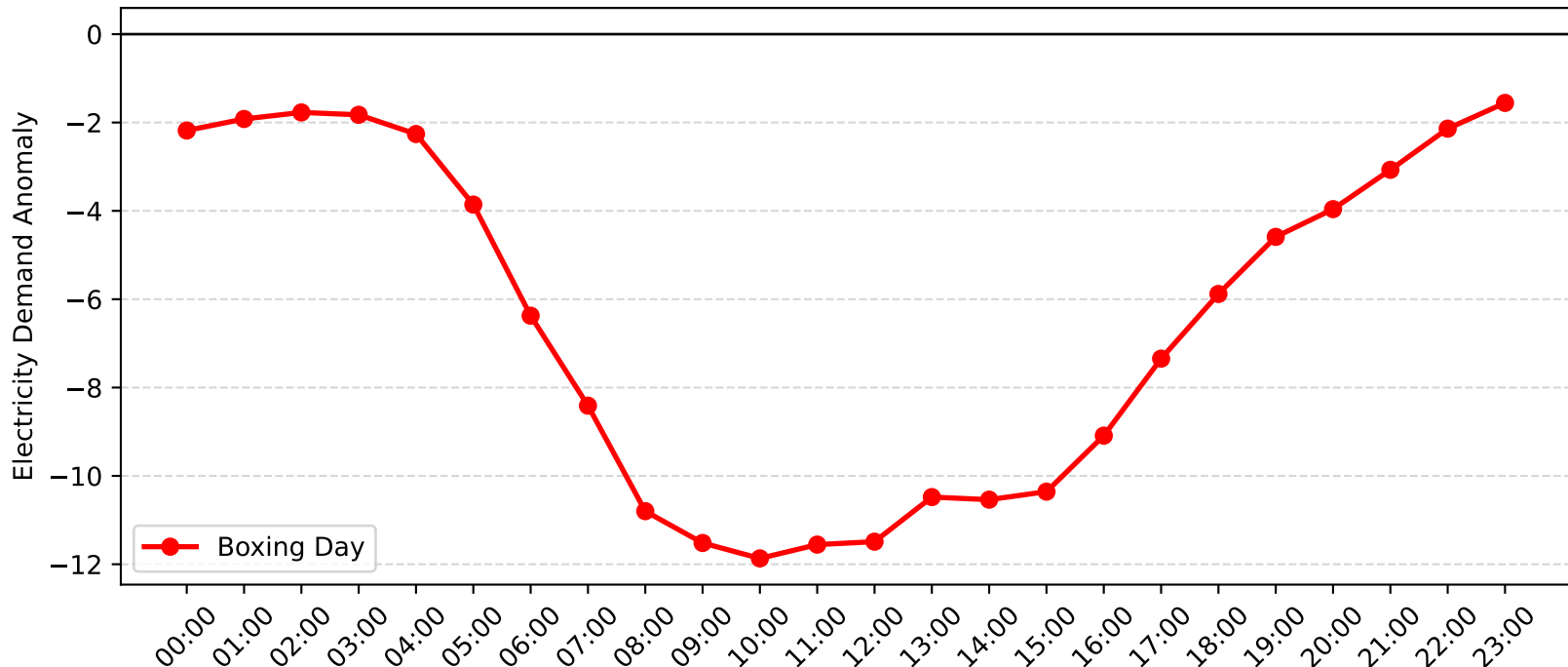
Homebush Bay Demand Anomaly: Boxing Day (2014-2015)
