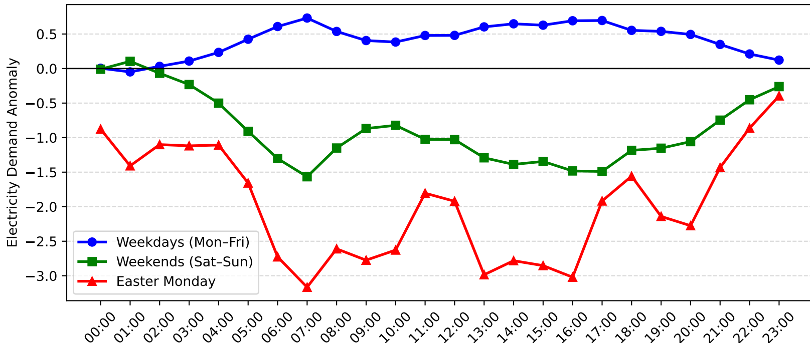
Charmhaven Demand Anomaly: Easter Monday vs Weekday/Weekend (2017-2018)
