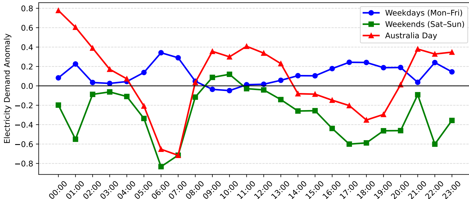
Morisset Demand Anomaly: Australia Day vs Weekday/Weekend (2012-2013)
