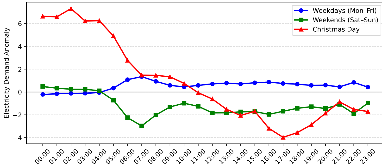
Dee Why West Demand Anomaly: Christmas Day vs Weekday/Weekend (2004-2005)
