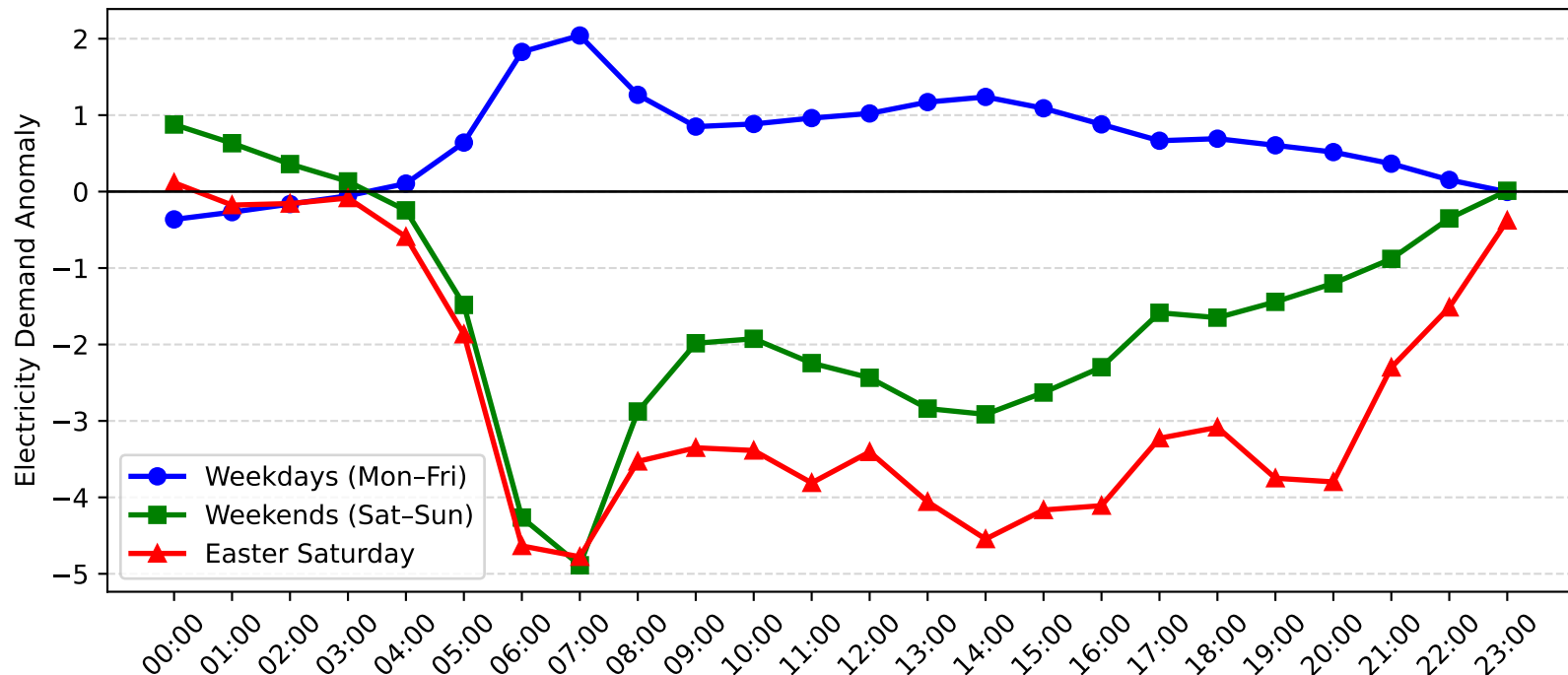
Mortdale Demand Anomaly: Easter Saturday vs Weekday/Weekend (2005-2006)
