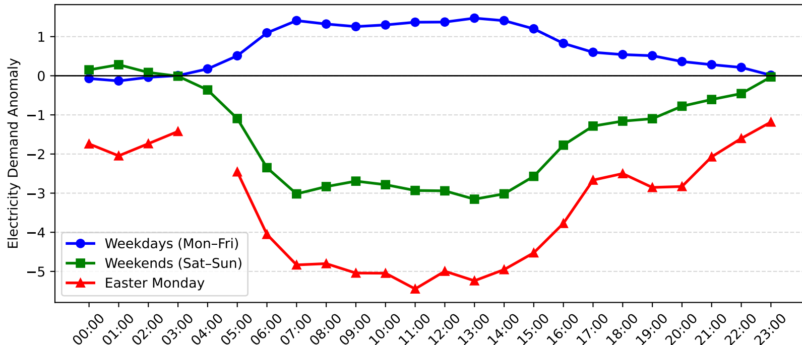
Wyong Demand Anomaly: Easter Monday vs Weekday/Weekend (2017-2018)
