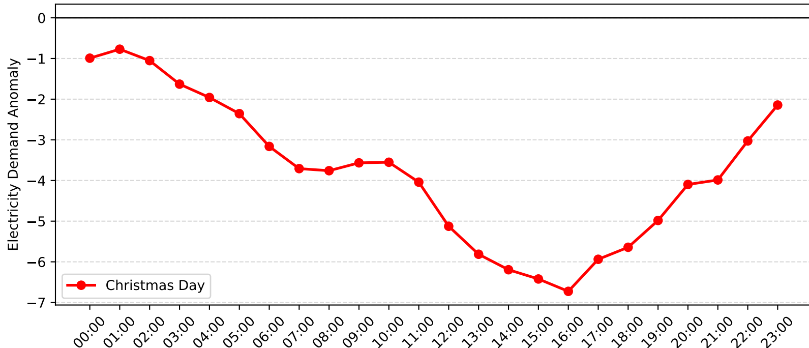
Bass Hill Demand Anomaly: Christmas Day (2007-2008)
