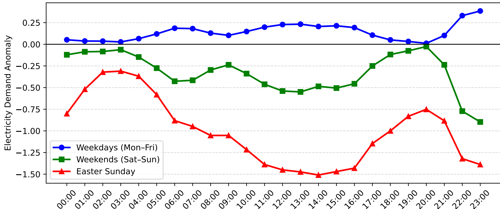
Muswellbrook Demand Anomaly: Easter Sunday vs Weekday/Weekend (2016-2017)
