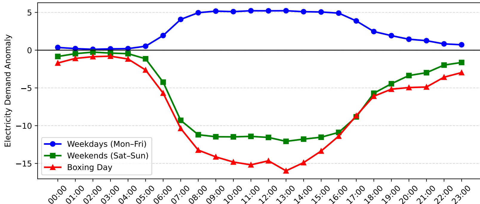
Gore Hill Demand Anomaly: Boxing Day vs Weekday/Weekend (2010-2011)
