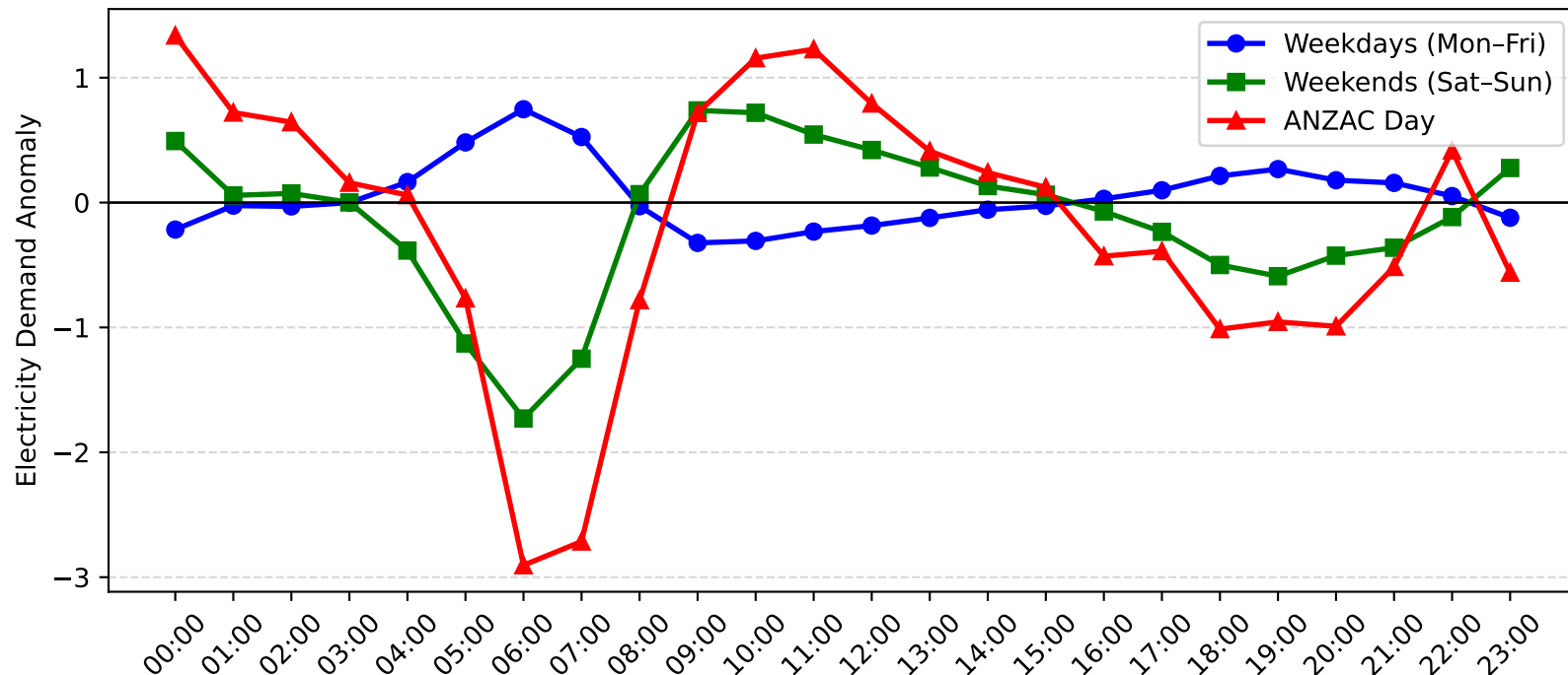
Umina Demand Anomaly: ANZAC Day vs Weekday/Weekend (2008-2009)
