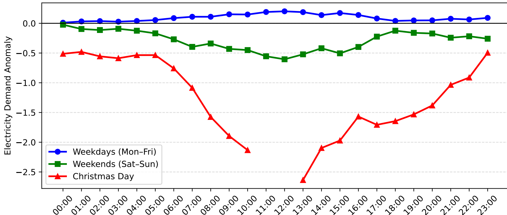
Rothbury Demand Anomaly: Christmas Day vs Weekday/Weekend (2008-2009)
