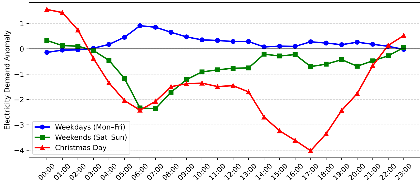
Revesby Demand Anomaly: Christmas Day vs Weekday/Weekend (2009-2010)
