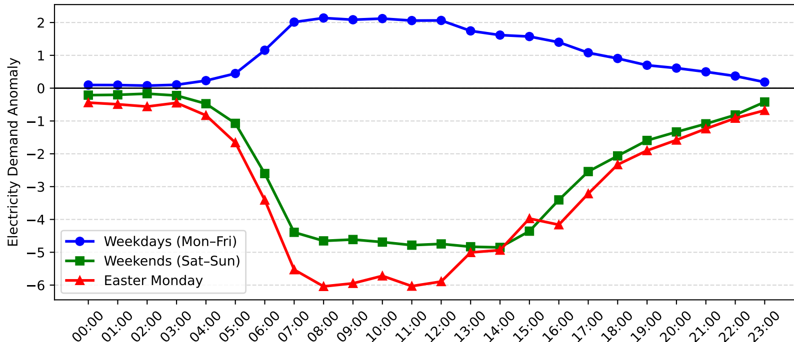
Bankstown Demand Anomaly: Easter Monday vs Weekday/Weekend (2013-2014)
