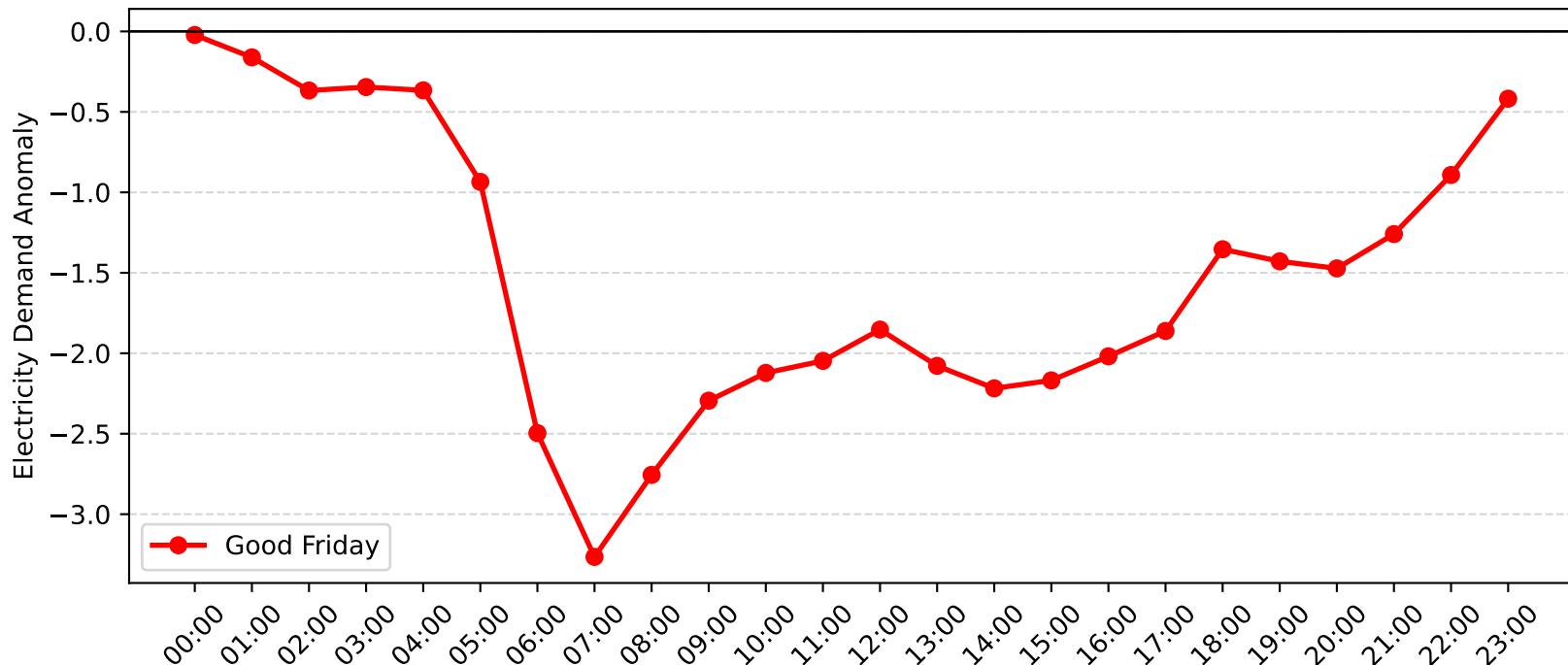
Arncliffe Demand Anomaly: Good Friday (2009-2010)
