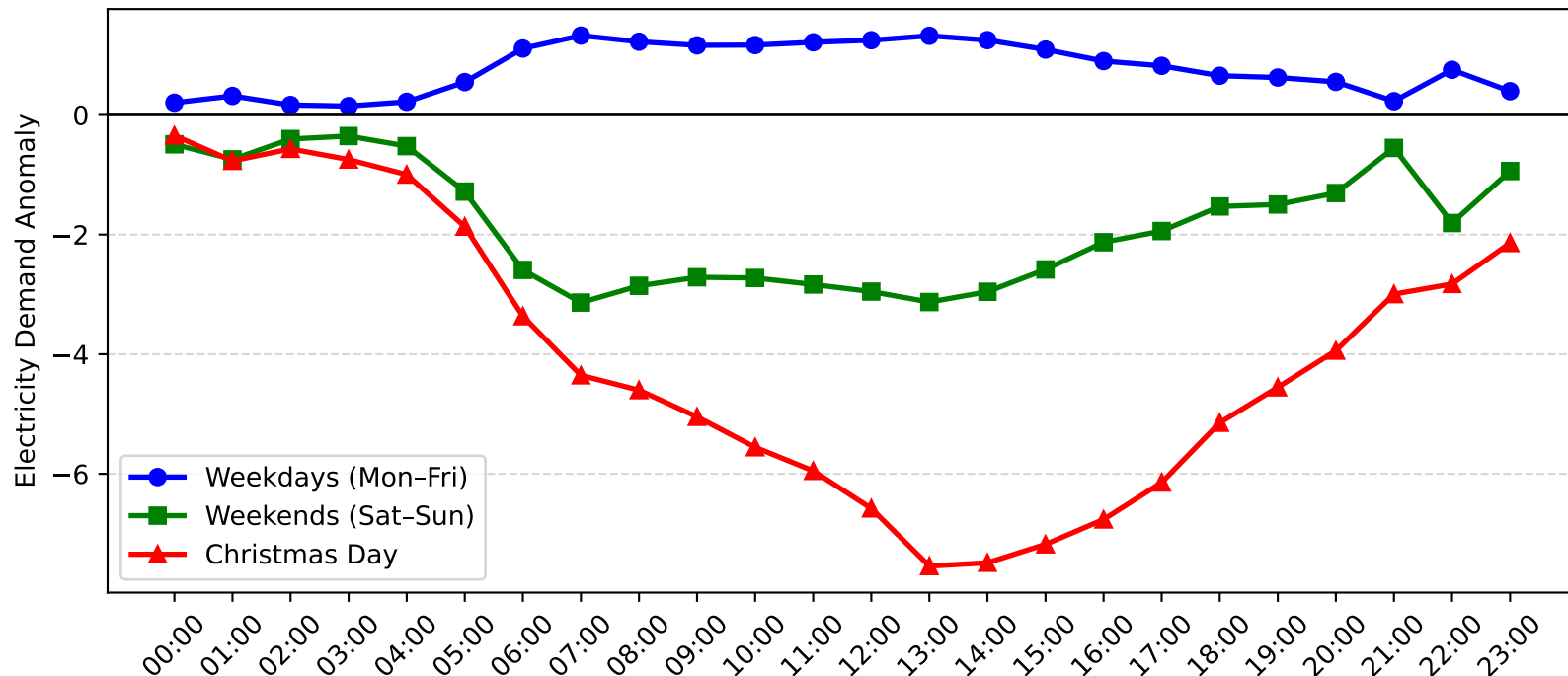
Argenton Demand Anomaly: Christmas Day vs Weekday/Weekend (2011-2012)
