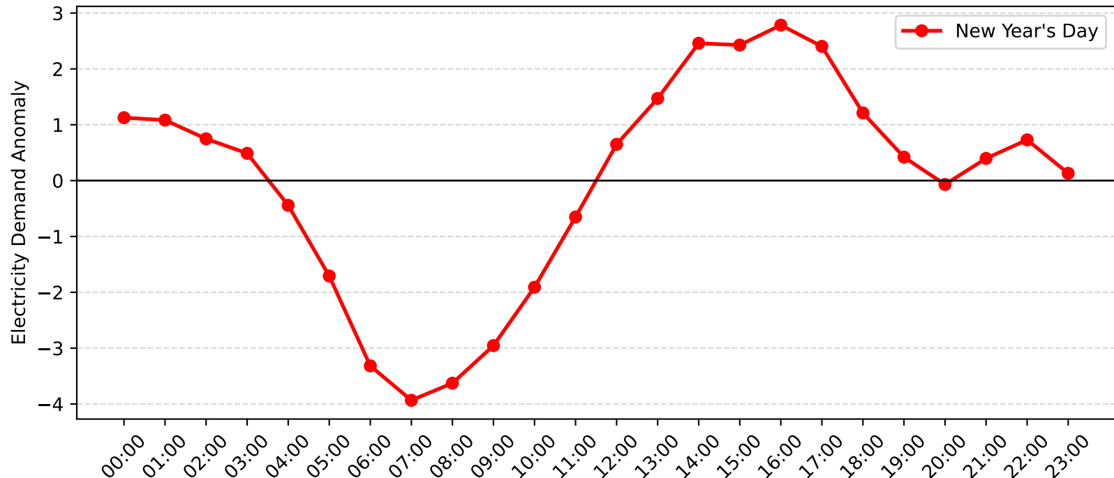
Revesby Demand Anomaly: New Year's Day (2010-2011)
