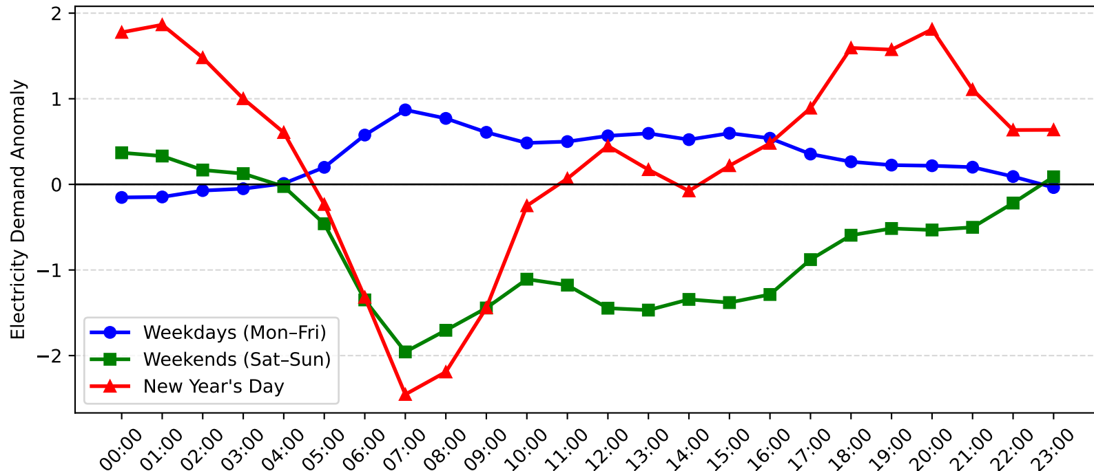
Arncliffe Demand Anomaly: New Year's Day vs Weekday/Weekend (2006-2007)
