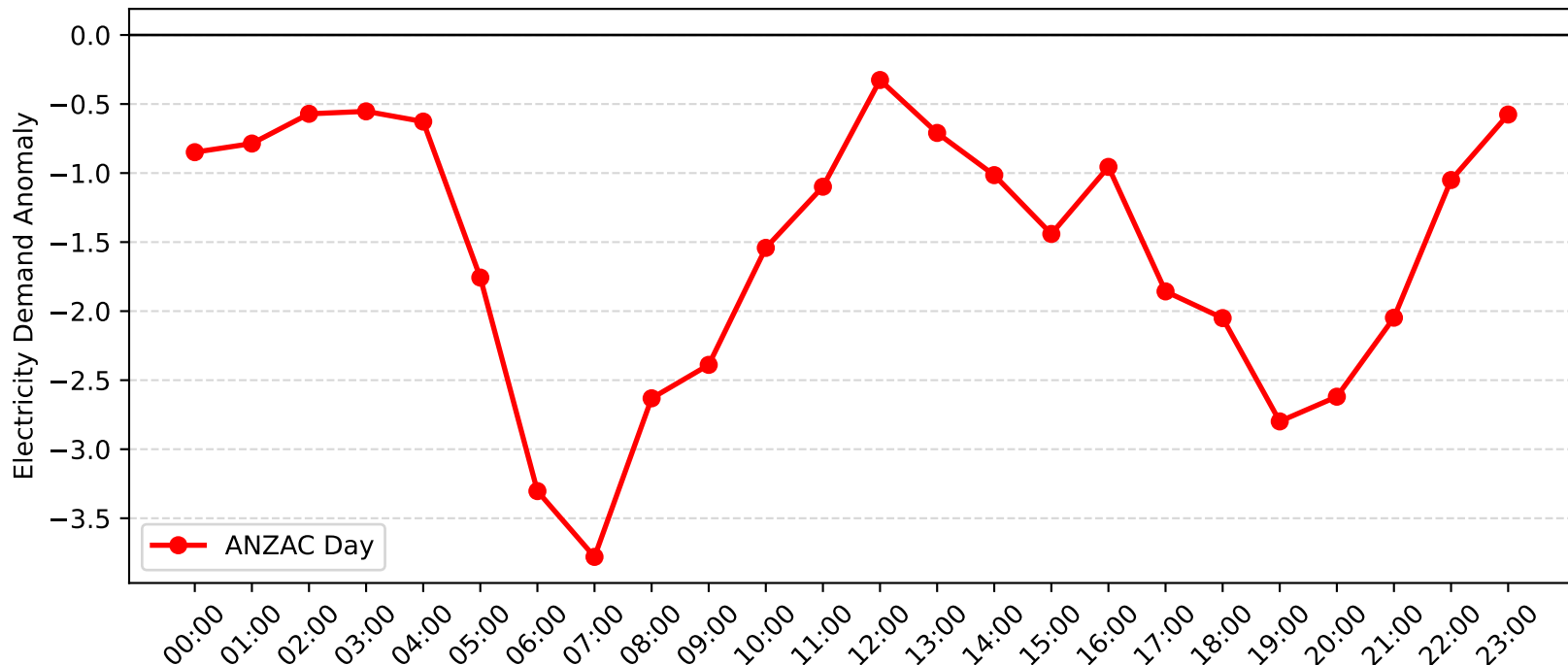
Charmhaven Demand Anomaly: ANZAC Day (2010-2011)
