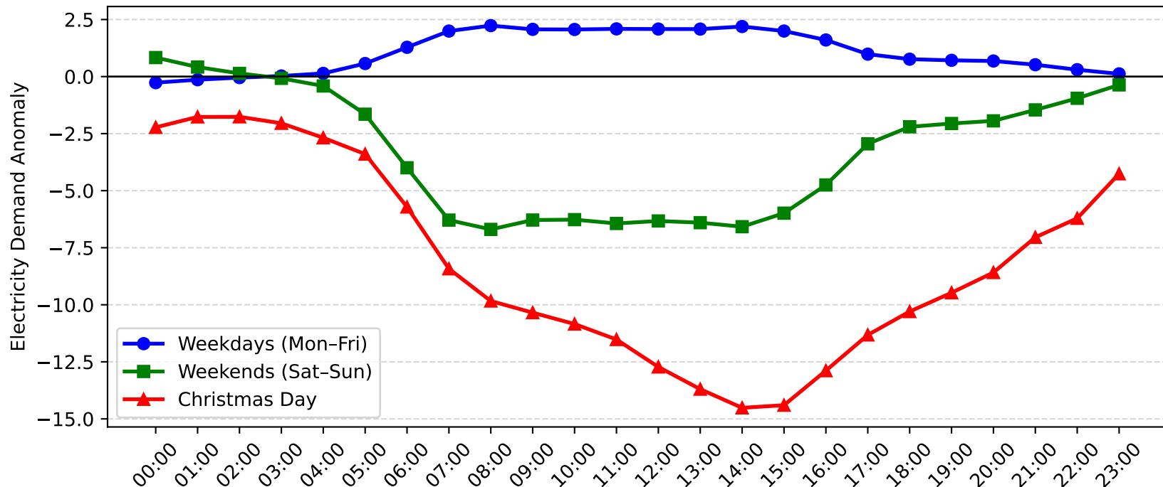
Marrickville Demand Anomaly: Christmas Day vs Weekday/Weekend (2013-2014)
