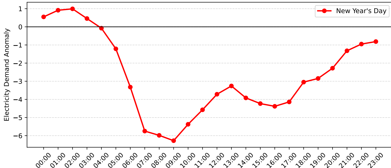
Top Ryde Demand Anomaly: New Year's Day (2013-2014)
