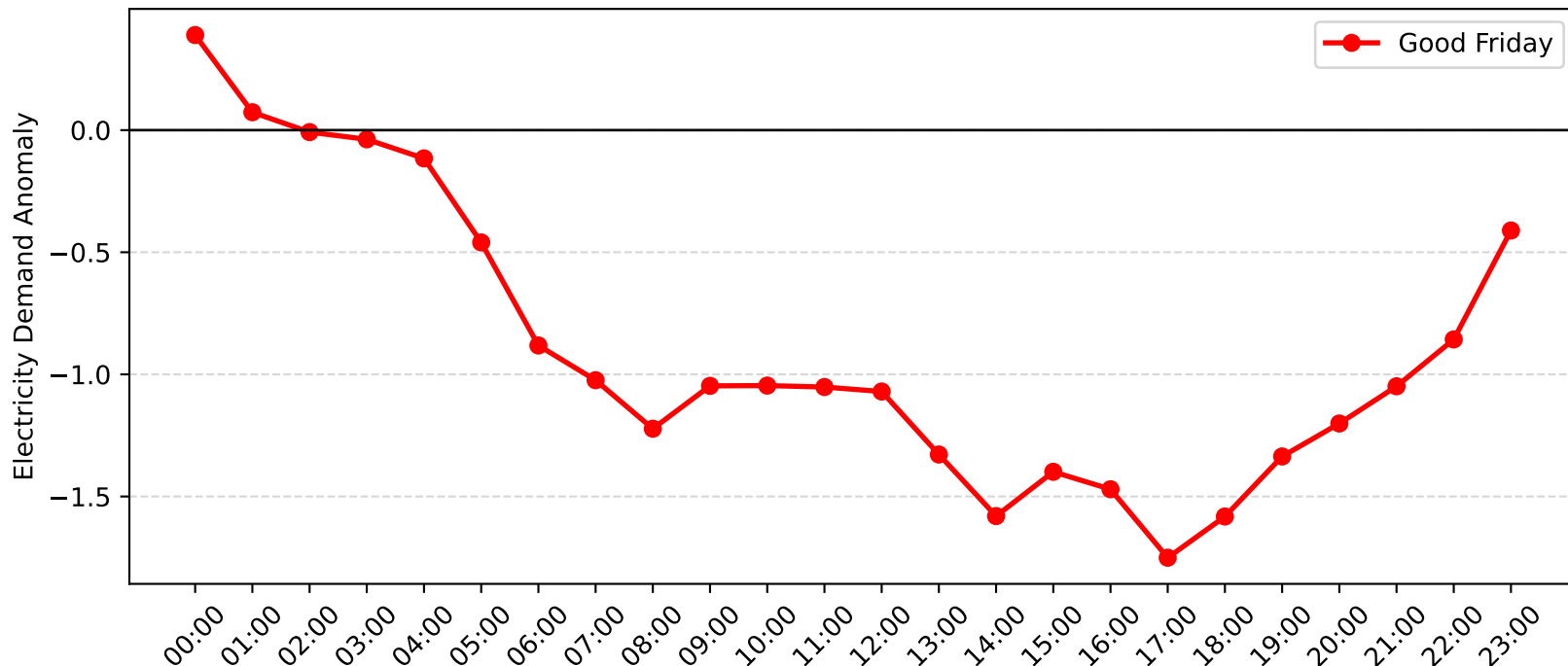
Muswellbrook Demand Anomaly: Good Friday (2014-2015)
