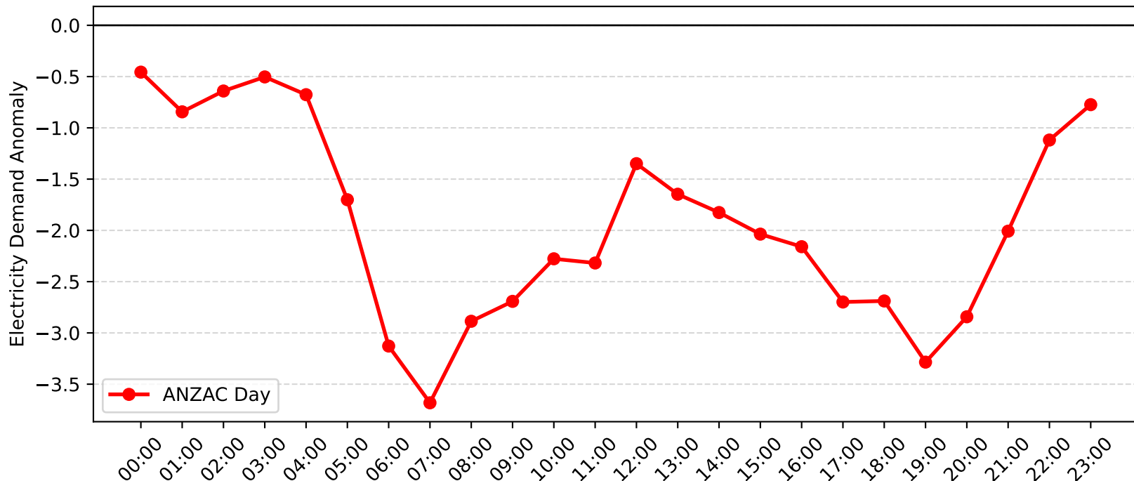
Charmhaven Demand Anomaly: ANZAC Day (2009-2010)
