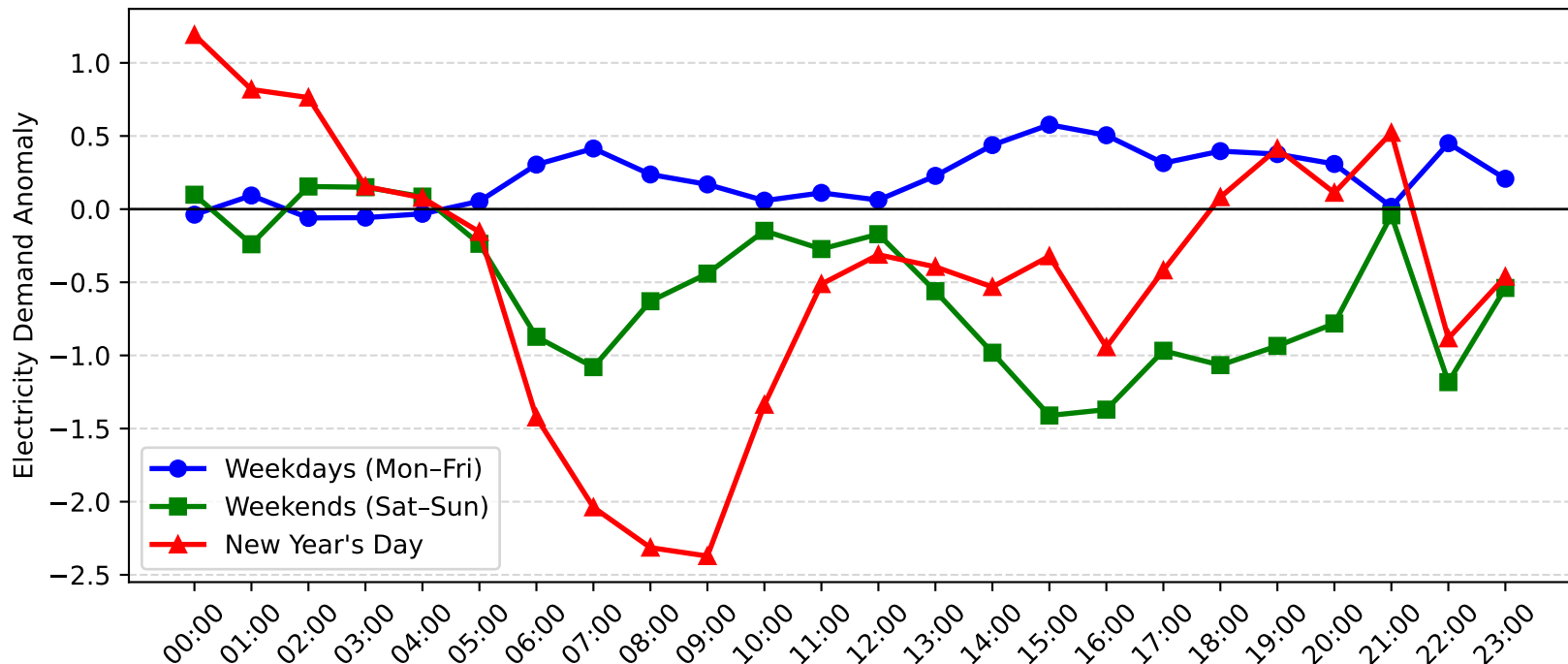
Charlestown Demand Anomaly: New Year's Day vs Weekday/Weekend (2013-2014)
