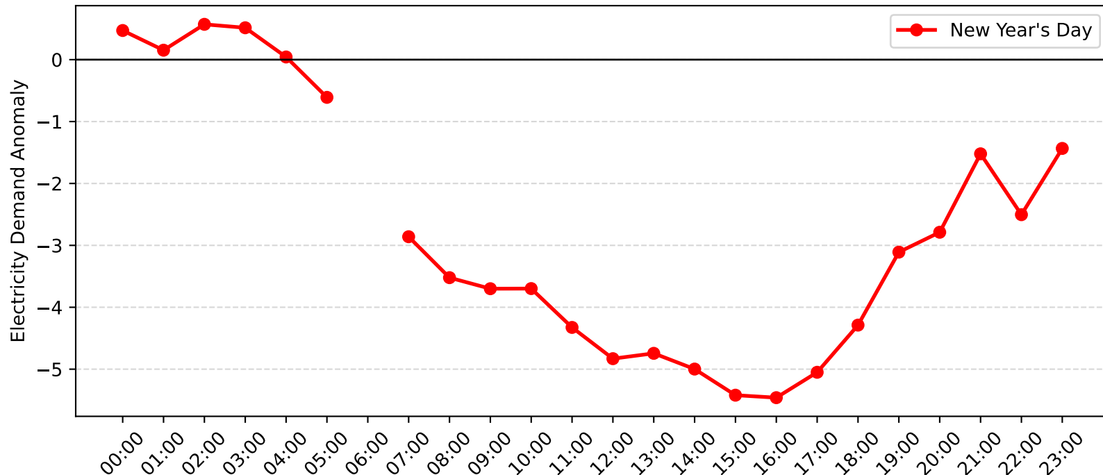
Charlestown Demand Anomaly: New Year's Day (2016-2017)
