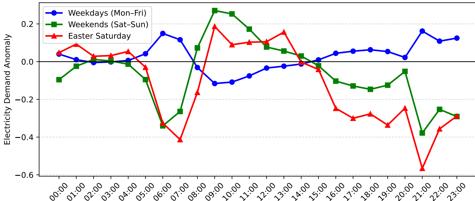
Jesmond Demand Anomaly: Easter Saturday vs Weekday/Weekend (2010-2011)
