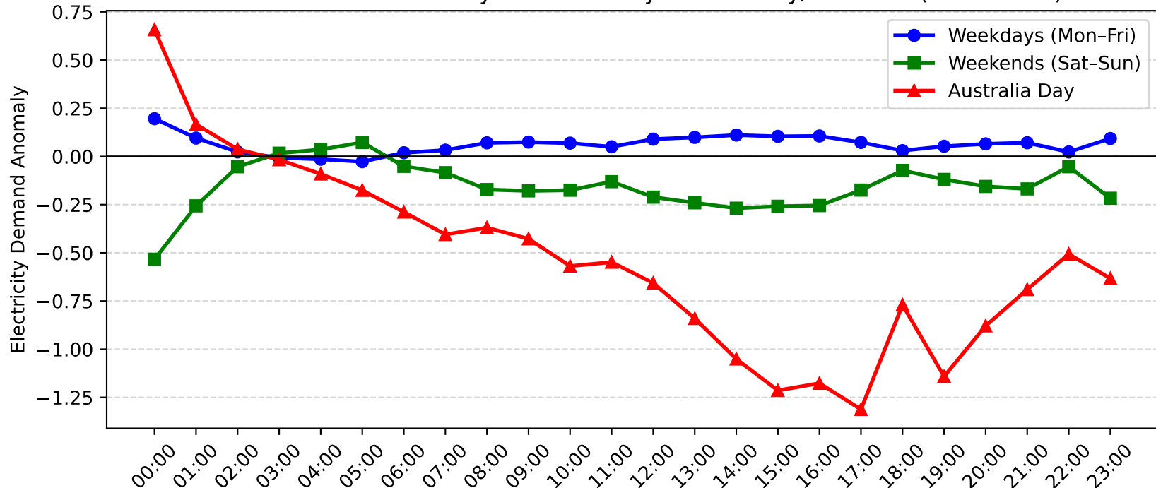
Telarah Demand Anomaly: Australia Day vs Weekday/Weekend (2004-2005)
