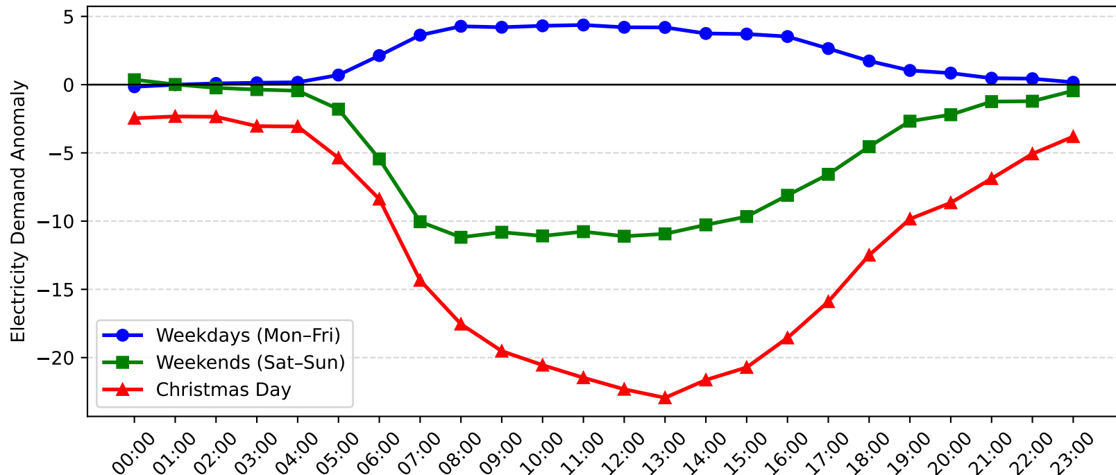
Zetland Demand Anomaly: Christmas Day vs Weekday/Weekend (2009-2010)
