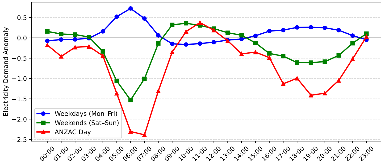
Woy Woy Demand Anomaly: ANZAC Day vs Weekday/Weekend (2010-2011)
