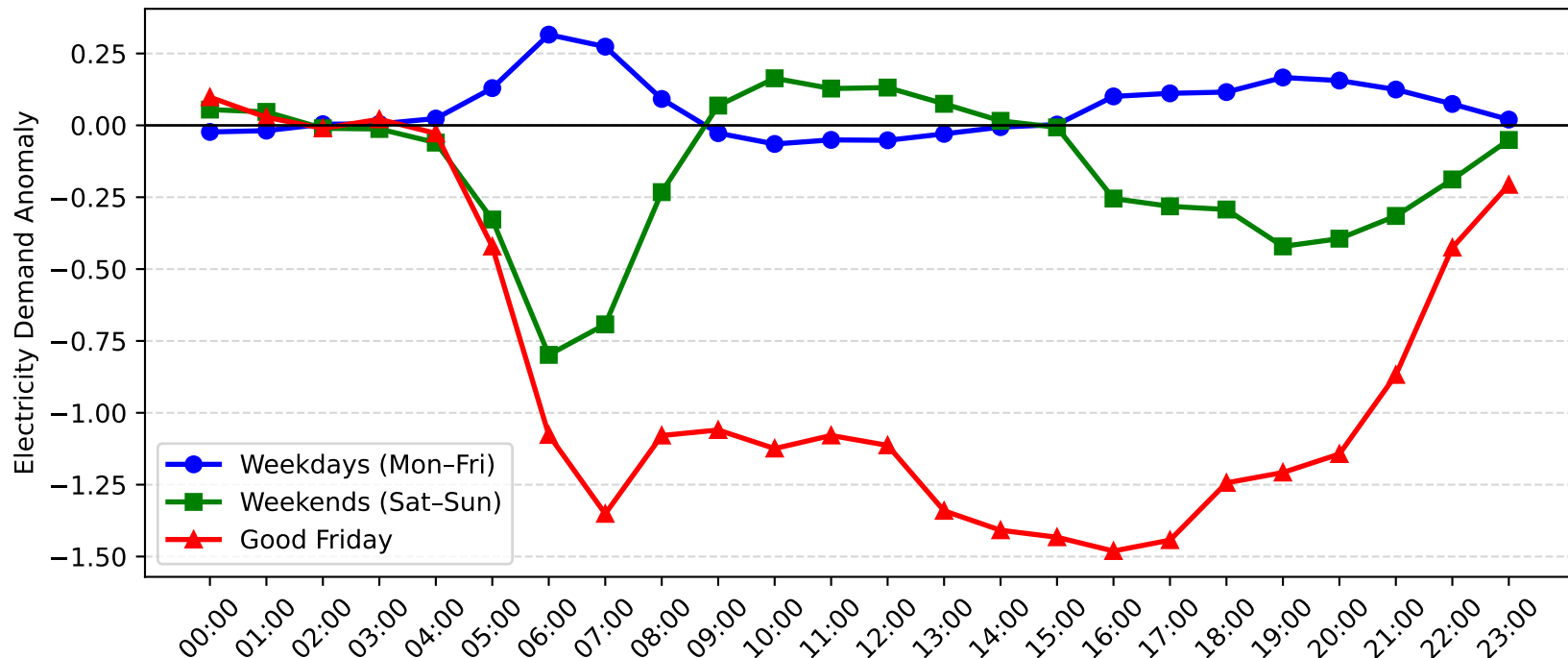
Narrabeen Demand Anomaly: Good Friday vs Weekday/Weekend (2013-2014)
