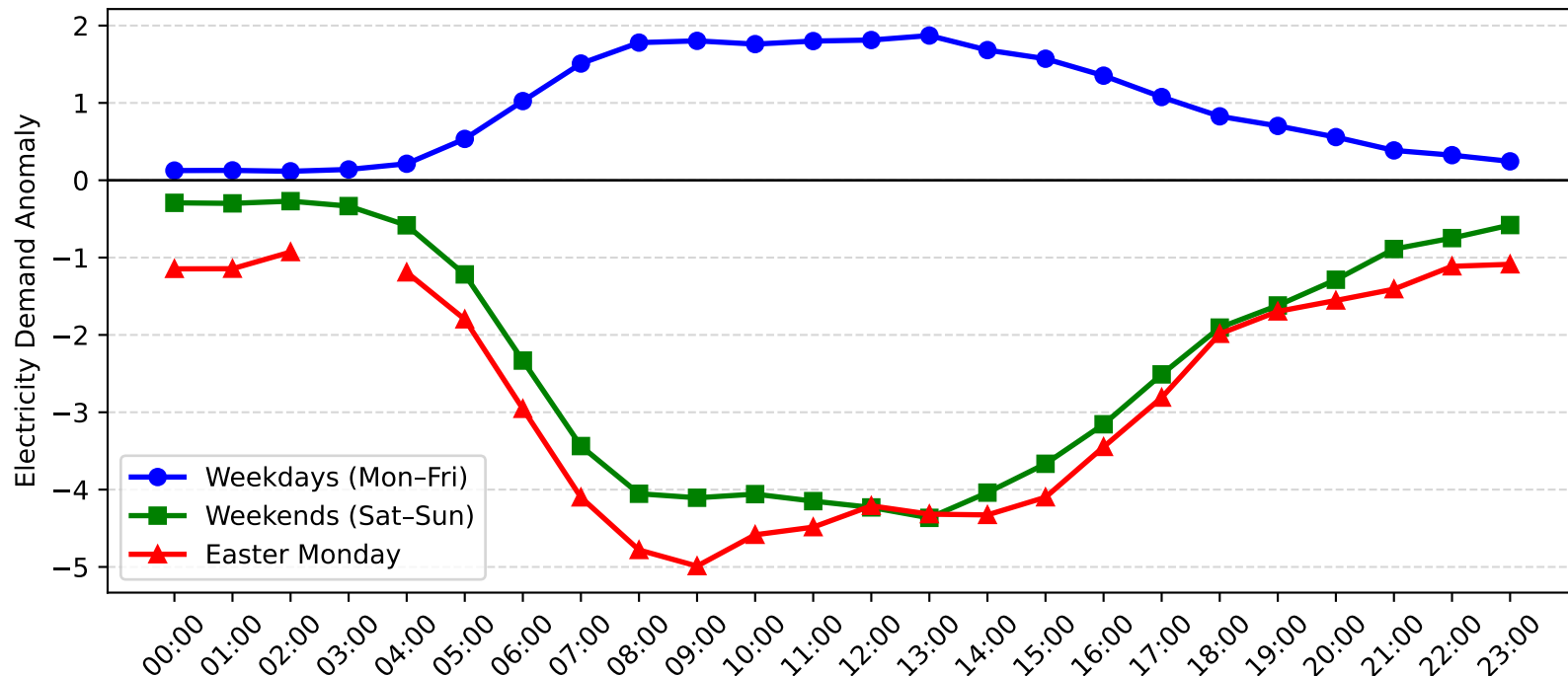
Auburn Demand Anomaly: Easter Monday vs Weekday/Weekend (2015-2016)
