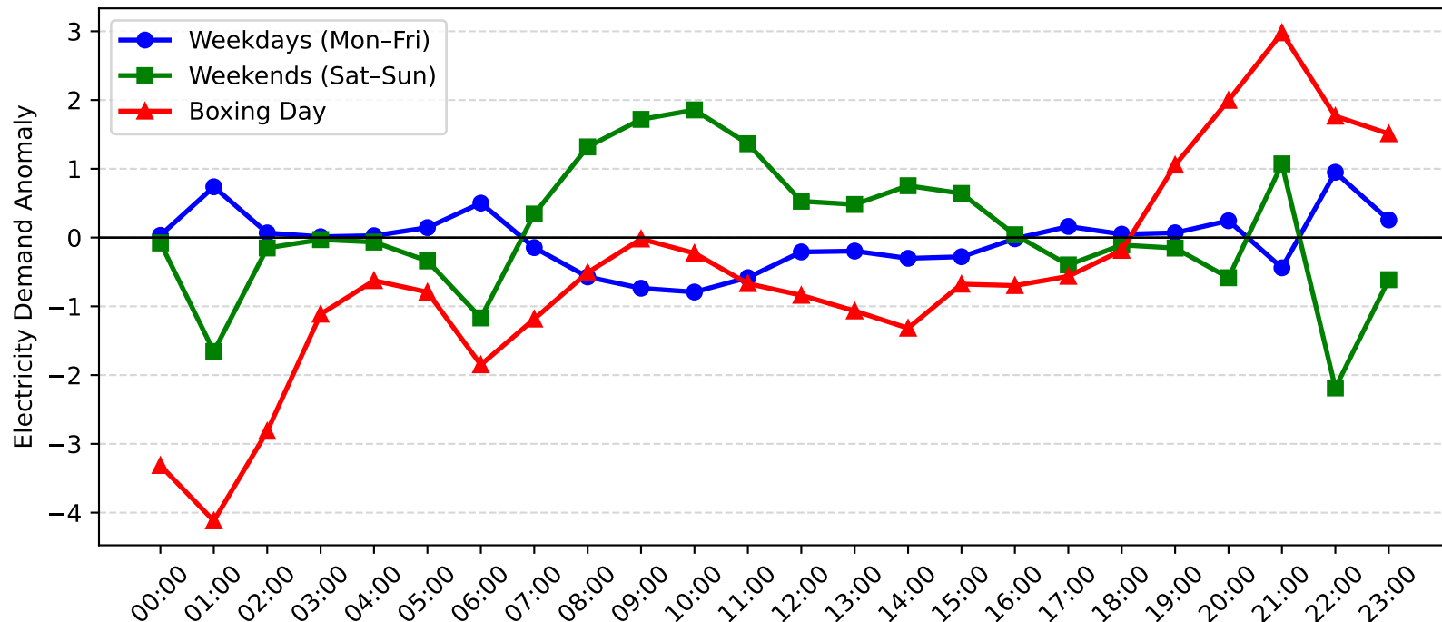
Nelson Bay Demand Anomaly: Boxing Day vs Weekday/Weekend (2005-2006)
