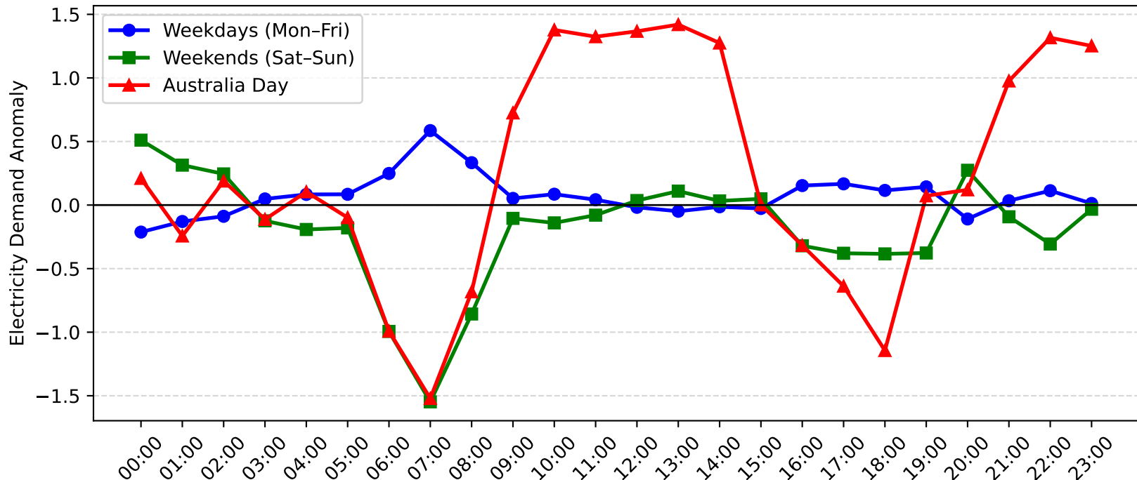
Balgowlah North Demand Anomaly: Australia Day vs Weekday/Weekend (2011-2012)
