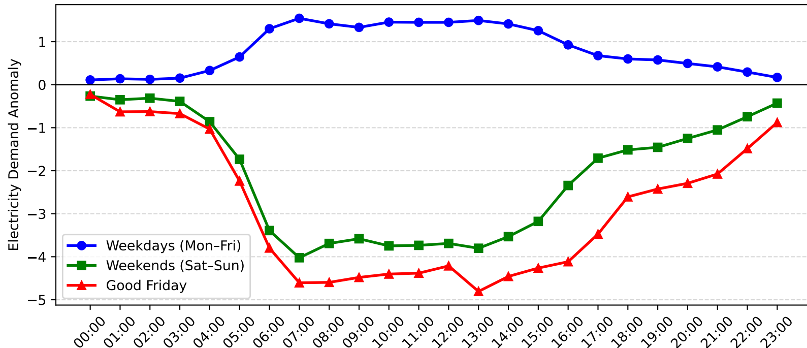
Wyong Demand Anomaly: Good Friday vs Weekday/Weekend (2012-2013)
