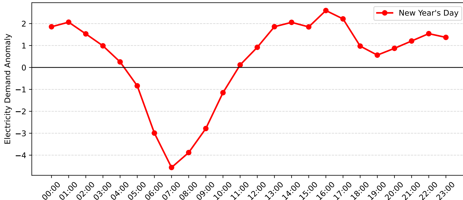
Mortdale Demand Anomaly: New Year's Day (2010-2011)
