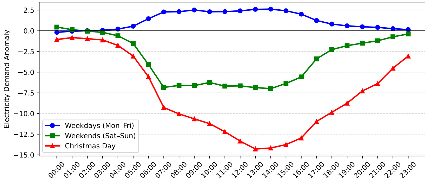
Marrickville Demand Anomaly: Christmas Day vs Weekday/Weekend (2007-2008)
