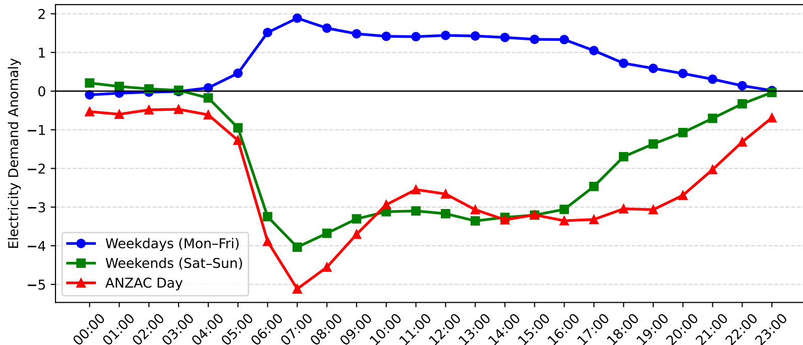
Pymble Demand Anomaly: ANZAC Day vs Weekday/Weekend (2010-2011)
