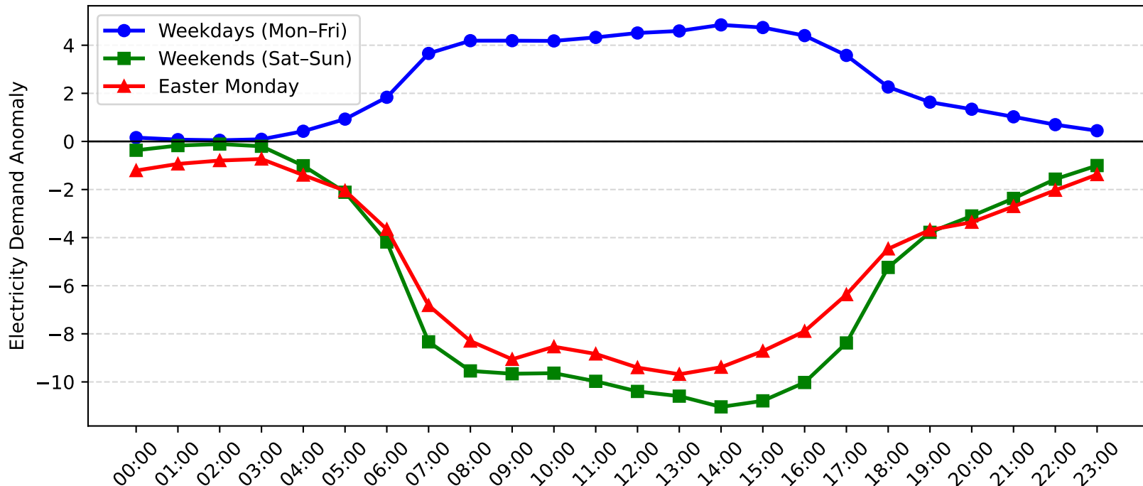
Gore Hill Demand Anomaly: Easter Monday vs Weekday/Weekend (2015-2016)
