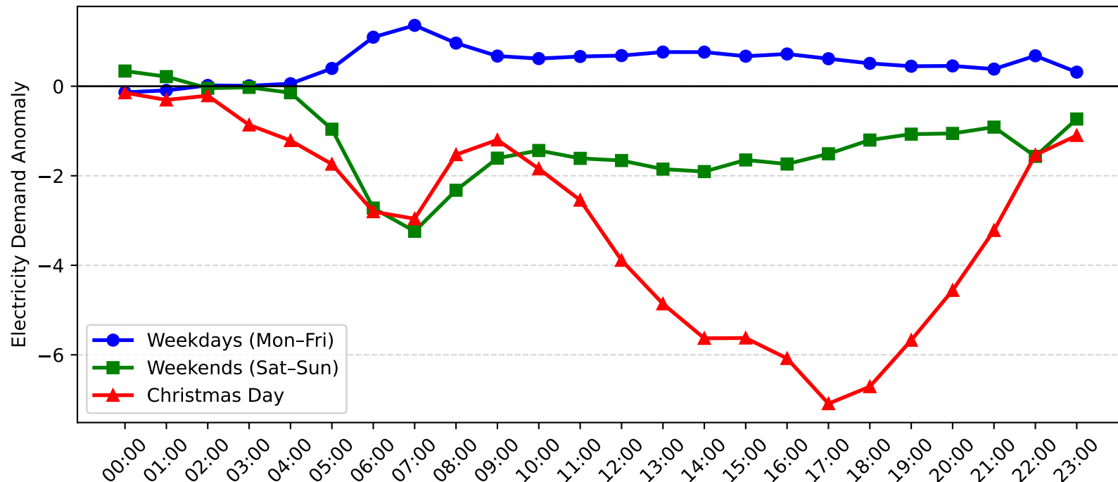
Dee Why West Demand Anomaly: Christmas Day vs Weekday/Weekend (2006-2007)
