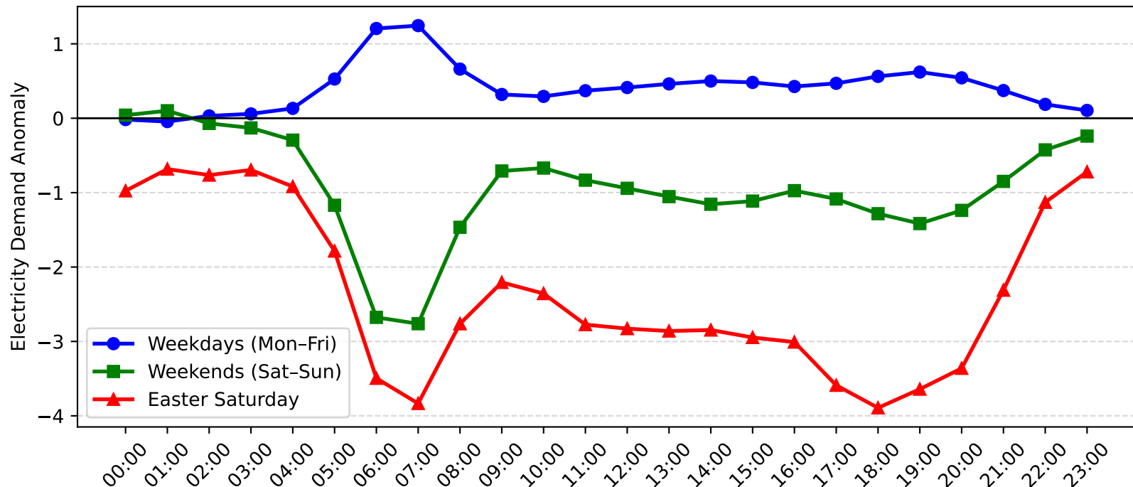
Dee Why West Demand Anomaly: Easter Saturday vs Weekday/Weekend (2016-2017)
