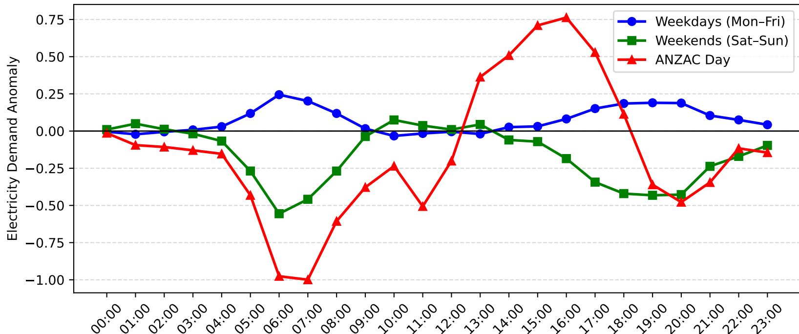
Narrabeen Demand Anomaly: ANZAC Day vs Weekday/Weekend (2017-2018)
