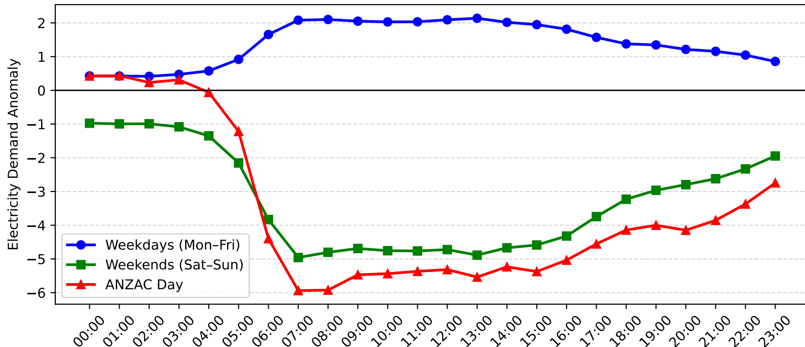
Leightonfield Demand Anomaly: ANZAC Day vs Weekday/Weekend (2008-2009)
