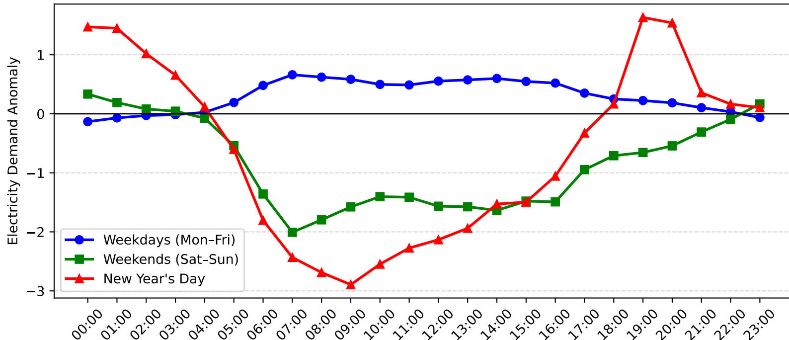
Rockdale Demand Anomaly: New Year's Day vs Weekday/Weekend (2008-2009)
