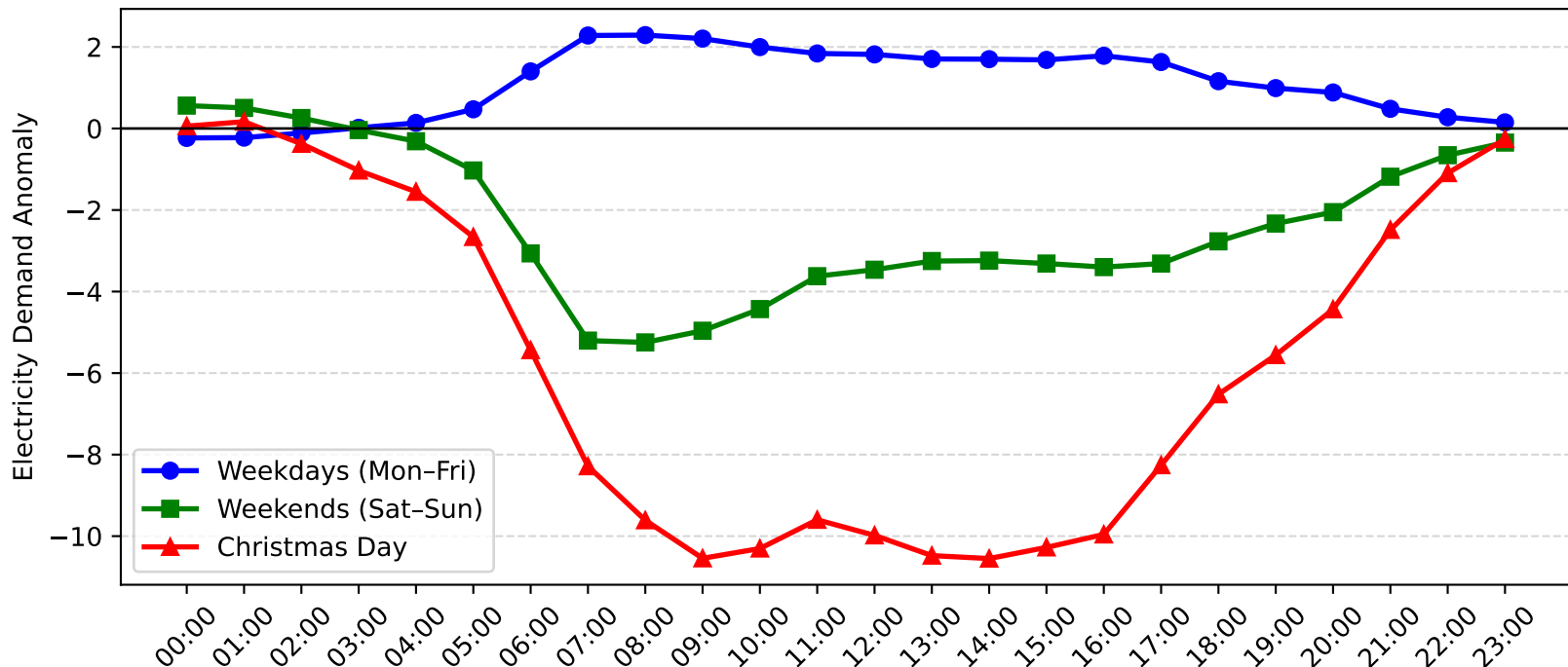
Burwood Demand Anomaly: Christmas Day vs Weekday/Weekend (2010-2011)
