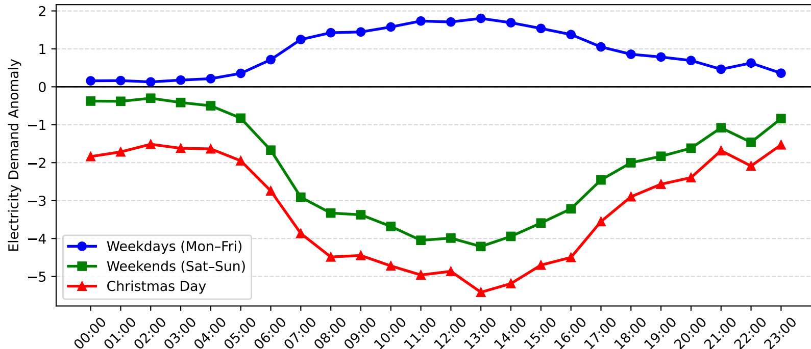
Mayfield West Demand Anomaly: Christmas Day vs Weekday/Weekend (2016-2017)
