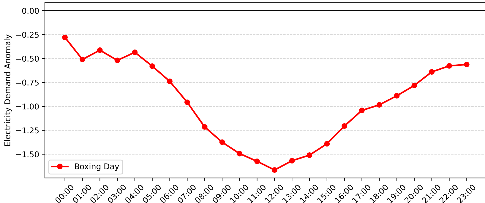
Rothbury Demand Anomaly: Boxing Day (2006-2007)
