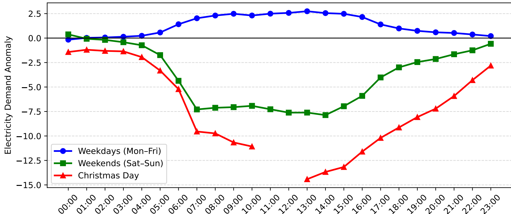
Marrickville Demand Anomaly: Christmas Day vs Weekday/Weekend (2008-2009)
