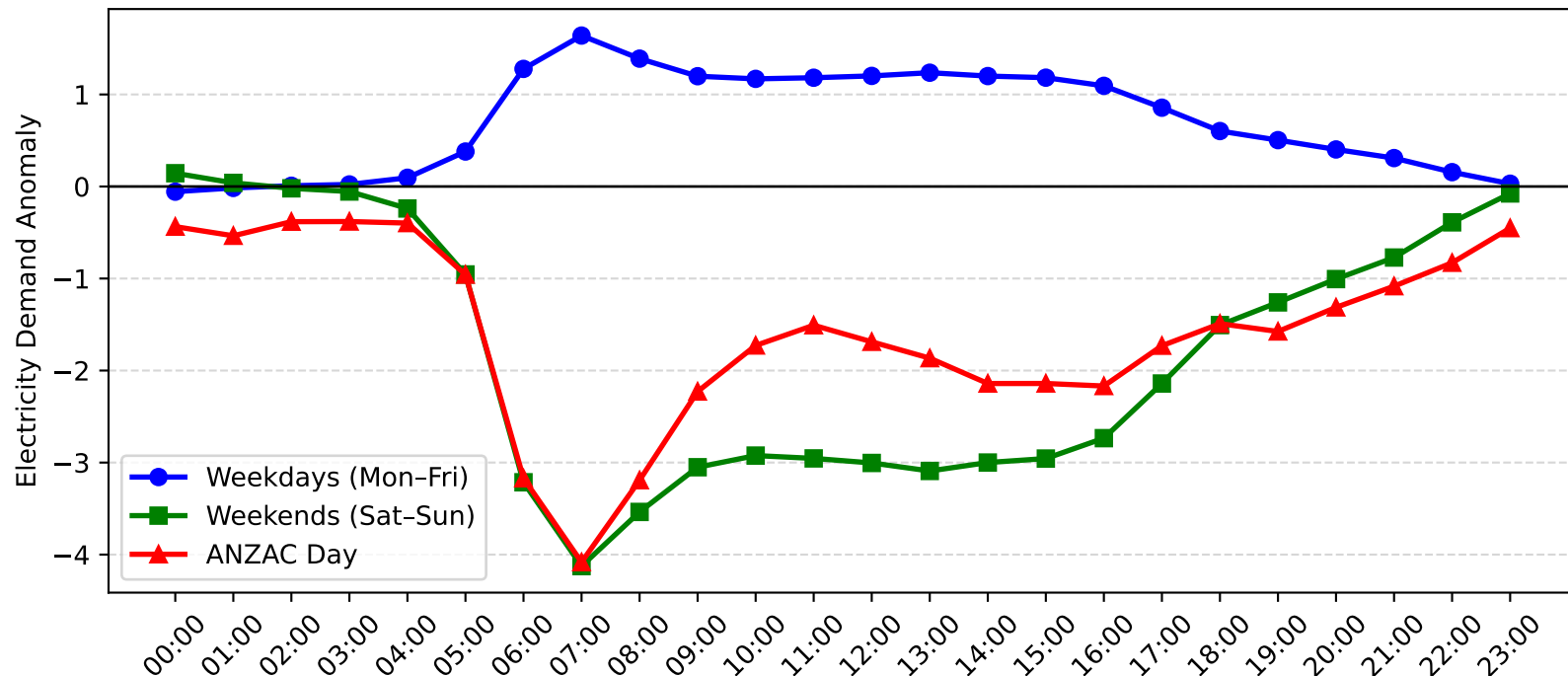
Pymble Demand Anomaly: ANZAC Day vs Weekday/Weekend (2011-2012)
