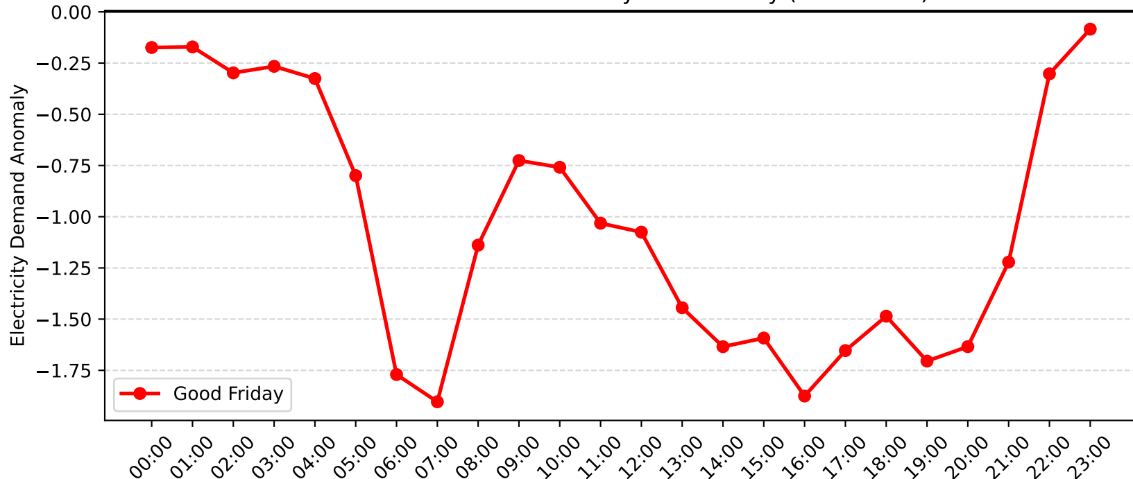
Narrabeen Demand Anomaly: Good Friday (2006-2007)
