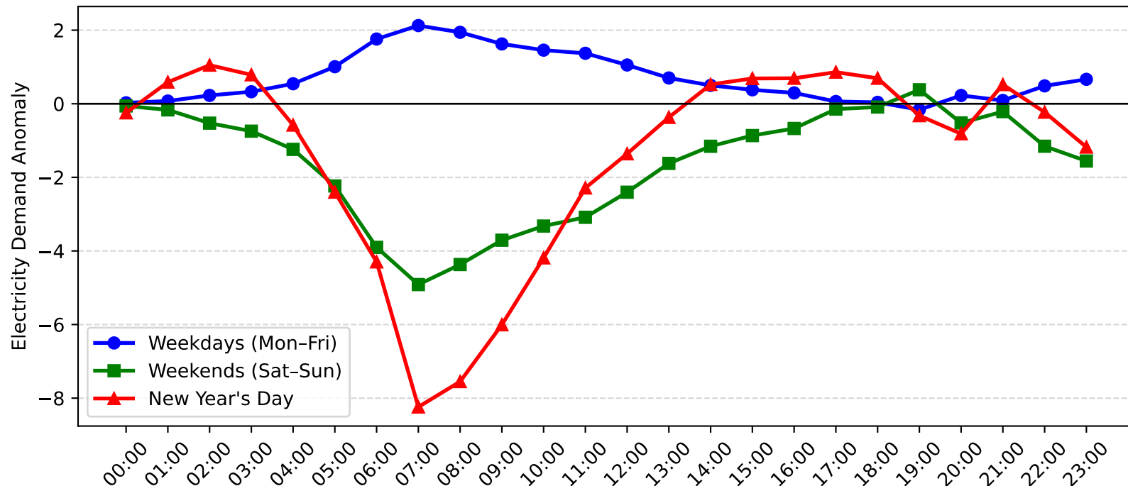
Meadowbank Demand Anomaly: New Year's Day vs Weekday/Weekend (2011-2012)
