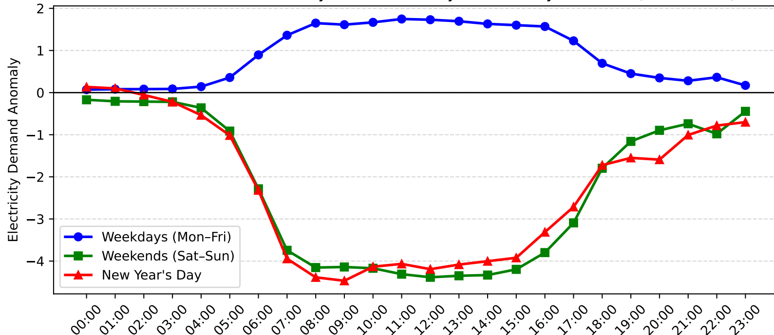
Beacon Hill Demand Anomaly: New Year's Day vs Weekday/Weekend (2010-2011)
