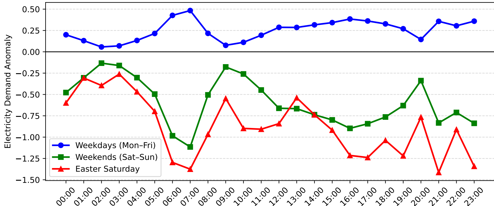
Jesmond Demand Anomaly: Easter Saturday vs Weekday/Weekend (2011-2012)
