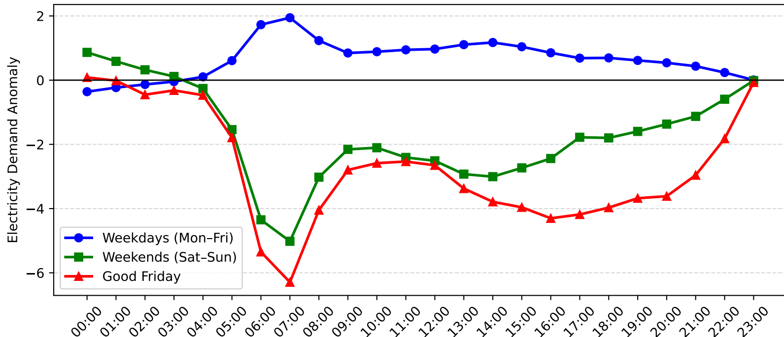
Mortdale Demand Anomaly: Good Friday vs Weekday/Weekend (2005-2006)
