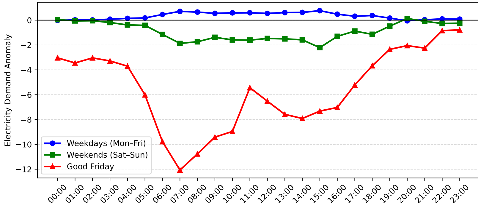
Campsie Demand Anomaly: Good Friday vs Weekday/Weekend (2004-2005)
