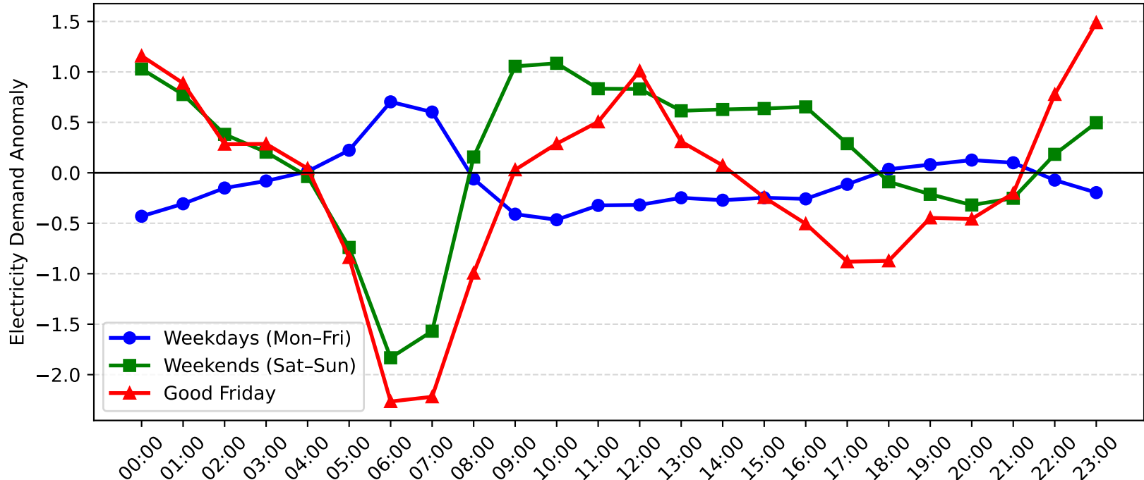
Avoca Demand Anomaly: Good Friday vs Weekday/Weekend (2012-2013)
