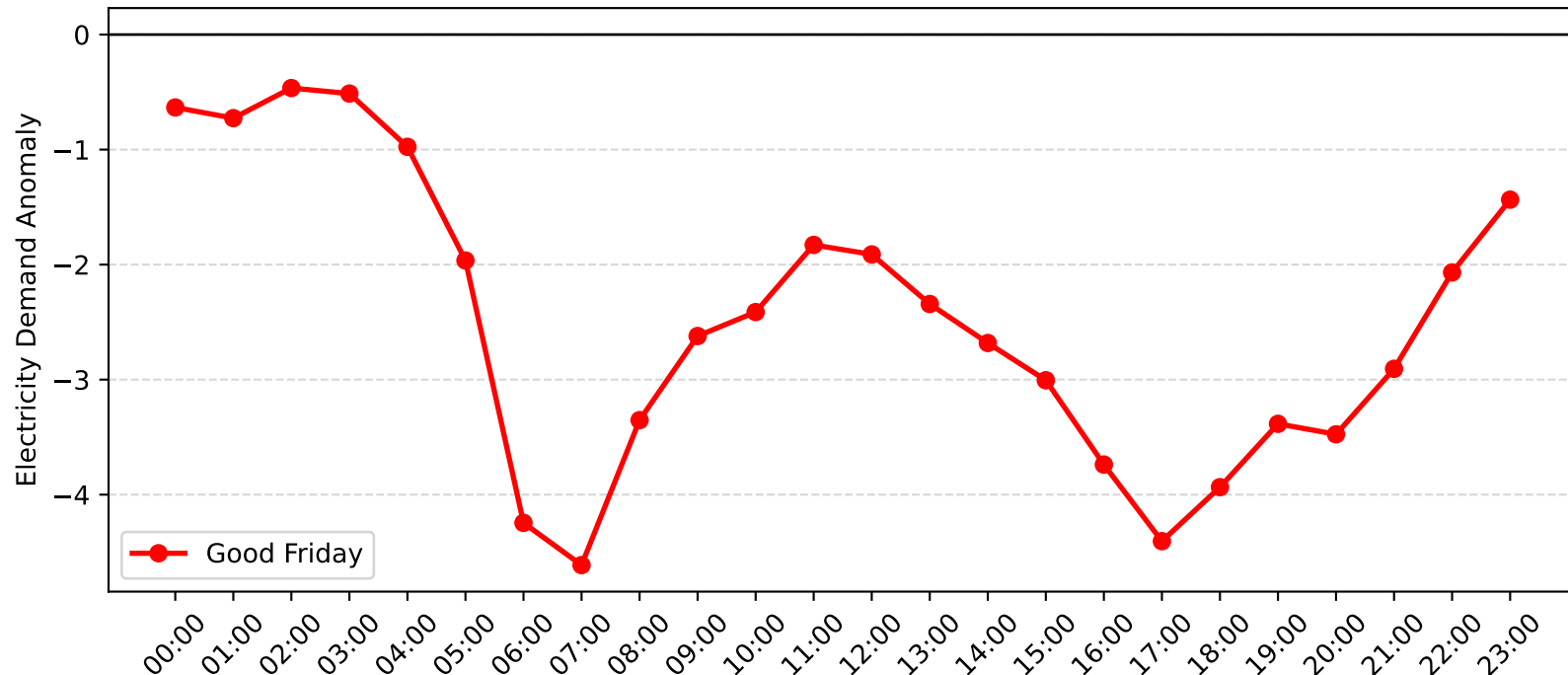
Revesby Demand Anomaly: Good Friday (2012-2013)
