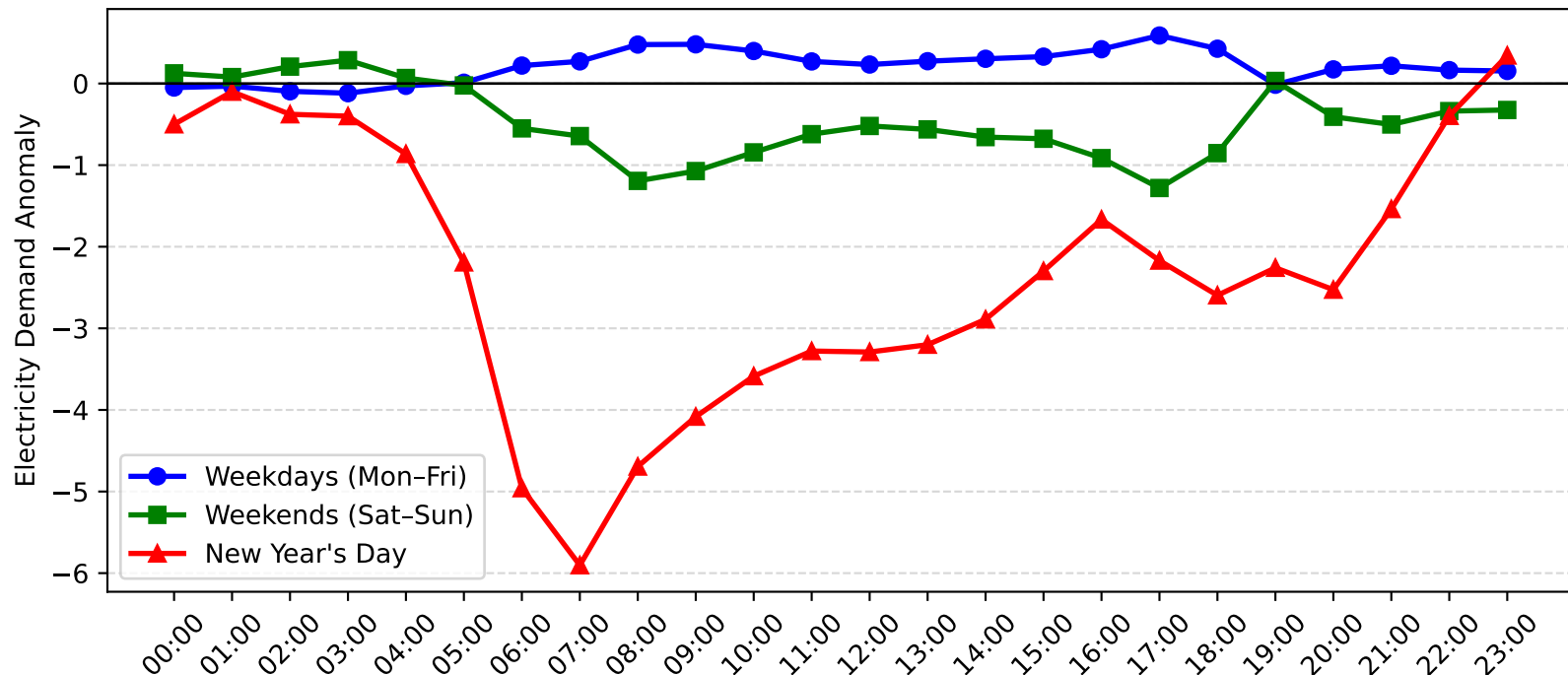
Mortdale Demand Anomaly: New Year's Day vs Weekday/Weekend (2004-2005)
