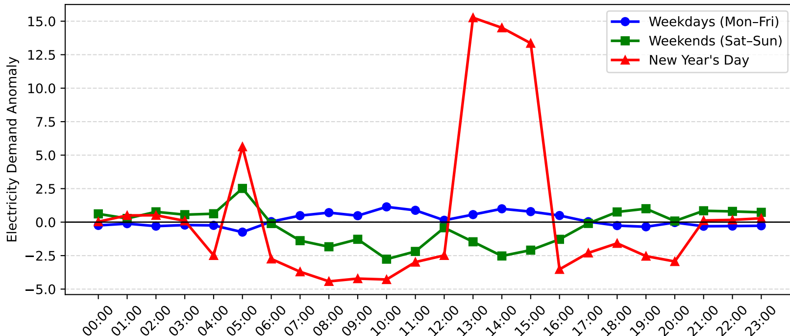
Kogarah Demand Anomaly: New Year's Day vs Weekday/Weekend (2010-2011)
