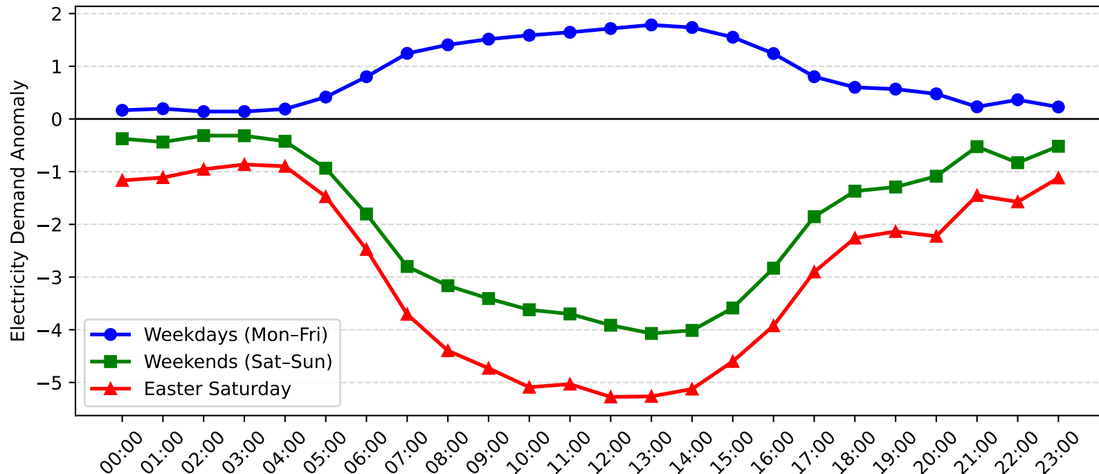
Broadmeadow Demand Anomaly: Easter Saturday vs Weekday/Weekend (2016-2017)
