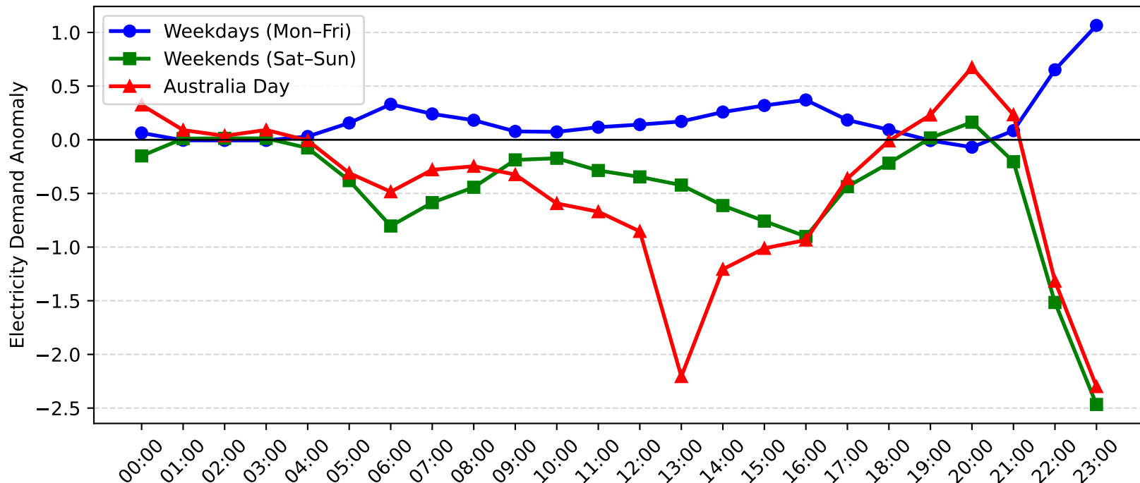
Muswellbrook Demand Anomaly: Australia Day vs Weekday/Weekend (2007-2008)
