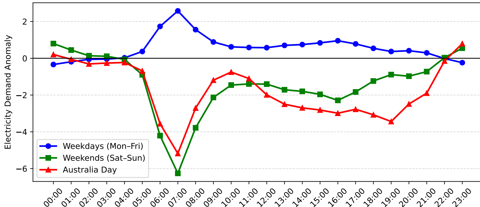
Mosman Demand Anomaly: Australia Day vs Weekday/Weekend (2007-2008)
