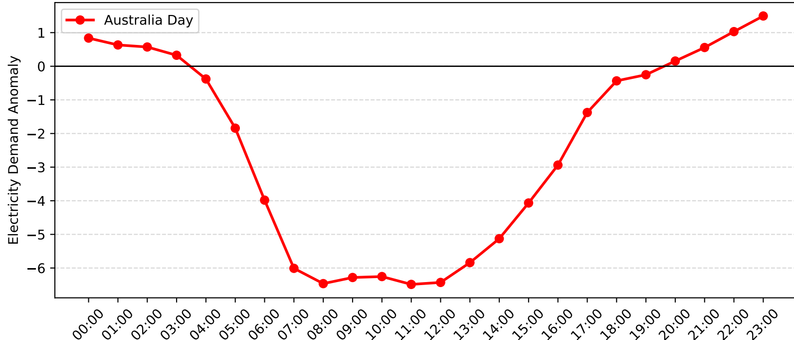
Homebush Bay Demand Anomaly: Australia Day (2012-2013)
