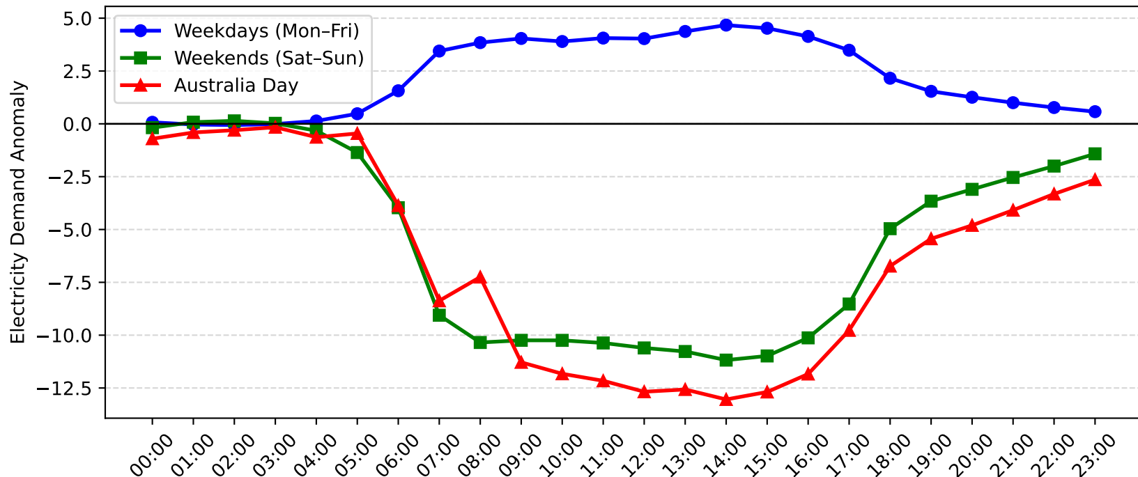
Gore Hill Demand Anomaly: Australia Day vs Weekday/Weekend (2014-2015)
