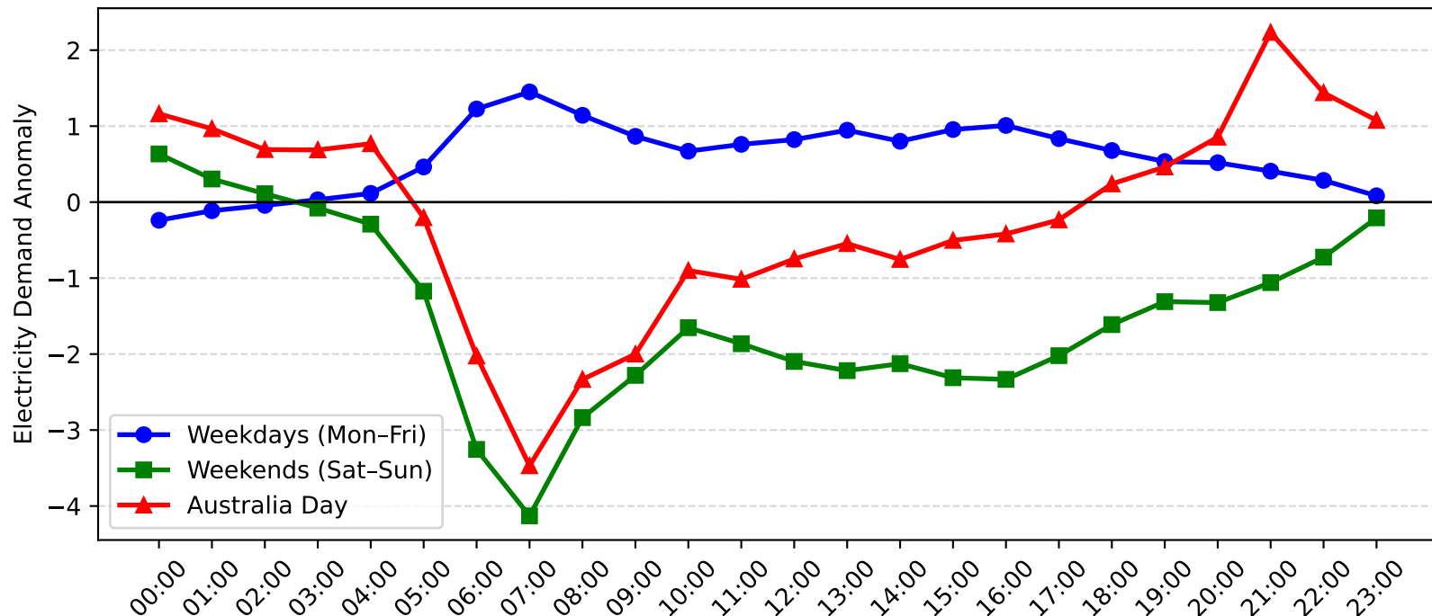
Dulwich Hill Demand Anomaly: Australia Day vs Weekday/Weekend (2009-2010)
