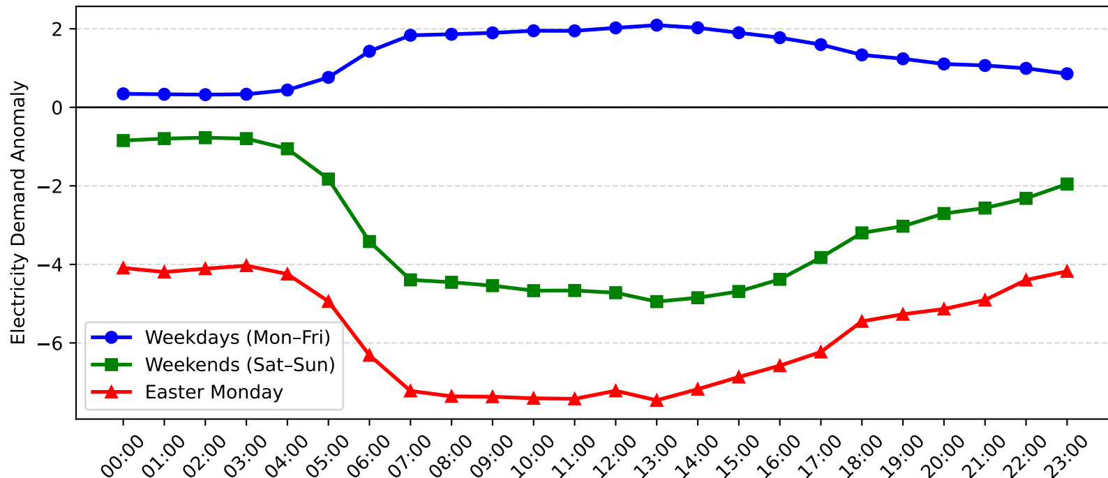
Leightonfield Demand Anomaly: Easter Monday vs Weekday/Weekend (2007-2008)
