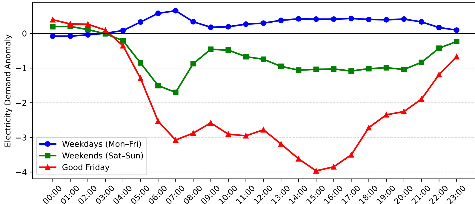
Charmhaven Demand Anomaly: Good Friday vs Weekday/Weekend (2012-2013)
