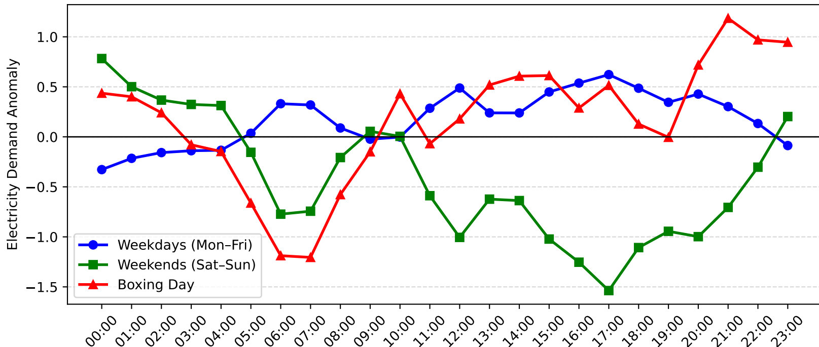
Avoca Demand Anomaly: Boxing Day vs Weekday/Weekend (2016-2017)
