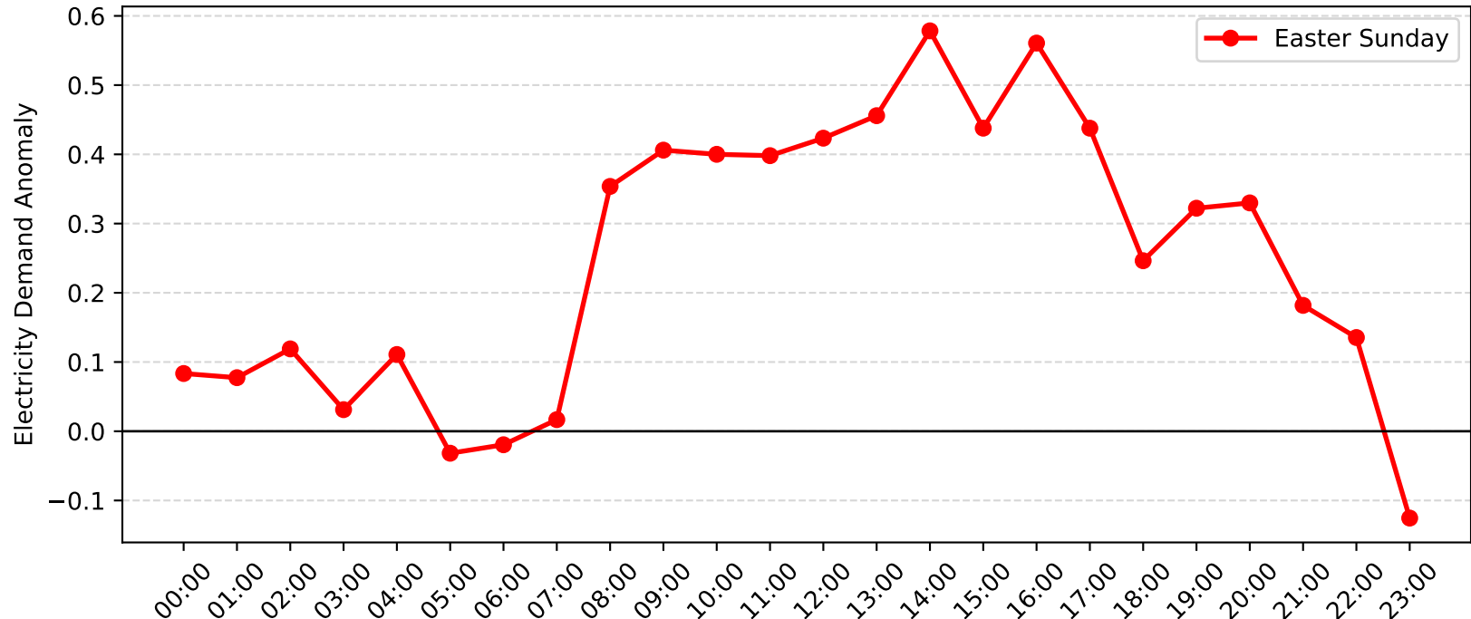
Rothbury Demand Anomaly: Easter Sunday (2012-2013)
