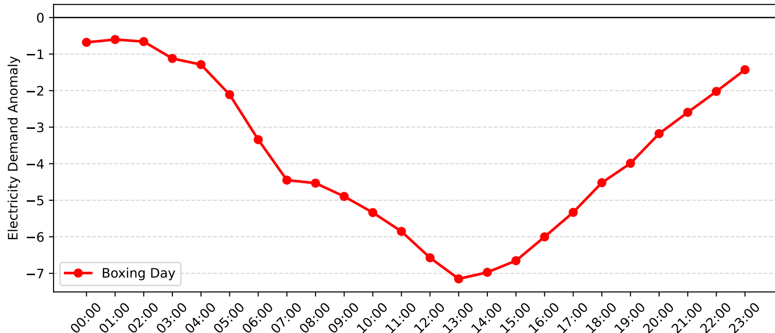
Wyong Demand Anomaly: Boxing Day (2012-2013)
