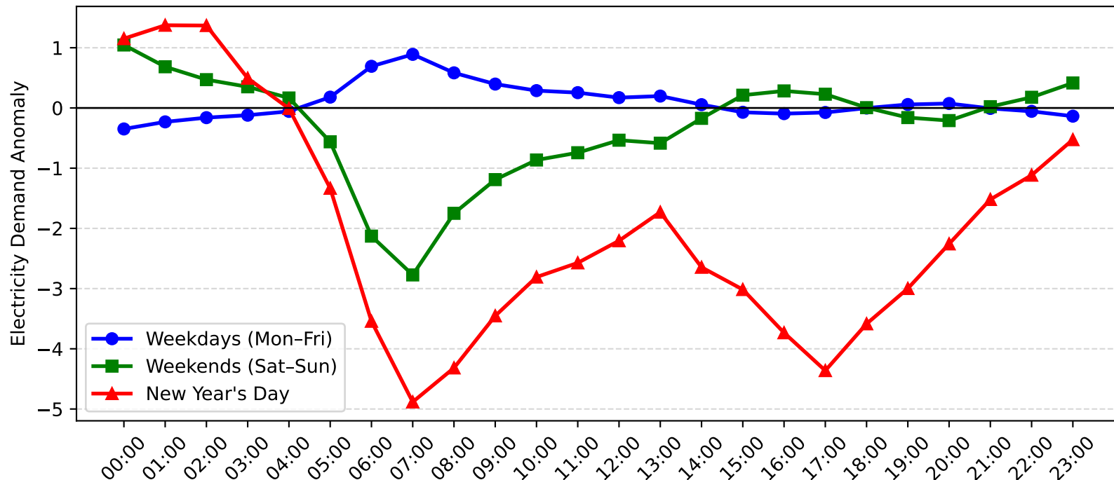
Mortdale Demand Anomaly: New Year's Day vs Weekday/Weekend (2014-2015)
