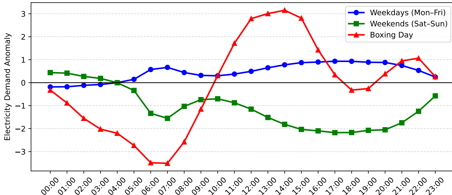
Mortdale Demand Anomaly: Boxing Day vs Weekday/Weekend (2016-2017)
