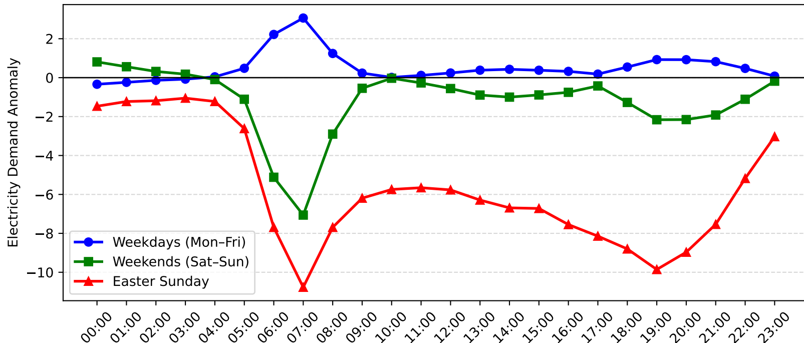
Mosman Demand Anomaly: Easter Sunday vs Weekday/Weekend (2011-2012)
