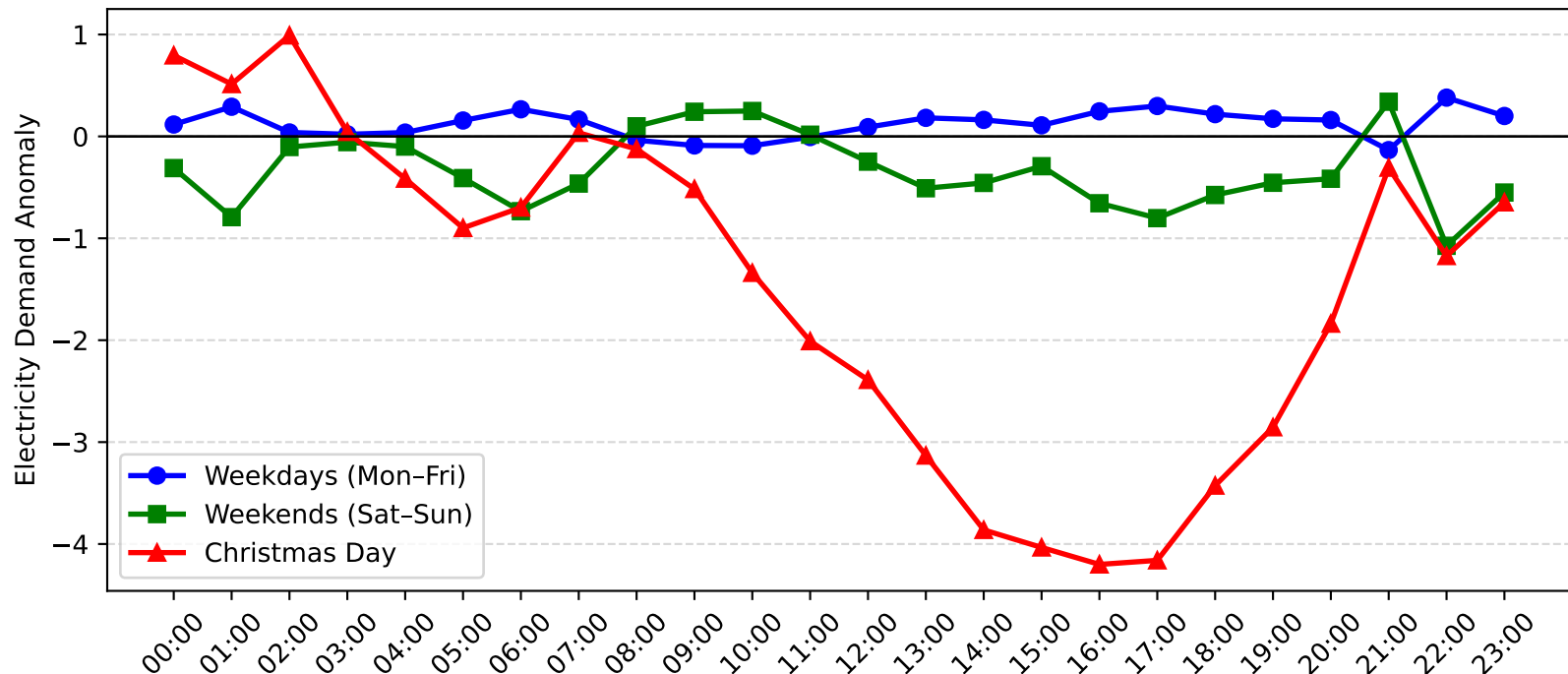
Nelson Bay Demand Anomaly: Christmas Day vs Weekday/Weekend (2014-2015)
