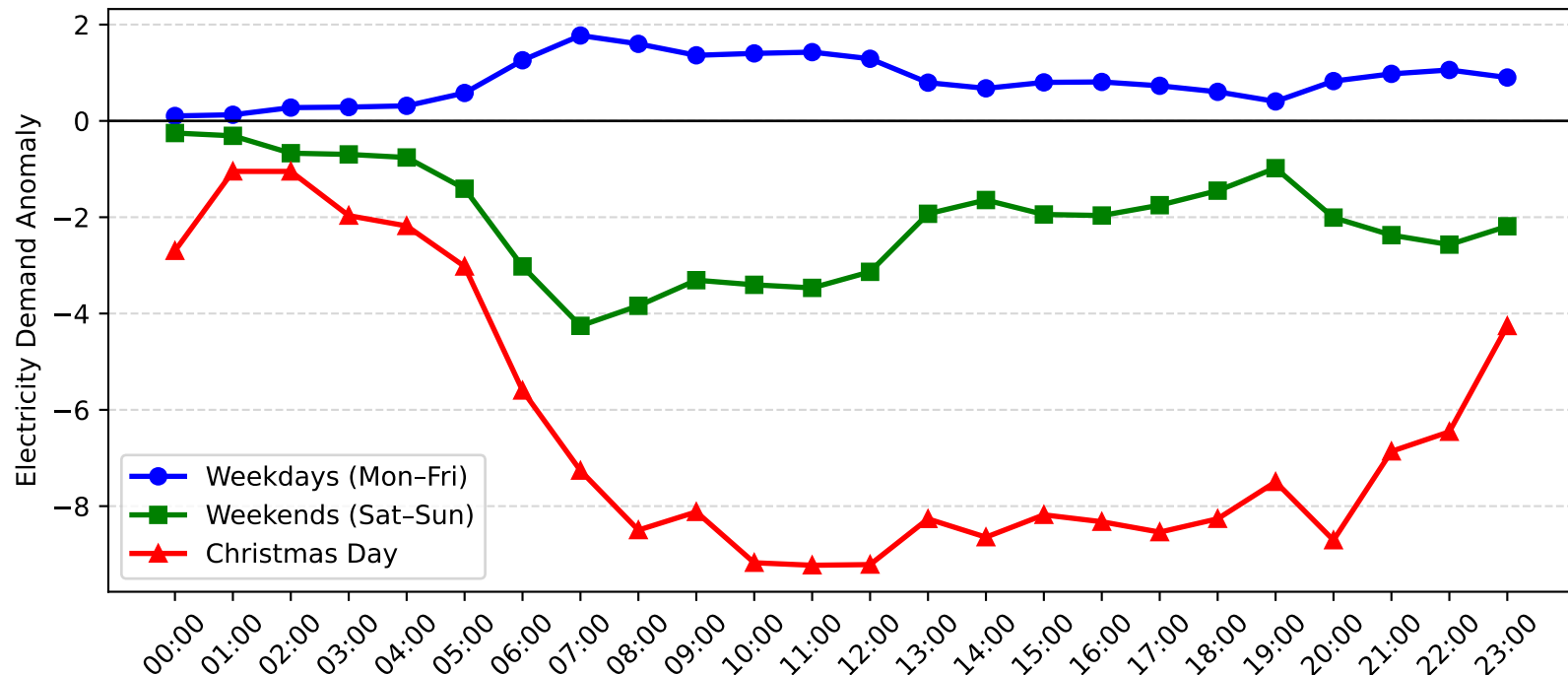
Meadowbank Demand Anomaly: Christmas Day vs Weekday/Weekend (2015-2016)
