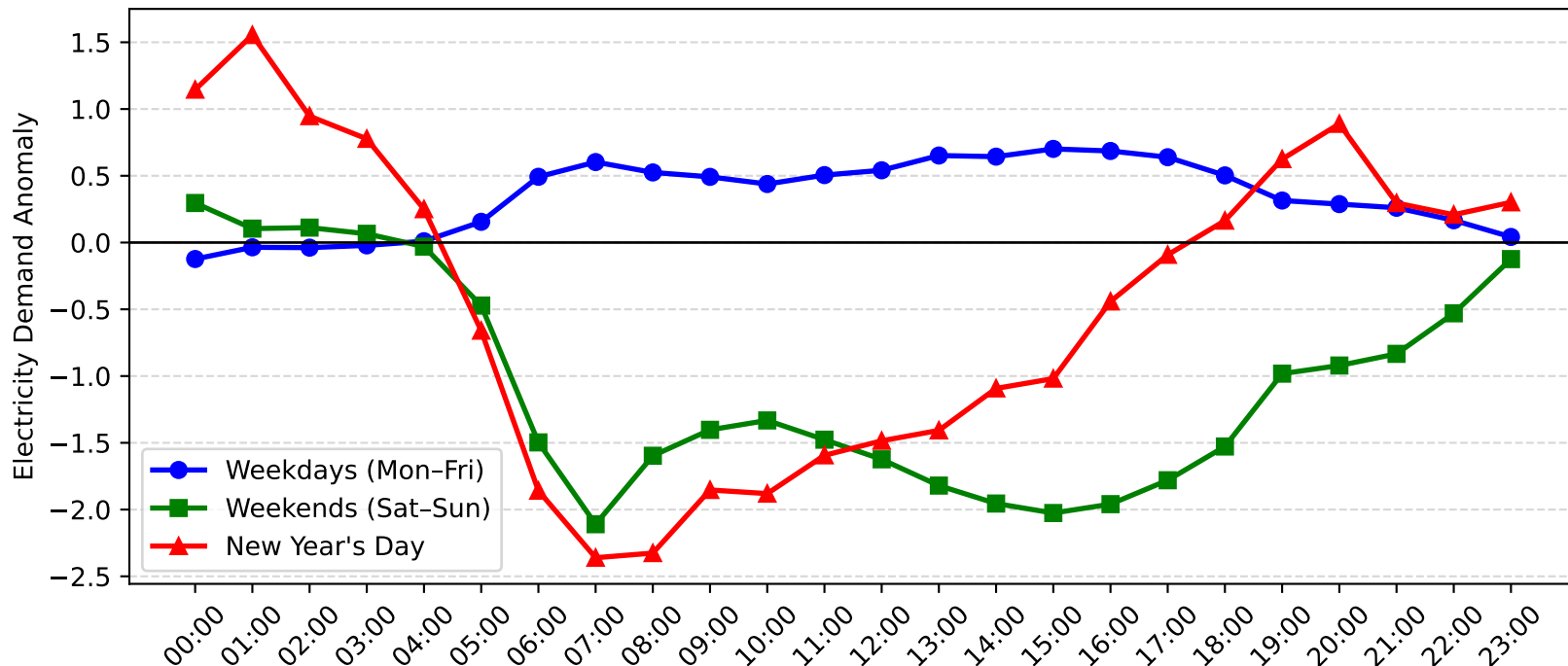
Blakehurst Demand Anomaly: New Year's Day vs Weekday/Weekend (2009-2010)
