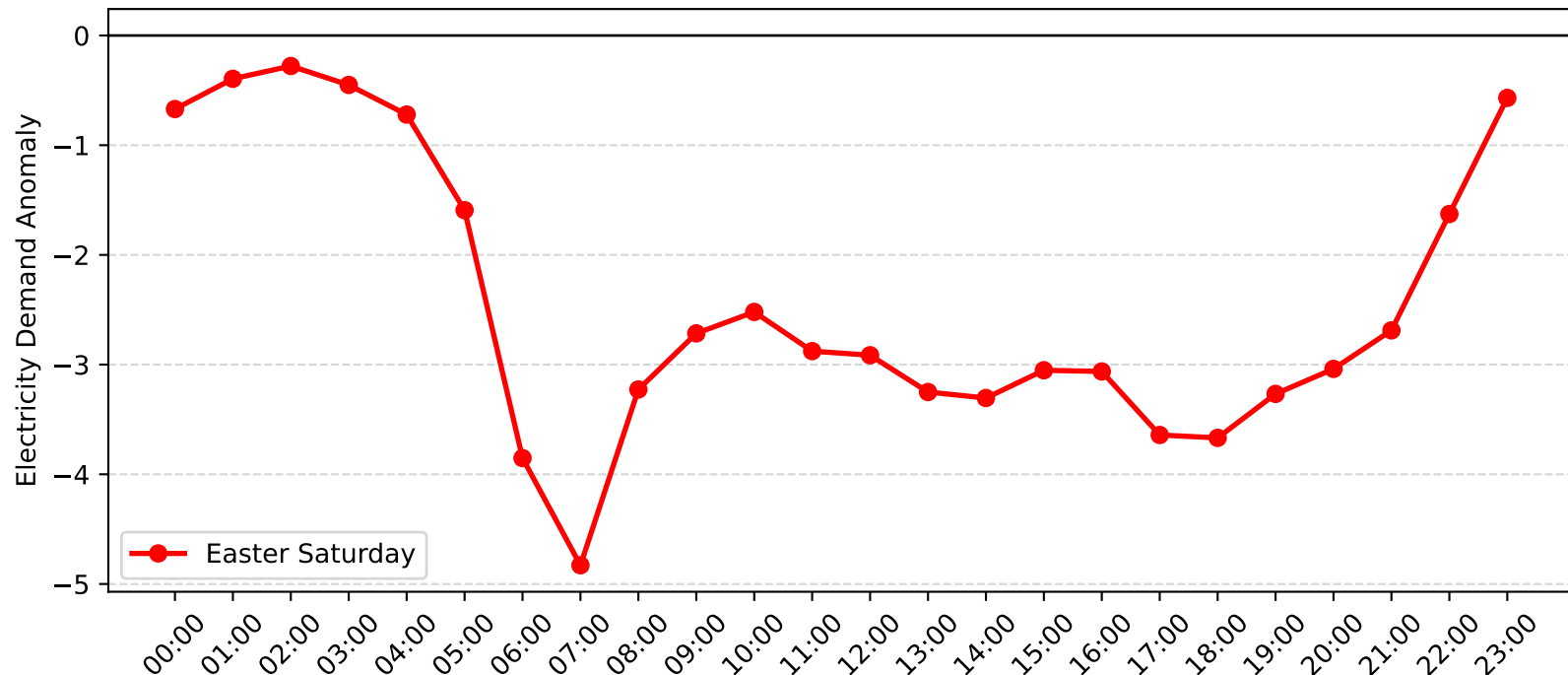
Mortdale Demand Anomaly: Easter Saturday (2013-2014)
