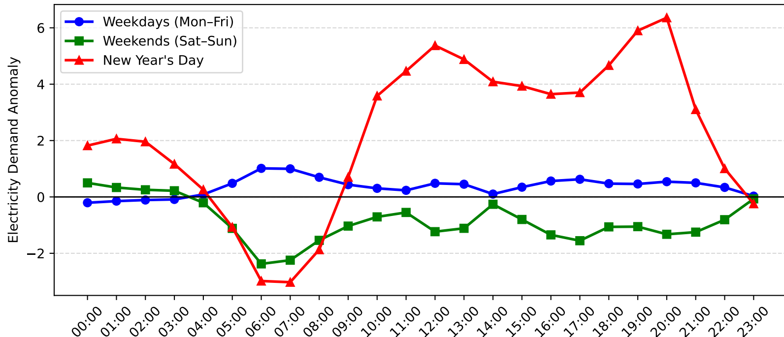
Revesby Demand Anomaly: New Year's Day vs Weekday/Weekend (2006-2007)
