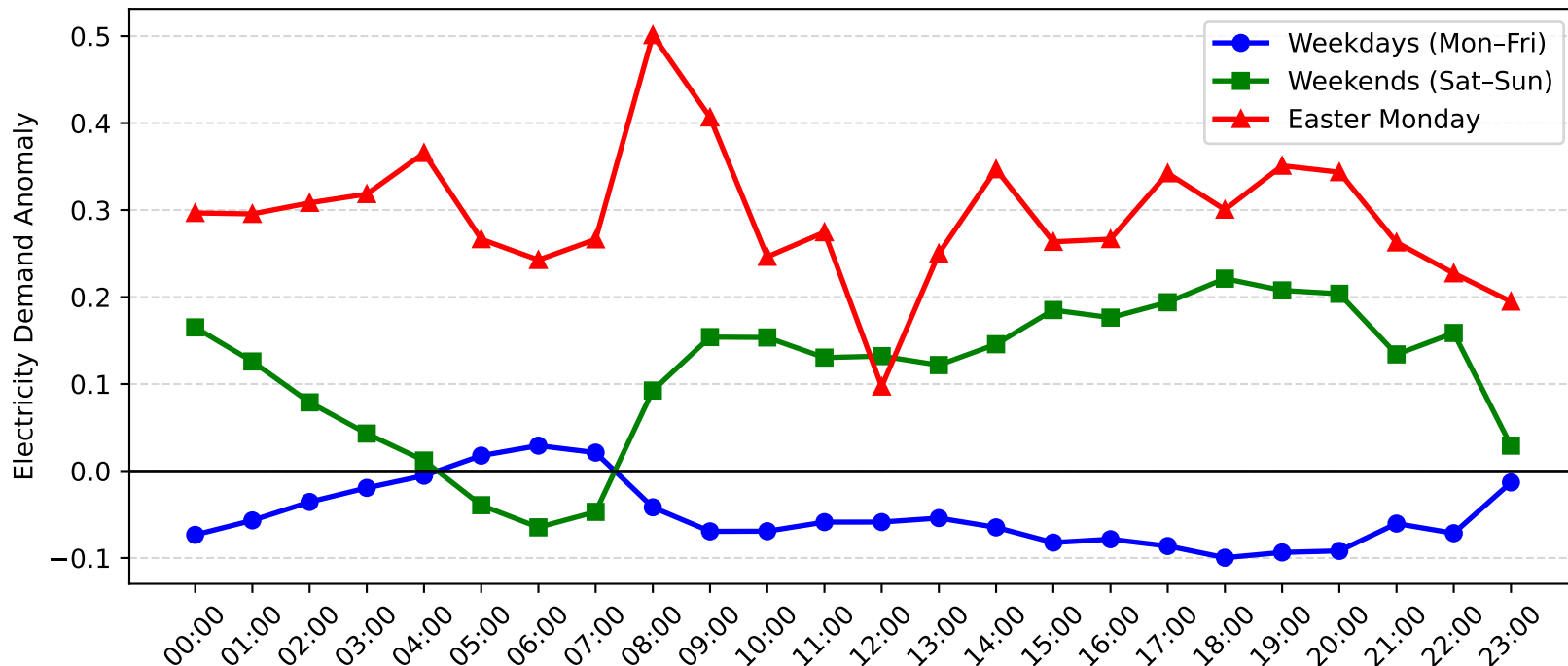
Rothbury Demand Anomaly: Easter Monday vs Weekday/Weekend (2016-2017)
