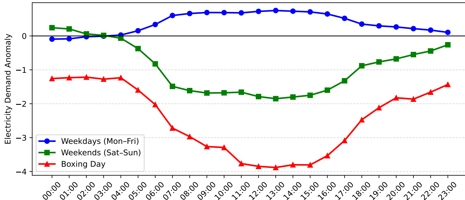
Lidcombe Demand Anomaly: Boxing Day vs Weekday/Weekend (2011-2012)
