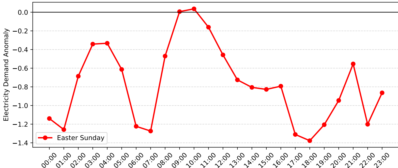
Jewells Demand Anomaly: Easter Sunday (2013-2014)
