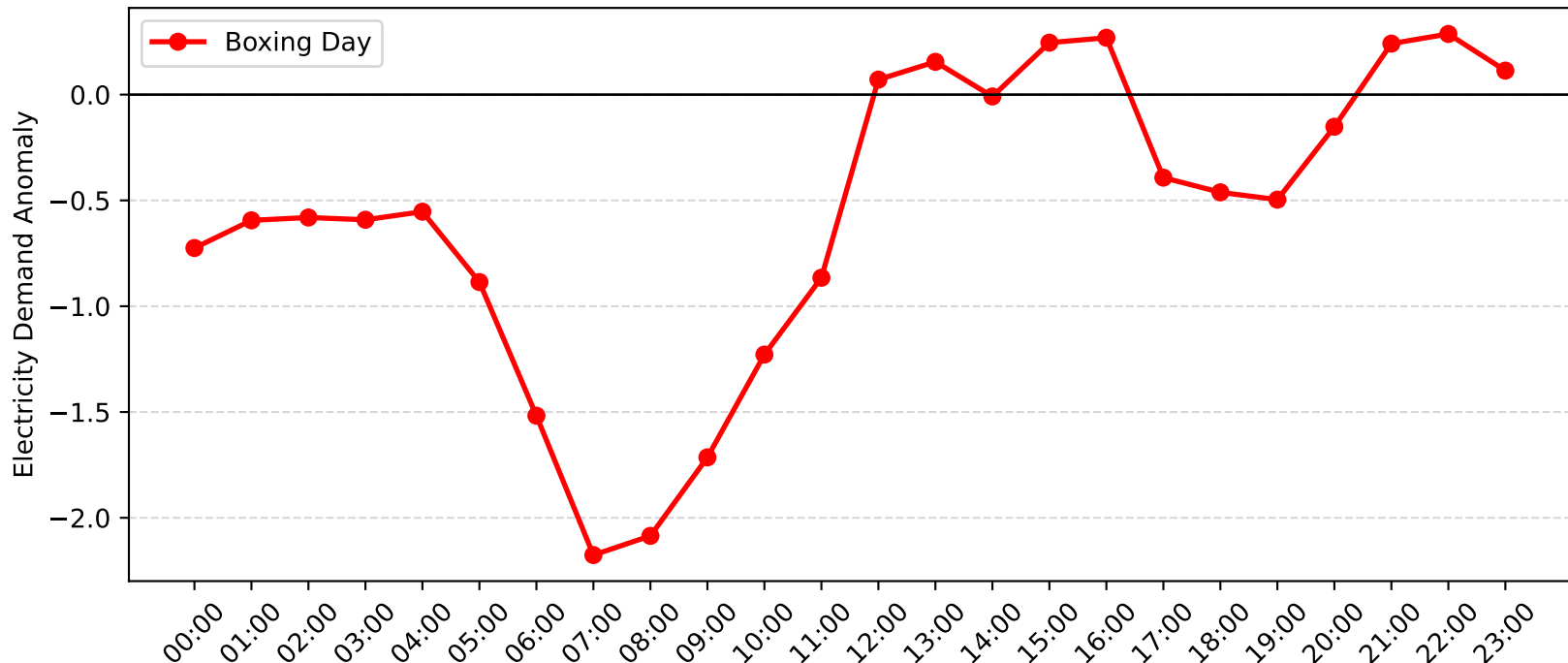
Pymble Demand Anomaly: Boxing Day (2016-2017)
