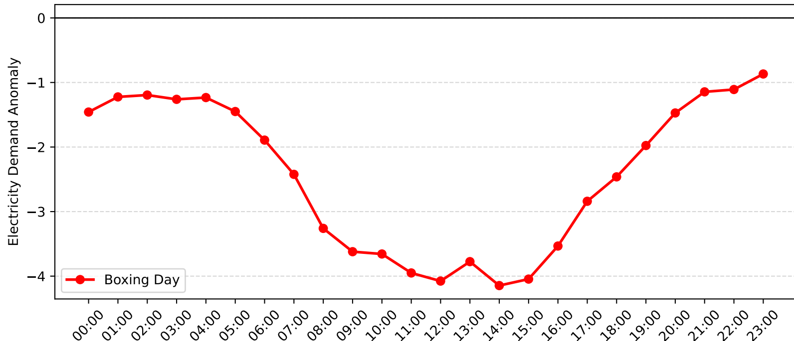
Lidcombe Demand Anomaly: Boxing Day (2013-2014)
