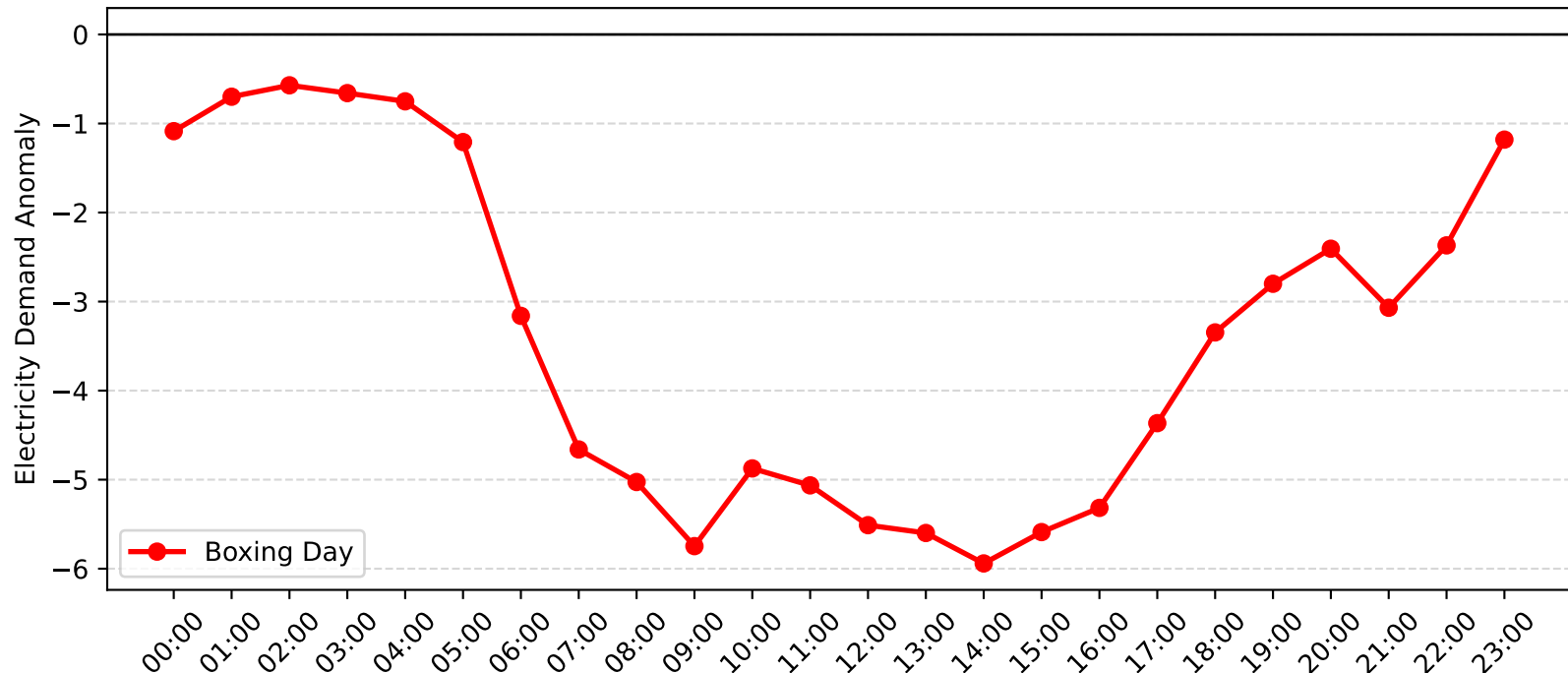
Pymble Demand Anomaly: Boxing Day (2008-2009)
