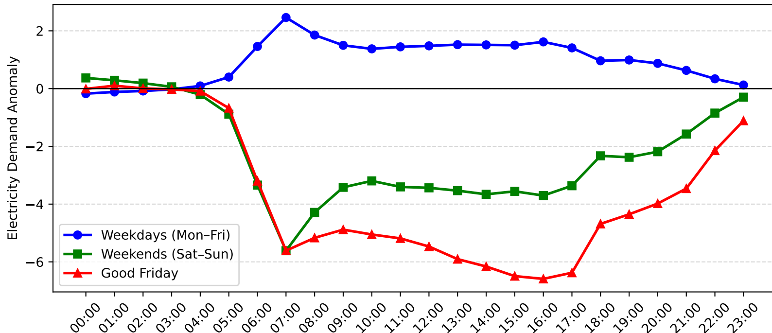
Chatswood Demand Anomaly: Good Friday vs Weekday/Weekend (2009-2010)
