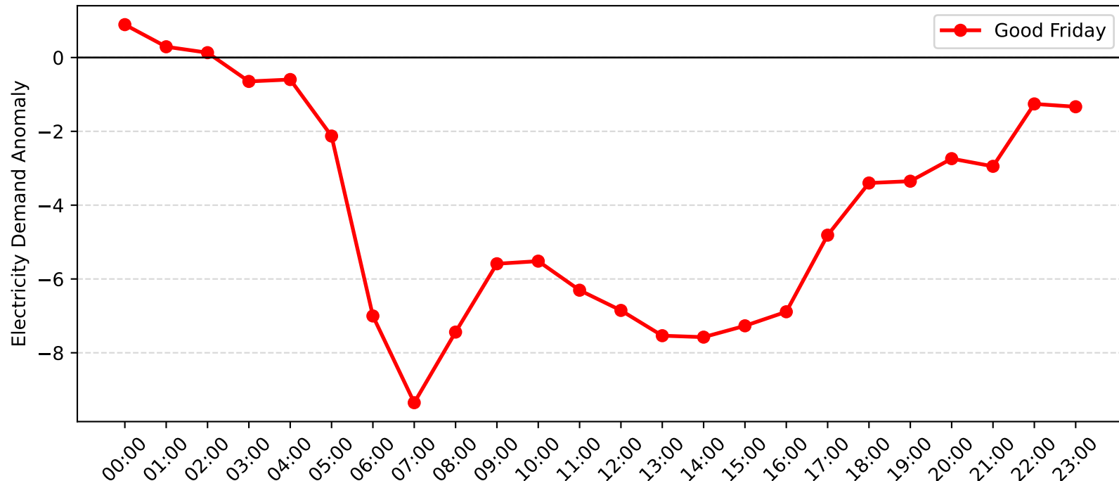
Chatswood Demand Anomaly: Good Friday (2004-2005)
