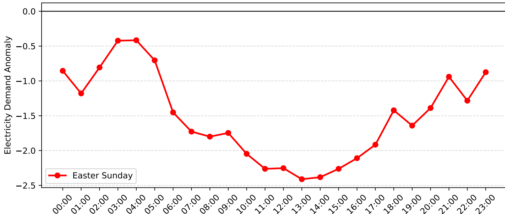
Gateshead Demand Anomaly: Easter Sunday (2009-2010)
