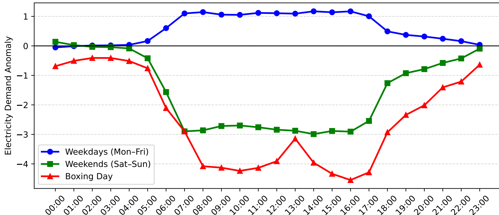
Pymble Demand Anomaly: Boxing Day vs Weekday/Weekend (2014-2015)
