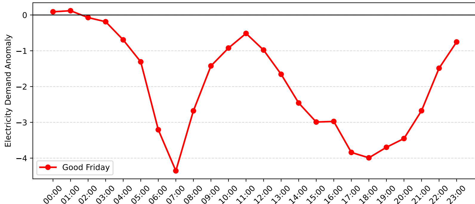
Dulwich Hill Demand Anomaly: Good Friday (2015-2016)
