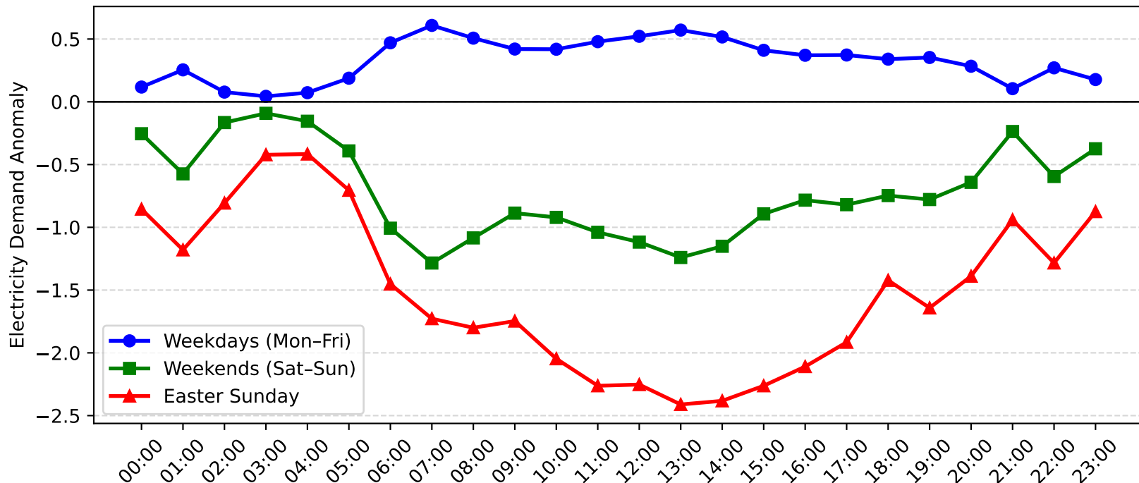
Gateshead Demand Anomaly: Easter Sunday vs Weekday/Weekend (2009-2010)
