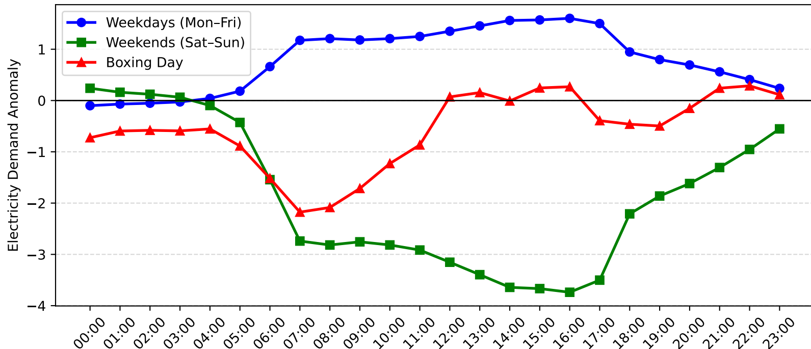
Pymble Demand Anomaly: Boxing Day vs Weekday/Weekend (2016-2017)
