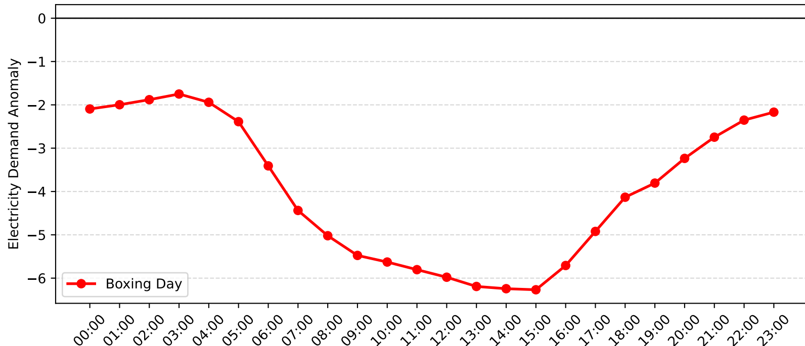
Lidcombe Demand Anomaly: Boxing Day (2006-2007)
