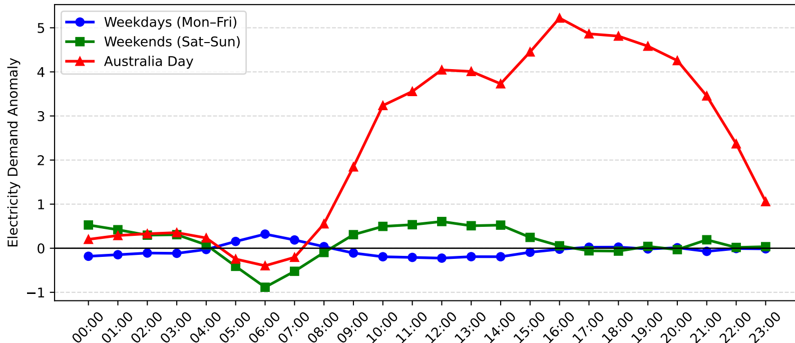
Woy Woy Demand Anomaly: Australia Day vs Weekday/Weekend (2010-2011)
