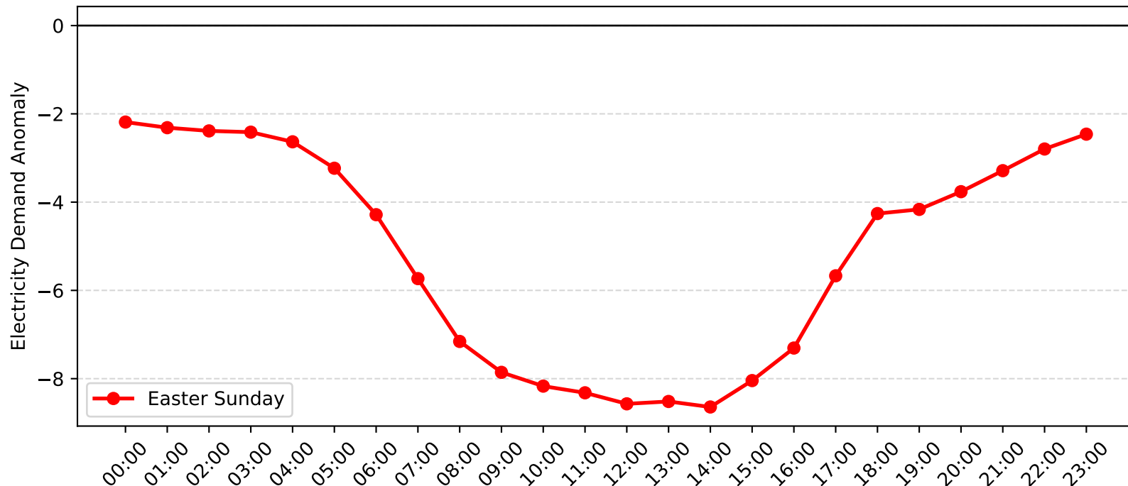
Caringbah Demand Anomaly: Easter Sunday (2009-2010)
