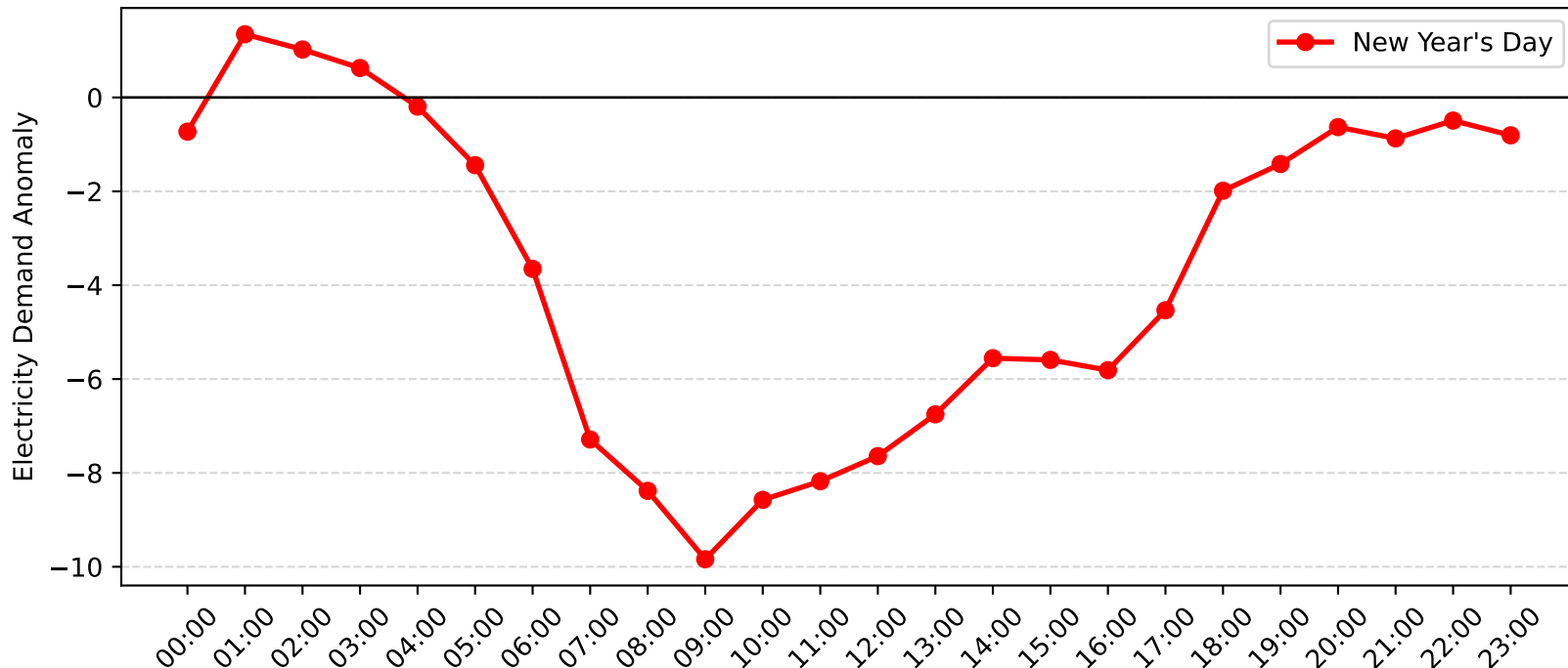
Burwood Demand Anomaly: New Year's Day (2009-2010)
