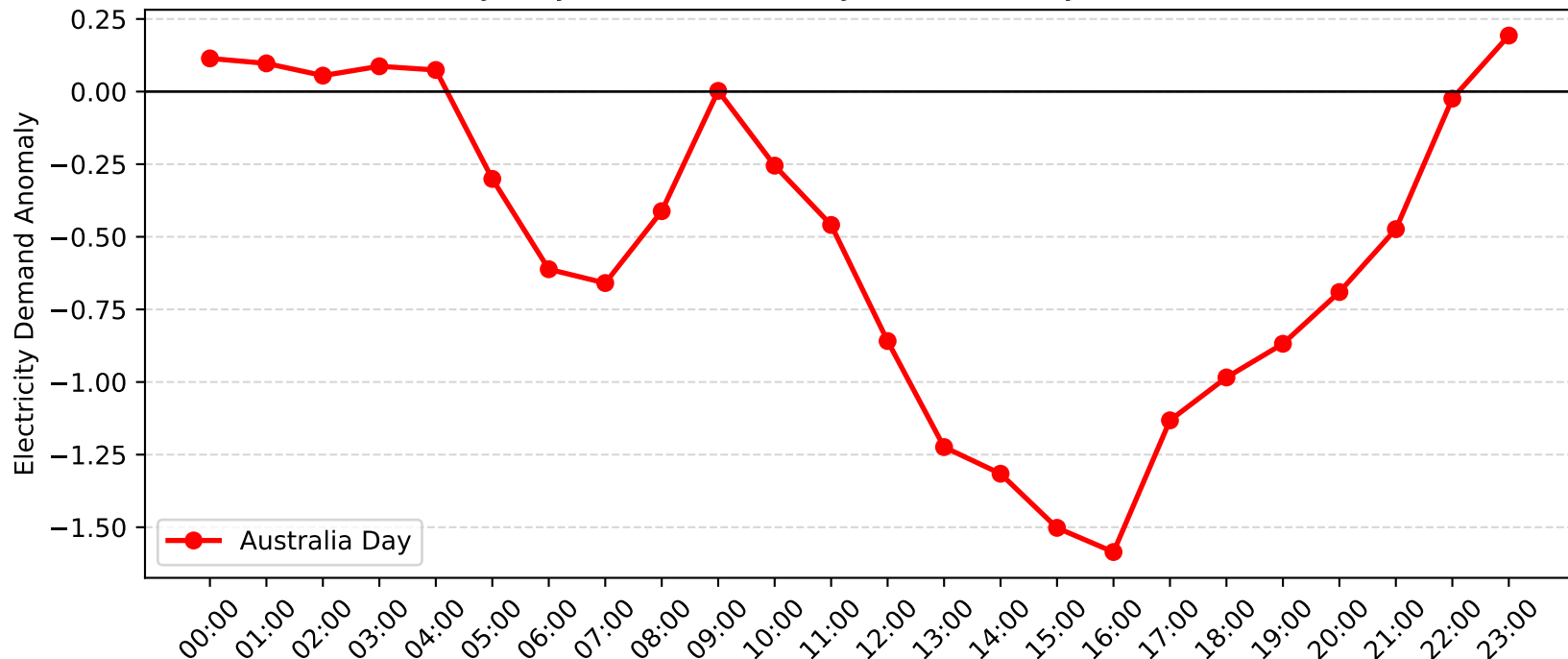
Woy Woy Demand Anomaly: Australia Day (2015-2016)
