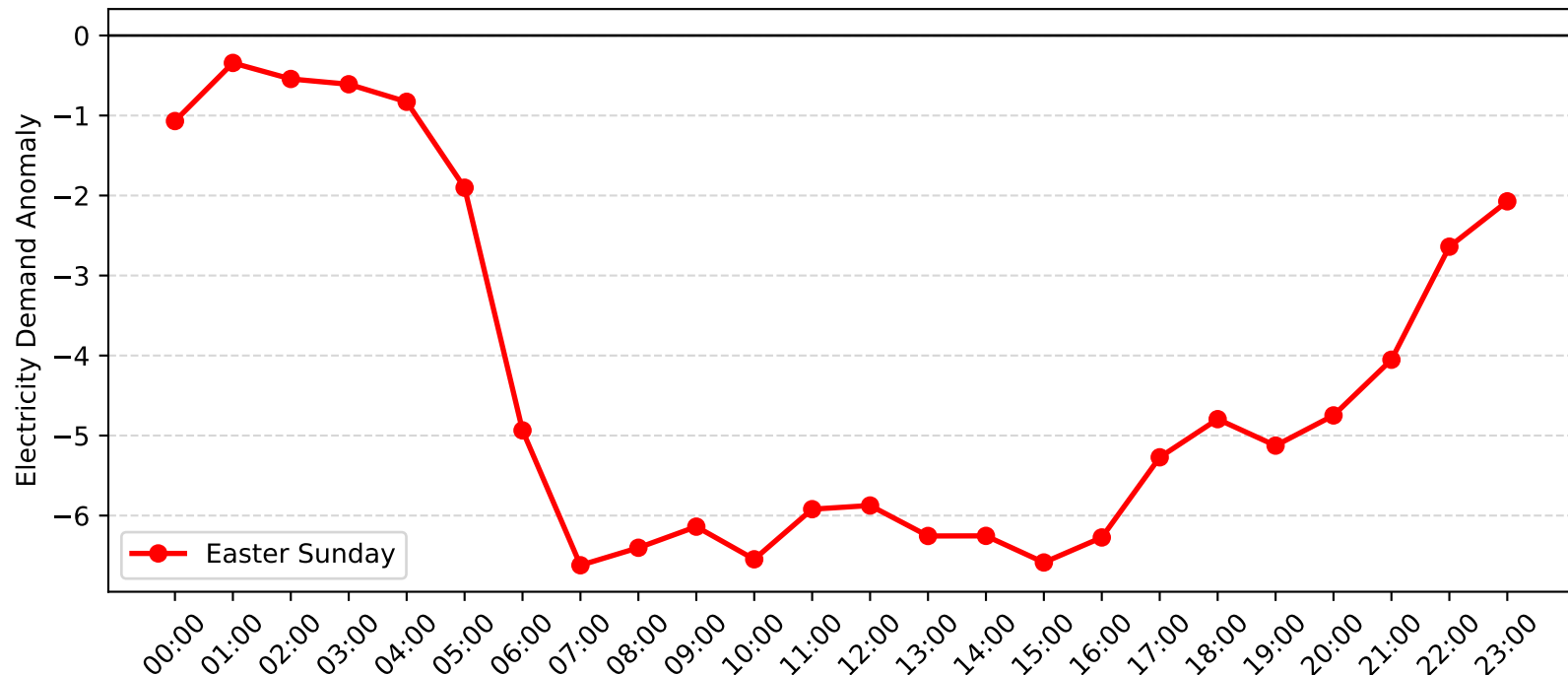
Dulwich Hill Demand Anomaly: Easter Sunday (2005-2006)
