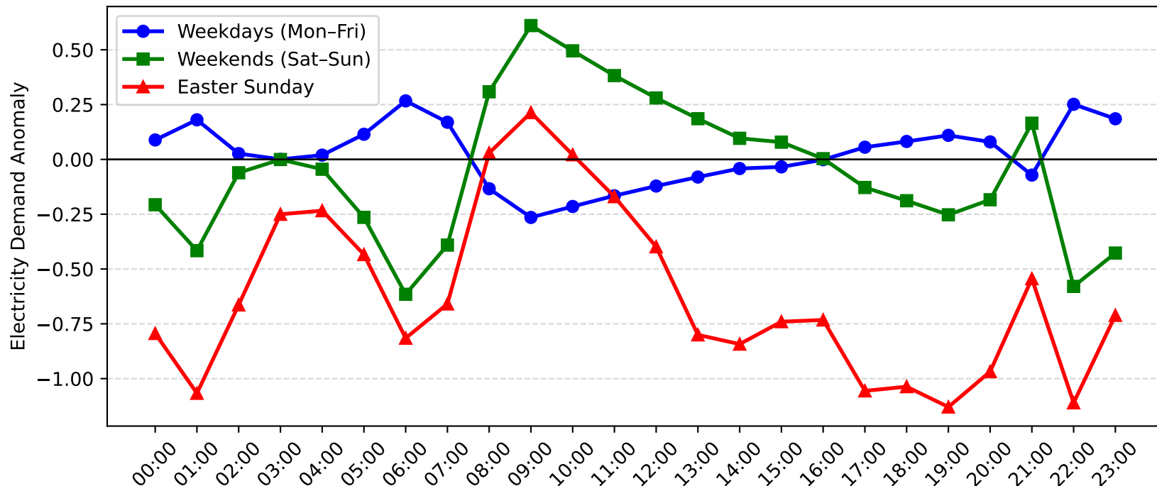
Jewells Demand Anomaly: Easter Sunday vs Weekday/Weekend (2014-2015)
