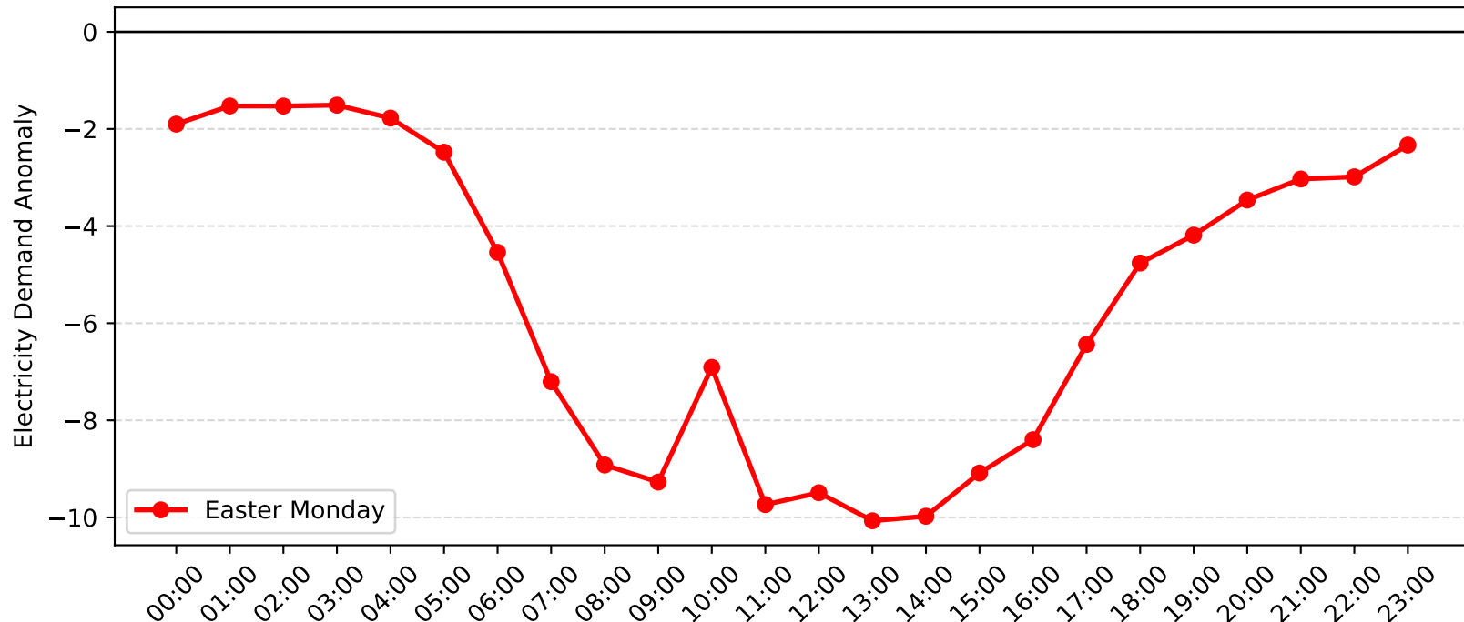
Mascot Demand Anomaly: Easter Monday (2006-2007)
