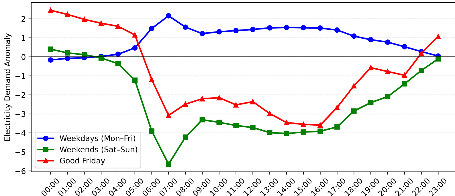
Chatswood Demand Anomaly: Good Friday vs Weekday/Weekend (2007-2008)
