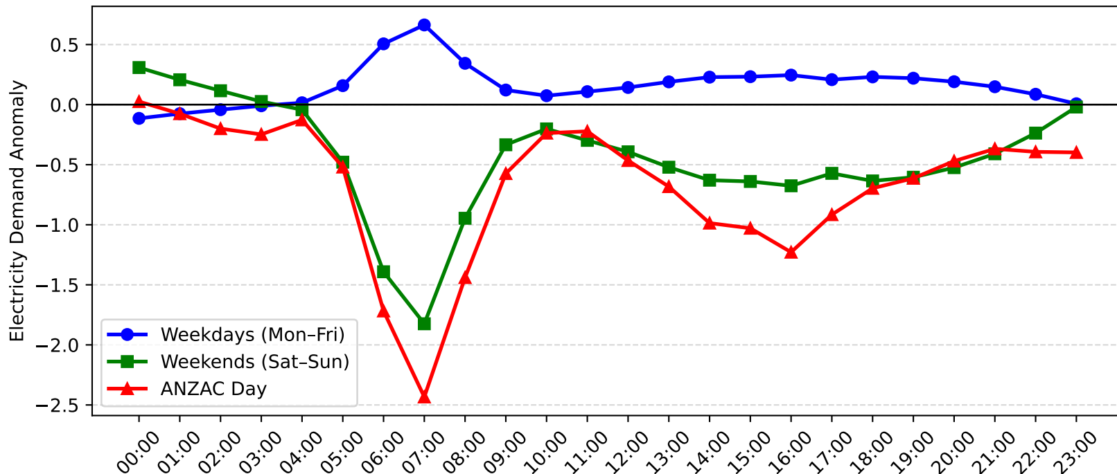
Blakehurst Demand Anomaly: ANZAC Day vs Weekday/Weekend (2012-2013)
