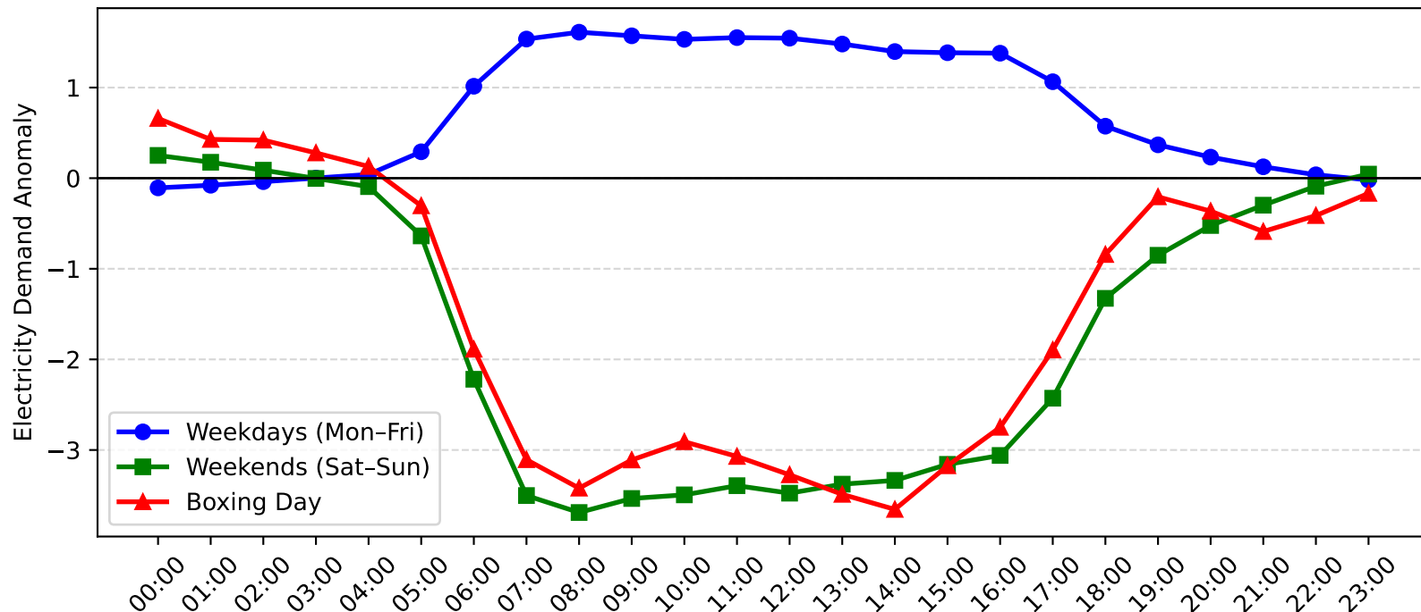
Pymble Demand Anomaly: Boxing Day vs Weekday/Weekend (2010-2011)
