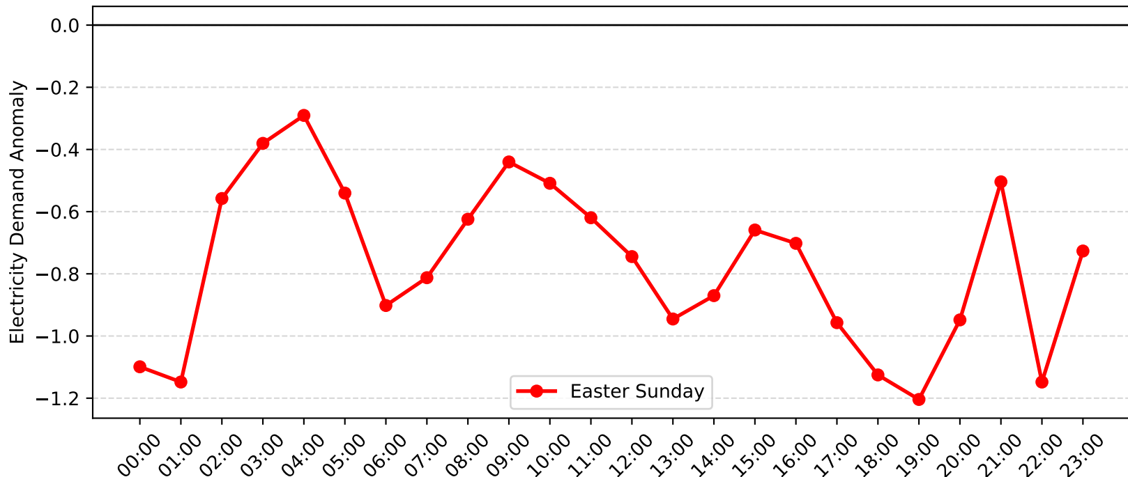
Jewells Demand Anomaly: Easter Sunday (2017-2018)
