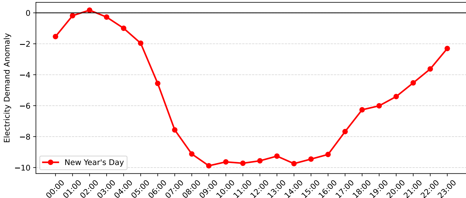
Burwood Demand Anomaly: New Year's Day (2015-2016)
