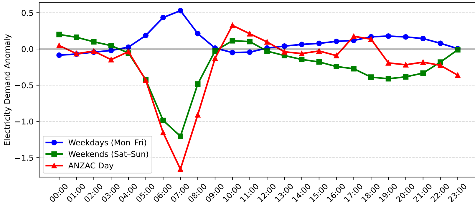
Blakehurst Demand Anomaly: ANZAC Day vs Weekday/Weekend (2016-2017)
