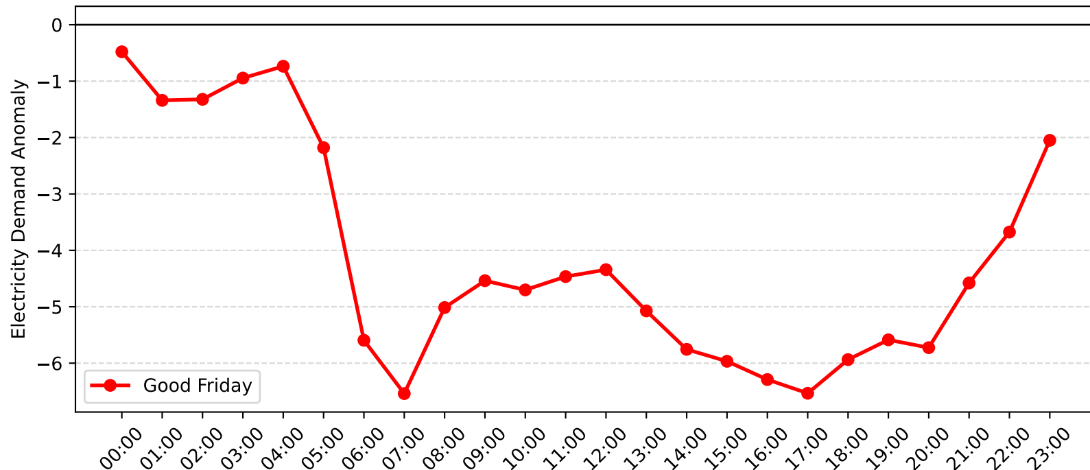
Pennant Hills Demand Anomaly: Good Friday (2012-2013)
