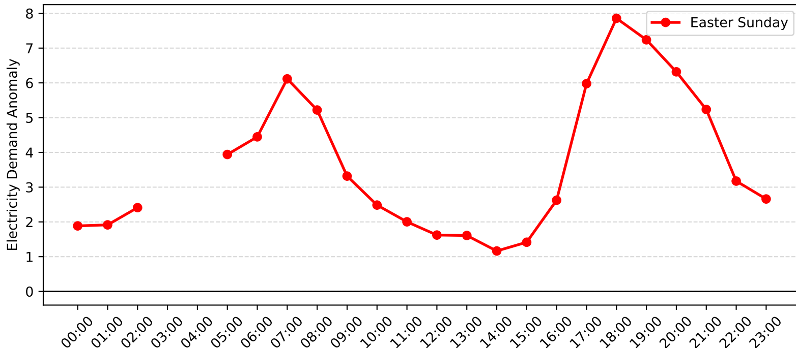
Caringbah Demand Anomaly: Easter Sunday (2004-2005)
