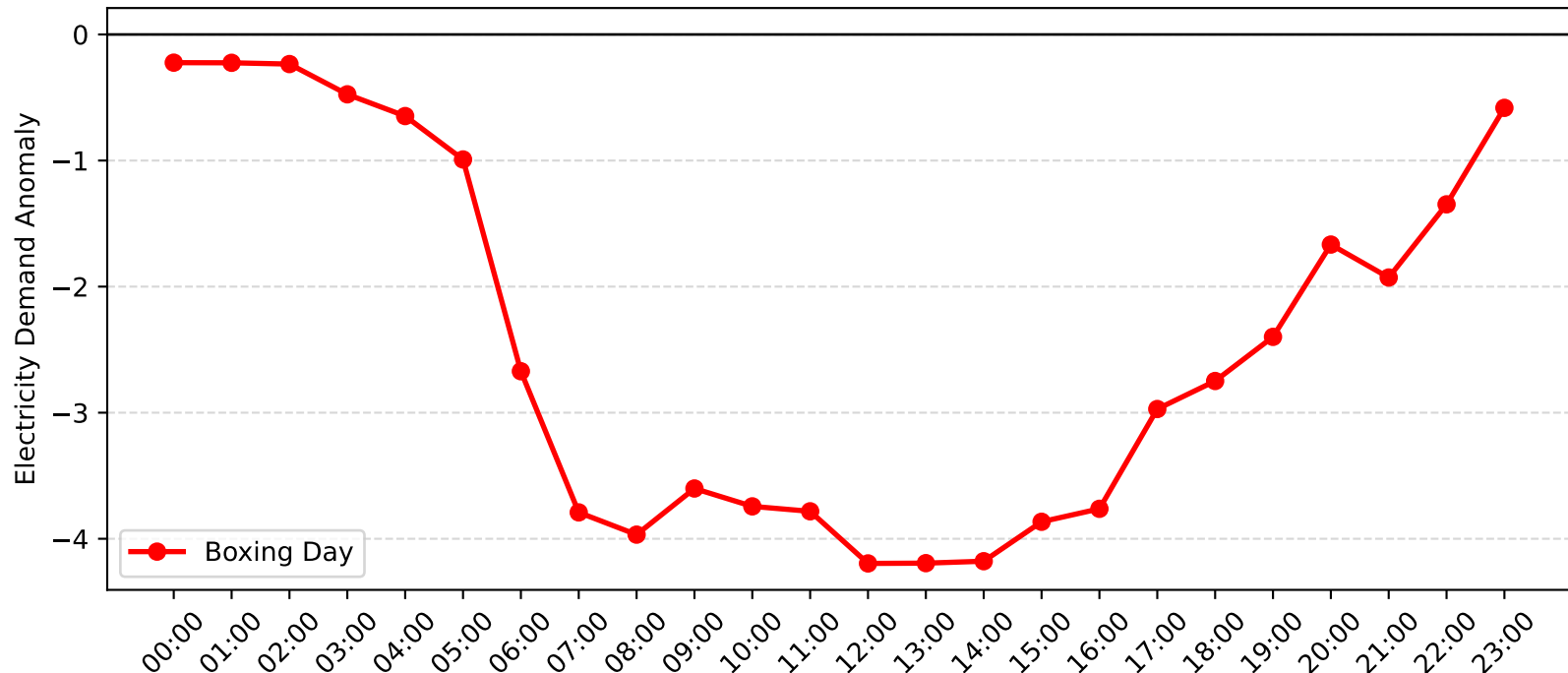
Pymble Demand Anomaly: Boxing Day (2007-2008)
