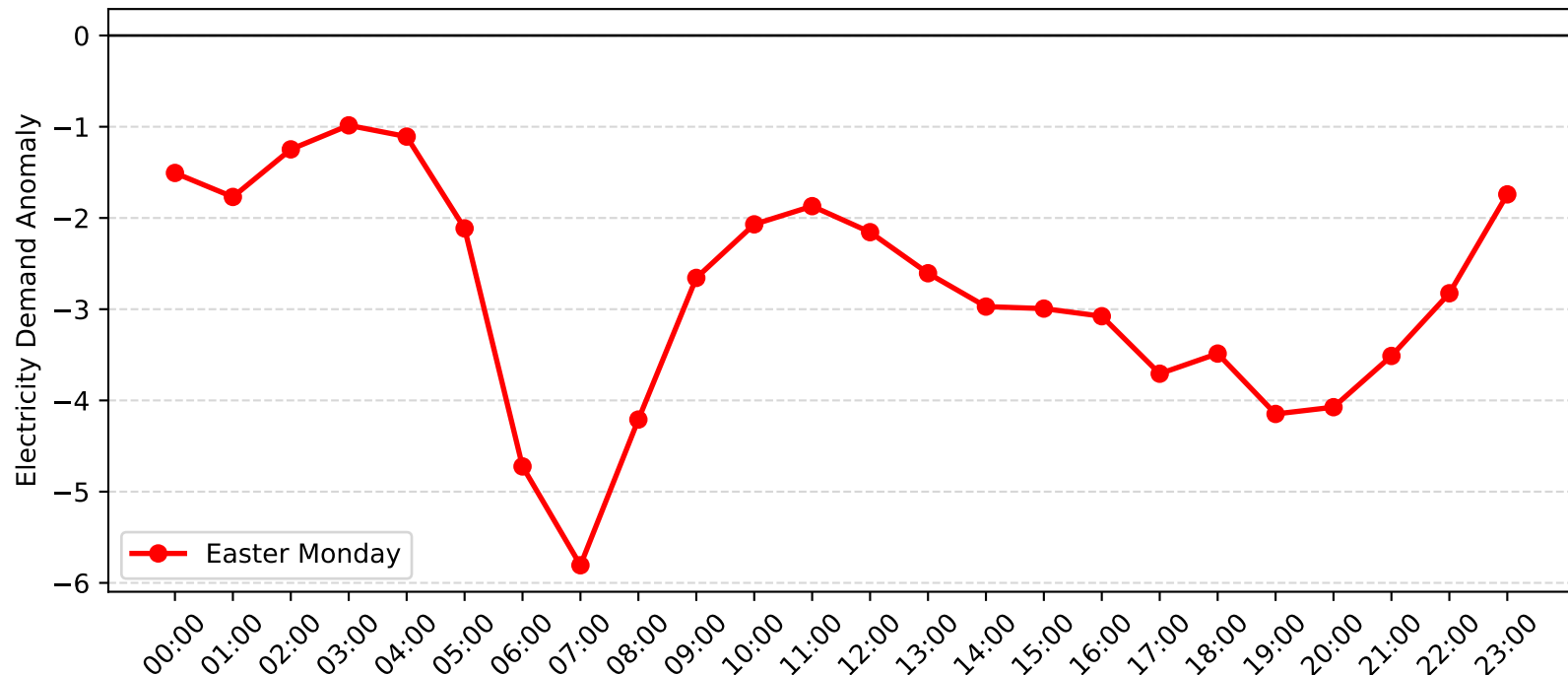
Mortdale Demand Anomaly: Easter Monday (2010-2011)
