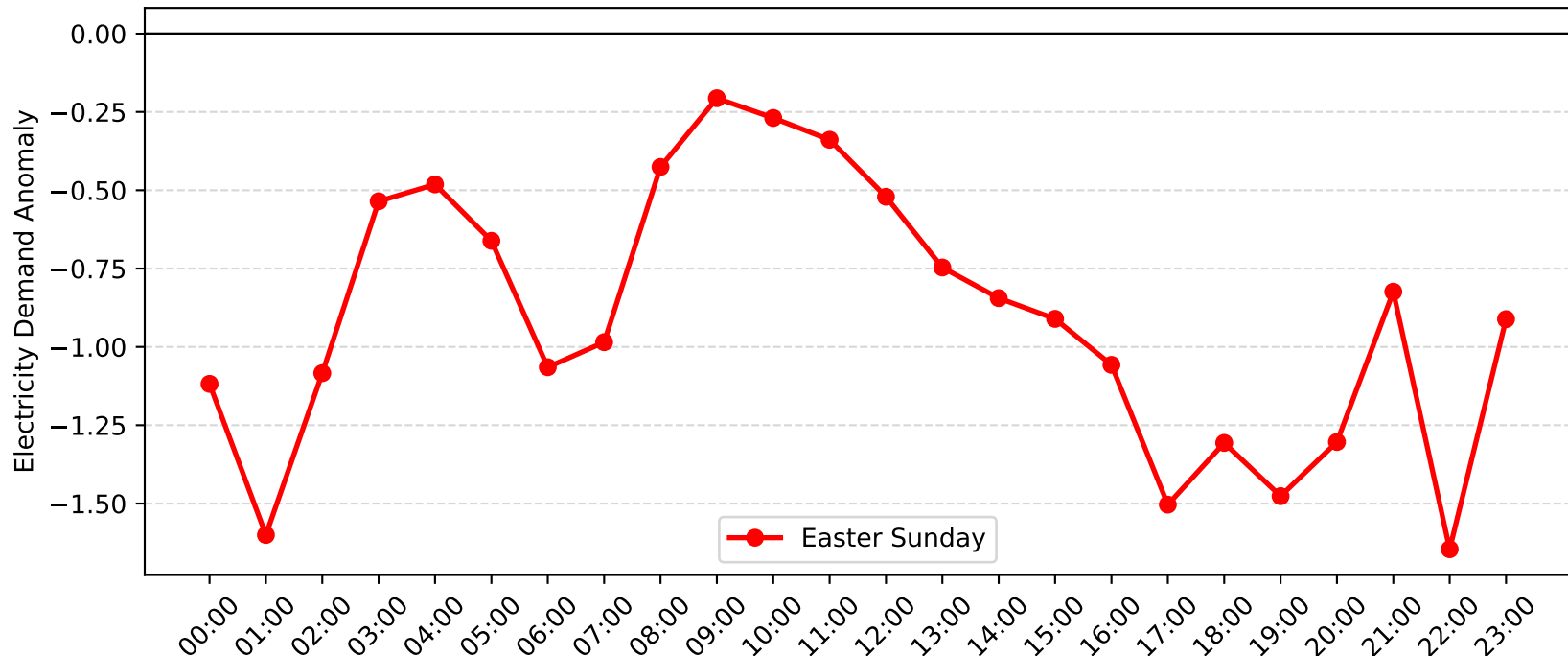
Jewells Demand Anomaly: Easter Sunday (2010-2011)
