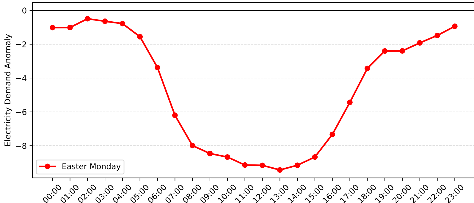
Mascot Demand Anomaly: Easter Monday (2008-2009)
