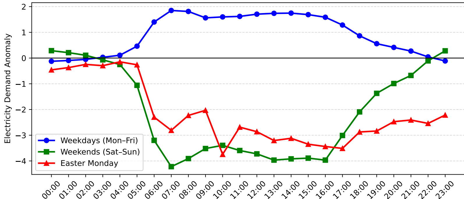
Pymble Demand Anomaly: Easter Monday vs Weekday/Weekend (2006-2007)
