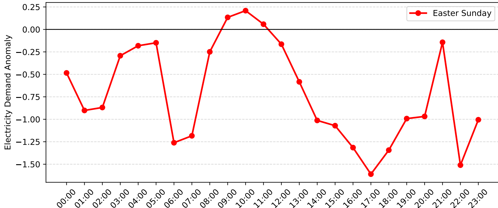
Jewells Demand Anomaly: Easter Sunday (2007-2008)
