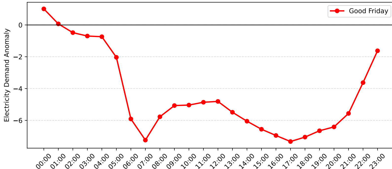
Pennant Hills Demand Anomaly: Good Friday (2013-2014)
