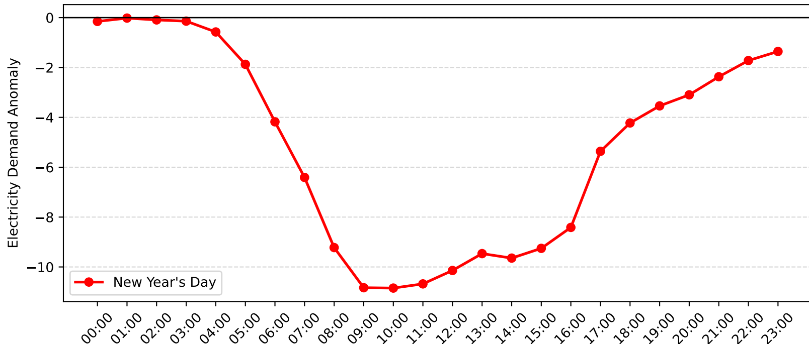
Brookvale Demand Anomaly: New Year's Day (2014-2015)
