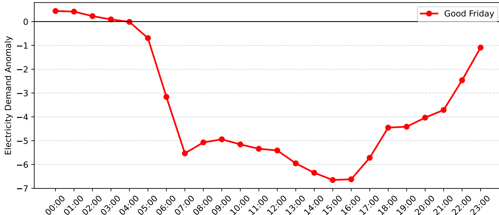
Chatswood Demand Anomaly: Good Friday (2008-2009)
