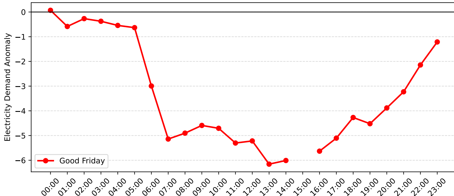
Chatswood Demand Anomaly: Good Friday (2017-2018)
