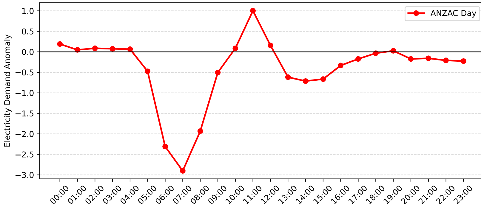
Blakehurst Demand Anomaly: ANZAC Day (2006-2007)
