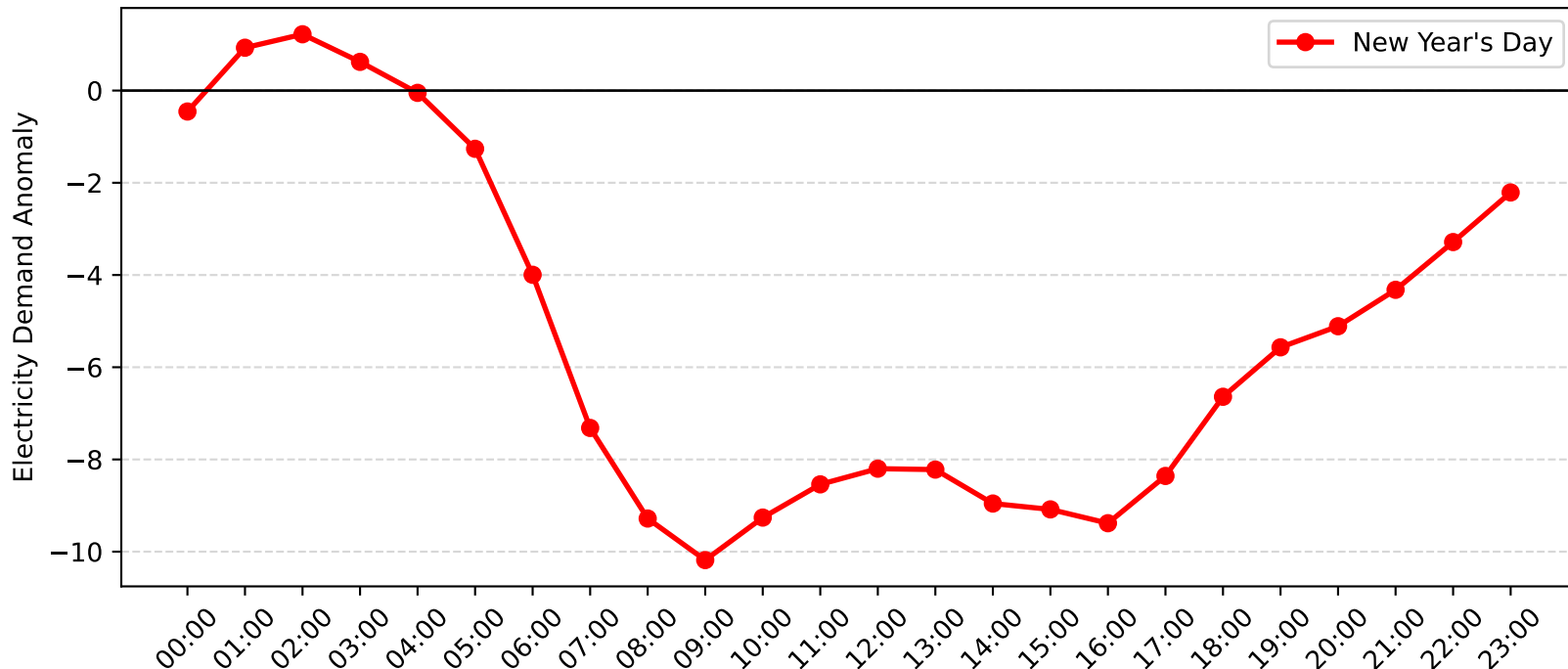
Burwood Demand Anomaly: New Year's Day (2016-2017)
