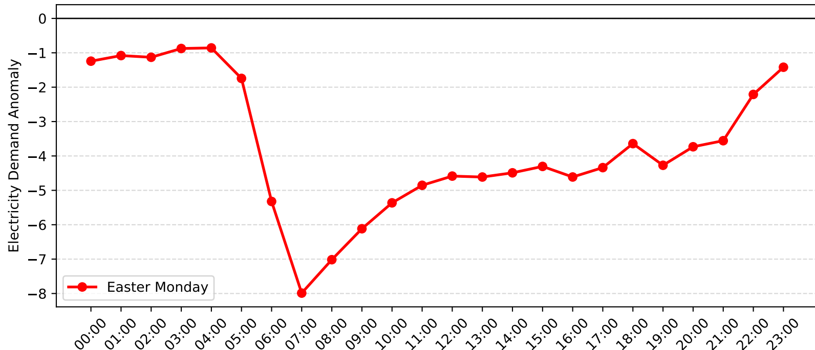
Epping Demand Anomaly: Easter Monday (2011-2012)
