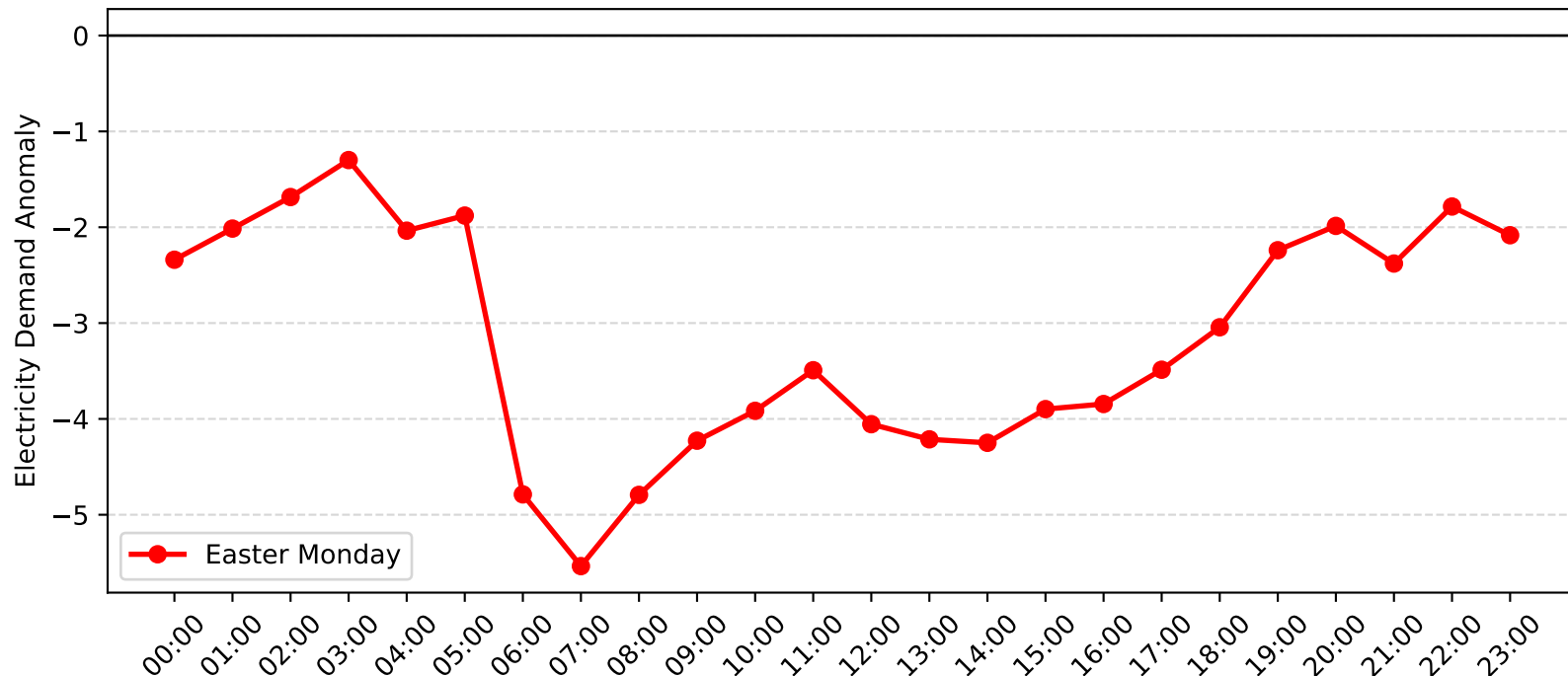
Matraville Demand Anomaly: Easter Monday (2012-2013)
