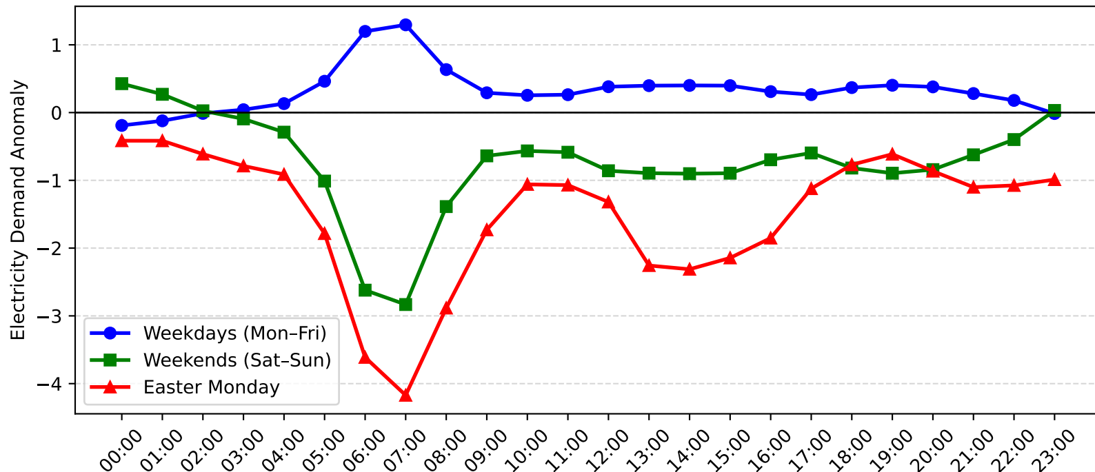
Mortdale Demand Anomaly: Easter Monday vs Weekday/Weekend (2016-2017)
