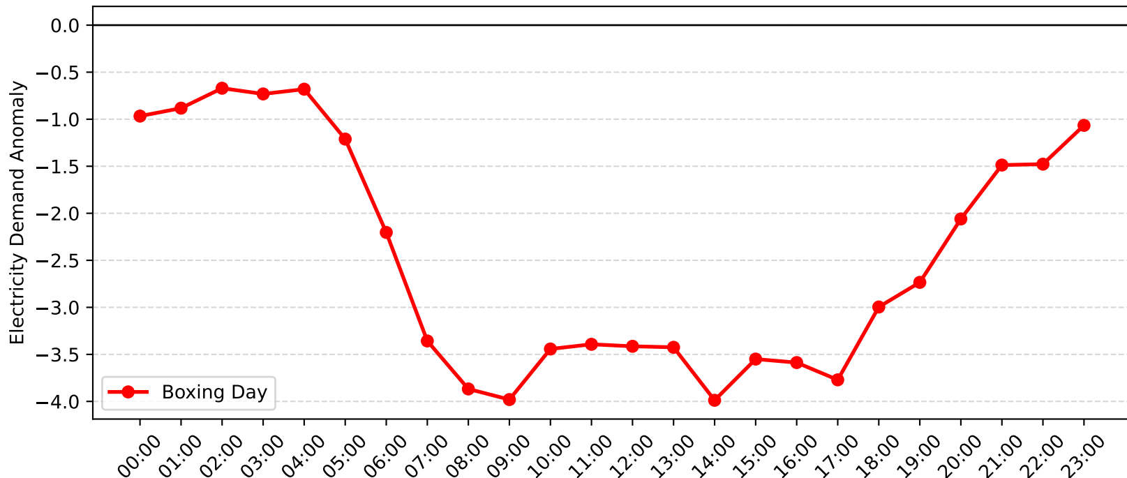
Pymble Demand Anomaly: Boxing Day (2004-2005)
