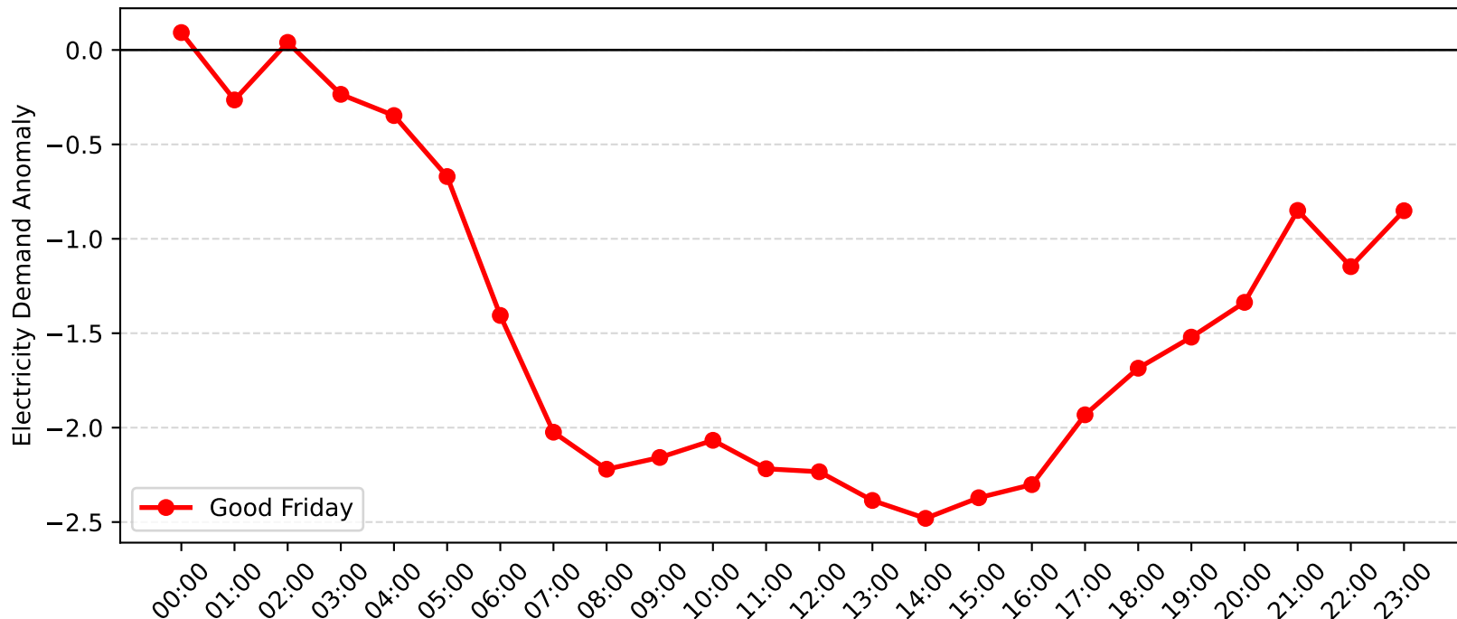
Gateshead Demand Anomaly: Good Friday (2010-2011)
