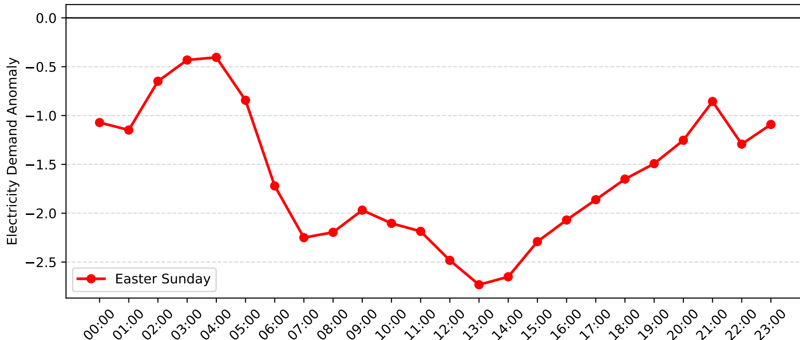
Gateshead Demand Anomaly: Easter Sunday (2013-2014)
