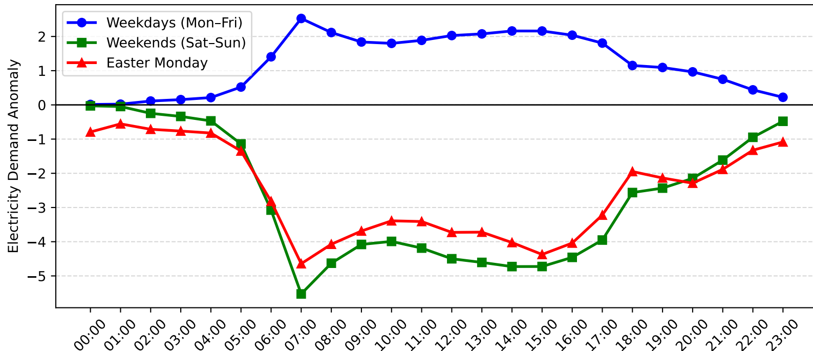
Epping Demand Anomaly: Easter Monday vs Weekday/Weekend (2016-2017)
