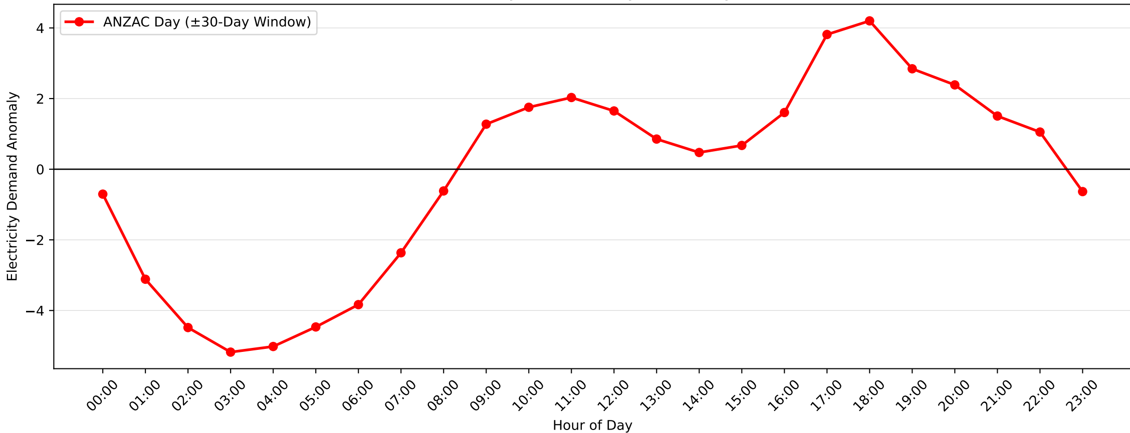
Blakehurst Demand Anomaly: ANZAC Day ( \pm 30 -Day Window, 2007-2008)
