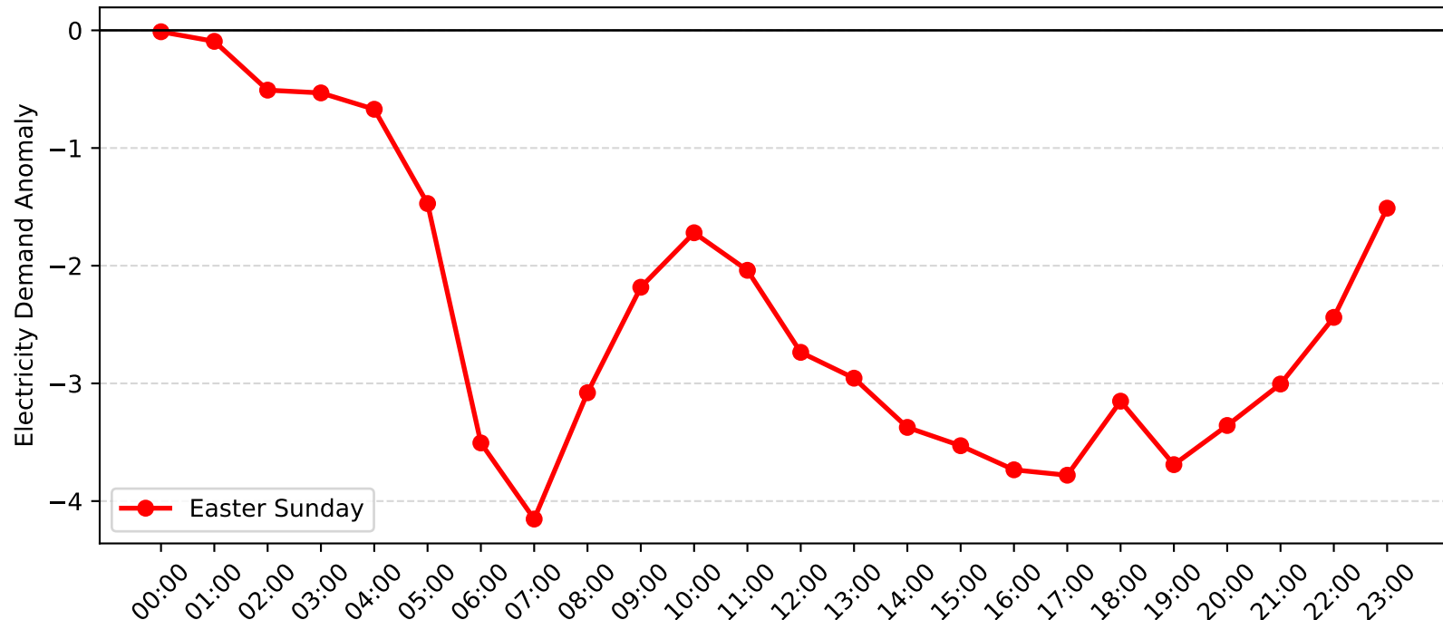
Dulwich Hill Demand Anomaly: Easter Sunday (2014-2015)
