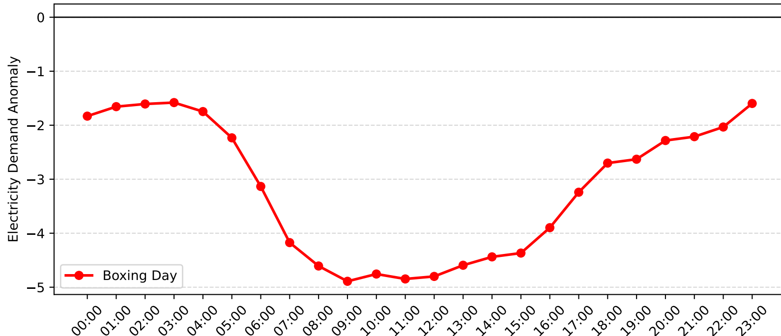
Lidcombe Demand Anomaly: Boxing Day (2007-2008)
