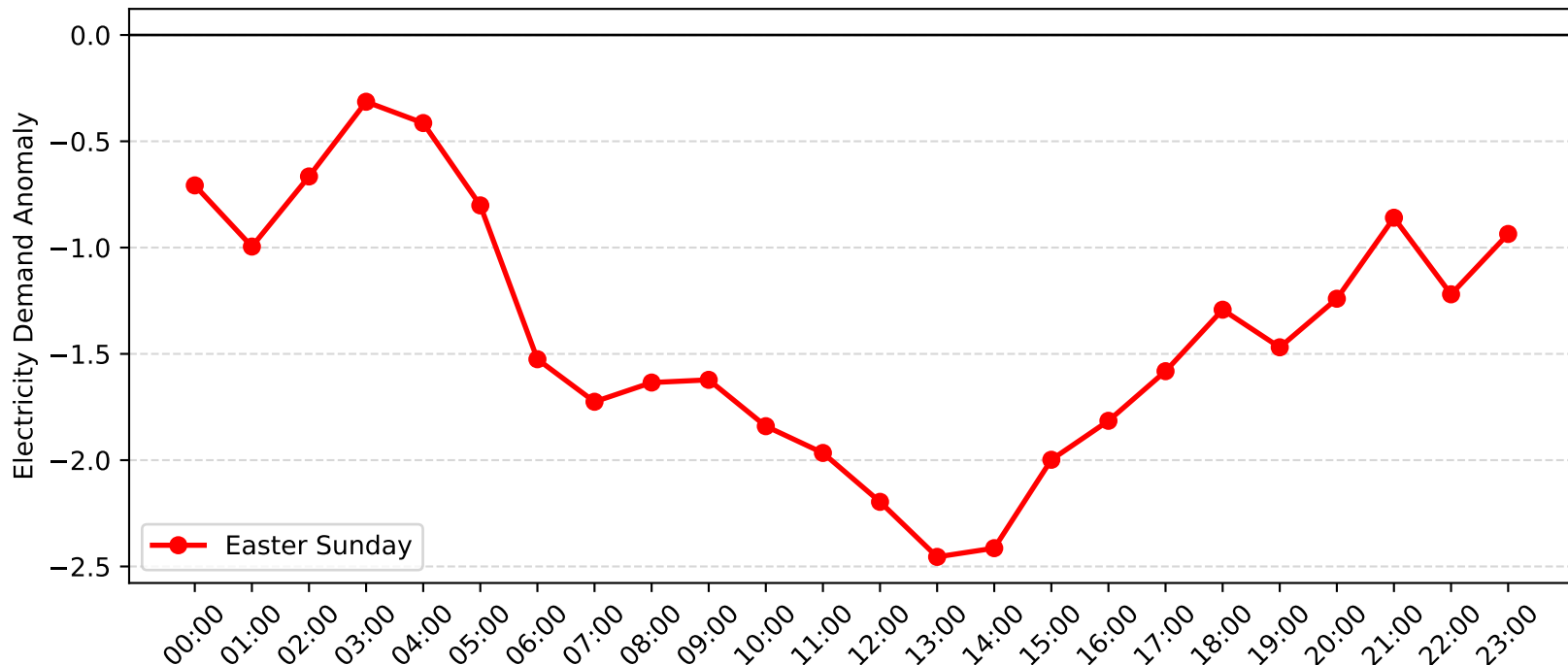
Gateshead Demand Anomaly: Easter Sunday (2014-2015)
