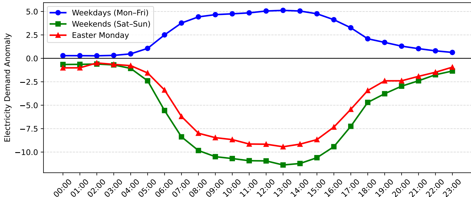
Mascot Demand Anomaly: Easter Monday vs Weekday/Weekend (2008-2009)
