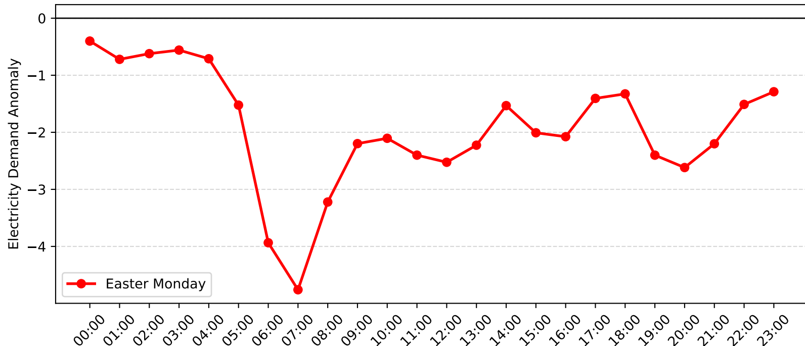
Mortdale Demand Anomaly: Easter Monday (2014-2015)
