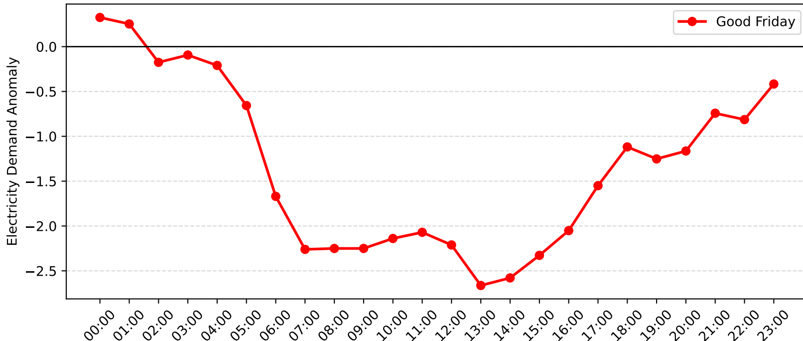
Gateshead Demand Anomaly: Good Friday (2006-2007)
