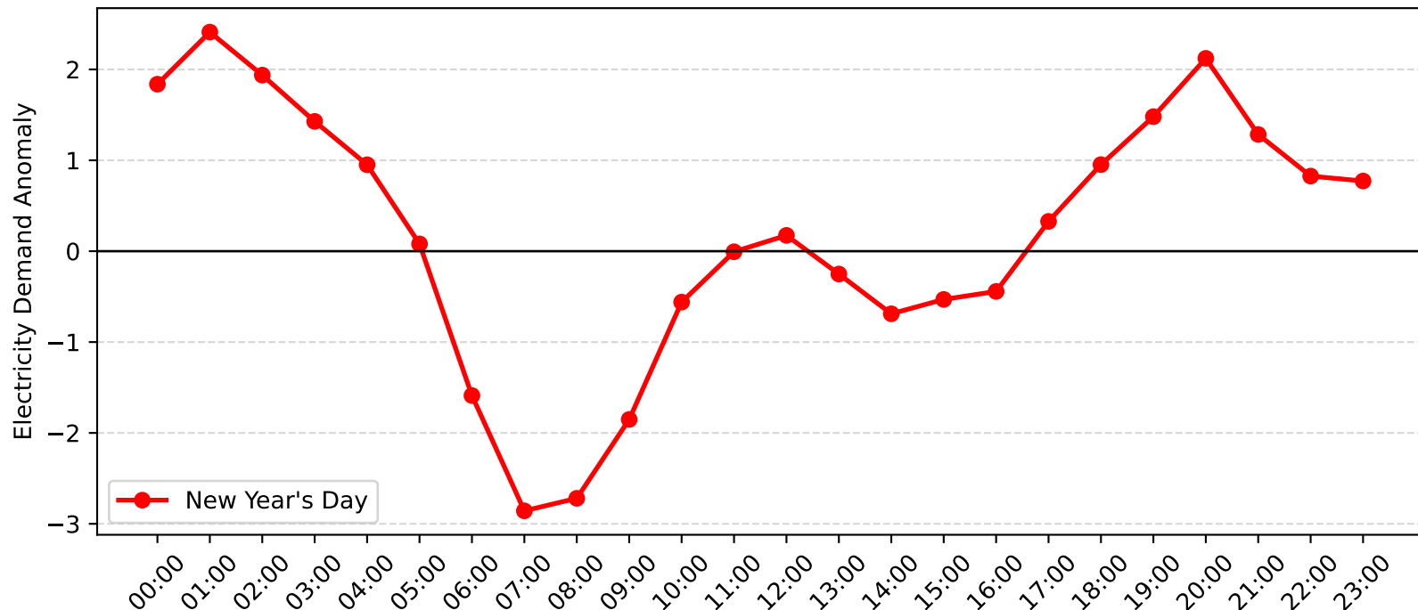
Five Dock Demand Anomaly: New Year's Day (2006-2007)
