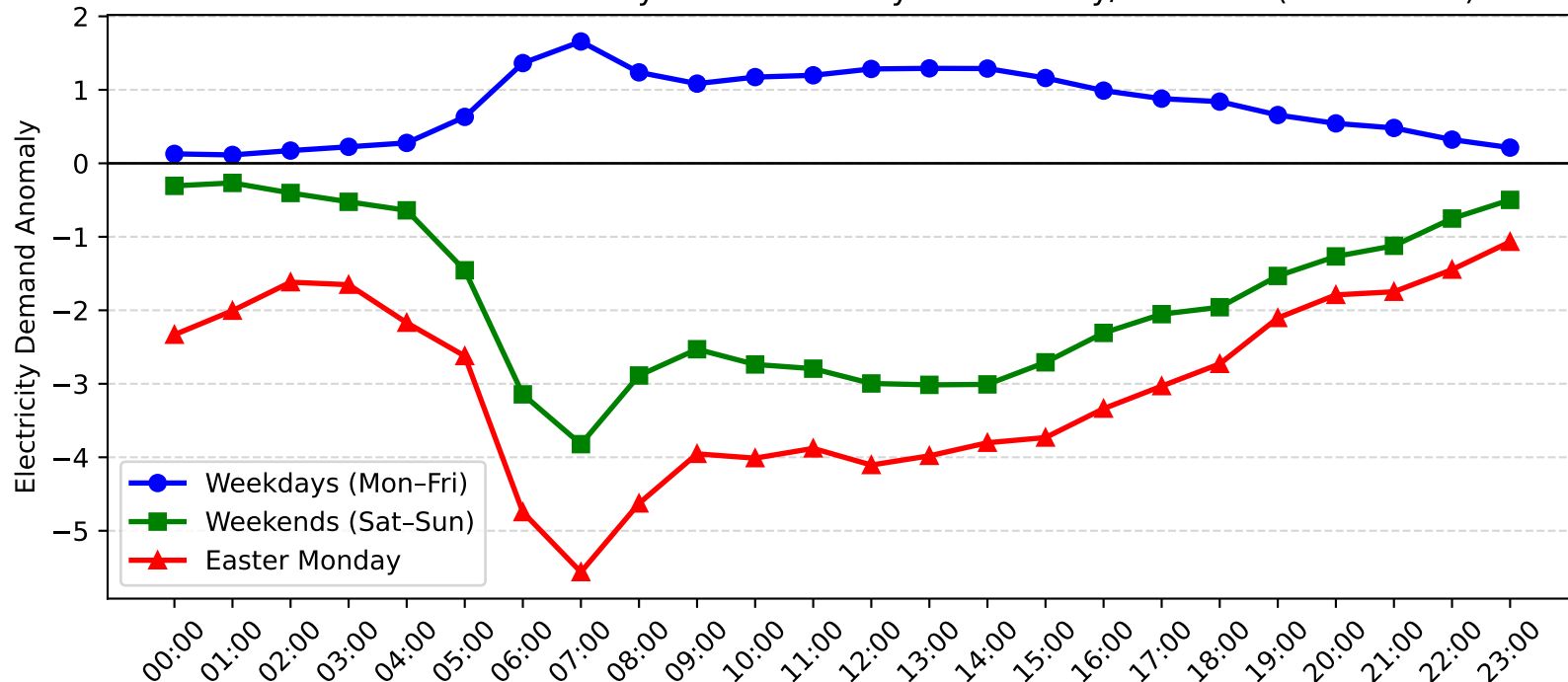
Matravlle Demand Anomaly: Easter Monday vs Weekday/Weekend (2013-2014)
