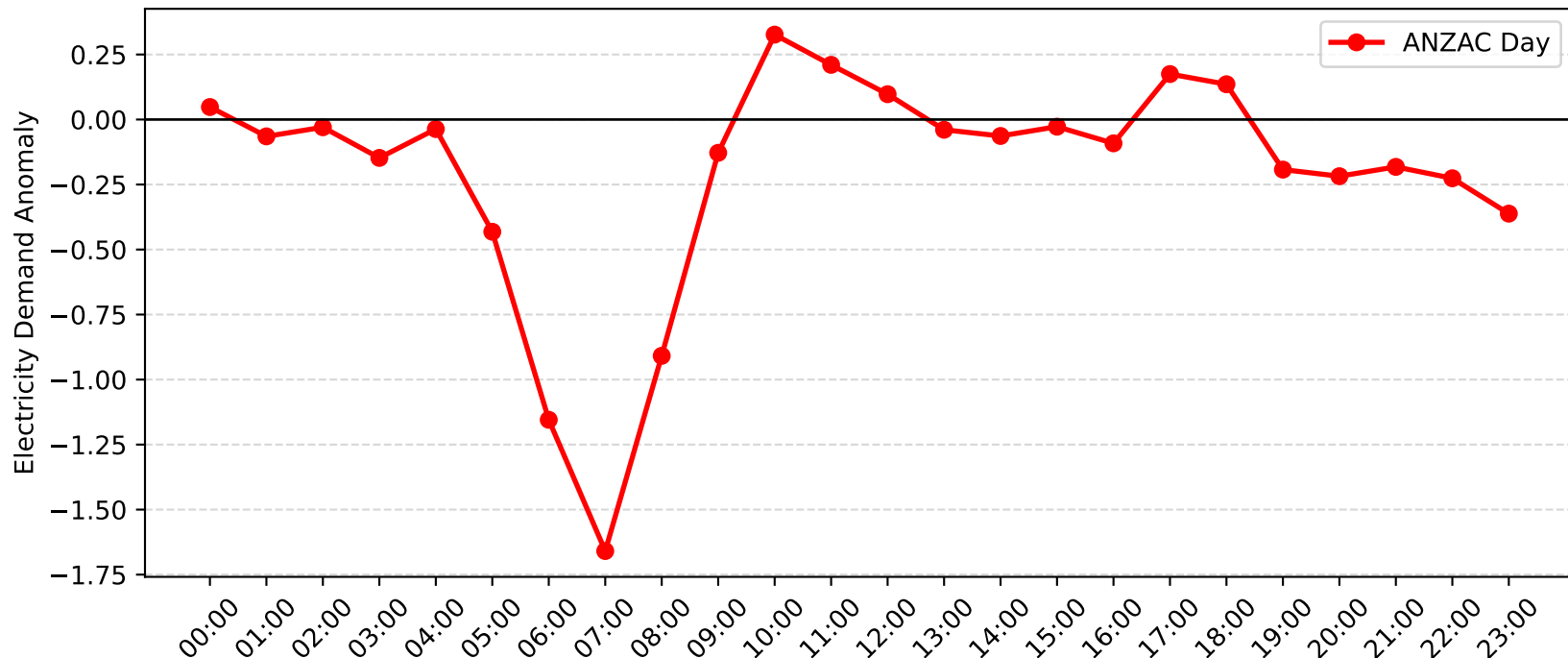
Blakehurst Demand Anomaly: ANZAC Day (2016-2017)
