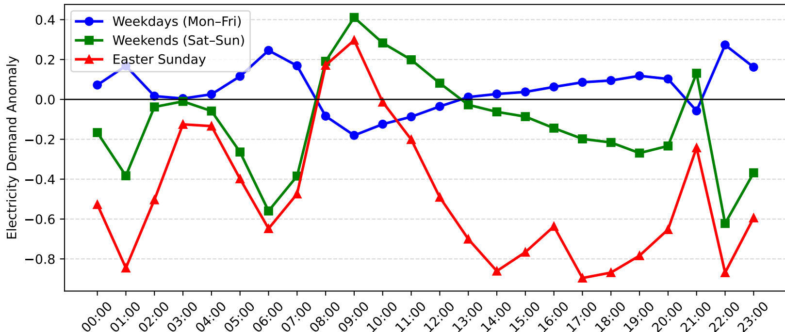
Jewells Demand Anomaly: Easter Sunday vs Weekday/Weekend (2015-2016)
