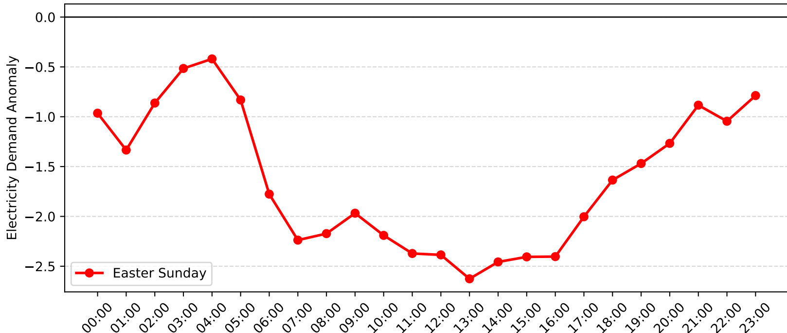
Gateshead Demand Anomaly: Easter Sunday (2008-2009)
