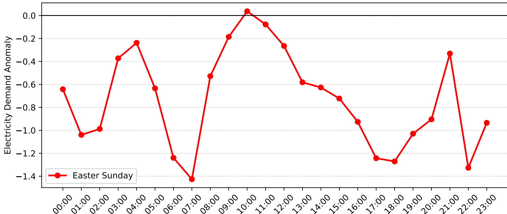
Jewells Demand Anomaly: Easter Sunday (2008-2009)
