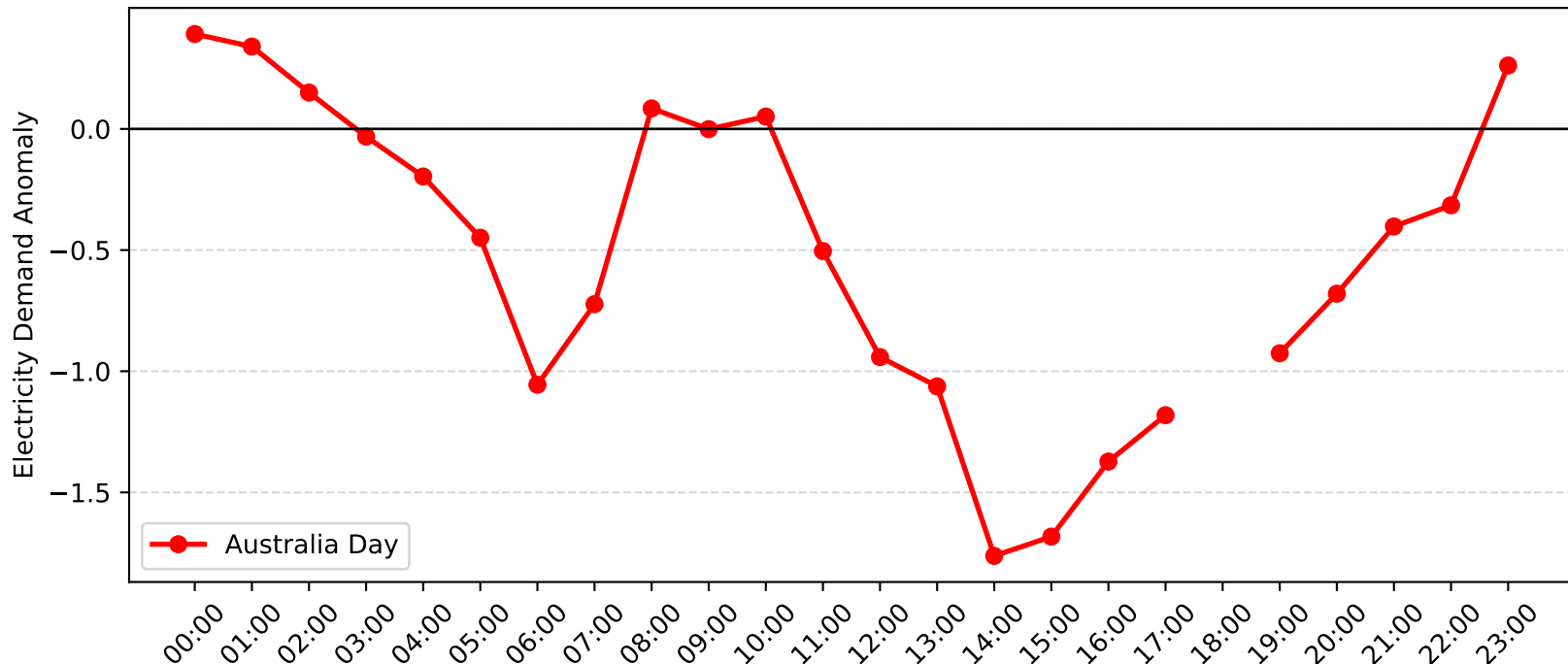
Woy Woy Demand Anomaly: Australia Day (2005-2006)
