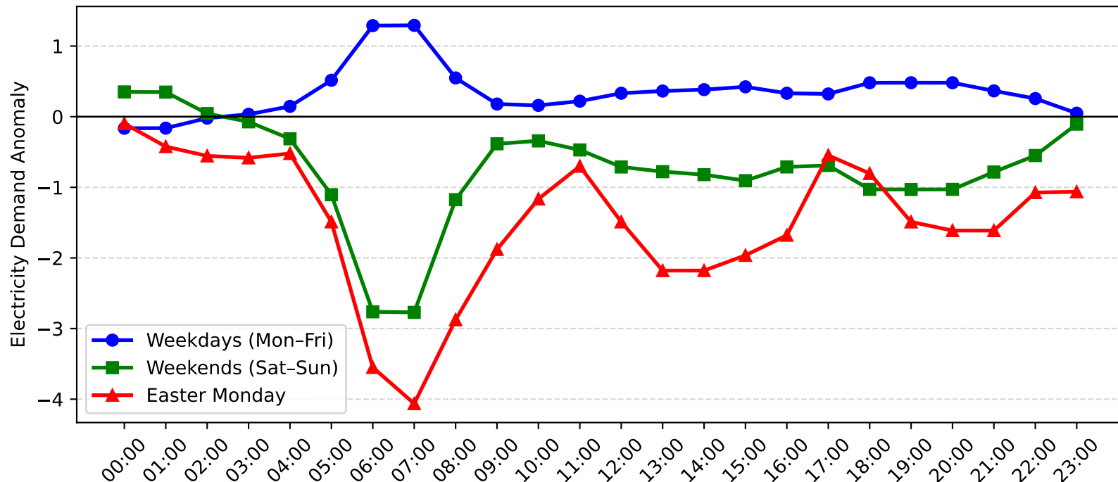
Mortdale Demand Anomaly: Easter Monday vs Weekday/Weekend (2017-2018)
