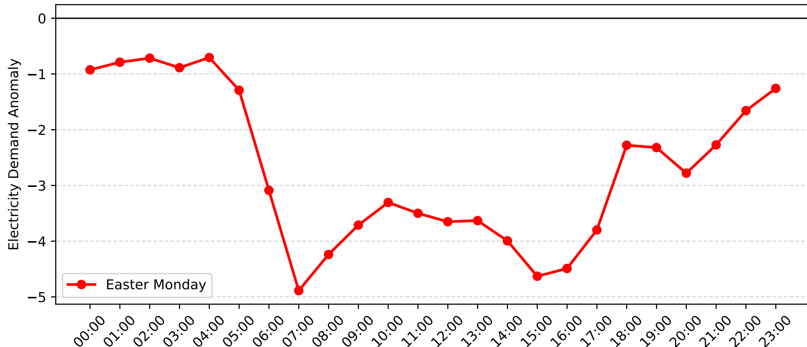
Epping Demand Anomaly: Easter Monday (2015-2016)
