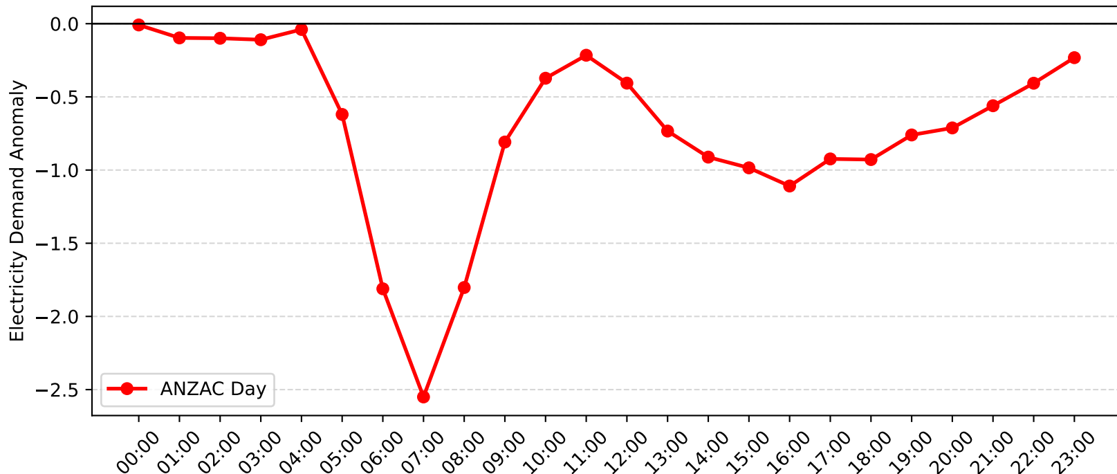
Blakehurst Demand Anomaly: ANZAC Day (2011-2012)
