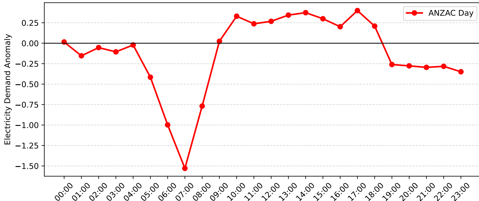
Blakehurst Demand Anomaly: ANZAC Day (2017-2018)
