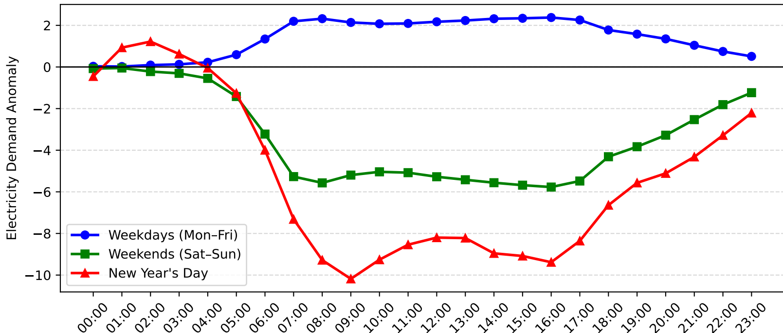
Burwood Demand Anomaly: New Year's Day vs Weekday/Weekend (2016-2017)
