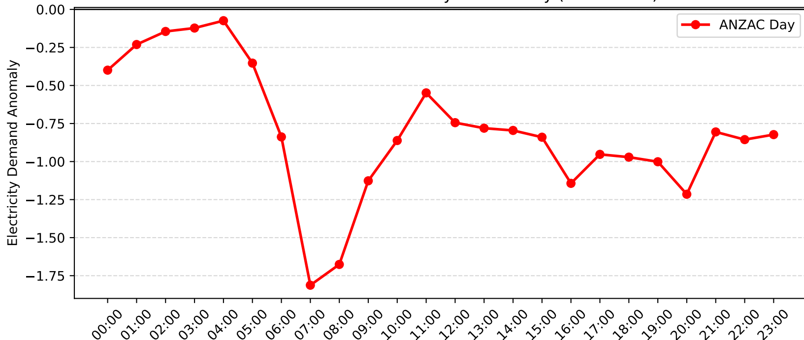
Blakehurst Demand Anomaly: ANZAC Day (2004-2005)
