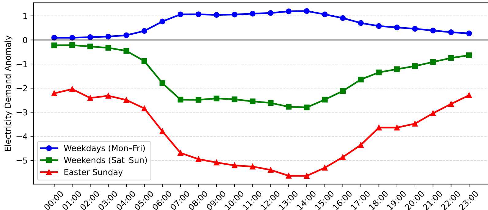
Caringbah Demand Anomaly: Easter Sunday vs Weekday/Weekend (2014-2015)
