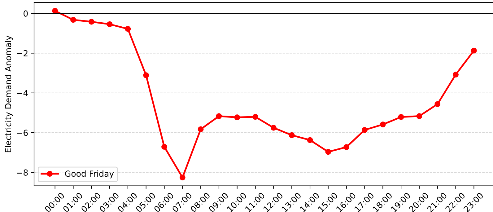
Dulwich Hill Demand Anomaly: Good Friday (2005-2006)
