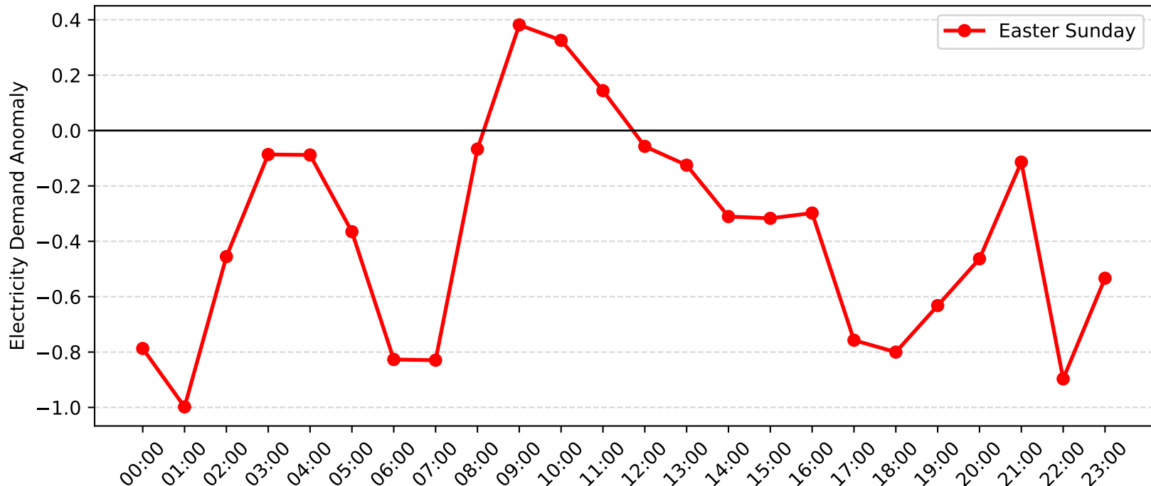
Jewells Demand Anomaly: Easter Sunday (2012-2013)
