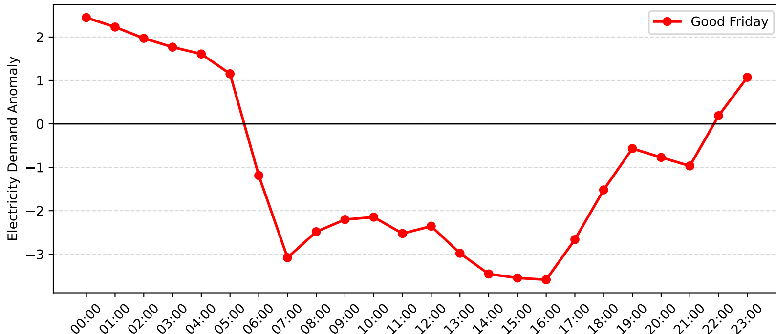
Chatswood Demand Anomaly: Good Friday (2007-2008)
