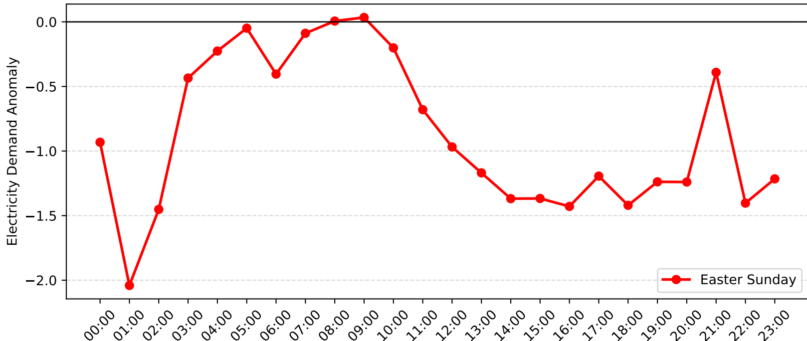
Jewells Demand Anomaly: Easter Sunday (2005-2006)
