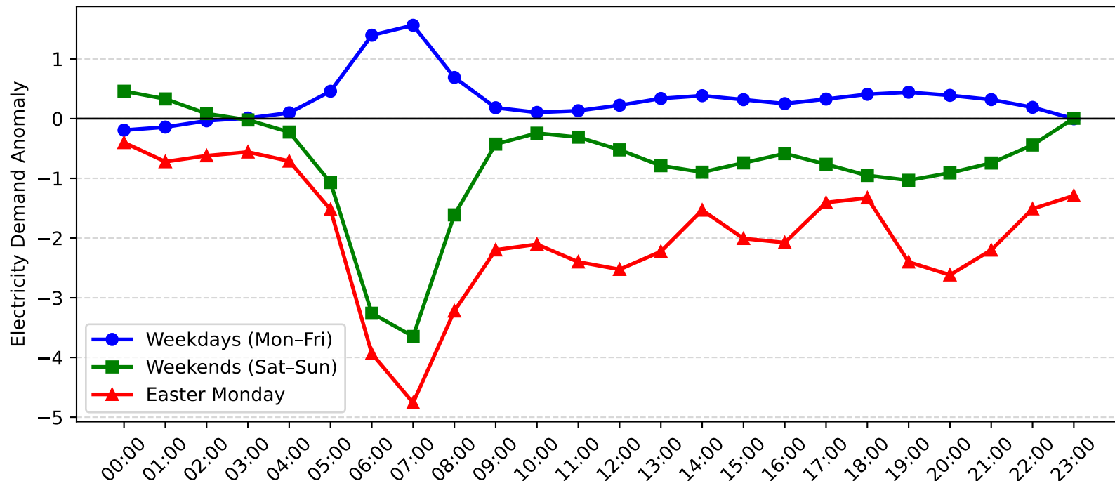
Mortdale Demand Anomaly: Easter Monday vs Weekday/Weekend (2014-2015)
