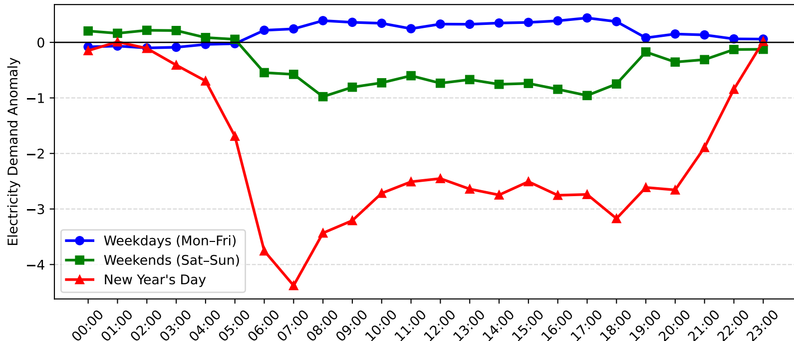
Five Dock Demand Anomaly: New Year's Day vs Weekday/Weekend (2004-2005)
