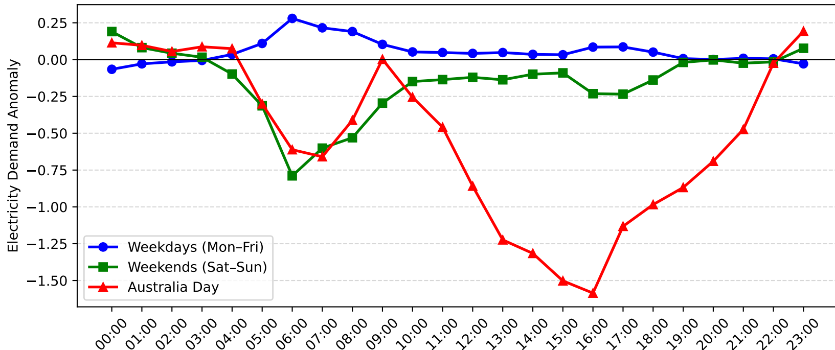
Woy Woy Demand Anomaly: Australia Day vs Weekday/Weekend (2015-2016)
