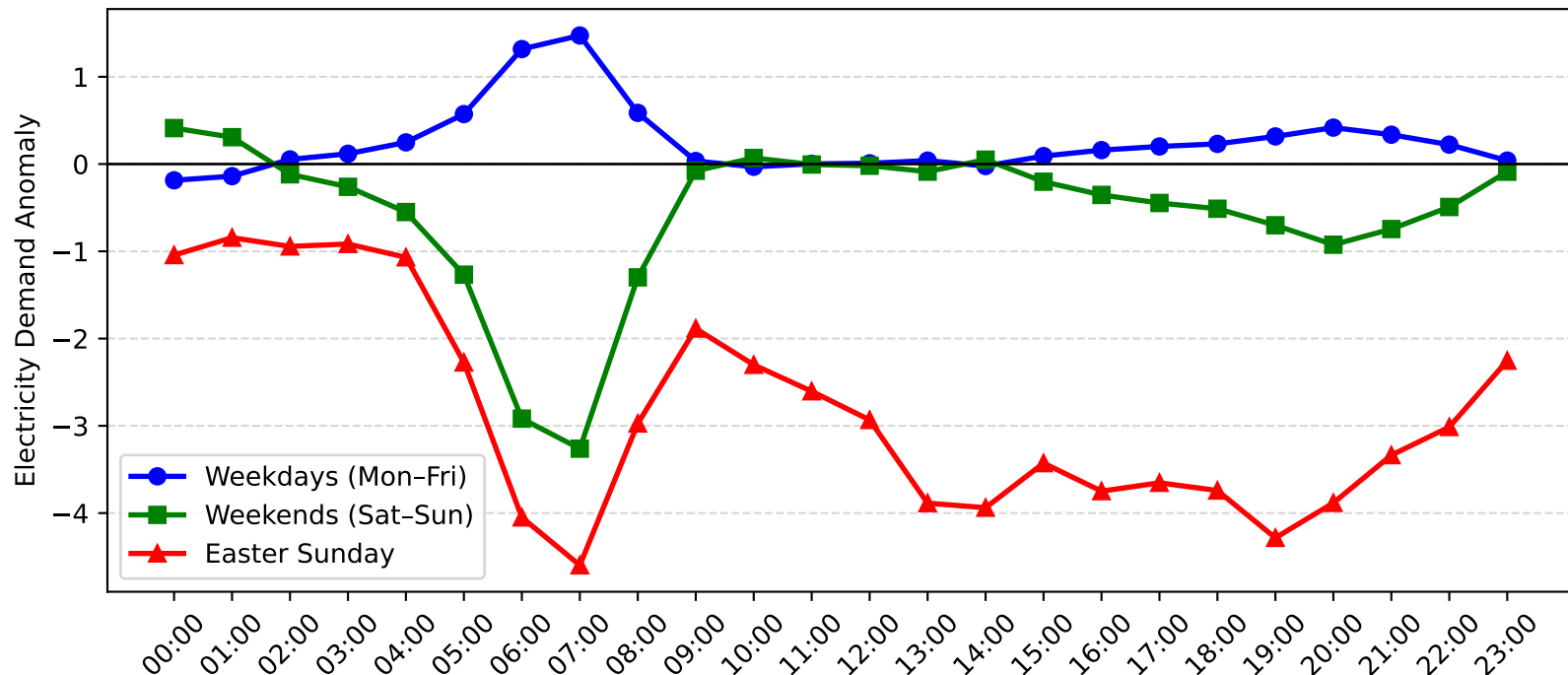
Dulwich Hill Demand Anomaly: Easter Sunday vs Weekday/Weekend (2017-2018)
