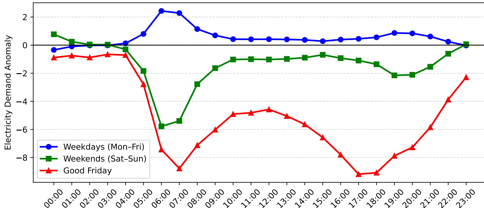
Pennant Hills Demand Anomaly: Good Friday vs Weekday/Weekend (2010-2011)
