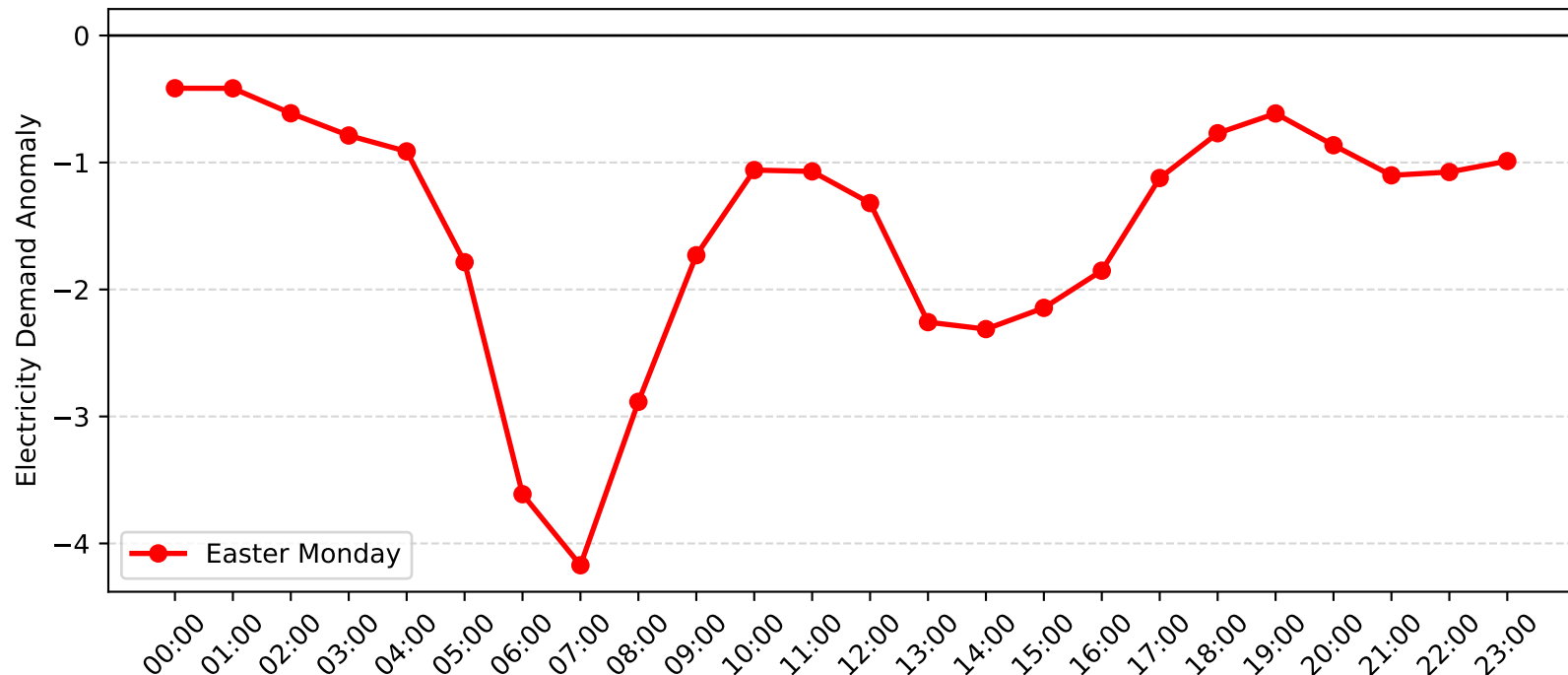
Mortdale Demand Anomaly: Easter Monday (2016-2017)
