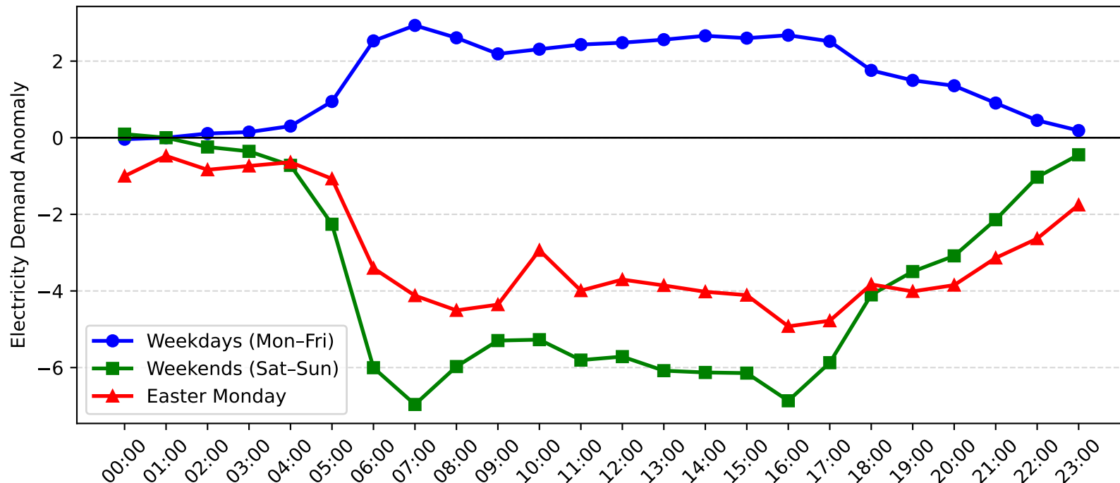
Epping Demand Anomaly: Easter Monday vs Weekday/Weekend (2006-2007)
