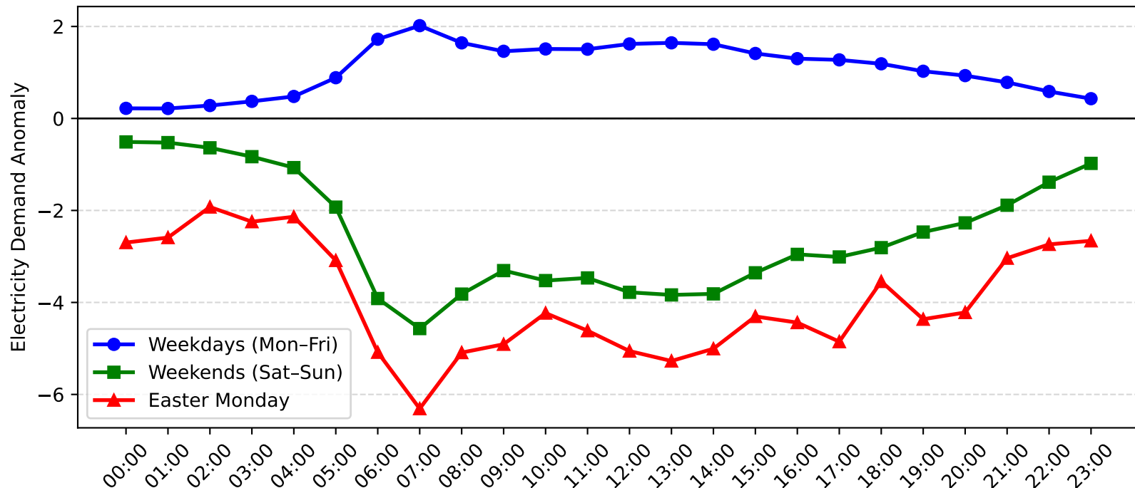
Matraverse Demand Anomaly: Easter Monday vs Weekday/Weekend (2010-2011)
