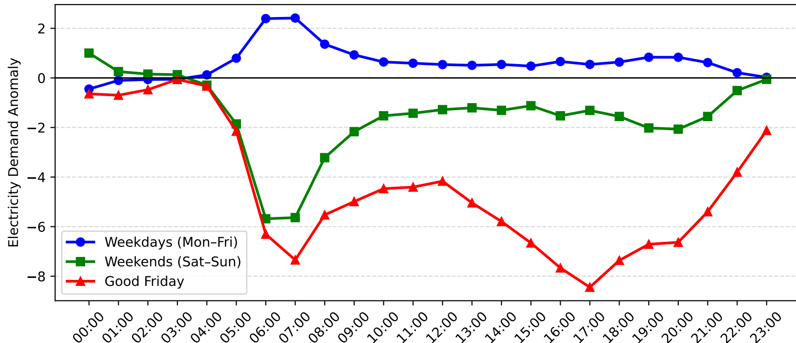
Pennant Hills Demand Anomaly: Good Friday vs Weekday/Weekend (2009-2010)
