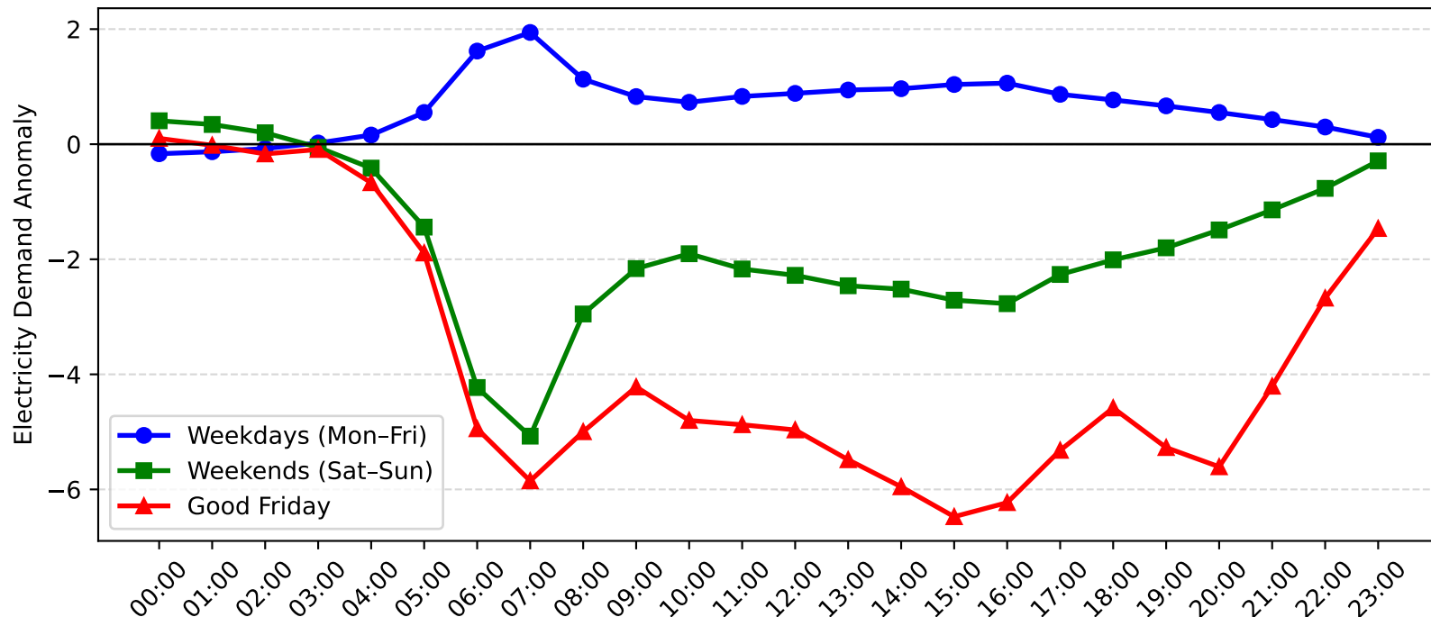
Dulwich Hill Demand Anomaly: Good Friday vs Weekday/Weekend (2007-2008)
