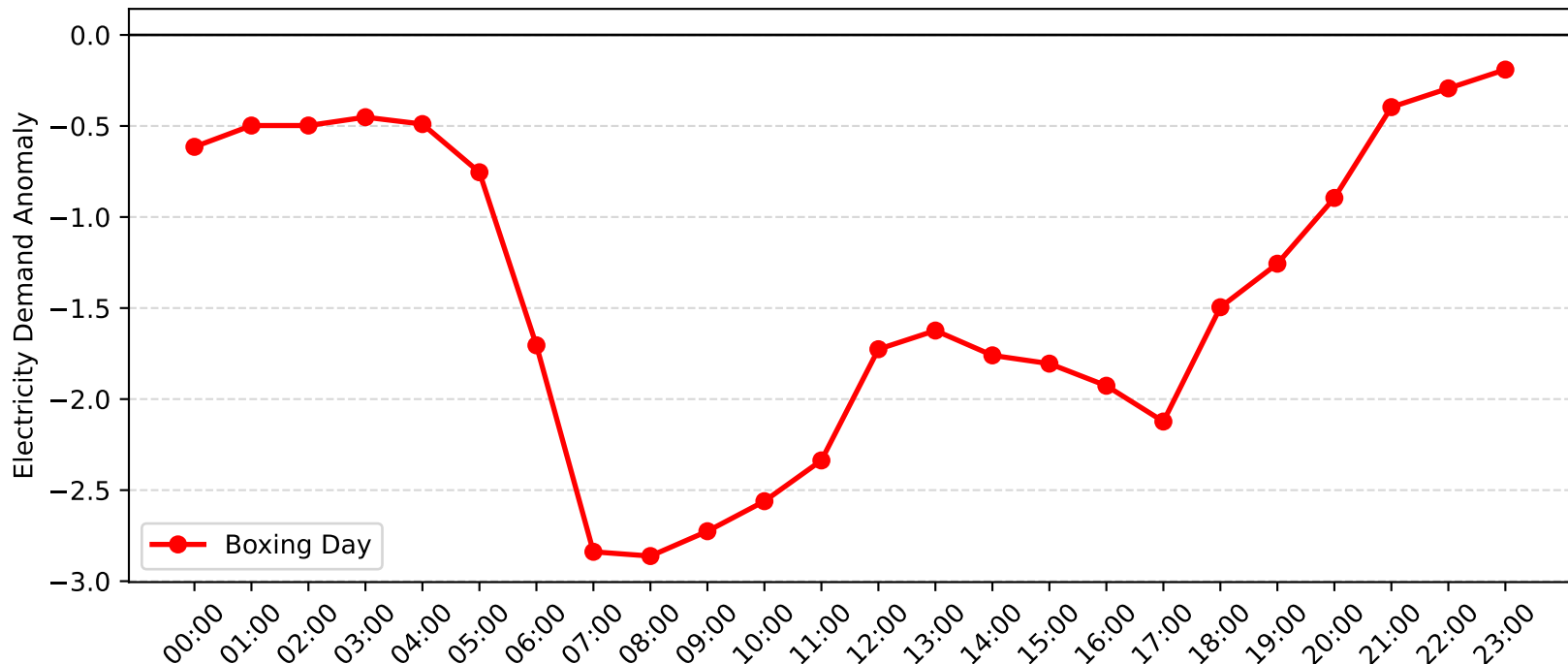
Pymble Demand Anomaly: Boxing Day (2015-2016)
