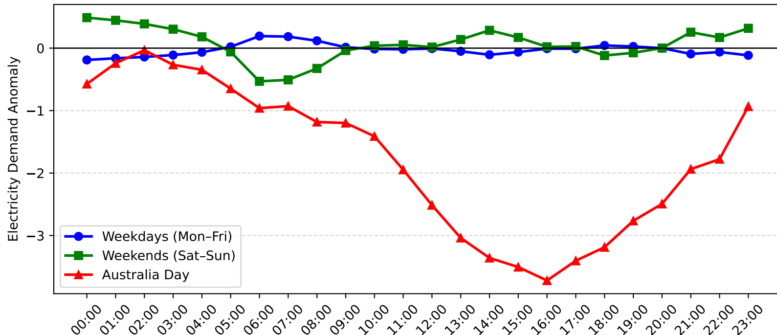
Woy Woy Demand Anomaly: Australia Day vs Weekday/Weekend (2017-2018)
