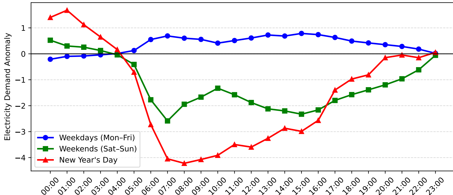
Five Dock Demand Anomaly: New Year's Day vs Weekday/Weekend (2009-2010)
