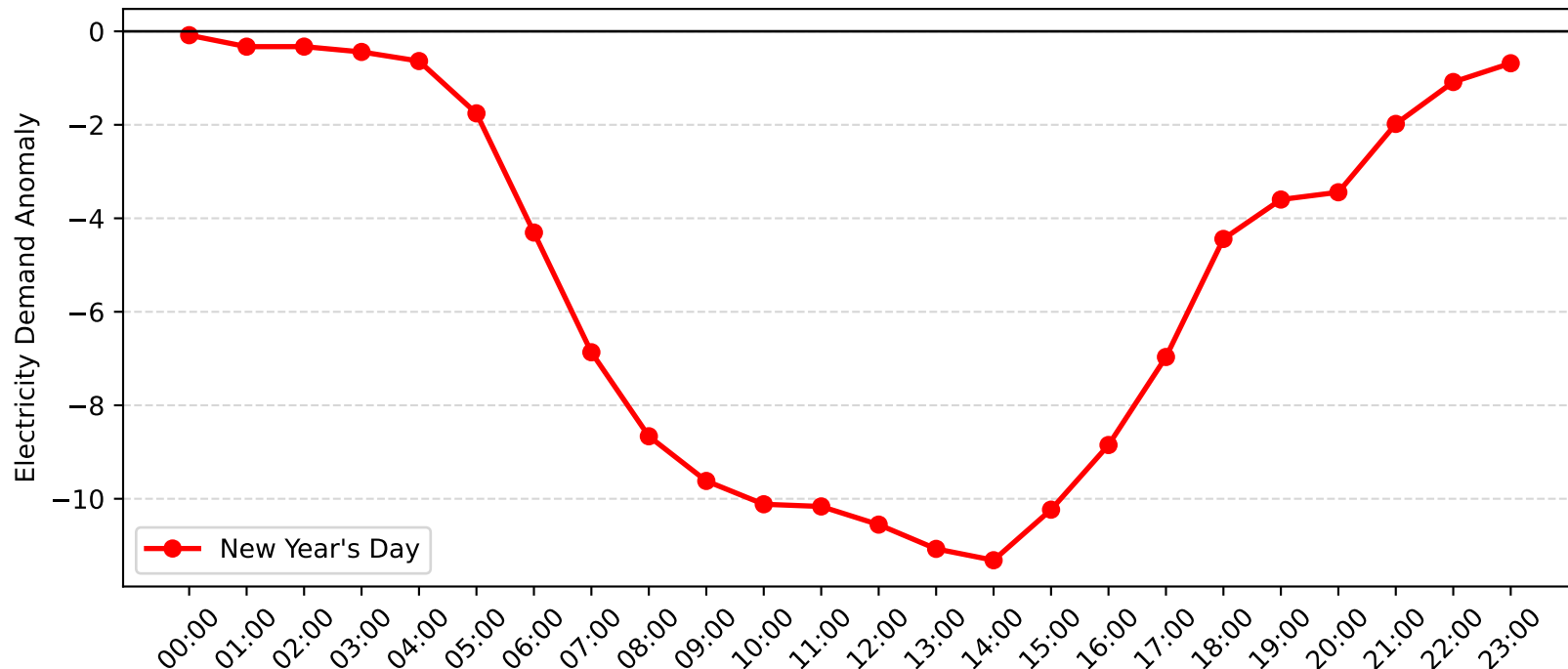
Brookvale Demand Anomaly: New Year's Day (2004-2005)
