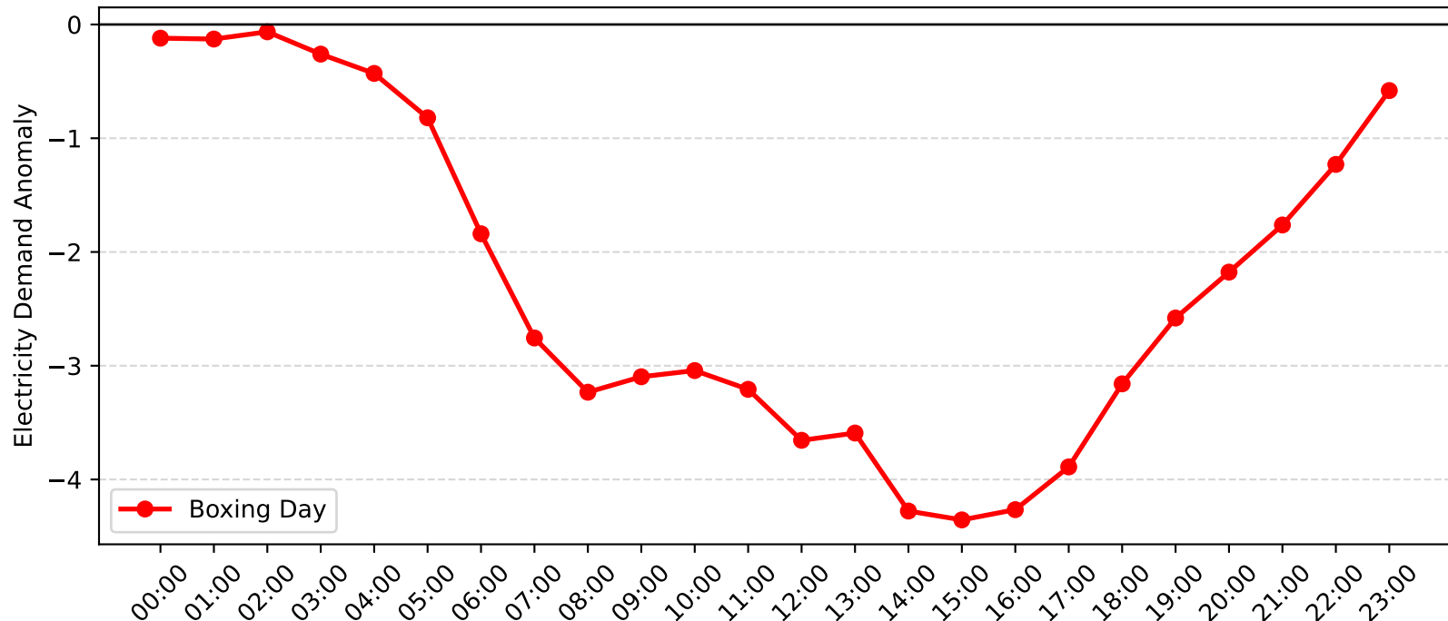
Pymble Demand Anomaly: Boxing Day (2013-2014)
