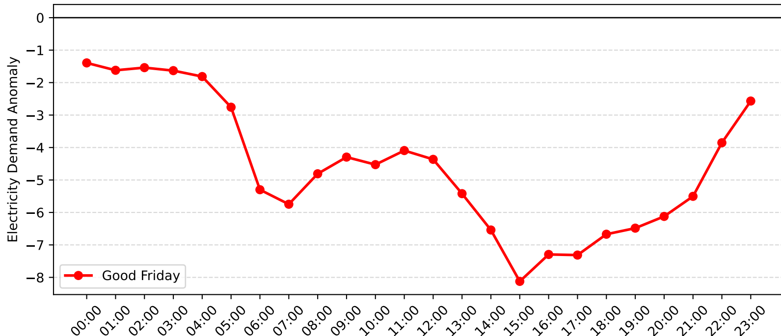
Pennant Hills Demand Anomaly: Good Friday (2016-2017)
