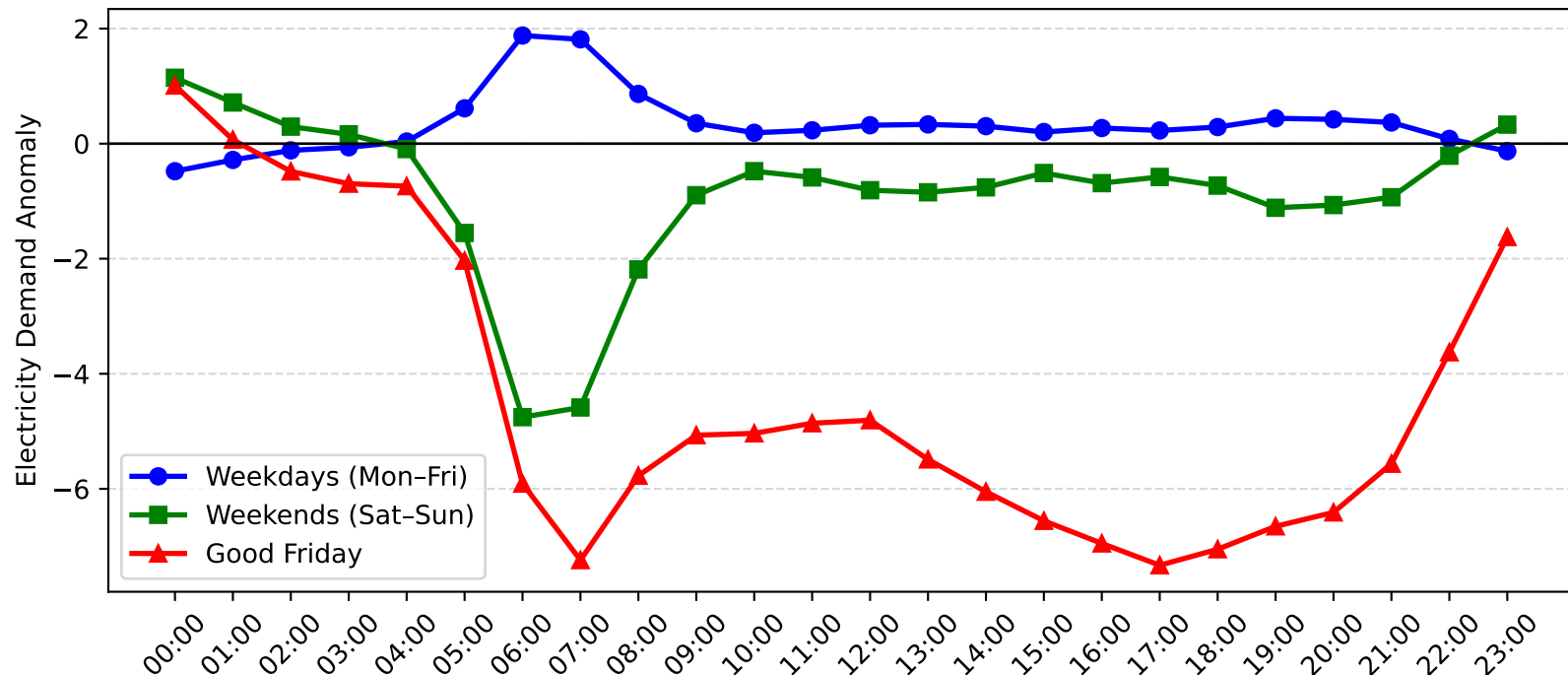
Pennant Hills Demand Anomaly: Good Friday vs Weekday/Weekend (2013-2014)
