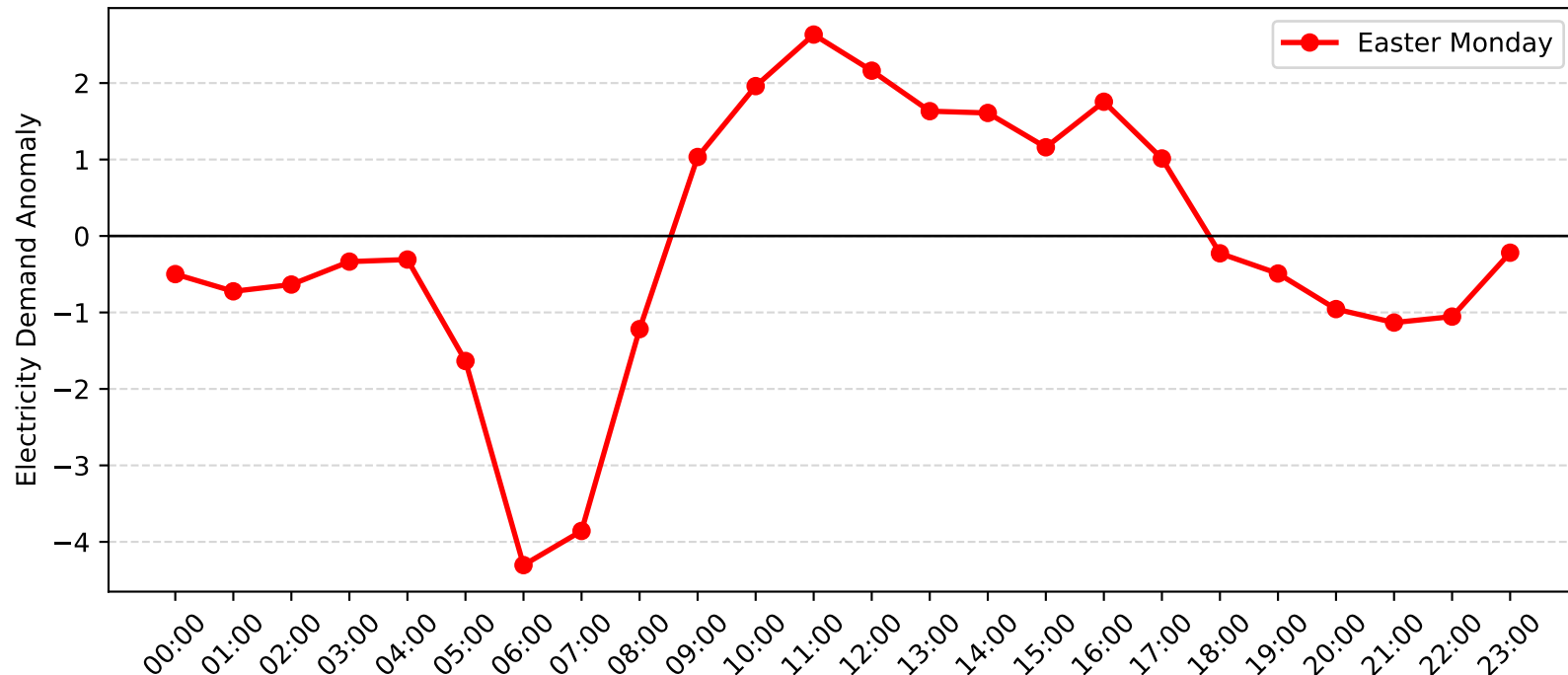
Cronulla Demand Anomaly: Easter Monday (2008-2009)
