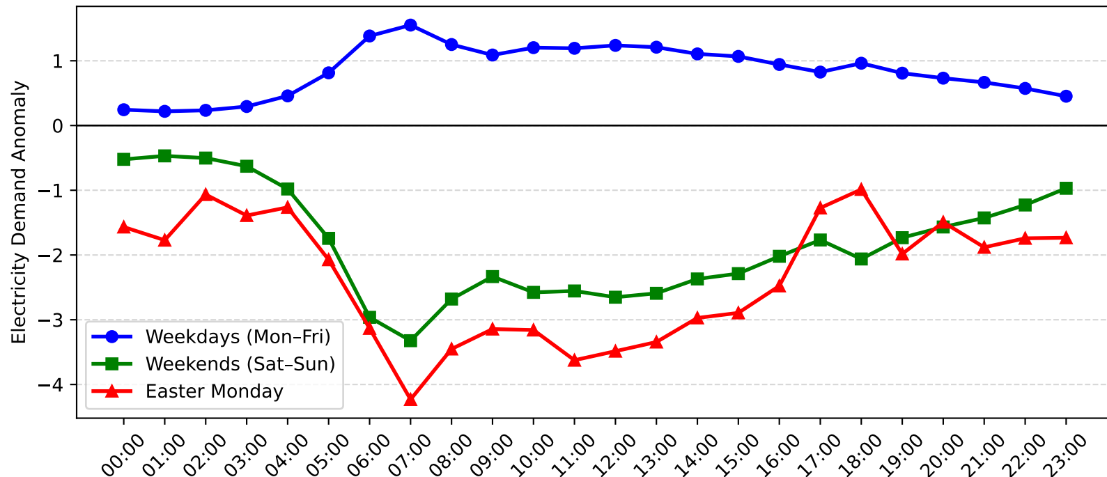
Matraverse Demand Anomaly: Easter Monday vs Weekday/Weekend (2017-2018)
