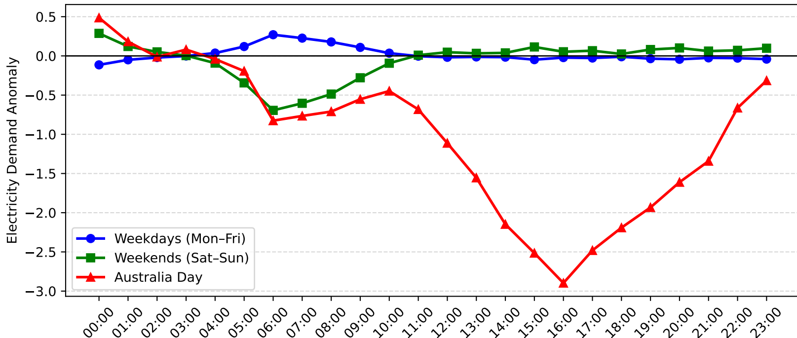
Woy Woy Demand Anomaly: Australia Day vs Weekday/Weekend (2014-2015)
