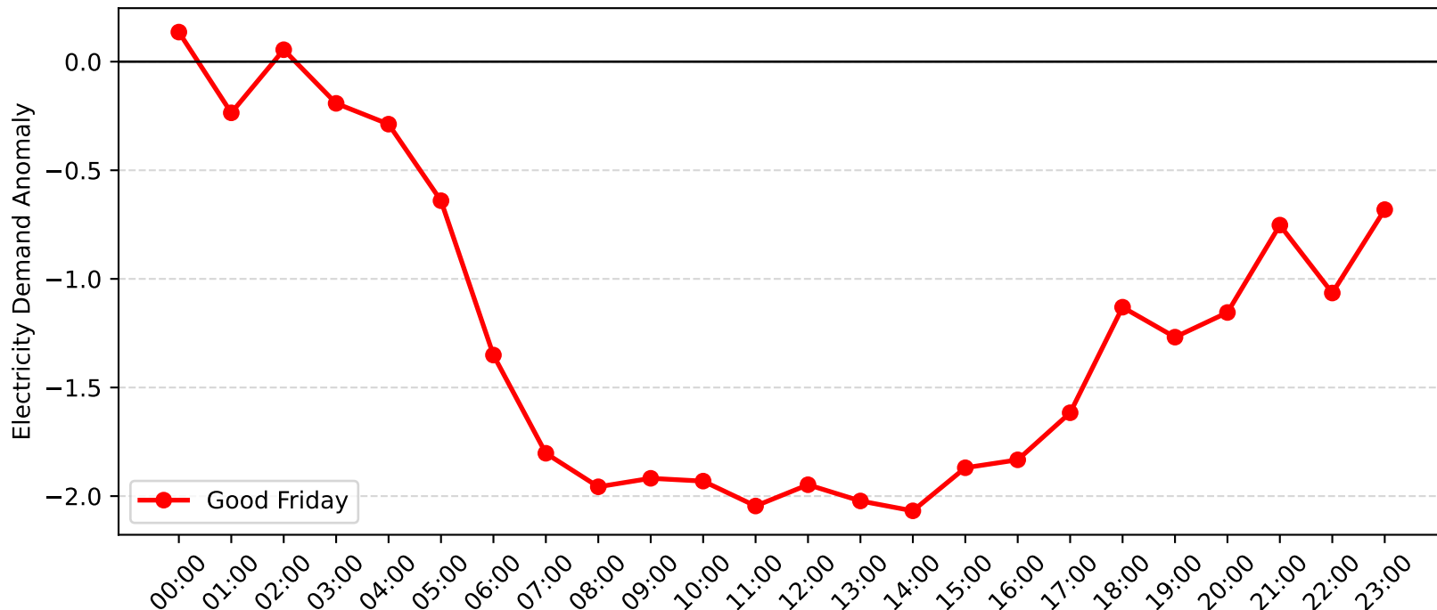
Gateshead Demand Anomaly: Good Friday (2011-2012)
