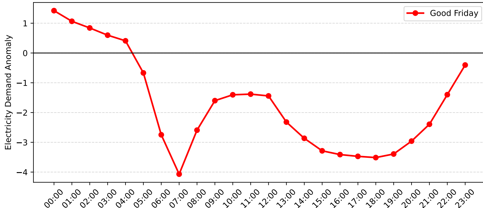
Dulwich Hill Demand Anomaly: Good Friday (2013-2014)
