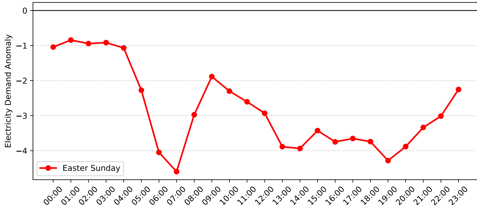
Dulwich Hill Demand Anomaly: Easter Sunday (2017-2018)
