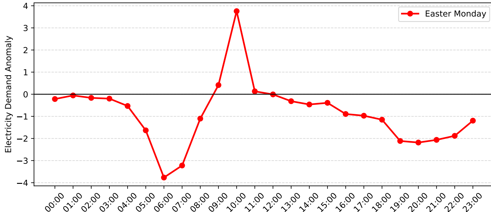
Cronulla Demand Anomaly: Easter Monday (2006-2007)
