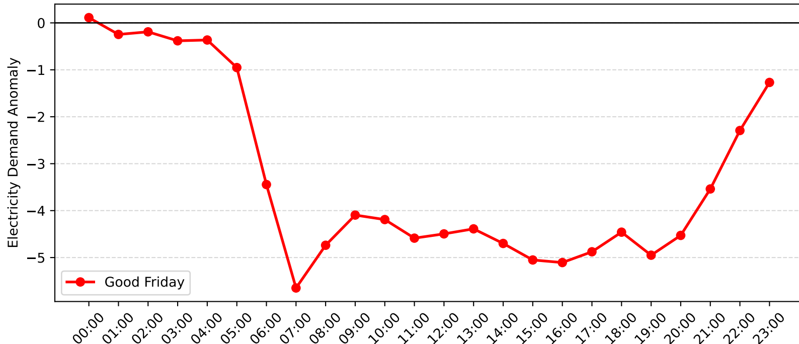
Chatswood Demand Anomaly: Good Friday (2011-2012)
