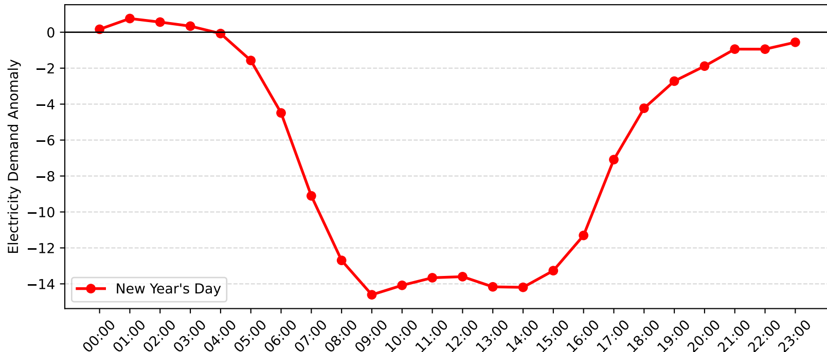
Brookvale Demand Anomaly: New Year's Day (2006-2007)
