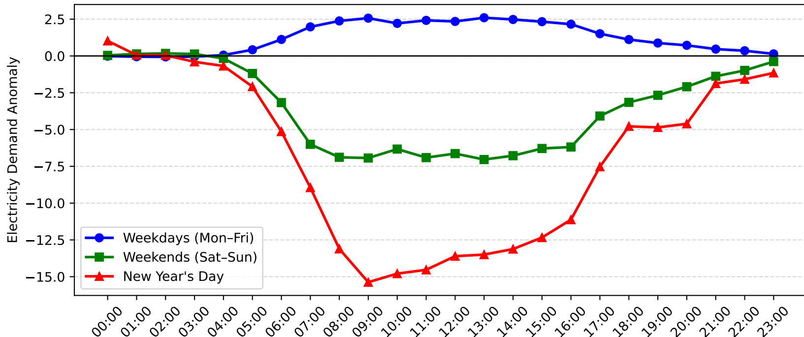
Brookvale Demand Anomaly: New Year's Day vs Weekday/Weekend (2008-2009)
