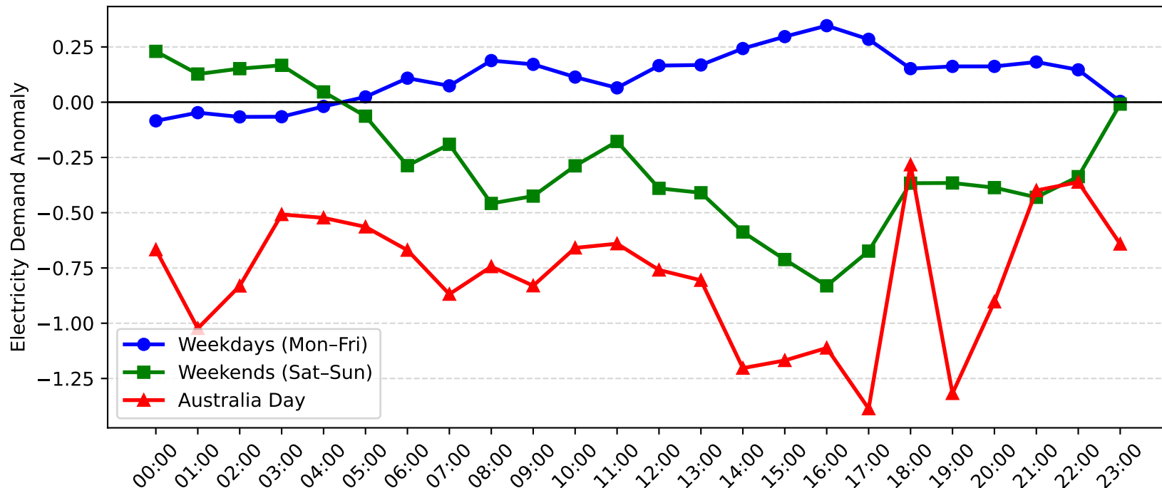
Woy Woy Demand Anomaly: Australia Day vs Weekday/Weekend (2004-2005)
