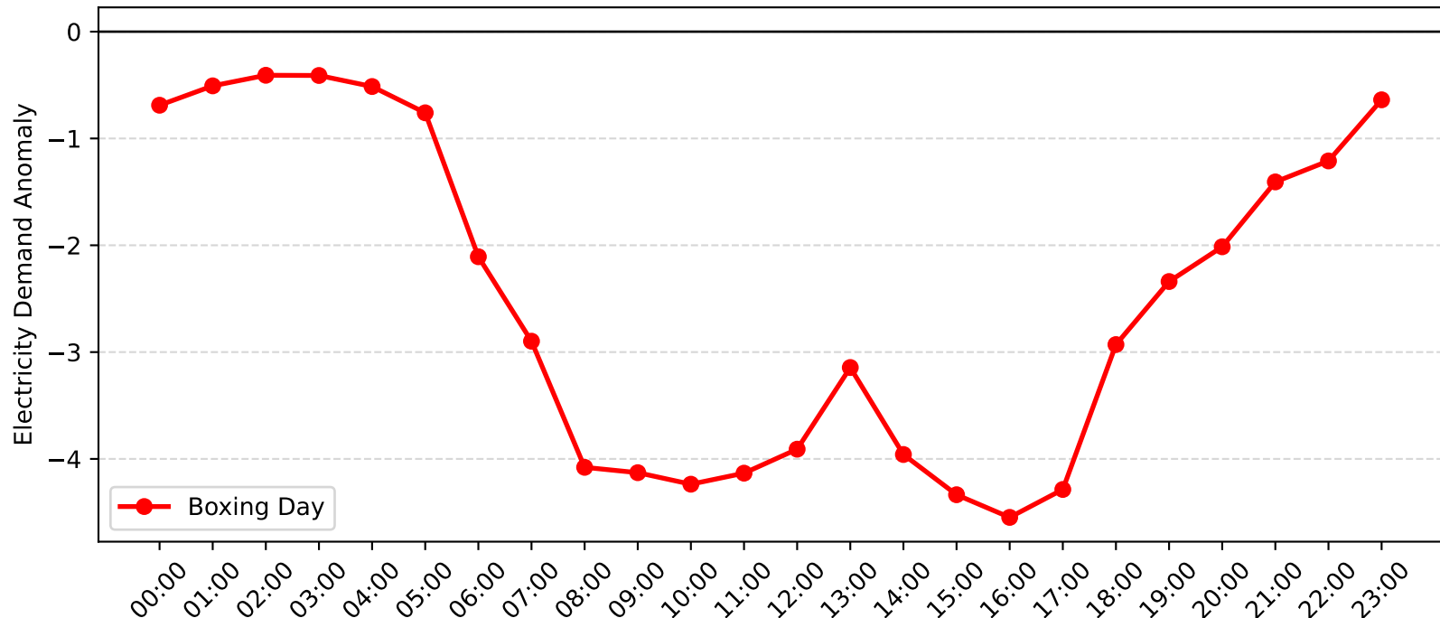
Pymble Demand Anomaly: Boxing Day (2014-2015)
