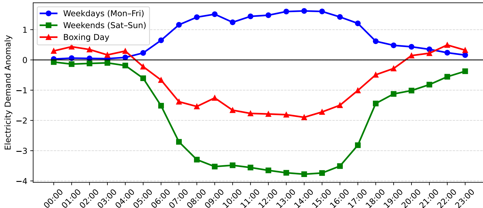
Beacon Hill Demand Anomaly: Boxing Day vs Weekday/Weekend (2016-2017)
