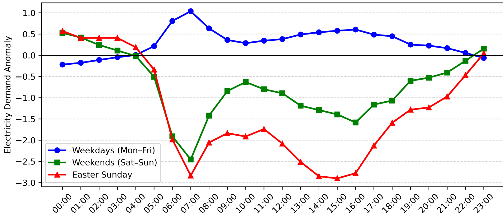
Blakehurst Demand Anomaly: Easter Sunday vs Weekday/Weekend (2005-2006)
