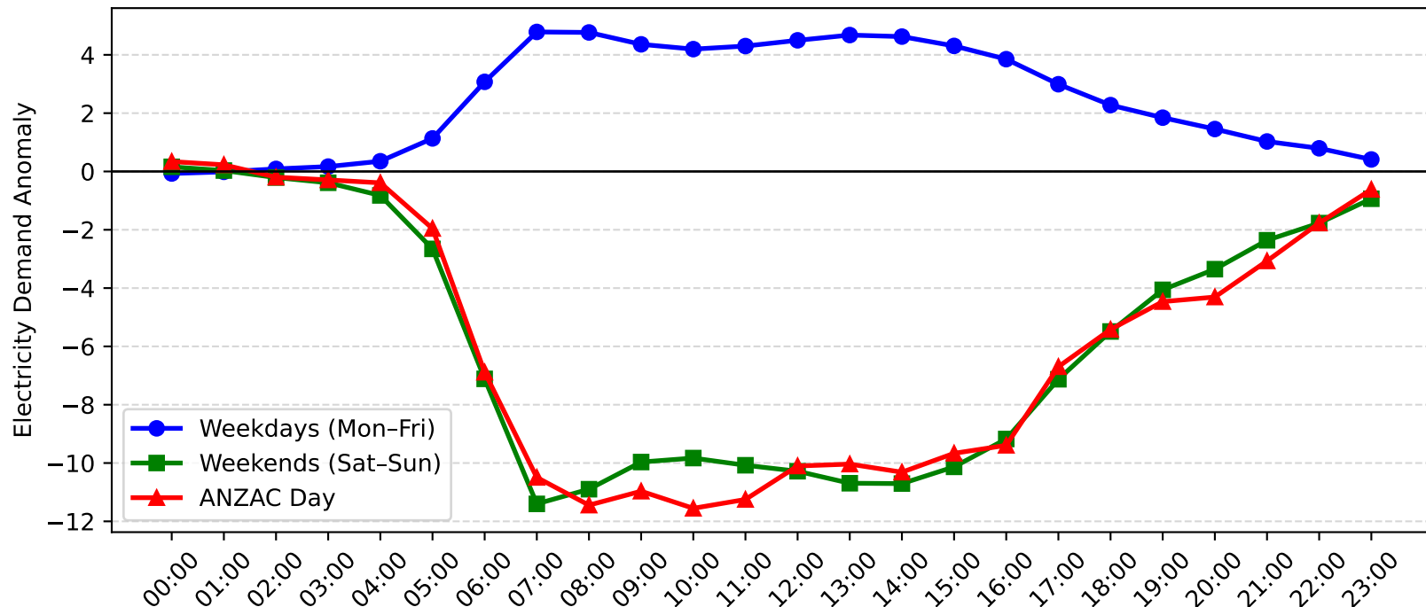
Zetland Demand Anomaly: ANZAC Day vs Weekday/Weekend (2008-2009)
