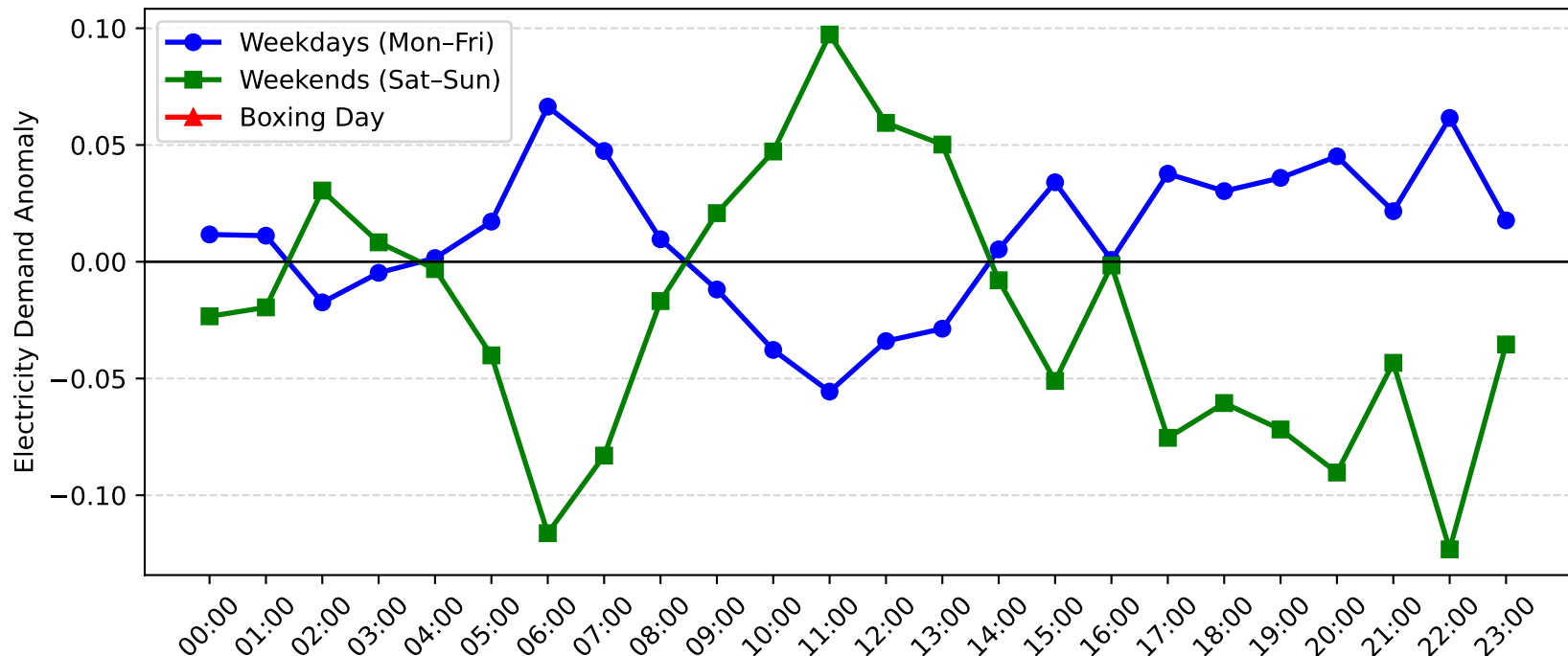
Jesmond Demand Anomaly: Boxing Day vs Weekday/Weekend (2009-2010)
