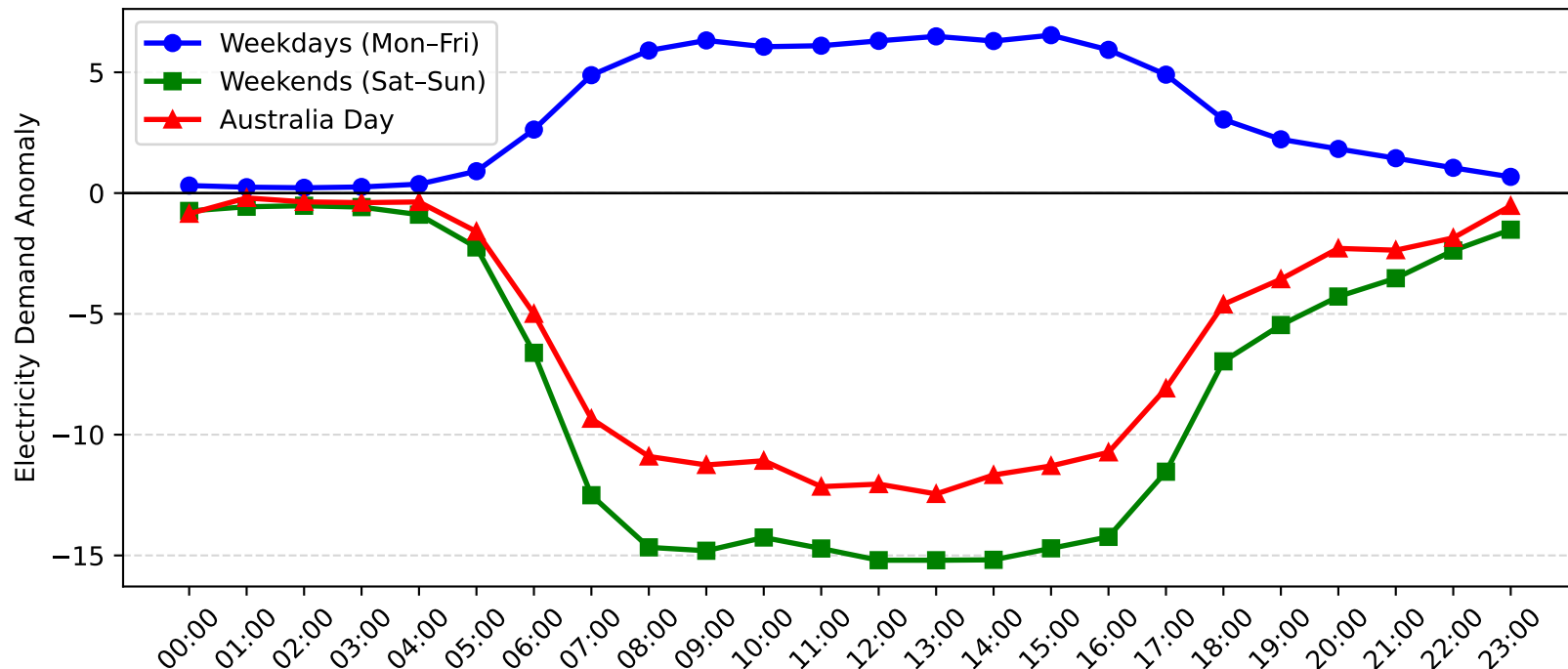
Gore Hill Demand Anomaly: Australia Day vs Weekday/Weekend (2008-2009)
