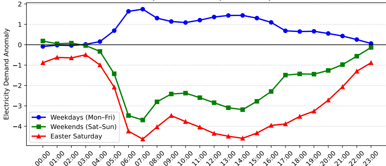
Kirrawee Demand Anomaly: Easter Saturday vs Weekday/Weekend (2009-2010)
