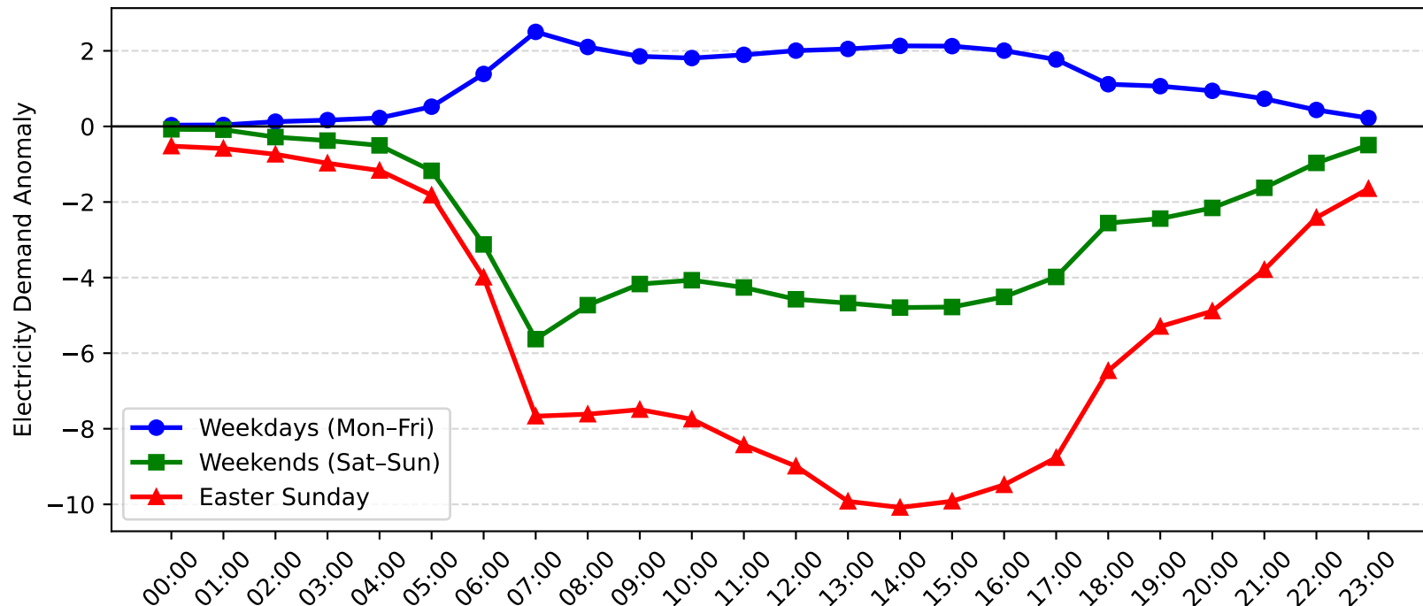
Epping Demand Anomaly: Easter Sunday vs Weekday/Weekend (2016-2017)
