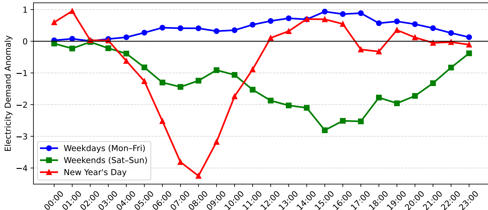
Charmhaven Demand Anomaly: New Year's Day vs Weekday/Weekend (2009-2010)
