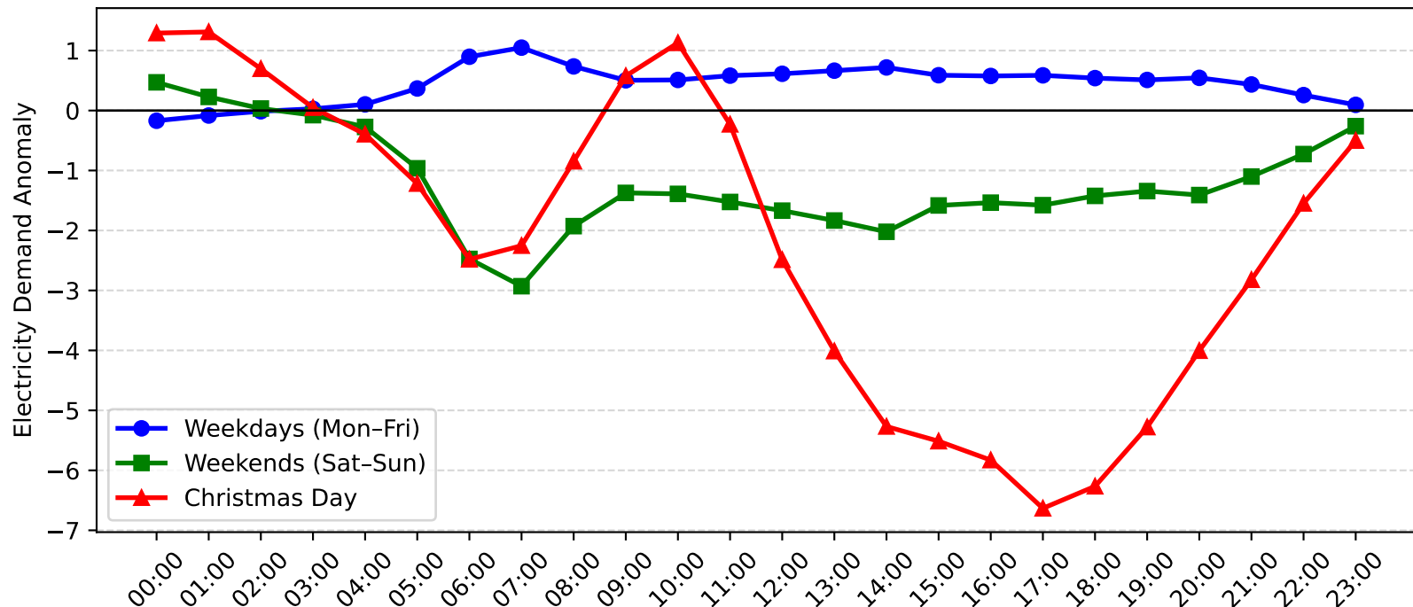
Mortdale Demand Anomaly: Christmas Day vs Weekday/Weekend (2014-2015)
