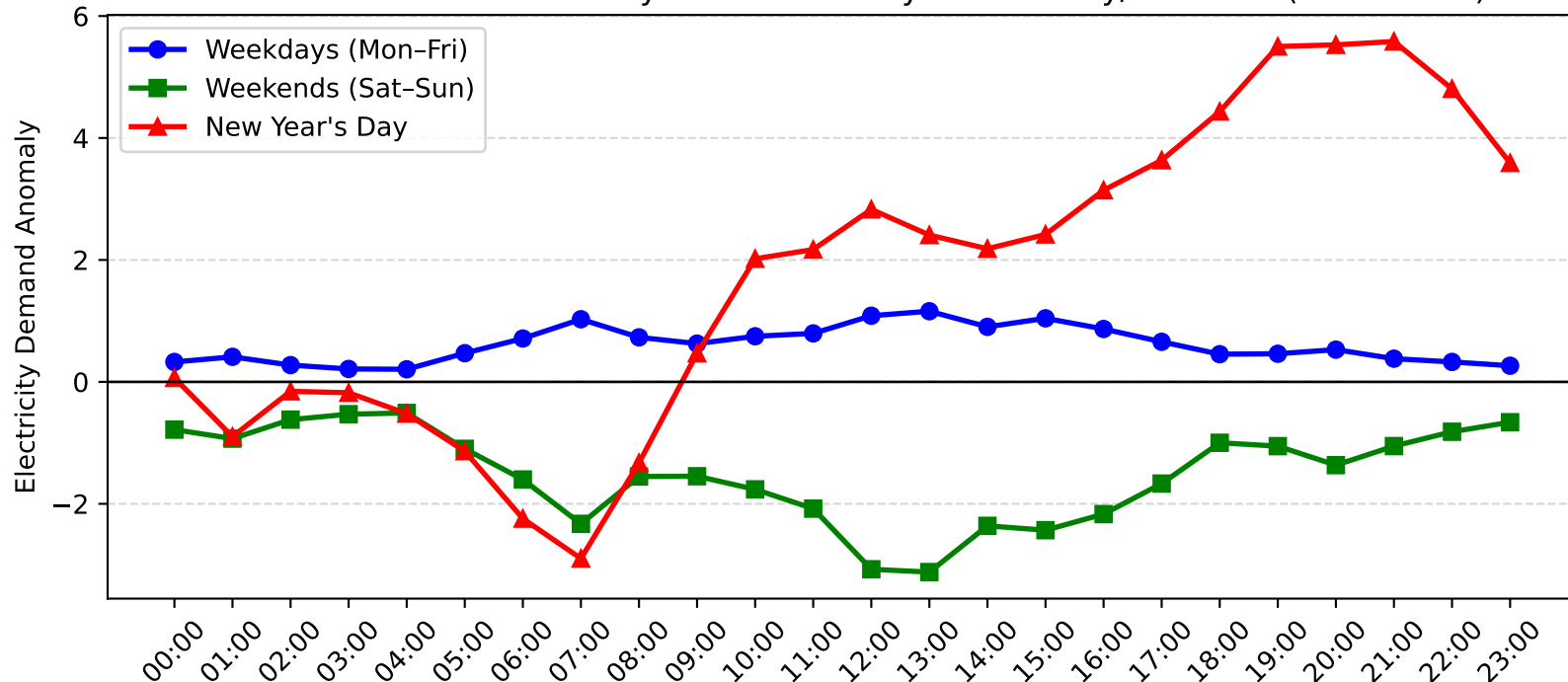
Rutherford Demand Anomaly: New Year's Day vs Weekday/Weekend (2005-2006)
