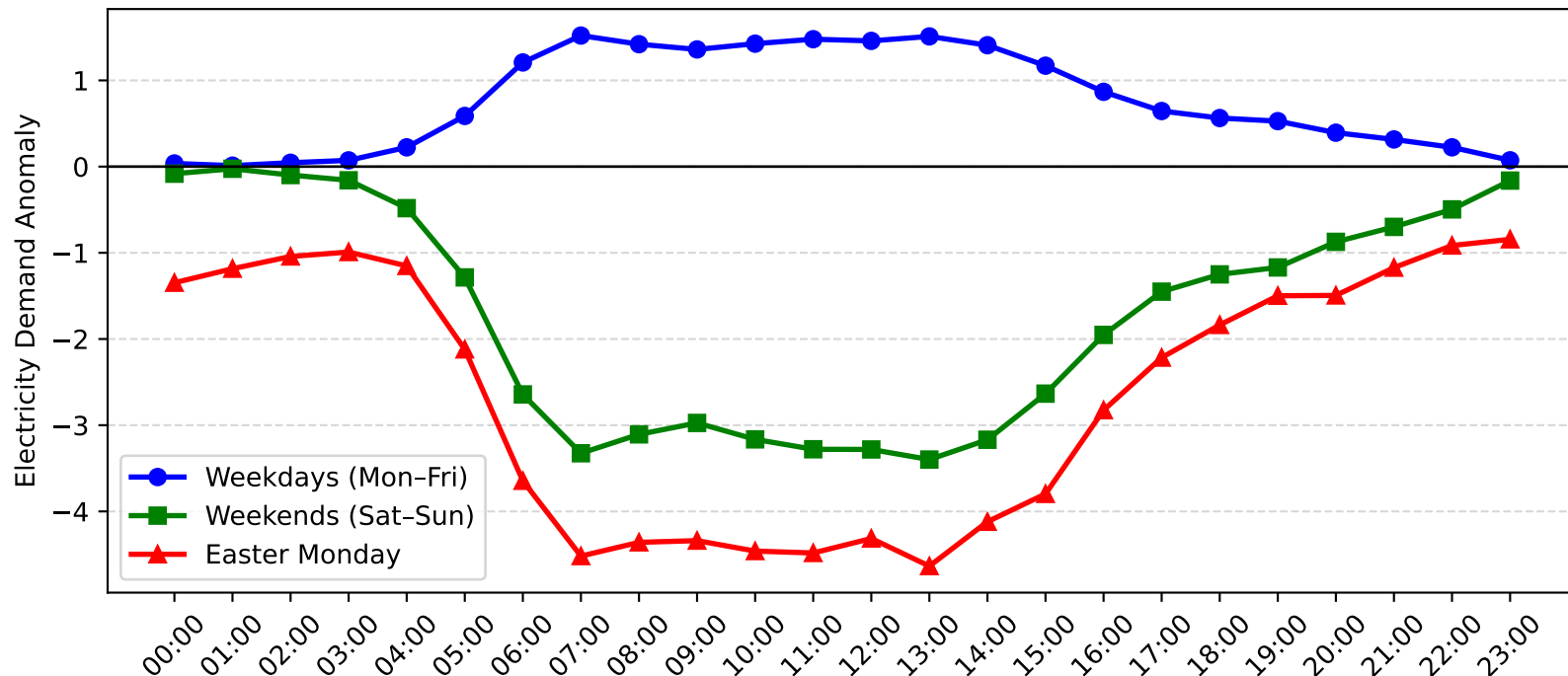
Wyong Demand Anomaly: Easter Monday vs Weekday/Weekend (2016-2017)
