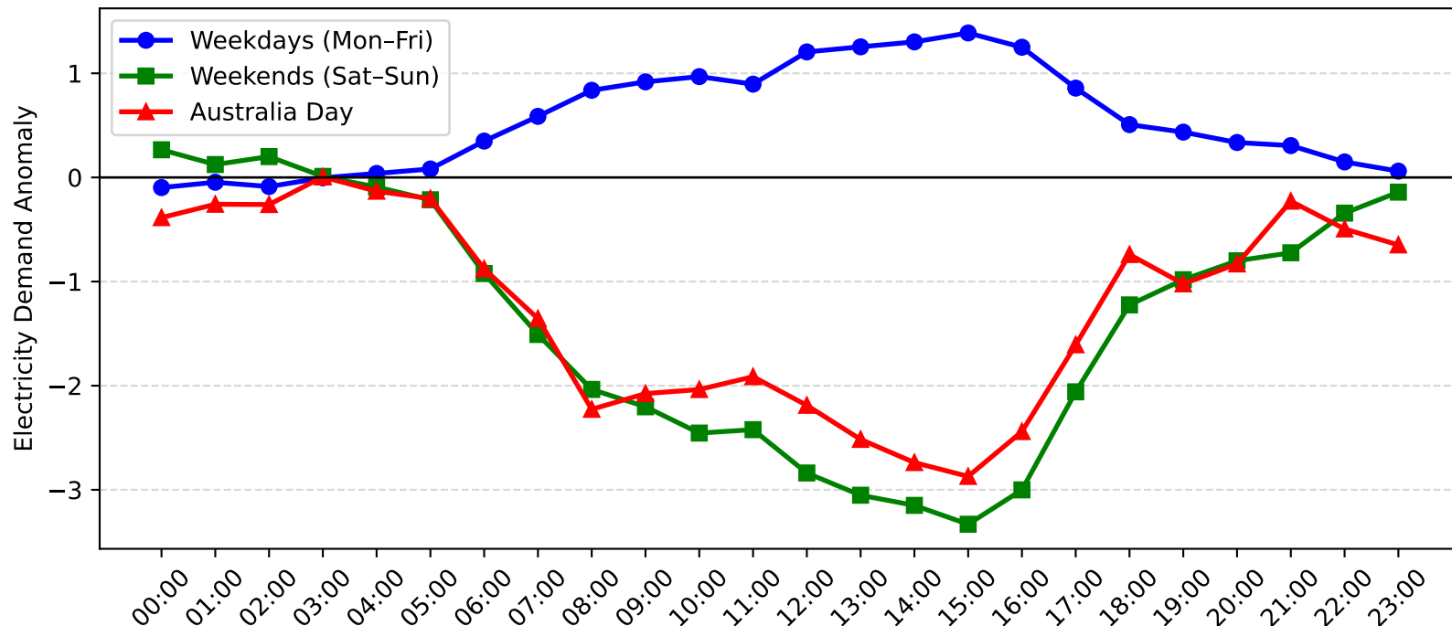
West Gosford Demand Anomaly: Australia Day vs Weekday/Weekend (2004-2005)
