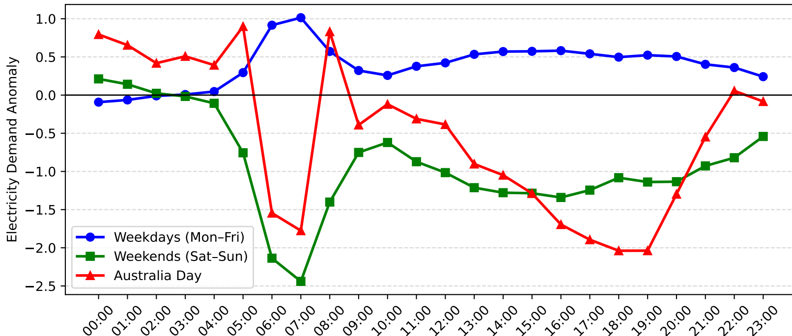
Dee Why West Demand Anomaly: Australia Day vs Weekday/Weekend (2013-2014)
