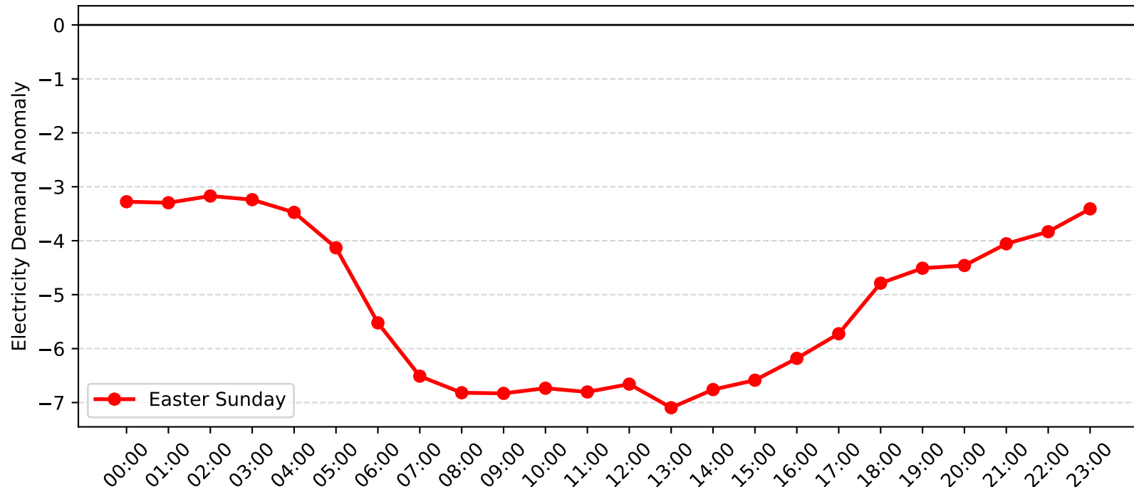
Leightonfield Demand Anomaly: Easter Sunday (2010-2011)
