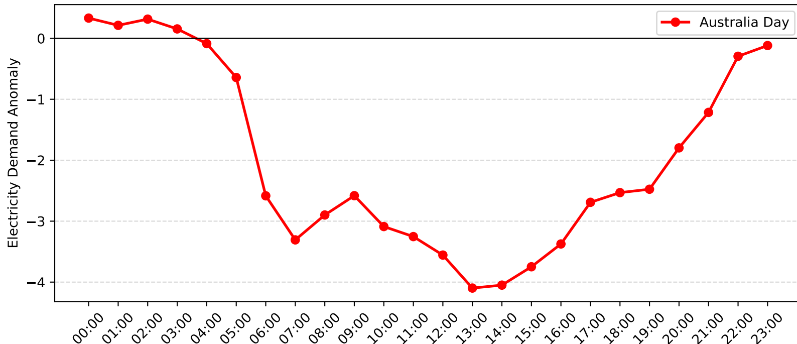
Kirrawee Demand Anomaly: Australia Day (2007-2008)
