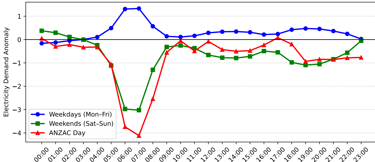
Mortdale Demand Anomaly: ANZAC Day vs Weekday/Weekend (2016-2017)
