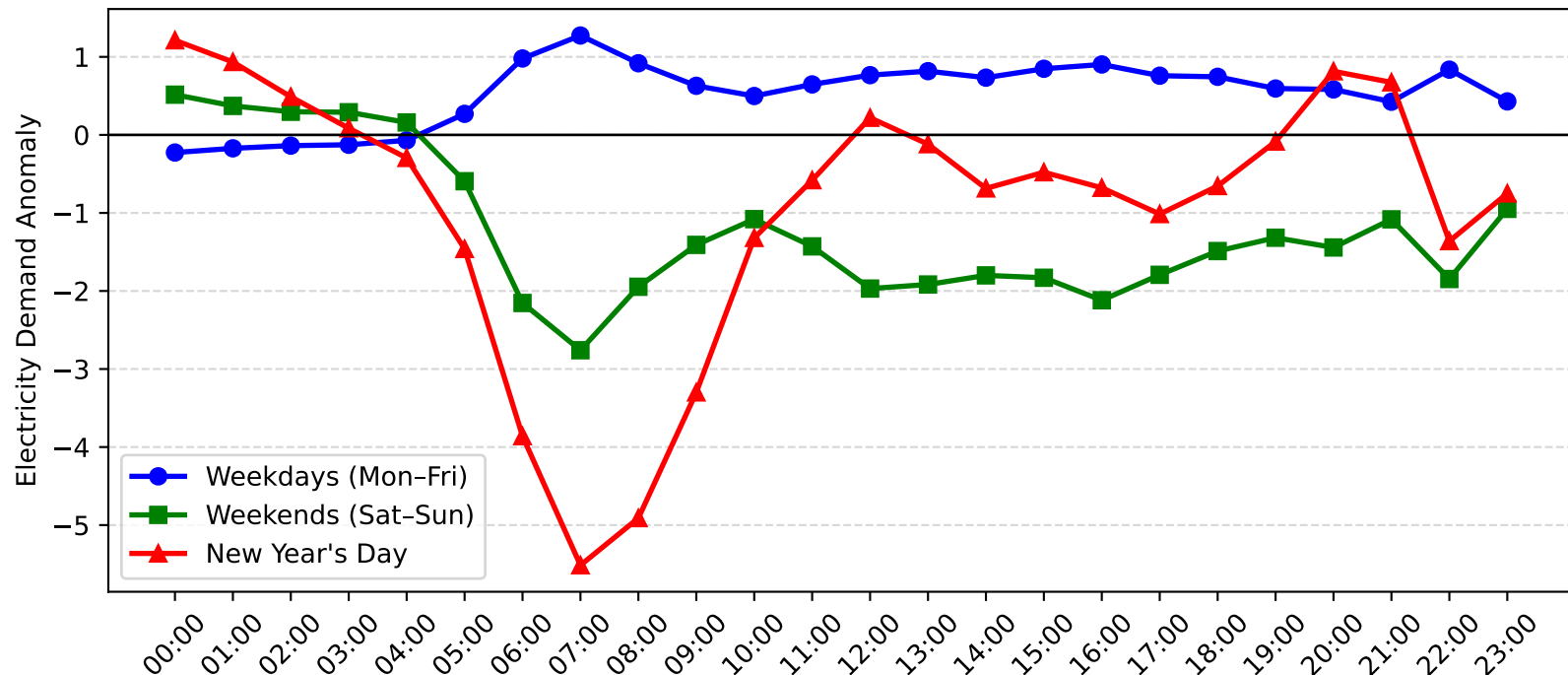
Dee Why West Demand Anomaly: New Year's Day vs Weekday/Weekend (2005-2006)
