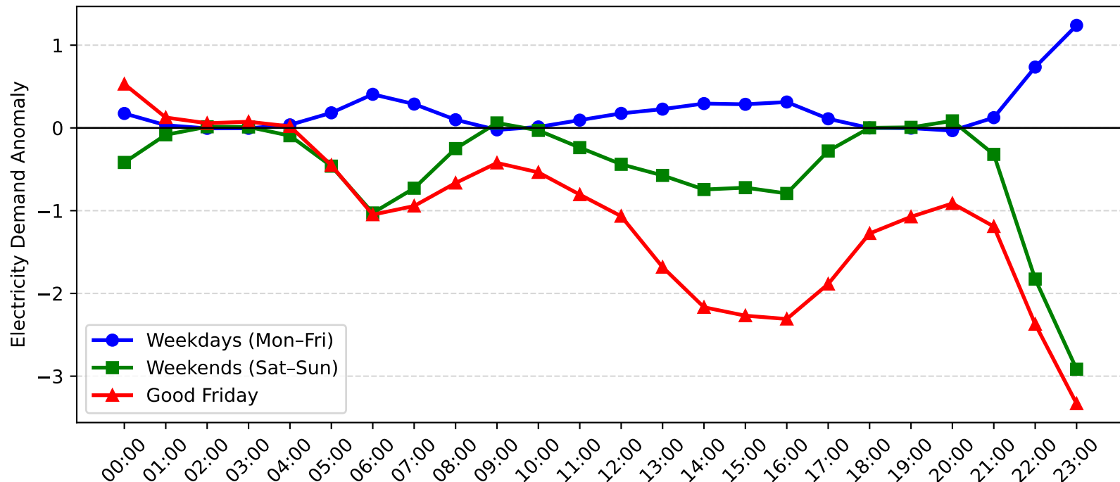
Muswellbrook Demand Anomaly: Good Friday vs Weekday/Weekend (2007-2008)
