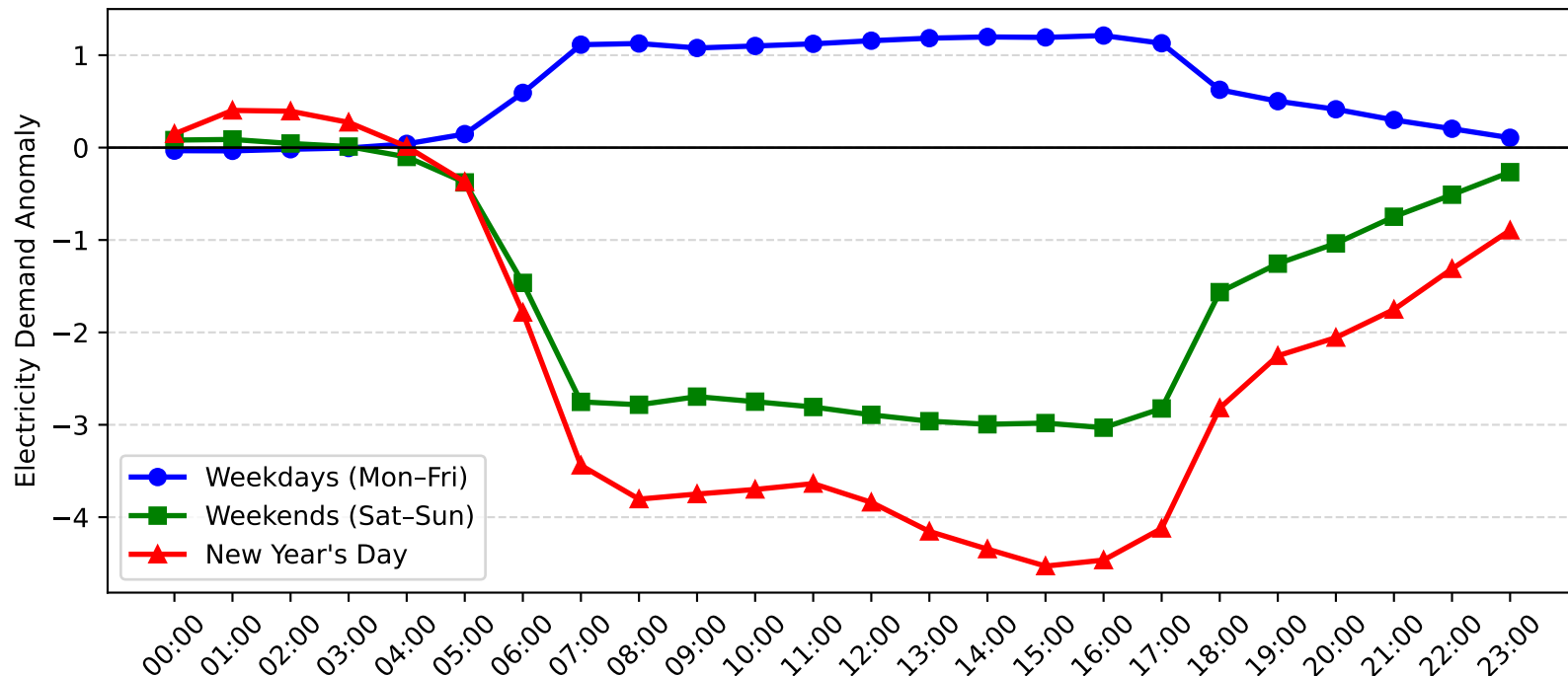
Pymble Demand Anomaly: New Year's Day vs Weekday/Weekend (2016-2017)
