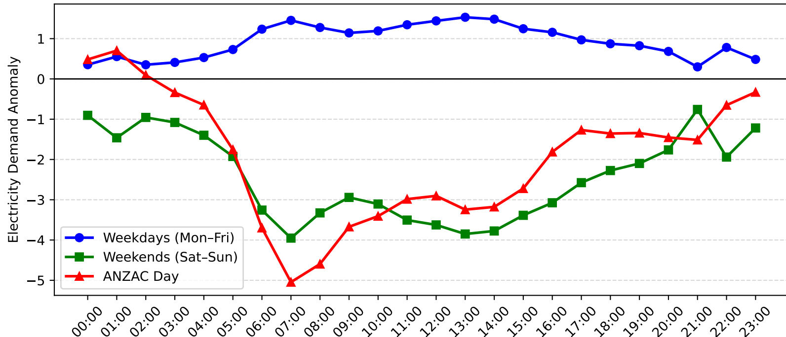
Cardiff Demand Anomaly: ANZAC Day vs Weekday/Weekend (2007-2008)
