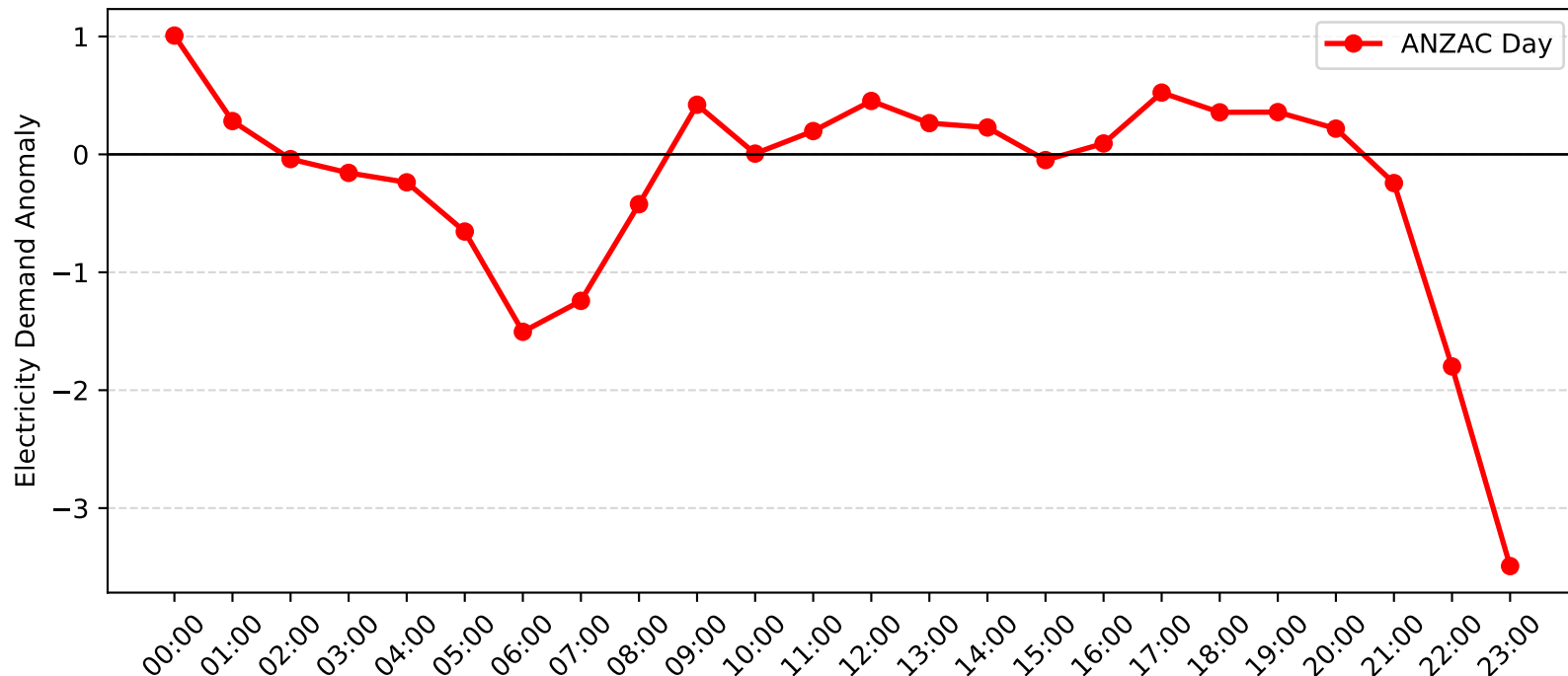
Muswellbrook Demand Anomaly: ANZAC Day (2007-2008)
