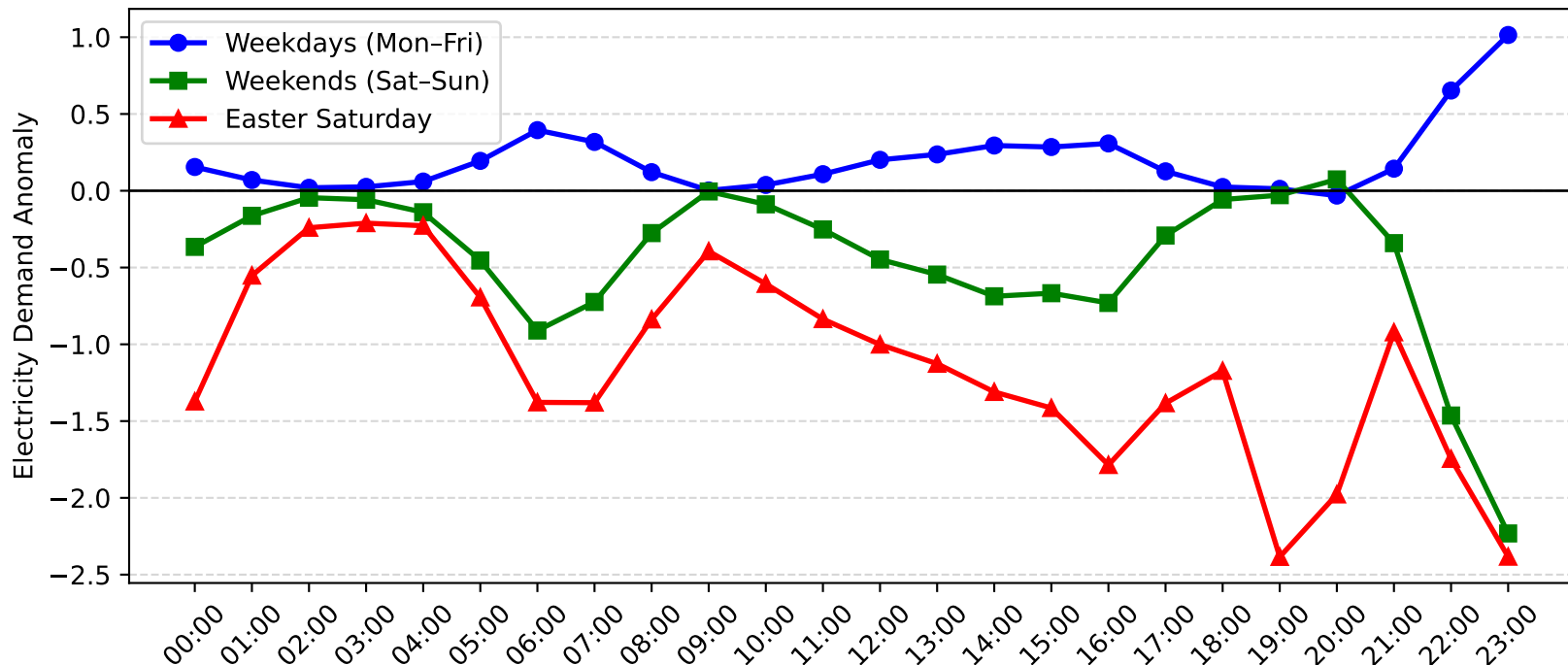
Muswellbrook Demand Anomaly: Easter Saturday vs Weekday/Weekend (2008-2009)
