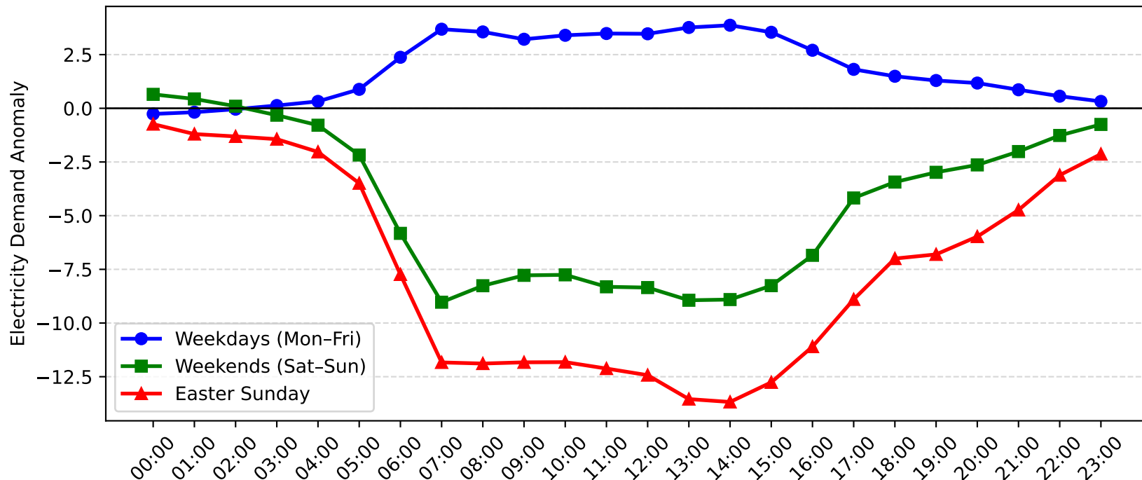
Marrickville Demand Anomaly: Easter Sunday vs Weekday/Weekend (2006-2007)
