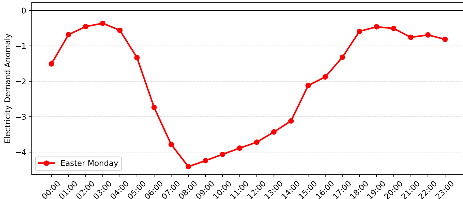
Rutherford Demand Anomaly: Easter Monday (2016-2017)
