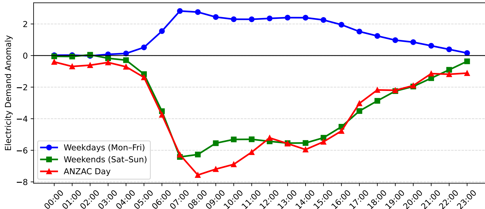
Zetland Demand Anomaly: ANZAC Day vs Weekday/Weekend (2016-2017)
