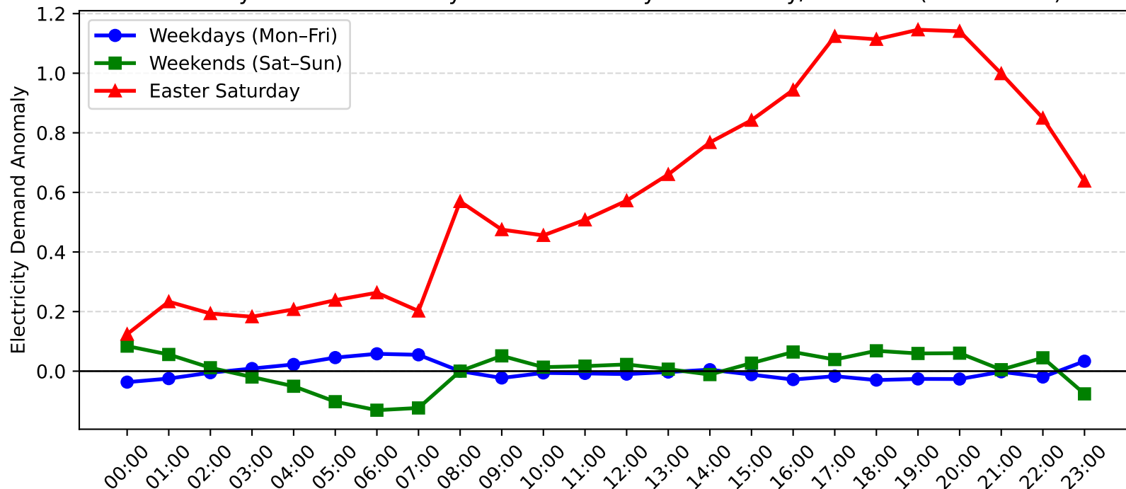
Rothbury Demand Anomaly: Easter Saturday vs Weekday/Weekend (2016-2017)
