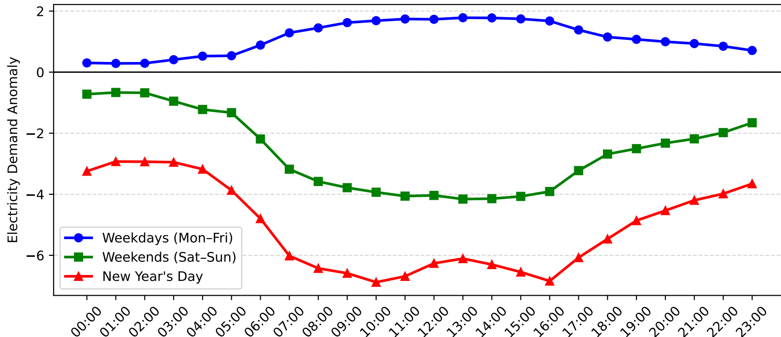
Leightonfield Demand Anomaly: New Year's Day vs Weekday/Weekend (2017-2018)
