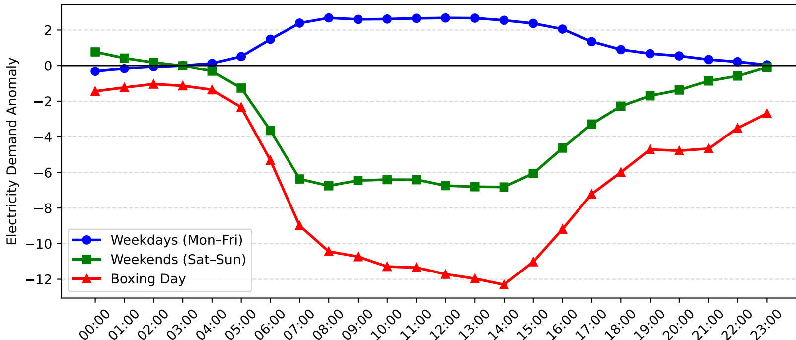
Marrickville Demand Anomaly: Boxing Day vs Weekday/Weekend (2009-2010)
