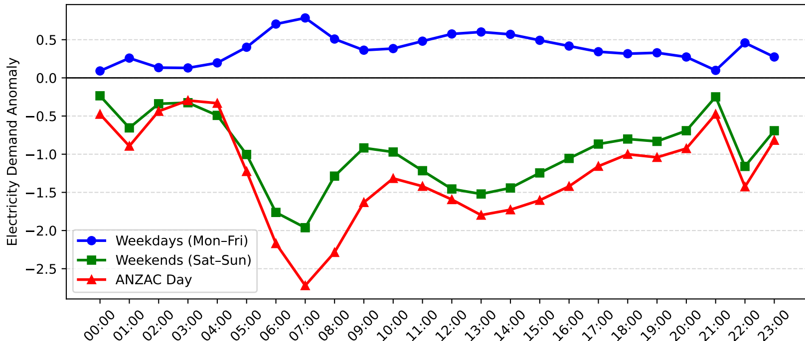
Cardiff Demand Anomaly: ANZAC Day vs Weekday/Weekend (2011-2012)
