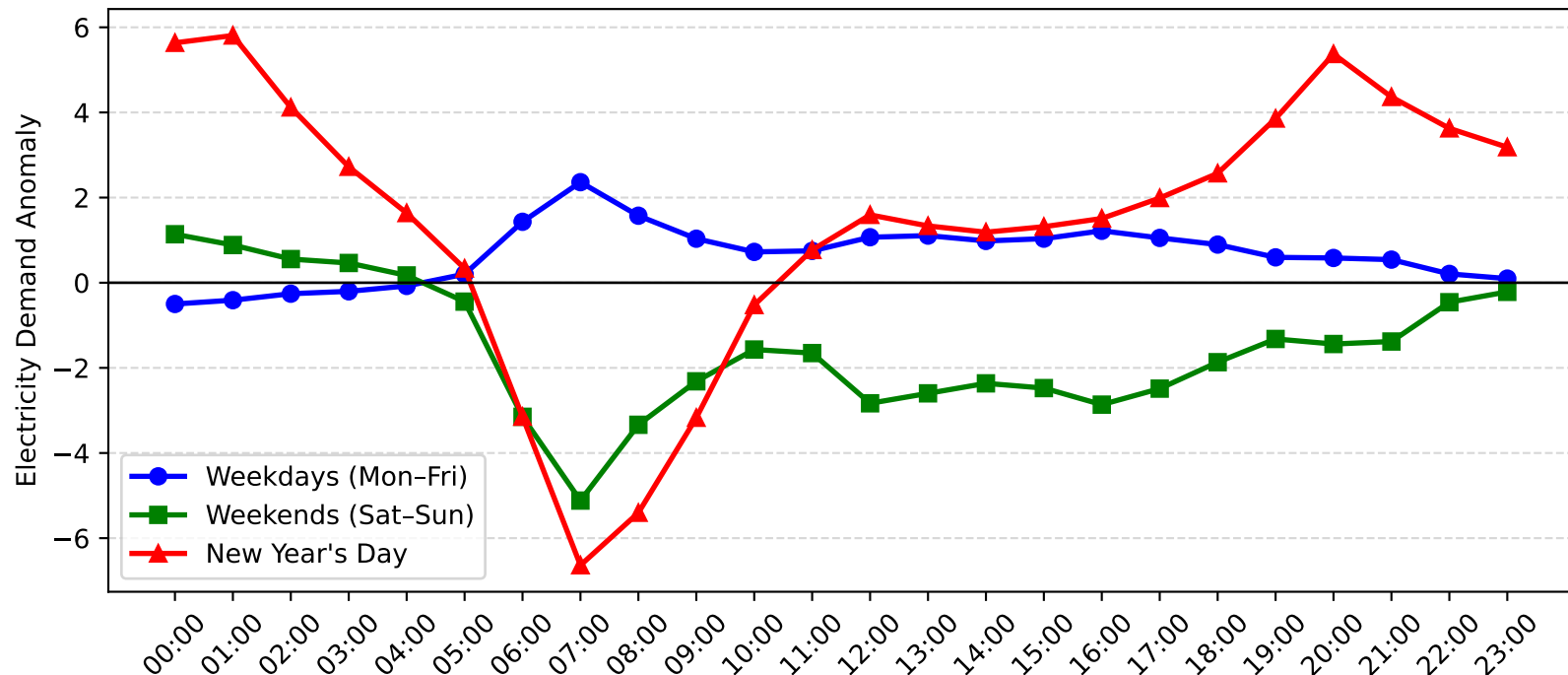
Mosman Demand Anomaly: New Year's Day vs Weekday/Weekend (2005-2006)
