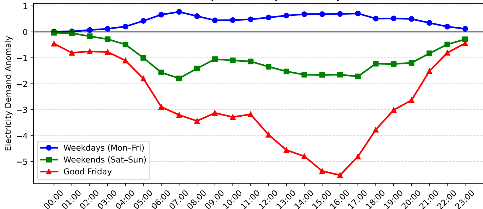
Charmhaven Demand Anomaly: Good Friday vs Weekday/Weekend (2016-2017)
