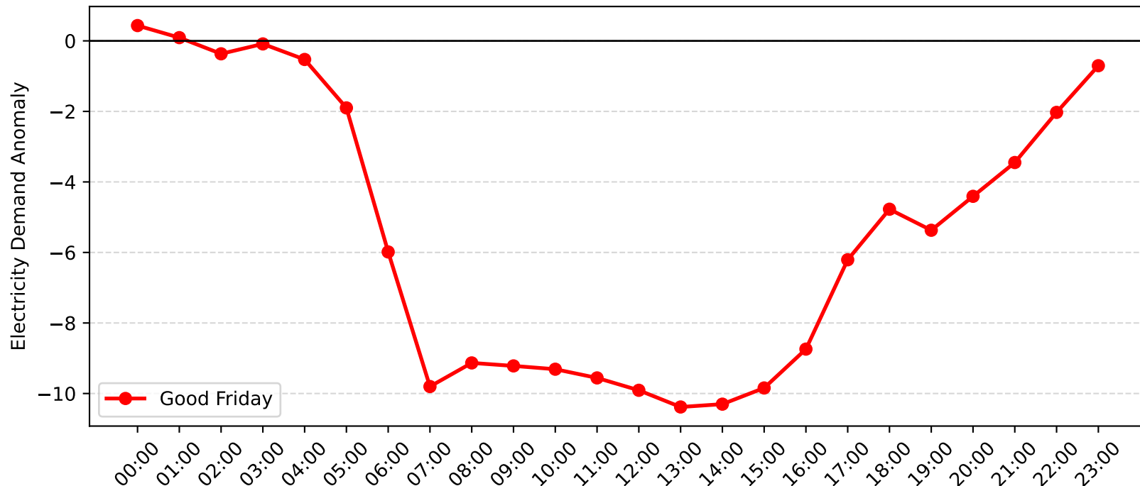
Marrickville Demand Anomaly: Good Friday (2006-2007)
