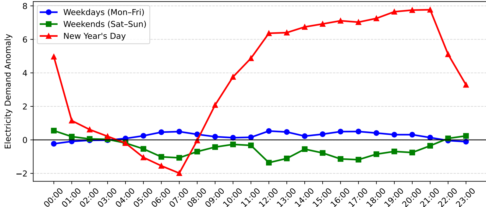
Charmhaven Demand Anomaly: New Year's Day vs Weekday/Weekend (2005-2006)
