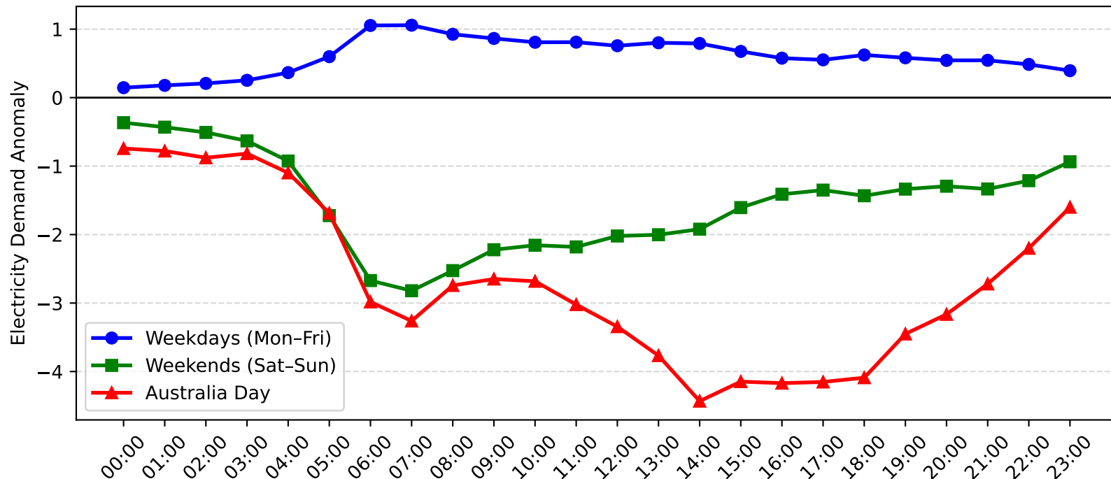
Lisarow Demand Anomaly: Australia Day vs Weekday/Weekend (2014-2015)
