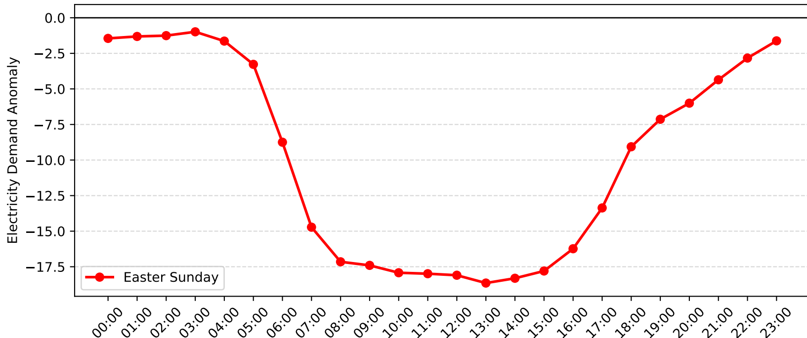
Gore Hill Demand Anomaly: Easter Sunday (2008-2009)
