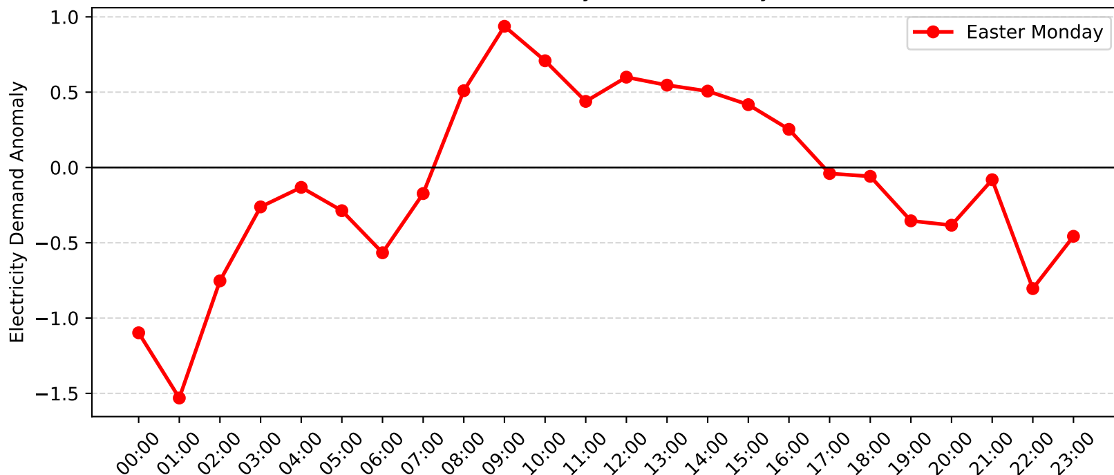
Swansea Demand Anomaly: Easter Monday (2011-2012)
