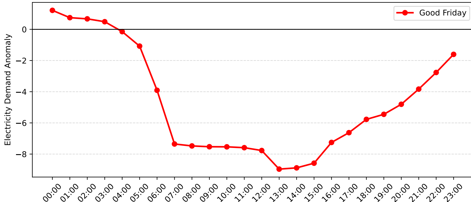
Marrickville Demand Anomaly: Good Friday (2012-2013)
