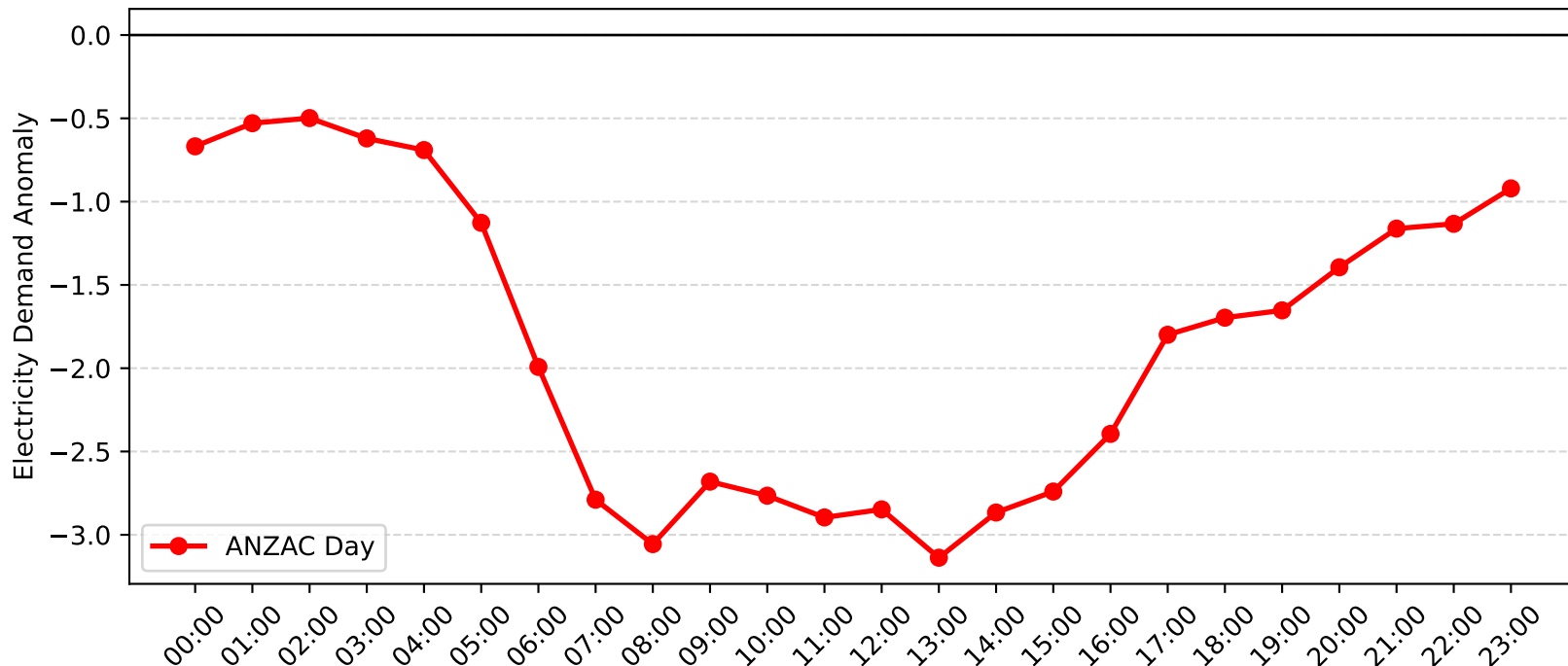
Mayfield West Demand Anomaly: ANZAC Day (2014-2015)
