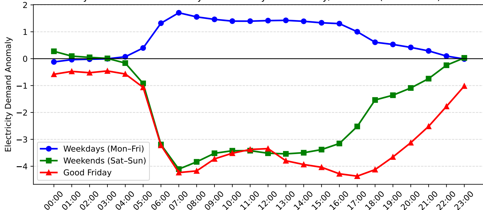
Pymble Demand Anomaly: Good Friday vs Weekday/Weekend (2010-2011)
