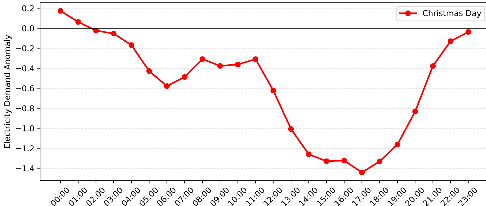
Narrabeen Demand Anomaly: Christmas Day (2015-2016)
