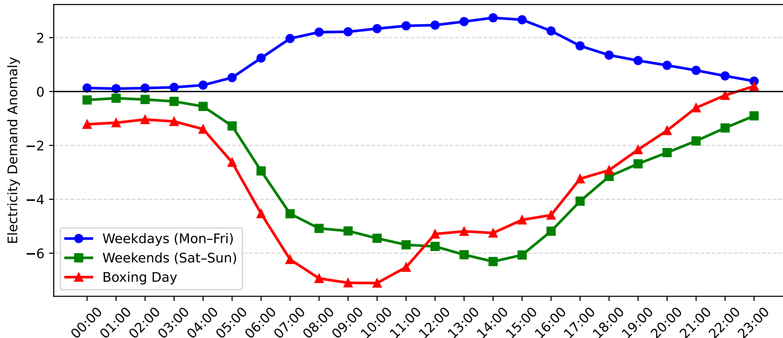
Bankstown Demand Anomaly: Boxing Day vs Weekday/Weekend (2015-2016)
