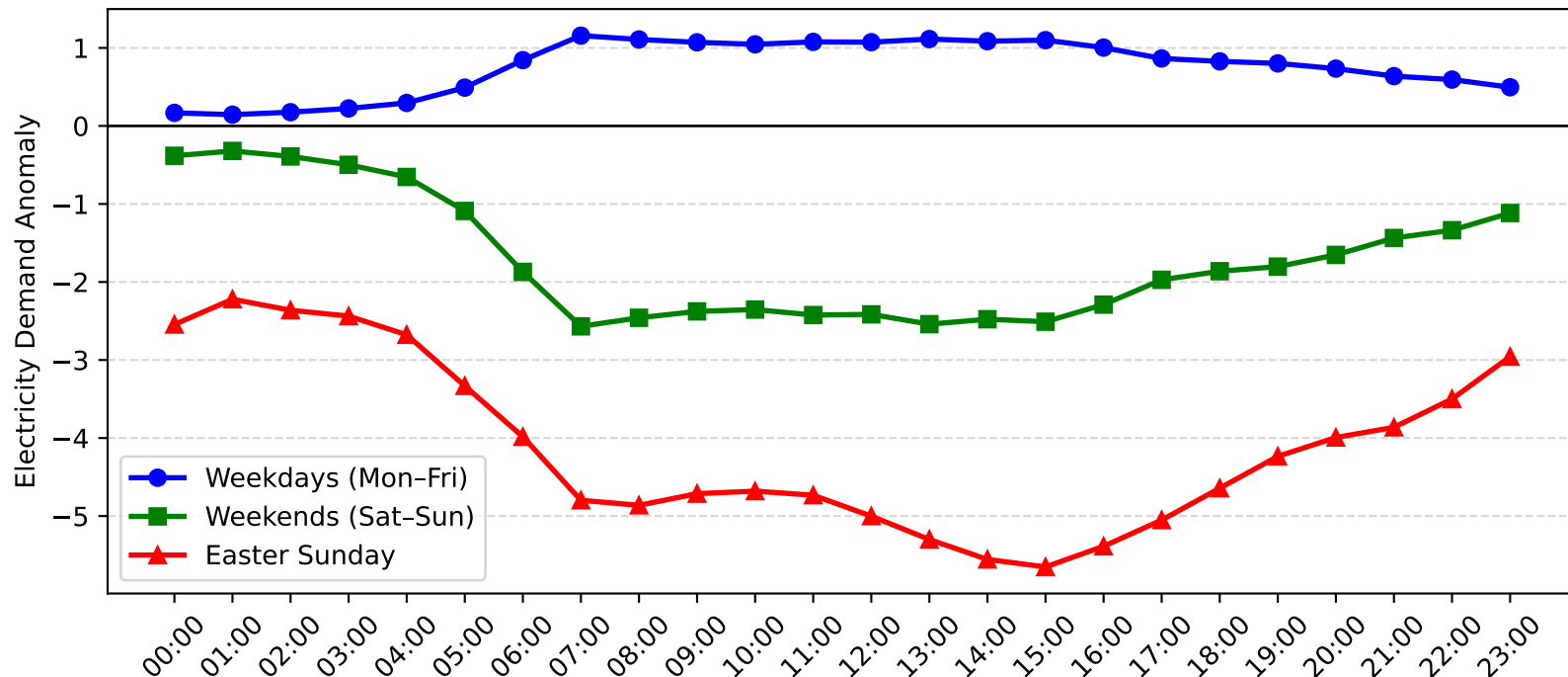
Bass Hill Demand Anomaly: Easter Sunday vs Weekday/Weekend (2016-2017)
