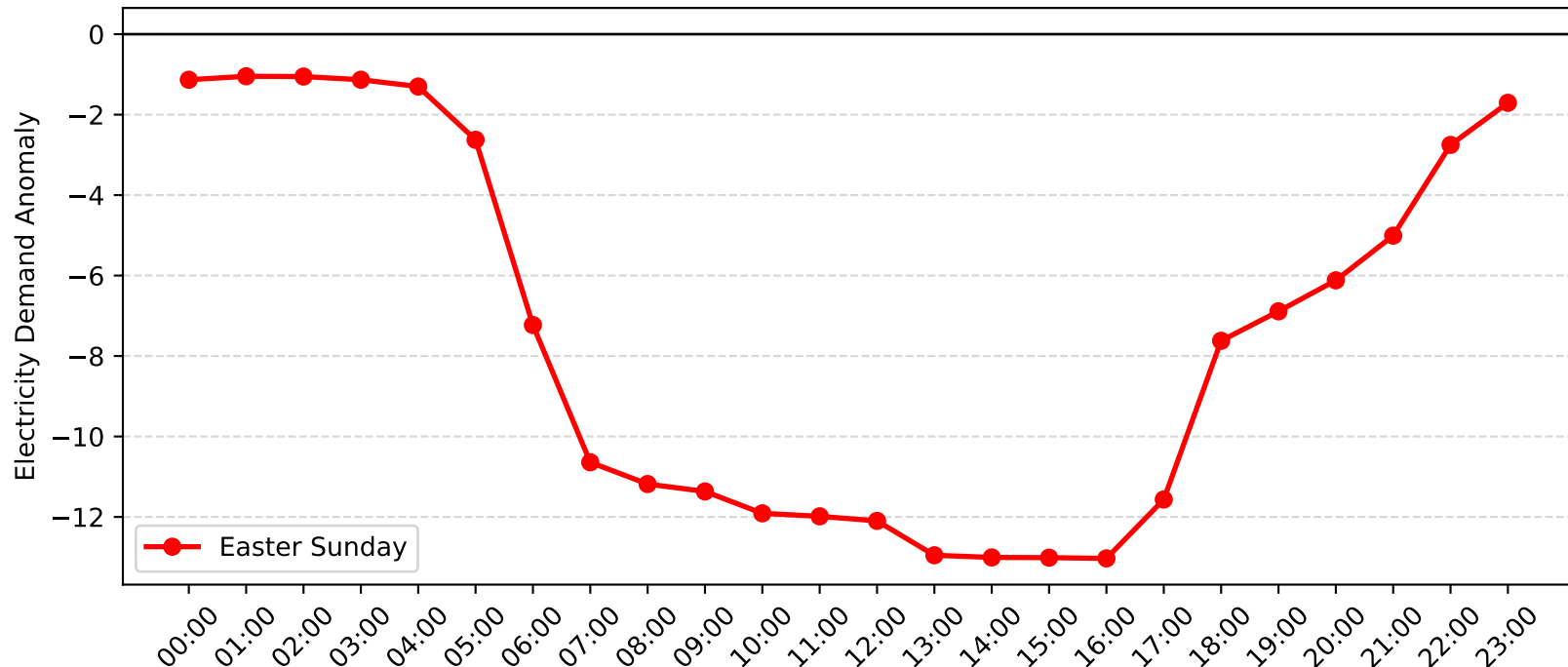
Epping Demand Anomaly: Easter Sunday (2008-2009)
