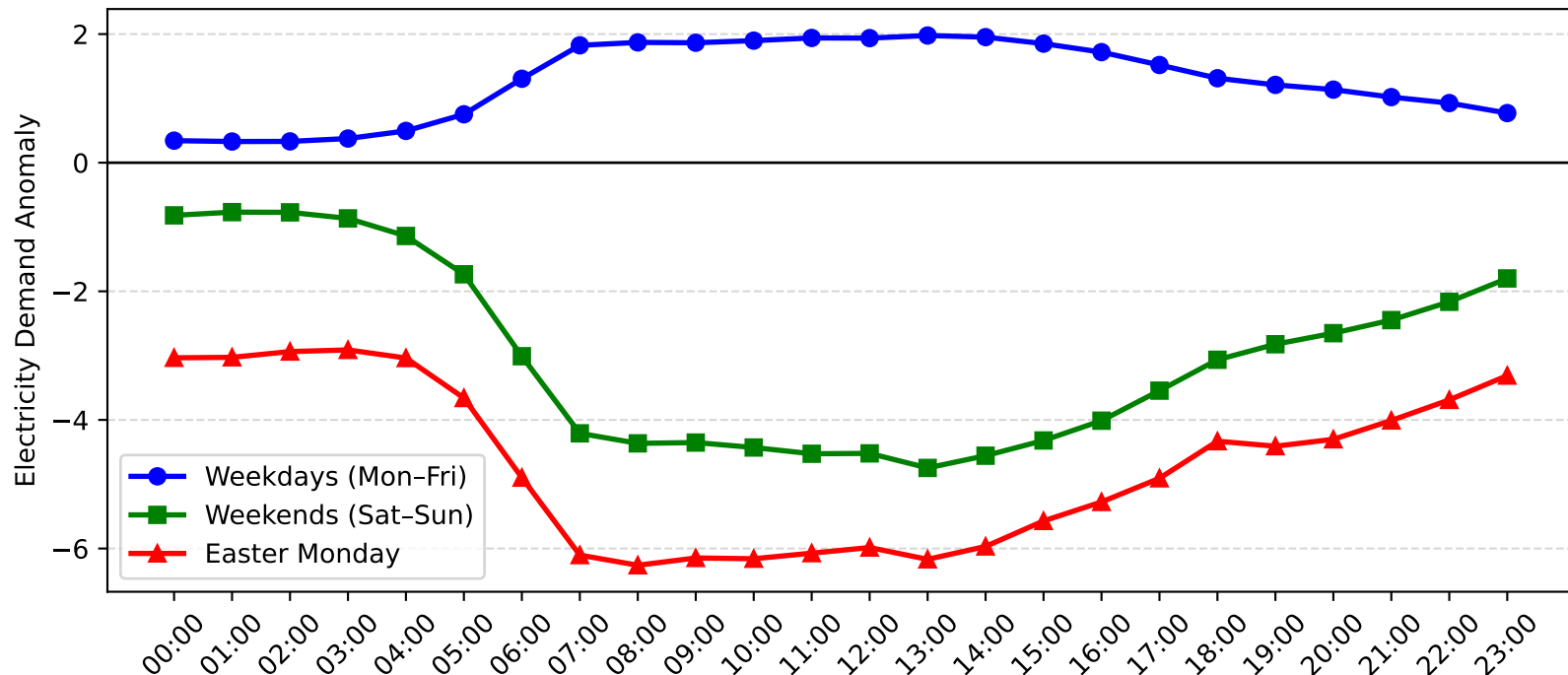
Leightonfield Demand Anomaly: Easter Monday vs Weekday/Weekend (2011-2012)
