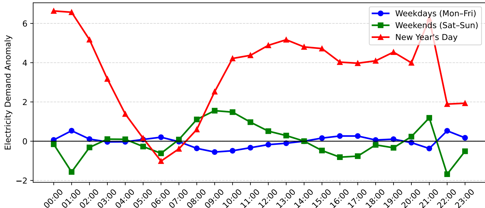
Nelson Bay Demand Anomaly: New Year's Day vs Weekday/Weekend (2009-2010)
