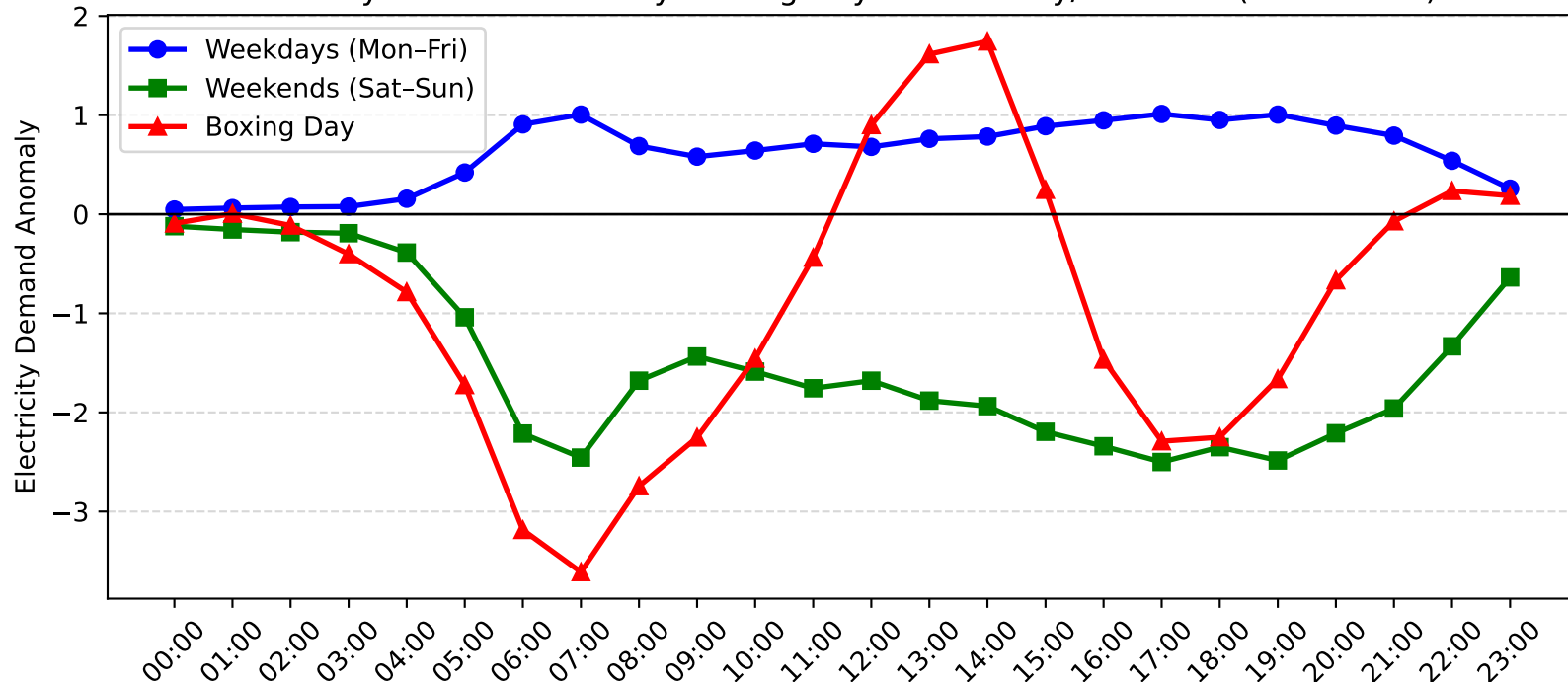
Revesby Demand Anomaly: Boxing Day vs Weekday/Weekend (2015-2016)
