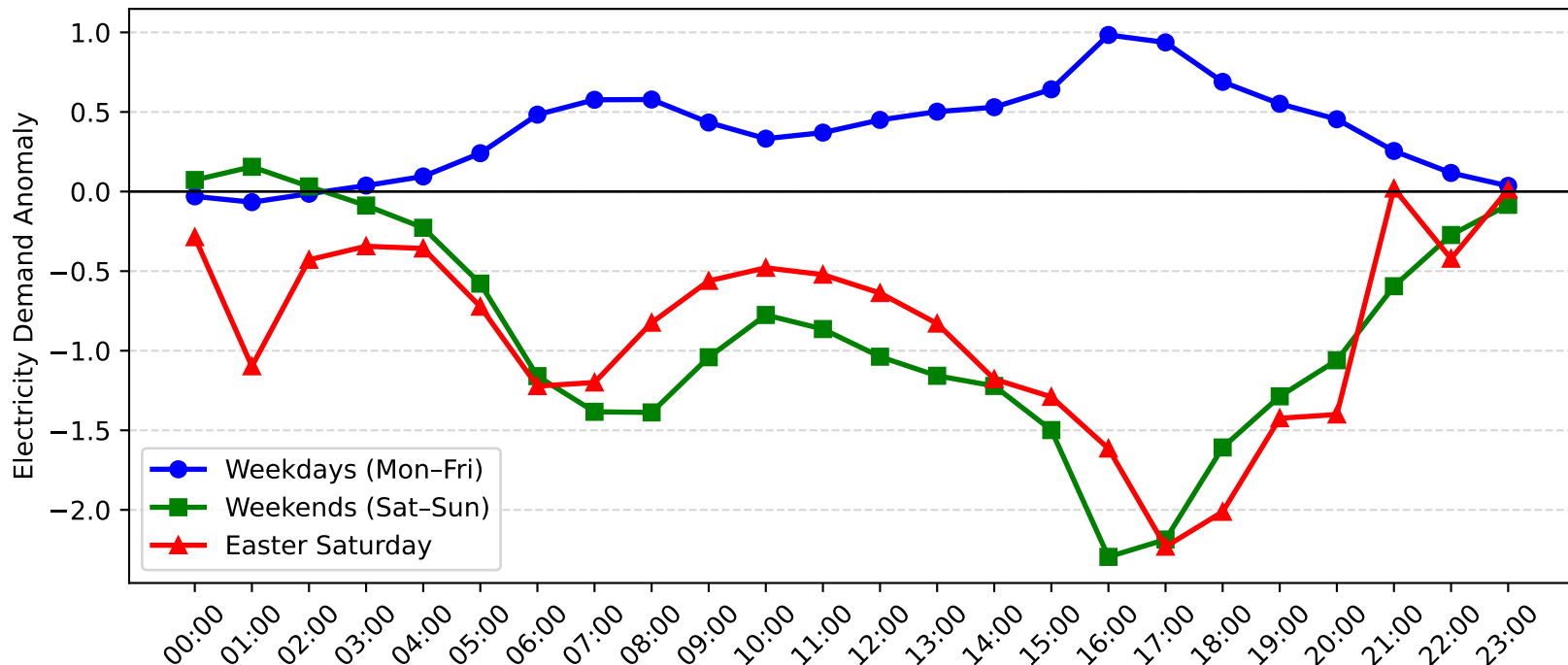
Erina Demand Anomaly: Easter Saturday vs Weekday/Weekend (2012-2013)
