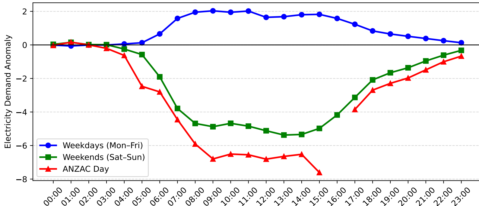
Green Square Demand Anomaly: ANZAC Day vs Weekday/Weekend (2014-2015)
