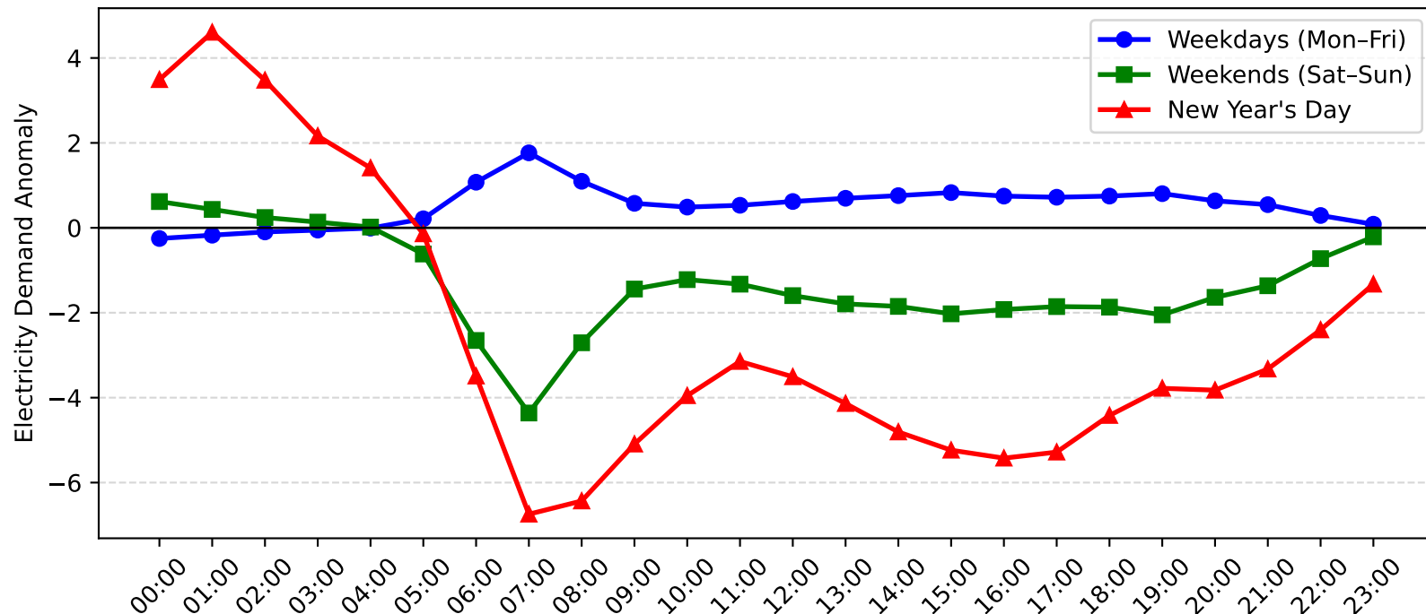
Mosman Demand Anomaly: New Year's Day vs Weekday/Weekend (2016-2017)
