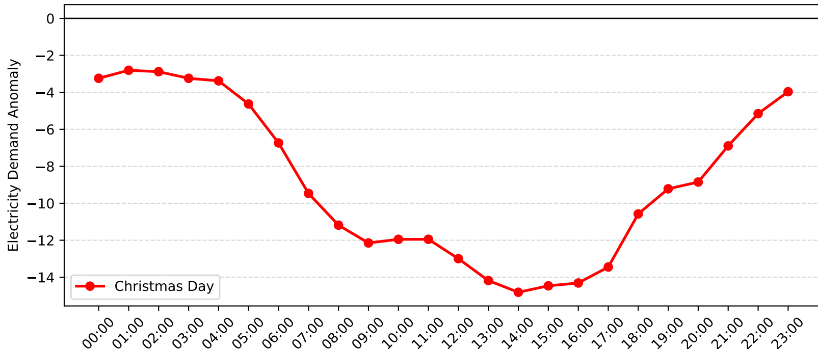
Burwood Demand Anomaly: Christmas Day (2016-2017)
