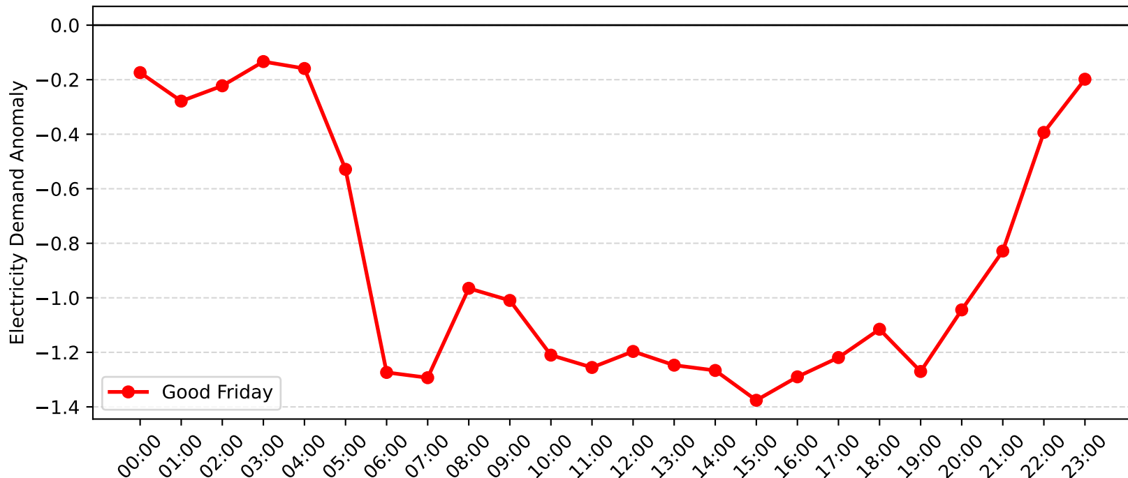
Narrabeen Demand Anomaly: Good Friday (2011-2012)
