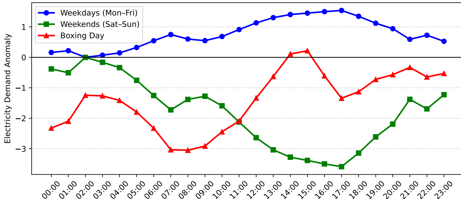
Jesmond Demand Anomaly: Boxing Day vs Weekday/Weekend (2015-2016)
