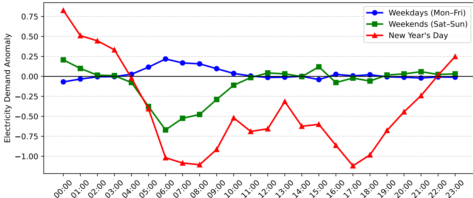
Woy Woy Demand Anomaly: New Year's Day vs Weekday/Weekend (2014-2015)
