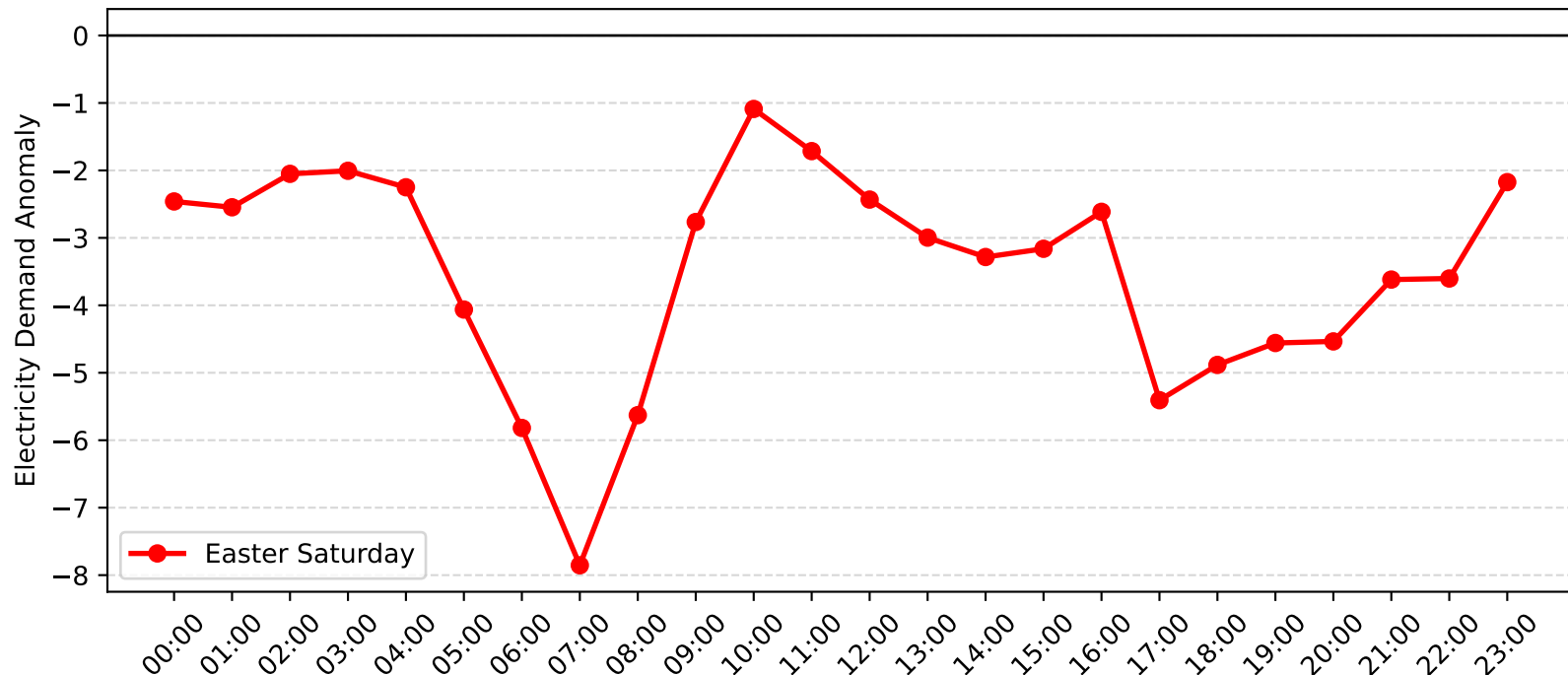
Meadowbank Demand Anomaly: Easter Saturday (2009-2010)
