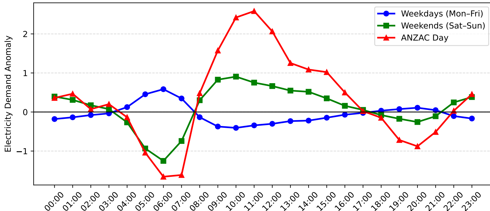
Umina Demand Anomaly: ANZAC Day vs Weekday/Weekend (2010-2011)
