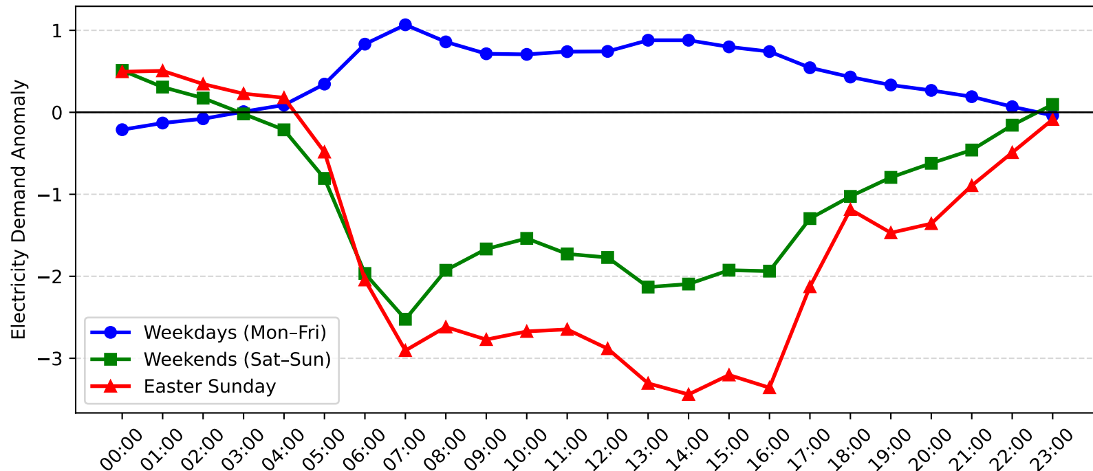
Rockdale Demand Anomaly: Easter Sunday vs Weekday/Weekend (2005-2006)
