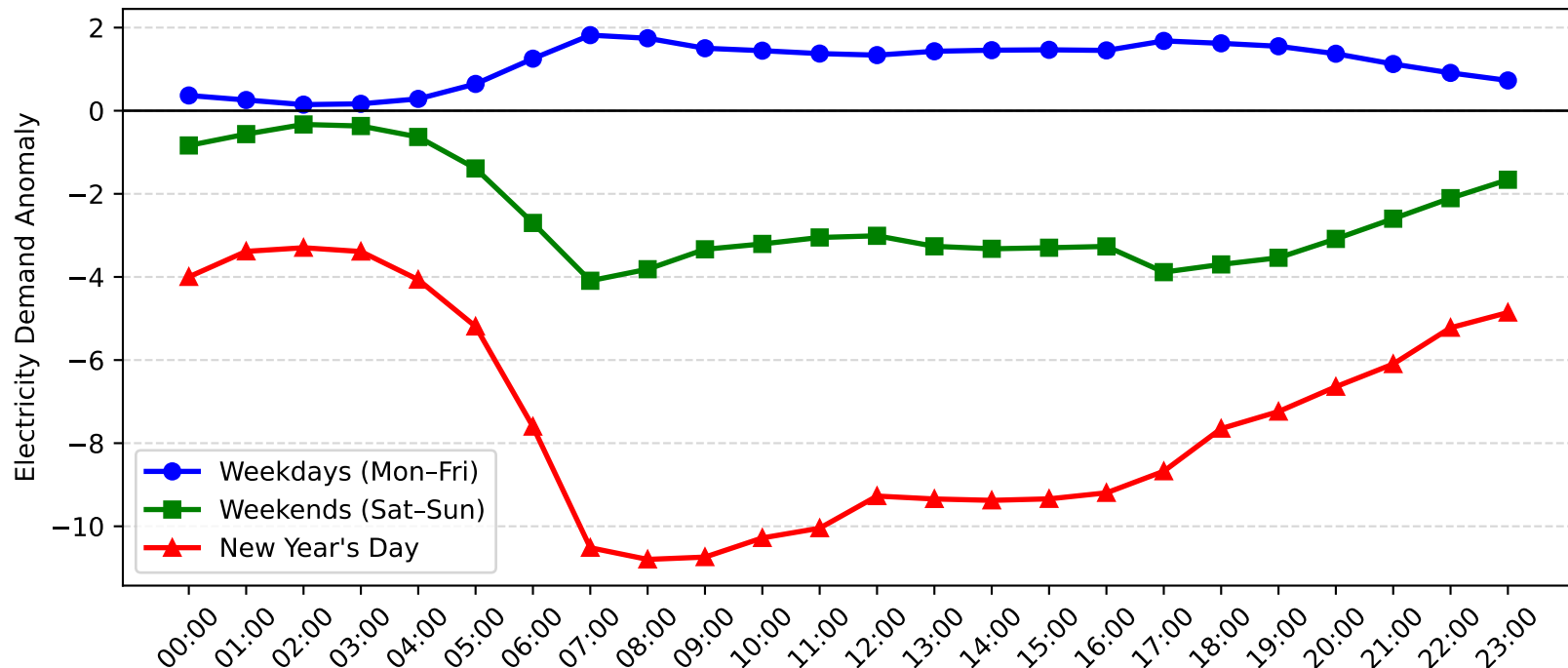
Maroubra Demand Anomaly: New Year's Day vs Weekday/Weekend (2011-2012)
