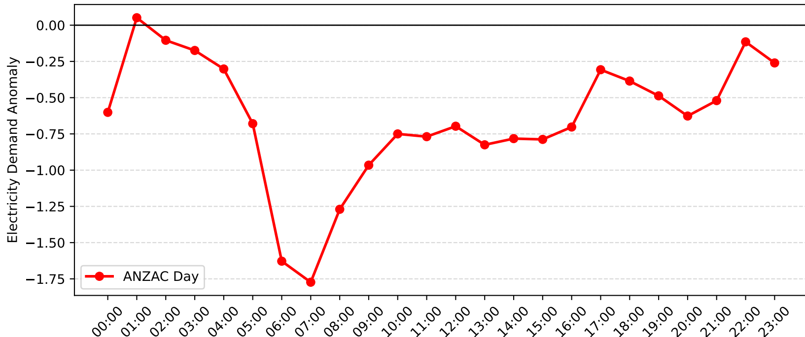
Morisset Demand Anomaly: ANZAC Day (2011-2012)
