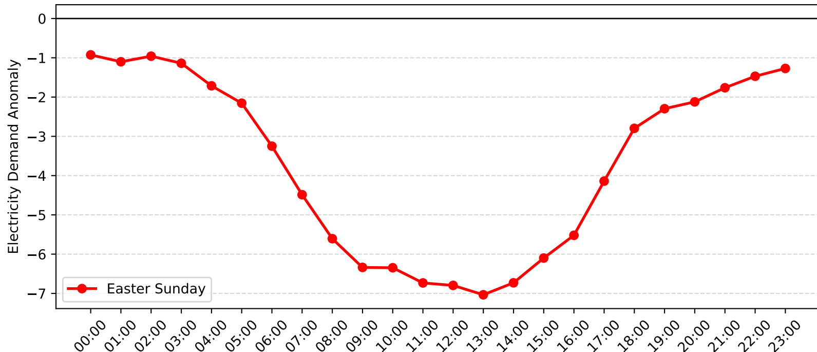
Auburn Demand Anomaly: Easter Sunday (2016-2017)
