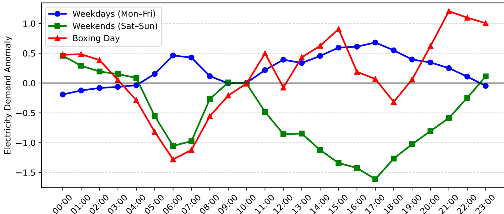
Avoca Demand Anomaly: Boxing Day vs Weekday/Weekend (2015-2016)
