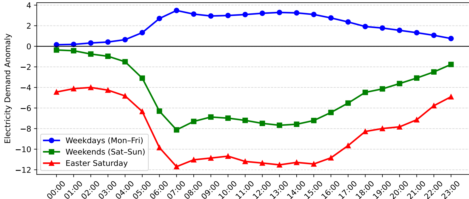
Sefton Demand Anomaly: Easter Saturday vs Weekday/Weekend (2012-2013)
