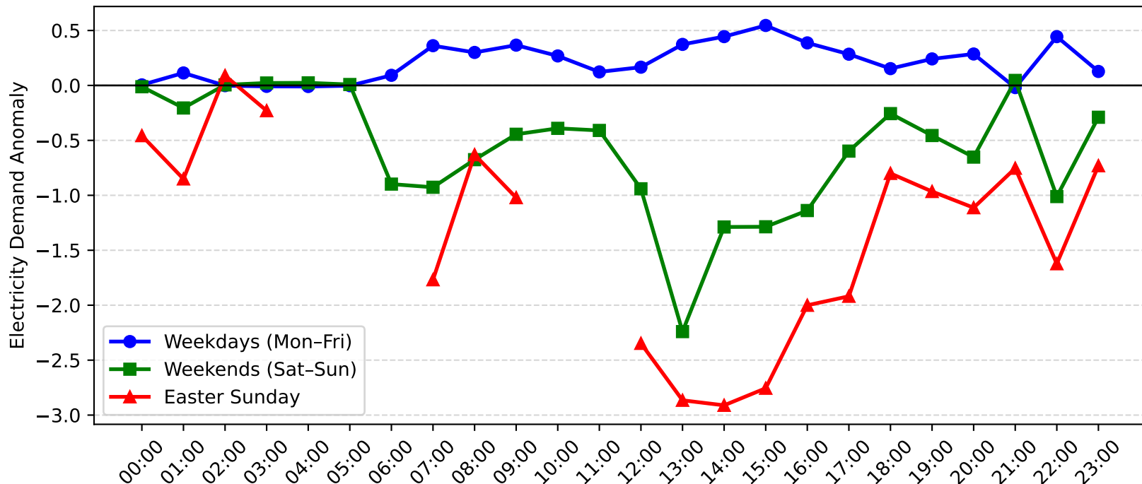
Adamstown Demand Anomaly: Easter Sunday vs Weekday/Weekend (2015-2016)
