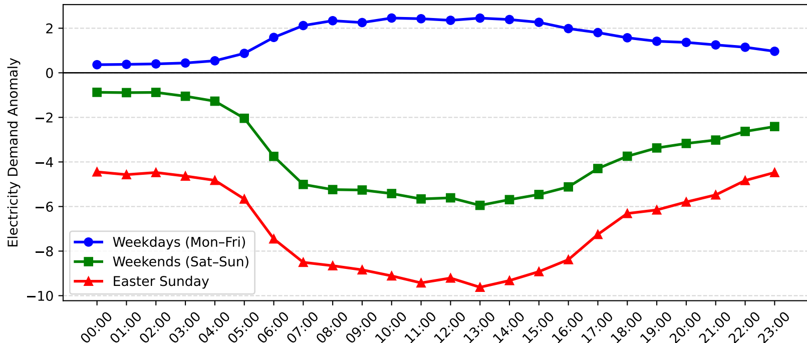
Leightonfield Demand Anomaly: Easter Sunday vs Weekday/Weekend (2005-2006)
