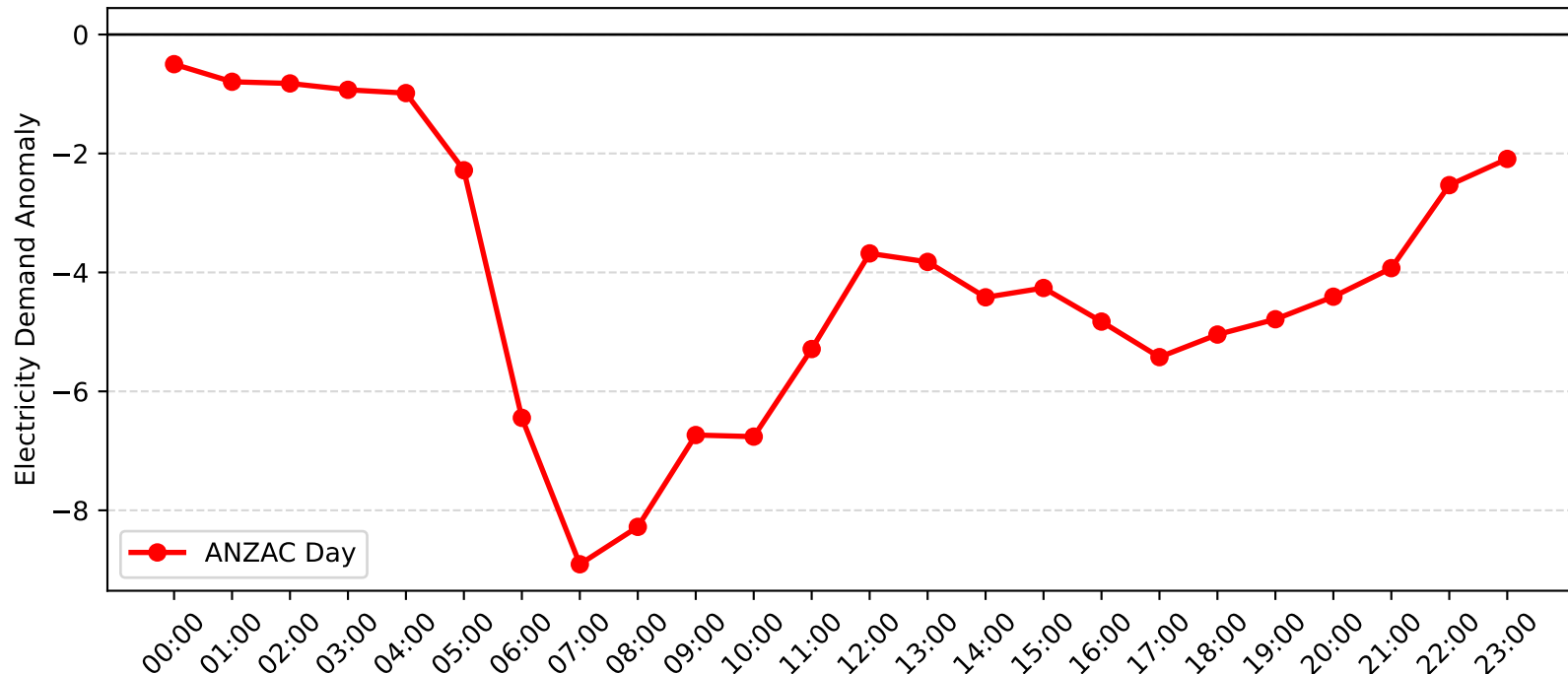
Epping Demand Anomaly: ANZAC Day (2008-2009)
