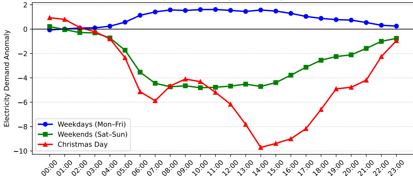
Sefton Demand Anomaly: Christmas Day vs Weekday/Weekend (2013-2014)
