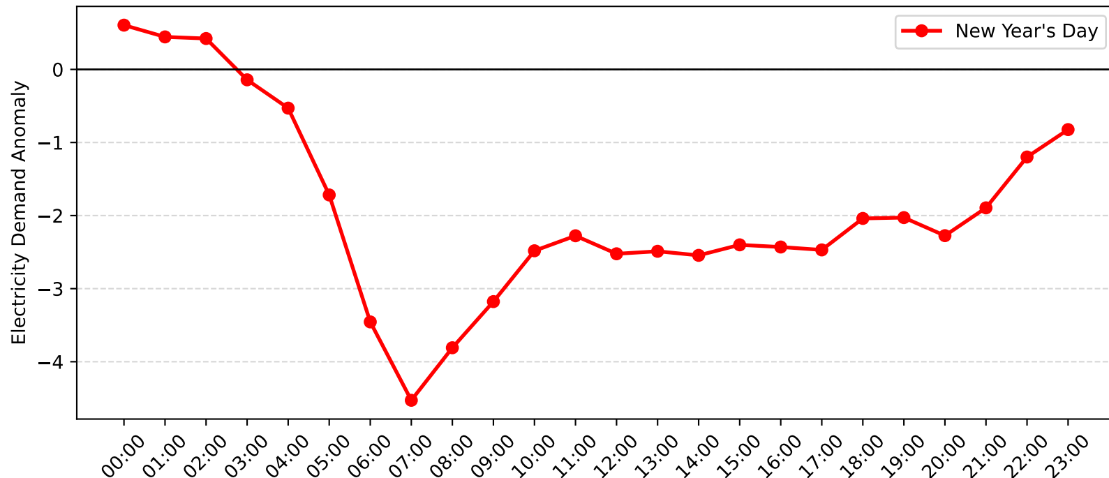
Dee Why West Demand Anomaly: New Year's Day (2014-2015)
