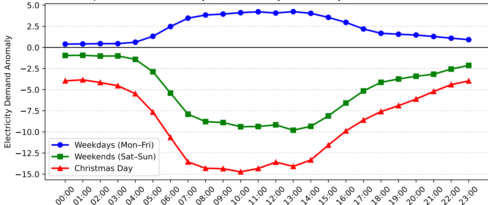
Milperra Demand Anomaly: Christmas Day vs Weekday/Weekend (2010-2011)
