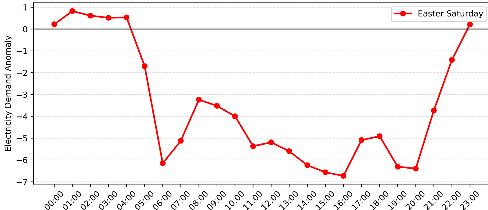
Pennant Hills Demand Anomaly: Easter Saturday (2005-2006)
