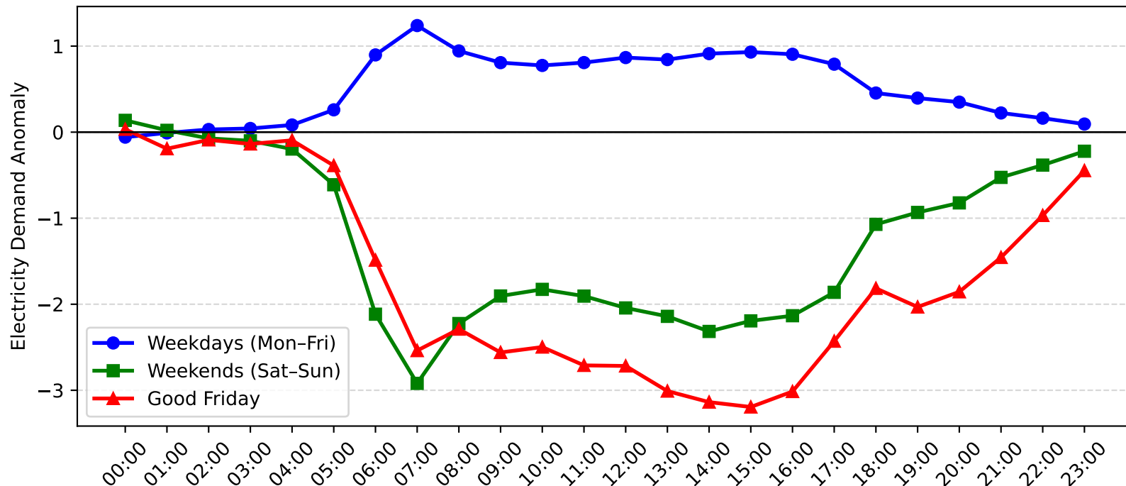
Pymble Demand Anomaly: Good Friday vs Weekday/Weekend (2017-2018)
