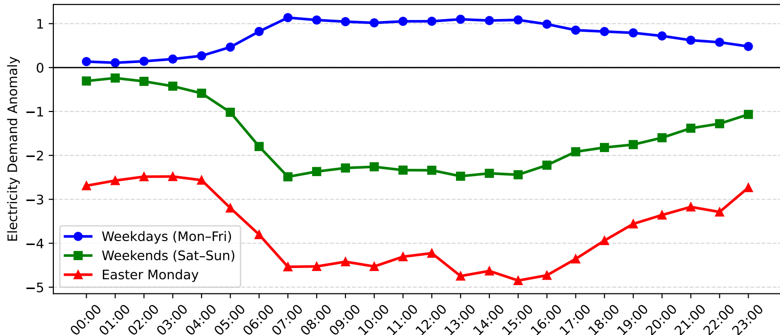
Bass Hill Demand Anomaly: Easter Monday vs Weekday/Weekend (2016-2017)
