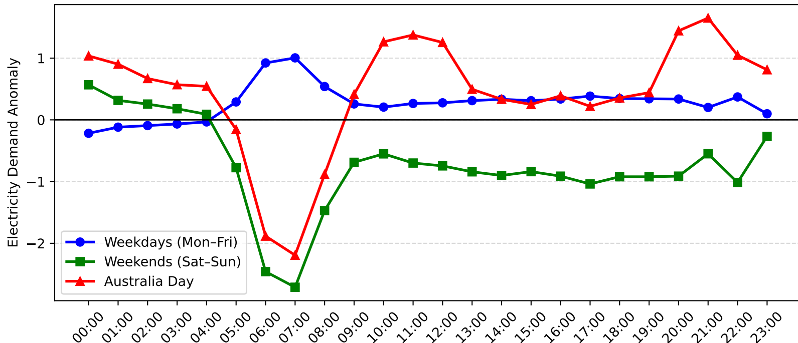
Dee Why West Demand Anomaly: Australia Day vs Weekday/Weekend (2011-2012)
