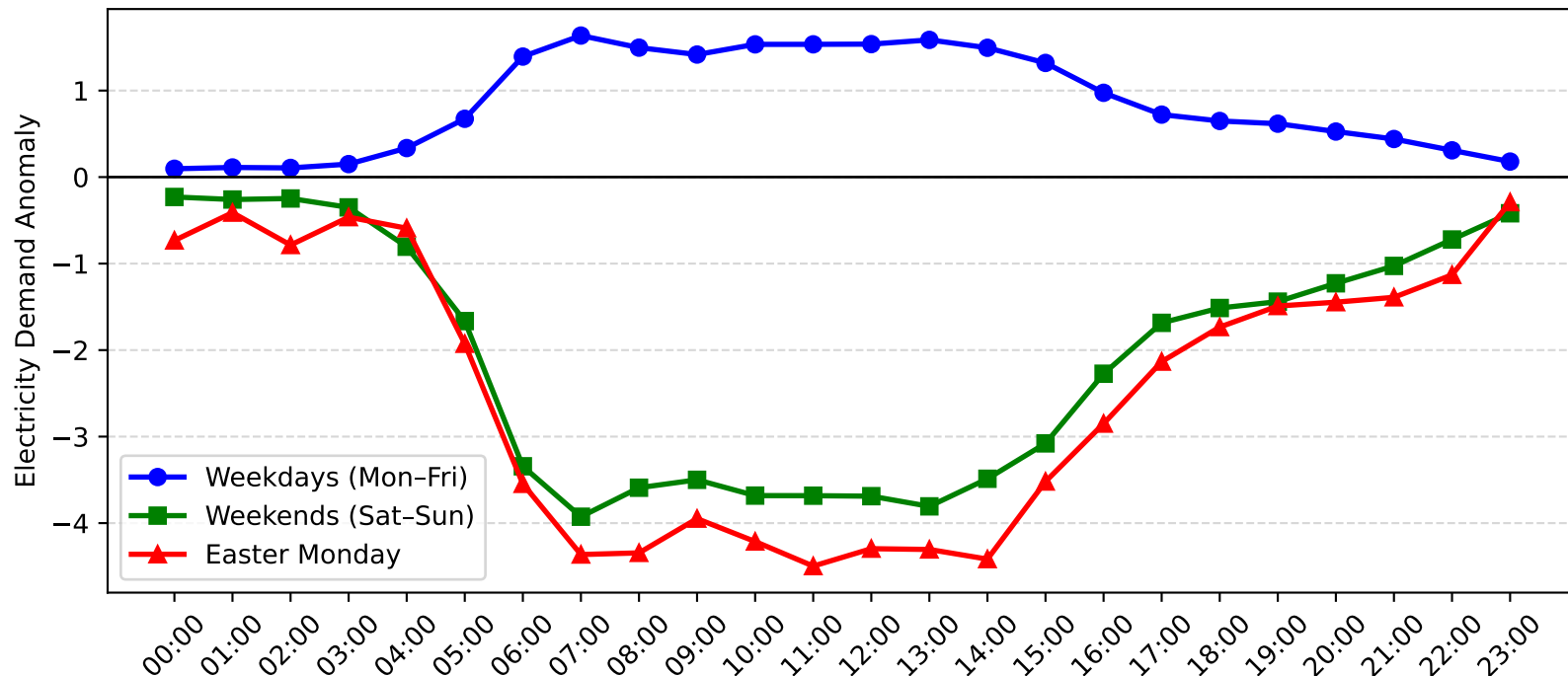
Wyong Demand Anomaly: Easter Monday vs Weekday/Weekend (2012-2013)
