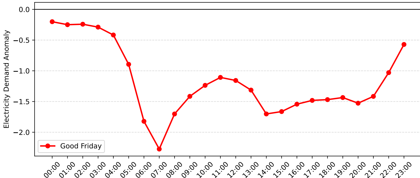
Arncliffe Demand Anomaly: Good Friday (2016-2017)
