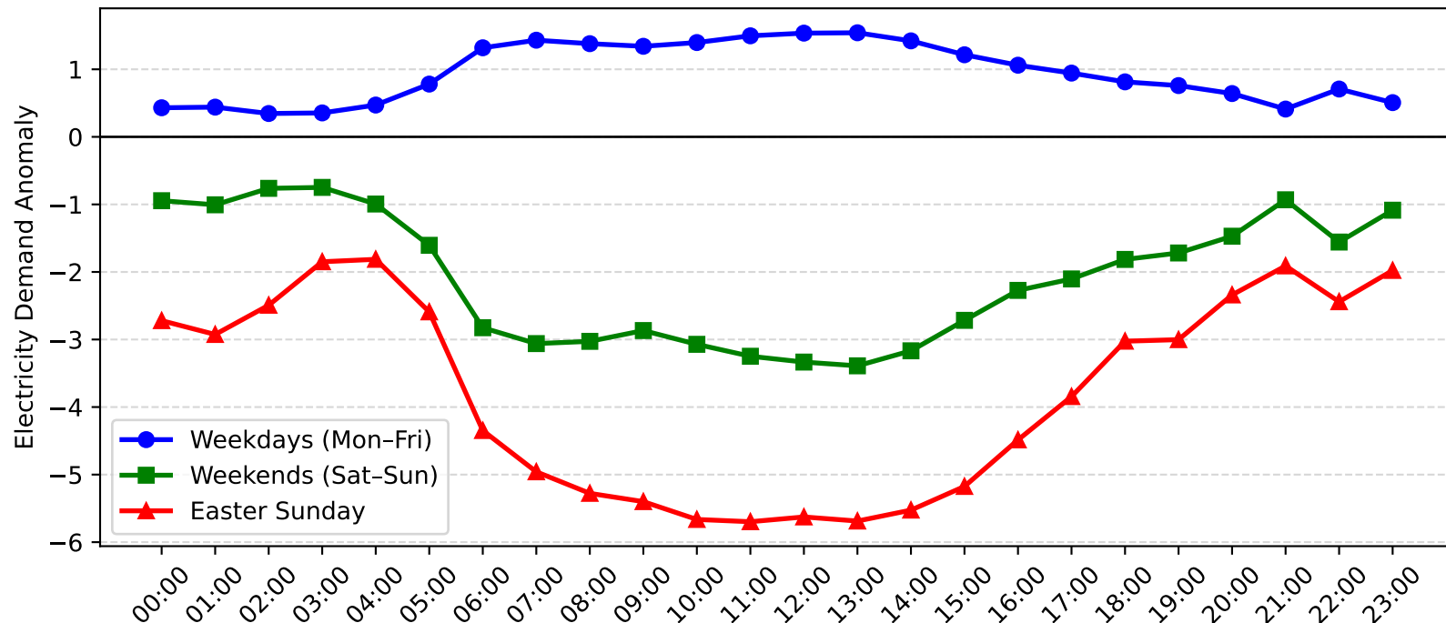
Argenton Demand Anomaly: Easter Sunday vs Weekday/Weekend (2010-2011)
