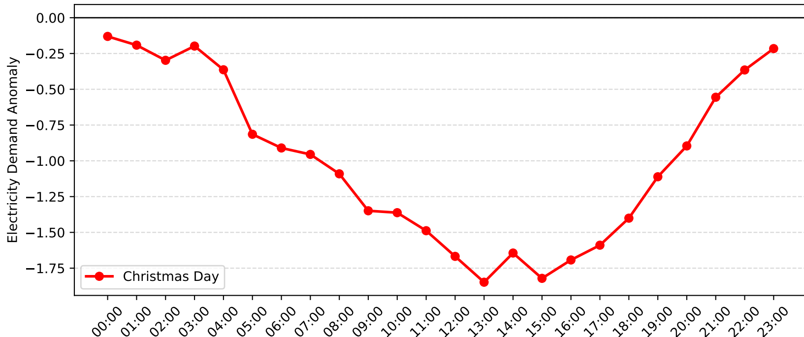
Narrabeen Demand Anomaly: Christmas Day (2009-2010)
