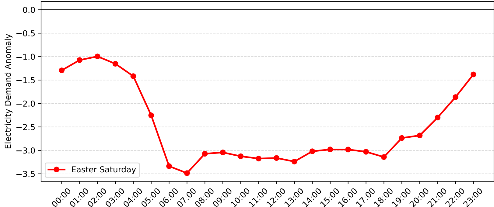
Lisarow Demand Anomaly: Easter Saturday (2012-2013)
