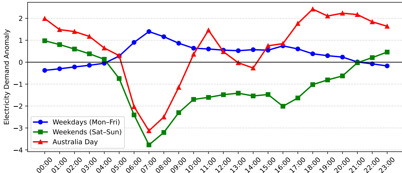
Punchbowl Demand Anomaly: Australia Day vs Weekday/Weekend (2011-2012)
