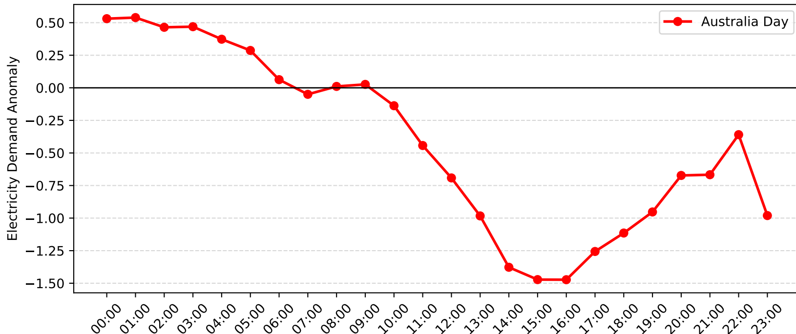
Telarah Demand Anomaly: Australia Day (2015-2016)
