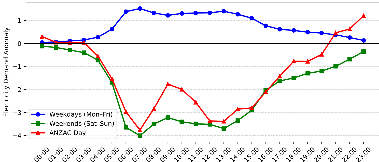
Wyong Demand Anomaly: ANZAC Day vs Weekday/Weekend (2013-2014)
