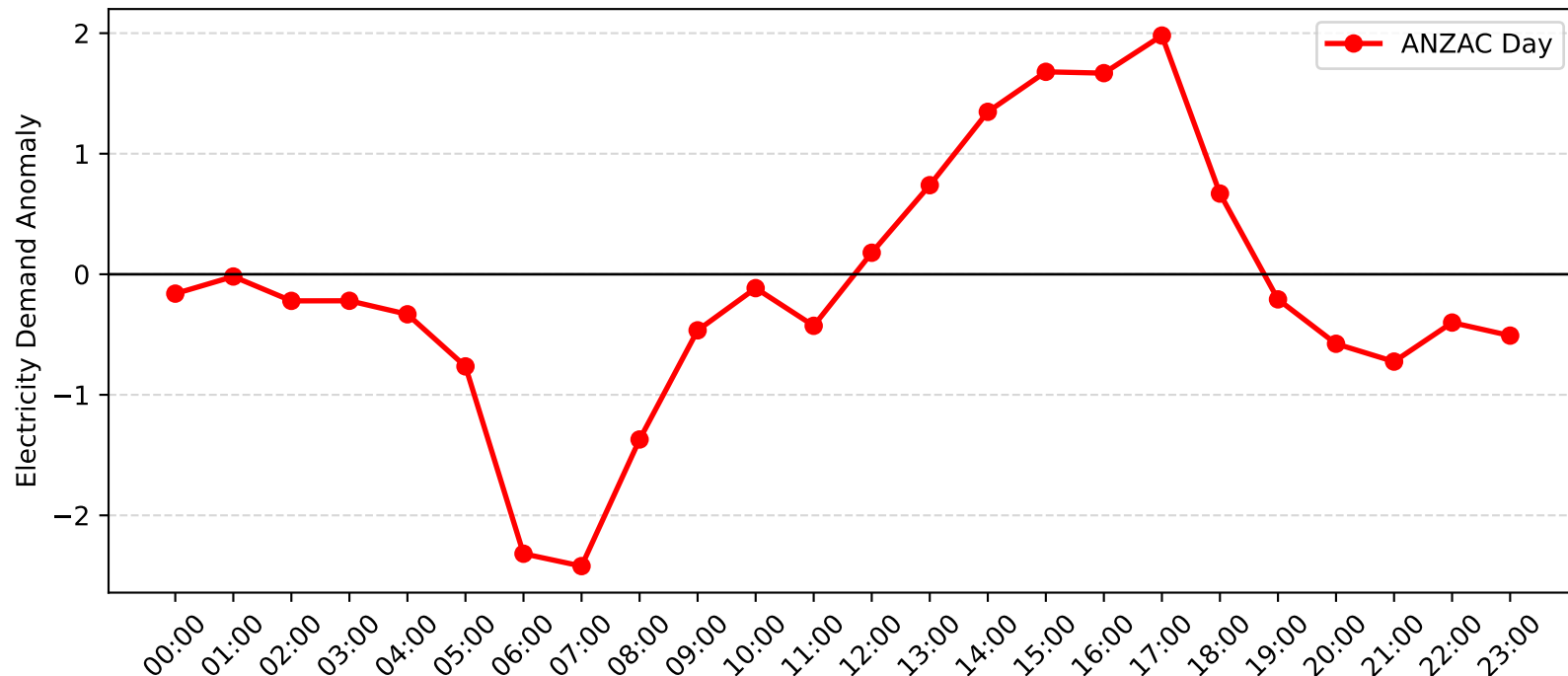
Balgowlah North Demand Anomaly: ANZAC Day (2017-2018)
