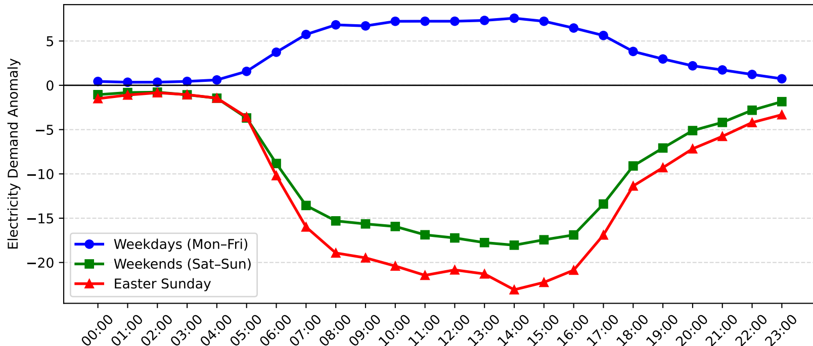
Gore Hill Demand Anomaly: Easter Sunday vs Weekday/Weekend (2005-2006)
