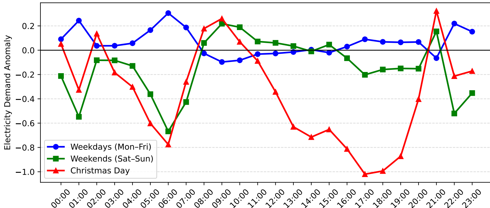
Morisset Demand Anomaly: Christmas Day vs Weekday/Weekend (2010-2011)
