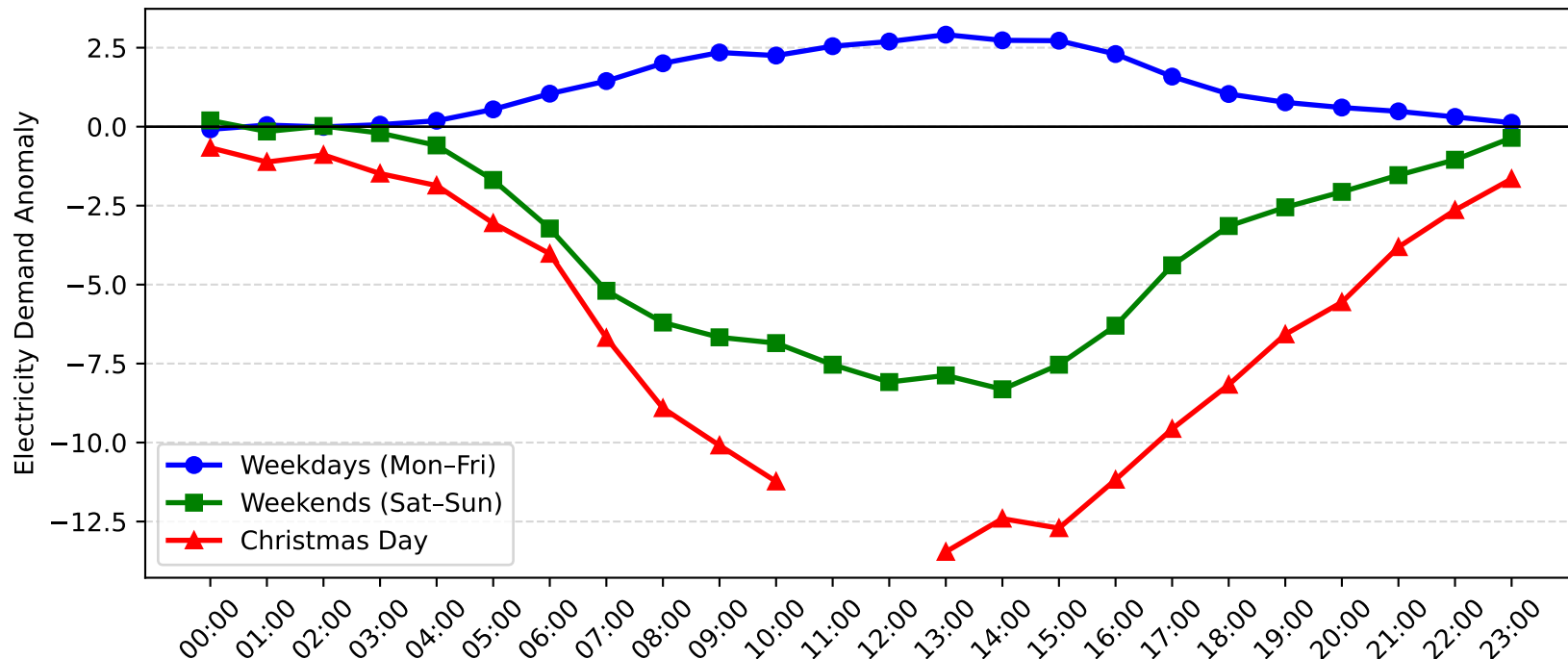
West Gosford Demand Anomaly: Christmas Day vs Weekday/Weekend (2008-2009)
