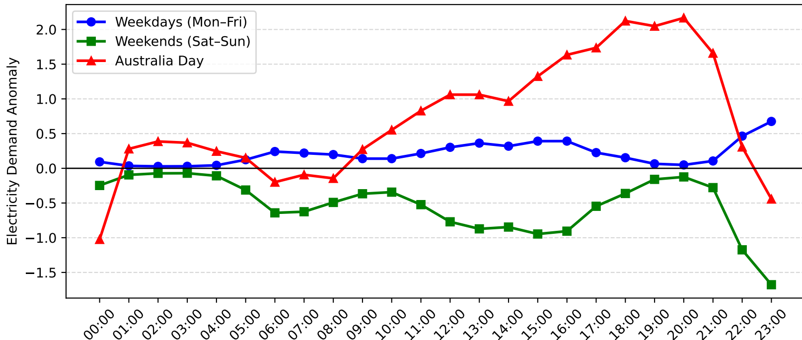
Muswellbrook Demand Anomaly: Australia Day vs Weekday/Weekend (2009-2010)
