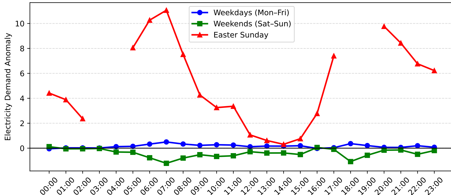
Revesby Demand Anomaly: Easter Sunday vs Weekday/Weekend (2004-2005)
