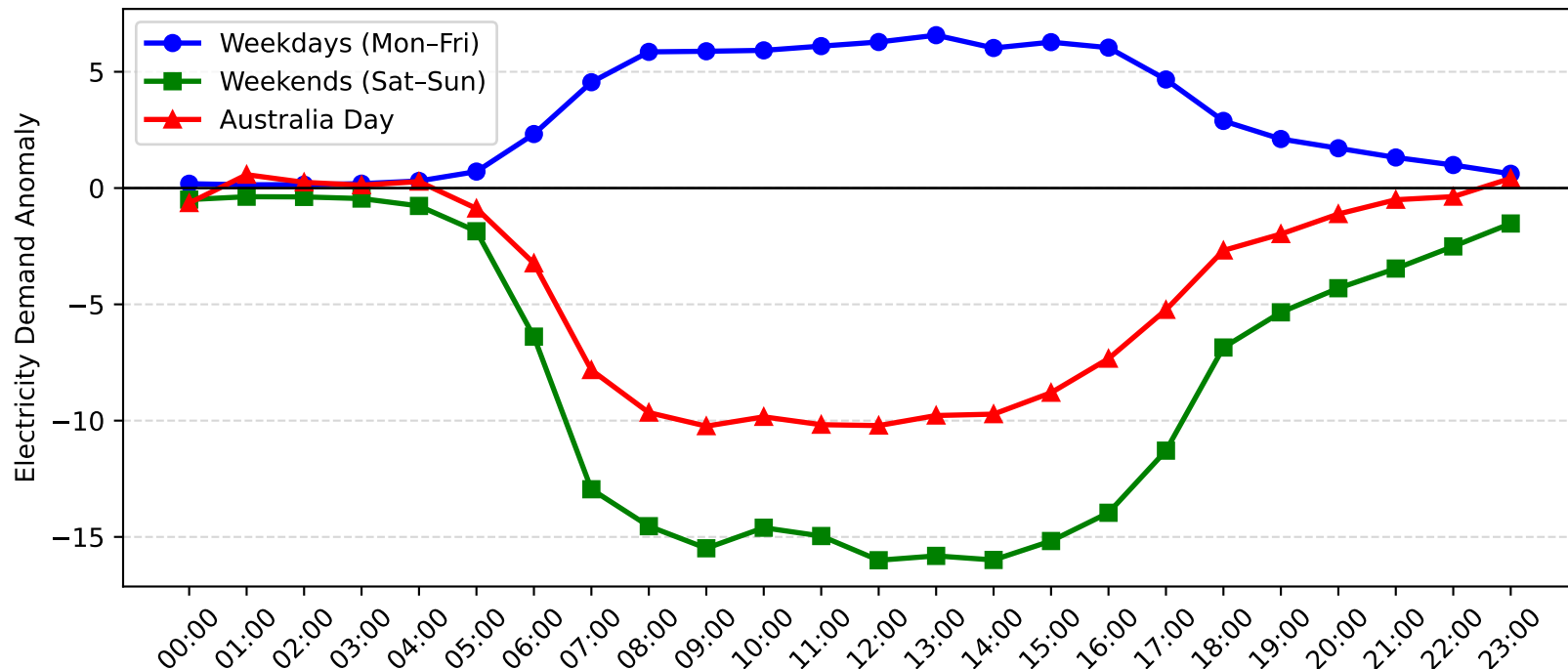
Gore Hill Demand Anomaly: Australia Day vs Weekday/Weekend (2009-2010)
