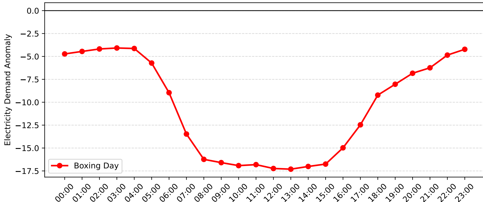
Gore Hill Demand Anomaly: Boxing Day (2006-2007)
