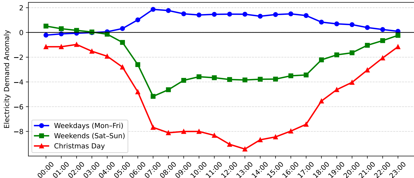
Chatswood Demand Anomaly: Christmas Day vs Weekday/Weekend (2009-2010)
