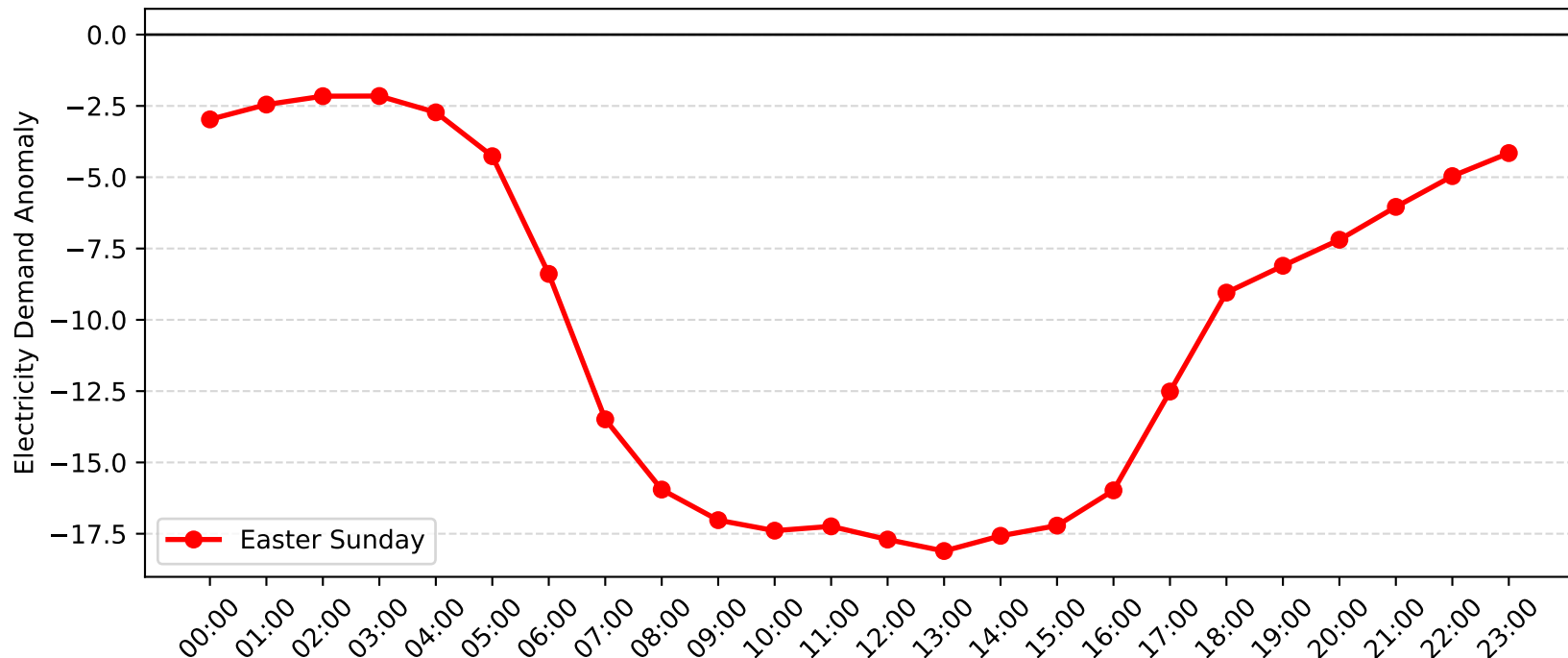
Gore Hill Demand Anomaly: Easter Sunday (2011-2012)
