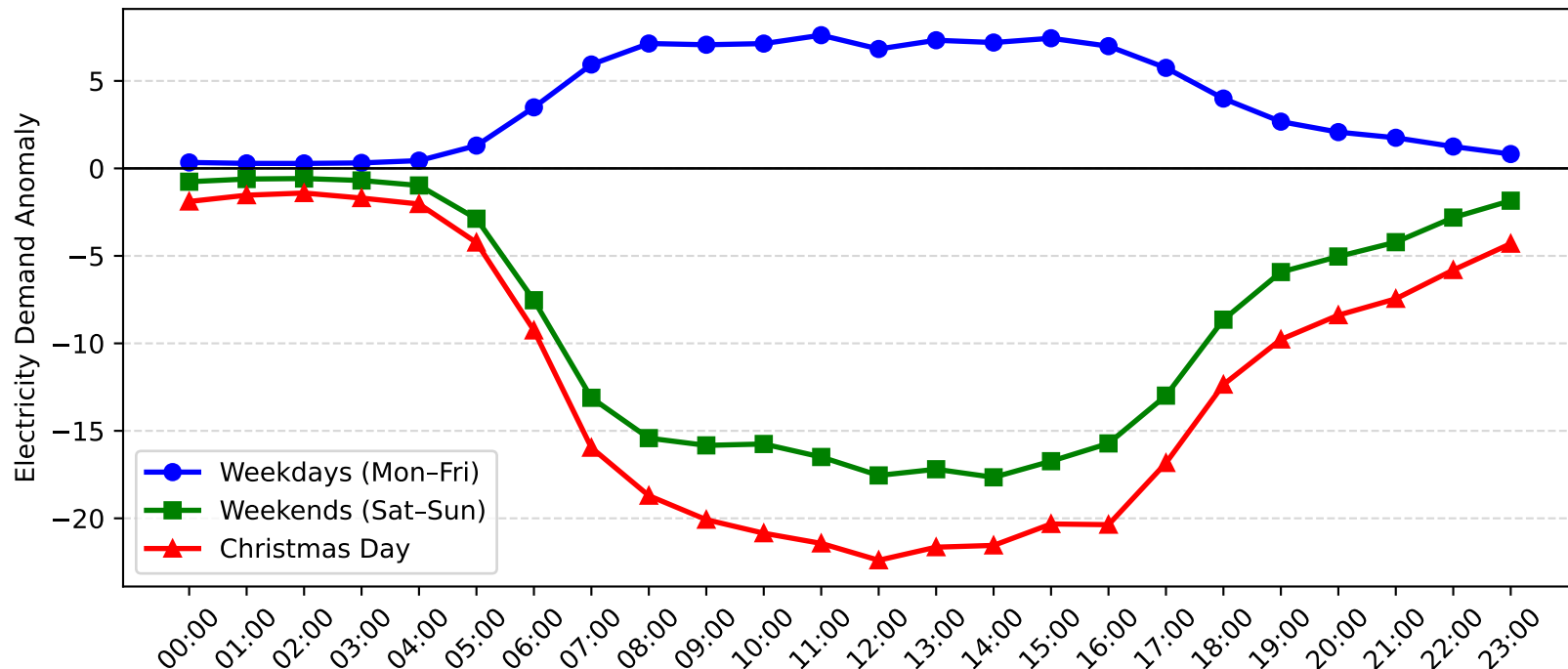
Gore Hill Demand Anomaly: Christmas Day vs Weekday/Weekend (2004-2005)
