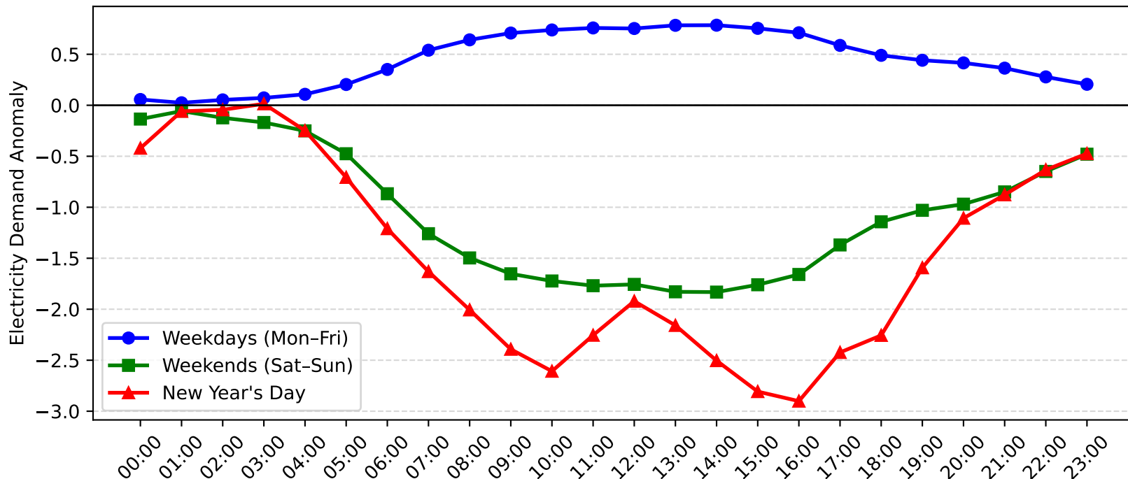
Lidcombe Demand Anomaly: New Year's Day vs Weekday/Weekend (2017-2018)
