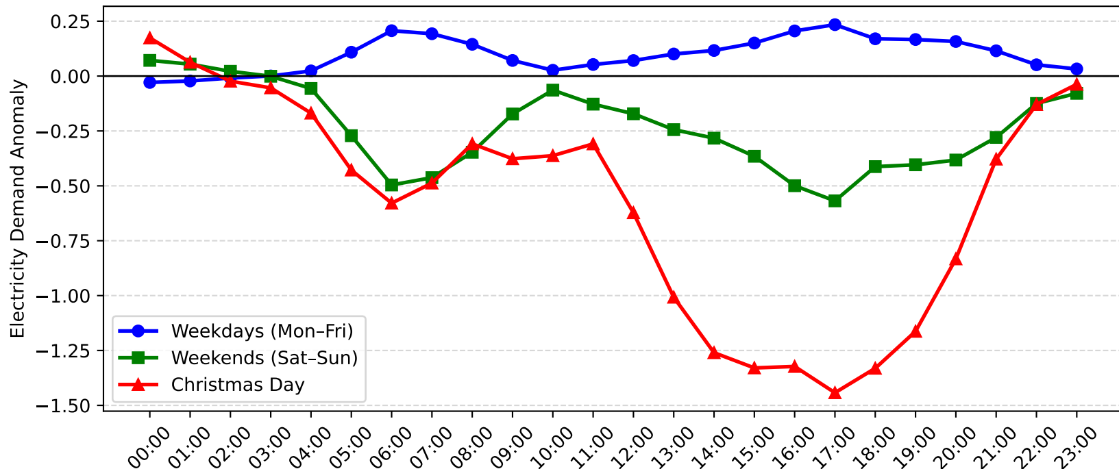
Narrabeen Demand Anomaly: Christmas Day vs Weekday/Weekend (2015-2016)
