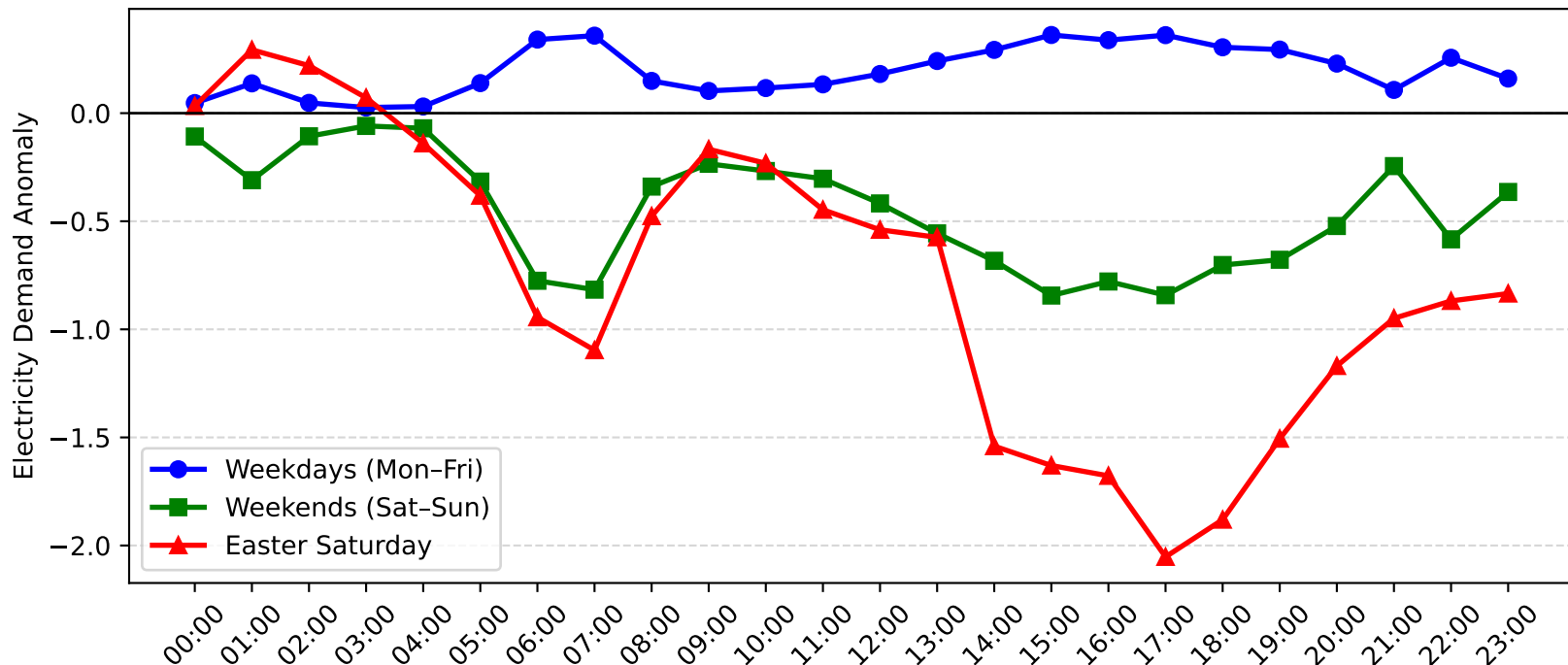
Maryland Demand Anomaly: Easter Saturday vs Weekday/Weekend (2015-2016)
