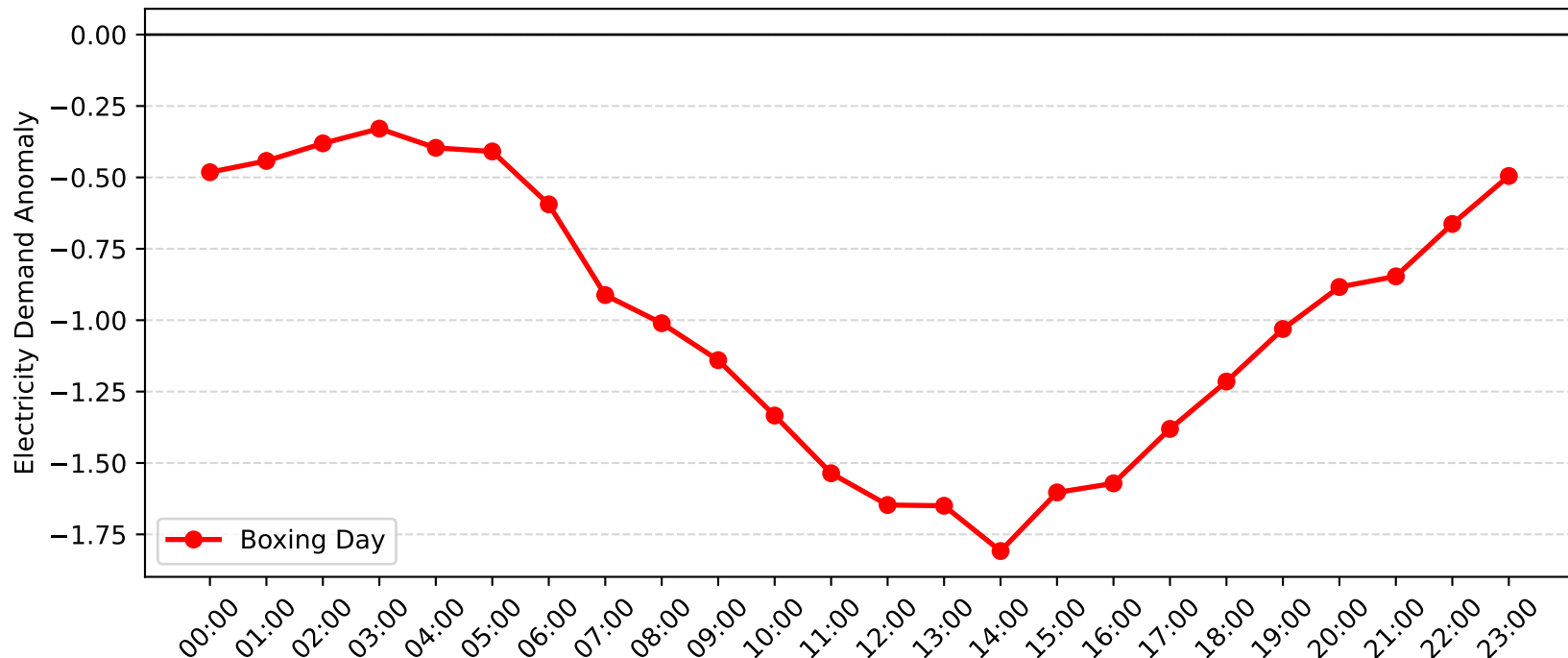
Rothbury Demand Anomaly: Boxing Day (2011-2012)
