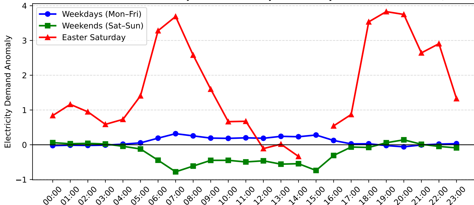
Arncliffe Demand Anomaly: Easter Saturday vs Weekday/Weekend (2004-2005)
