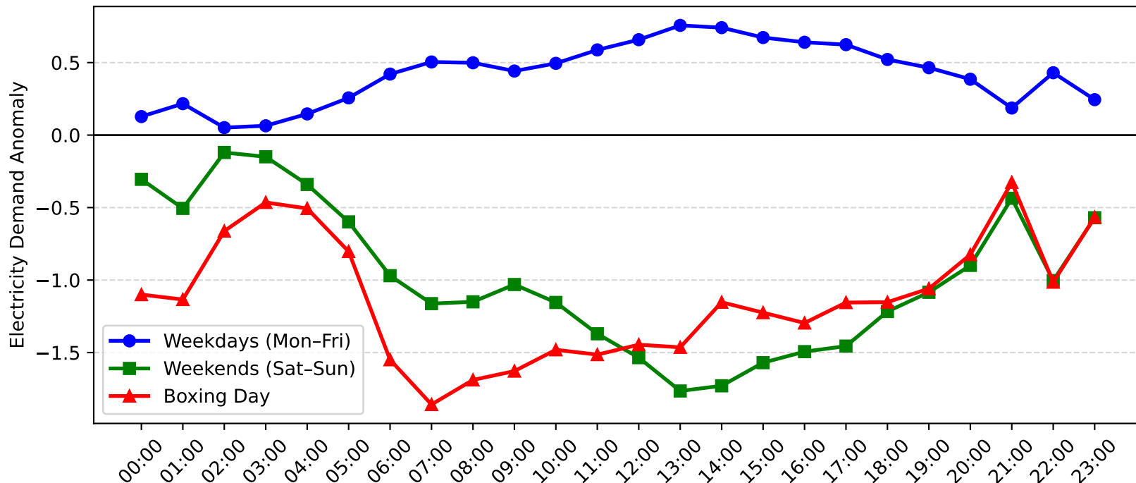
Gateshead Demand Anomaly: Boxing Day vs Weekday/Weekend (2015-2016)
