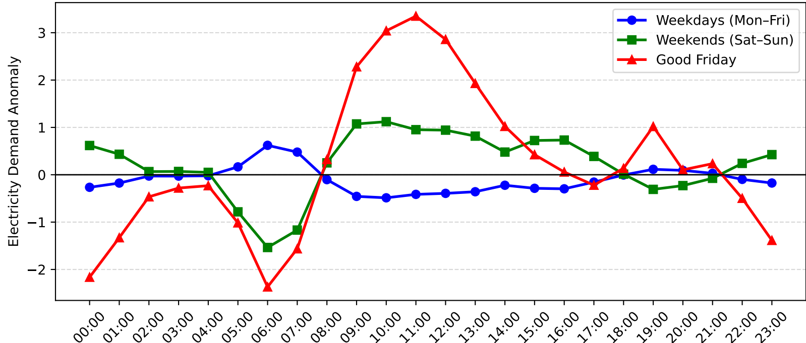
Avoca Demand Anomaly: Good Friday vs Weekday/Weekend (2015-2016)
