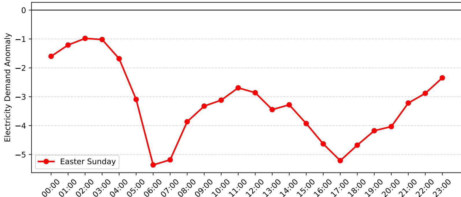
Revesby Demand Anomaly: Easter Sunday (2008-2009)
