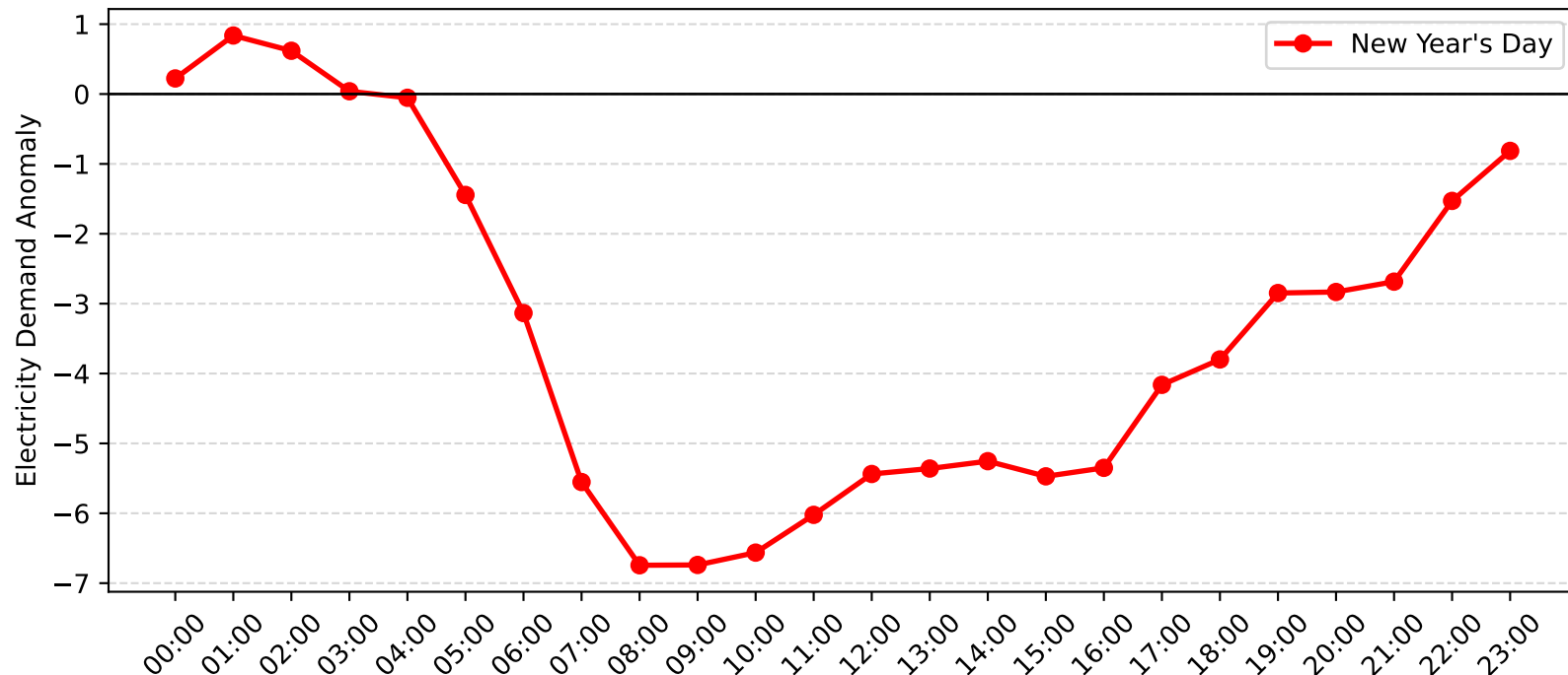
Maroubra Demand Anomaly: New Year's Day (2017-2018)
