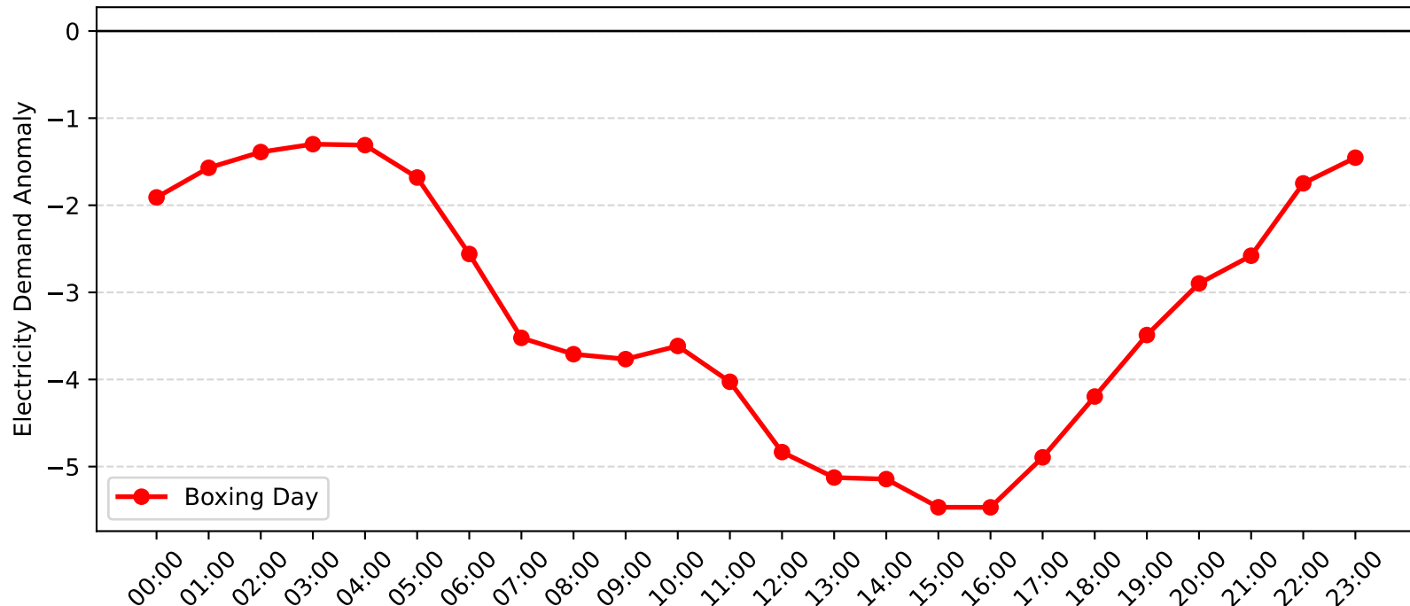
Jesmond Demand Anomaly: Boxing Day (2011-2012)
