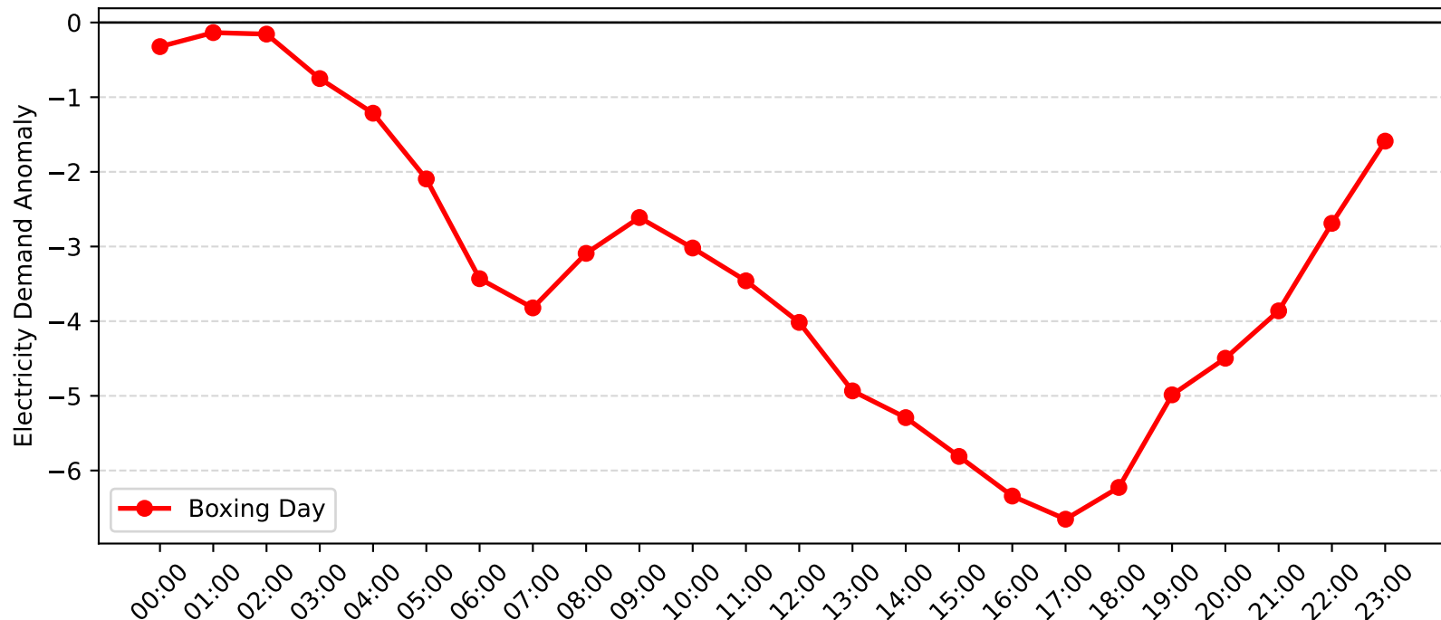
Revesby Demand Anomaly: Boxing Day (2012-2013)
