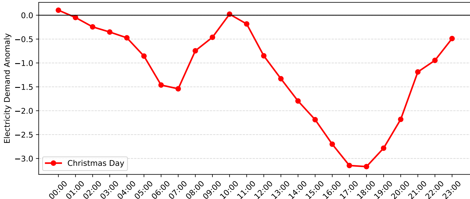
Balgowlah North Demand Anomaly: Christmas Day (2016-2017)
