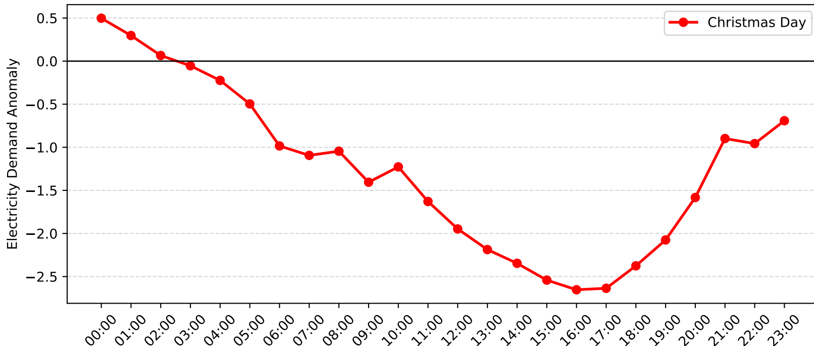
Narrabeen Demand Anomaly: Christmas Day (2004-2005)
