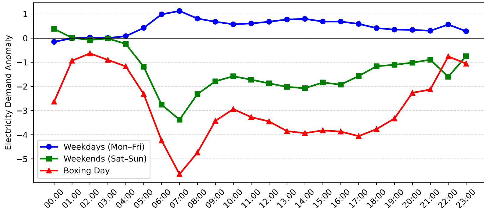
Dee Why West Demand Anomaly: Boxing Day vs Weekday/Weekend (2007-2008)
