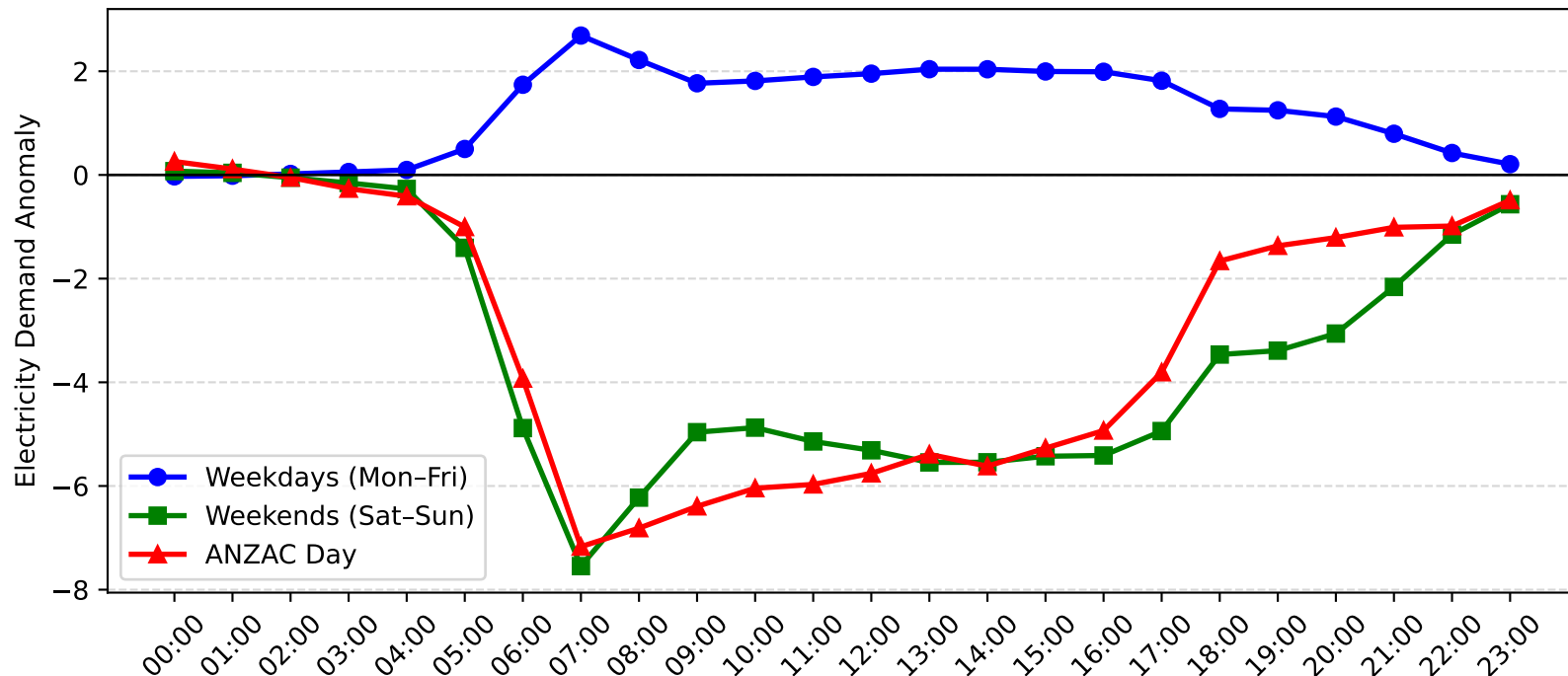
Epping Demand Anomaly: ANZAC Day vs Weekday/Weekend (2012-2013)
