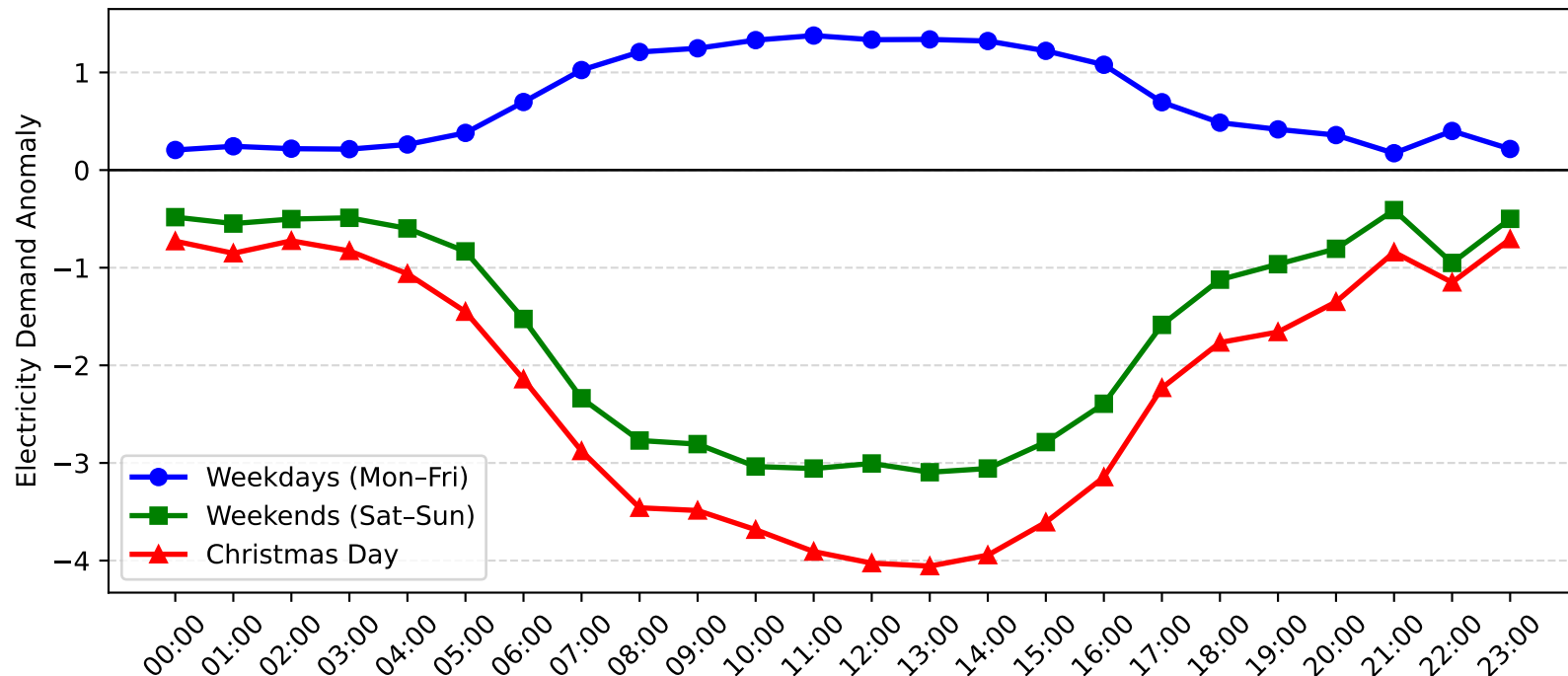
Mayfield West Demand Anomaly: Christmas Day vs Weekday/Weekend (2010-2011)
