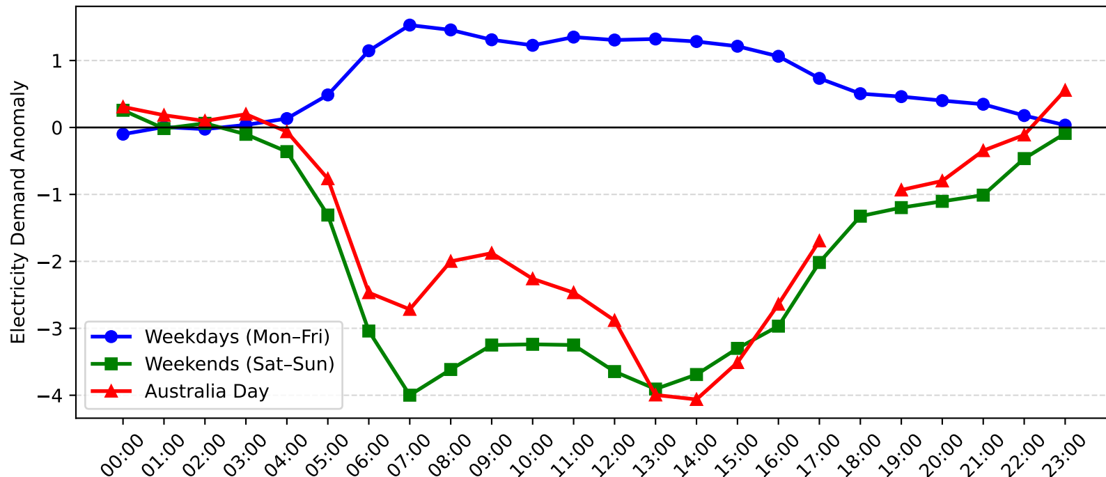
Kirrawee Demand Anomaly: Australia Day vs Weekday/Weekend (2005-2006)
