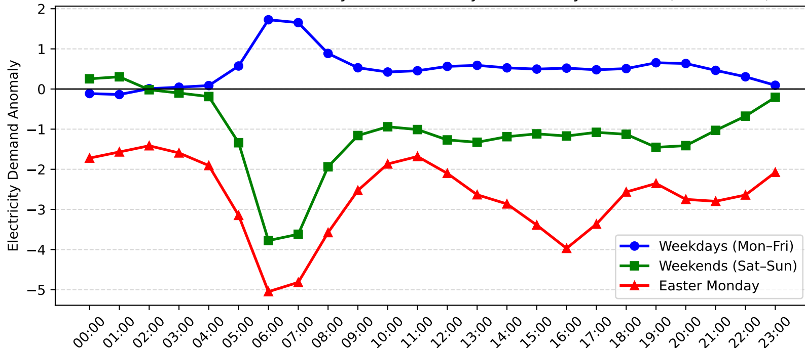
Pennant Hills Demand Anomaly: Easter Monday vs Weekday/Weekend (2016-2017)
