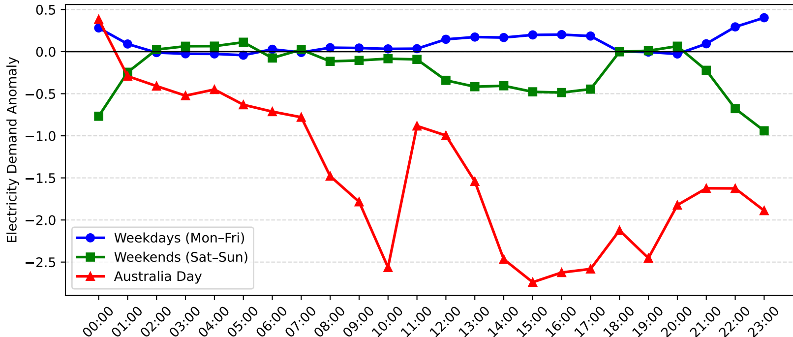
Muswellbrook Demand Anomaly: Australia Day vs Weekday/Weekend (2004-2005)
