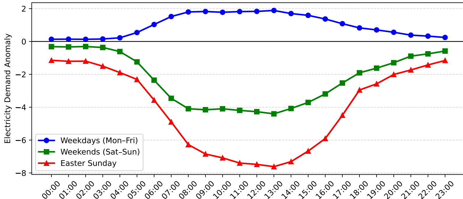
Auburn Demand Anomaly: Easter Sunday vs Weekday/Weekend (2015-2016)
