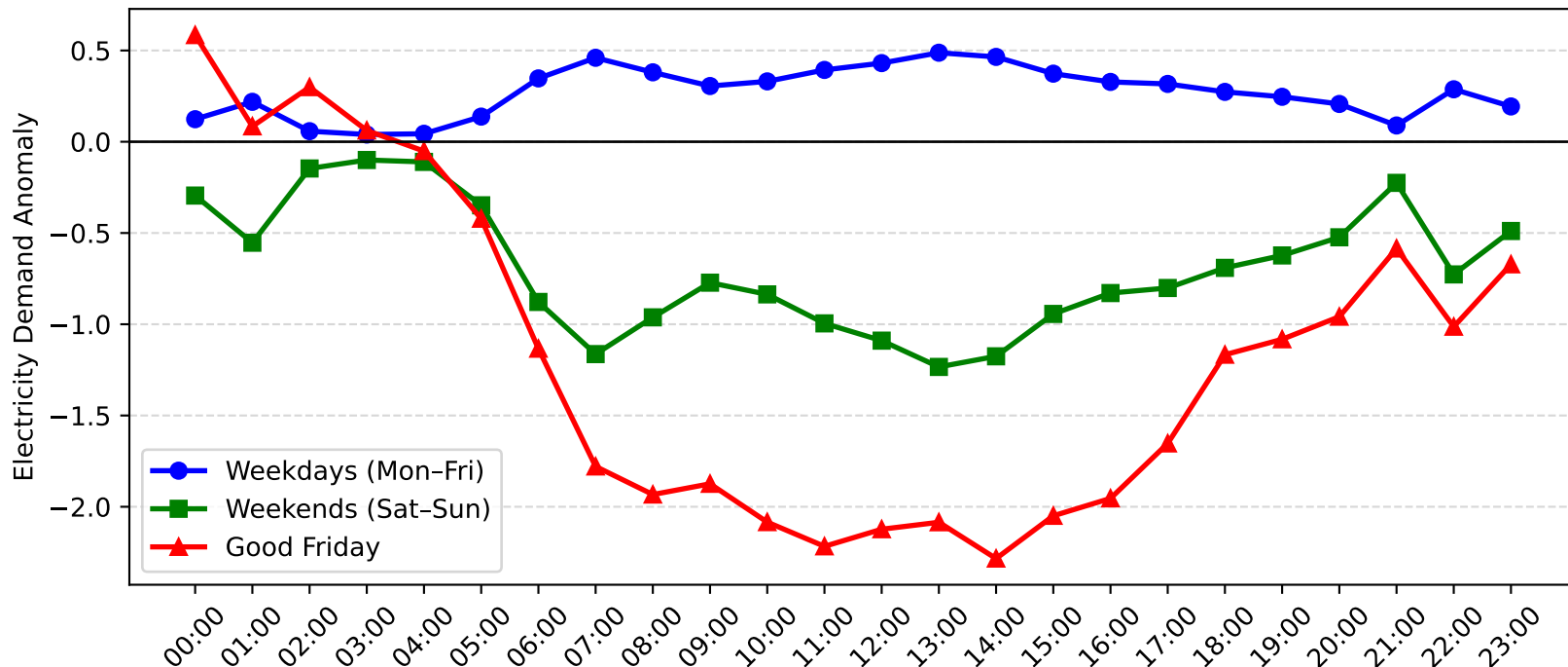
Gateshead Demand Anomaly: Good Friday vs Weekday/Weekend (2012-2013)
