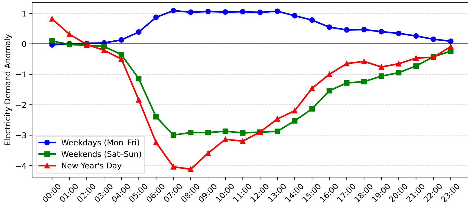
Wyong Demand Anomaly: New Year's Day vs Weekday/Weekend (2013-2014)
