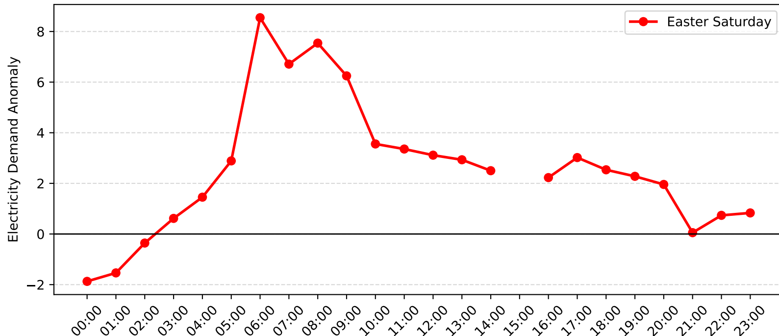
Gore Hill Demand Anomaly: Easter Saturday (2004-2005)
