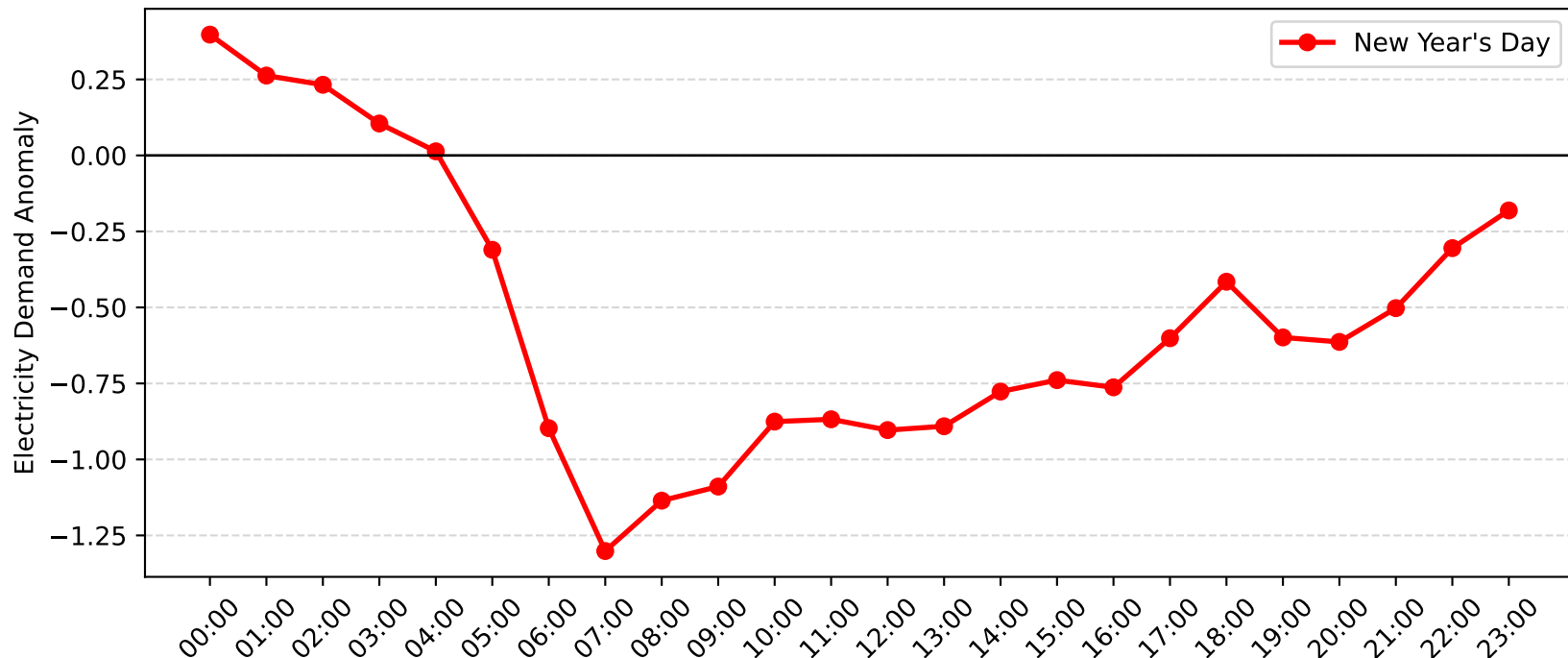
Narrabeen Demand Anomaly: New Year's Day (2013-2014)
