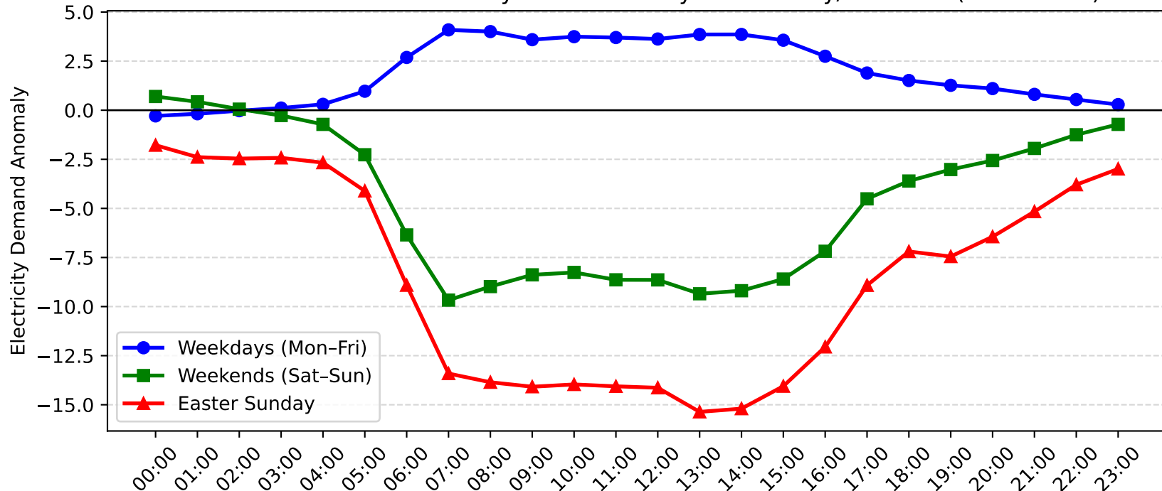
Marrickville Demand Anomaly: Easter Sunday vs Weekday/Weekend (2005-2006)
