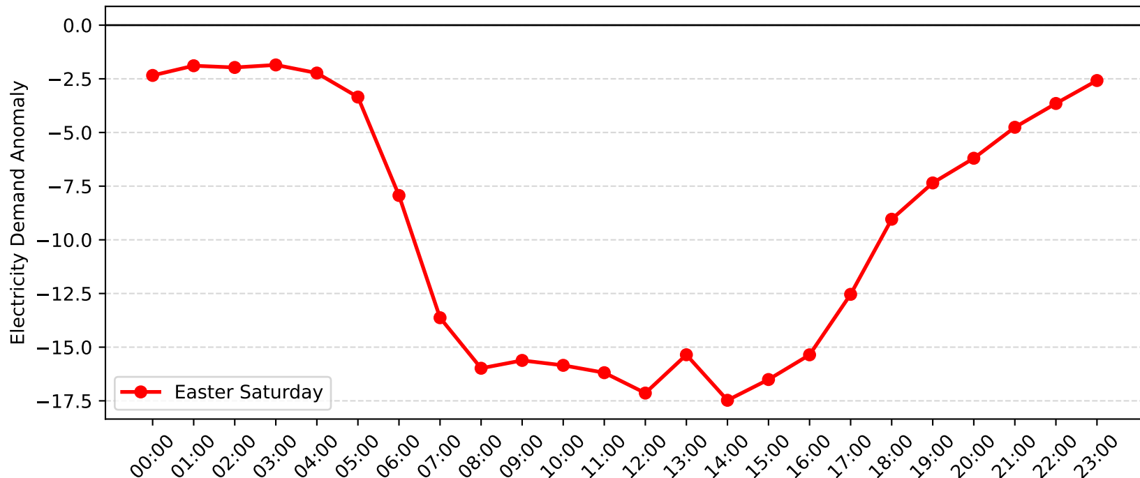
Gore Hill Demand Anomaly: Easter Saturday (2009-2010)
