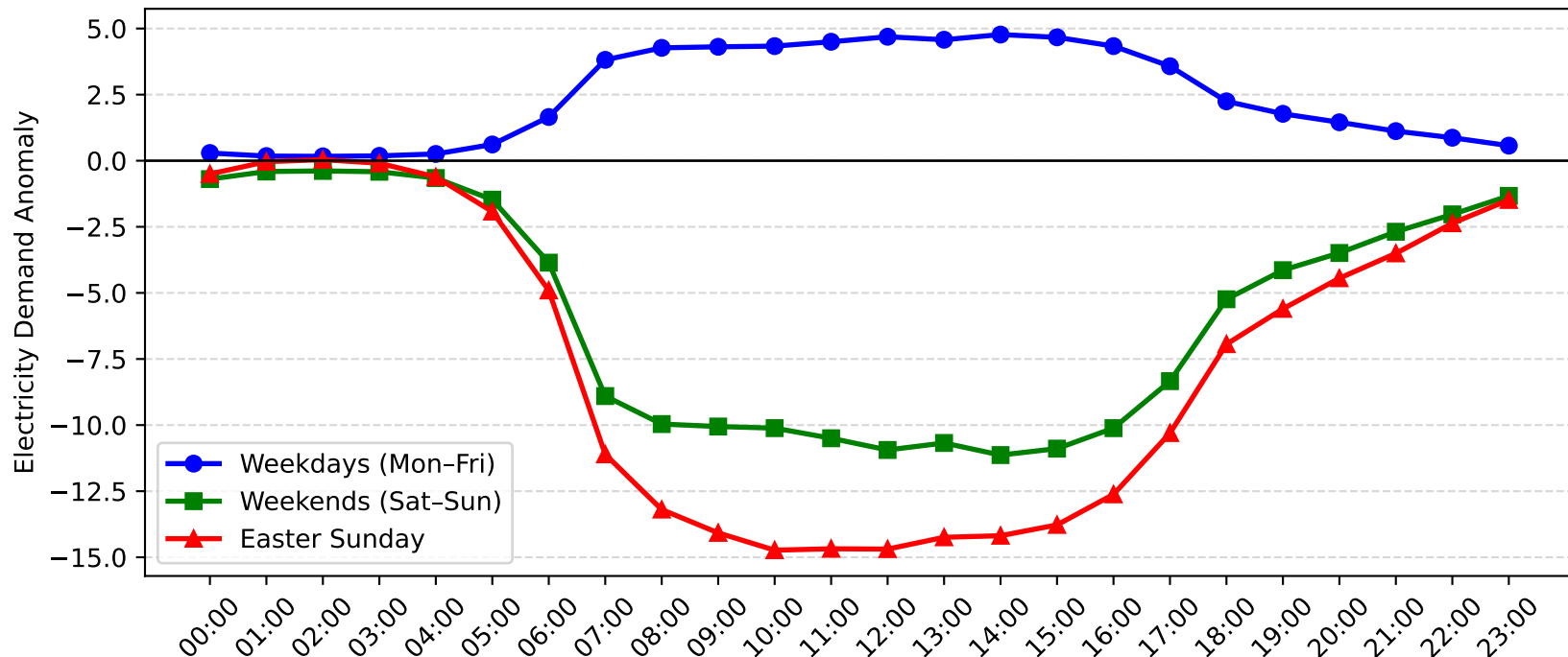
Gore Hill Demand Anomaly: Easter Sunday vs Weekday/Weekend (2013-2014)
