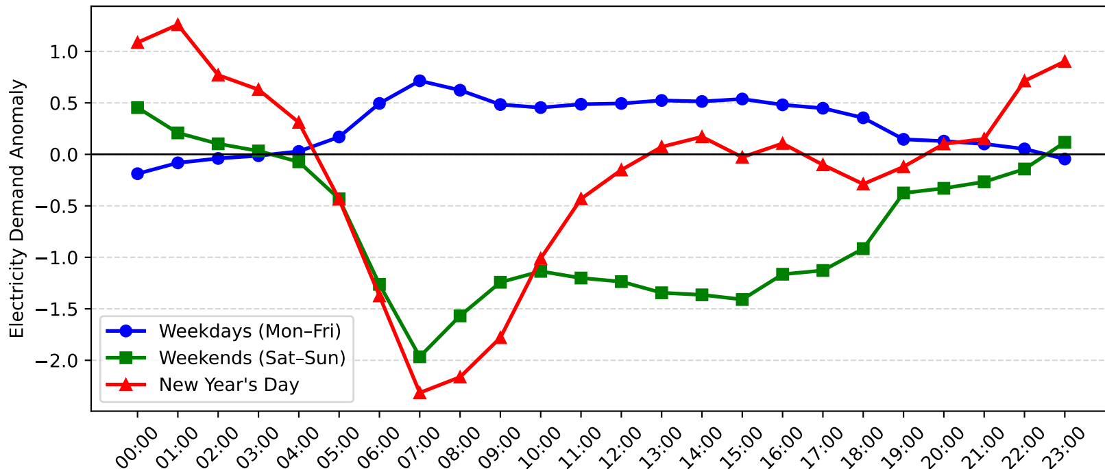
Blakehurst Demand Anomaly: New Year's Day vs Weekday/Weekend (2010-2011)
