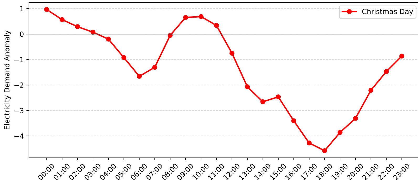
Dee Why West Demand Anomaly: Christmas Day (2011-2012)
