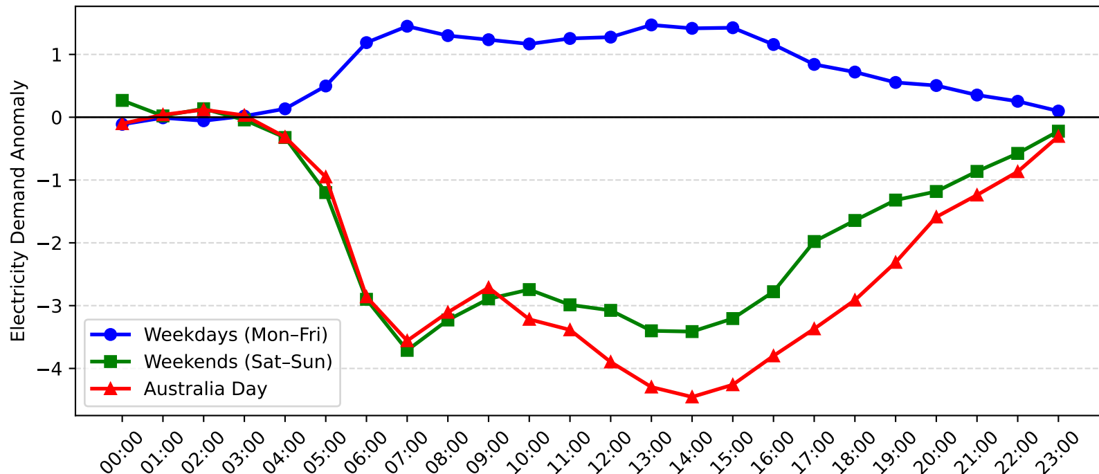
Kirrawee Demand Anomaly: Australia Day vs Weekday/Weekend (2008-2009)
