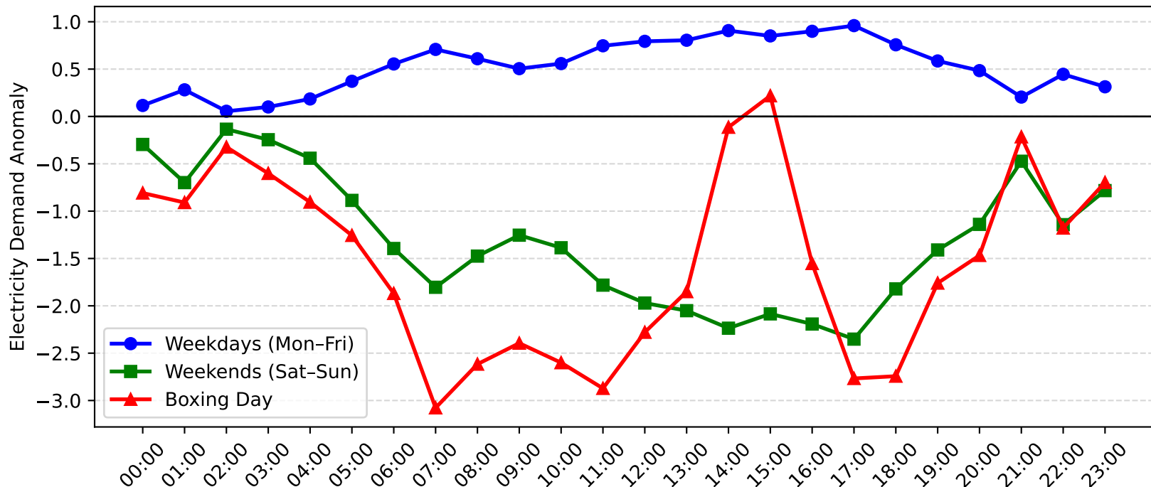
Jesmond Demand Anomaly: Boxing Day vs Weekday/Weekend (2014-2015)
