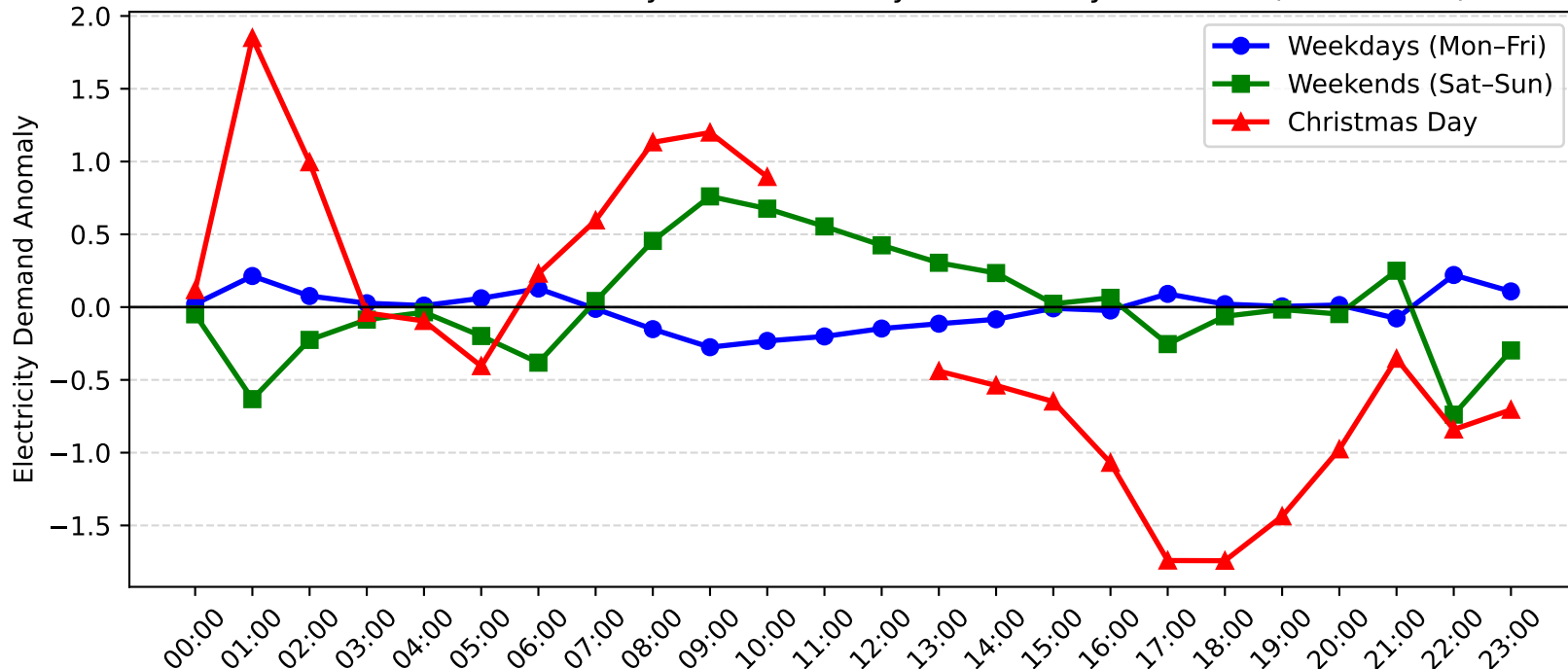
Swansea Demand Anomaly: Christmas Day vs Weekday/Weekend (2008-2009)
