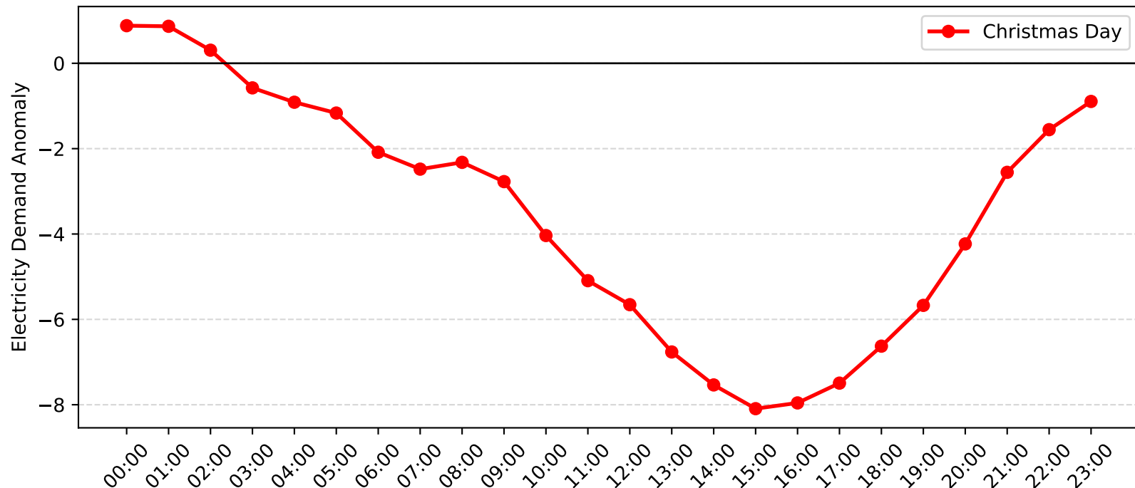
Jesmond Demand Anomaly: Christmas Day (2014-2015)
