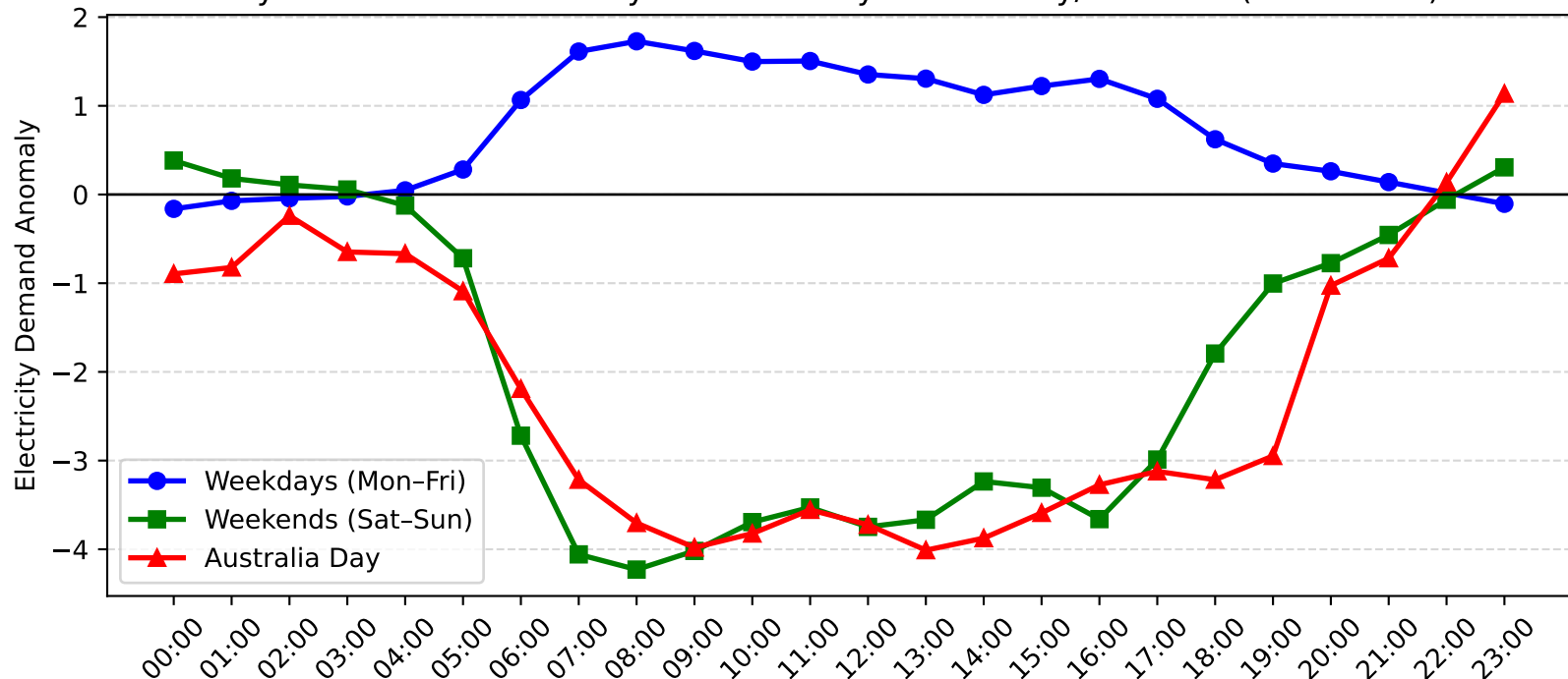
Pymble Demand Anomaly: Australia Day vs Weekday/Weekend (2006-2007)
