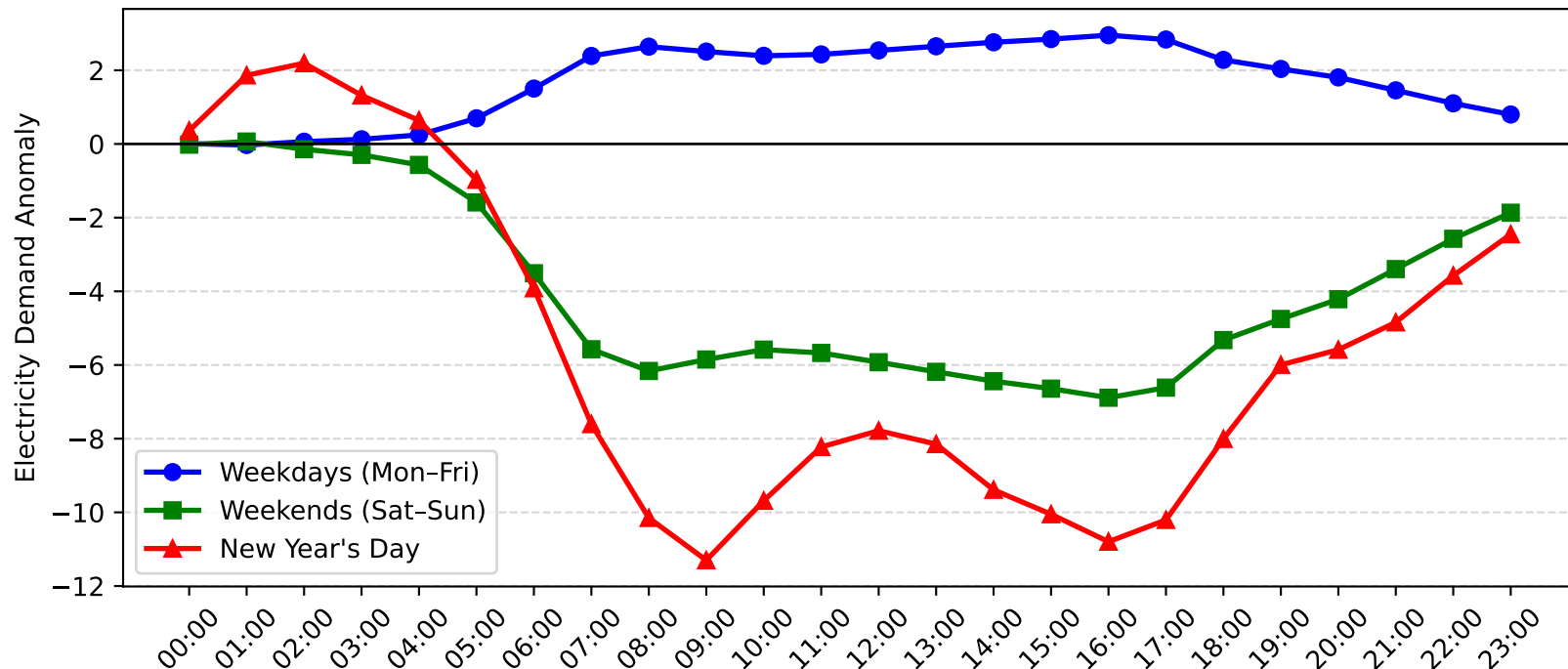
Burwood Demand Anomaly: New Year's Day vs Weekday/Weekend (2017-2018)
