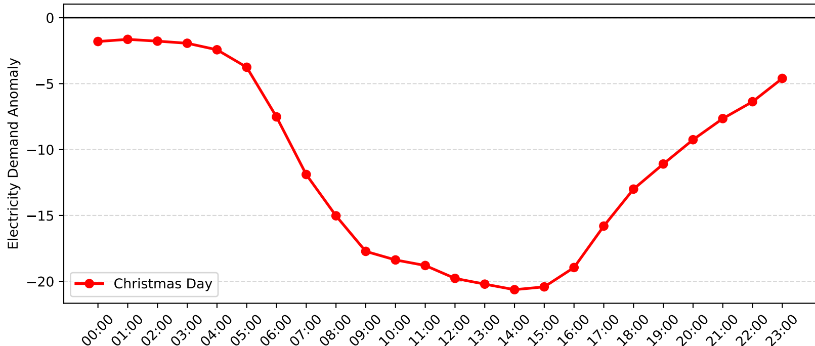
Zetland Demand Anomaly: Christmas Day (2006-2007)
