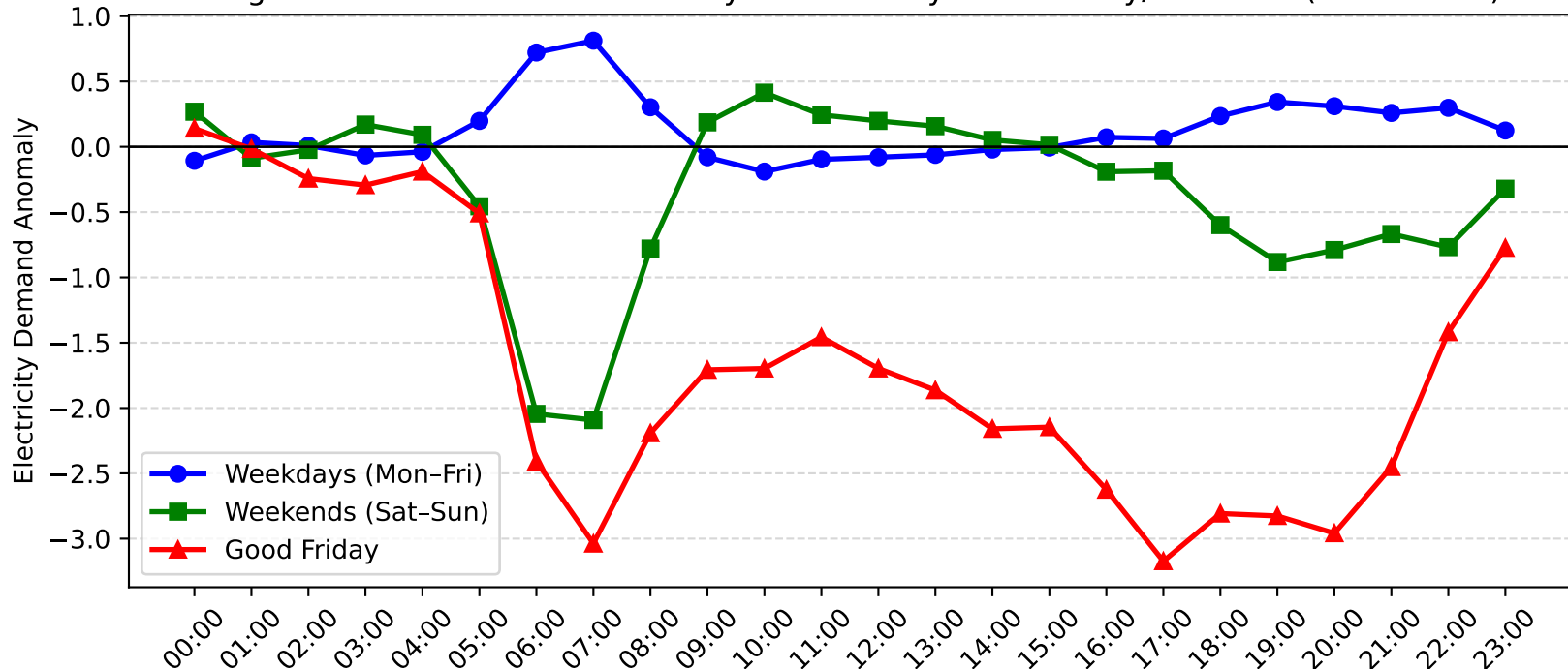
Balgowlah North Demand Anomaly: Good Friday vs Weekday/Weekend (2012-2013)
