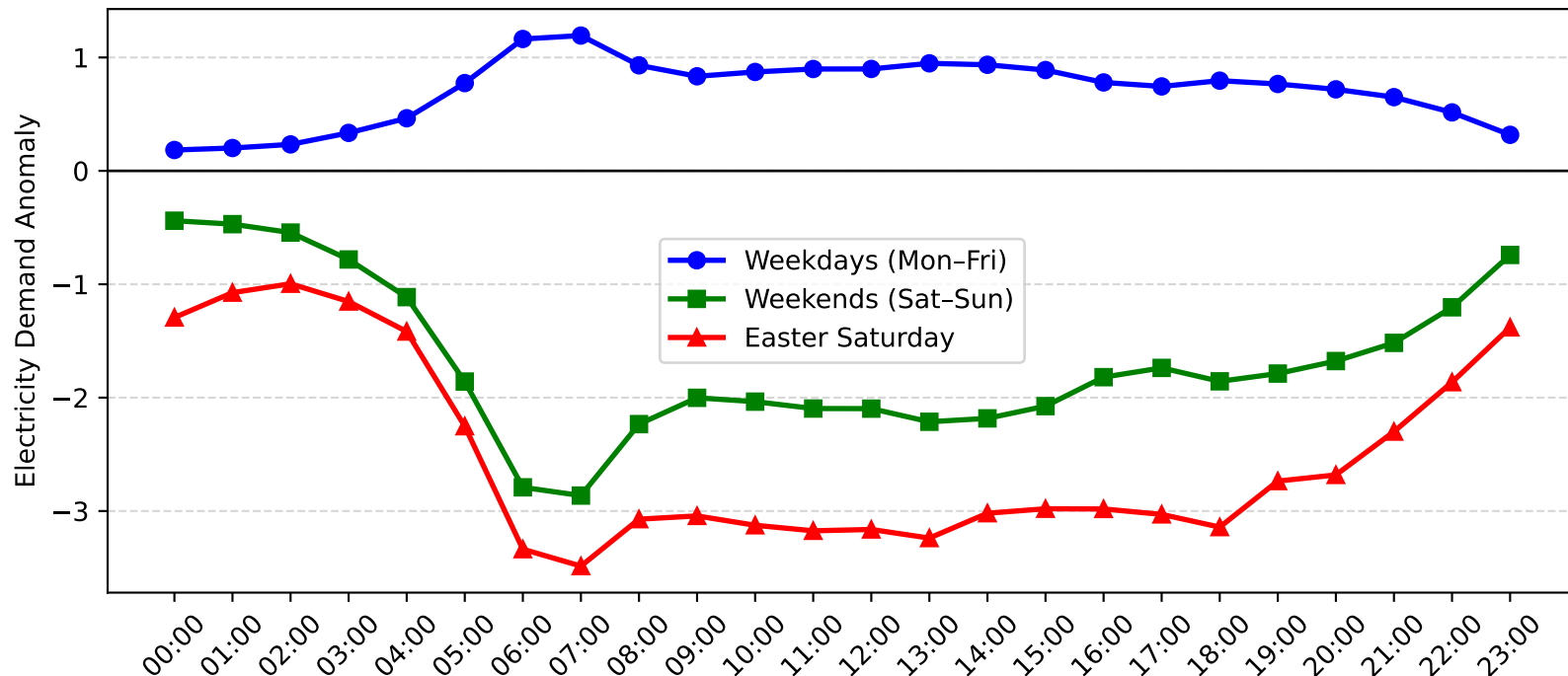
Lisarow Demand Anomaly: Easter Saturday vs Weekday/Weekend (2012-2013)
