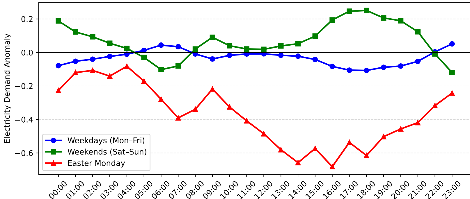
Rothbury Demand Anomaly: Easter Monday vs Weekday/Weekend (2013-2014)
