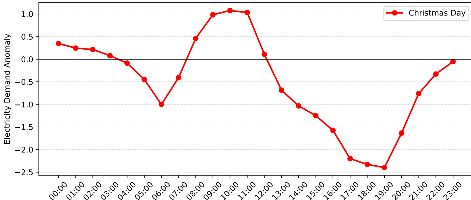
Harbord Demand Anomaly: Christmas Day (2014-2015)
