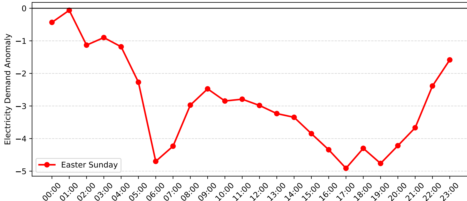
Revesby Demand Anomaly: Easter Sunday (2014-2015)
