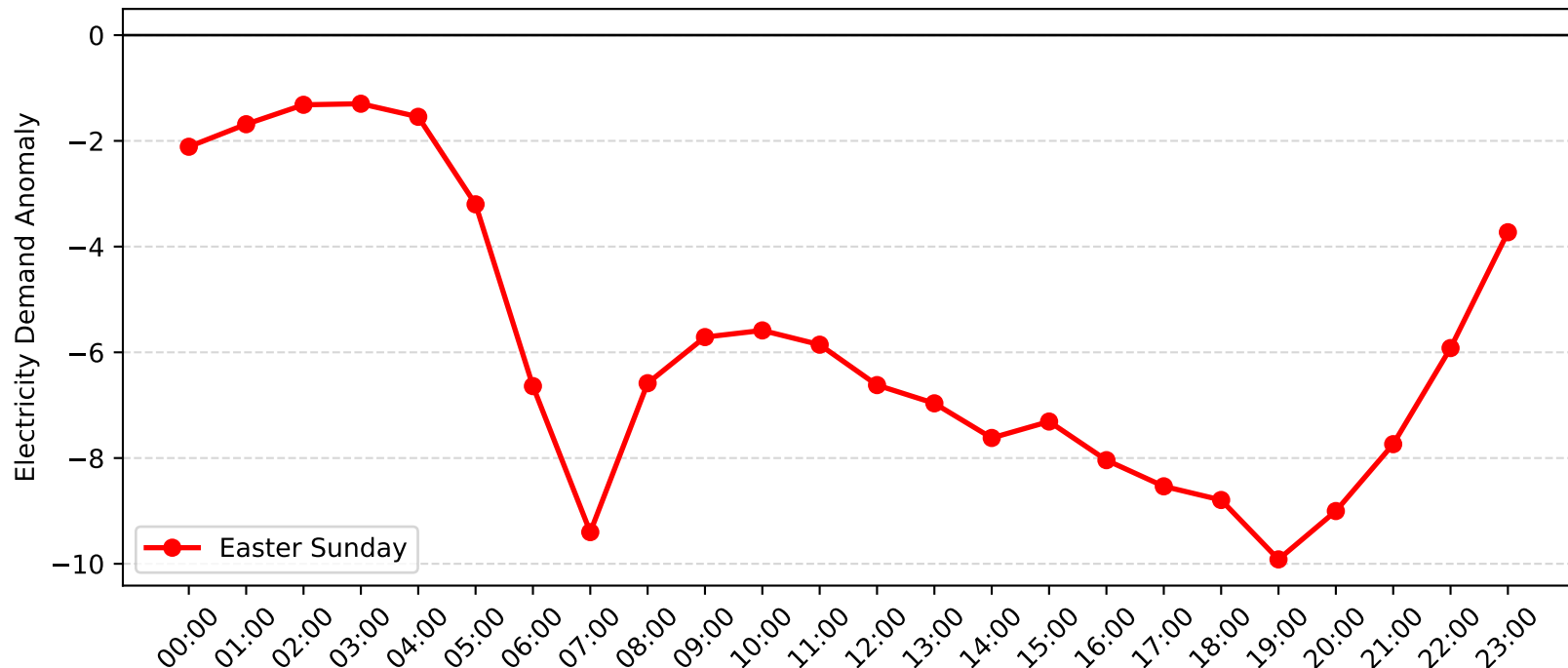
Mosman Demand Anomaly: Easter Sunday (2010-2011)
