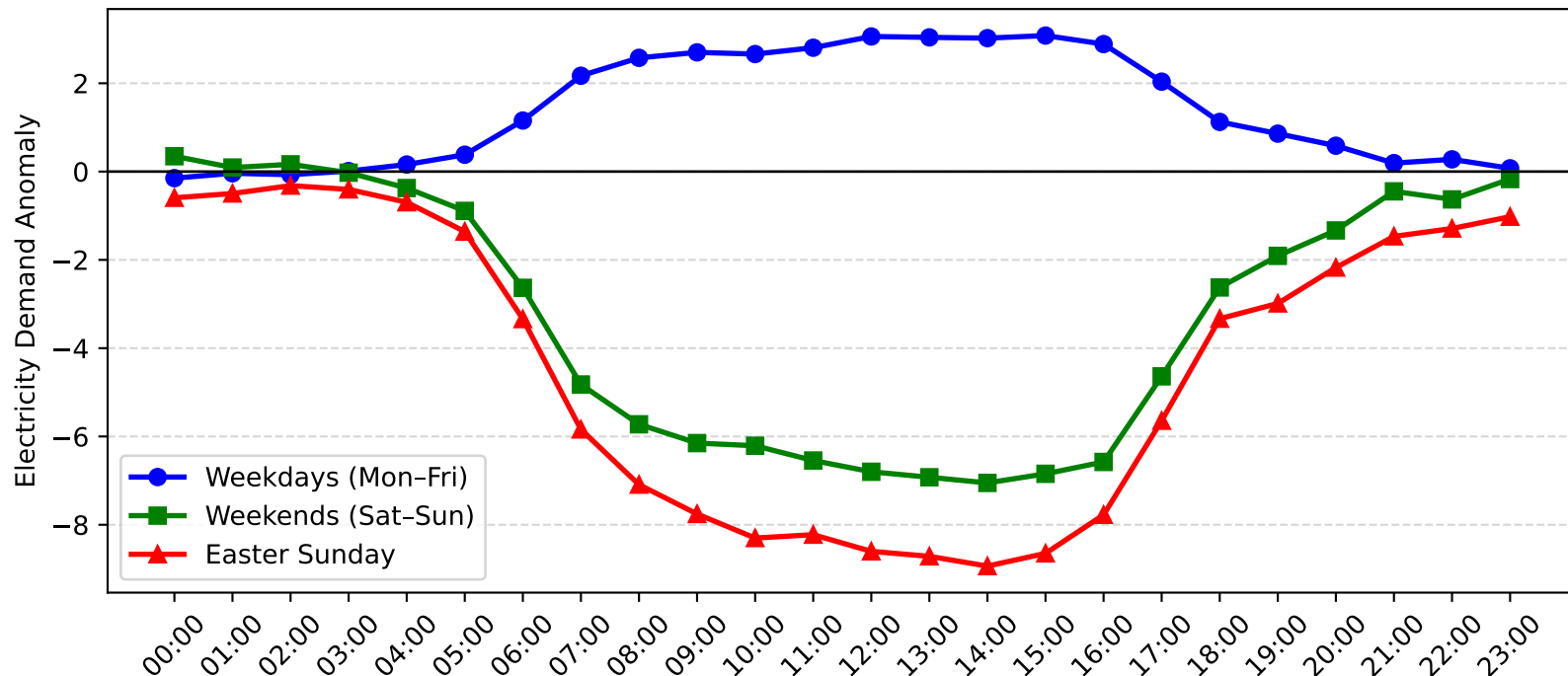
Newcastle Cbd Demand Anomaly: Easter Sunday vs Weekday/Weekend (2008-2009)
