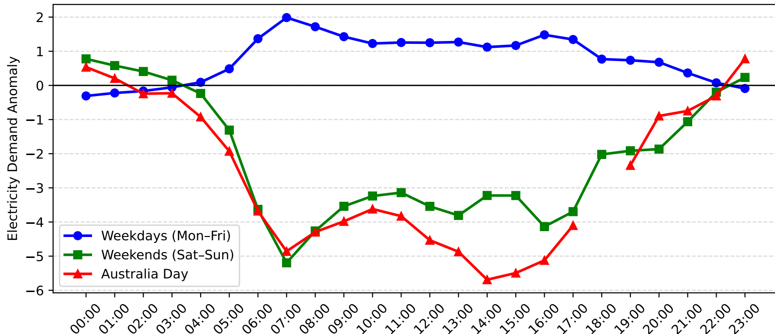
Punchbowl Demand Anomaly: Australia Day vs Weekday/Weekend (2005-2006)
