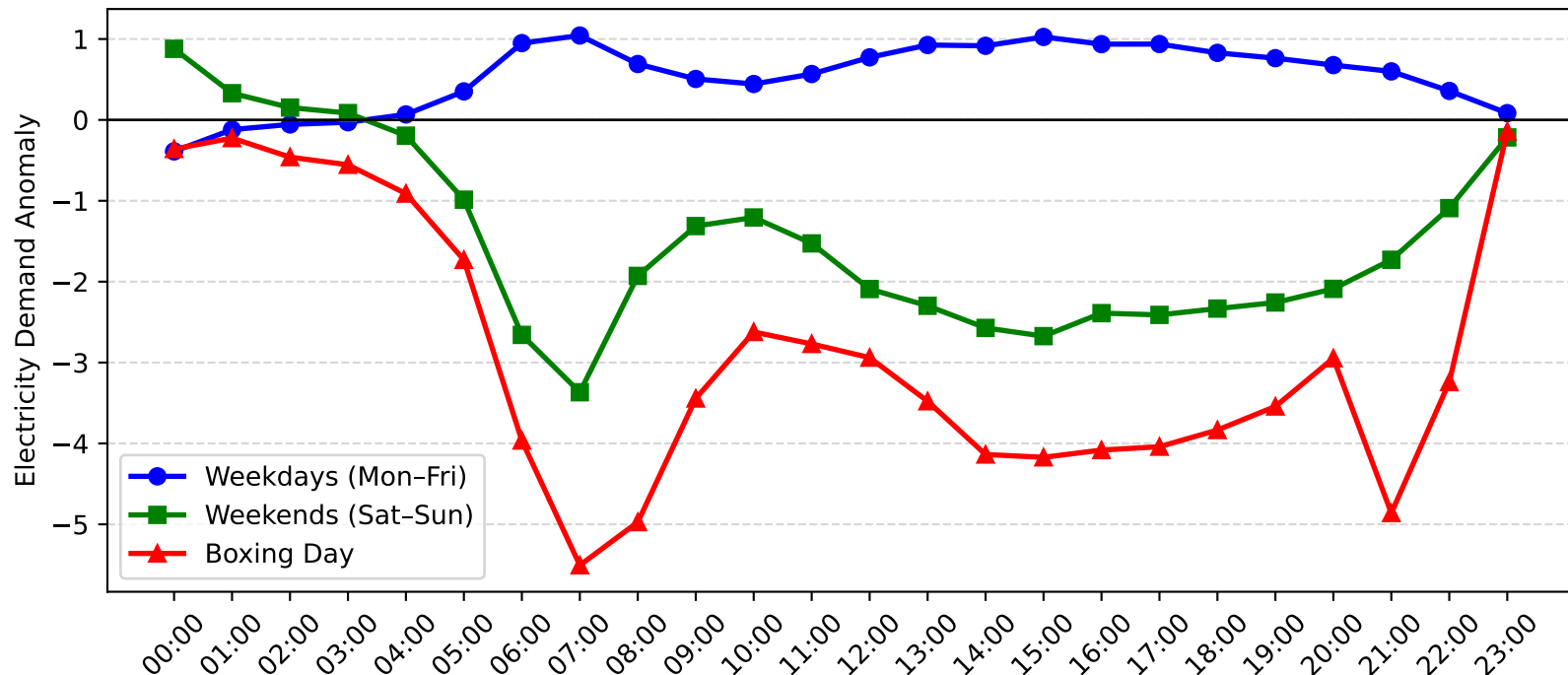
Mortdale Demand Anomaly: Boxing Day vs Weekday/Weekend (2008-2009)
