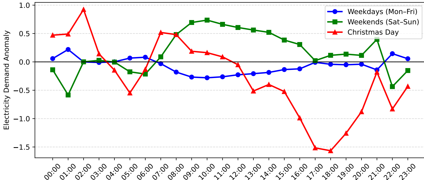
Swansea Demand Anomaly: Christmas Day vs Weekday/Weekend (2009-2010)
