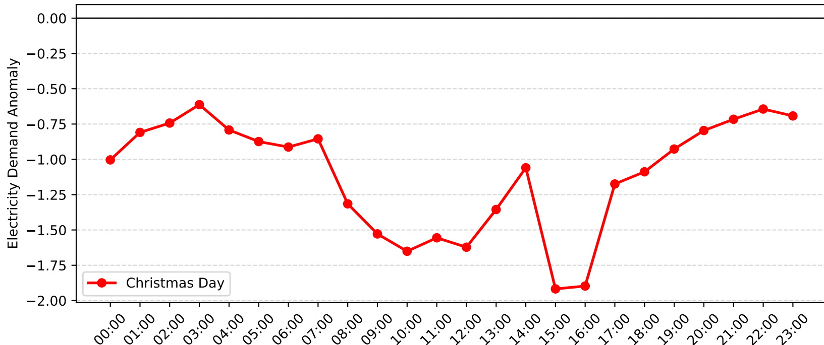
Rothbury Demand Anomaly: Christmas Day (2016-2017)
