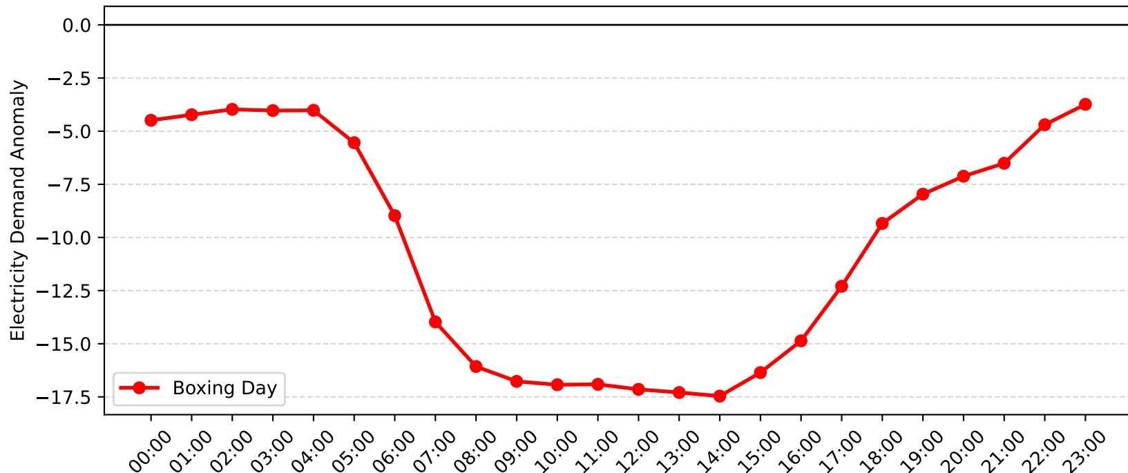
Gore Hill Demand Anomaly: Boxing Day (2005-2006)
