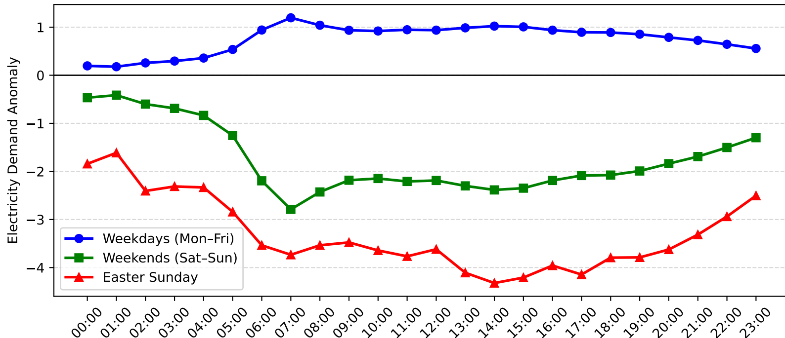
Bass Hill Demand Anomaly: Easter Sunday vs Weekday/Weekend (2014-2015)
