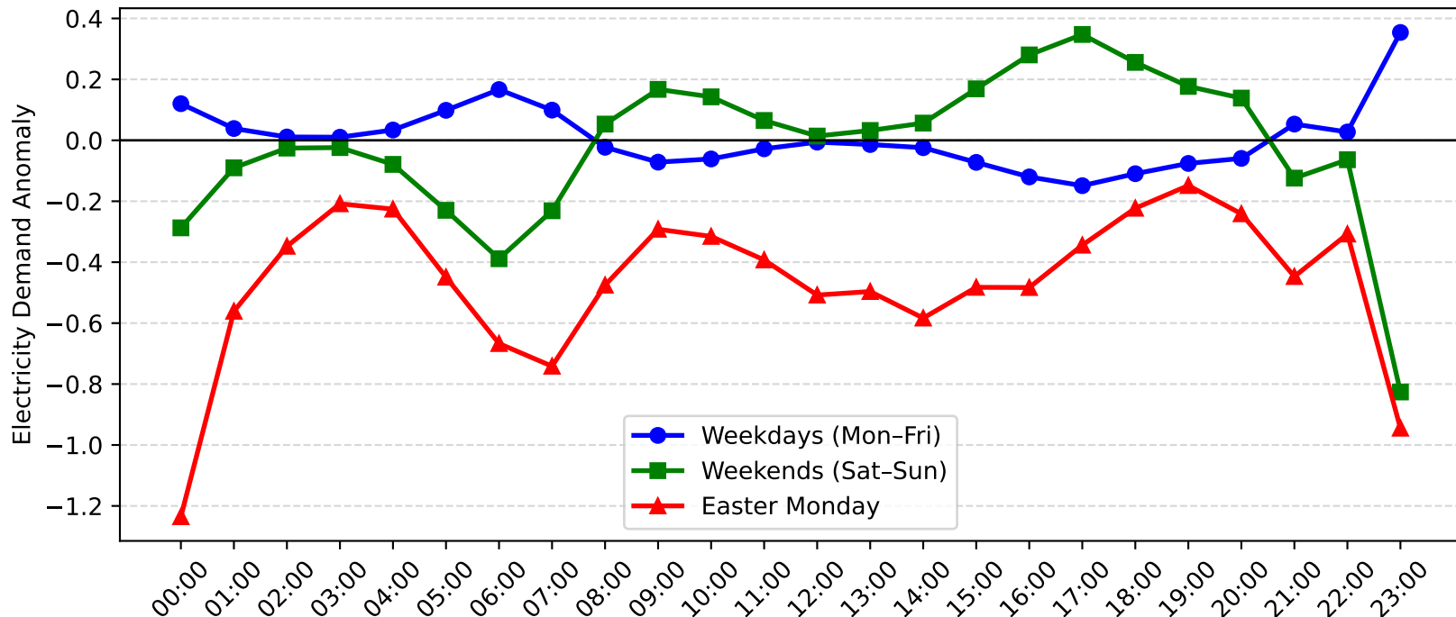
Telarah Demand Anomaly: Easter Monday vs Weekday/Weekend (2013-2014)
