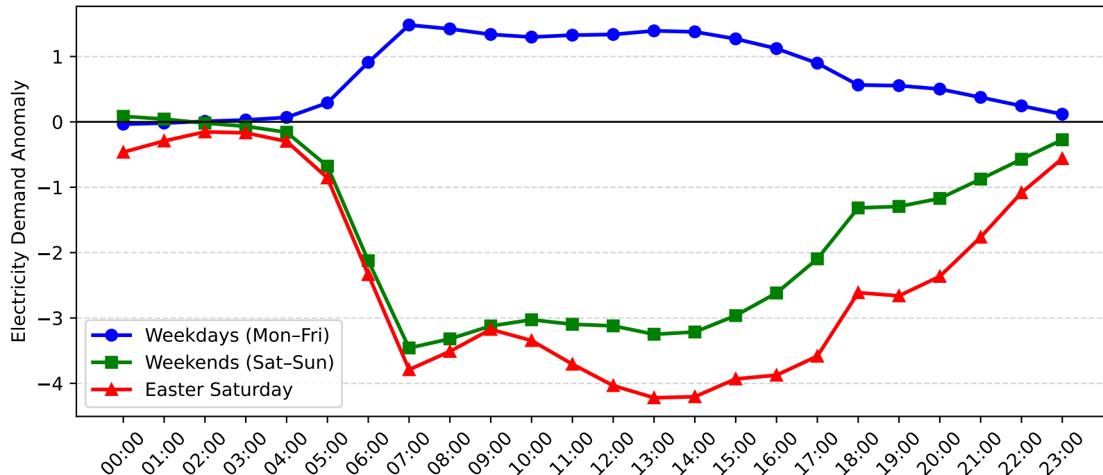
Concord Demand Anomaly: Easter Saturday vs Weekday/Weekend (2014-2015)
