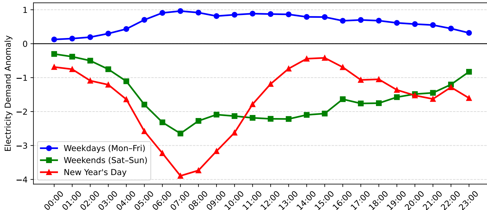
Lisarow Demand Anomaly: New Year's Day vs Weekday/Weekend (2010-2011)
