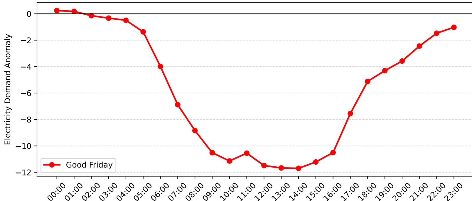
Brookvale Demand Anomaly: Good Friday (2013-2014)
