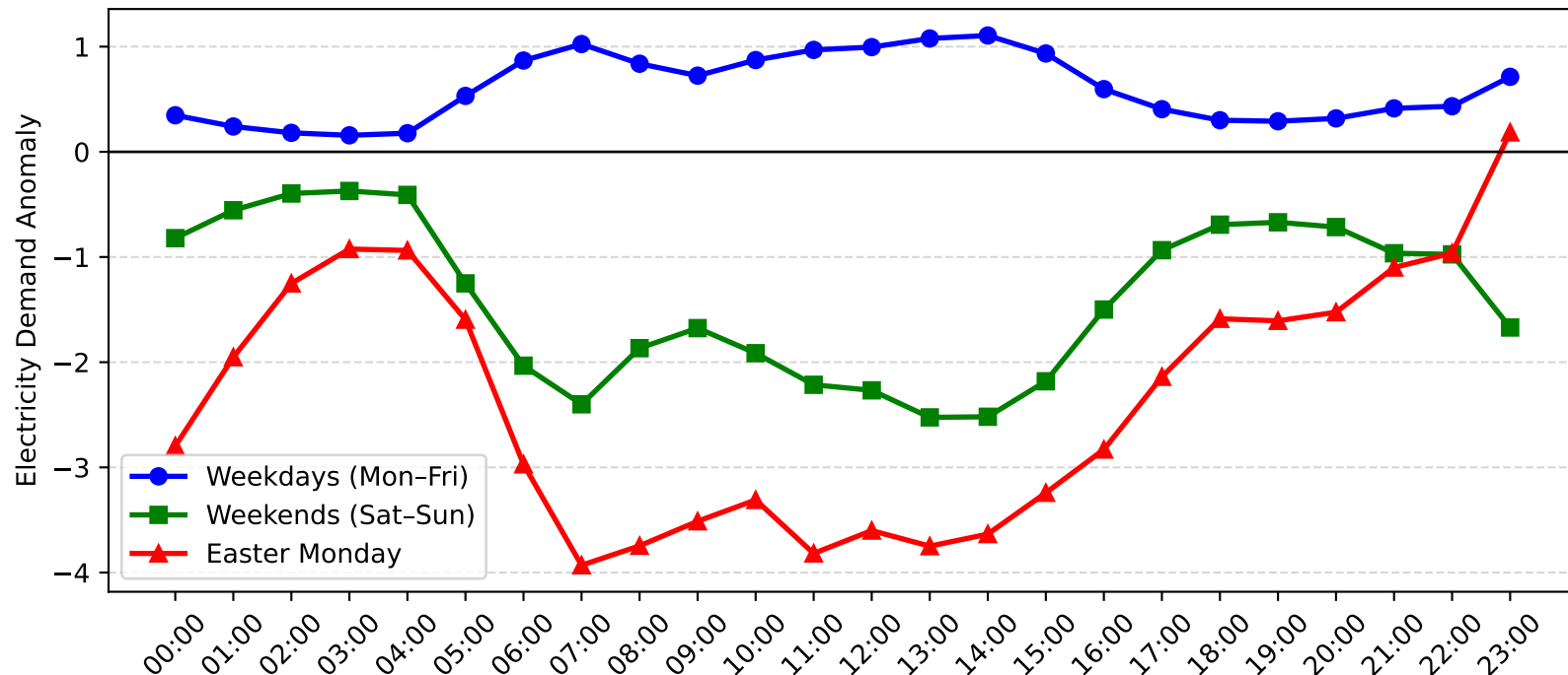
Rutherford Demand Anomaly: Easter Monday vs Weekday/Weekend (2006-2007)
