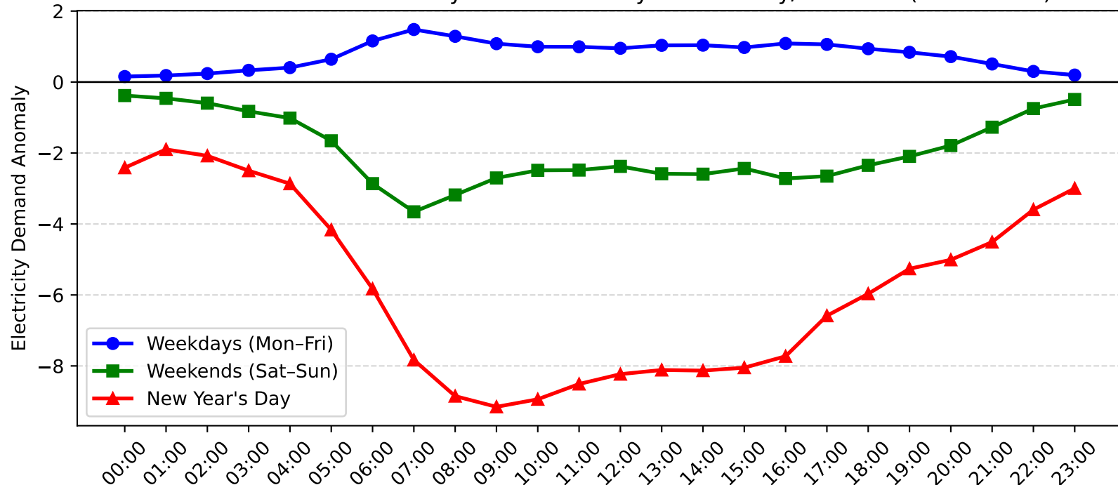
Maroubra Demand Anomaly: New Year's Day vs Weekday/Weekend (2016-2017)
