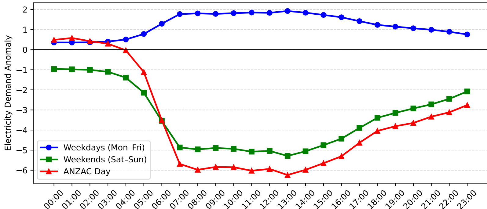
Leightonfield Demand Anomaly: ANZAC Day vs Weekday/Weekend (2012-2013)
