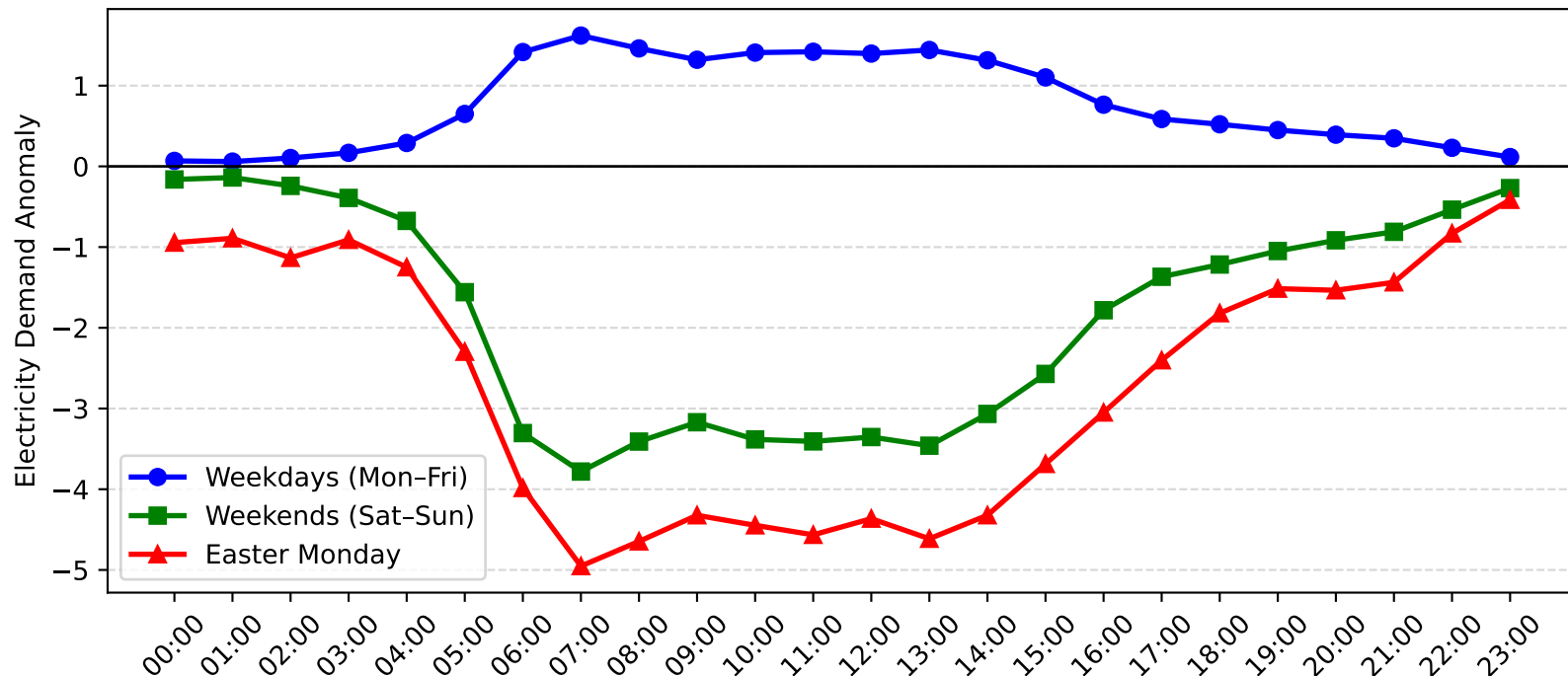
Wyong Demand Anomaly: Easter Monday vs Weekday/Weekend (2013-2014)
