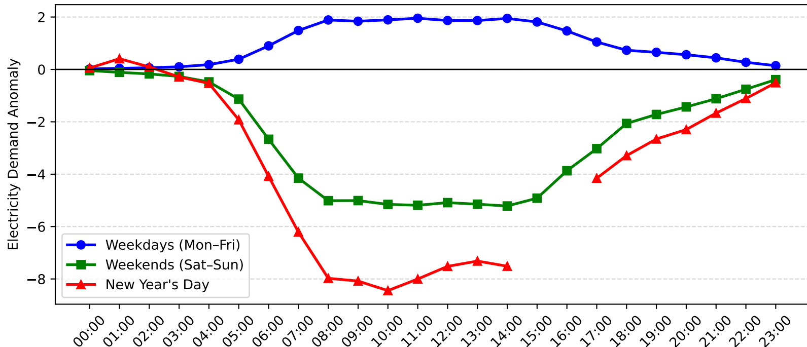
Bankstown Demand Anomaly: New Year's Day vs Weekday/Weekend (2015-2016)
