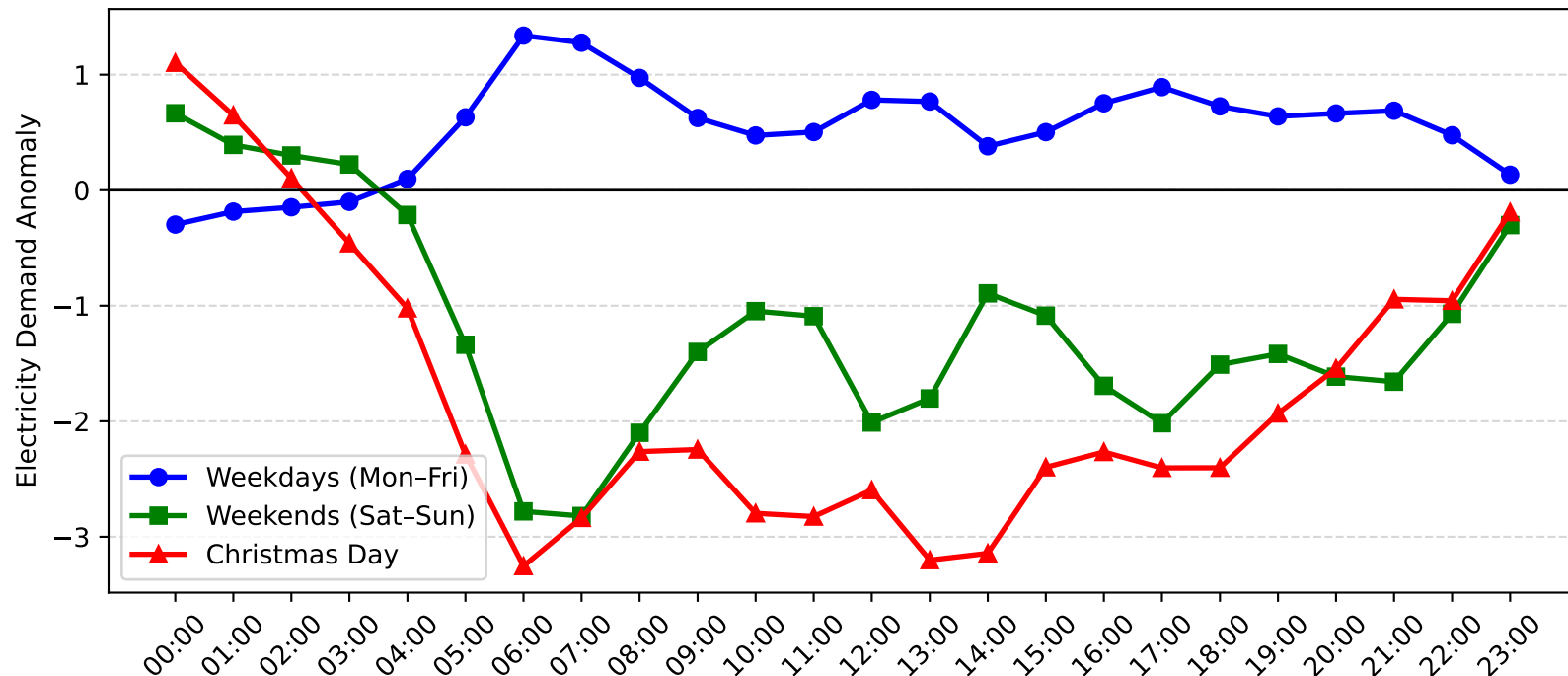
Revesby Demand Anomaly: Christmas Day vs Weekday/Weekend (2004-2005)
