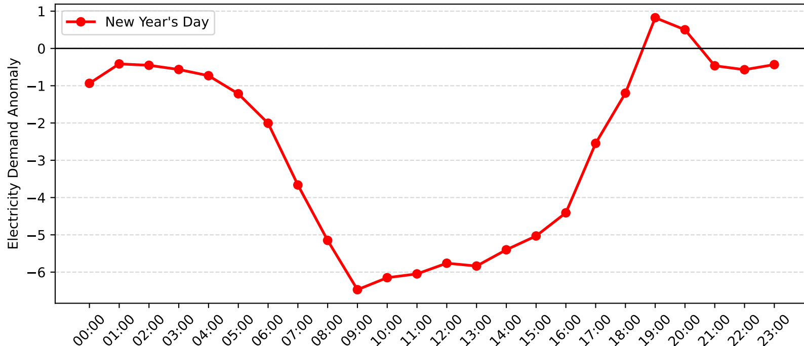
Auburn Demand Anomaly: New Year's Day (2008-2009)
