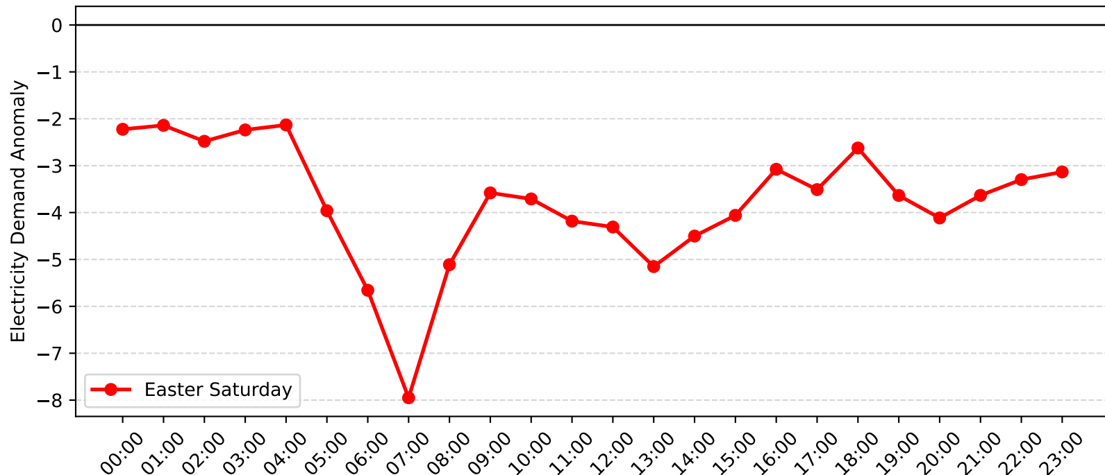
Meadowbank Demand Anomaly: Easter Saturday (2008-2009)
