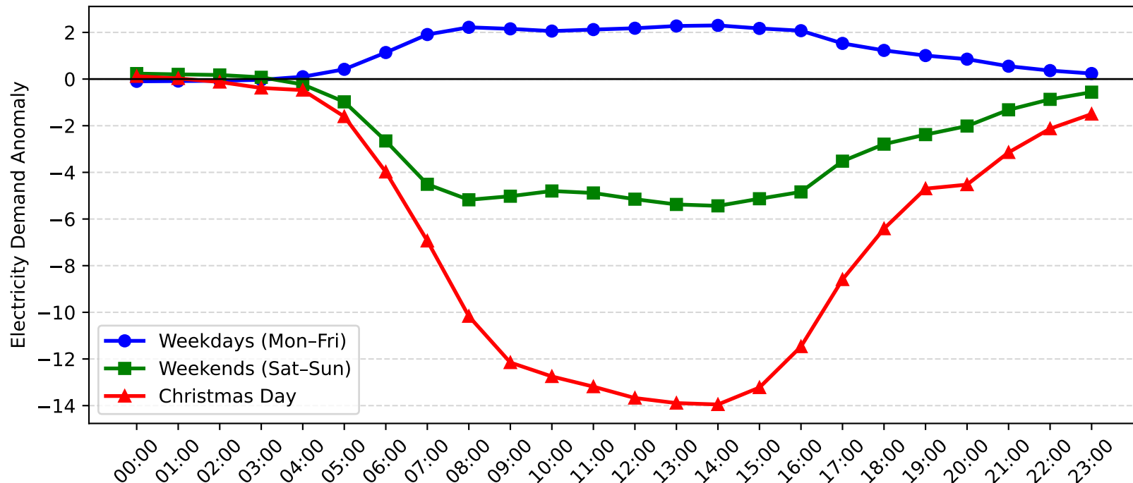
Brookvale Demand Anomaly: Christmas Day vs Weekday/Weekend (2011-2012)
