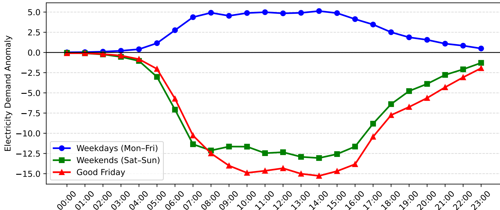
Zetland Demand Anomaly: Good Friday vs Weekday/Weekend (2006-2007)
