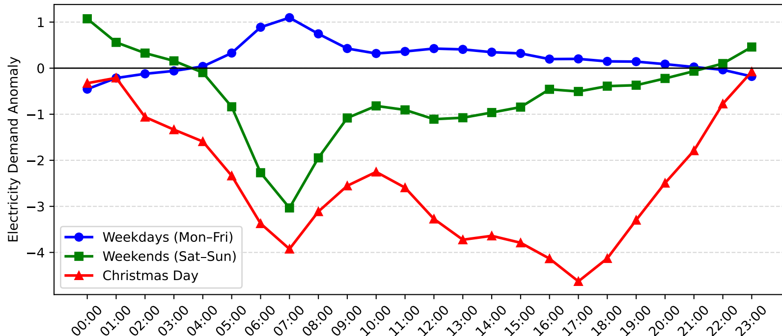
Mortdale Demand Anomaly: Christmas Day vs Weekday/Weekend (2009-2010)
