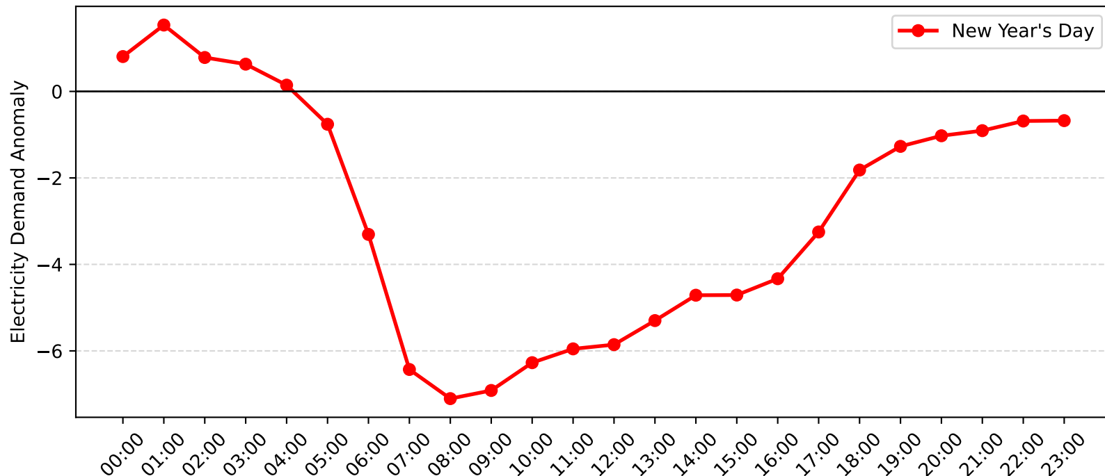
Chatswood Demand Anomaly: New Year's Day (2009-2010)
