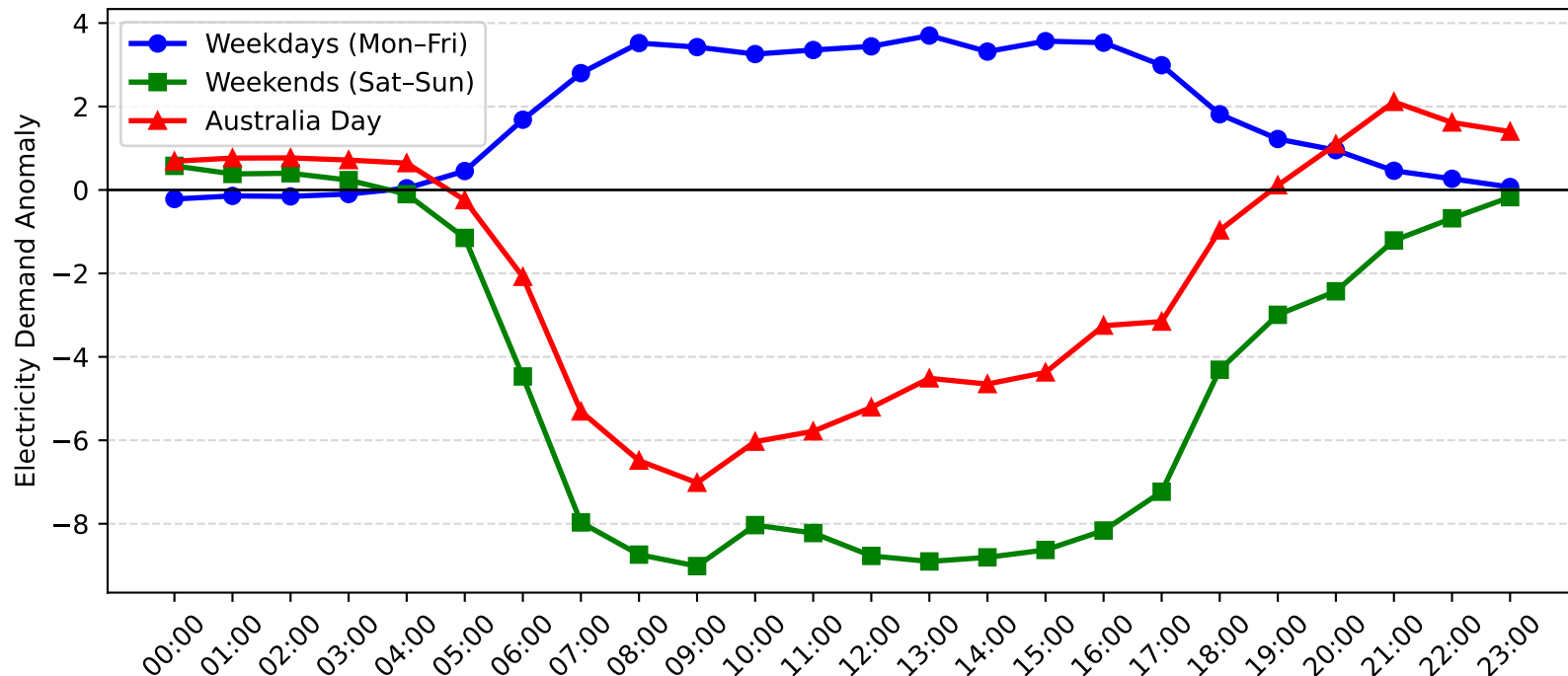
Castle Cove Demand Anomaly: Australia Day vs Weekday/Weekend (2009-2010)
