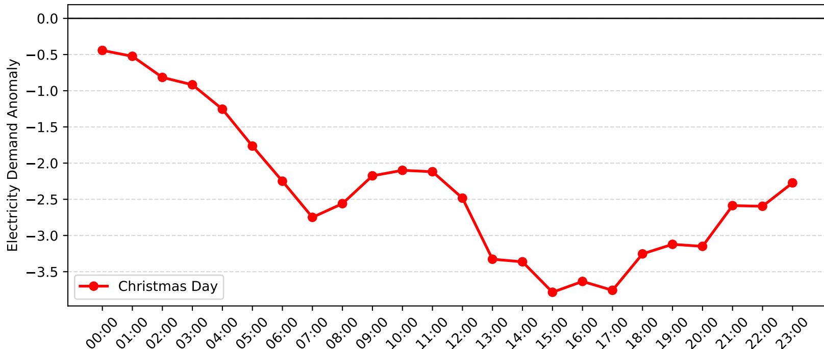
Bass Hill Demand Anomaly: Christmas Day (2011-2012)
