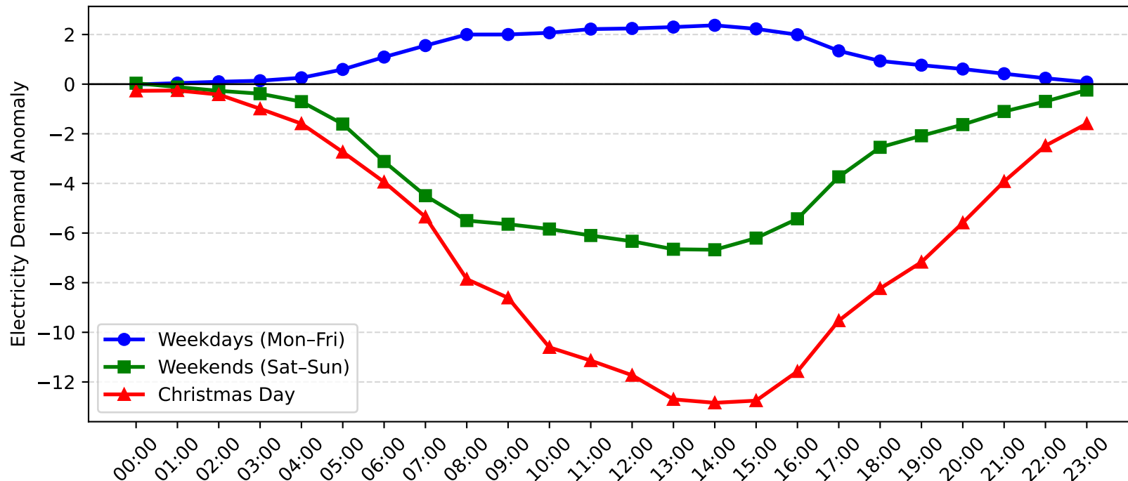
West Gosford Demand Anomaly: Christmas Day vs Weekday/Weekend (2014-2015)
