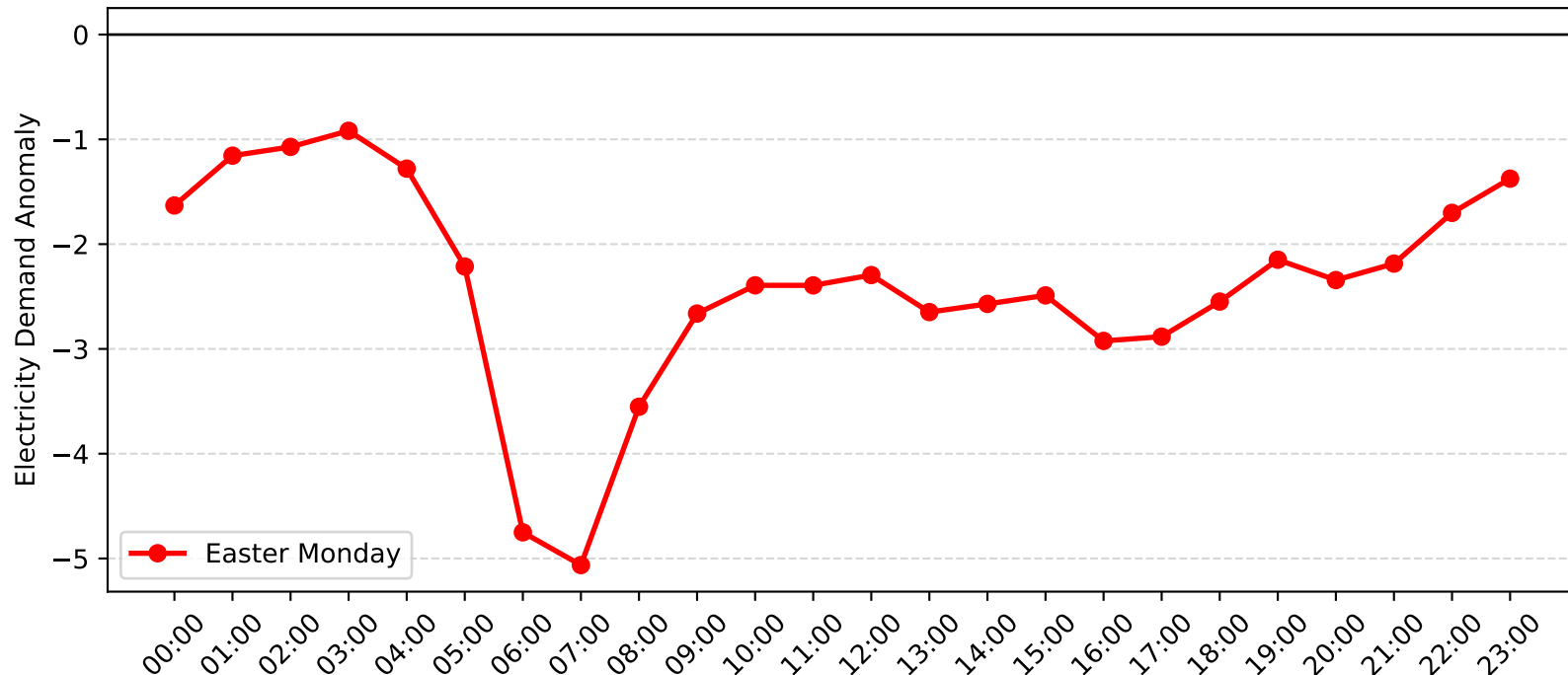
Revesby Demand Anomaly: Easter Monday (2013-2014)
