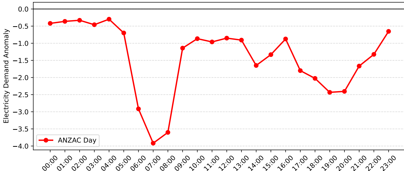
Balgowlah North Demand Anomaly: ANZAC Day (2015-2016)
