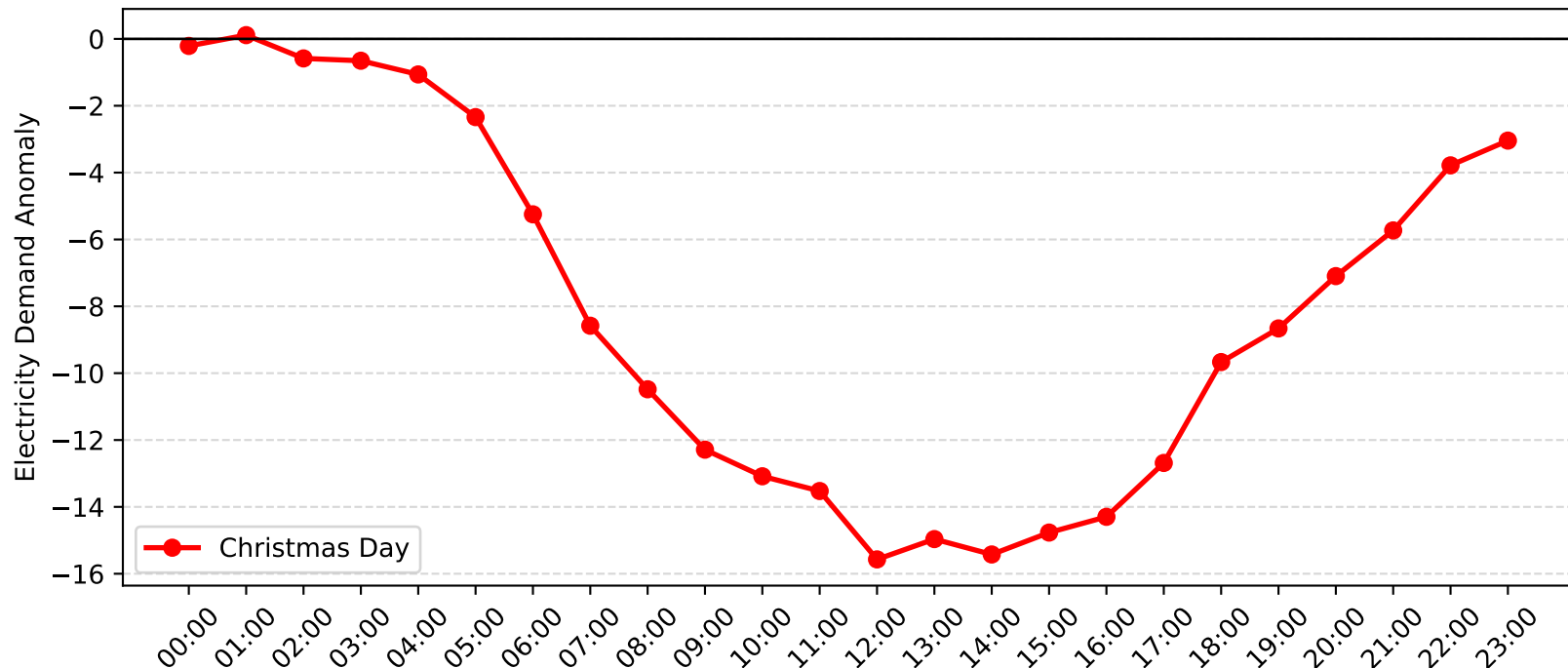
Burwood Demand Anomaly: Christmas Day (2005-2006)
