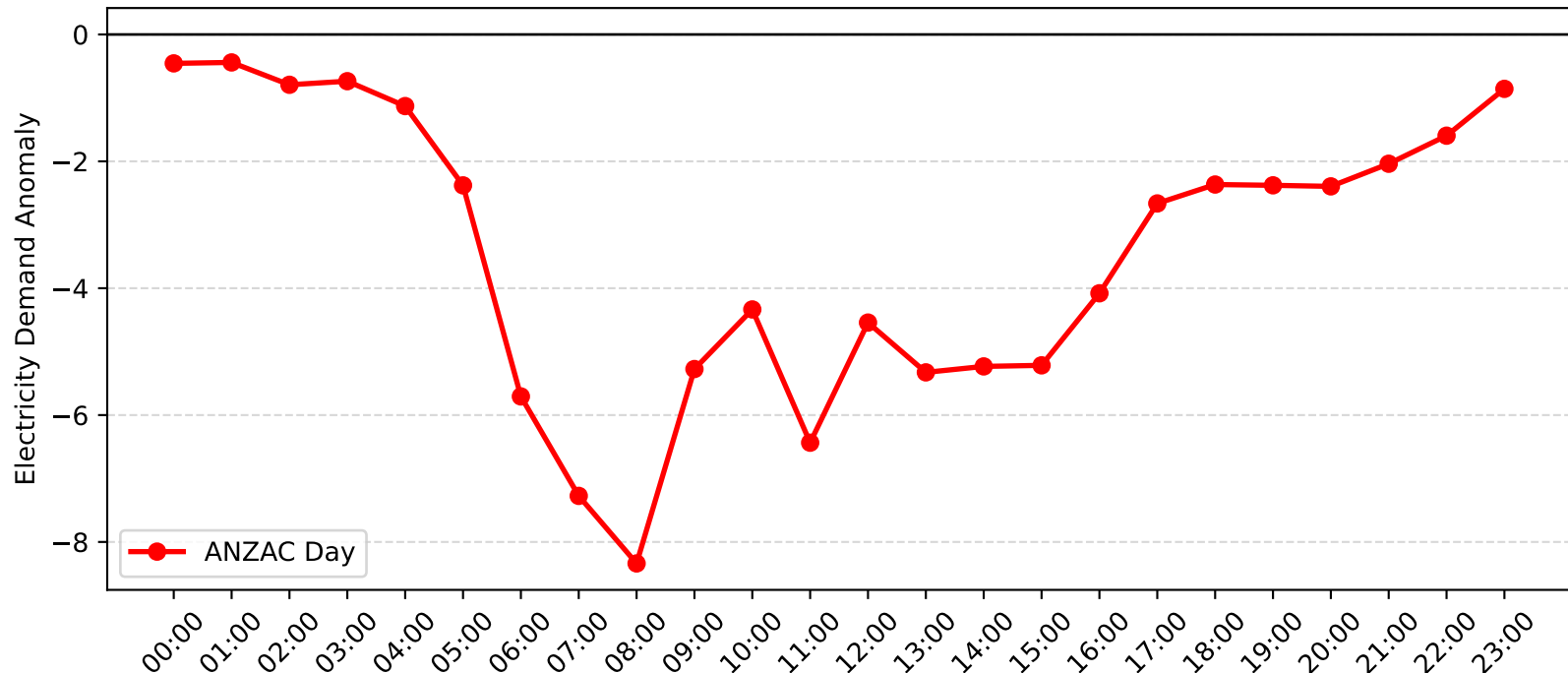
Sefton Demand Anomaly: ANZAC Day (2005-2006)
