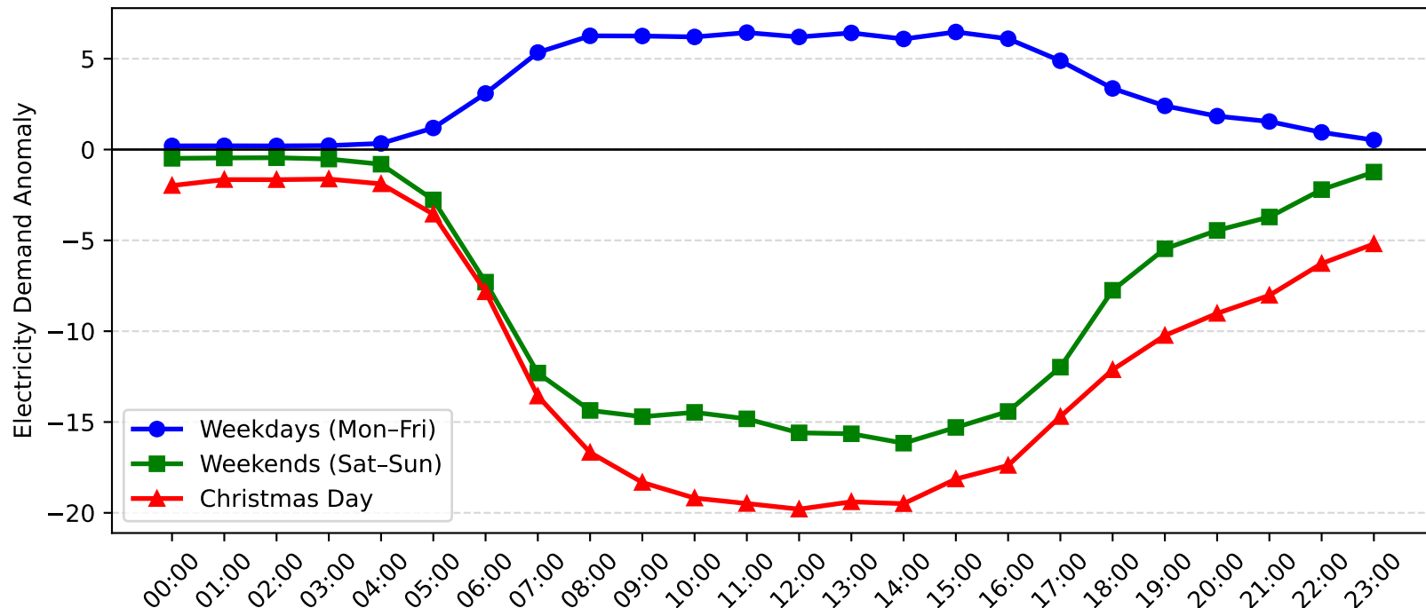
Gore Hill Demand Anomaly: Christmas Day vs Weekday/Weekend (2005-2006)
