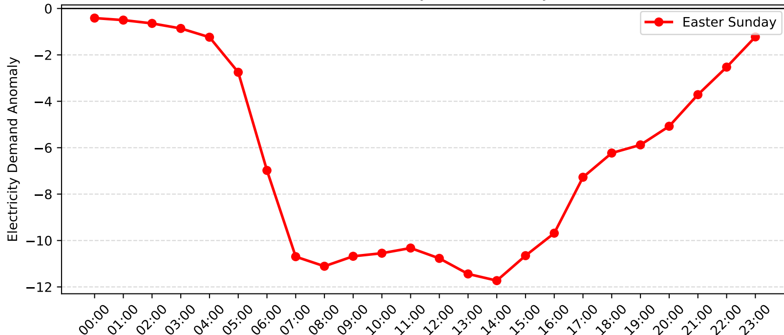
Marrickville Demand Anomaly: Easter Sunday (2008-2009)
