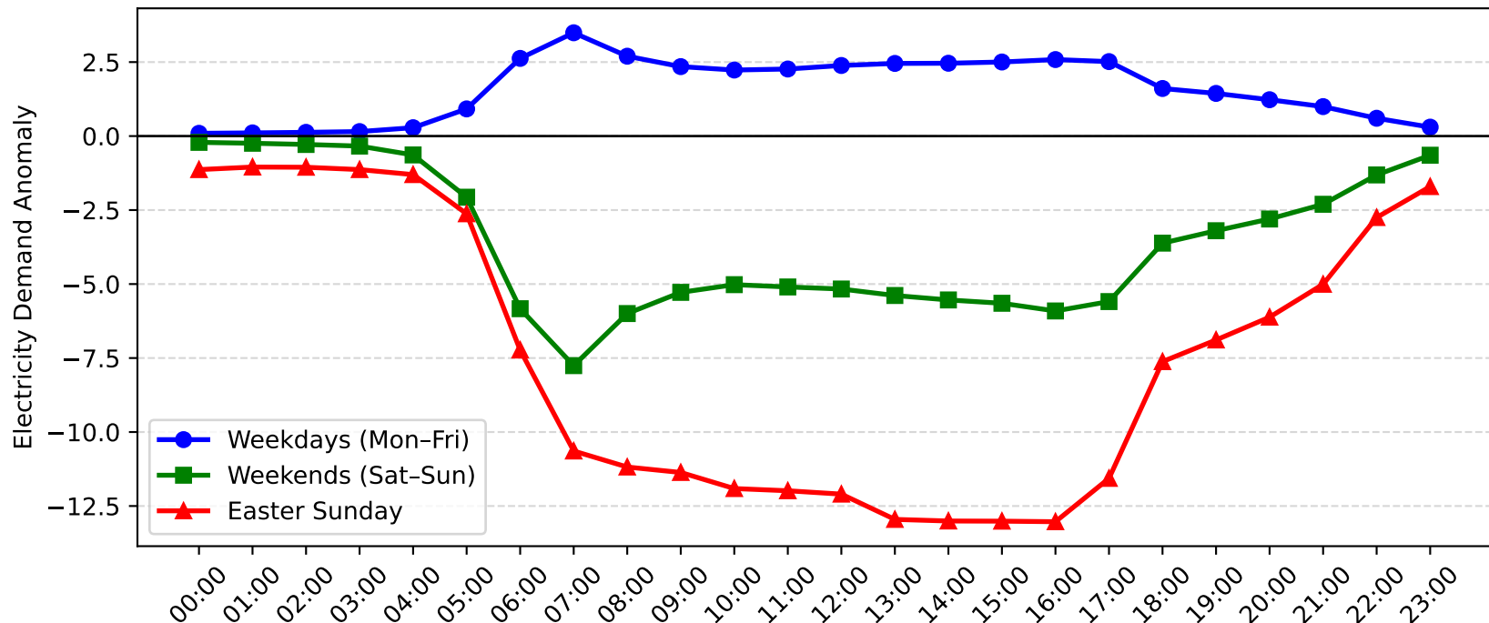
Epping Demand Anomaly: Easter Sunday vs Weekday/Weekend (2008-2009)
