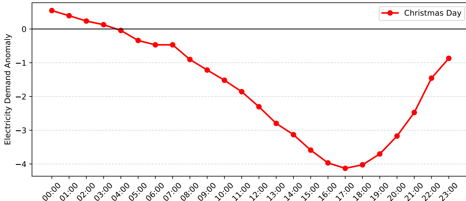
Muswellbrook Demand Anomaly: Christmas Day (2012-2013)
