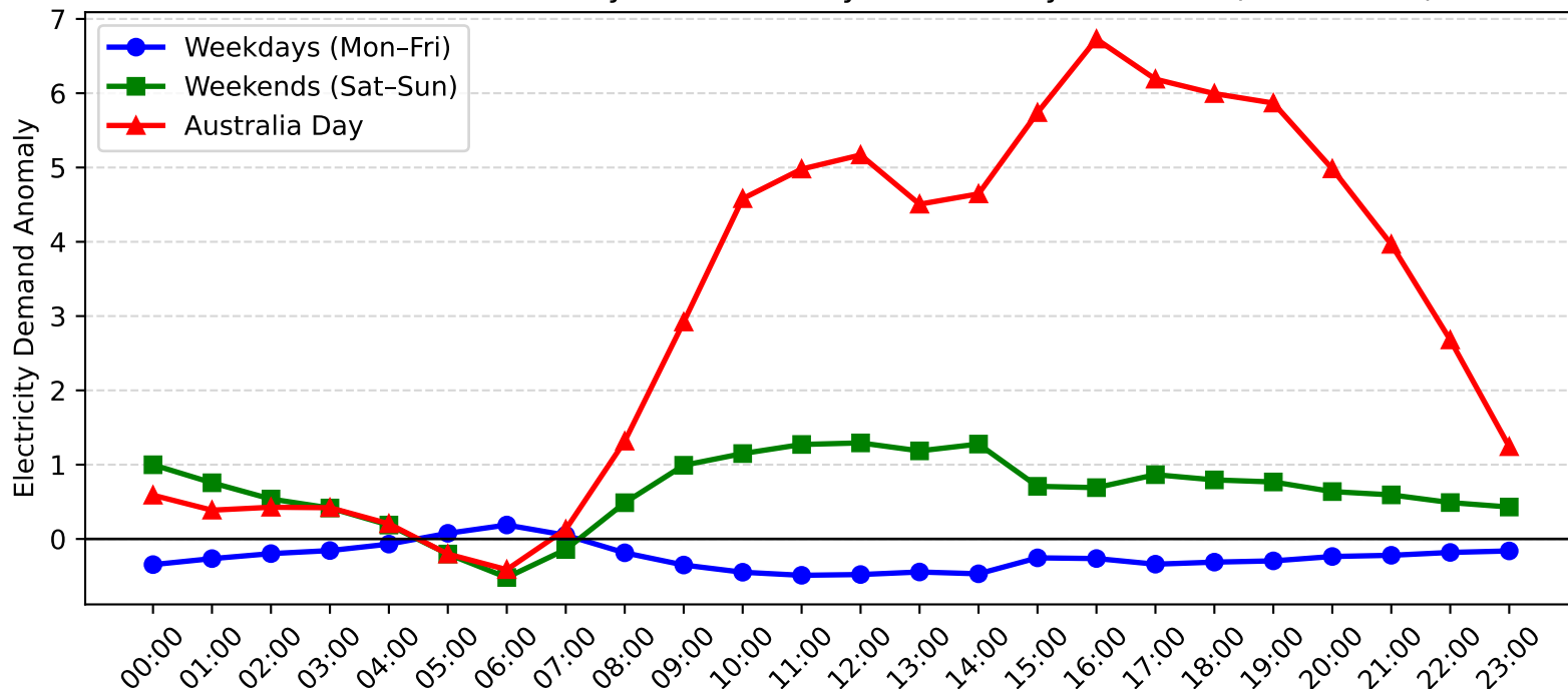
Umina Demand Anomaly: Australia Day vs Weekday/Weekend (2010-2011)
