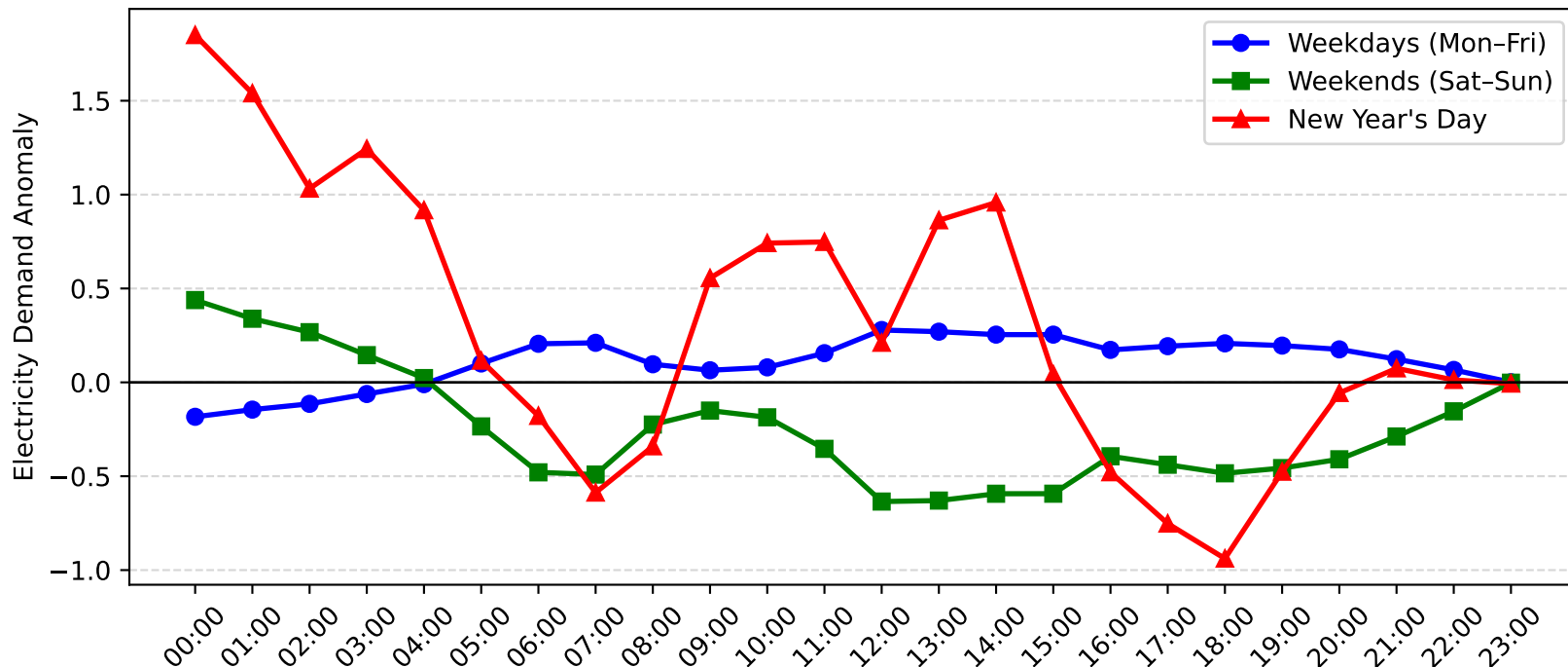
Noraville Demand Anomaly: New Year's Day vs Weekday/Weekend (2017-2018)
