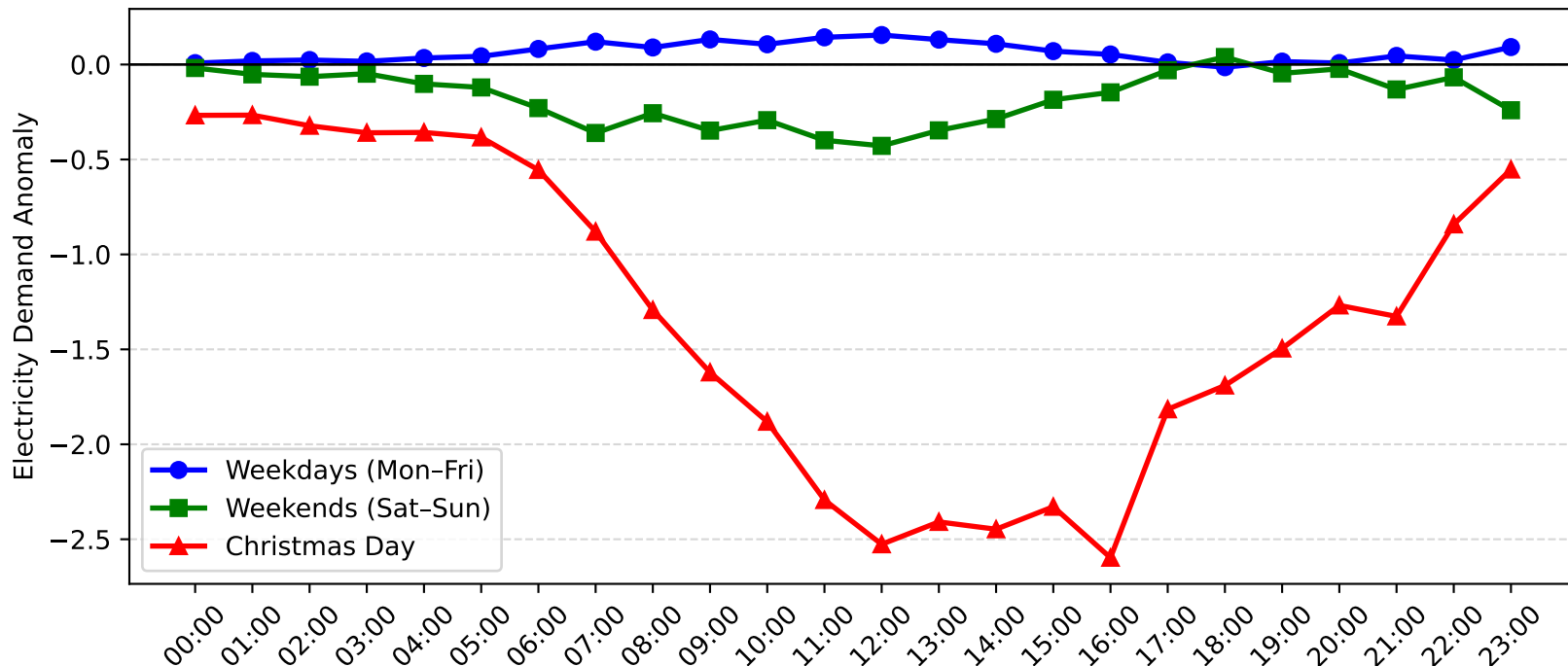
Rothbury Demand Anomaly: Christmas Day vs Weekday/Weekend (2007-2008)
