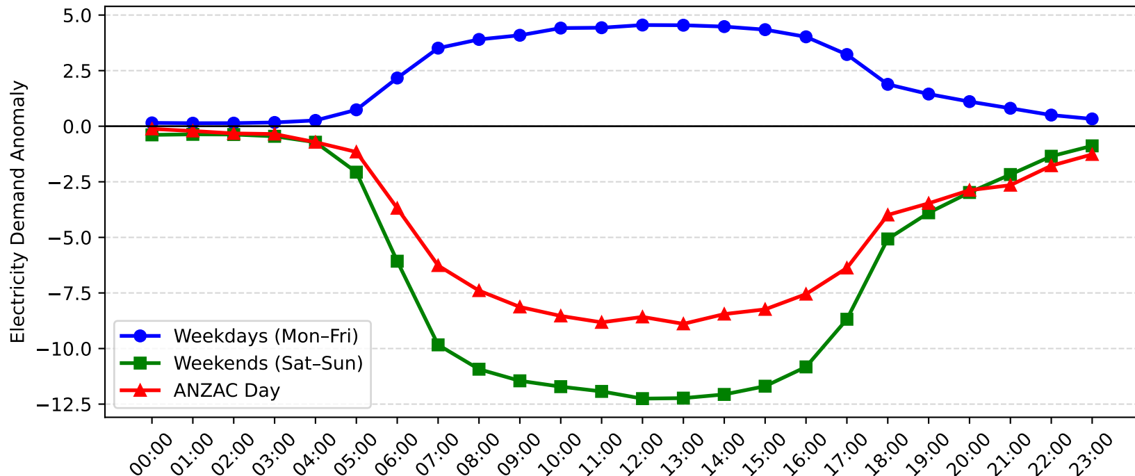
Macquarie Park Demand Anomaly: ANZAC Day vs Weekday/Weekend (2012-2013)
