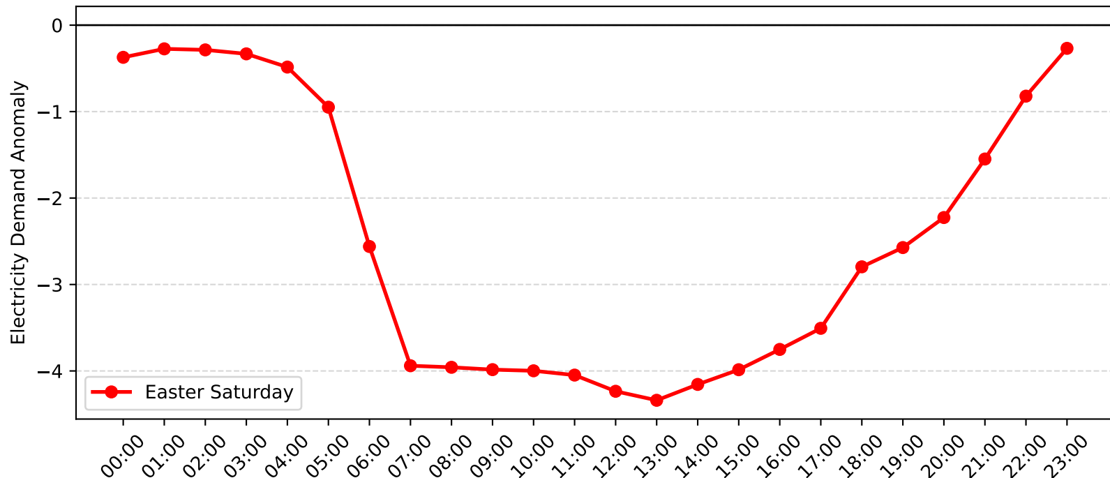
Concord Demand Anomaly: Easter Saturday (2013-2014)
