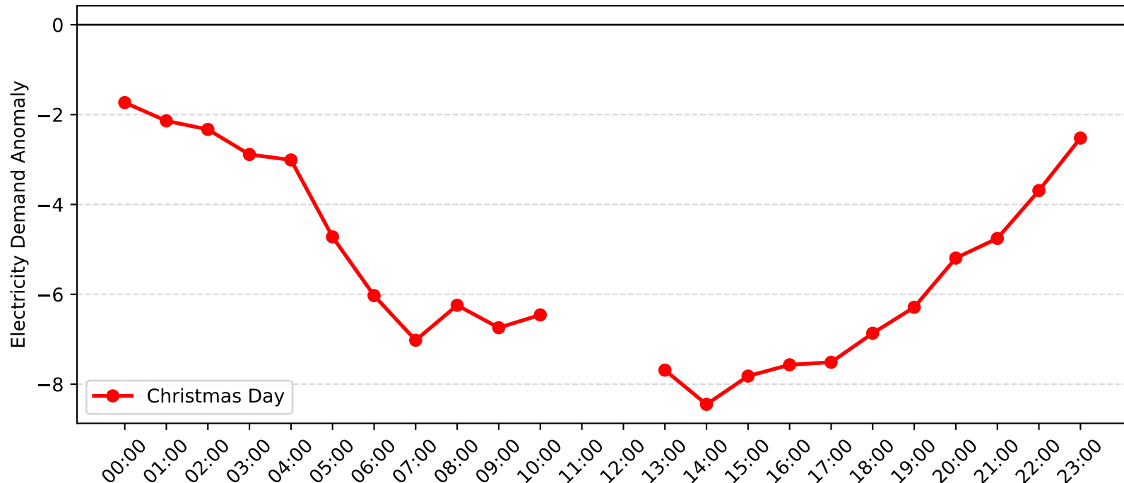
Matraverse Demand Anomaly: Christmas Day (2008-2009)
