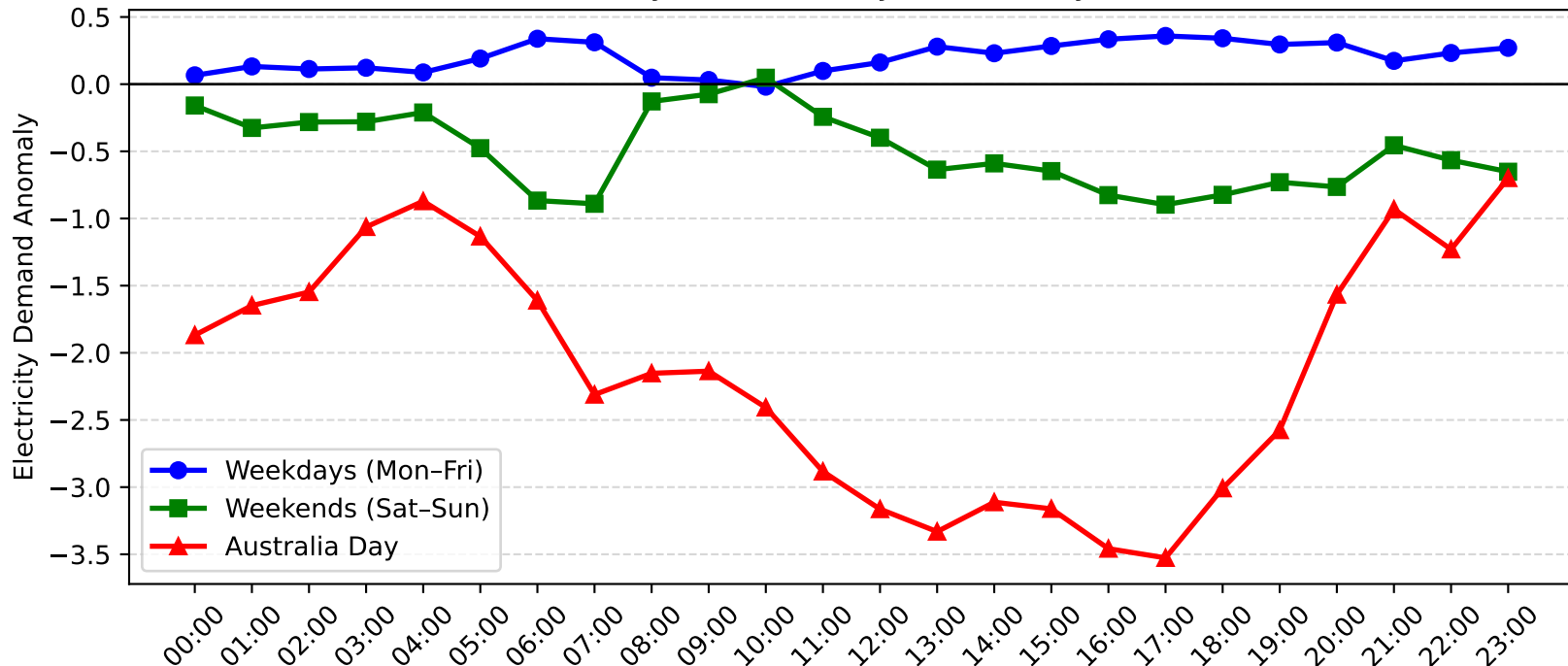
Morisset Demand Anomaly: Australia Day vs Weekday/Weekend (2008-2009)
