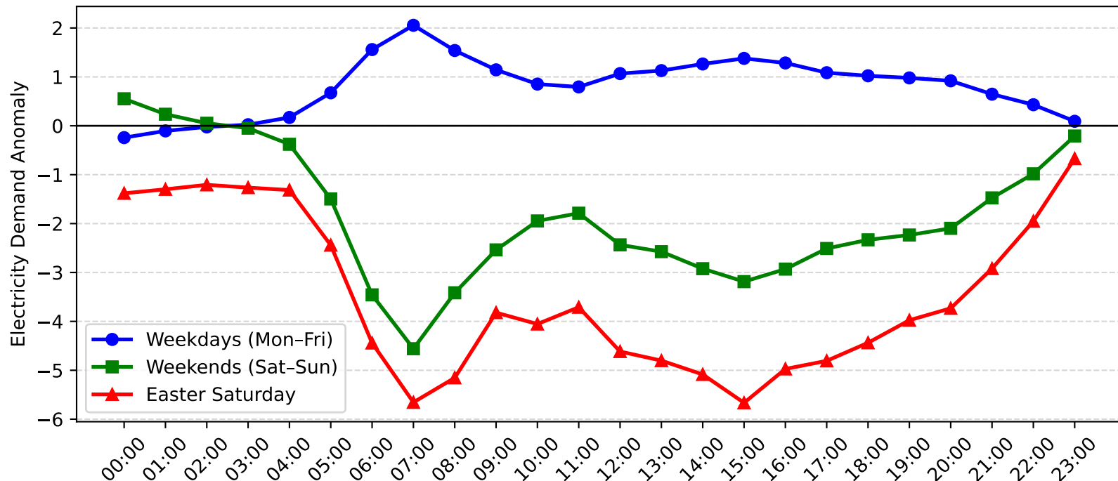
Kogarah Demand Anomaly: Easter Saturday vs Weekday/Weekend (2016-2017)
