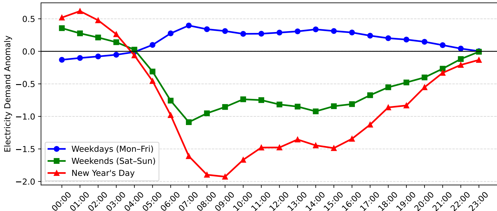
Rockdale Demand Anomaly: New Year's Day vs Weekday/Weekend (2013-2014)
