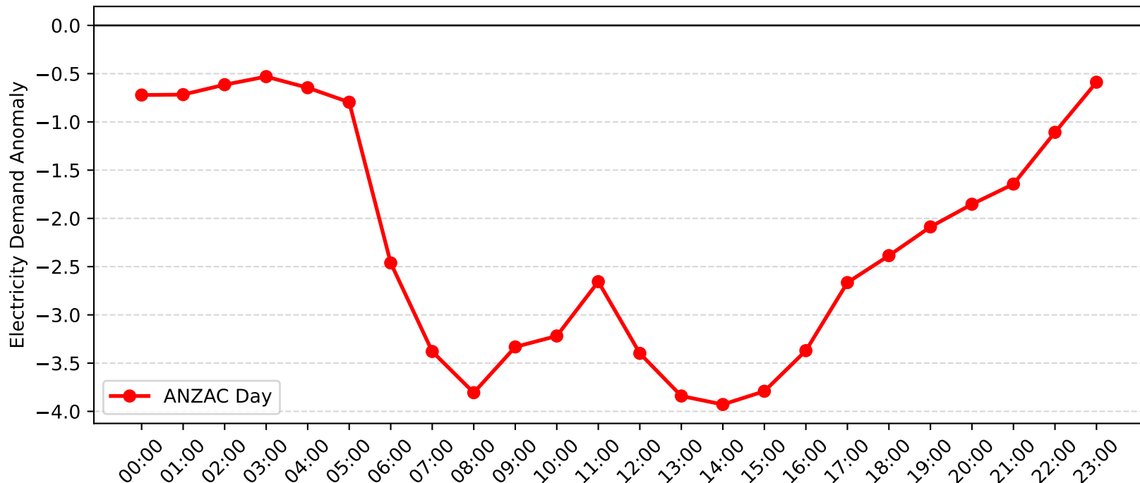
Beacon Hill Demand Anomaly: ANZAC Day (2005-2006)
