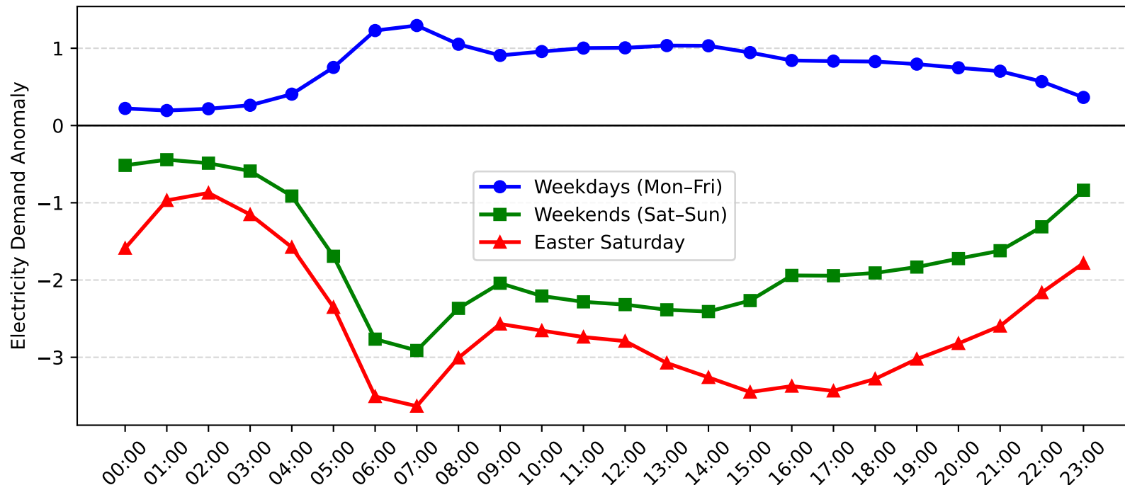
Lisarow Demand Anomaly: Easter Saturday vs Weekday/Weekend (2015-2016)
