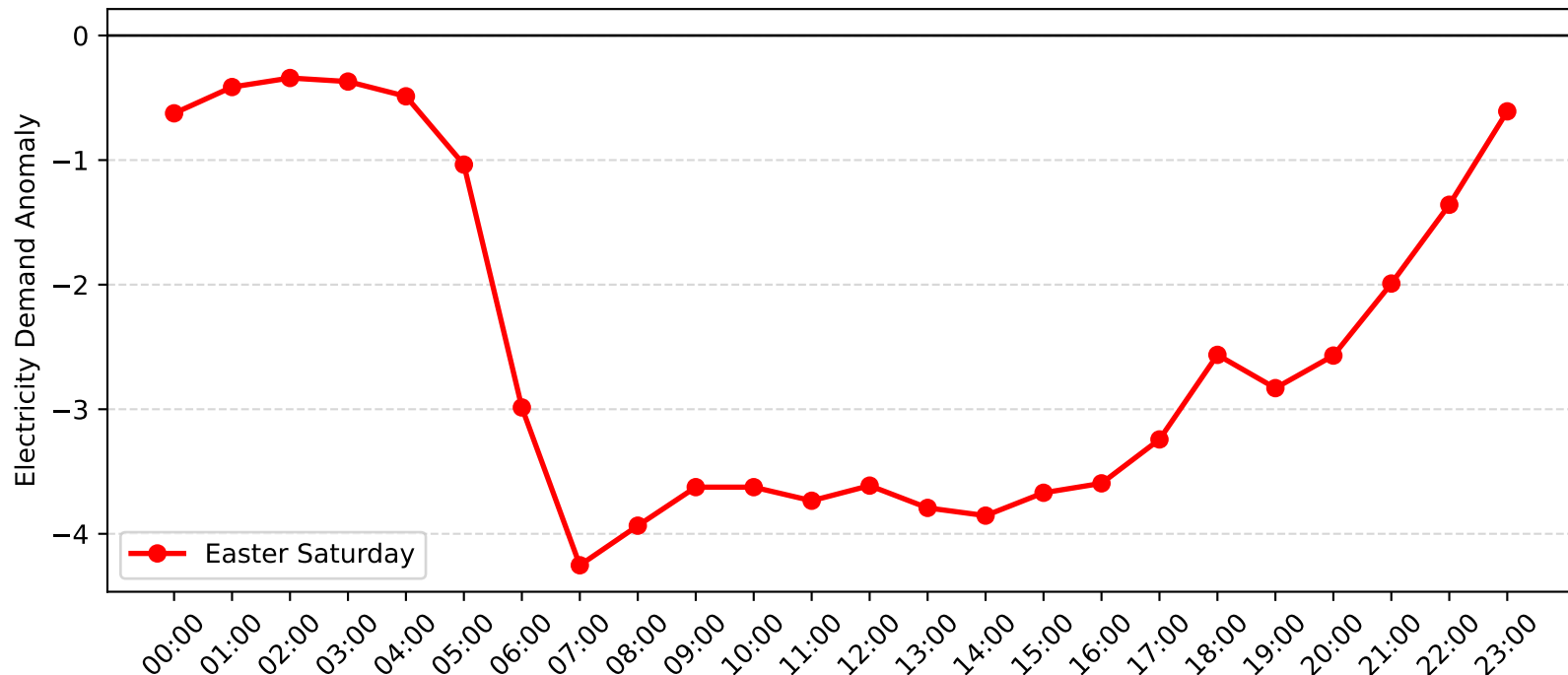
Concord Demand Anomaly: Easter Saturday (2011-2012)
