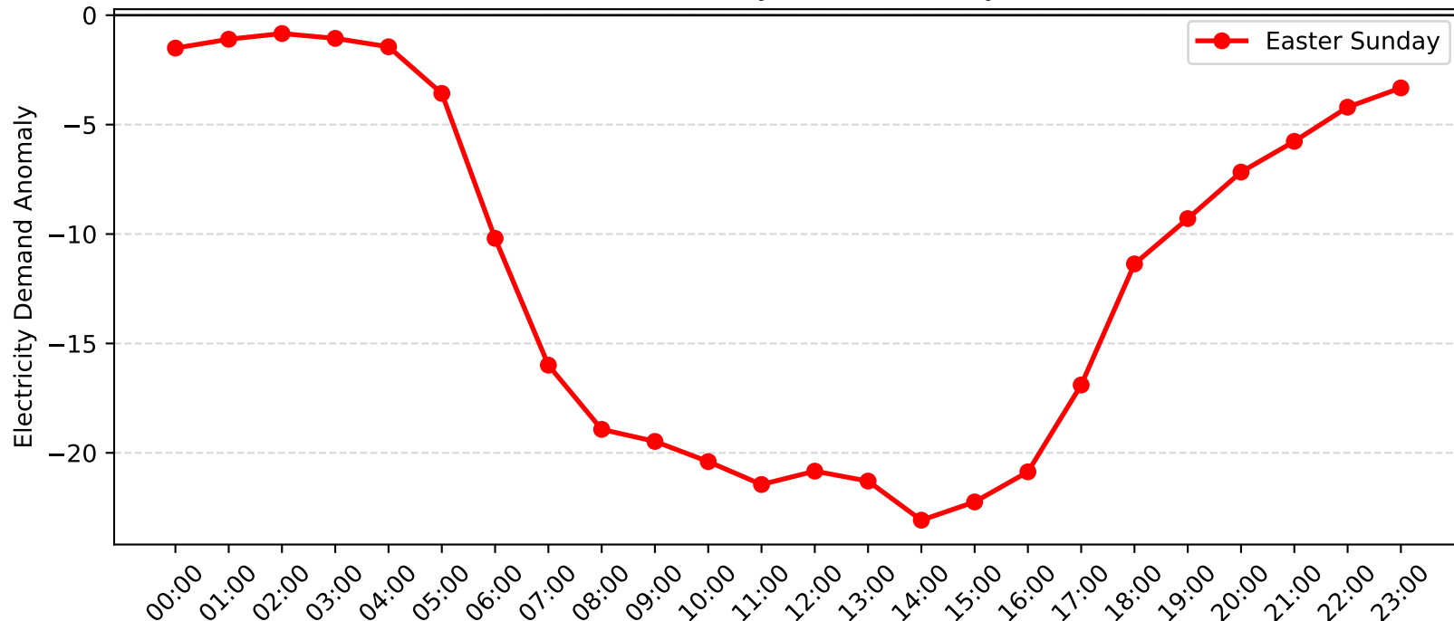
Gore Hill Demand Anomaly: Easter Sunday (2005-2006)
