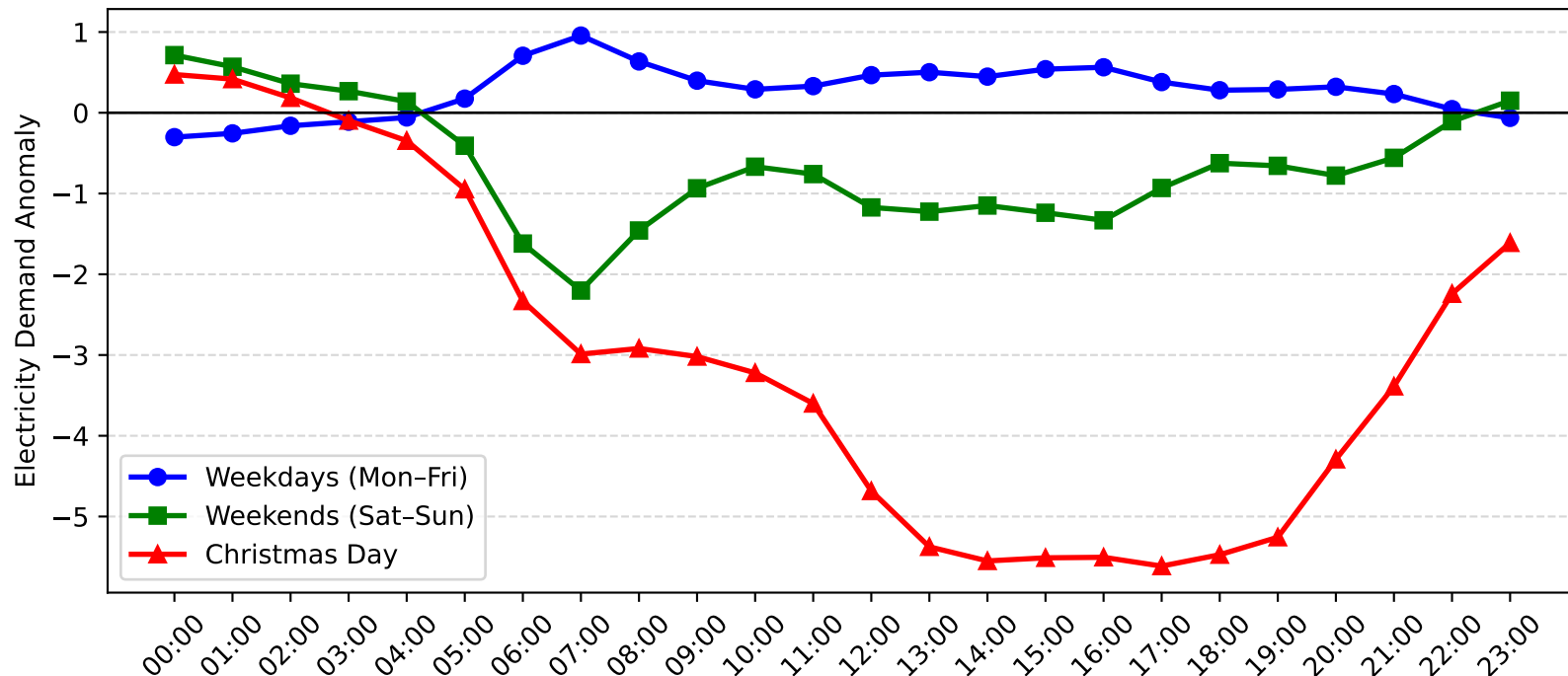
Five Dock Demand Anomaly: Christmas Day vs Weekday/Weekend (2005-2006)
