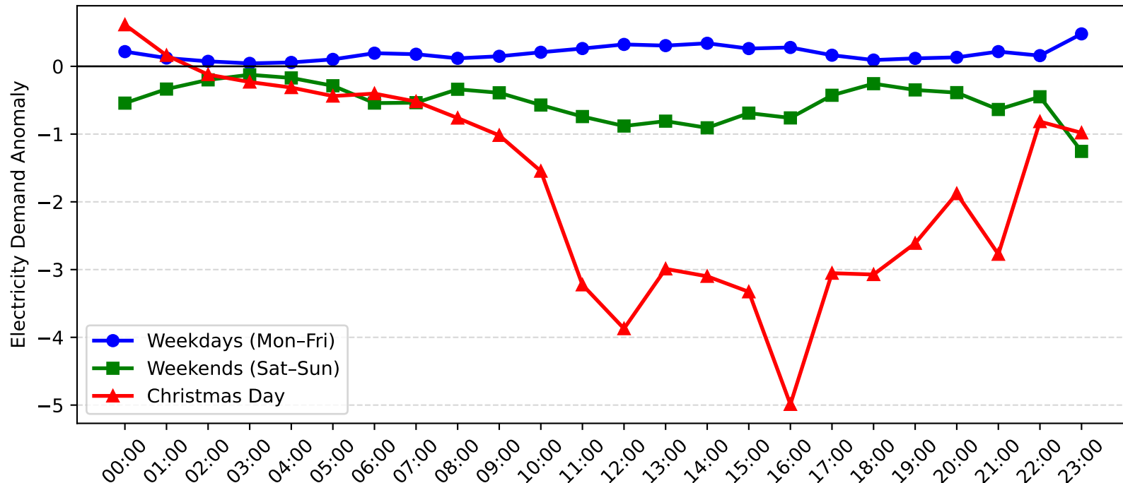
Telarah Demand Anomaly: Christmas Day vs Weekday/Weekend (2007-2008)
