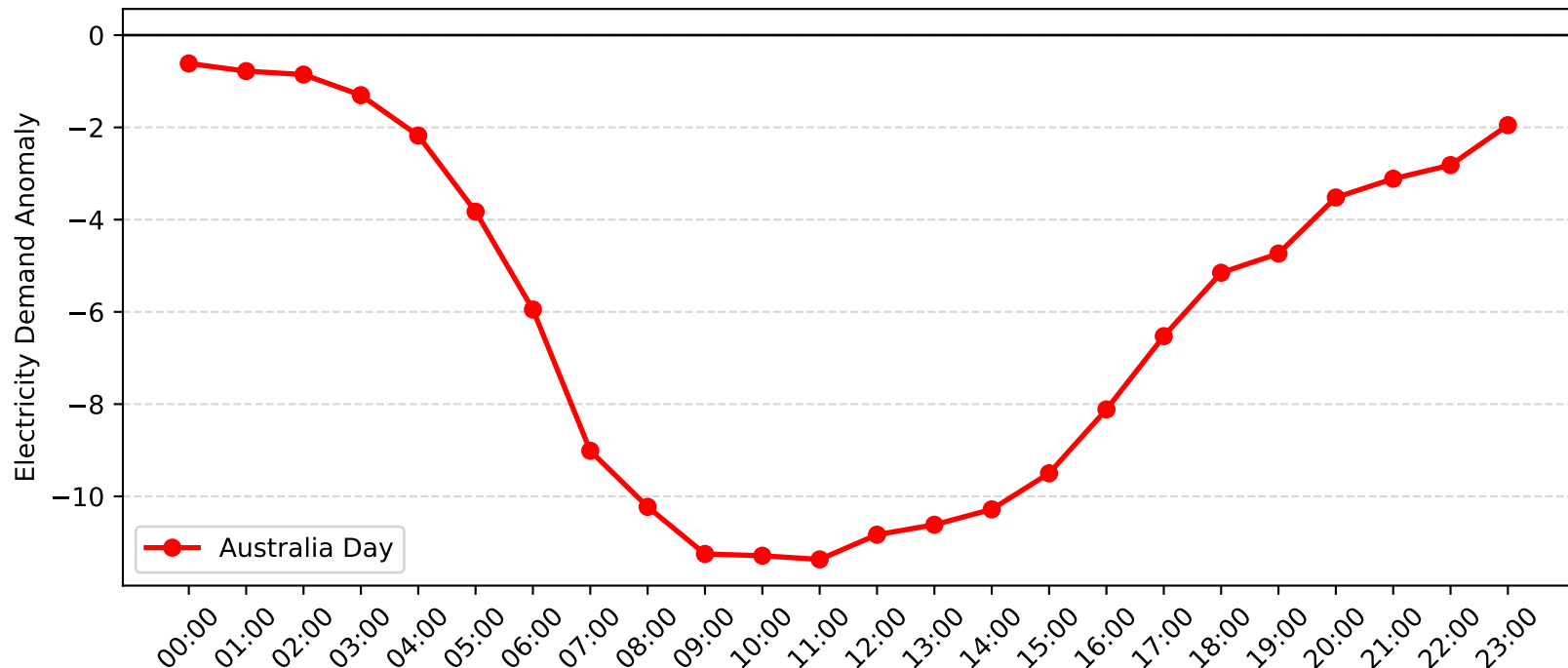
Homebush Bay Demand Anomaly: Australia Day (2008-2009)
