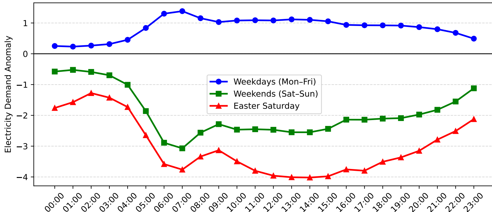
Lisarow Demand Anomaly: Easter Saturday vs Weekday/Weekend (2016-2017)
