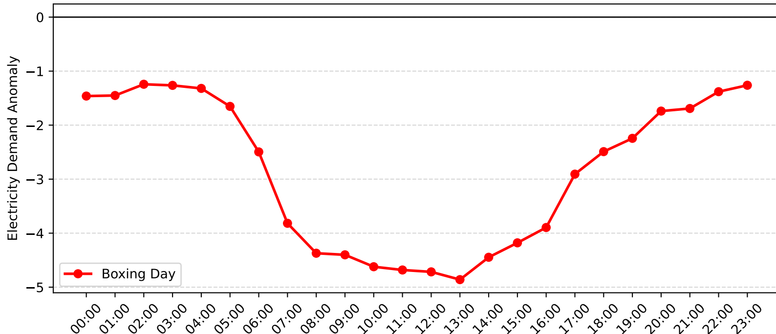
Mayfield West Demand Anomaly: Boxing Day (2011-2012)
