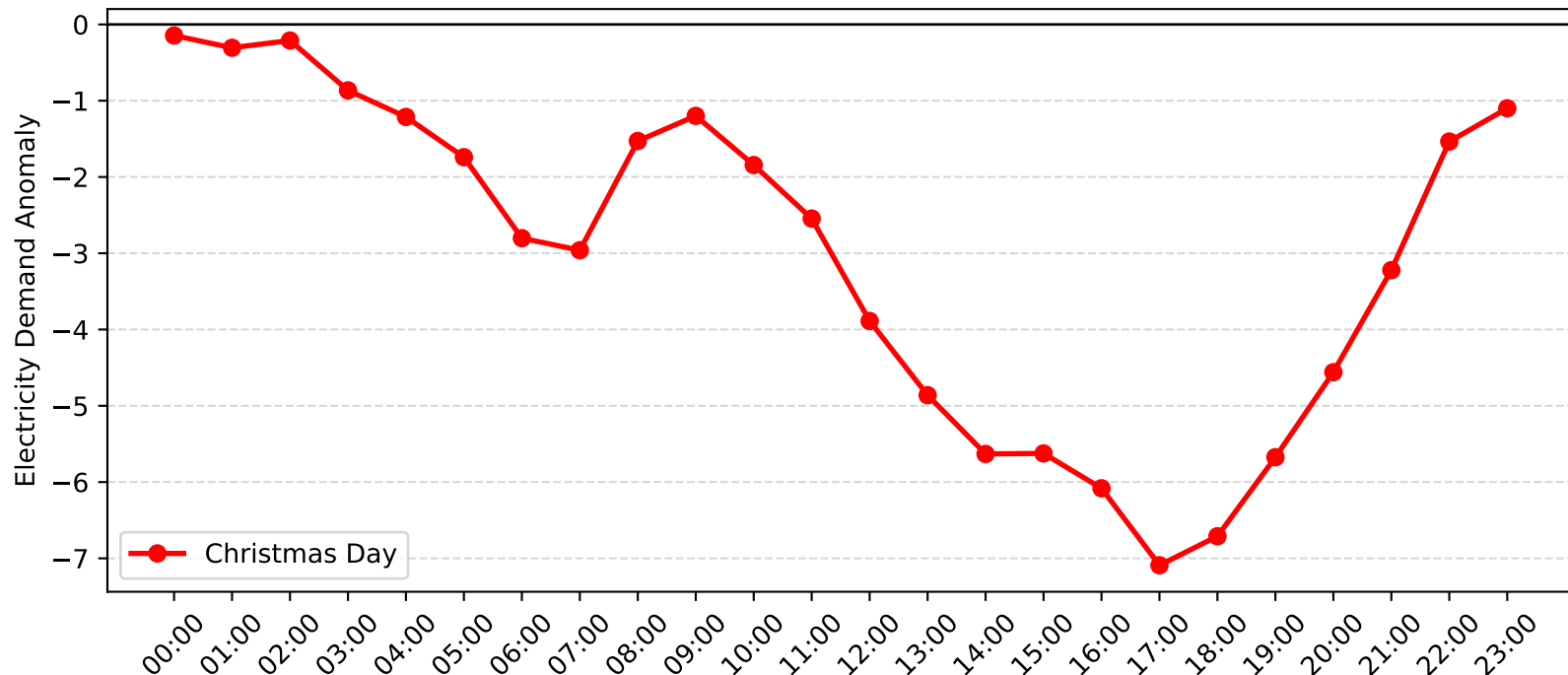
Dee Why West Demand Anomaly: Christmas Day (2006-2007)
