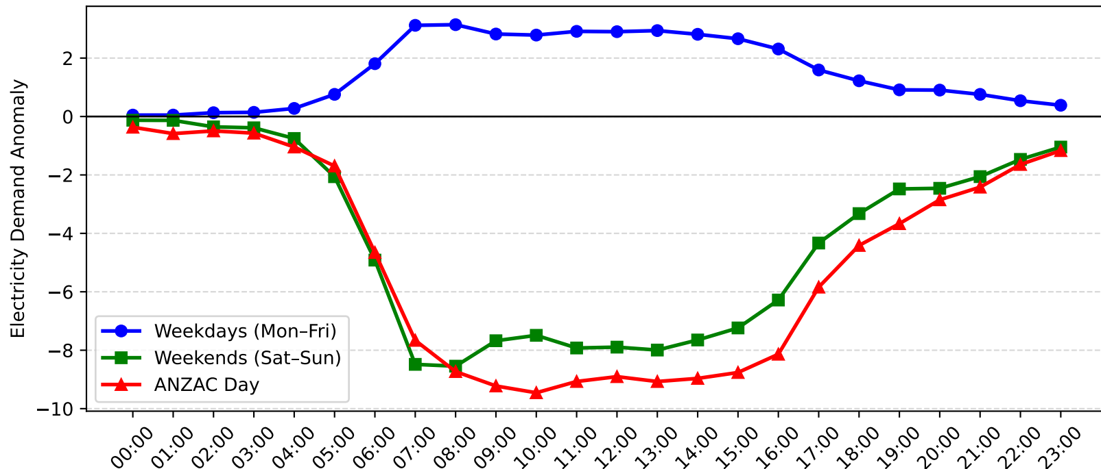
Zetland Demand Anomaly: ANZAC Day vs Weekday/Weekend (2012-2013)
