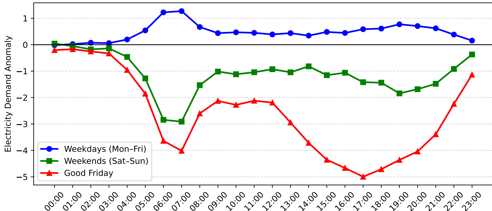
Revesby Demand Anomaly: Good Friday vs Weekday/Weekend (2016-2017)
