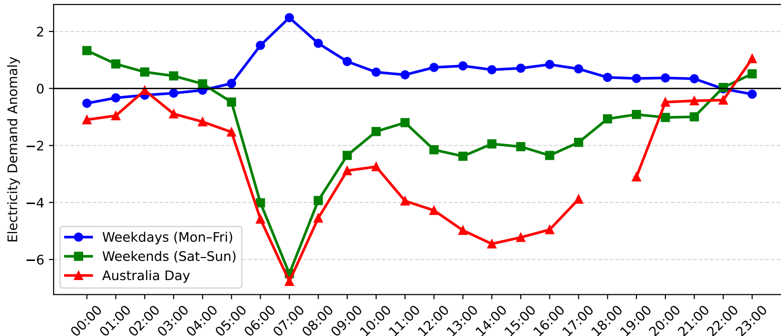
Mosman Demand Anomaly: Australia Day vs Weekday/Weekend (2005-2006)
