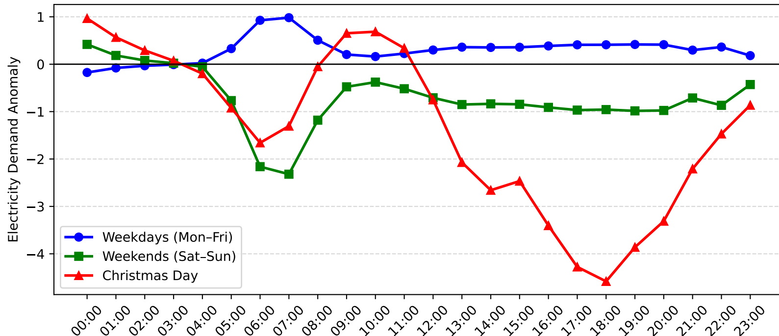
Dee Why West Demand Anomaly: Christmas Day vs Weekday/Weekend (2011-2012)
