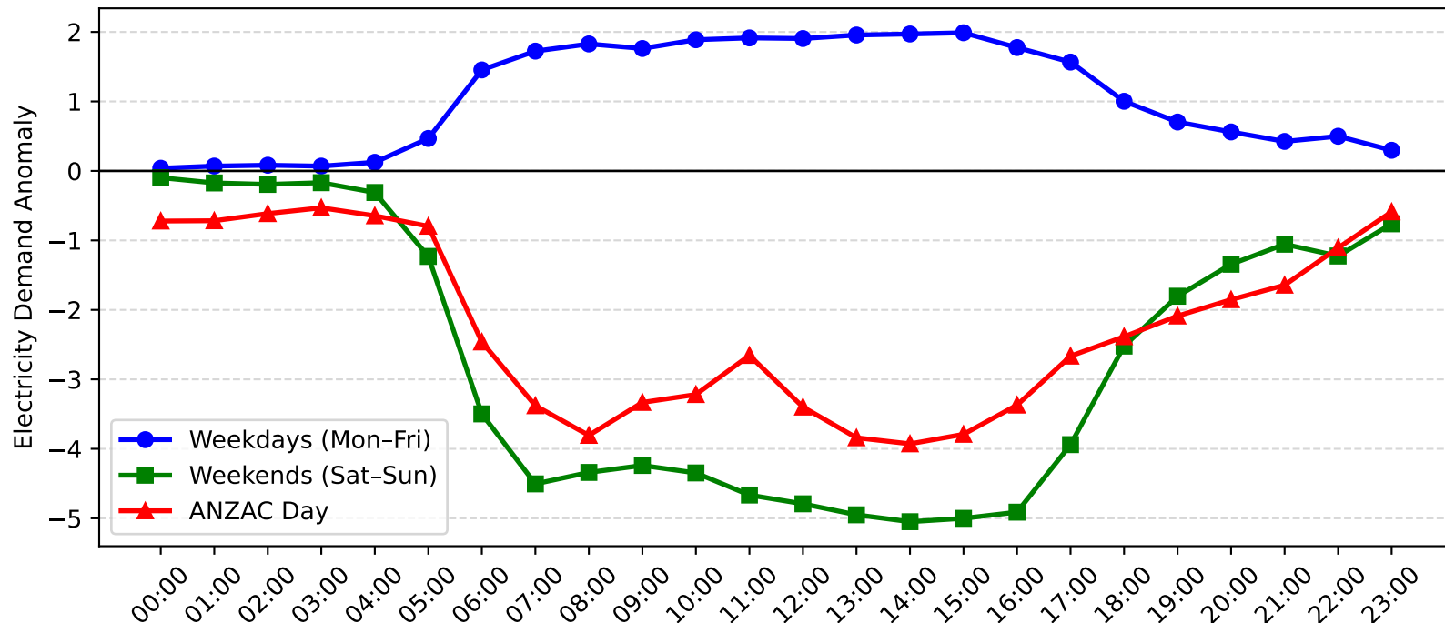
Beacon Hill Demand Anomaly: ANZAC Day vs Weekday/Weekend (2005-2006)
