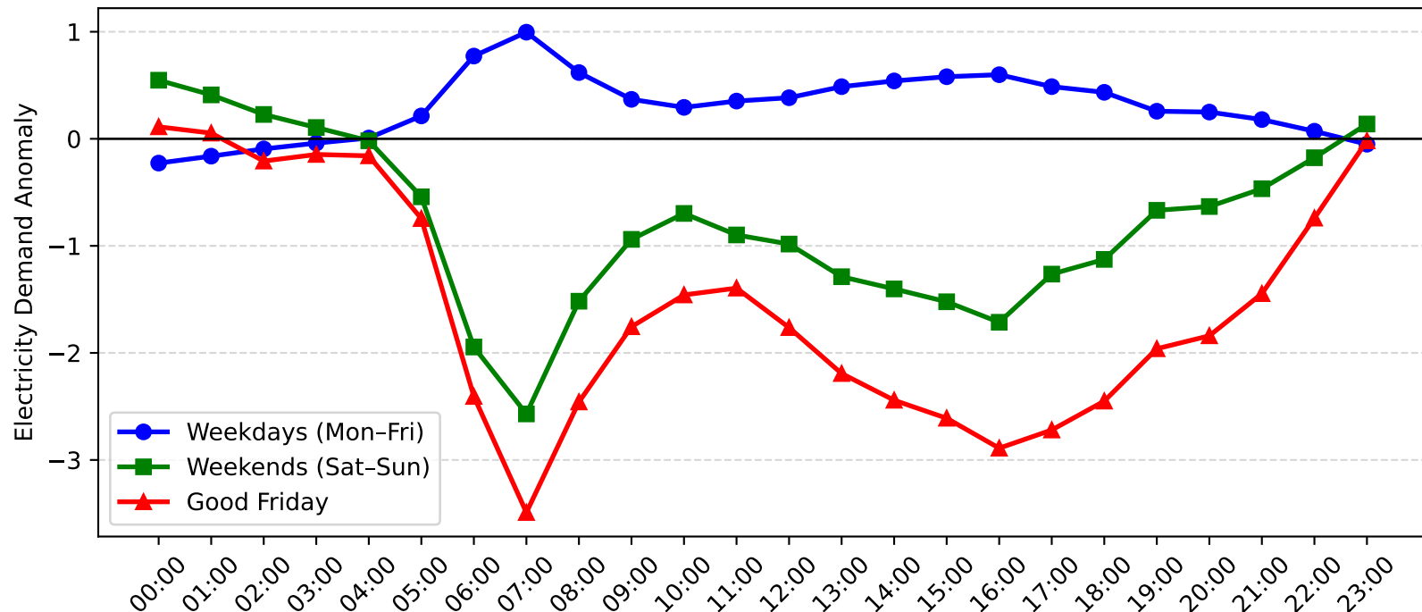
Blakehurst Demand Anomaly: Good Friday vs Weekday/Weekend (2005-2006)
