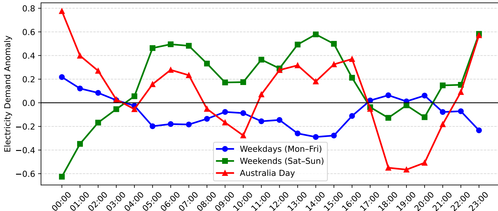
Rutherford Demand Anomaly: Australia Day vs Weekday/Weekend (2004-2005)
