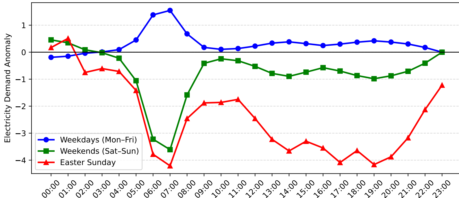
Mortdale Demand Anomaly: Easter Sunday vs Weekday/Weekend (2014-2015)
