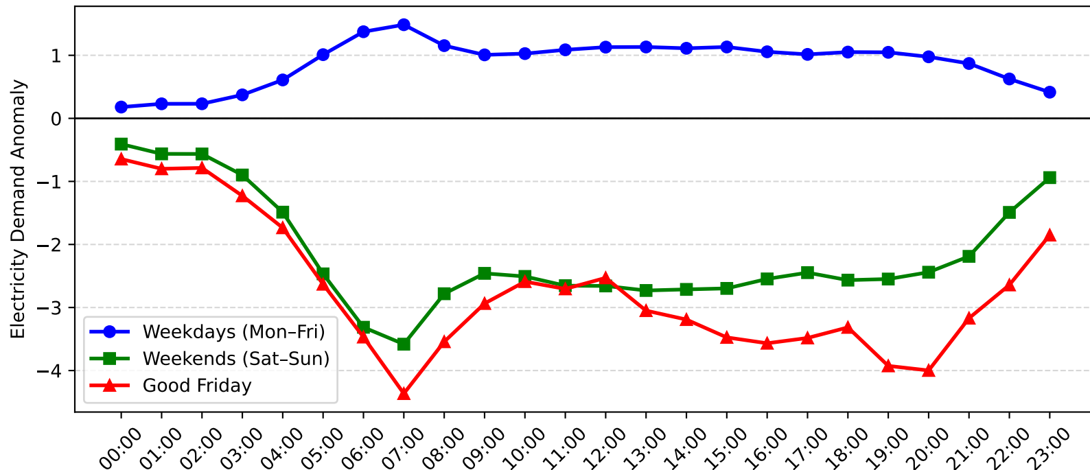
Lisarow Demand Anomaly: Good Friday vs Weekday/Weekend (2008-2009)
