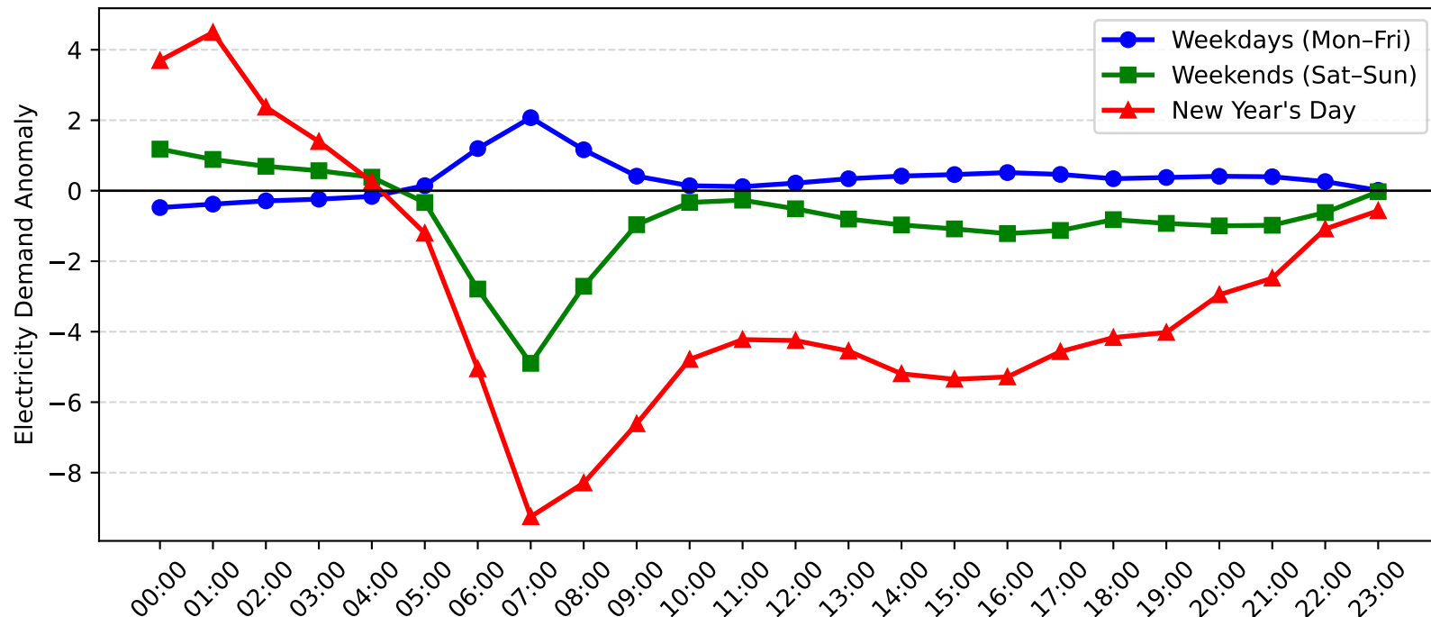
Mosman Demand Anomaly: New Year's Day vs Weekday/Weekend (2012-2013)
