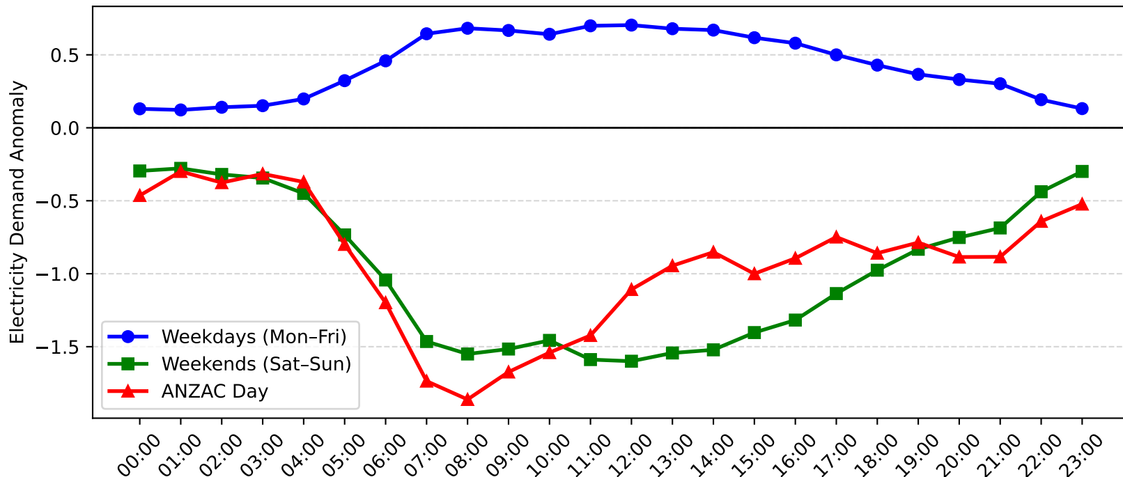
Lidcombe Demand Anomaly: ANZAC Day vs Weekday/Weekend (2017-2018)
