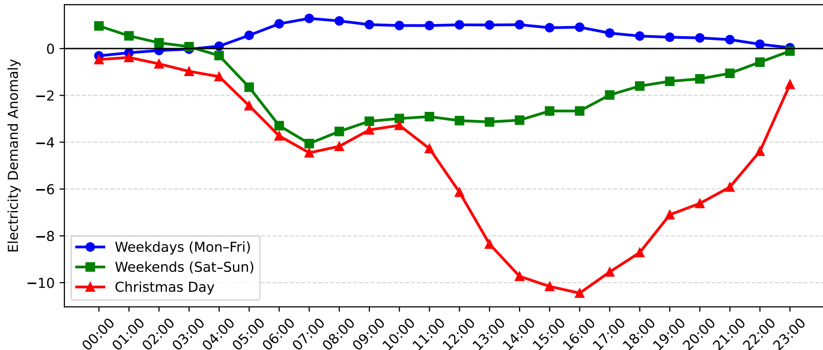
Campsie Demand Anomaly: Christmas Day vs Weekday/Weekend (2013-2014)
