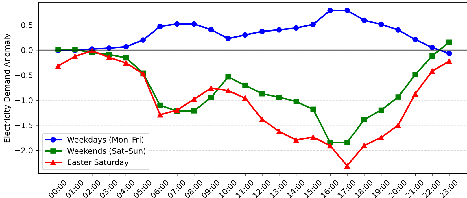
Erina Demand Anomaly: Easter Saturday vs Weekday/Weekend (2014-2015)
