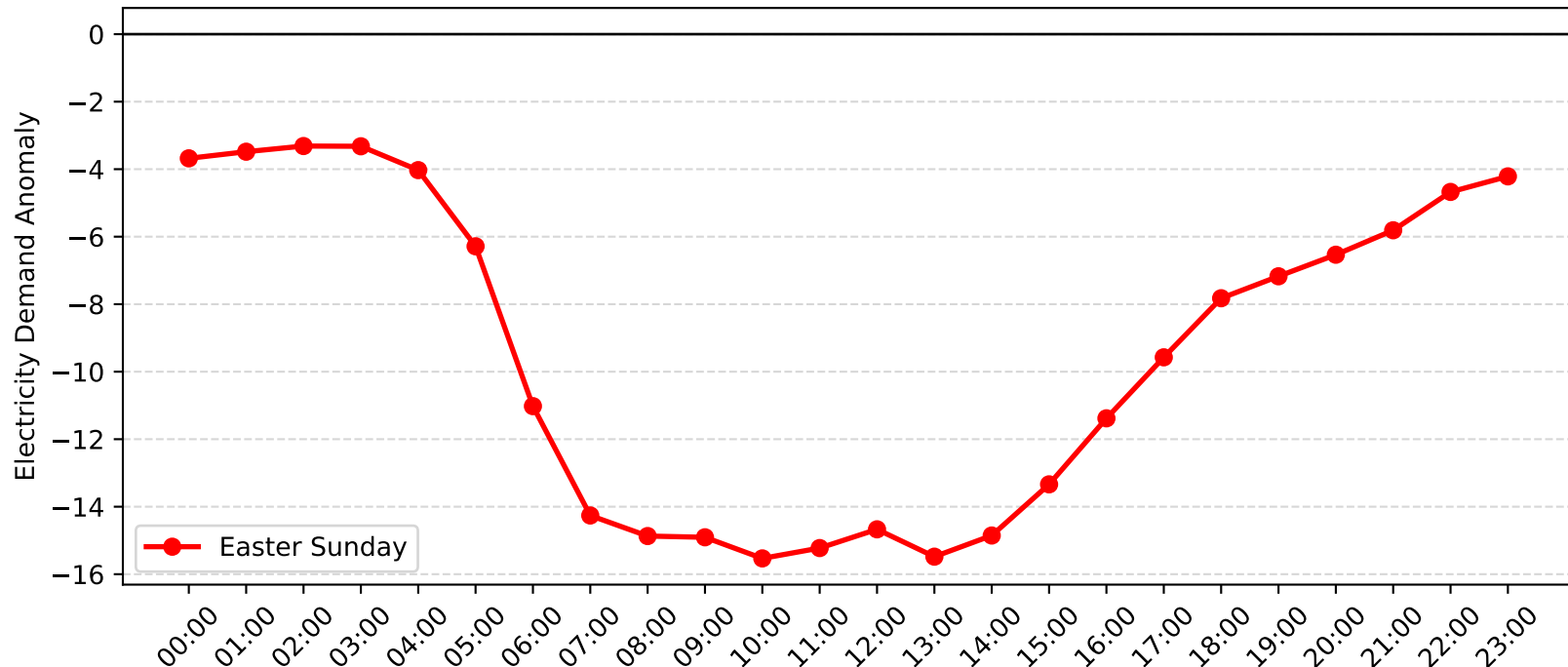
Milperra Demand Anomaly: Easter Sunday (2007-2008)
