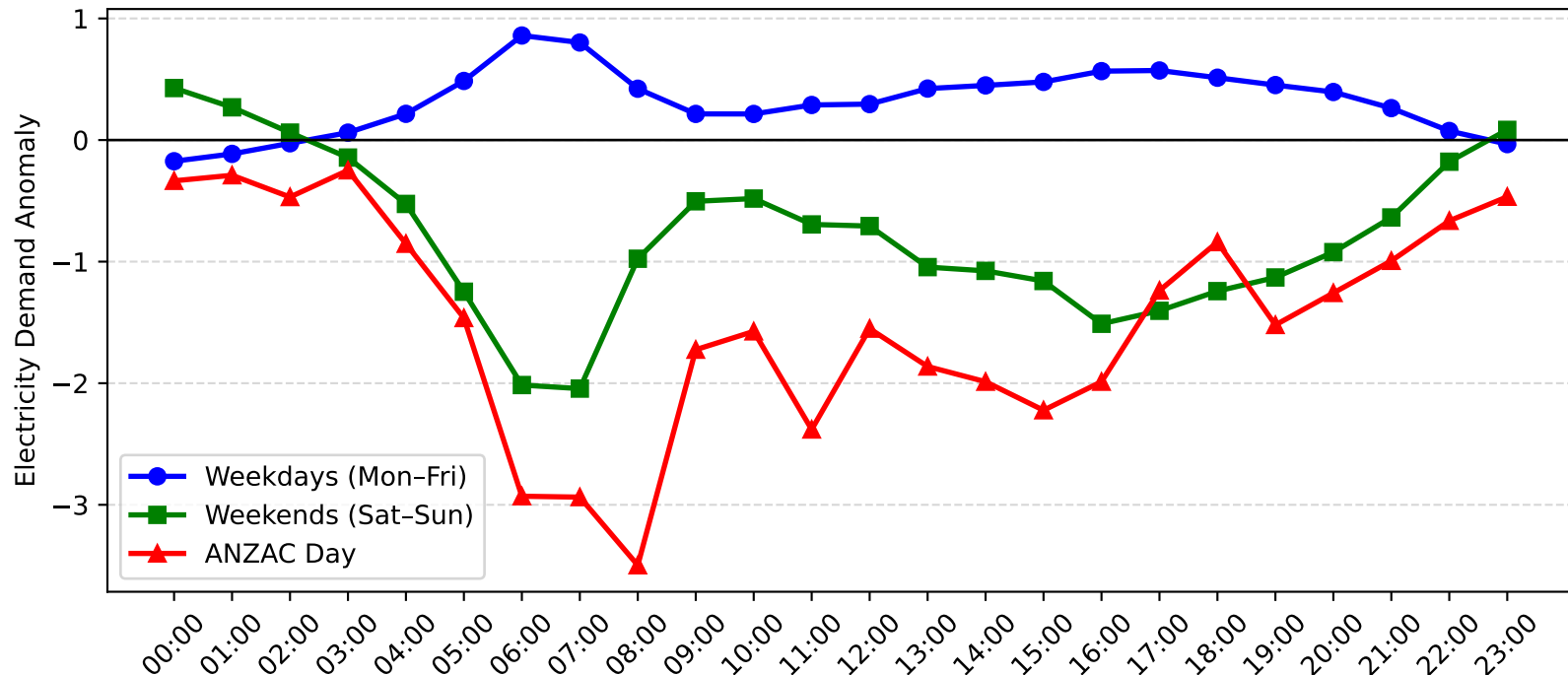
Charmhaven Demand Anomaly: ANZAC Day vs Weekday/Weekend (2005-2006)
