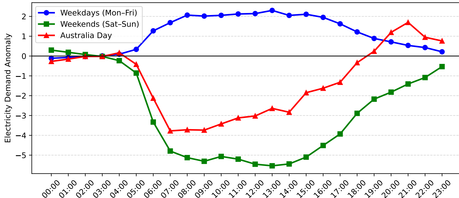
Concord Demand Anomaly: Australia Day vs Weekday/Weekend (2009-2010)
