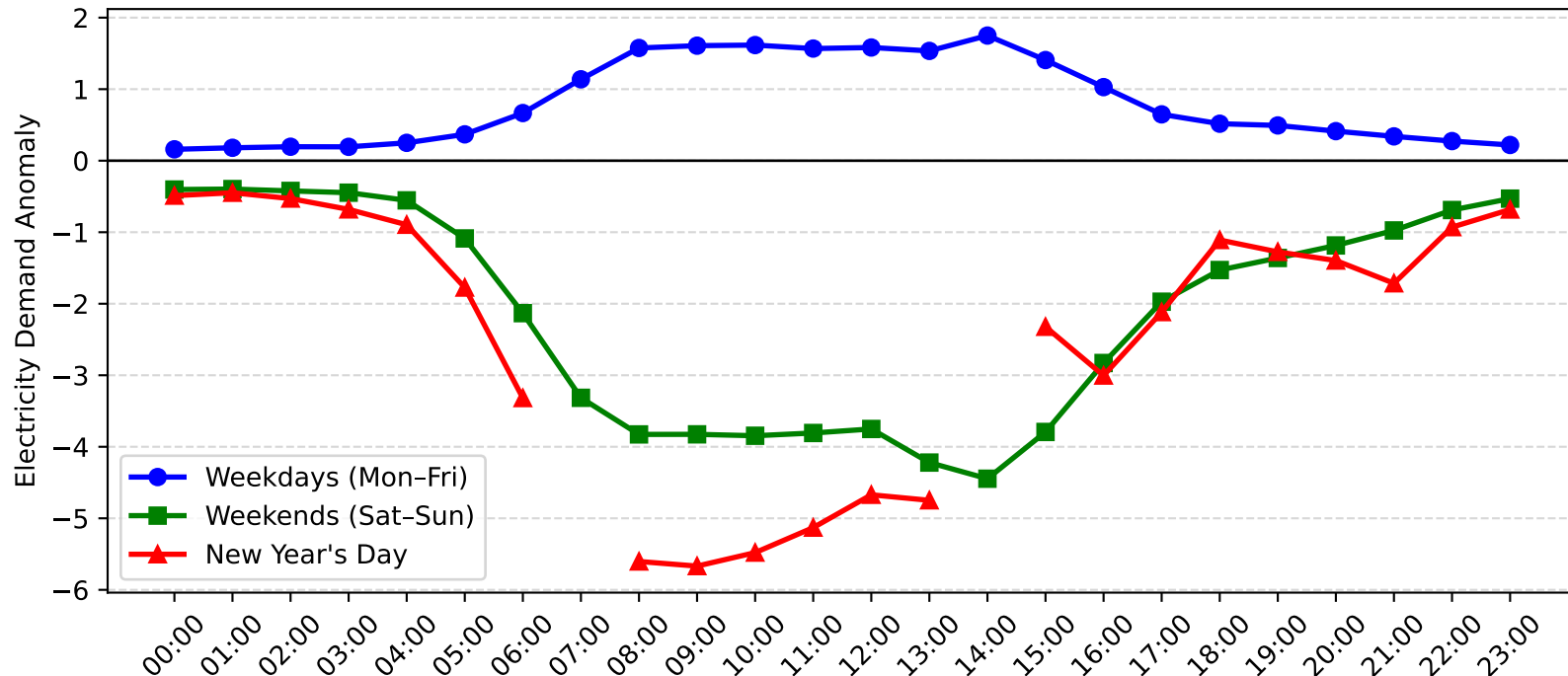
Bankstown Demand Anomaly: New Year's Day vs Weekday/Weekend (2011-2012)
