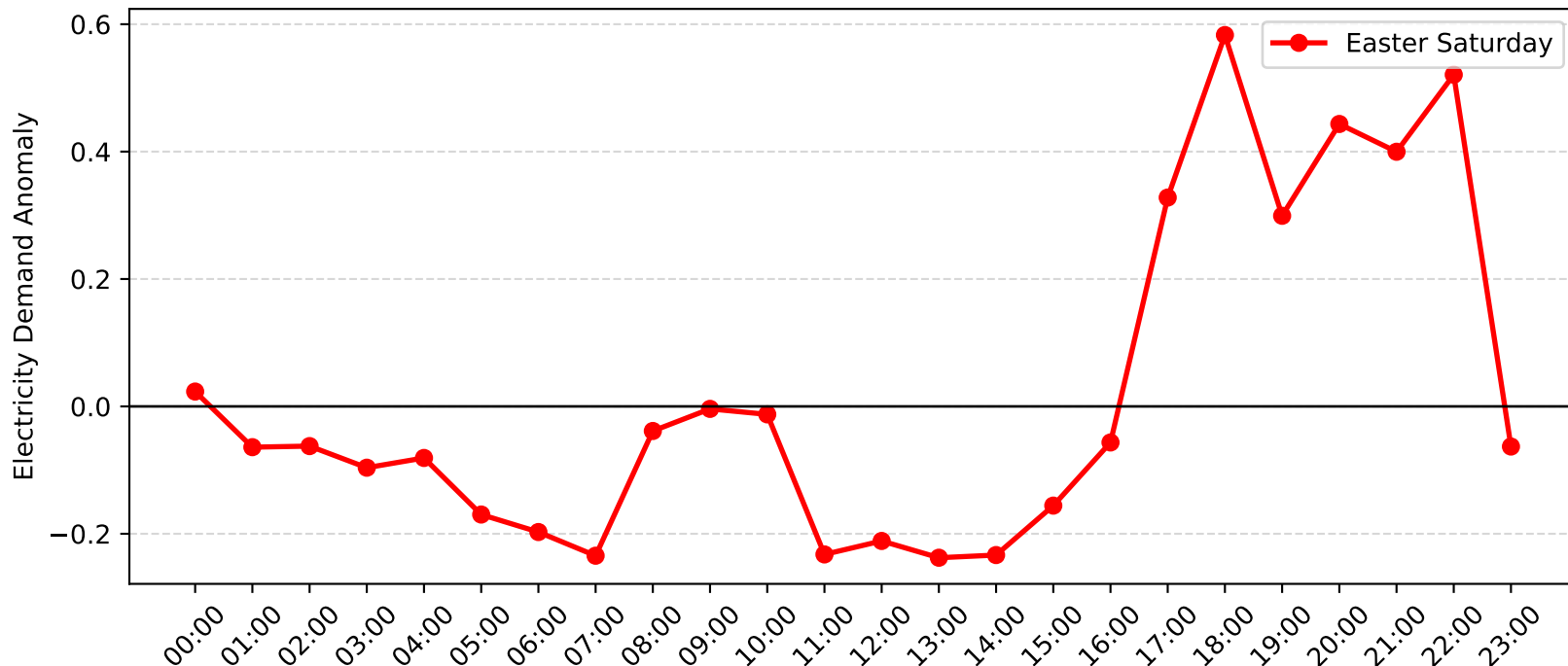
Rothbury Demand Anomaly: Easter Saturday (2008-2009)
