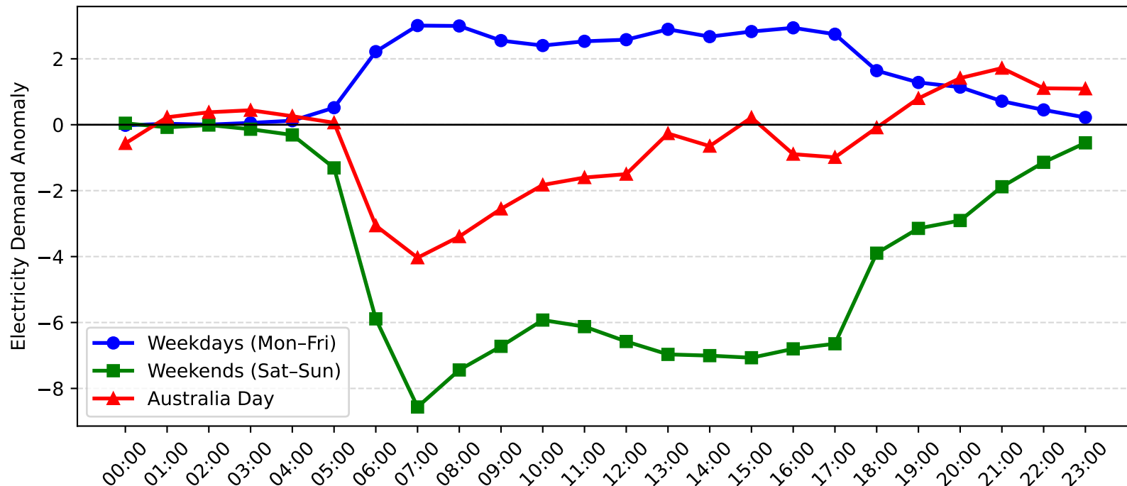
Epping Demand Anomaly: Australia Day vs Weekday/Weekend (2009-2010)
