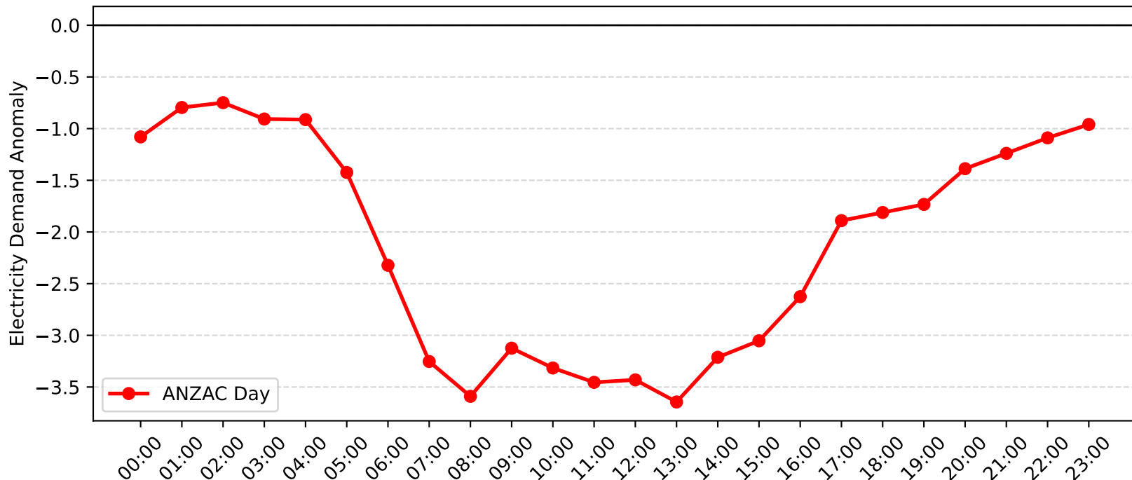
Mayfield West Demand Anomaly: ANZAC Day (2015-2016)
