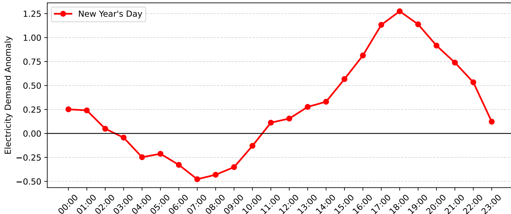
Rothbury Demand Anomaly: New Year's Day (2011-2012)
