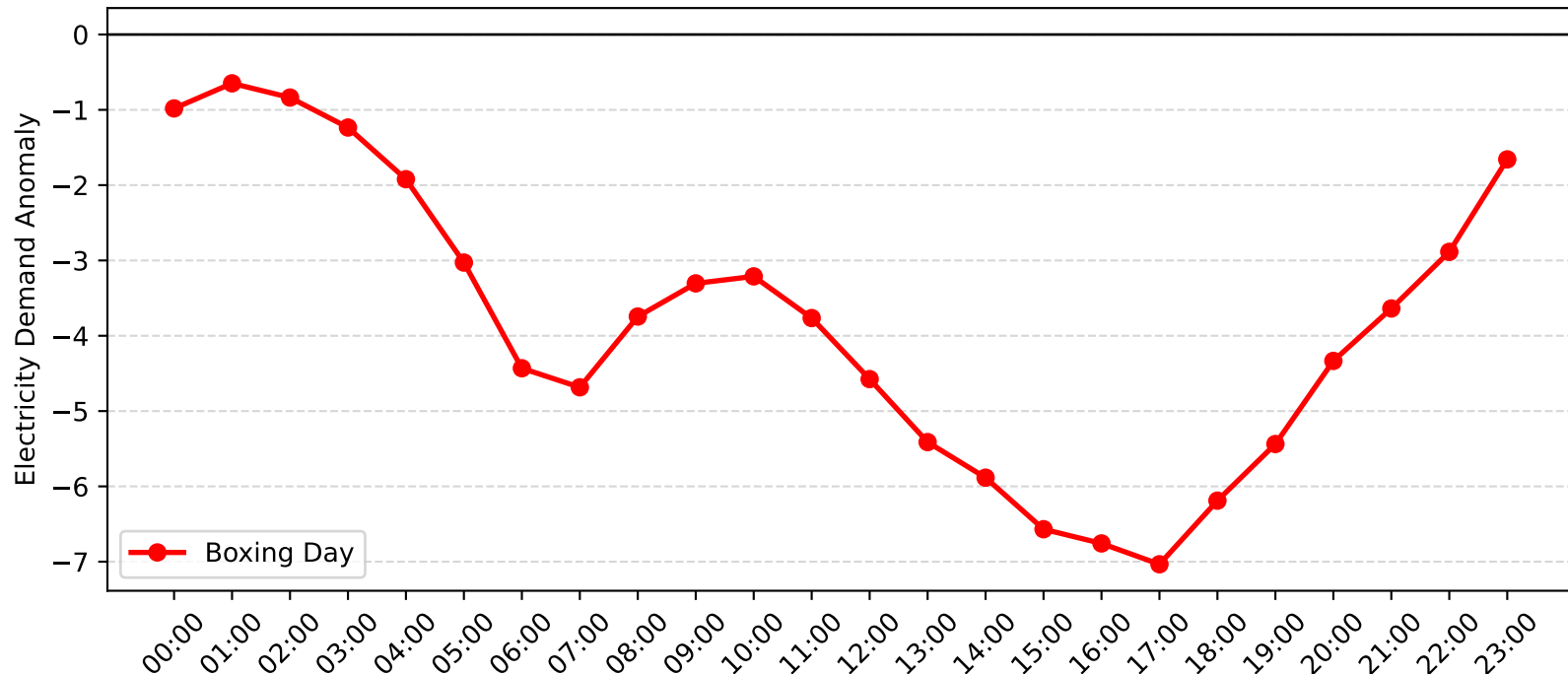
Revesby Demand Anomaly: Boxing Day (2006-2007)
