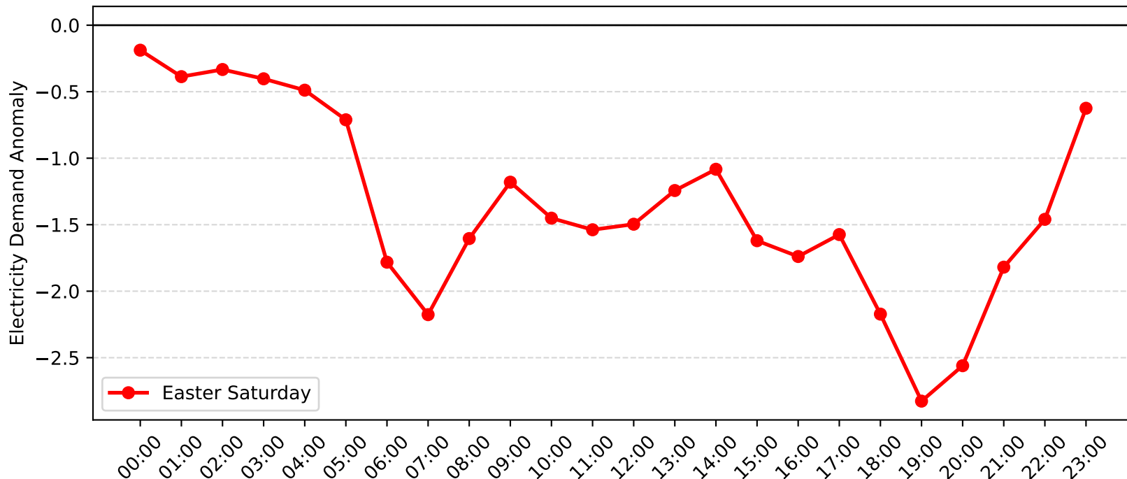
Balgowlah North Demand Anomaly: Easter Saturday (2017-2018)
