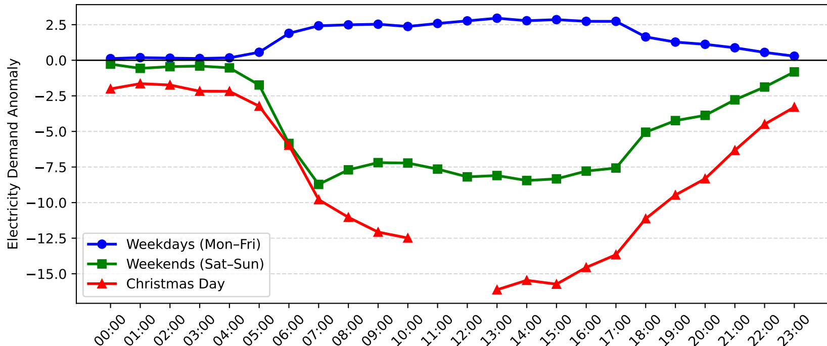
Epping Demand Anomaly: Christmas Day vs Weekday/Weekend (2008-2009)
