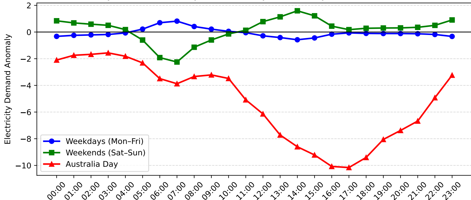
Revesby Demand Anomaly: Australia Day vs Weekday/Weekend (2017-2018)
