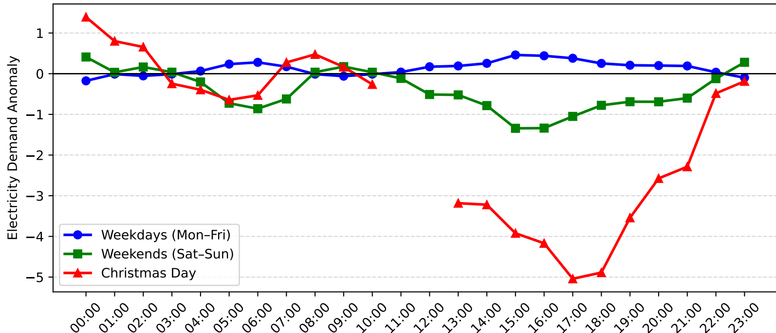
Umina Demand Anomaly: Christmas Day vs Weekday/Weekend (2008-2009)
