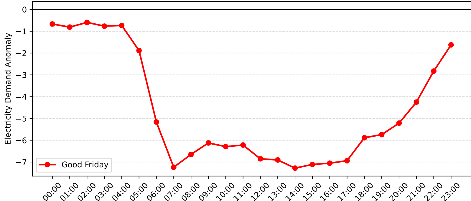
Hunters Hill Demand Anomaly: Good Friday (2009-2010)
