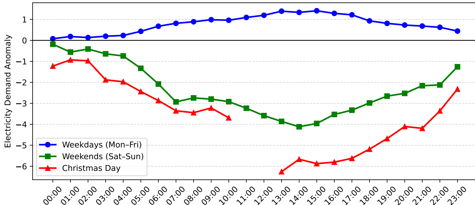
Bass Hill Demand Anomaly: Christmas Day vs Weekday/Weekend (2008-2009)
