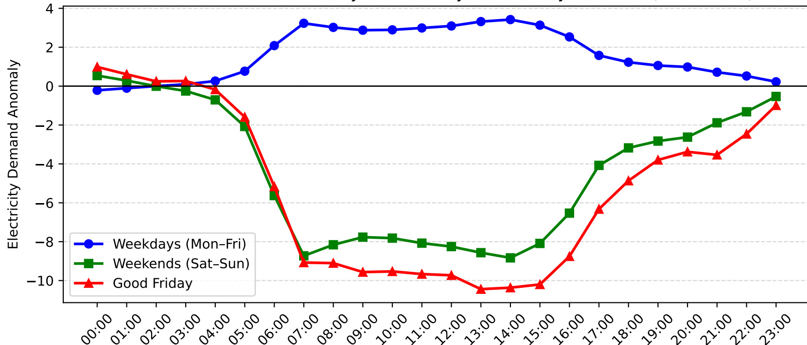
Marrickville Demand Anomaly: Good Friday vs Weekday/Weekend (2007-2008)
