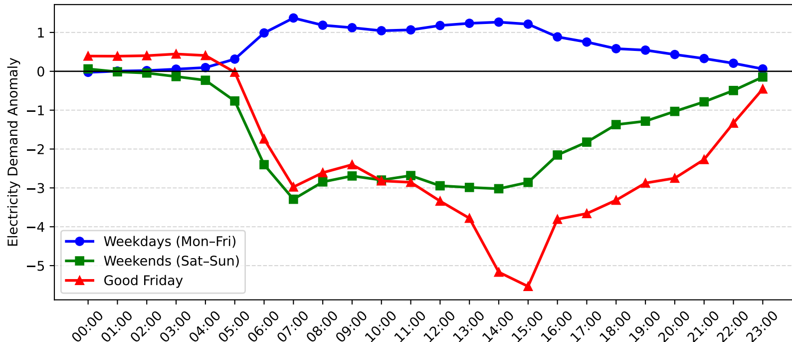
Hunters Hill Demand Anomaly: Good Friday vs Weekday/Weekend (2016-2017)
