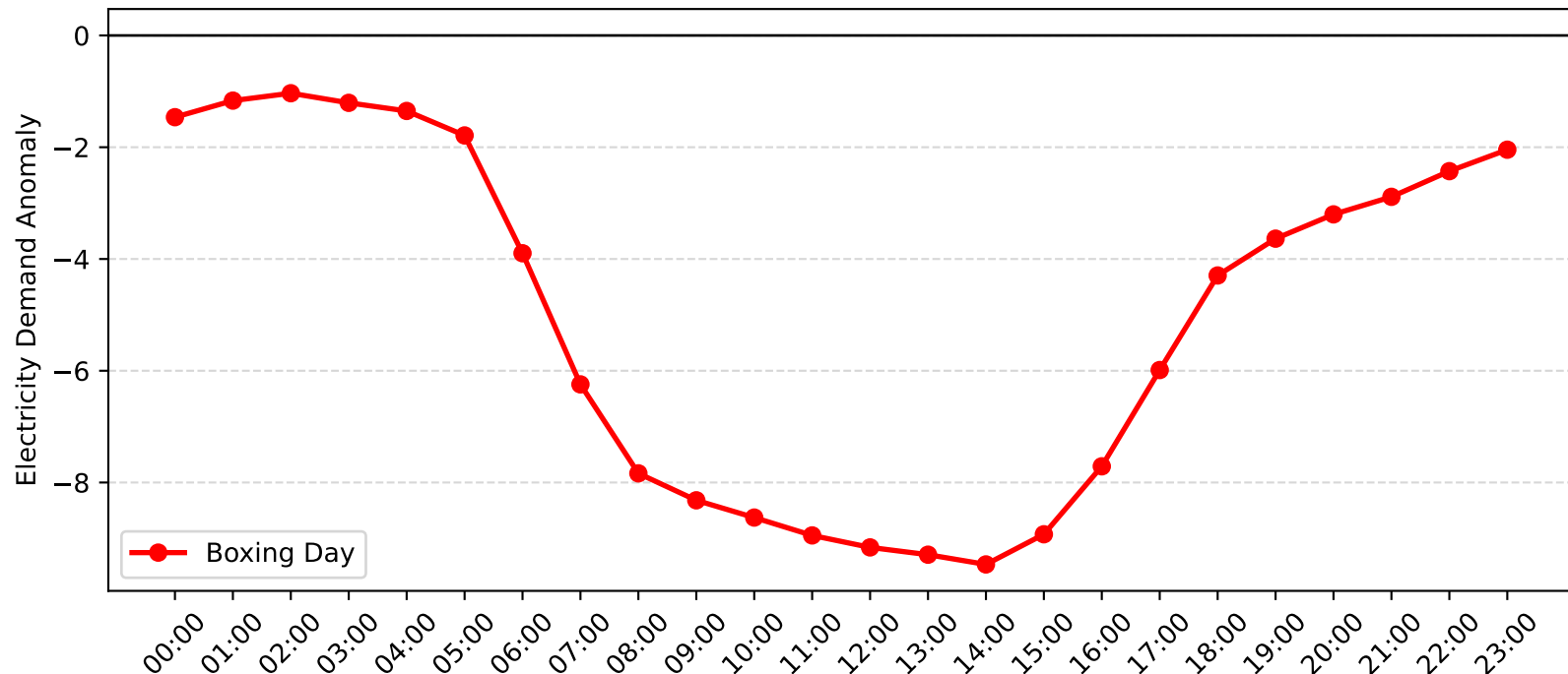
Mascot Demand Anomaly: Boxing Day (2011-2012)
