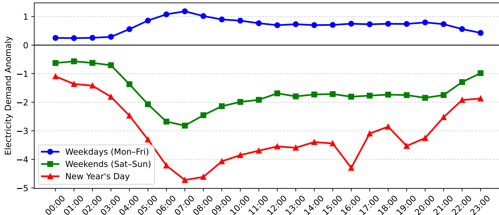
Lisarow Demand Anomaly: New Year's Day vs Weekday/Weekend (2007-2008)
