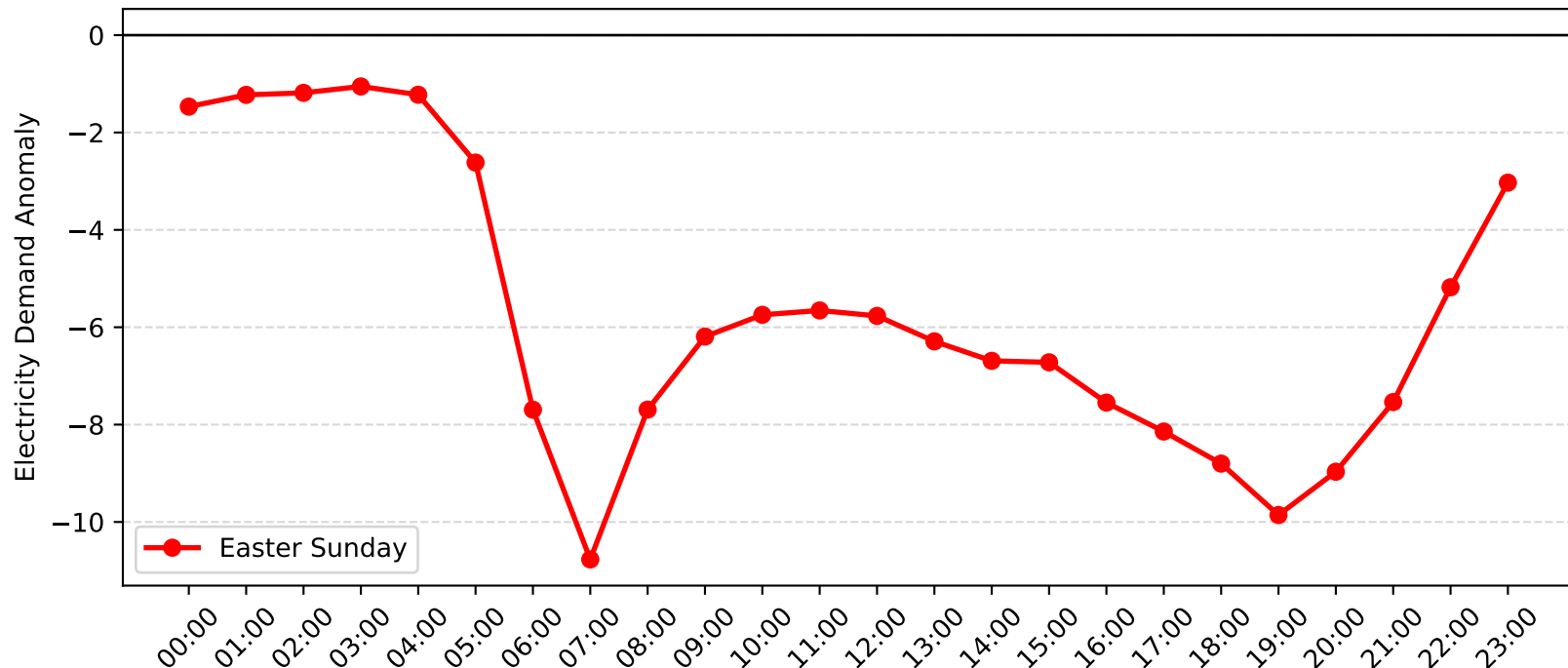
Mosman Demand Anomaly: Easter Sunday (2011-2012)
