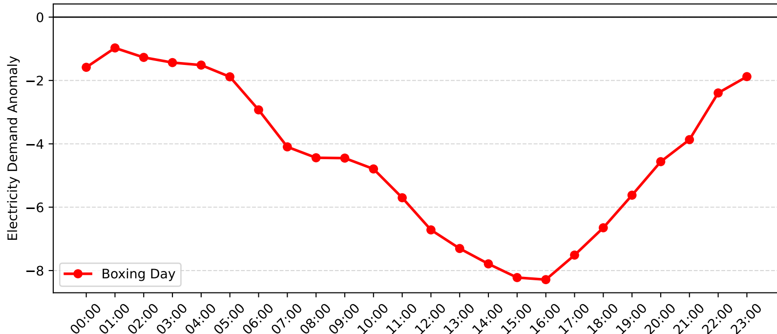
Jesmond Demand Anomaly: Boxing Day (2012-2013)
