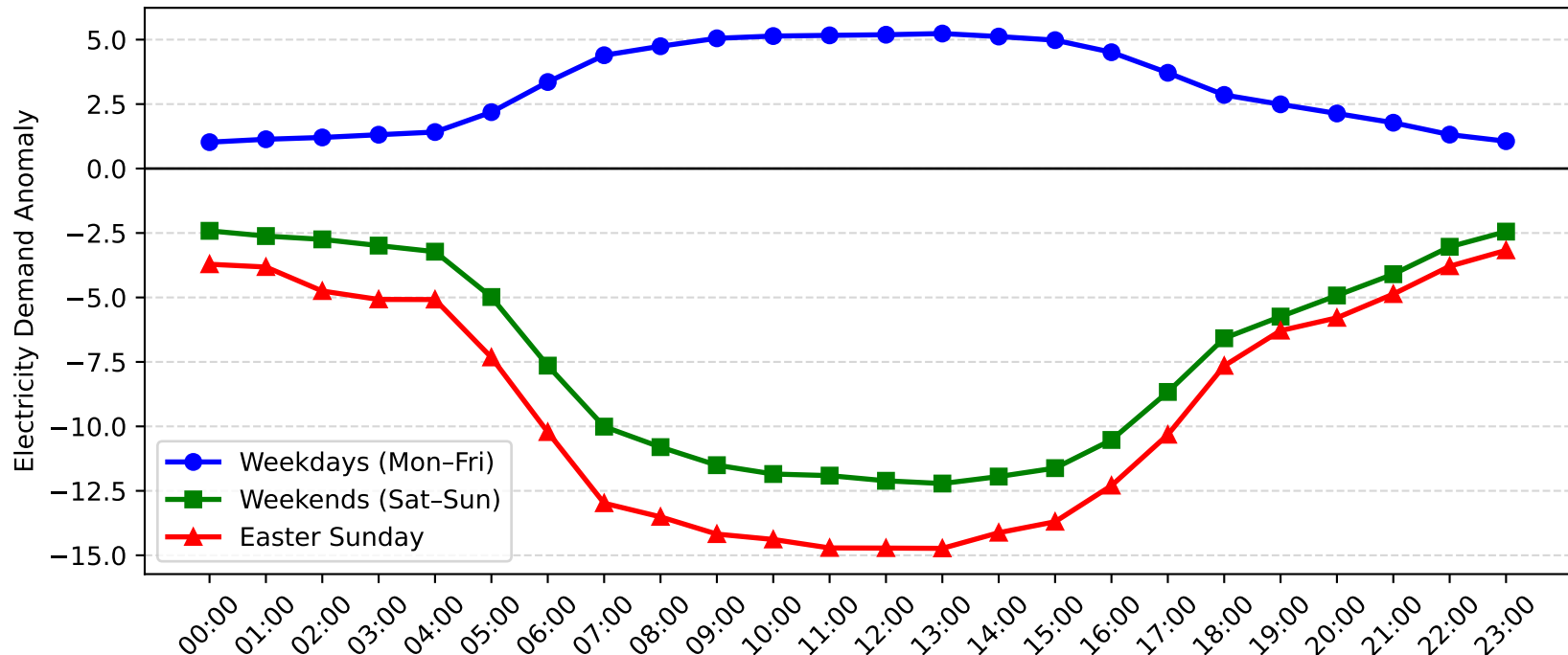
Flemington Demand Anomaly: Easter Sunday vs Weekday/Weekend (2015-2016)
