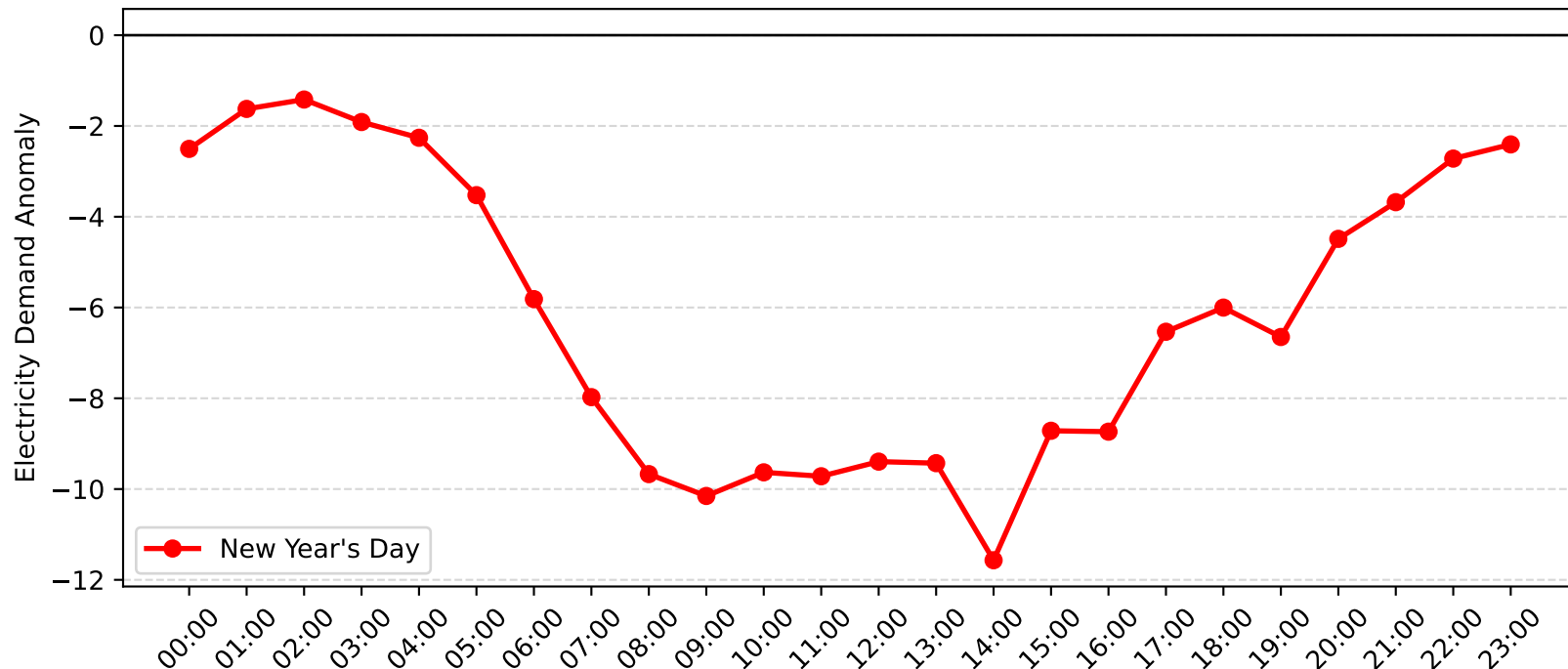
Maroubra Demand Anomaly: New Year's Day (2007-2008)
