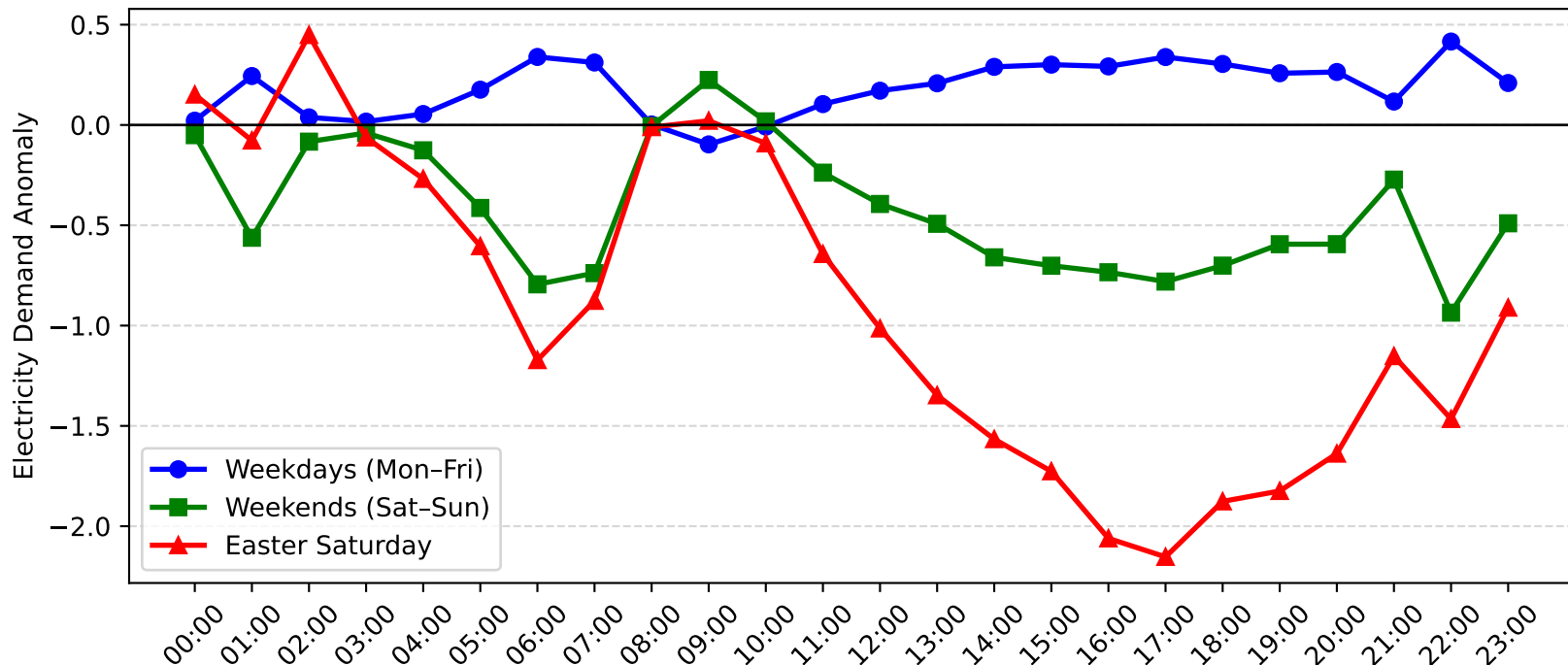
Maryland Demand Anomaly: Easter Saturday vs Weekday/Weekend (2006-2007)
