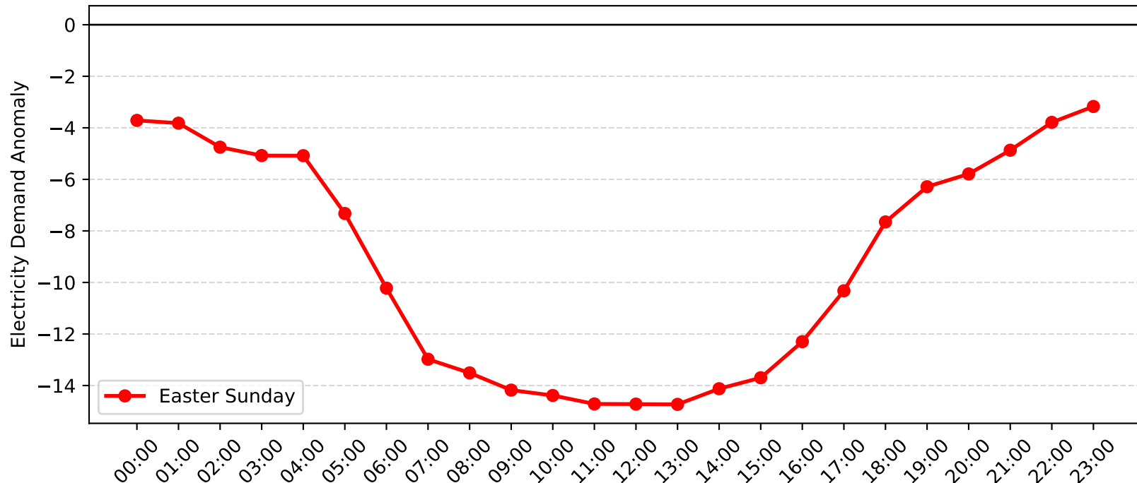
Flemington Demand Anomaly: Easter Sunday (2015-2016)
