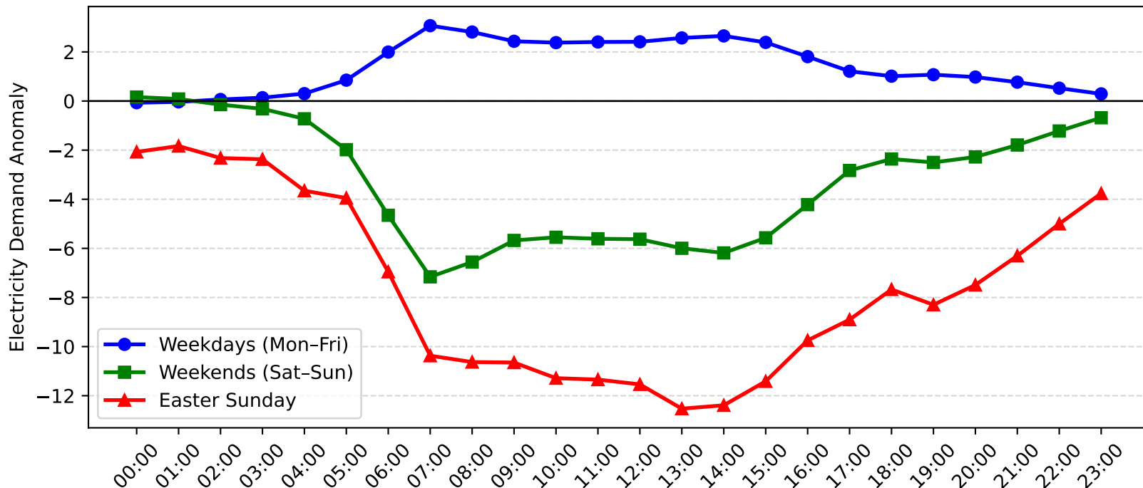
Marrickville Demand Anomaly: Easter Sunday vs Weekday/Weekend (2014-2015)
