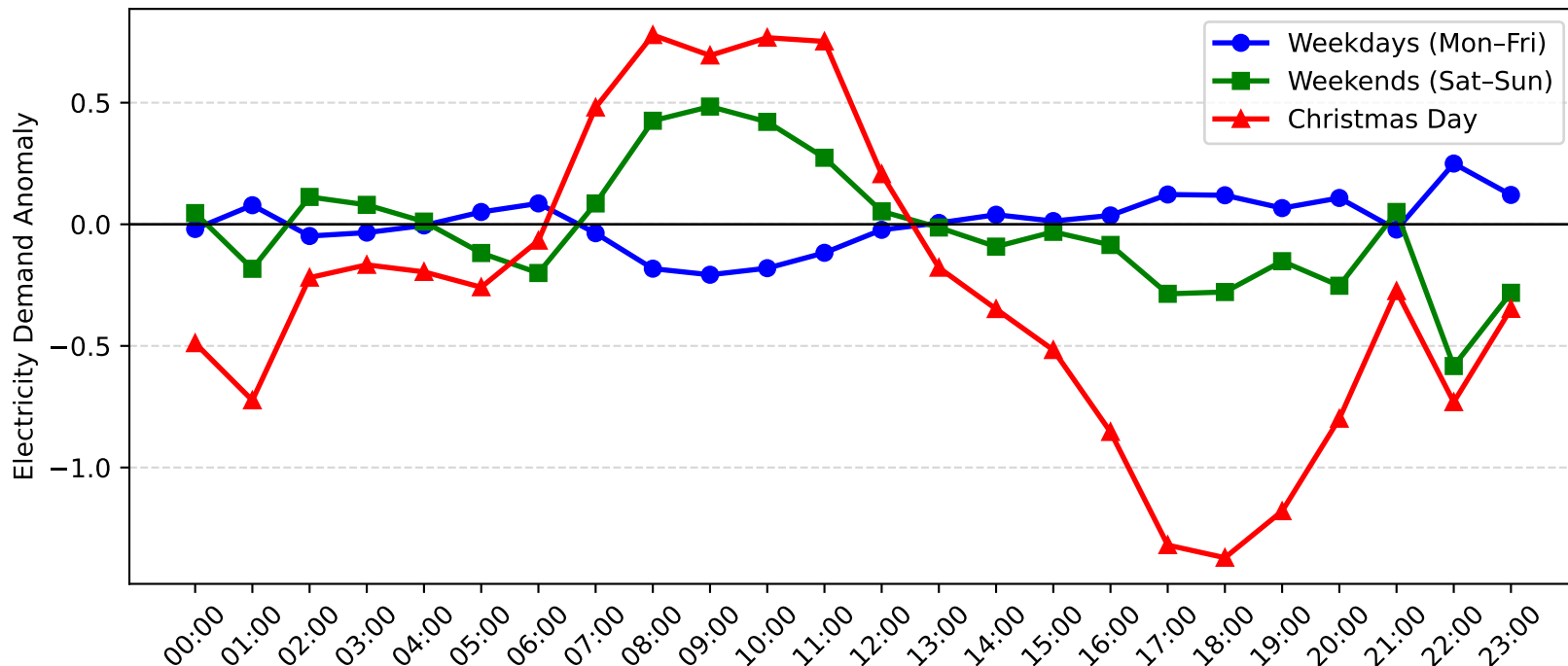
Swansea Demand Anomaly: Christmas Day vs Weekday/Weekend (2016-2017)
