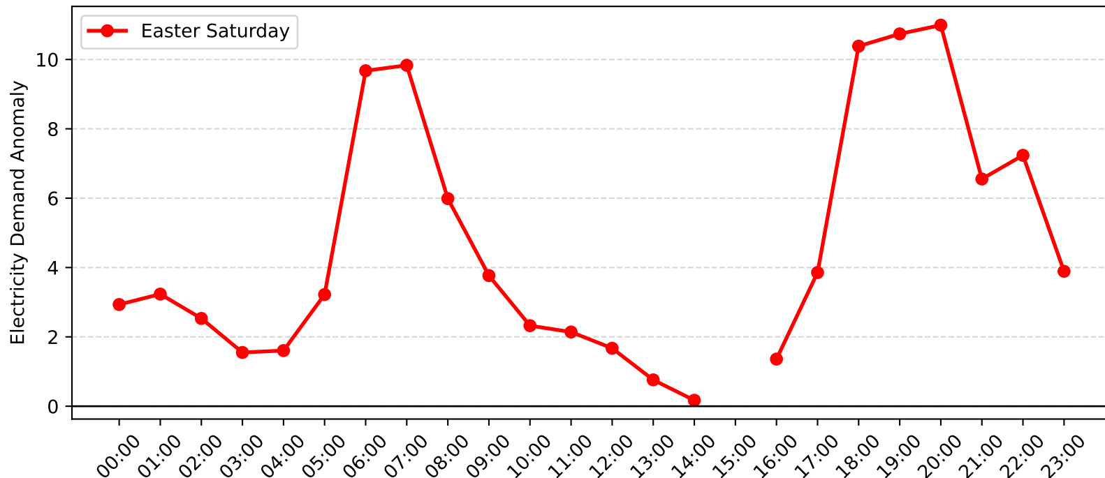
Mortdale Demand Anomaly: Easter Saturday (2004-2005)
