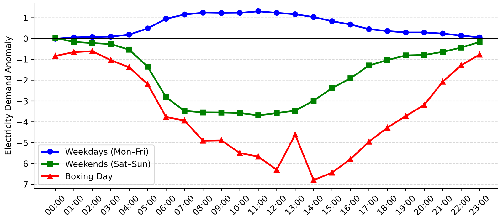
Wyong Demand Anomaly: Boxing Day vs Weekday/Weekend (2013-2014)
