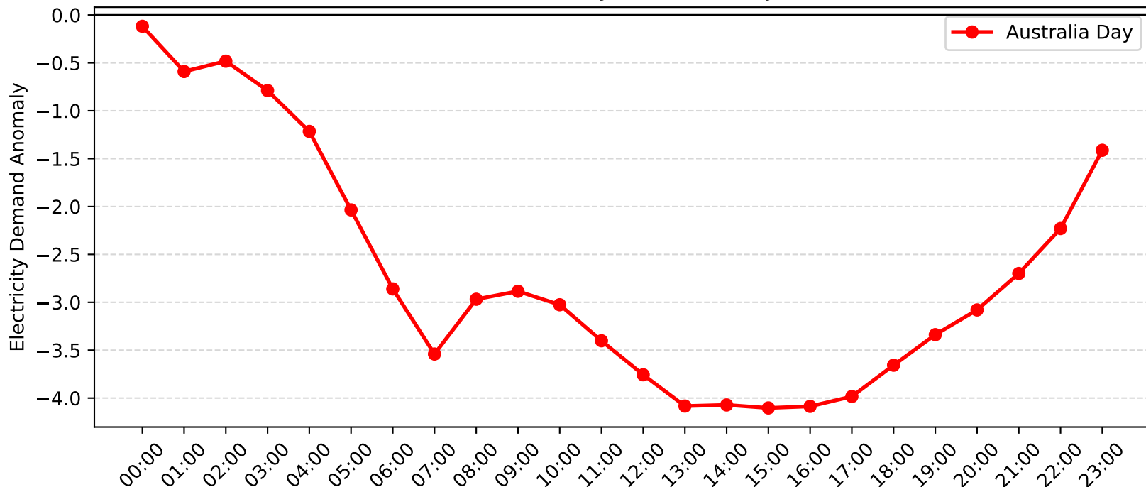
Lisarow Demand Anomaly: Australia Day (2008-2009)
