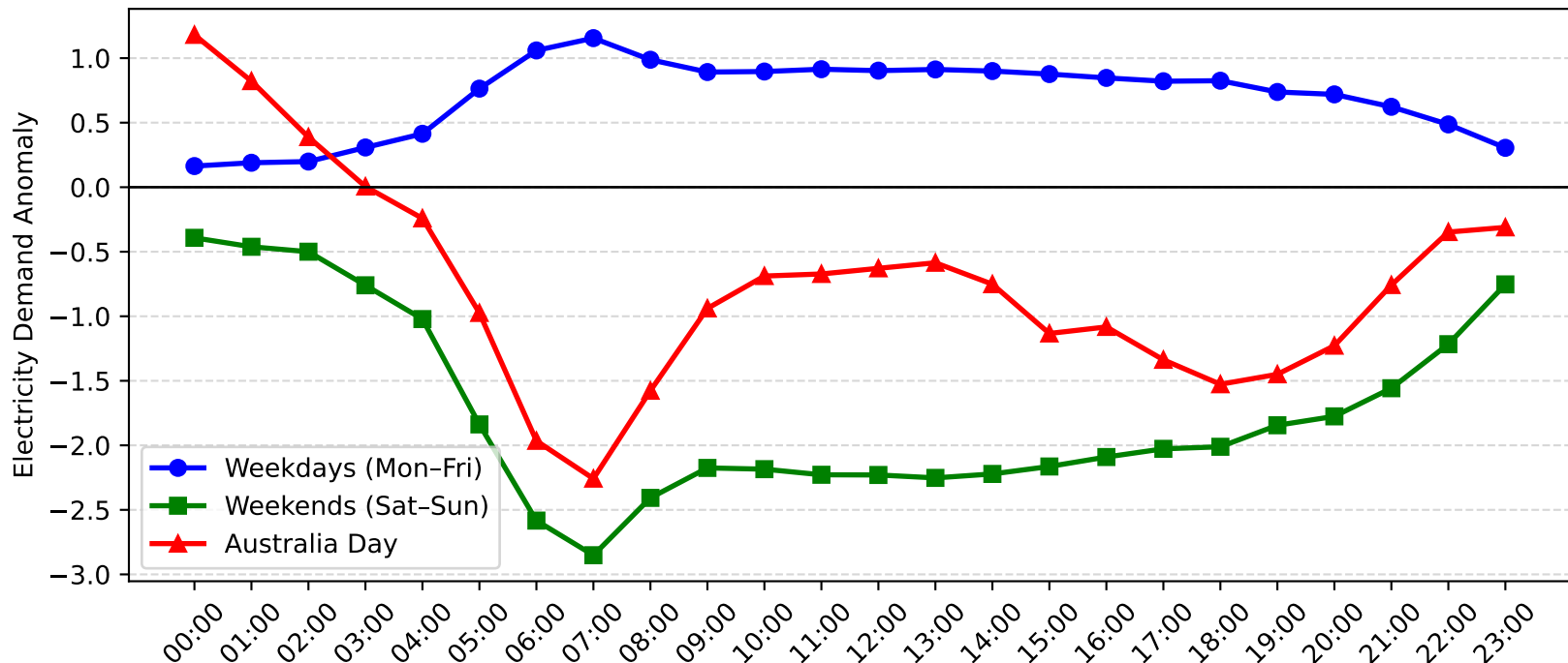
Lisarow Demand Anomaly: Australia Day vs Weekday/Weekend (2012-2013)
