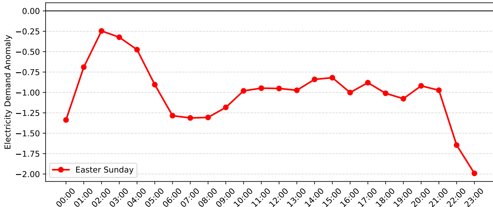
Muswellbrook Demand Anomaly: Easter Sunday (2011-2012)
