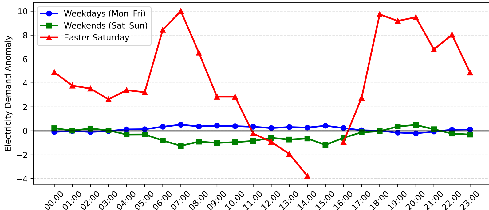
Meadowbank Demand Anomaly: Easter Saturday vs Weekday/Weekend (2004-2005)
