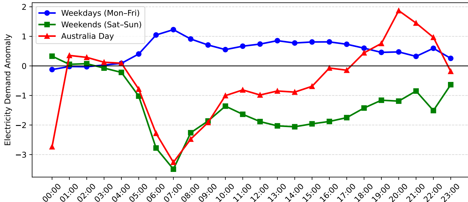
Dee Why West Demand Anomaly: Australia Day vs Weekday/Weekend (2009-2010)
