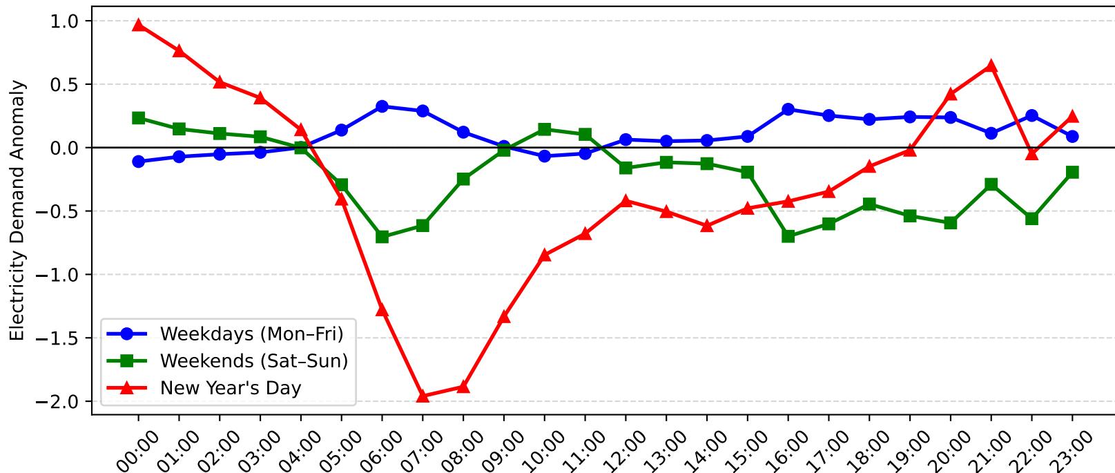
Narrabeen Demand Anomaly: New Year's Day vs Weekday/Weekend (2005-2006)
