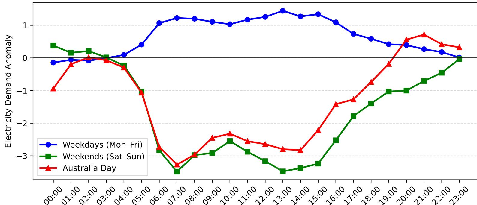
Kirrawee Demand Anomaly: Australia Day vs Weekday/Weekend (2009-2010)
