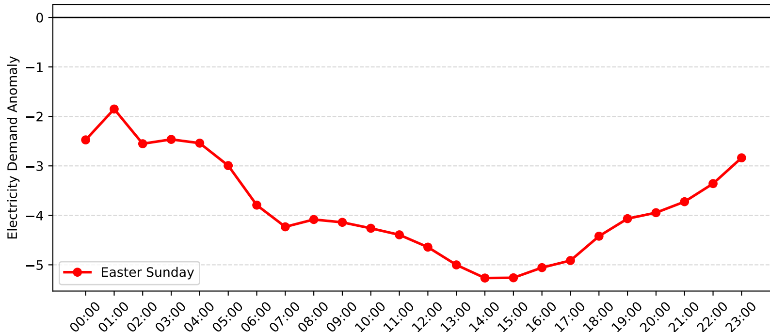
Bass Hill Demand Anomaly: Easter Sunday (2015-2016)
