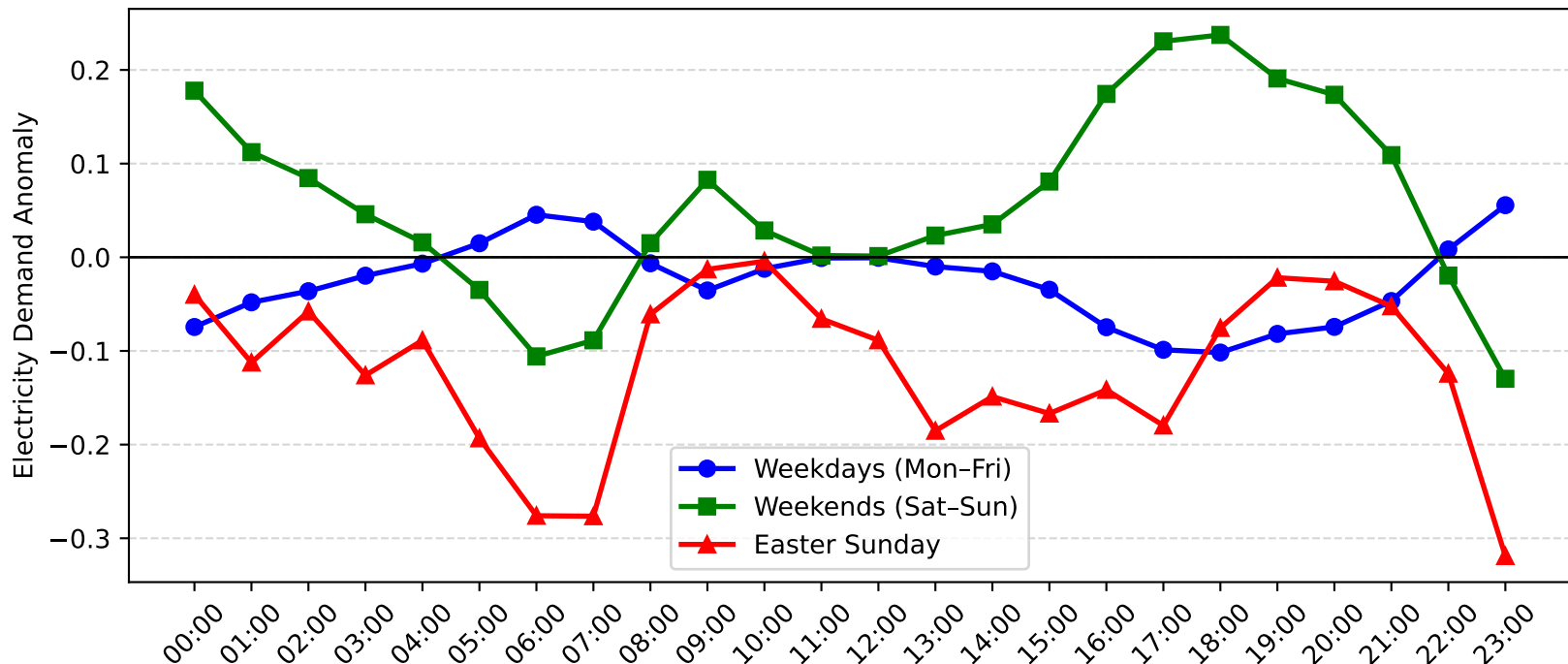
Rothbury Demand Anomaly: Easter Sunday vs Weekday/Weekend (2013-2014)
