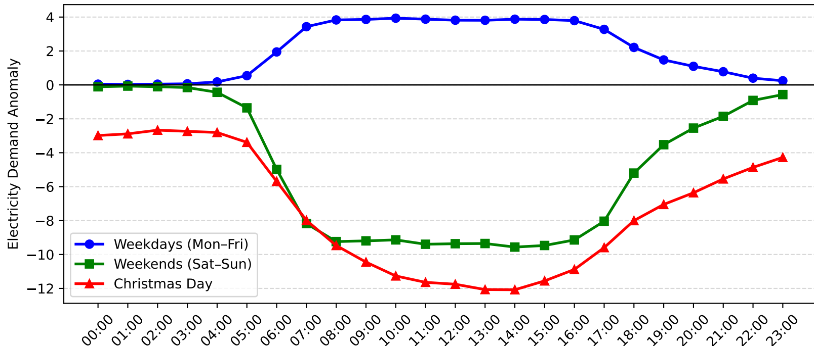
Macquarie Park Demand Anomaly: Christmas Day vs Weekday/Weekend (2006-2007)
