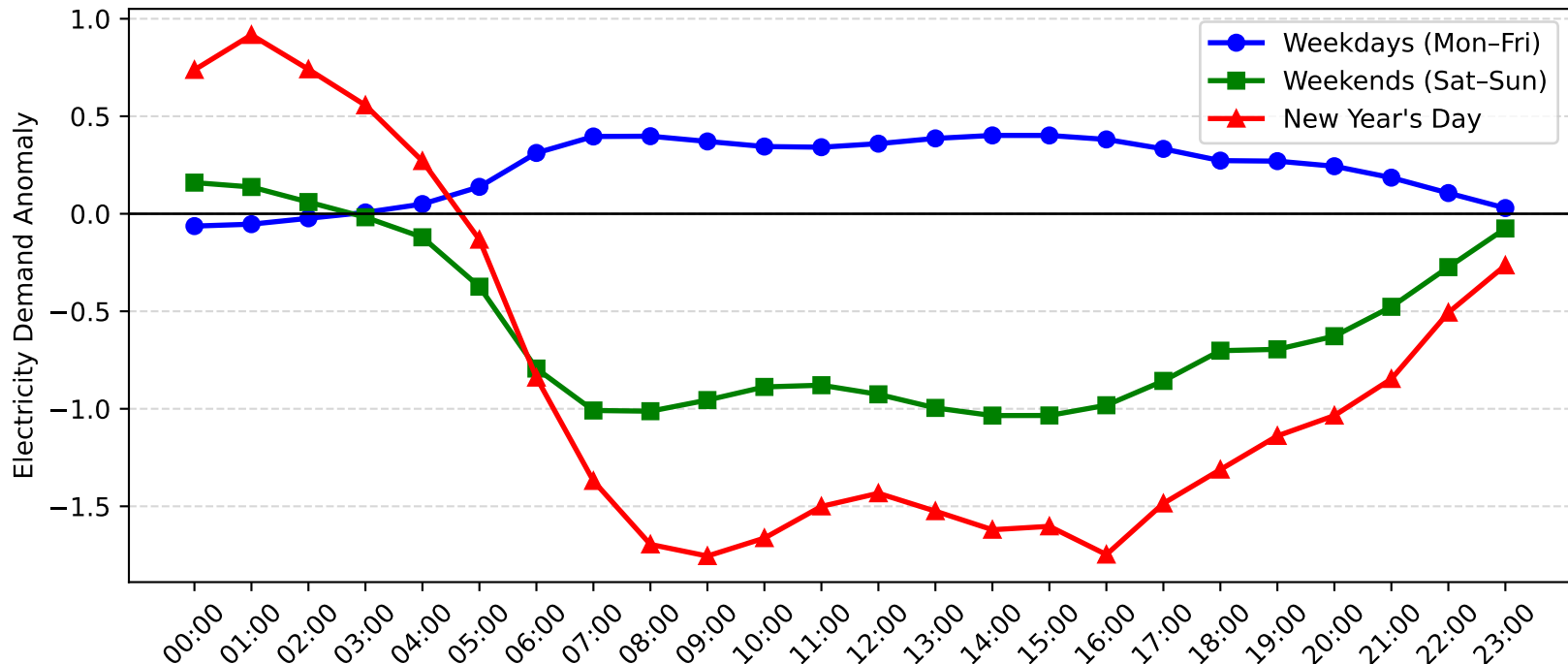
Rockdale Demand Anomaly: New Year's Day vs Weekday/Weekend (2016-2017)
