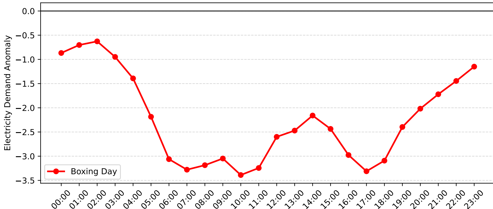
Lisarow Demand Anomaly: Boxing Day (2014-2015)
