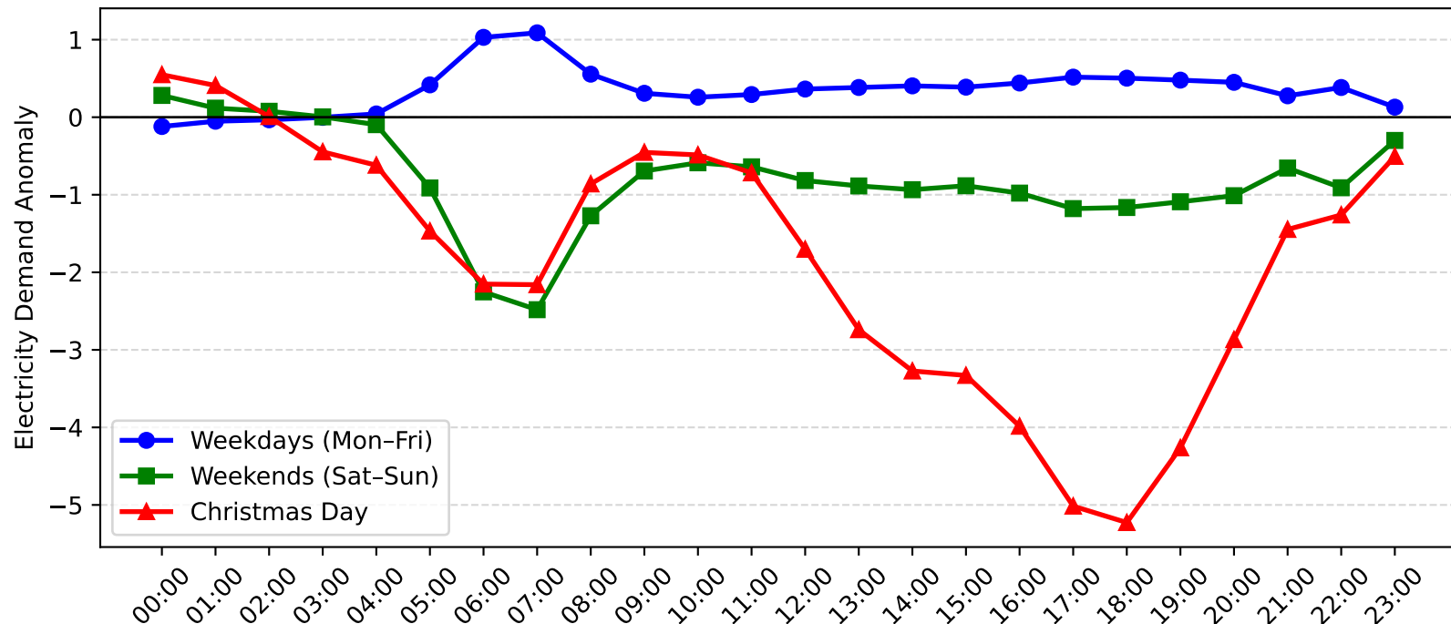
Dee Why West Demand Anomaly: Christmas Day vs Weekday/Weekend (2010-2011)
