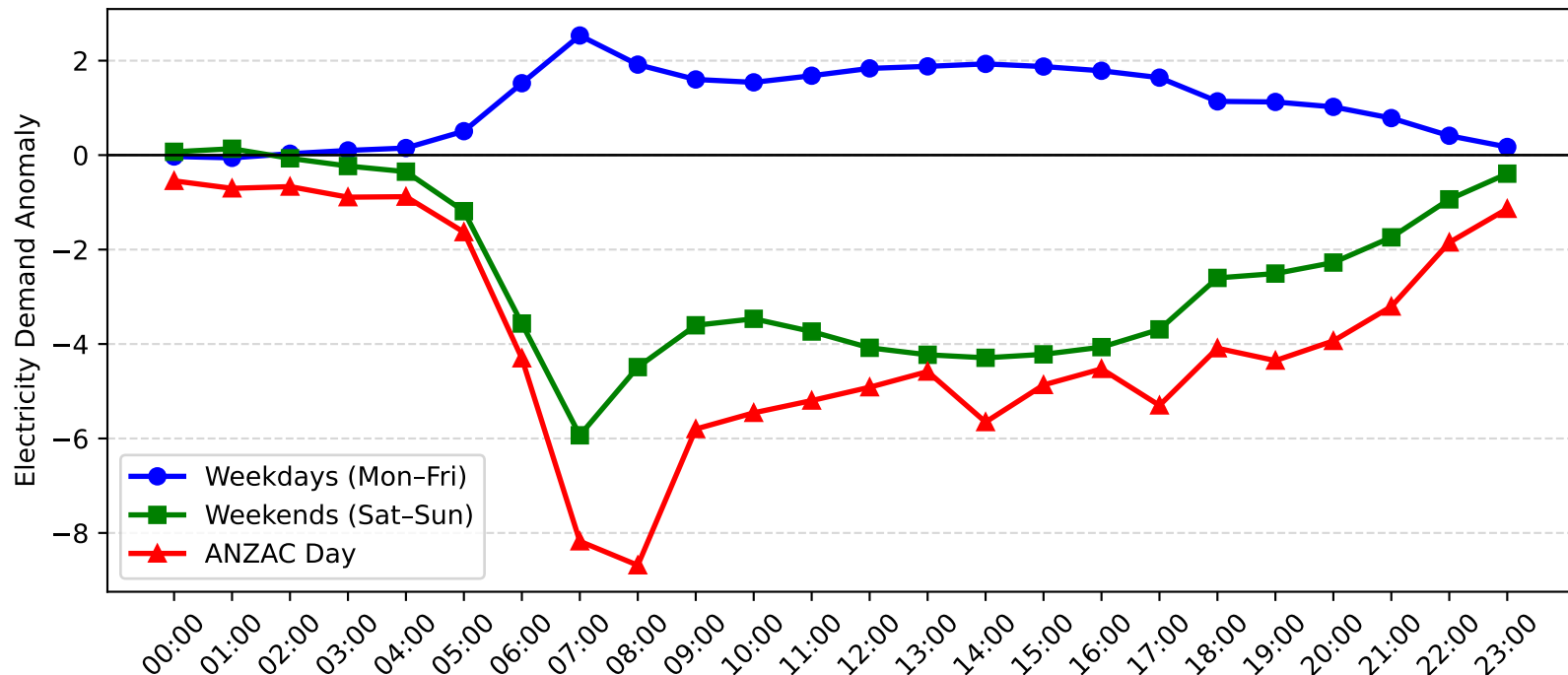
Epping Demand Anomaly: ANZAC Day vs Weekday/Weekend (2015-2016)
