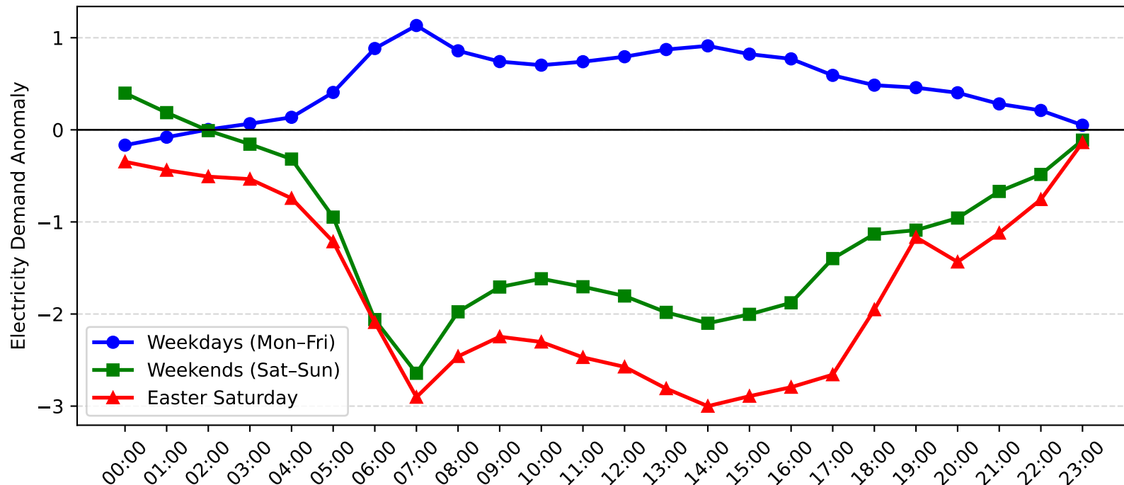
Rockdale Demand Anomaly: Easter Saturday vs Weekday/Weekend (2007-2008)
