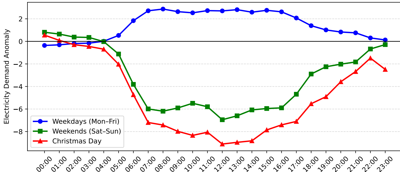
Hunters Hill Demand Anomaly: Christmas Day vs Weekday/Weekend (2004-2005)
