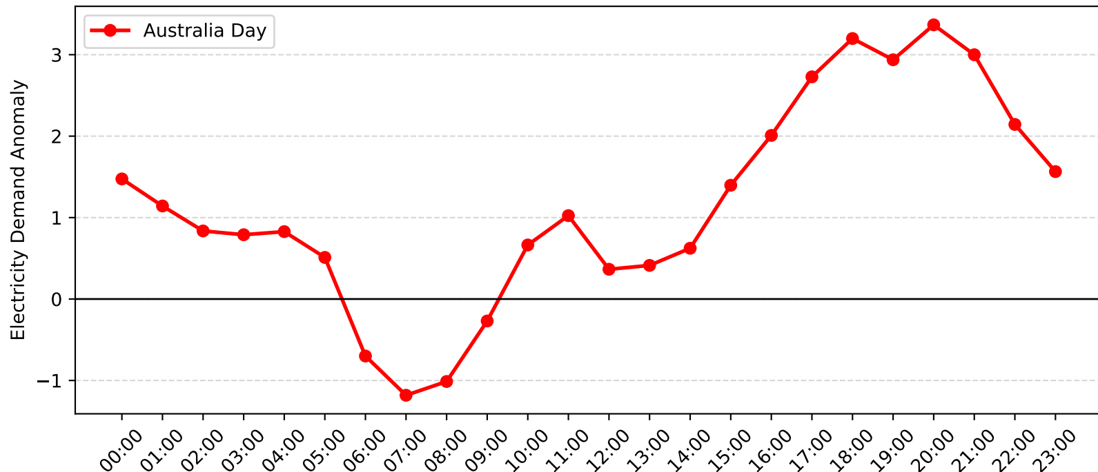
Concord Demand Anomaly: Australia Day (2011-2012)
