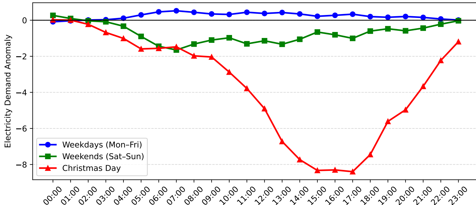
Charmhaven Demand Anomaly: Christmas Day vs Weekday/Weekend (2013-2014)
