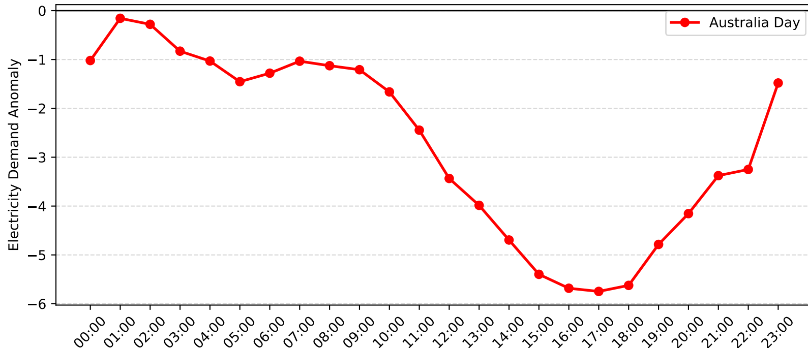
Umina Demand Anomaly: Australia Day (2017-2018)
