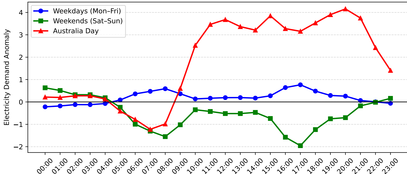
Erina Demand Anomaly: Australia Day vs Weekday/Weekend (2010-2011)
