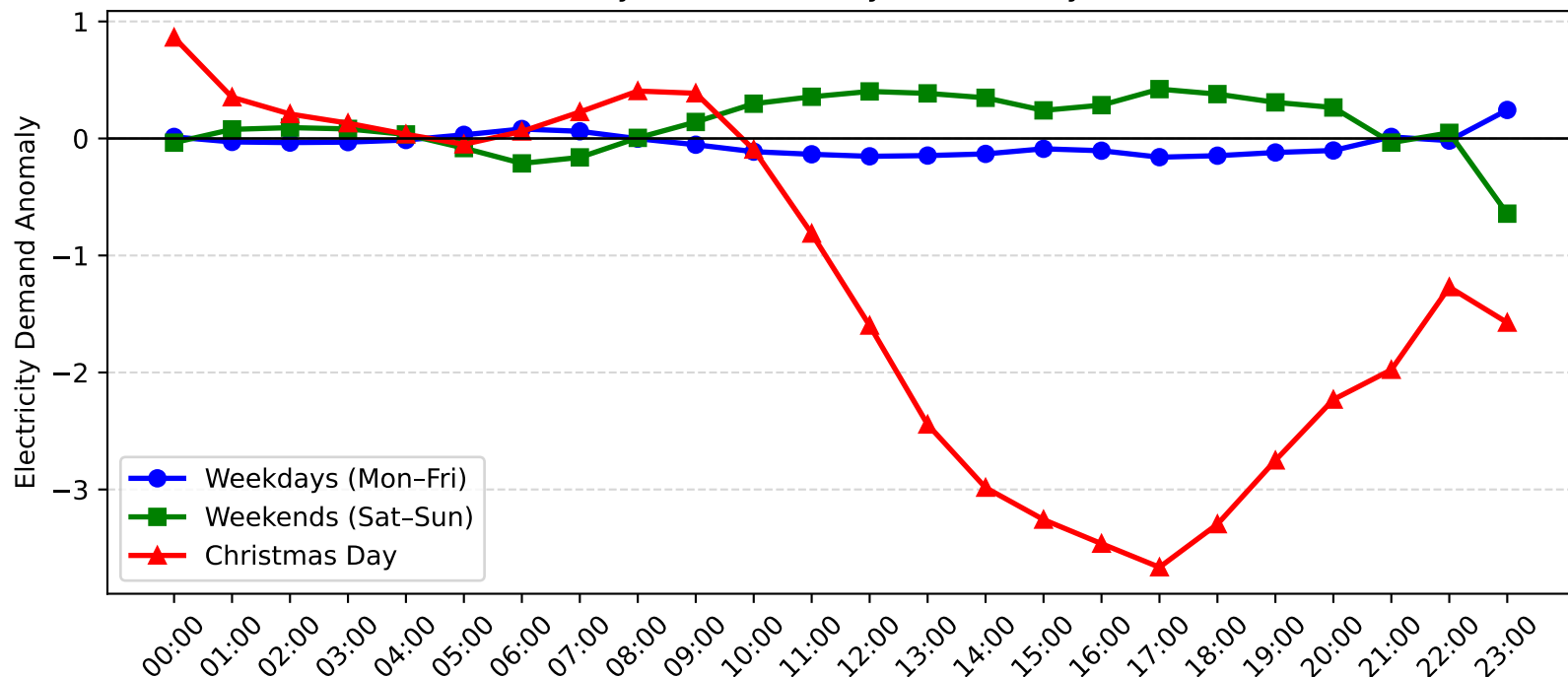
Telarah Demand Anomaly: Christmas Day vs Weekday/Weekend (2012-2013)
