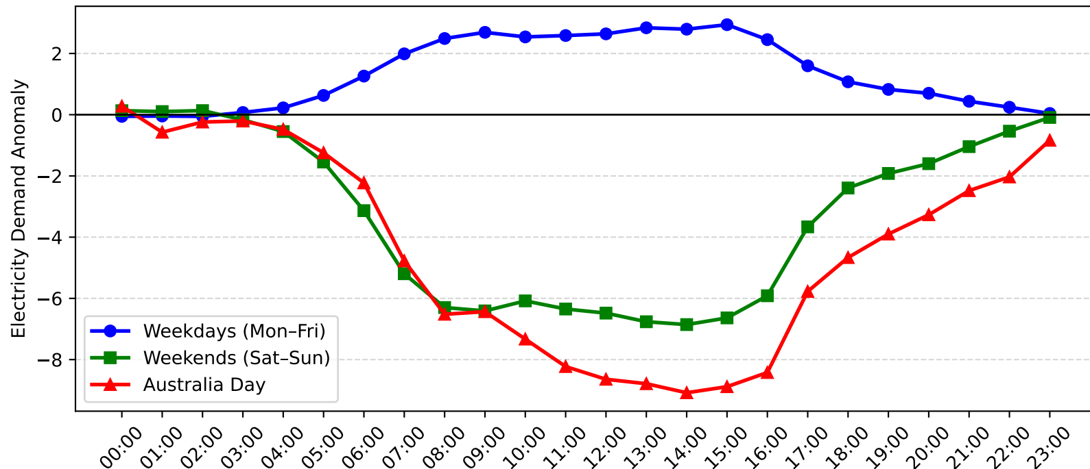
West Gosford Demand Anomaly: Australia Day vs Weekday/Weekend (2008-2009)
