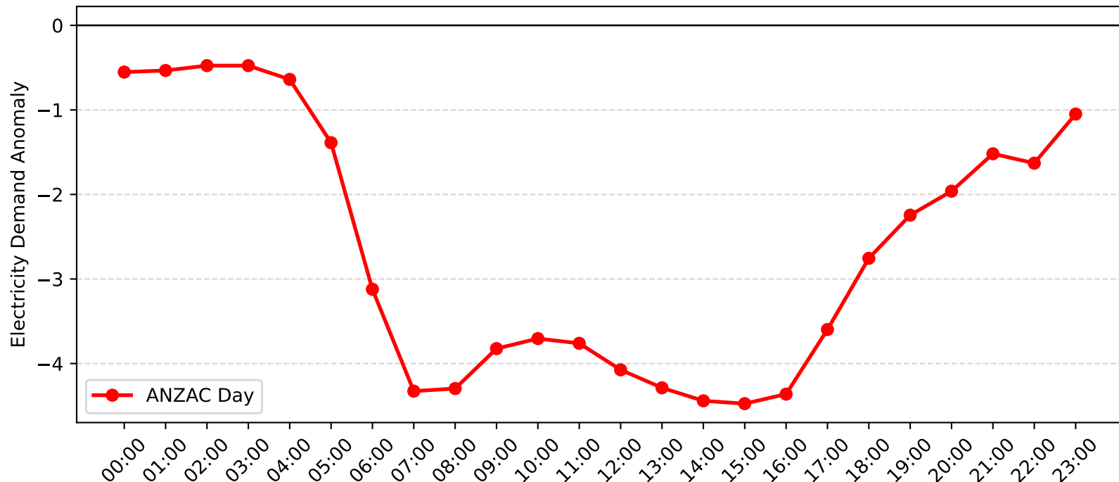
Beacon Hill Demand Anomaly: ANZAC Day (2009-2010)
