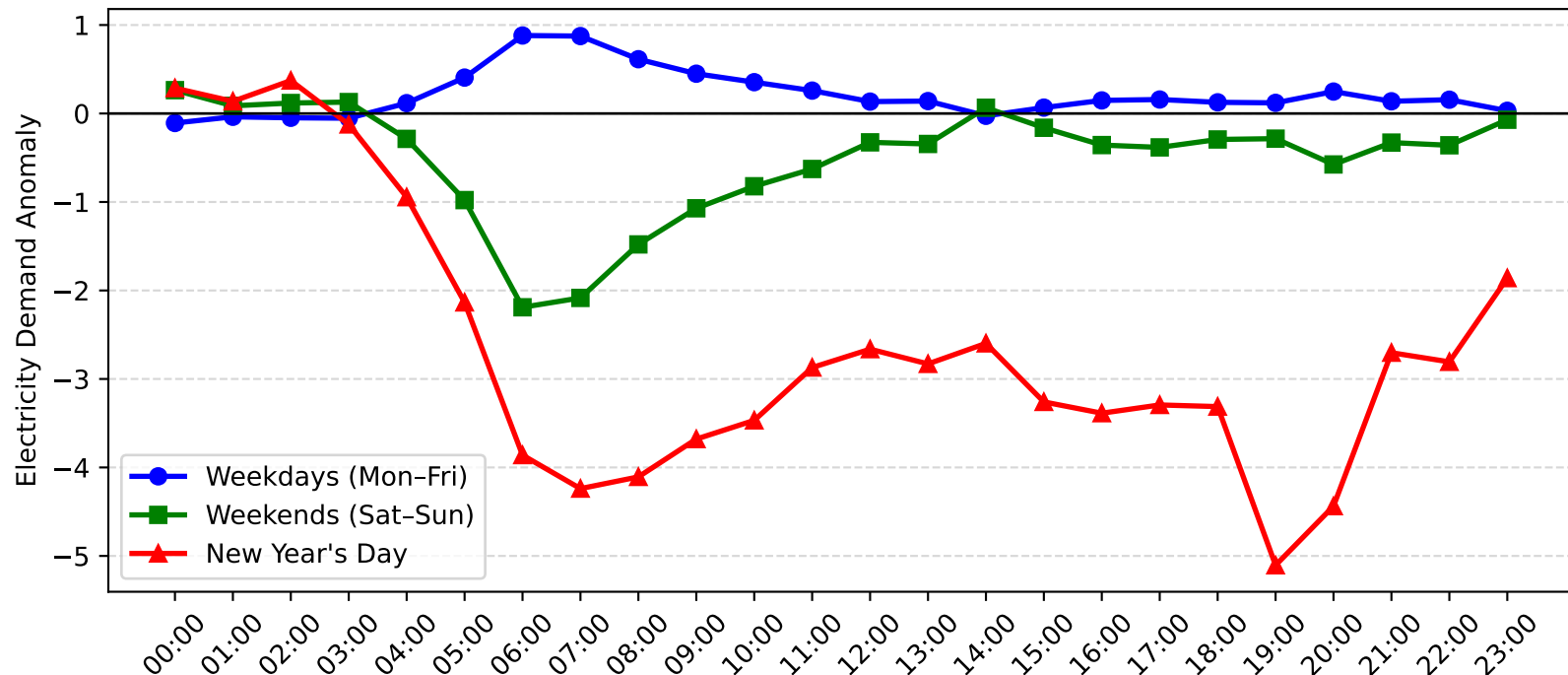
Revesby Demand Anomaly: New Year's Day vs Weekday/Weekend (2007-2008)
