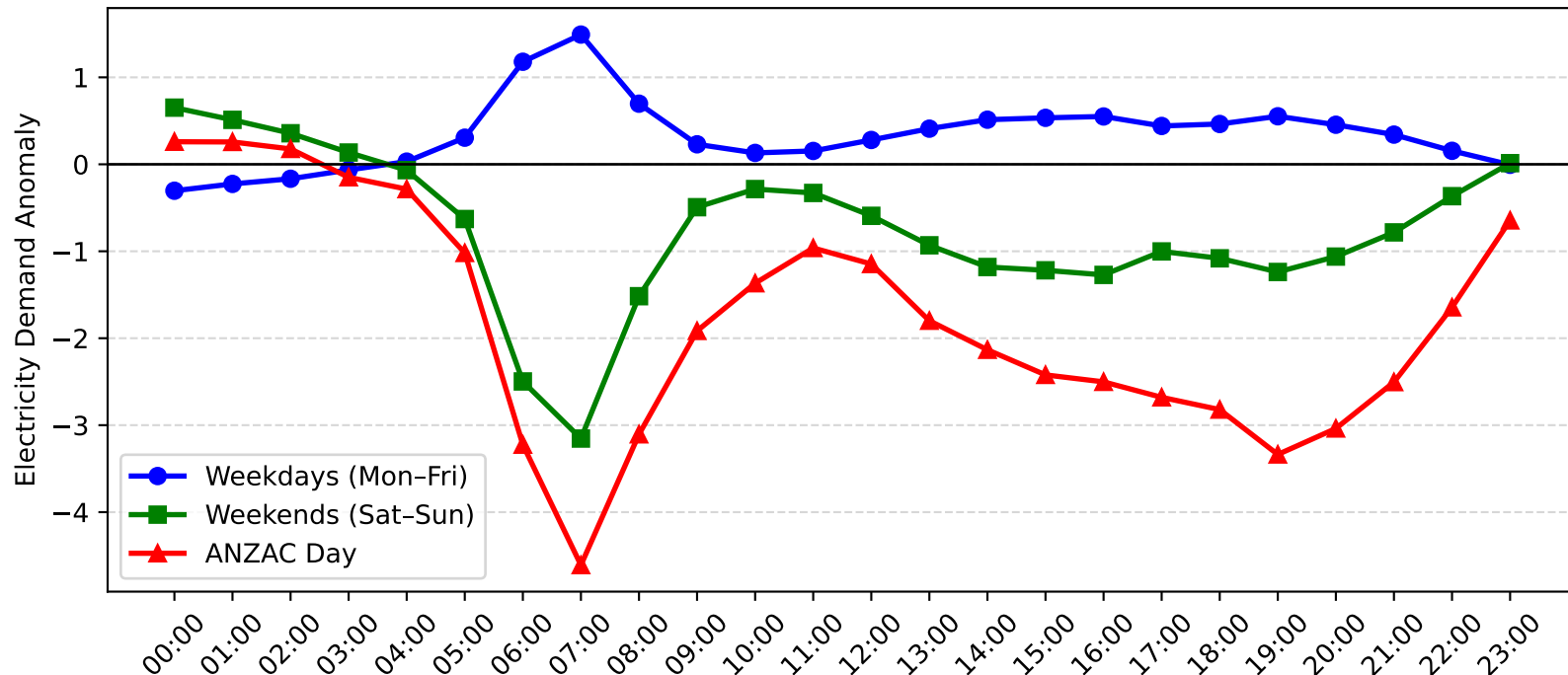
Five Dock Demand Anomaly: ANZAC Day vs Weekday/Weekend (2009-2010)
