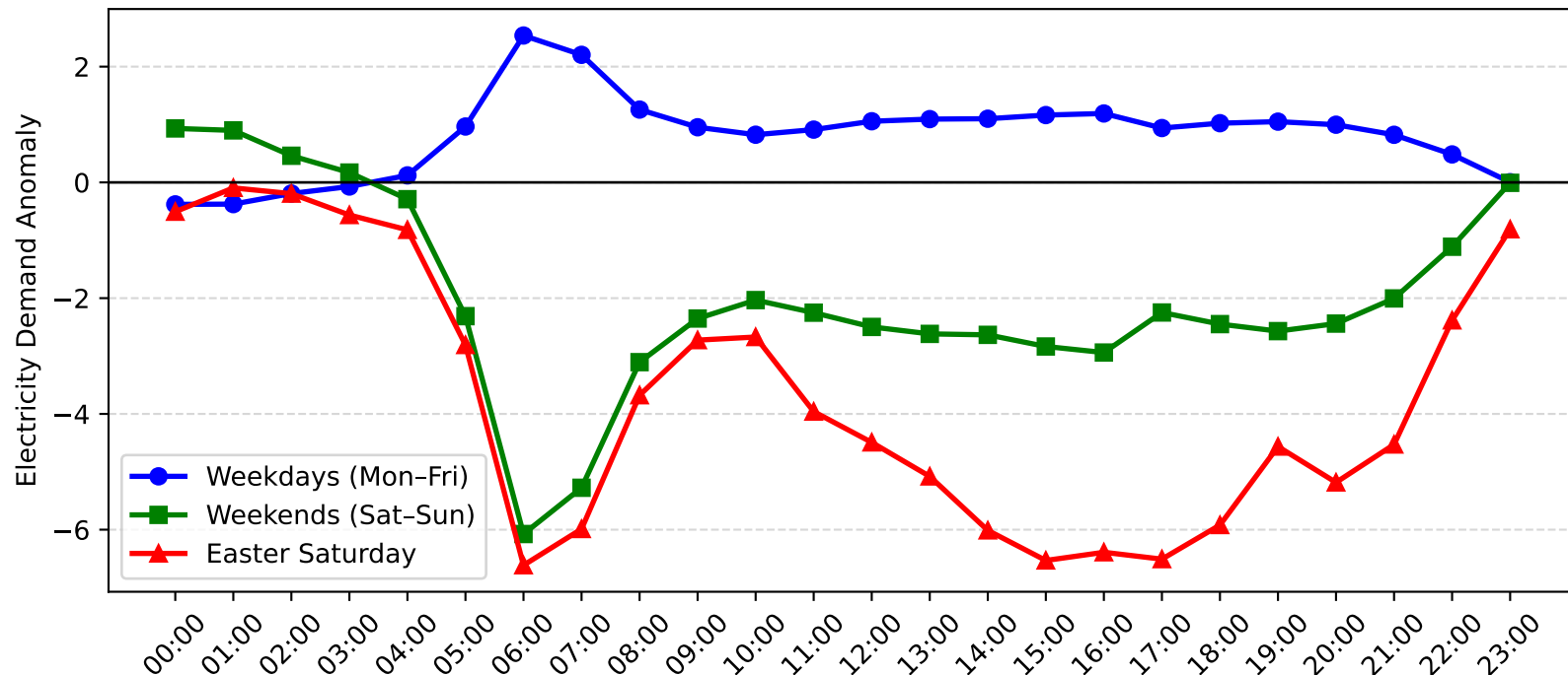
Pennant Hills Demand Anomaly: Easter Saturday vs Weekday/Weekend (2007-2008)
