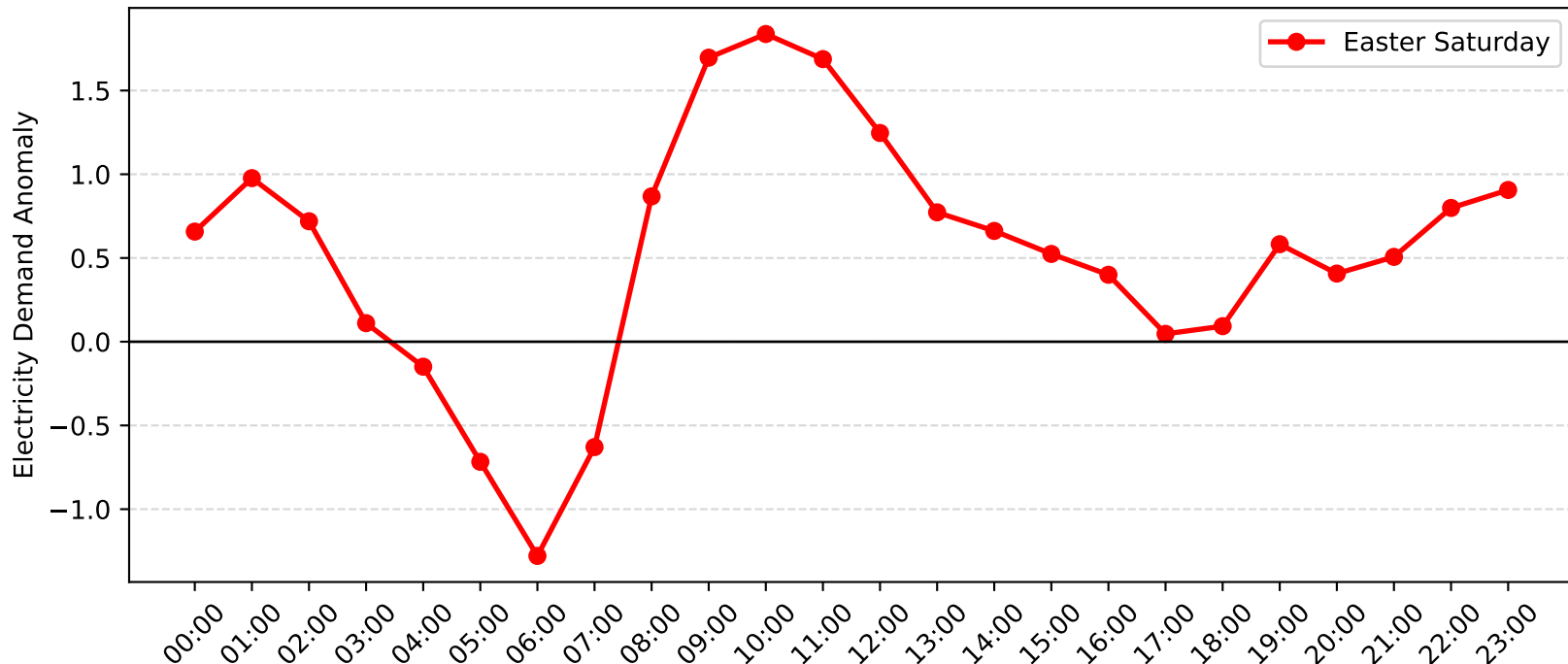
Umina Demand Anomaly: Easter Saturday (2015-2016)
