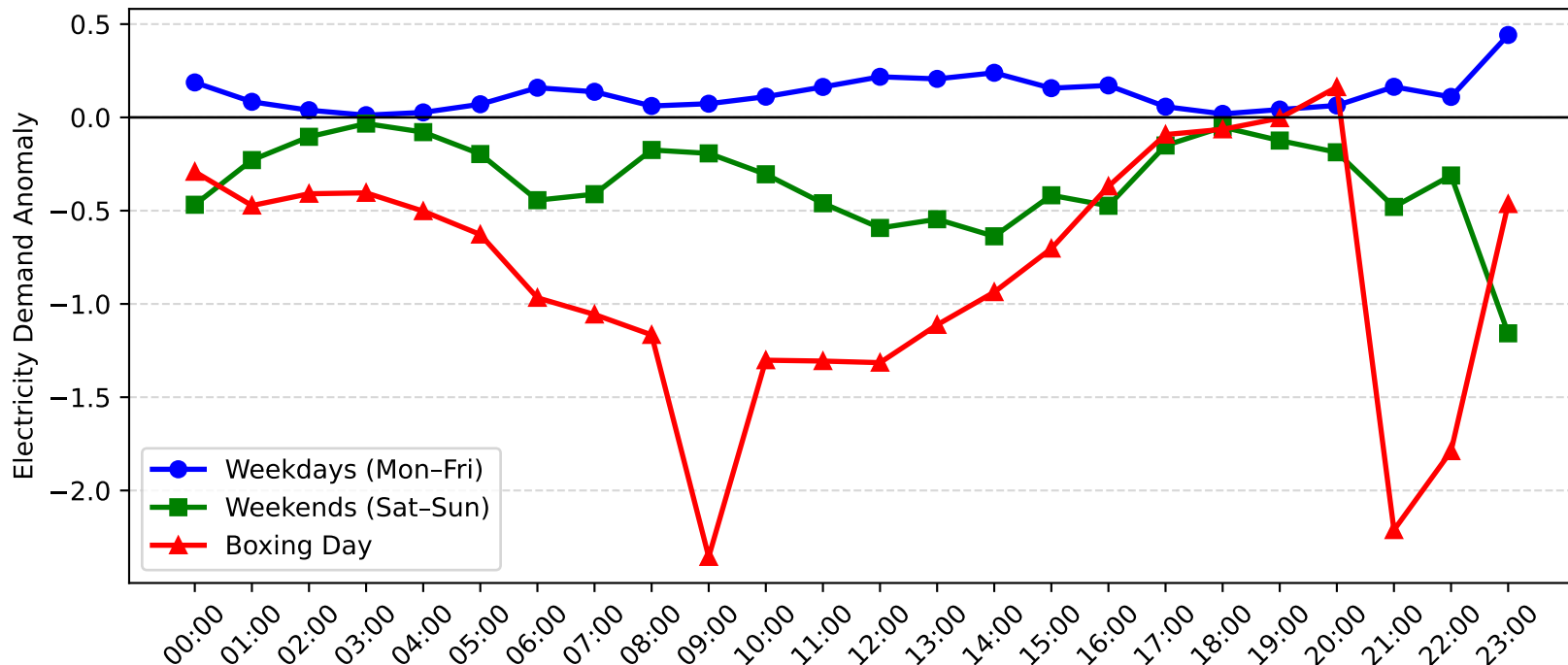
Telarah Demand Anomaly: Boxing Day vs Weekday/Weekend (2007-2008)
