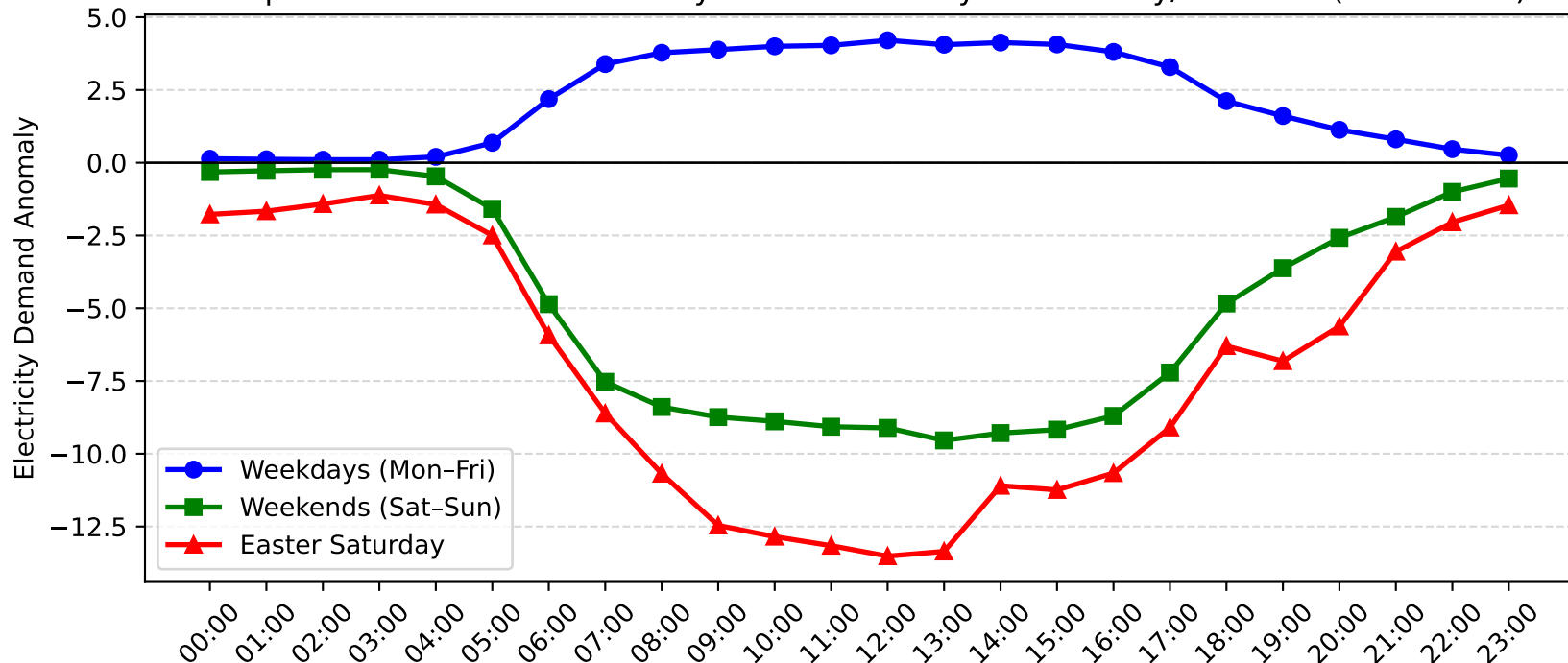
Macquarie Park Demand Anomaly: Easter Saturday vs Weekday/Weekend (2008-2009)
