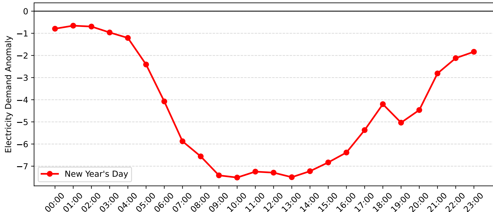
Concord Demand Anomaly: New Year's Day (2007-2008)
