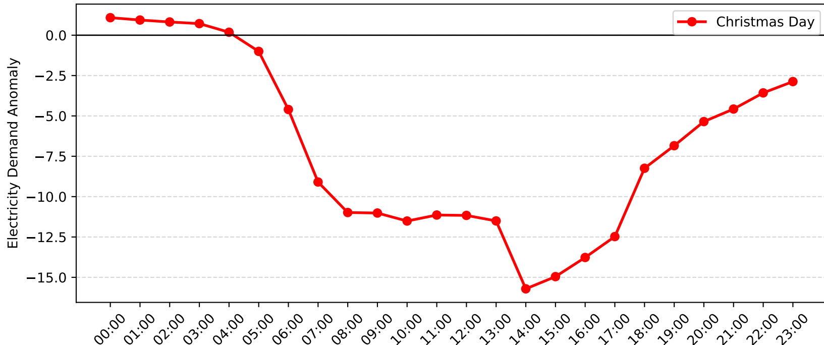
Macquarie Park Demand Anomaly: Christmas Day (2009-2010)
