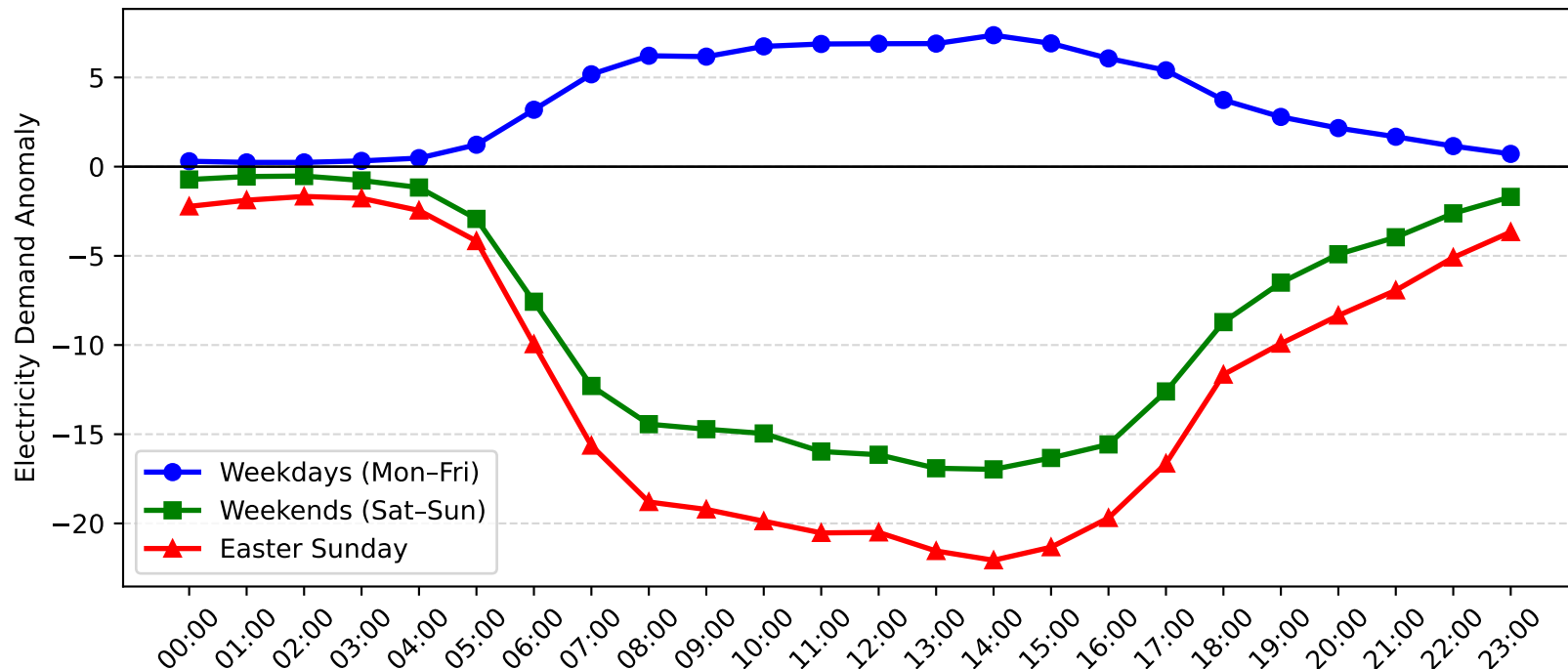
Gore Hill Demand Anomaly: Easter Sunday vs Weekday/Weekend (2006-2007)
