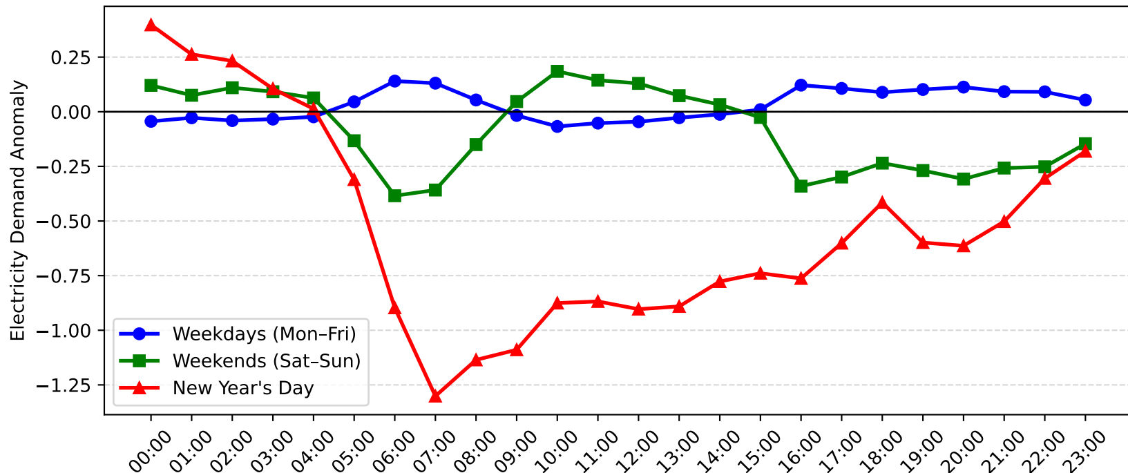
Narrabeen Demand Anomaly: New Year's Day vs Weekday/Weekend (2013-2014)
