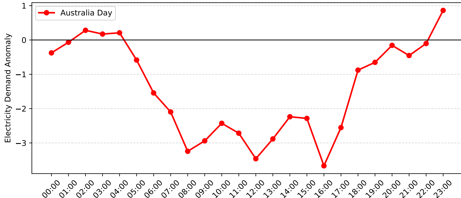
Erina Demand Anomaly: Australia Day (2006-2007)
