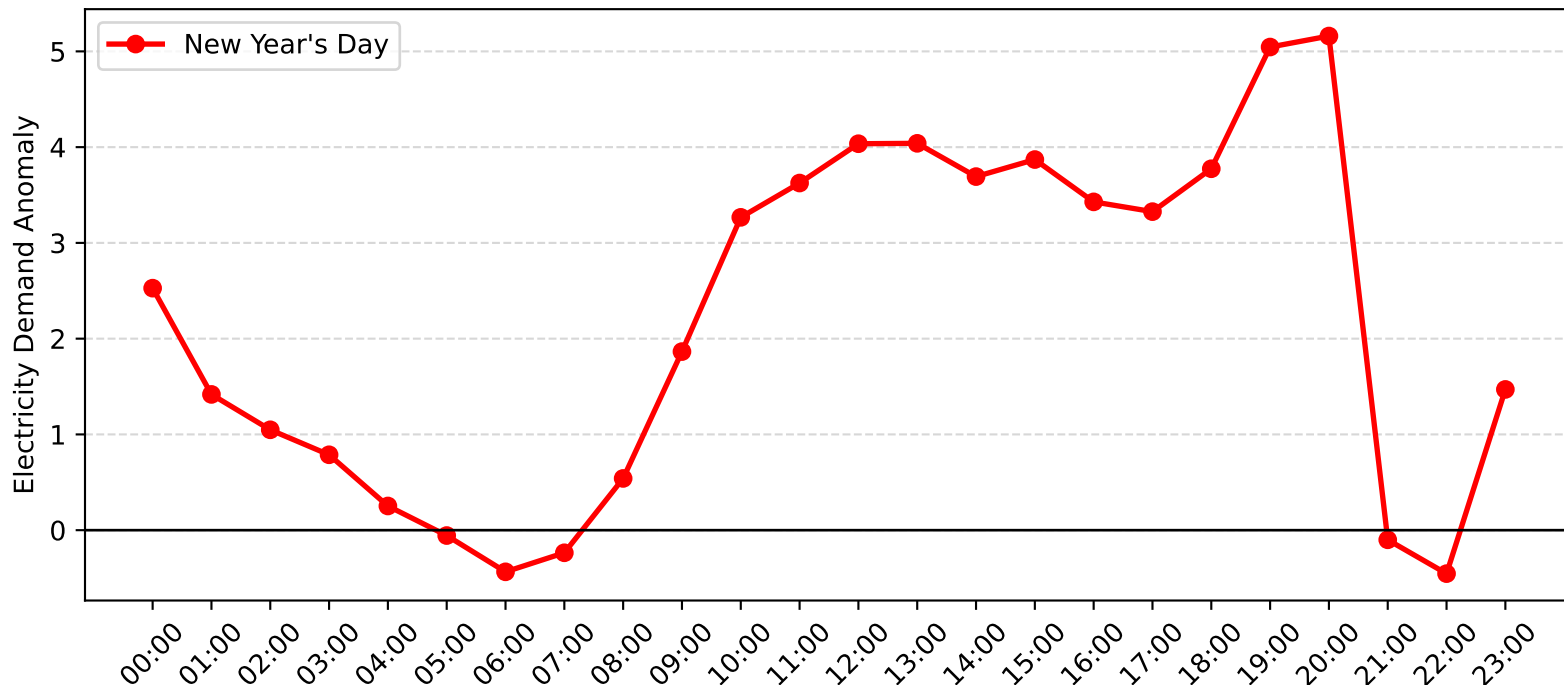
Noraville Demand Anomaly: New Year's Day (2006-2007)
