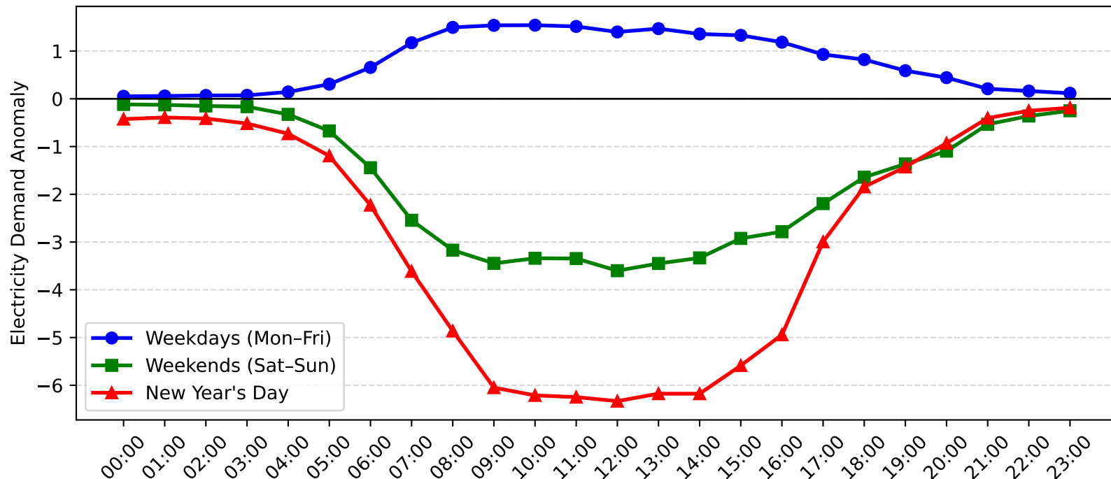
Auburn Demand Anomaly: New Year's Day vs Weekday/Weekend (2005-2006)
