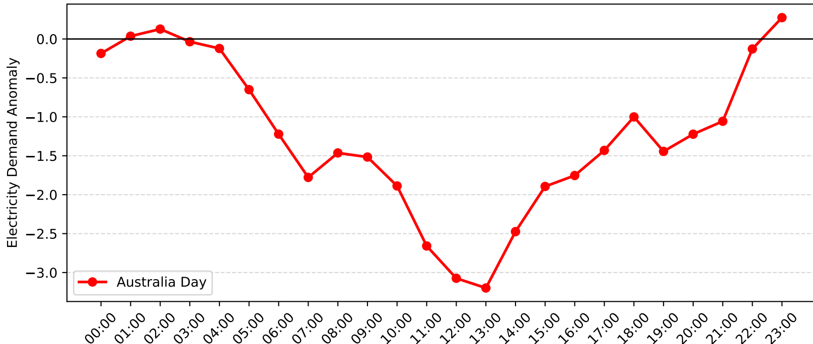
Charmhaven Demand Anomaly: Australia Day (2006-2007)
