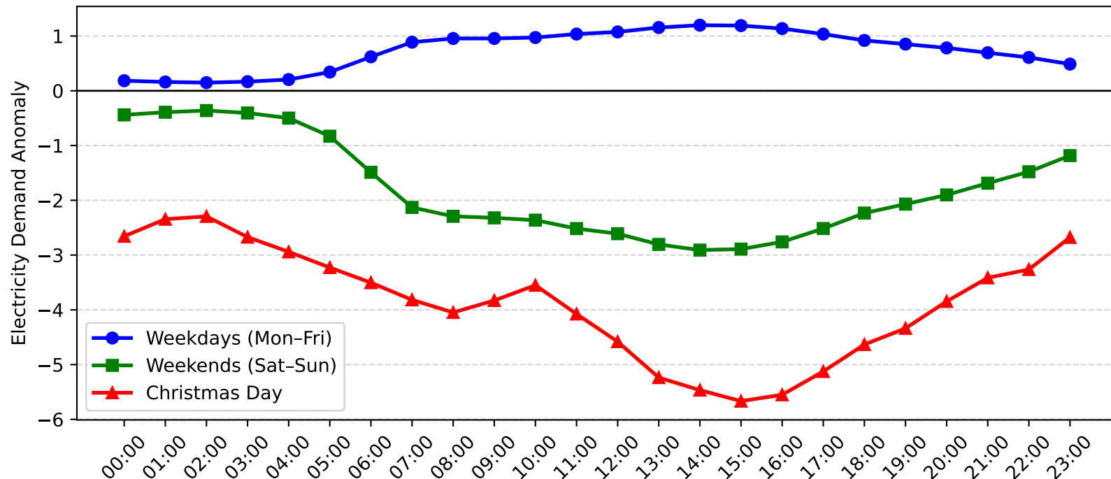
Bass Hill Demand Anomaly: Christmas Day vs Weekday/Weekend (2015-2016)
