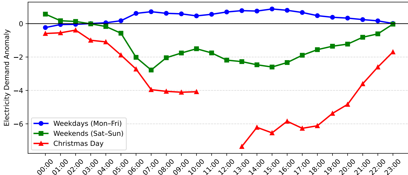
Five Dock Demand Anomaly: Christmas Day vs Weekday/Weekend (2008-2009)
