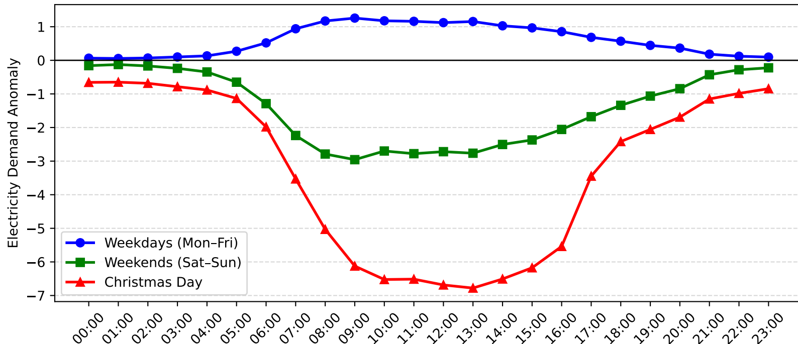
Auburn Demand Anomaly: Christmas Day vs Weekday/Weekend (2006-2007)
