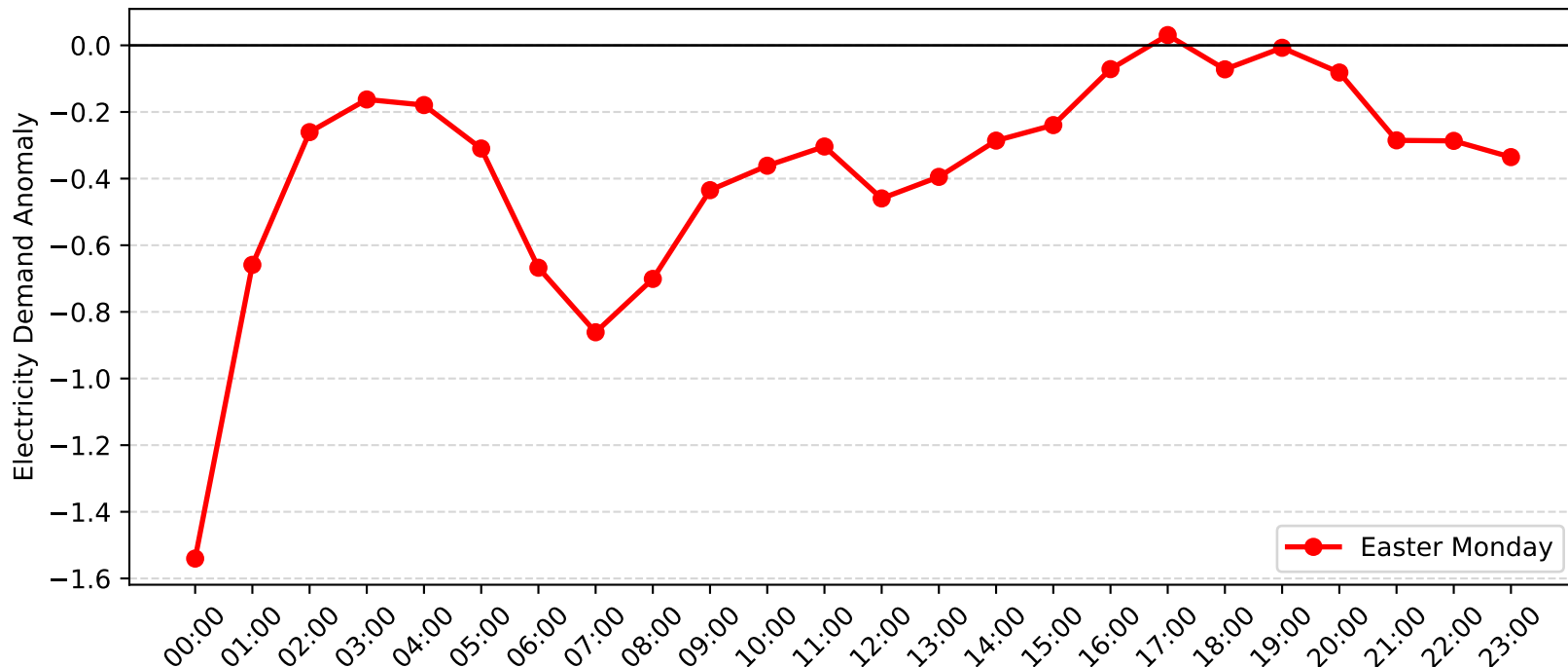
Telarah Demand Anomaly: Easter Monday (2008-2009)
