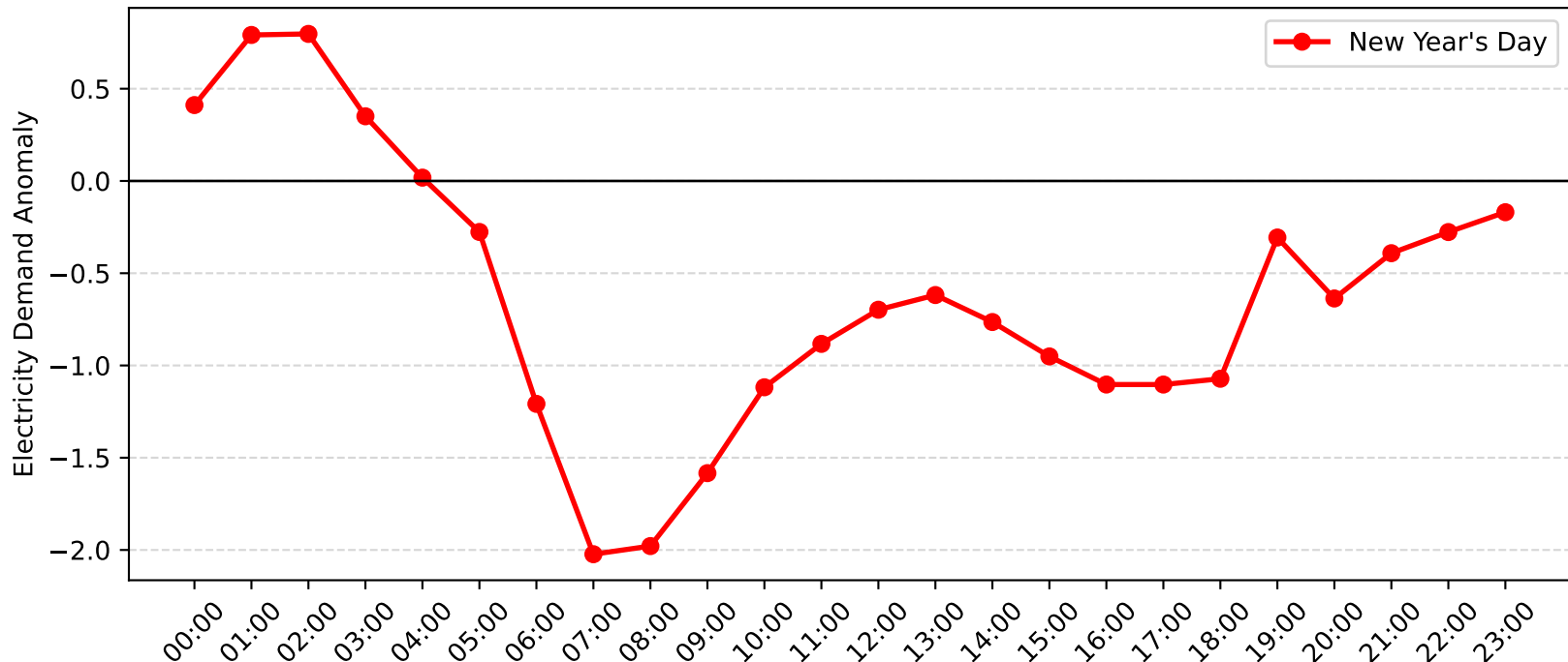
Blakehurst Demand Anomaly: New Year's Day (2013-2014)
