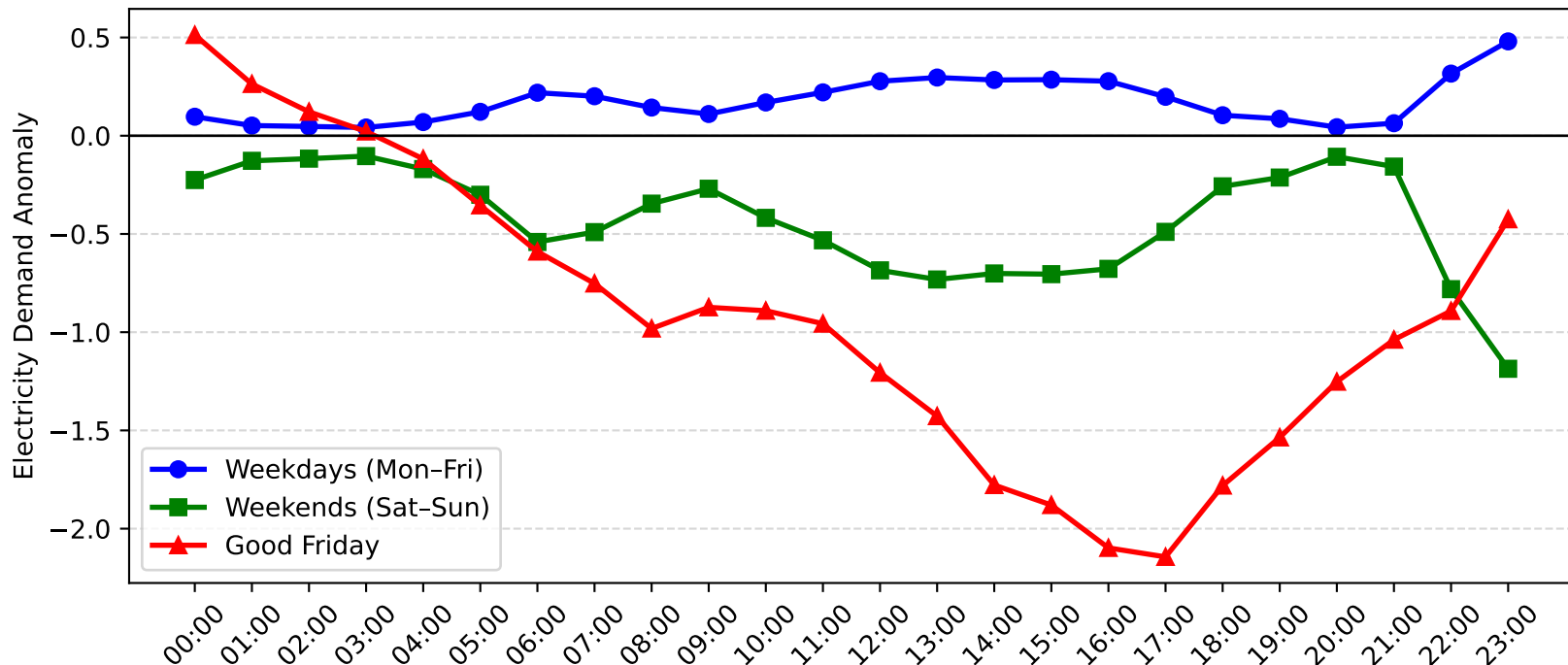
Muswellbrook Demand Anomaly: Good Friday vs Weekday/Weekend (2015-2016)
