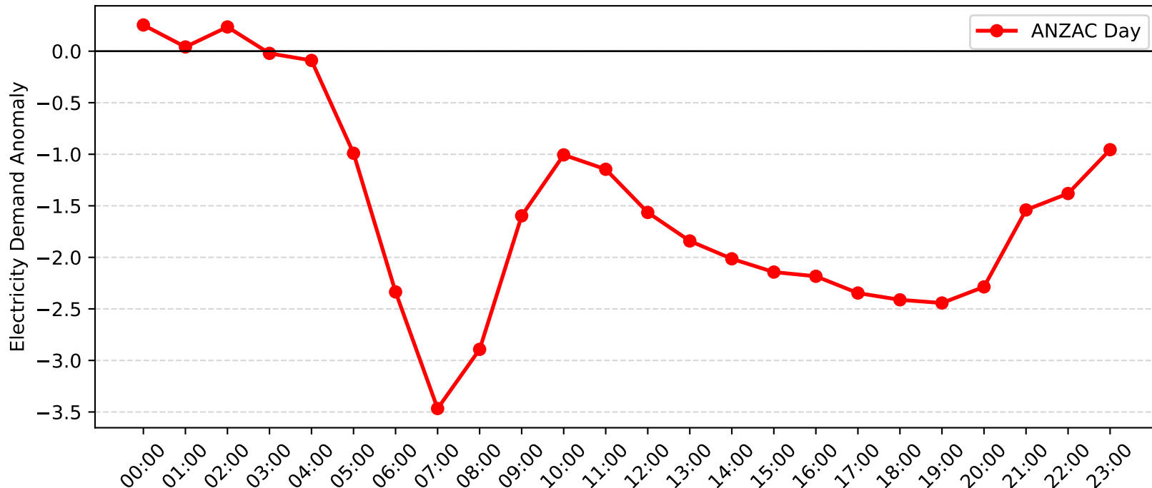
Jesmond Demand Anomaly: ANZAC Day (2014-2015)
