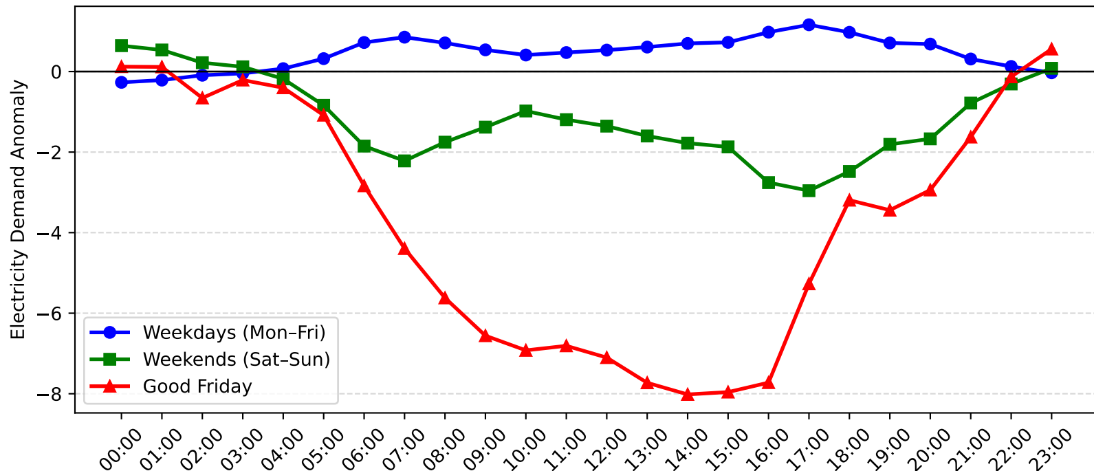
Erina Demand Anomaly: Good Friday vs Weekday/Weekend (2006-2007)
