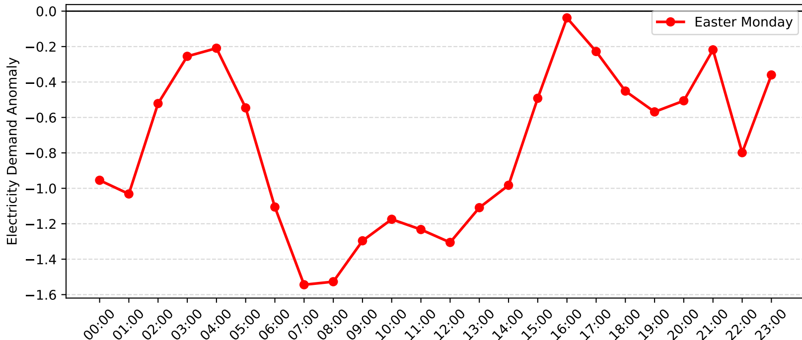
Gateshead Demand Anomaly: Easter Monday (2015-2016)
