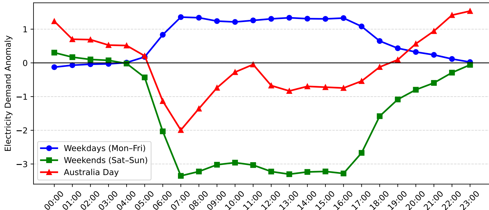
Pymble Demand Anomaly: Australia Day vs Weekday/Weekend (2012-2013)
