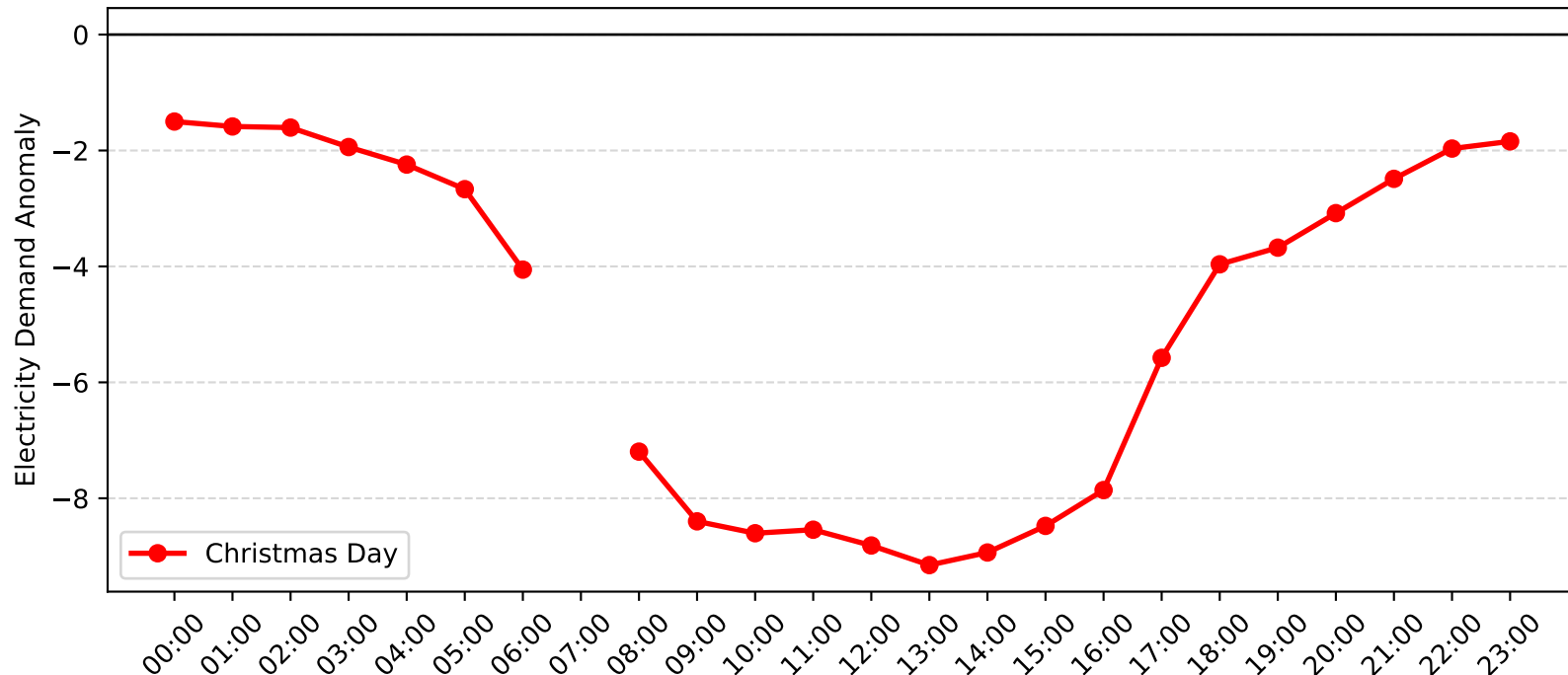
Auburn Demand Anomaly: Christmas Day (2016-2017)
