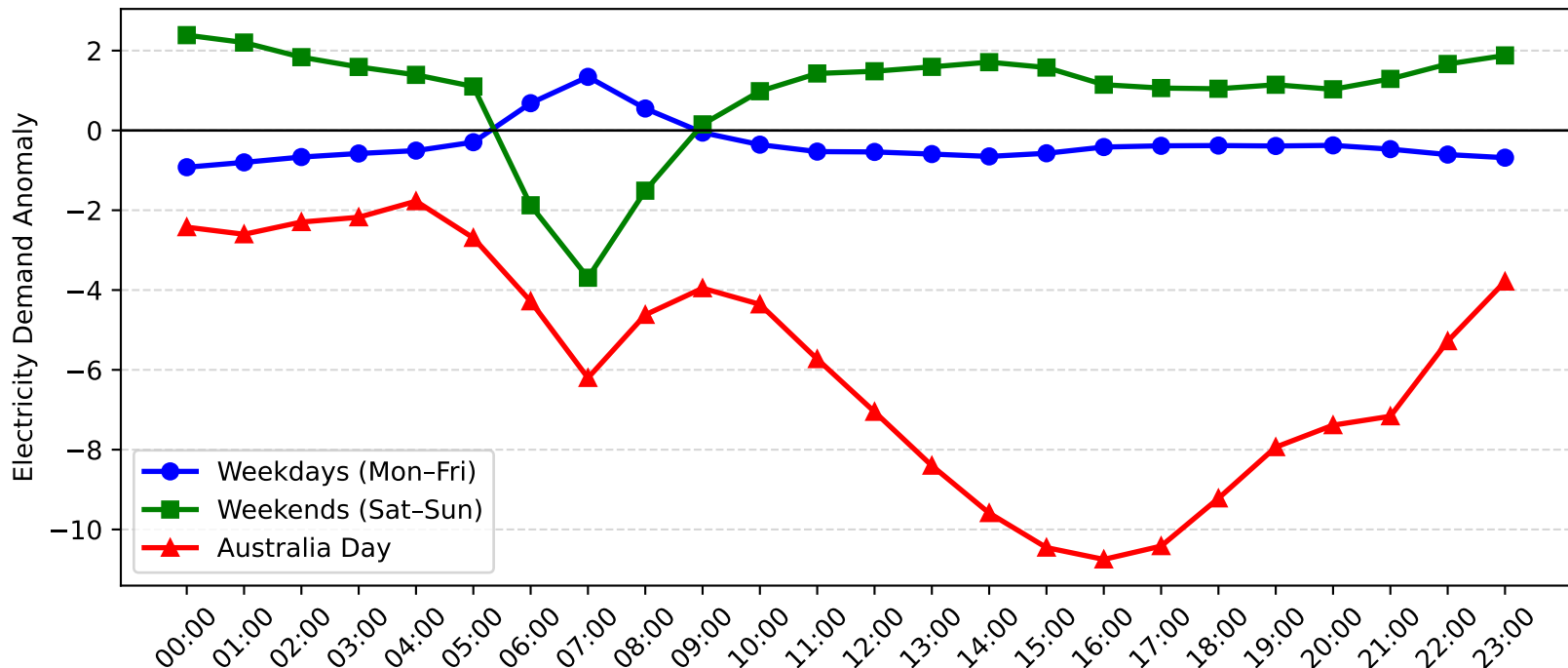
Mosman Demand Anomaly: Australia Day vs Weekday/Weekend (2017-2018)
