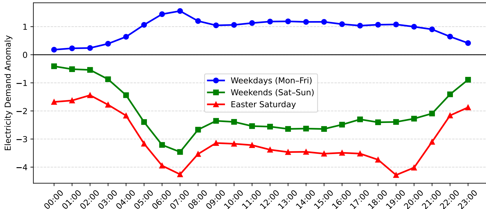
Lisarow Demand Anomaly: Easter Saturday vs Weekday/Weekend (2008-2009)
