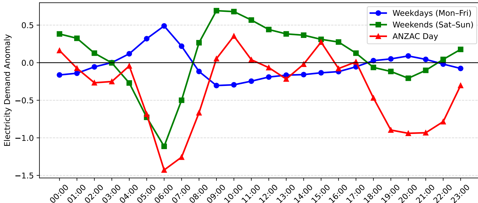
Umina Demand Anomaly: ANZAC Day vs Weekday/Weekend (2016-2017)
