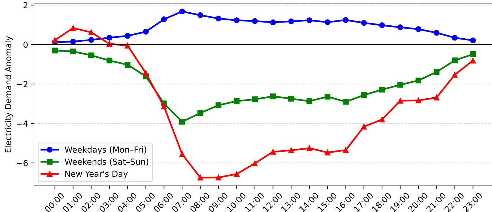
Maroubra Demand Anomaly: New Year's Day vs Weekday/Weekend (2017-2018)
