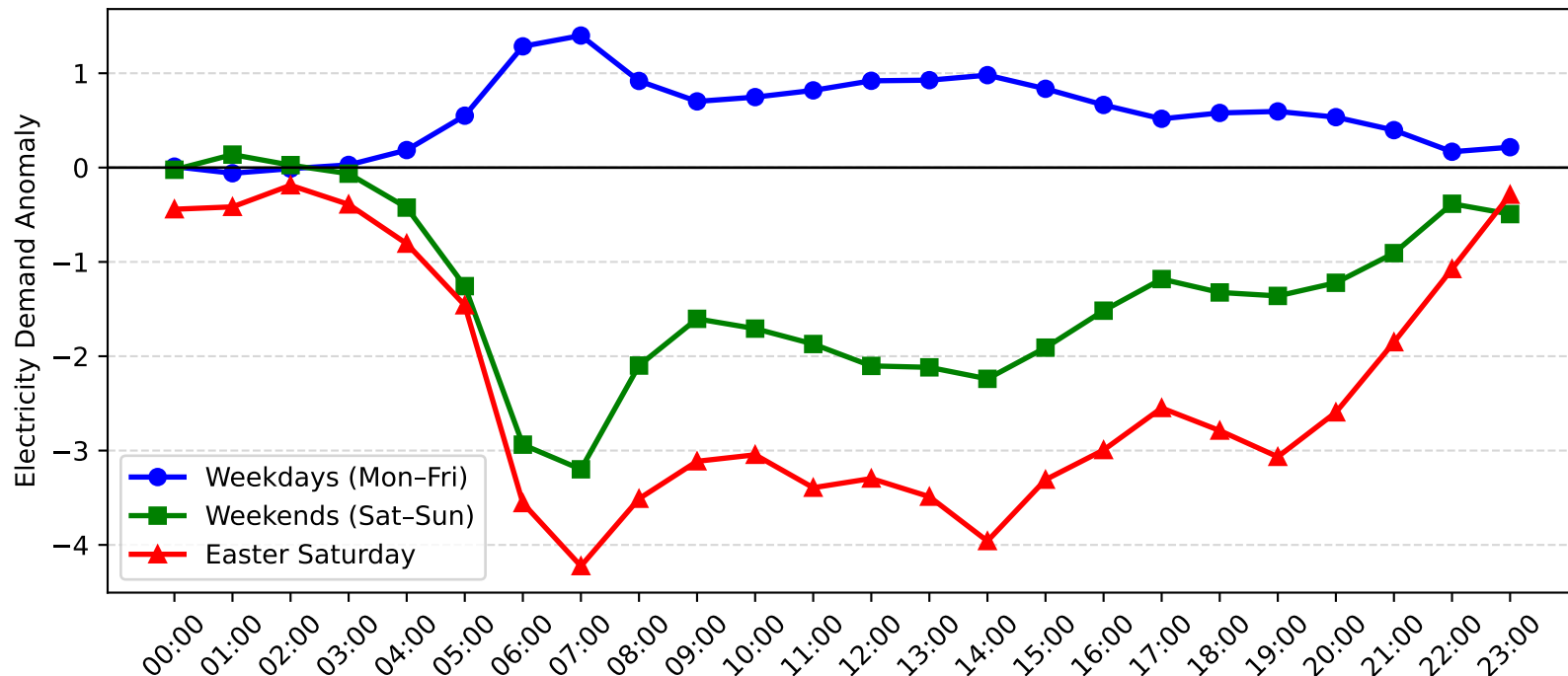
Kirrawee Demand Anomaly: Easter Saturday vs Weekday/Weekend (2017-2018)
