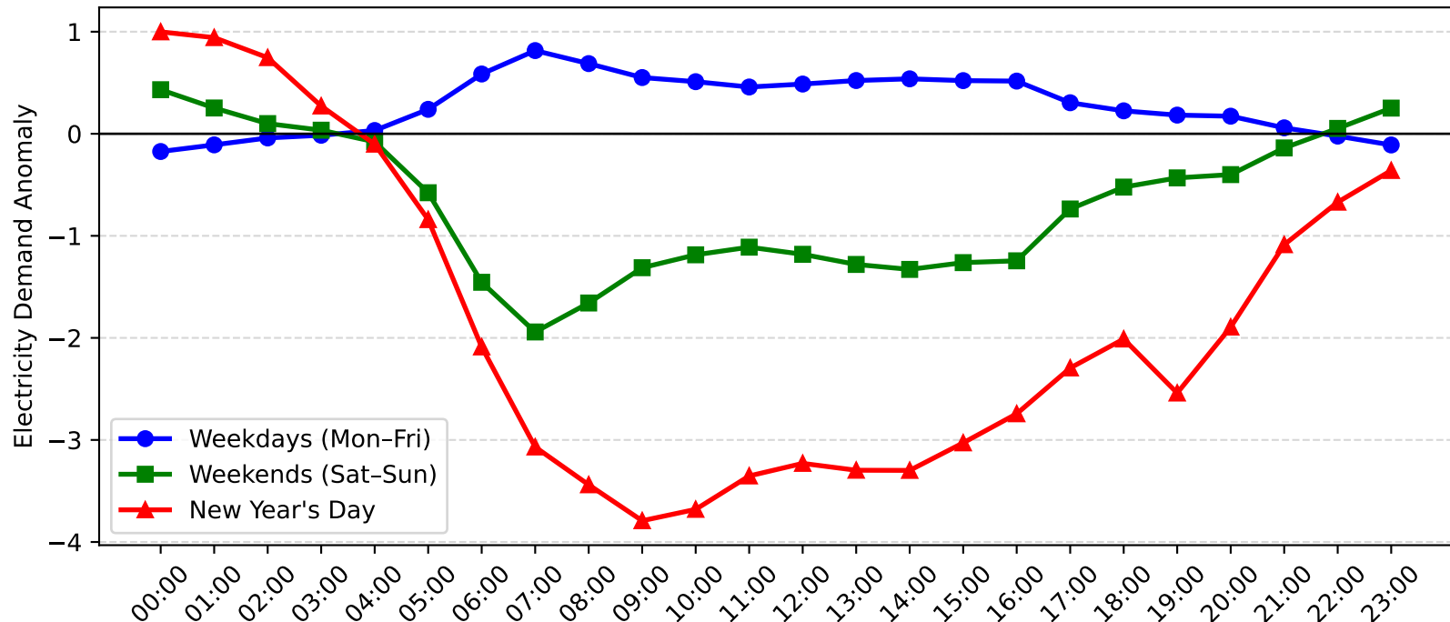
Rockdale Demand Anomaly: New Year's Day vs Weekday/Weekend (2007-2008)
