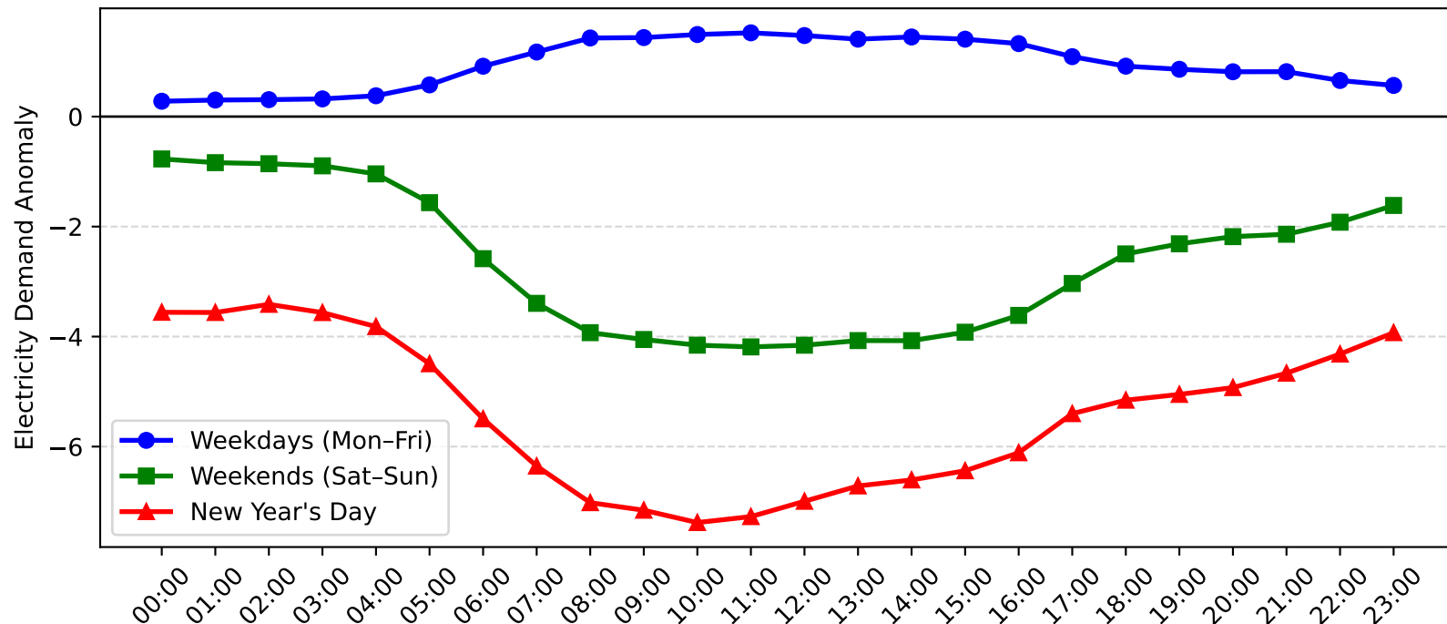
Leightonfield Demand Anomaly: New Year's Day vs Weekday/Weekend (2015-2016)
