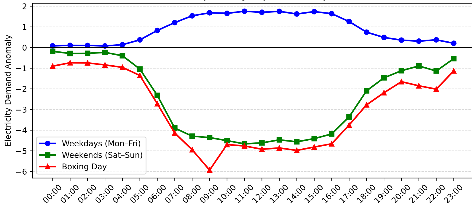
Beacon Hill Demand Anomaly: Boxing Day vs Weekday/Weekend (2008-2009)
