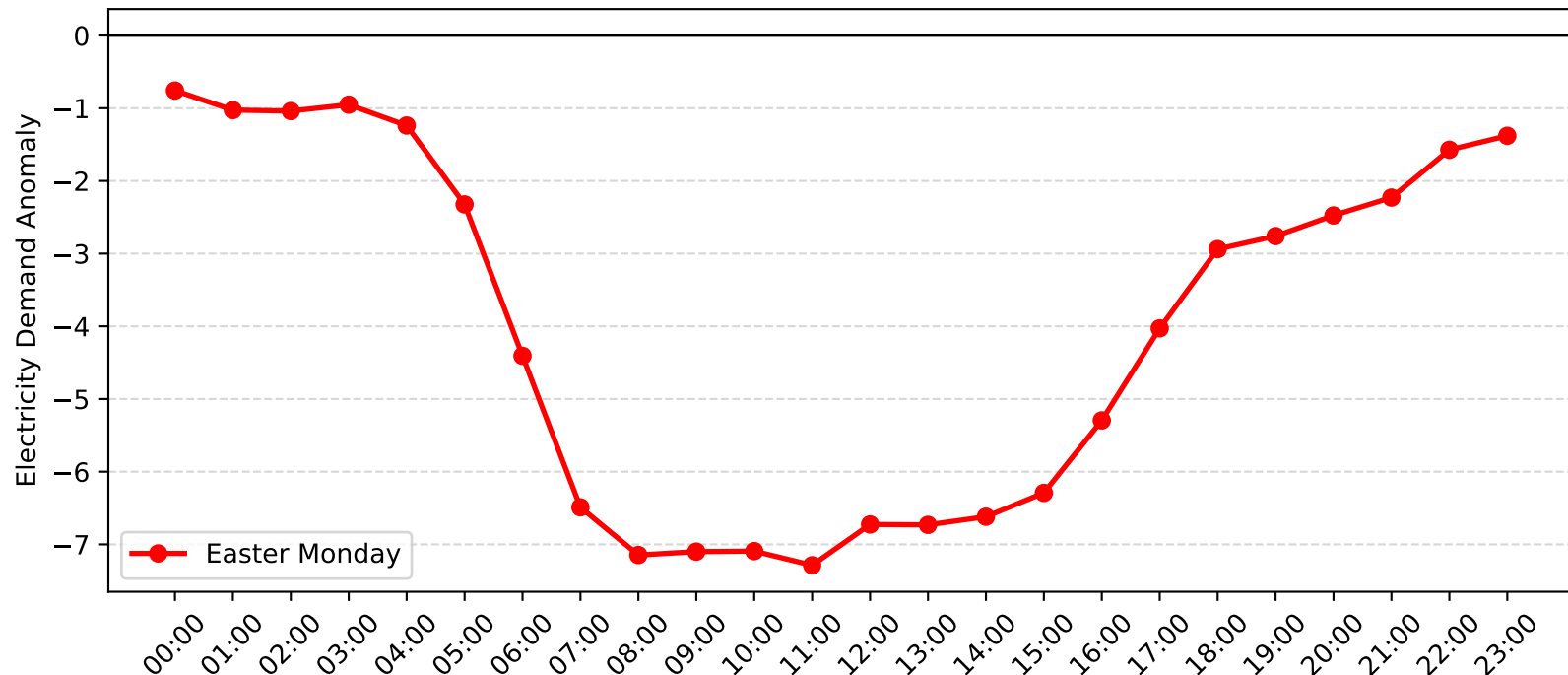
Bankstown Demand Anomaly: Easter Monday (2014-2015)
