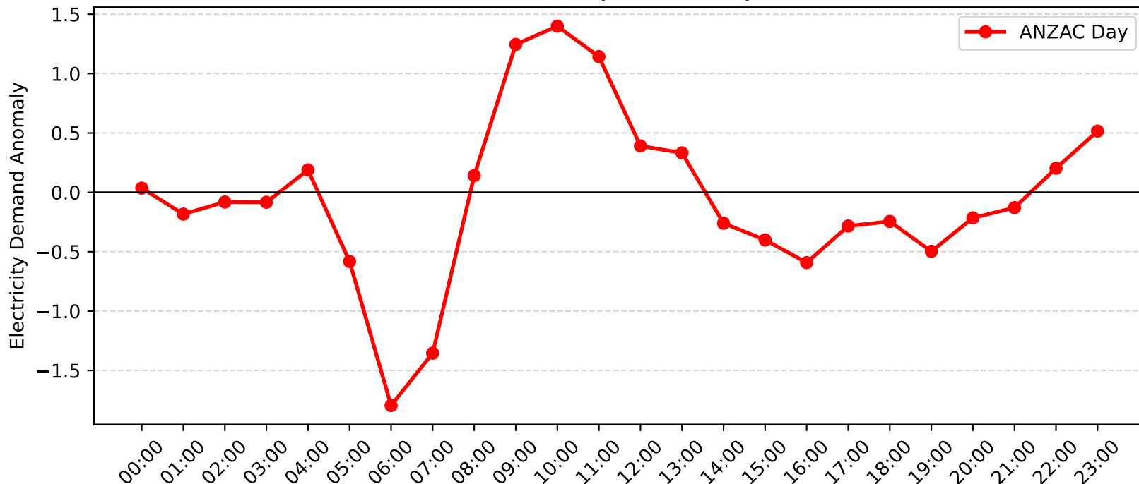
Umina Demand Anomaly: ANZAC Day (2013-2014)
