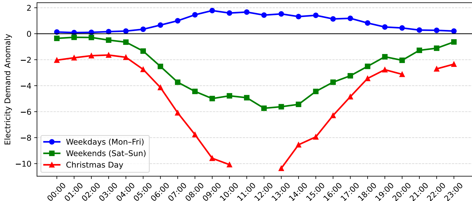
Auburn Demand Anomaly: Christmas Day vs Weekday/Weekend (2008-2009)
