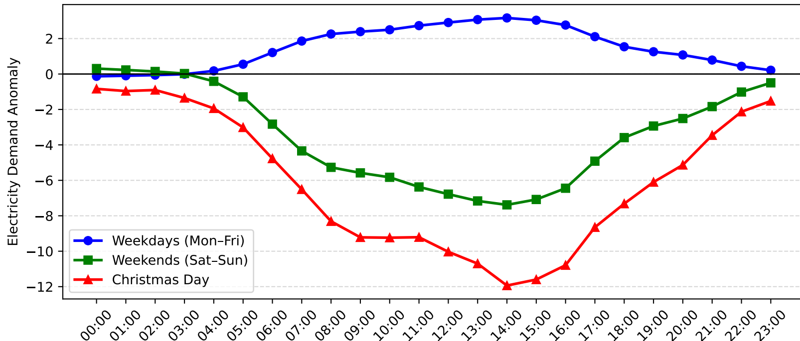
West Gosford Demand Anomaly: Christmas Day vs Weekday/Weekend (2016-2017)
