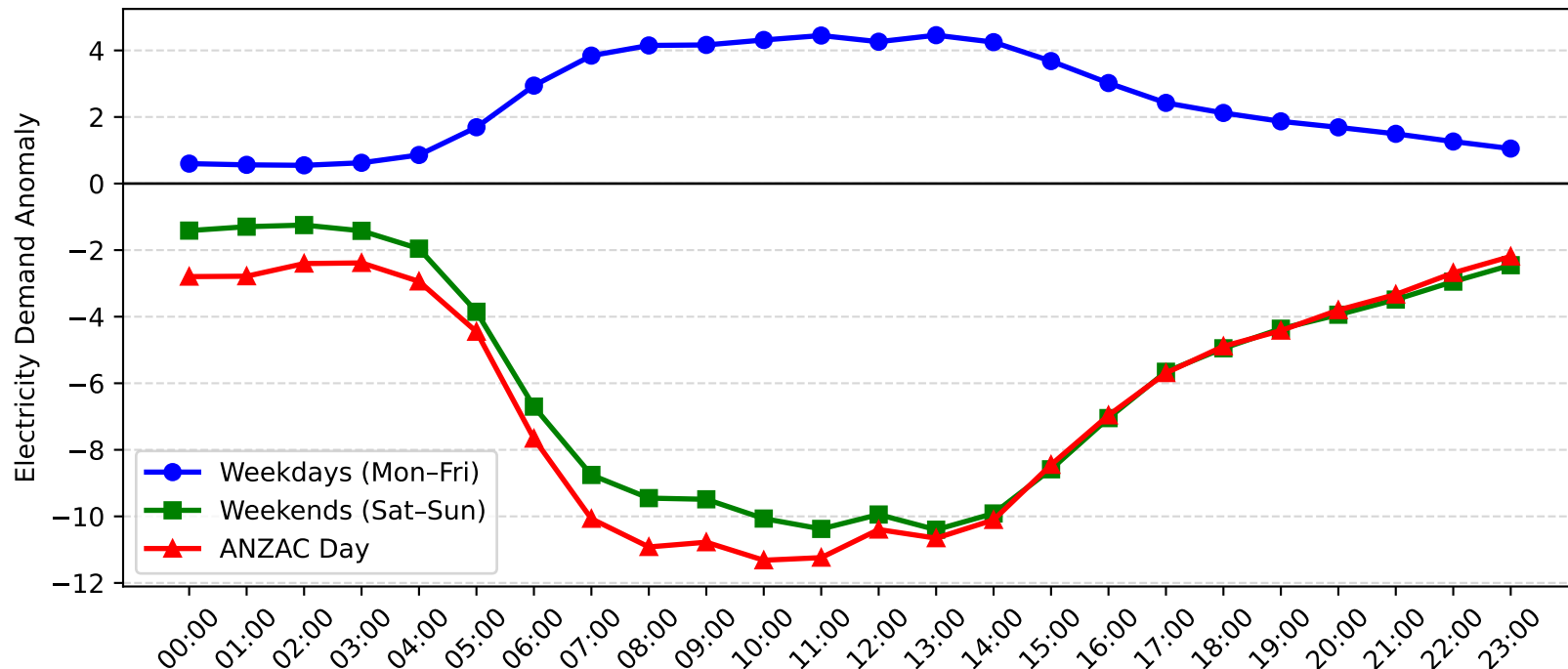
Milperra Demand Anomaly: ANZAC Day vs Weekday/Weekend (2015-2016)
