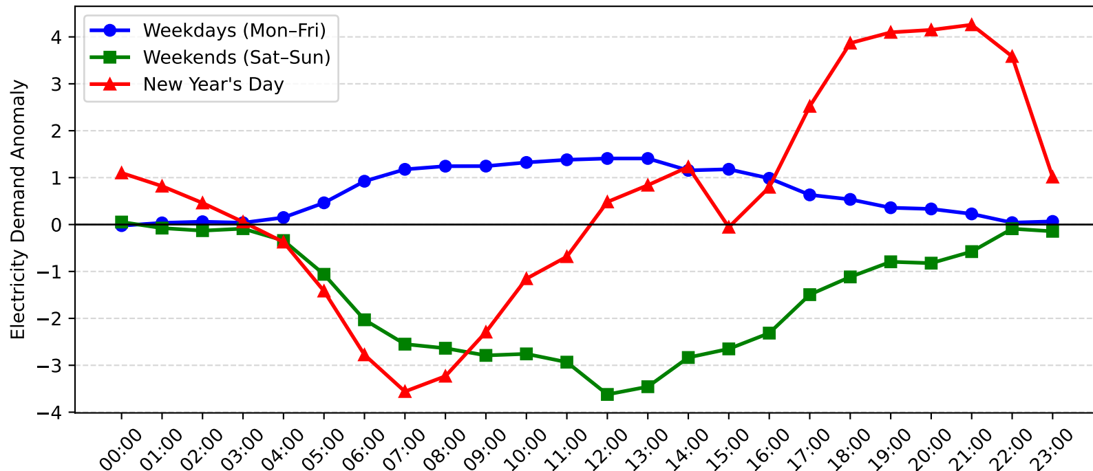
Wyong Demand Anomaly: New Year's Day vs Weekday/Weekend (2005-2006)
