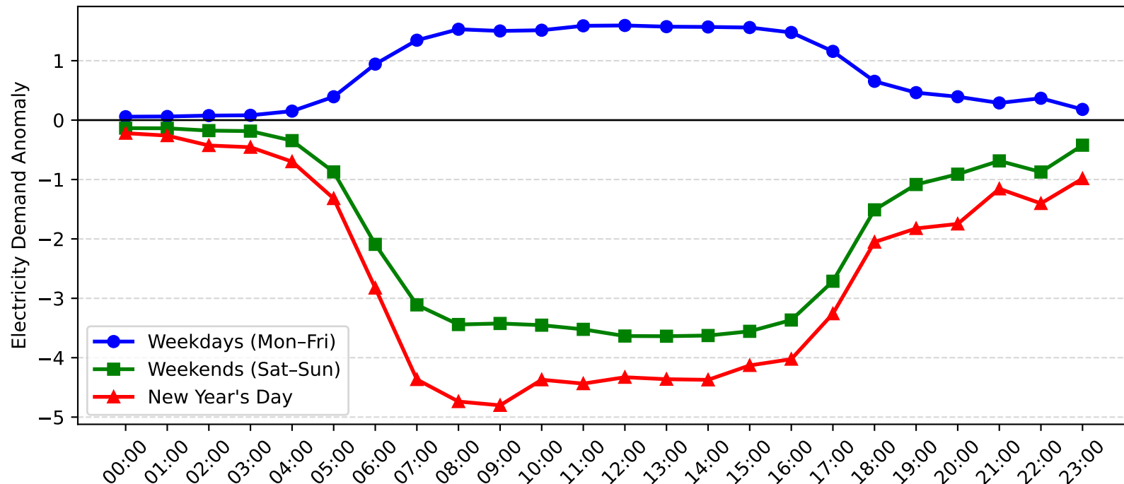
Beacon Hill Demand Anomaly: New Year's Day vs Weekday/Weekend (2011-2012)
