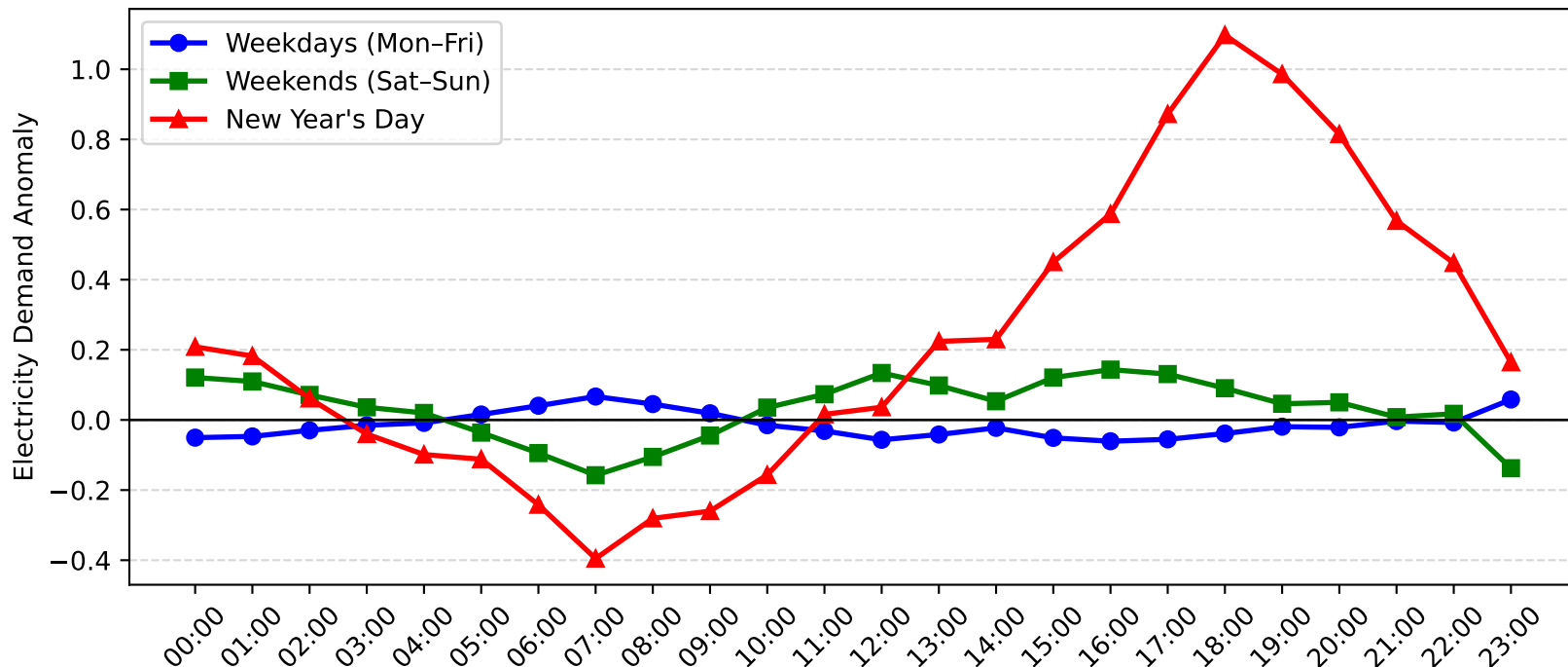
Rothbury Demand Anomaly: New Year's Day vs Weekday/Weekend (2012-2013)
