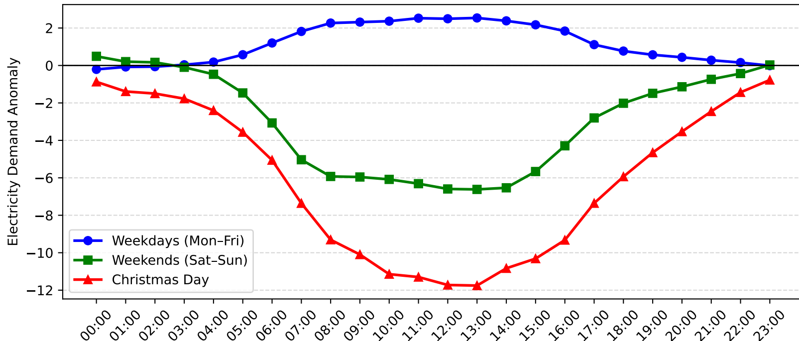
West Gosford Demand Anomaly: Christmas Day vs Weekday/Weekend (2009-2010)
