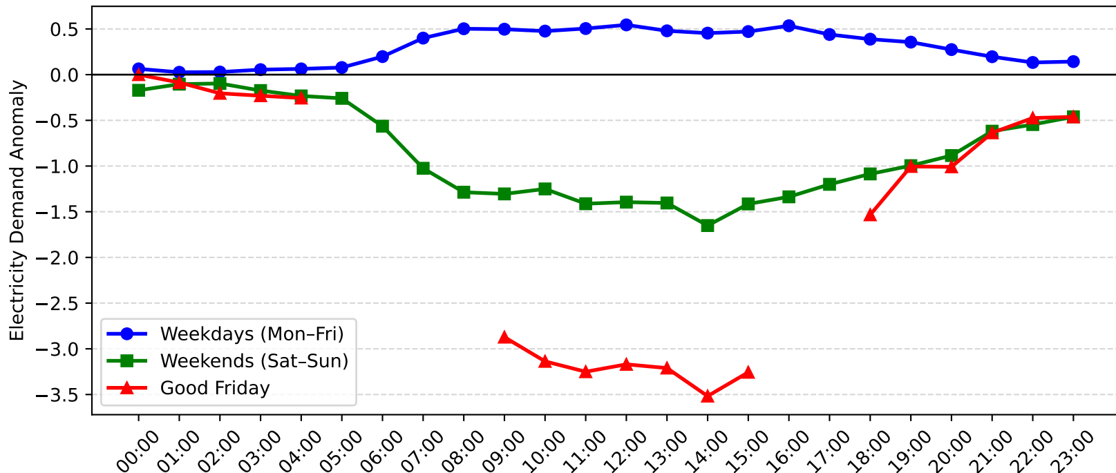
Green Square Demand Anomaly: Good Friday vs Weekday/Weekend (2006-2007)
