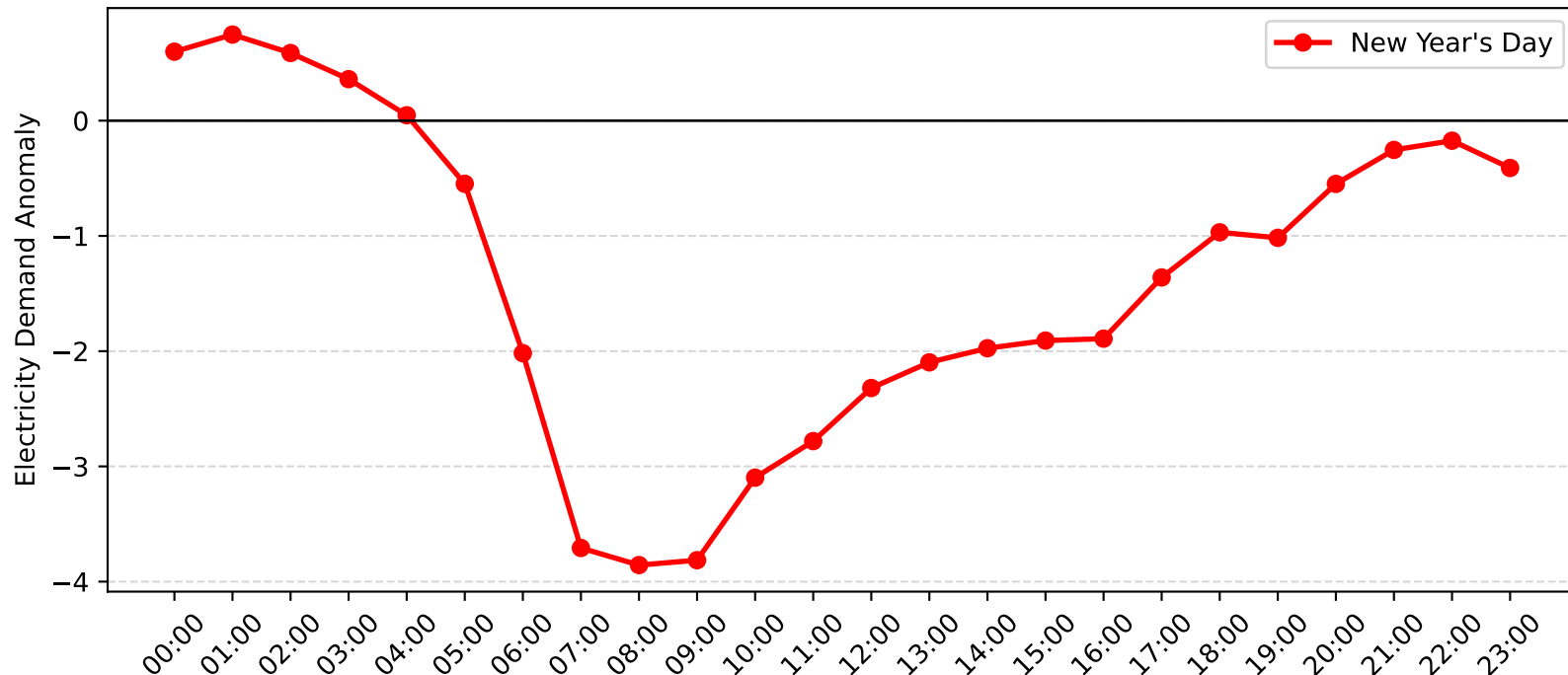
Pymble Demand Anomaly: New Year's Day (2012-2013)
