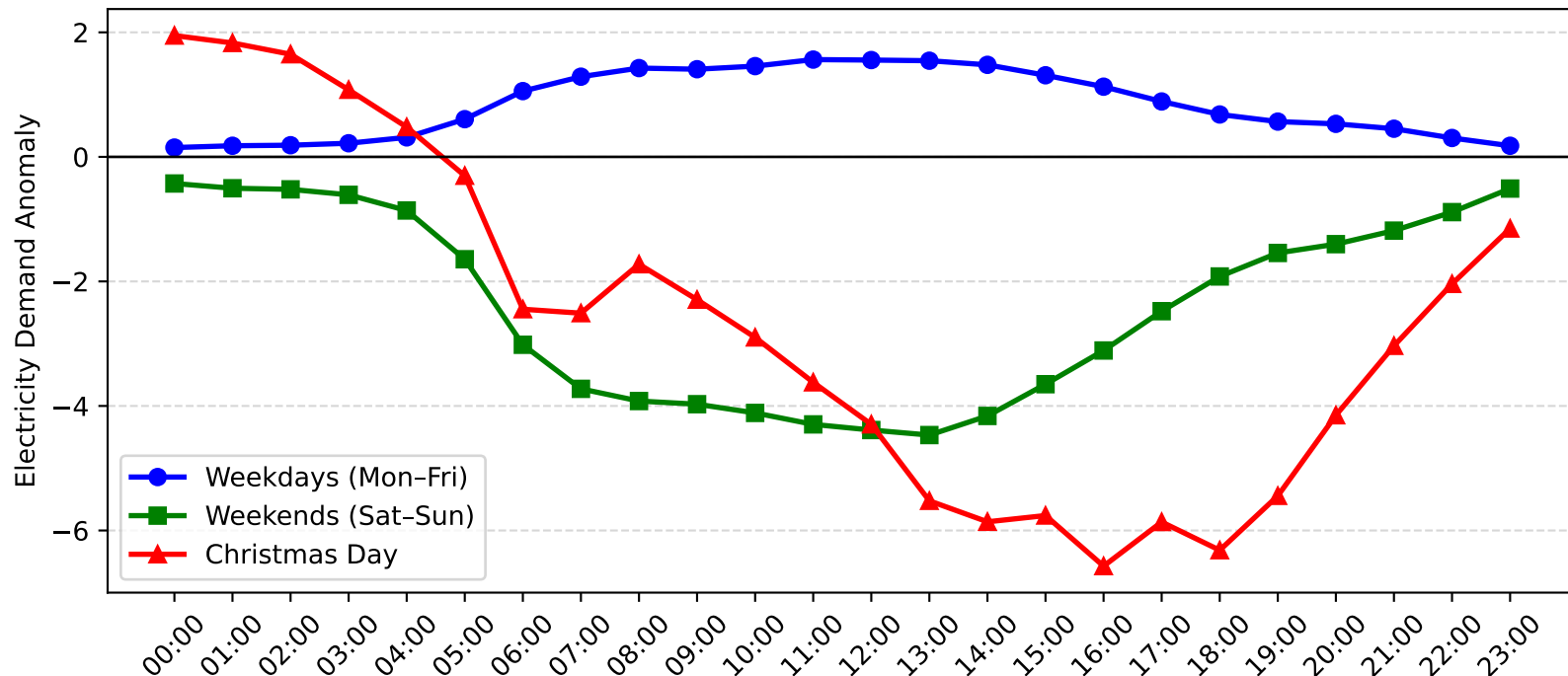
Wyong Demand Anomaly: Christmas Day vs Weekday/Weekend (2014-2015)
