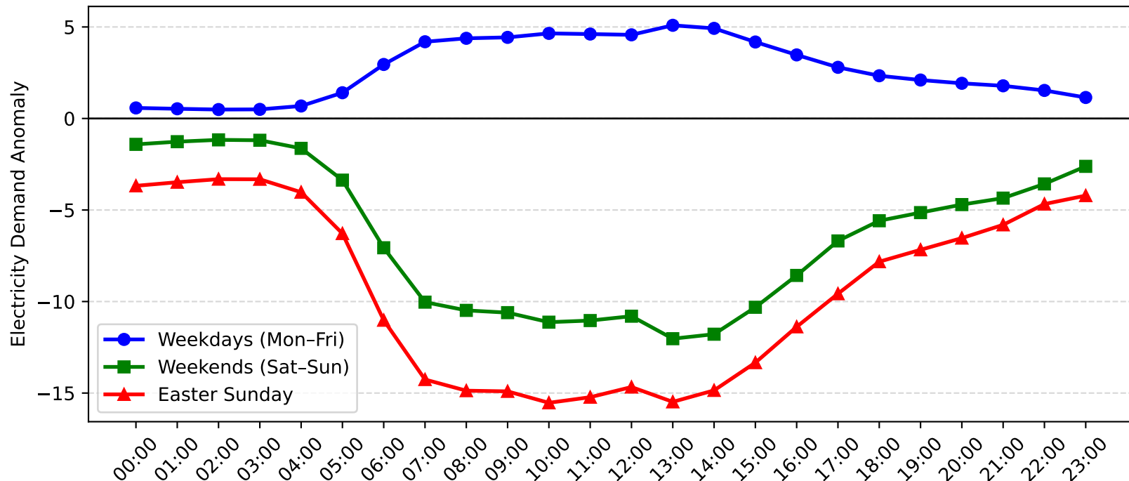
Milperra Demand Anomaly: Easter Sunday vs Weekday/Weekend (2007-2008)
