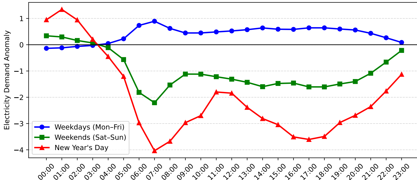
Mortdale Demand Anomaly: New Year's Day vs Weekday/Weekend (2016-2017)
