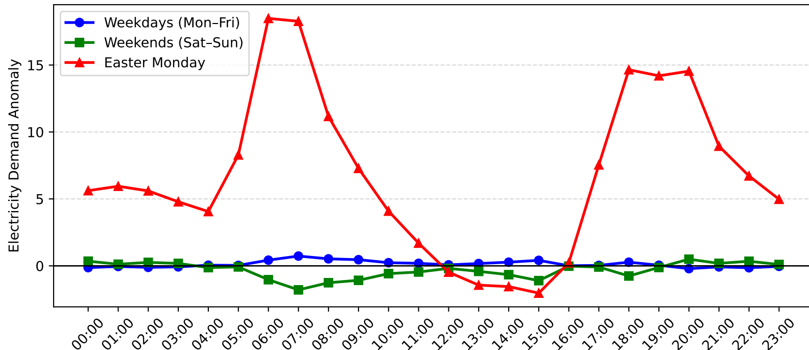
Pennant Hills Demand Anomaly: Easter Monday vs Weekday/Weekend (2004-2005)
