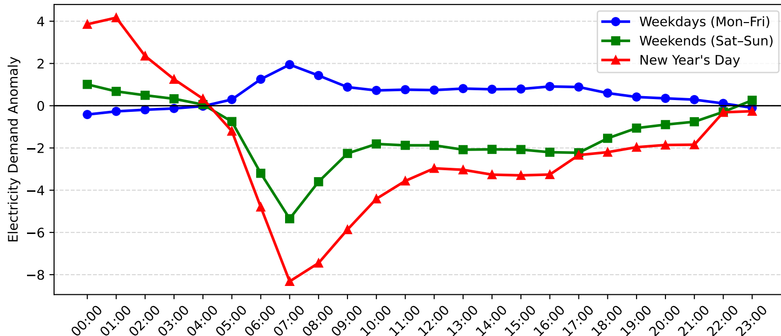
Mosman Demand Anomaly: New Year's Day vs Weekday/Weekend (2010-2011)
