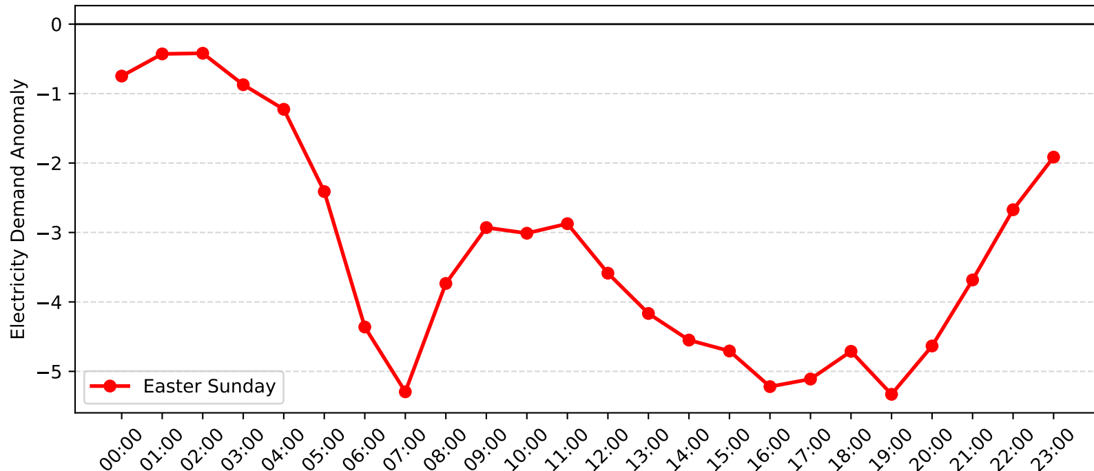
Mortdale Demand Anomaly: Easter Sunday (2009-2010)
