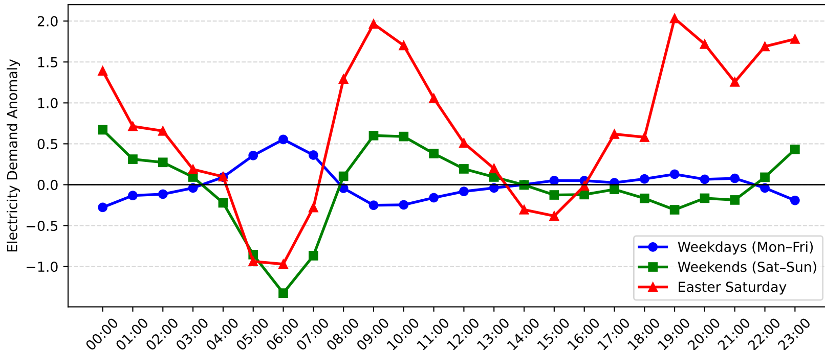
Umina Demand Anomaly: Easter Saturday vs Weekday/Weekend (2007-2008)
