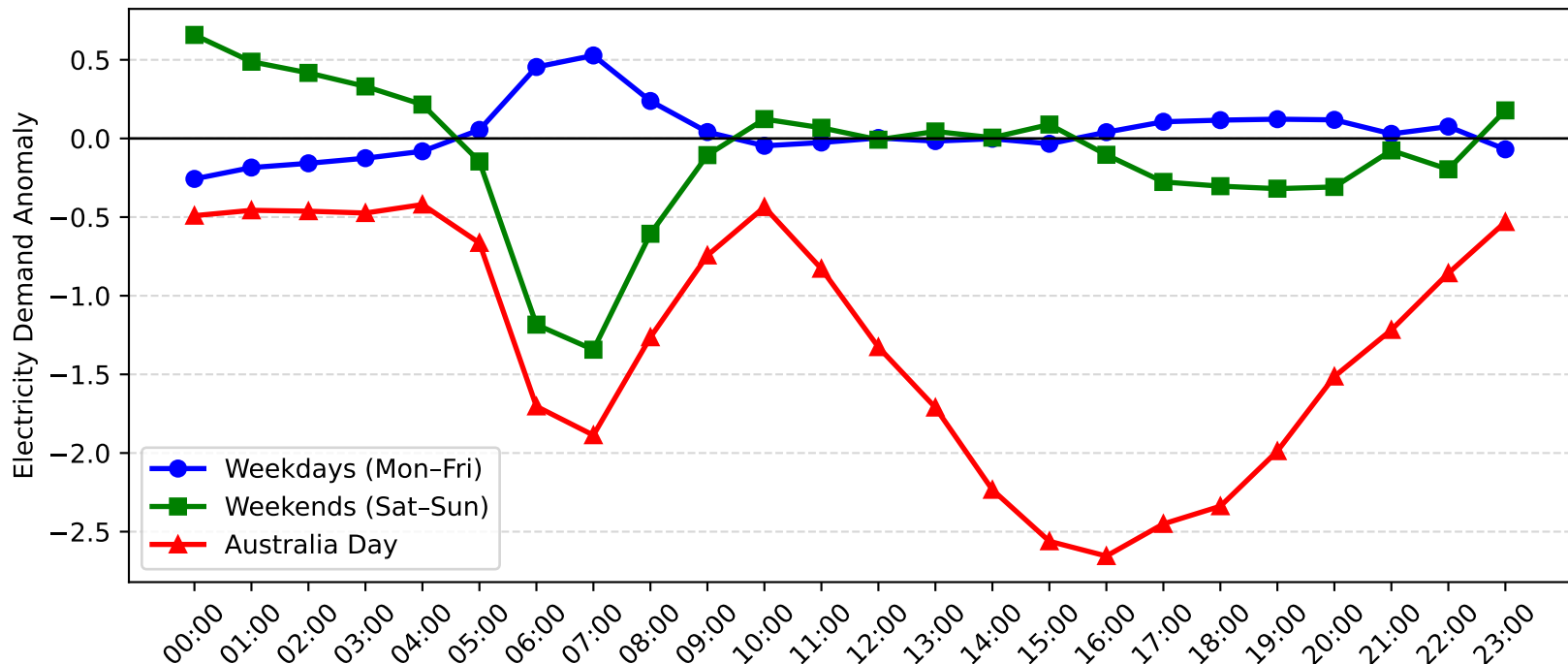
Balgowlah North Demand Anomaly: Australia Day vs Weekday/Weekend (2016-2017)
