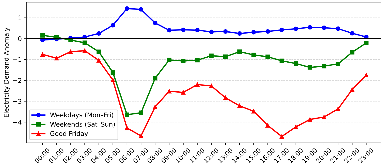
Revesby Demand Anomaly: Good Friday vs Weekday/Weekend (2013-2014)
