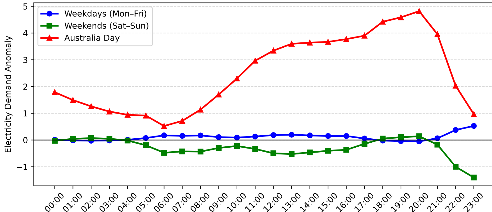
Muswellbrook Demand Anomaly: Australia Day vs Weekday/Weekend (2010-2011)
