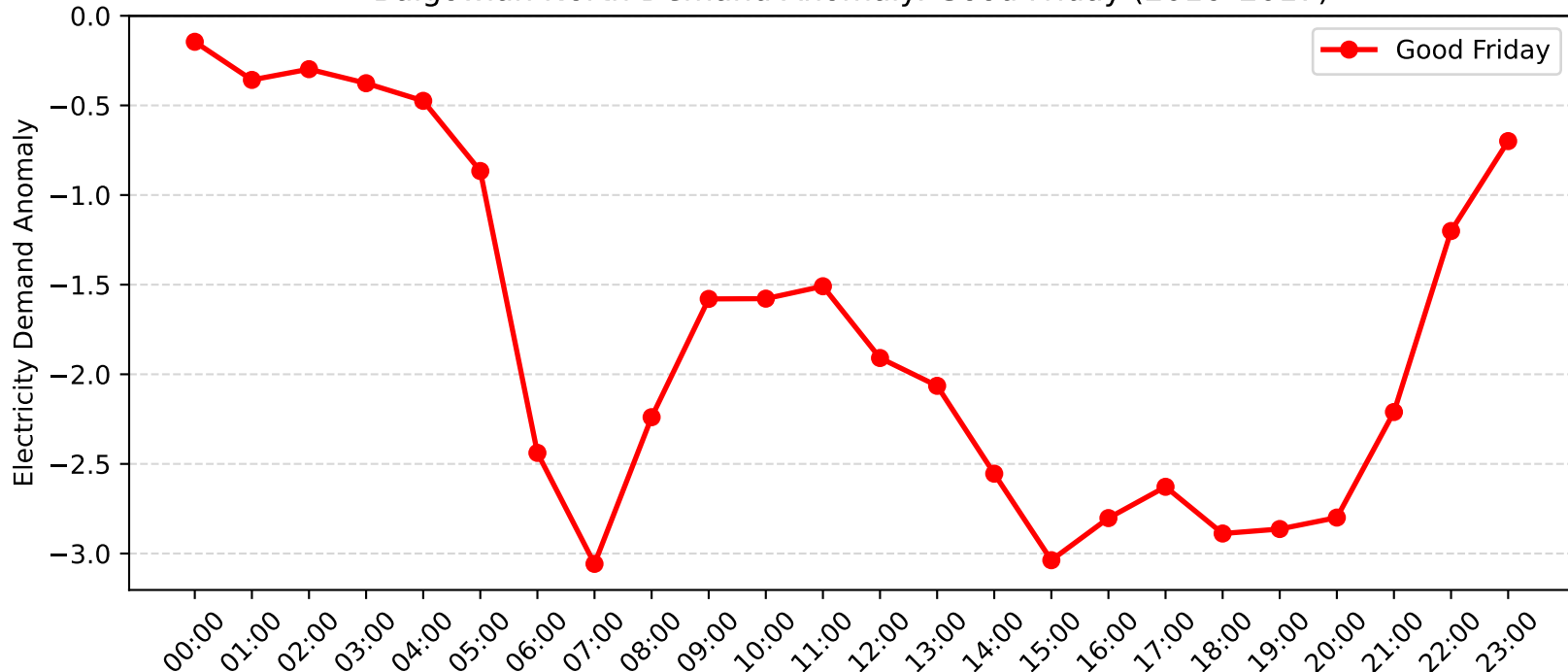
Balgowlah North Demand Anomaly: Good Friday (2016-2017)
