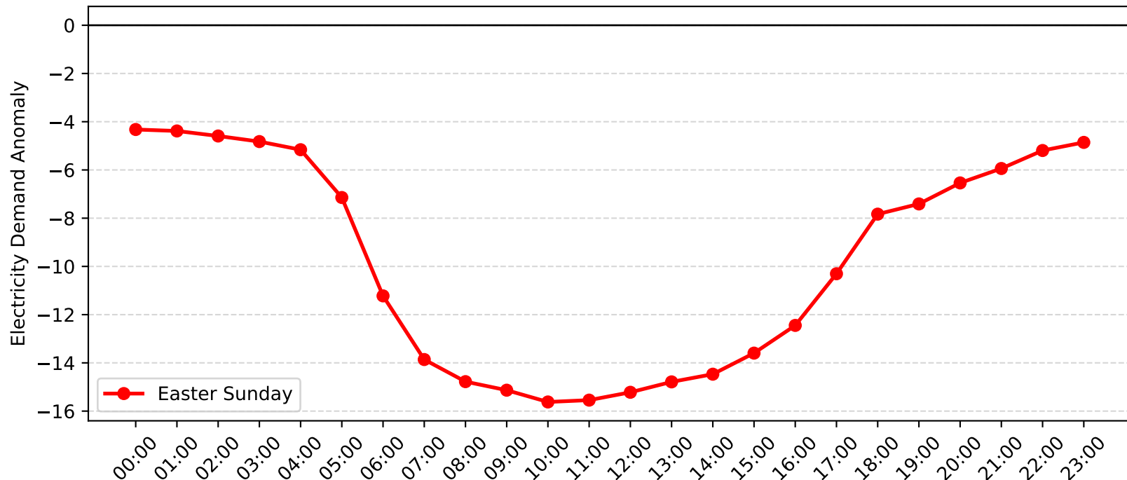
Flemington Demand Anomaly: Easter Sunday (2011-2012)
