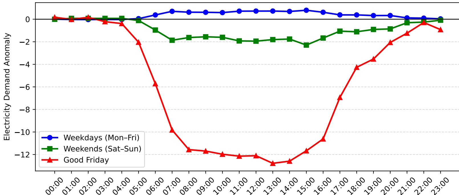
Brookvale Demand Anomaly: Good Friday vs Weekday/Weekend (2004-2005)
