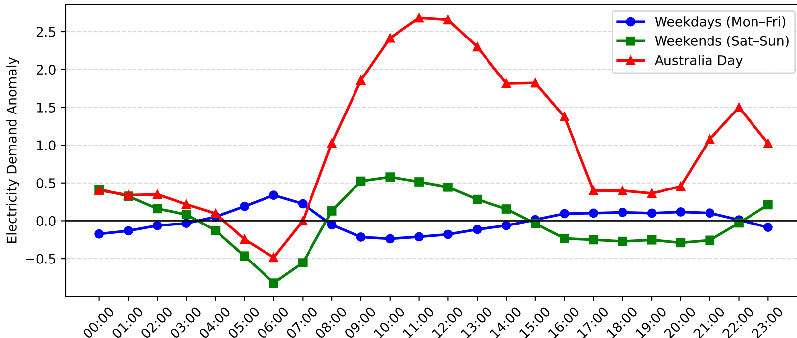
Umina Demand Anomaly: Australia Day vs Weekday/Weekend (2012-2013)
