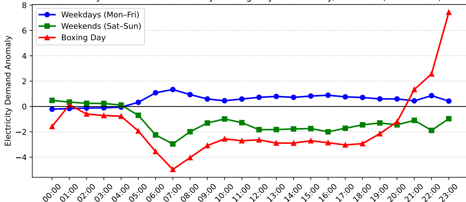
Dee Why West Demand Anomaly: Boxing Day vs Weekday/Weekend (2004-2005)
