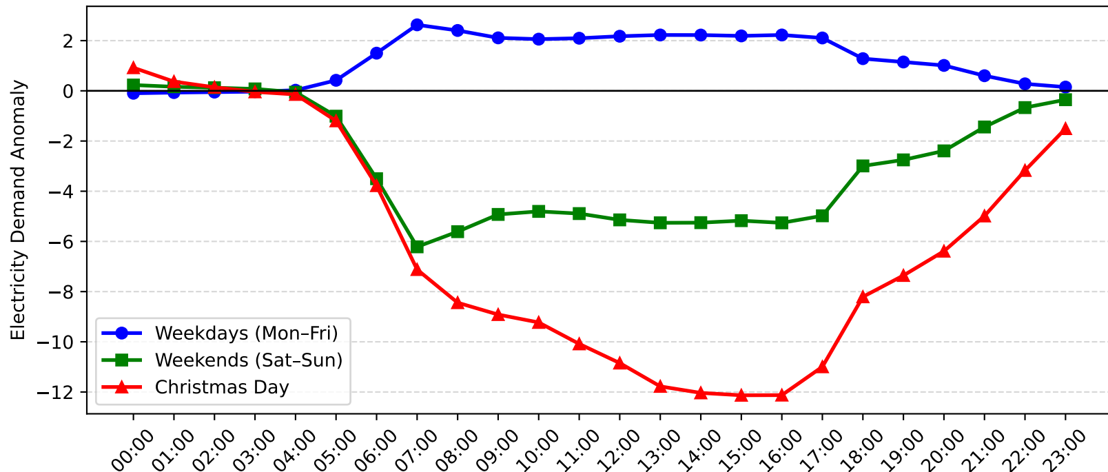
Epping Demand Anomaly: Christmas Day vs Weekday/Weekend (2011-2012)
