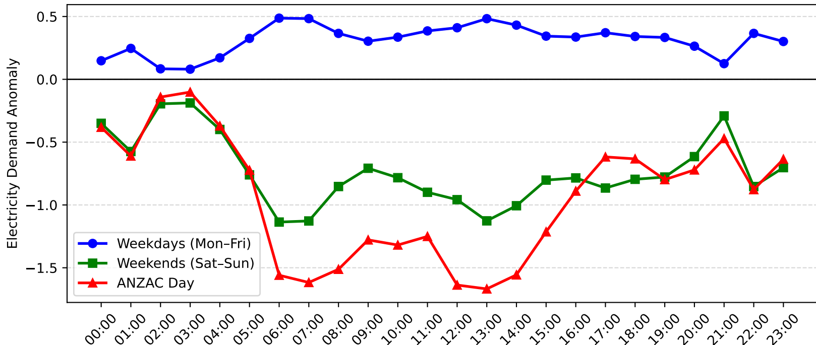
Gateshead Demand Anomaly: ANZAC Day vs Weekday/Weekend (2016-2017)
