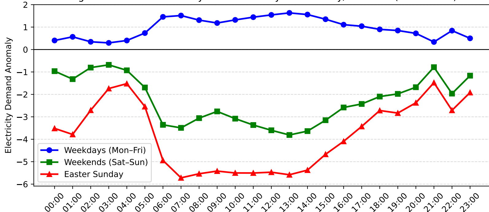
Argenton Demand Anomaly: Easter Sunday vs Weekday/Weekend (2011-2012)
