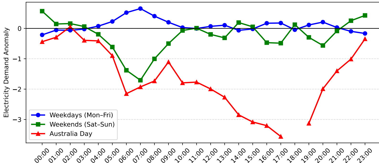
Charmhaven Demand Anomaly: Australia Day vs Weekday/Weekend (2005-2006)
