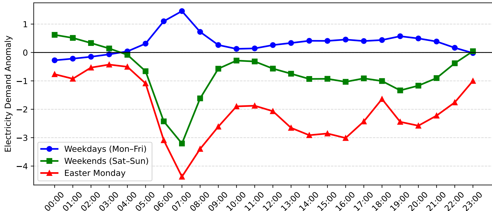
Five Dock Demand Anomaly: Easter Monday vs Weekday/Weekend (2010-2011)
