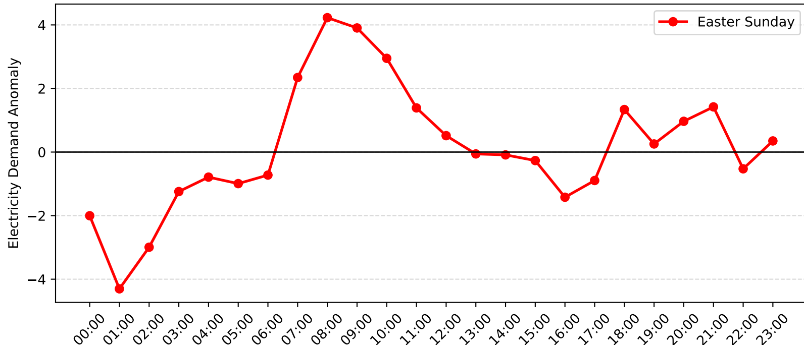
Nelson Bay Demand Anomaly: Easter Sunday (2005-2006)
