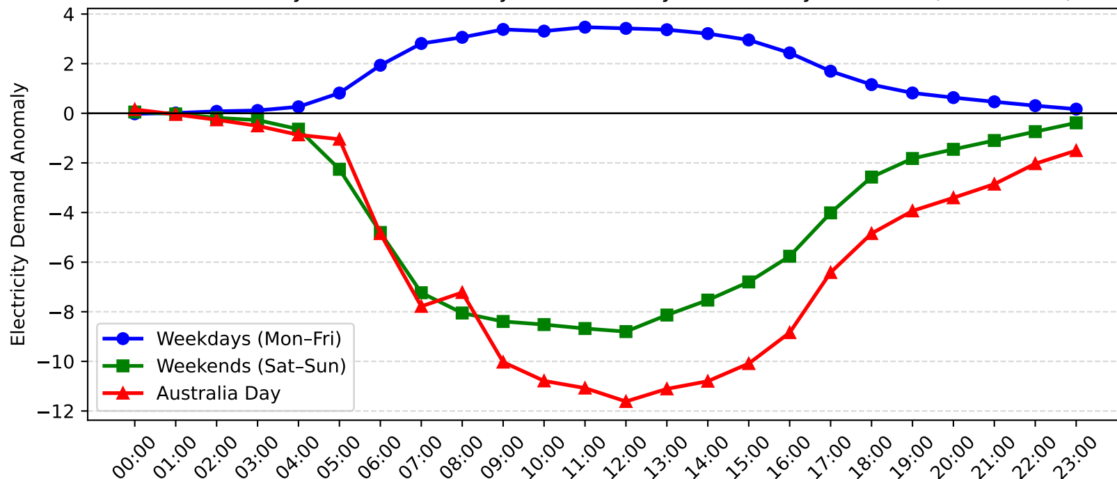
Homebush Bay Demand Anomaly: Australia Day vs Weekday/Weekend (2014-2015)
