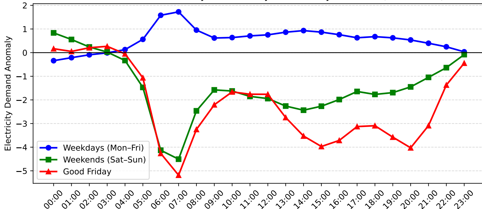
Mortdale Demand Anomaly: Good Friday vs Weekday/Weekend (2007-2008)
