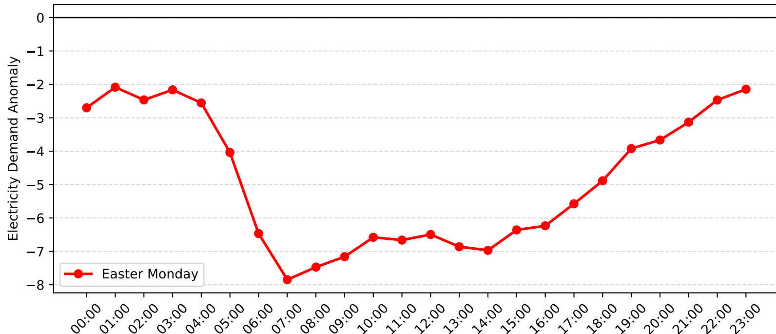
Sefton Demand Anomaly: Easter Monday (2013-2014)
