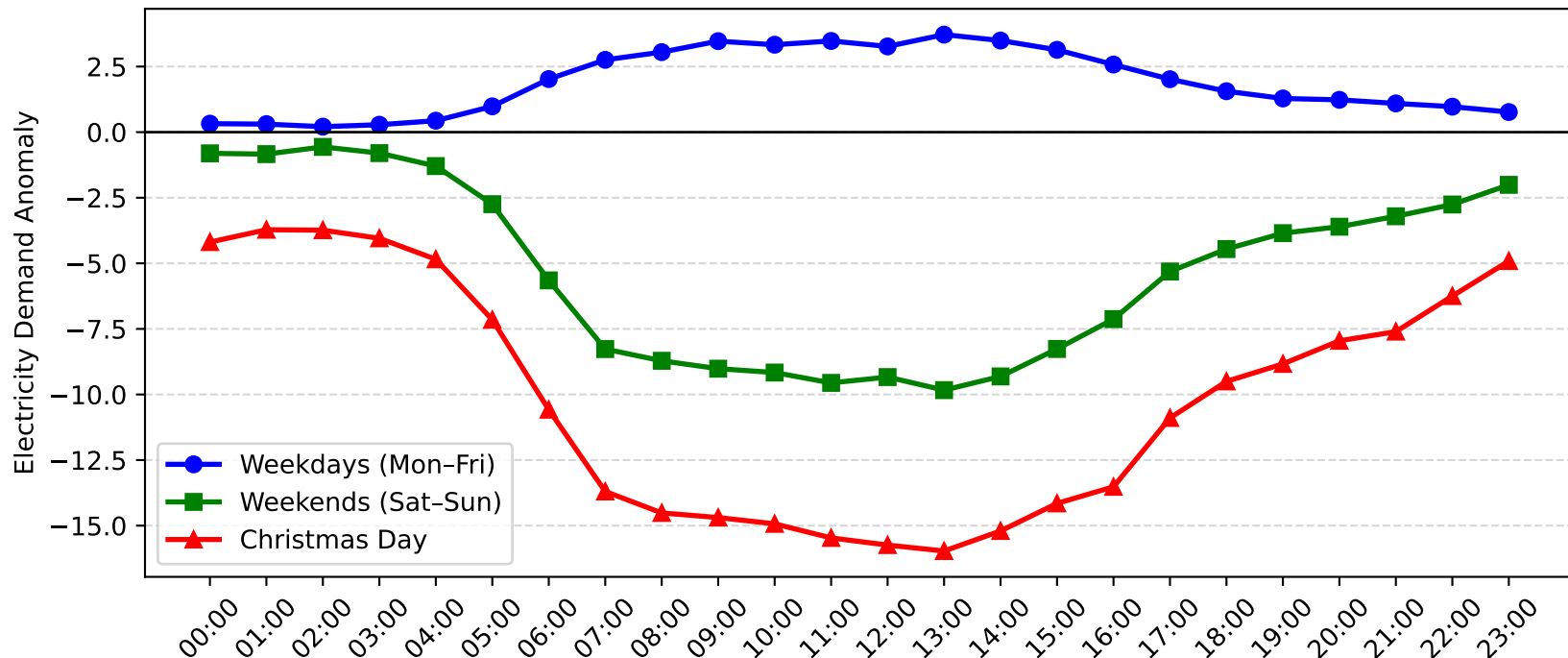
Milperra Demand Anomaly: Christmas Day vs Weekday/Weekend (2007-2008)
