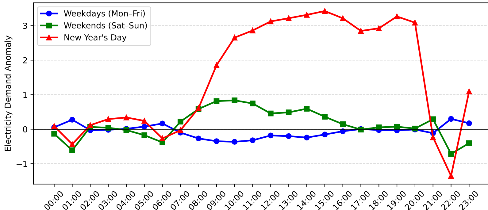
Swansea Demand Anomaly: New Year's Day vs Weekday/Weekend (2006-2007)
