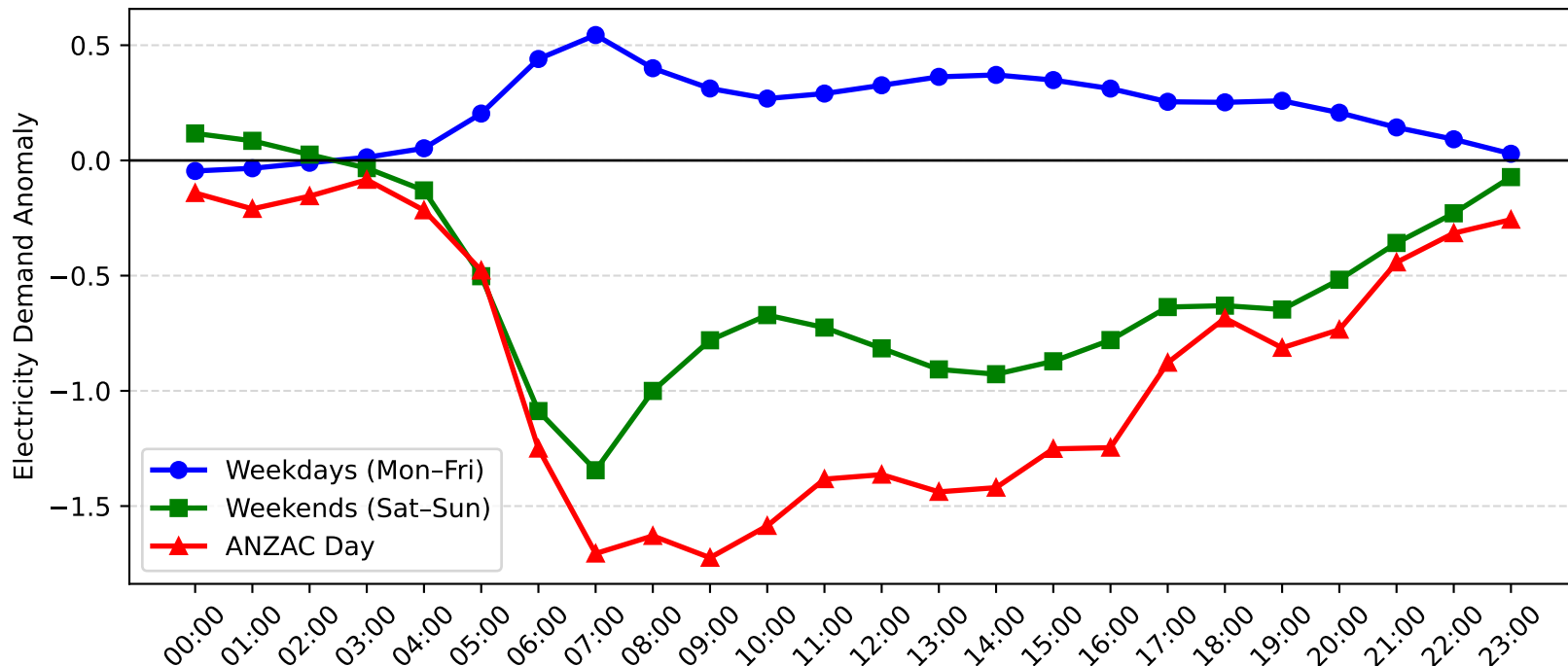
Rockdale Demand Anomaly: ANZAC Day vs Weekday/Weekend (2011-2012)
