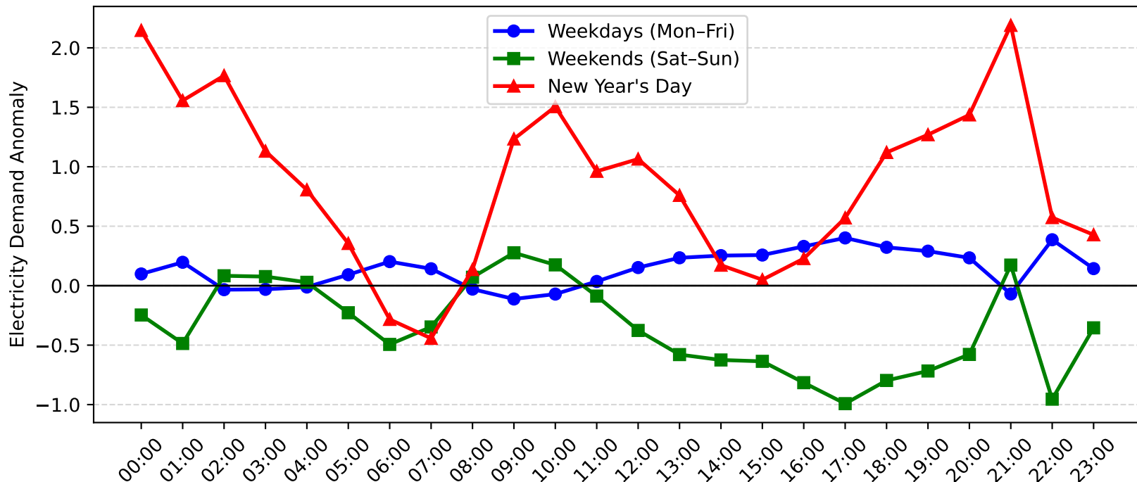
Nelson Bay Demand Anomaly: New Year's Day vs Weekday/Weekend (2016-2017)
