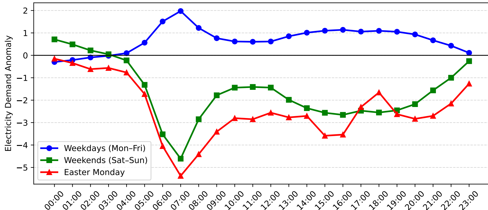
Kogarah Demand Anomaly: Easter Monday vs Weekday/Weekend (2014-2015)
