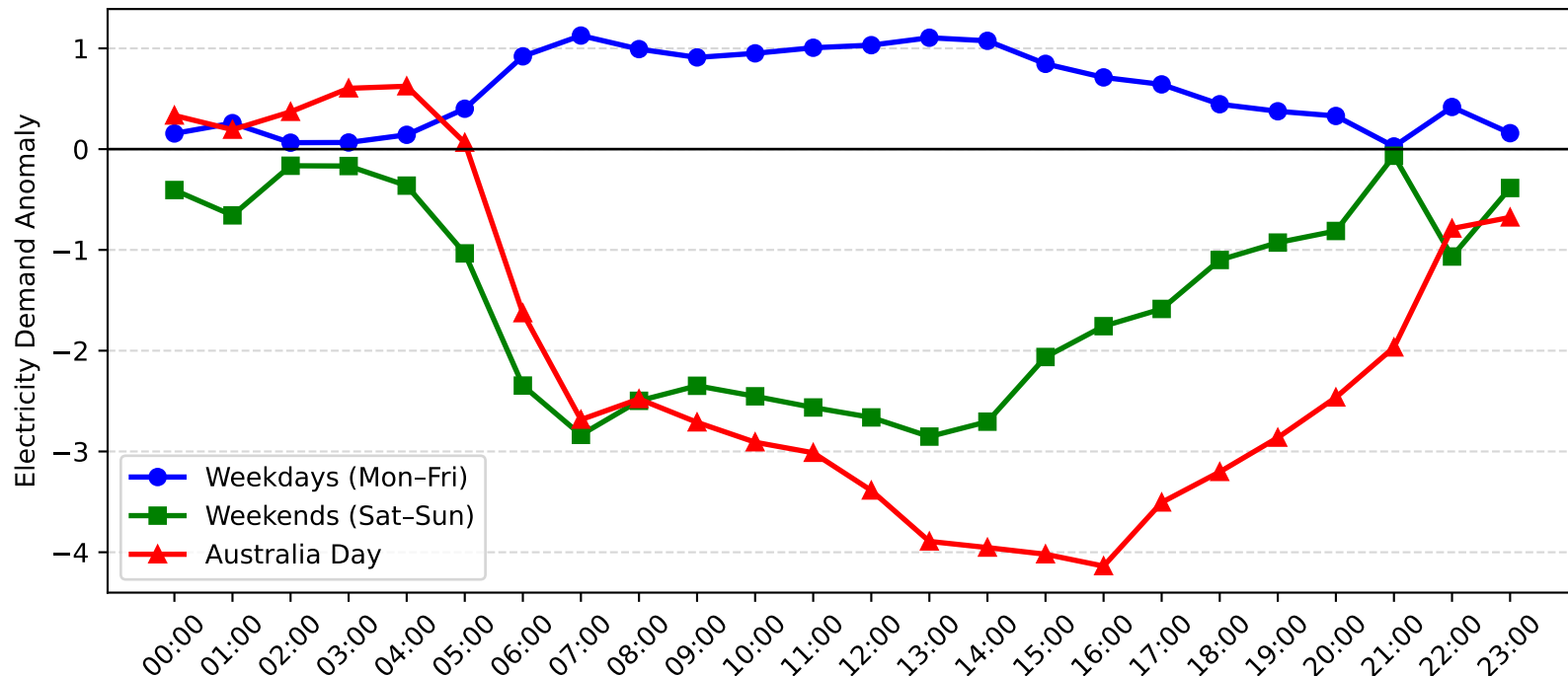
Argenton Demand Anomaly: Australia Day vs Weekday/Weekend (2015-2016)
