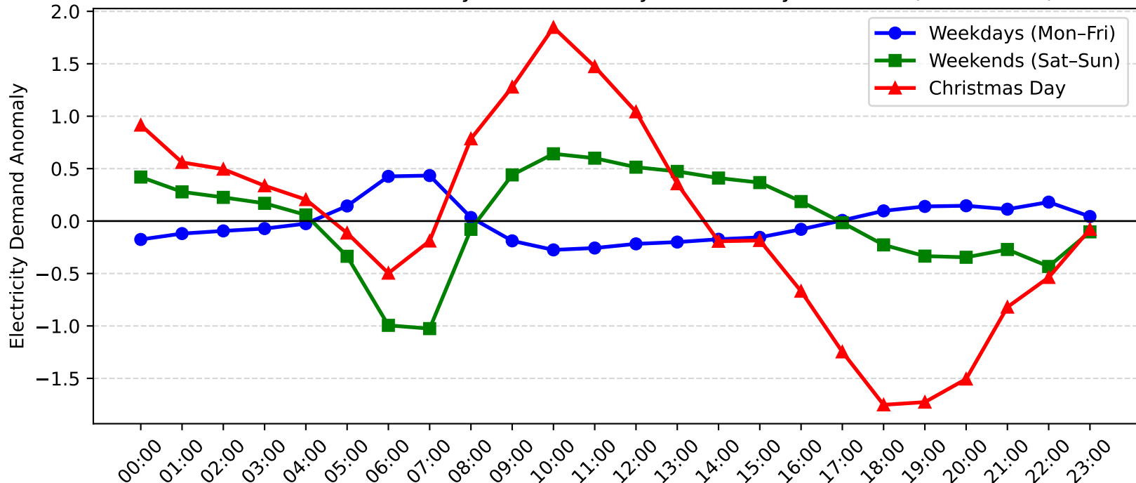
Harbord Demand Anomaly: Christmas Day vs Weekday/Weekend (2011-2012)
