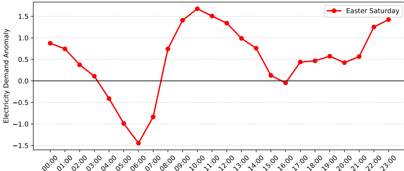
Umina Demand Anomaly: Easter Saturday (2010-2011)
