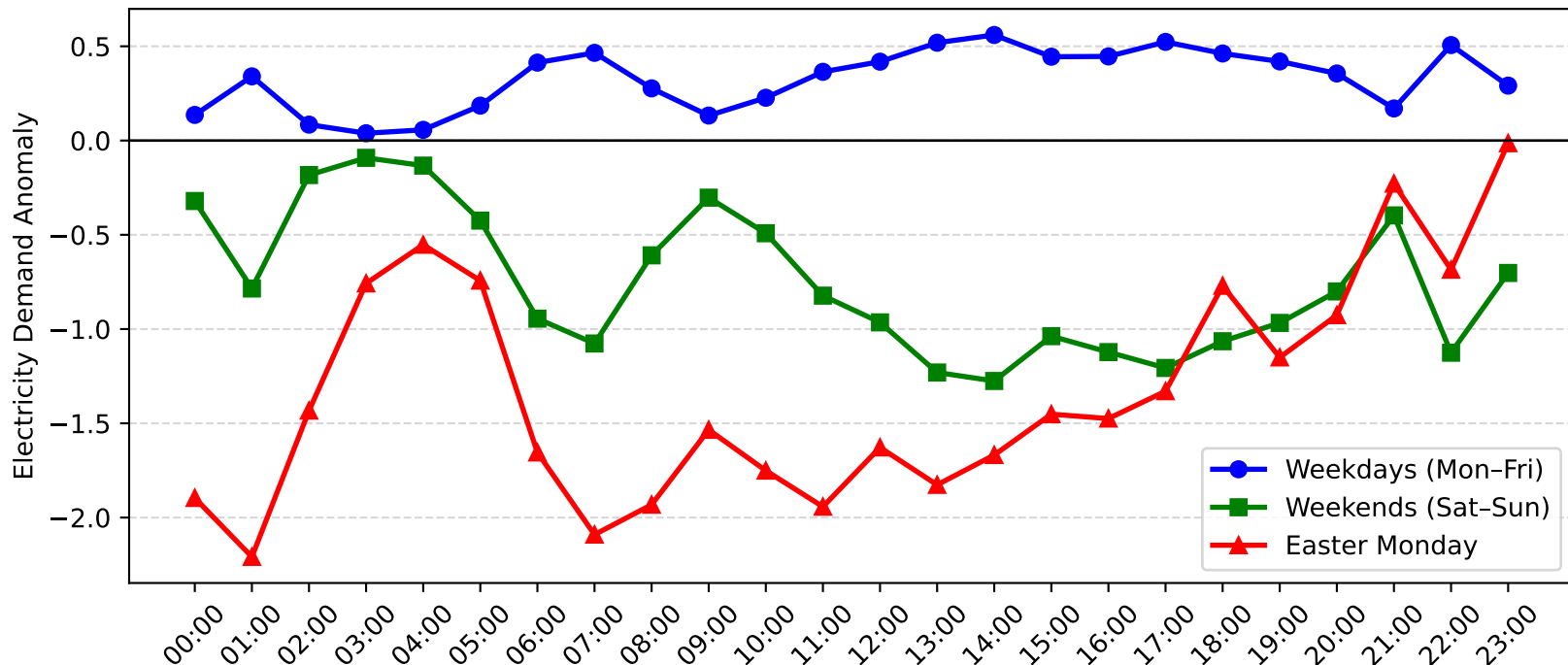
Gateshead Demand Anomaly: Easter Monday vs Weekday/Weekend (2005-2006)
