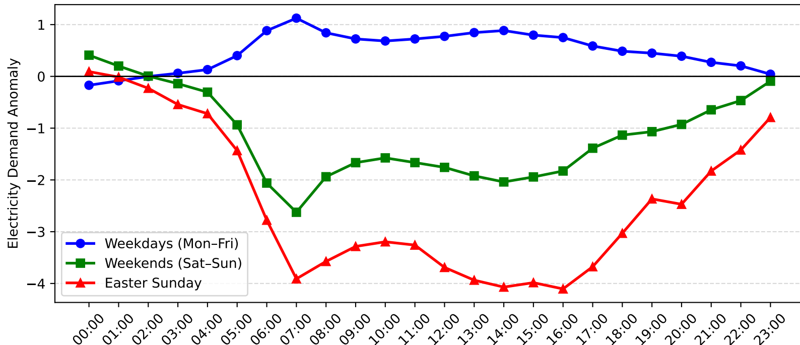
Rockdale Demand Anomaly: Easter Sunday vs Weekday/Weekend (2007-2008)
