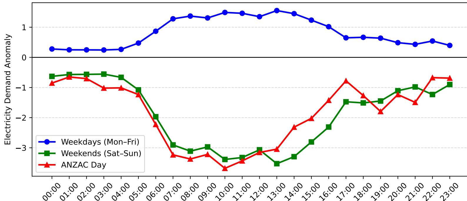
Mayfield West Demand Anomaly: ANZAC Day vs Weekday/Weekend (2017-2018)
