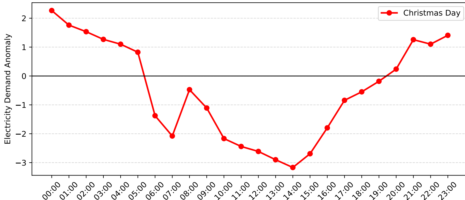
Broadmeadow Demand Anomaly: Christmas Day (2014-2015)
