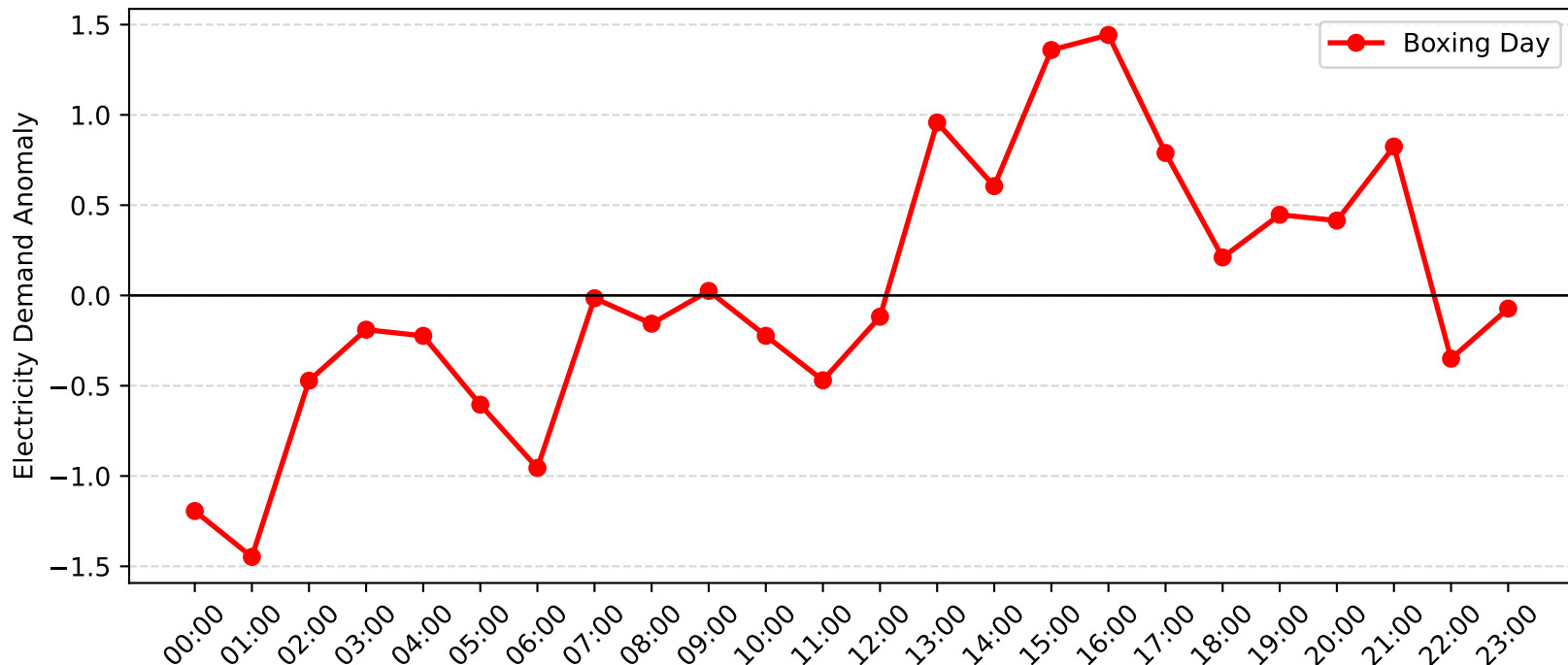
Nelson Bay Demand Anomaly: Boxing Day (2014-2015)
