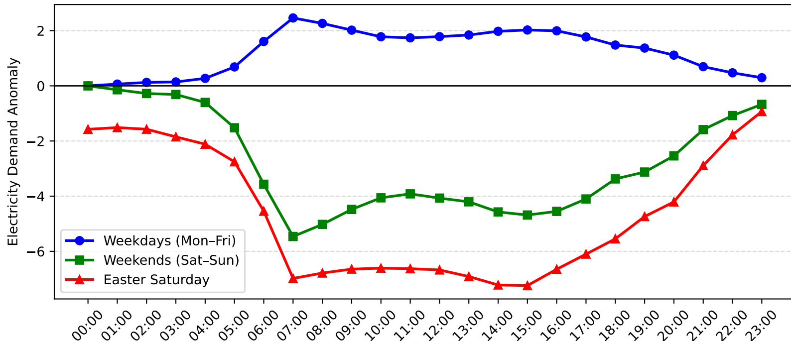
Burwood Demand Anomaly: Easter Saturday vs Weekday/Weekend (2016-2017)
