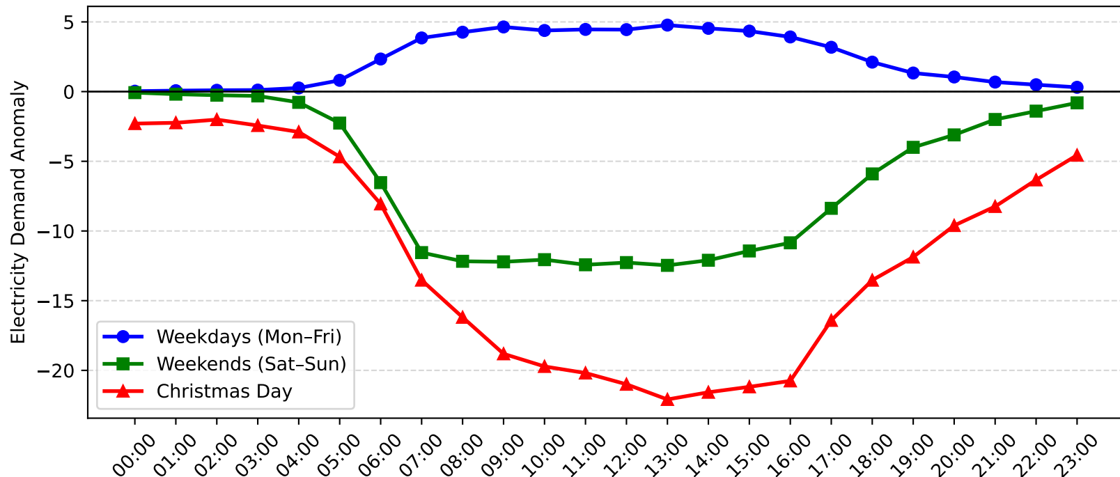
Zetland Demand Anomaly: Christmas Day vs Weekday/Weekend (2007-2008)
