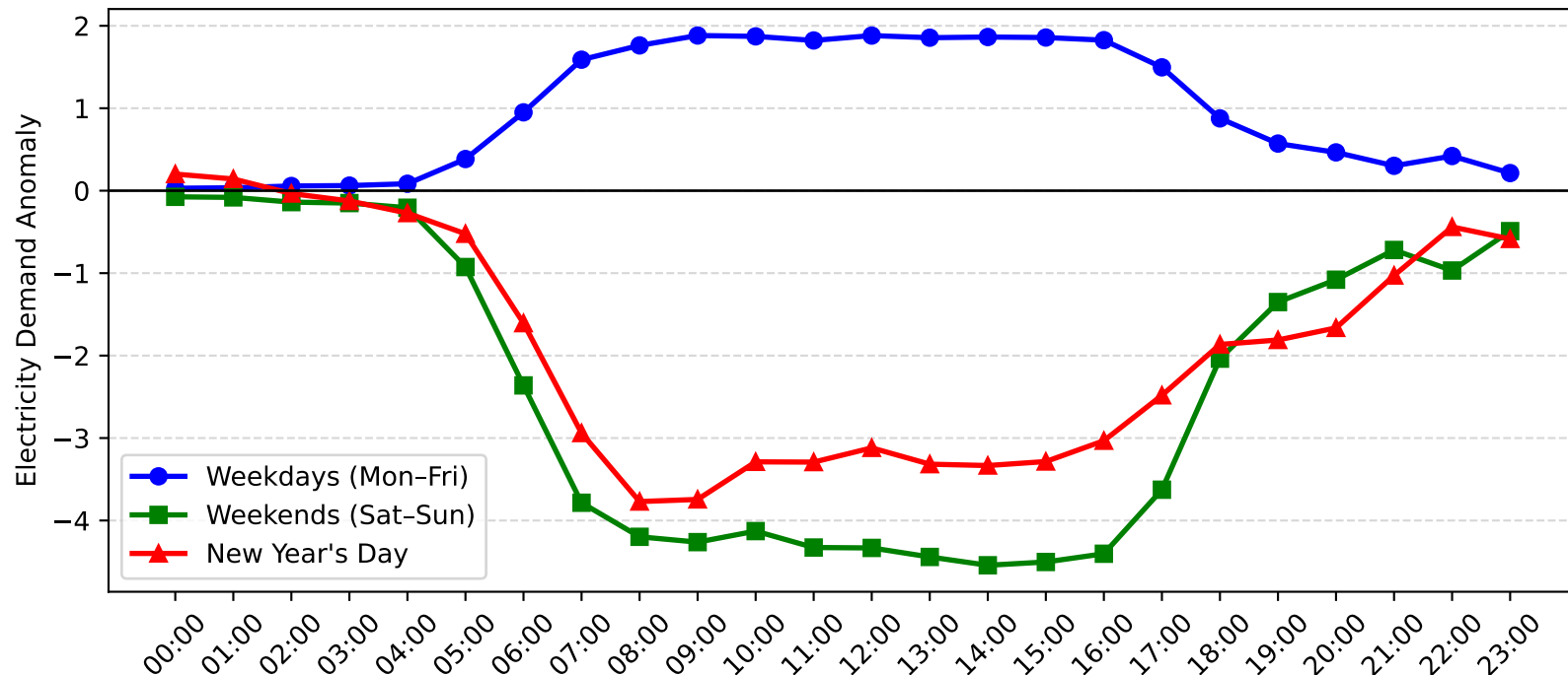
Beacon Hill Demand Anomaly: New Year's Day vs Weekday/Weekend (2007-2008)
