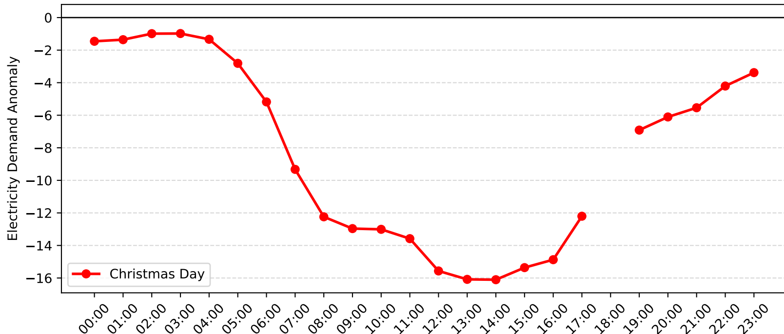
Gore Hill Demand Anomaly: Christmas Day (2016-2017)
