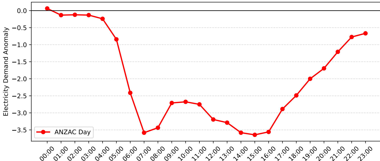
Beacon Hill Demand Anomaly: ANZAC Day (2008-2009)
