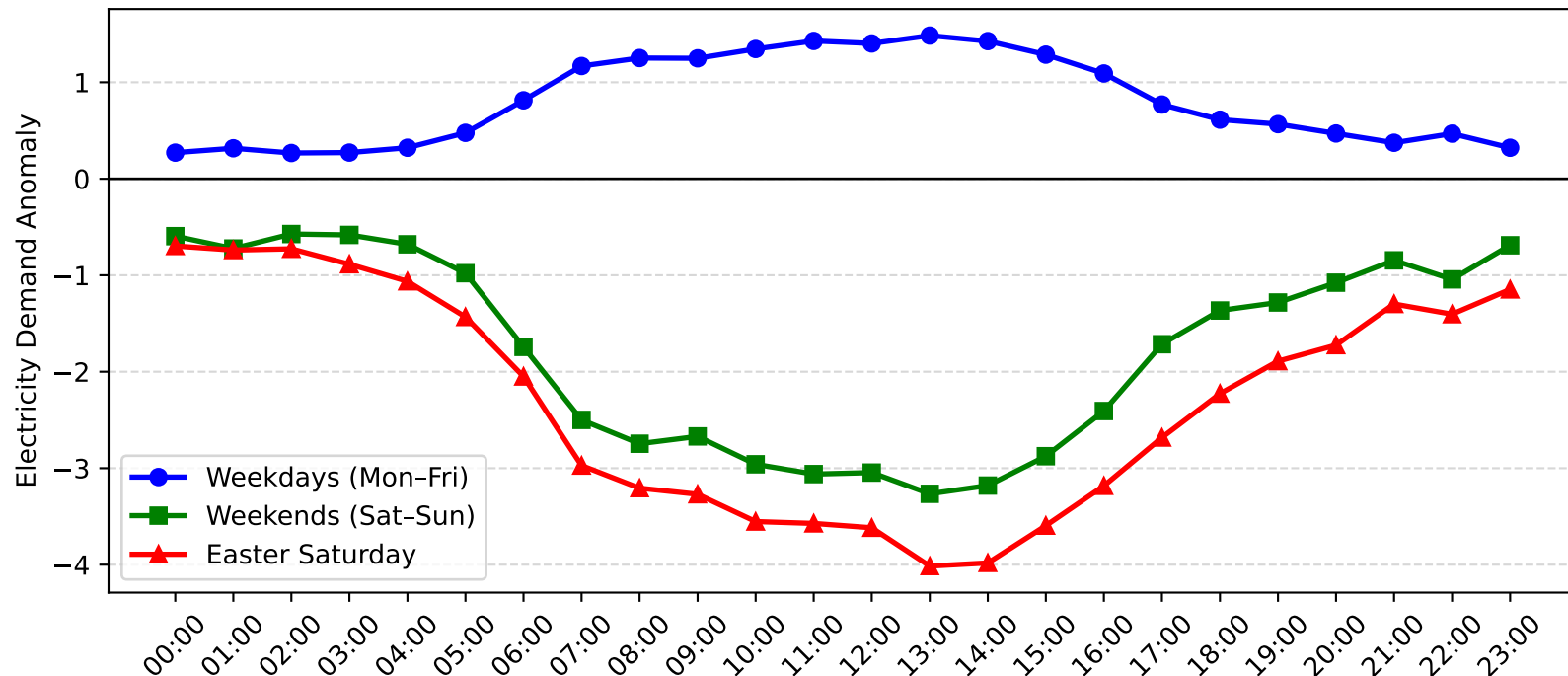
Mayfield West Demand Anomaly: Easter Saturday vs Weekday/Weekend (2010-2011)
