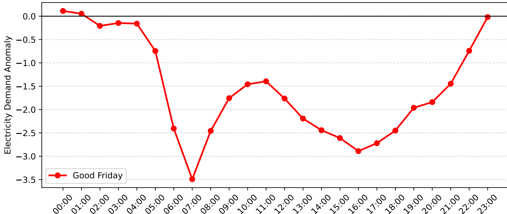
Blakehurst Demand Anomaly: Good Friday (2005-2006)
