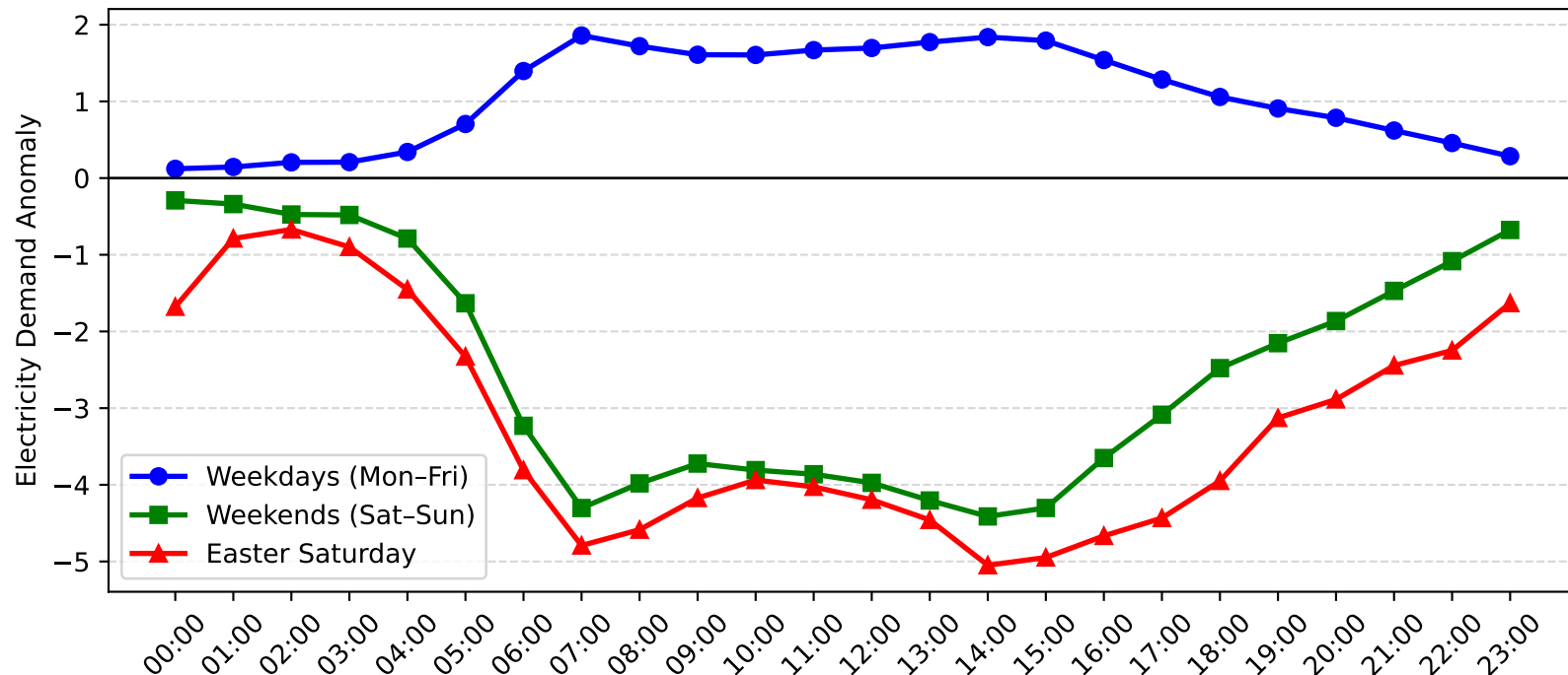
Sefton Demand Anomaly: Easter Saturday vs Weekday/Weekend (2015-2016)
