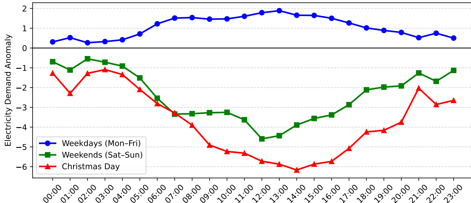
Cardiff Demand Anomaly: Christmas Day vs Weekday/Weekend (2004-2005)
