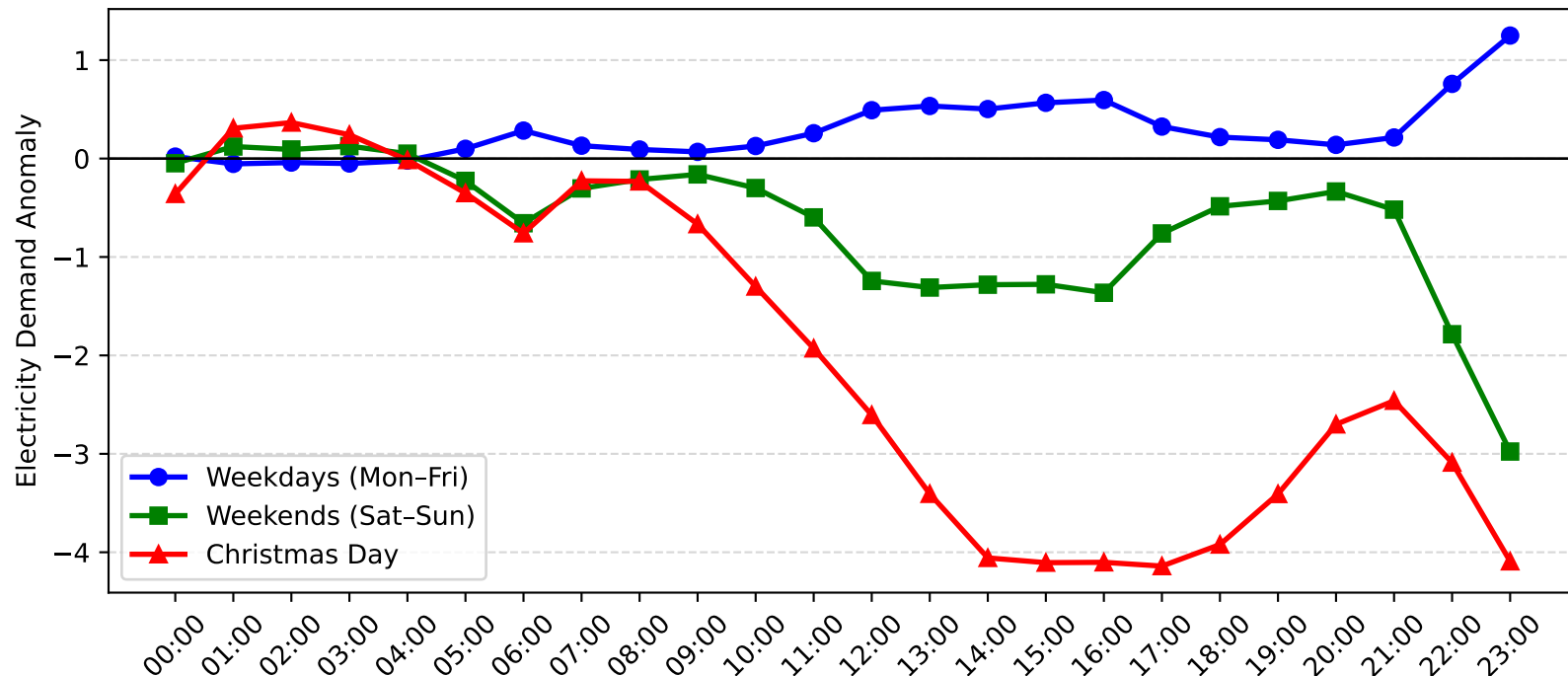
Muswellbrook Demand Anomaly: Christmas Day vs Weekday/Weekend (2005-2006)
