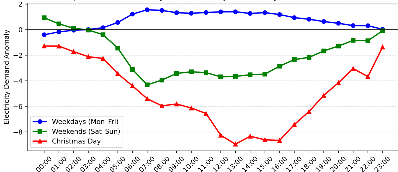
Campsie Demand Anomaly: Christmas Day vs Weekday/Weekend (2009-2010)
