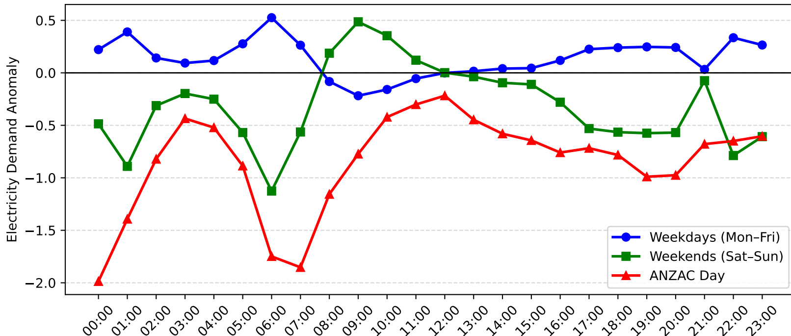
Morisset Demand Anomaly: ANZAC Day vs Weekday/Weekend (2010-2011)
