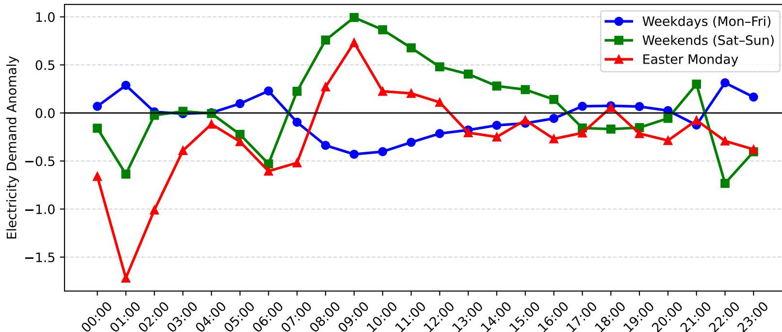
Swansea Demand Anomaly: Easter Monday vs Weekday/Weekend (2006-2007)
