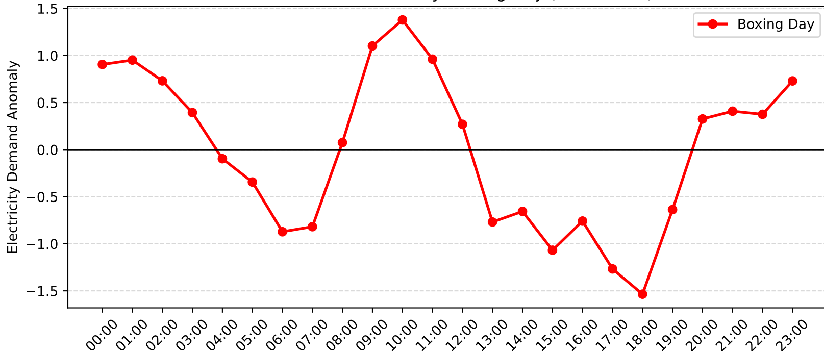
Avoca Demand Anomaly: Boxing Day (2011-2012)
