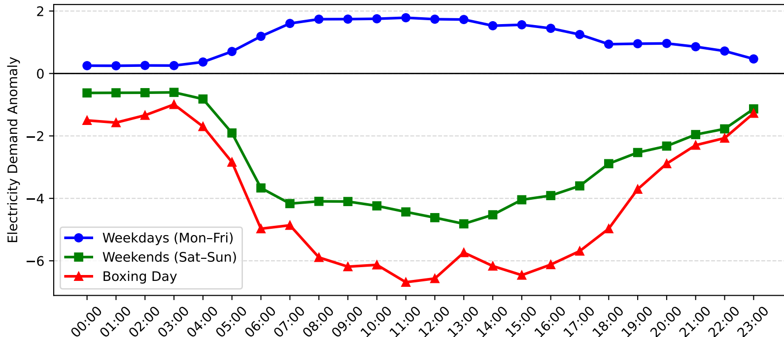
Potts Hill Demand Anomaly: Boxing Day vs Weekday/Weekend (2014-2015)
