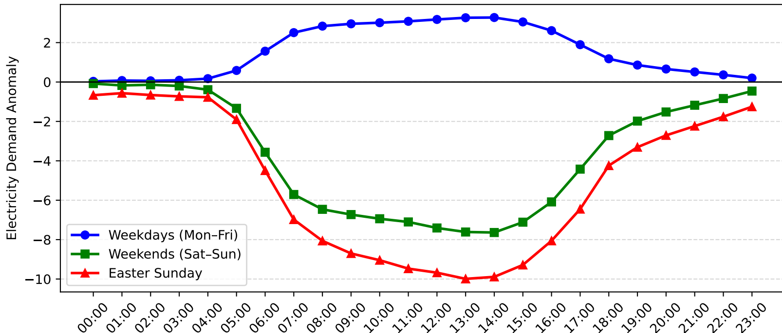
Mascot Demand Anomaly: Easter Sunday vs Weekday/Weekend (2015-2016)
