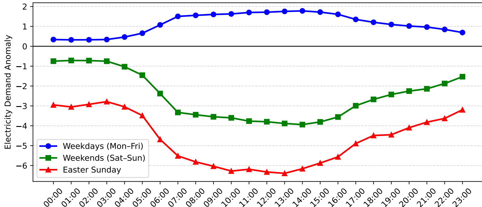
Leightonfield Demand Anomaly: Easter Sunday vs Weekday/Weekend (2017-2018)
