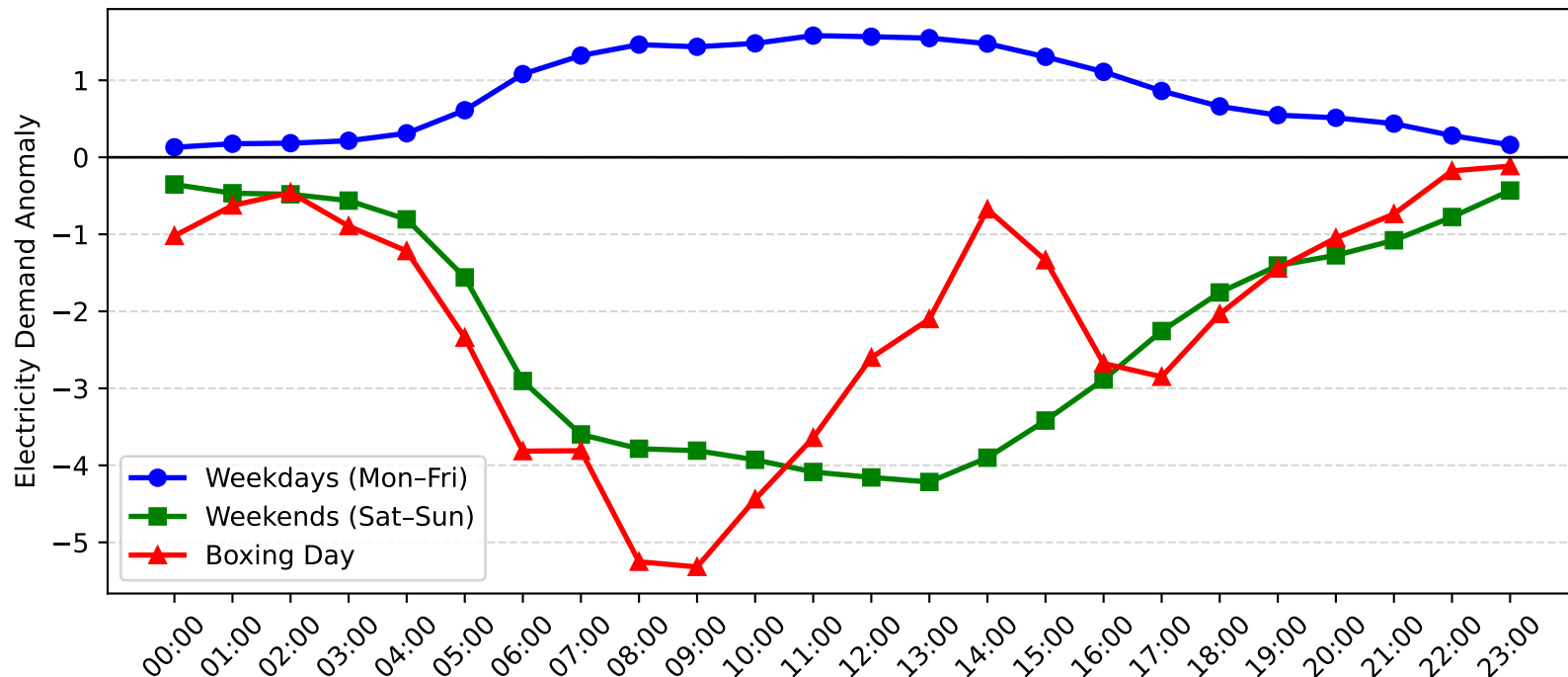
Wyong Demand Anomaly: Boxing Day vs Weekday/Weekend (2014-2015)
