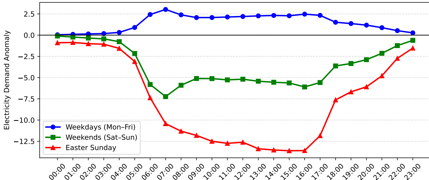
Epping Demand Anomaly: Easter Sunday vs Weekday/Weekend (2007-2008)
