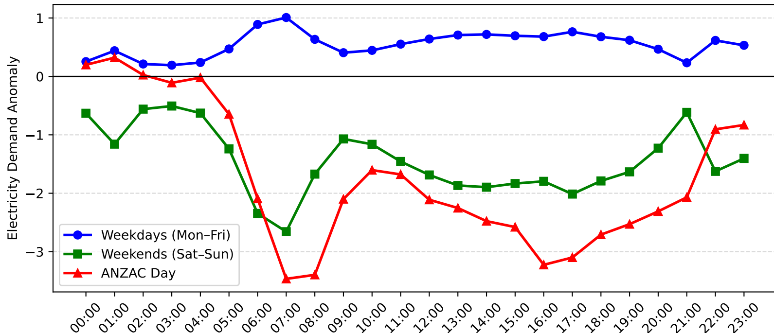
Jesmond Demand Anomaly: ANZAC Day vs Weekday/Weekend (2013-2014)
