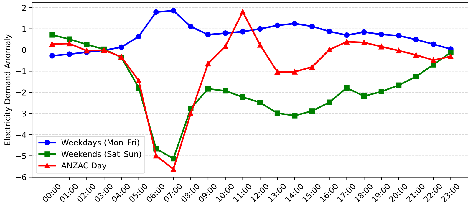
Mortdale Demand Anomaly: ANZAC Day vs Weekday/Weekend (2006-2007)
