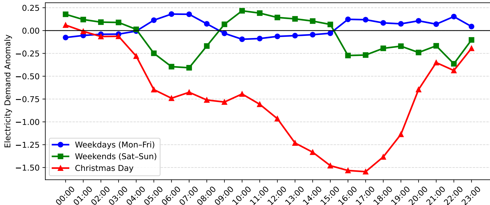
Narrabeen Demand Anomaly: Christmas Day vs Weekday/Weekend (2010-2011)
