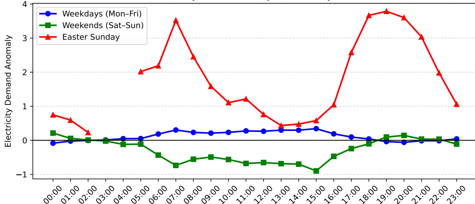
Rockdale Demand Anomaly: Easter Sunday vs Weekday/Weekend (2004-2005)
