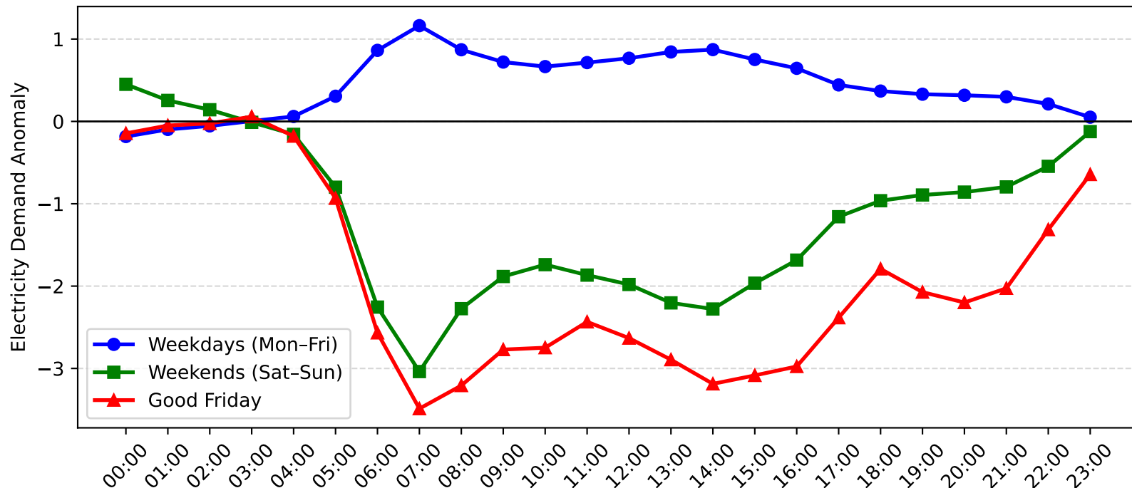
Arnccliffe Demand Anomaly: Good Friday vs Weekday/Weekend (2007-2008)
