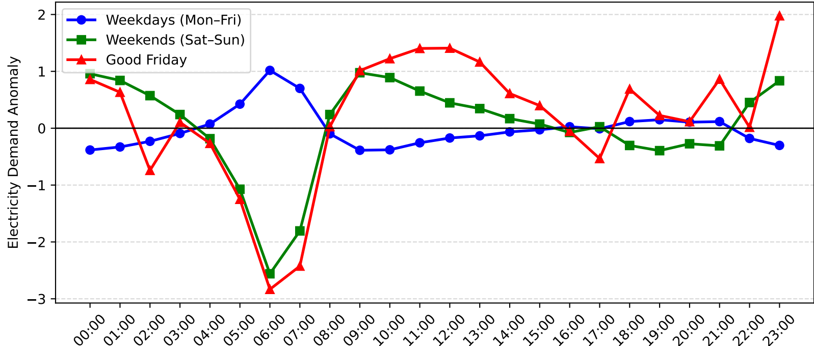
Avoca Demand Anomaly: Good Friday vs Weekday/Weekend (2005-2006)
