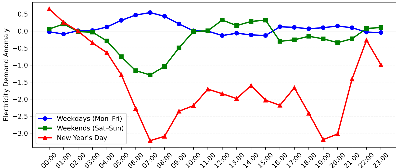
Charmhaven Demand Anomaly: New Year's Day vs Weekday/Weekend (2007-2008)
