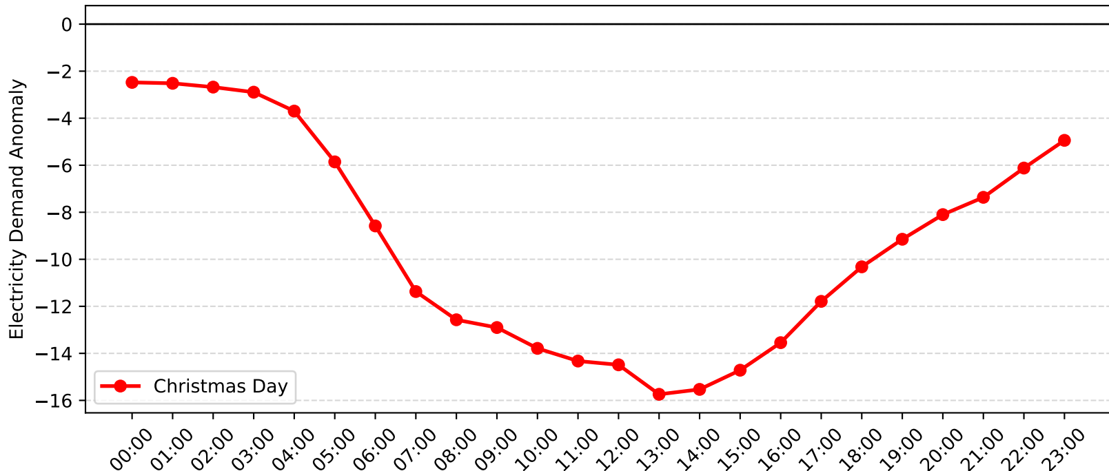
Milperra Demand Anomaly: Christmas Day (2012-2013)
