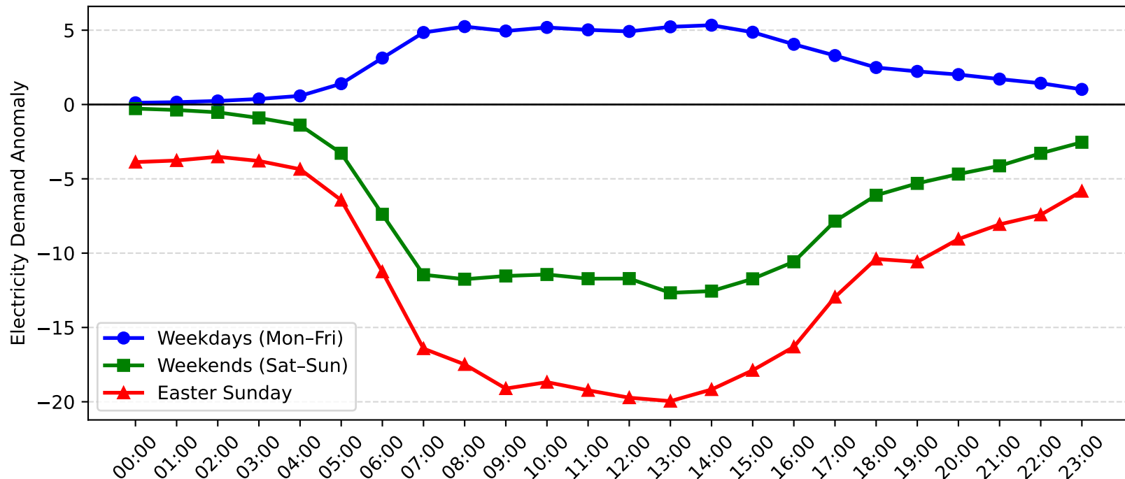
St. Peters Demand Anomaly: Easter Sunday vs Weekday/Weekend (2005-2006)
