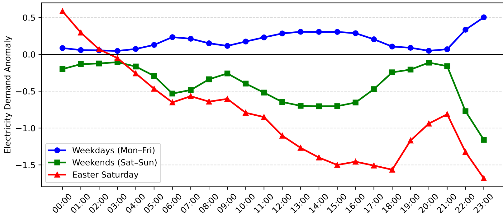
Muswellbrook Demand Anomaly: Easter Saturday vs Weekday/Weekend (2015-2016)
