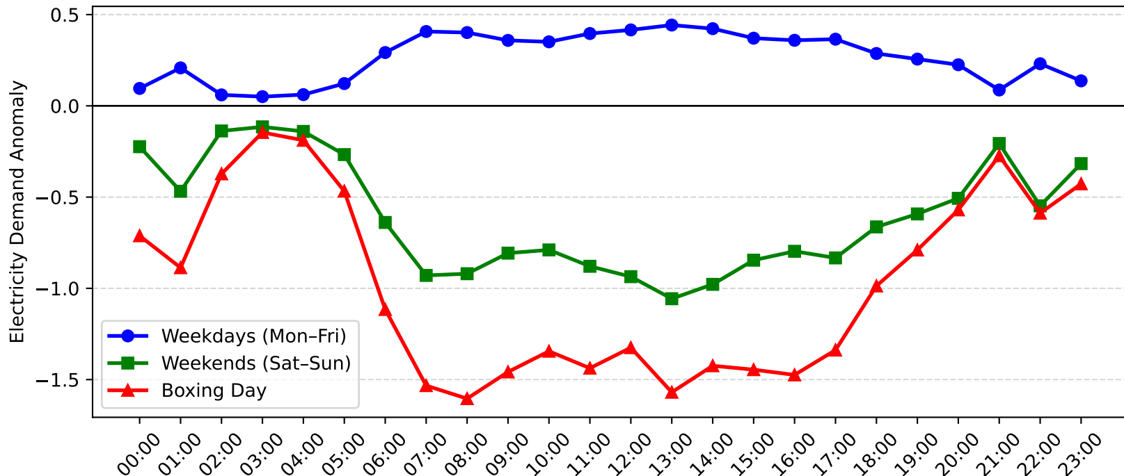
Gateshead Demand Anomaly: Boxing Day vs Weekday/Weekend (2010-2011)
