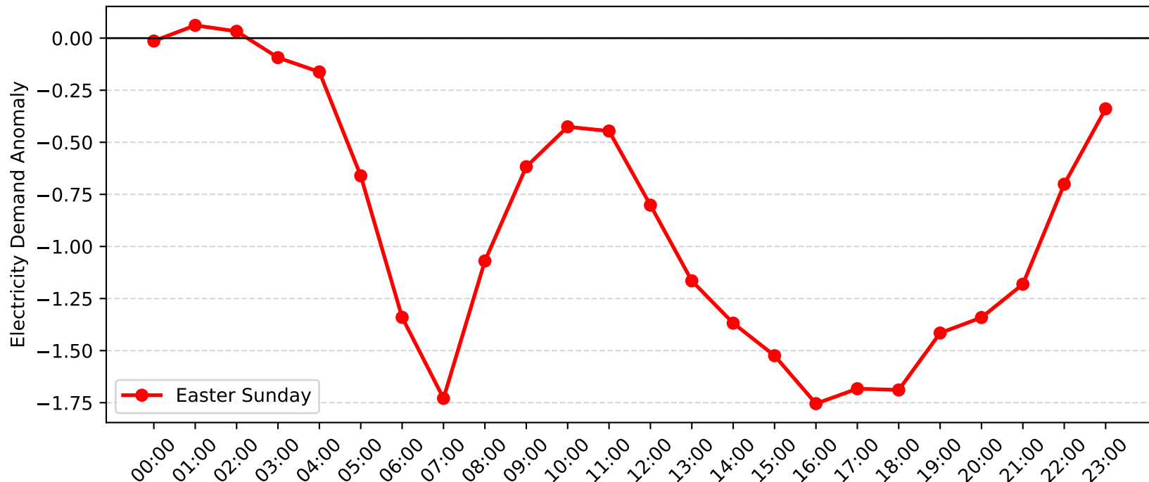
Blakehurst Demand Anomaly: Easter Sunday (2016-2017)
