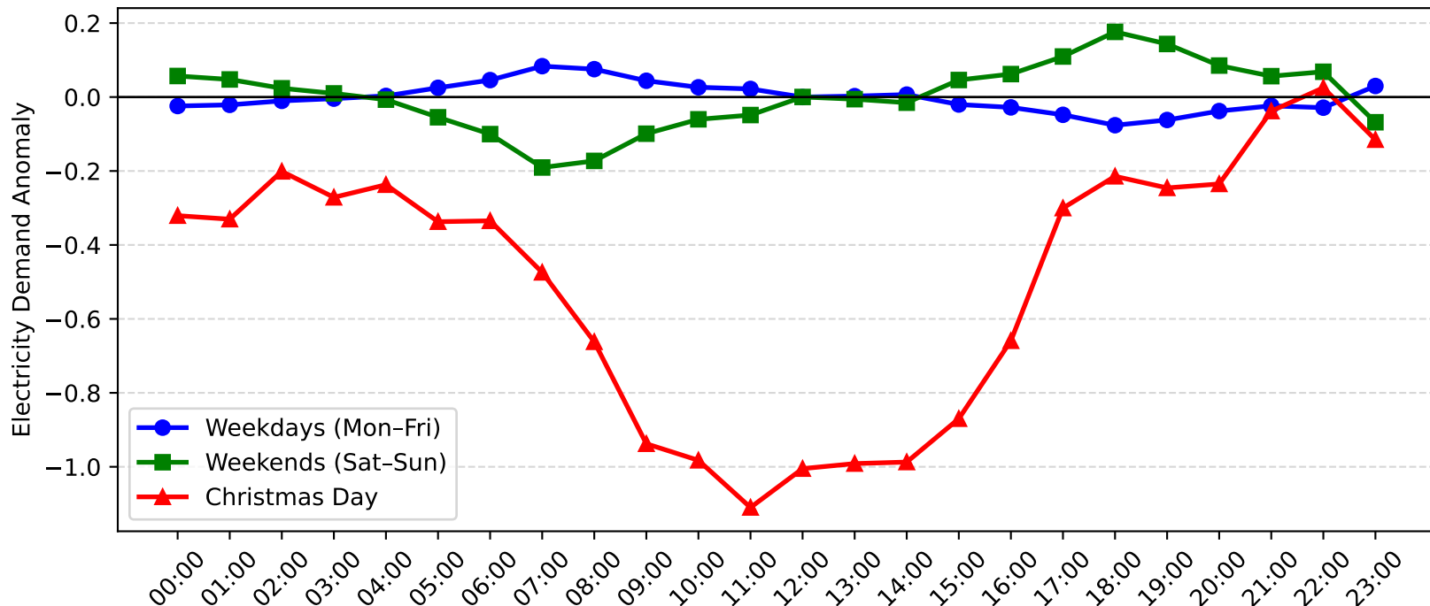
Rothbury Demand Anomaly: Christmas Day vs Weekday/Weekend (2010-2011)
