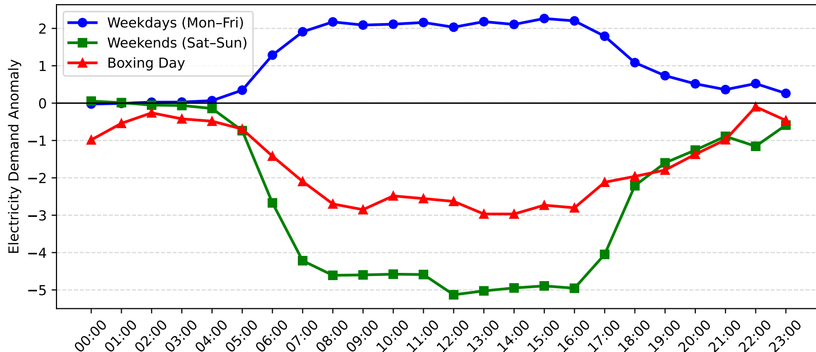
Beacon Hill Demand Anomaly: Boxing Day vs Weekday/Weekend (2004-2005)
