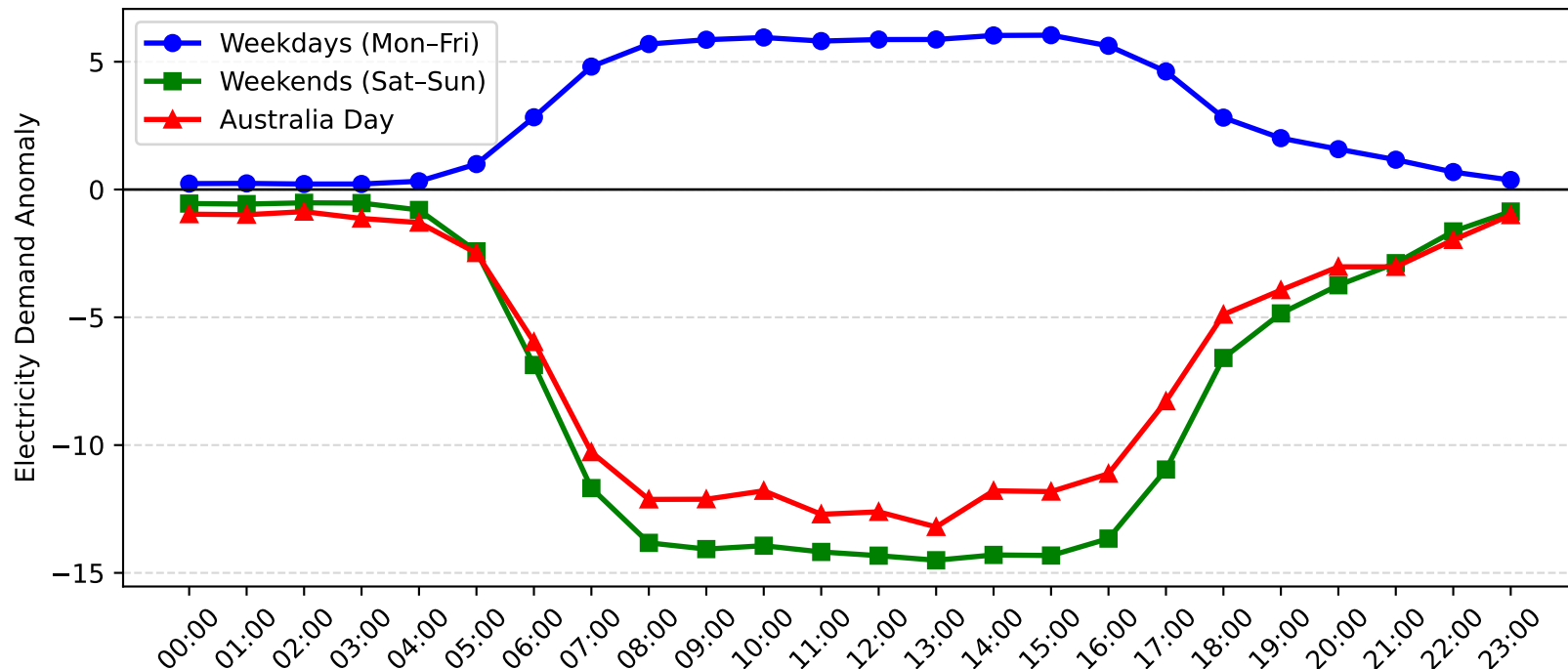
Gore Hill Demand Anomaly: Australia Day vs Weekday/Weekend (2007-2008)
