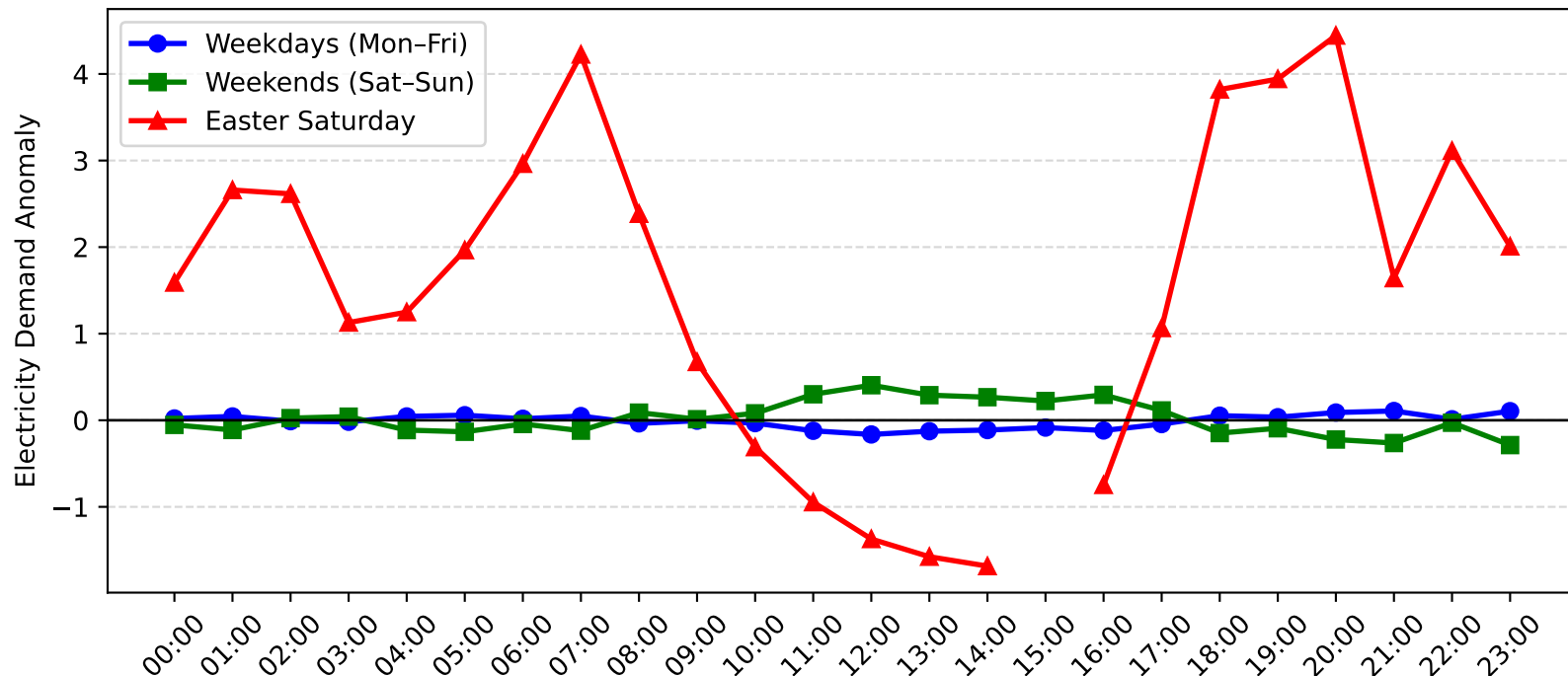
Umina Demand Anomaly: Easter Saturday vs Weekday/Weekend (2004-2005)
