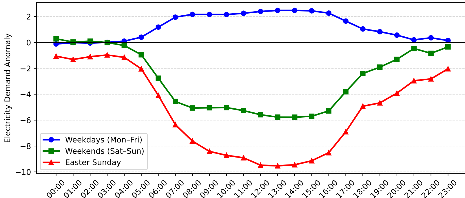
Newcastle Cbd Demand Anomaly: Easter Sunday vs Weekday/Weekend (2014-2015)
