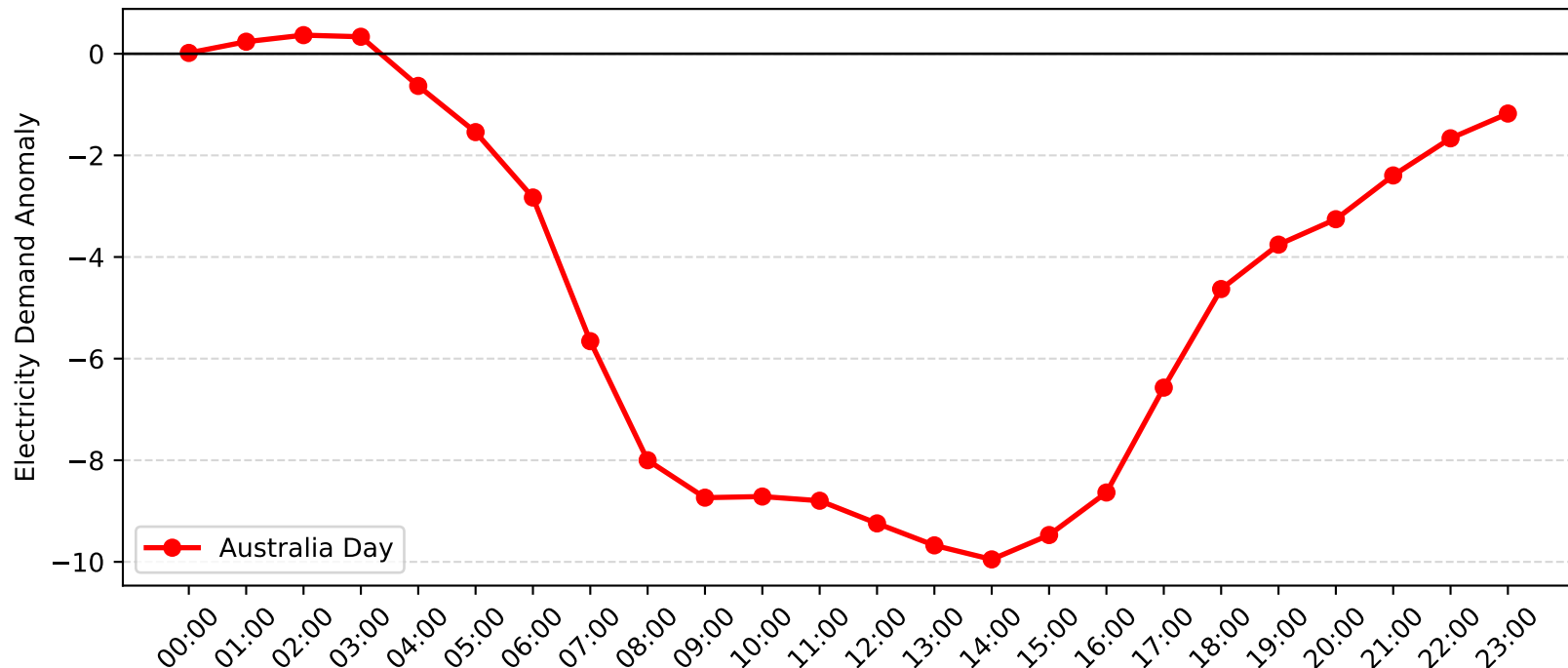
Gore Hill Demand Anomaly: Australia Day (2015-2016)
