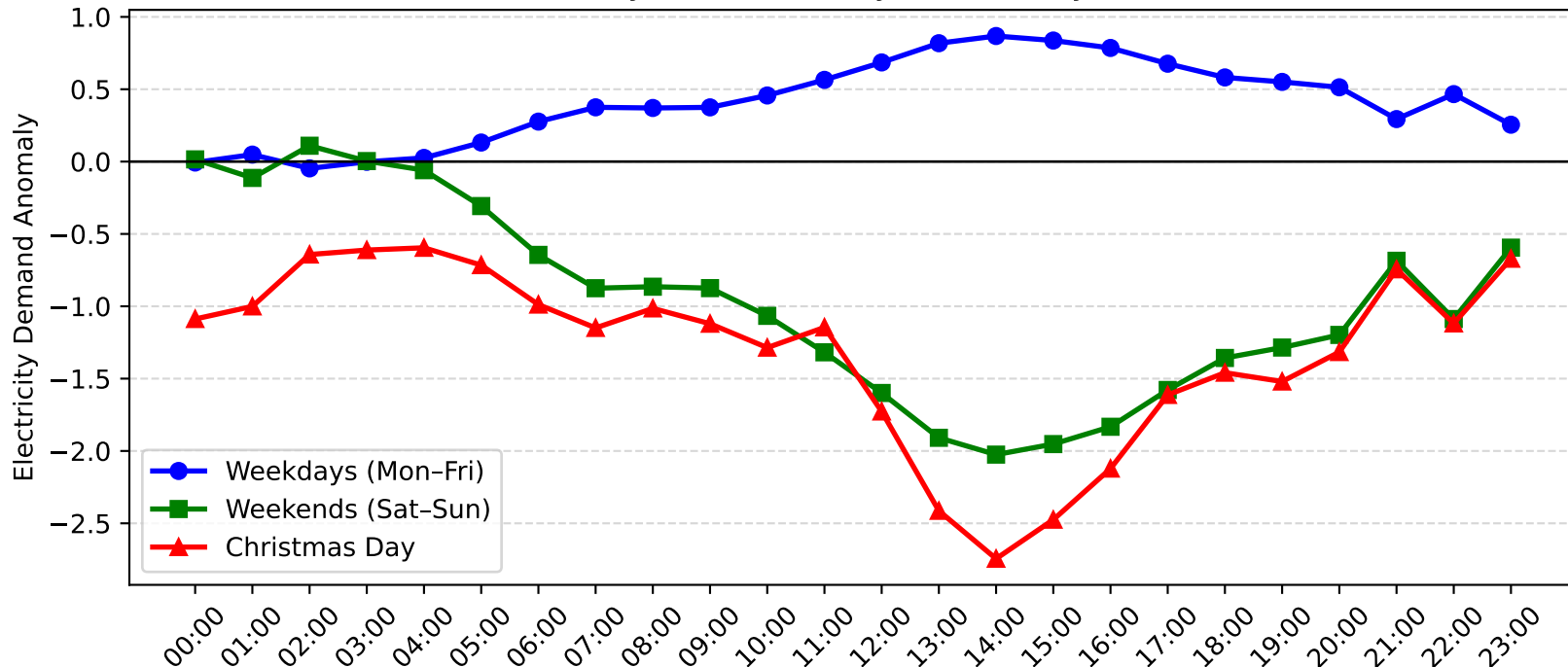
Cardiff Demand Anomaly: Christmas Day vs Weekday/Weekend (2016-2017)
