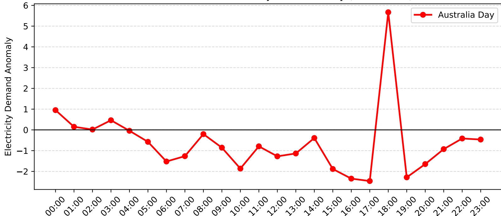
Chatswood Demand Anomaly: Australia Day (2004-2005)
