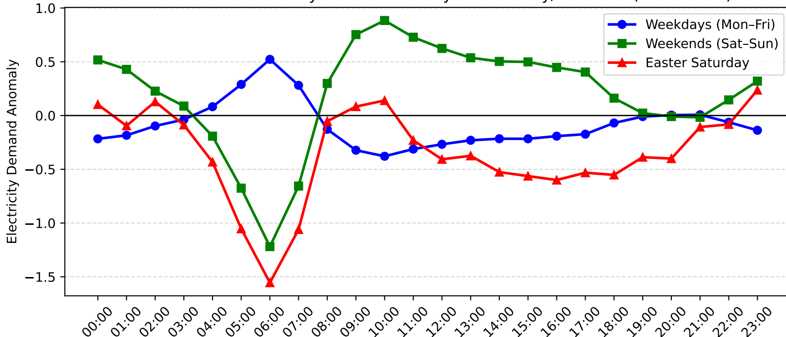
Umina Demand Anomaly: Easter Saturday vs Weekday/Weekend (2013-2014)
