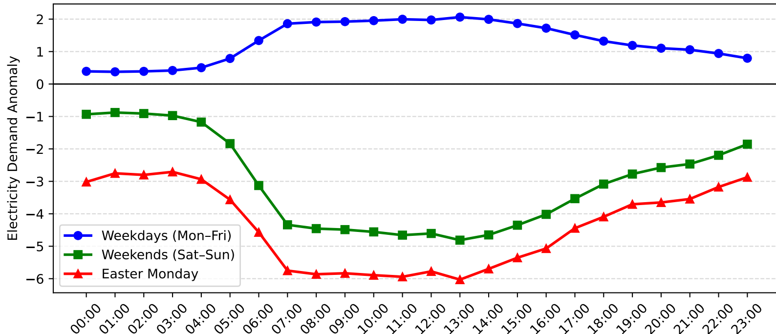
Leightonfield Demand Anomaly: Easter Monday vs Weekday/Weekend (2013-2014)
