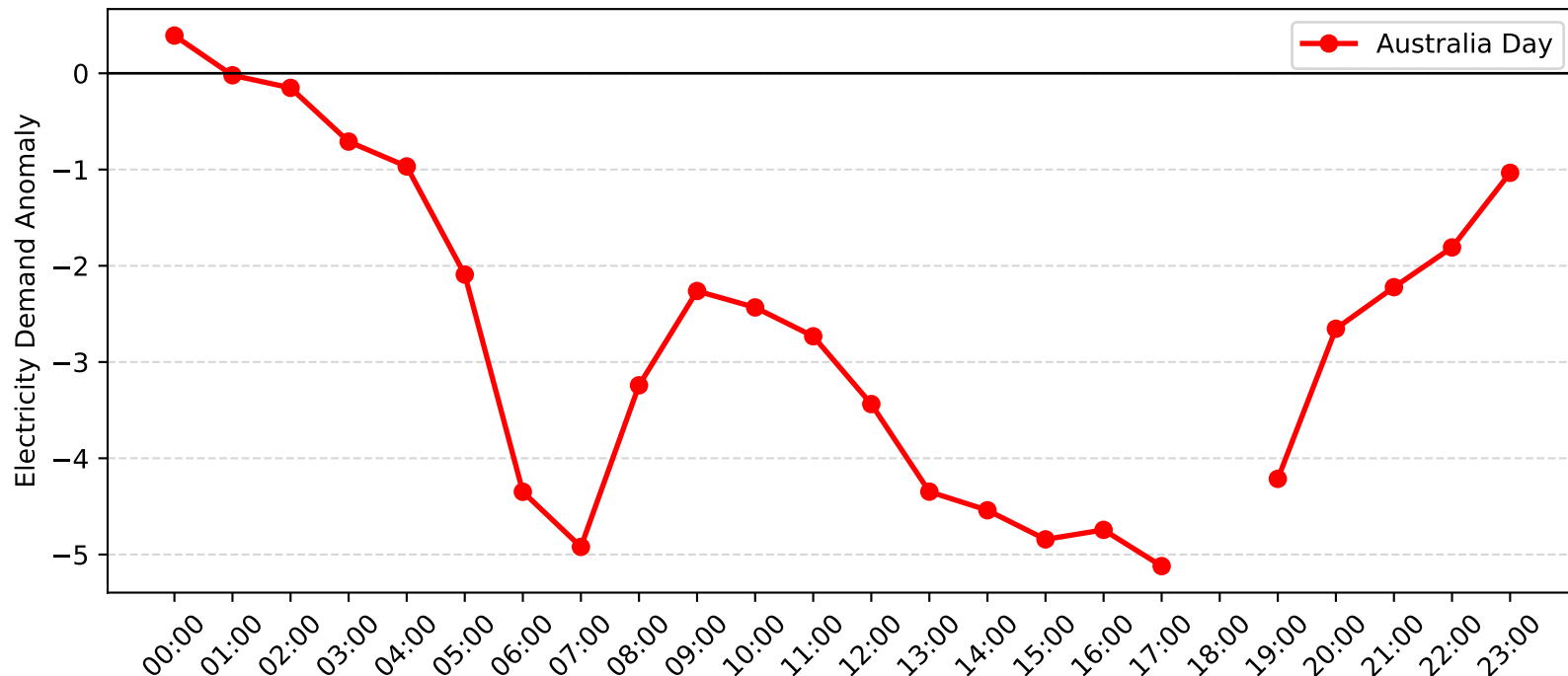
Dulwich Hill Demand Anomaly: Australia Day (2005-2006)
