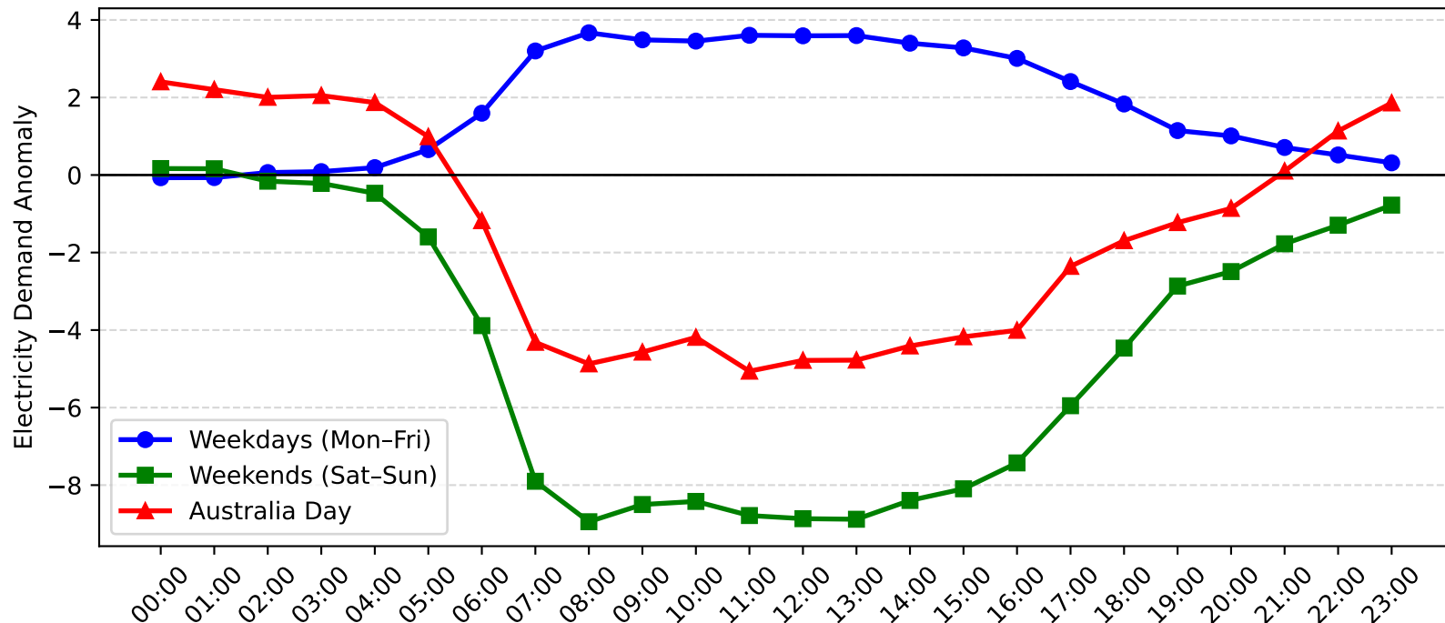
Zetland Demand Anomaly: Australia Day vs Weekday/Weekend (2012-2013)
