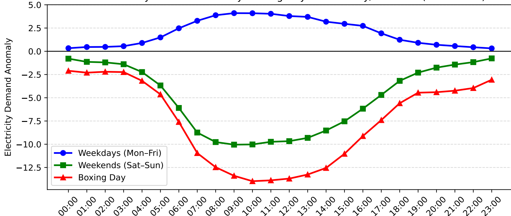
Homebush Bay Demand Anomaly: Boxing Day vs Weekday/Weekend (2009-2010)
