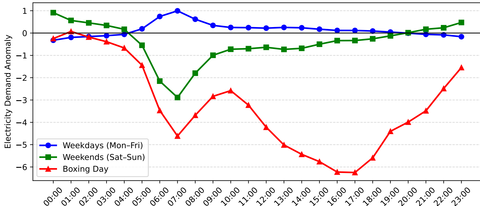
Mortdale Demand Anomaly: Boxing Day vs Weekday/Weekend (2012-2013)
