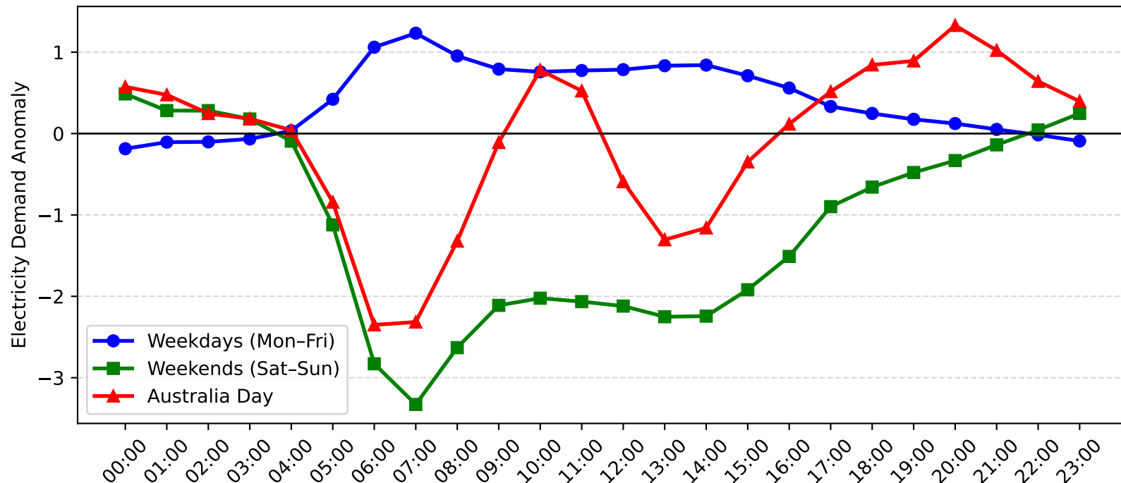
Kirrawee Demand Anomaly: Australia Day vs Weekday/Weekend (2011-2012)
