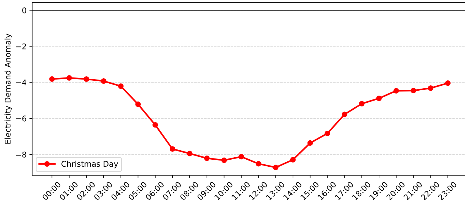
Leightonfield Demand Anomaly: Christmas Day (2004-2005)
