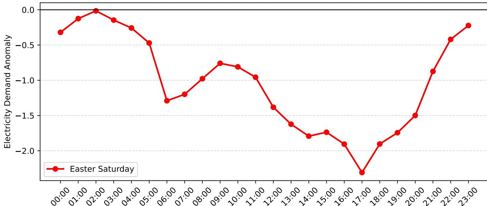
Erina Demand Anomaly: Easter Saturday (2014-2015)
