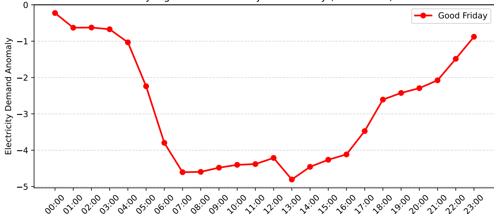
Wyong Demand Anomaly: Good Friday (2012-2013)
