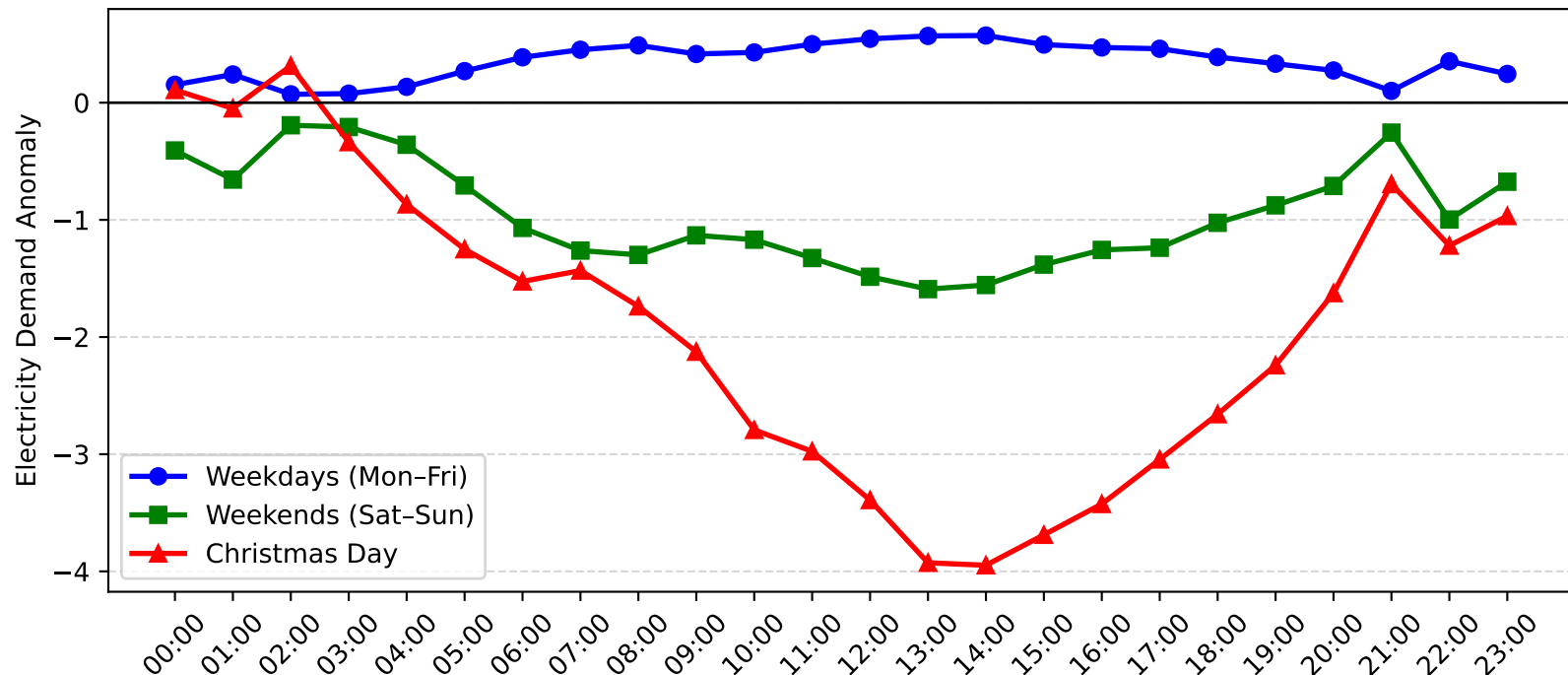
Gateshead Demand Anomaly: Christmas Day vs Weekday/Weekend (2014-2015)
