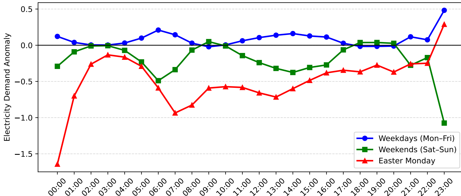
Telarah Demand Anomaly: Easter Monday vs Weekday/Weekend (2007-2008)
