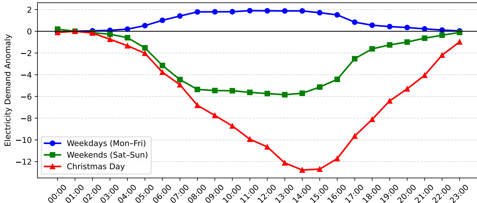
West Gosford Demand Anomaly: Christmas Day vs Weekday/Weekend (2013-2014)
