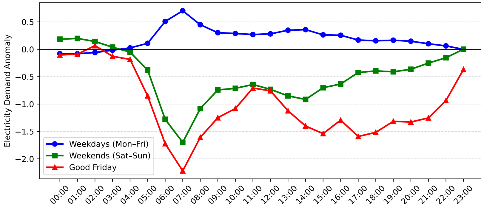
Arncliffe Demand Anomaly: Good Friday vs Weekday/Weekend (2015-2016)
