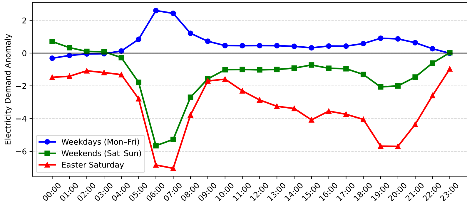
Pennant Hills Demand Anomaly: Easter Saturday vs Weekday/Weekend (2010-2011)
