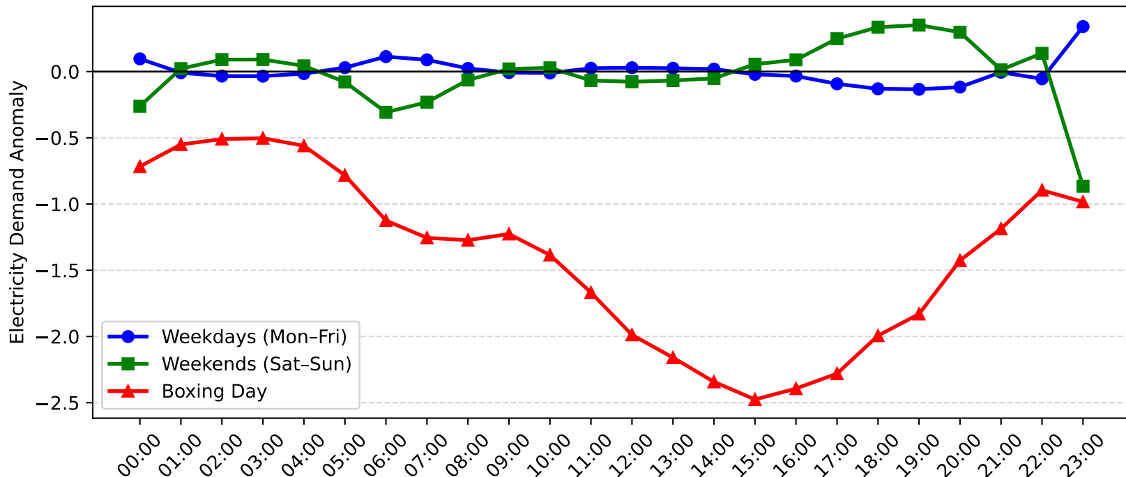
Telarah Demand Anomaly: Boxing Day vs Weekday/Weekend (2006-2007)
