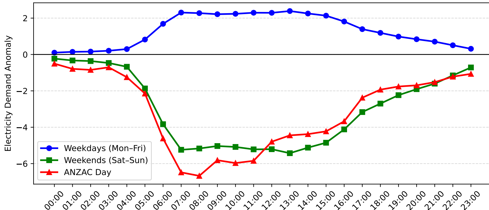
Bankstown Demand Anomaly: ANZAC Day vs Weekday/Weekend (2017-2018)
