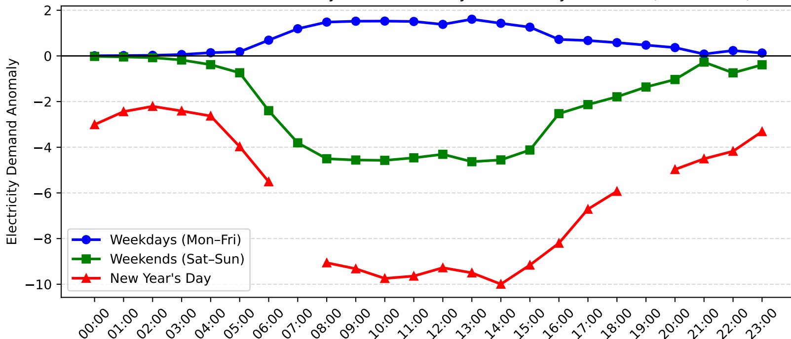
Bankstown Demand Anomaly: New Year's Day vs Weekday/Weekend (2014-2015)
