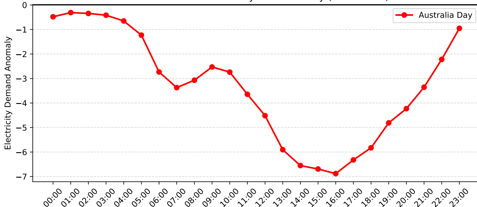
Kirrawee Demand Anomaly: Australia Day (2017-2018)
