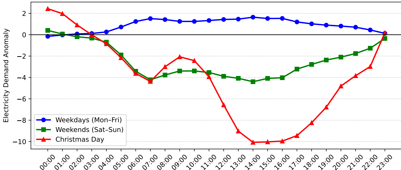
Campsie Demand Anomaly: Christmas Day vs Weekday/Weekend (2014-2015)
