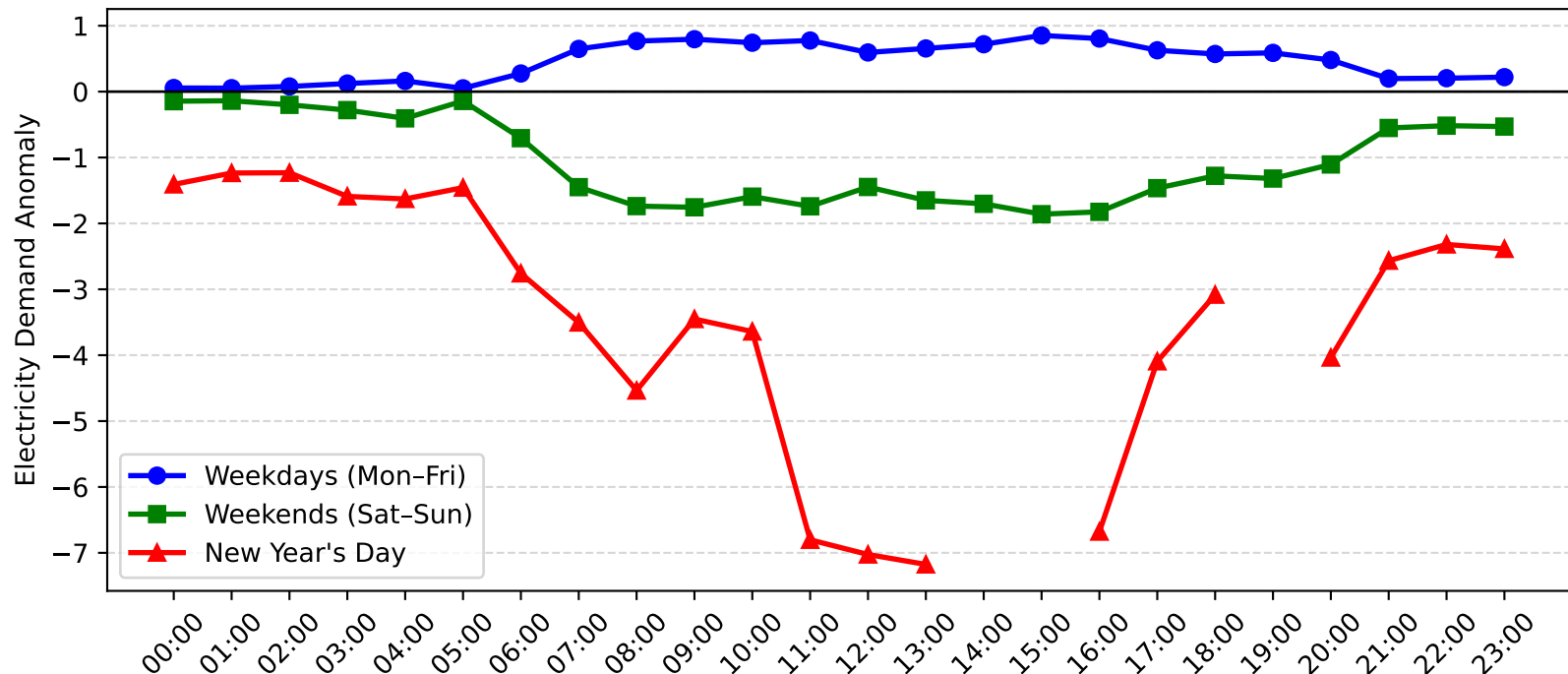
Green Square Demand Anomaly: New Year's Day vs Weekday/Weekend (2007-2008)
