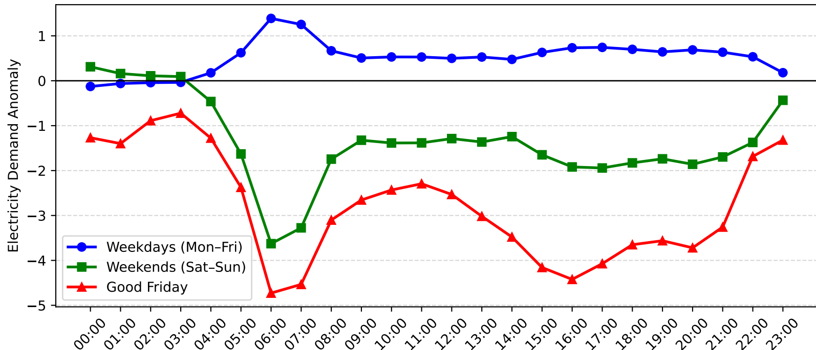
Revesby Demand Anomaly: Good Friday vs Weekday/Weekend (2007-2008)
