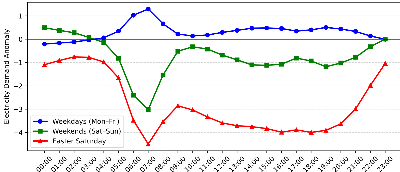
Five Dock Demand Anomaly: Easter Saturday vs Weekday/Weekend (2013-2014)
