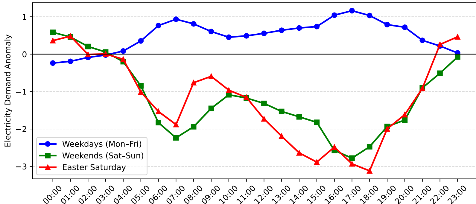
Erina Demand Anomaly: Easter Saturday vs Weekday/Weekend (2007-2008)
