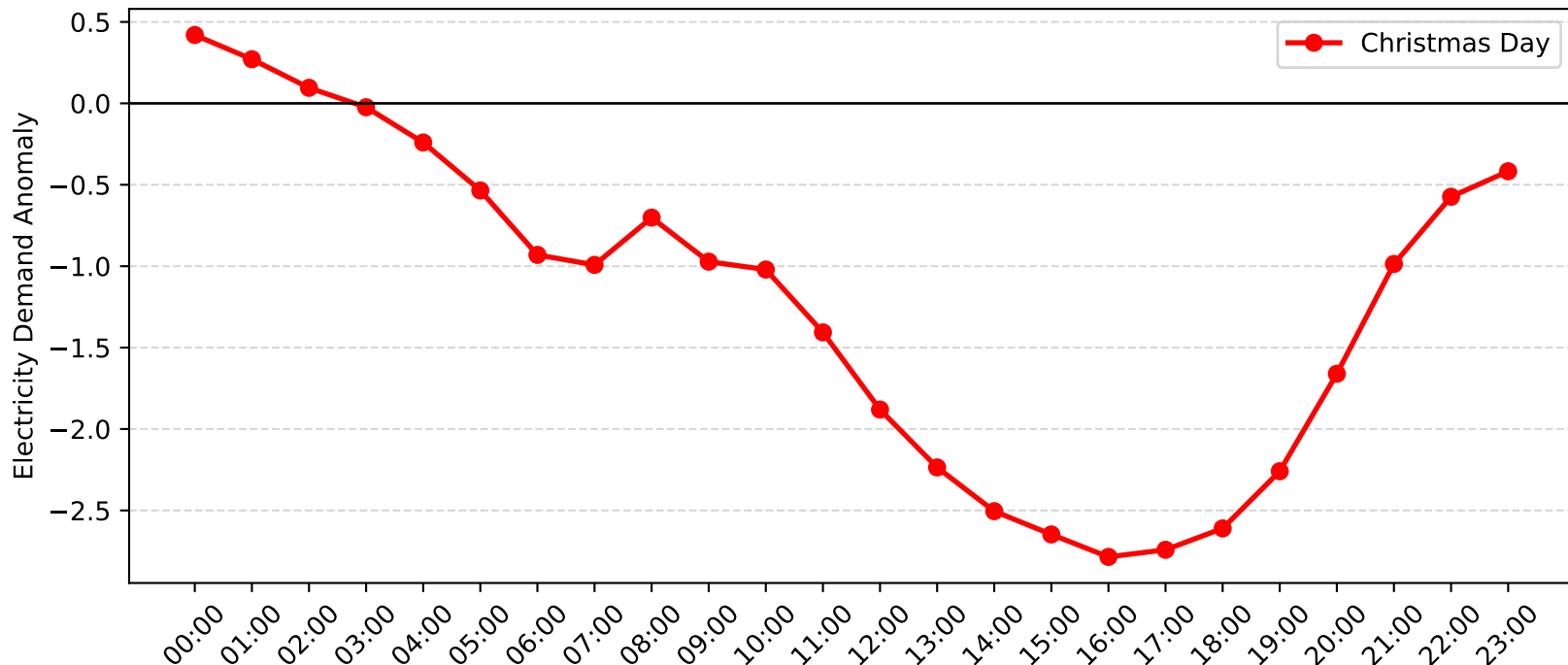
Narrabeen Demand Anomaly: Christmas Day (2005-2006)
