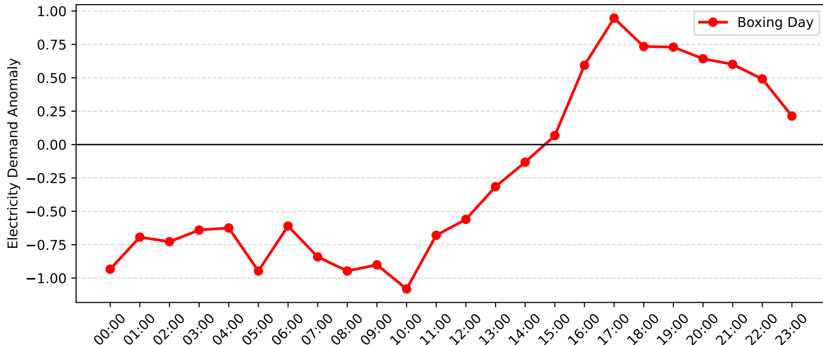
Rothbury Demand Anomaly: Boxing Day (2016-2017)
