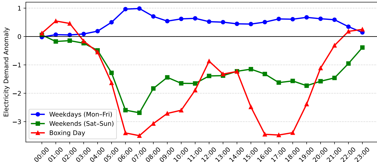
Revesby Demand Anomaly: Boxing Day vs Weekday/Weekend (2014-2015)
