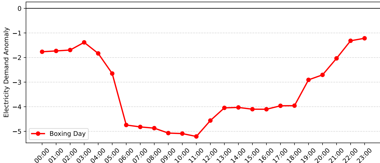
Potts Hill Demand Anomaly: Boxing Day (2015-2016)
