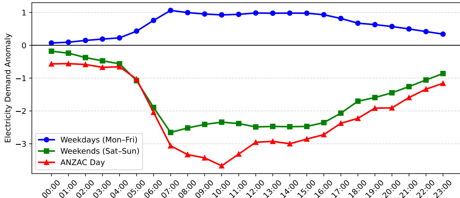
Lidcombe Demand Anomaly: ANZAC Day vs Weekday/Weekend (2011-2012)
