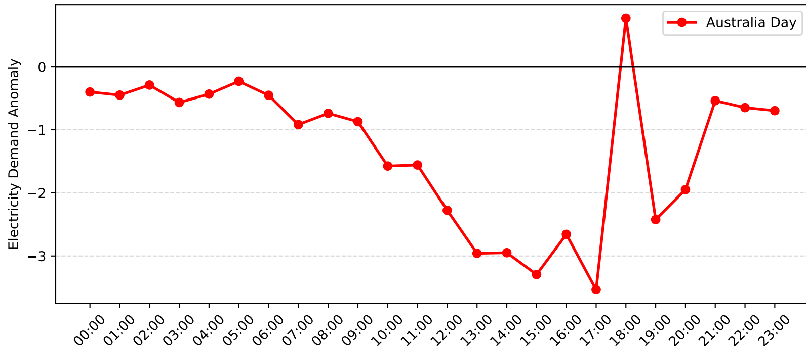
Epping Demand Anomaly: Australia Day (2004-2005)
