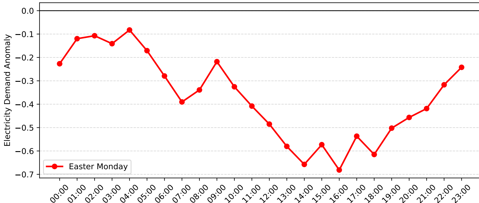
Rothbury Demand Anomaly: Easter Monday (2013-2014)
