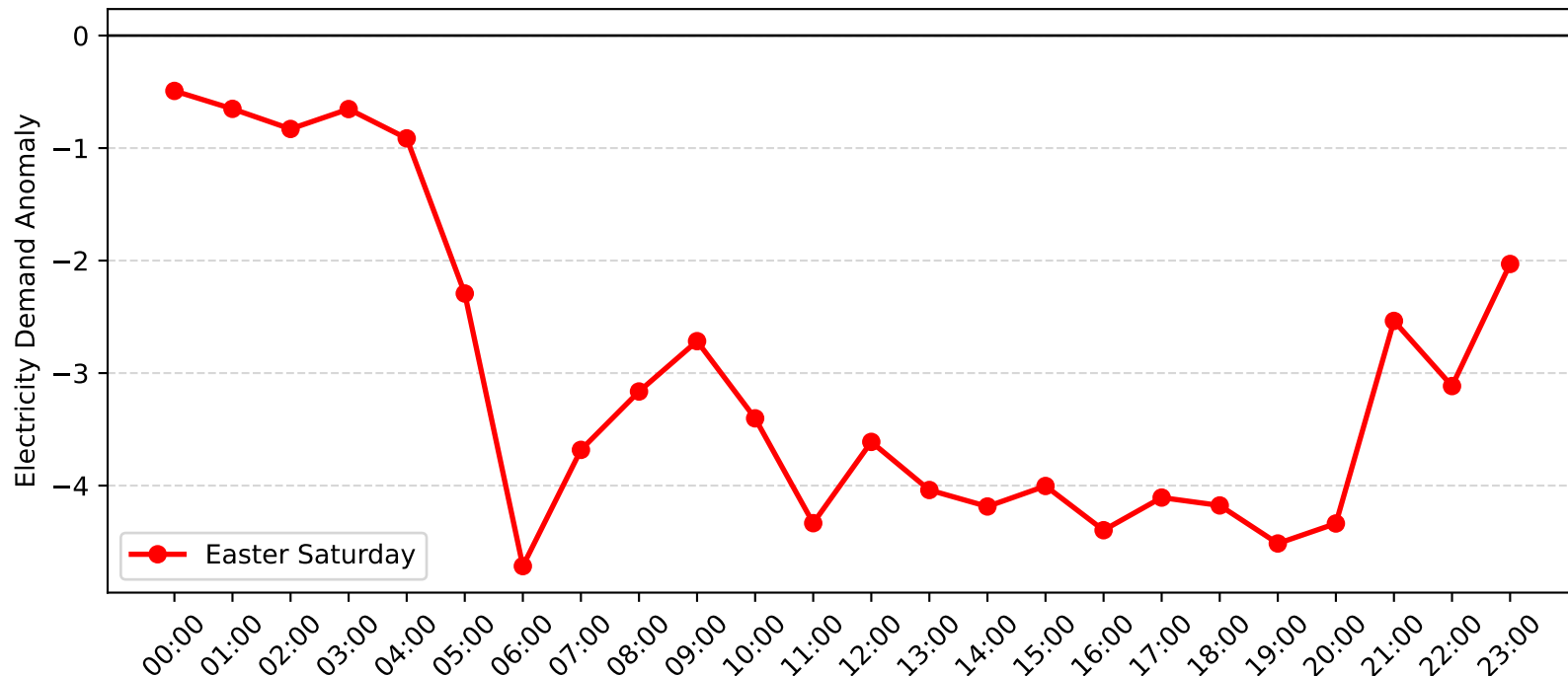
Dee Why West Demand Anomaly: Easter Saturday (2005-2006)
