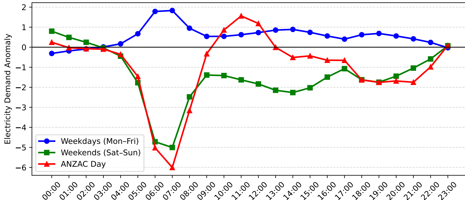
Mortdale Demand Anomaly: ANZAC Day vs Weekday/Weekend (2007-2008)
