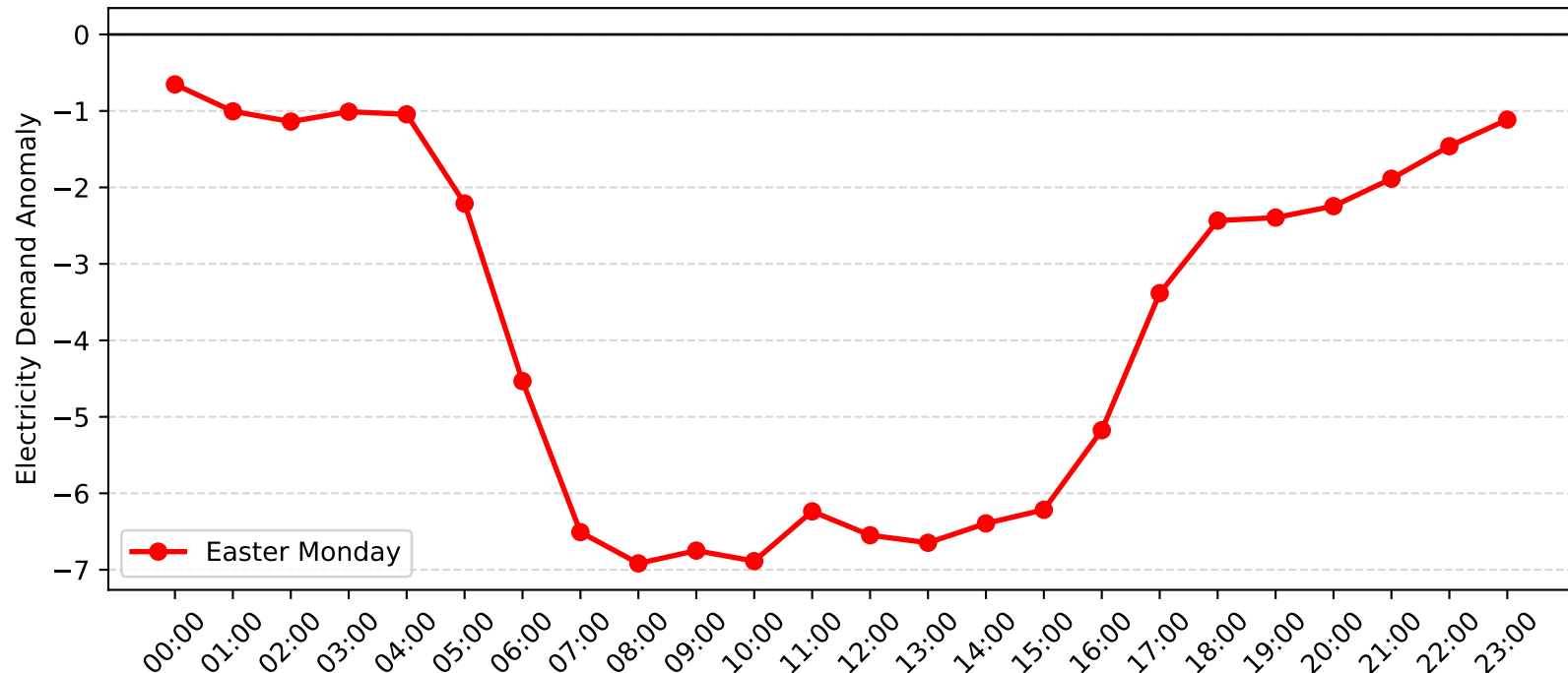
Bankstown Demand Anomaly: Easter Monday (2017-2018)
