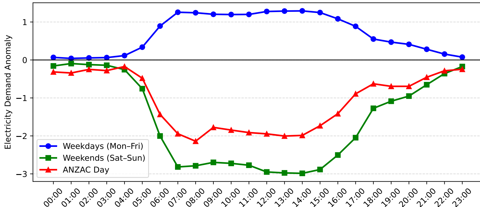
Beacon Hill Demand Anomaly: ANZAC Day vs Weekday/Weekend (2016-2017)
