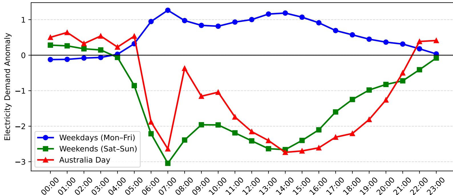
Kirrawee Demand Anomaly: Australia Day vs Weekday/Weekend (2013-2014)
