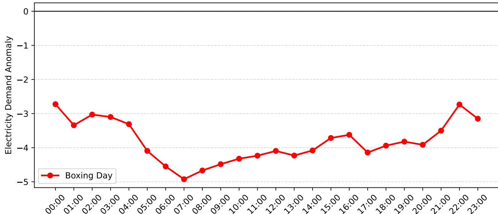
Lisarow Demand Anomaly: Boxing Day (2004-2005)
