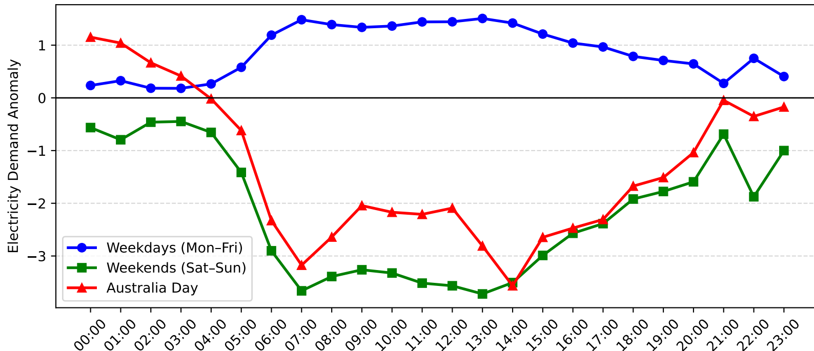
Argenton Demand Anomaly: Australia Day vs Weekday/Weekend (2012-2013)
