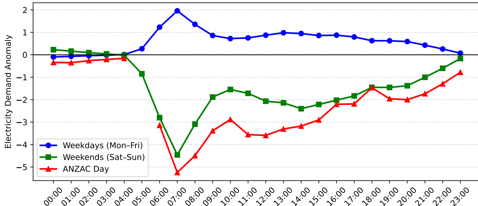
Chatswood Demand Anomaly: ANZAC Day vs Weekday/Weekend (2015-2016)
