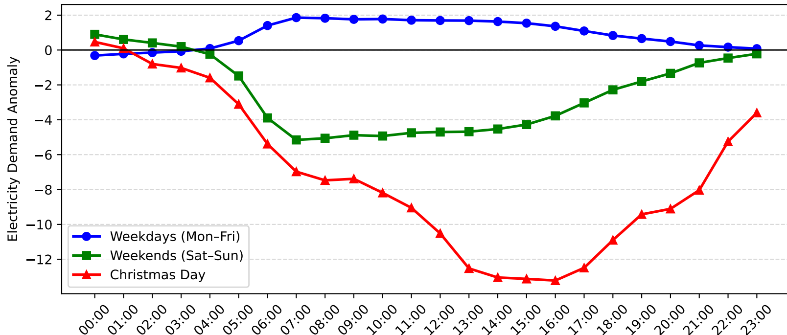
Sefton Demand Anomaly: Christmas Day vs Weekday/Weekend (2012-2013)
