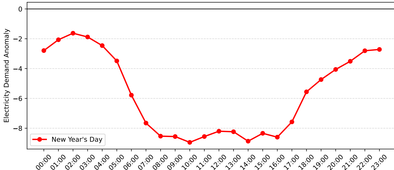
Maroubra Demand Anomaly: New Year's Day (2005-2006)
