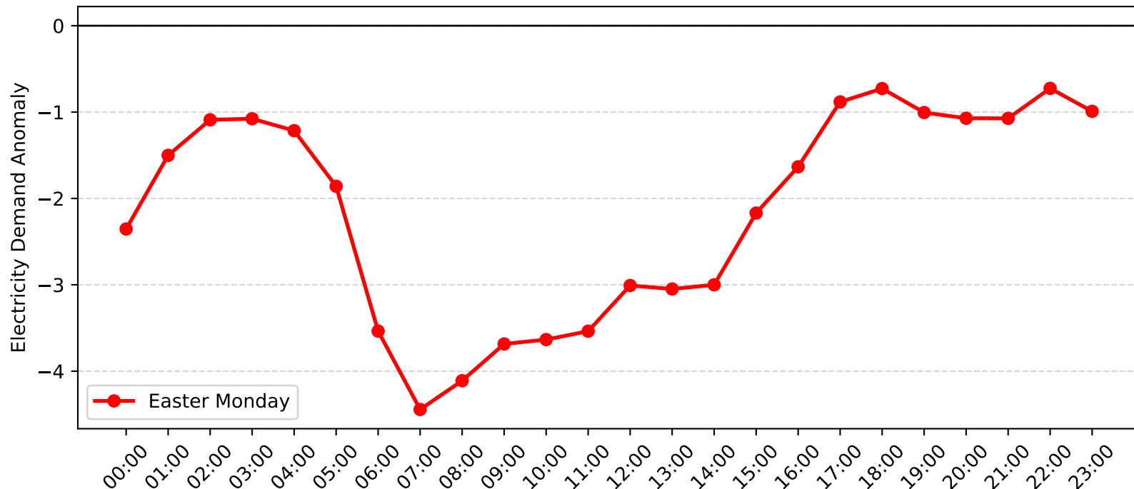
Rutherford Demand Anomaly: Easter Monday (2014-2015)
