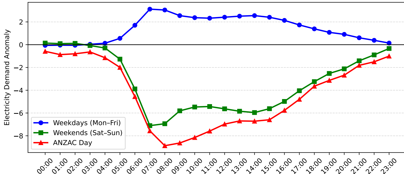
Zetland Demand Anomaly: ANZAC Day vs Weekday/Weekend (2015-2016)
