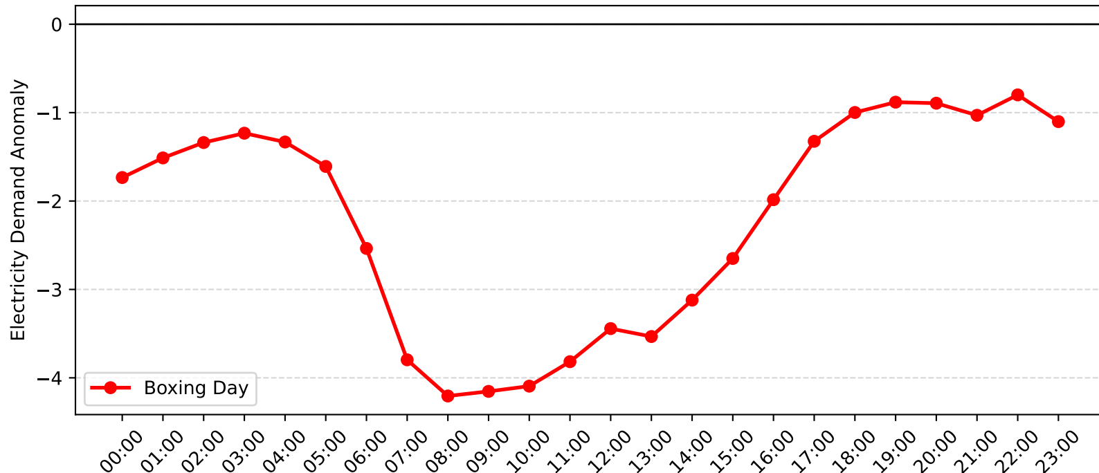
Mayfield West Demand Anomaly: Boxing Day (2016-2017)
