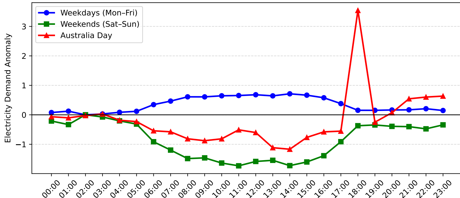
Kirrawee Demand Anomaly: Australia Day vs Weekday/Weekend (2004-2005)
