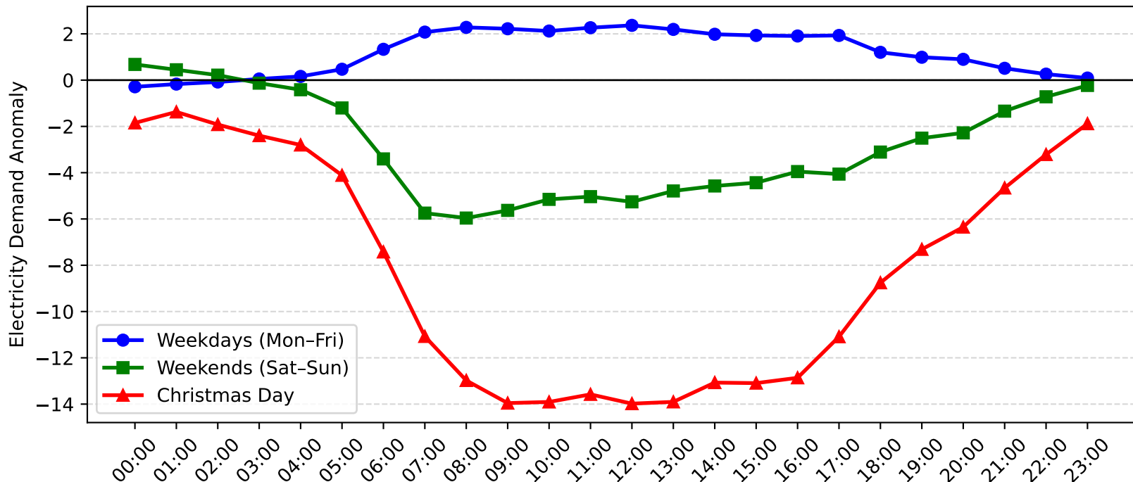
Burwood Demand Anomaly: Christmas Day vs Weekday/Weekend (2009-2010)
