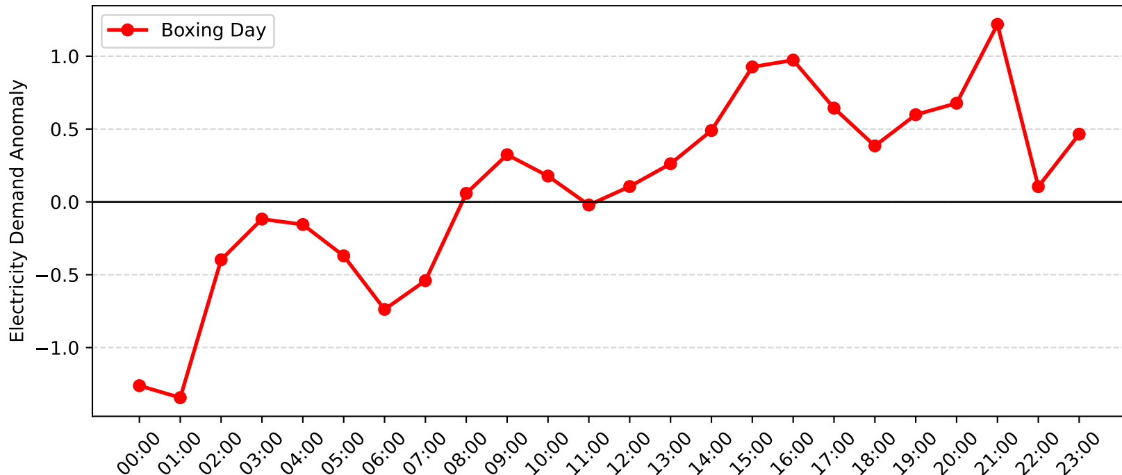
Nelson Bay Demand Anomaly: Boxing Day (2015-2016)
