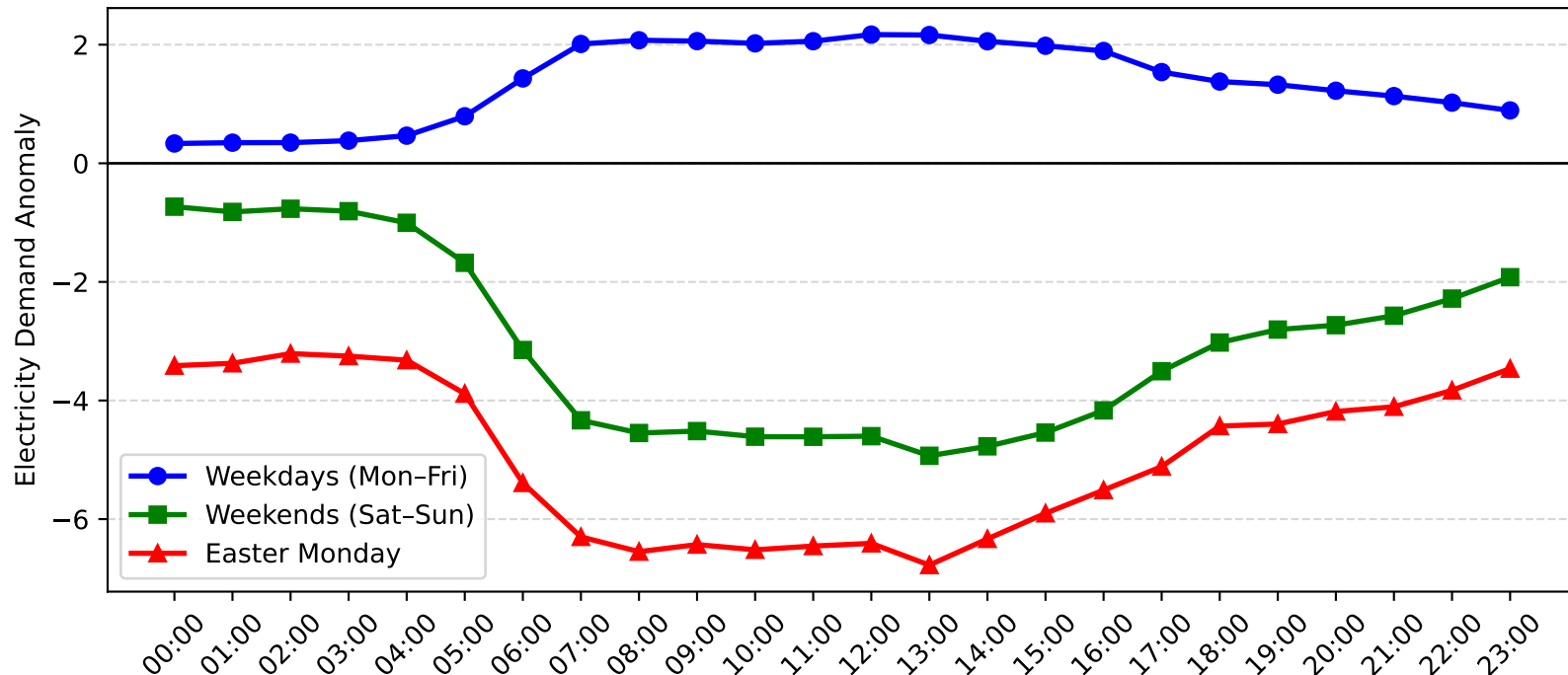
Leightonfield Demand Anomaly: Easter Monday vs Weekday/Weekend (2009-2010)
