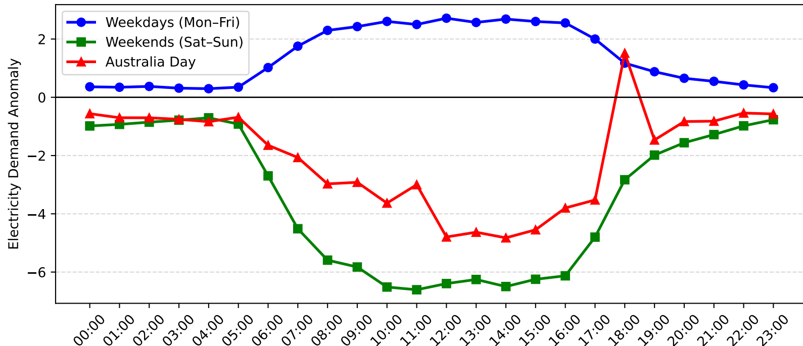
Gore Hill Demand Anomaly: Australia Day vs Weekday/Weekend (2004-2005)
