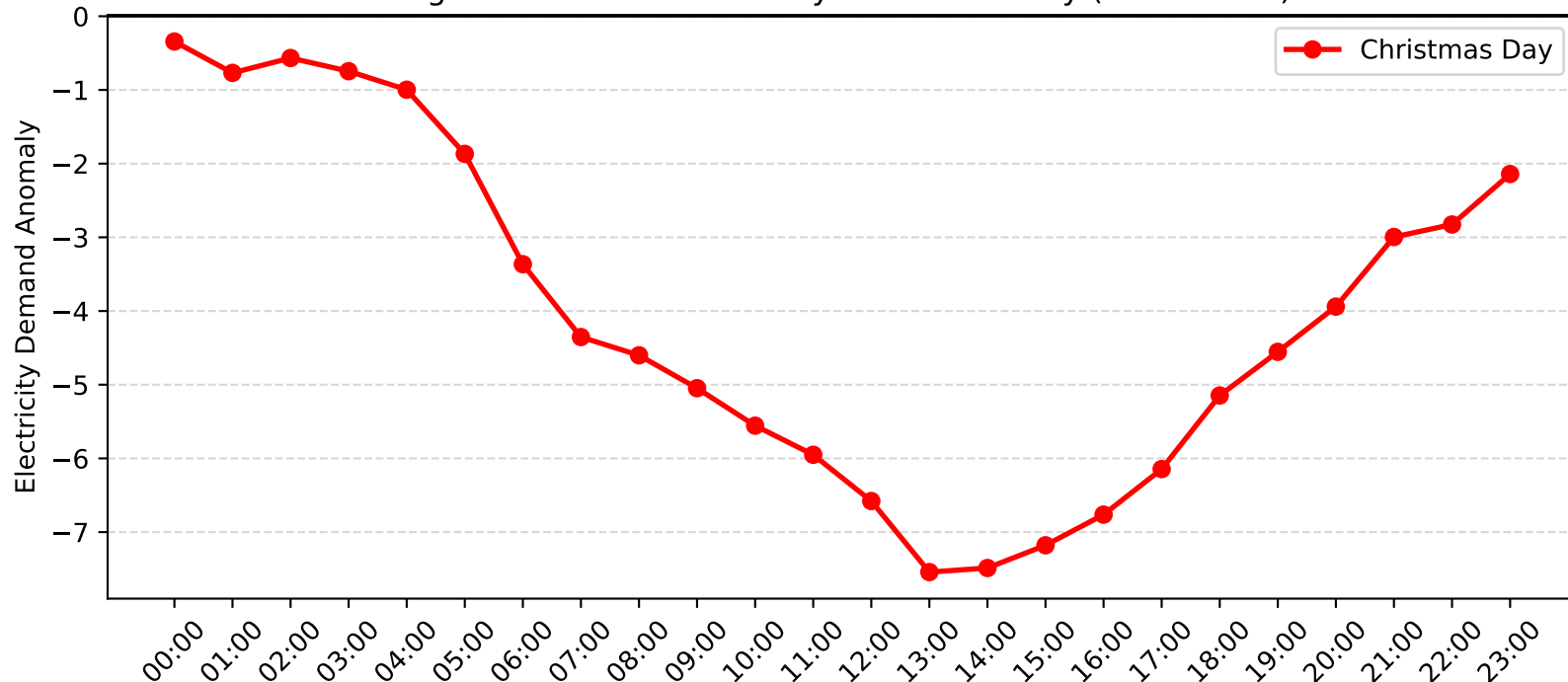
Argenton Demand Anomaly: Christmas Day (2011-2012)
