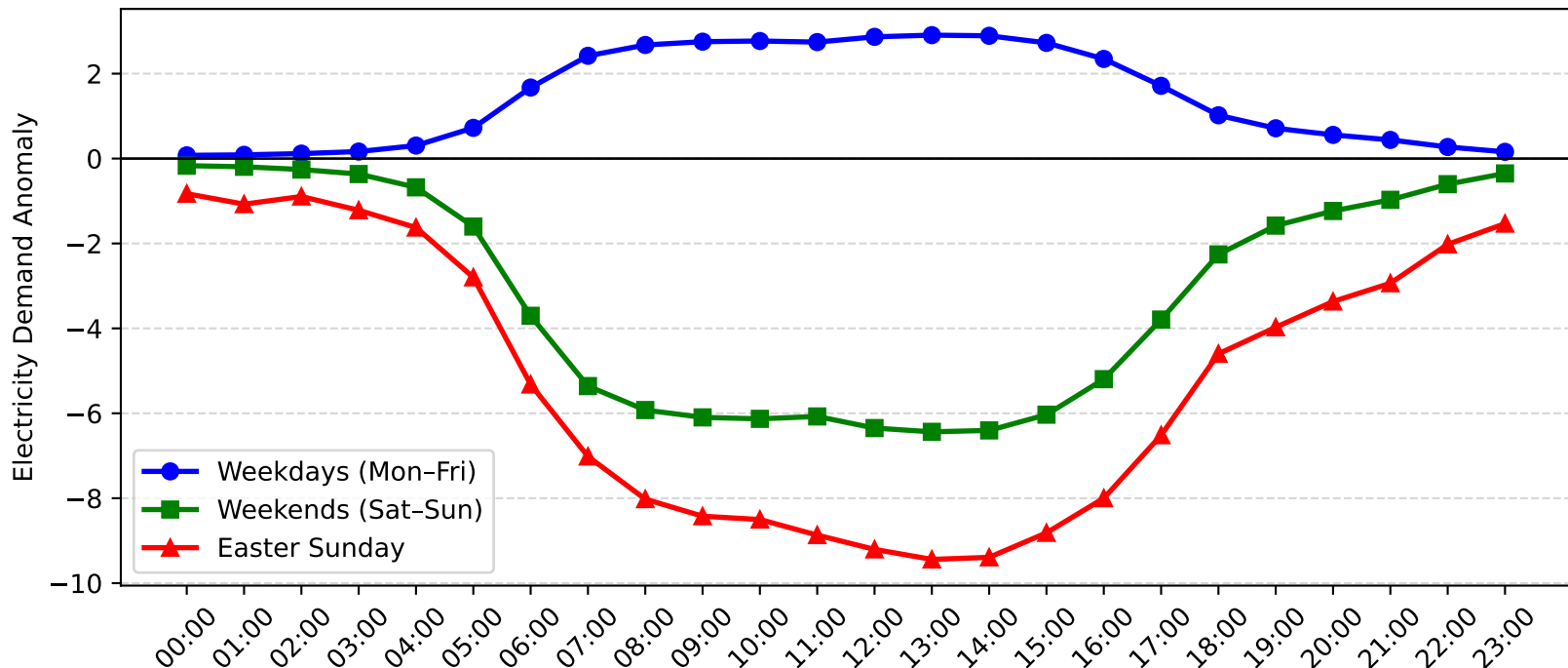
Mascot Demand Anomaly: Easter Sunday vs Weekday/Weekend (2017-2018)
