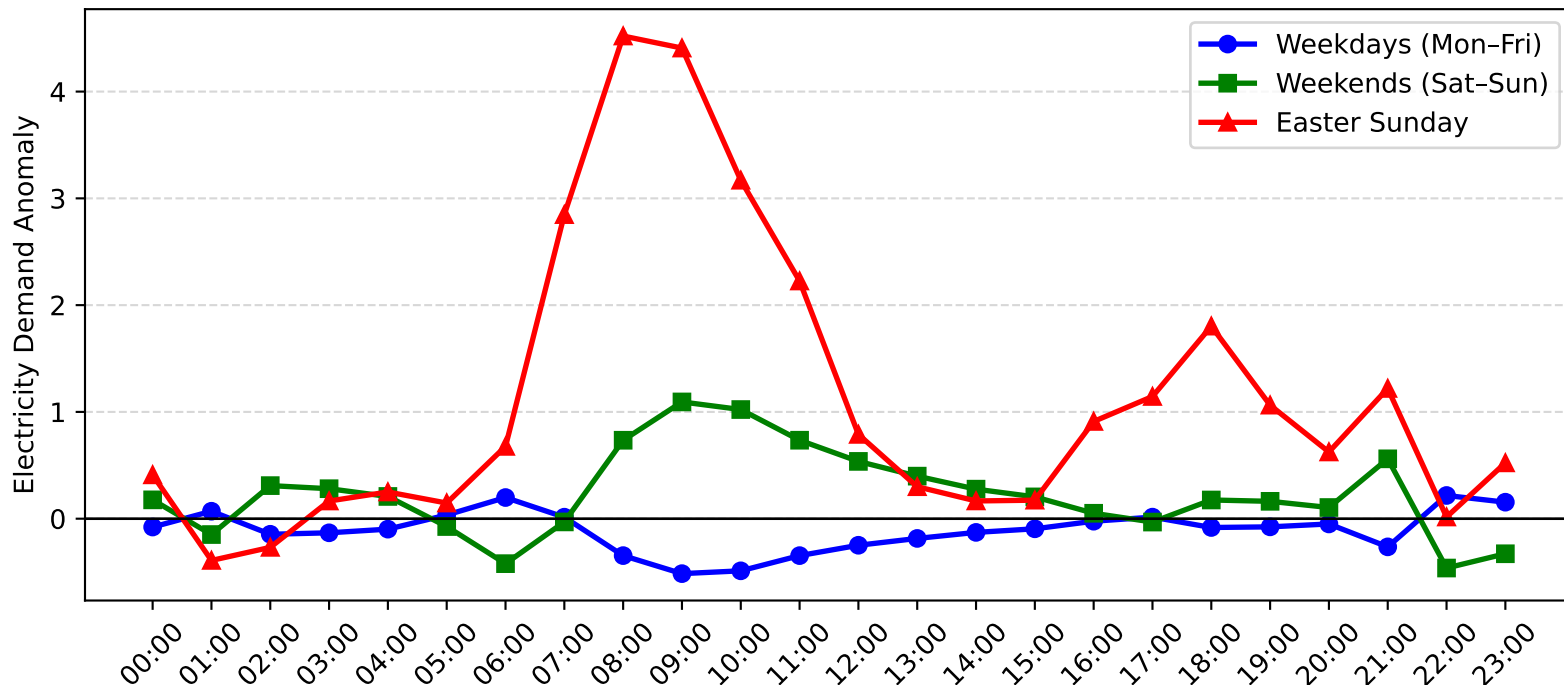
Nelson Bay Demand Anomaly: Easter Sunday vs Weekday/Weekend (2015-2016)
