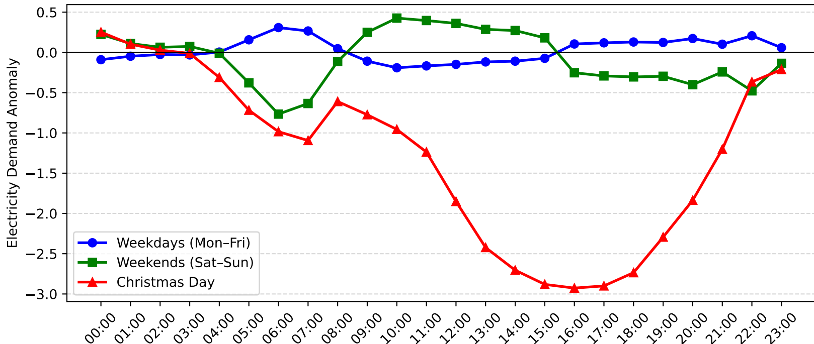
Narrabeen Demand Anomaly: Christmas Day vs Weekday/Weekend (2006-2007)
