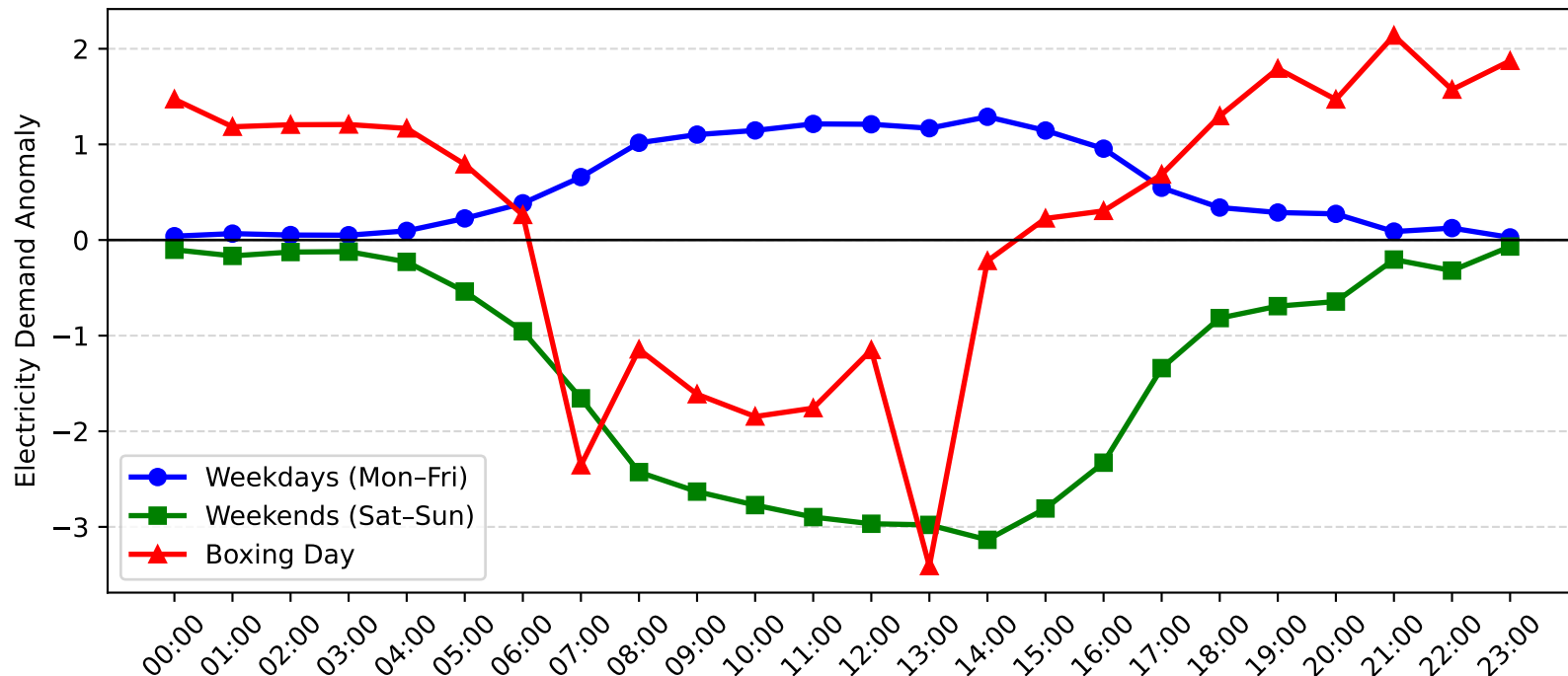
Broadmeadow Demand Anomaly: Boxing Day vs Weekday/Weekend (2014-2015)
