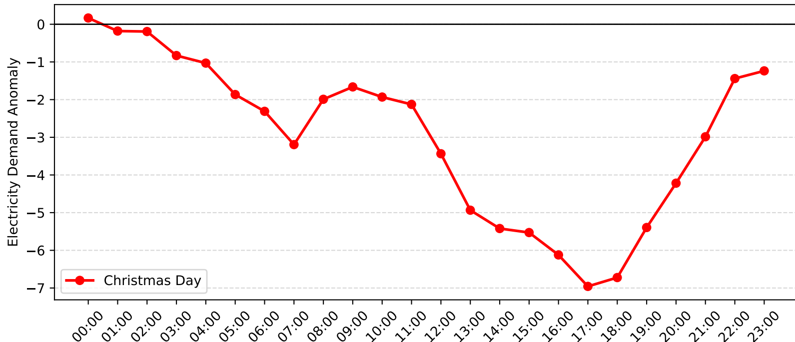
Dee Why West Demand Anomaly: Christmas Day (2007-2008)
