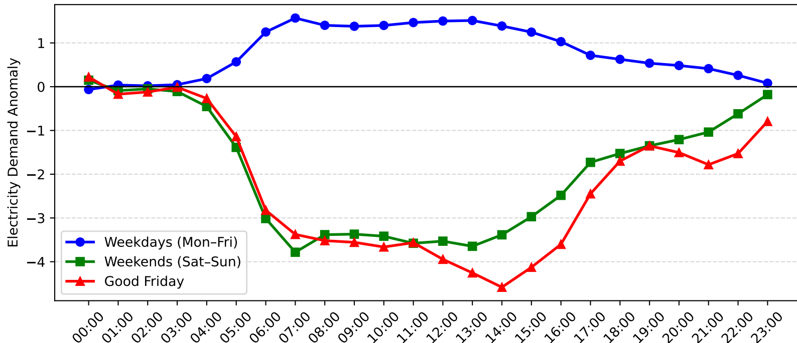
Wyong Demand Anomaly: Good Friday vs Weekday/Weekend (2008-2009)
