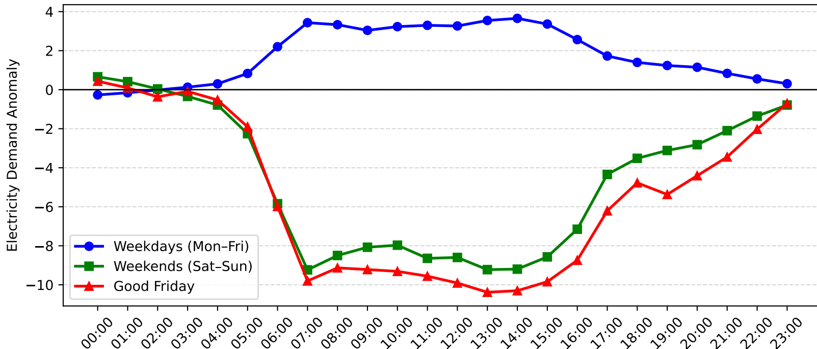
Marrickville Demand Anomaly: Good Friday vs Weekday/Weekend (2006-2007)
