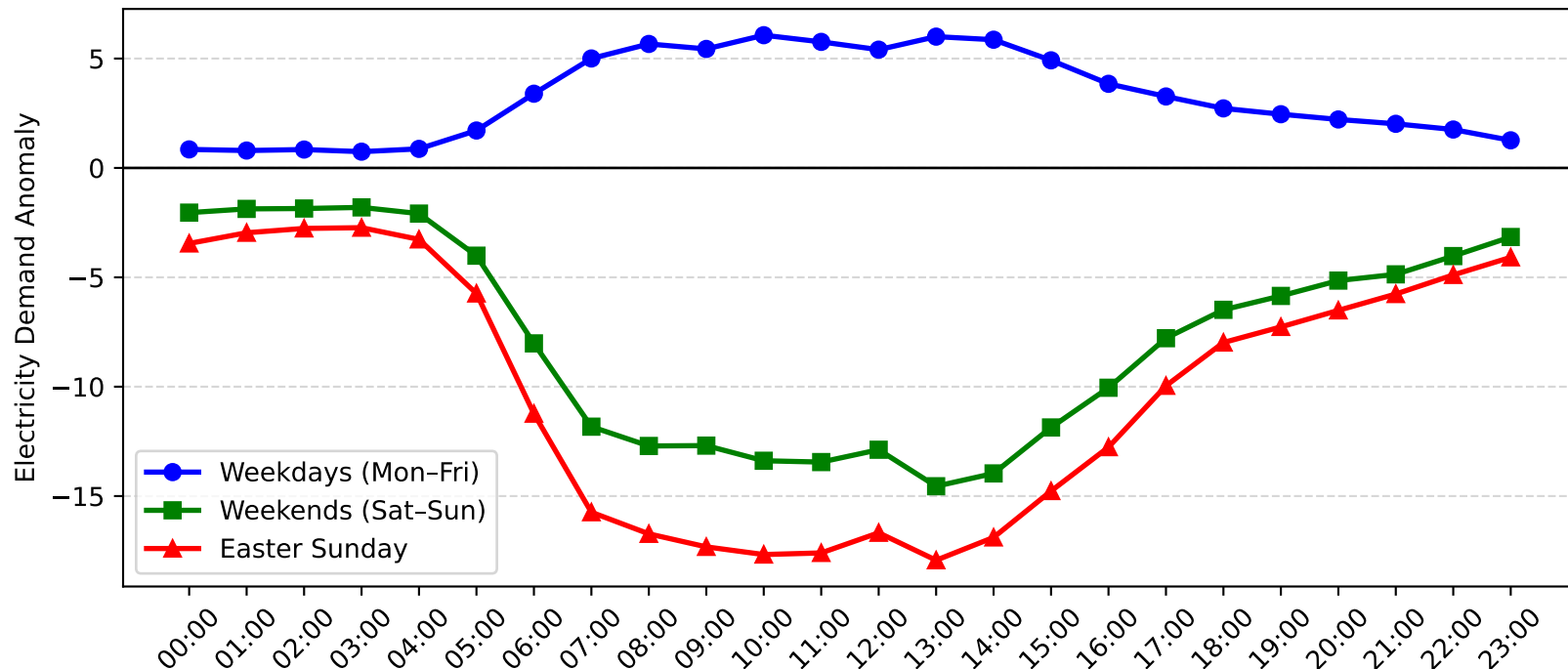
Milperra Demand Anomaly: Easter Sunday vs Weekday/Weekend (2005-2006)
