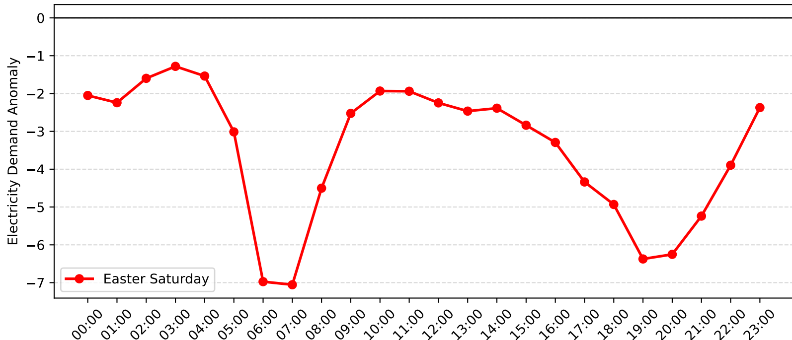
Pennant Hills Demand Anomaly: Easter Saturday (2011-2012)
