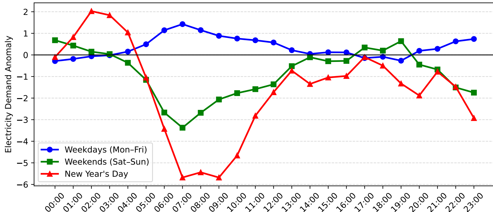
Meadowbank Demand Anomaly: New Year's Day vs Weekday/Weekend (2012-2013)
