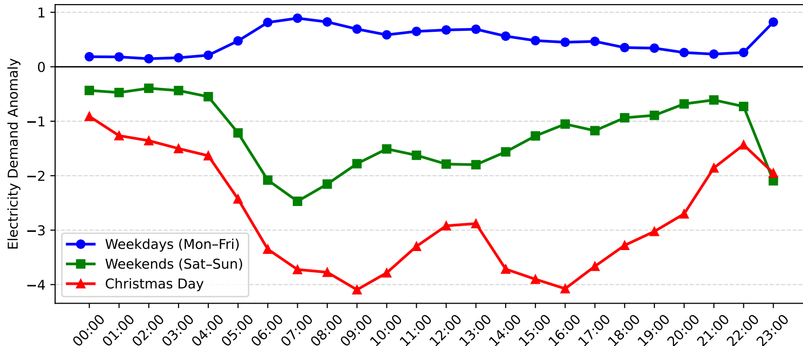
Rutherford Demand Anomaly: Christmas Day vs Weekday/Weekend (2009-2010)
