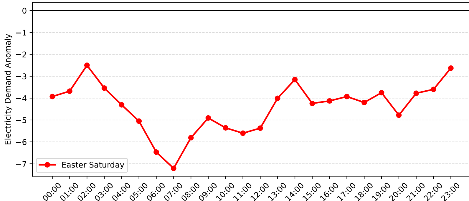
Meadowbank Demand Anomaly: Easter Saturday (2016-2017)
