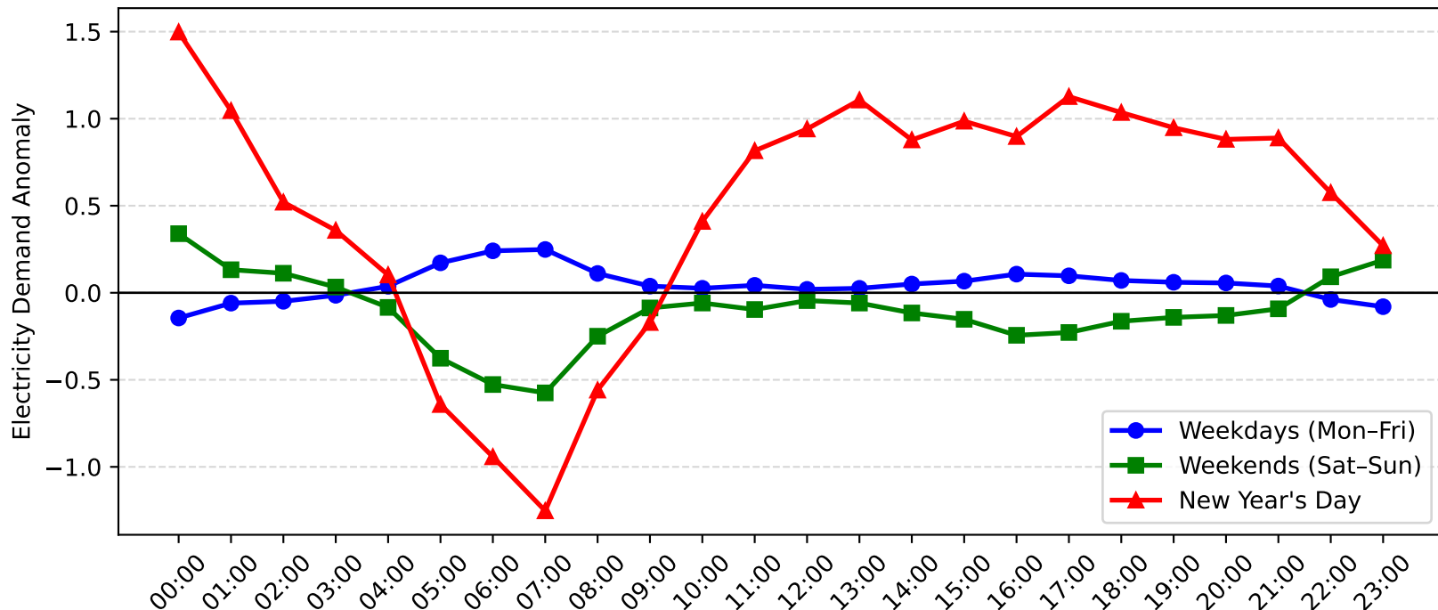
Noraville Demand Anomaly: New Year's Day vs Weekday/Weekend (2011-2012)
