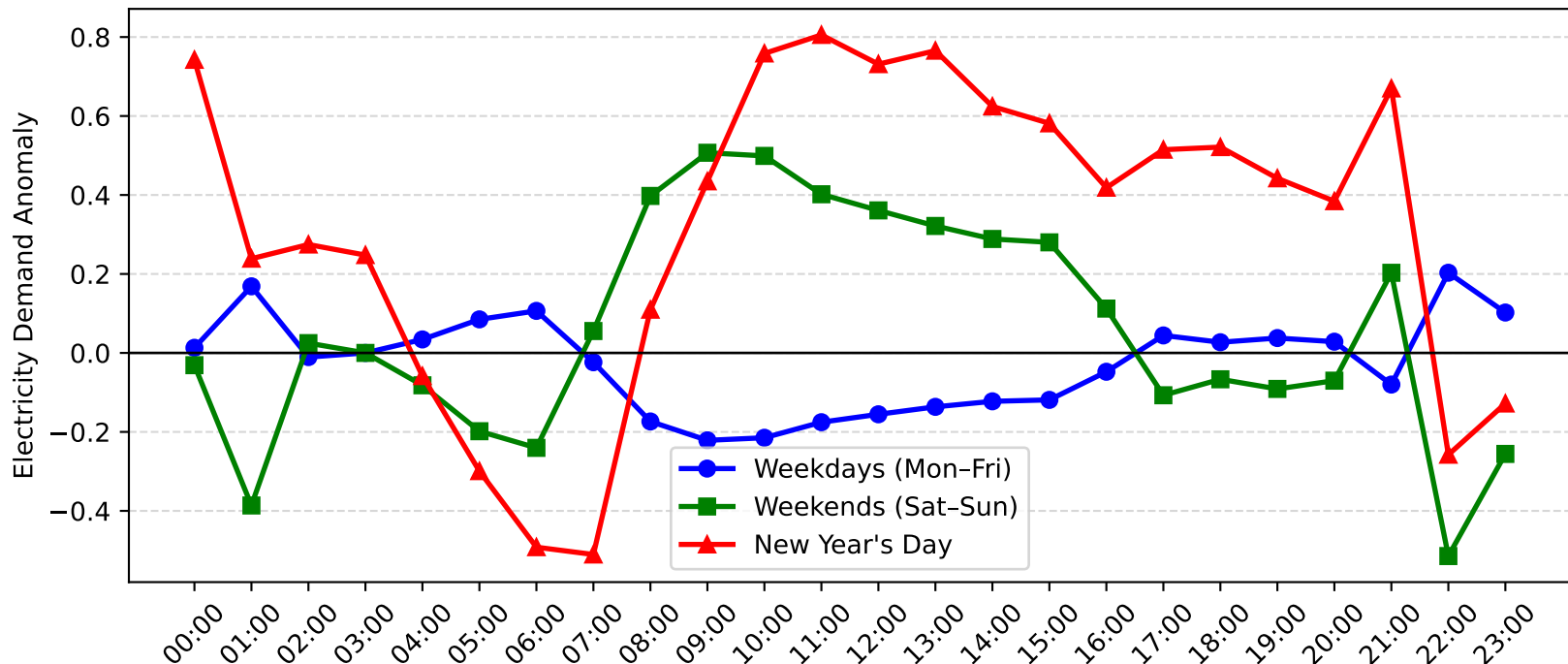
Swansea Demand Anomaly: New Year's Day vs Weekday/Weekend (2011-2012)
