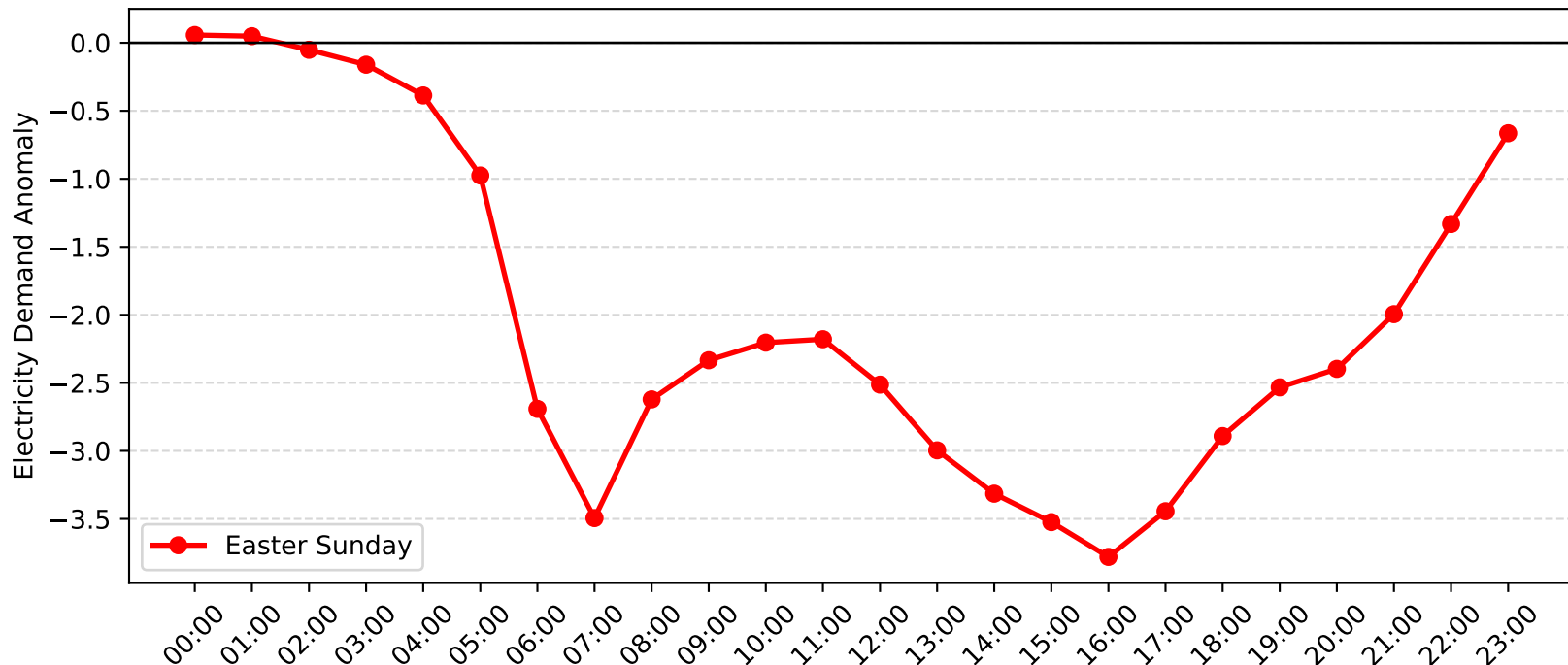
Blakehurst Demand Anomaly: Easter Sunday (2006-2007)
