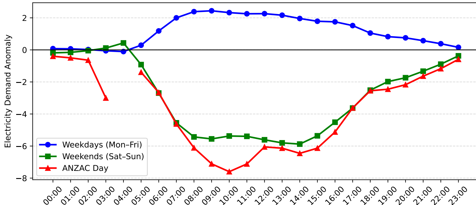
Green Square Demand Anomaly: ANZAC Day vs Weekday/Weekend (2016-2017)
