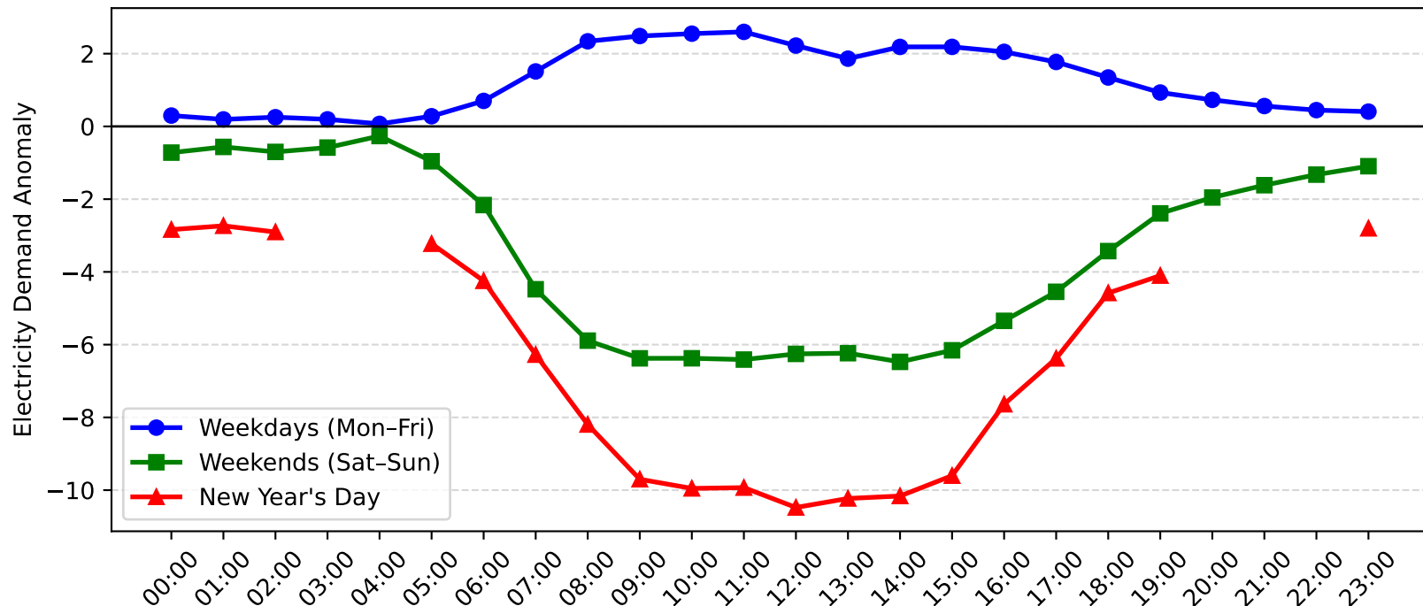
Green Square Demand Anomaly: New Year's Day vs Weekday/Weekend (2010-2011)
