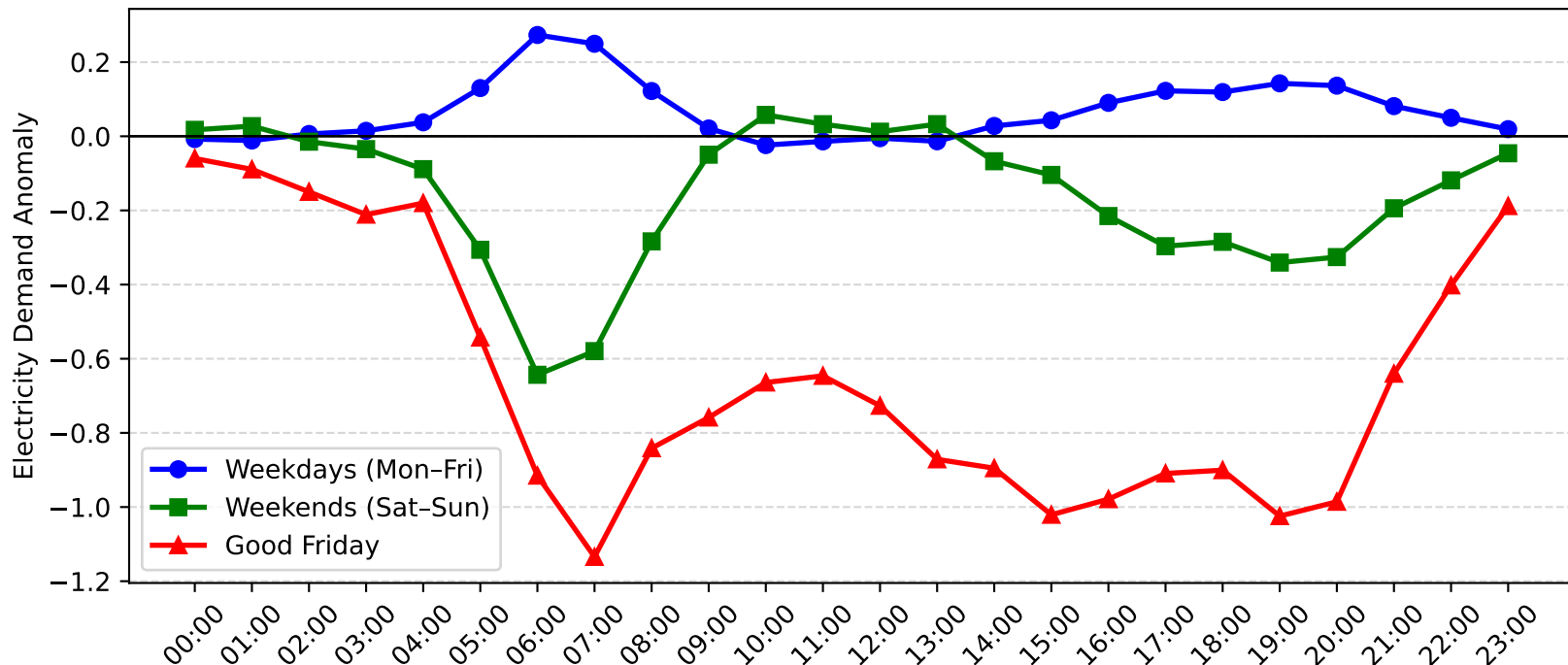
Narrabeen Demand Anomaly: Good Friday vs Weekday/Weekend (2016-2017)
