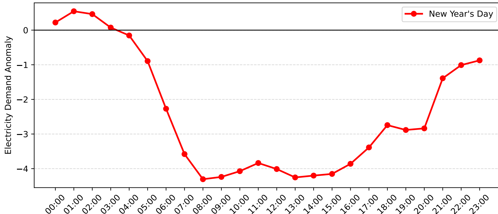
Pymble Demand Anomaly: New Year's Day (2007-2008)
