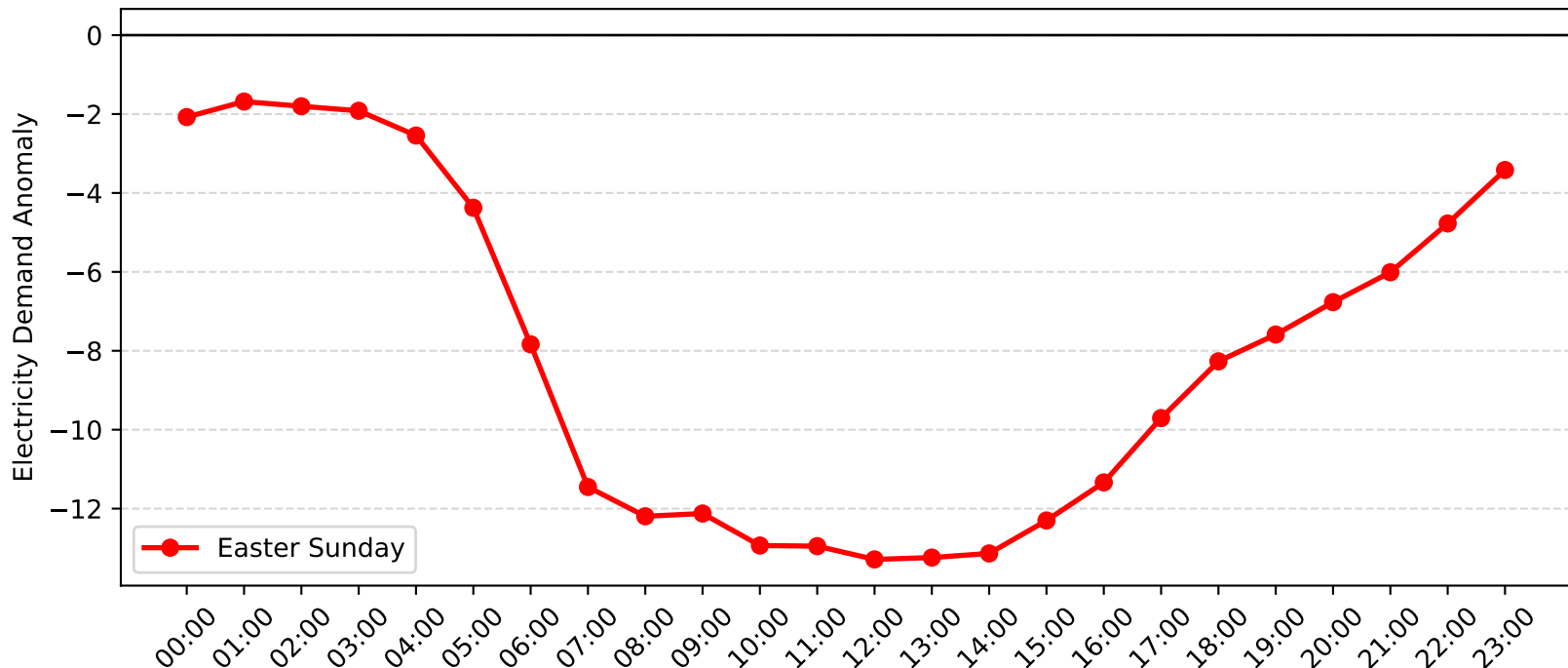
St. Peters Demand Anomaly: Easter Sunday (2010-2011)
