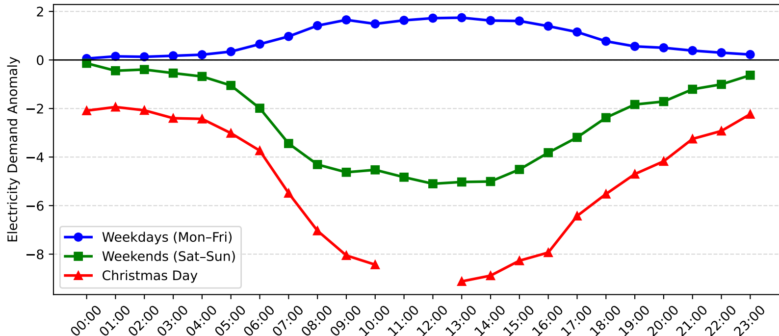
Caringbah Demand Anomaly: Christmas Day vs Weekday/Weekend (2008-2009)
