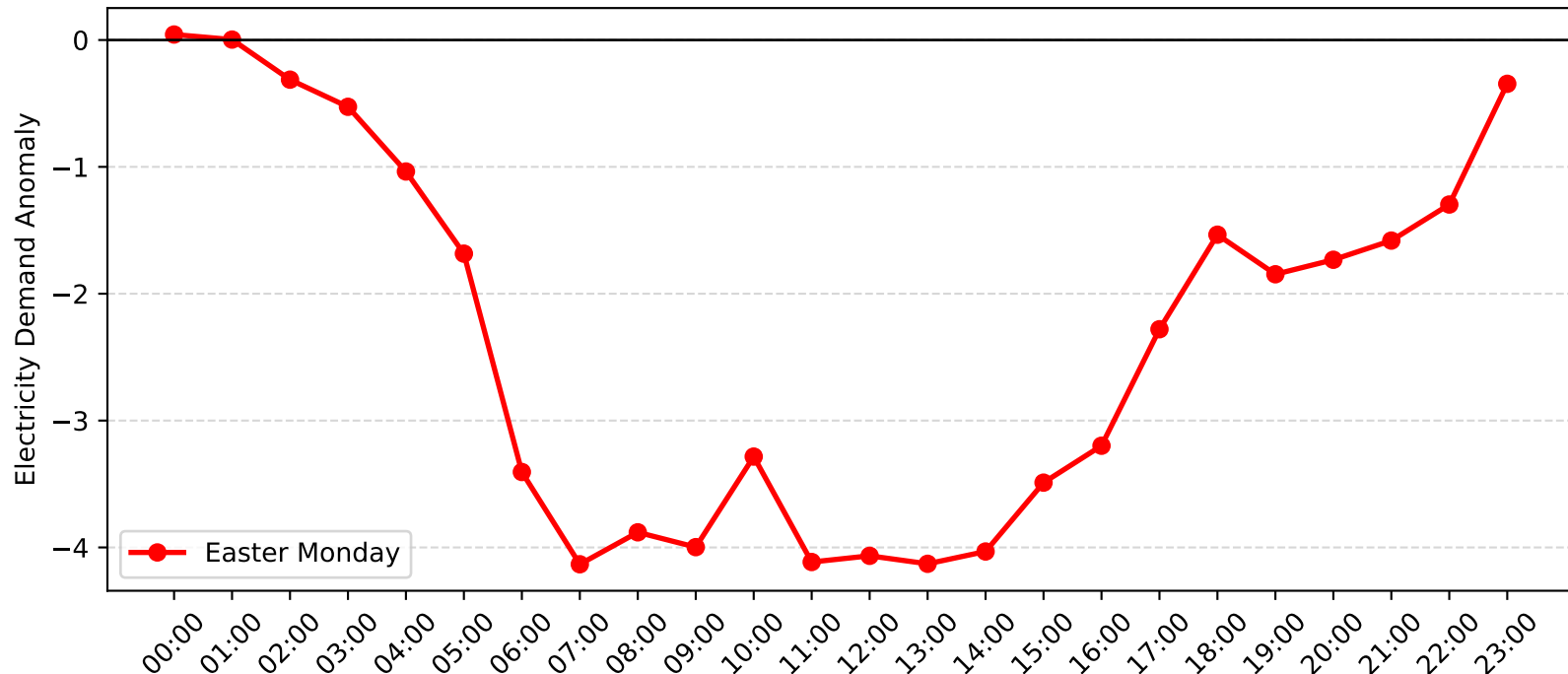
Wyong Demand Anomaly: Easter Monday (2006-2007)
