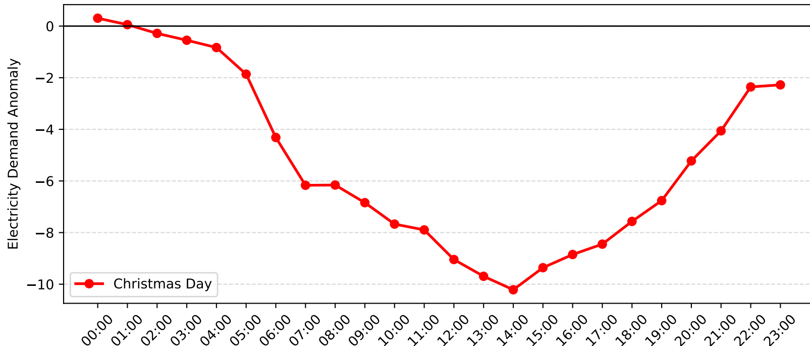
Hunters Hill Demand Anomaly: Christmas Day (2005-2006)
