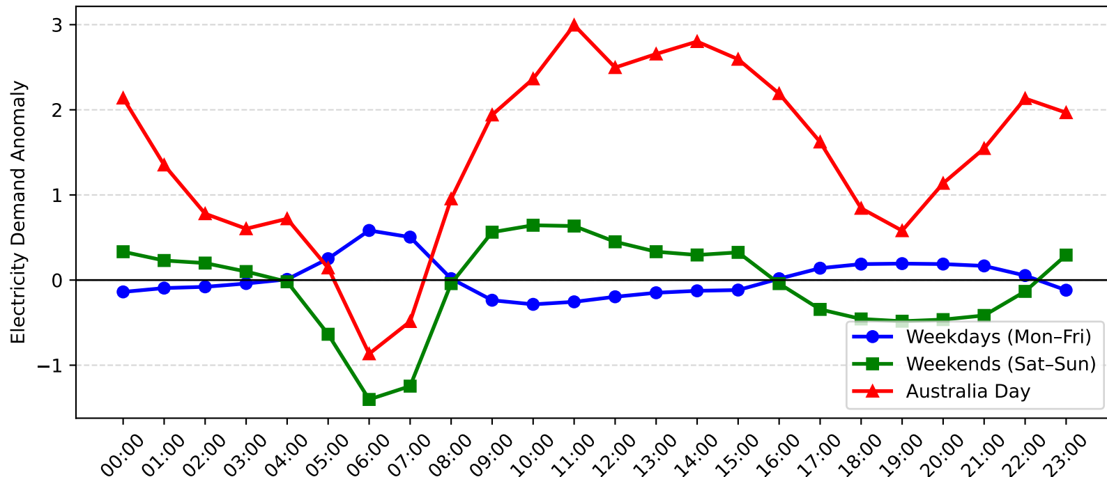
Avoca Demand Anomaly: Australia Day vs Weekday/Weekend (2012-2013)
