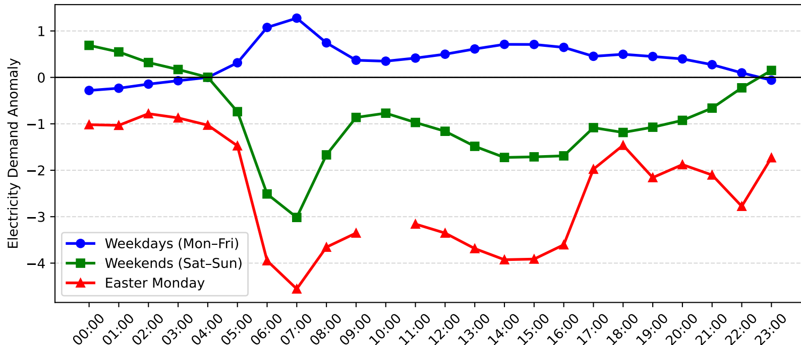
Five Dock Demand Anomaly: Easter Monday vs Weekday/Weekend (2005-2006)
