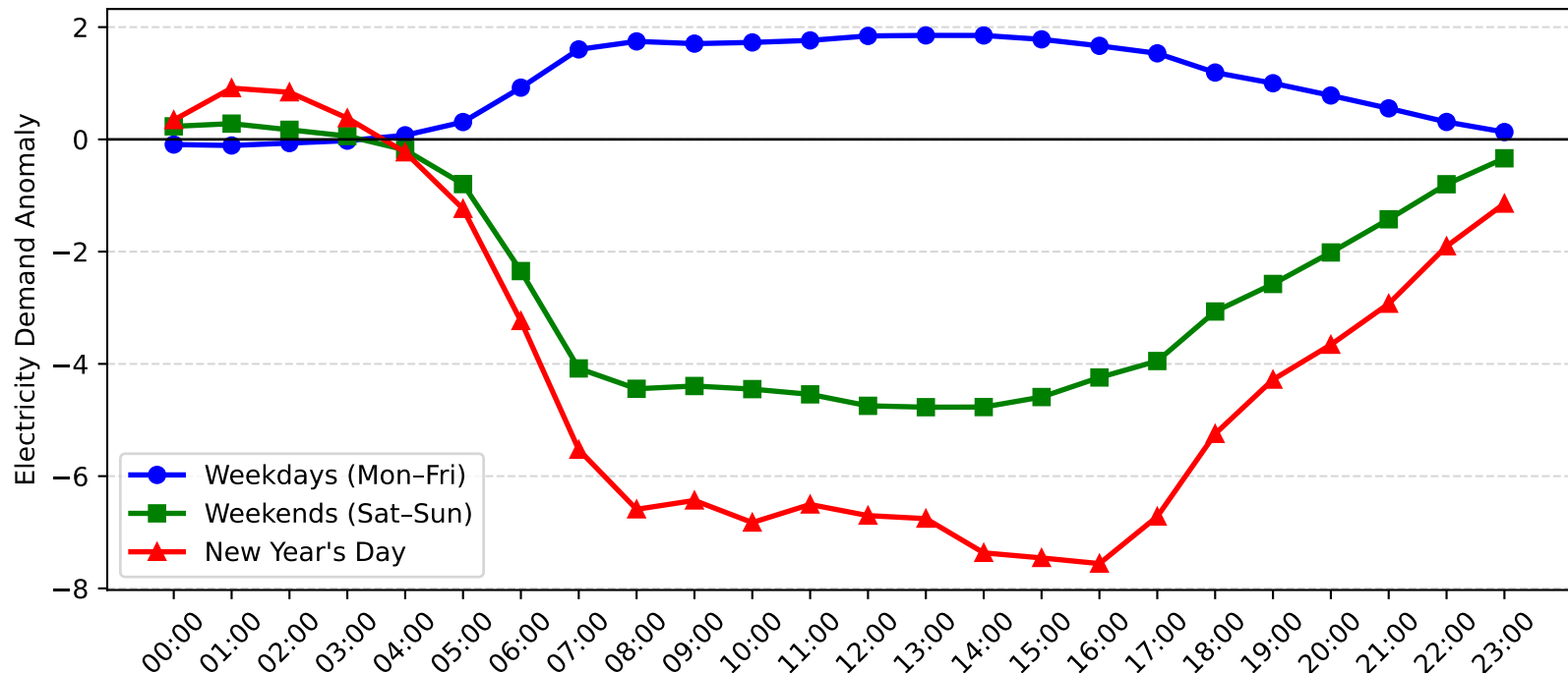
Top Ryde Demand Anomaly: New Year's Day vs Weekday/Weekend (2016-2017)
