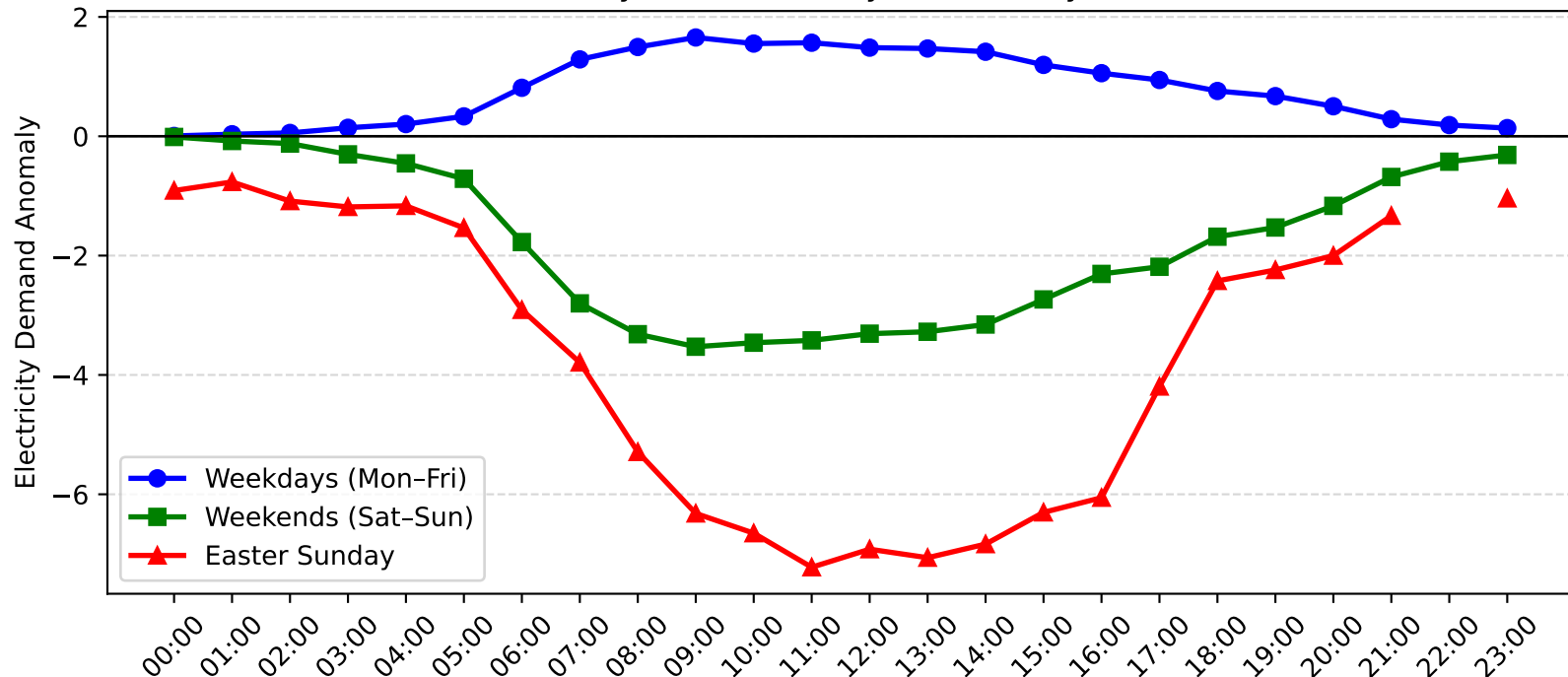
Auburn Demand Anomaly: Easter Sunday vs Weekday/Weekend (2009-2010)
