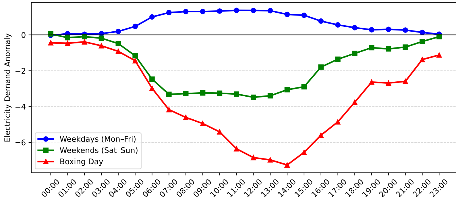
Wyong Demand Anomaly: Boxing Day vs Weekday/Weekend (2009-2010)
