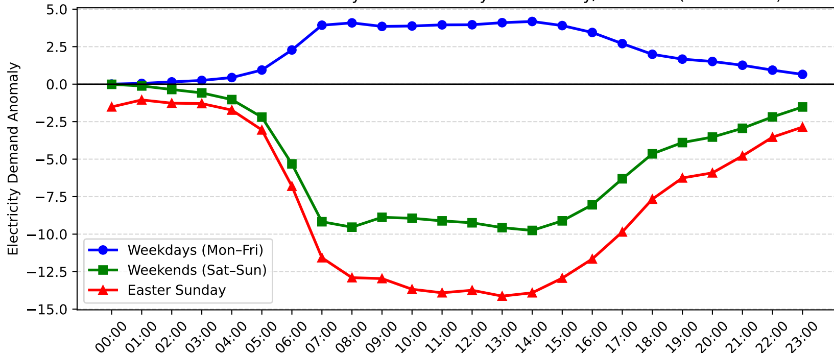
St. Peters Demand Anomaly: Easter Sunday vs Weekday/Weekend (2012-2013)
