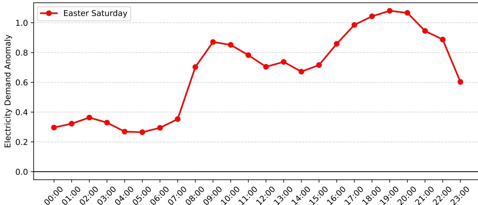
Rothbury Demand Anomaly: Easter Saturday (2015-2016)
