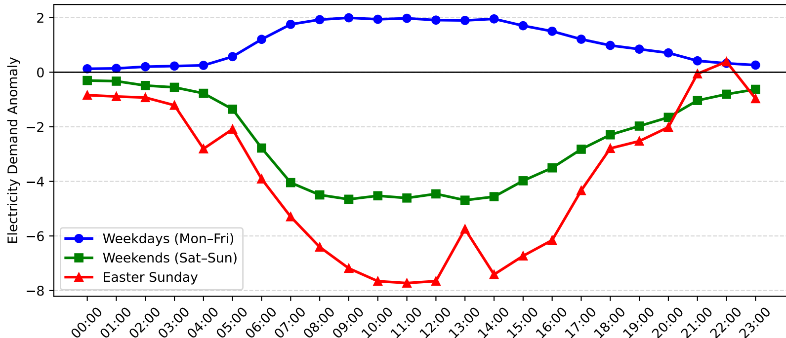
Auburn Demand Anomaly: Easter Sunday vs Weekday/Weekend (2011-2012)
