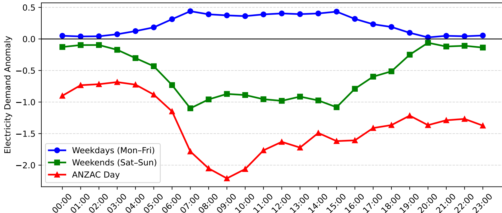
Lidcombe Demand Anomaly: ANZAC Day vs Weekday/Weekend (2004-2005)
