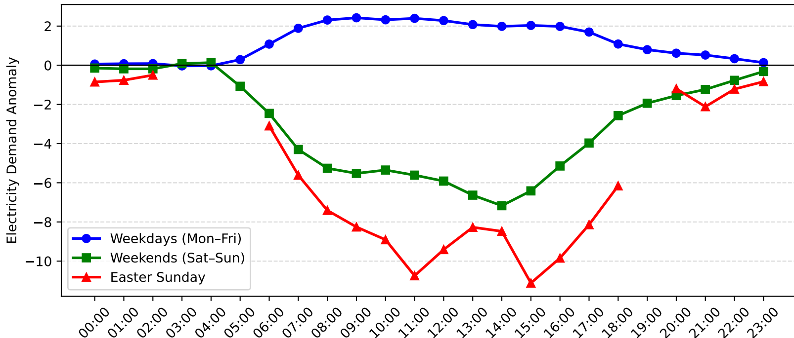
Green Square Demand Anomaly: Easter Sunday vs Weekday/Weekend (2015-2016)
