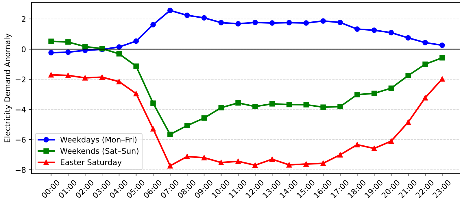
Burwood Demand Anomaly: Easter Saturday vs Weekday/Weekend (2010-2011)
