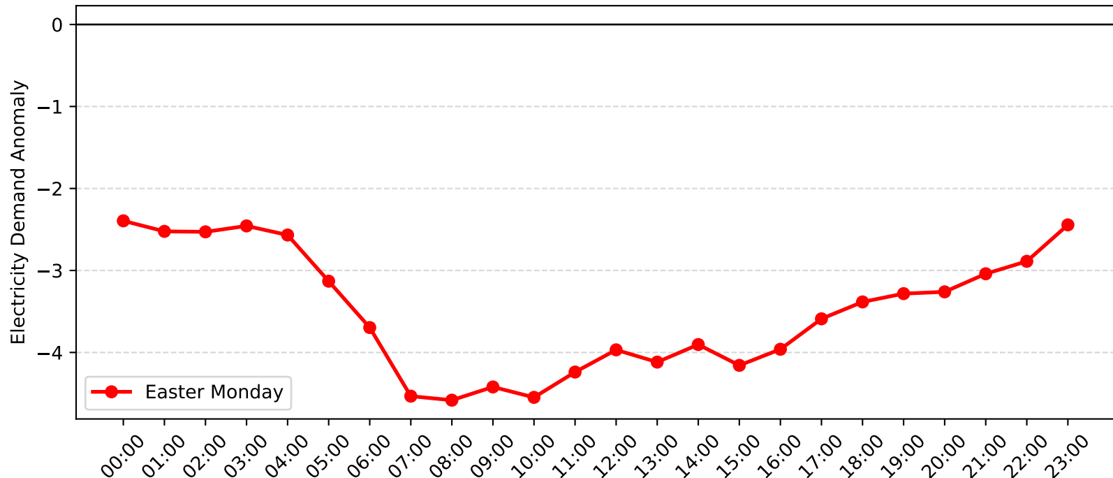
Bass Hill Demand Anomaly: Easter Monday (2017-2018)
