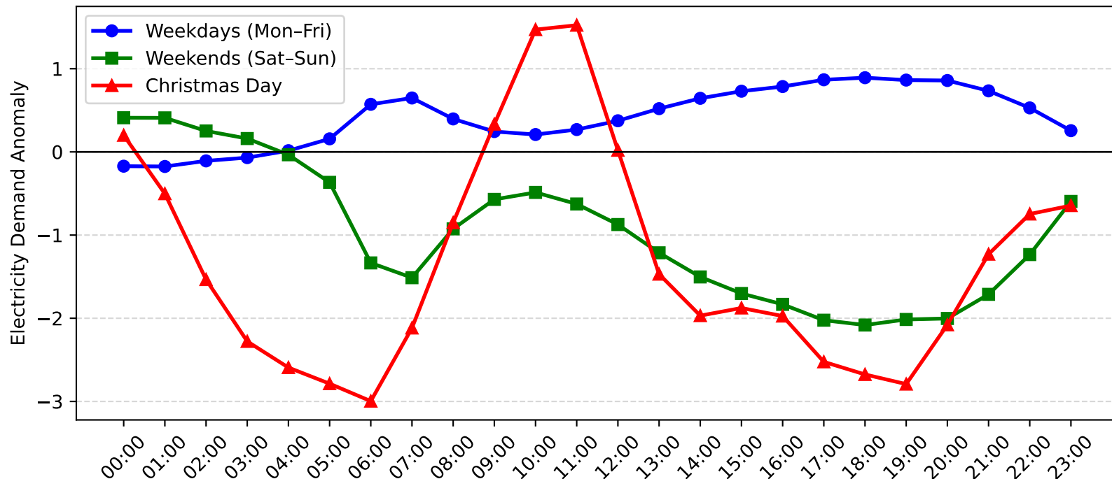
Mortdale Demand Anomaly: Christmas Day vs Weekday/Weekend (2016-2017)
