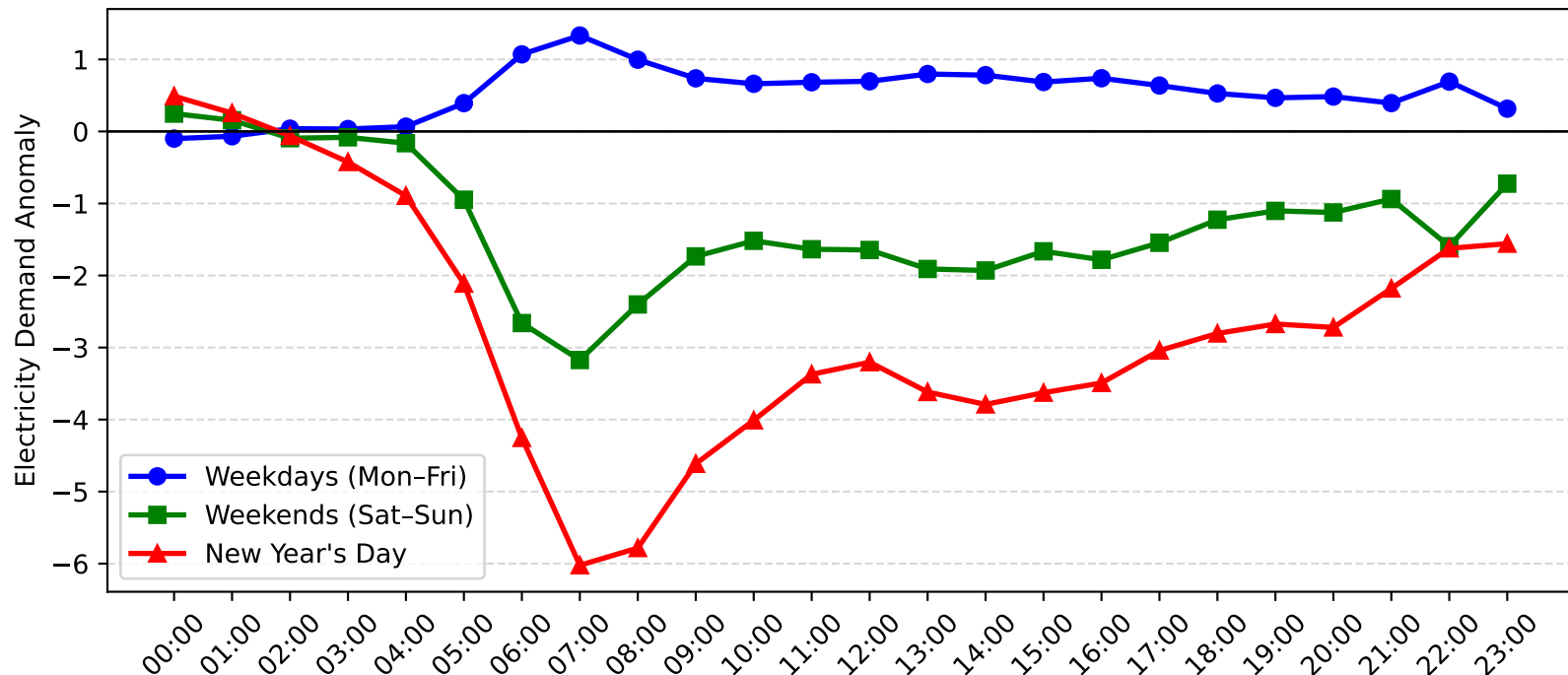
Dee Why West Demand Anomaly: New Year's Day vs Weekday/Weekend (2007-2008)
