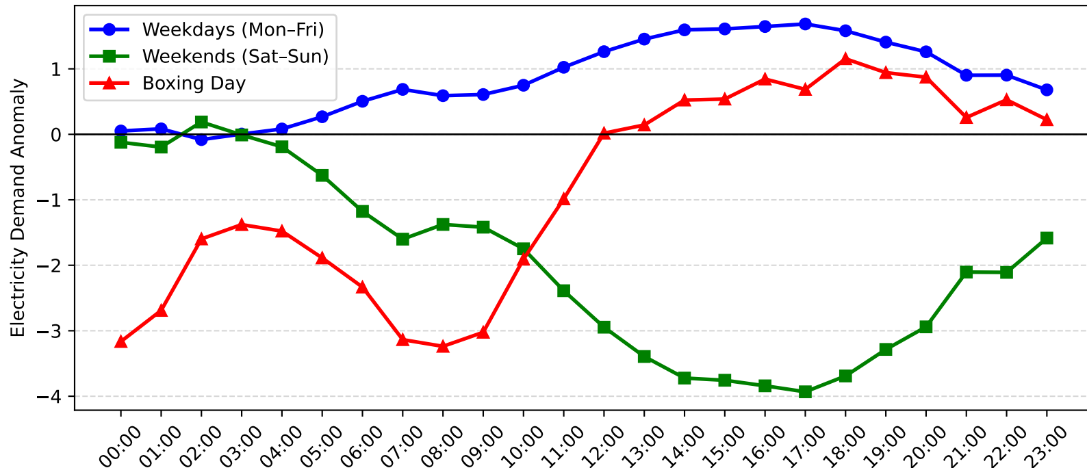
Jesmond Demand Anomaly: Boxing Day vs Weekday/Weekend (2016-2017)
