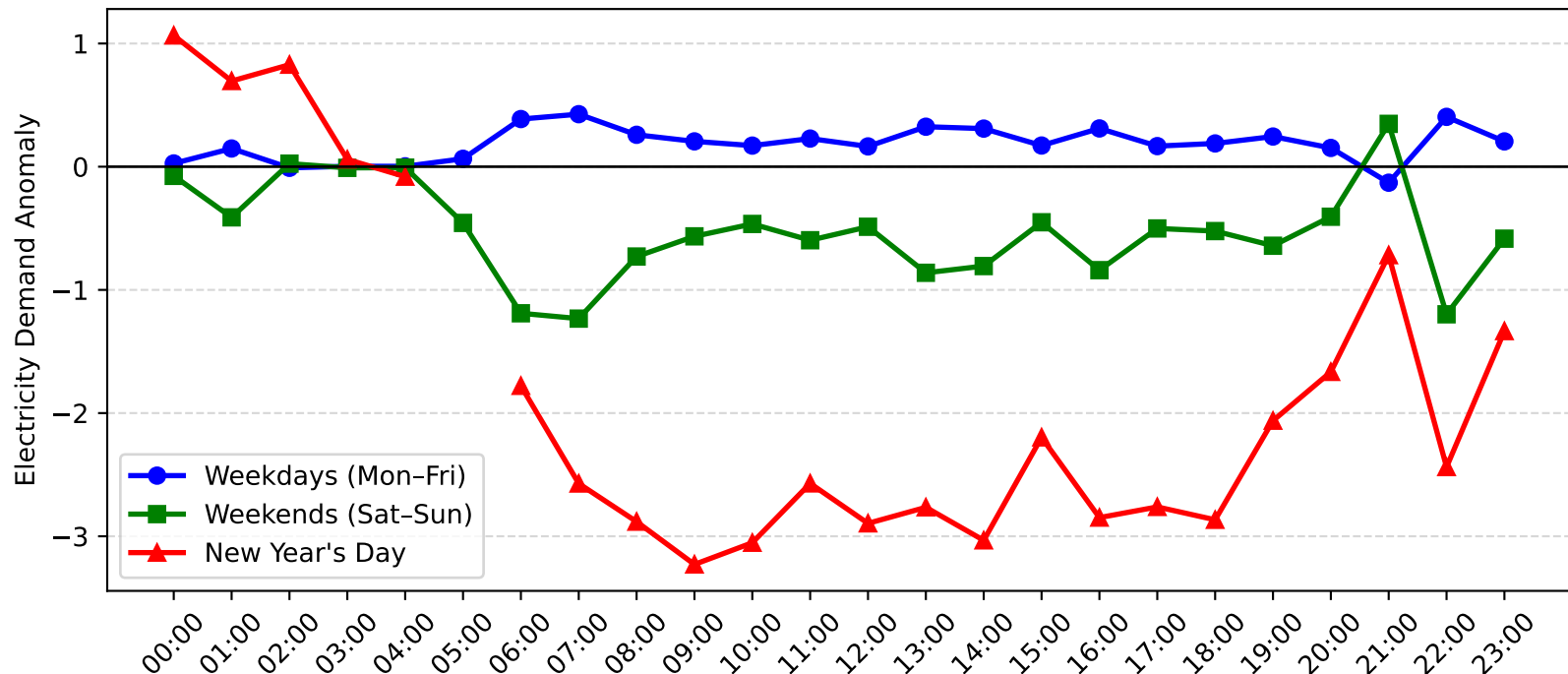
Charlestown Demand Anomaly: New Year's Day vs Weekday/Weekend (2014-2015)
