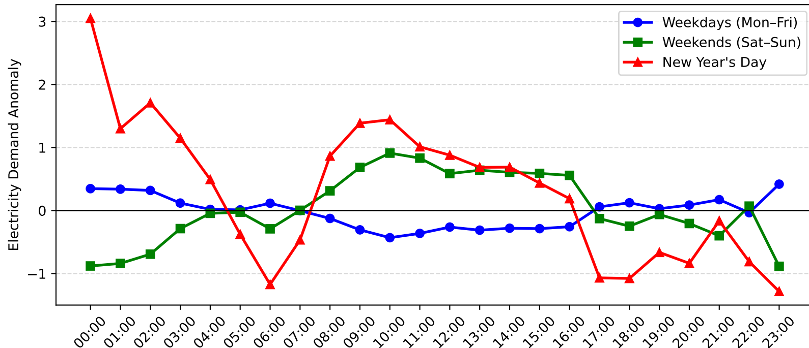
Nelson Bay Demand Anomaly: New Year's Day vs Weekday/Weekend (2004-2005)
