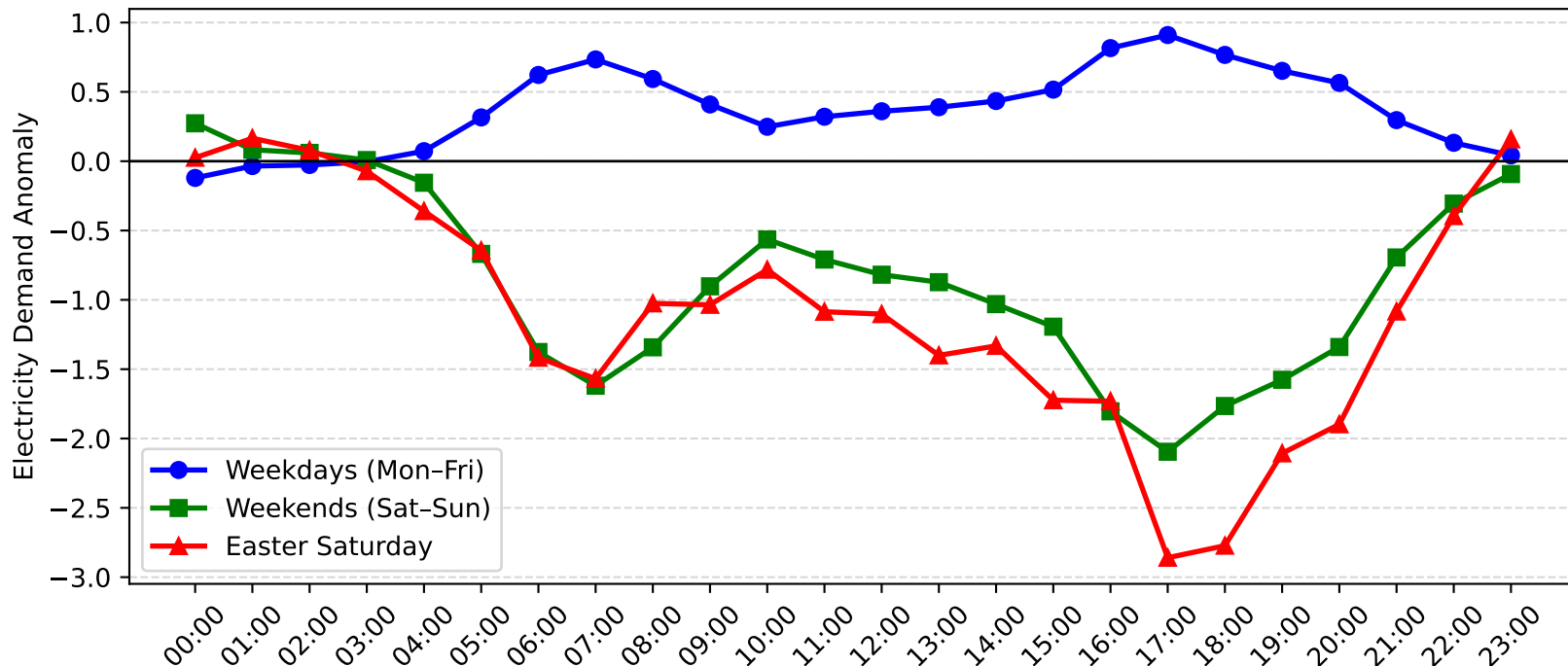
Erina Demand Anomaly: Easter Saturday vs Weekday/Weekend (2010-2011)
