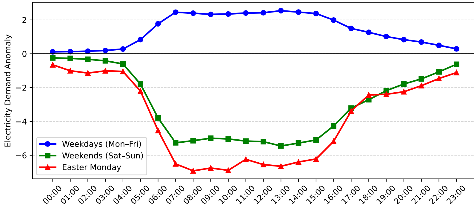
Bankstown Demand Anomaly: Easter Monday vs Weekday/Weekend (2017-2018)
