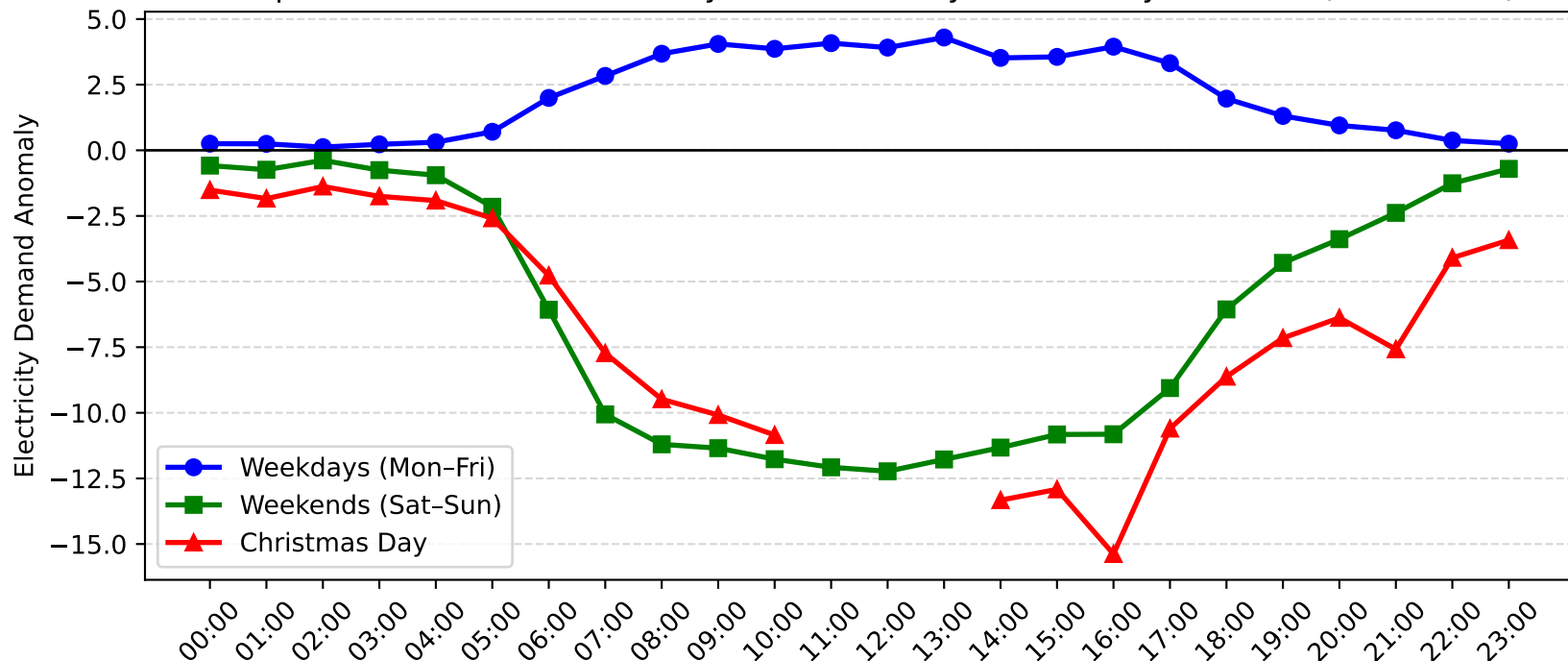
Macquarie Park Demand Anomaly: Christmas Day vs Weekday/Weekend (2008-2009)
