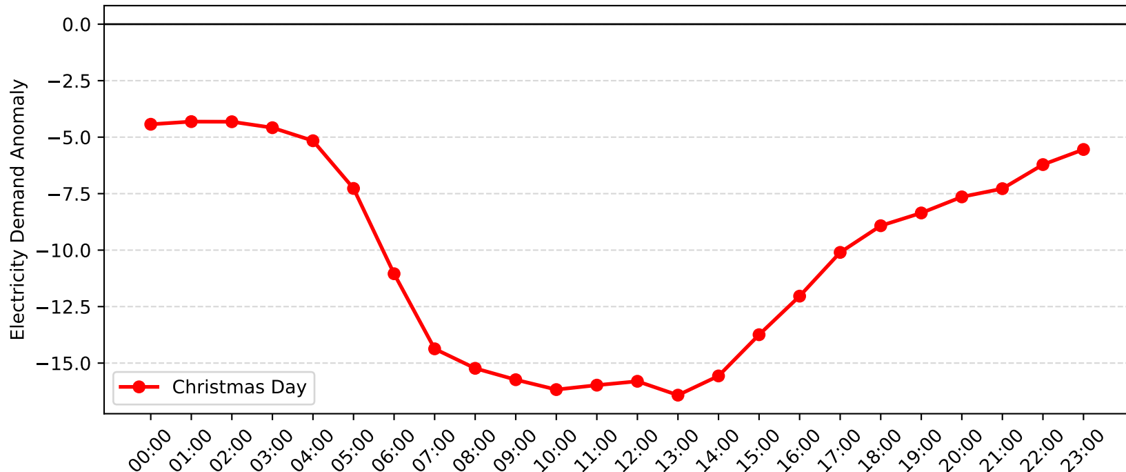
Milperra Demand Anomaly: Christmas Day (2005-2006)
