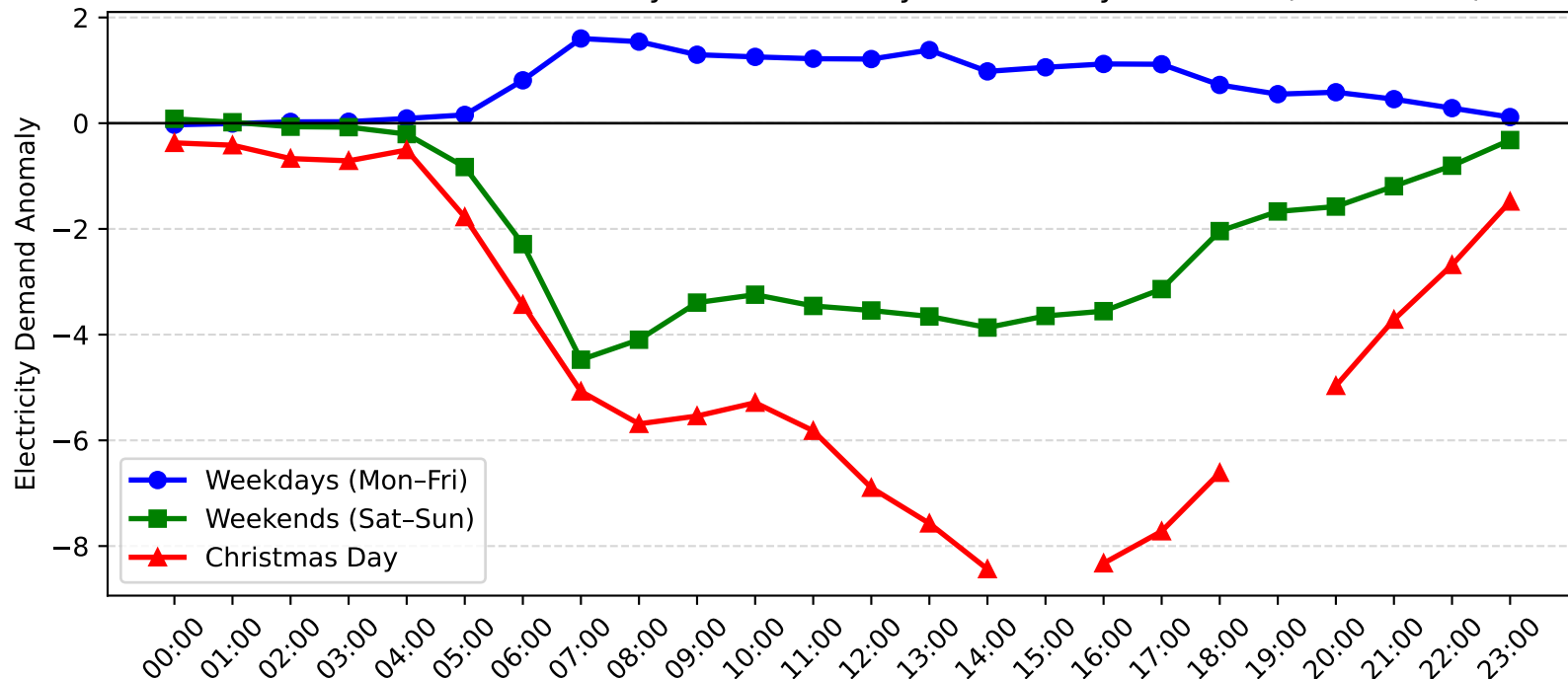
Chatswood Demand Anomaly: Christmas Day vs Weekday/Weekend (2014-2015)
