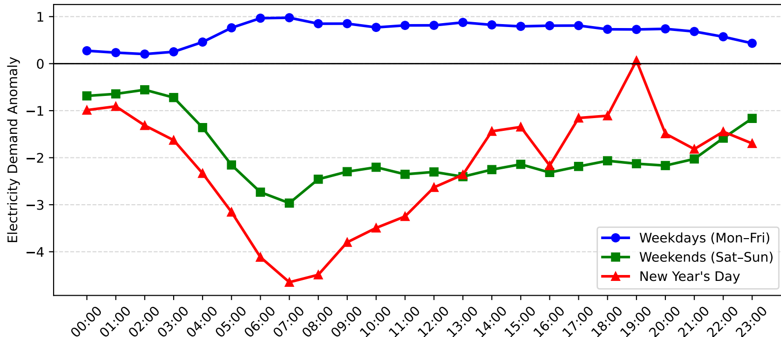
Lisarow Demand Anomaly: New Year's Day vs Weekday/Weekend (2008-2009)
