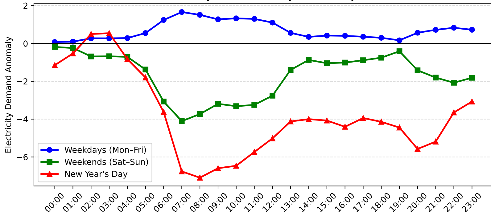
Meadowbank Demand Anomaly: New Year's Day vs Weekday/Weekend (2016-2017)
