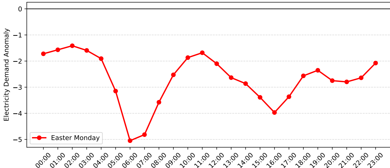
Pennant Hills Demand Anomaly: Easter Monday (2016-2017)
