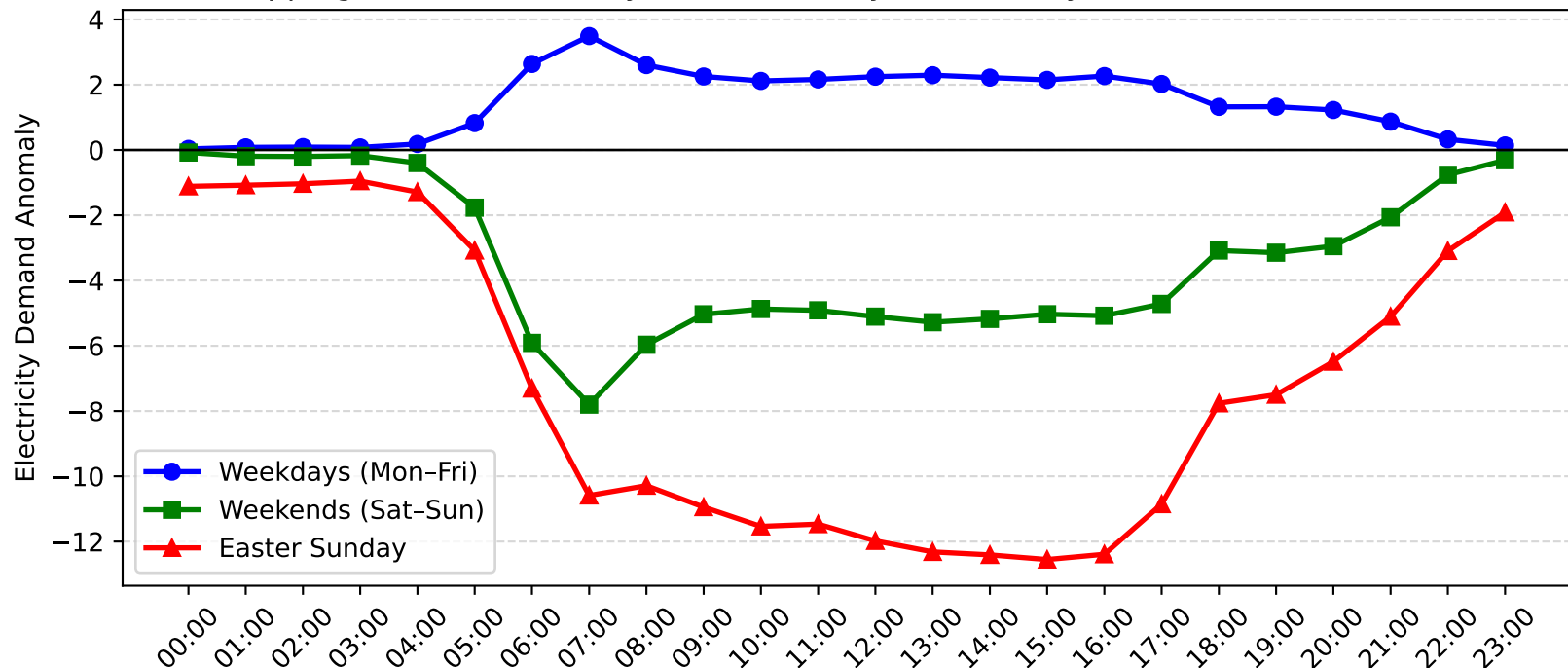
Epping Demand Anomaly: Easter Sunday vs Weekday/Weekend (2010-2011)
