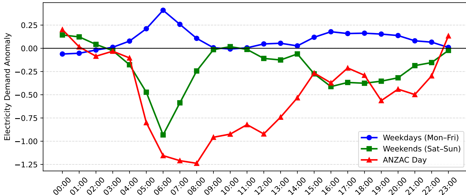
Woy Woy Demand Anomaly: ANZAC Day vs Weekday/Weekend (2016-2017)
