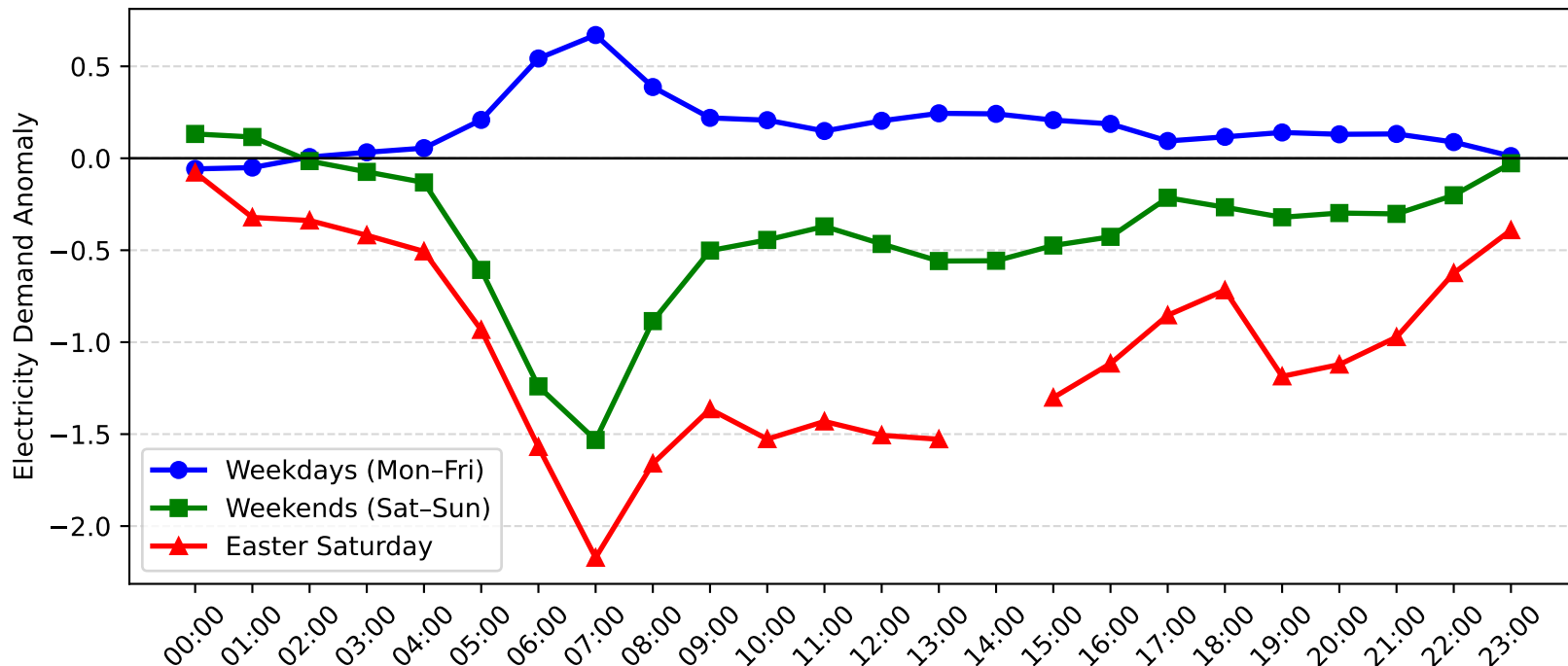
Arncliffe Demand Anomaly: Easter Saturday vs Weekday/Weekend (2017-2018)
