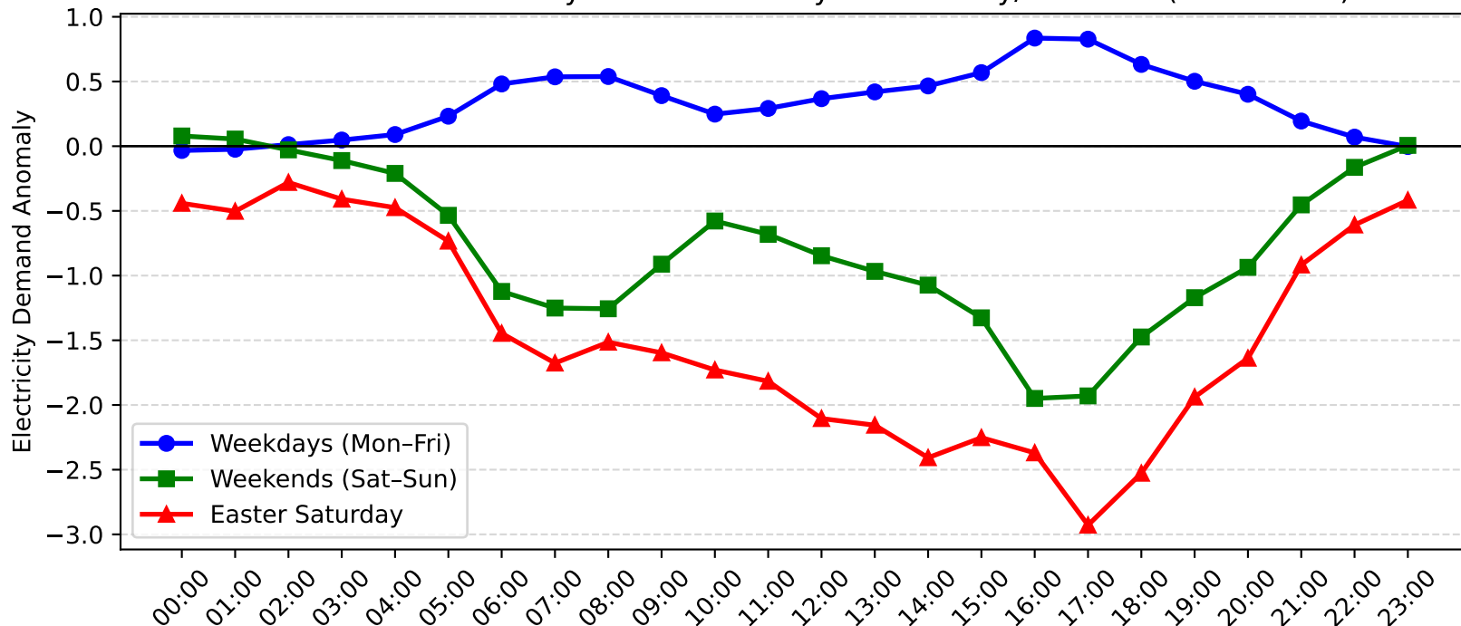
Erina Demand Anomaly: Easter Saturday vs Weekday/Weekend (2013-2014)
