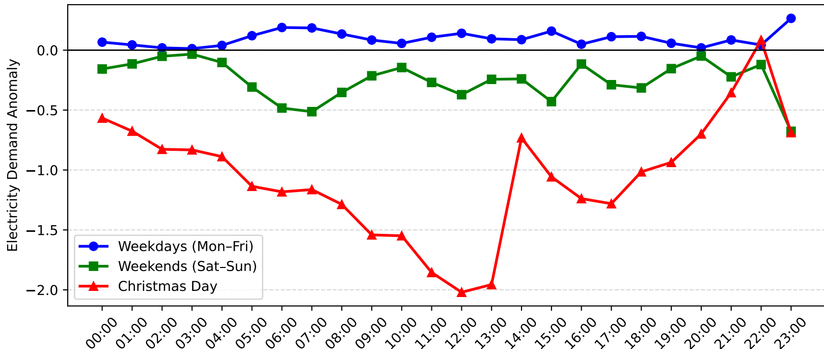
Telarah Demand Anomaly: Christmas Day vs Weekday/Weekend (2009-2010)
