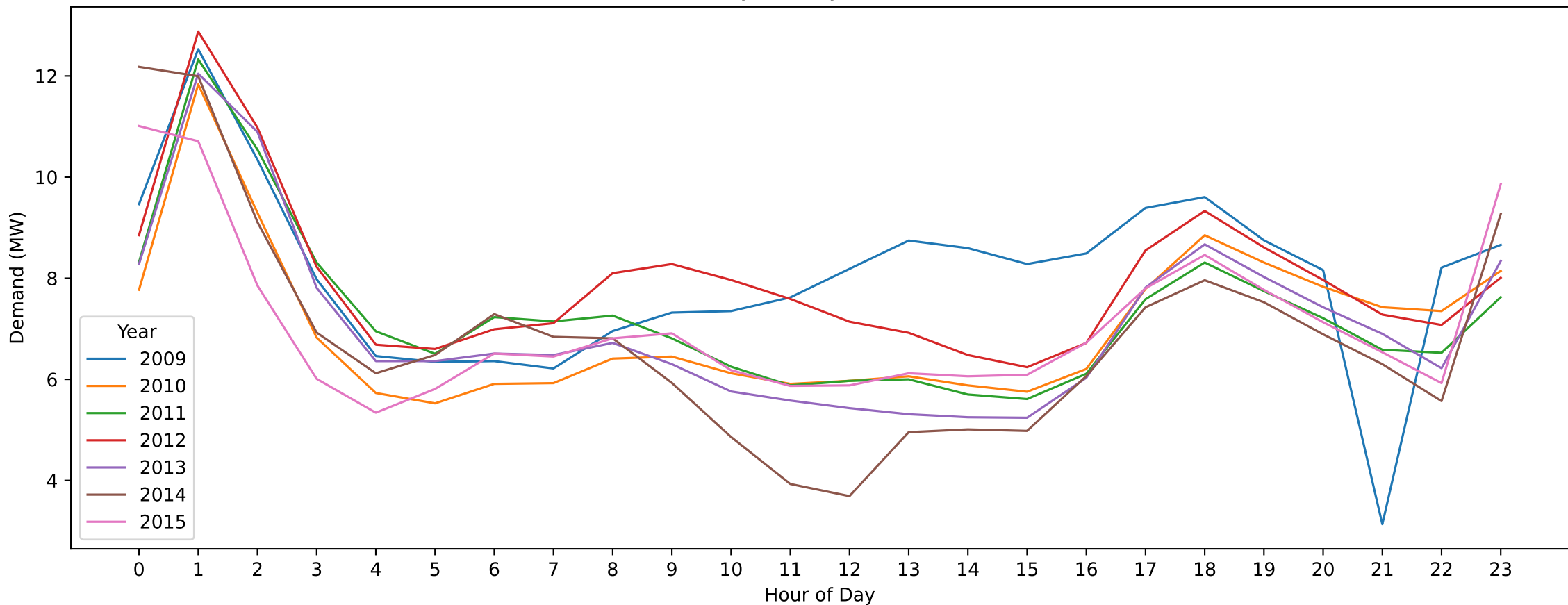
MYT — ANZAC Day (Hourly Demand Across Years)
