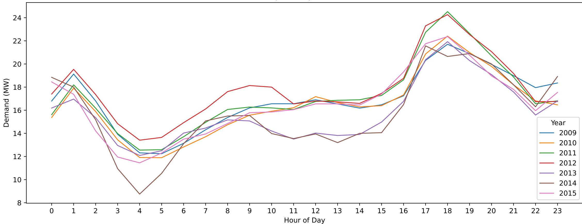
TGN — ANZAC Day (Hourly Demand Across Years)
