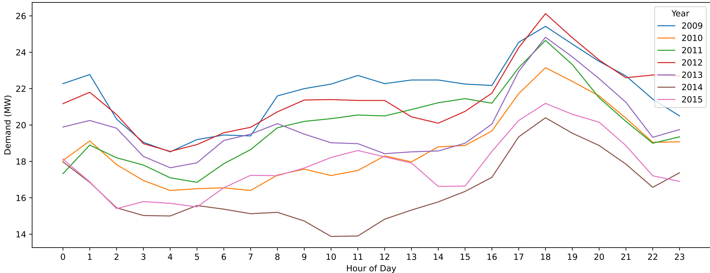
WO — ANZAC Day (Hourly Demand Across Years)
