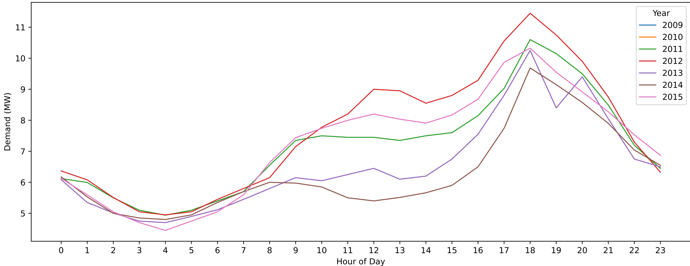
LYD — ANZAC Day (Hourly Demand Across Years)
