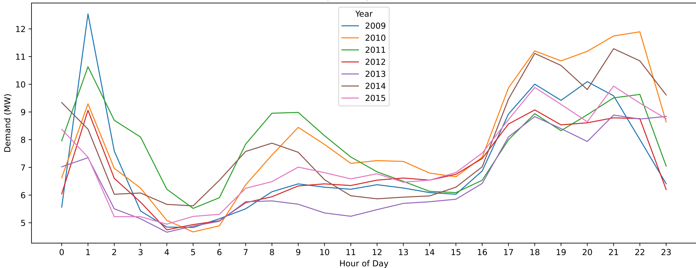
PHI — ANZAC Day (Hourly Demand Across Years)
