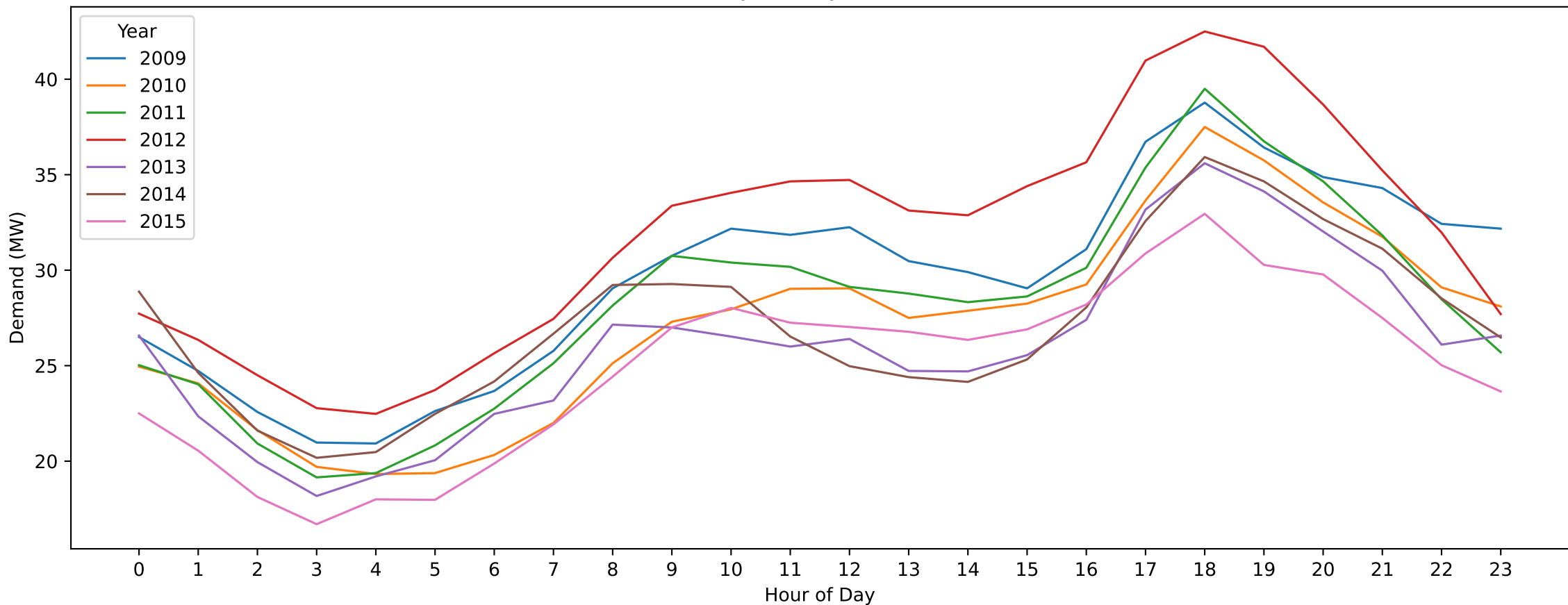
CYN — ANZAC Day (Hourly Demand Across Years)
