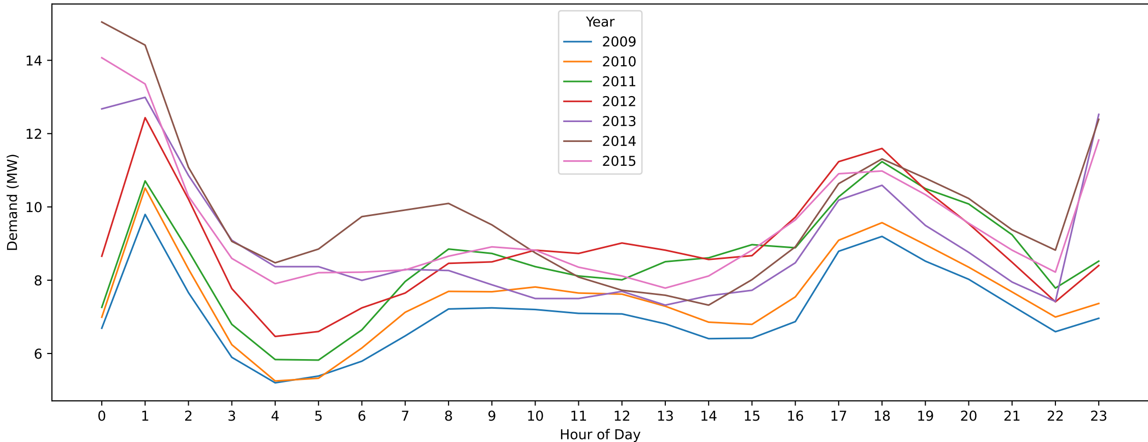
LLG — ANZAC Day (Hourly Demand Across Years)
