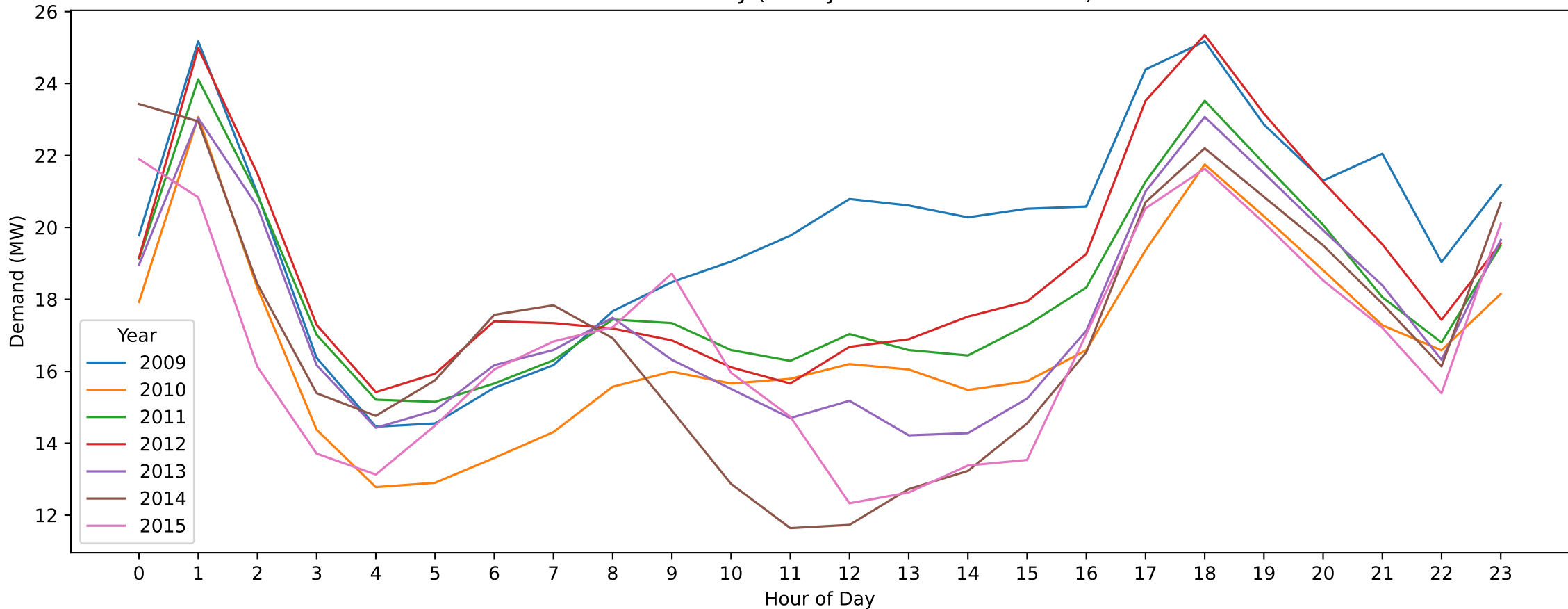
WN — ANZAC Day (Hourly Demand Across Years)
