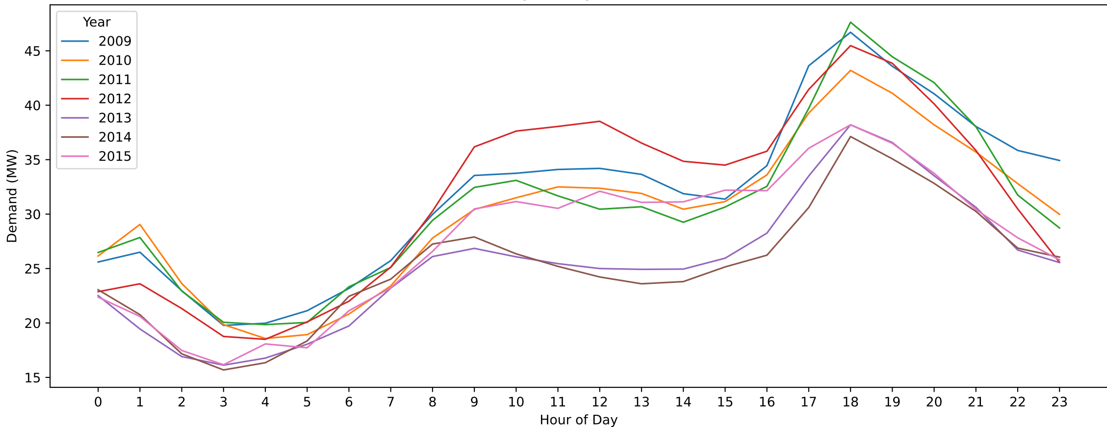
ELM — ANZAC Day (Hourly Demand Across Years)
