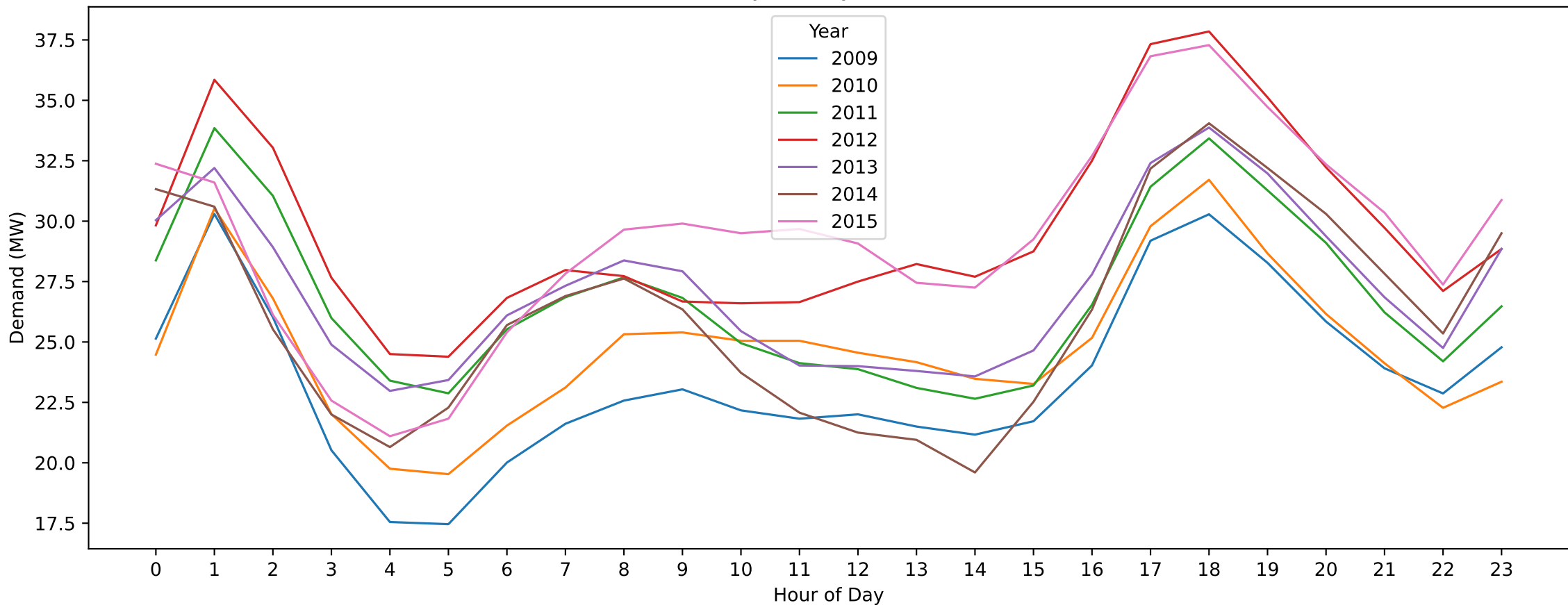
WGL — ANZAC Day (Hourly Demand Across Years)
