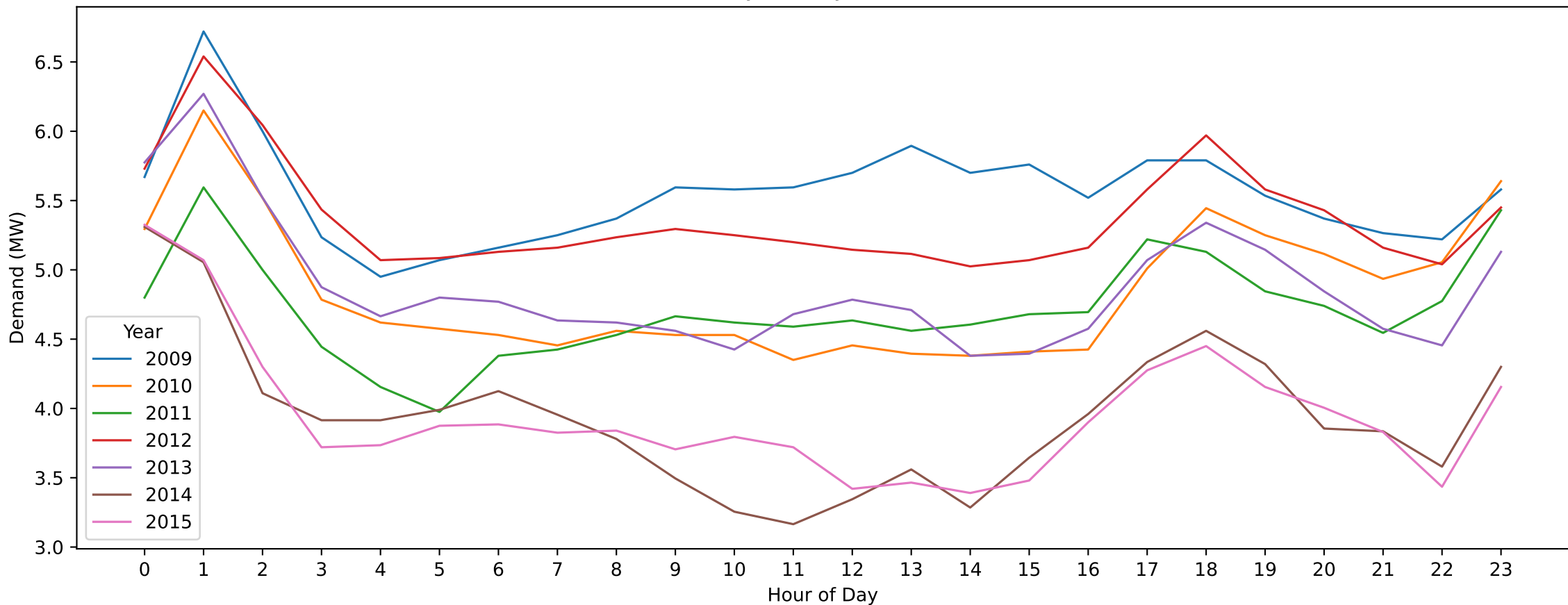
BWA — ANZAC Day (Hourly Demand Across Years)
