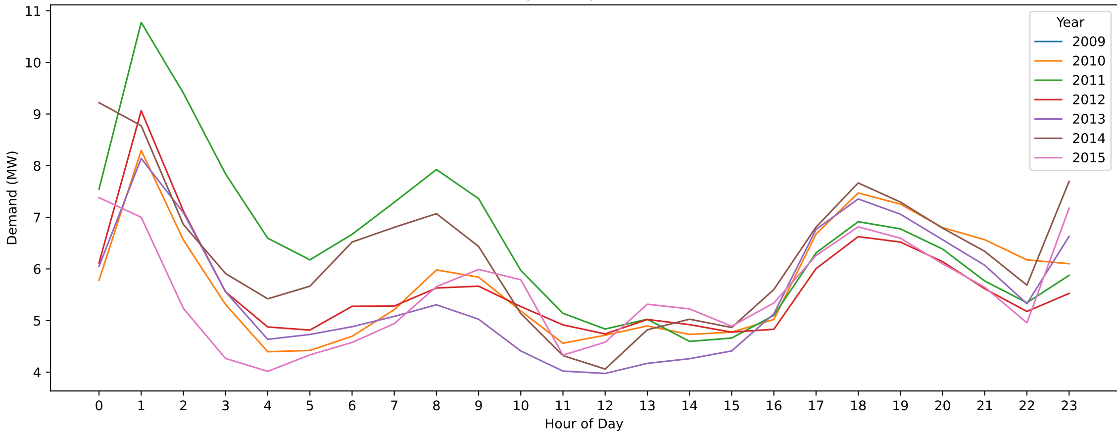
BRT — ANZAC Day (Hourly Demand Across Years)
