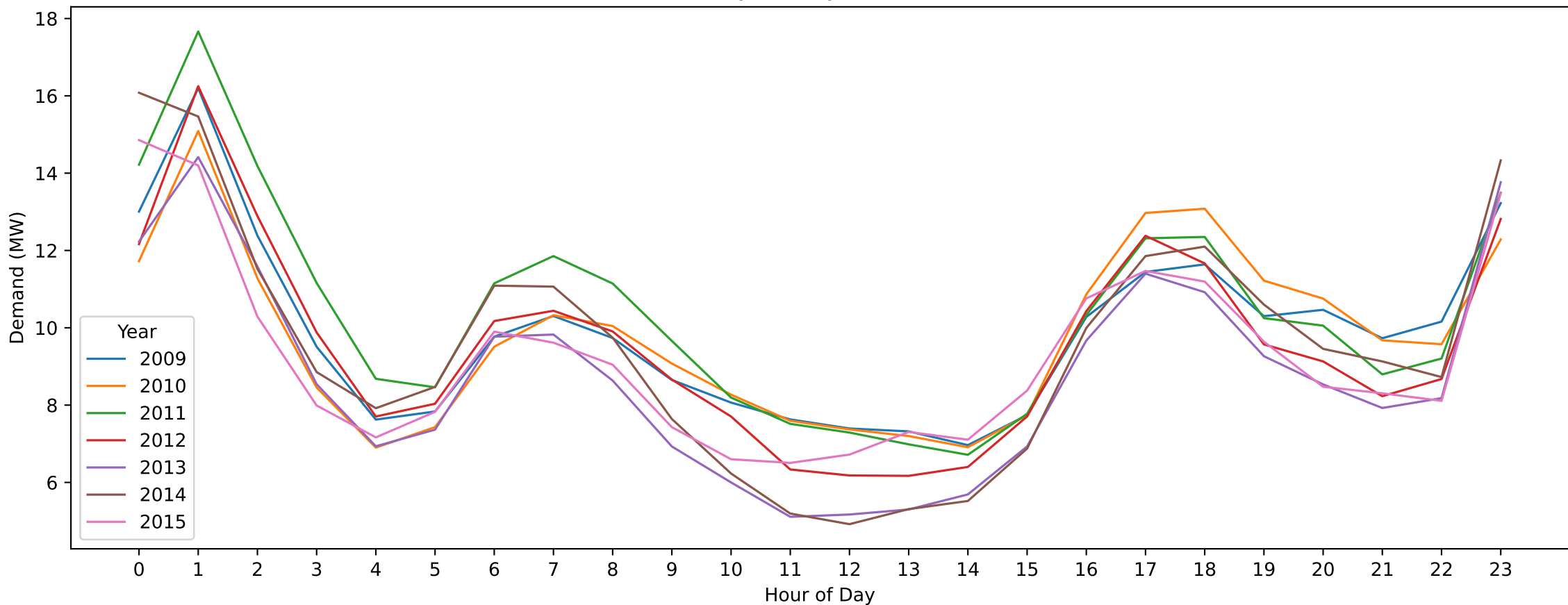
FTR — ANZAC Day (Hourly Demand Across Years)
