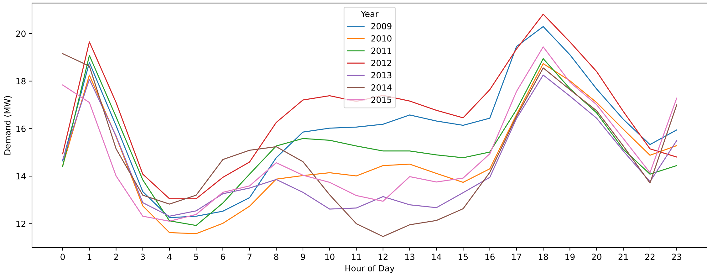
SMR — ANZAC Day (Hourly Demand Across Years)
