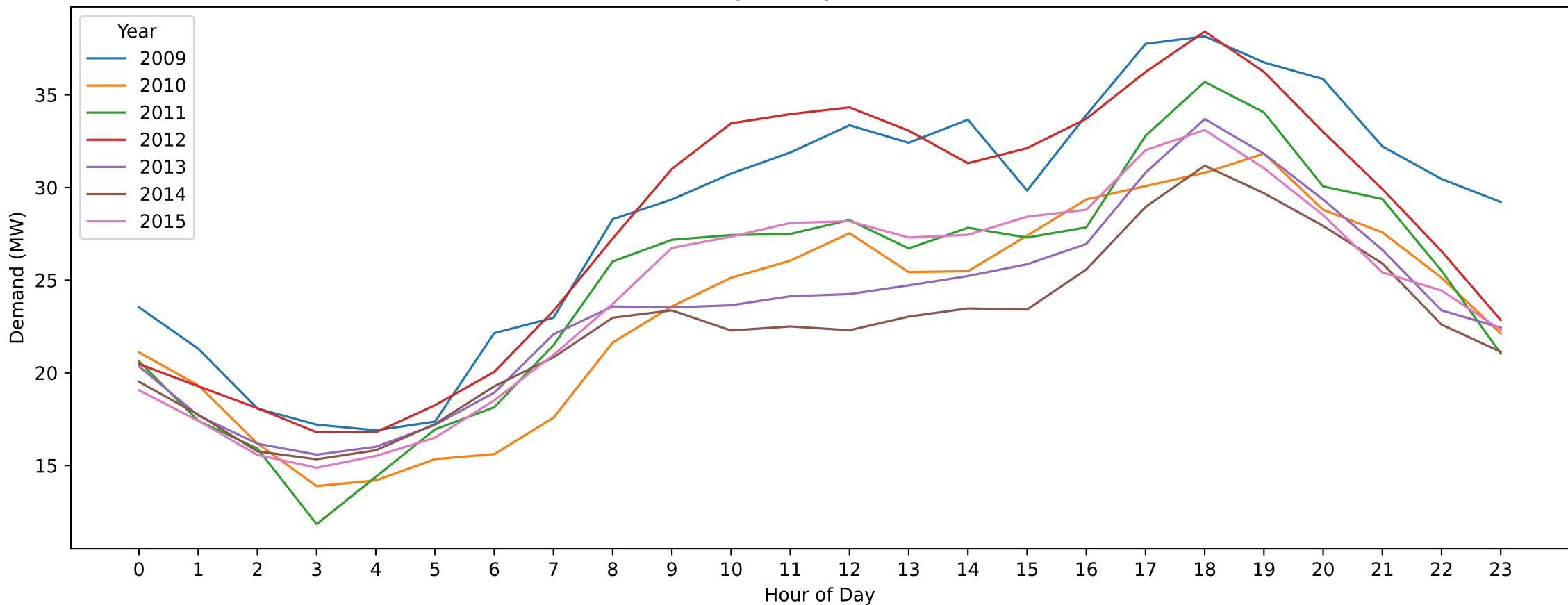
WT — ANZAC Day (Hourly Demand Across Years)
