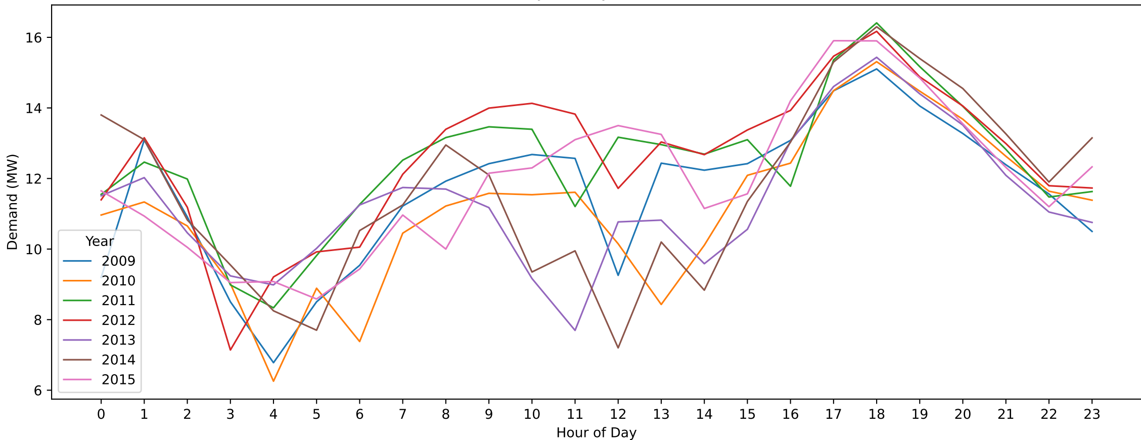
SLE — ANZAC Day (Hourly Demand Across Years)
