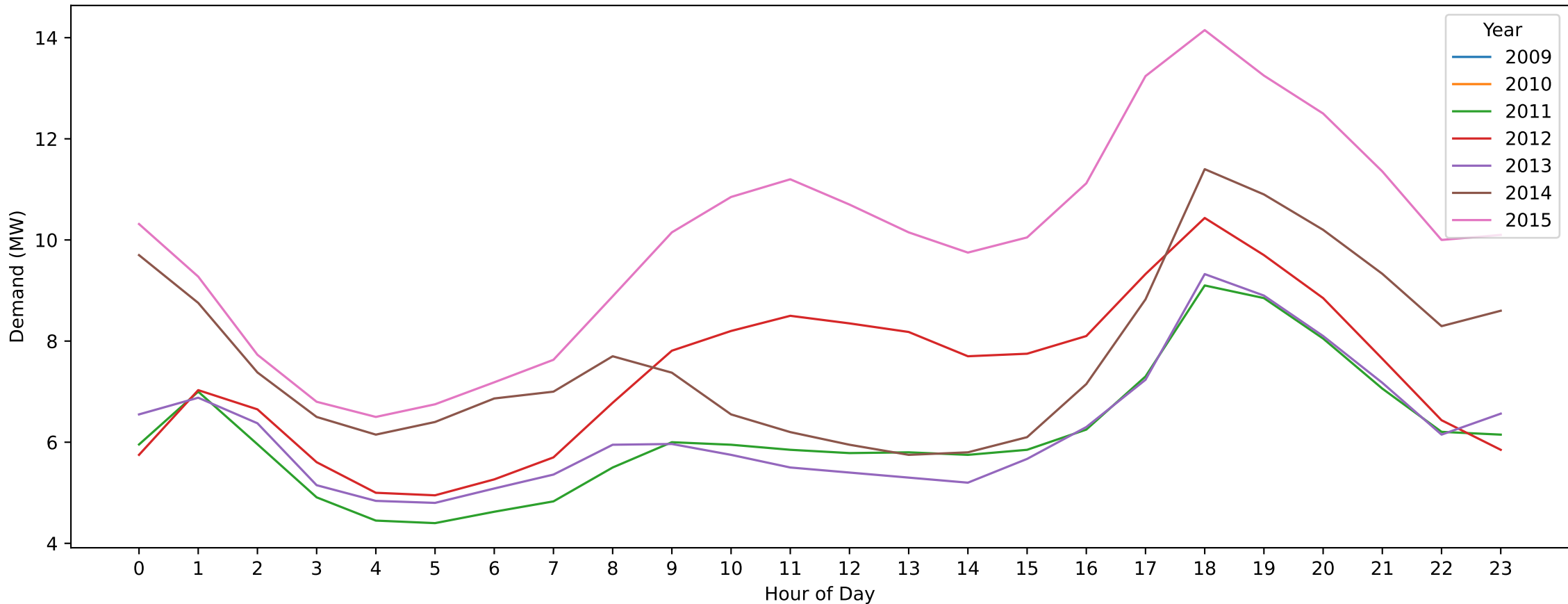
KLO — ANZAC Day (Hourly Demand Across Years)
