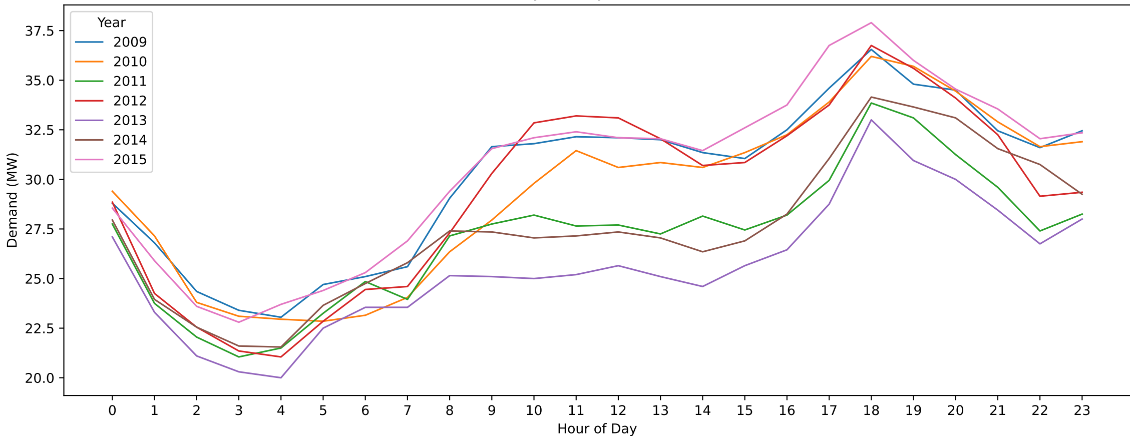
TT — ANZAC Day (Hourly Demand Across Years)
