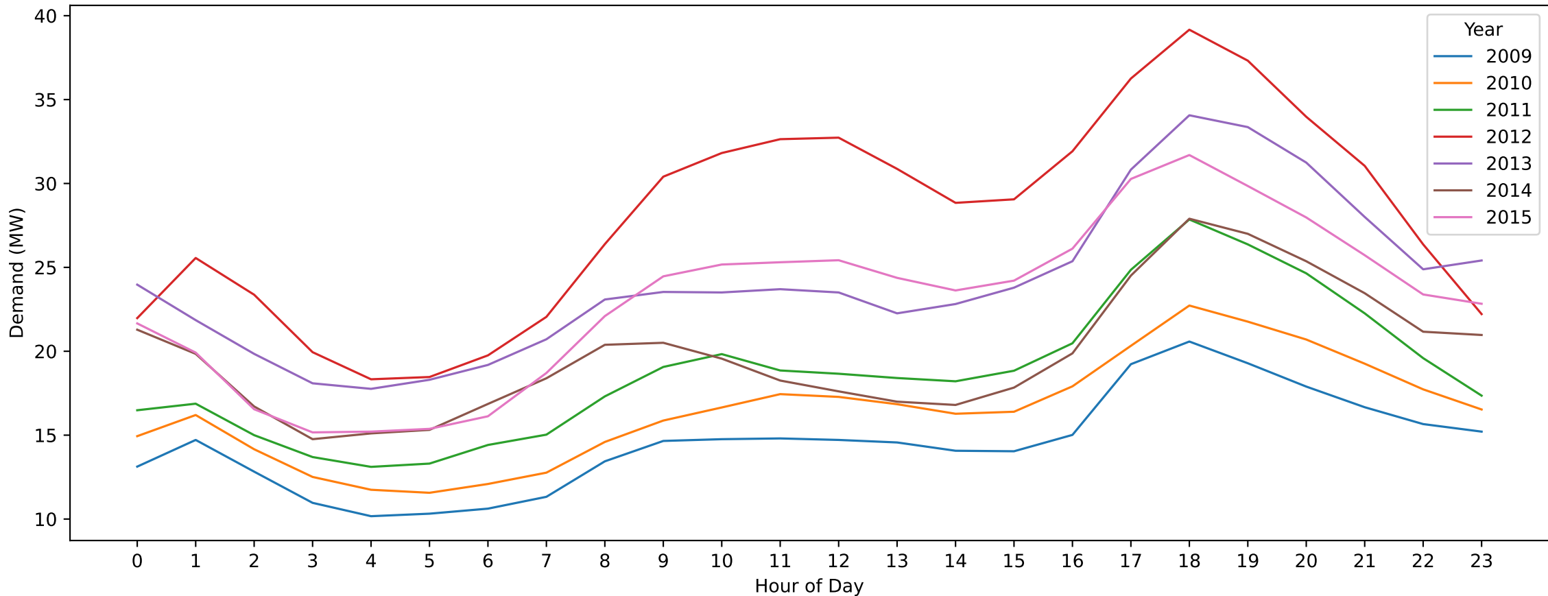
DRN — ANZAC Day (Hourly Demand Across Years)
