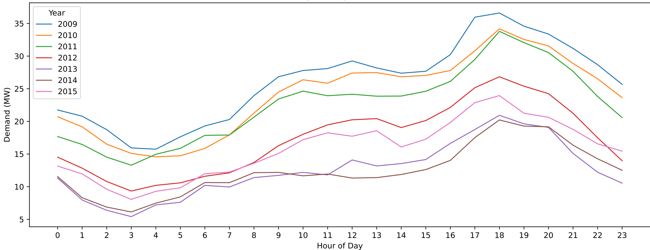
HPK — ANZAC Day (Hourly Demand Across Years)
