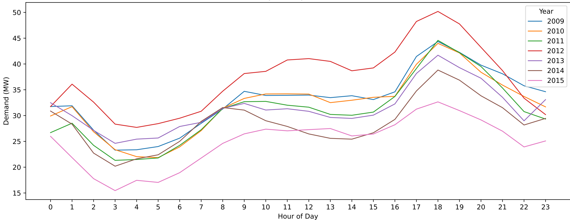
LDL — ANZAC Day (Hourly Demand Across Years)
