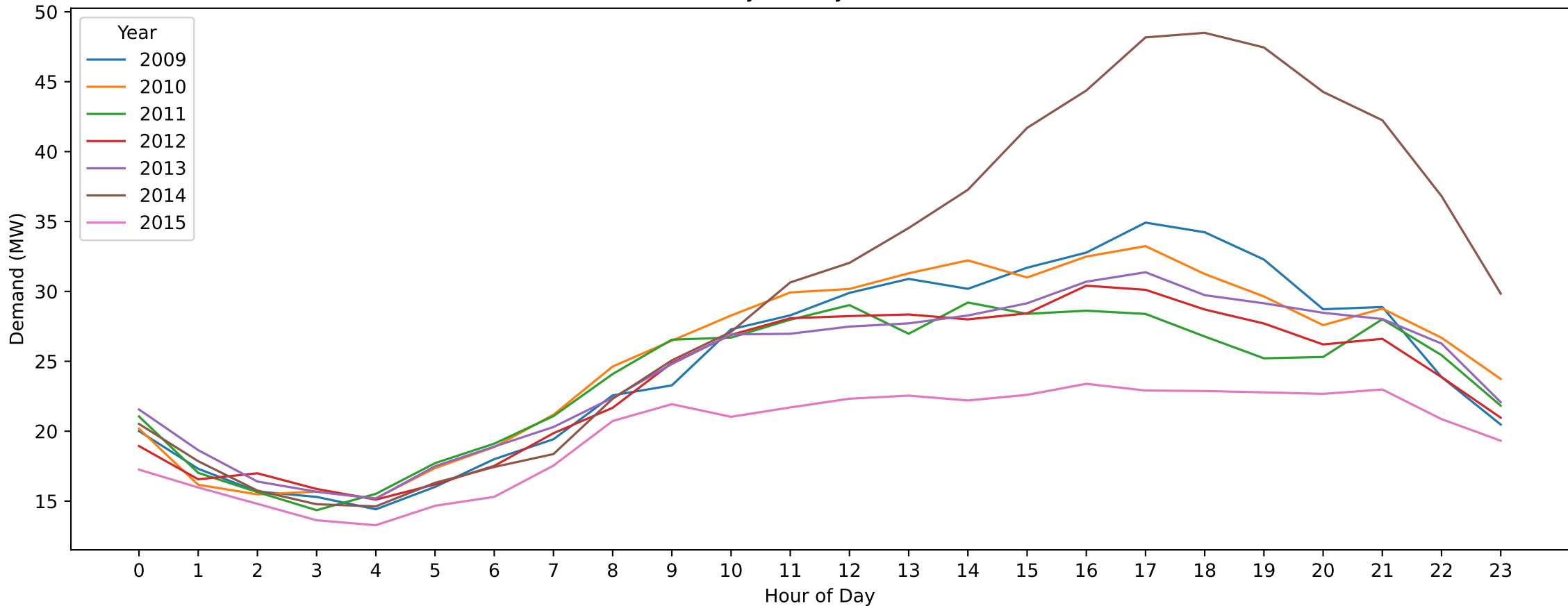
WT — Australia Day (Hourly Demand Across Years)
