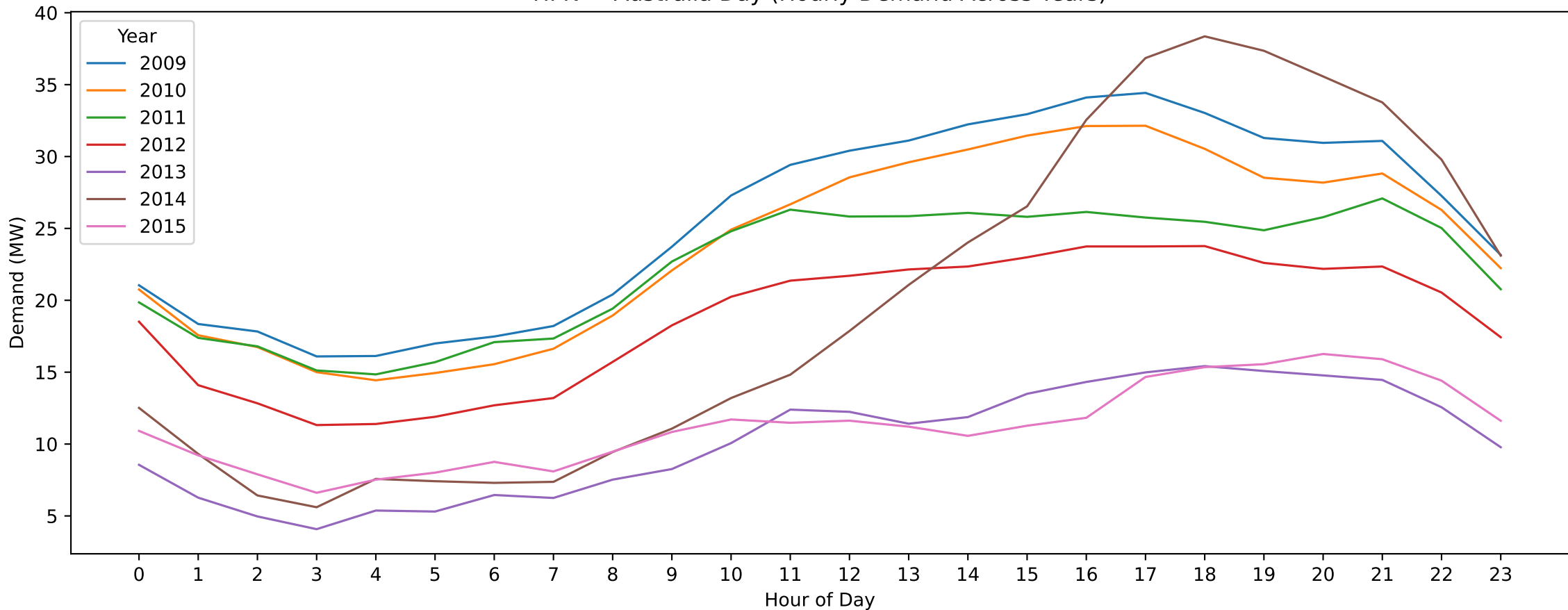
HPK — Australia Day (Hourly Demand Across Years)
