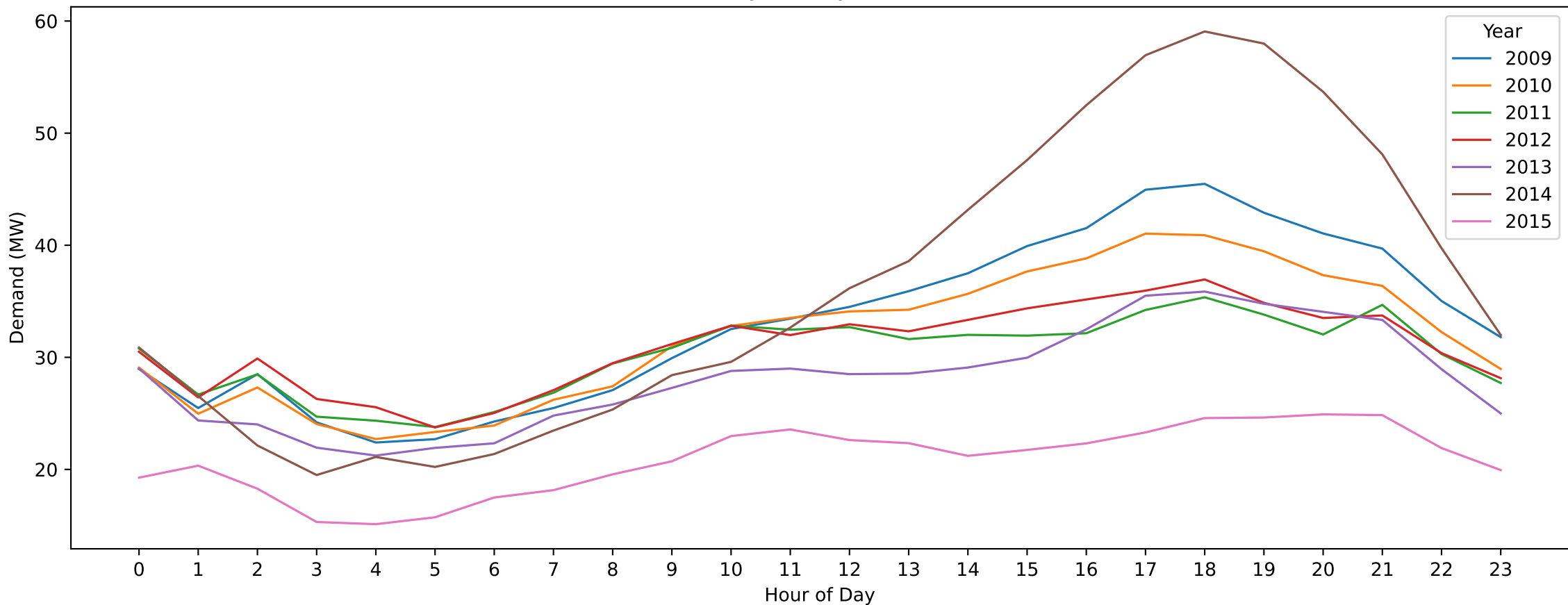
LDL — Australia Day (Hourly Demand Across Years)
