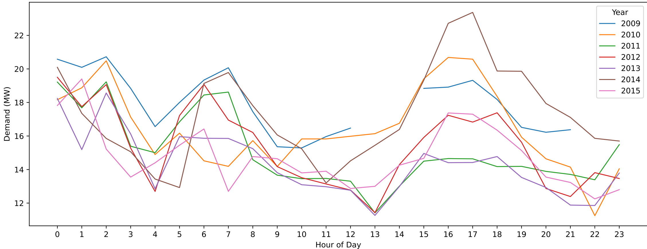
MFA — Australia Day (Hourly Demand Across Years)
