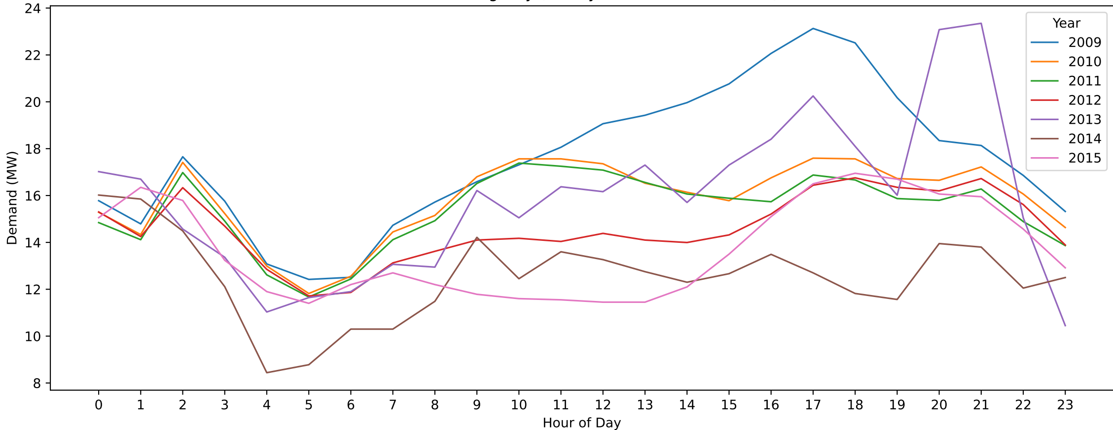
TGN — Boxing Day (Hourly Demand Across Years)
