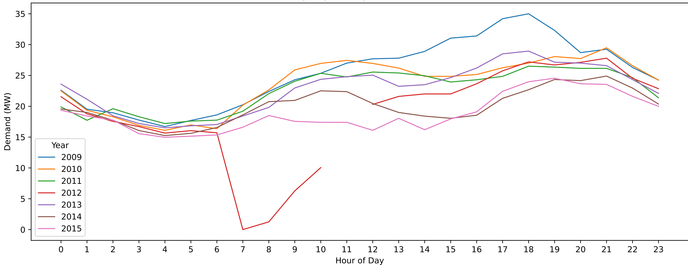
FGY — Boxing Day (Hourly Demand Across Years)
