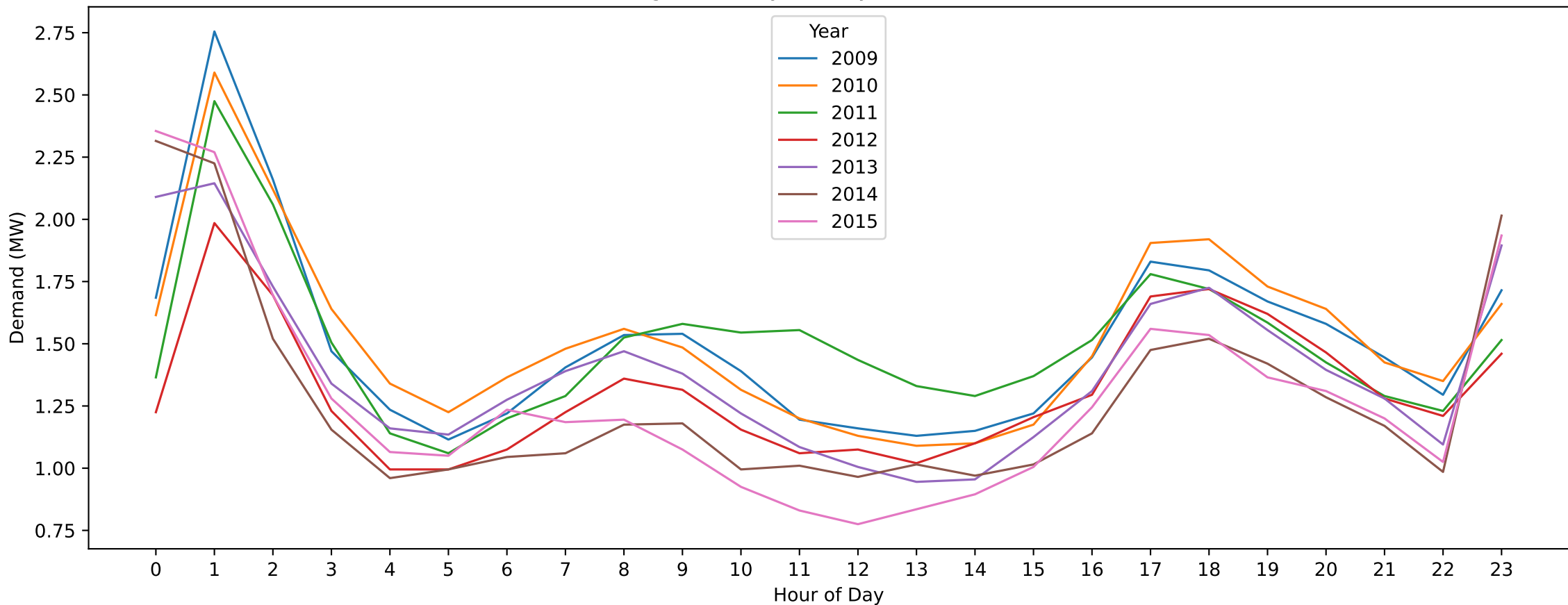
CNR — King's Birthday (Hourly Demand Across Years)
