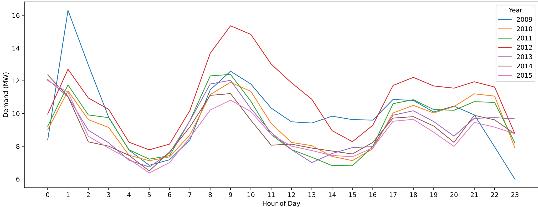
PHI — King's Birthday (Hourly Demand Across Years)
