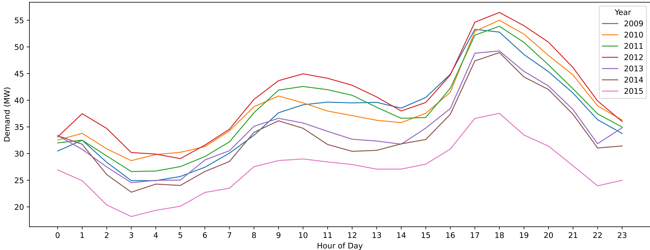
LDL — King's Birthday (Hourly Demand Across Years)
