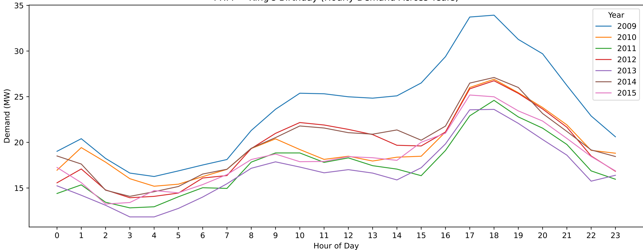
PHM — King's Birthday (Hourly Demand Across Years)
