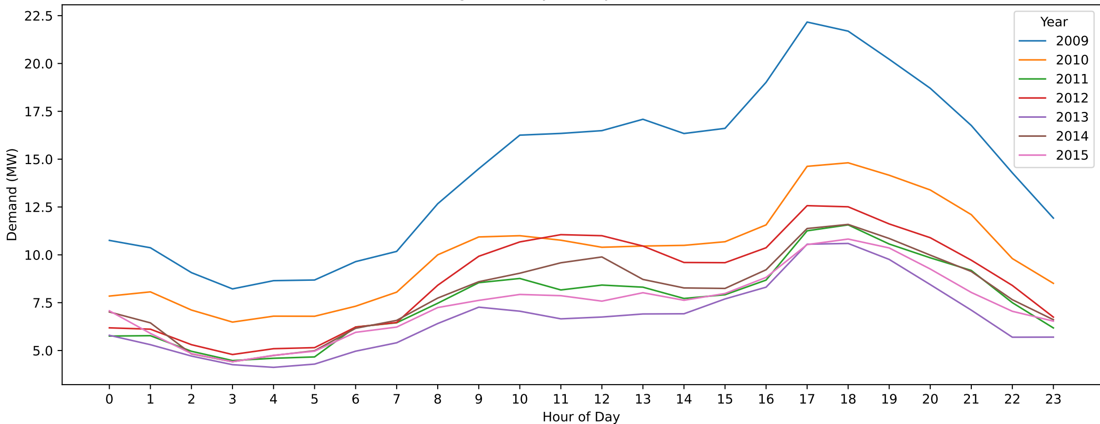
BWN — King's Birthday (Hourly Demand Across Years)
