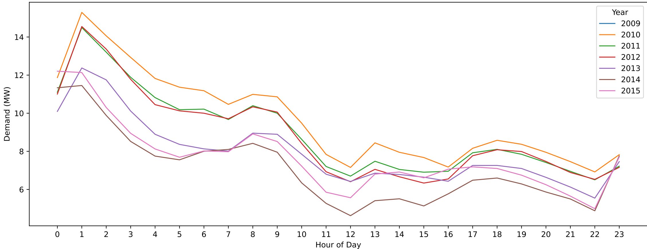
BRT — King's Birthday (Hourly Demand Across Years)
