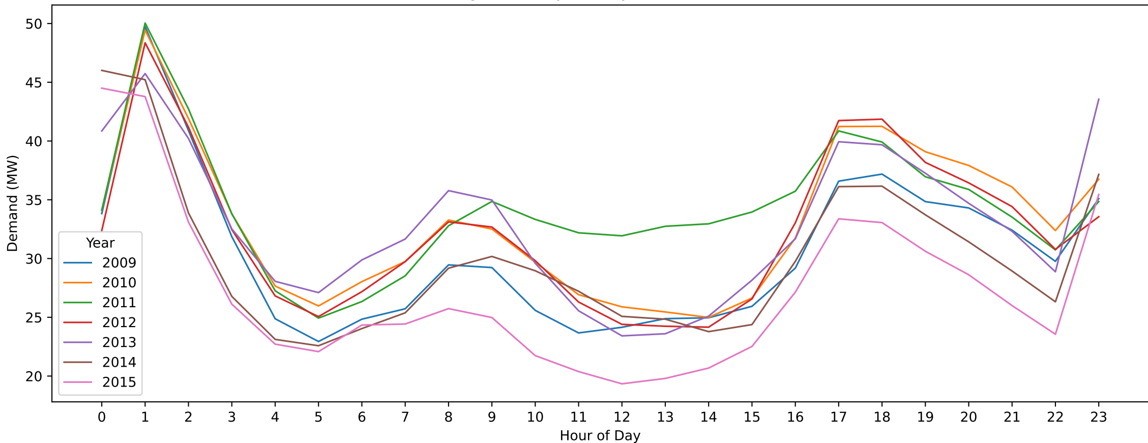
BDL — King's Birthday (Hourly Demand Across Years)
