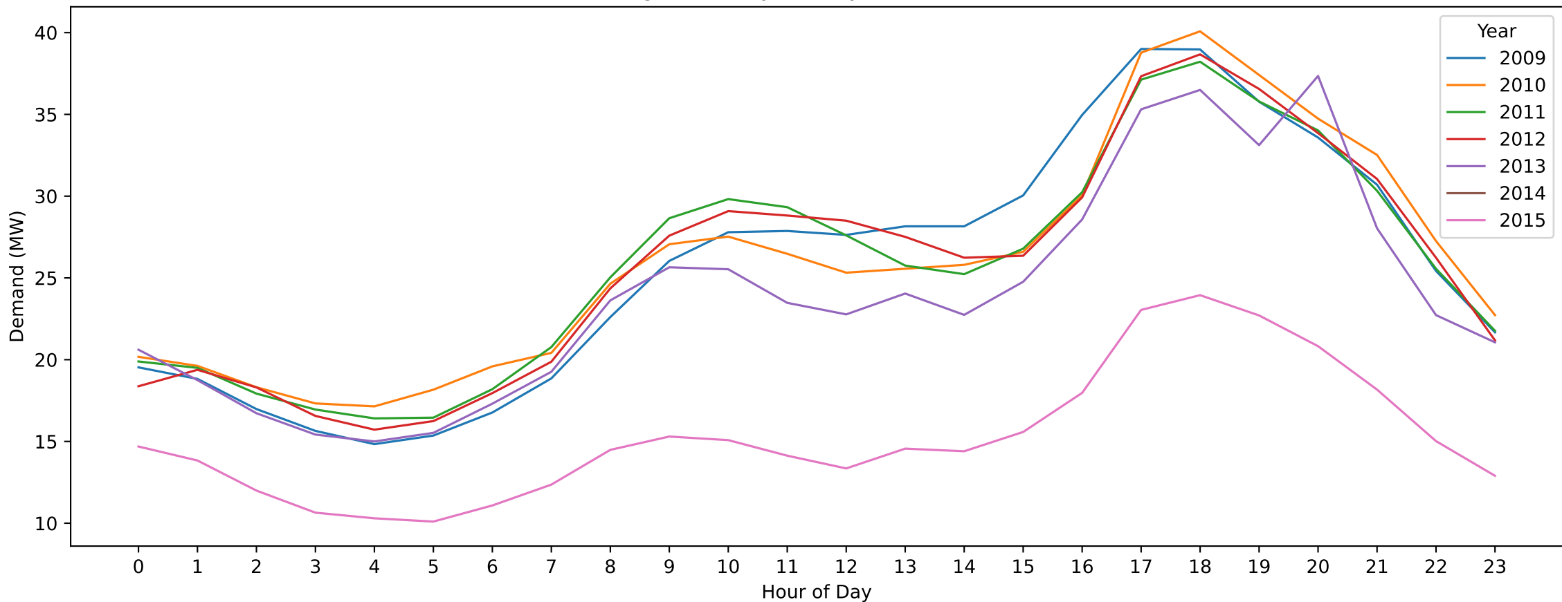
RWN — King's Birthday (Hourly Demand Across Years)
