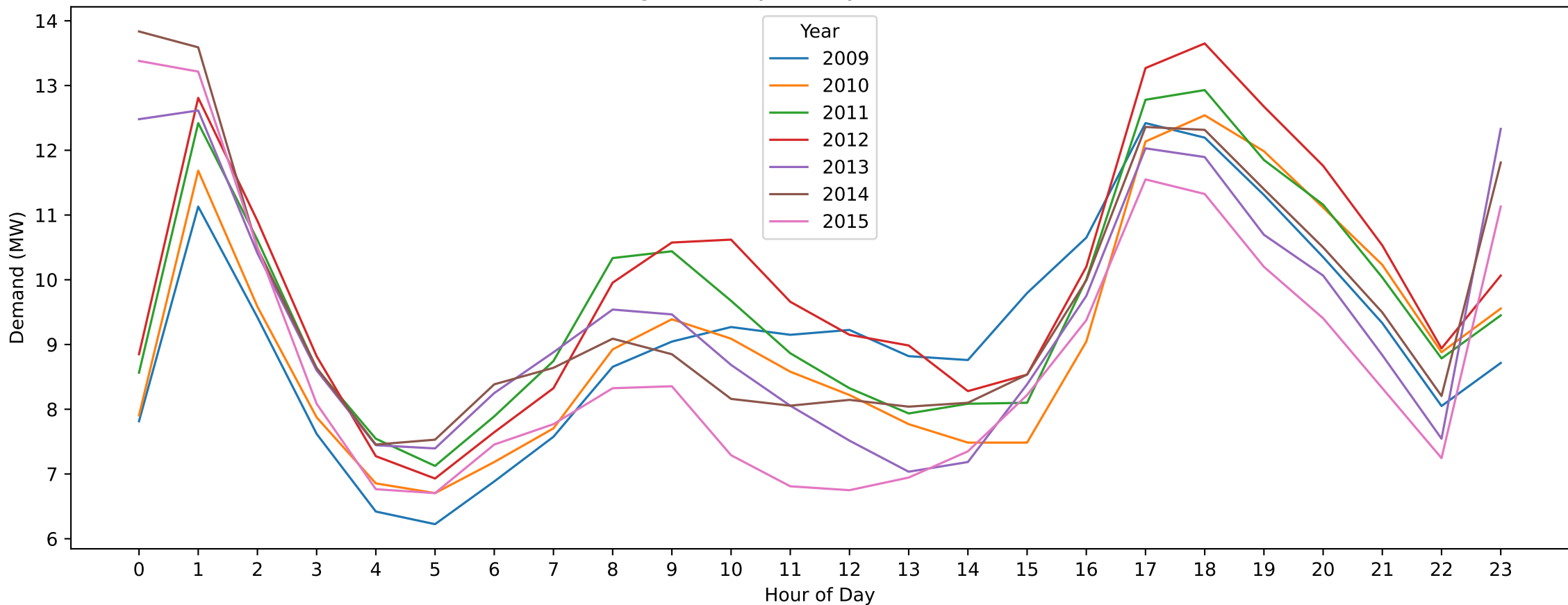
LLG — King's Birthday (Hourly Demand Across Years)
