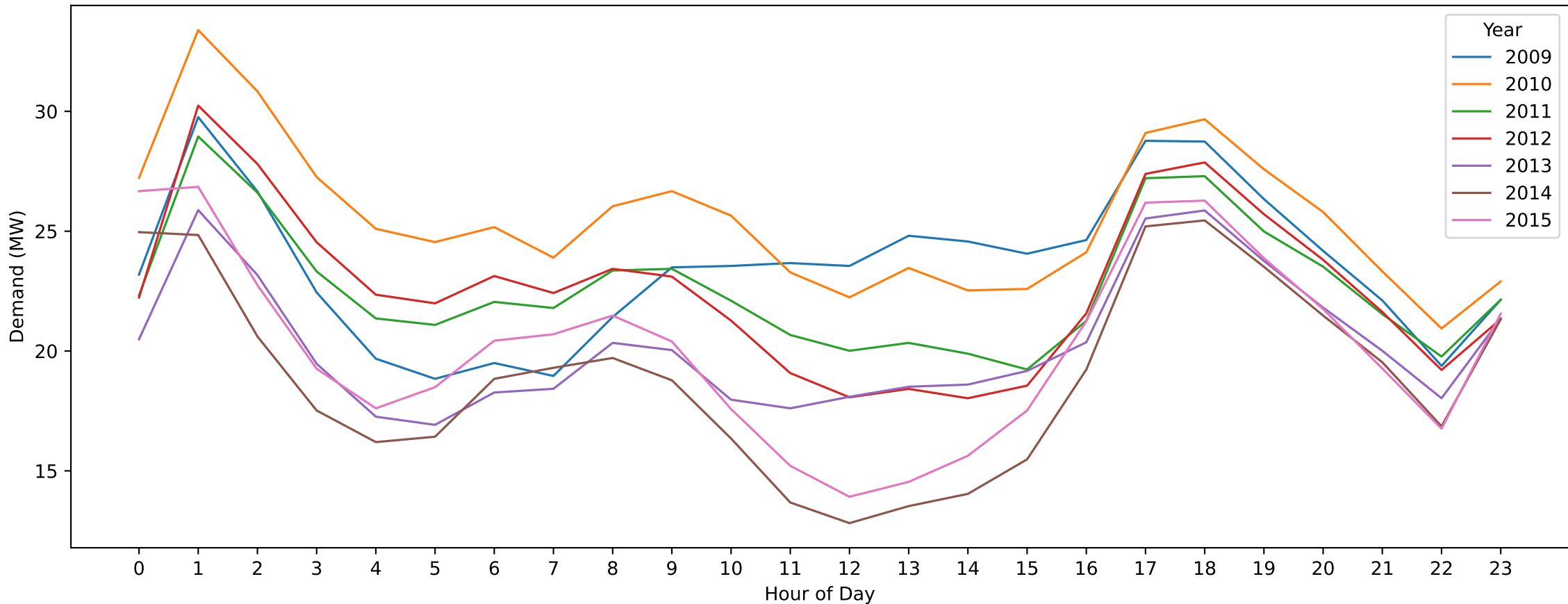
WN — King's Birthday (Hourly Demand Across Years)
