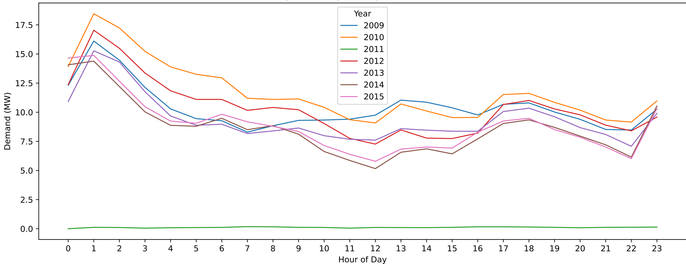
MYT — King's Birthday (Hourly Demand Across Years)
