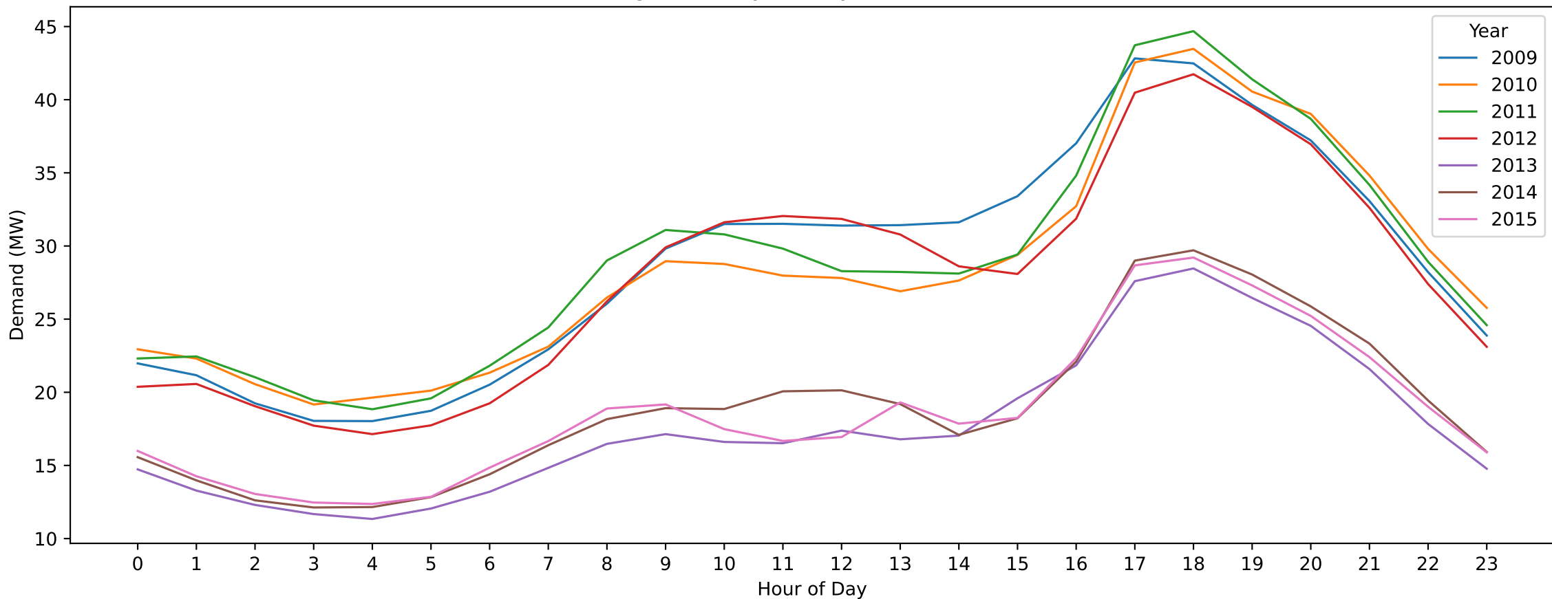
CLN — King's Birthday (Hourly Demand Across Years)
