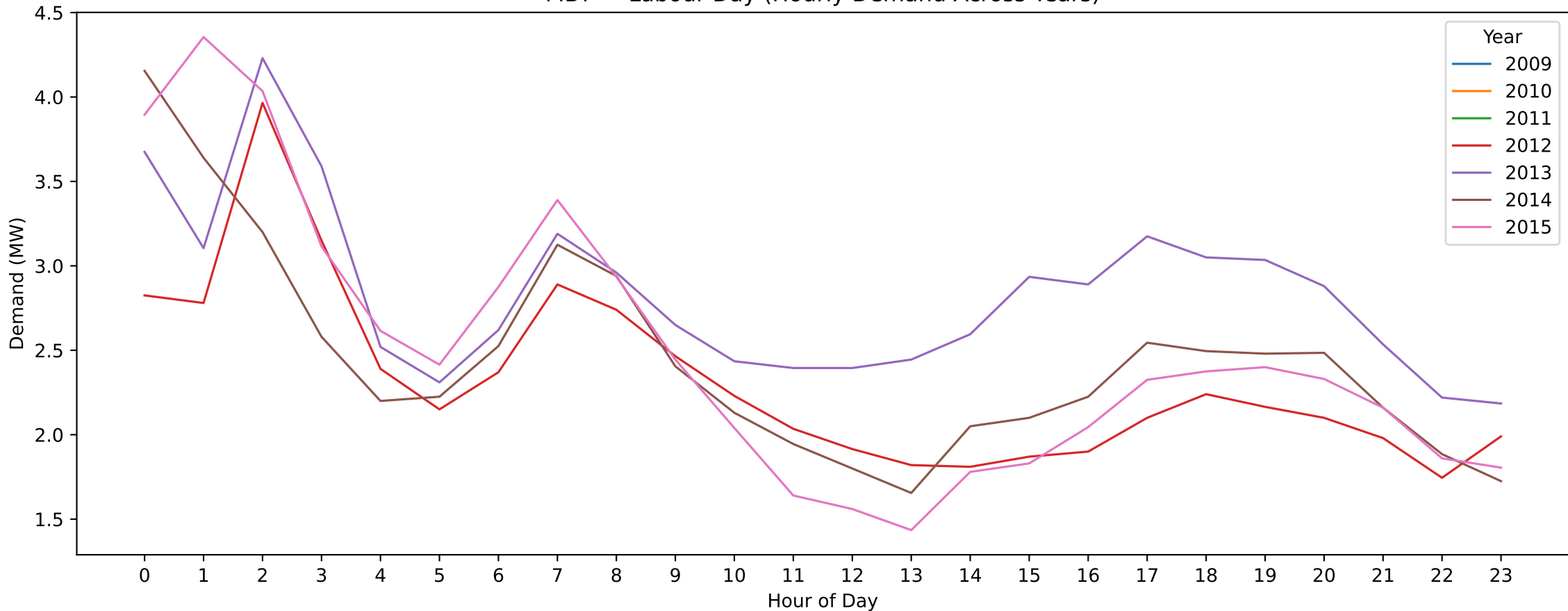
MBY — Labour Day (Hourly Demand Across Years)
