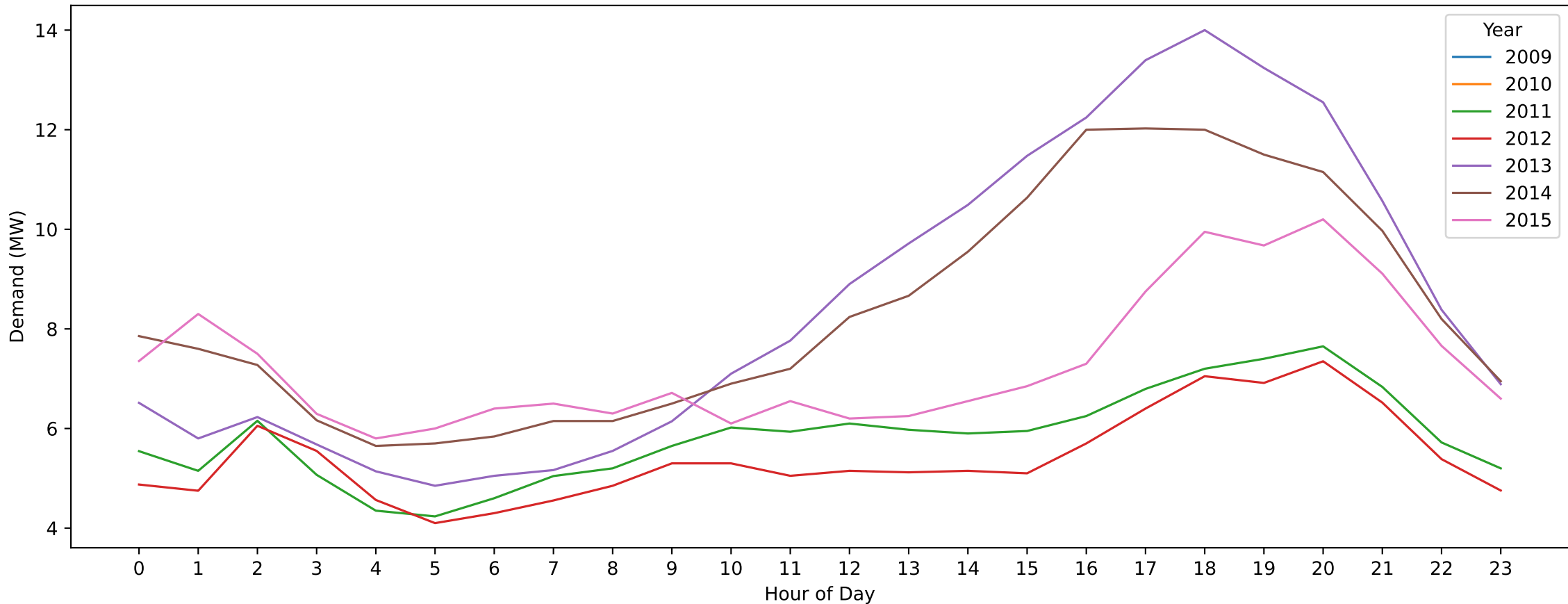
KLO — Labour Day (Hourly Demand Across Years)
