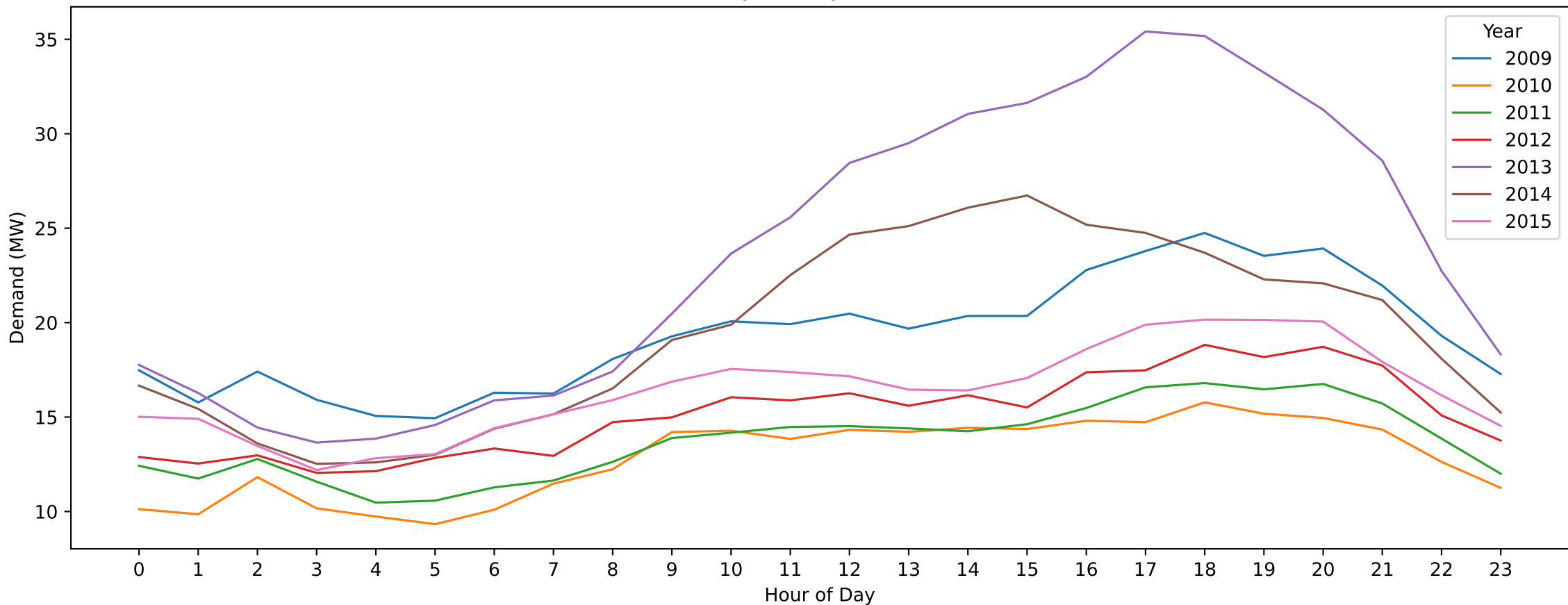
PHM — Labour Day (Hourly Demand Across Years)
