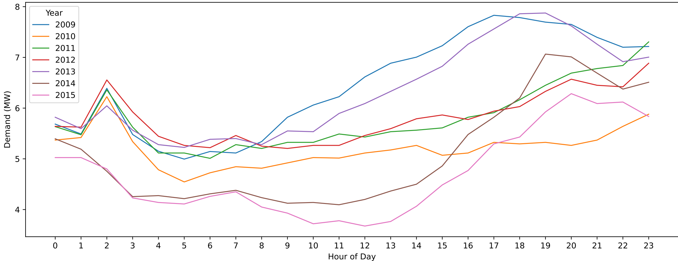
BWA — Labour Day (Hourly Demand Across Years)
