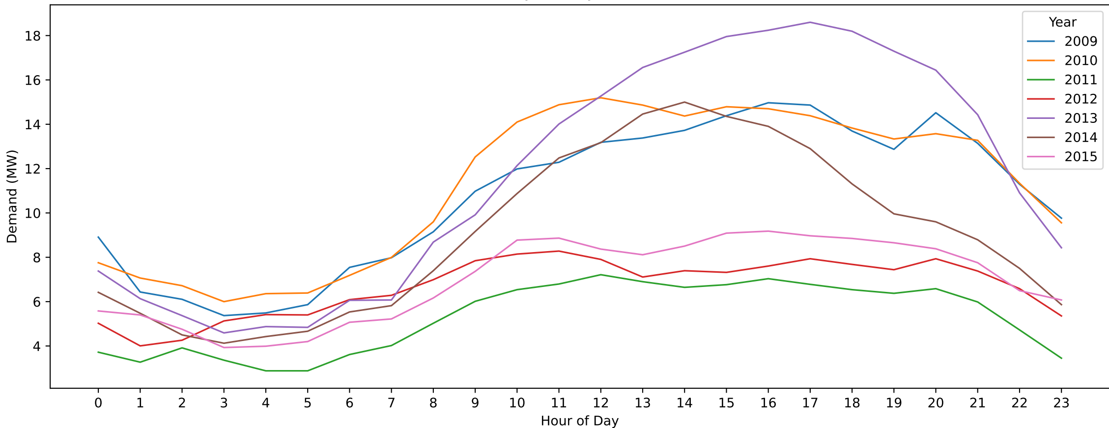
NRN — Labour Day (Hourly Demand Across Years)
