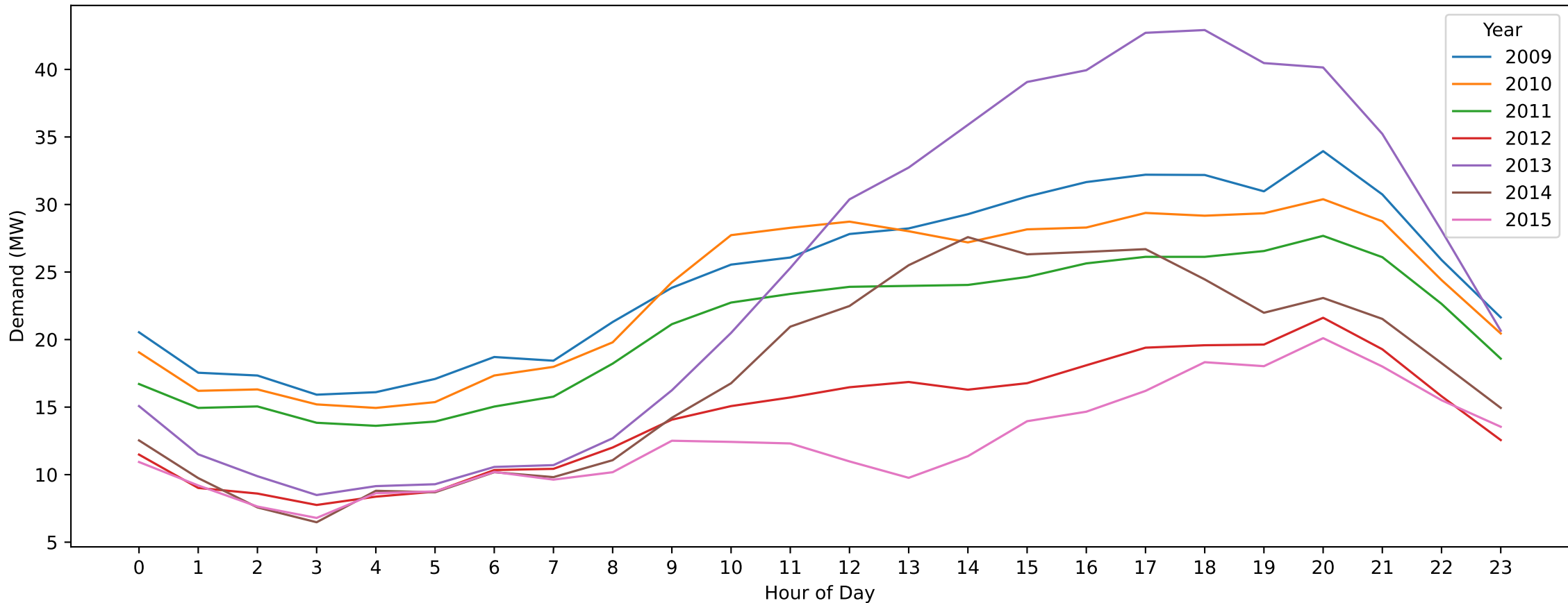
HPK — Labour Day (Hourly Demand Across Years)
