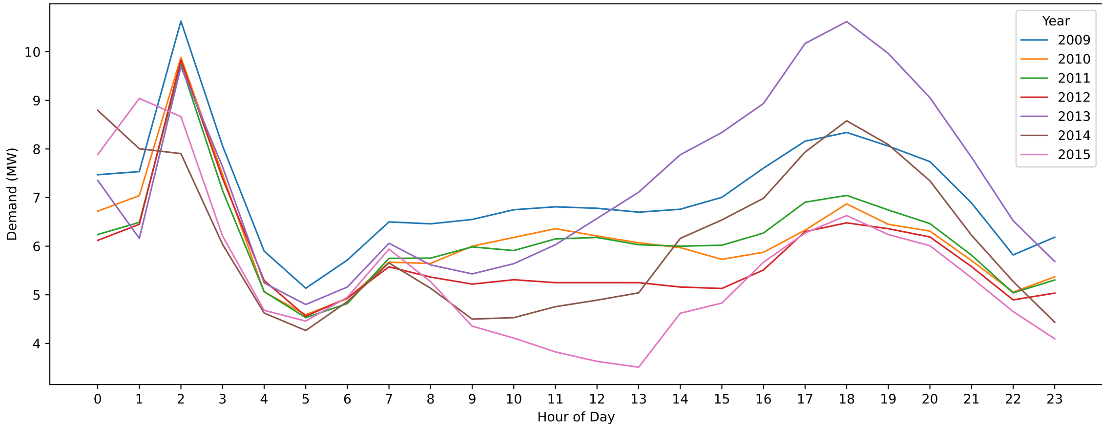
MYT — Labour Day (Hourly Demand Across Years)
