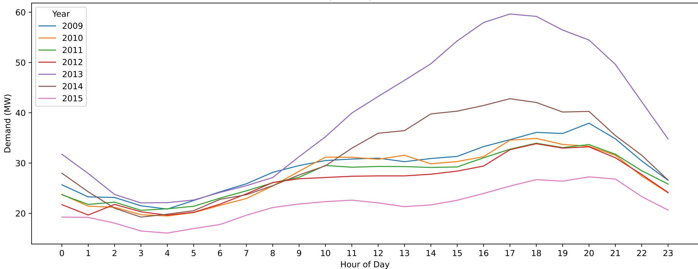
CYN — Labour Day (Hourly Demand Across Years)
