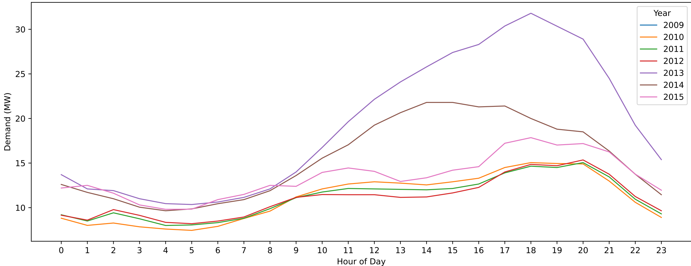
OFR — Labour Day (Hourly Demand Across Years)
