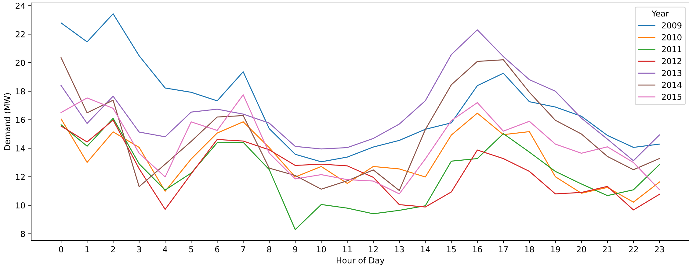
MFA — Labour Day (Hourly Demand Across Years)
