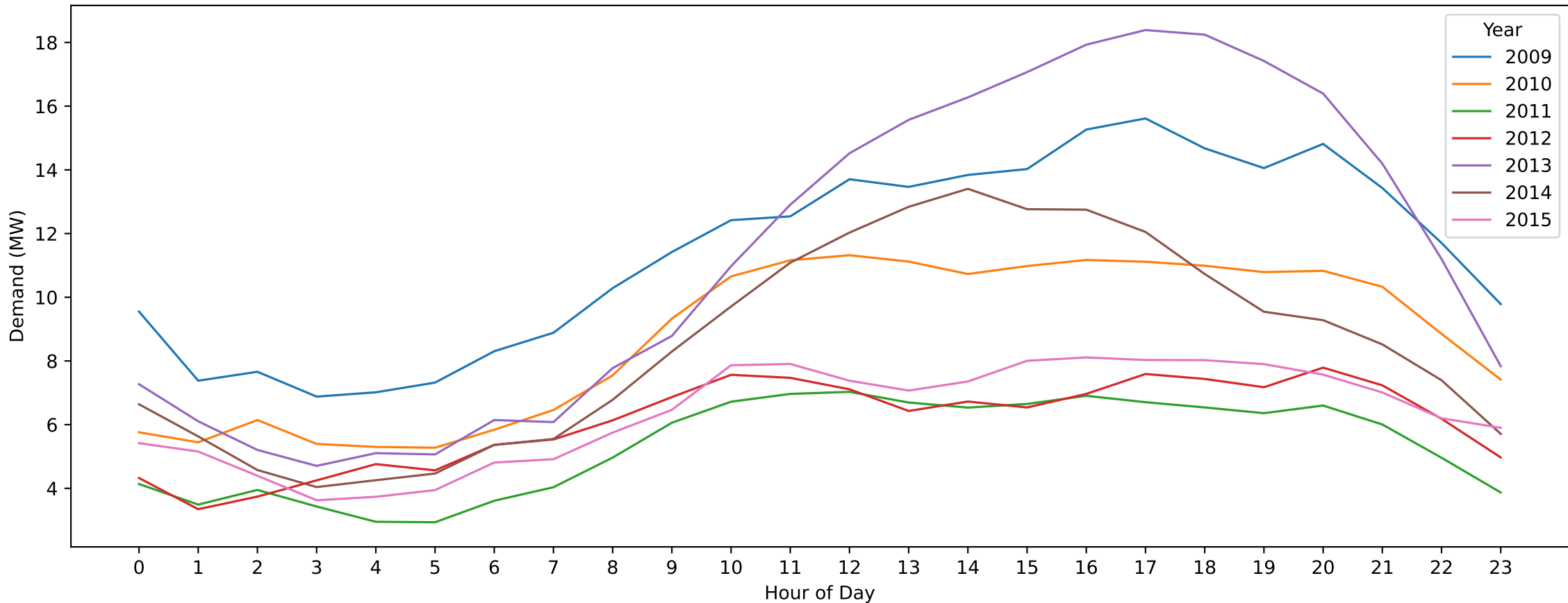
BWN — Labour Day (Hourly Demand Across Years)
