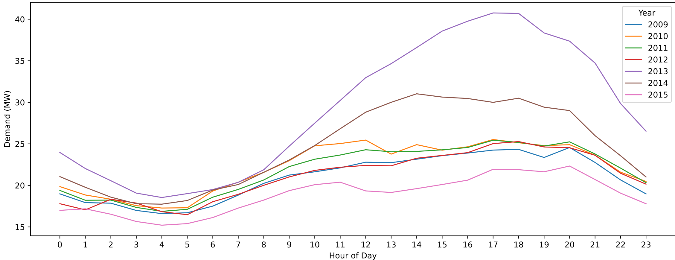
BWR — Labour Day (Hourly Demand Across Years)
