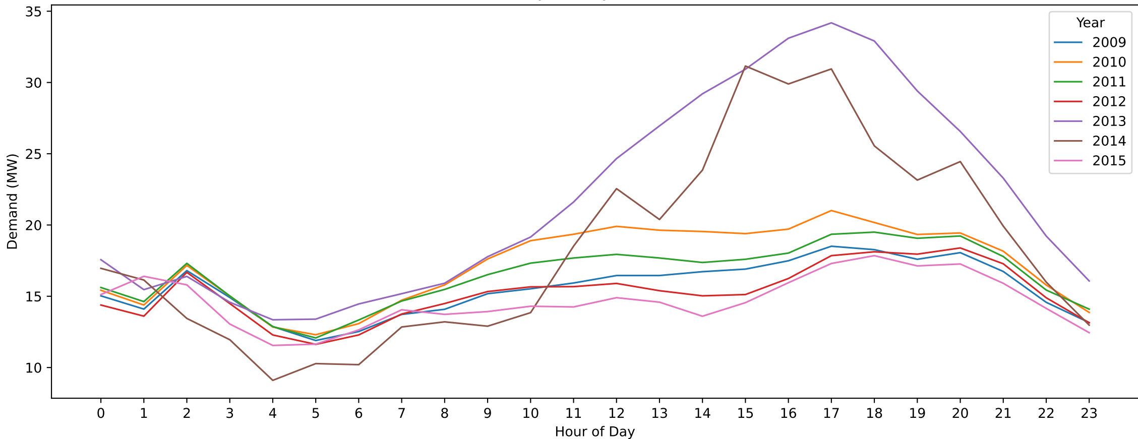
TGN — Labour Day (Hourly Demand Across Years)
