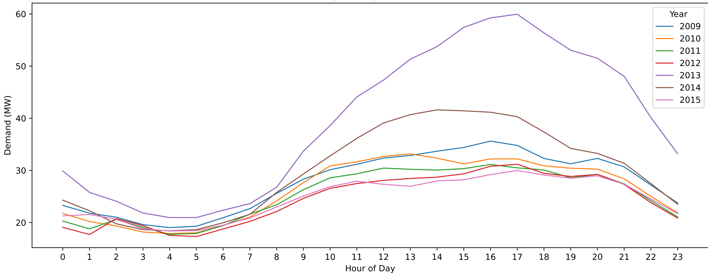
BRA — Labour Day (Hourly Demand Across Years)
