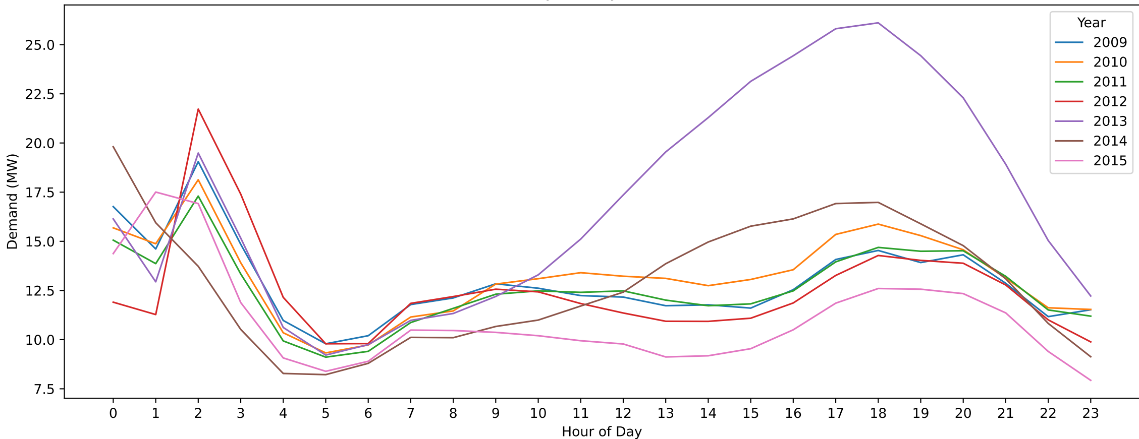
WYK — Labour Day (Hourly Demand Across Years)
