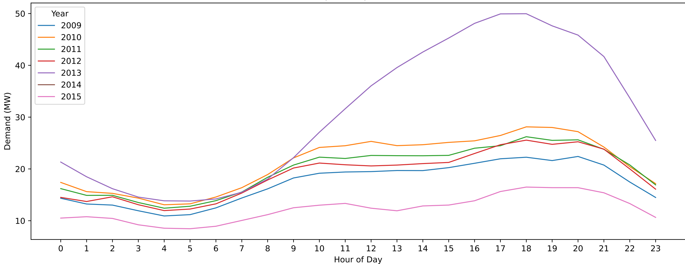
RWN — Labour Day (Hourly Demand Across Years)
