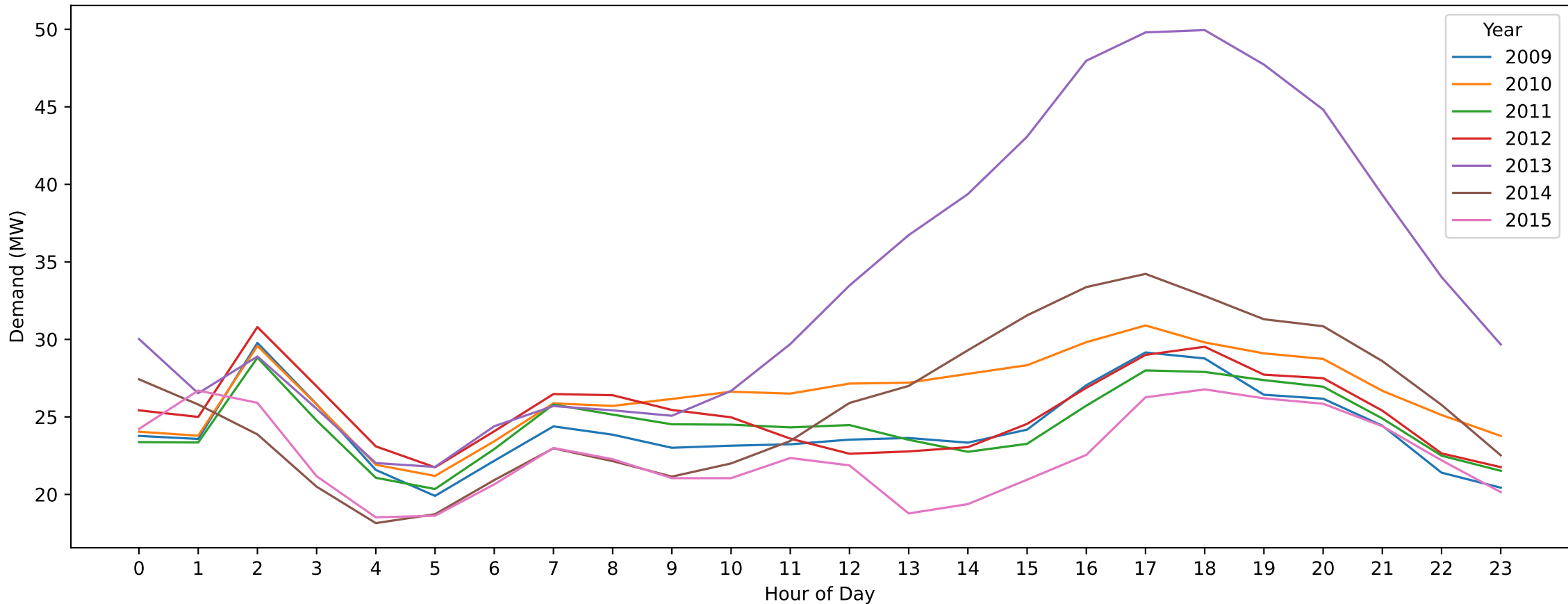
WGL — Labour Day (Hourly Demand Across Years)
