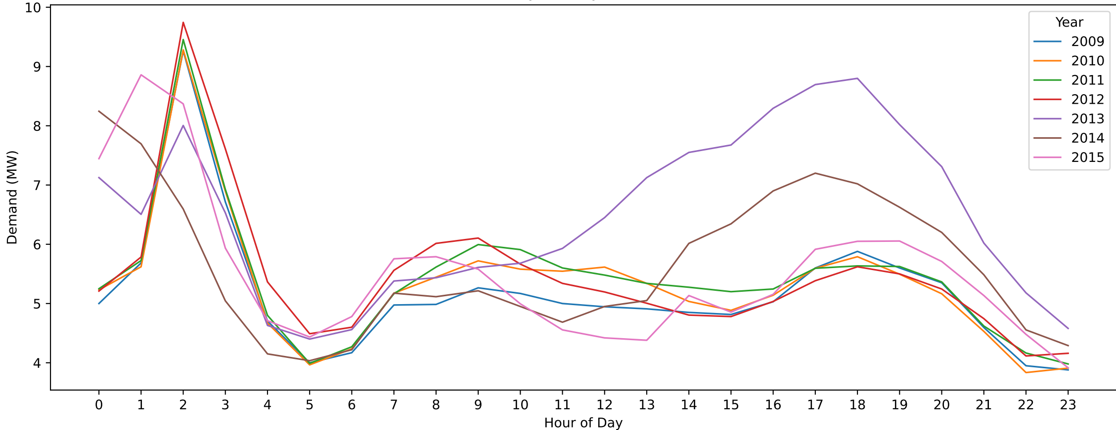
MSD — Labour Day (Hourly Demand Across Years)
