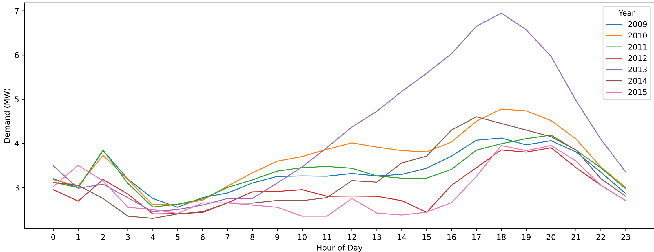
KMS — Labour Day (Hourly Demand Across Years)
