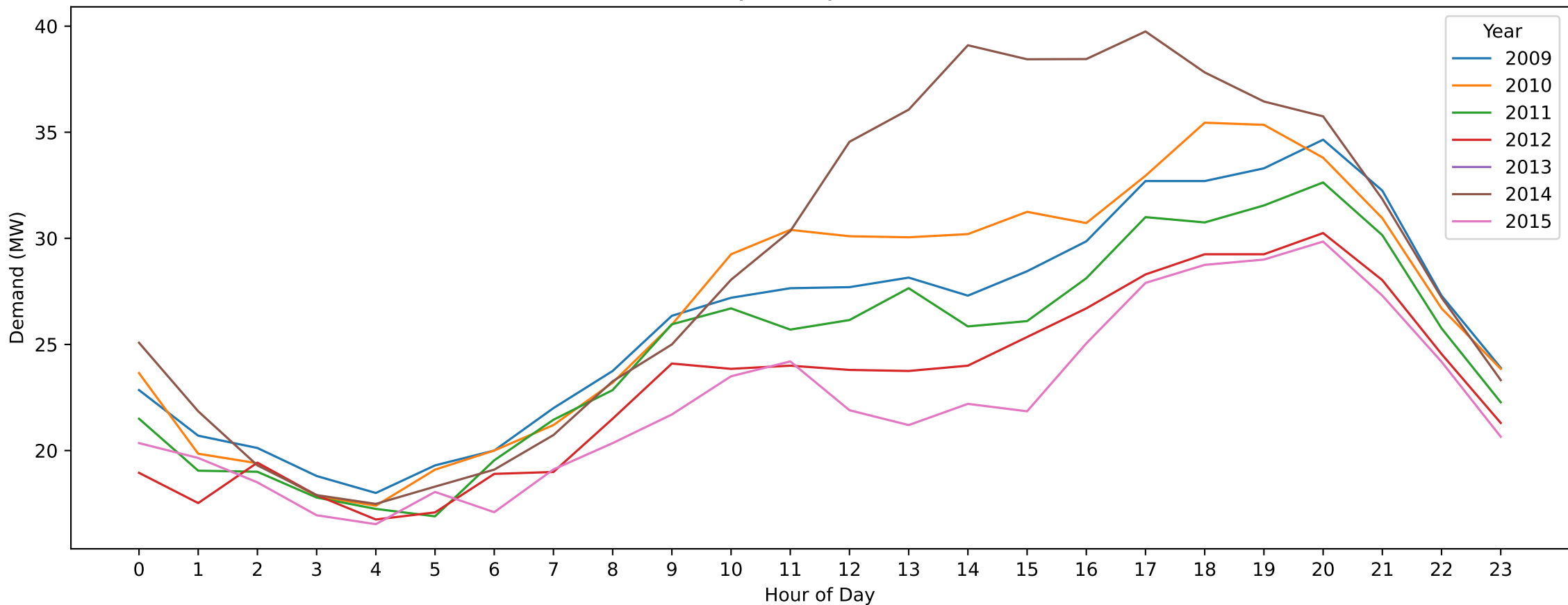
FGY — Labour Day (Hourly Demand Across Years)
