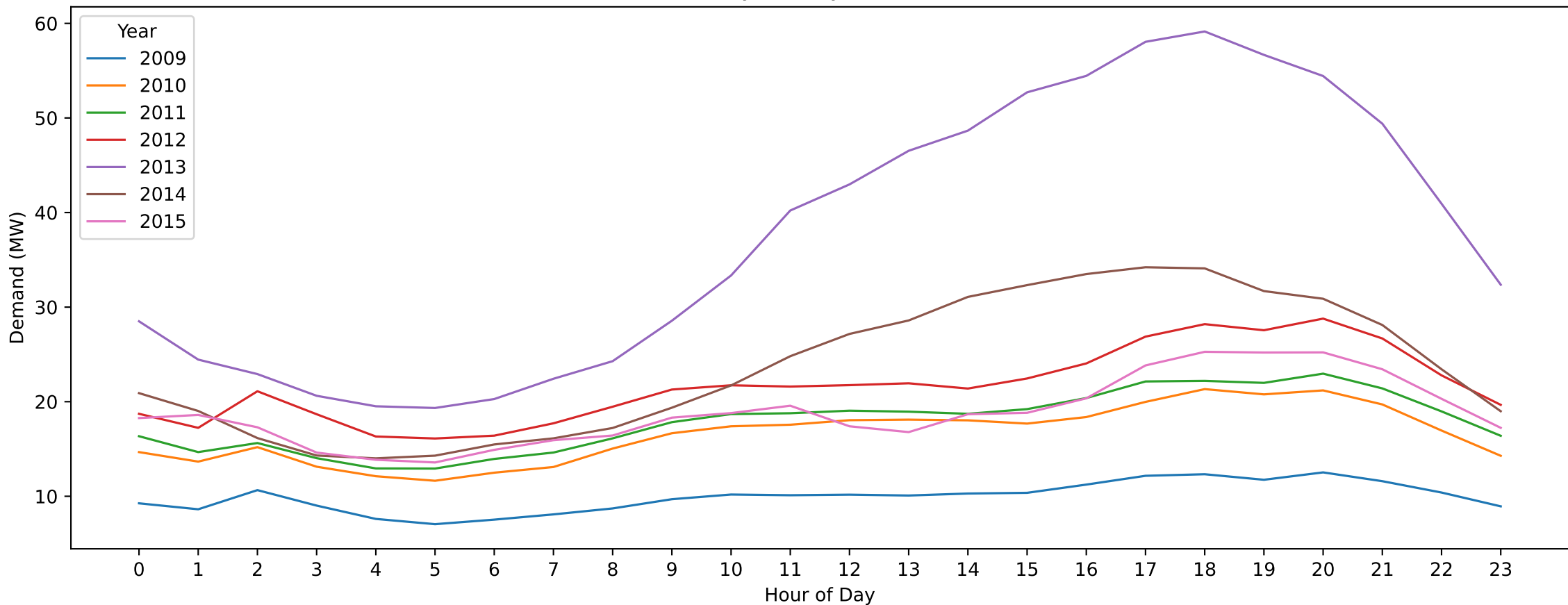
DRN — Labour Day (Hourly Demand Across Years)
