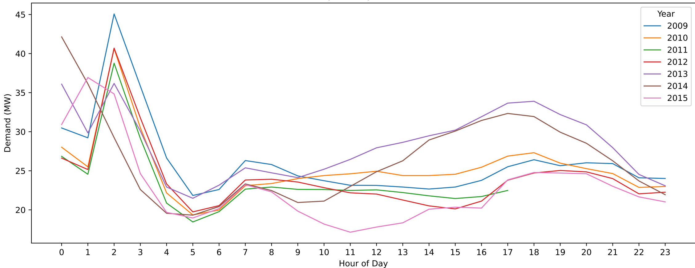
BDL — Labour Day (Hourly Demand Across Years)
