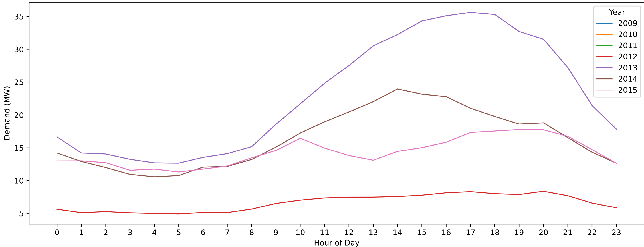
CRE — Labour Day (Hourly Demand Across Years)
