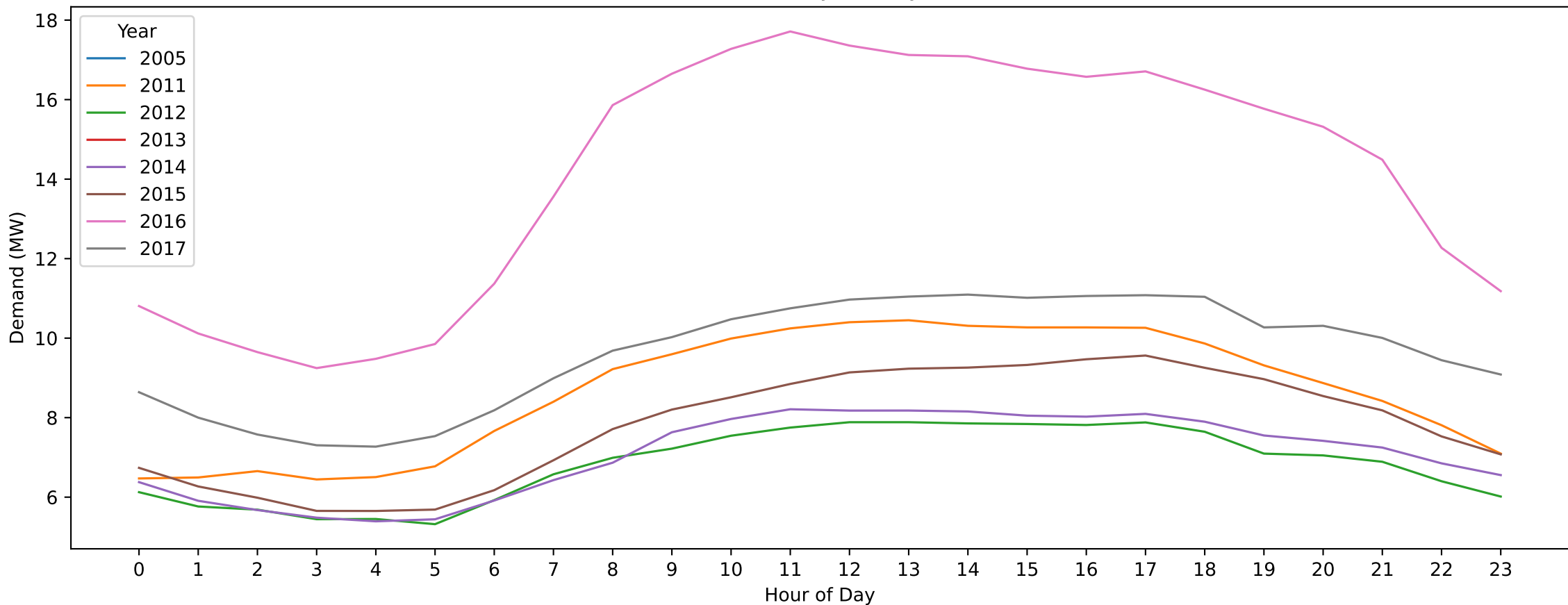
Heffernan Lane — Christmas Day (Hourly Demand Across Years)
