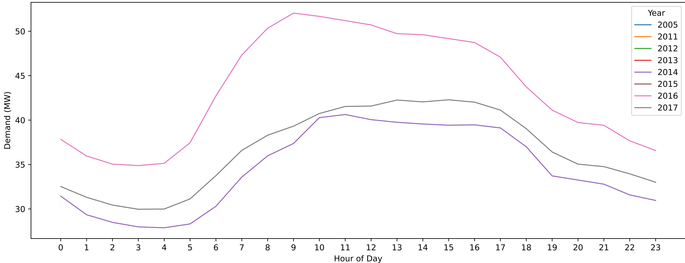
McIlwraith PI — Christmas Day (Hourly Demand Across Years)
