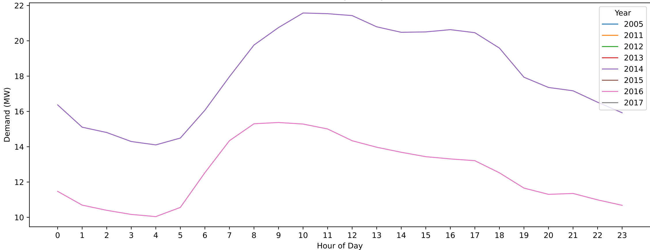
South Melbourne — Christmas Day (Hourly Demand Across Years)
