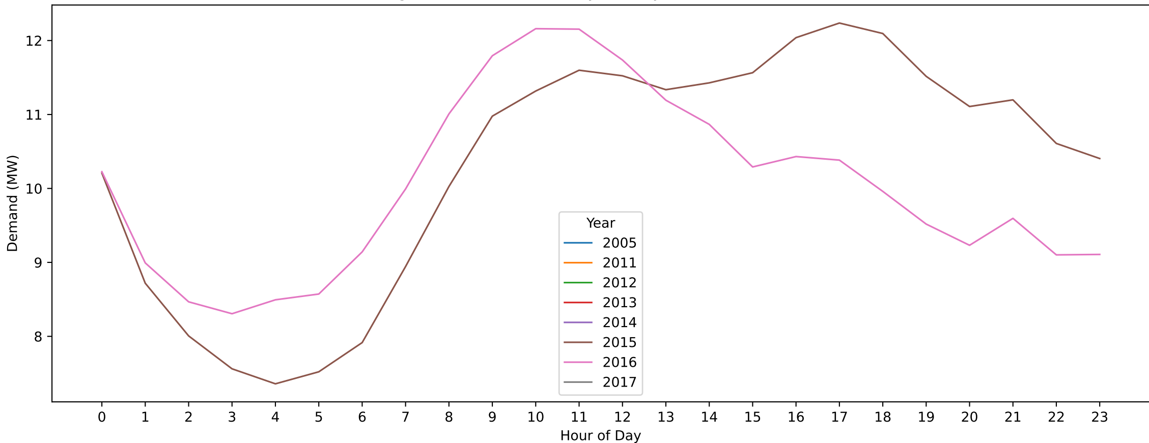
Collingwood — Christmas Day (Hourly Demand Across Years)
