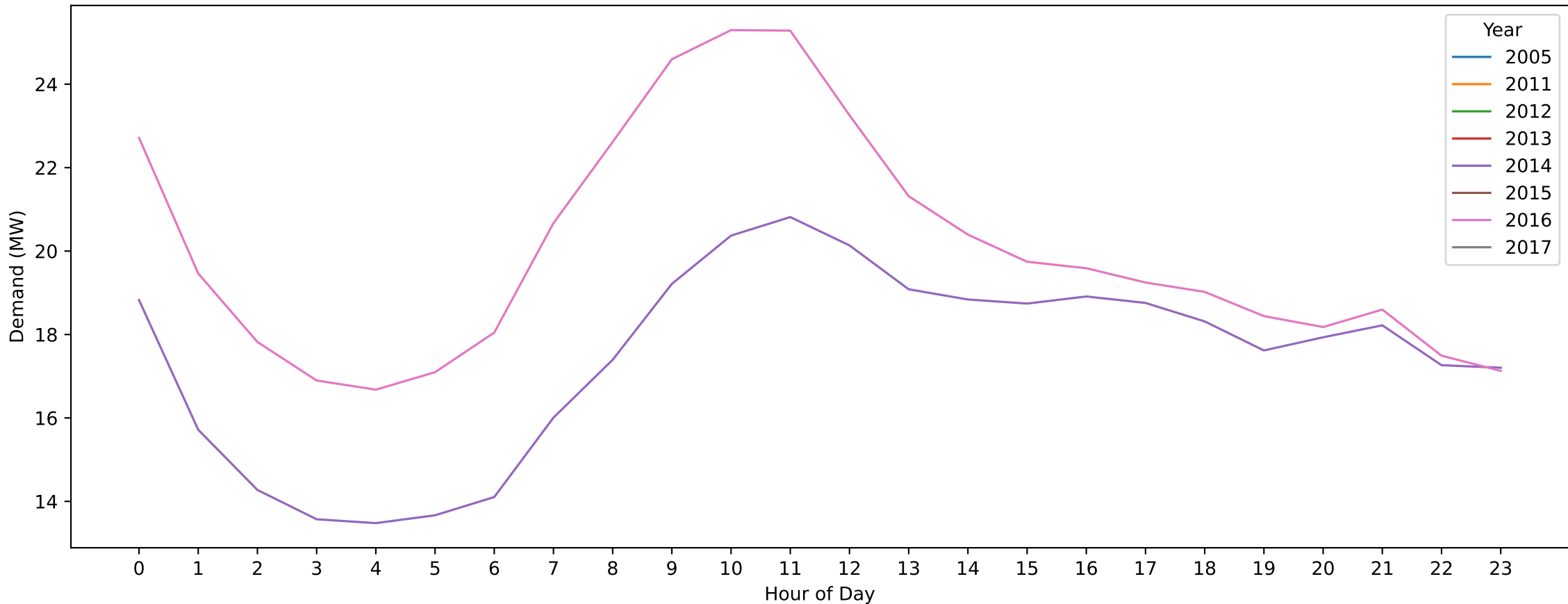
Toorak — Christmas Day (Hourly Demand Across Years)
