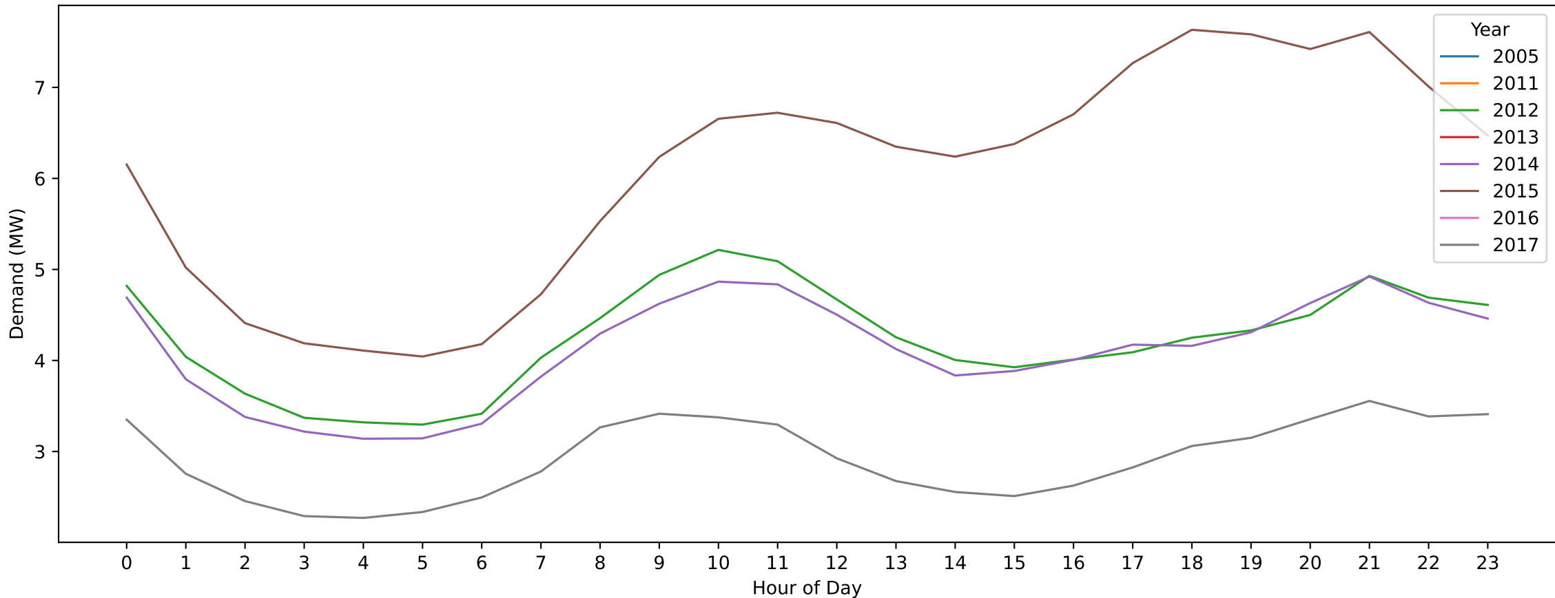
Fitzroy — Christmas Day (Hourly Demand Across Years)
