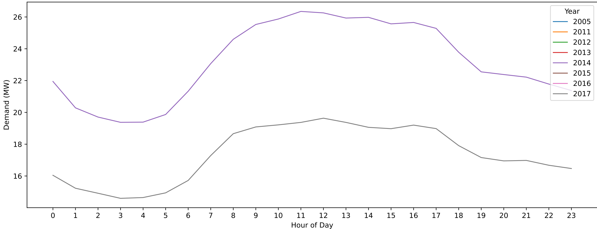
Flinders/Ramsden — Christmas Day (Hourly Demand Across Years)
