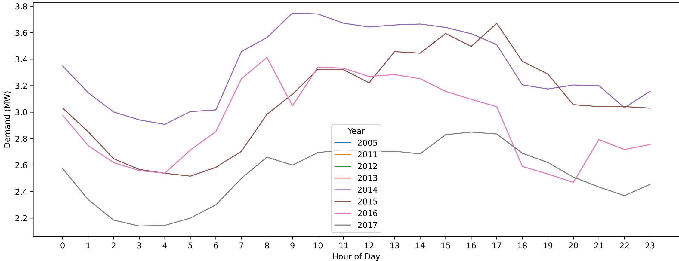
Spencer St — Christmas Day (Hourly Demand Across Years)
