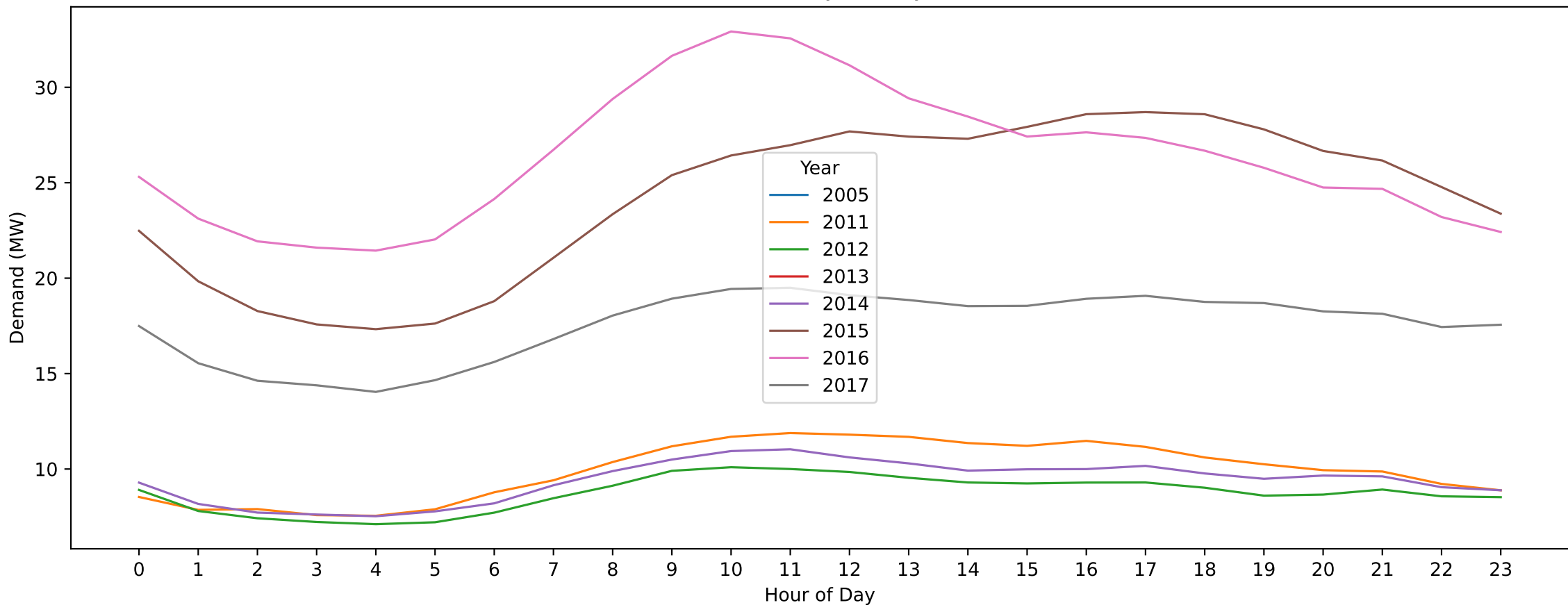
North Richmond — Christmas Day (Hourly Demand Across Years)
