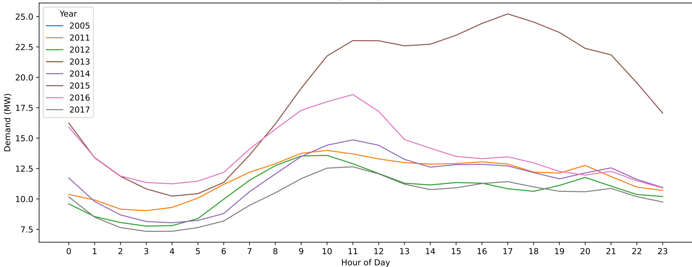
Kew — Christmas Day (Hourly Demand Across Years)
