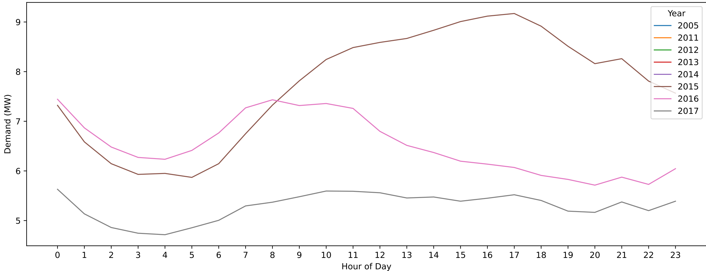
Port Melbourne — Christmas Day (Hourly Demand Across Years)
