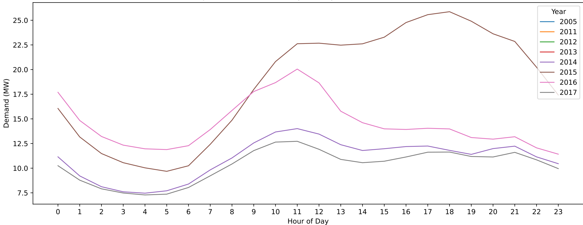
Deepdene — Christmas Day (Hourly Demand Across Years)
