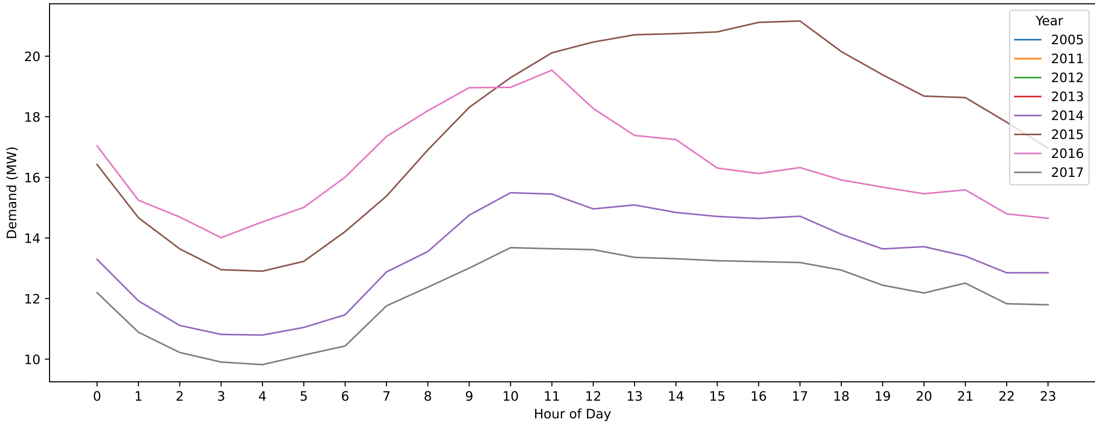
Montagne — Christmas Day (Hourly Demand Across Years)
