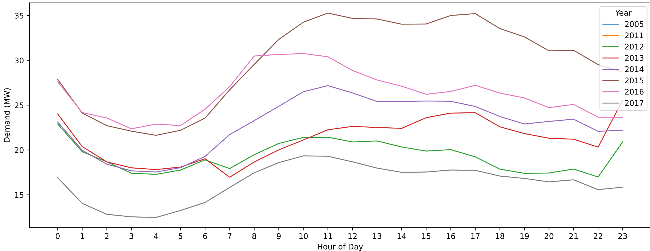
Albert Park — Christmas Day (Hourly Demand Across Years)
