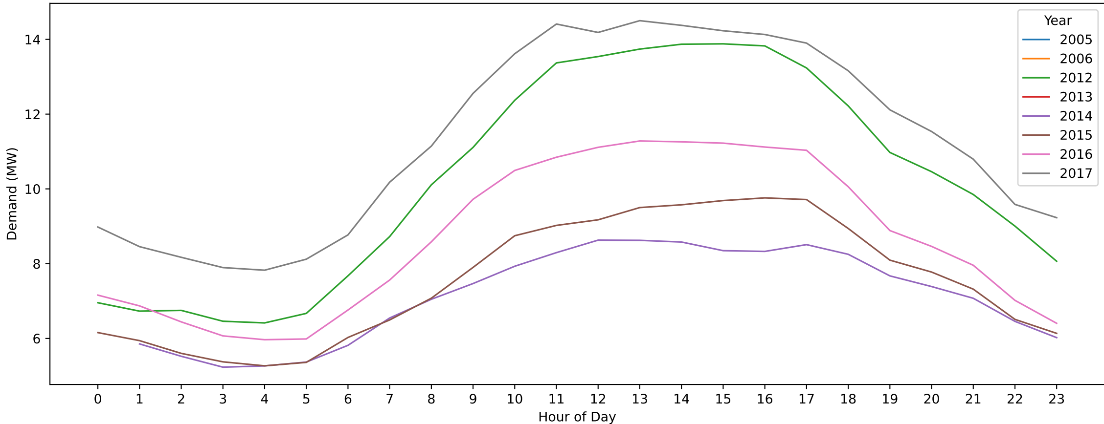
Heffernan Lane — New Year's Day (Hourly Demand Across Years)
