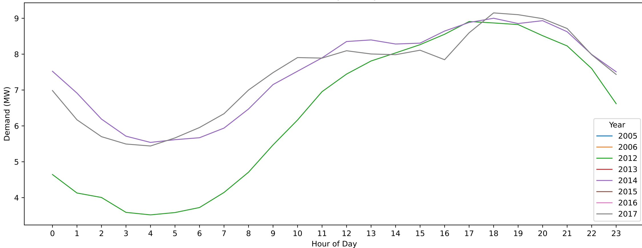
West Brunswick — New Year's Day (Hourly Demand Across Years)
