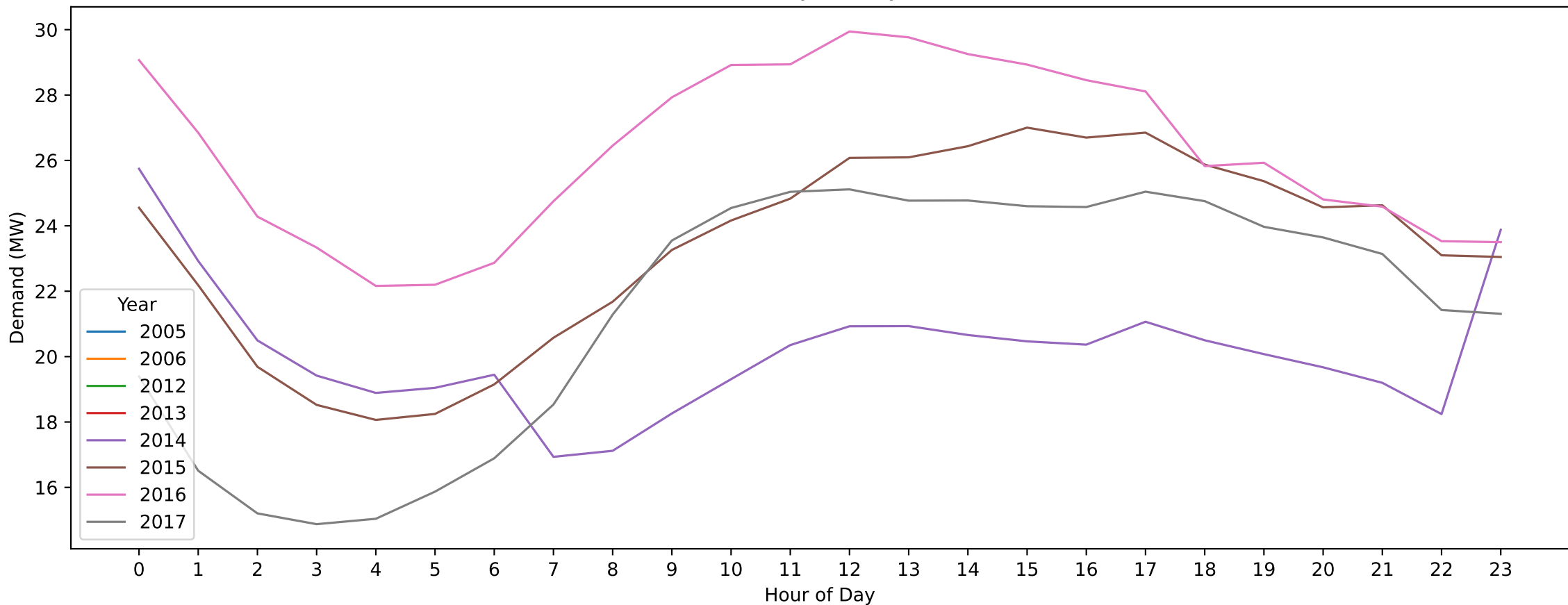
Albert Park — New Year's Day (Hourly Demand Across Years)
