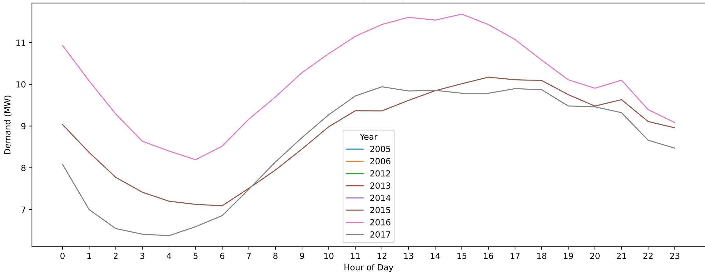
Collingwood — New Year's Day (Hourly Demand Across Years)
