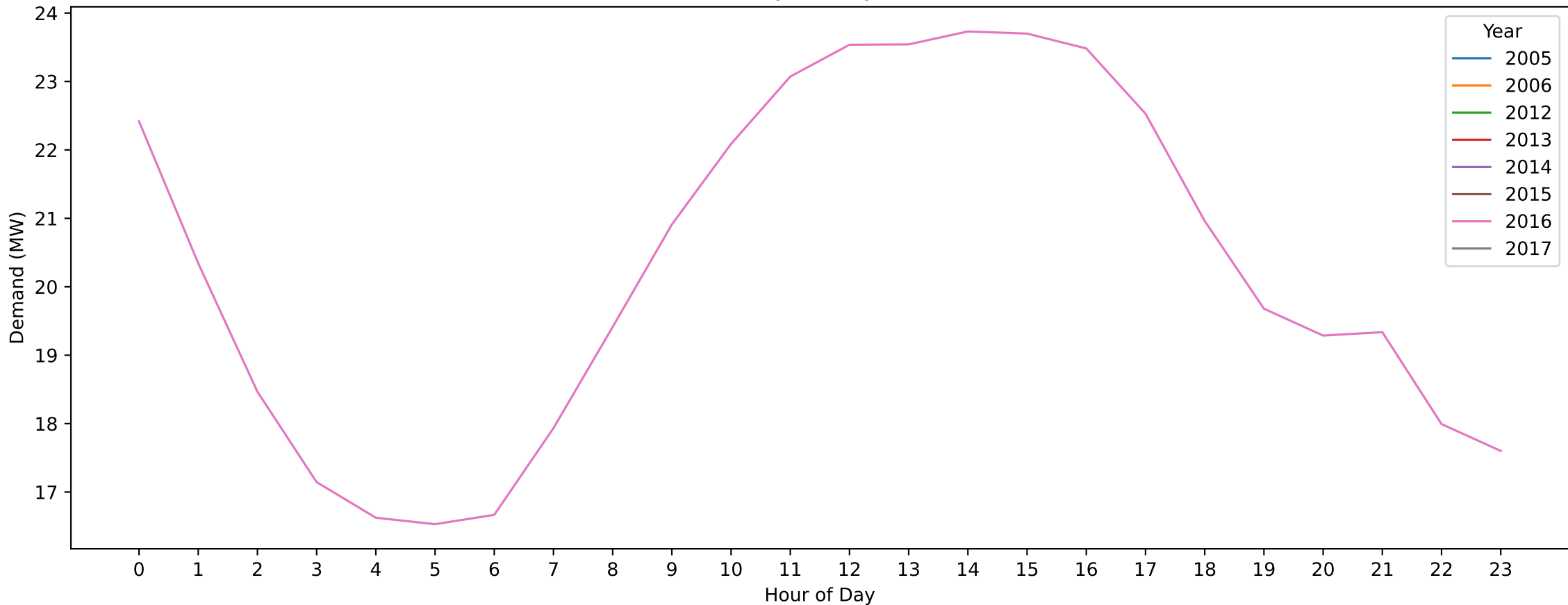
Toorak — New Year's Day (Hourly Demand Across Years)
