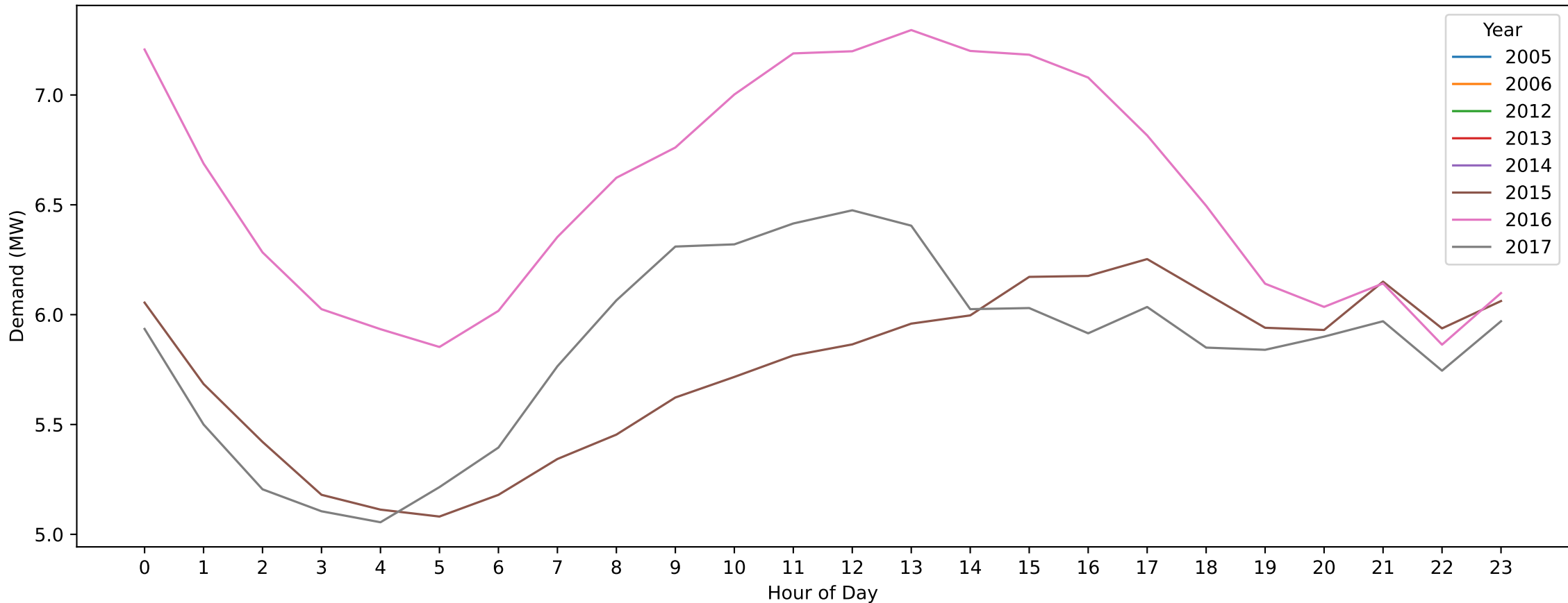
Port Melbourne — New Year's Day (Hourly Demand Across Years)
