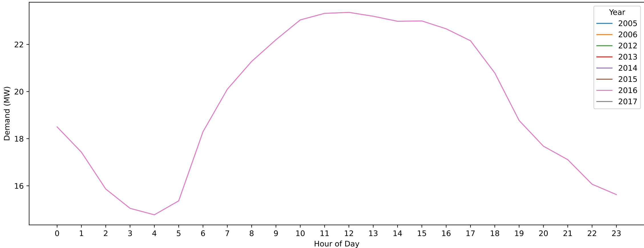
South Melbourne — New Year's Day (Hourly Demand Across Years)
