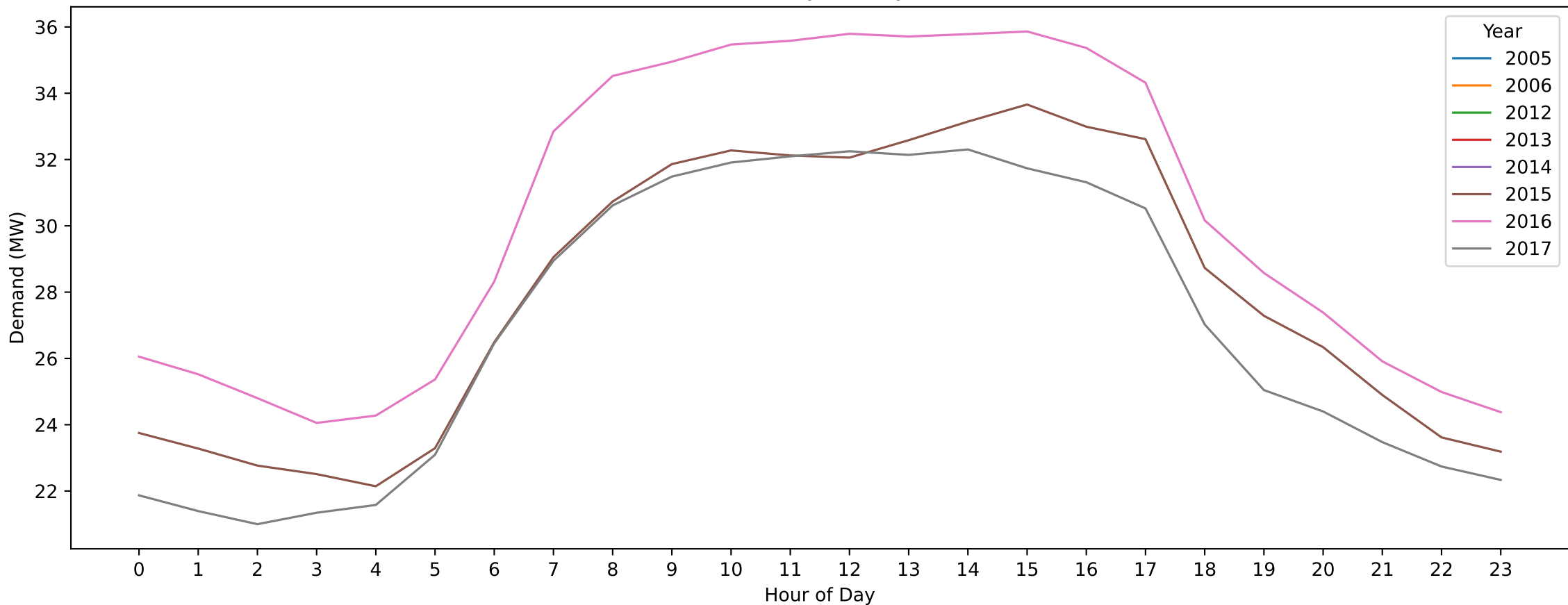
Little Queen — New Year's Day (Hourly Demand Across Years)
