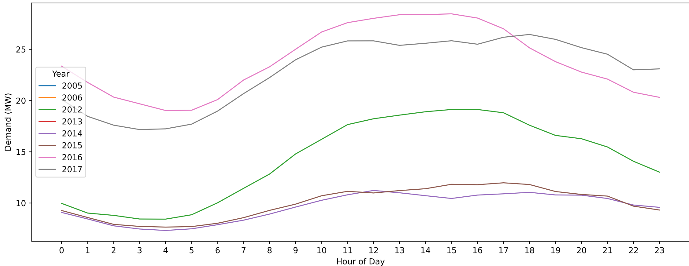
North Richmond — New Year's Day (Hourly Demand Across Years)
