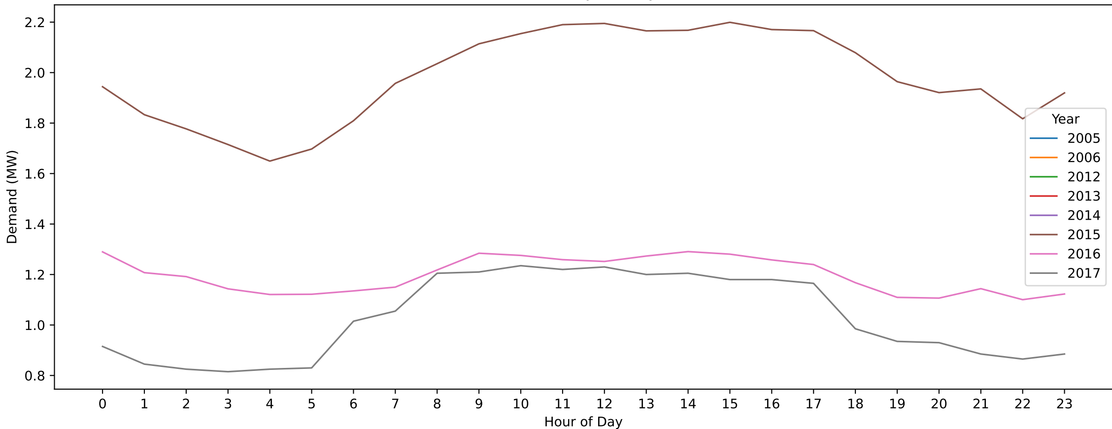
Tavistock Place — New Year's Day (Hourly Demand Across Years)
