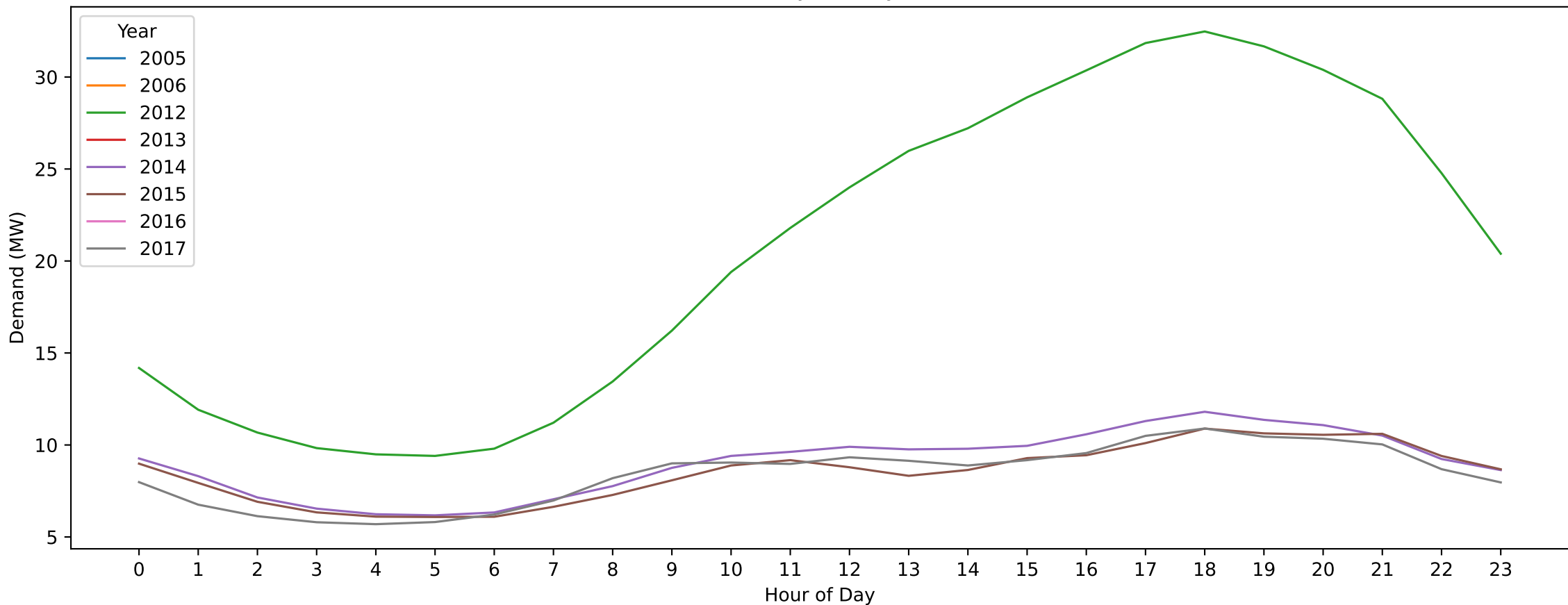
Riversdale — New Year's Day (Hourly Demand Across Years)
