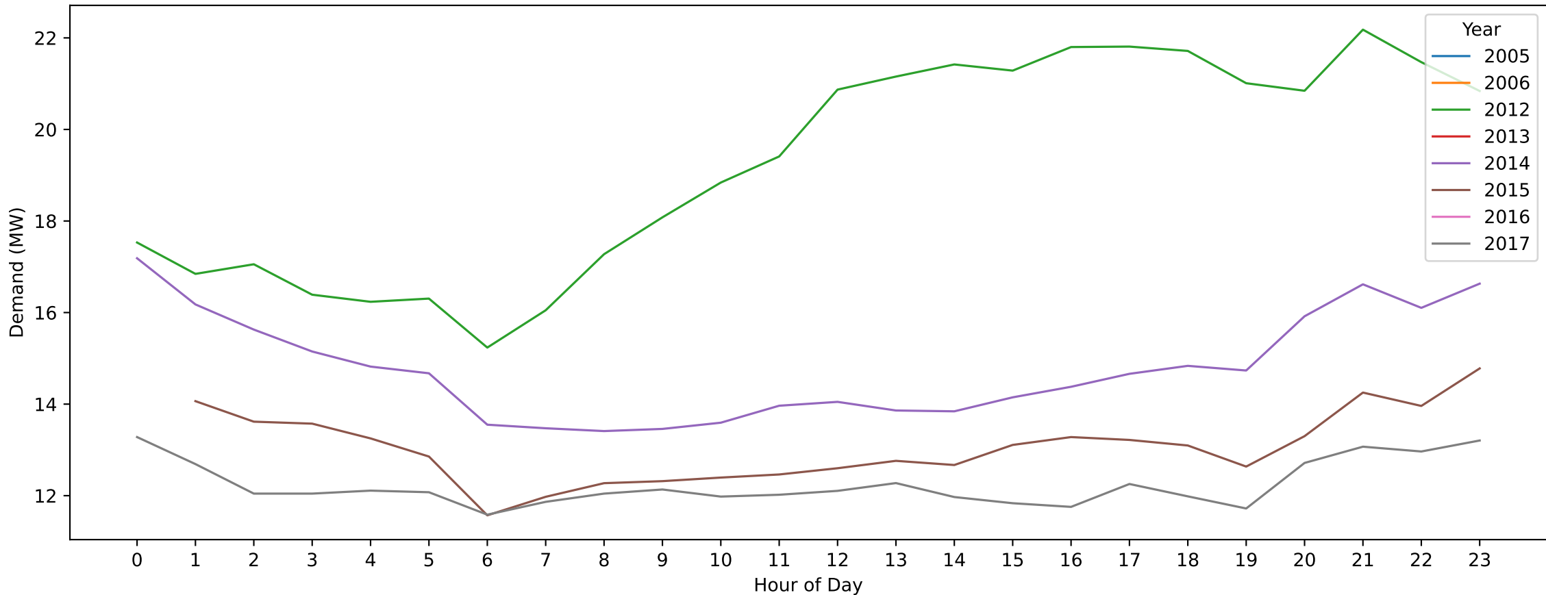
Dock Area — New Year's Day (Hourly Demand Across Years)
