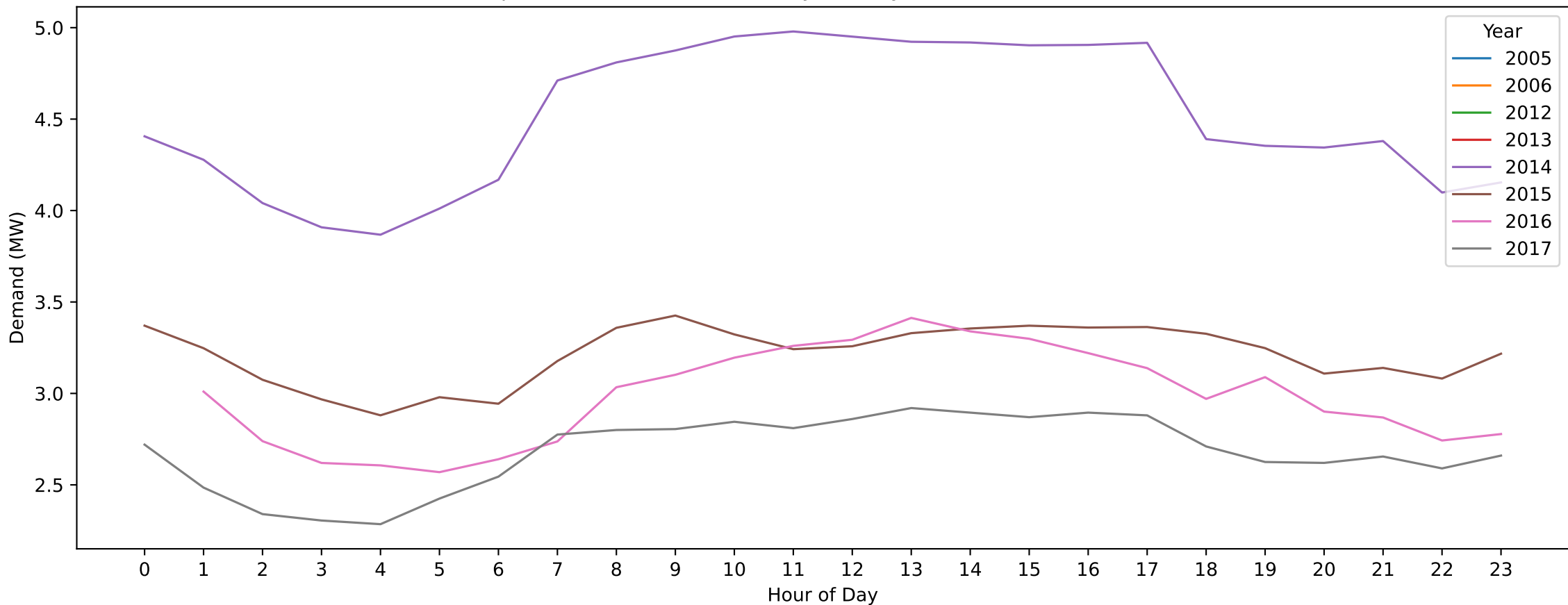
Spencer St — New Year's Day (Hourly Demand Across Years)
