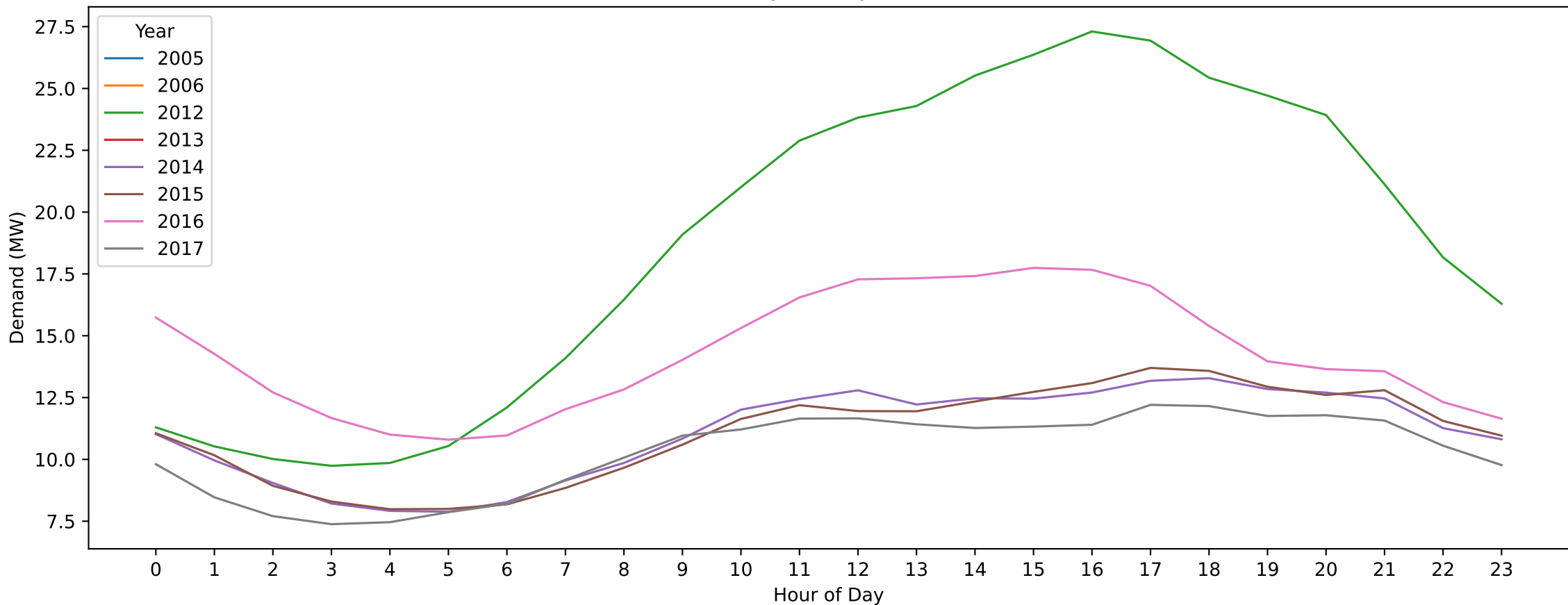
Kew — New Year's Day (Hourly Demand Across Years)
