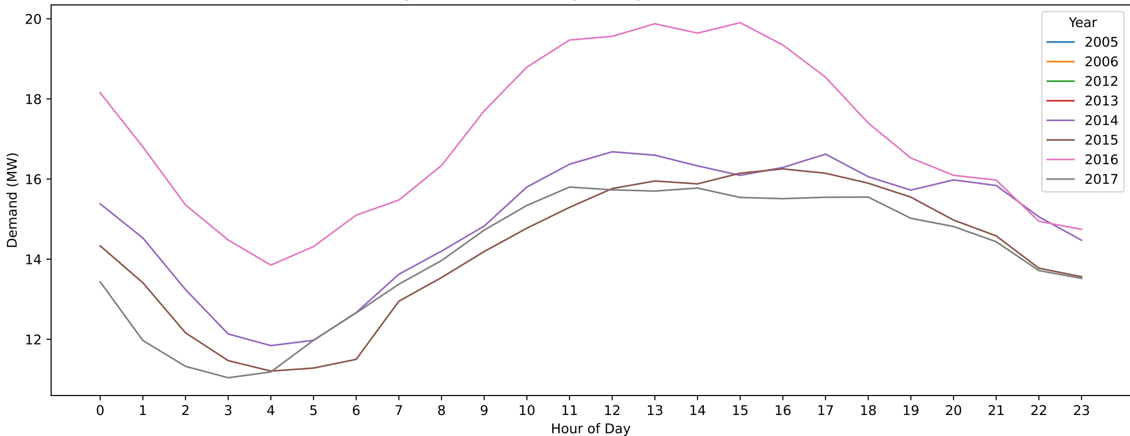
Montagne — New Year's Day (Hourly Demand Across Years)
