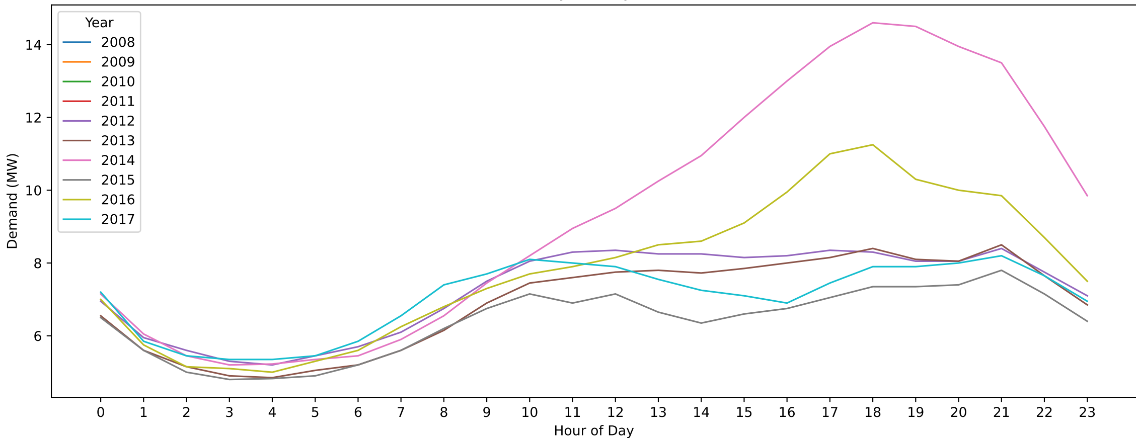
Fairfield — Australia Day (Hourly Demand Across Years)
