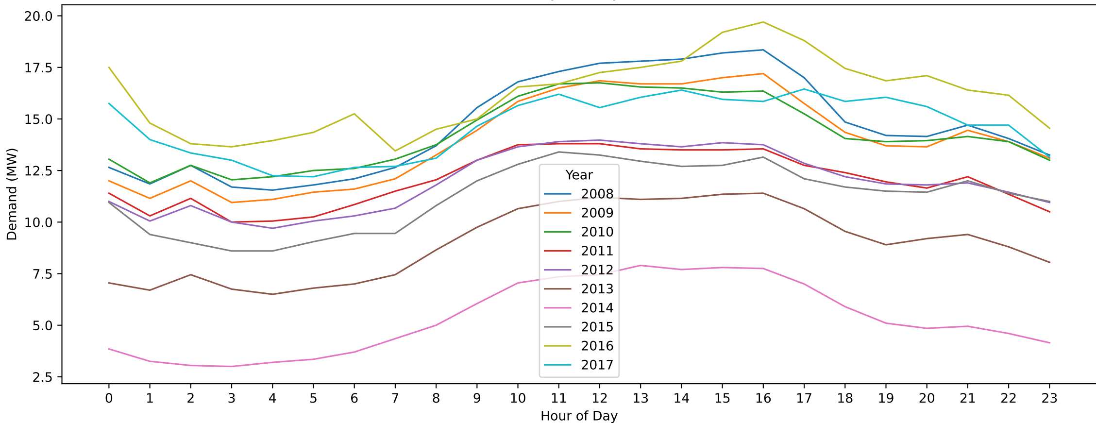
Yarraville — Australia Day (Hourly Demand Across Years)
