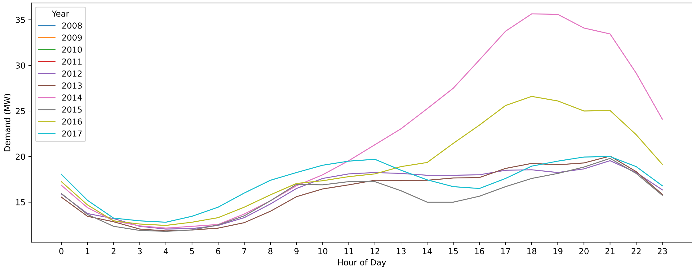
Coburg South — Australia Day (Hourly Demand Across Years)
