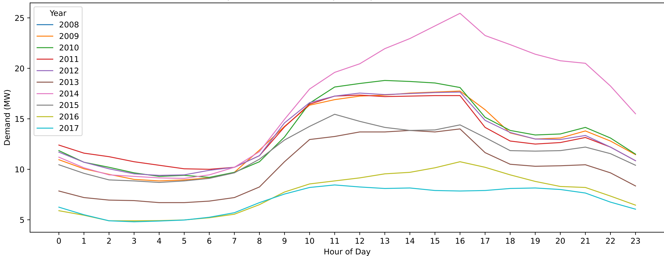
Braybrook — Australia Day (Hourly Demand Across Years)
