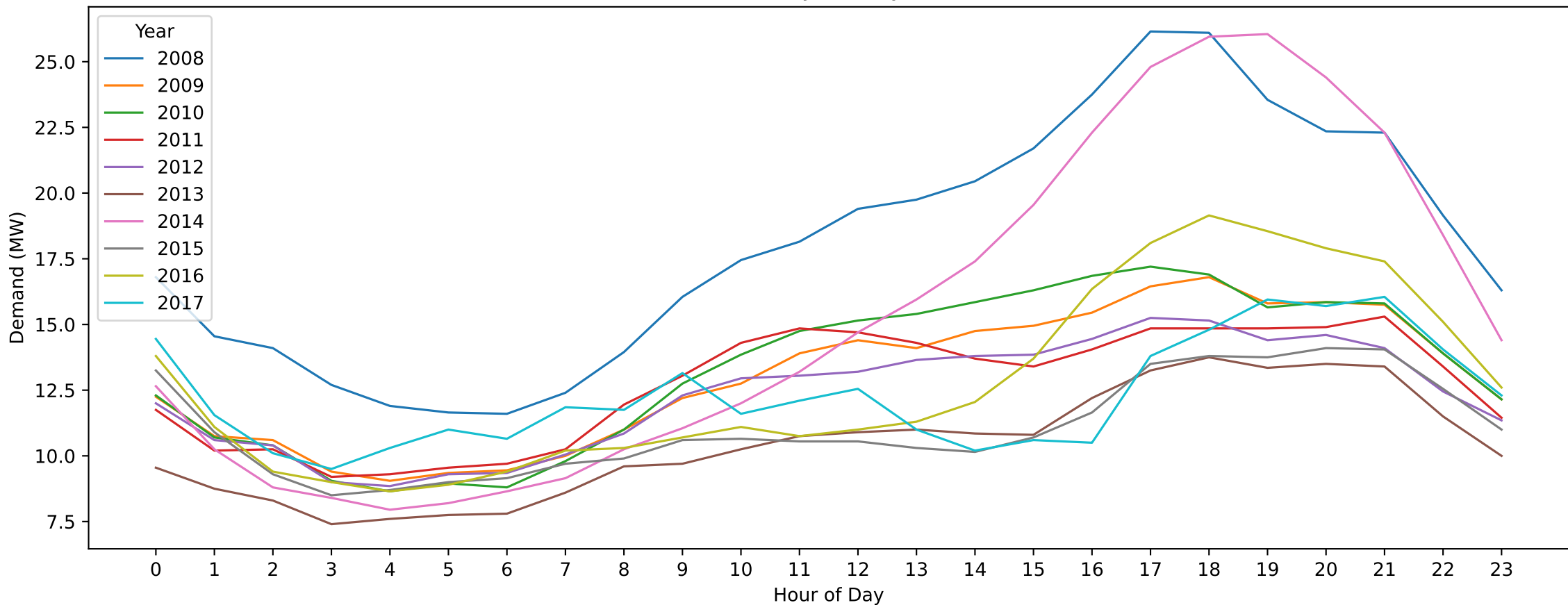
Pascoe Vale — Australia Day (Hourly Demand Across Years)
