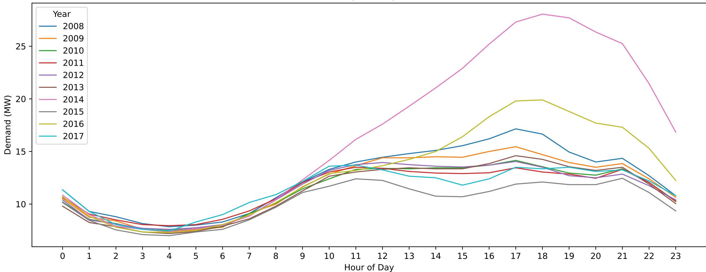
Essendon — Australia Day (Hourly Demand Across Years)
