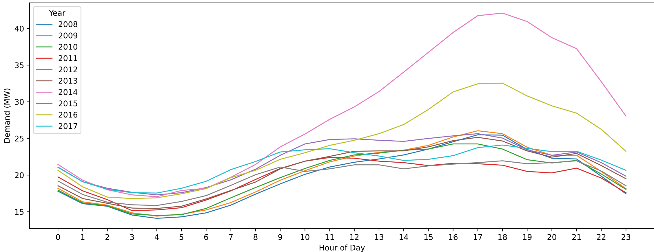
North Heidelberg — Australia Day (Hourly Demand Across Years)
