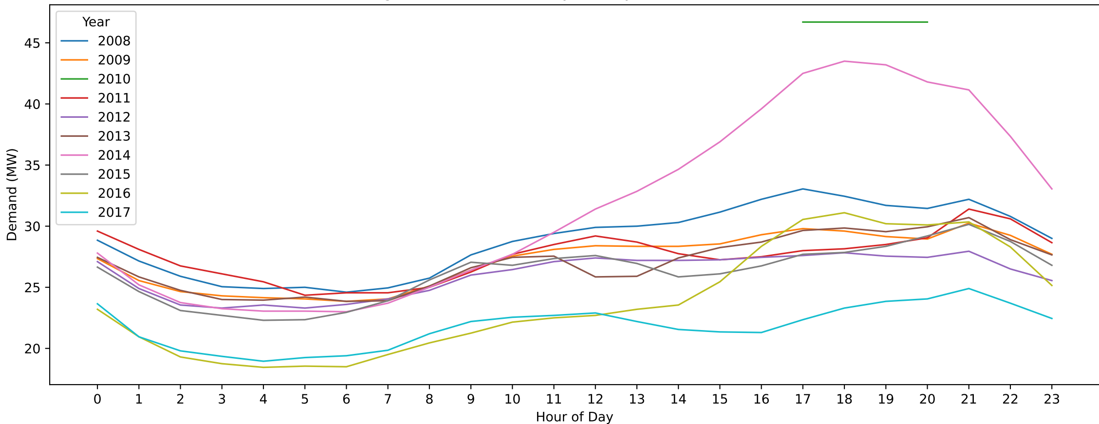
Coburg North — Australia Day (Hourly Demand Across Years)
