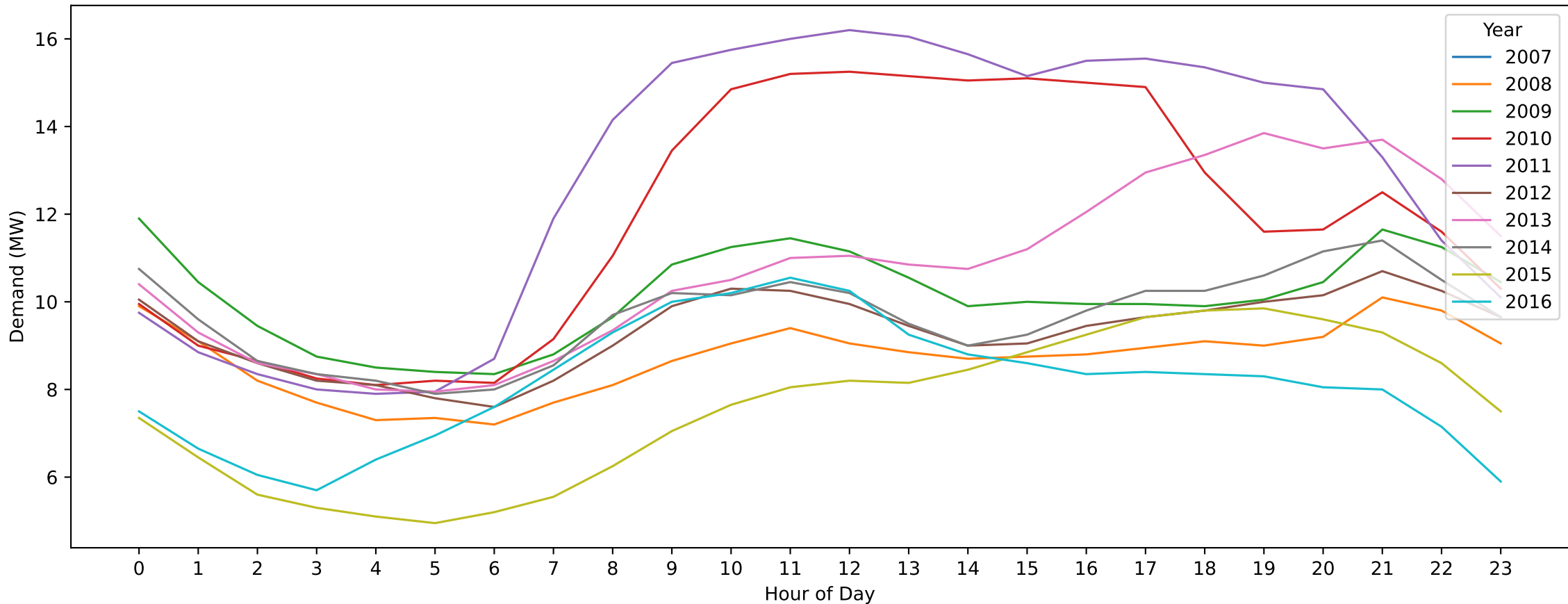
Braybrook — Christmas Day (Hourly Demand Across Years)
