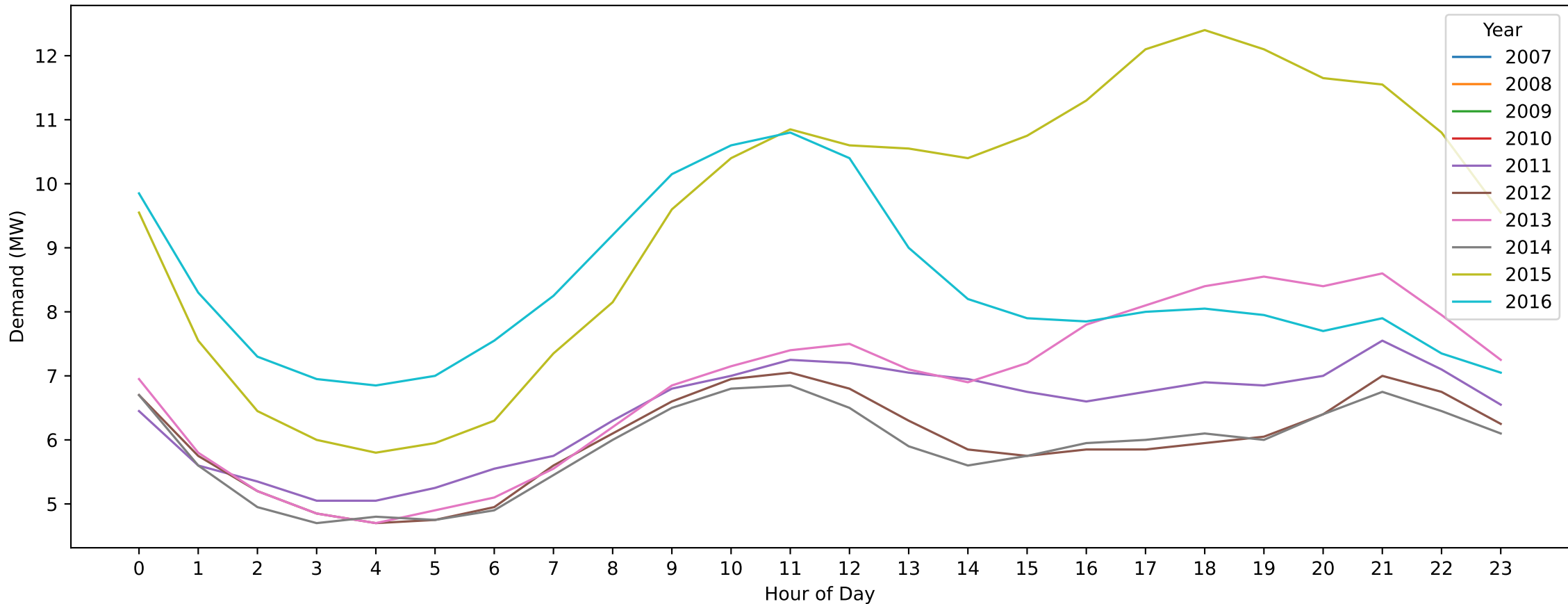
Fairfield — Christmas Day (Hourly Demand Across Years)
