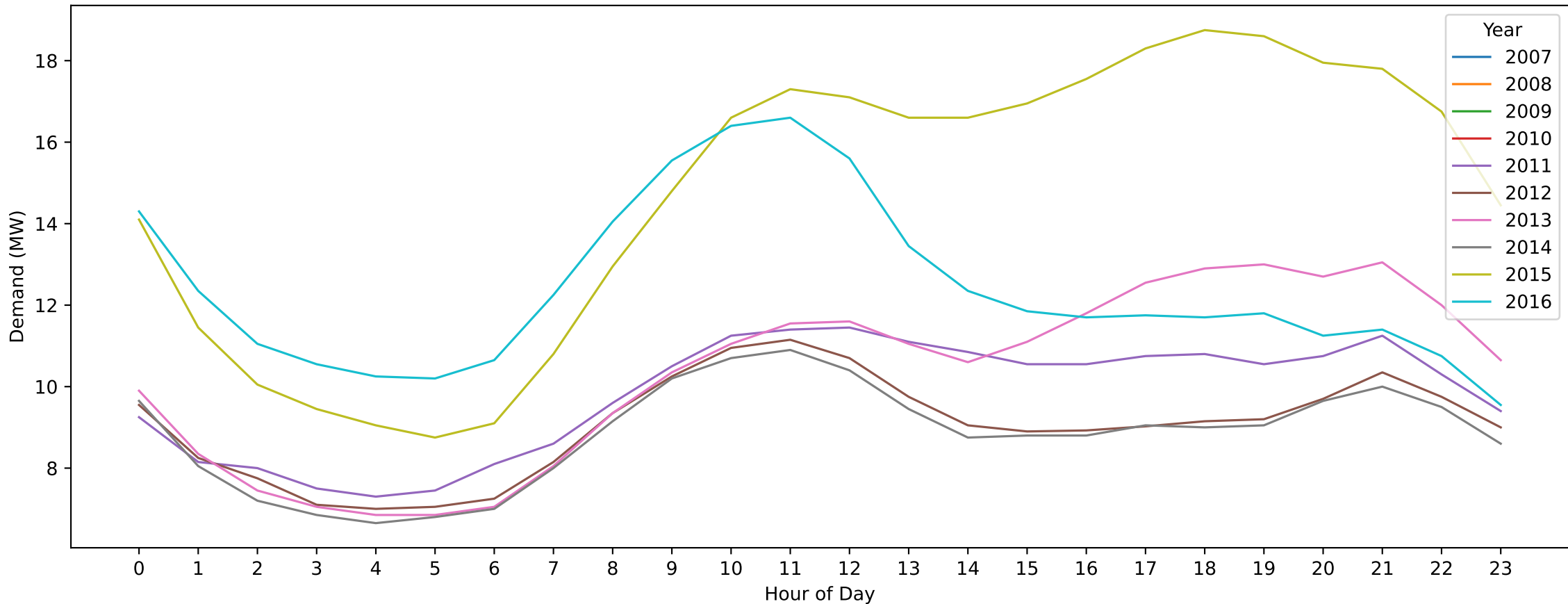
North Essendon — Christmas Day (Hourly Demand Across Years)
