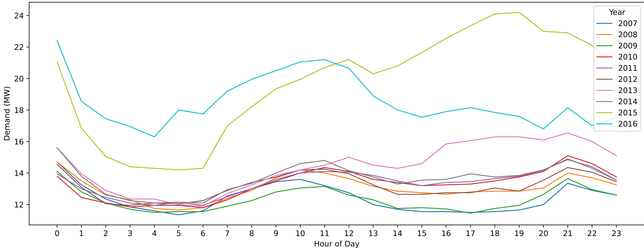
Footscray West — Christmas Day (Hourly Demand Across Years)
