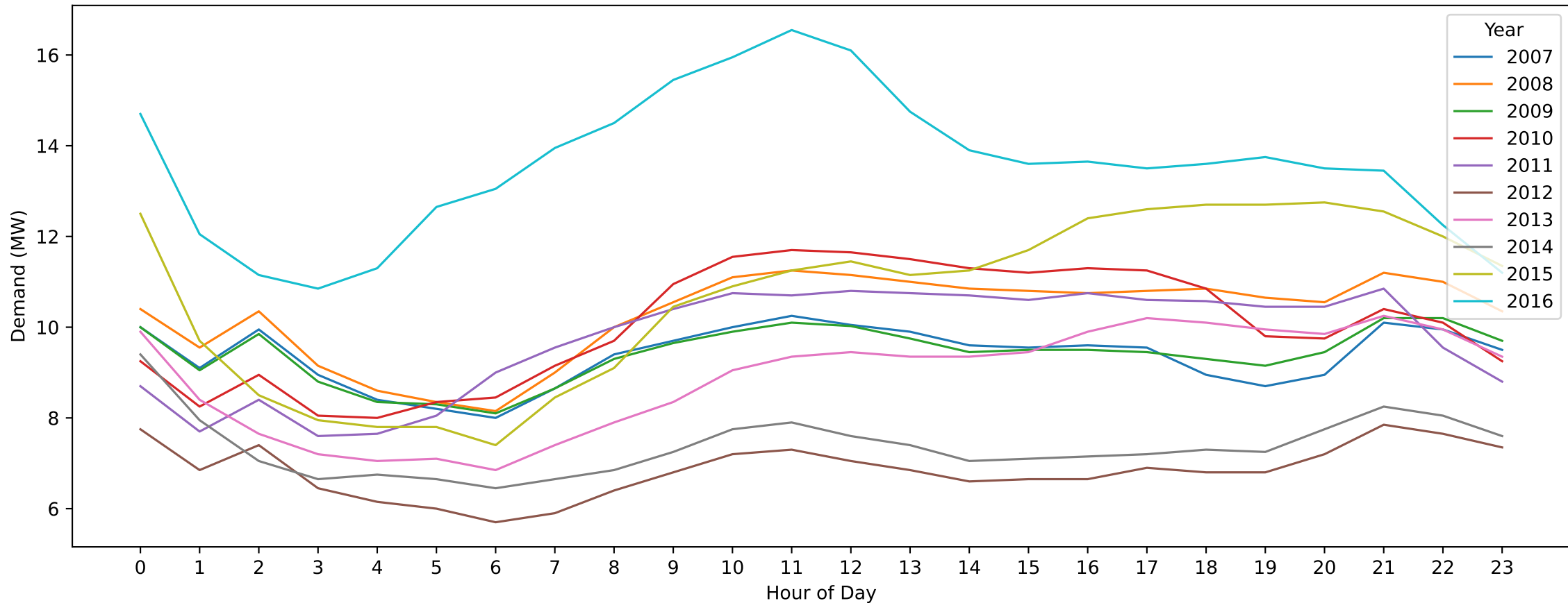
Yarraville — Christmas Day (Hourly Demand Across Years)
