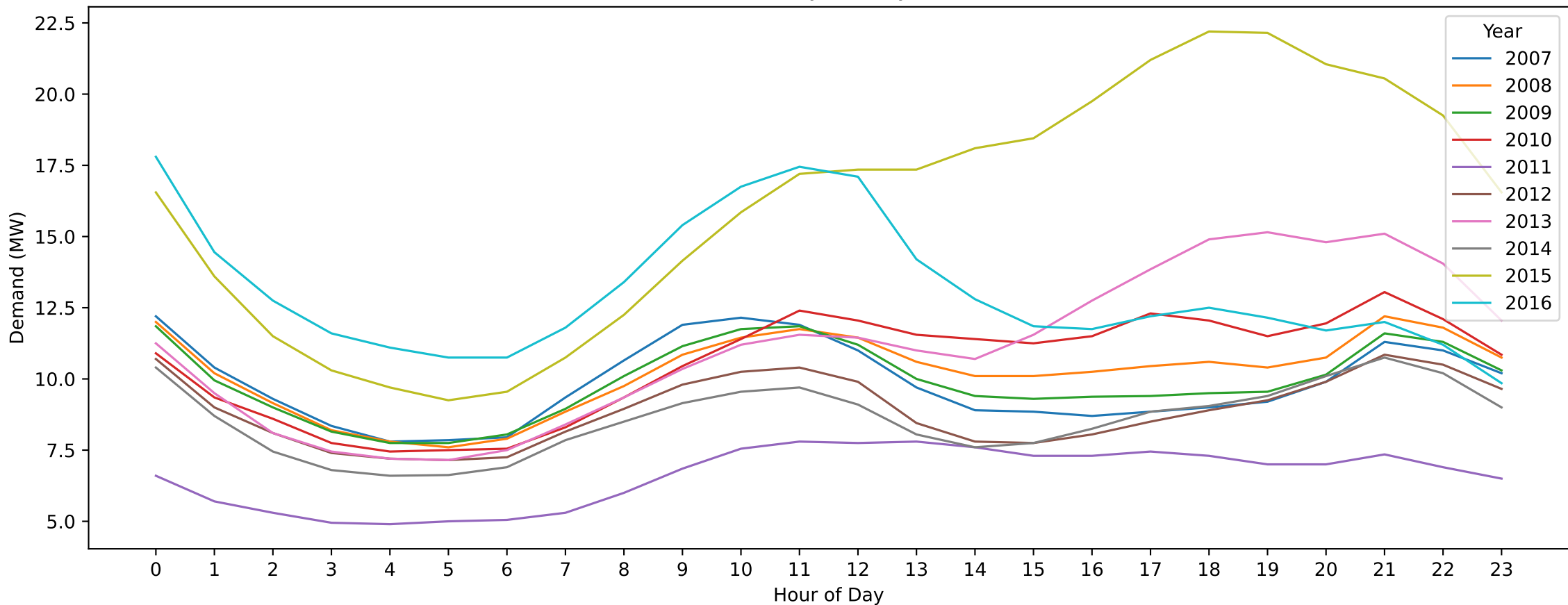
Pascoe Vale — Christmas Day (Hourly Demand Across Years)
