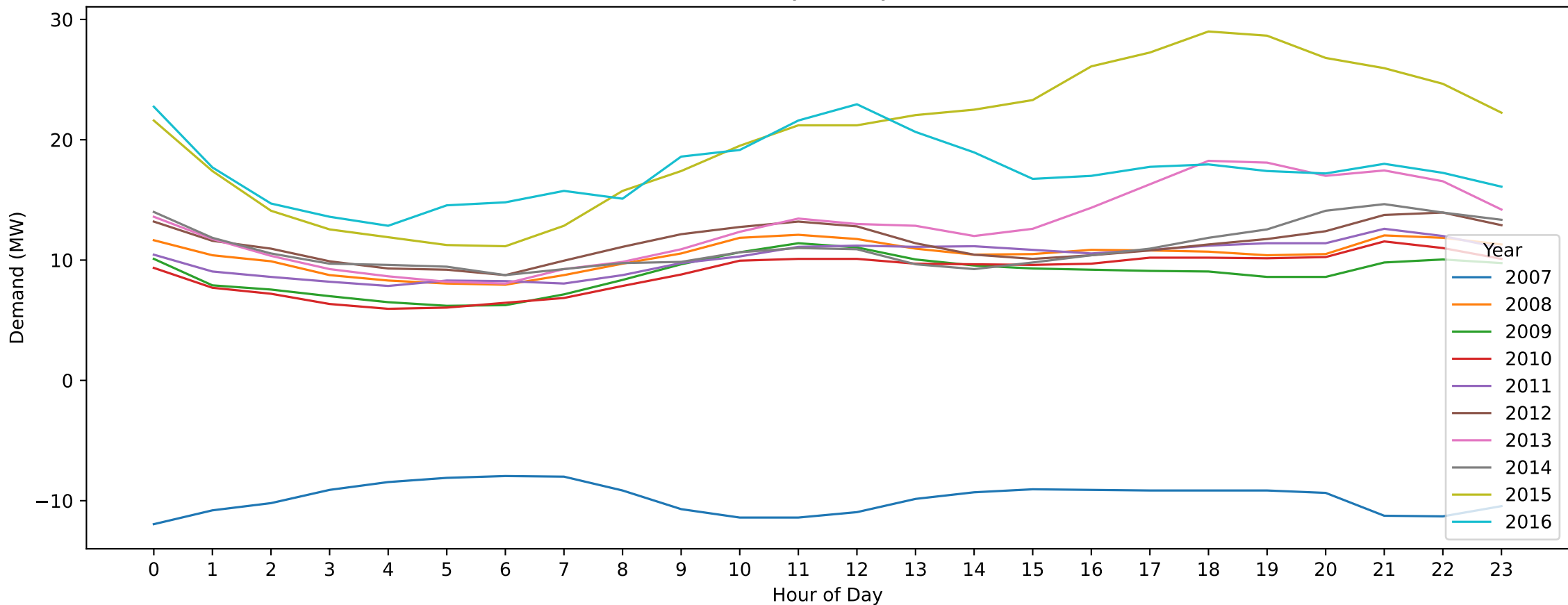
Coolaroo — Christmas Day (Hourly Demand Across Years)
