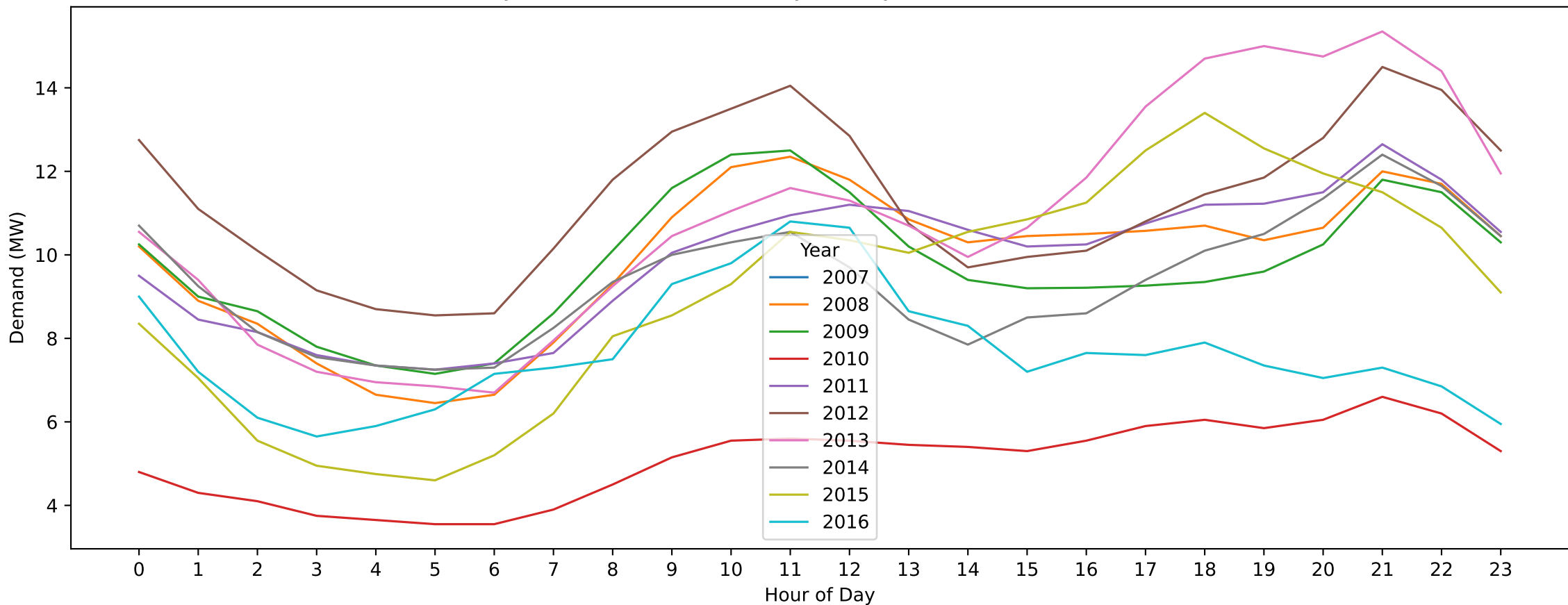
Sydenham — Christmas Day (Hourly Demand Across Years)
