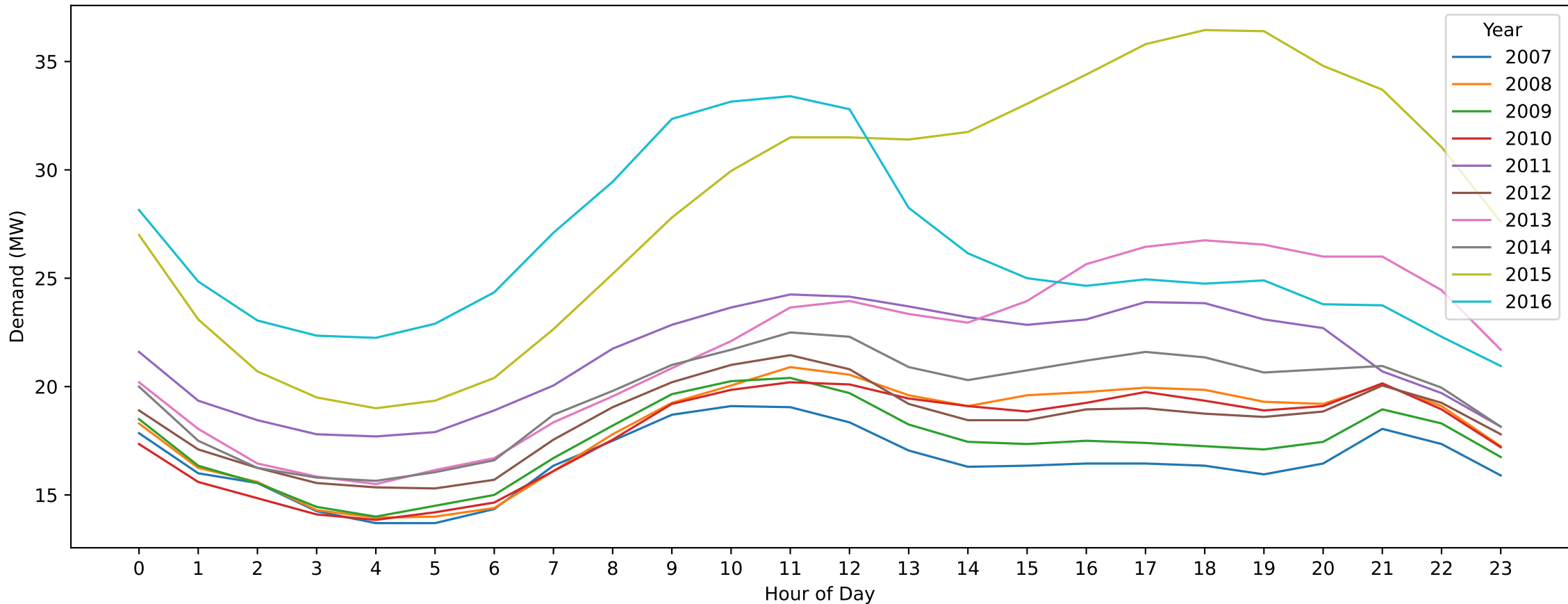
North Heidelberg — Christmas Day (Hourly Demand Across Years)
