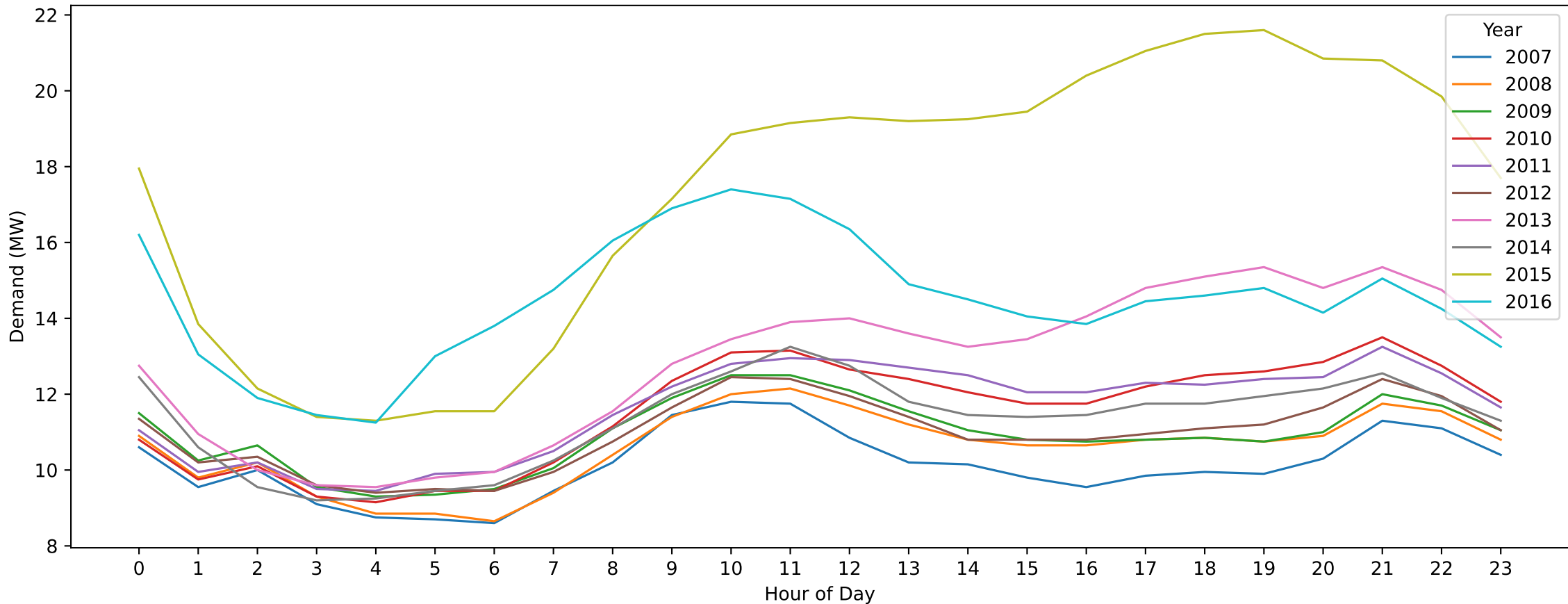
Flemington — Christmas Day (Hourly Demand Across Years)
