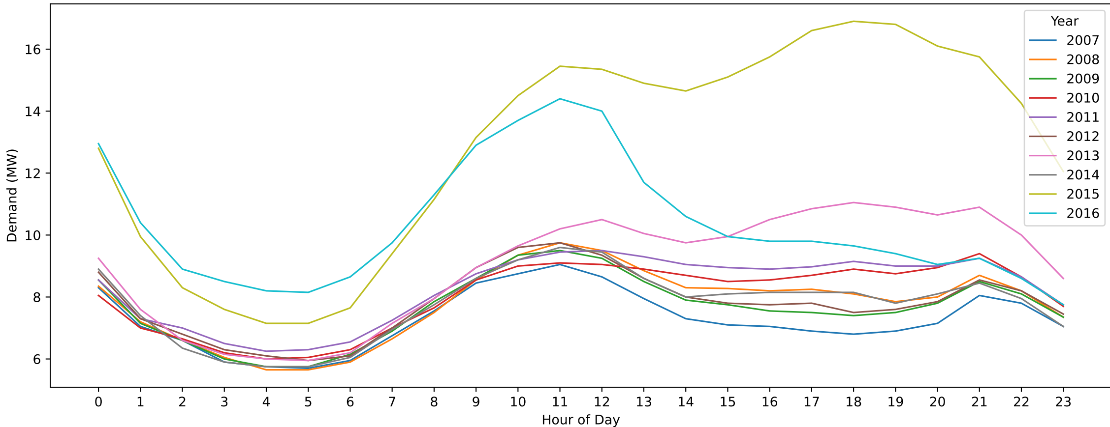
Heidelberg — Christmas Day (Hourly Demand Across Years)
