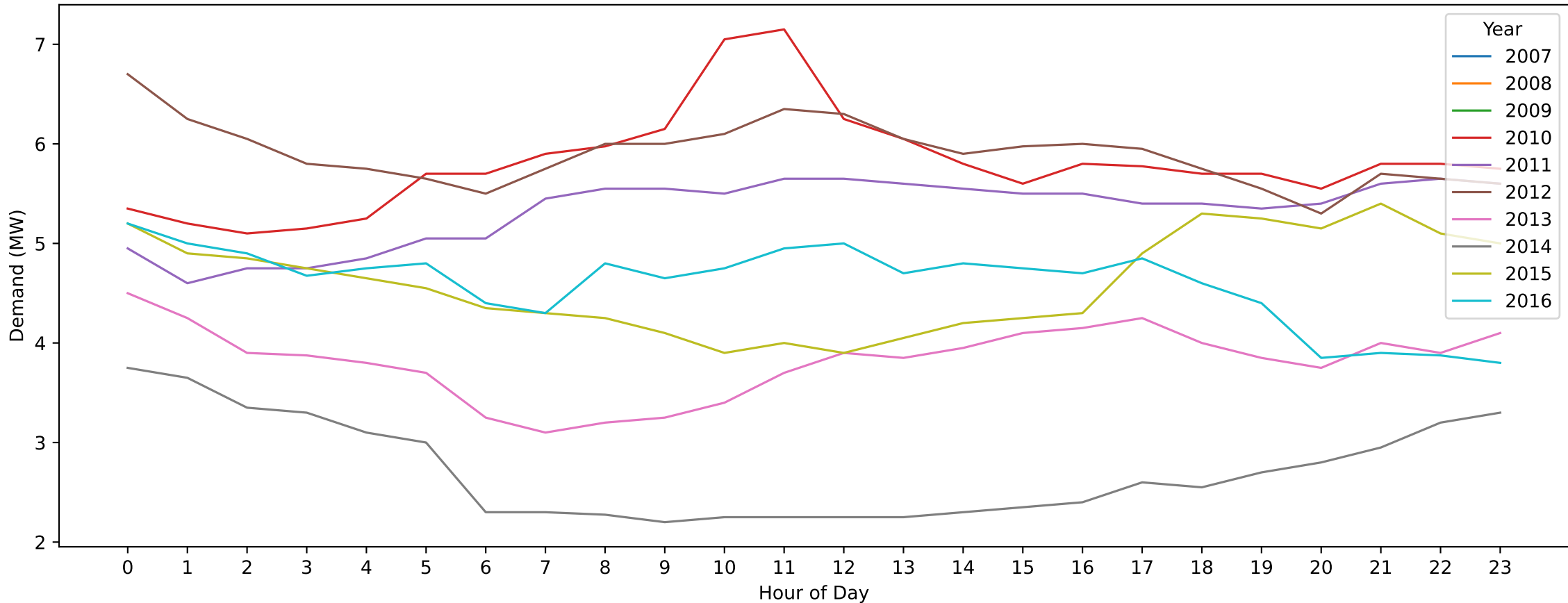
Tottenham — Christmas Day (Hourly Demand Across Years)
