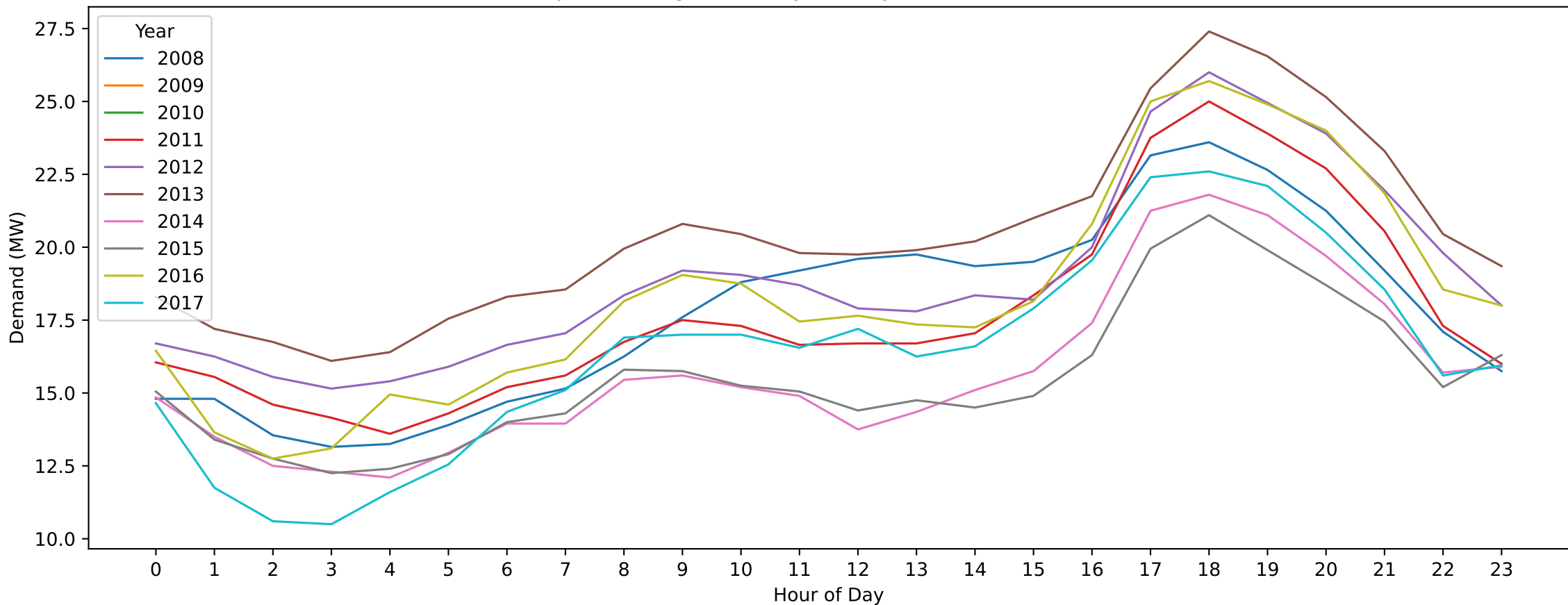
Newport — King's Birthday (Hourly Demand Across Years)
