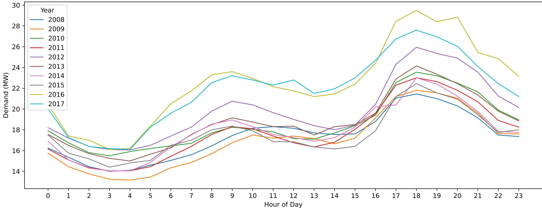
Footscray West — King's Birthday (Hourly Demand Across Years)
