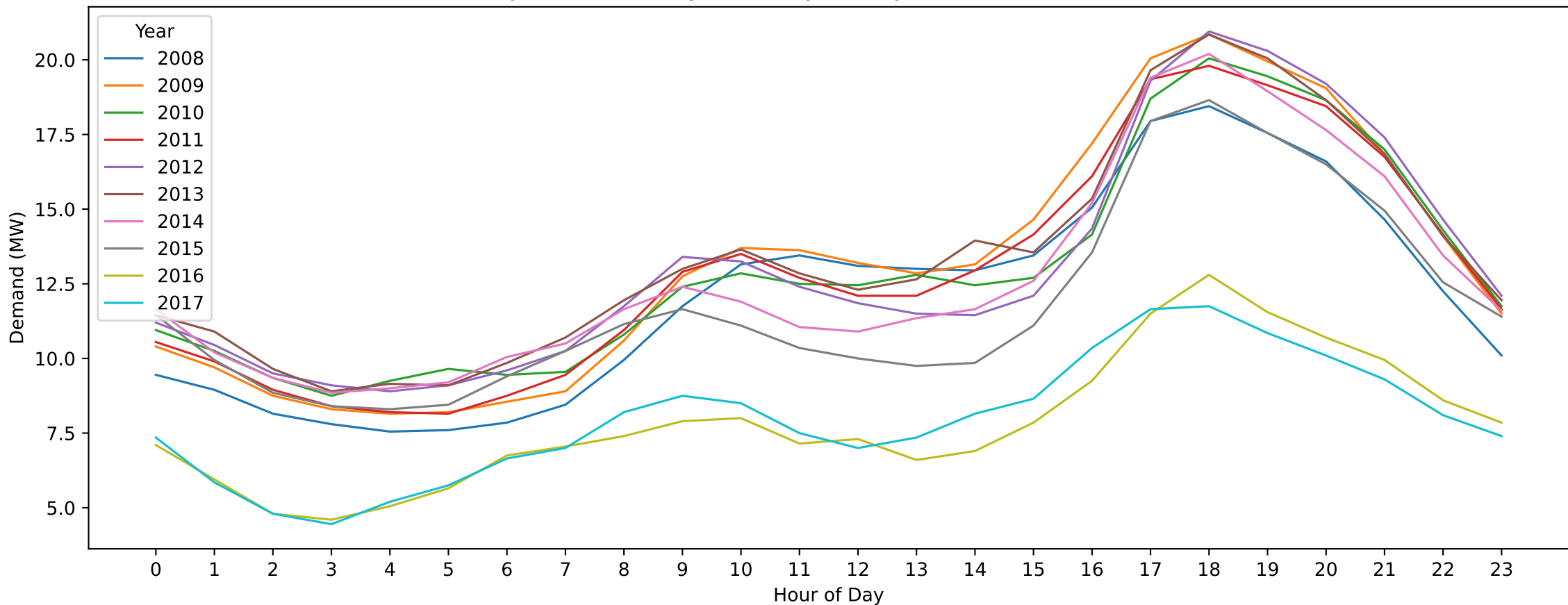
Sydenham — King's Birthday (Hourly Demand Across Years)
