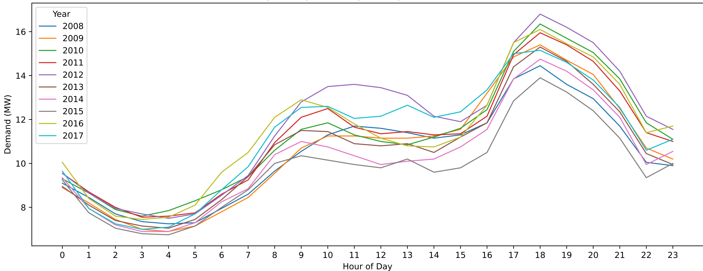
Heidelberg — King's Birthday (Hourly Demand Across Years)
