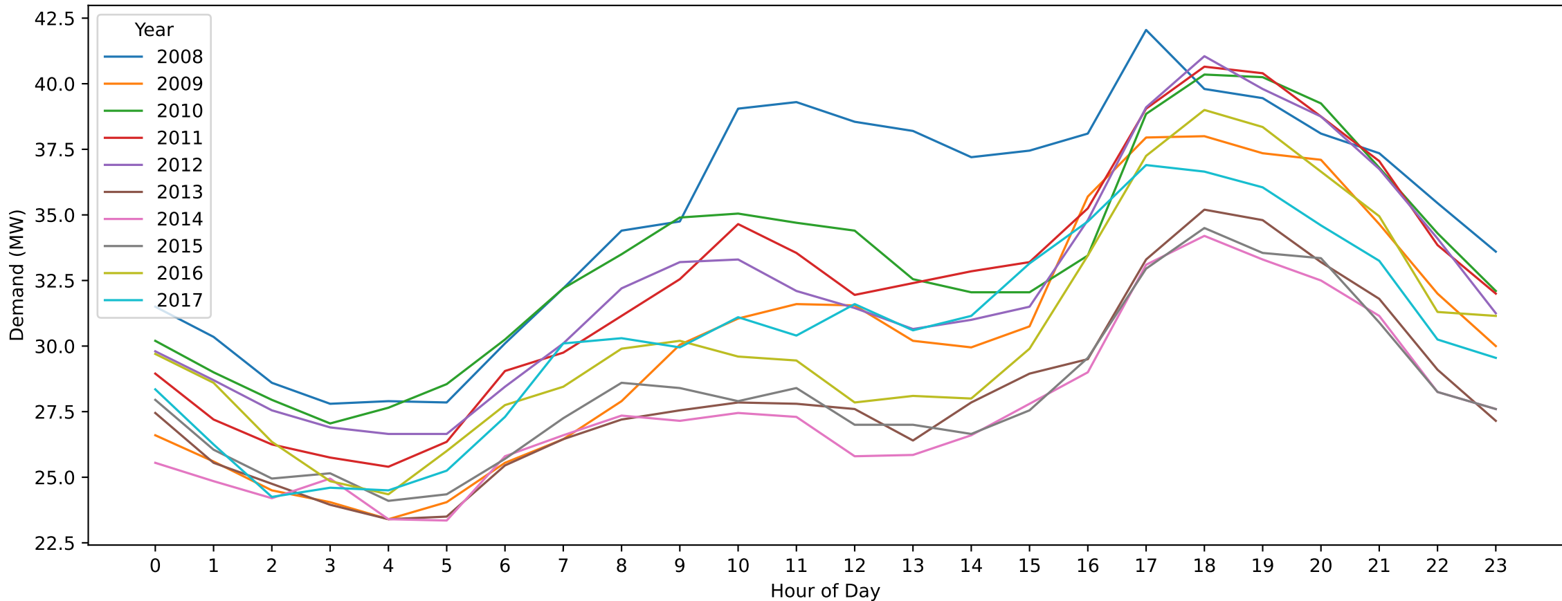
Somerton — King's Birthday (Hourly Demand Across Years)
