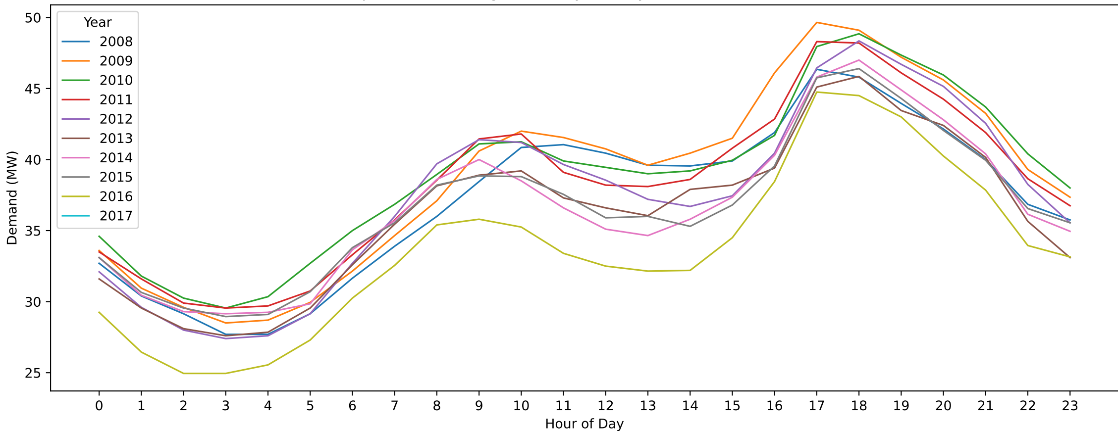
Airport West — King's Birthday (Hourly Demand Across Years)
