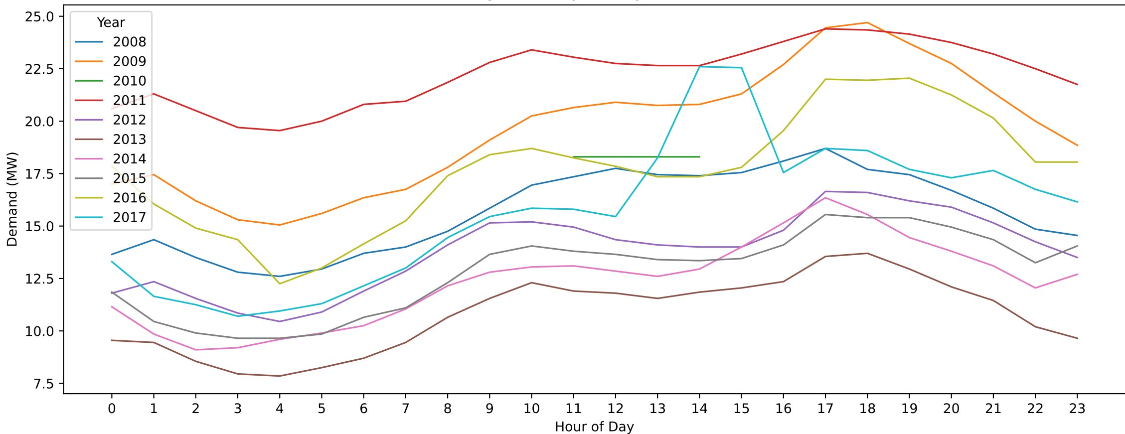
Yarraville — King's Birthday (Hourly Demand Across Years)
