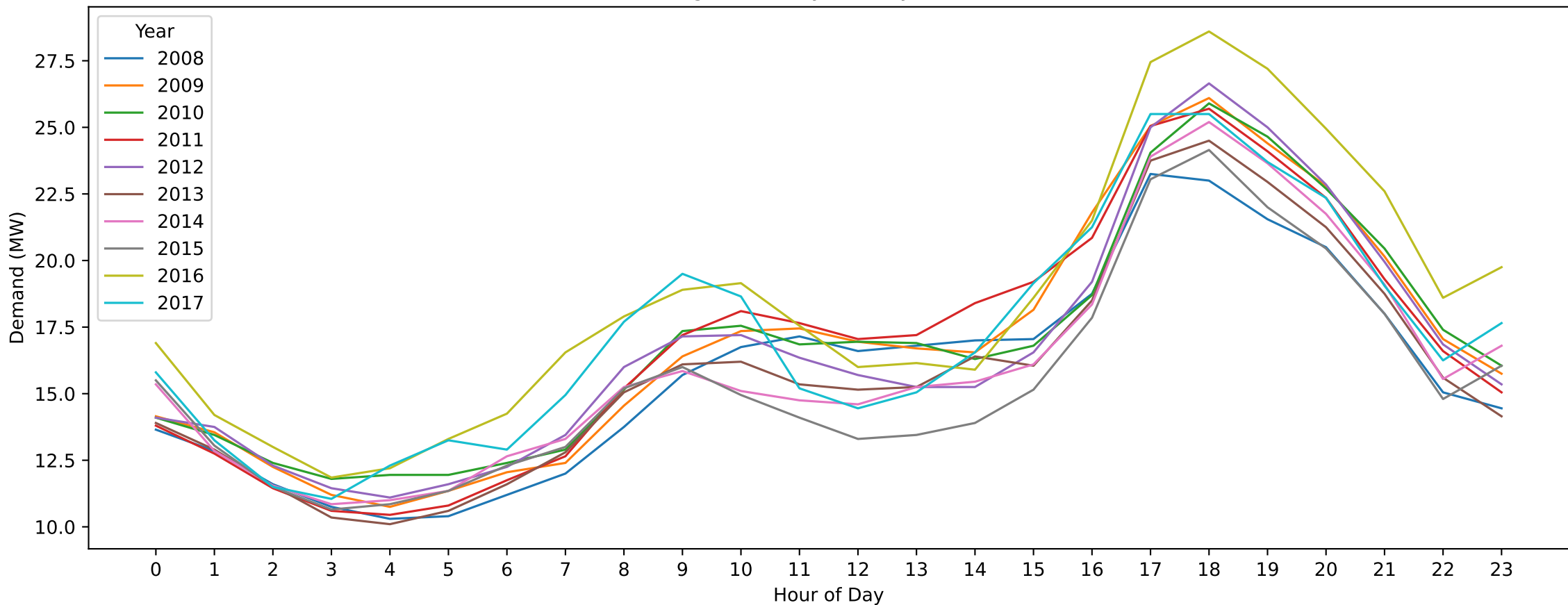
Pascoe Vale — King's Birthday (Hourly Demand Across Years)
