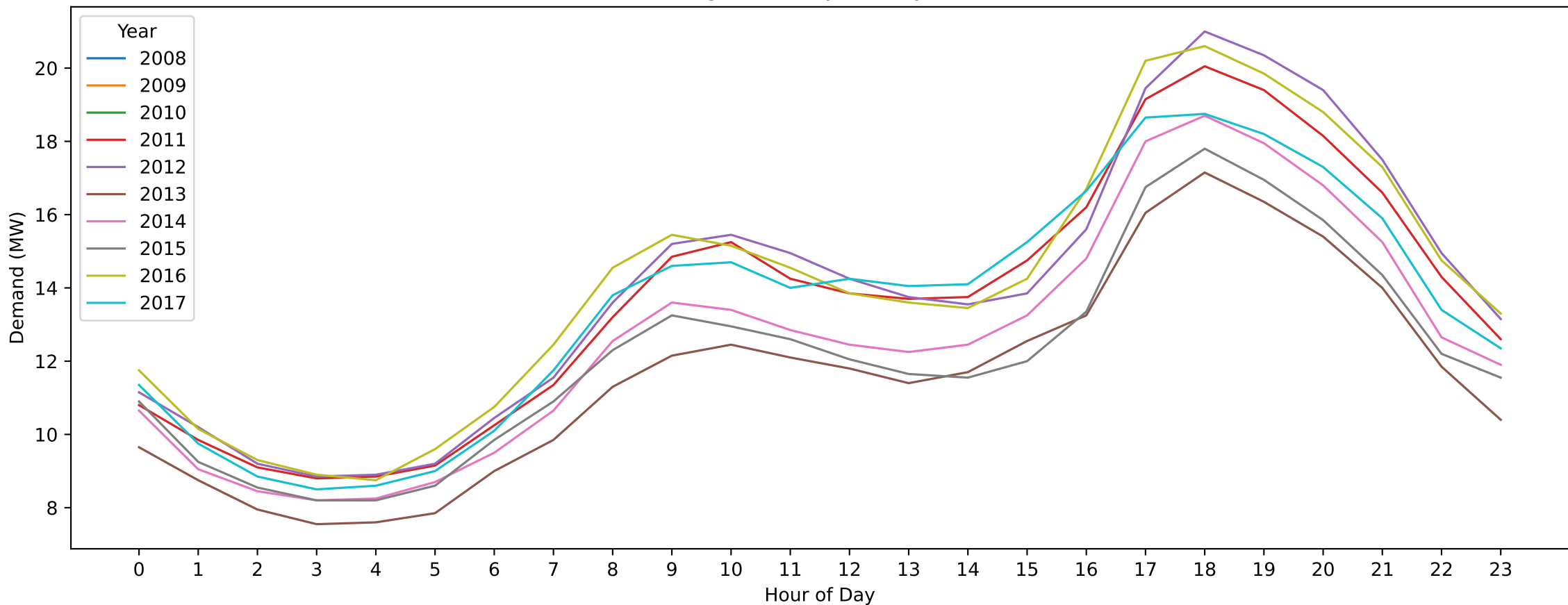
North Essendon — King's Birthday (Hourly Demand Across Years)
