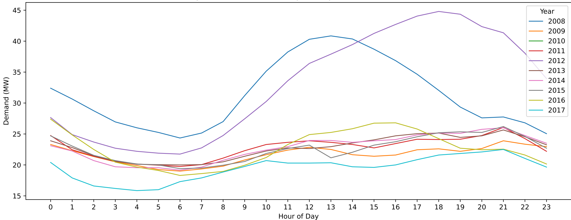
Coburg North — New Year's Day (Hourly Demand Across Years)
