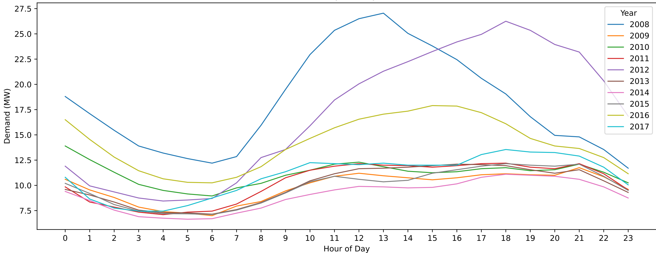
Essendon — New Year's Day (Hourly Demand Across Years)
