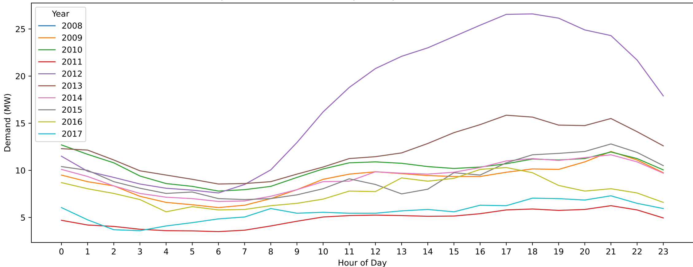
Sydenham — New Year's Day (Hourly Demand Across Years)
