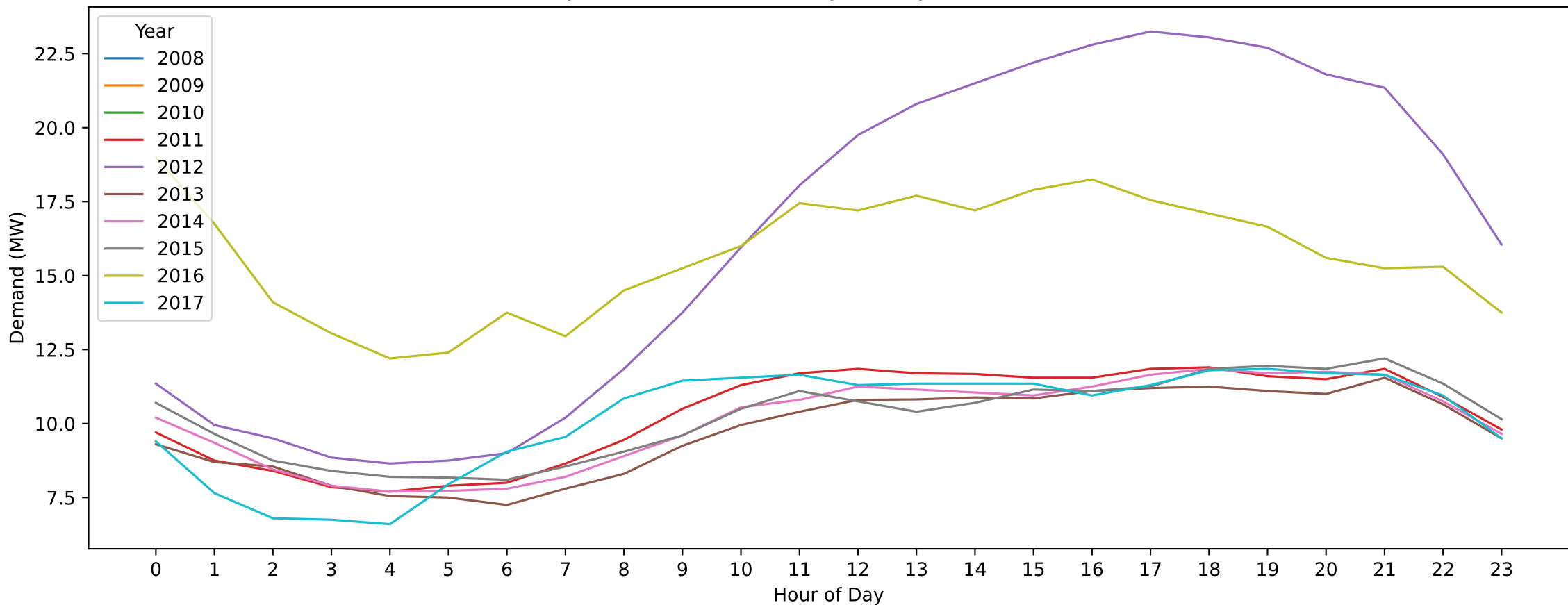
Footscray East — New Year's Day (Hourly Demand Across Years)
