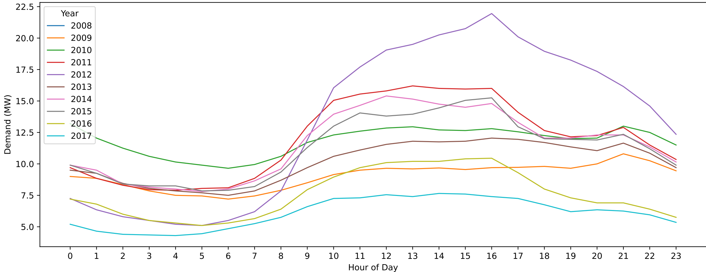
Braybrook — New Year's Day (Hourly Demand Across Years)
