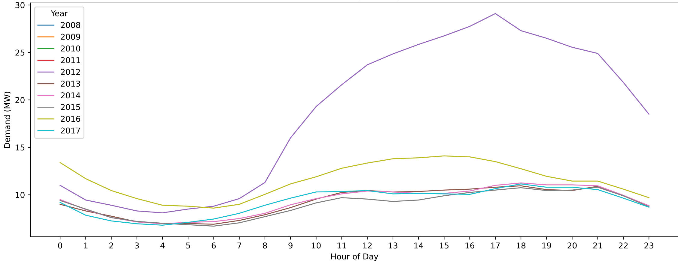
North Essendon — New Year's Day (Hourly Demand Across Years)
