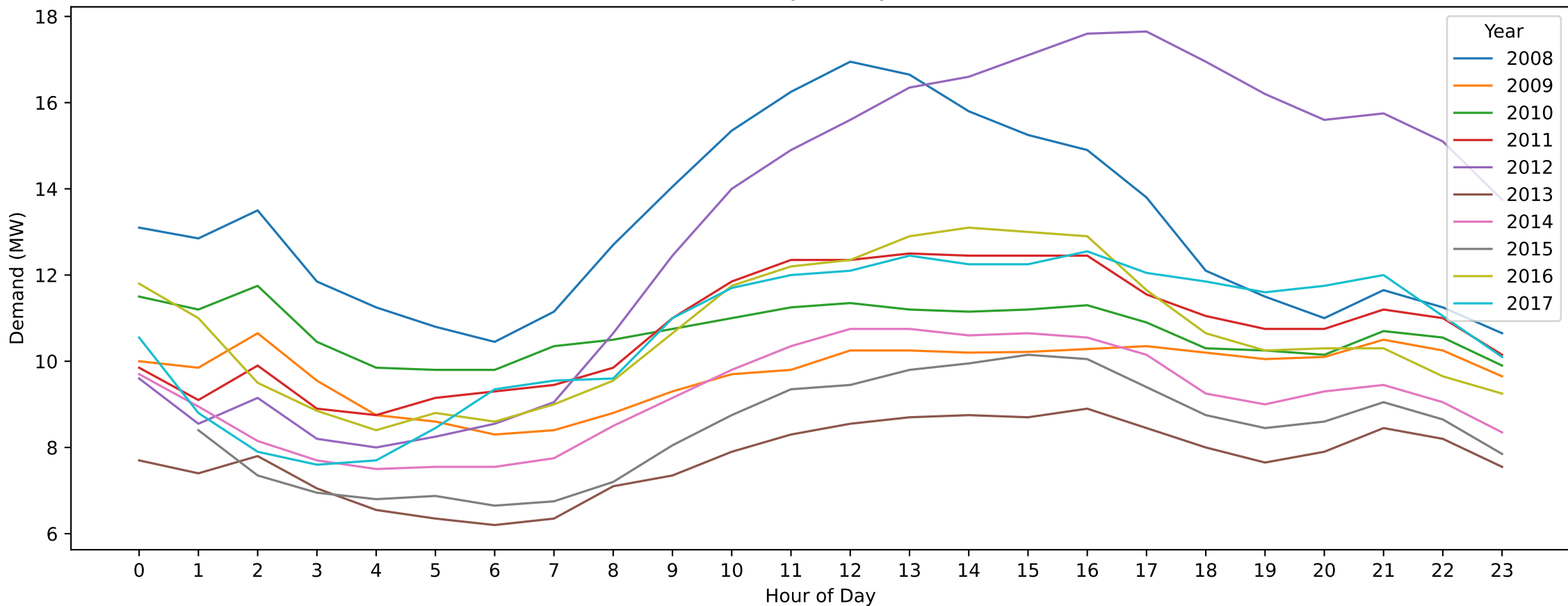
Yarraville — New Year's Day (Hourly Demand Across Years)
