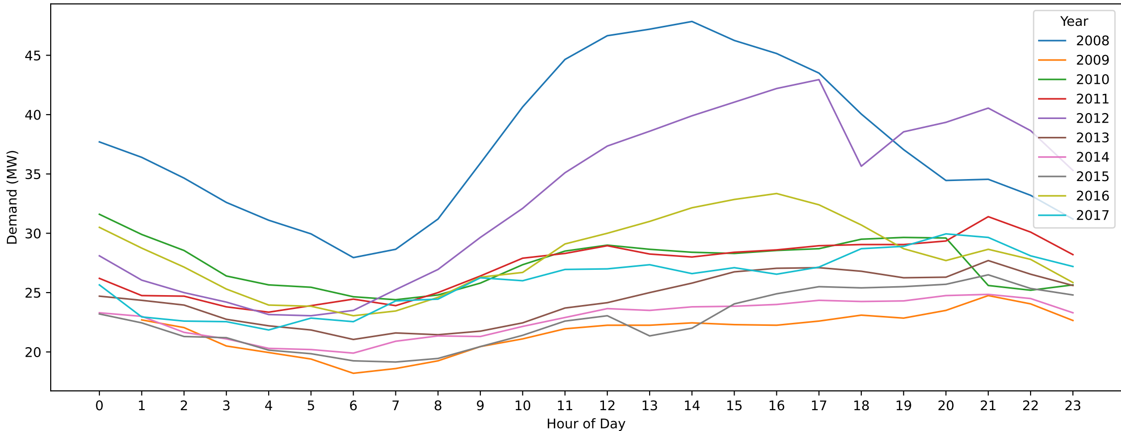
Somerton — New Year's Day (Hourly Demand Across Years)
