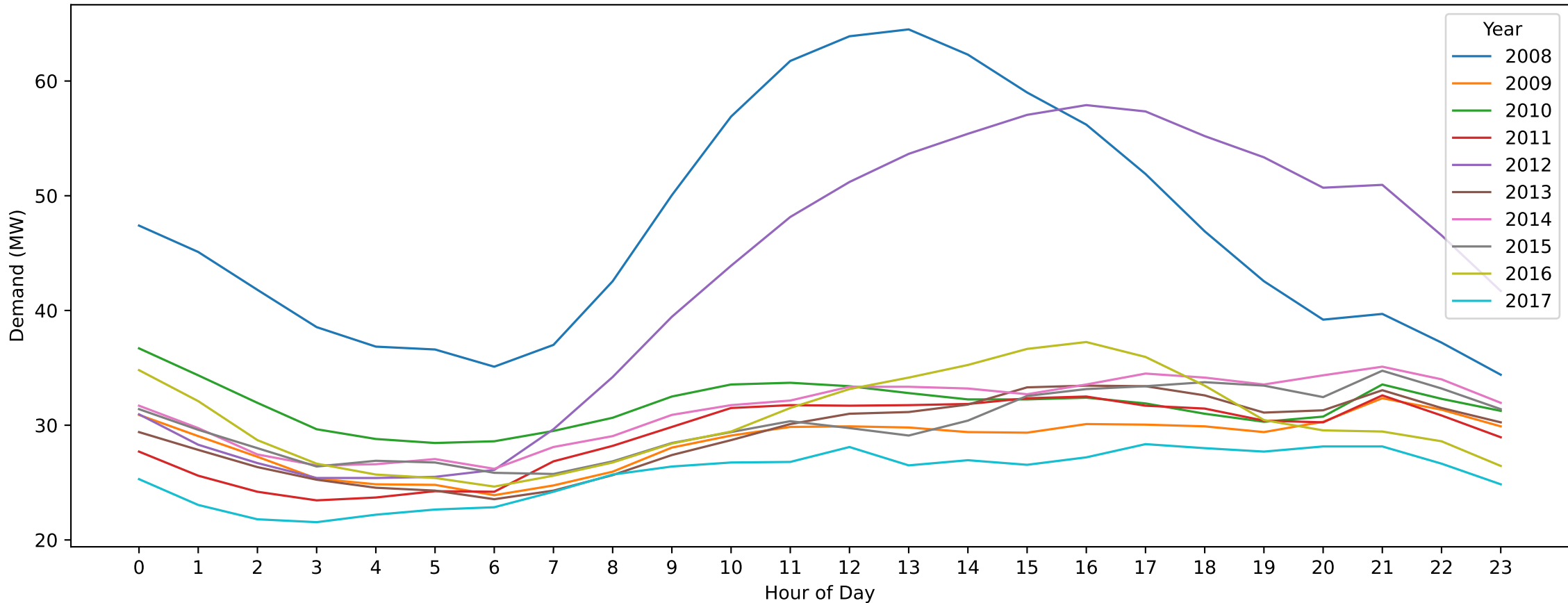
Airport West — New Year's Day (Hourly Demand Across Years)
