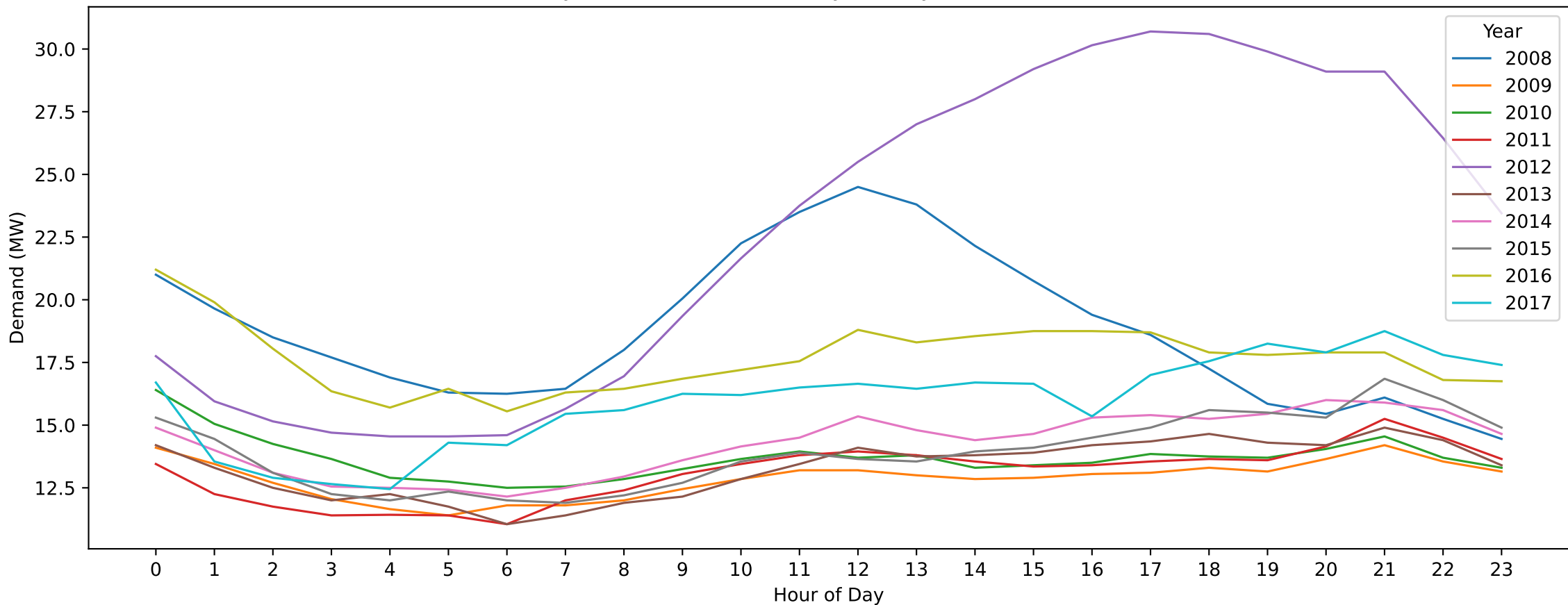
Footscray West — New Year's Day (Hourly Demand Across Years)
