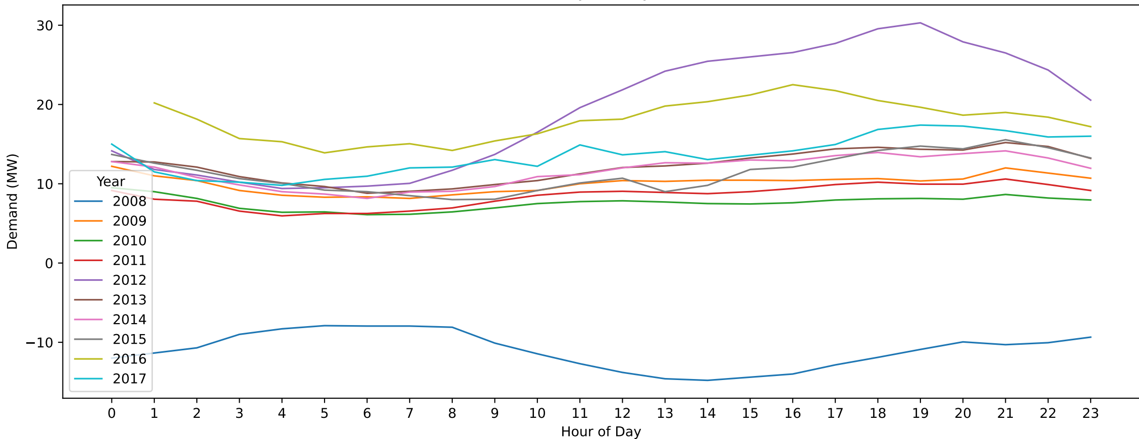
Coolaroo — New Year's Day (Hourly Demand Across Years)
