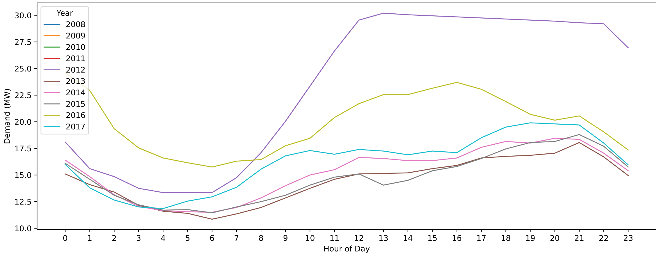
Coburg South — New Year's Day (Hourly Demand Across Years)
