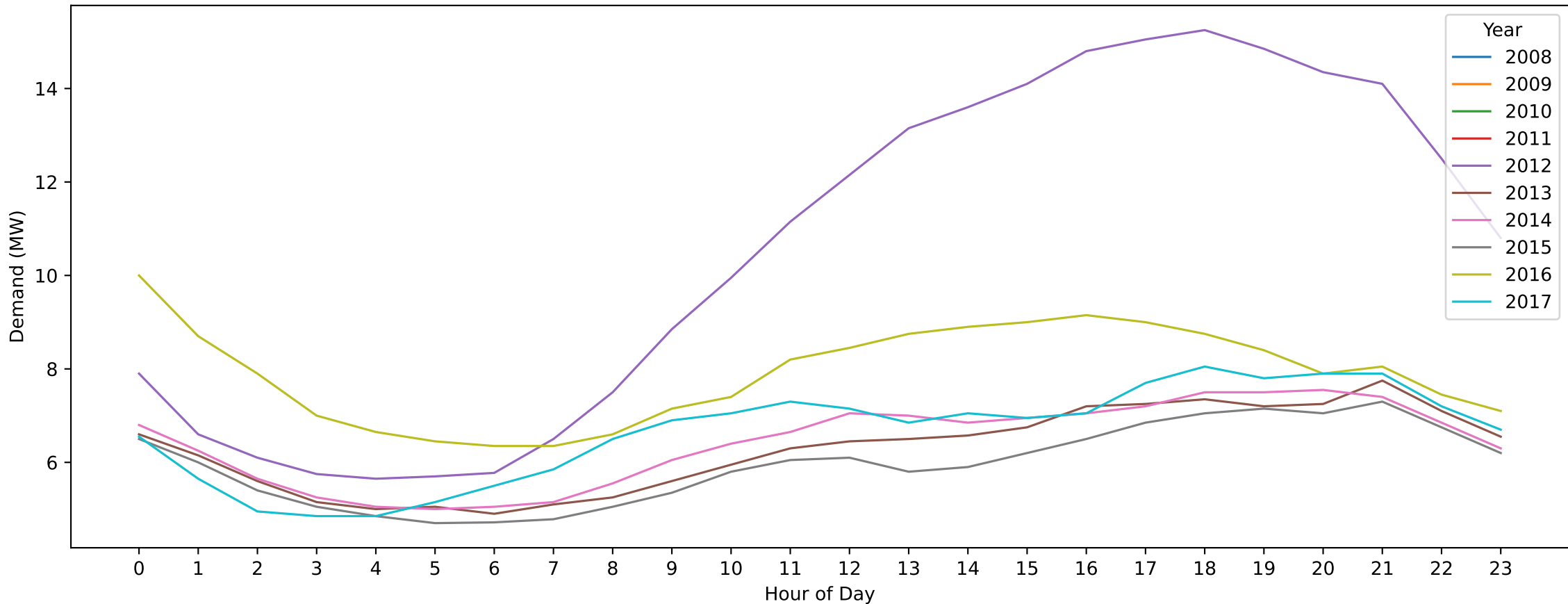
Fairfield — New Year's Day (Hourly Demand Across Years)
