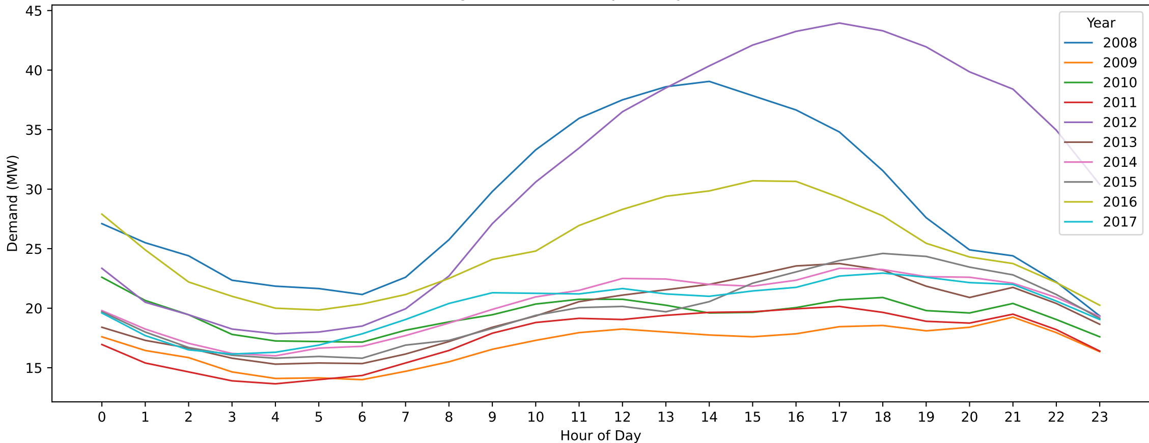
North Heidelberg — New Year's Day (Hourly Demand Across Years)
