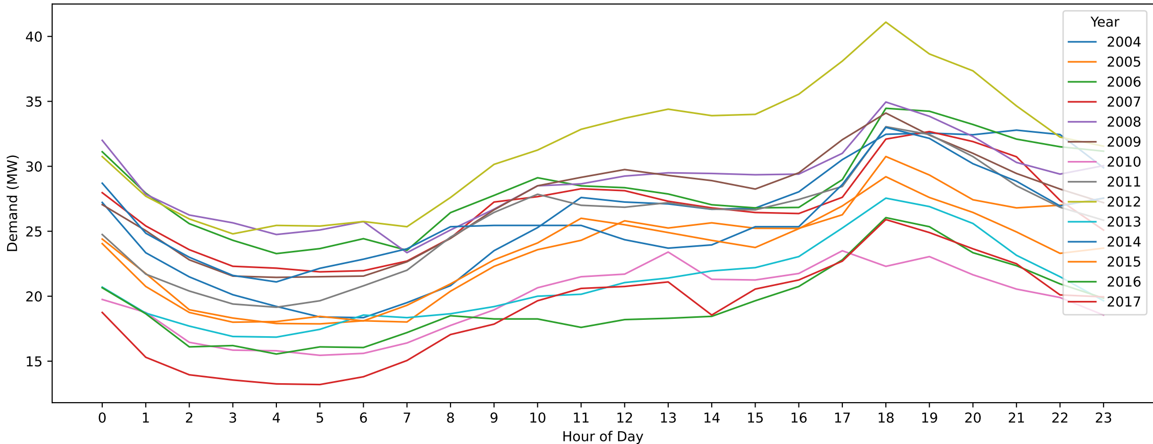
NP — ANZAC Day (Hourly Demand Across Years)
