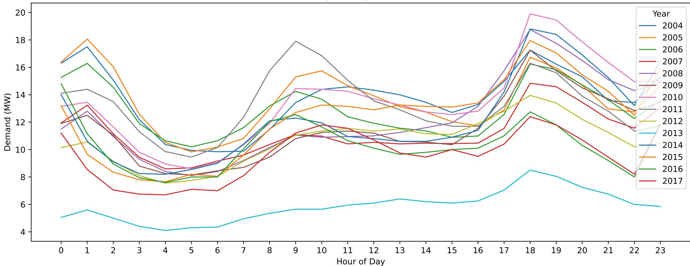
STO — ANZAC Day (Hourly Demand Across Years)
