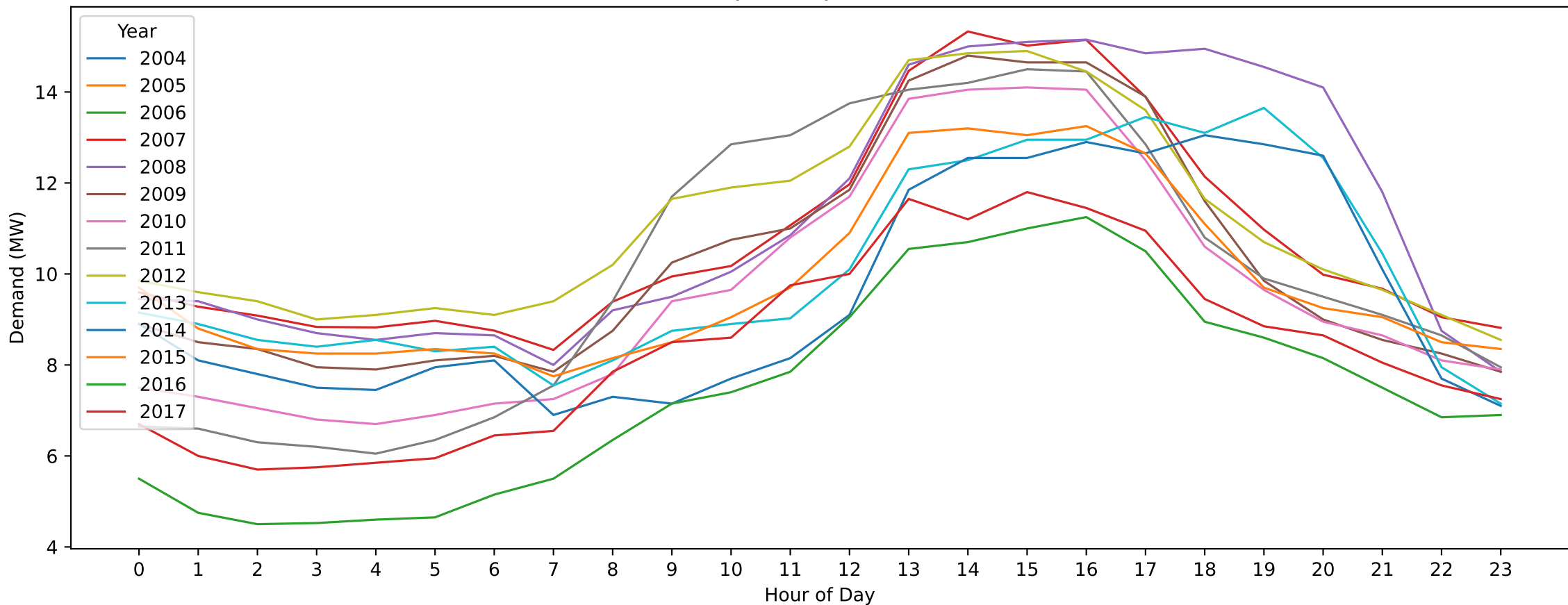
CM — ANZAC Day (Hourly Demand Across Years)
