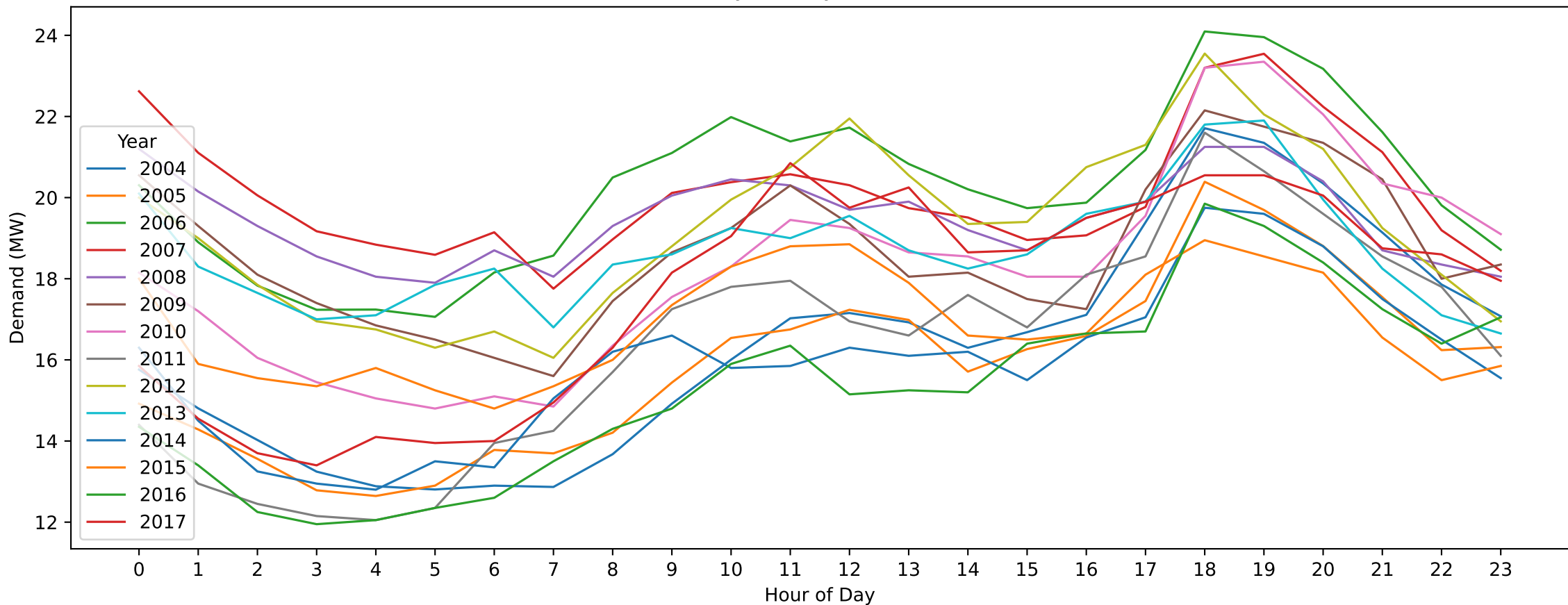
MC — ANZAC Day (Hourly Demand Across Years)
