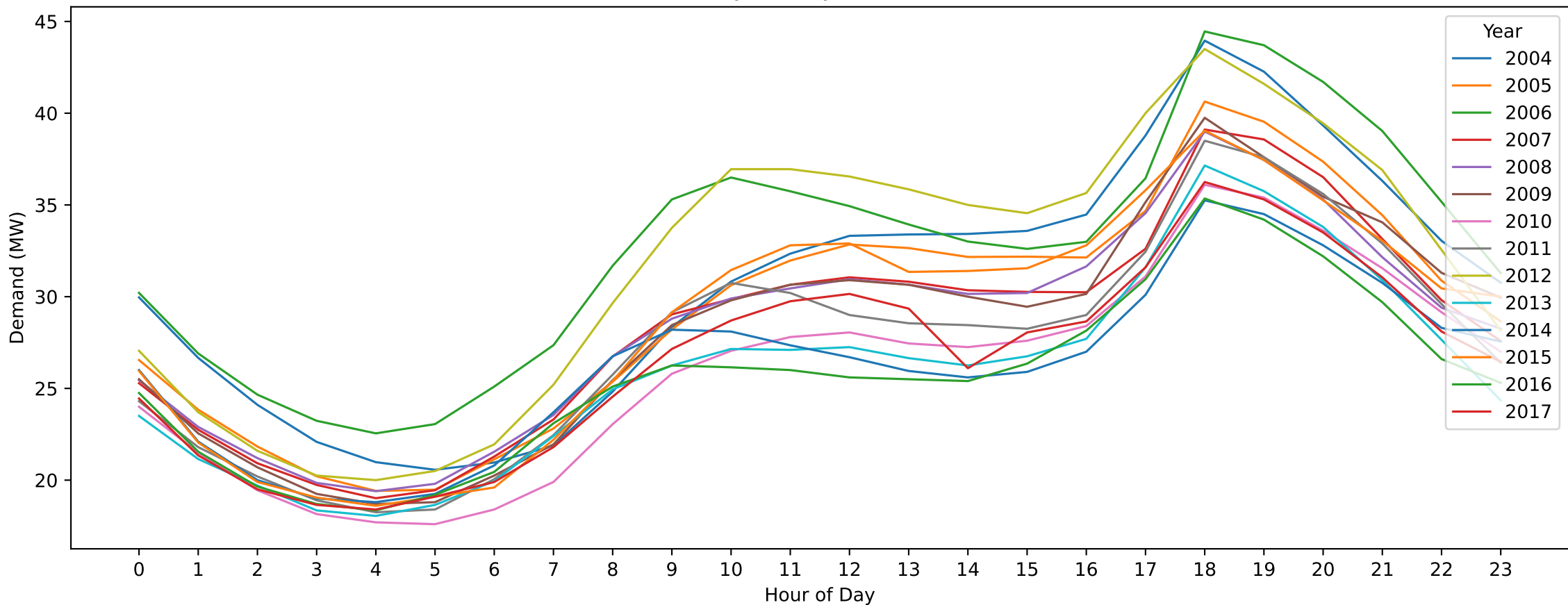
DC — ANZAC Day (Hourly Demand Across Years)
