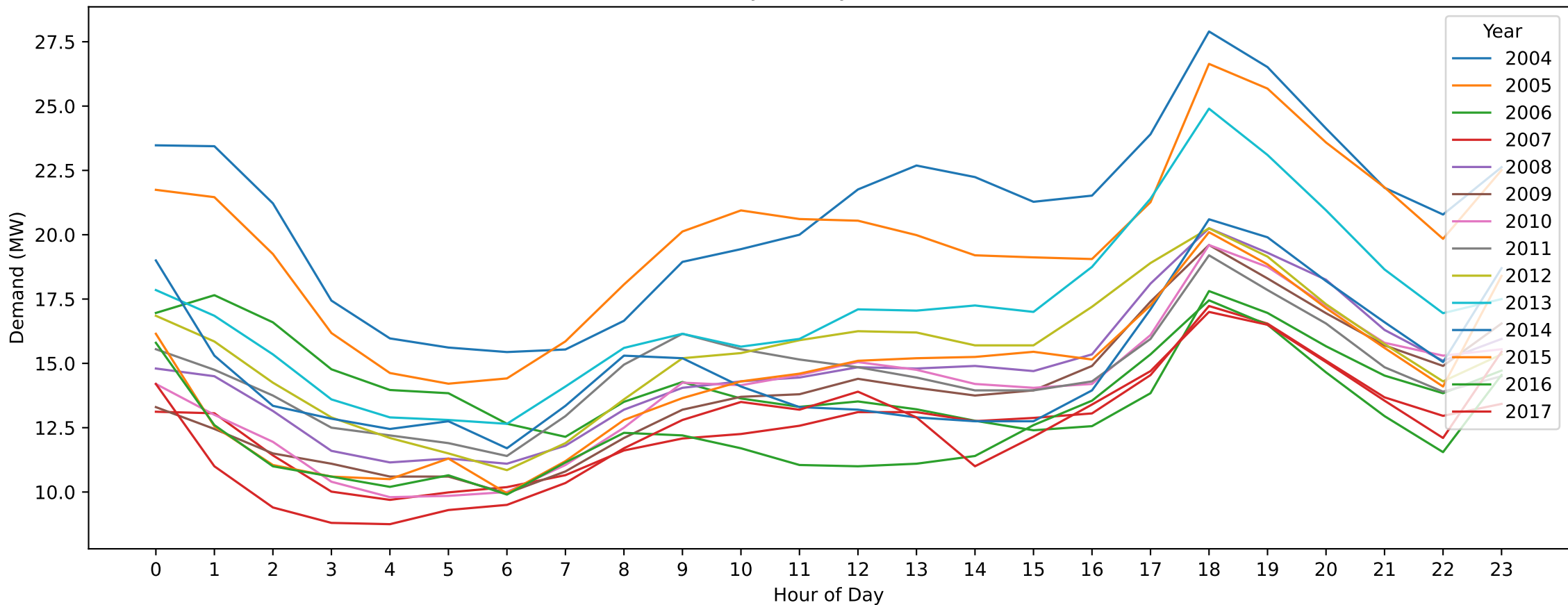
RBD — ANZAC Day (Hourly Demand Across Years)
