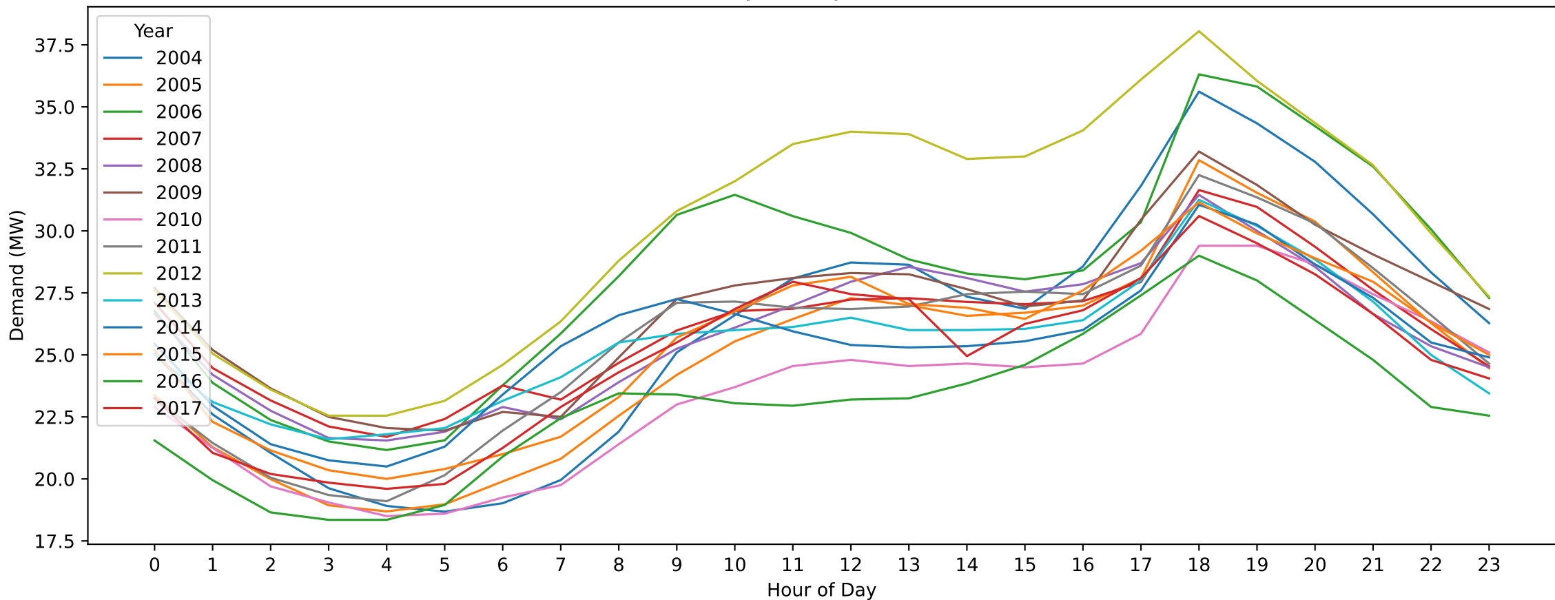
MGE — ANZAC Day (Hourly Demand Across Years)
