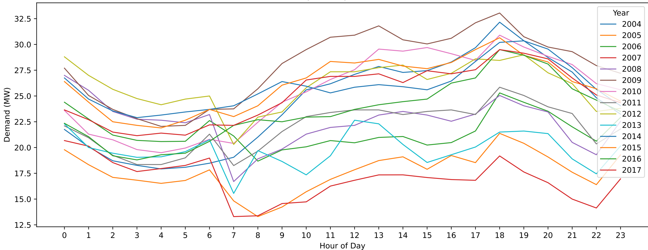
DN — ANZAC Day (Hourly Demand Across Years)
