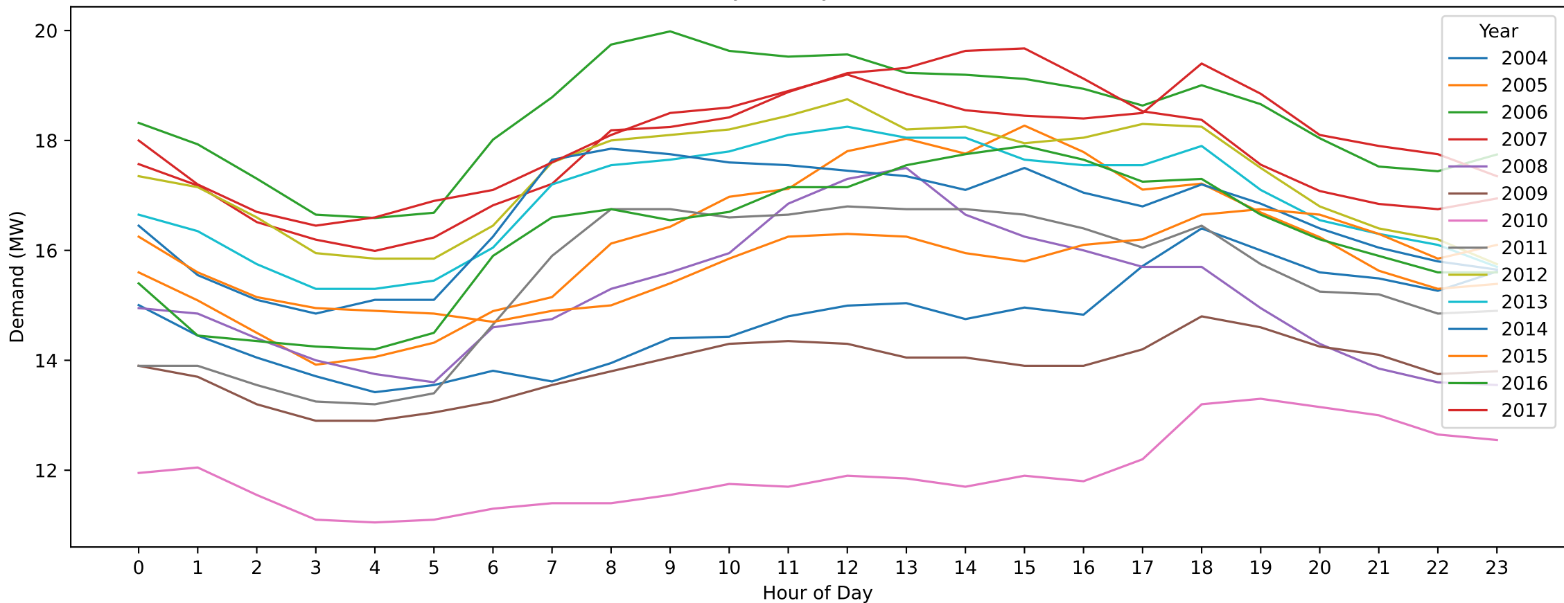
NO — ANZAC Day (Hourly Demand Across Years)
