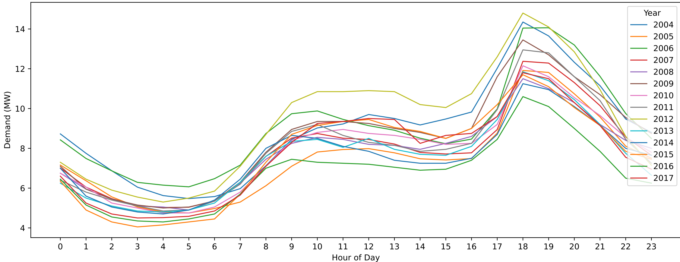
BR — ANZAC Day (Hourly Demand Across Years)
