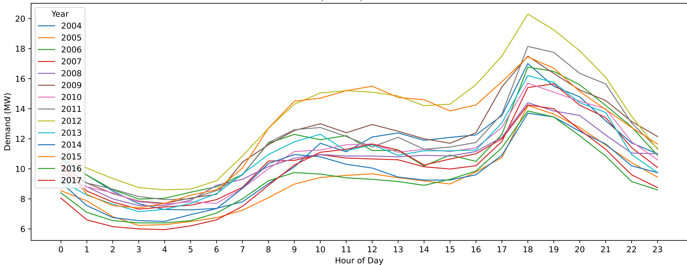
SR — ANZAC Day (Hourly Demand Across Years)
