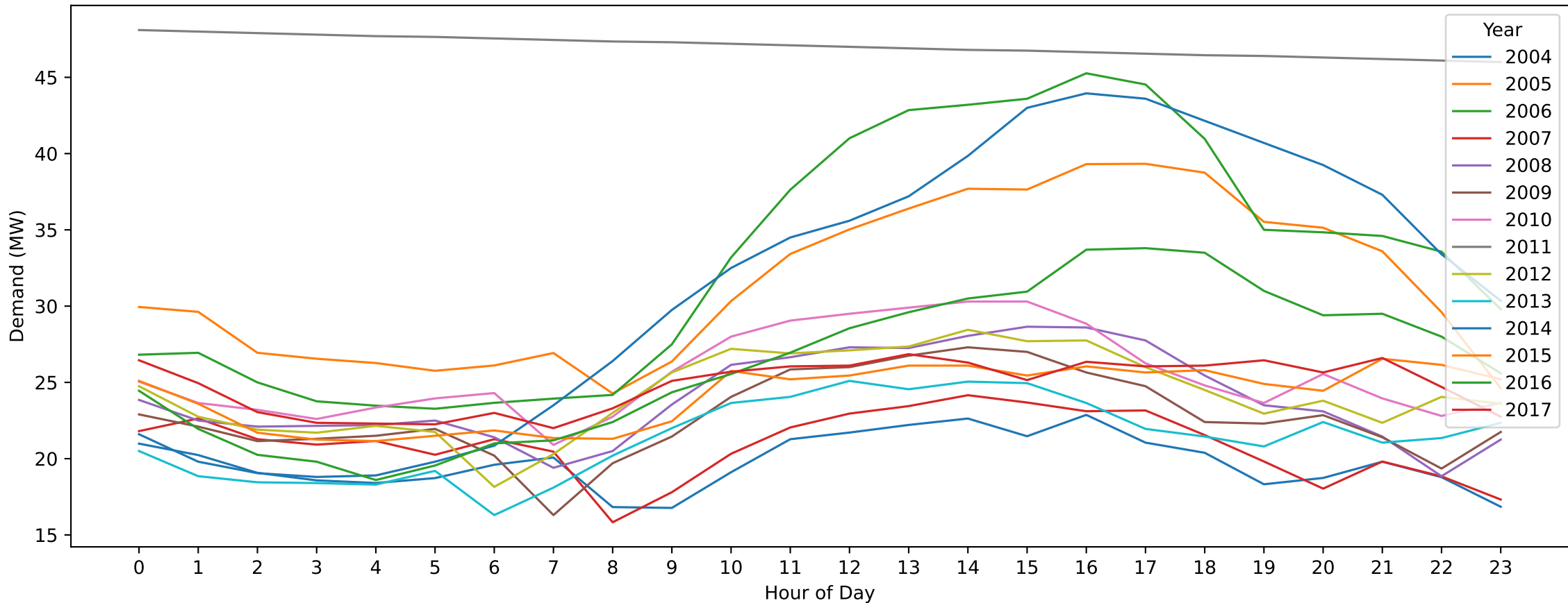
DN — Australia Day (Hourly Demand Across Years)
