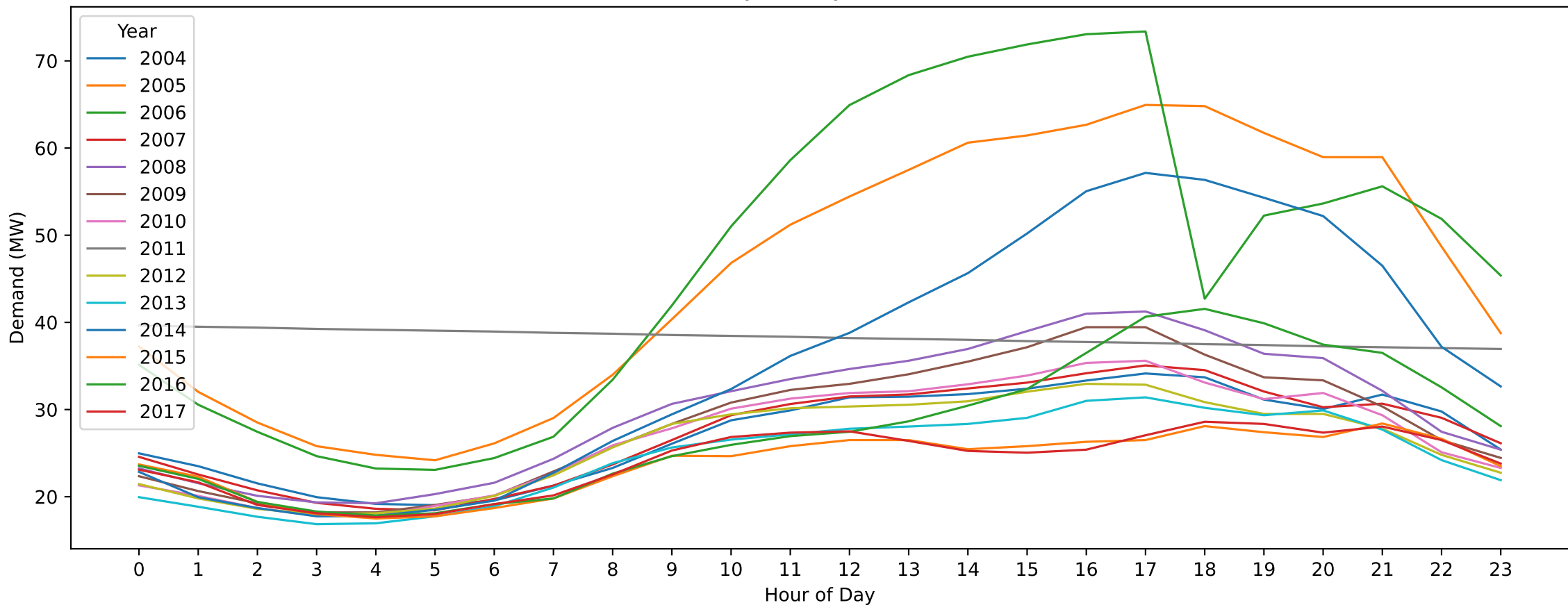
DC — Australia Day (Hourly Demand Across Years)
