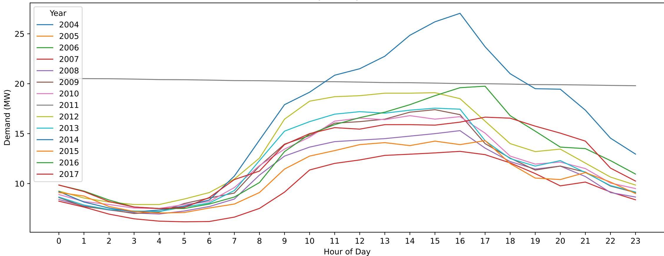
OAK — Australia Day (Hourly Demand Across Years)
