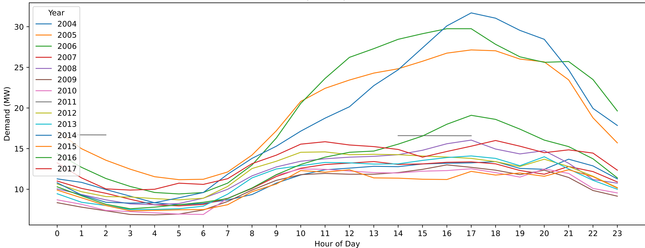
MR — Australia Day (Hourly Demand Across Years)
