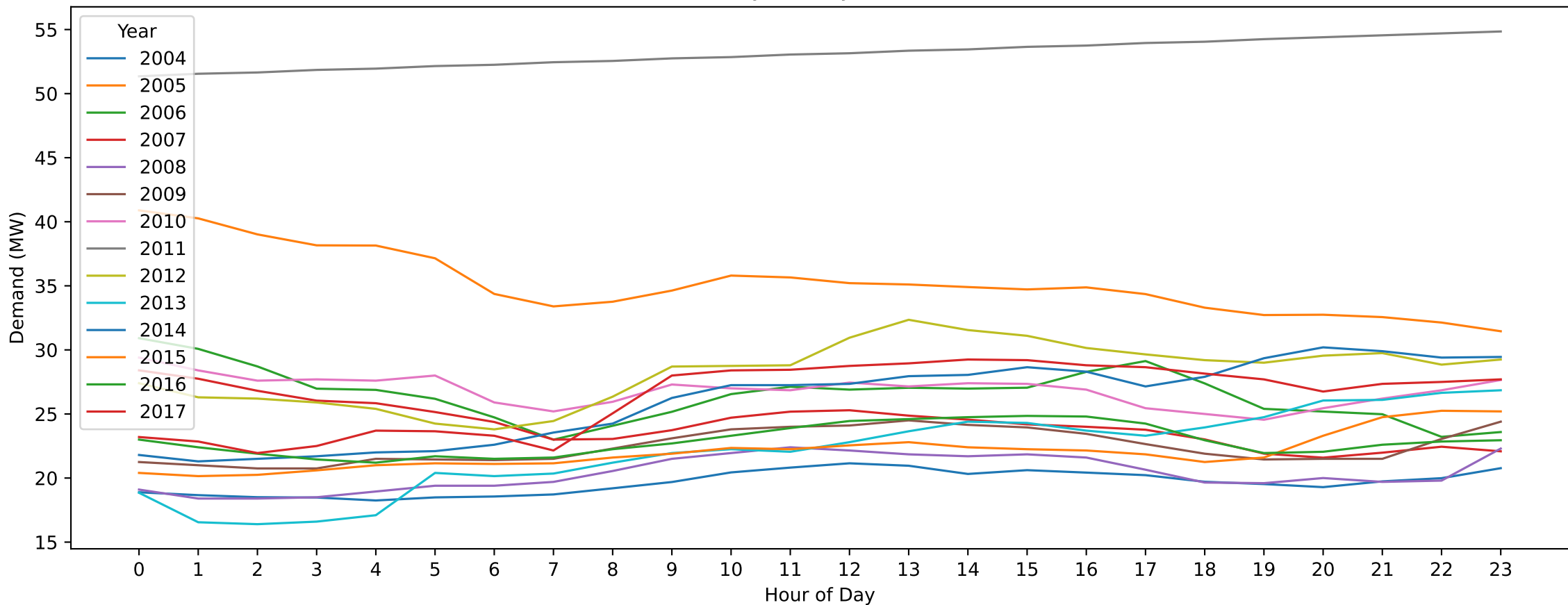
DSH — Australia Day (Hourly Demand Across Years)
