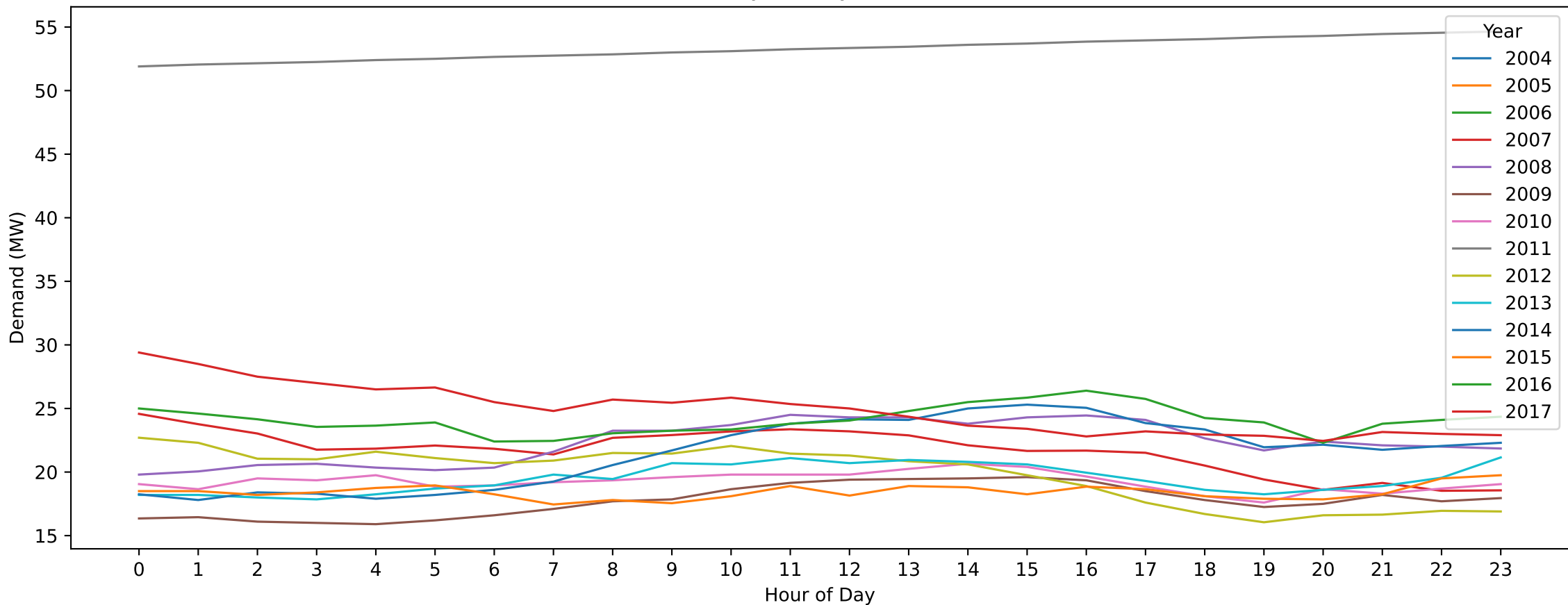
DVY — Australia Day (Hourly Demand Across Years)
