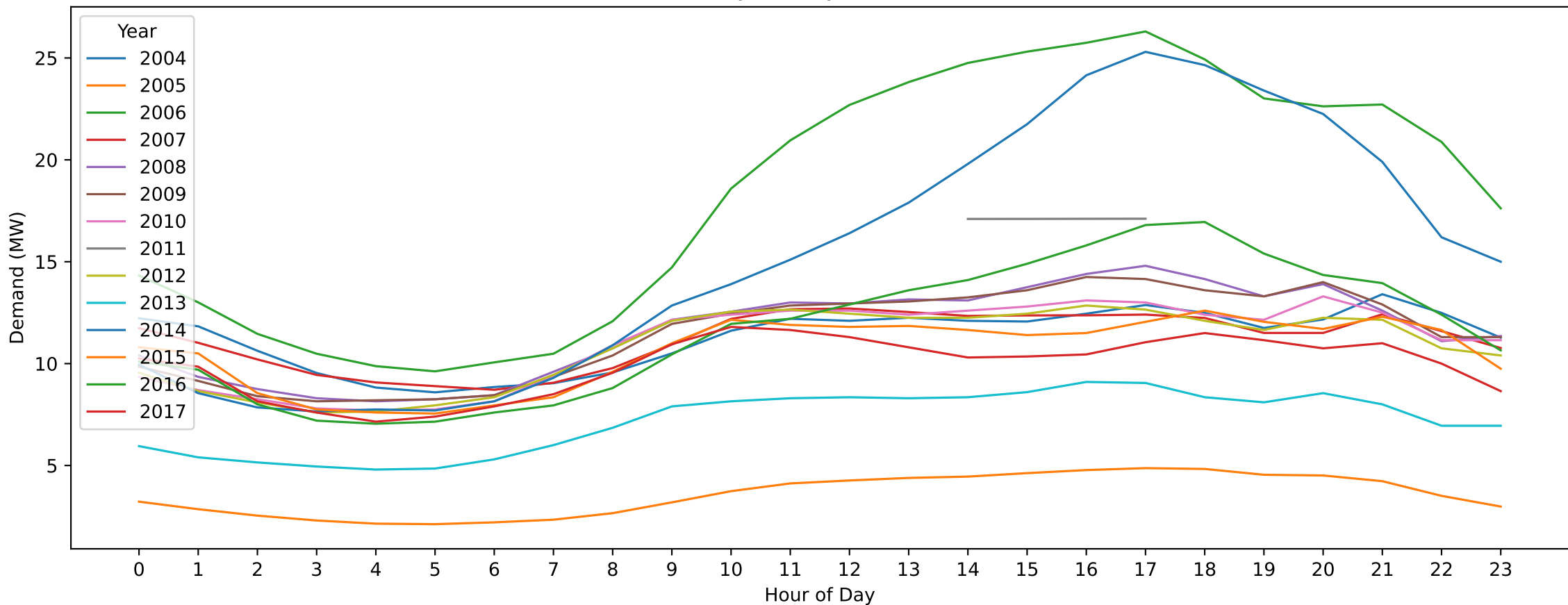
M — Australia Day (Hourly Demand Across Years)
