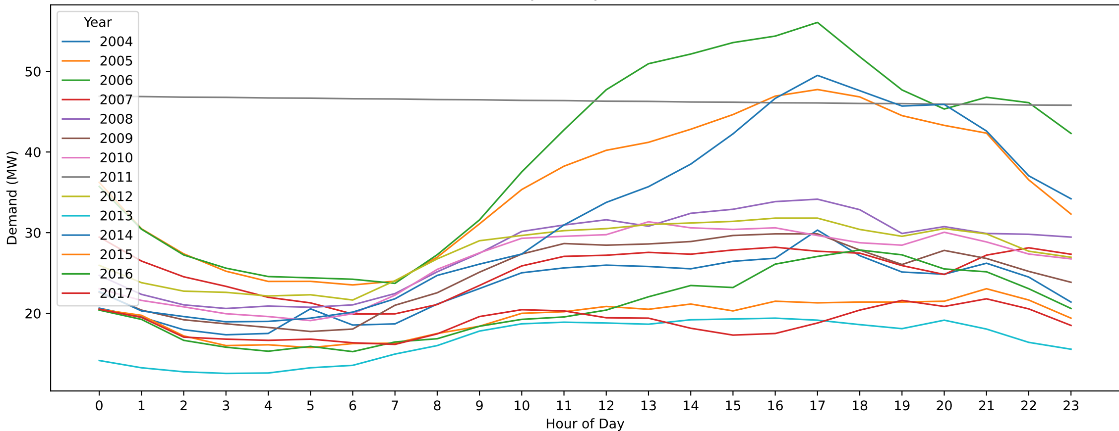
NP — Australia Day (Hourly Demand Across Years)
