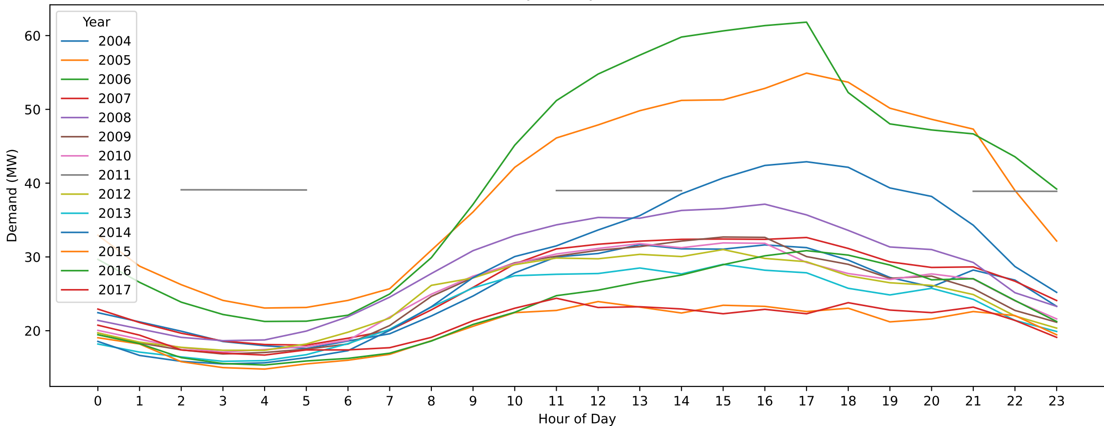
GW — Australia Day (Hourly Demand Across Years)
