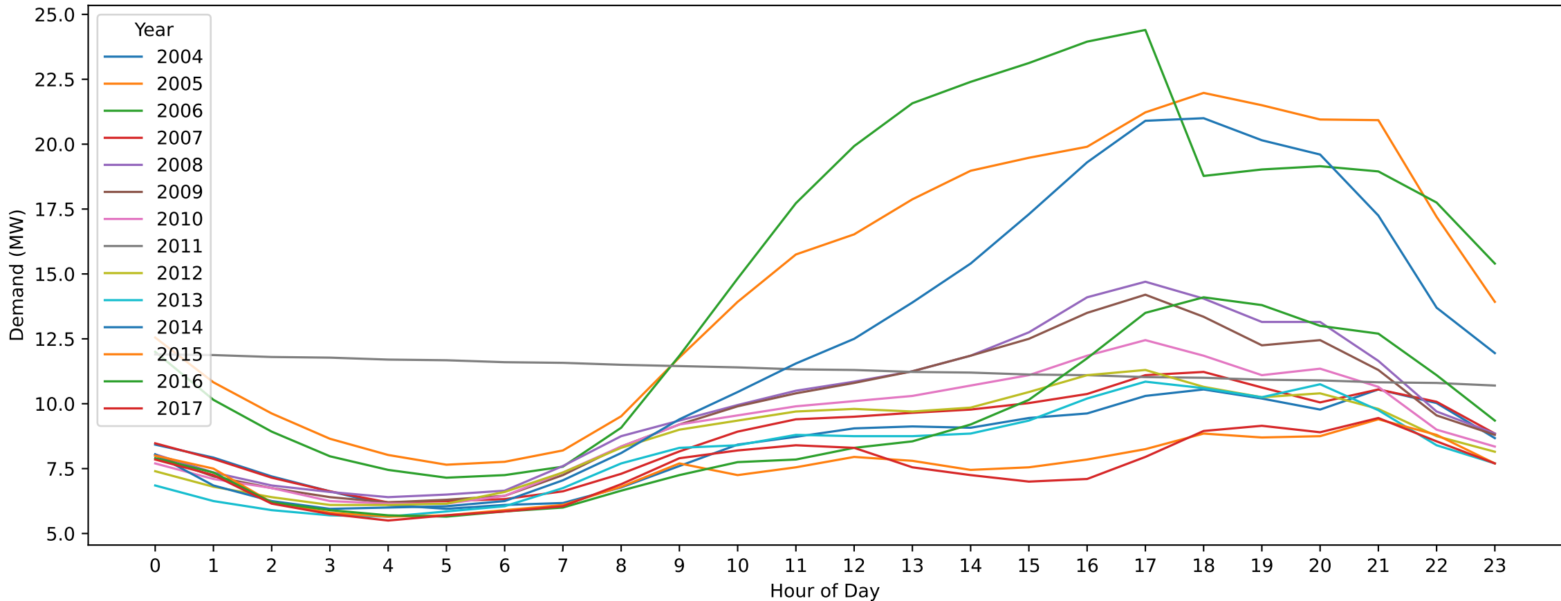
BU — Australia Day (Hourly Demand Across Years)
