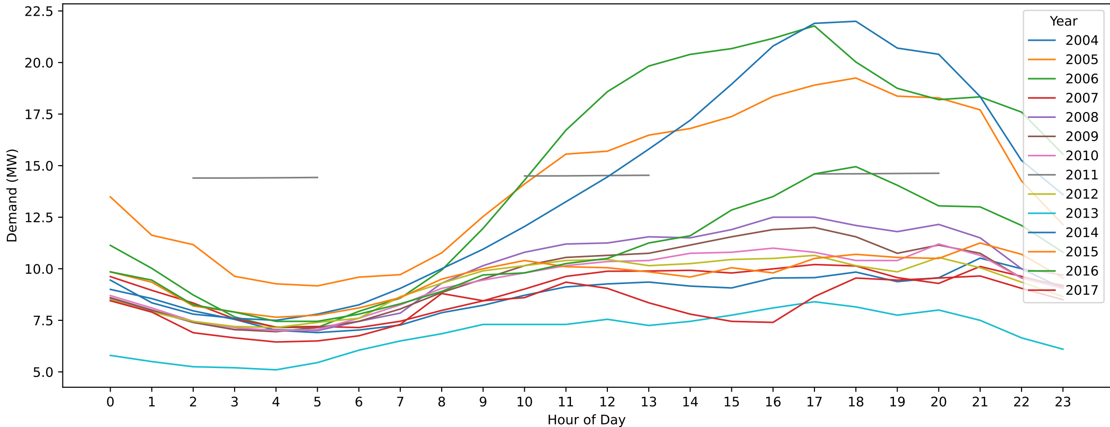
CDA — Australia Day (Hourly Demand Across Years)
