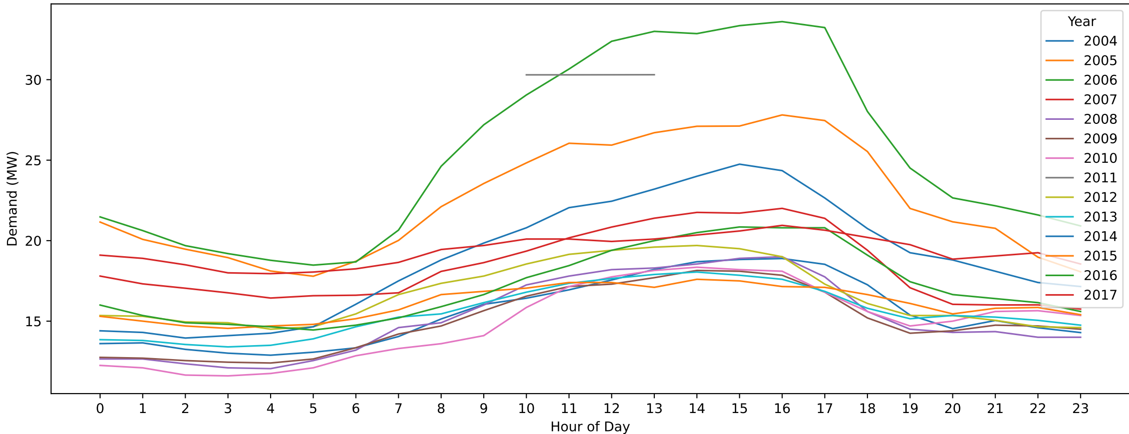
NO — Australia Day (Hourly Demand Across Years)
