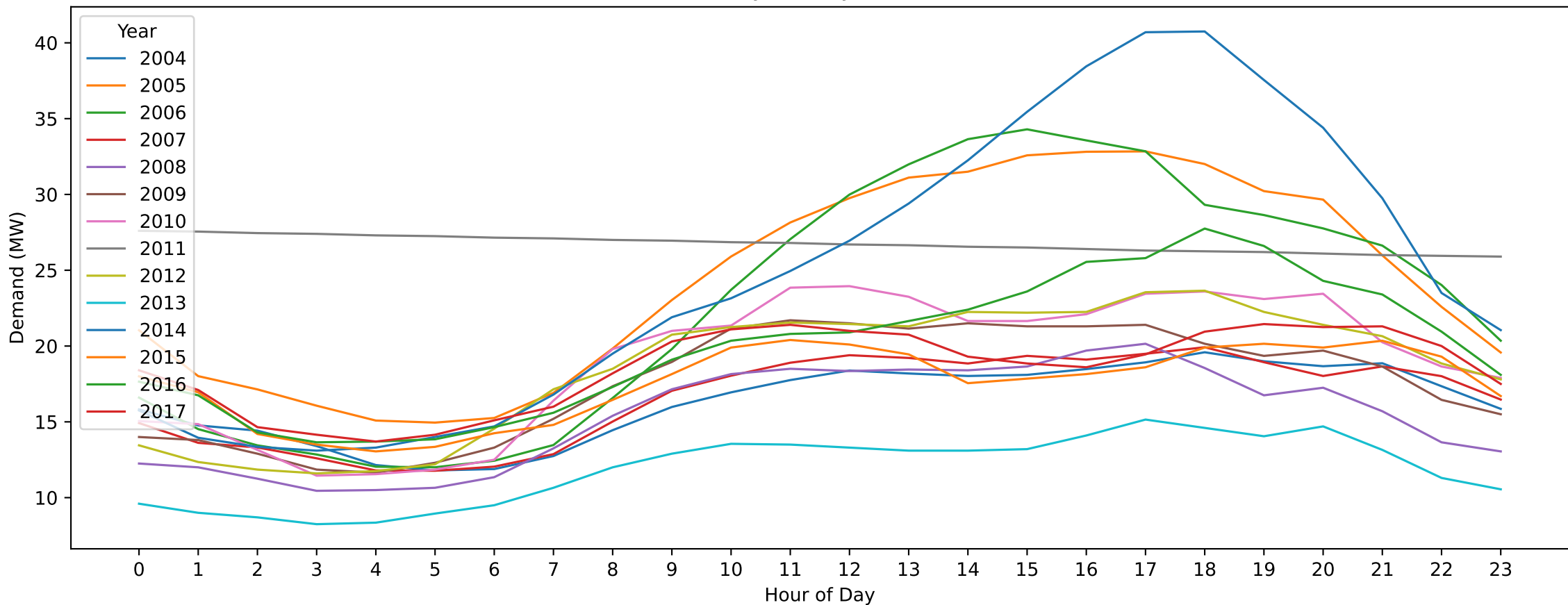
MTN — Australia Day (Hourly Demand Across Years)
