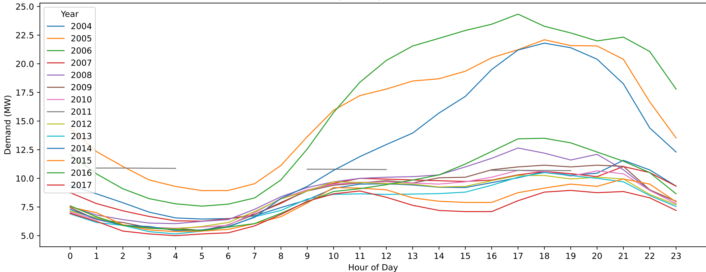
BT — Australia Day (Hourly Demand Across Years)
