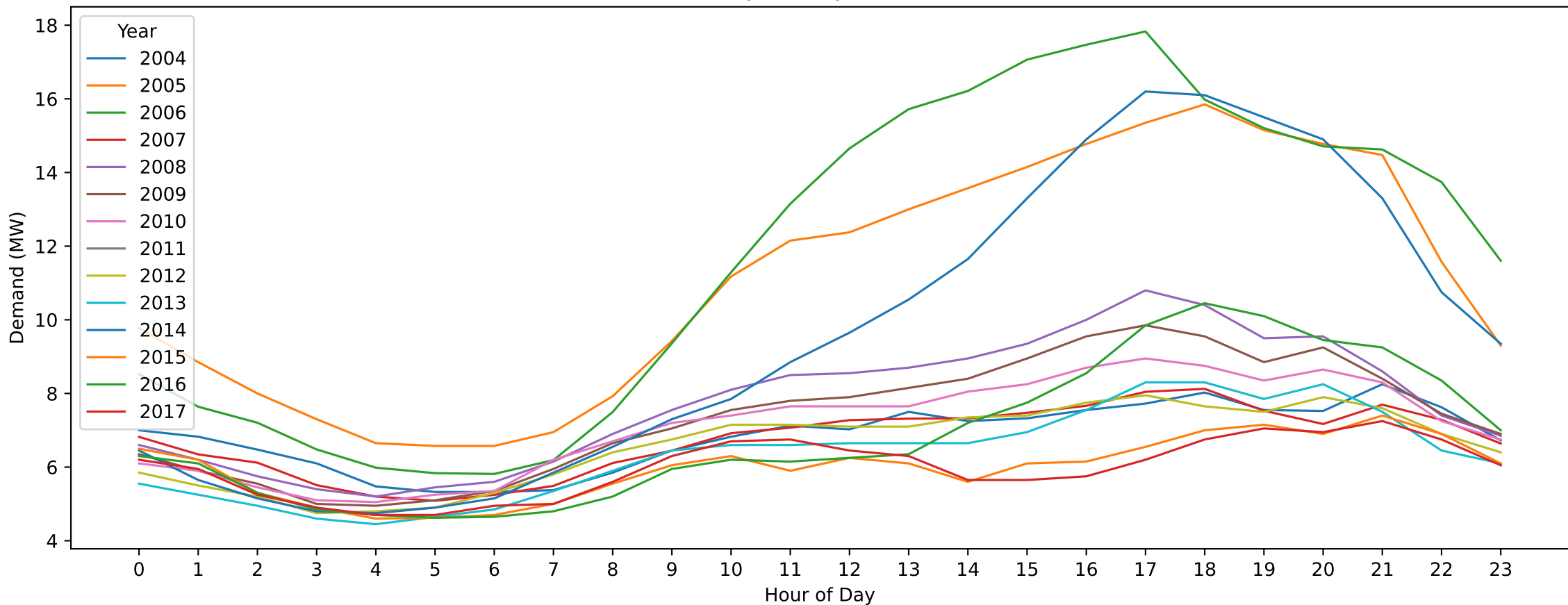
BW — Australia Day (Hourly Demand Across Years)
