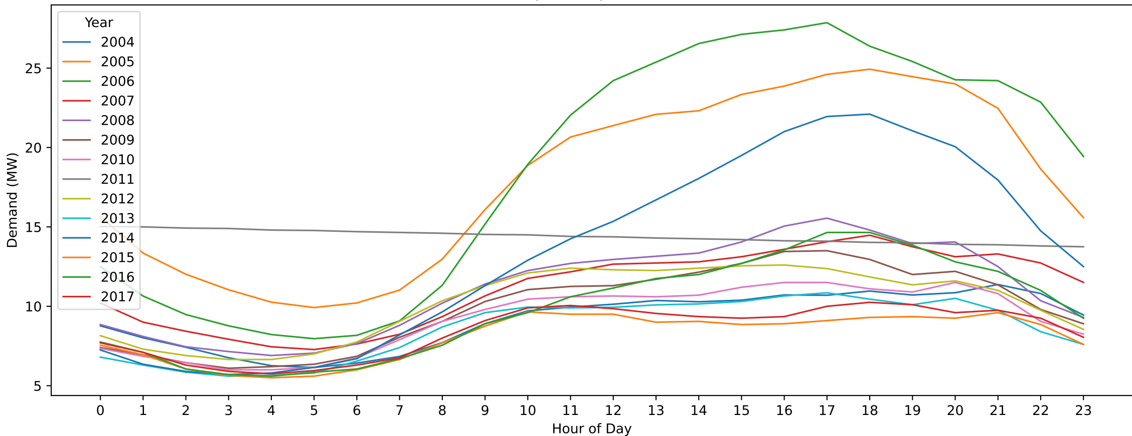
EL — Australia Day (Hourly Demand Across Years)
