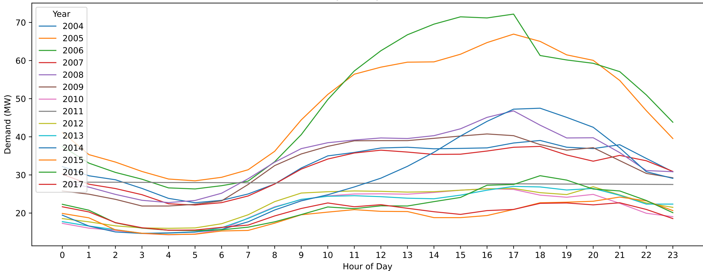
FSH — Australia Day (Hourly Demand Across Years)
